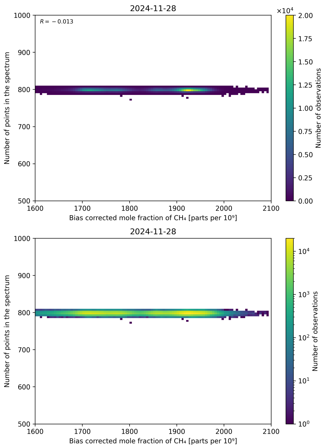
Figure 68: Scatter density plot of “Bias corrected mole fraction of CH 4 ” against “Number of points in the spectrum” for 2024-11-27 to 2024-11-29.
