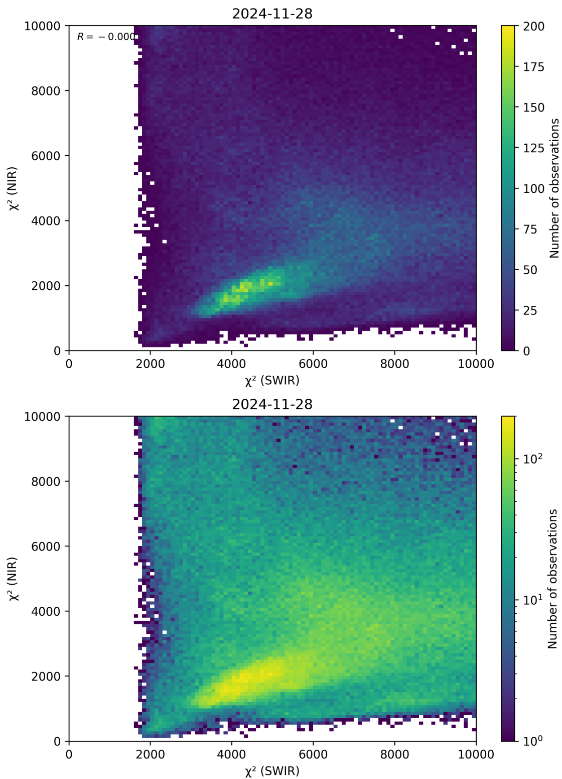
Figure 47: Scatter density plot of “ \chi^2 (SWIR)” against “ \chi^2 (NIR)” for 2024-11-27 to 2024-11-29.
