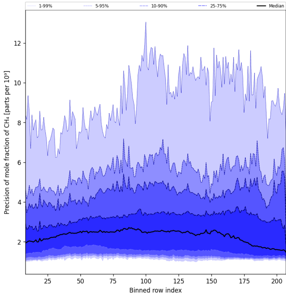
Figure 35: Along track statistics of “Precision of mole fraction of CH 4 ” for 2024-11-27 to 2024-11-29
