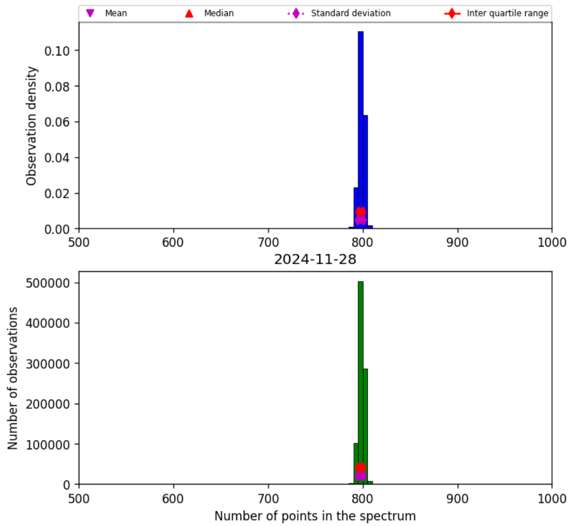
Figure 26: Histogram of “Number of points in the spectrum” for 2024-11-27 to 2024-11-29
