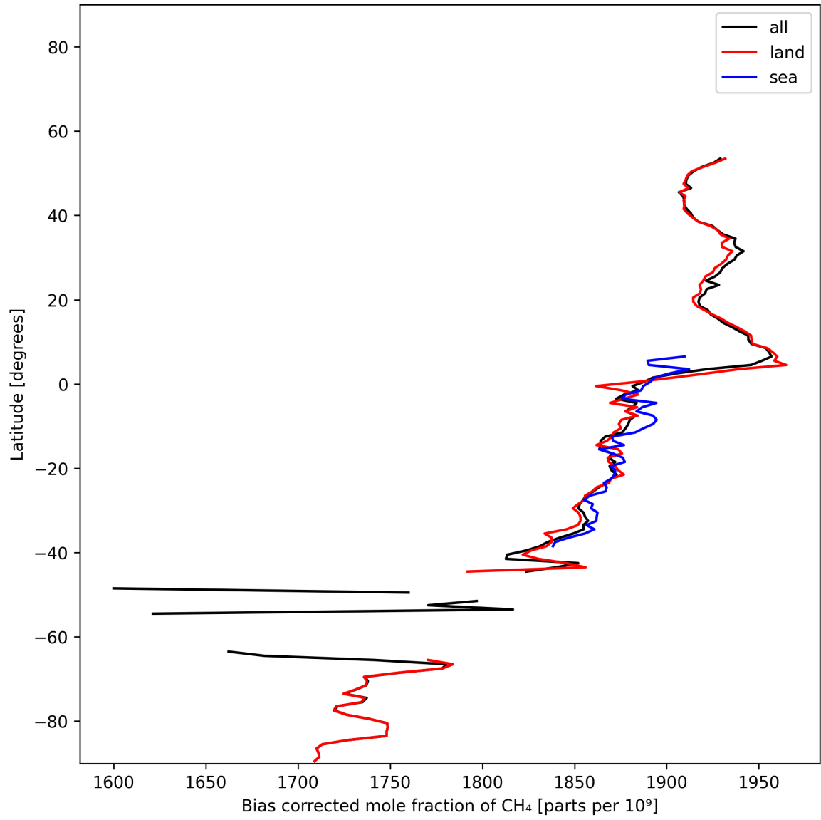
Figure 14: Zonal average of “Bias corrected mole fraction of CH 4 ” for 2024-11-27 to 2024-11-29.
