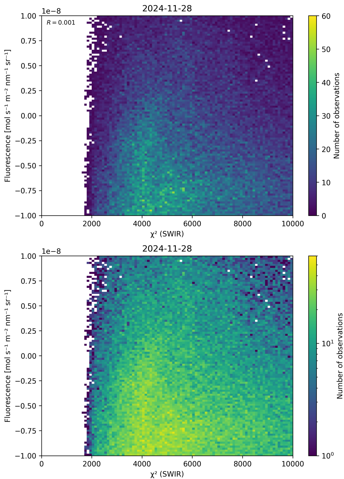
Figure 49: Scatter density plot of “ \chi^2 (SWIR)” against “Fluorescence” for 2024-11-27 to 2024-11-29.
