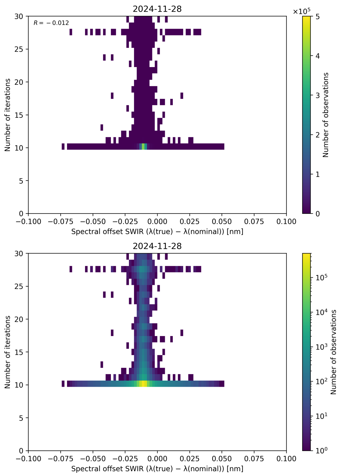
Figure 121: Scatter density plot of “Spectral offset SWIR ( \lambda_{\text{true}} - \lambda_{\text{nominal}} )” against “Number of iterations” for 2024-11-27 to 2024-11-29.
