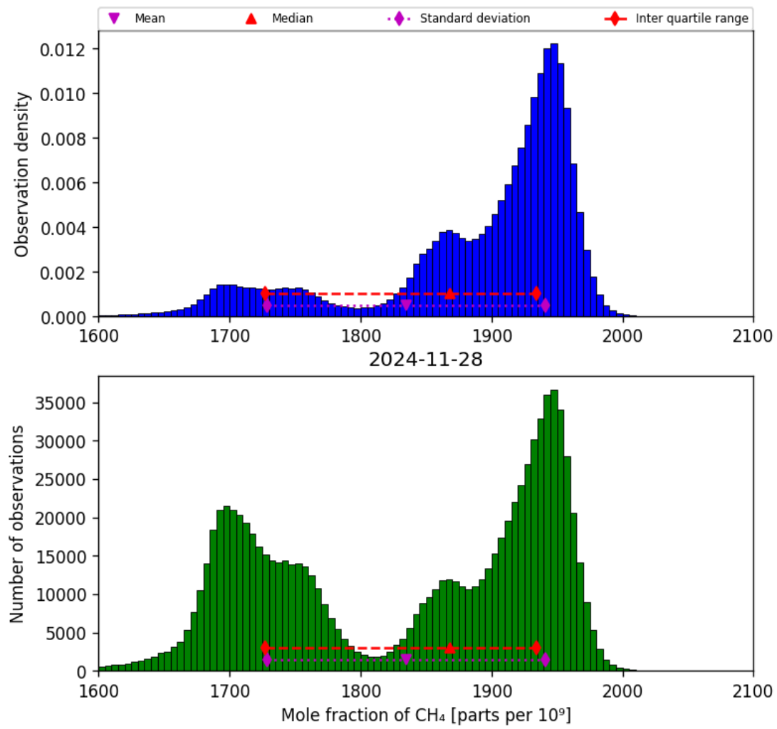
Figure 23: Histogram of “Mole fraction of CH 4 ” for 2024-11-27 to 2024-11-29
