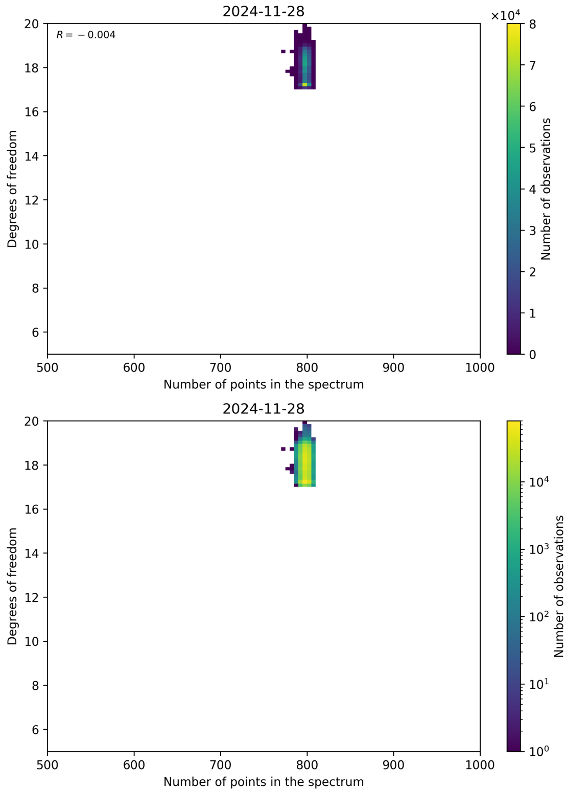
Figure 90: Scatter density plot of “Number of points in the spectrum” against “Degrees of freedom” for 2024-11-27 to 2024-11-29.
