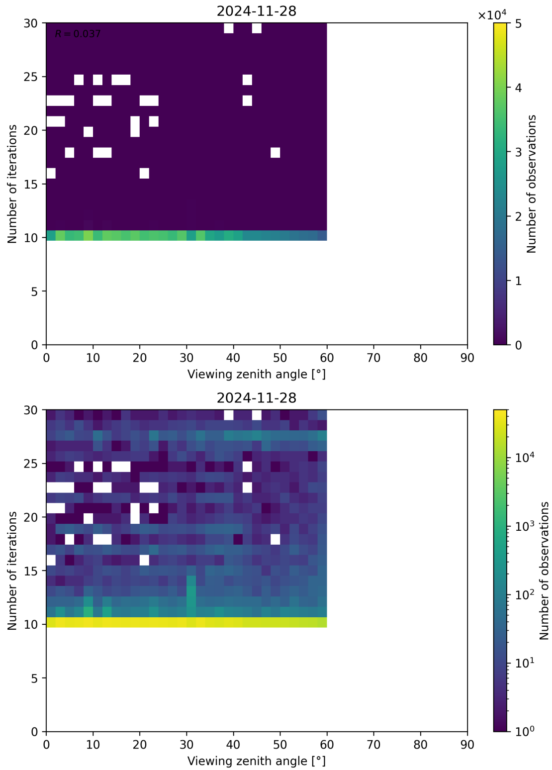
Figure 113: Scatter density plot of “Viewing zenith angle” against “Number of iterations” for 2024-11-27 to 2024-11-29.
