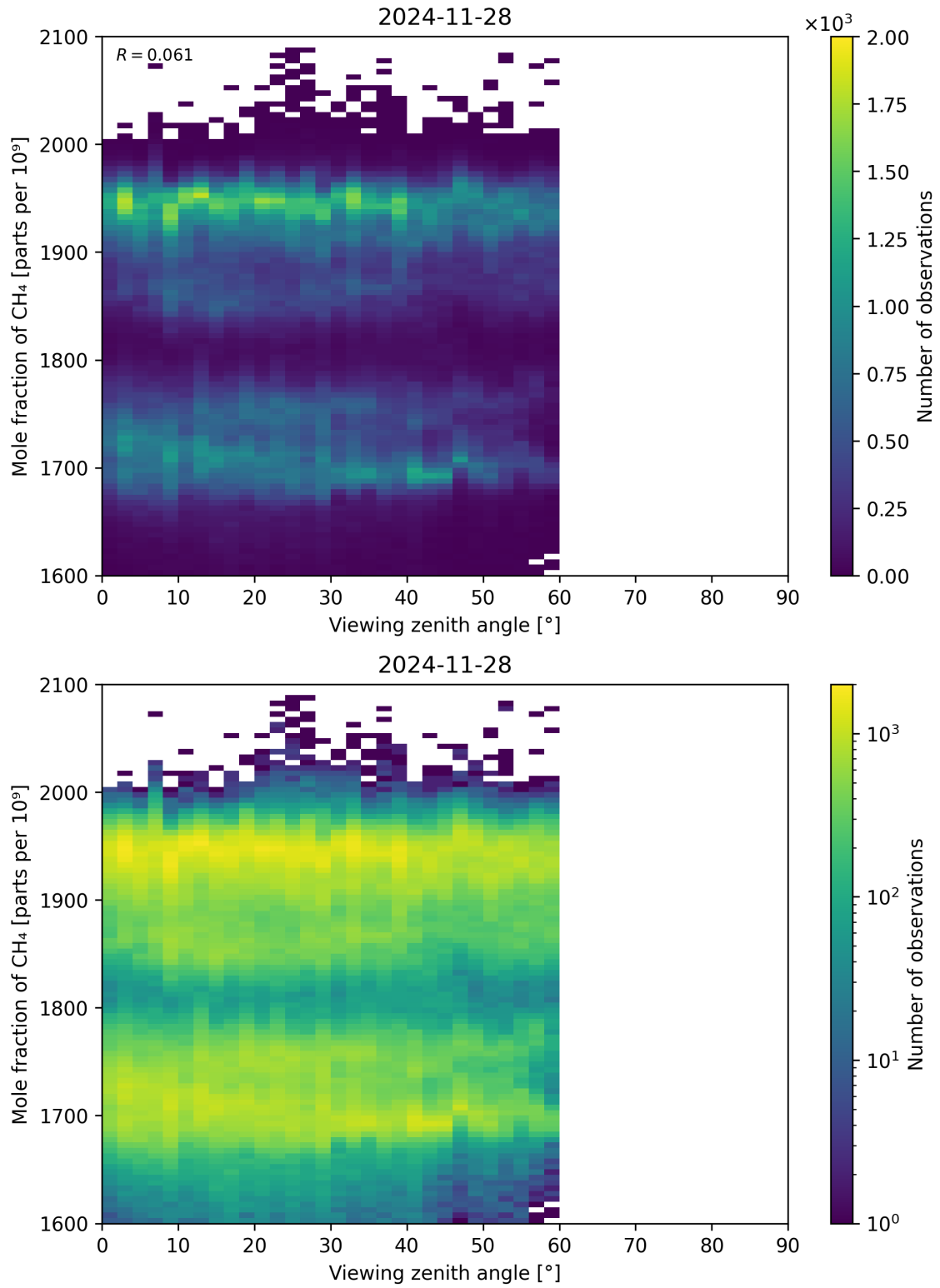
Figure 110: Scatter density plot of “Viewing zenith angle” against “Mole fraction of \text{CH}_4 ” for 2024-11-27 to 2024-11-29.
