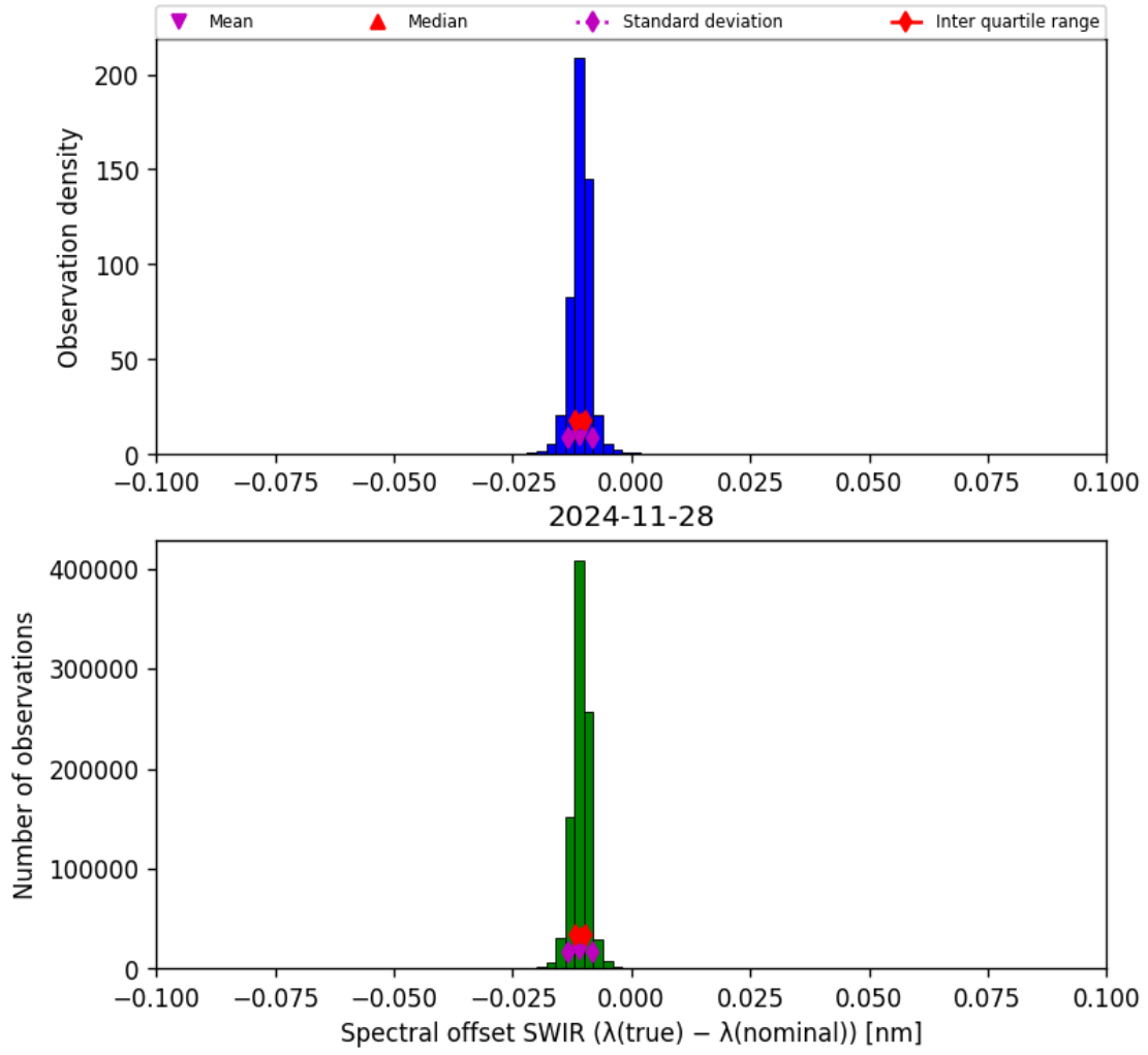
Figure 27: Histogram of “Spectral offset SWIR ( \lambda_{\text{true}} - \lambda_{\text{nominal}} )” for 2024-11-27 to 2024-11-29
