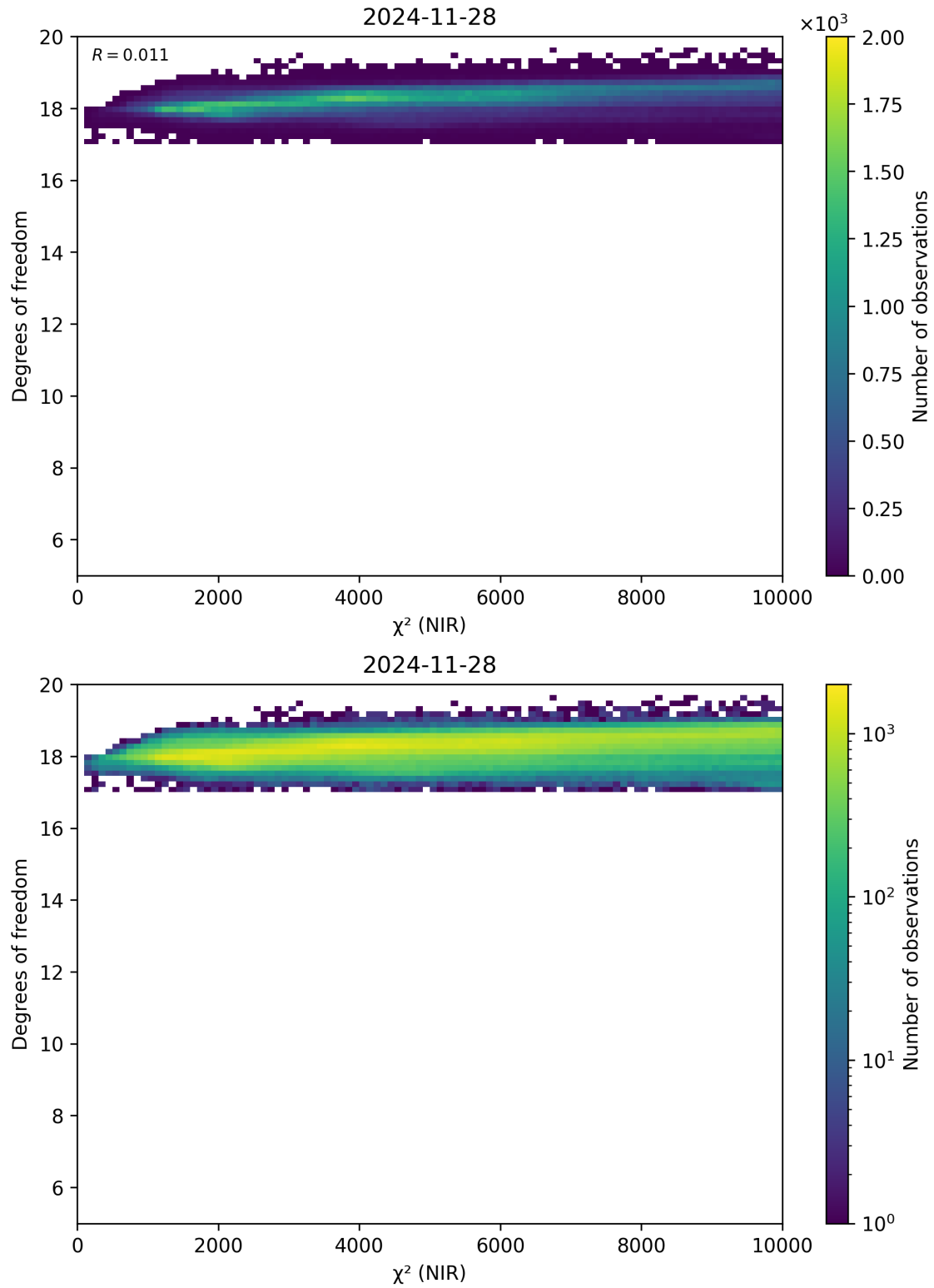
Figure 44: Scatter density plot of “ \chi^2 (NIR)” against “Degrees of freedom” for 2024-11-27 to 2024-11-29.
