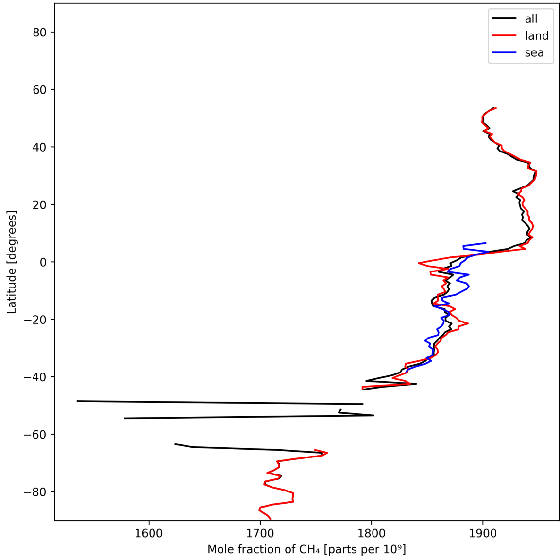
Figure 12: Zonal average of “Mole fraction of \text{CH}_4 ” for 2024-11-27 to 2024-11-29.
