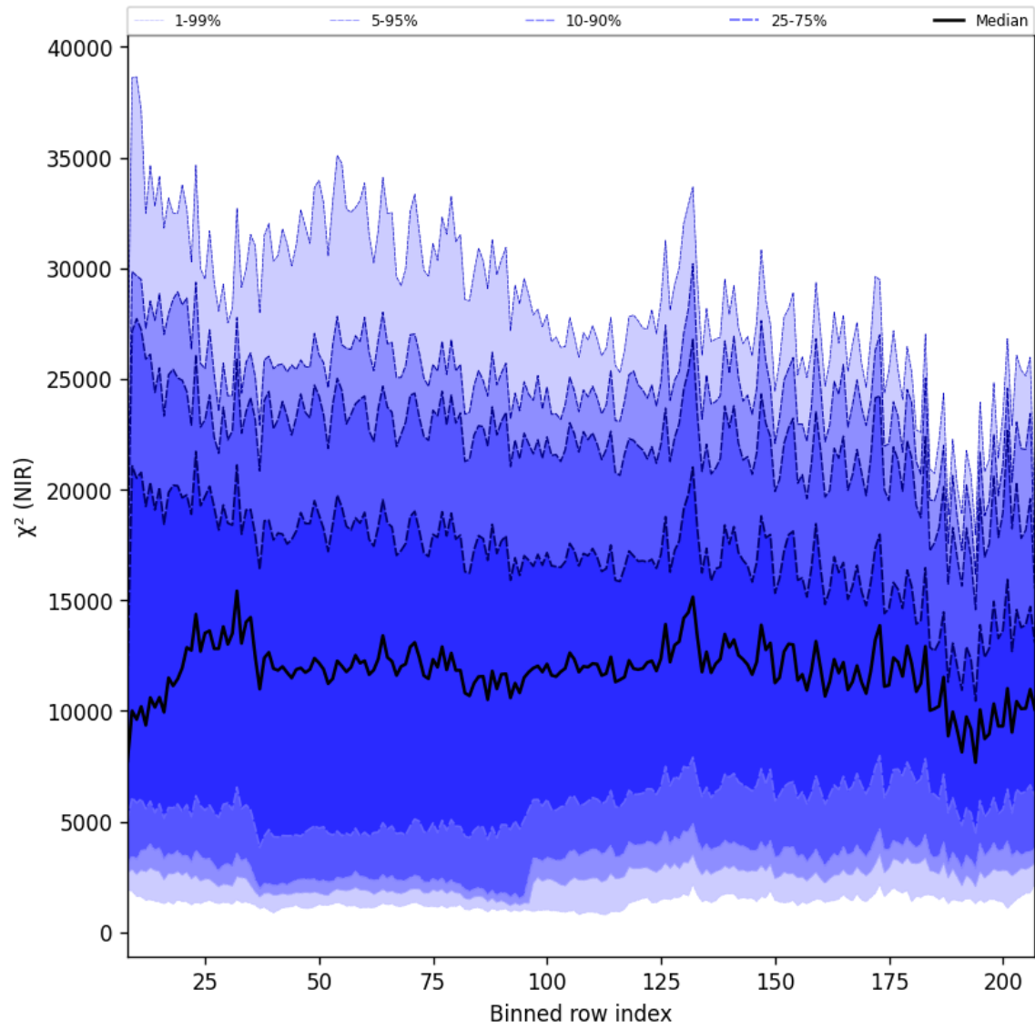
Figure 40: Along track statistics of “ \chi^2 (NIR)” for 2024-11-27 to 2024-11-29
