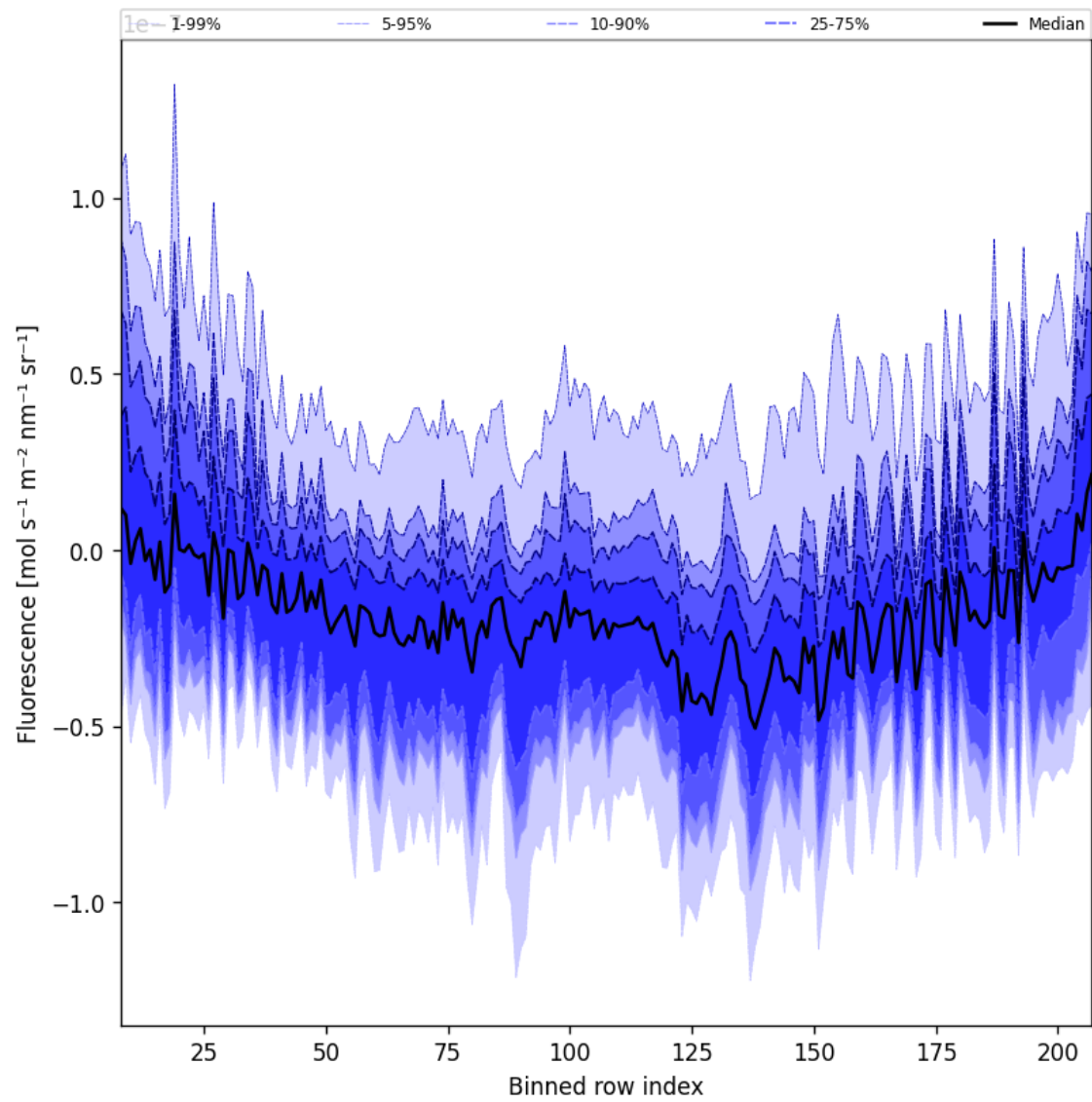
Figure 43: Along track statistics of “Fluorescence” for 2024-11-27 to 2024-11-29
