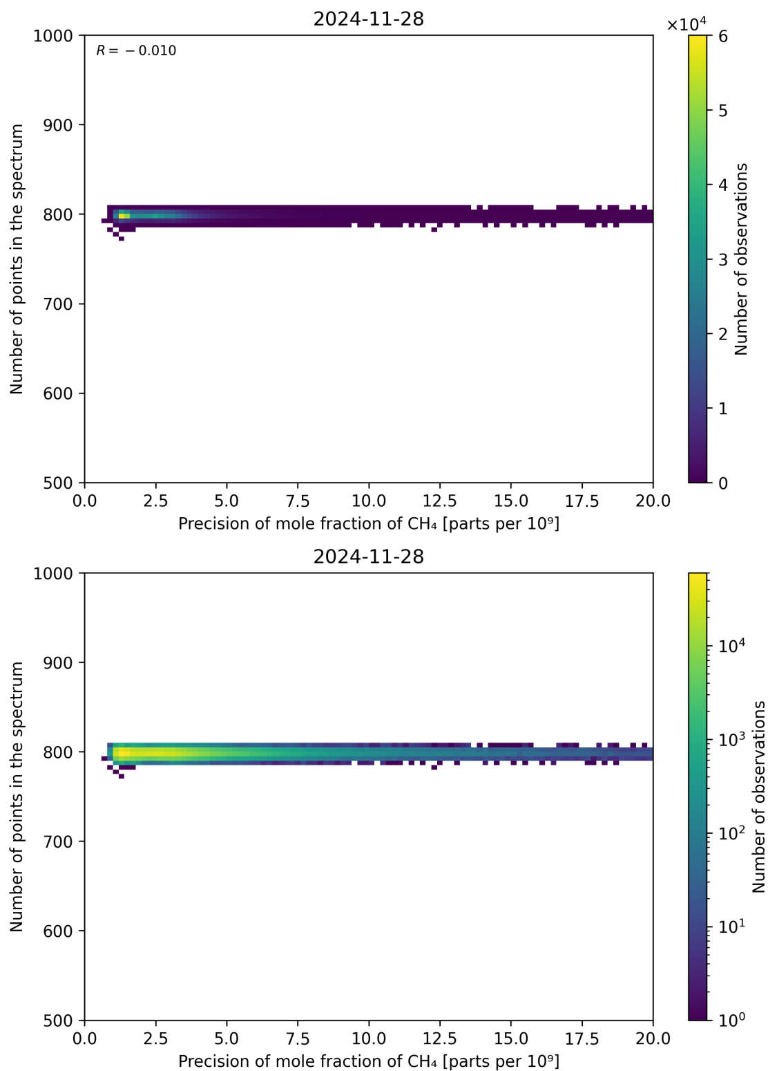
Figure 84: Scatter density plot of “Precision of mole fraction of CH 4 ” against “Number of points in the spectrum” for 2024-11-27 to 2024-11-29.
