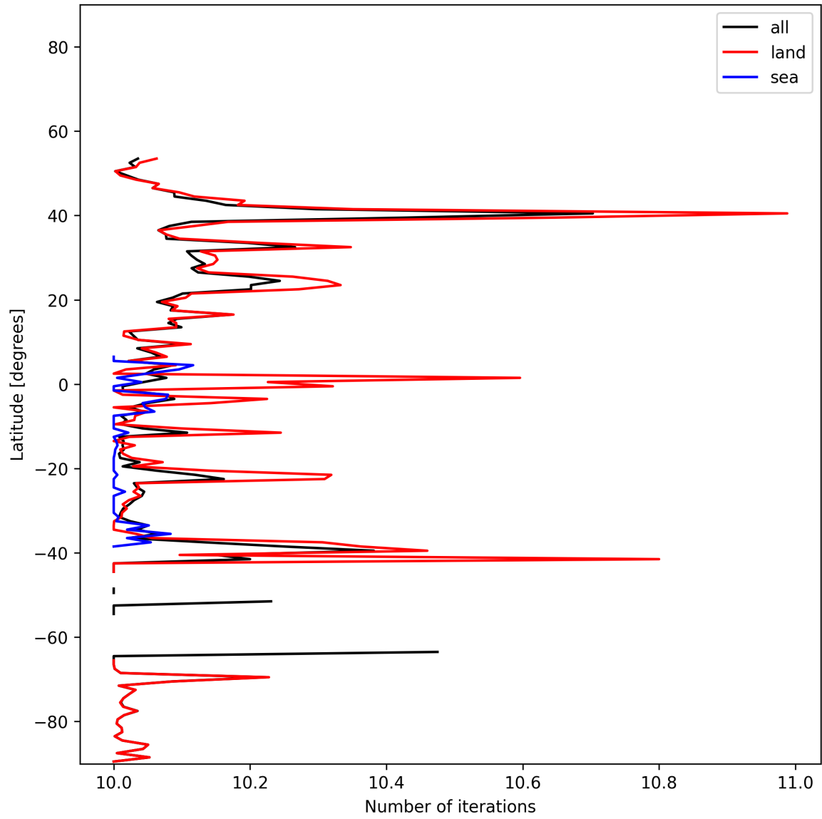
Figure 20: Zonal average of “Number of iterations” for 2024-11-27 to 2024-11-29.
