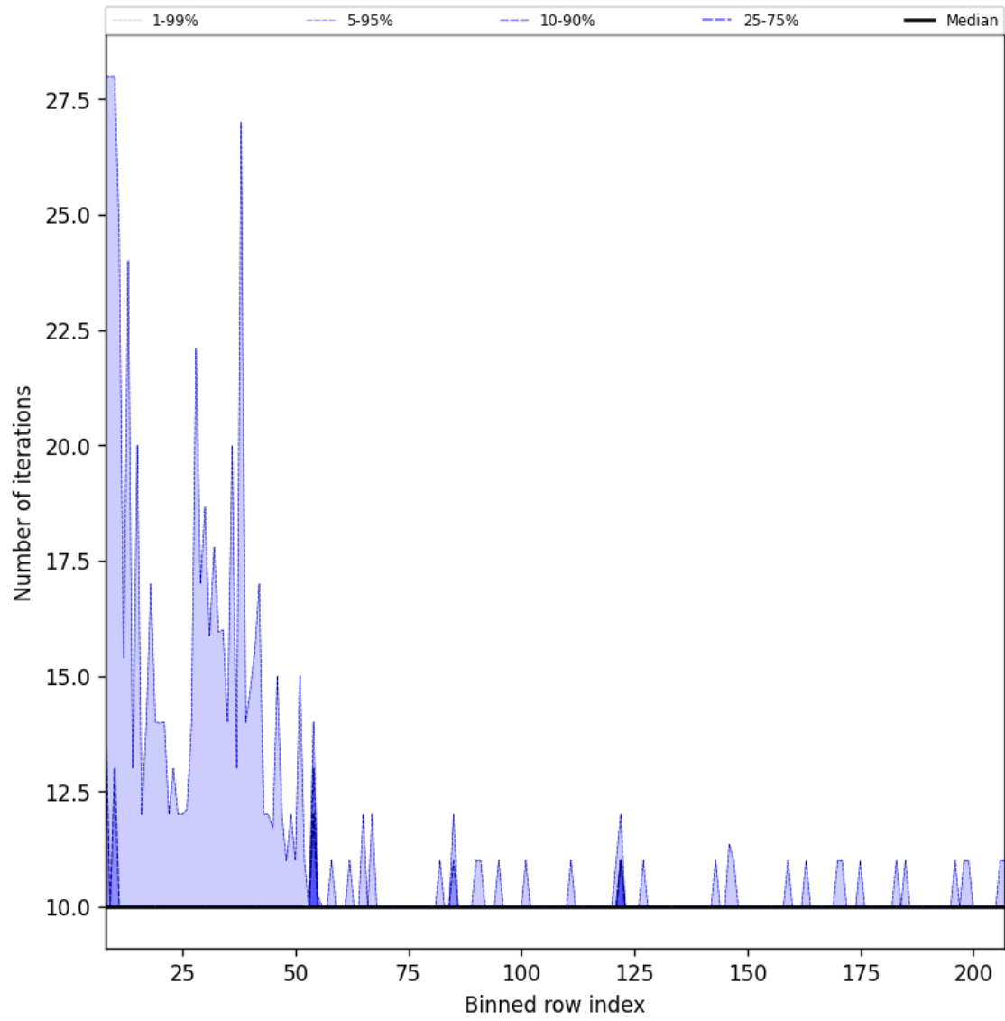
Figure 42: Along track statistics of “Number of iterations” for 2024-11-27 to 2024-11-29
