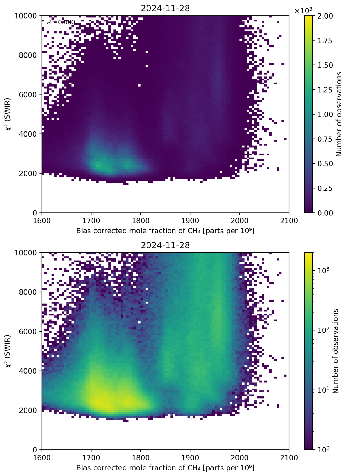
Figure 64: Scatter density plot of “Bias corrected mole fraction of \text{CH}_4 ” against “ \chi^2 (SWIR)” for 2024-11-27 to 2024-11-29.
