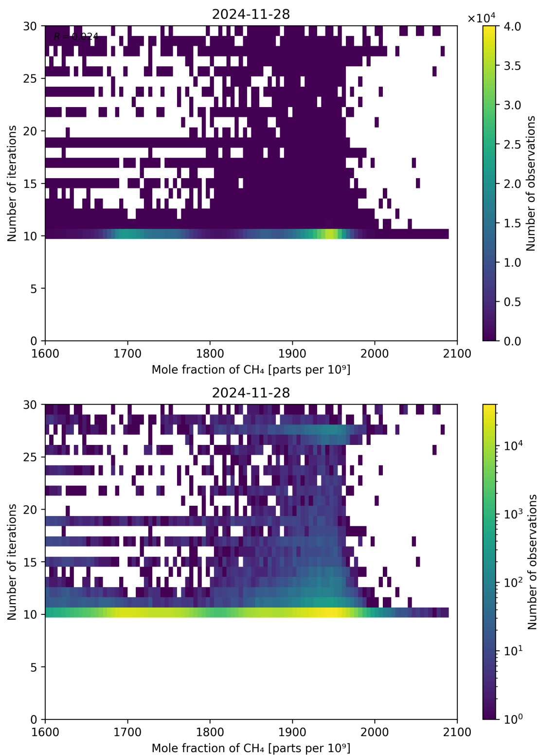
Figure 76: Scatter density plot of “Mole fraction of CH 4 ” against “Number of iterations” for 2024-11-27 to 2024-11-29.
