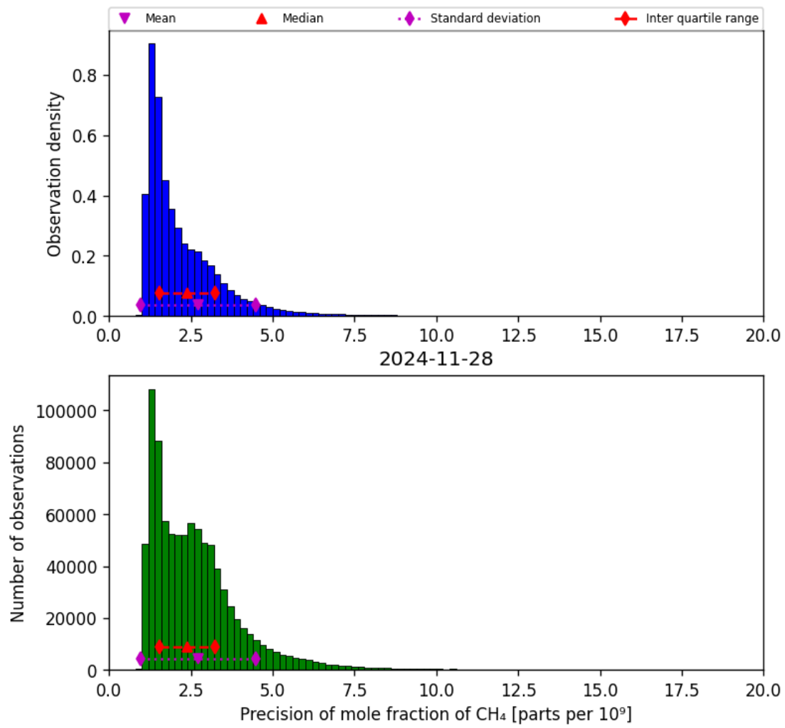
Figure 24: Histogram of “Precision of mole fraction of CH 4 ” for 2024-11-27 to 2024-11-29
