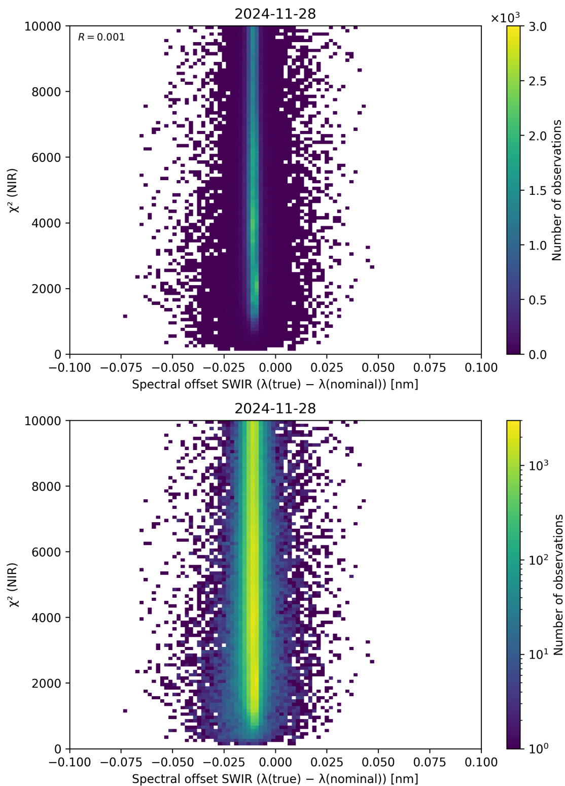
Figure 117: Scatter density plot of “Spectral offset SWIR ( \lambda_{\text{true}} - \lambda_{\text{nominal}} )” against “ \chi^2 (NIR)” for 2024-11-27 to 2024-11-29.
