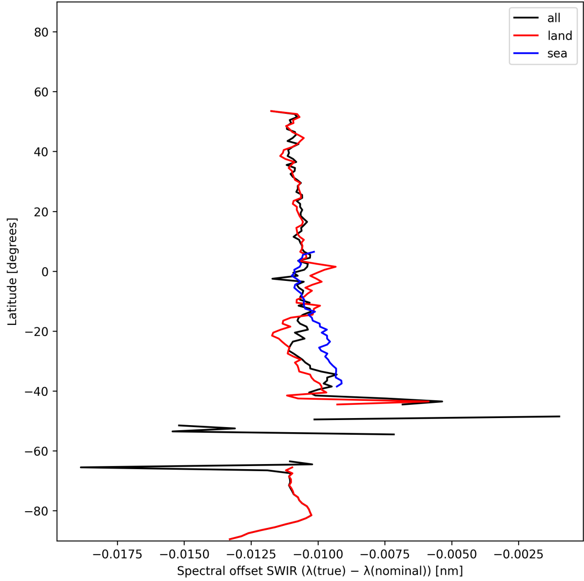
Figure 16: Zonal average of “Spectral offset SWIR ( \lambda_{\text{true}} - \lambda_{\text{nominal}} )” for 2024-11-27 to 2024-11-29.
