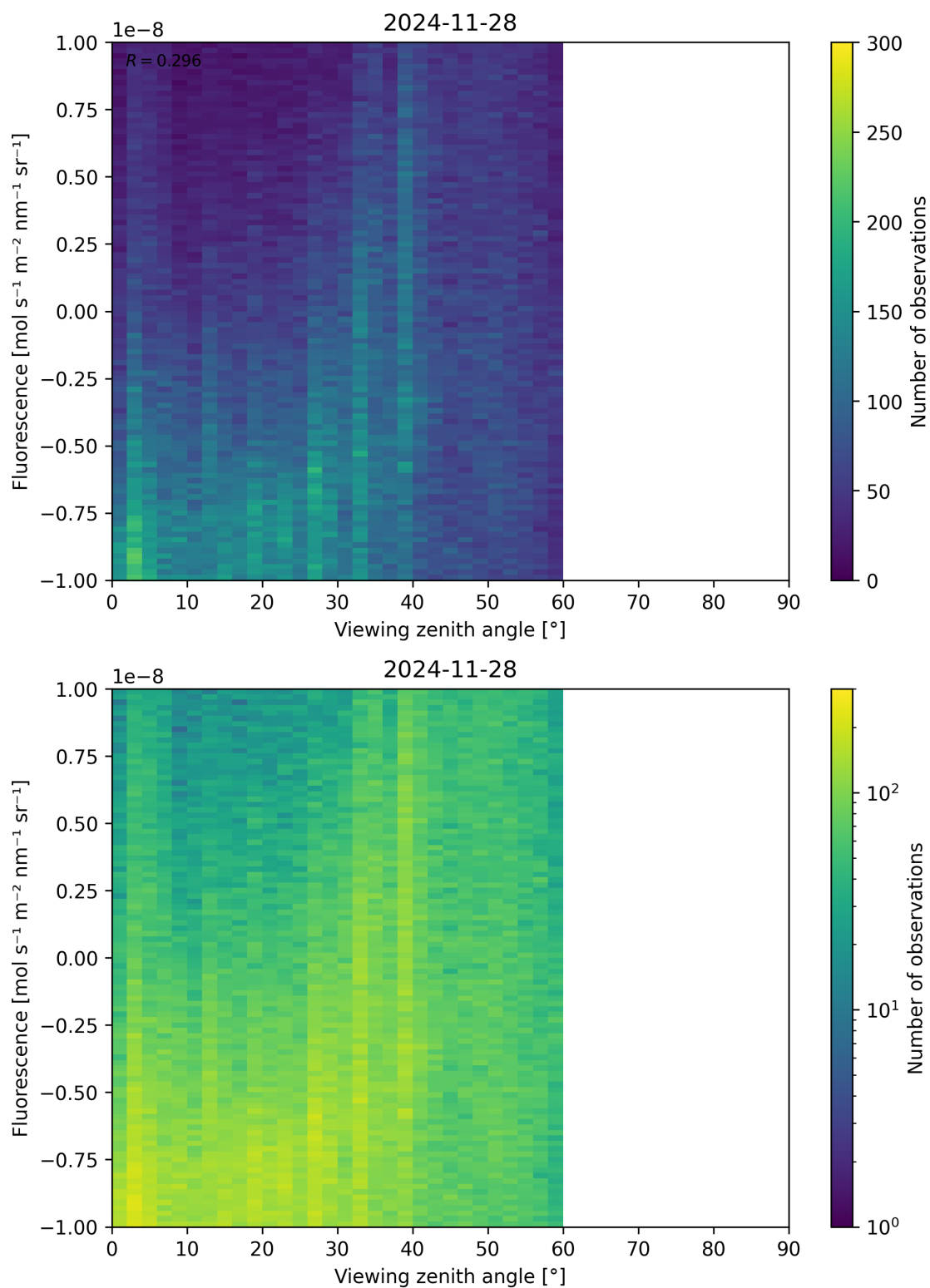
Figure 108: Scatter density plot of “Viewing zenith angle” against “Fluorescence” for 2024-11-27 to 2024-11-29.
