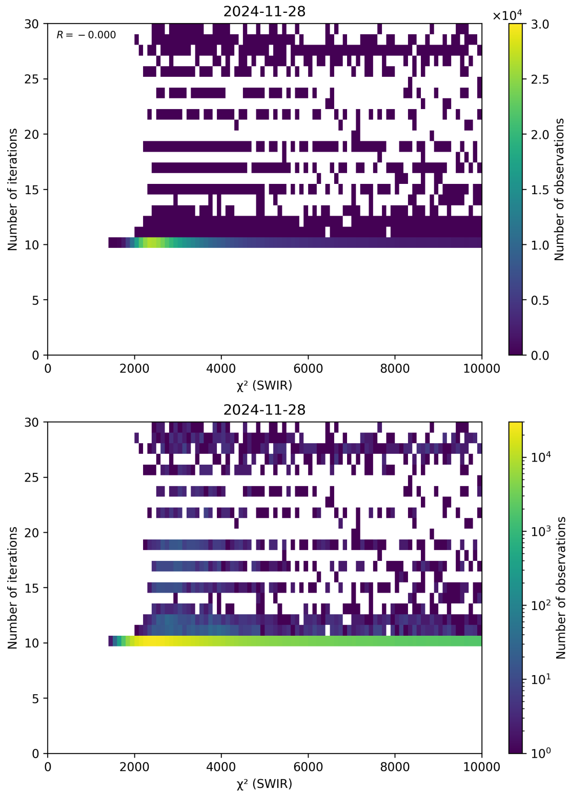
Figure 50: Scatter density plot of “ \chi^2 (SWIR)” against “Number of iterations” for 2024-11-27 to 2024-11-29.
