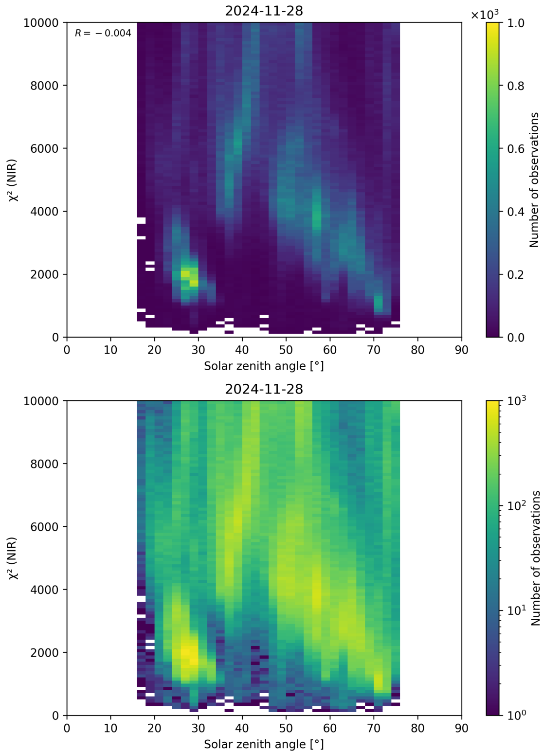
Figure 94: Scatter density plot of “Solar zenith angle” against “ \chi^2 (NIR)” for 2024-11-27 to 2024-11-29.
