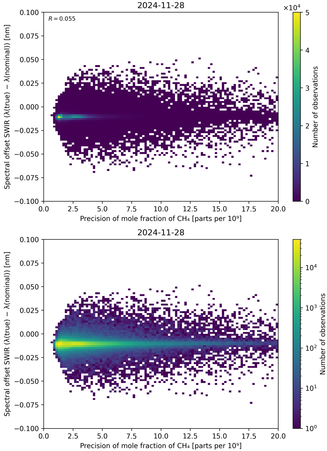
Figure 85: Scatter density plot of “Precision of mole fraction of CH 4 ” against “Spectral offset SWIR ( \lambda_{\text{true}} - \lambda_{\text{nominal}} )” for 2024-11-27 to 2024-11-29.
