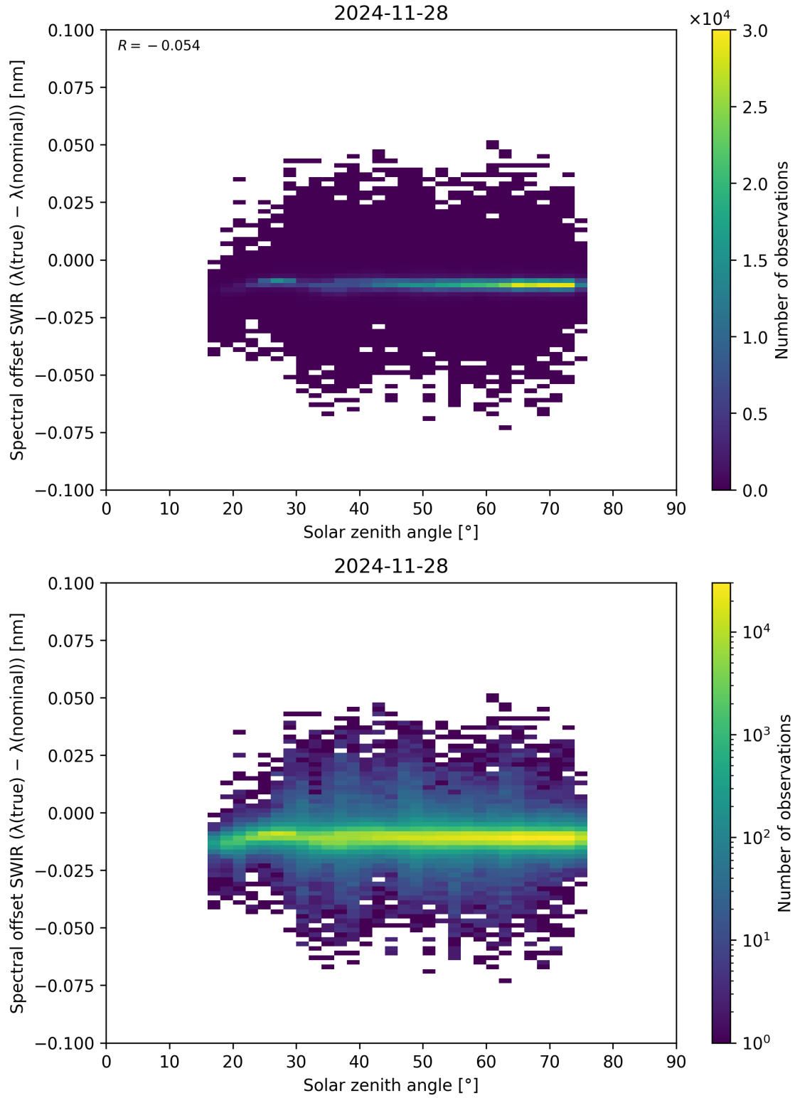
Figure 104: Scatter density plot of “Solar zenith angle” against “Spectral offset SWIR ( \lambda_{\text{true}} - \lambda_{\text{nominal}} )” for 2024-11-27 to 2024-11-29.
