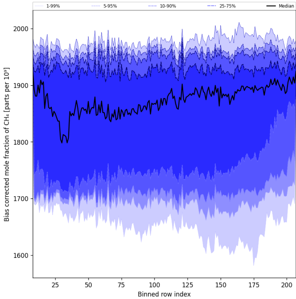
Figure 36: Along track statistics of “Bias corrected mole fraction of CH 4 ” for 2024-11-27 to 2024-11-29
