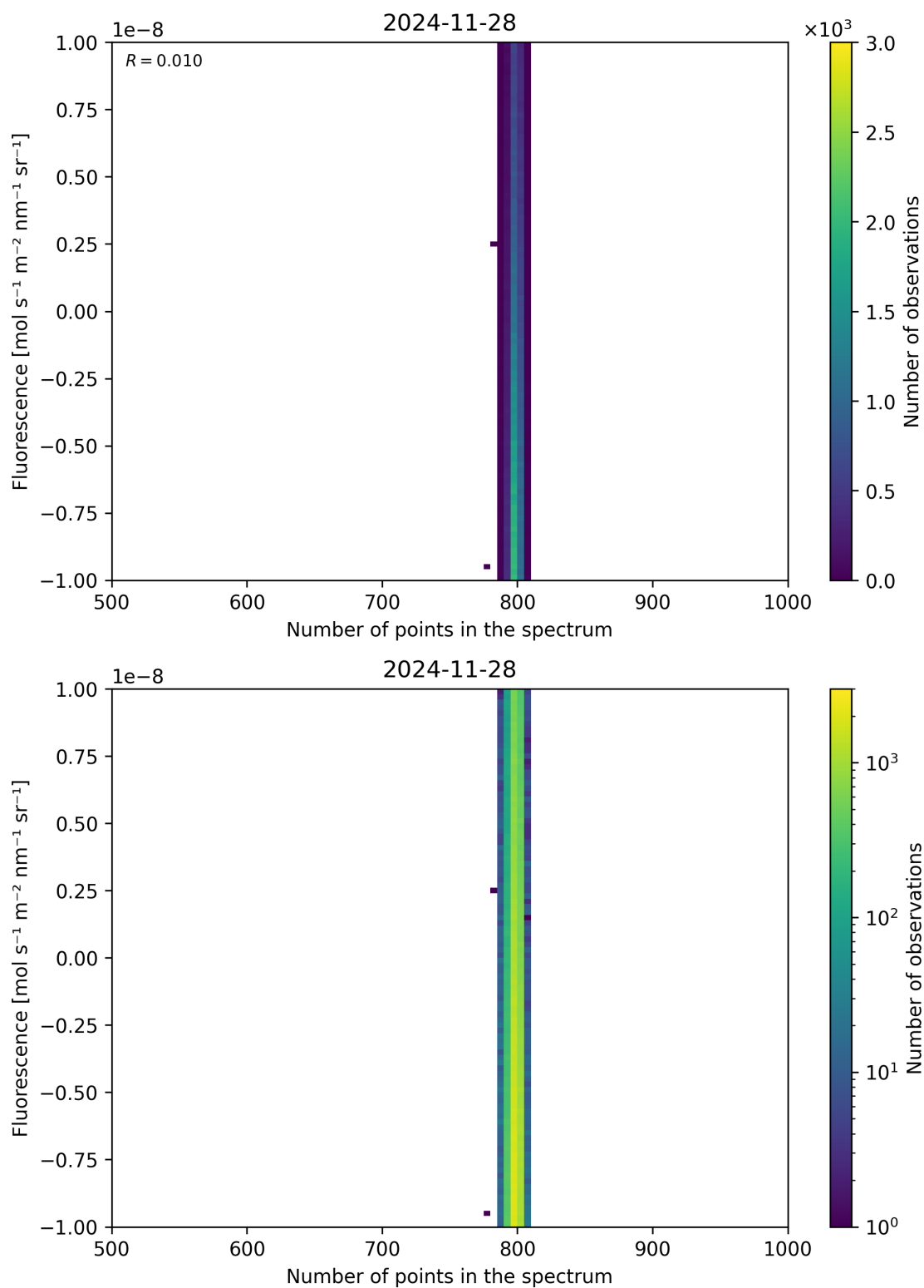
Figure 91: Scatter density plot of “Number of points in the spectrum” against “Fluorescence” for 2024-11-27 to 2024-11-29.
