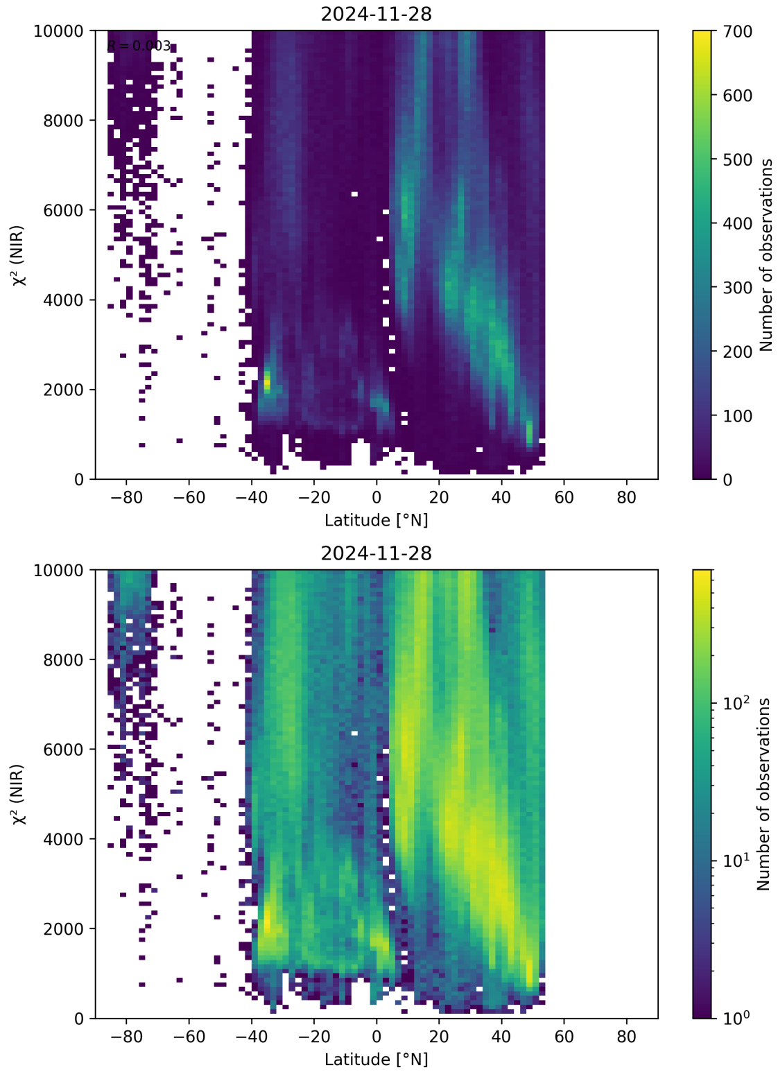
Figure 53: Scatter density plot of “Latitude” against “ \chi^2 (NIR)” for 2024-11-27 to 2024-11-29.
