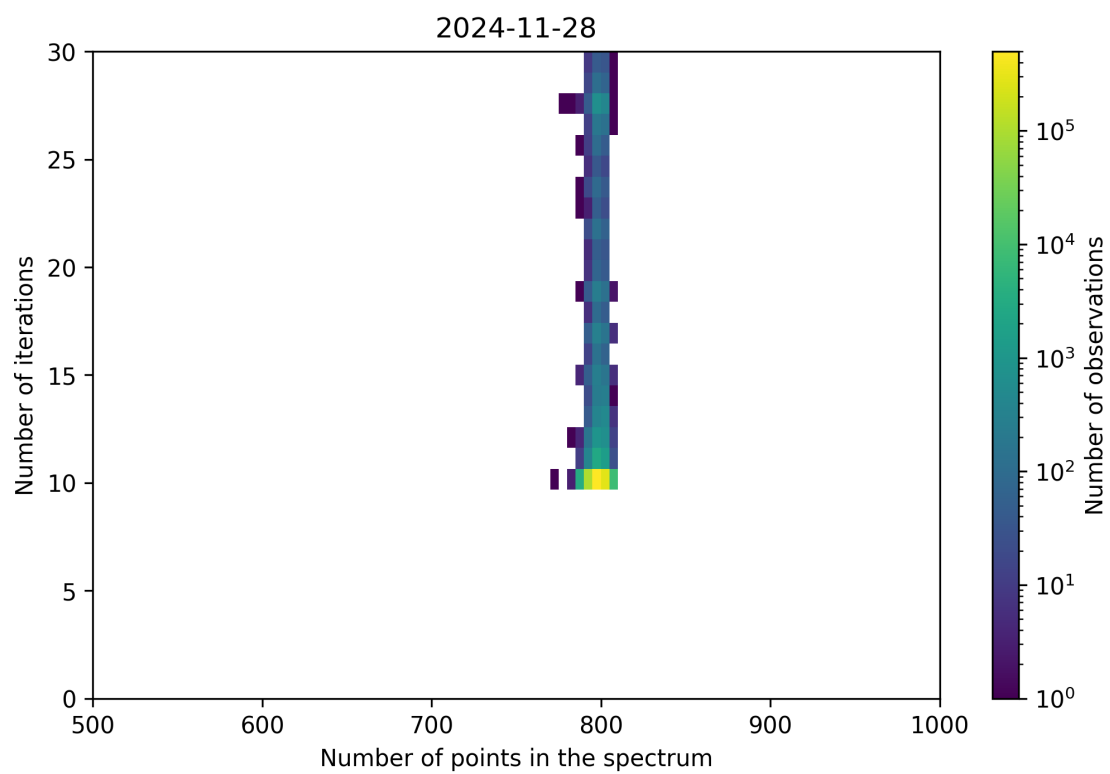
Figure 92: Scatter density plot of “Number of points in the spectrum” against “Number of iterations” for 2024-11-27 to 2024-11-29.
