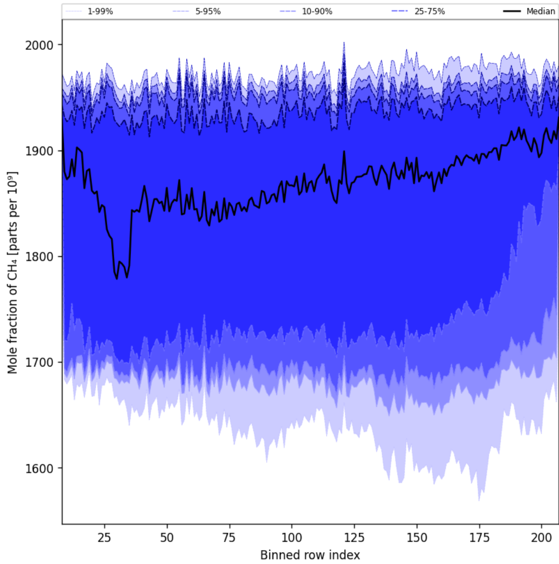
Figure 34: Along track statistics of “Mole fraction of CH 4 ” for 2024-11-27 to 2024-11-29
