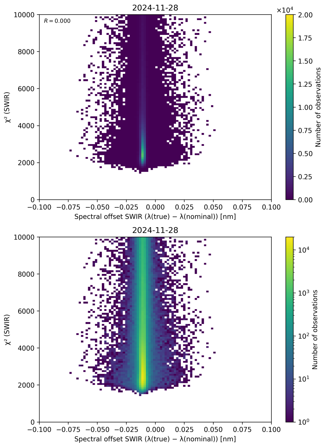
Figure 118: Scatter density plot of “Spectral offset SWIR ( \lambda_{\text{true}} - \lambda_{\text{nominal}} )” against “ \chi^2 (SWIR)” for 2024-11-27 to 2024-11-29.
