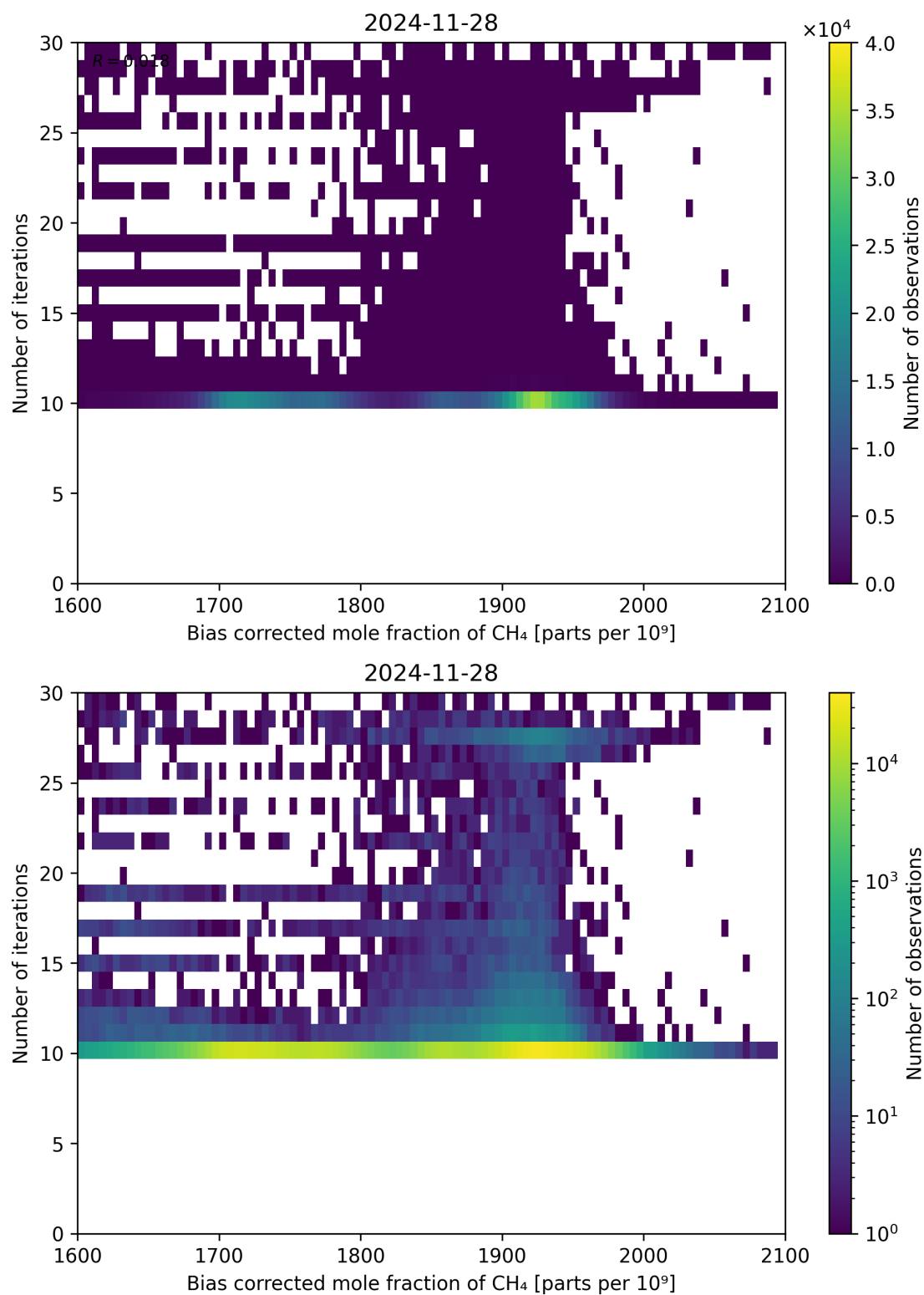
Figure 67: Scatter density plot of “Bias corrected mole fraction of \text{CH}_4 ” against “Number of iterations” for 2024-11-27 to 2024-11-29.
