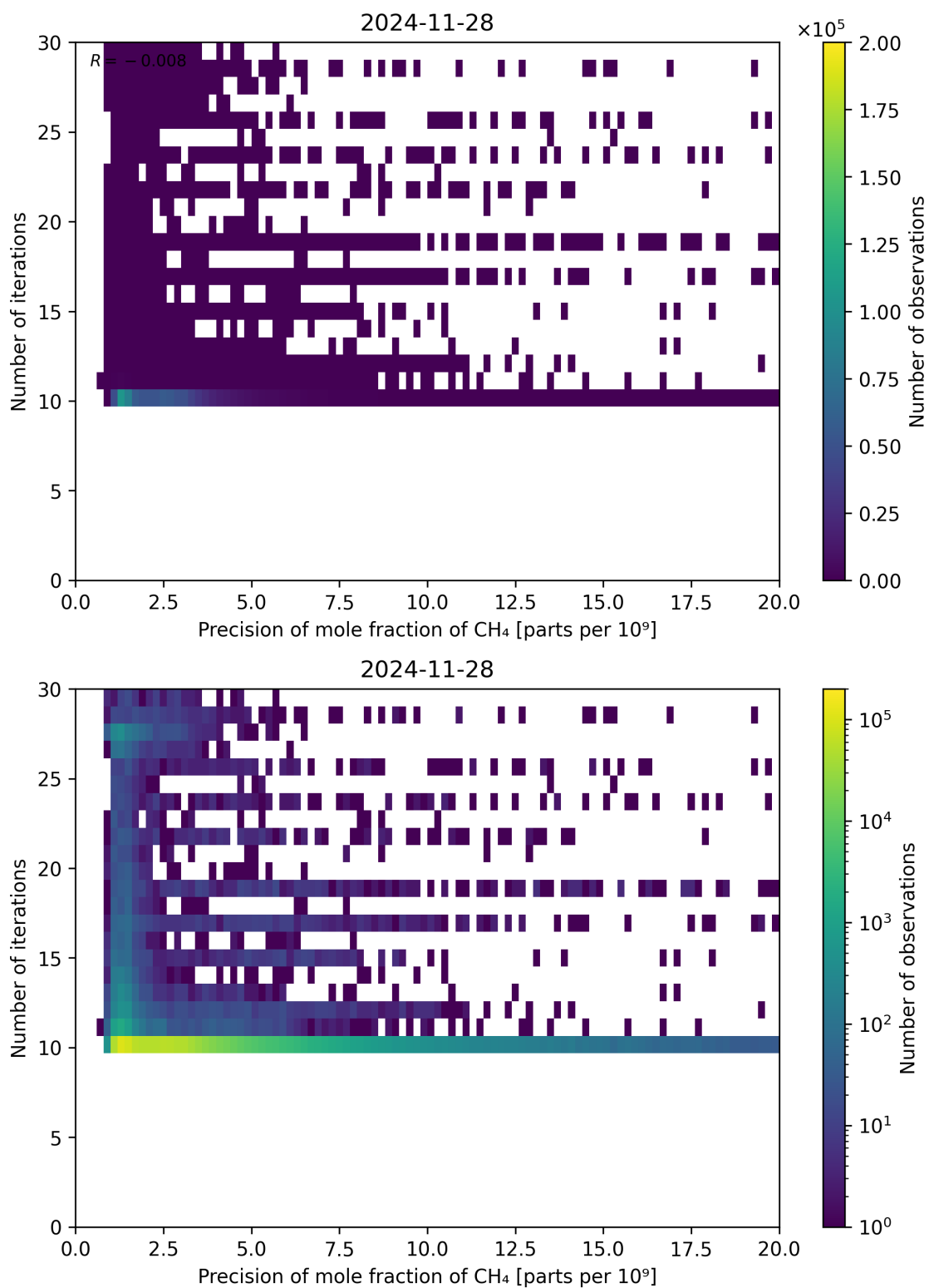
Figure 83: Scatter density plot of “Precision of mole fraction of CH 4 ” against “Number of iterations” for 2024-11-27 to 2024-11-29.
