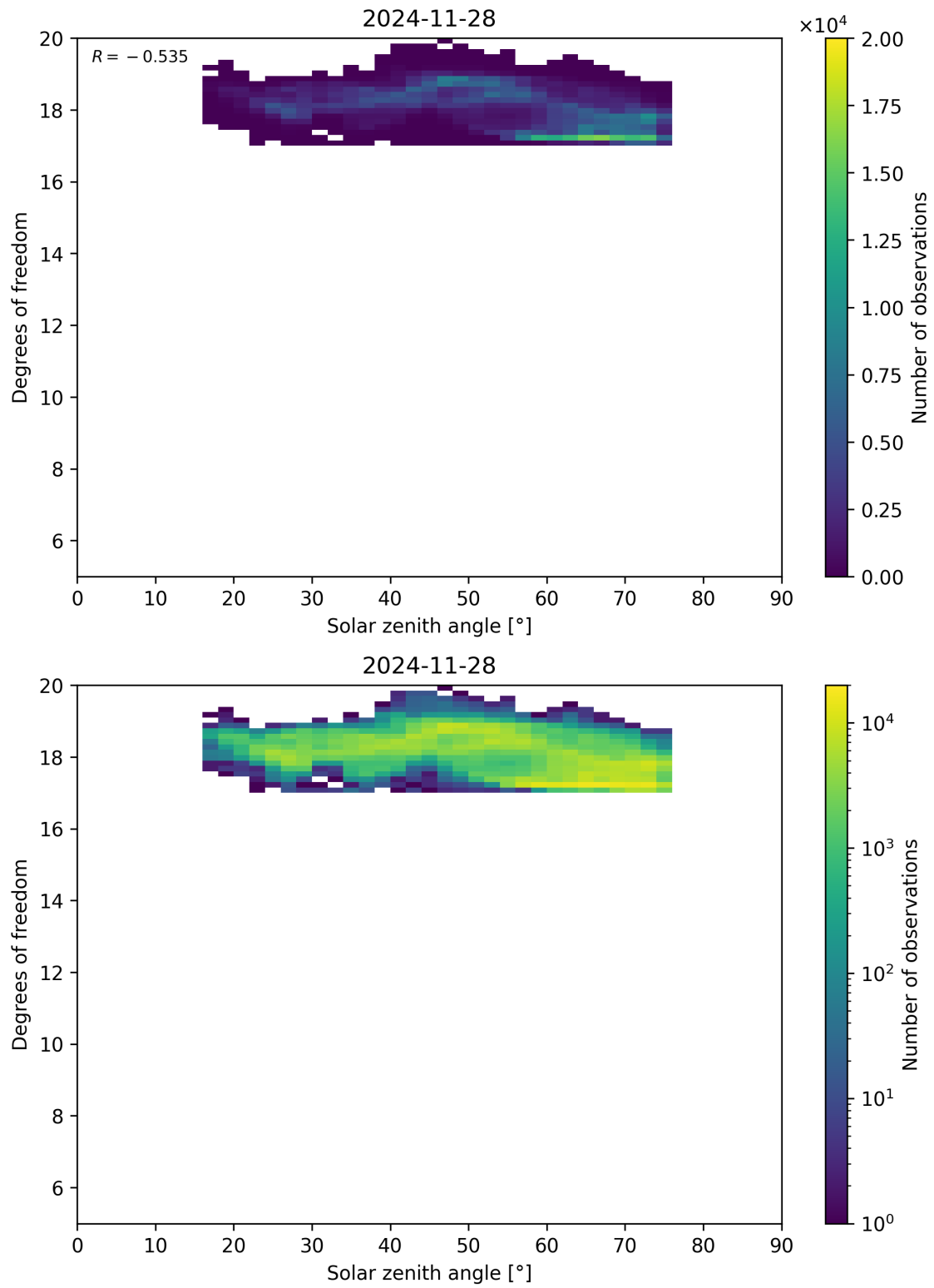
Figure 96: Scatter density plot of “Solar zenith angle” against “Degrees of freedom” for 2024-11-27 to 2024-11-29.
