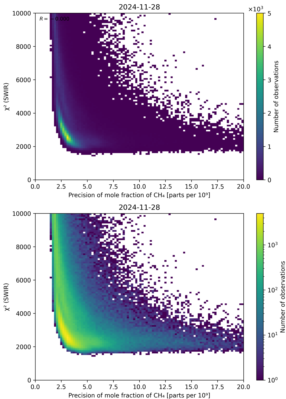
Figure 79: Scatter density plot of “Precision of mole fraction of \text{CH}_4 ” against “ \chi^2 (SWIR)” for 2024-11-27 to 2024-11-29.
