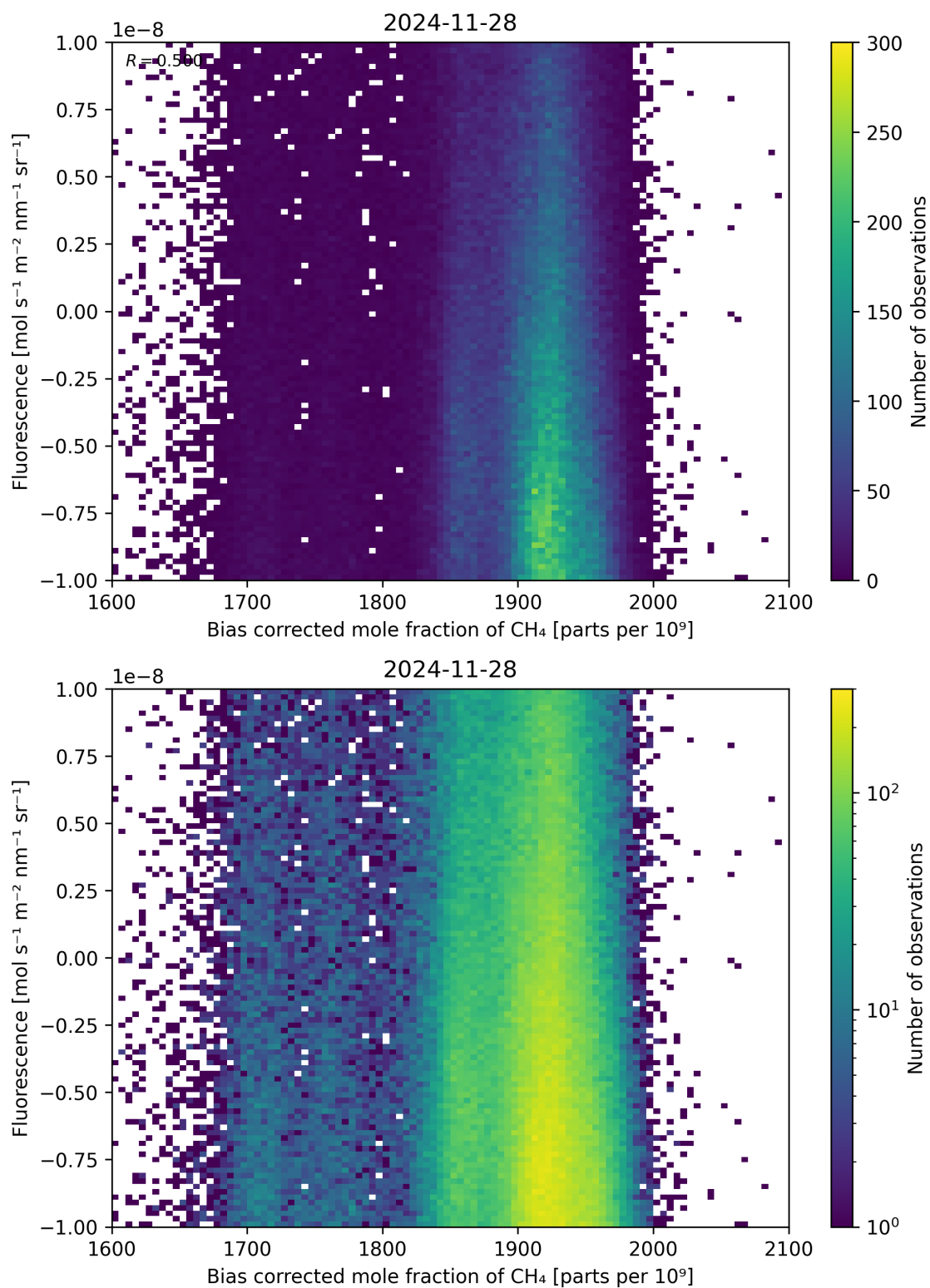
Figure 66: Scatter density plot of “Bias corrected mole fraction of \text{CH}_4 ” against “Fluorescence” for 2024-11-27 to 2024-11-29.
