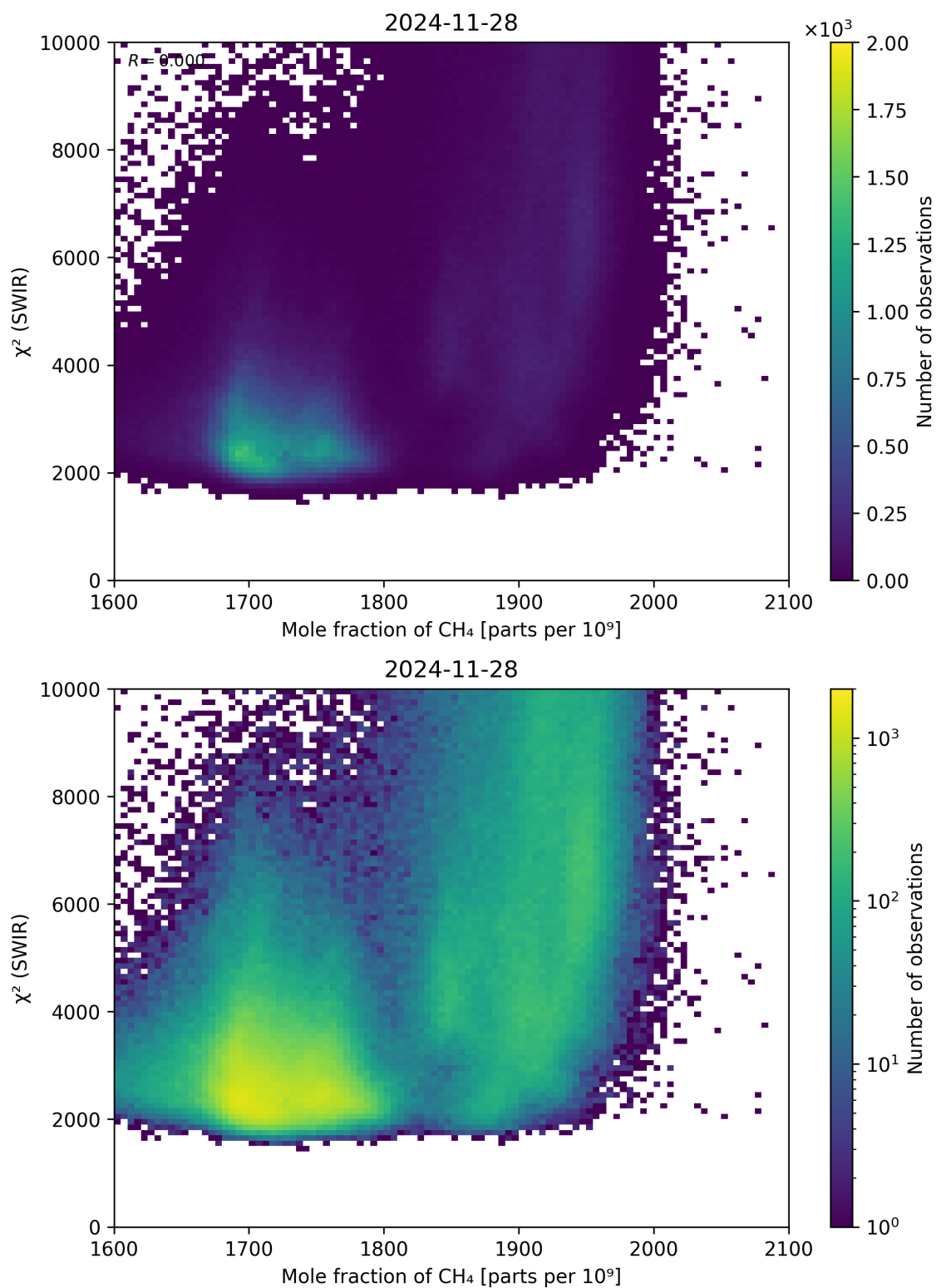
Figure 71: Scatter density plot of “Mole fraction of \text{CH}_4 ” against “ \chi^2 (SWIR)” for 2024-11-27 to 2024-11-29.
