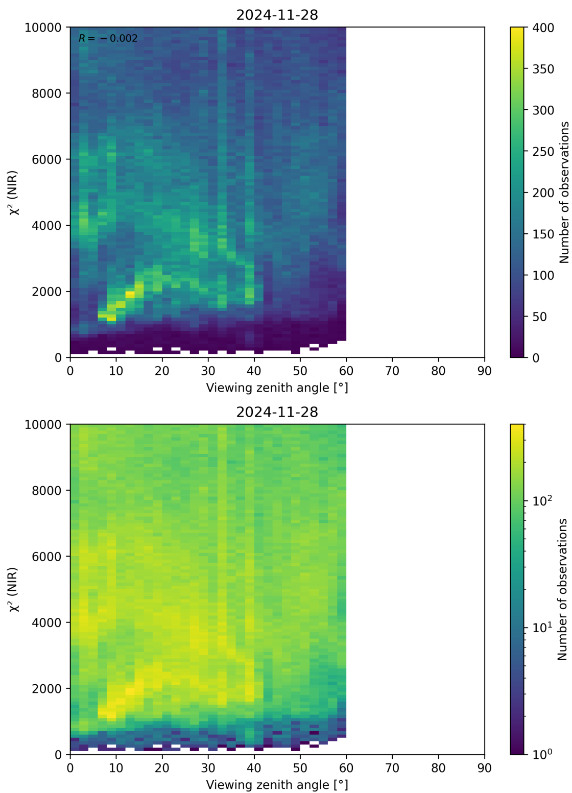
Figure 105: Scatter density plot of “Viewing zenith angle” against “ \chi^2 (NIR)” for 2024-11-27 to 2024-11-29.
