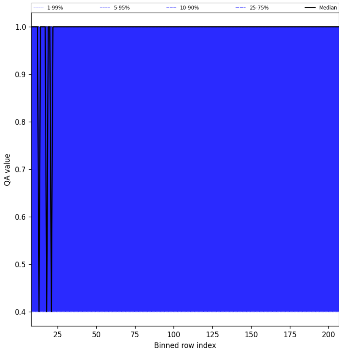
Figure 33: Along track statistics of “QA value” for 2024-11-27 to 2024-11-29
