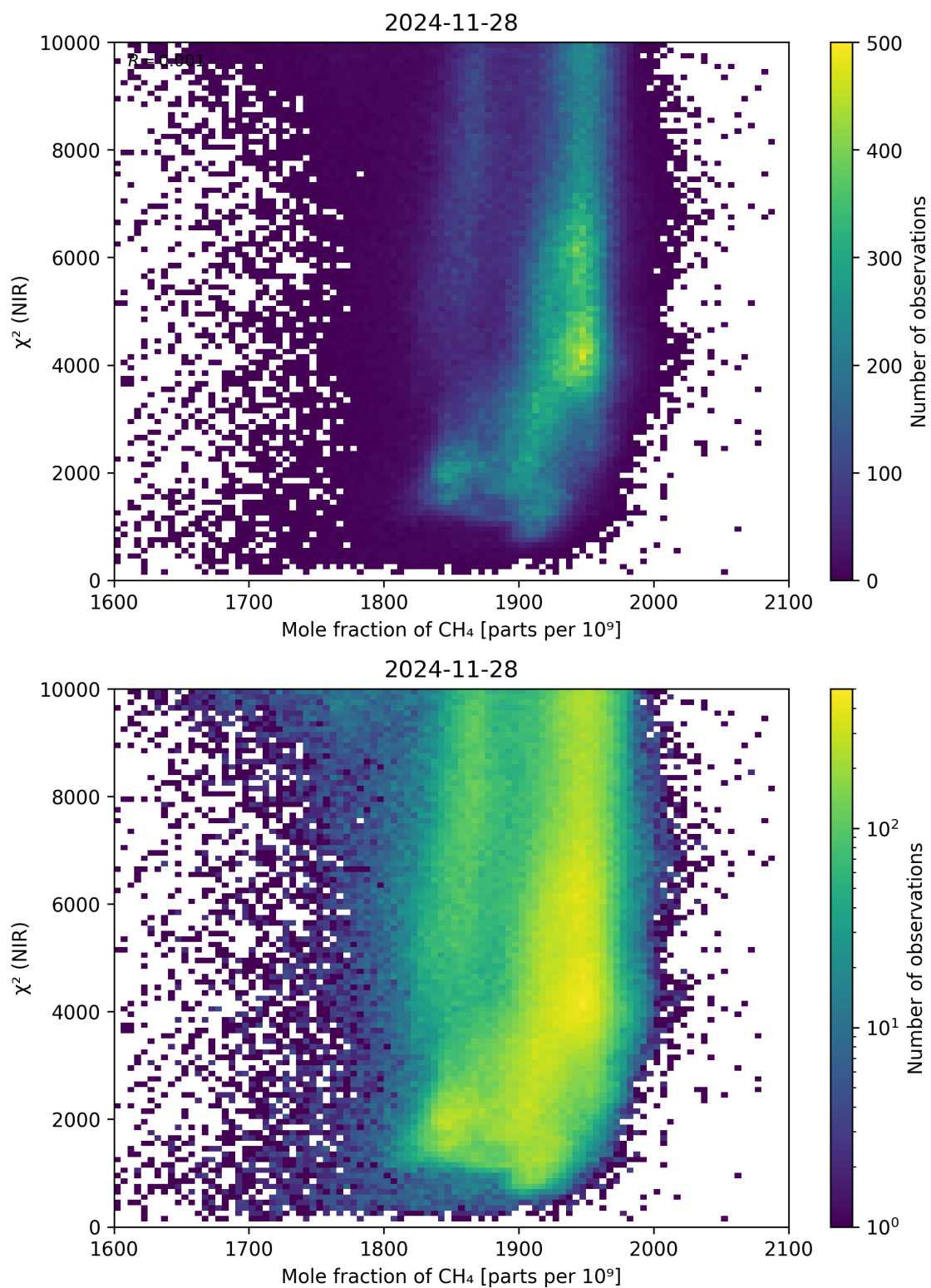
Figure 70: Scatter density plot of “Mole fraction of \text{CH}_4 ” against “ \chi^2 (NIR)” for 2024-11-27 to 2024-11-29.
