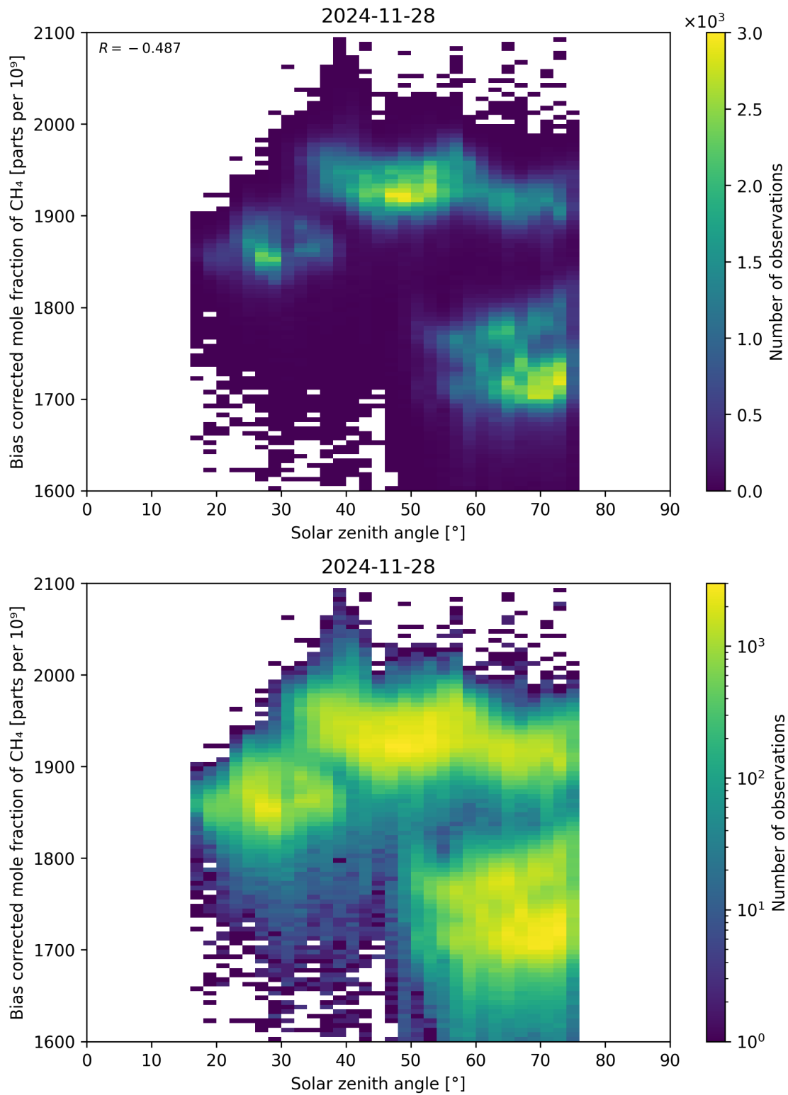
Figure 100: Scatter density plot of “Solar zenith angle” against “Bias corrected mole fraction of CH 4 ” for 2024-11-27 to 2024-11-29.
