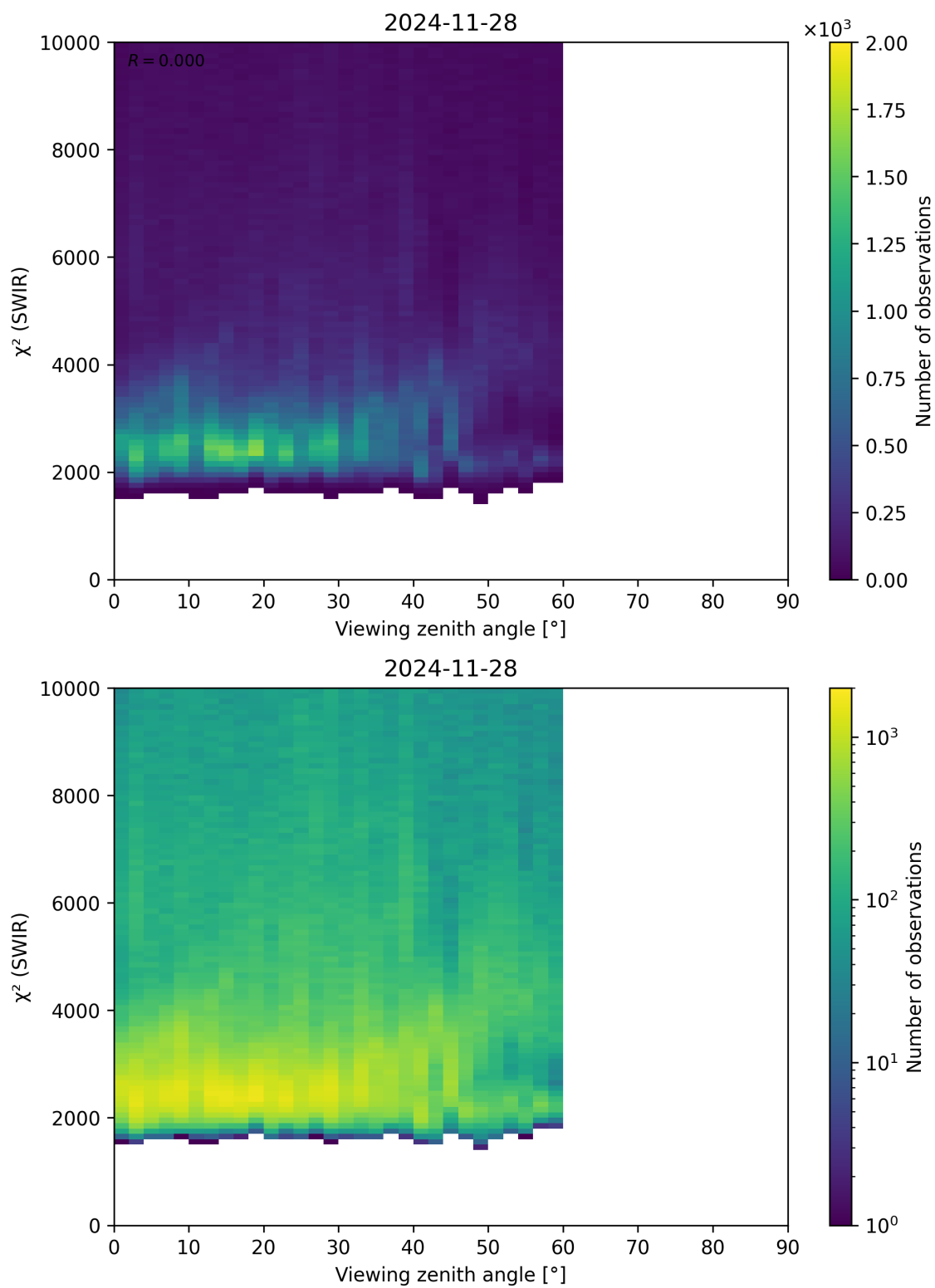
Figure 106: Scatter density plot of “Viewing zenith angle” against “ \chi^2 (SWIR)” for 2024-11-27 to 2024-11-29.
