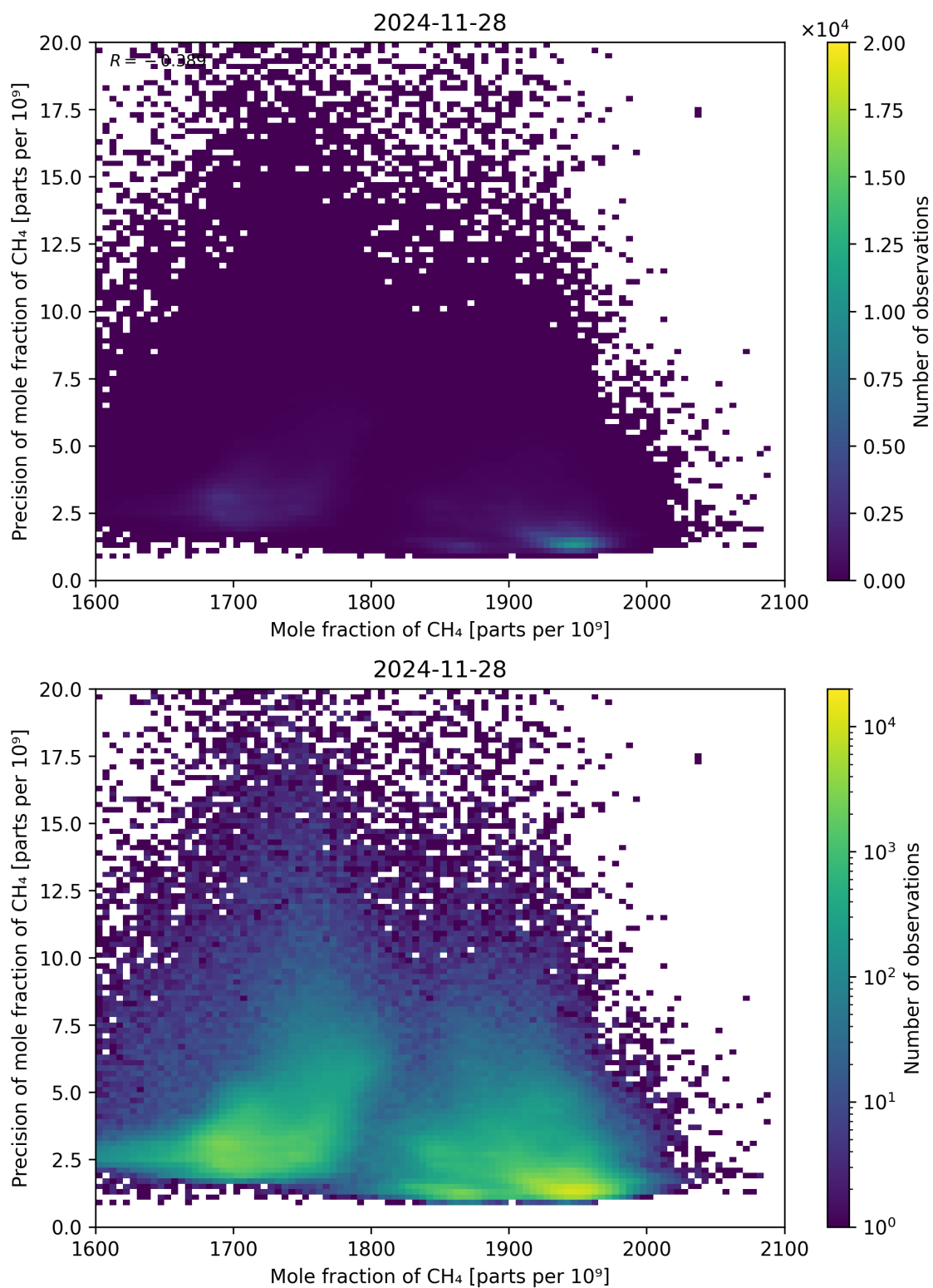
Figure 75: Scatter density plot of “Mole fraction of CH 4 ” against “Precision of mole fraction of CH 4 ” for 2024-11-27 to 2024-11-29.
