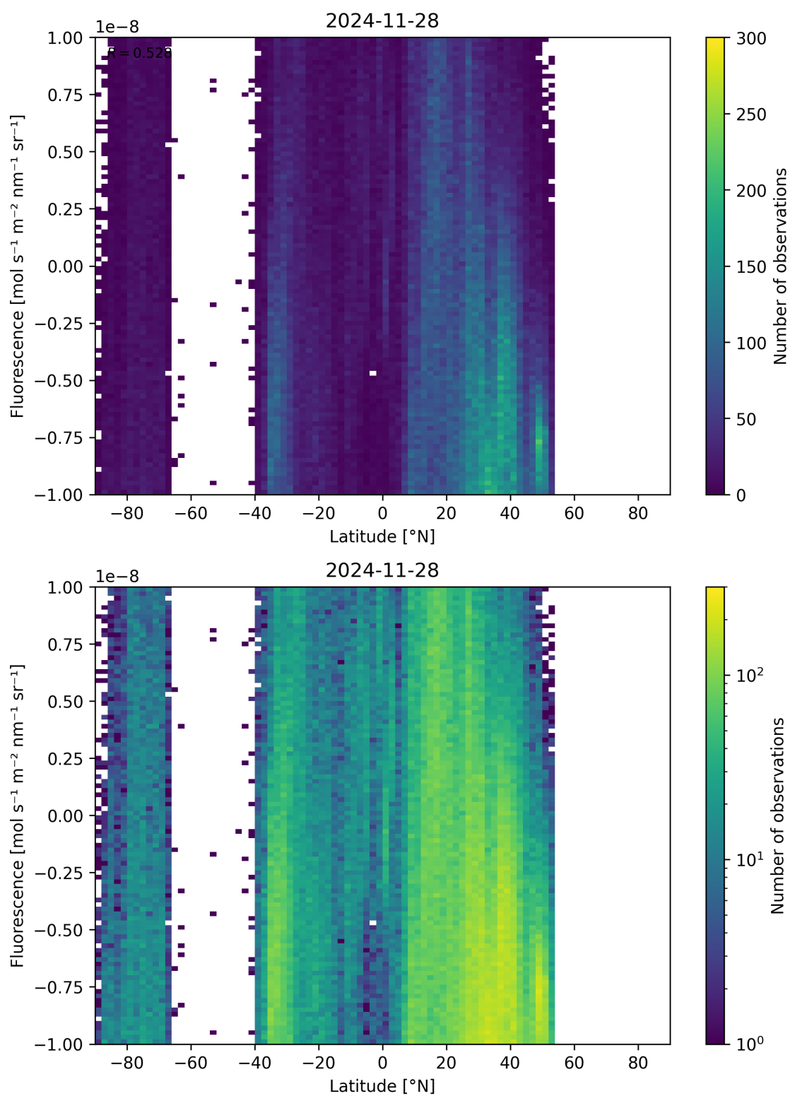
Figure 56: Scatter density plot of “Latitude” against “Fluorescence” for 2024-11-27 to 2024-11-29.
