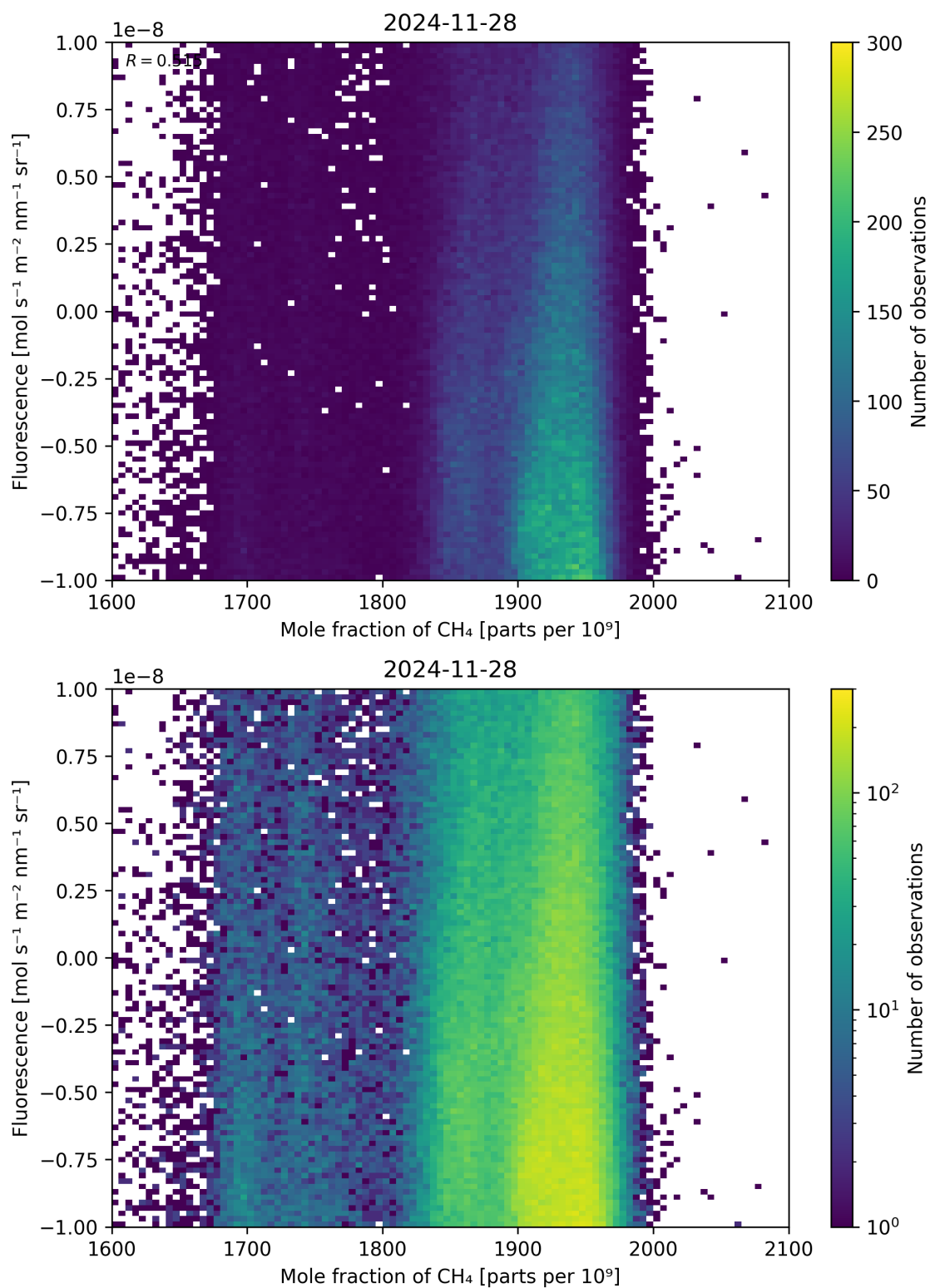
Figure 73: Scatter density plot of “Mole fraction of \text{CH}_4 ” against “Fluorescence” for 2024-11-27 to 2024-11-29.
