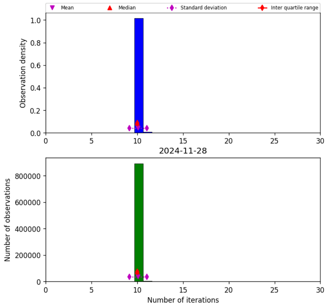
Figure 31: Histogram of “Number of iterations” for 2024-11-27 to 2024-11-29
