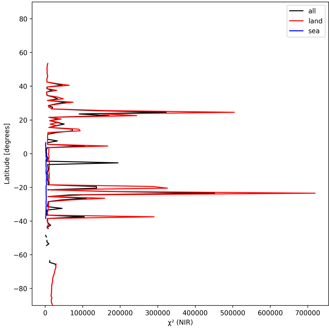
Figure 18: Zonal average of “ \chi^2 (NIR)” for 2024-11-27 to 2024-11-29.
