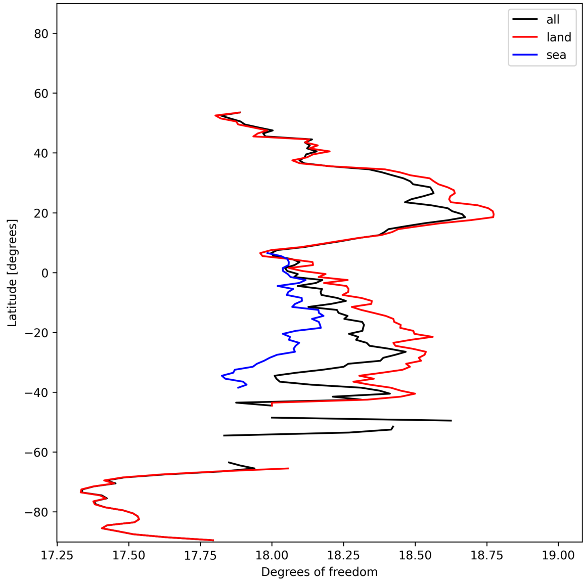
Figure 19: Zonal average of “Degrees of freedom” for 2024-11-27 to 2024-11-29.
