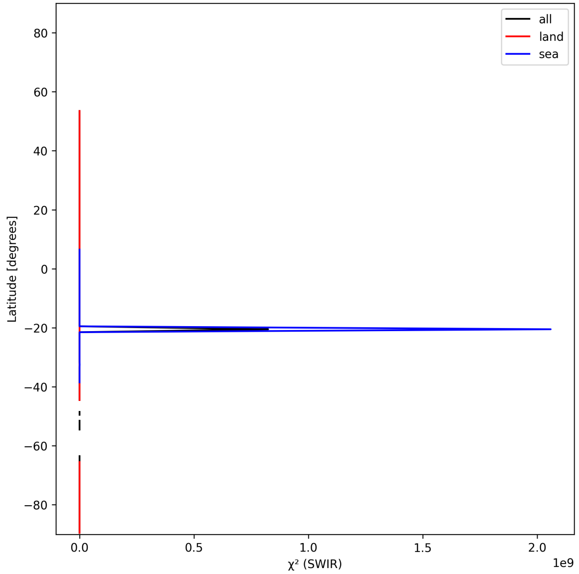
Figure 17: Zonal average of “ \chi^2 (SWIR)” for 2024-11-27 to 2024-11-29.
