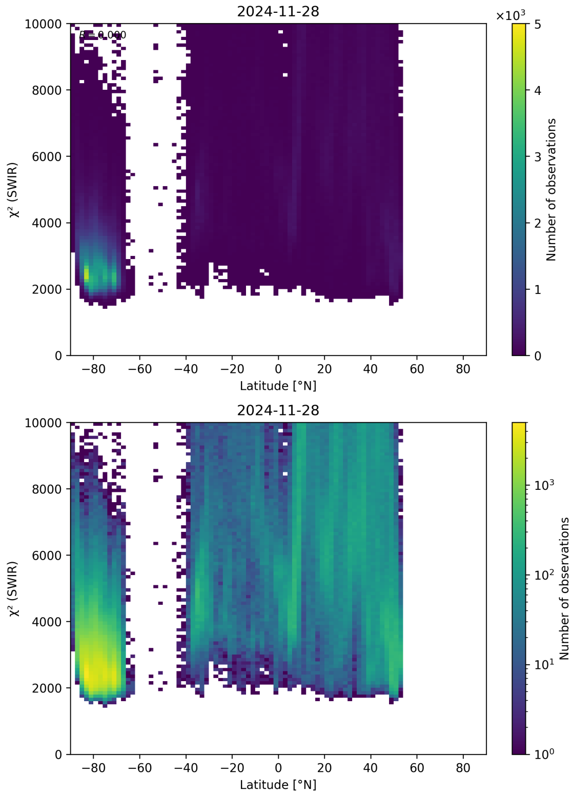
Figure 54: Scatter density plot of “Latitude” against “ \chi^2 (SWIR)” for 2024-11-27 to 2024-11-29.
