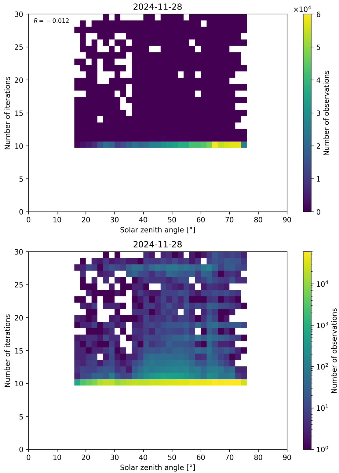
Figure 102: Scatter density plot of “Solar zenith angle” against “Number of iterations” for 2024-11-27 to 2024-11-29.
