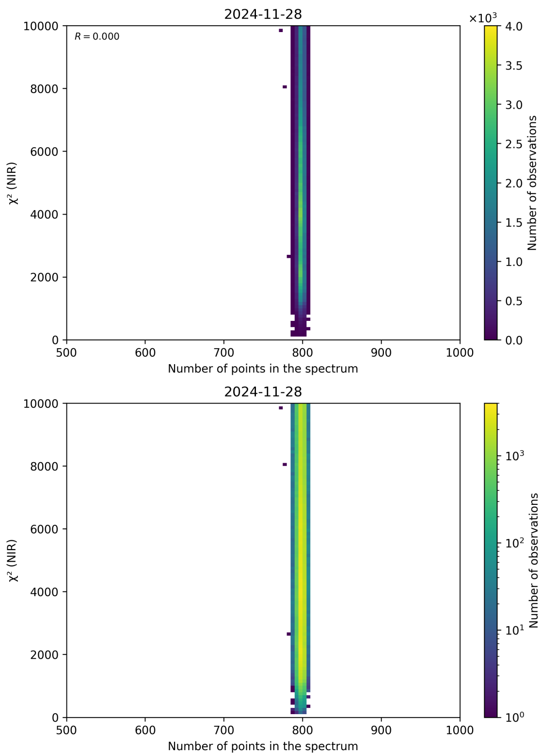
Figure 88: Scatter density plot of “Number of points in the spectrum” against “ \chi^2 (NIR)” for 2024-11-27 to 2024-11-29.
