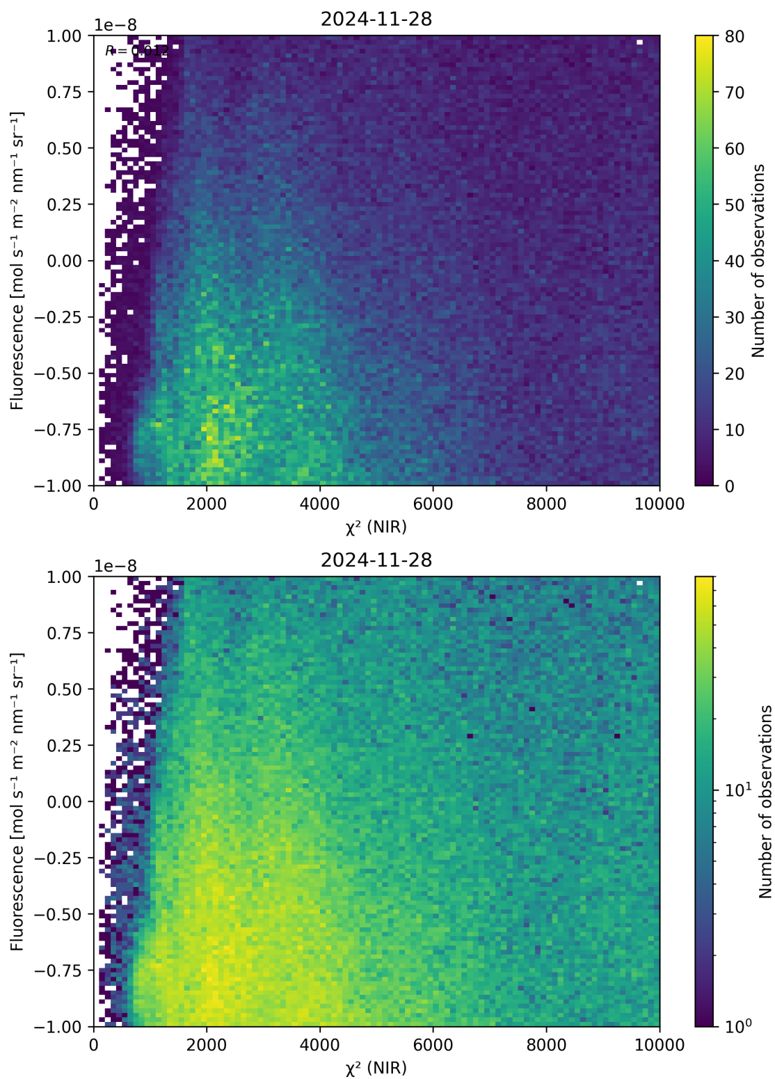
Figure 45: Scatter density plot of “ \chi^2 (NIR)” against “Fluorescence” for 2024-11-27 to 2024-11-29.
