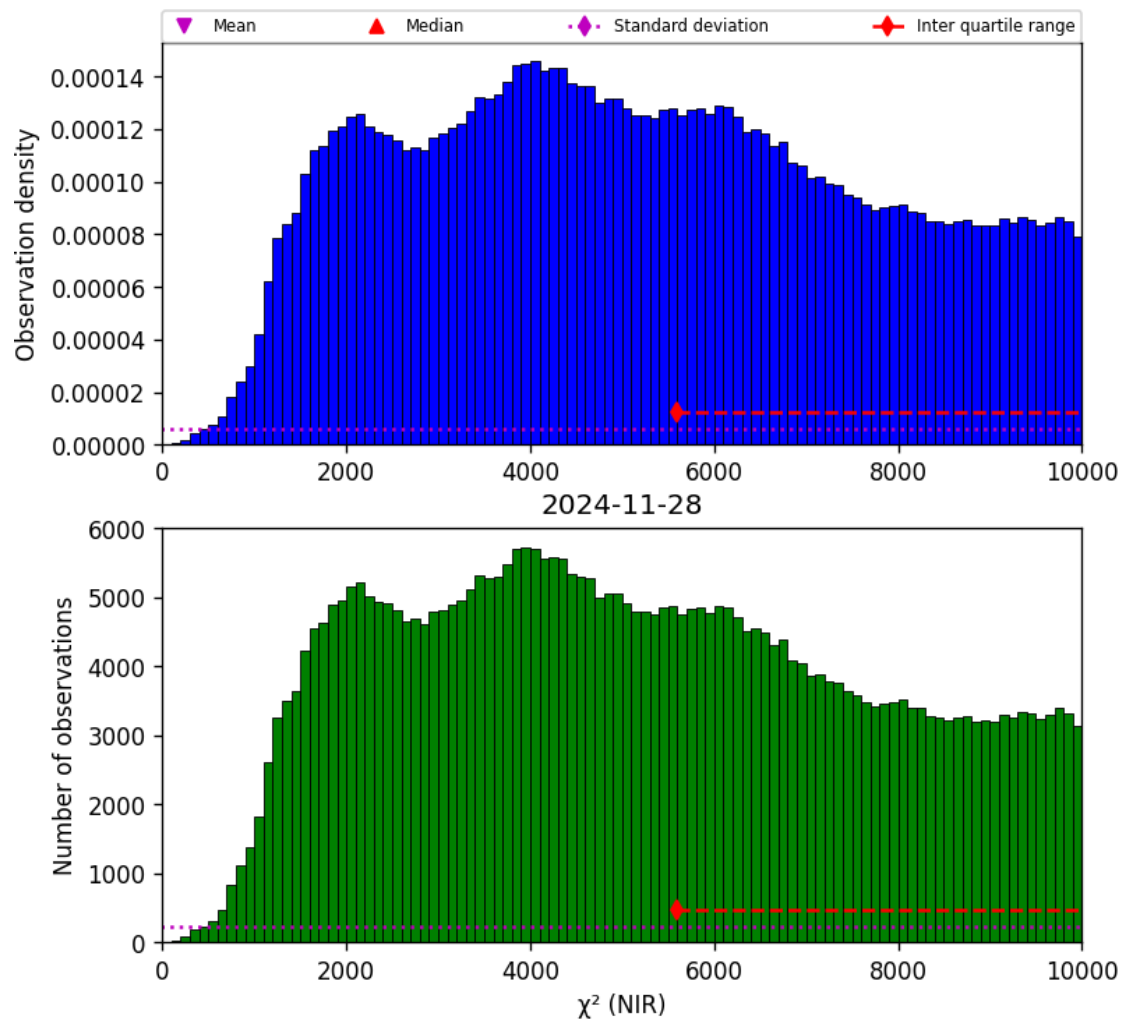
Figure 29: Histogram of “ \chi^2 (NIR)” for 2024-11-27 to 2024-11-29
