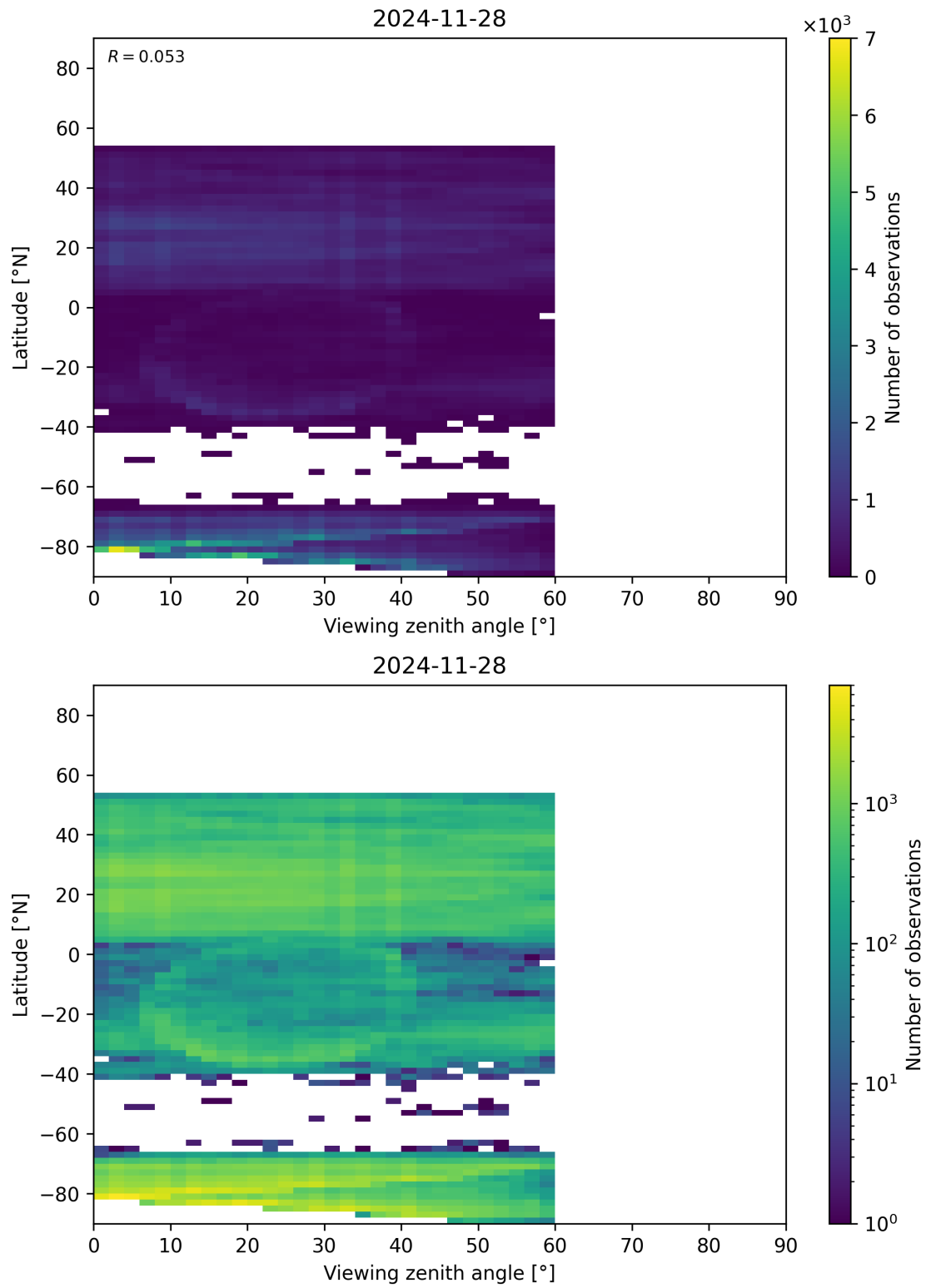
Figure 109: Scatter density plot of “Viewing zenith angle” against “Latitude” for 2024-11-27 to 2024-11-29.
