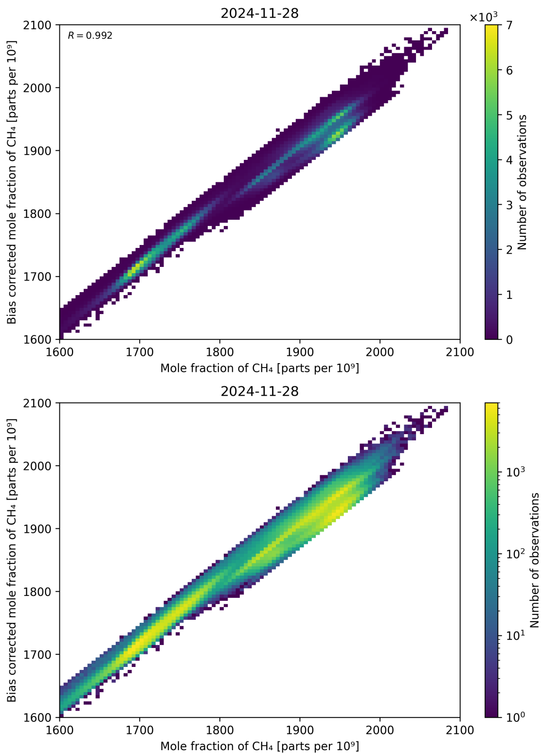
Figure 74: Scatter density plot of “Mole fraction of CH 4 ” against “Bias corrected mole fraction of CH 4 ” for 2024-11-27 to 2024-11-29.
