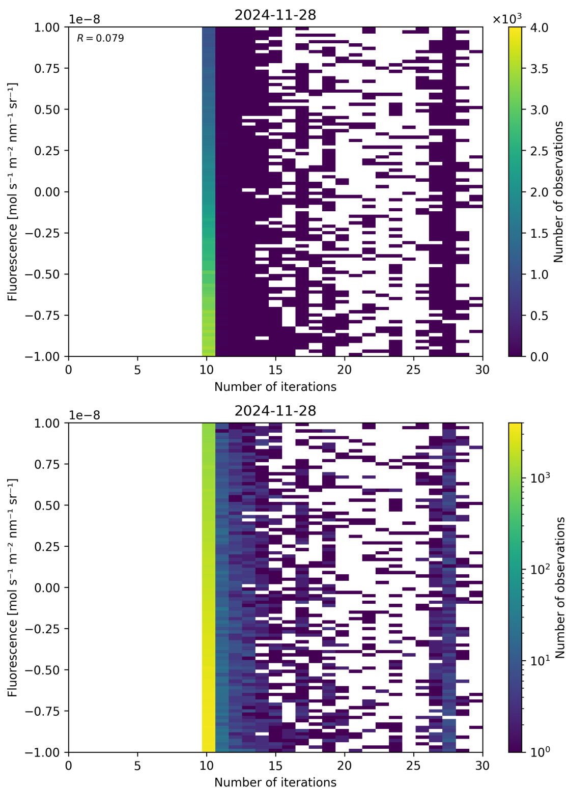
Figure 87: Scatter density plot of “Number of iterations” against “Fluorescence” for 2024-11-27 to 2024-11-29.
