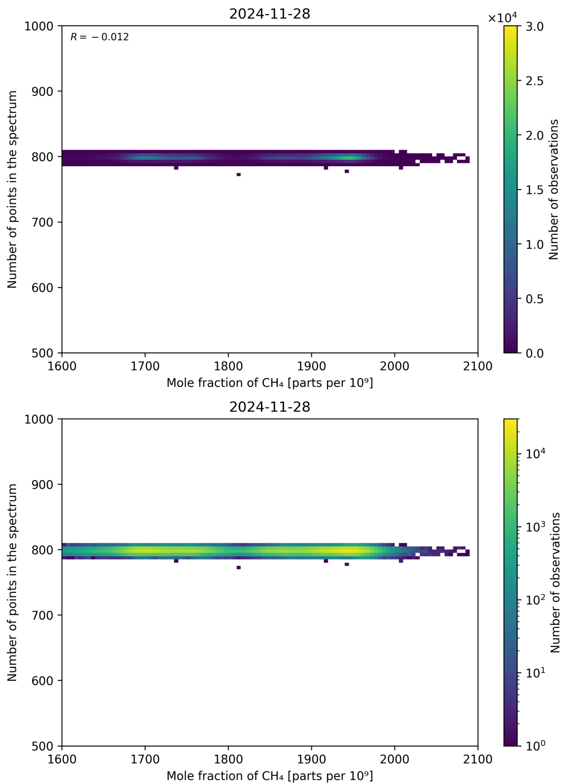
Figure 77: Scatter density plot of “Mole fraction of CH 4 ” against “Number of points in the spectrum” for 2024-11-27 to 2024-11-29.
