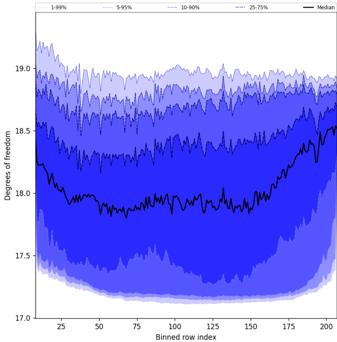
Figure 41: Along track statistics of “Degrees of freedom” for 2024-11-27 to 2024-11-29
