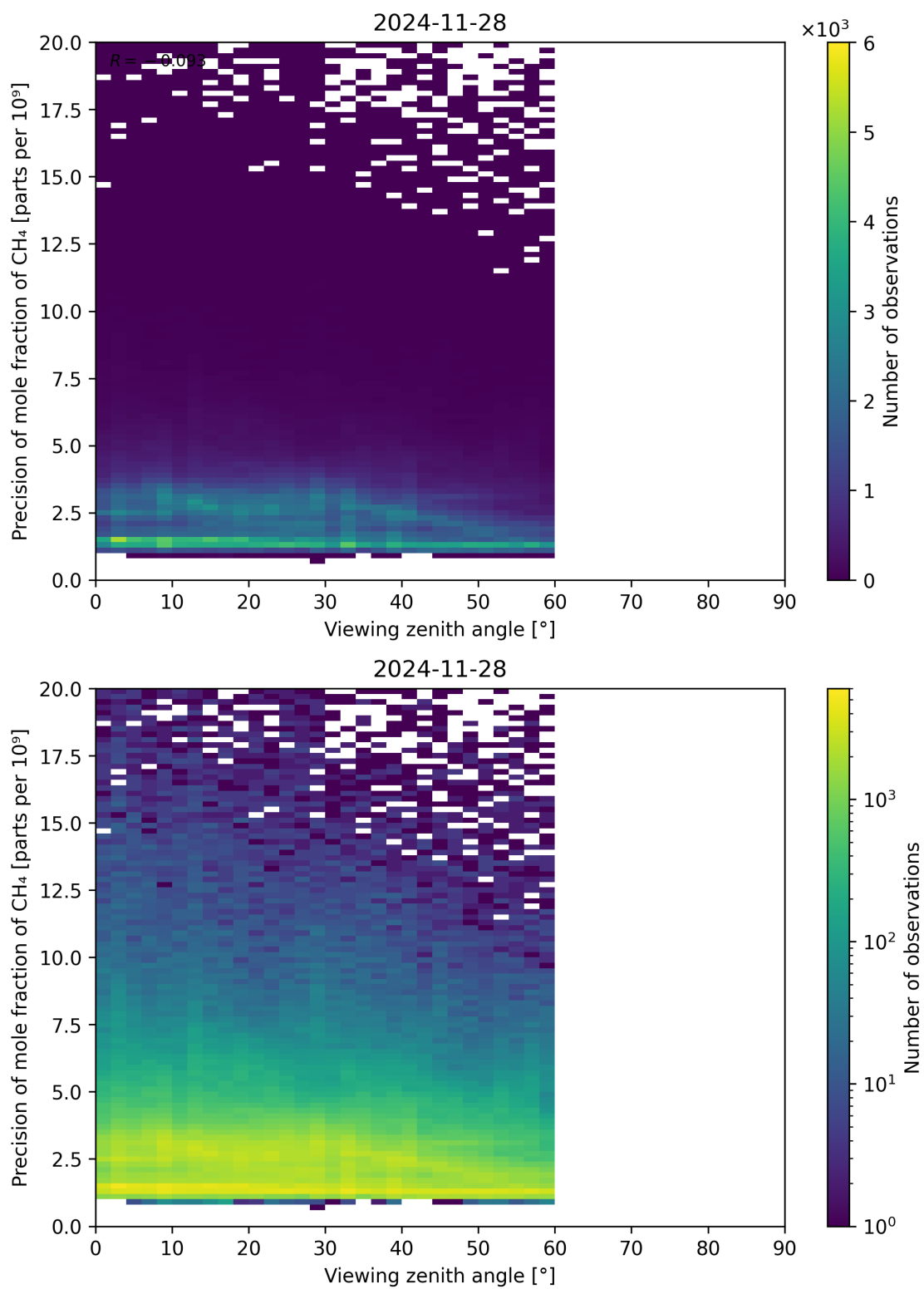
Figure 112: Scatter density plot of “Viewing zenith angle” against “Precision of mole fraction of CH 4 ” for 2024-11-27 to 2024-11-29.
