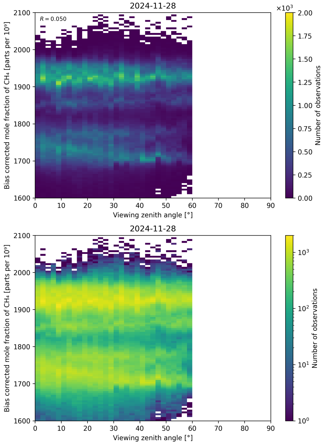
Figure 111: Scatter density plot of “Viewing zenith angle” against “Bias corrected mole fraction of CH 4 ” for 2024-11-27 to 2024-11-29.
