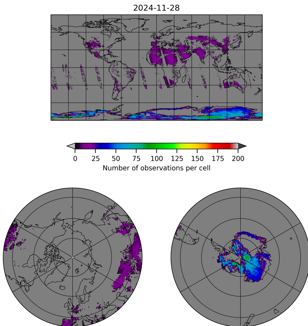
Figure 10: Map of the number of observations for 2024-11-27 to 2024-11-29
