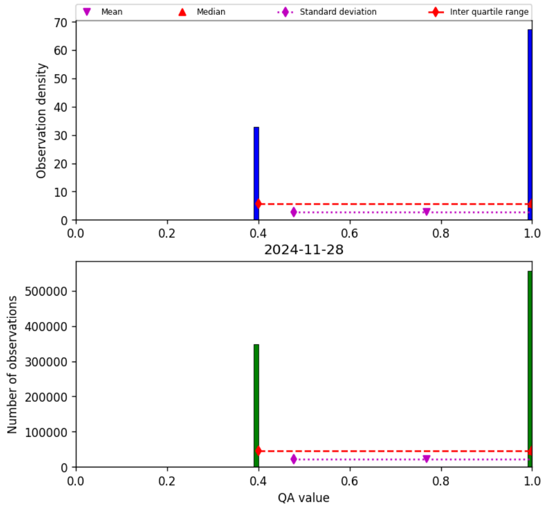
Figure 22: Histogram of “QA value” for 2024-11-27 to 2024-11-29
