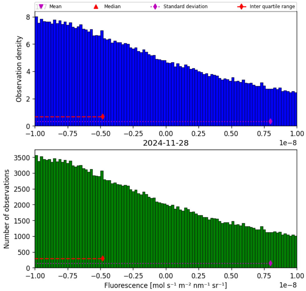
Figure 32: Histogram of “Fluorescence” for 2024-11-27 to 2024-11-29
