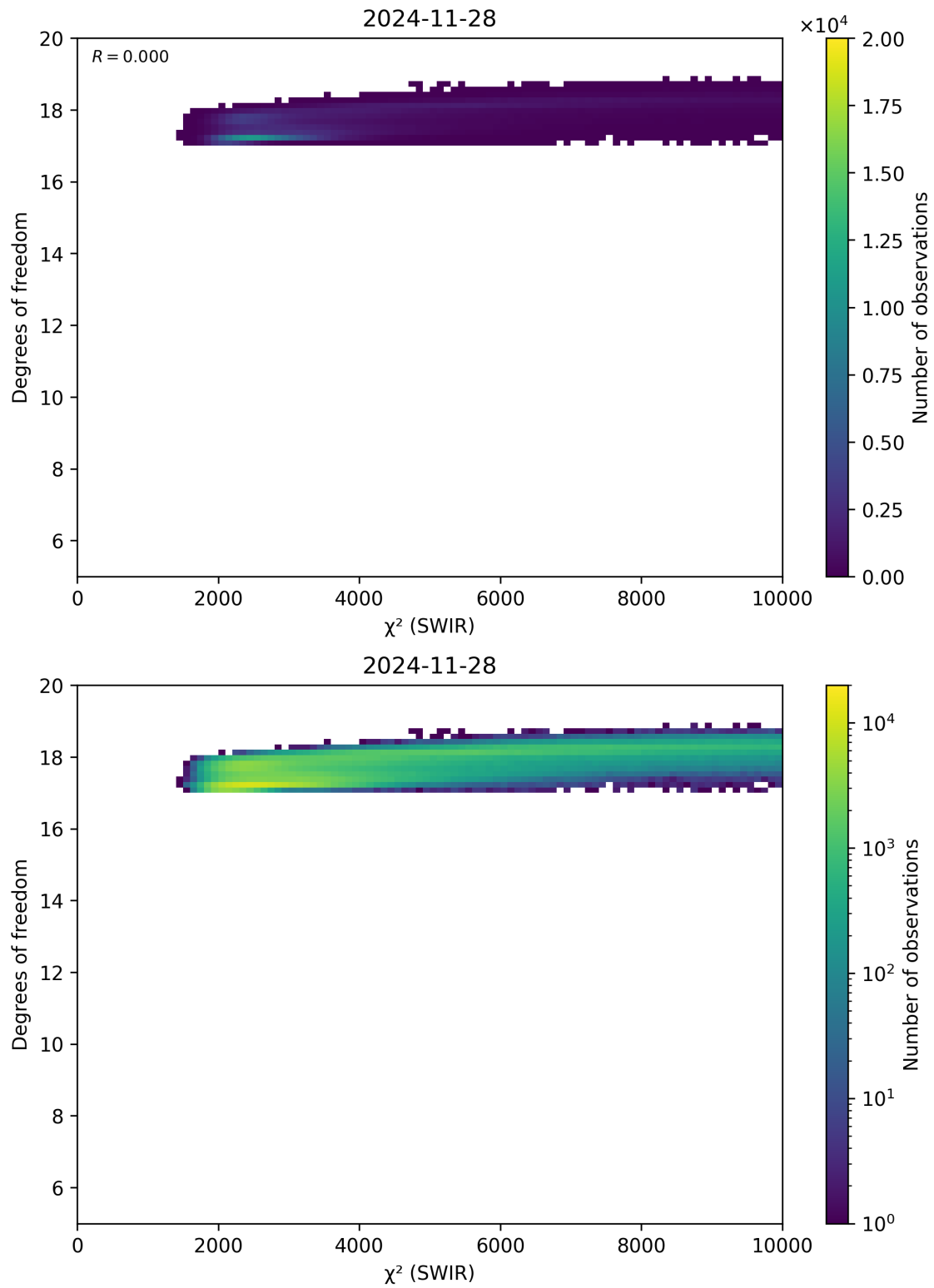
Figure 48: Scatter density plot of “ \chi^2 (SWIR)” against “Degrees of freedom” for 2024-11-27 to 2024-11-29.
