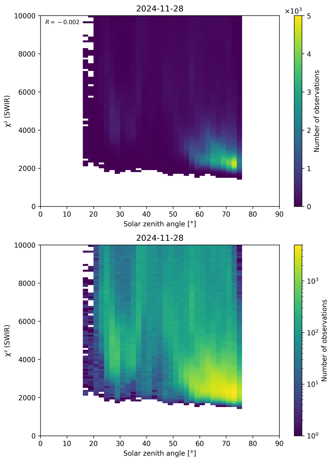
Figure 95: Scatter density plot of “Solar zenith angle” against “ \chi^2 (SWIR)” for 2024-11-27 to 2024-11-29.
