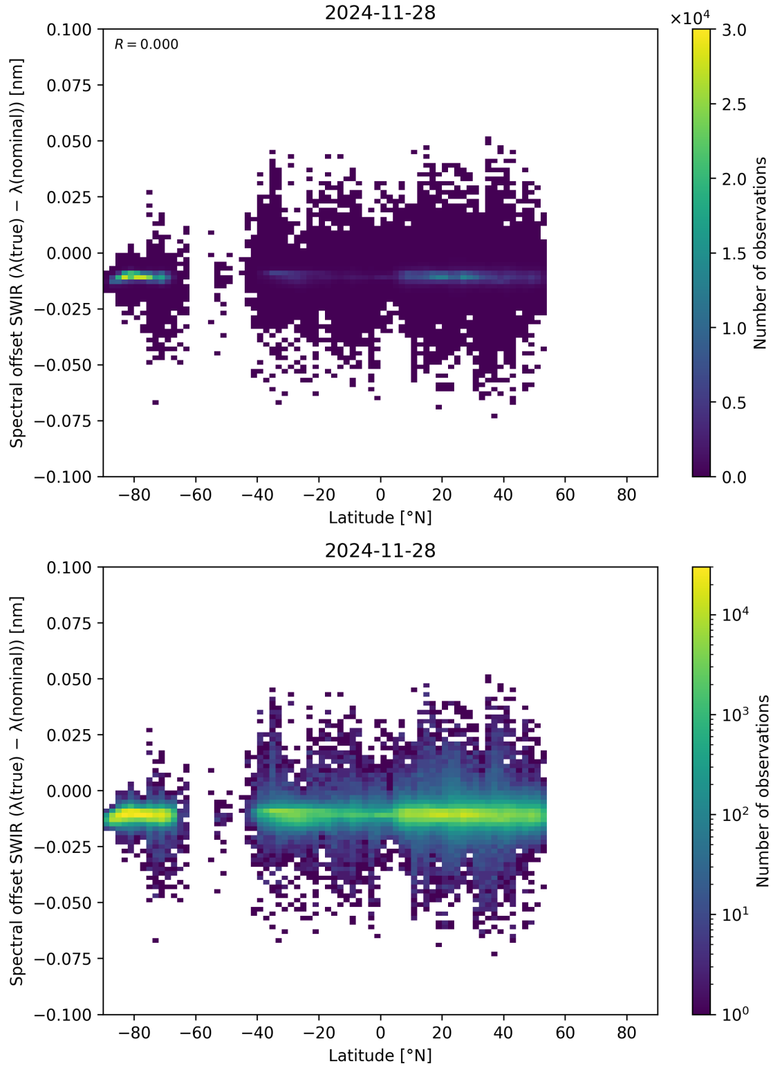
Figure 62: Scatter density plot of “Latitude” against “Spectral offset SWIR ( \lambda_{\text{true}} - \lambda_{\text{nominal}} )” for 2024-11-27 to 2024-11-29.
