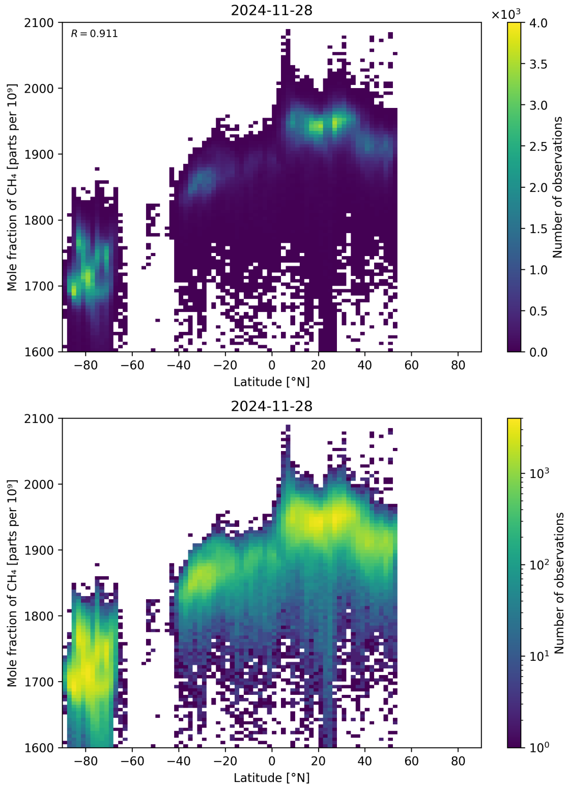
Figure 57: Scatter density plot of “Latitude” against “Mole fraction of CH 4 ” for 2024-11-27 to 2024-11-29.
