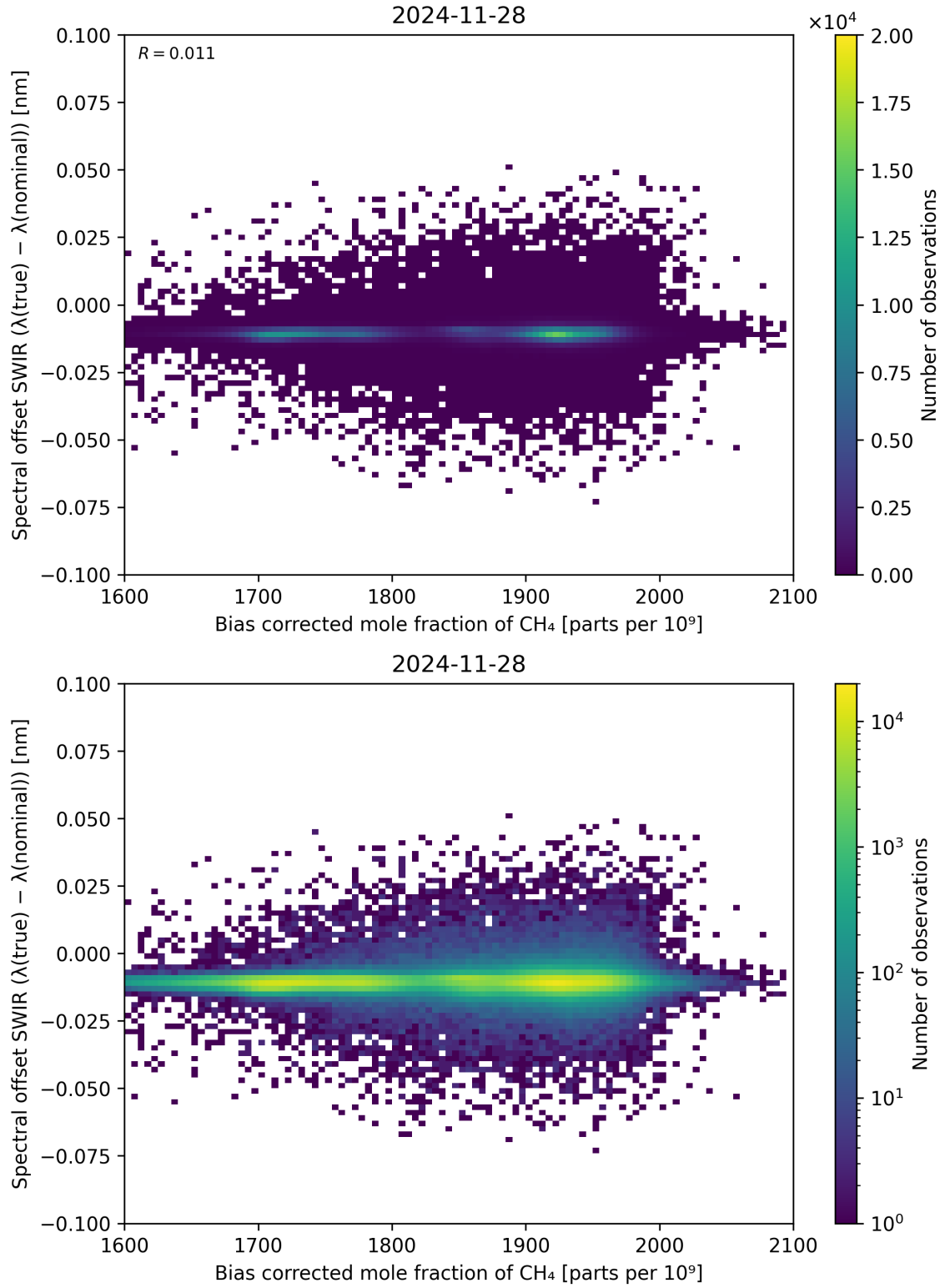
Figure 69: Scatter density plot of “Bias corrected mole fraction of \text{CH}_4 ” against “Spectral offset SWIR ( \lambda_{\text{true}} - \lambda_{\text{nominal}} )” for 2024-11-27 to 2024-11-29.
