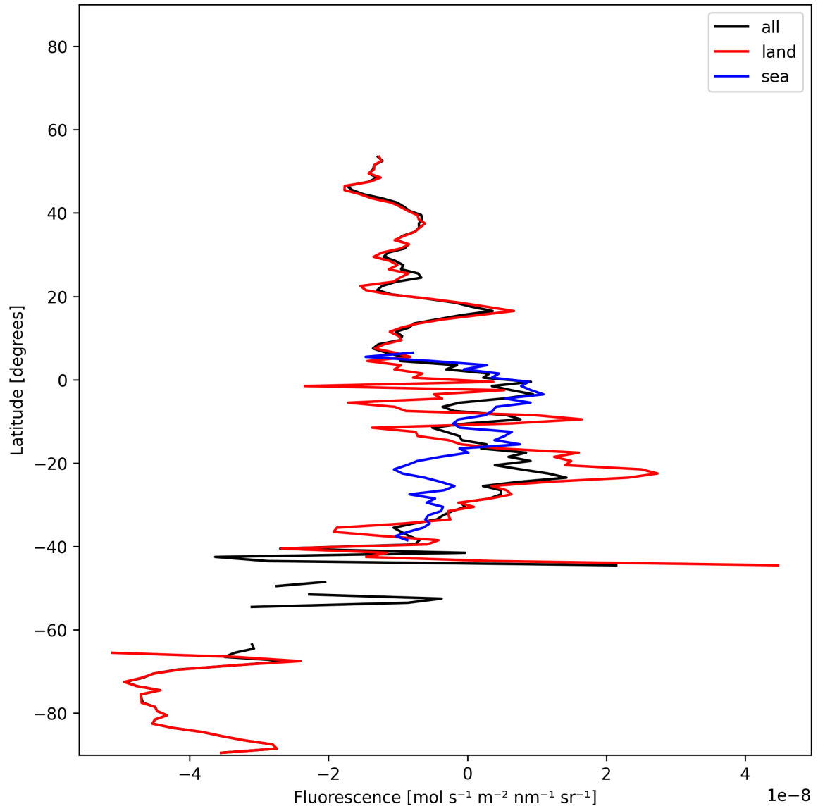
Figure 21: Zonal average of “Fluorescence” for 2024-11-27 to 2024-11-29.
