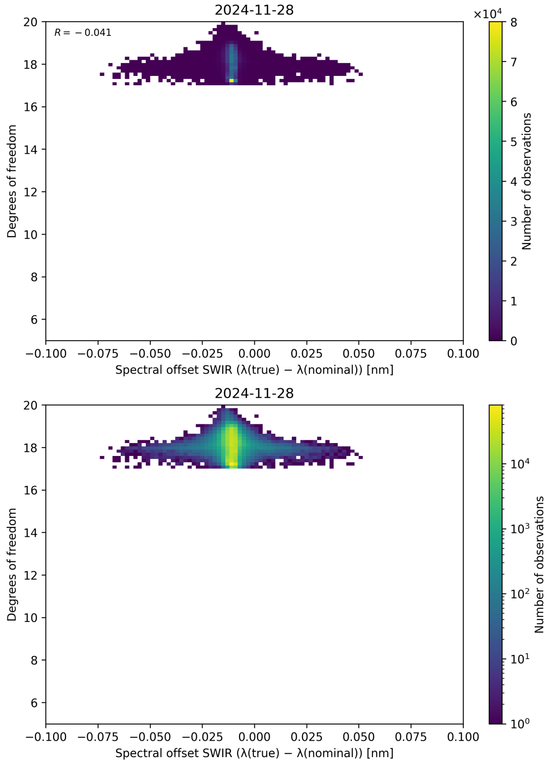
Figure 119: Scatter density plot of “Spectral offset SWIR ( \lambda_{\text{true}} - \lambda_{\text{nominal}} )” against “Degrees of freedom” for 2024-11-27 to 2024-11-29.
