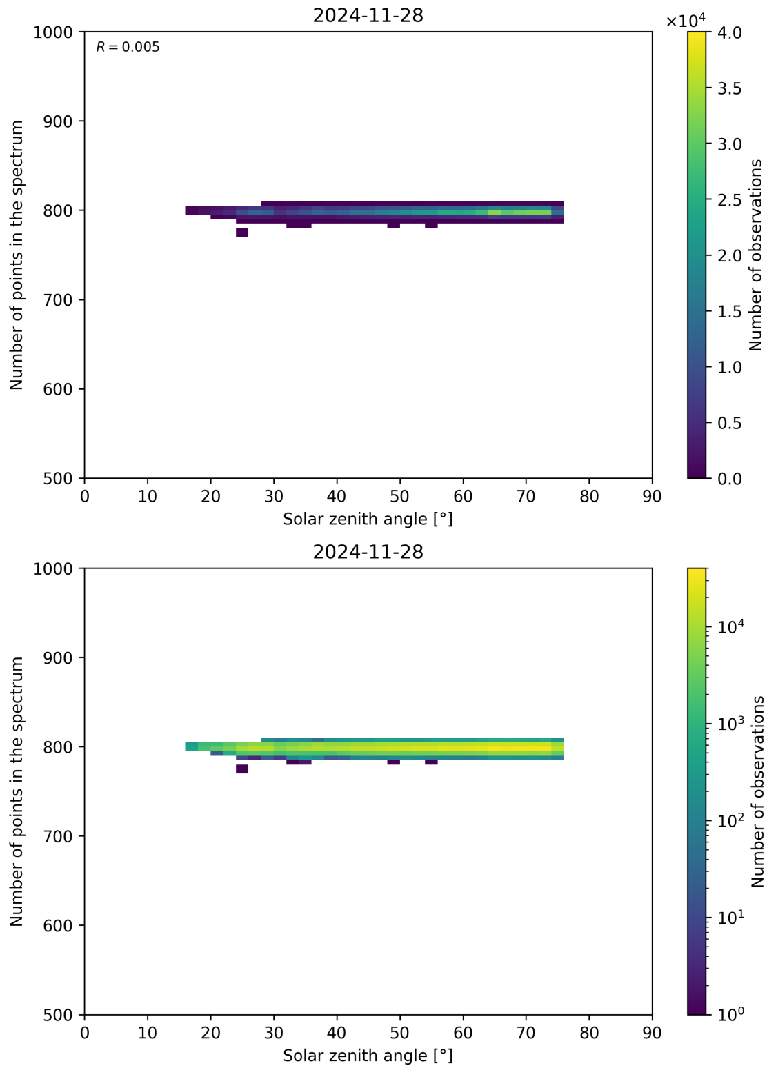
Figure 103: Scatter density plot of “Solar zenith angle” against “Number of points in the spectrum” for 2024-11-27 to 2024-11-29.
