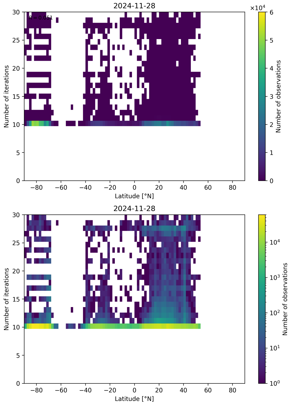
Figure 60: Scatter density plot of “Latitude” against “Number of iterations” for 2024-11-27 to 2024-11-29.
