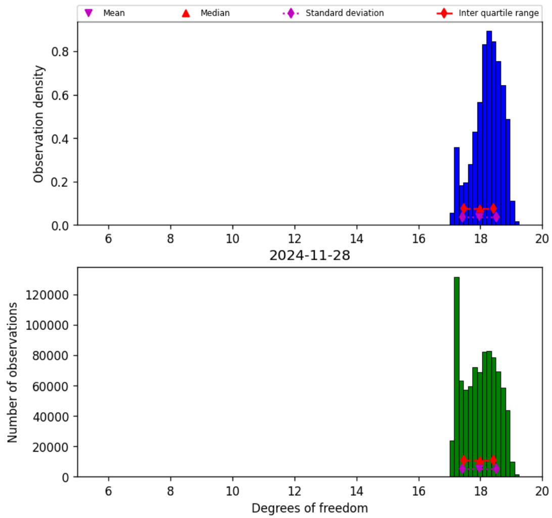
Figure 30: Histogram of “Degrees of freedom” for 2024-11-27 to 2024-11-29
