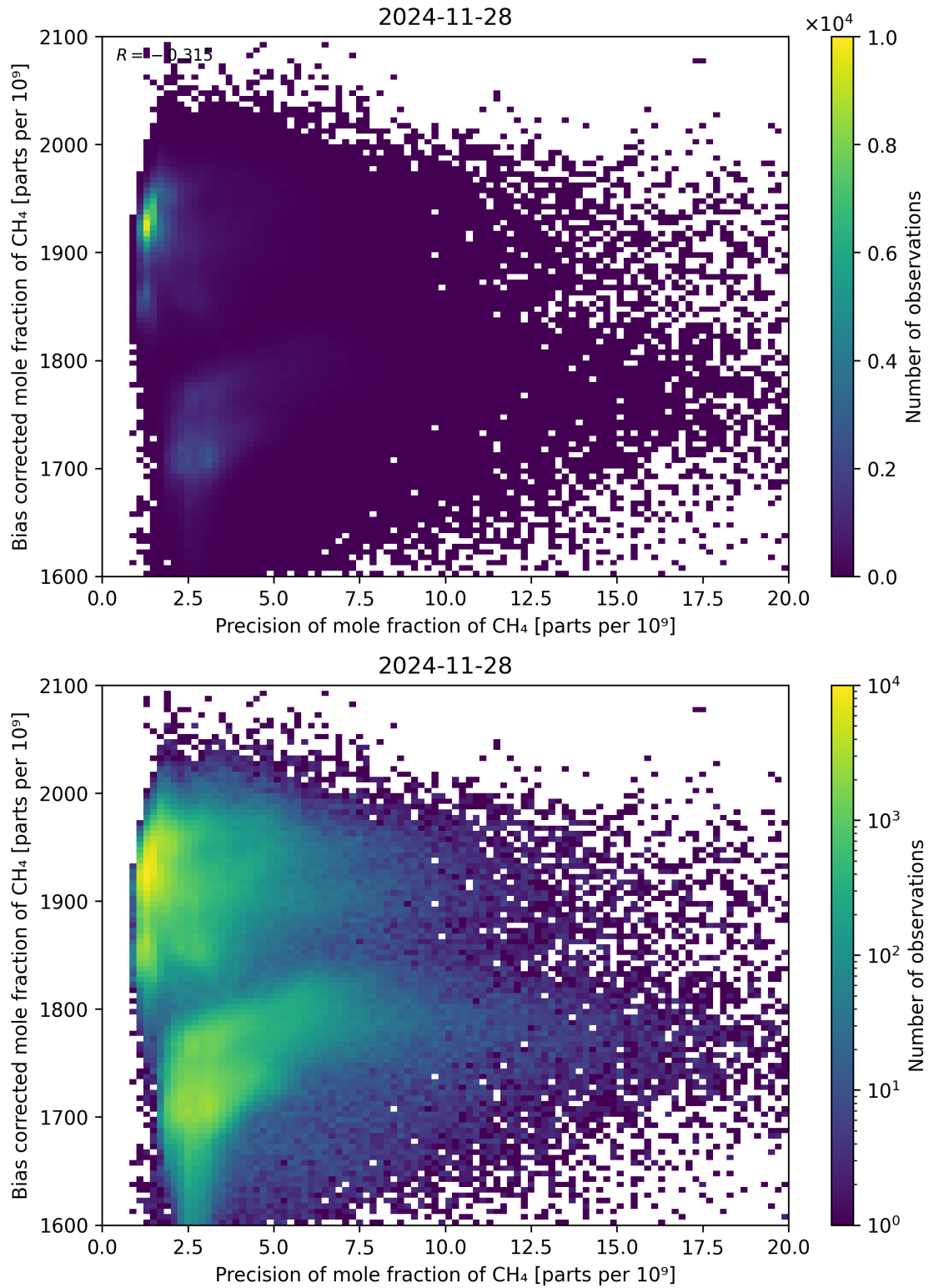
Figure 82: Scatter density plot of “Precision of mole fraction of CH 4 ” against “Bias corrected mole fraction of CH 4 ” for 2024-11-27 to 2024-11-29.
