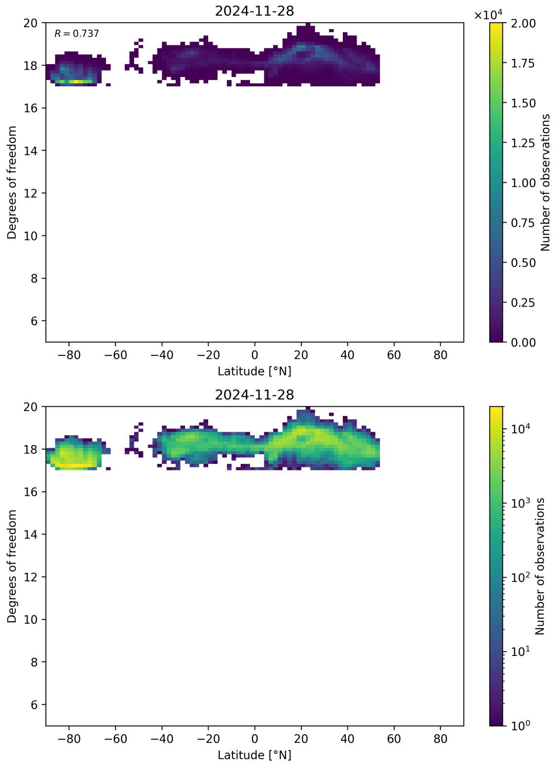
Figure 55: Scatter density plot of “Latitude” against “Degrees of freedom” for 2024-11-27 to 2024-11-29.
