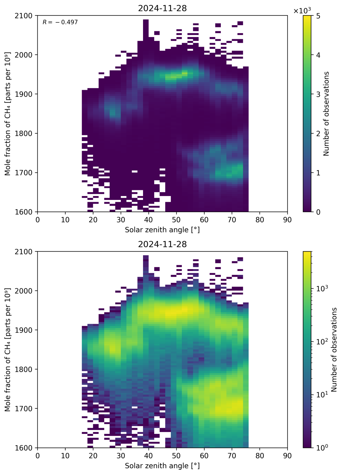
Figure 99: Scatter density plot of “Solar zenith angle” against “Mole fraction of CH 4 ” for 2024-11-27 to 2024-11-29.
