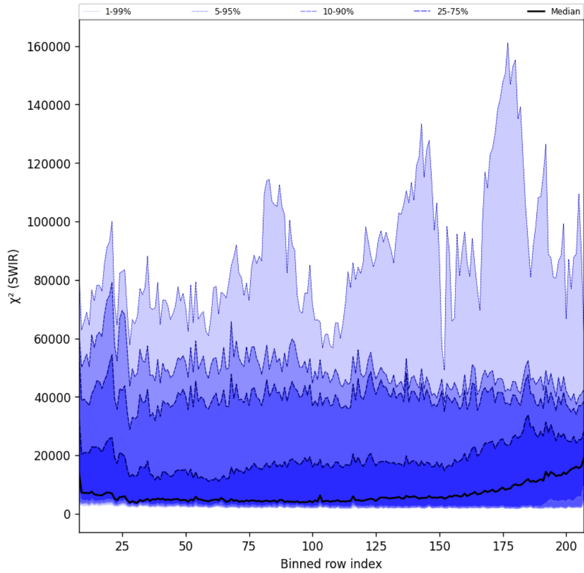
Figure 39: Along track statistics of “ \chi^2 (SWIR)” for 2024-11-27 to 2024-11-29
