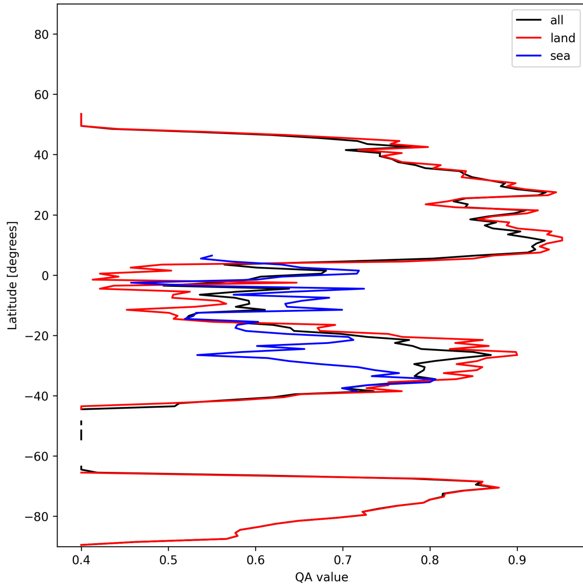
Figure 11: Zonal average of “QA value” for 2024-11-27 to 2024-11-29.
