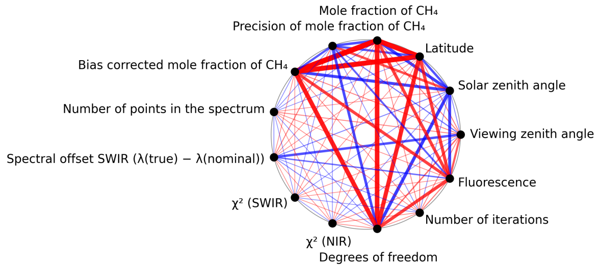
Figure 1: Map of correlation graph for 2024-11-27 to 2024-11-29.
