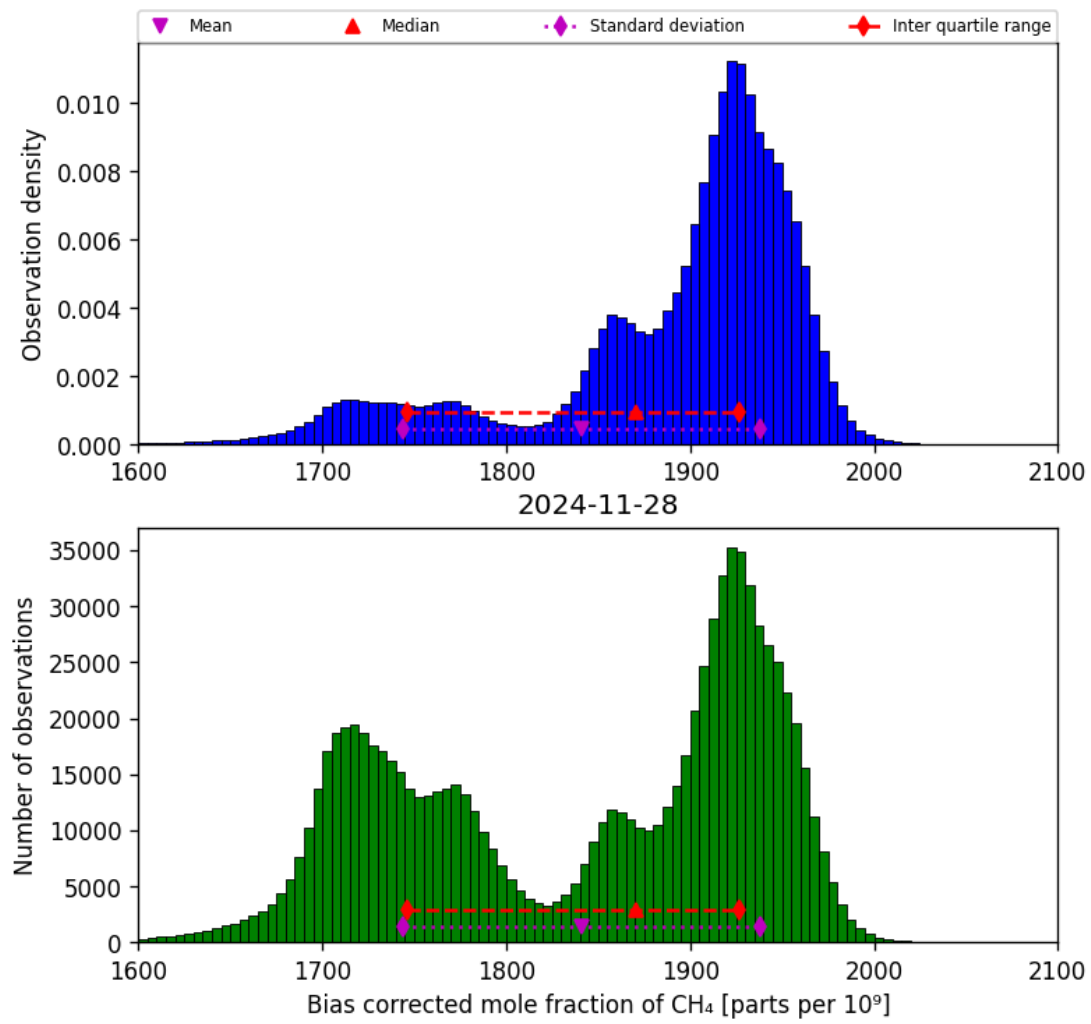
Figure 25: Histogram of “Bias corrected mole fraction of CH 4 ” for 2024-11-27 to 2024-11-29
