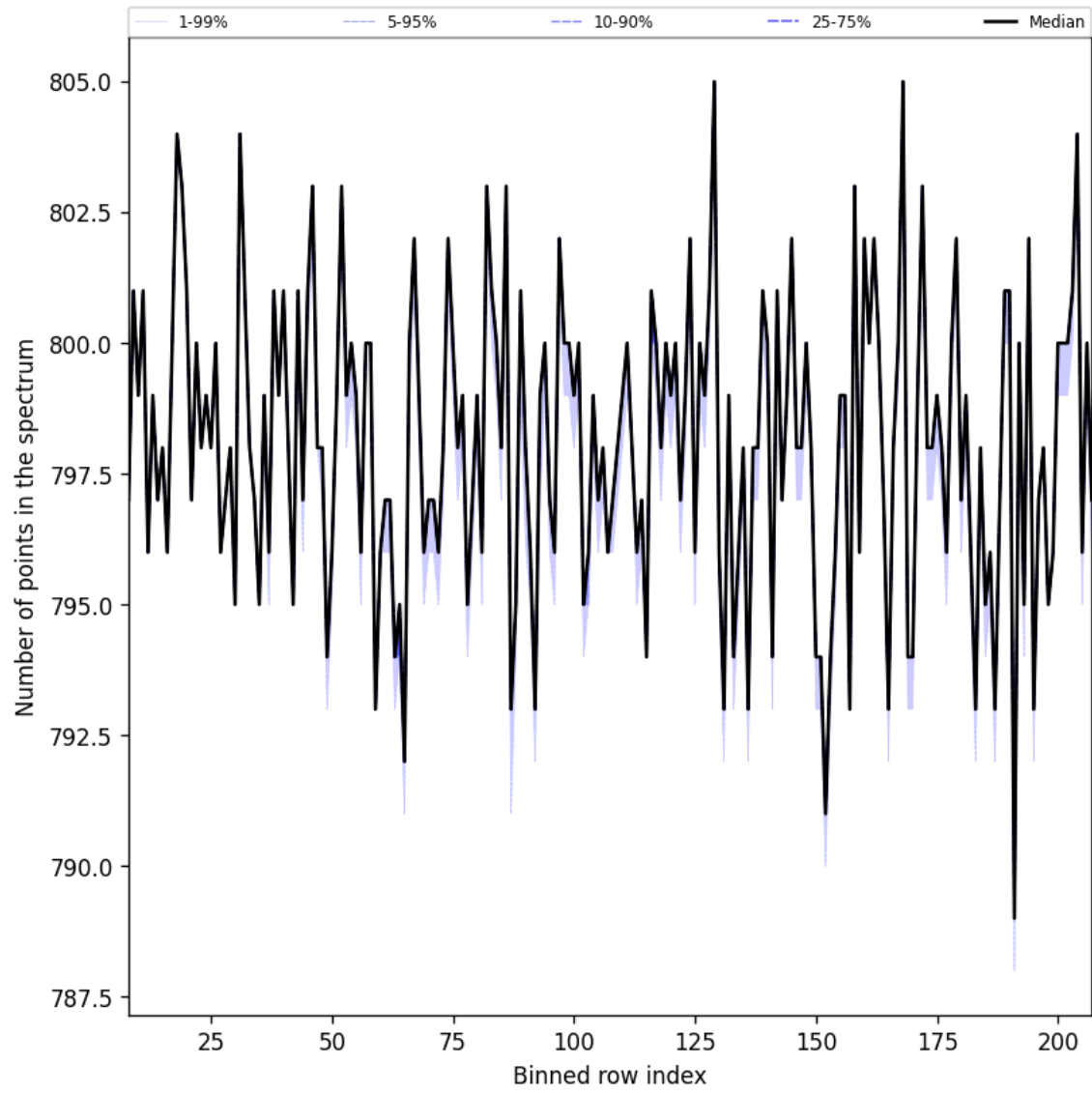
Figure 37: Along track statistics of “Number of points in the spectrum” for 2024-11-27 to 2024-11-29
