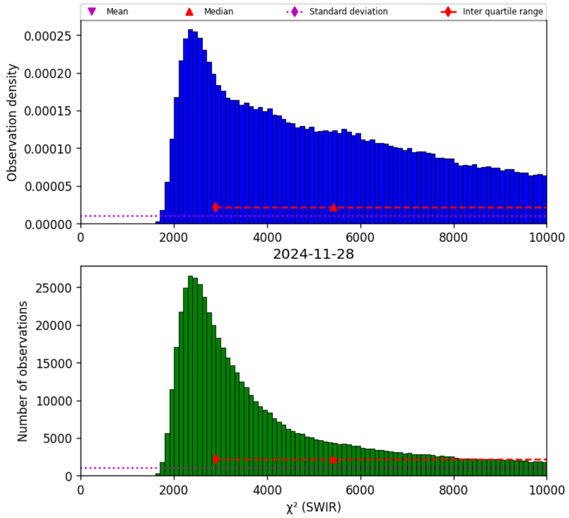
Figure 28: Histogram of “ \chi^2 (SWIR)” for 2024-11-27 to 2024-11-29
