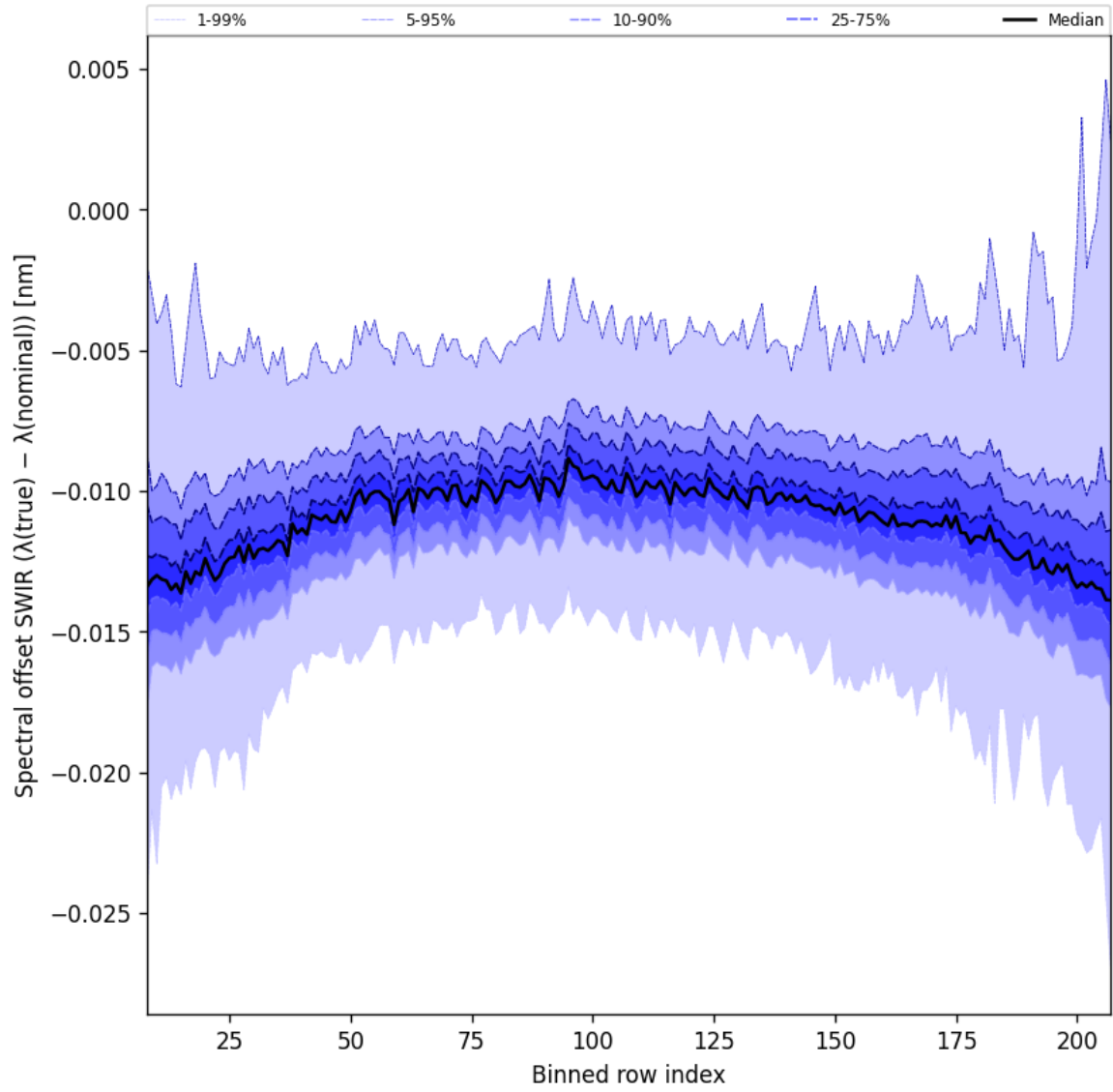
Figure 38: Along track statistics of “Spectral offset SWIR ( \lambda_{\text{true}} - \lambda_{\text{nominal}} )” for 2024-11-27 to 2024-11-29
