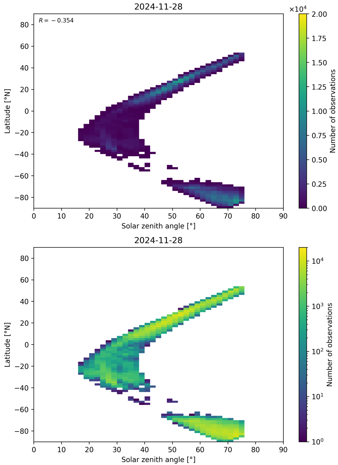
Figure 98: Scatter density plot of “Solar zenith angle” against “Latitude” for 2024-11-27 to 2024-11-29.
