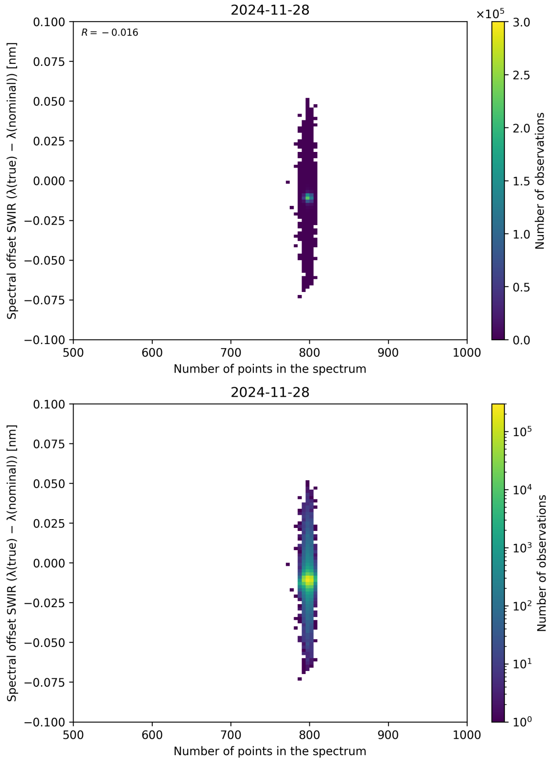
Figure 93: Scatter density plot of “Number of points in the spectrum” against “Spectral offset SWIR ( \lambda_{\text{true}} - \lambda_{\text{nominal}} )” for 2024-11-27 to 2024-11-29.
