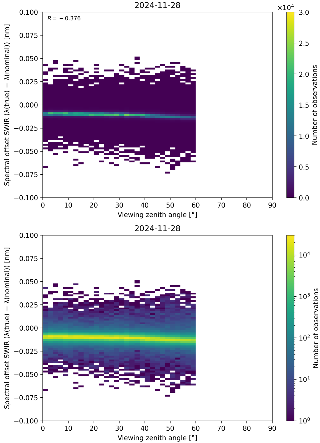
Figure 116: Scatter density plot of “Viewing zenith angle” against “Spectral offset SWIR ( \lambda_{\text{true}} - \lambda_{\text{nominal}} )” for 2024-11-27 to 2024-11-29.
