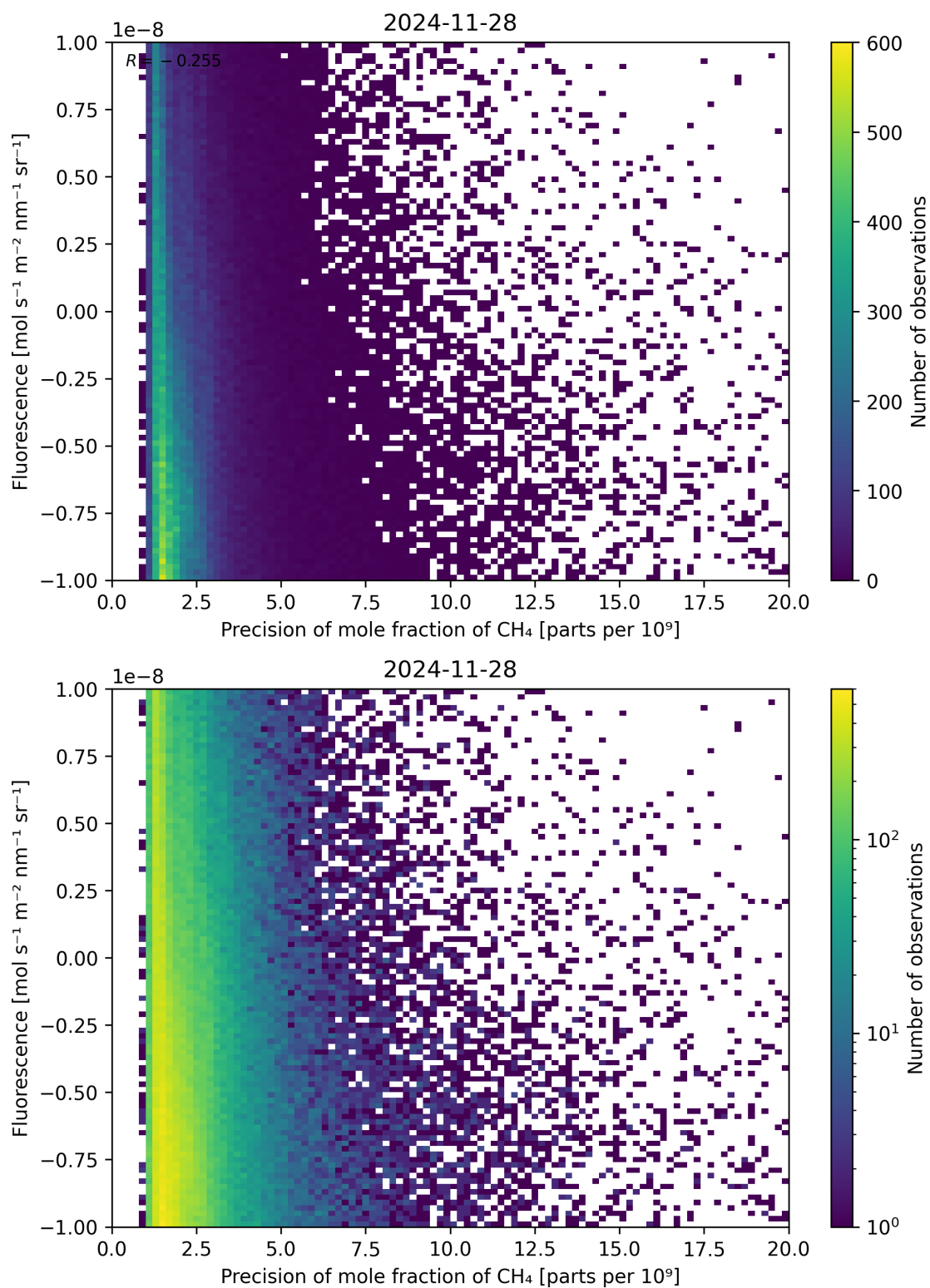
Figure 81: Scatter density plot of “Precision of mole fraction of CH 4 ” against “Fluorescence” for 2024-11-27 to 2024-11-29.
