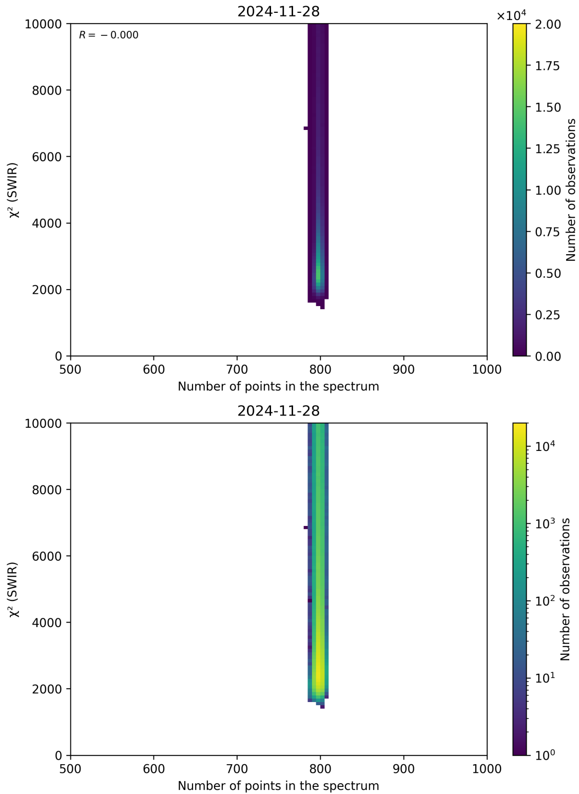
Figure 89: Scatter density plot of “Number of points in the spectrum” against “ \chi^2 (SWIR)” for 2024-11-27 to 2024-11-29.
