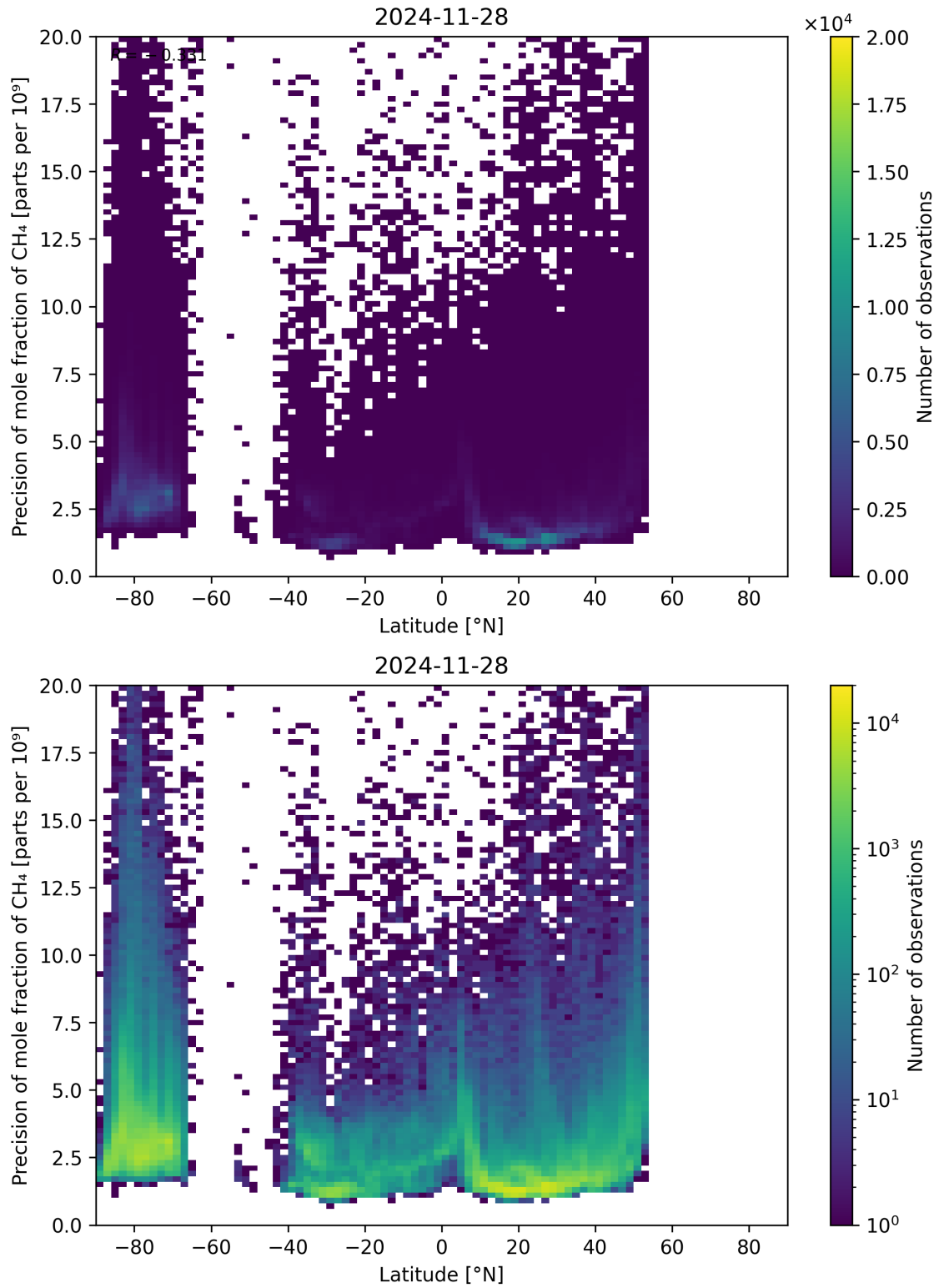
Figure 59: Scatter density plot of “Latitude” against “Precision of mole fraction of CH 4 ” for 2024-11-27 to 2024-11-29.
