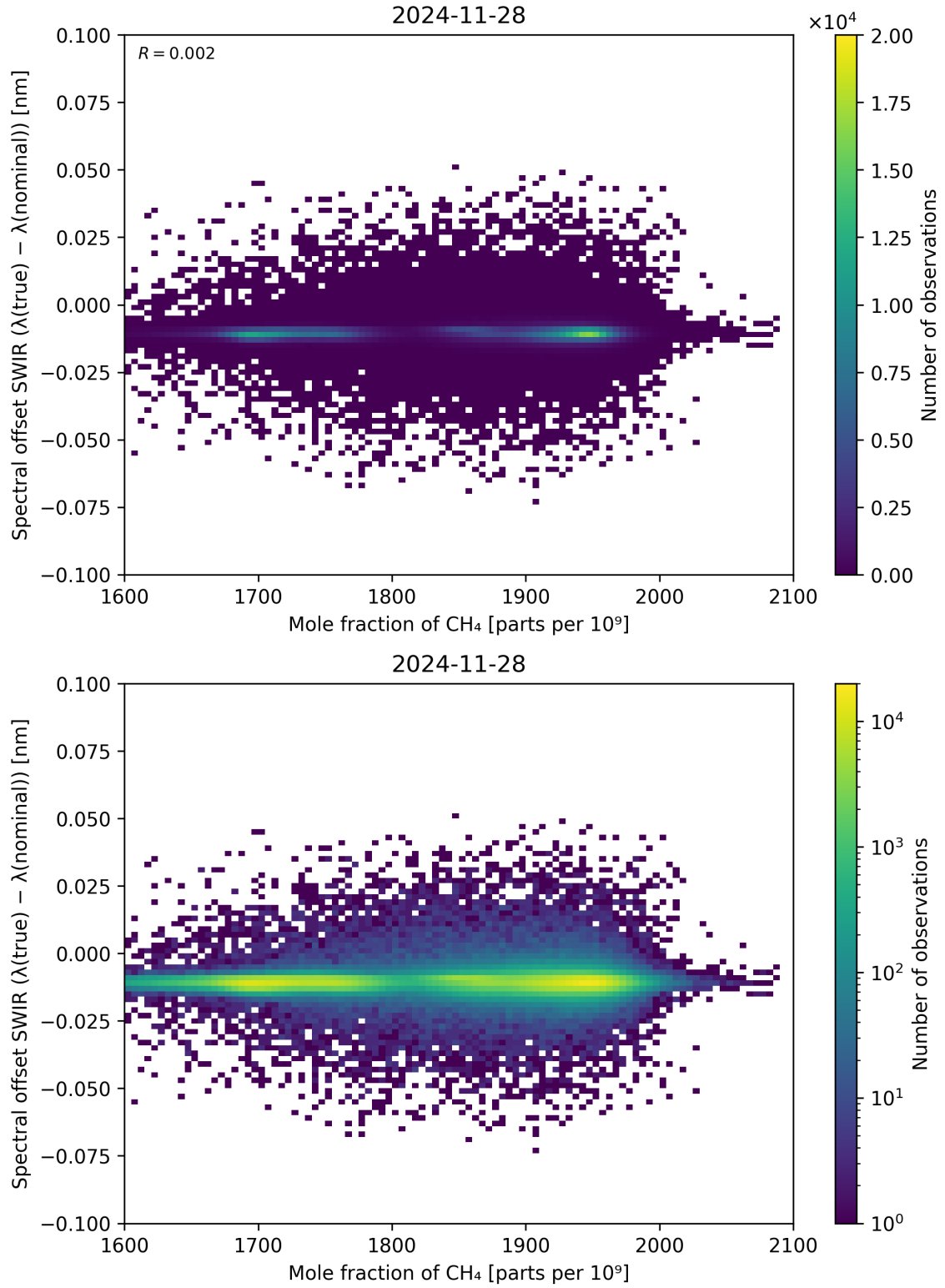
Figure 86: Scatter density plot of “Mole fraction of \text{CH}_4 ” against “Spectral offset SWIR ( \lambda_{\text{true}} - \lambda_{\text{nominal}} )” for 2024-11-27 to 2024-11-29.
