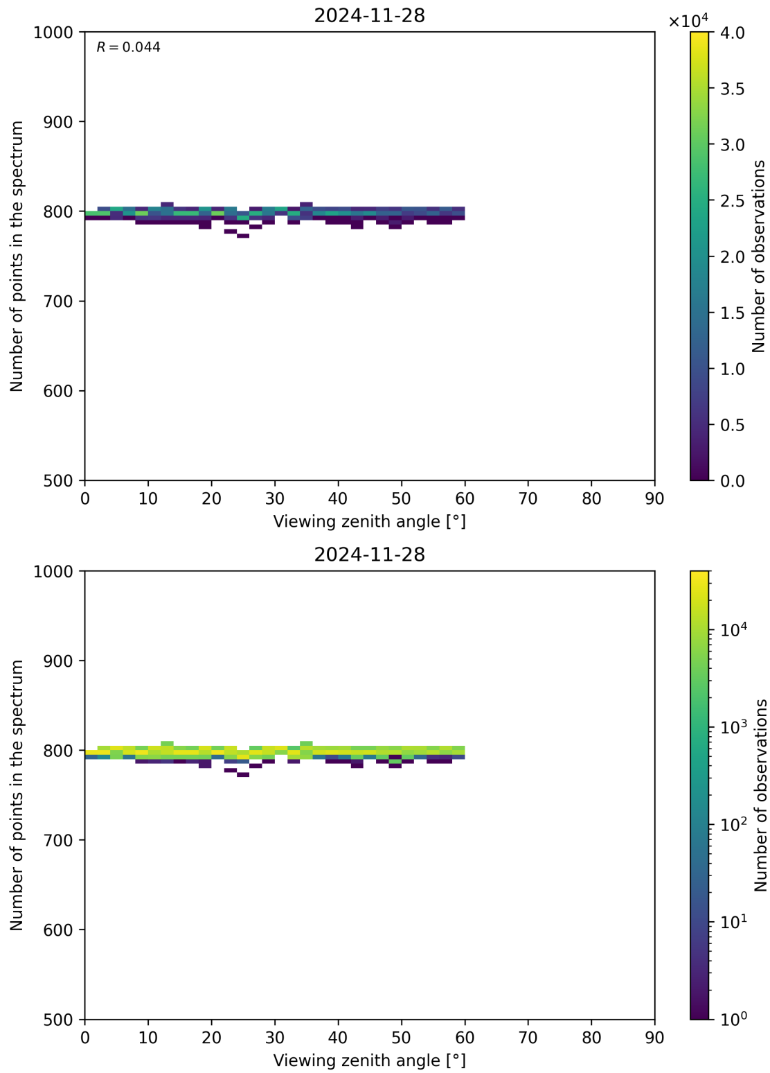
Figure 114: Scatter density plot of “Viewing zenith angle” against “Number of points in the spectrum” for 2024-11-27 to 2024-11-29.
