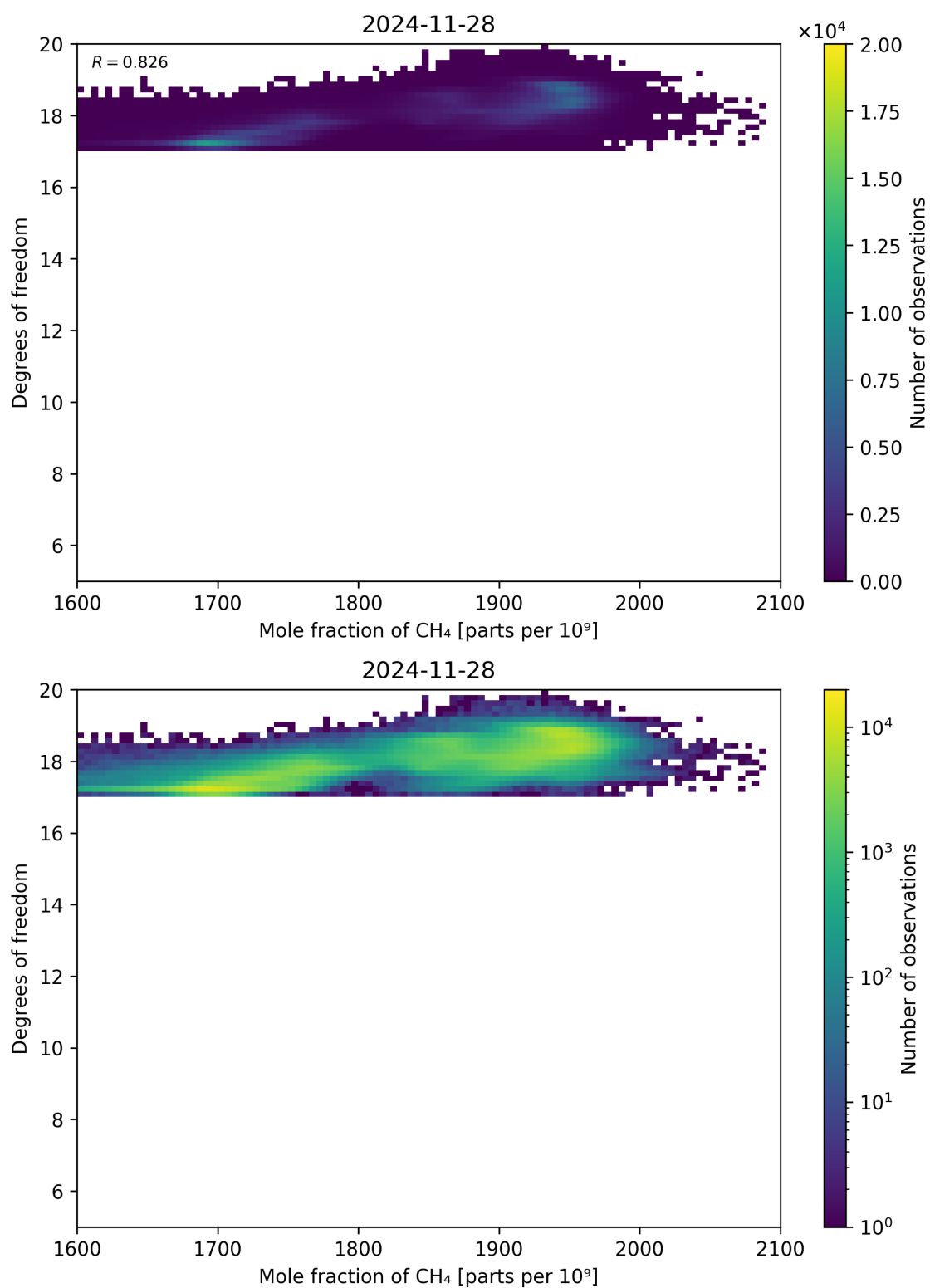
Figure 72: Scatter density plot of “Mole fraction of CH 4 ” against “Degrees of freedom” for 2024-11-27 to 2024-11-29.
