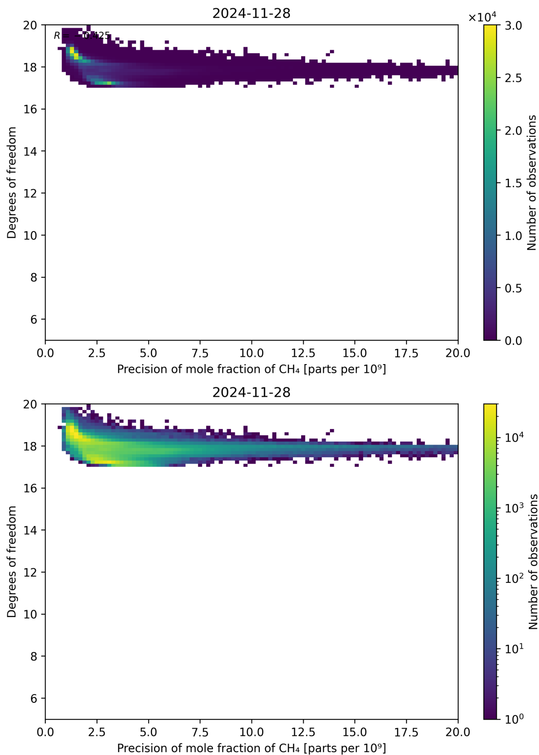
Figure 80: Scatter density plot of “Precision of mole fraction of CH 4 ” against “Degrees of freedom” for 2024-11-27 to 2024-11-29.
