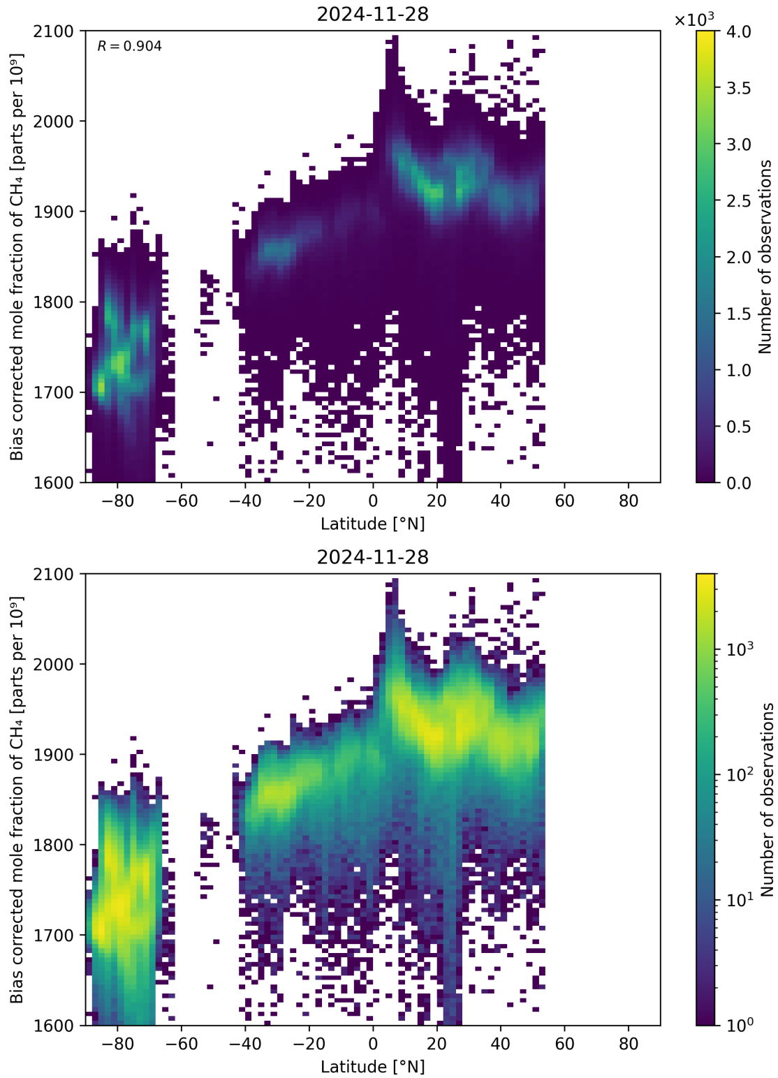
Figure 58: Scatter density plot of “Latitude” against “Bias corrected mole fraction of CH 4 ” for 2024-11-27 to 2024-11-29.
