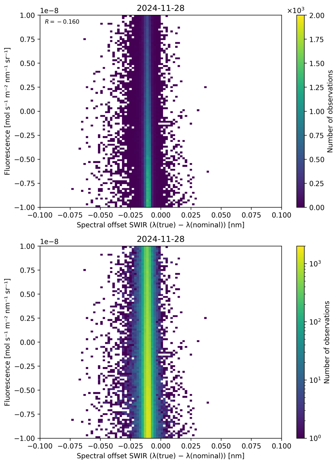
Figure 120: Scatter density plot of “Spectral offset SWIR ( \lambda_{\text{true}} - \lambda_{\text{nominal}} )” against “Fluorescence” for 2024-11-27 to 2024-11-29.
