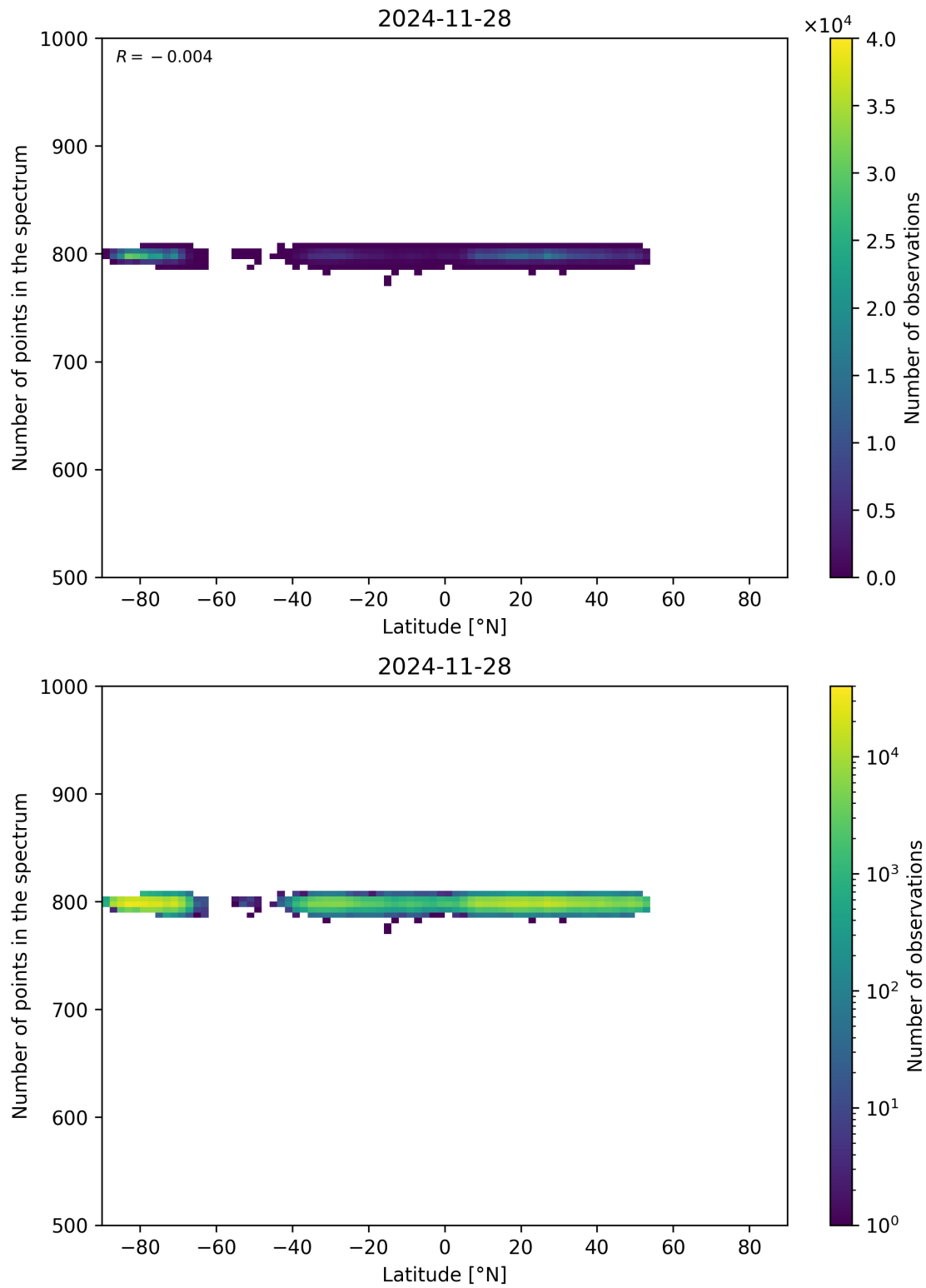
Figure 61: Scatter density plot of “Latitude” against “Number of points in the spectrum” for 2024-11-27 to 2024-11-29.
