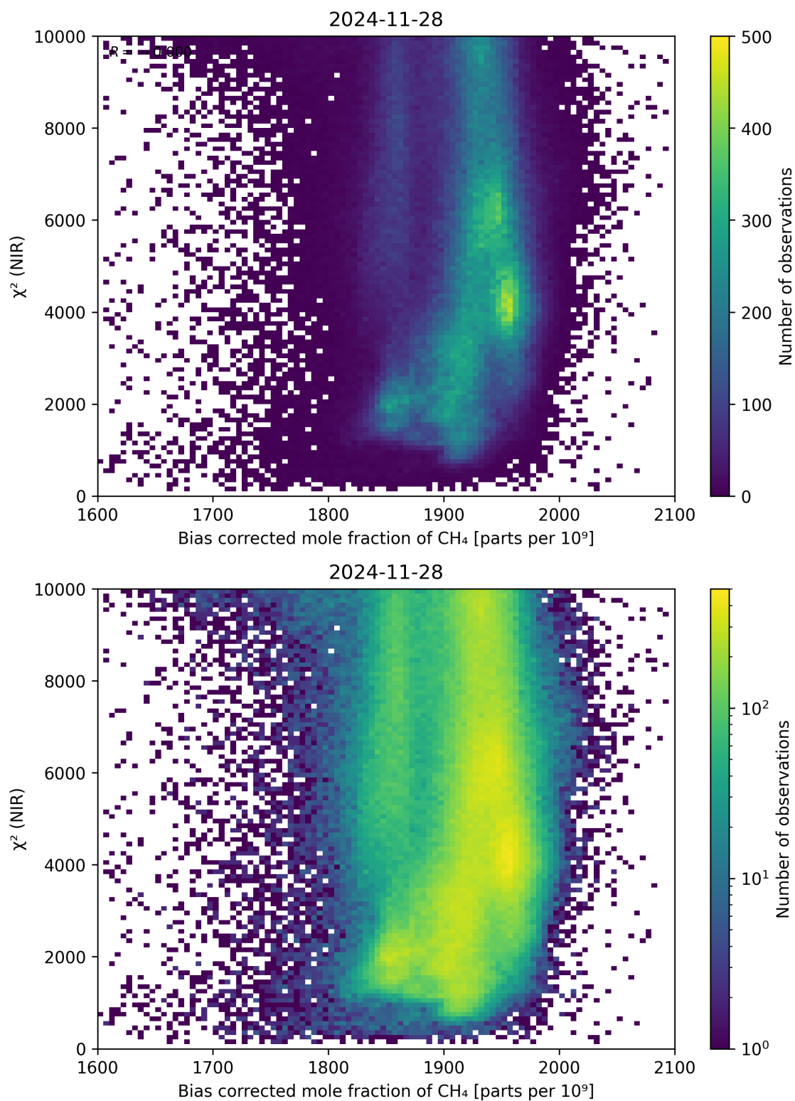
Figure 63: Scatter density plot of “Bias corrected mole fraction of CH 4 ” against “ \chi^2 (NIR)” for 2024-11-27 to 2024-11-29.
