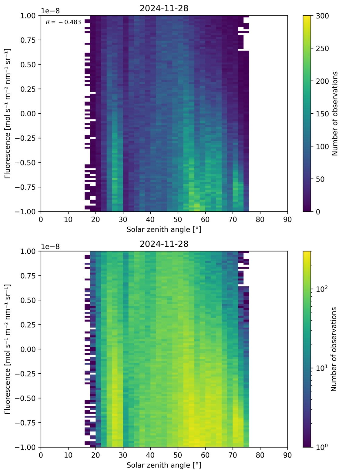
Figure 97: Scatter density plot of “Solar zenith angle” against “Fluorescence” for 2024-11-27 to 2024-11-29.
