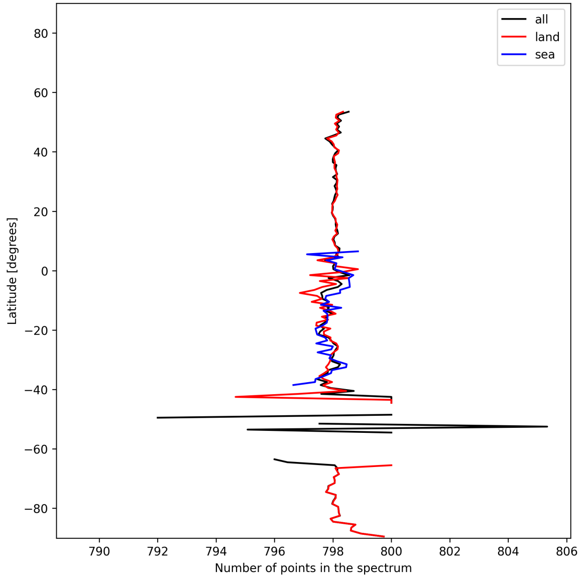
Figure 15: Zonal average of “Number of points in the spectrum” for 2024-11-27 to 2024-11-29.
