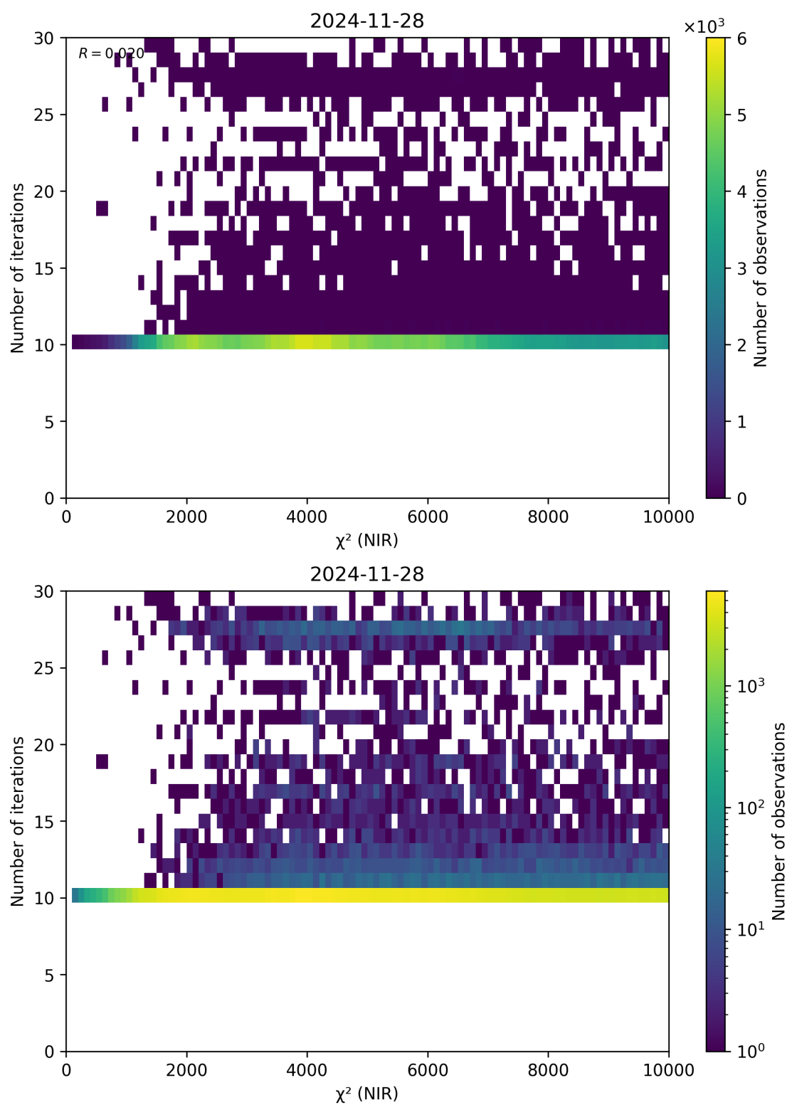
Figure 46: Scatter density plot of “ \chi^2 (NIR)” against “Number of iterations” for 2024-11-27 to 2024-11-29.
