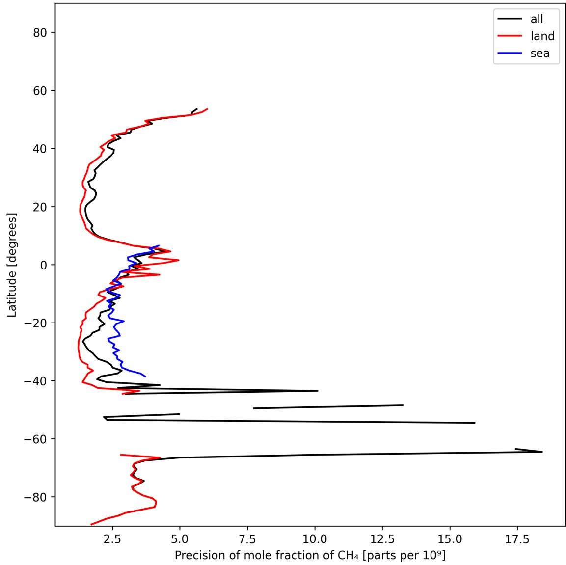
Figure 13: Zonal average of “Precision of mole fraction of CH 4 ” for 2024-11-27 to 2024-11-29.
