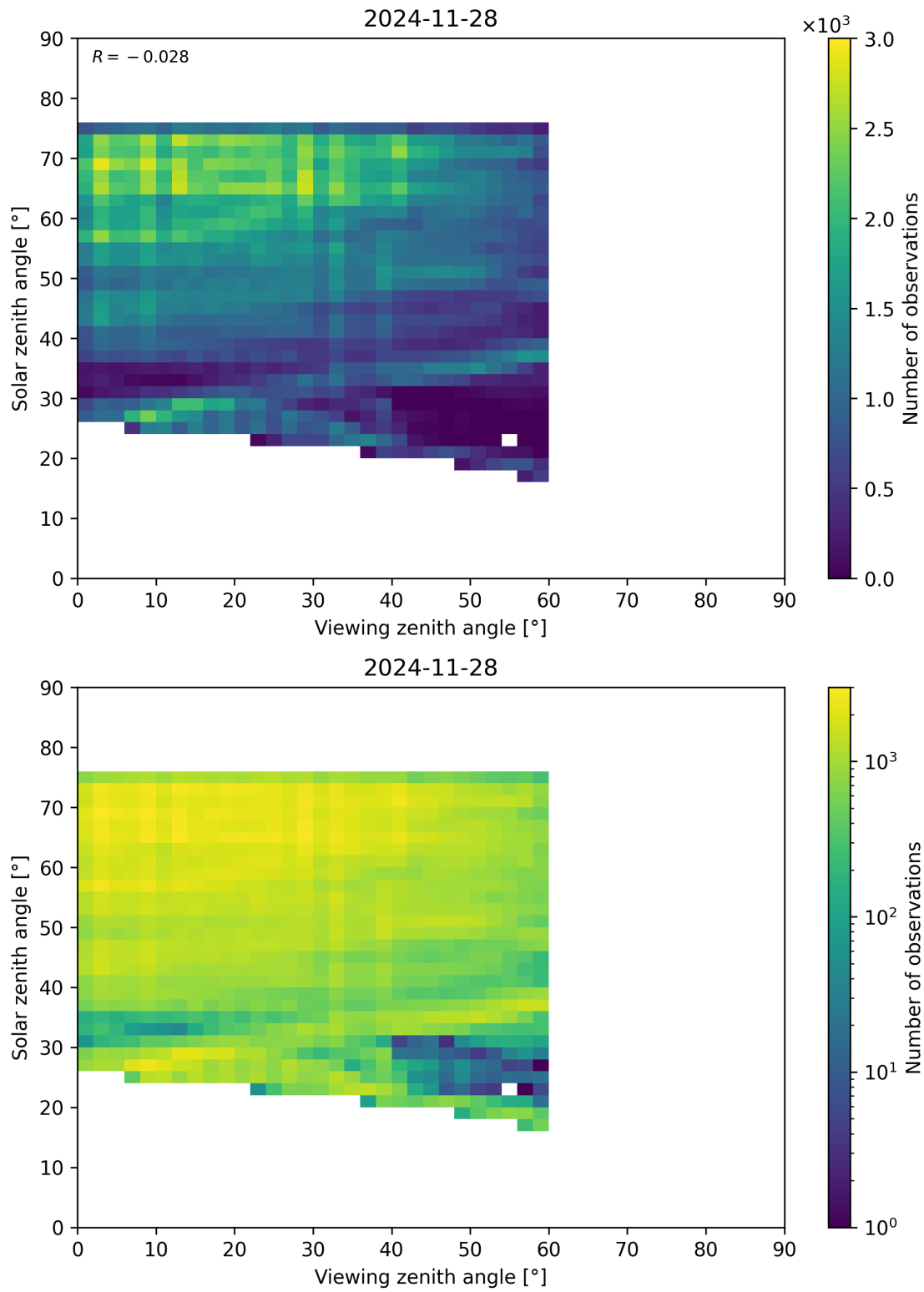
Figure 115: Scatter density plot of “Viewing zenith angle” against “Solar zenith angle” for 2024-11-27 to 2024-11-29.
