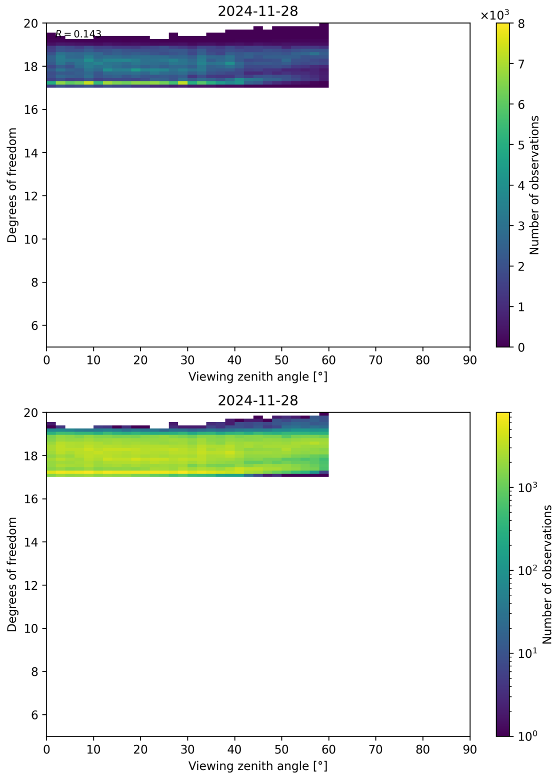
Figure 107: Scatter density plot of “Viewing zenith angle” against “Degrees of freedom” for 2024-11-27 to 2024-11-29.
