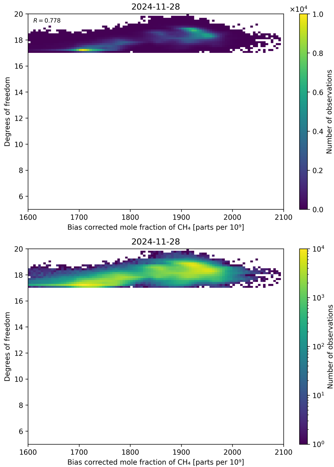
Figure 65: Scatter density plot of “Bias corrected mole fraction of \text{CH}_4 ” against “Degrees of freedom” for 2024-11-27 to 2024-11-29.
