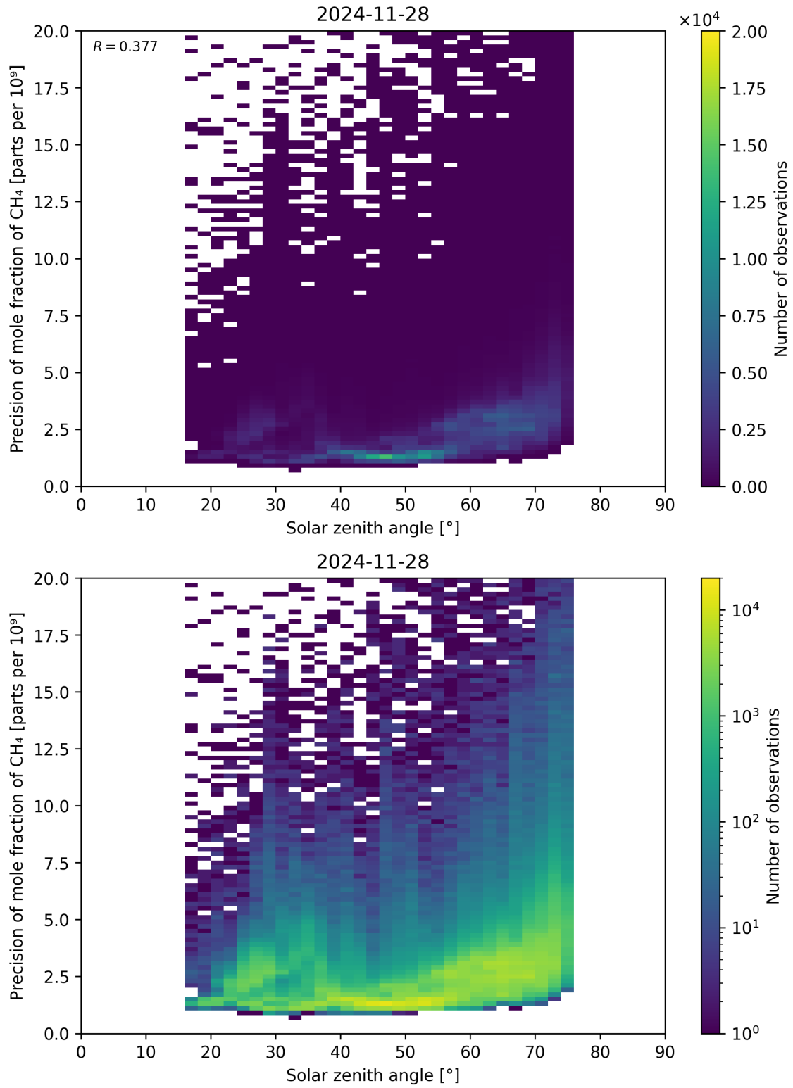
Figure 101: Scatter density plot of “Solar zenith angle” against “Precision of mole fraction of \text{CH}_4 ” for 2024-11-27 to 2024-11-29.
