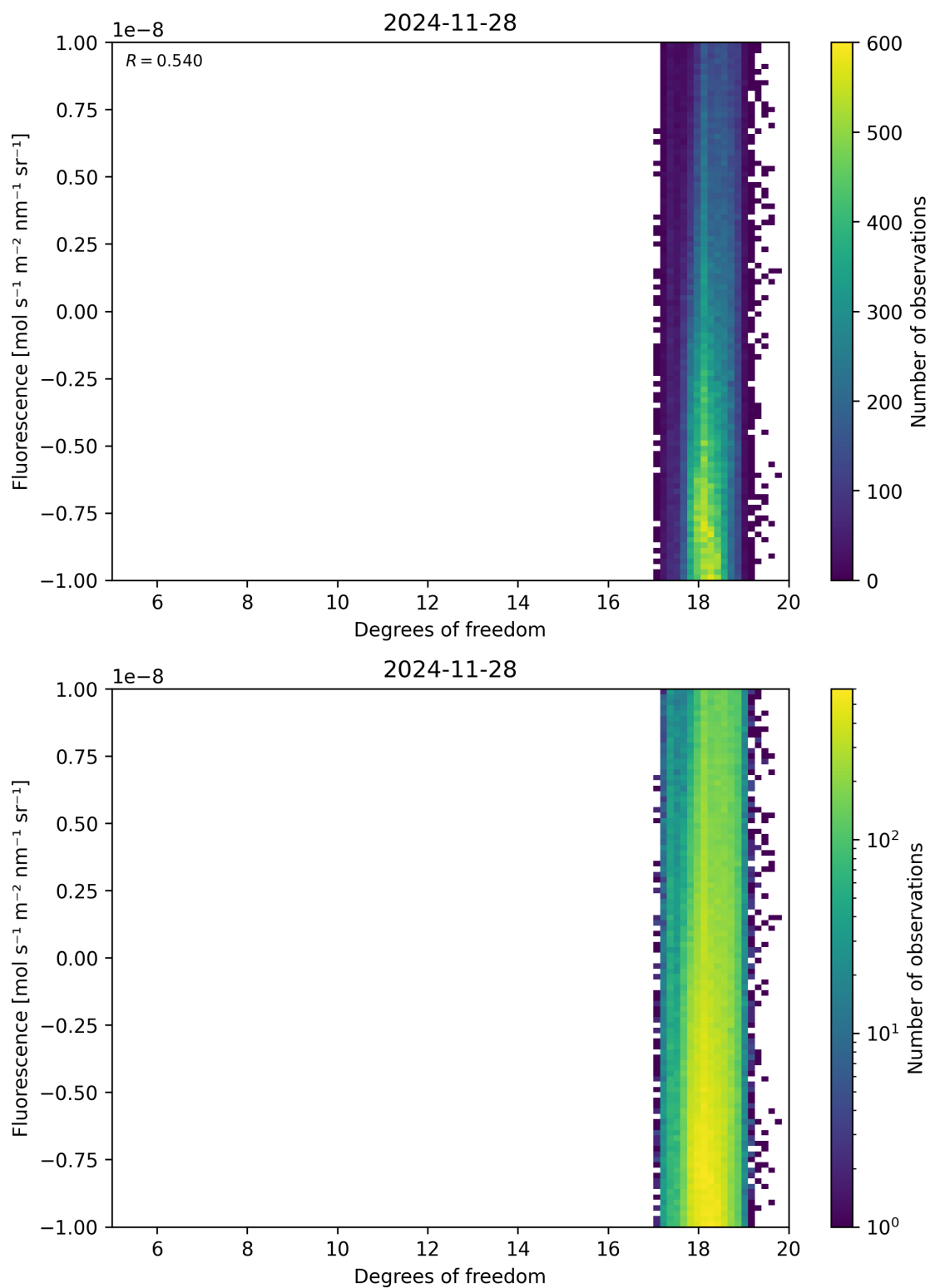
Figure 51: Scatter density plot of “Degrees of freedom” against “Fluorescence” for 2024-11-27 to 2024-11-29.
