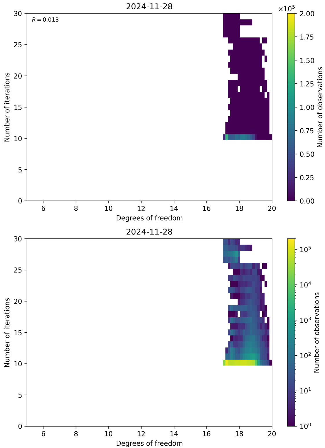
Figure 52: Scatter density plot of “Degrees of freedom” against “Number of iterations” for 2024-11-27 to 2024-11-29.
