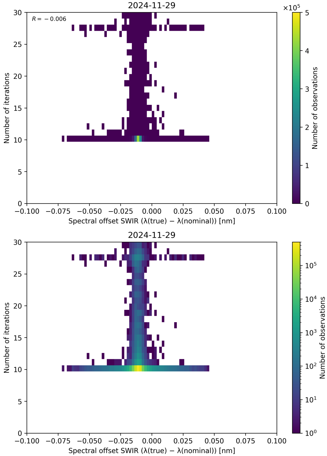
Figure 121: Scatter density plot of “Spectral offset SWIR ( \lambda_{\text{true}} - \lambda_{\text{nominal}} )” against “Number of iterations” for 2024-11-28 to 2024-11-30.
