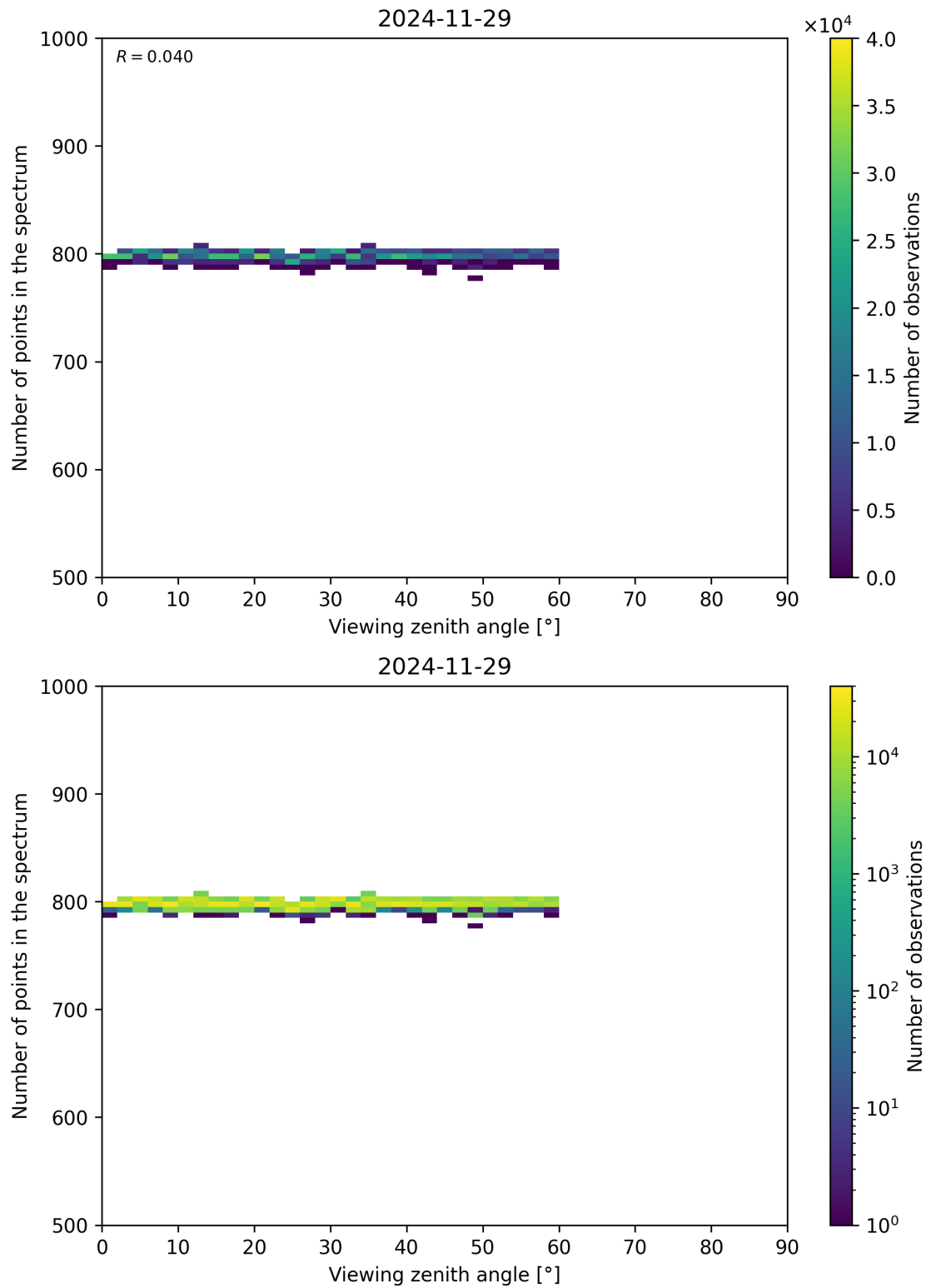
Figure 114: Scatter density plot of “Viewing zenith angle” against “Number of points in the spectrum” for 2024-11-28 to 2024-11-30.
