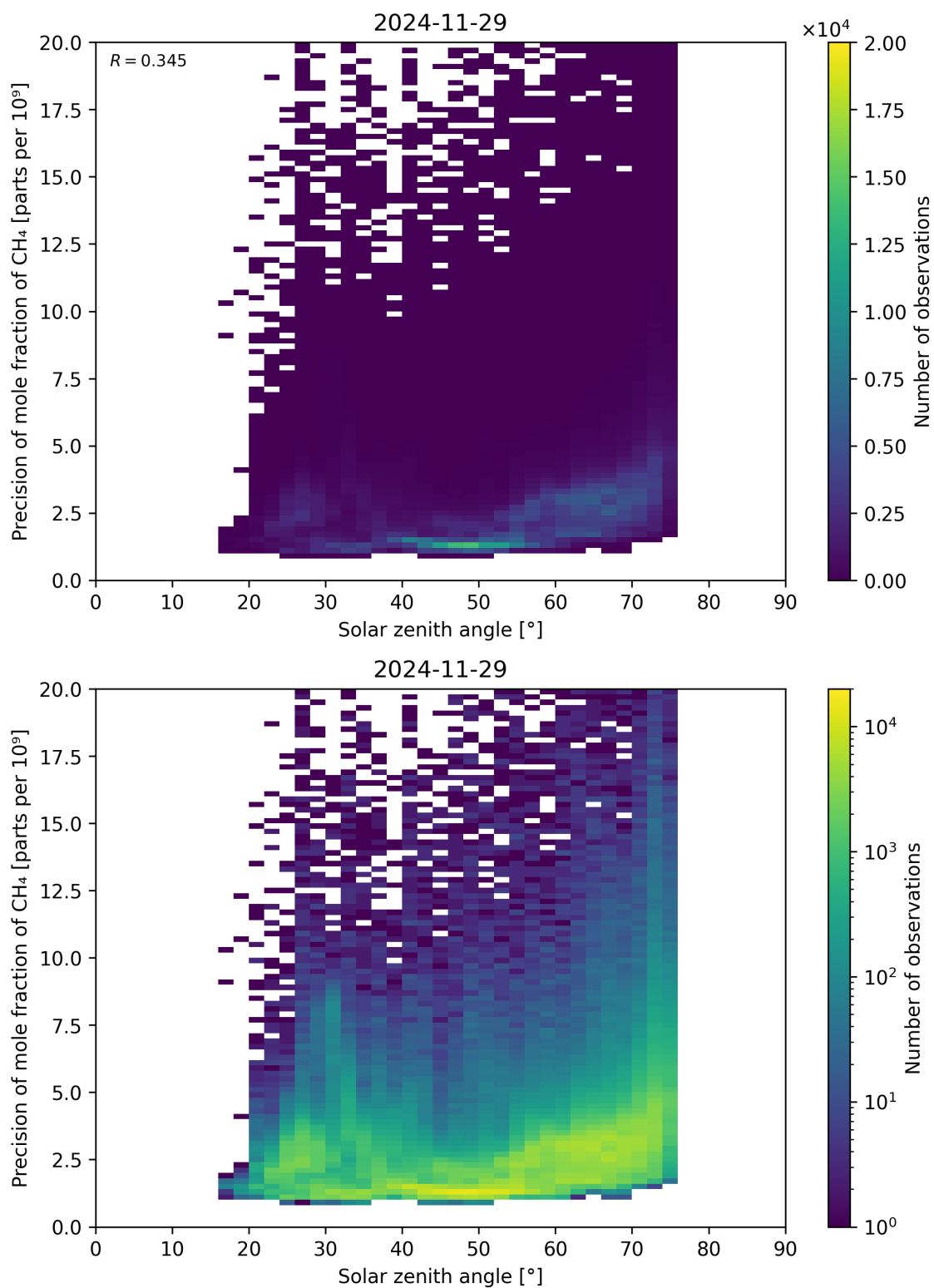
Figure 101: Scatter density plot of “Solar zenith angle” against “Precision of mole fraction of \text{CH}_4 ” for 2024-11-28 to 2024-11-30.
