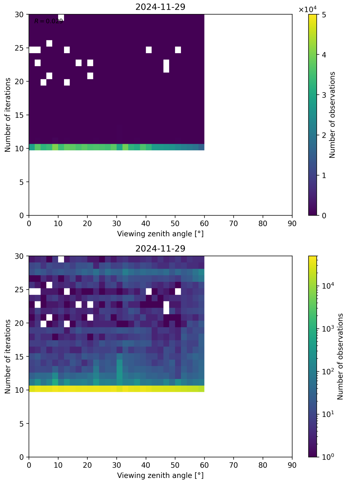
Figure 113: Scatter density plot of “Viewing zenith angle” against “Number of iterations” for 2024-11-28 to 2024-11-30.
