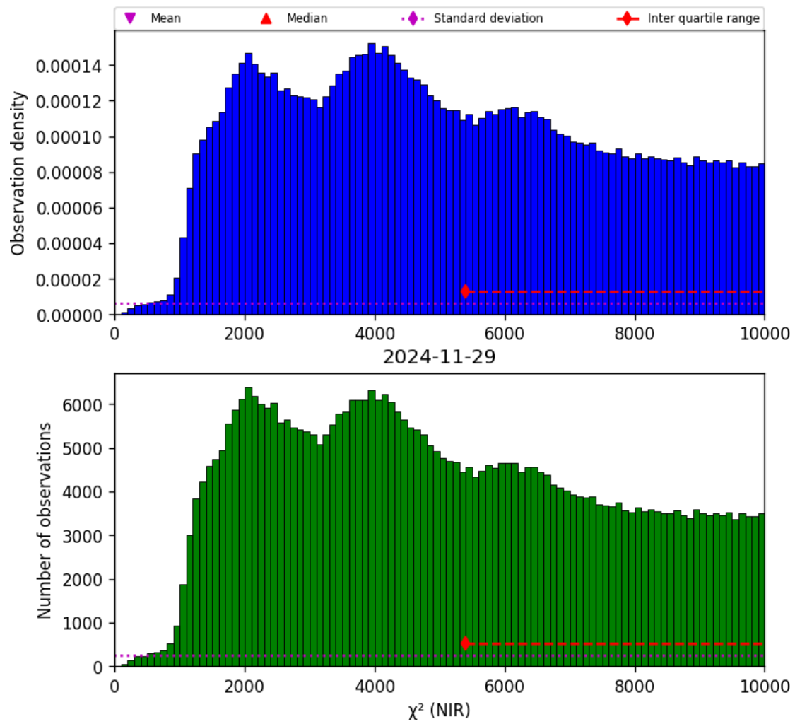
Figure 29: Histogram of “ \chi^2 (NIR)” for 2024-11-28 to 2024-11-30
