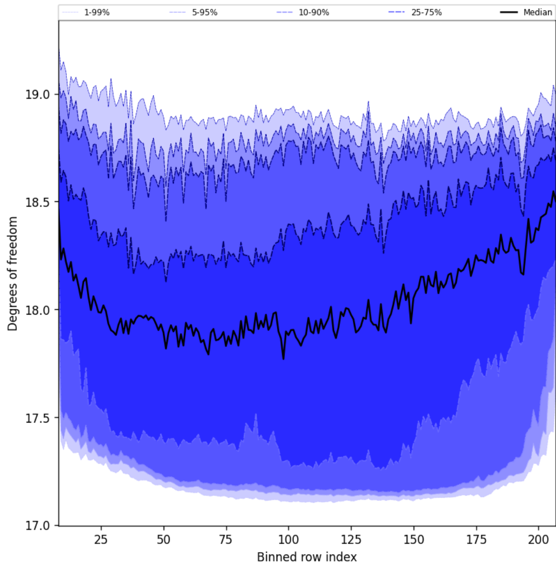
Figure 41: Along track statistics of “Degrees of freedom” for 2024-11-28 to 2024-11-30
