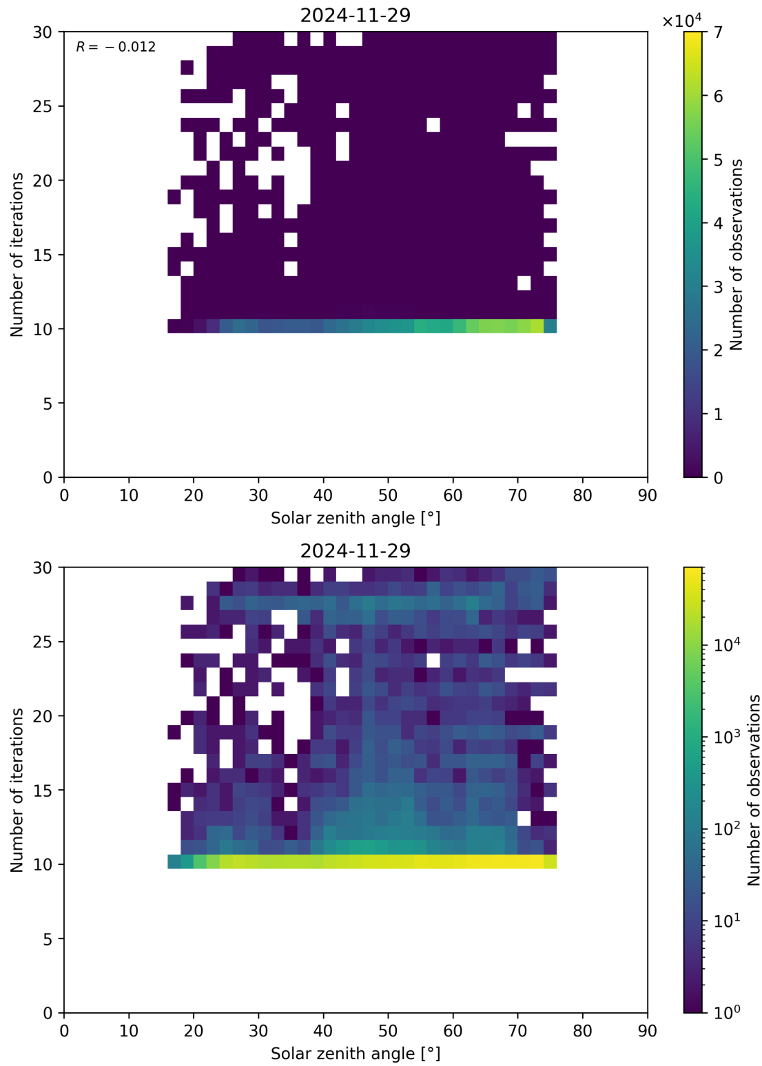
Figure 102: Scatter density plot of “Solar zenith angle” against “Number of iterations” for 2024-11-28 to 2024-11-30.
