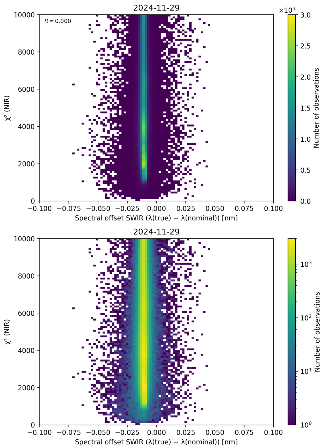
Figure 117: Scatter density plot of “Spectral offset SWIR ( \lambda_{\text{true}} - \lambda_{\text{nominal}} )” against “ \chi^2 (NIR)” for 2024-11-28 to 2024-11-30.
