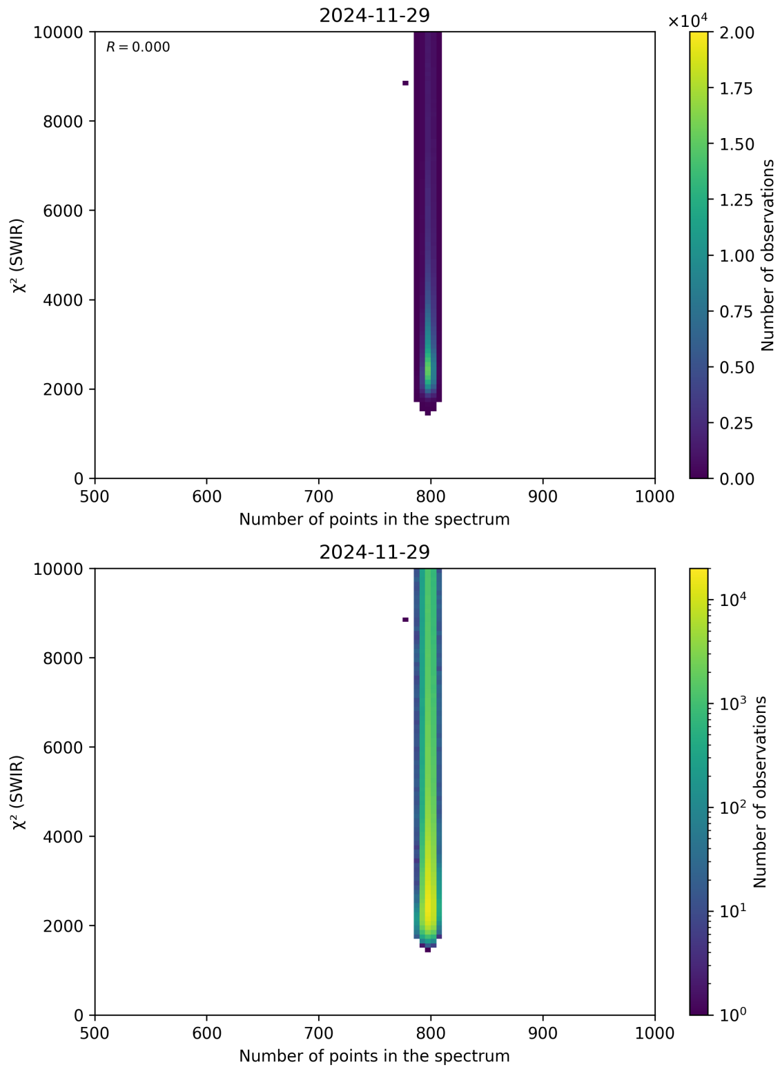
Figure 89: Scatter density plot of “Number of points in the spectrum” against “ \chi^2 (SWIR)” for 2024-11-28 to 2024-11-30.
