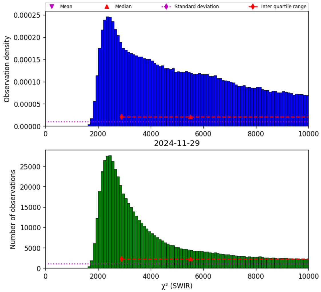
Figure 28: Histogram of “ \chi^2 (SWIR)” for 2024-11-28 to 2024-11-30
