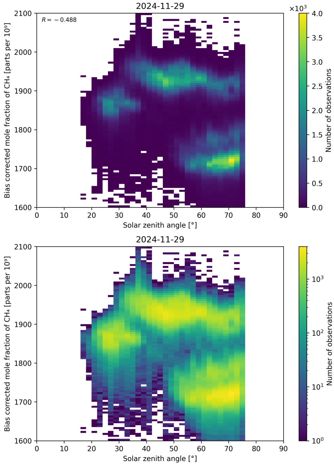
Figure 100: Scatter density plot of “Solar zenith angle” against “Bias corrected mole fraction of CH 4 ” for 2024-11-28 to 2024-11-30.
