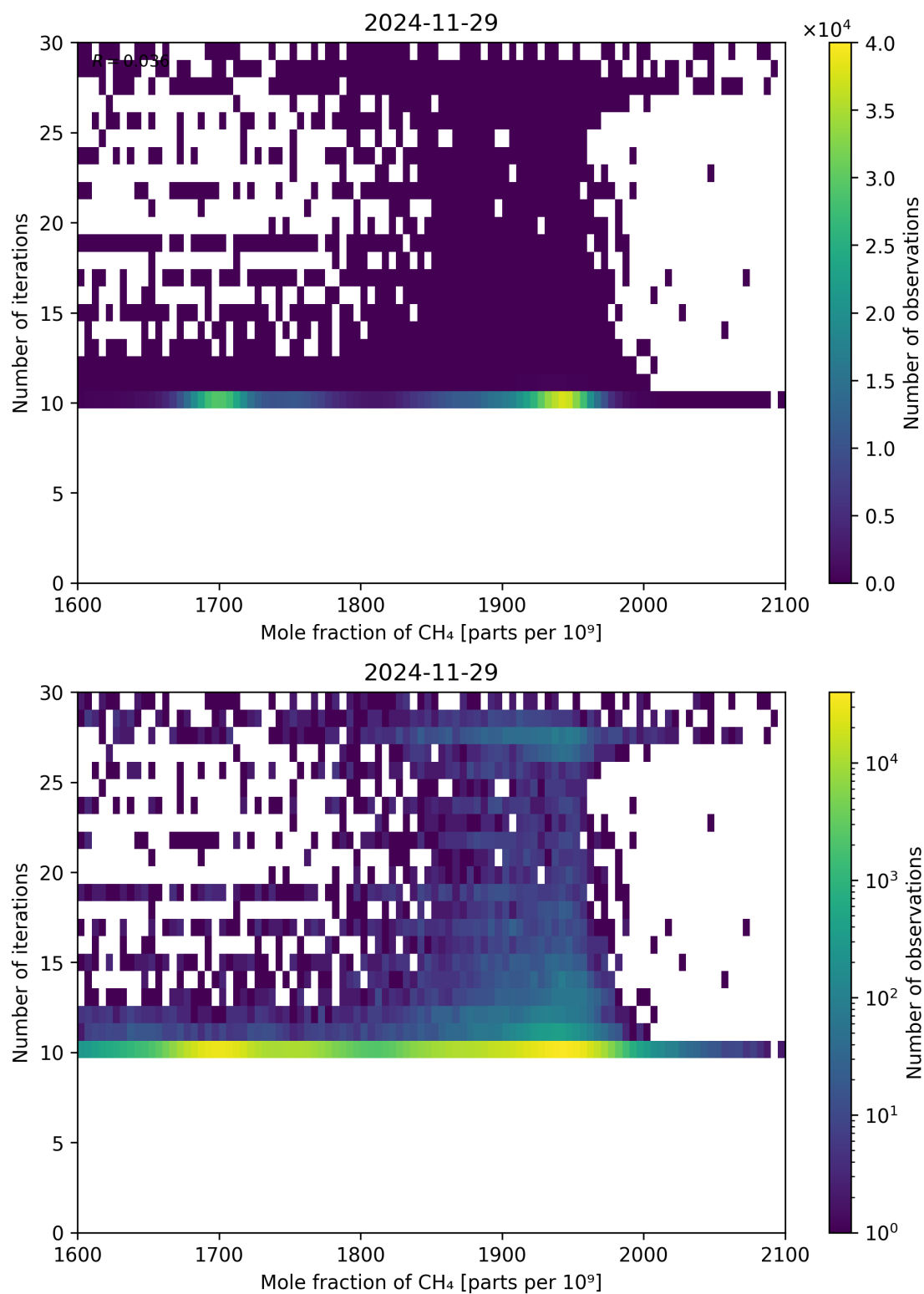
Figure 76: Scatter density plot of “Mole fraction of CH 4 ” against “Number of iterations” for 2024-11-28 to 2024-11-30.
