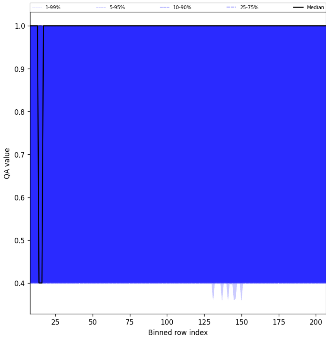
Figure 33: Along track statistics of “QA value” for 2024-11-28 to 2024-11-30
