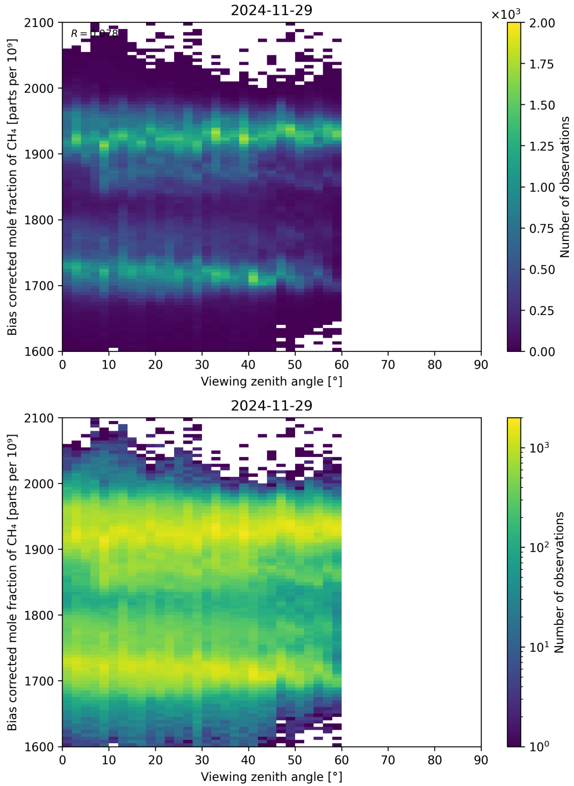
Figure 111: Scatter density plot of “Viewing zenith angle” against “Bias corrected mole fraction of CH 4 ” for 2024-11-28 to 2024-11-30.
