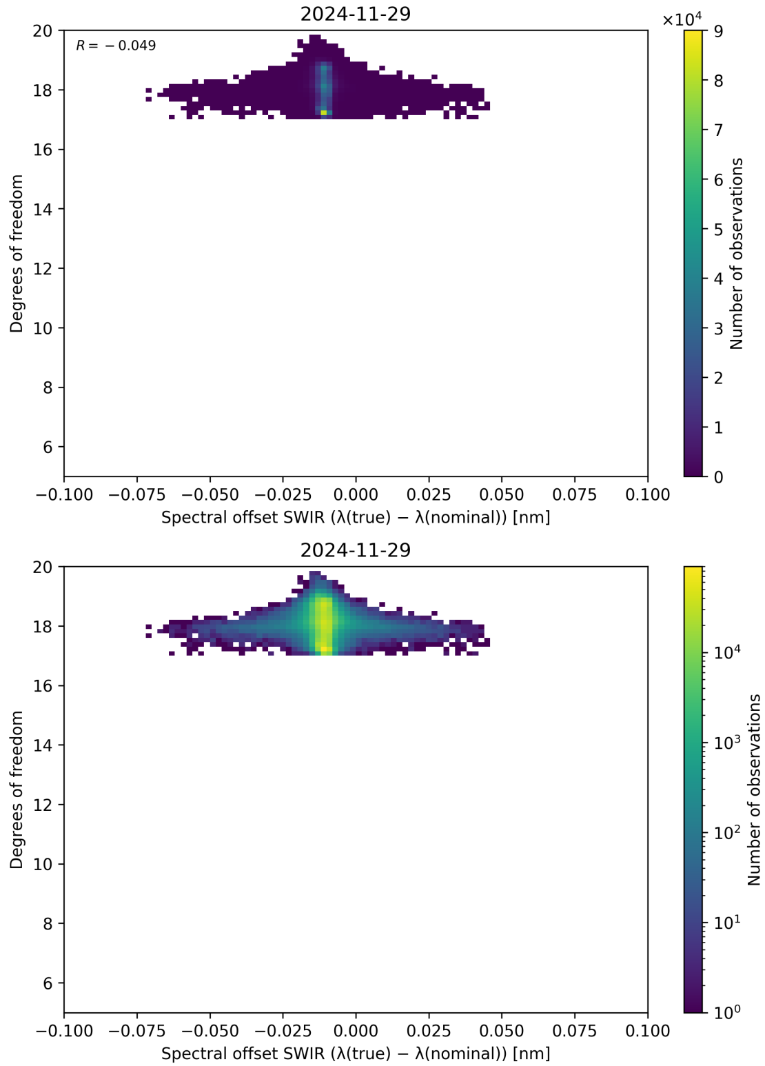
Figure 119: Scatter density plot of “Spectral offset SWIR ( \lambda_{\text{true}} - \lambda_{\text{nominal}} )” against “Degrees of freedom” for 2024-11-28 to 2024-11-30.
