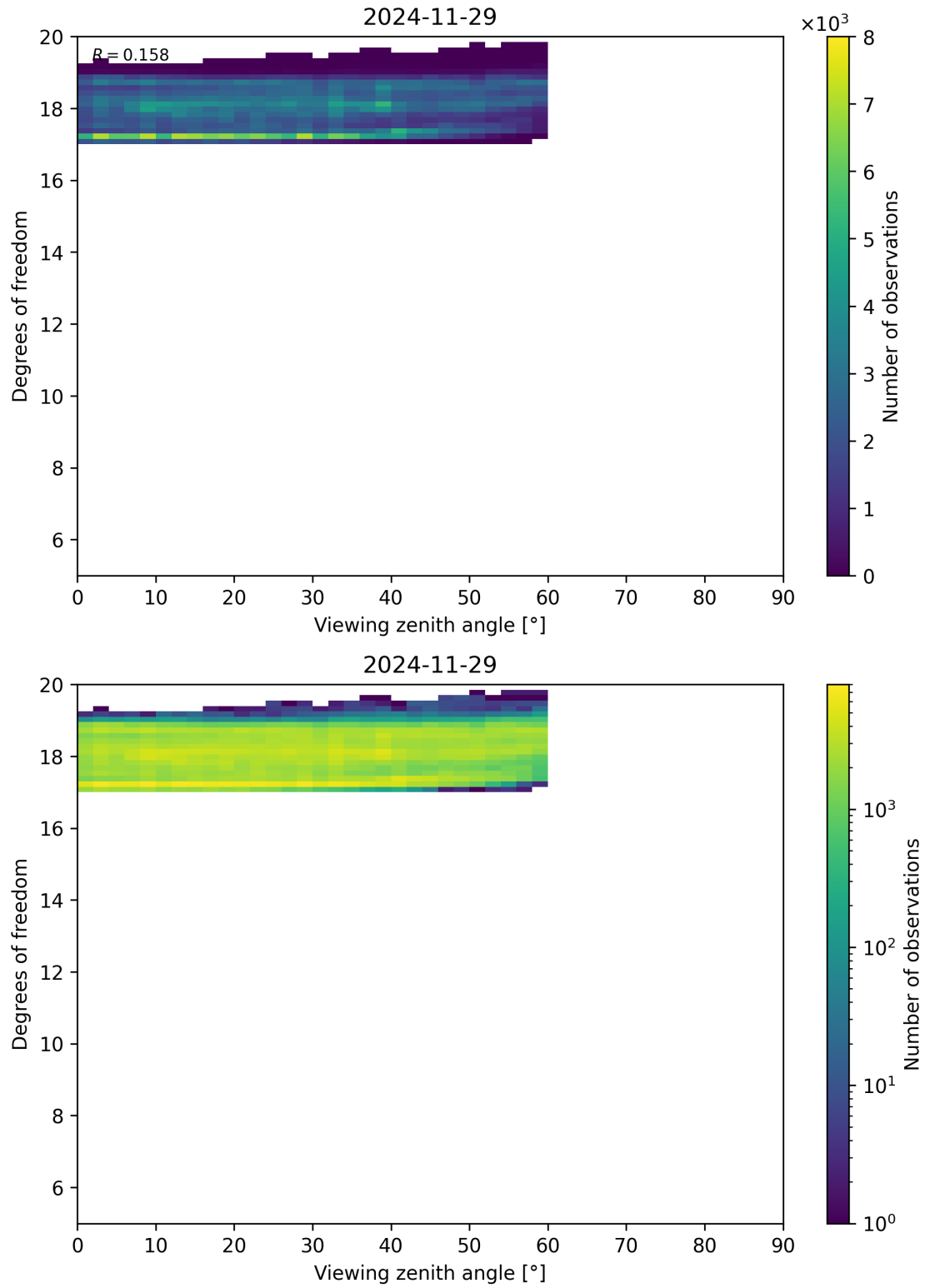
Figure 107: Scatter density plot of “Viewing zenith angle” against “Degrees of freedom” for 2024-11-28 to 2024-11-30.
