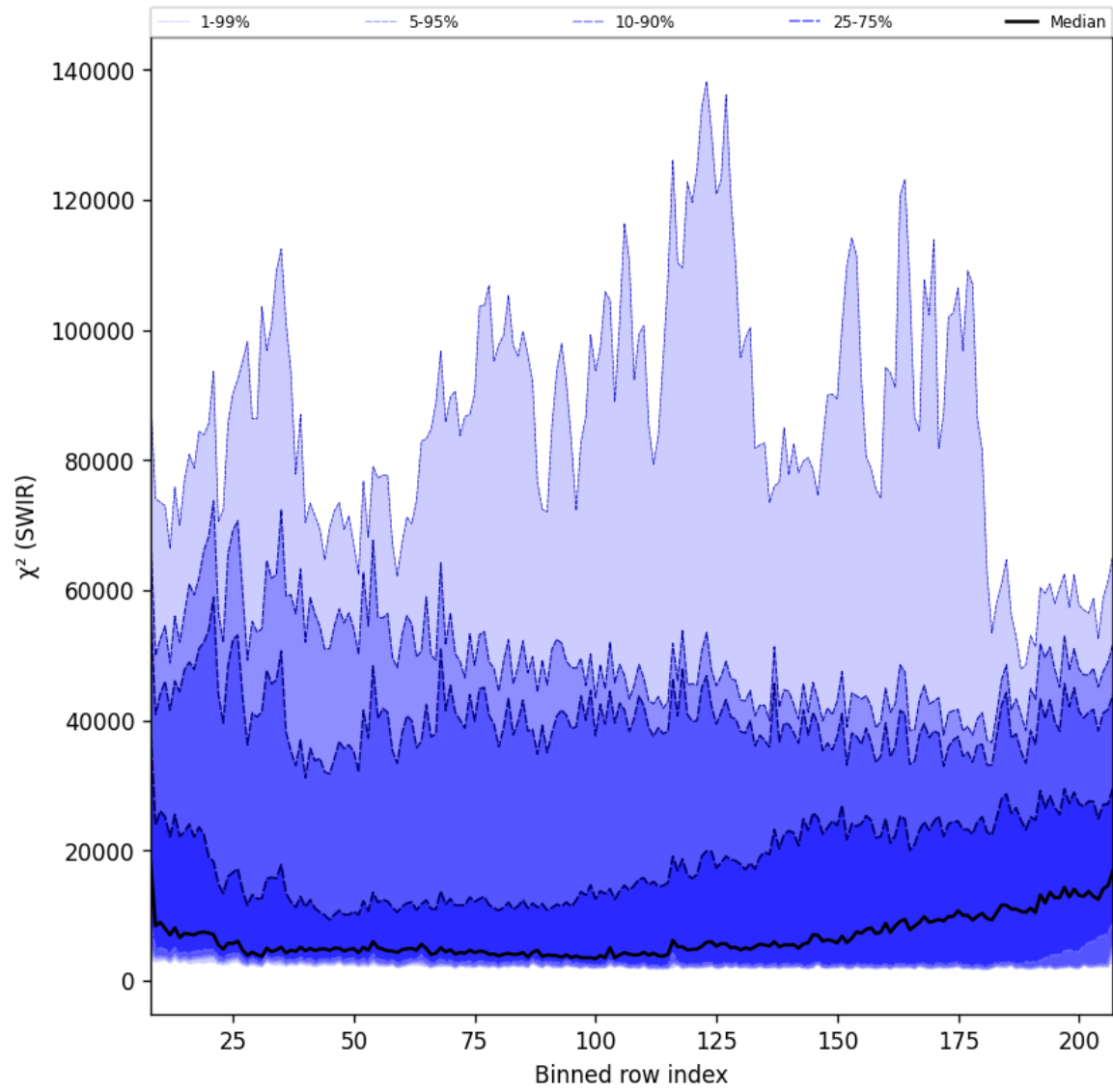
Figure 39: Along track statistics of “ \chi^2 (SWIR)” for 2024-11-28 to 2024-11-30
