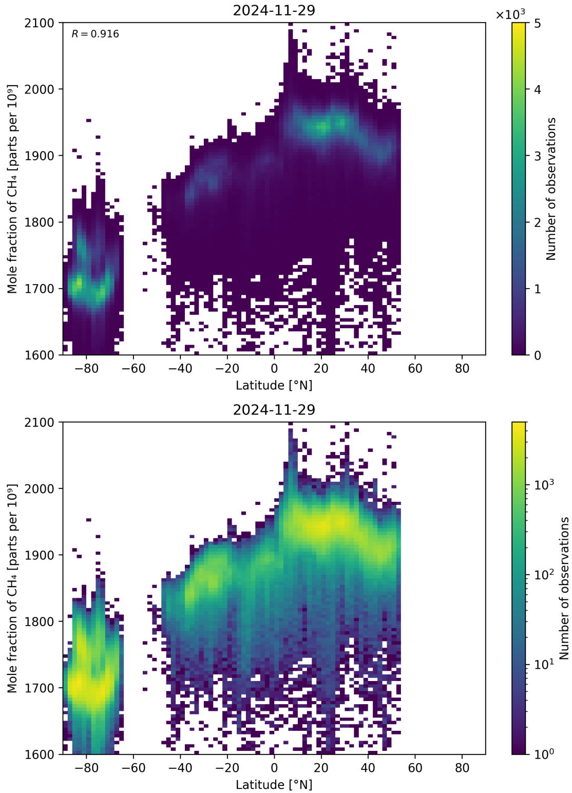
Figure 57: Scatter density plot of “Latitude” against “Mole fraction of CH 4 ” for 2024-11-28 to 2024-11-30.
