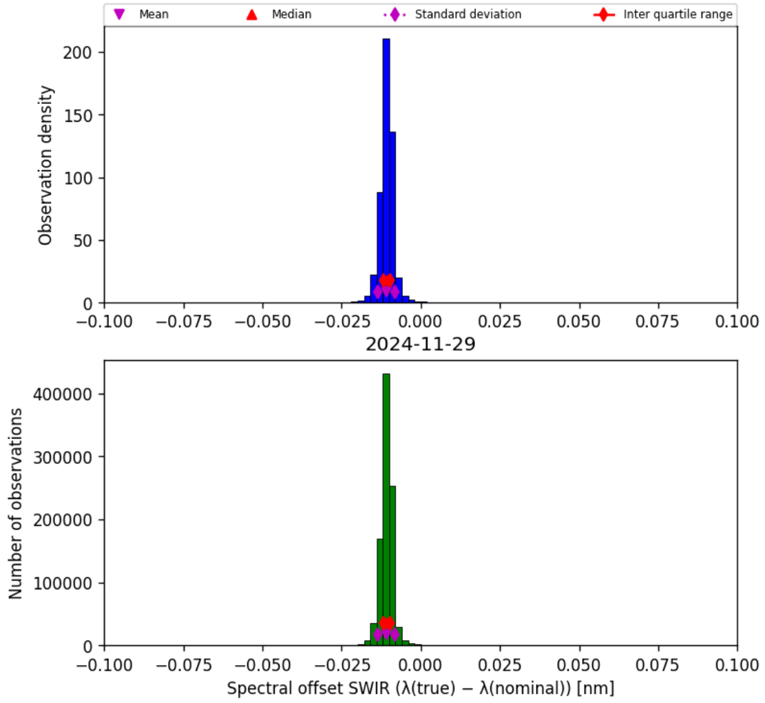
Figure 27: Histogram of “Spectral offset SWIR ( \lambda_{\text{true}} - \lambda_{\text{nominal}} )” for 2024-11-28 to 2024-11-30
