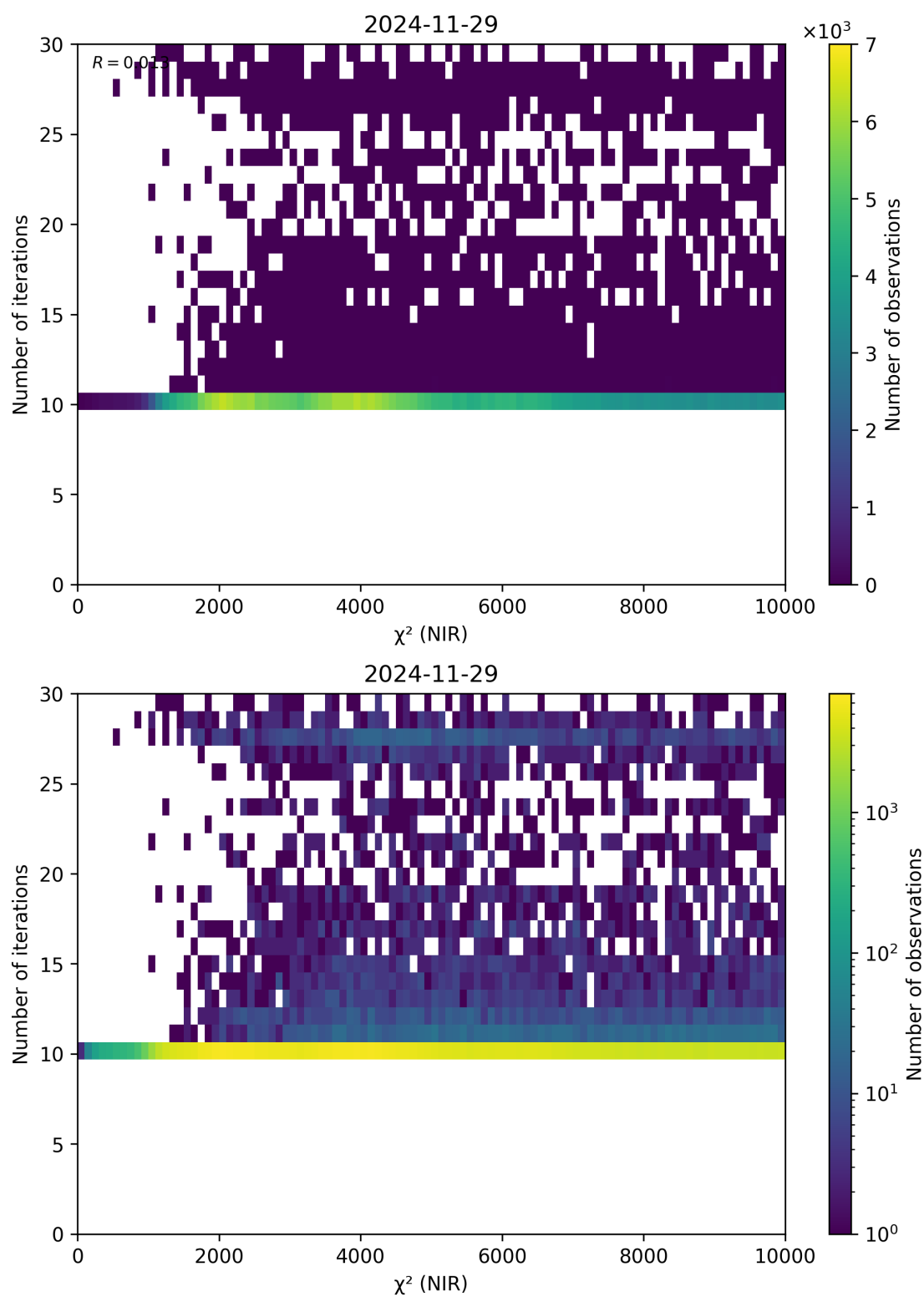
Figure 46: Scatter density plot of “ \chi^2 (NIR)” against “Number of iterations” for 2024-11-28 to 2024-11-30.
