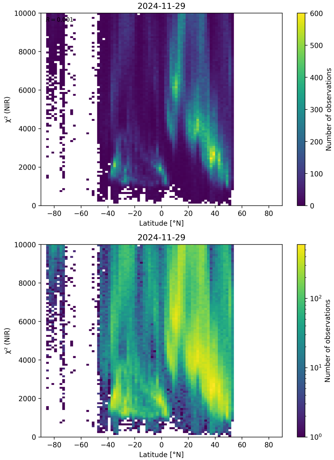
Figure 53: Scatter density plot of “Latitude” against “ \chi^2 (NIR)” for 2024-11-28 to 2024-11-30.
