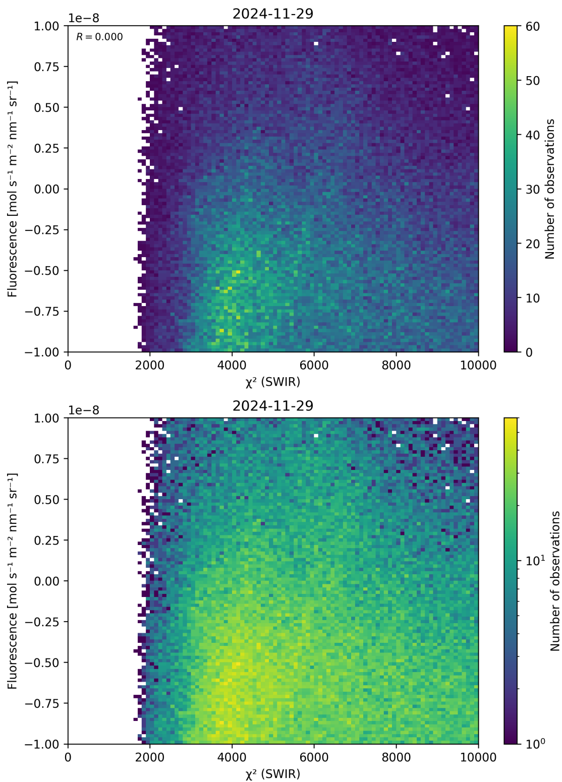
Figure 49: Scatter density plot of “ \chi^2 (SWIR)” against “Fluorescence” for 2024-11-28 to 2024-11-30.
