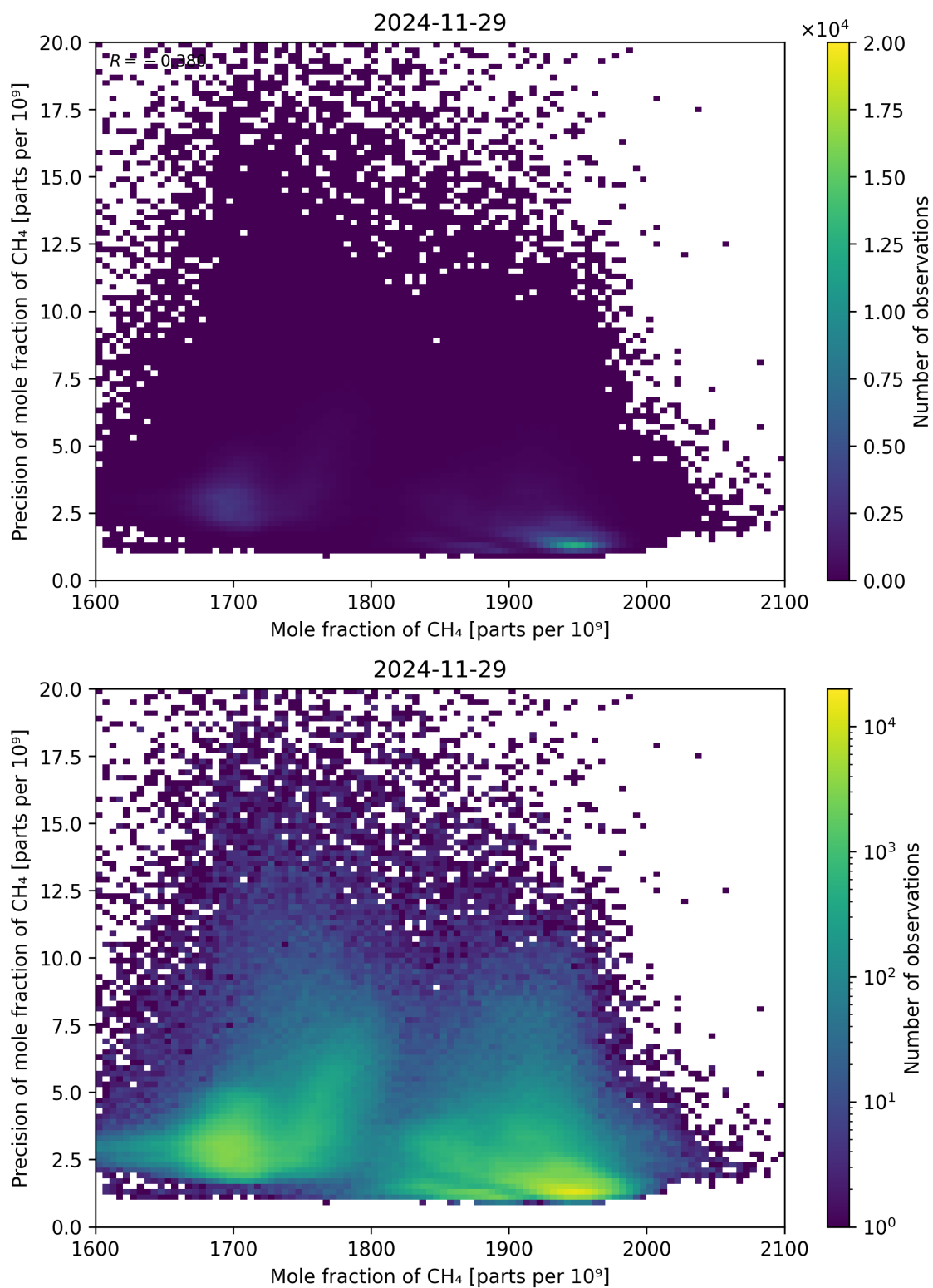
Figure 75: Scatter density plot of “Mole fraction of CH 4 ” against “Precision of mole fraction of CH 4 ” for 2024-11-28 to 2024-11-30.
