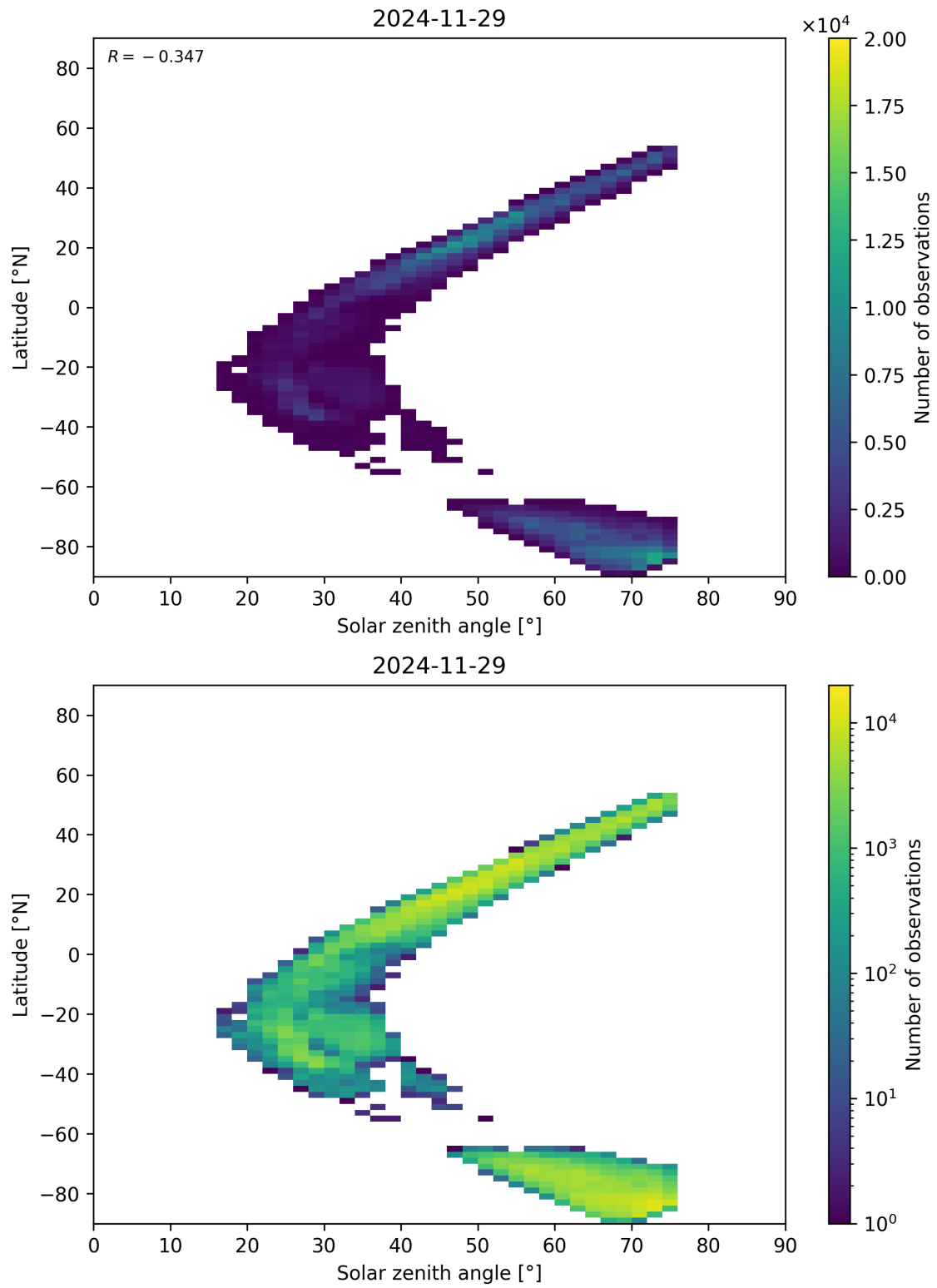
Figure 98: Scatter density plot of “Solar zenith angle” against “Latitude” for 2024-11-28 to 2024-11-30.
