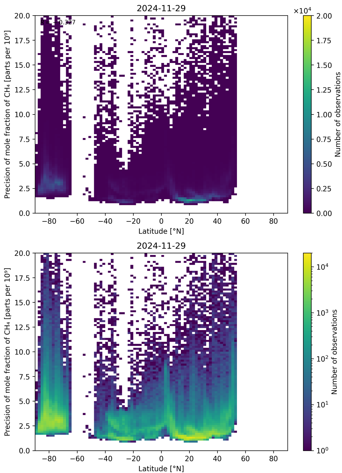
Figure 59: Scatter density plot of “Latitude” against “Precision of mole fraction of CH 4 ” for 2024-11-28 to 2024-11-30.
