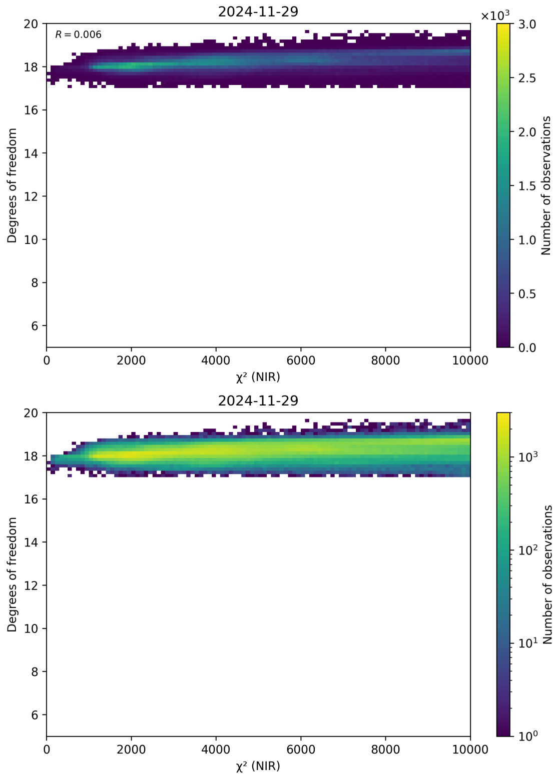
Figure 44: Scatter density plot of “ \chi^2 (NIR)” against “Degrees of freedom” for 2024-11-28 to 2024-11-30.
