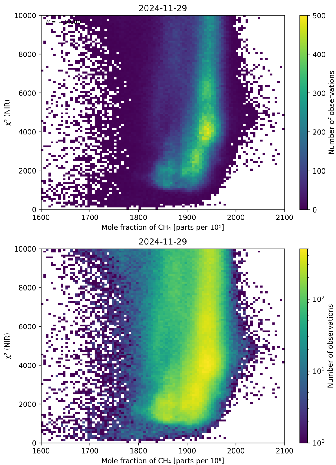
Figure 70: Scatter density plot of “Mole fraction of CH 4 ” against “ \chi^2 (NIR)” for 2024-11-28 to 2024-11-30.
