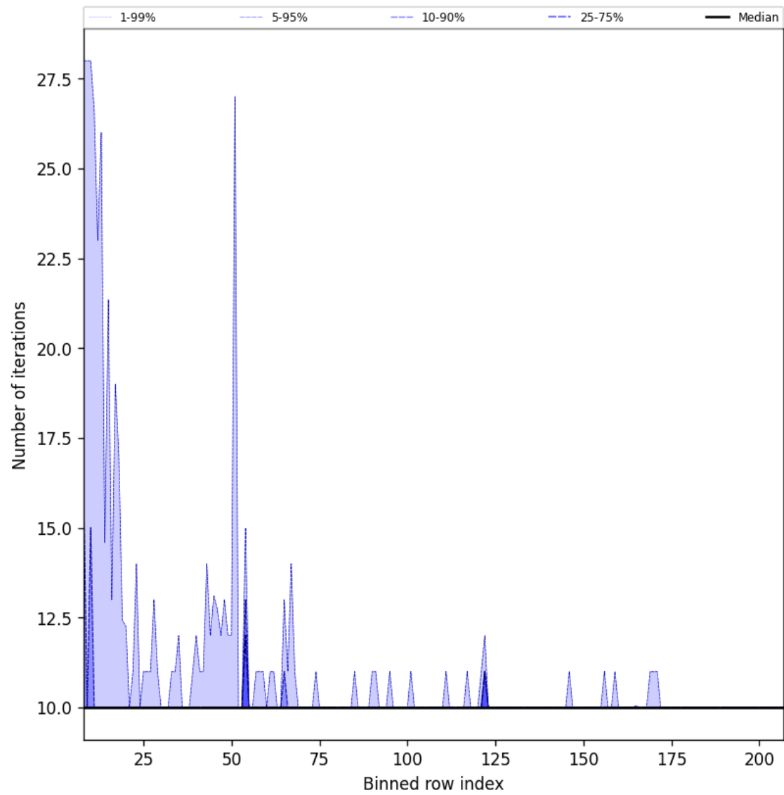
Figure 42: Along track statistics of “Number of iterations” for 2024-11-28 to 2024-11-30
