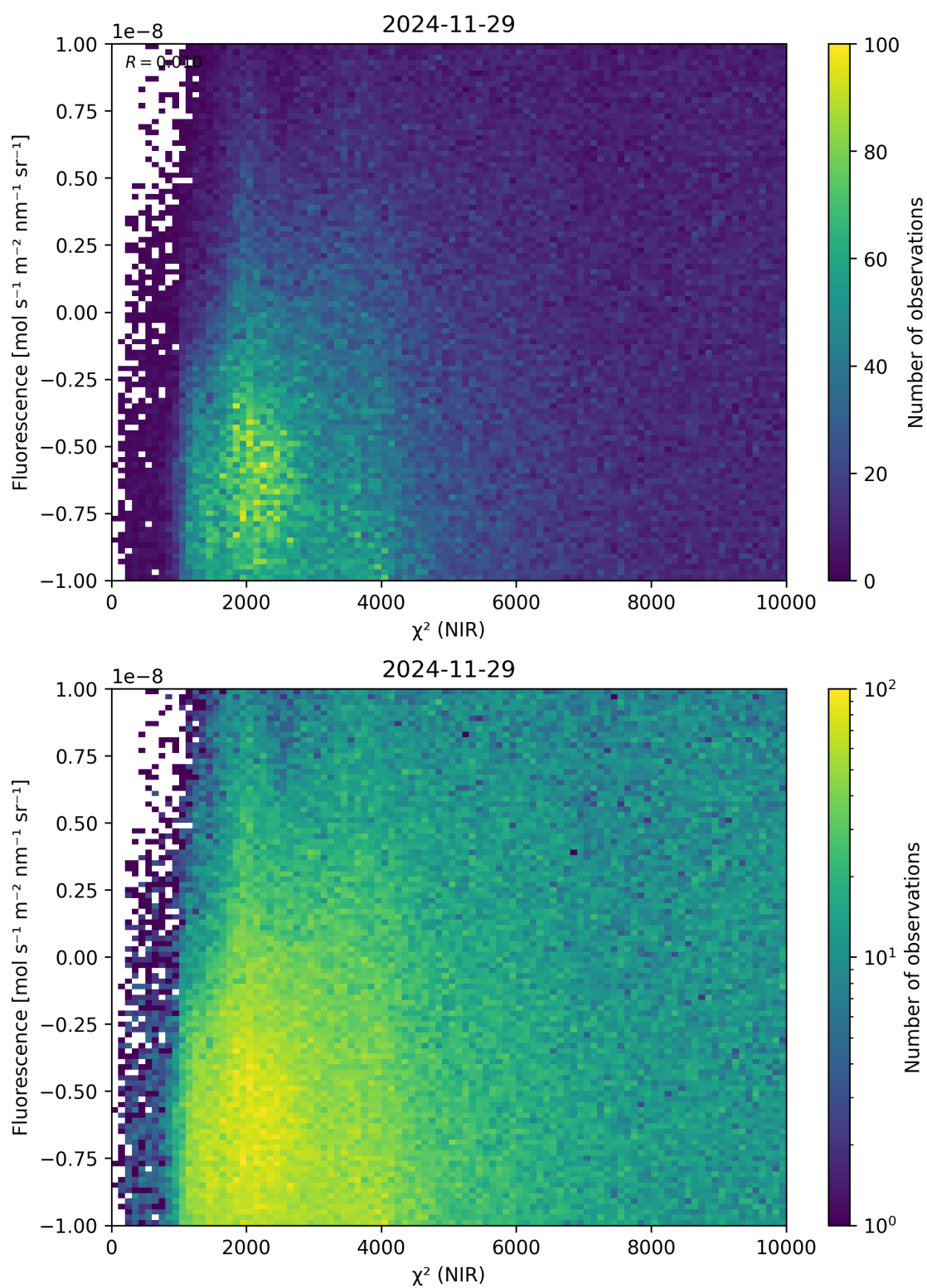
Figure 45: Scatter density plot of “ \chi^2 (NIR)” against “Fluorescence” for 2024-11-28 to 2024-11-30.
