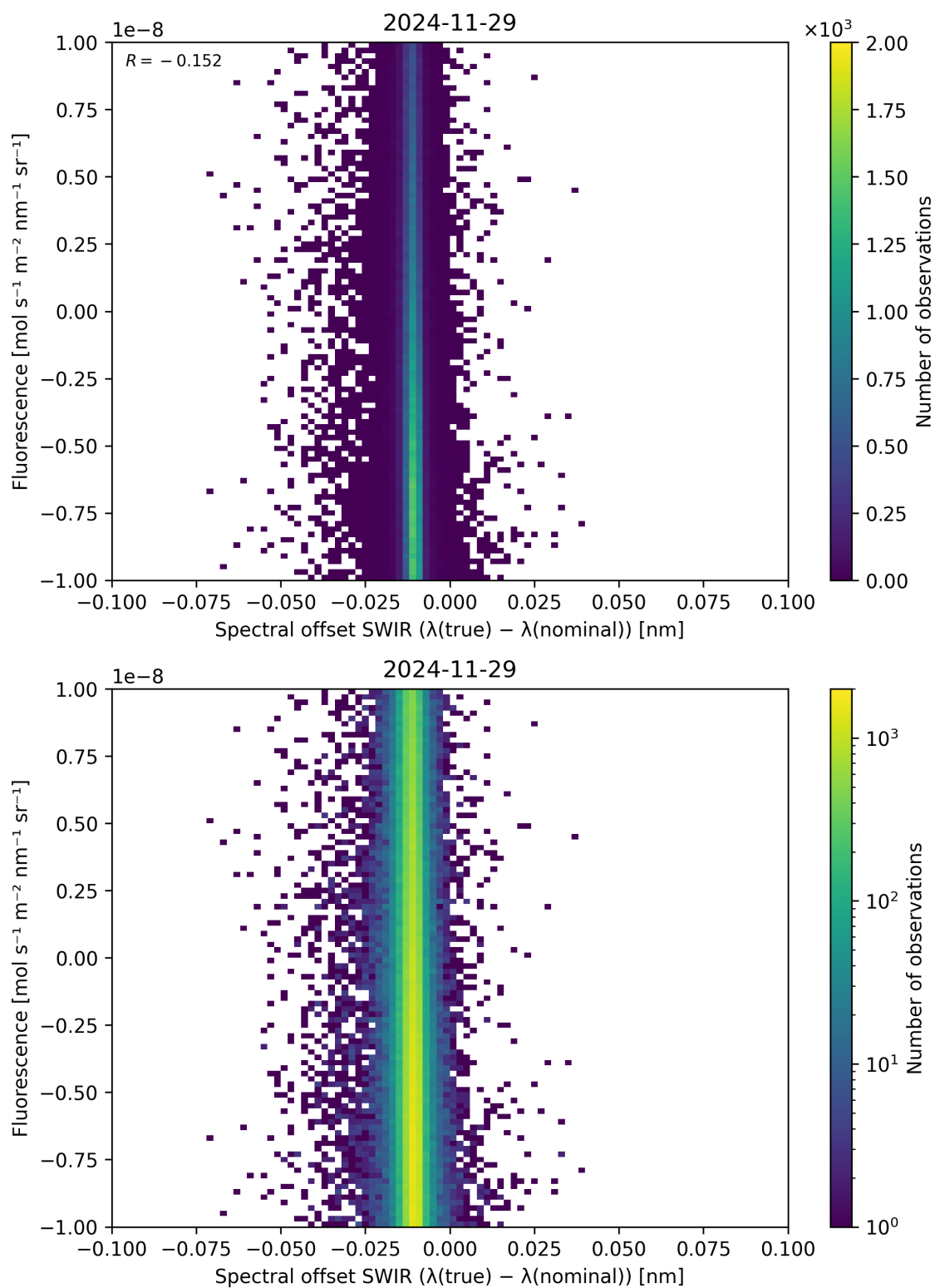
Figure 120: Scatter density plot of “Spectral offset SWIR ( \lambda_{\text{true}} - \lambda_{\text{nominal}} )” against “Fluorescence” for 2024-11-28 to 2024-11-30.
