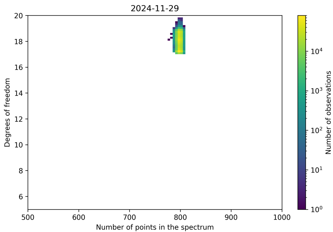
Figure 90: Scatter density plot of “Number of points in the spectrum” against “Degrees of freedom” for 2024-11-28 to 2024-11-30.
