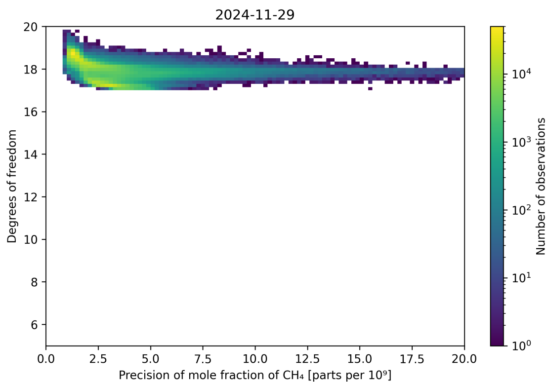
Figure 80: Scatter density plot of “Precision of mole fraction of \text{CH}_4 ” against “Degrees of freedom” for 2024-11-28 to 2024-11-30.
