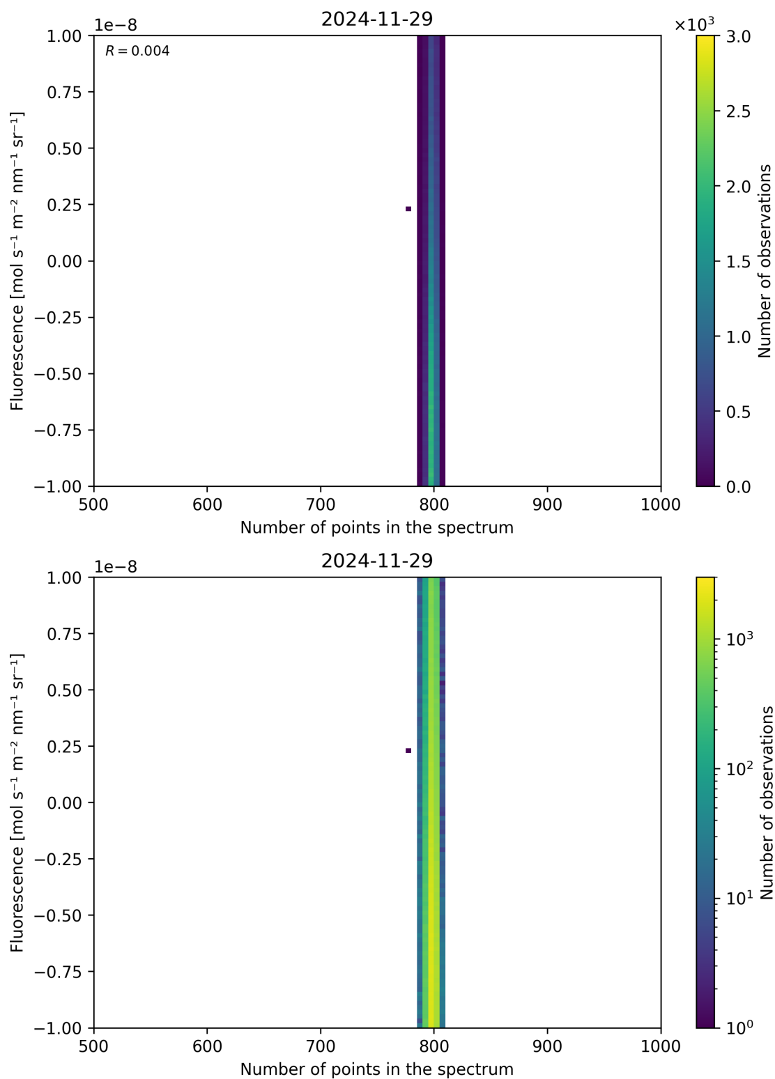
Figure 91: Scatter density plot of “Number of points in the spectrum” against “Fluorescence” for 2024-11-28 to 2024-11-30.
