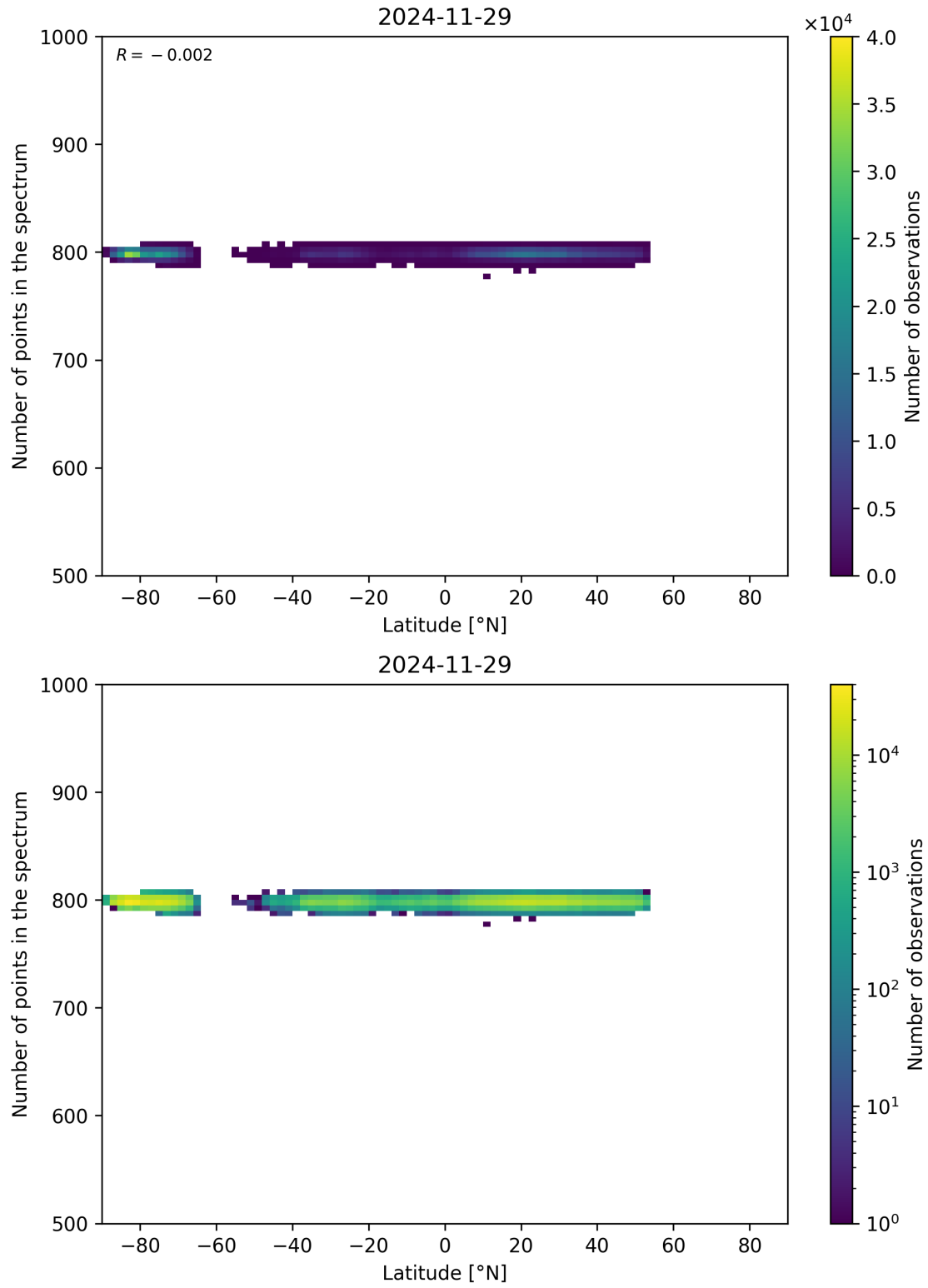
Figure 61: Scatter density plot of “Latitude” against “Number of points in the spectrum” for 2024-11-28 to 2024-11-30.
