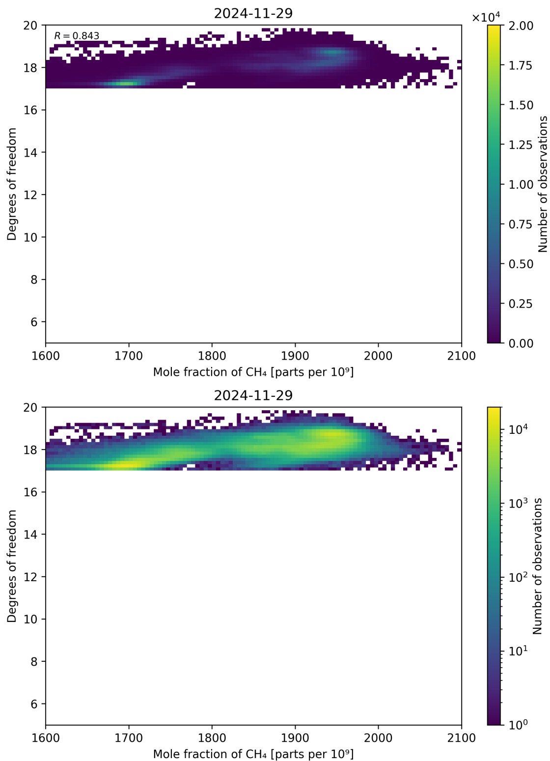
Figure 72: Scatter density plot of “Mole fraction of CH 4 ” against “Degrees of freedom” for 2024-11-28 to 2024-11-30.
