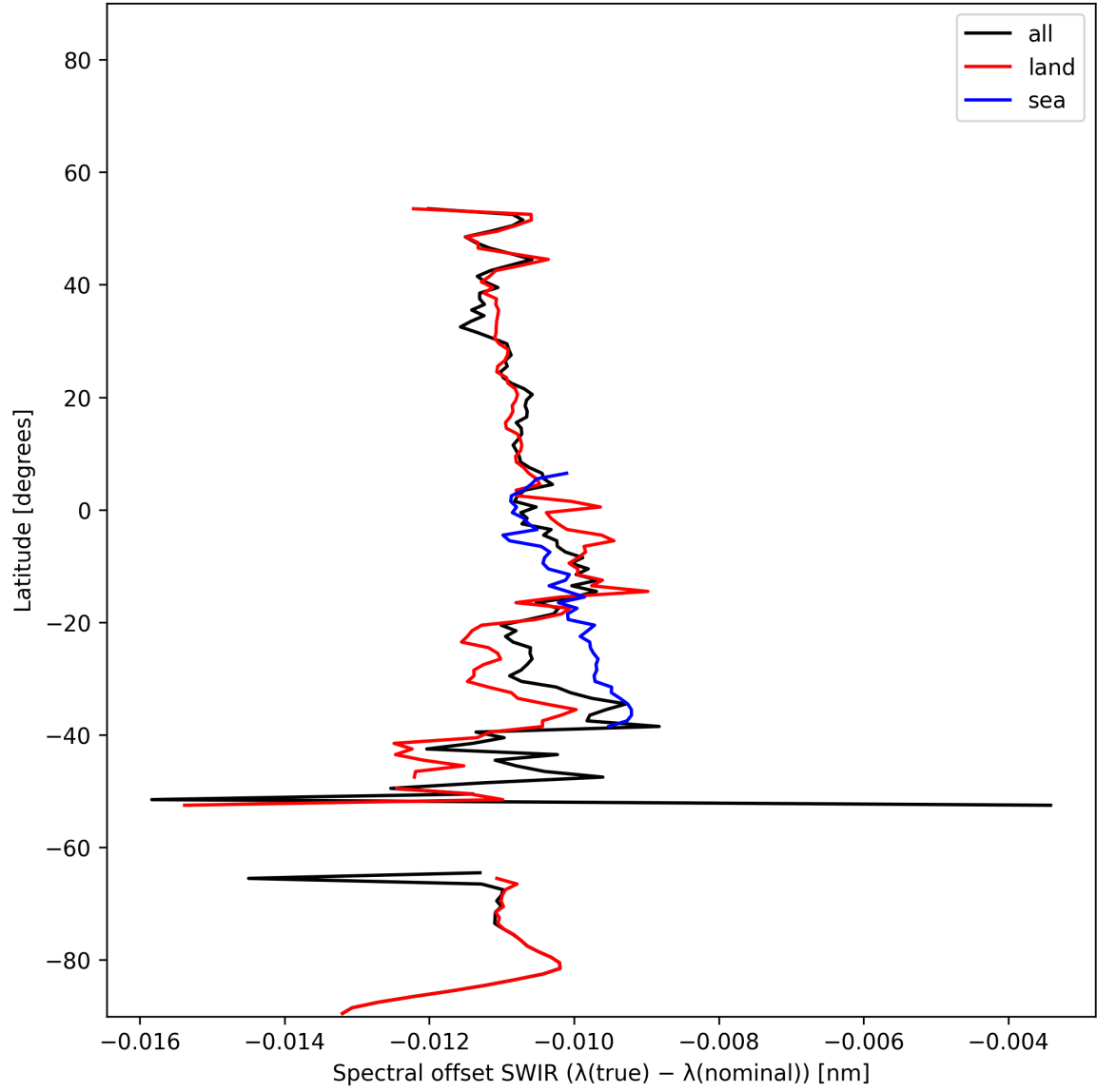
Figure 16: Zonal average of “Spectral offset SWIR ( \lambda_{\text{true}} - \lambda_{\text{nominal}} )” for 2024-11-28 to 2024-11-30.
