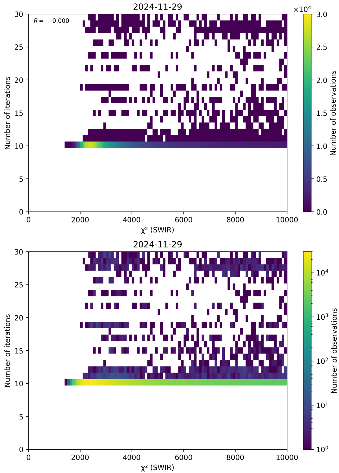
Figure 50: Scatter density plot of “ \chi^2 (SWIR)” against “Number of iterations” for 2024-11-28 to 2024-11-30.
