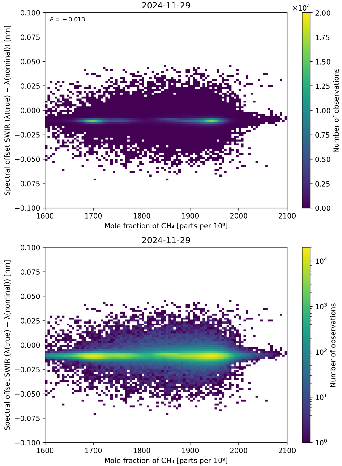
Figure 86: Scatter density plot of “Mole fraction of CH 4 ” against “Spectral offset SWIR ( \lambda_{\text{true}} - \lambda_{\text{nominal}} )” for 2024-11-28 to 2024-11-30.
