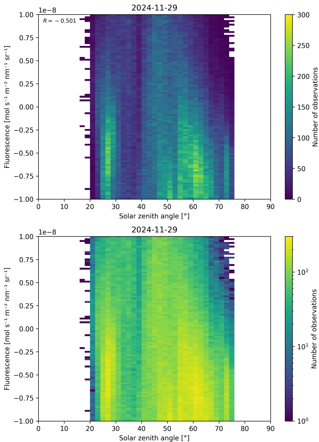
Figure 97: Scatter density plot of “Solar zenith angle” against “Fluorescence” for 2024-11-28 to 2024-11-30.
