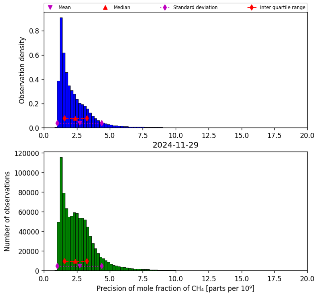
Figure 24: Histogram of “Precision of mole fraction of CH 4 ” for 2024-11-28 to 2024-11-30
