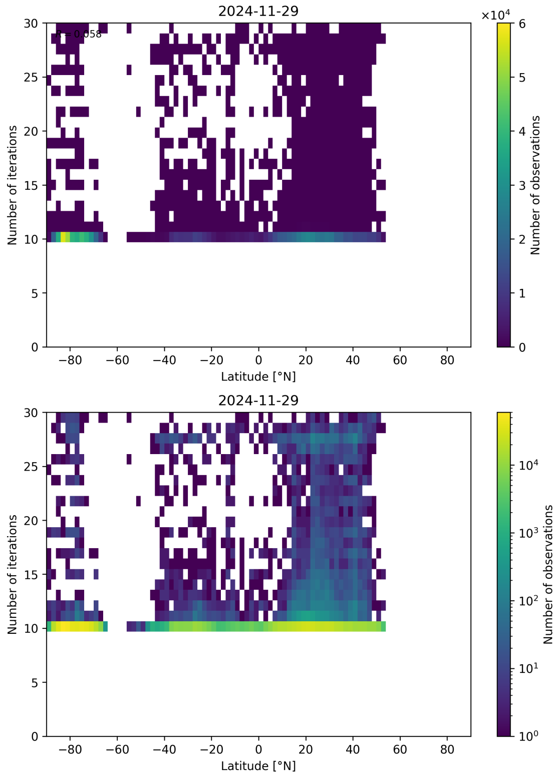
Figure 60: Scatter density plot of “Latitude” against “Number of iterations” for 2024-11-28 to 2024-11-30.
