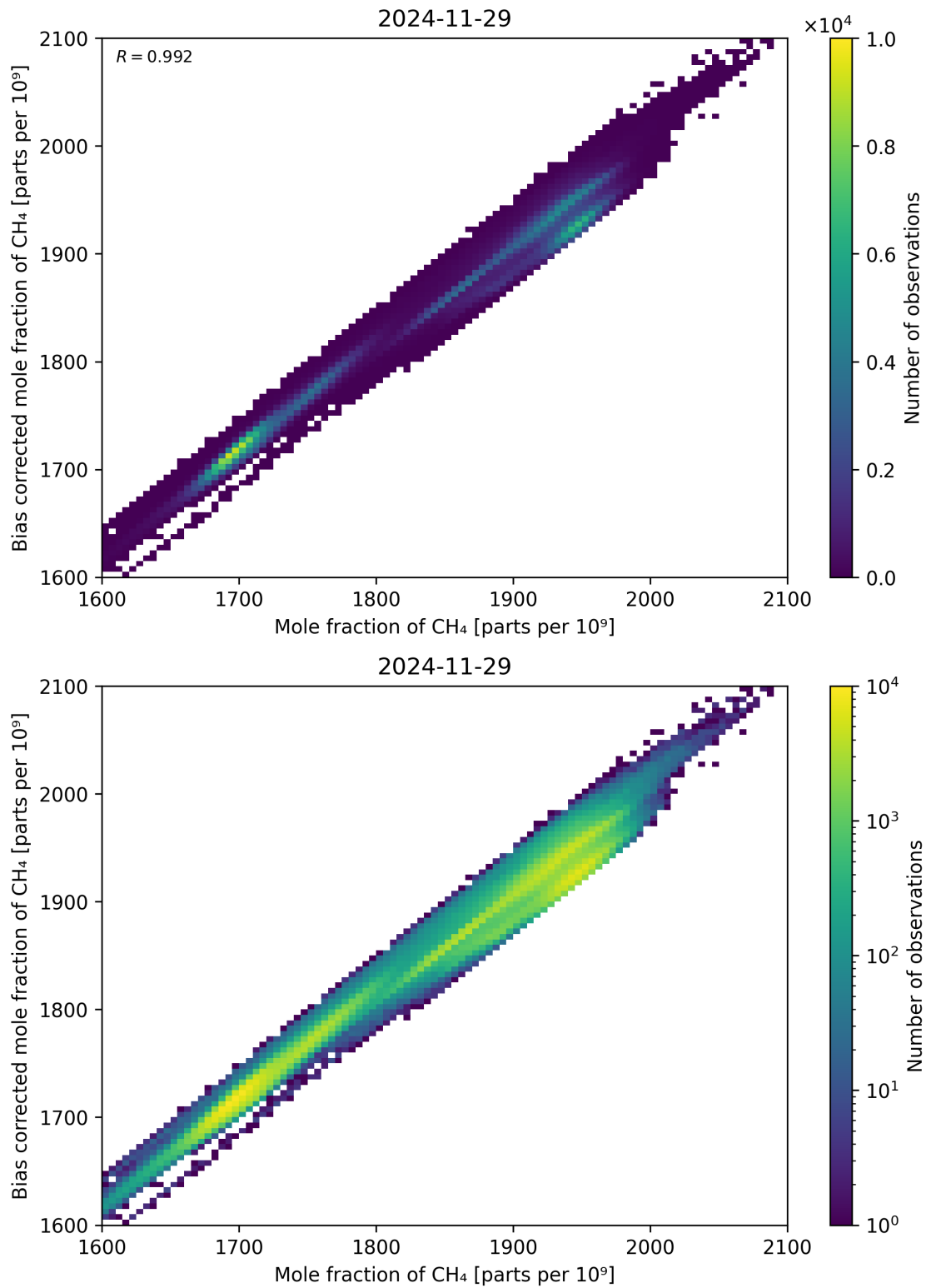
Figure 74: Scatter density plot of “Mole fraction of CH 4 ” against “Bias corrected mole fraction of CH 4 ” for 2024-11-28 to 2024-11-30.
