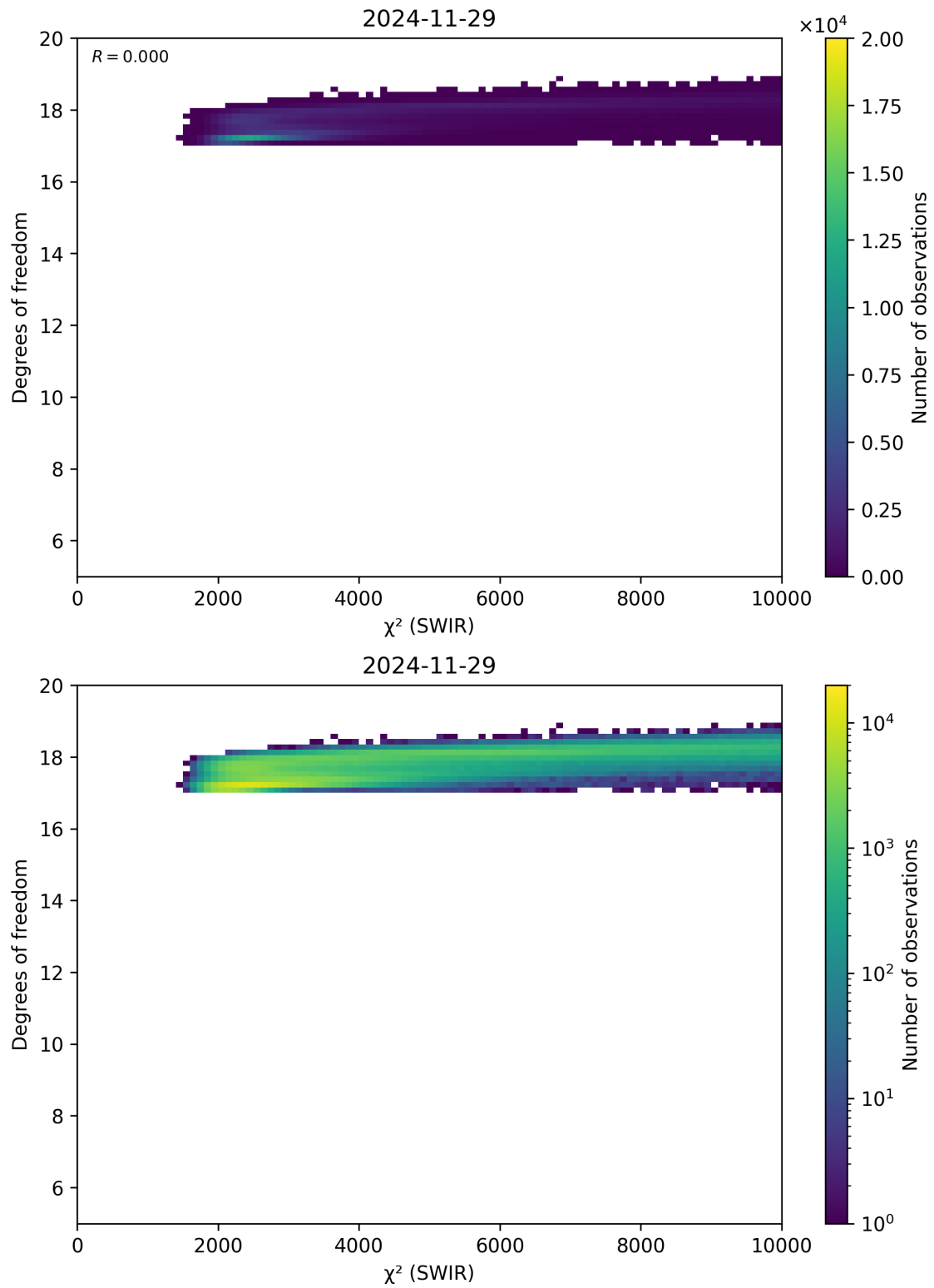
Figure 48: Scatter density plot of “ \chi^2 (SWIR)” against “Degrees of freedom” for 2024-11-28 to 2024-11-30.
