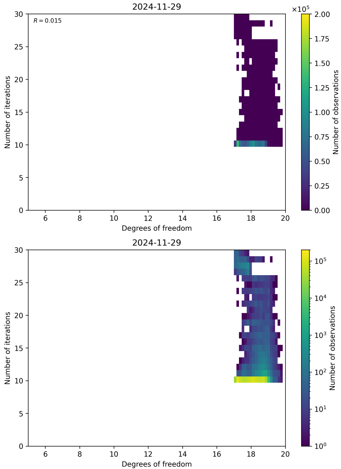
Figure 52: Scatter density plot of “Degrees of freedom” against “Number of iterations” for 2024-11-28 to 2024-11-30.
