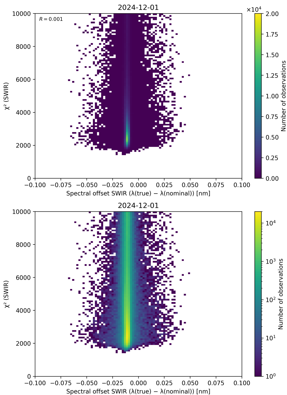
Figure 118: Scatter density plot of “Spectral offset SWIR ( \lambda_{\text{true}} - \lambda_{\text{nominal}} )” against “ \chi^2 (SWIR)” for 2024-11-30 to 2024-12-02.
