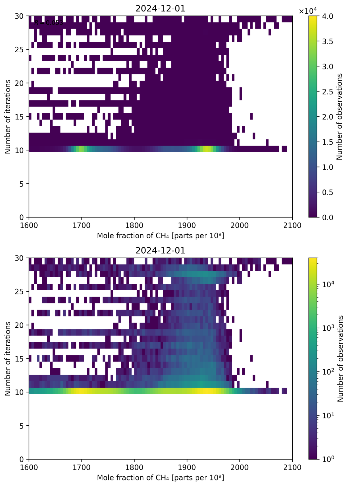
Figure 76: Scatter density plot of “Mole fraction of CH 4 ” against “Number of iterations” for 2024-11-30 to 2024-12-02.
