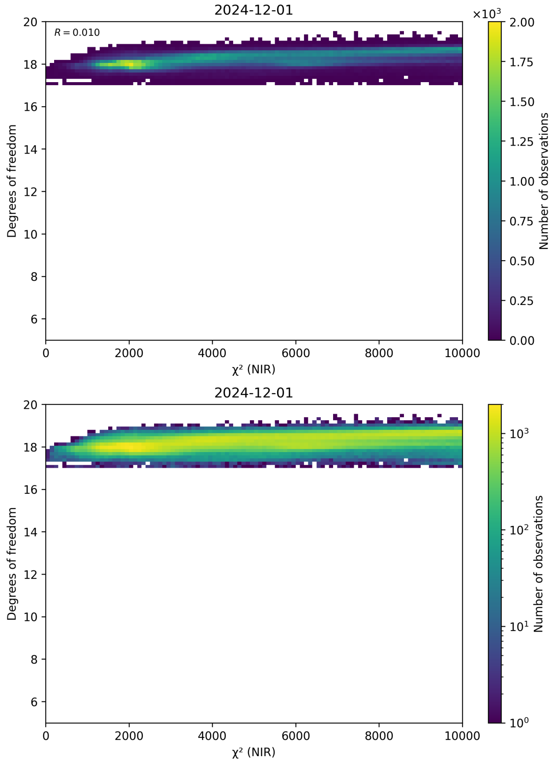
Figure 44: Scatter density plot of “ \chi^2 (NIR)” against “Degrees of freedom” for 2024-11-30 to 2024-12-02.
