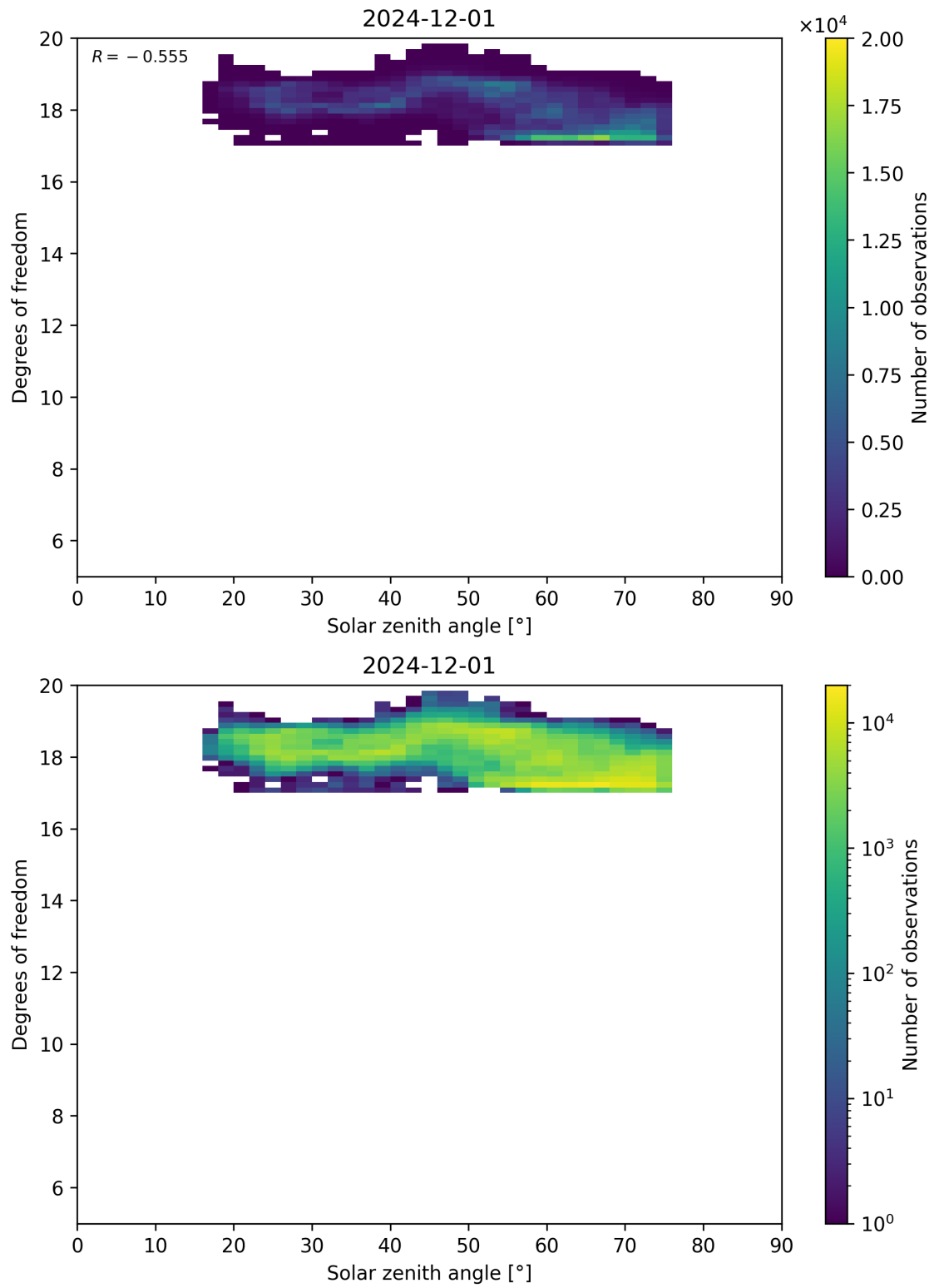
Figure 96: Scatter density plot of “Solar zenith angle” against “Degrees of freedom” for 2024-11-30 to 2024-12-02.
