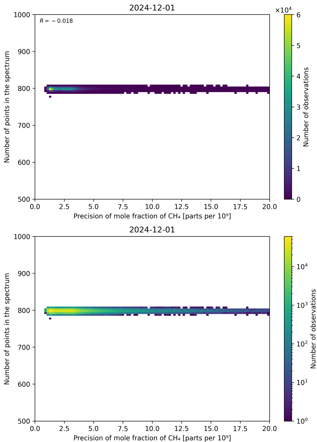
Figure 84: Scatter density plot of “Precision of mole fraction of CH 4 ” against “Number of points in the spectrum” for 2024-11-30 to 2024-12-02.
