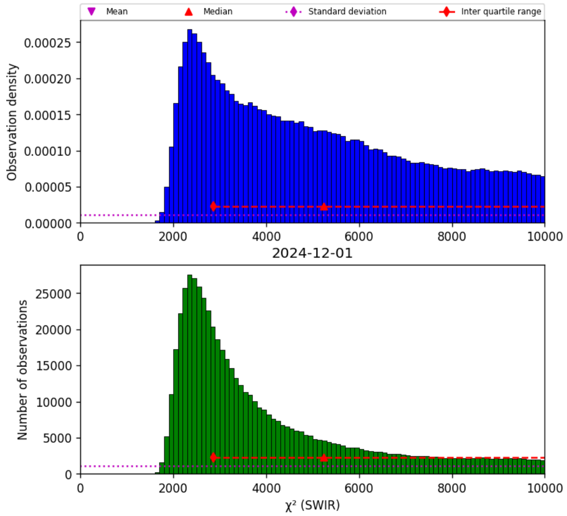
Figure 28: Histogram of “ \chi^2 (SWIR)” for 2024-11-30 to 2024-12-02
