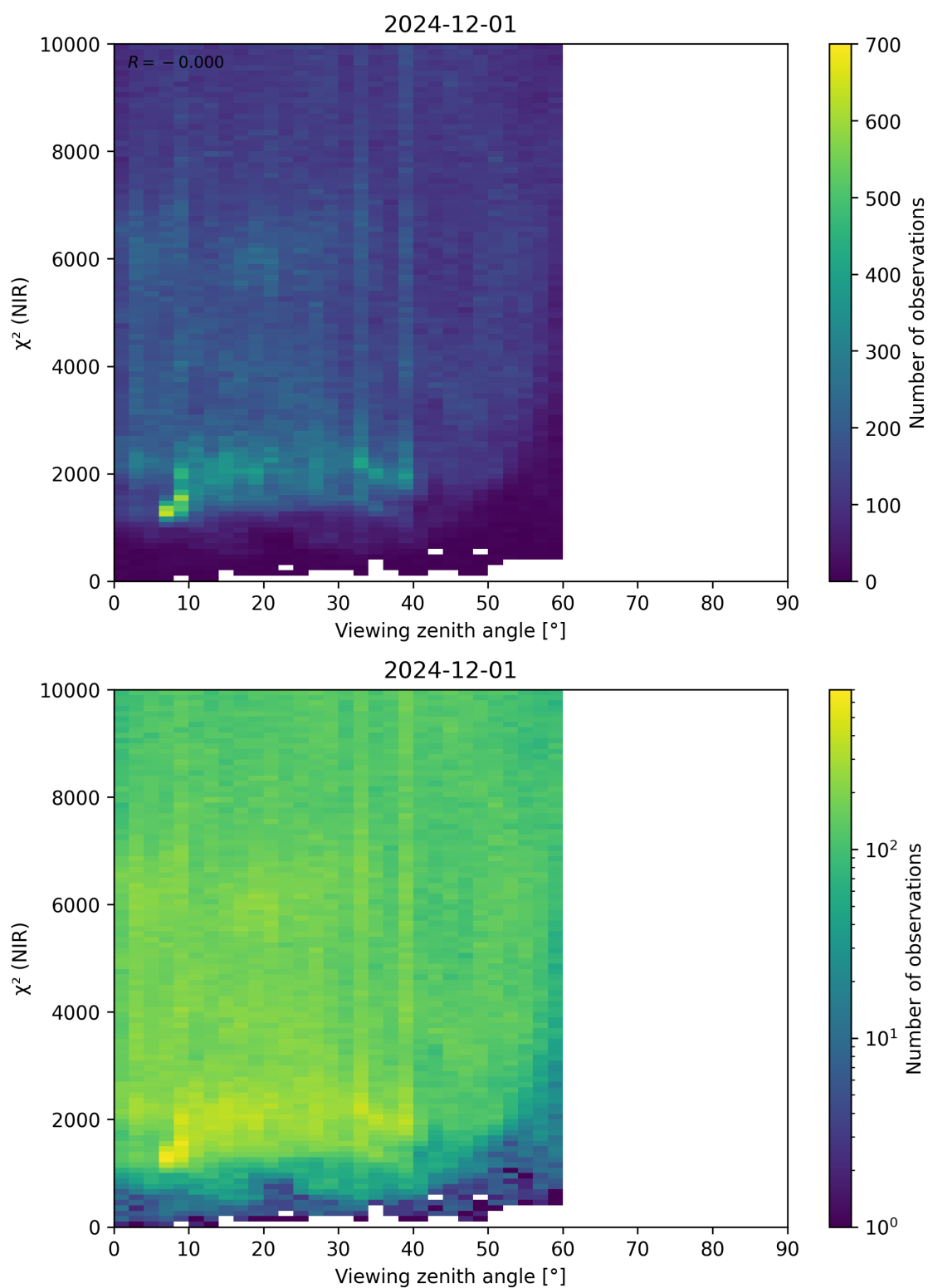
Figure 105: Scatter density plot of “Viewing zenith angle” against “ \chi^2 (NIR)” for 2024-11-30 to 2024-12-02.
