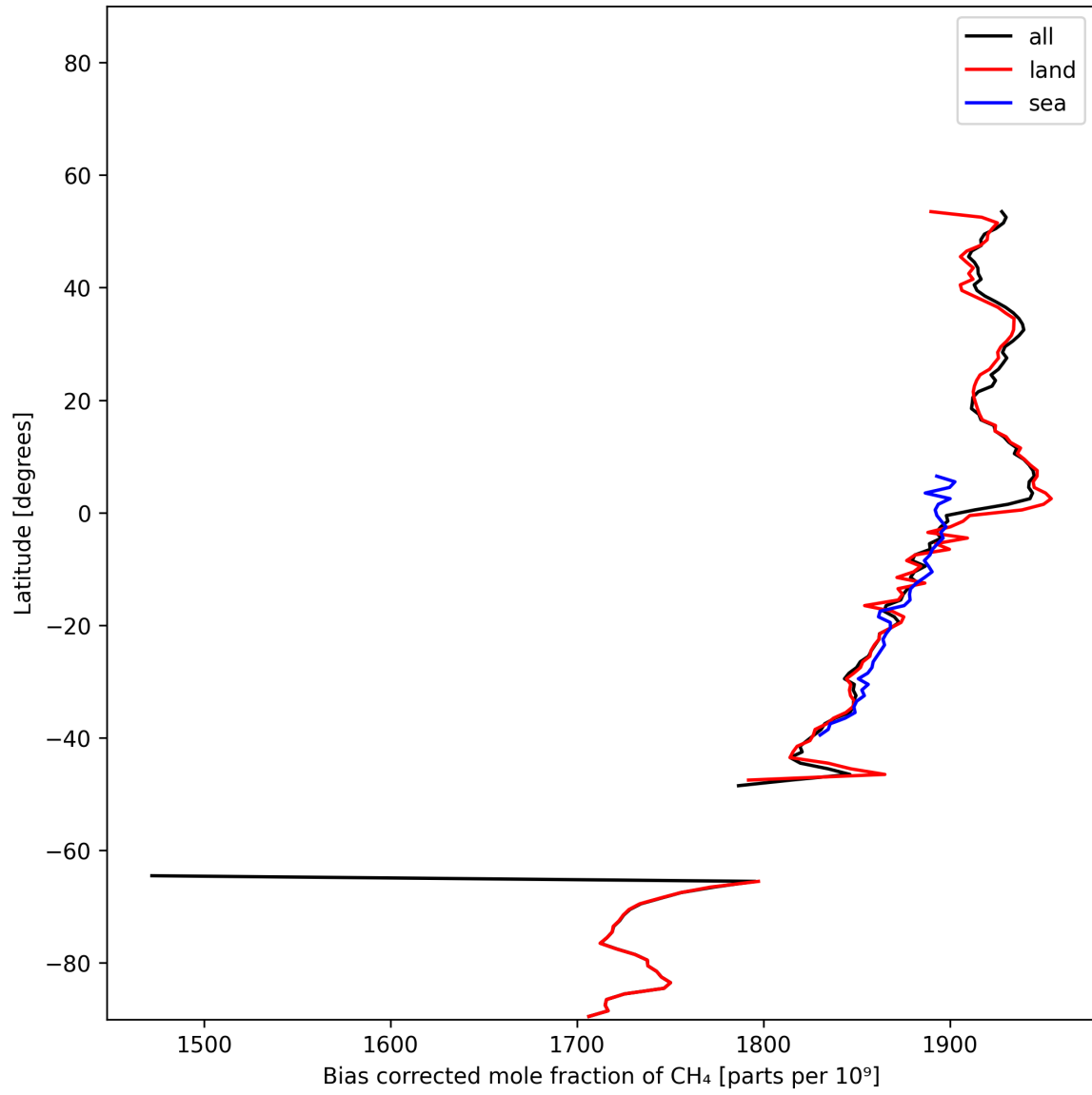
Figure 14: Zonal average of “Bias corrected mole fraction of CH 4 ” for 2024-11-30 to 2024-12-02.
