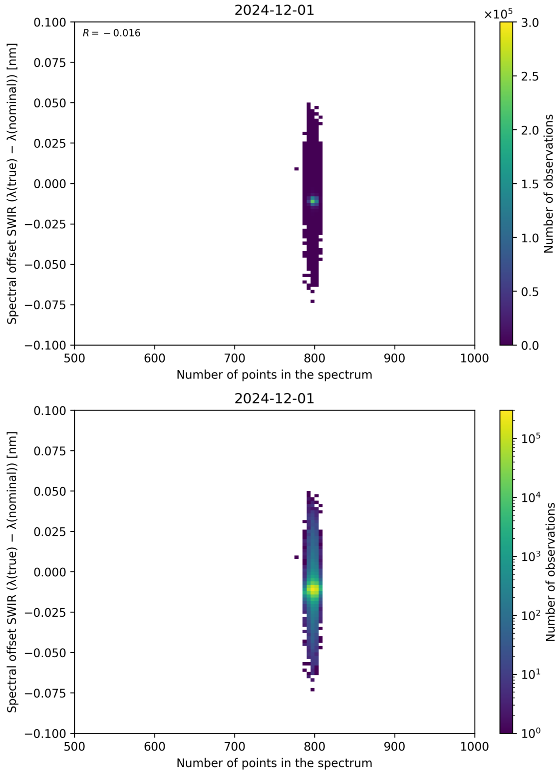
Figure 93: Scatter density plot of “Number of points in the spectrum” against “Spectral offset SWIR ( \lambda_{\text{true}} - \lambda_{\text{nominal}} )” for 2024-11-30 to 2024-12-02.
