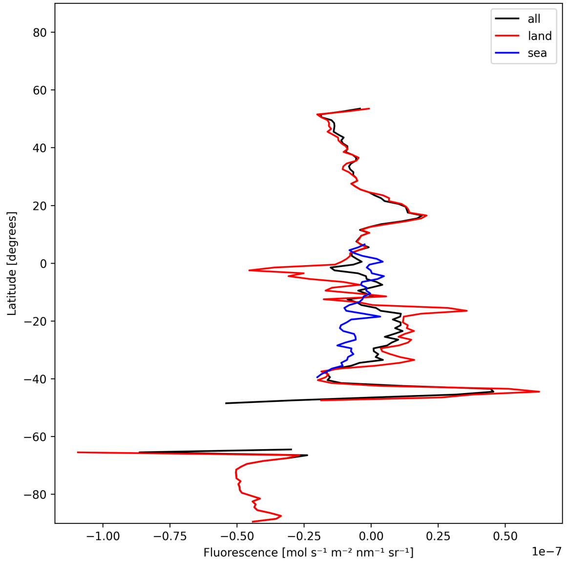
Figure 21: Zonal average of “Fluorescence” for 2024-11-30 to 2024-12-02.
