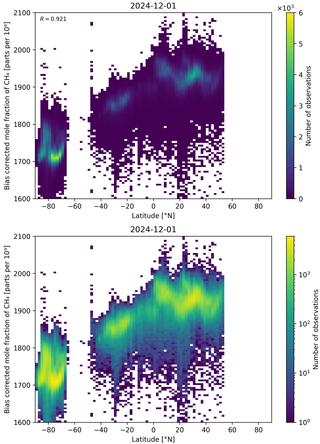
Figure 58: Scatter density plot of “Latitude” against “Bias corrected mole fraction of CH 4 ” for 2024-11-30 to 2024-12-02.
