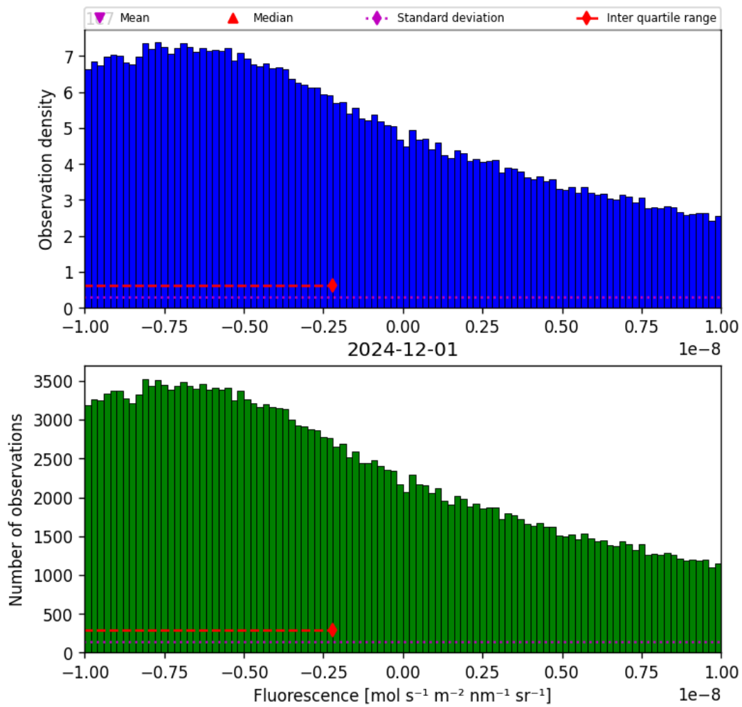
Figure 32: Histogram of “Fluorescence” for 2024-11-30 to 2024-12-02
