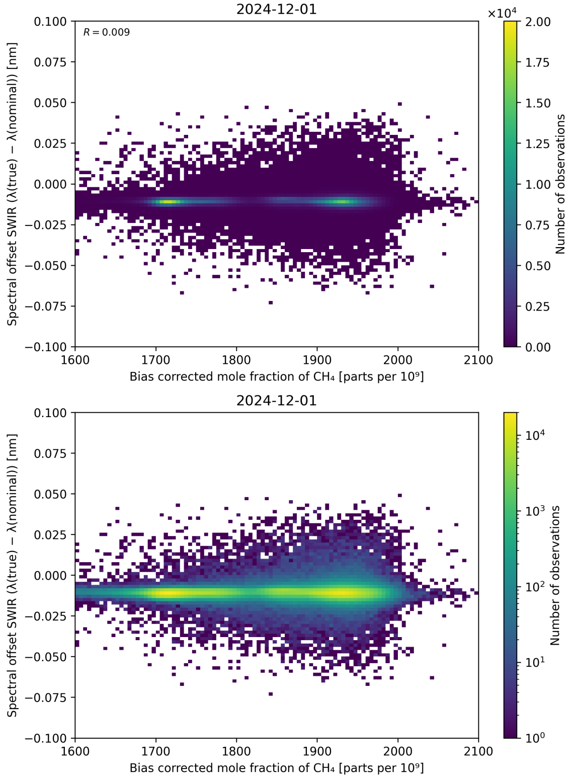
Figure 69: Scatter density plot of “Bias corrected mole fraction of \text{CH}_4 ” against “Spectral offset SWIR ( \lambda_{\text{true}} - \lambda_{\text{nominal}} )” for 2024-11-30 to 2024-12-02.
