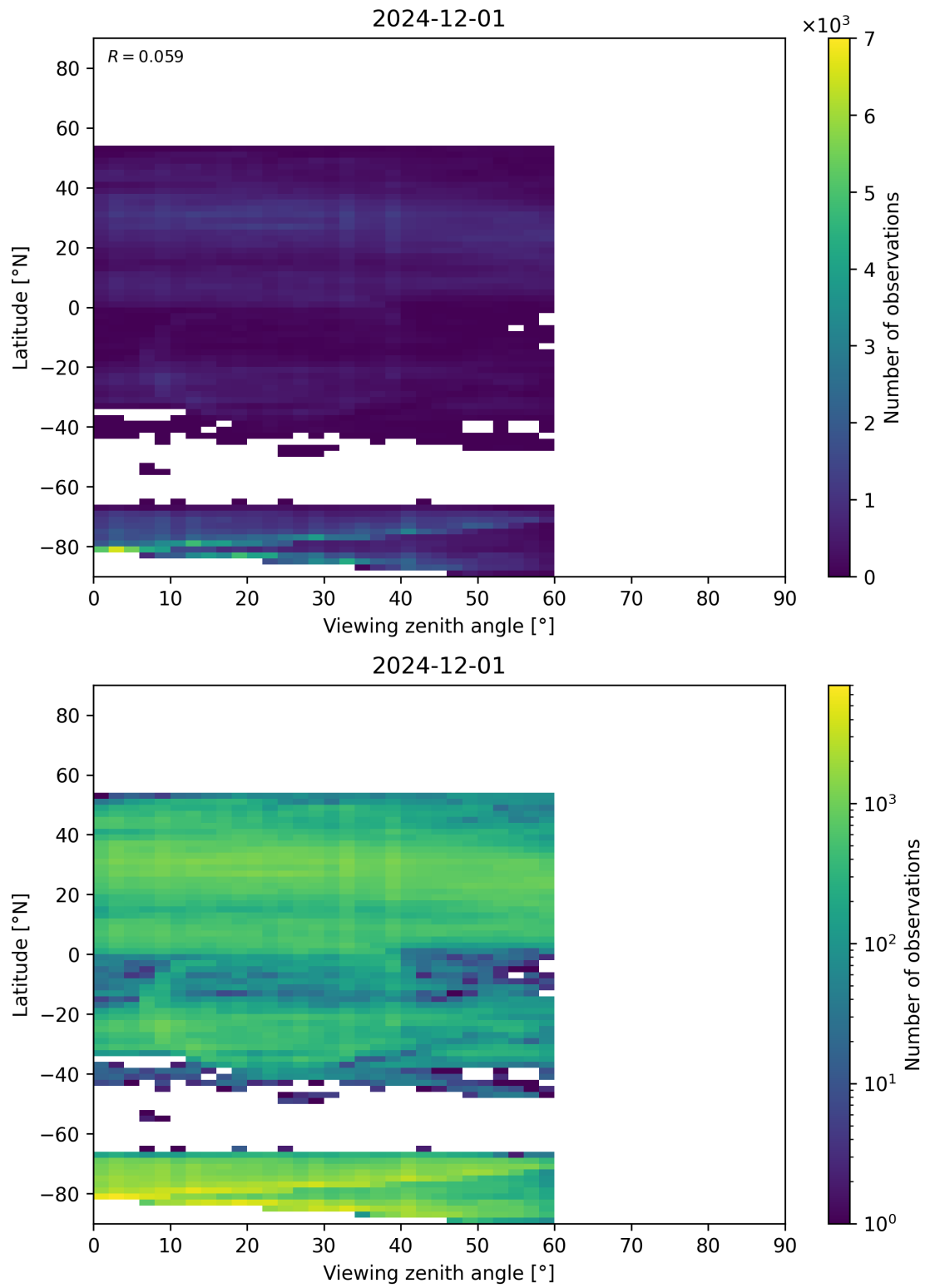
Figure 109: Scatter density plot of “Viewing zenith angle” against “Latitude” for 2024-11-30 to 2024-12-02.
