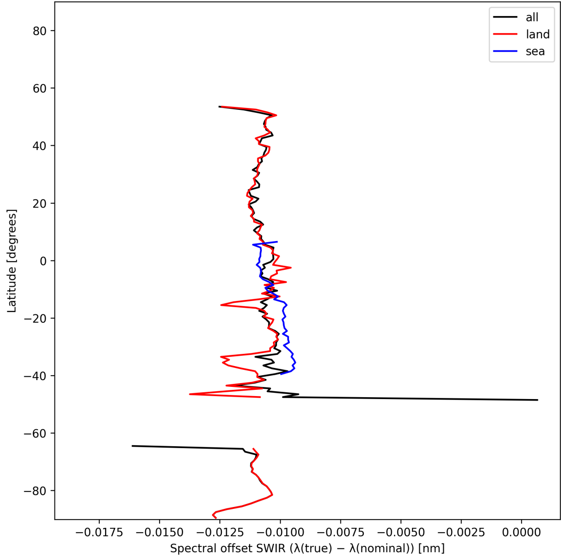
Figure 16: Zonal average of “Spectral offset SWIR ( \lambda_{\text{true}} - \lambda_{\text{nominal}} )” for 2024-11-30 to 2024-12-02.
