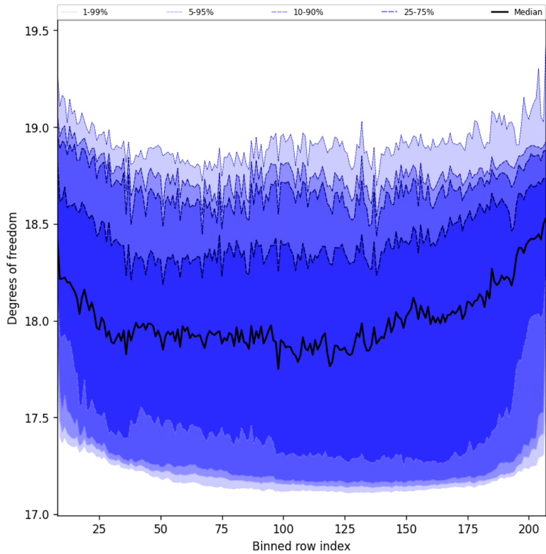
Figure 41: Along track statistics of “Degrees of freedom” for 2024-11-30 to 2024-12-02
