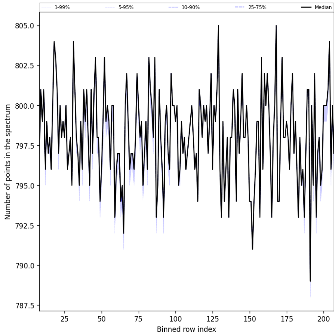
Figure 37: Along track statistics of “Number of points in the spectrum” for 2024-11-30 to 2024-12-02
