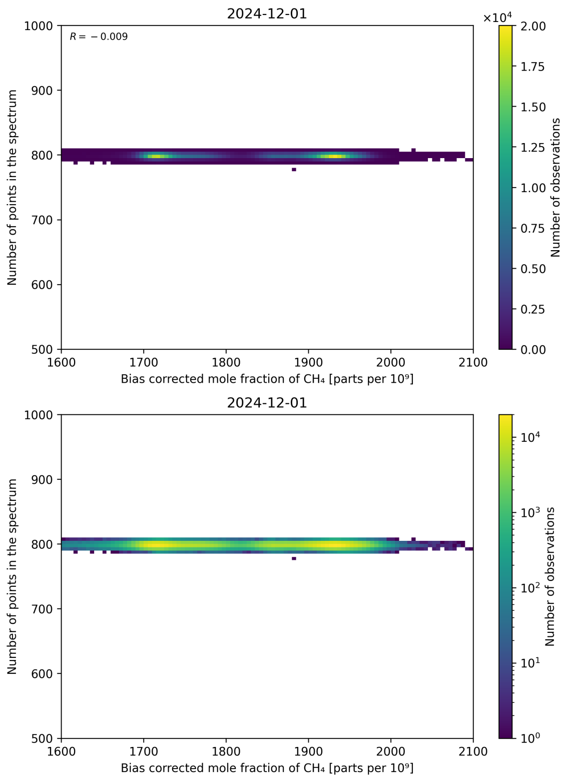
Figure 68: Scatter density plot of “Bias corrected mole fraction of CH 4 ” against “Number of points in the spectrum” for 2024-11-30 to 2024-12-02.
