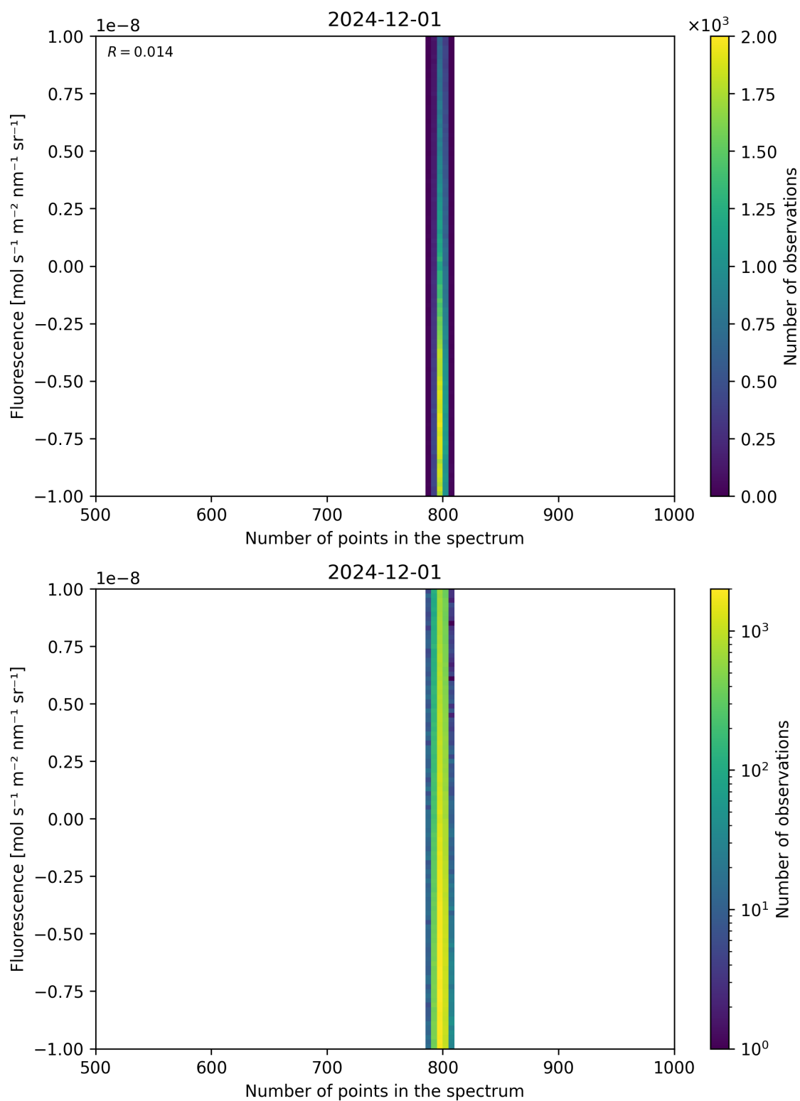
Figure 91: Scatter density plot of “Number of points in the spectrum” against “Fluorescence” for 2024-11-30 to 2024-12-02.
