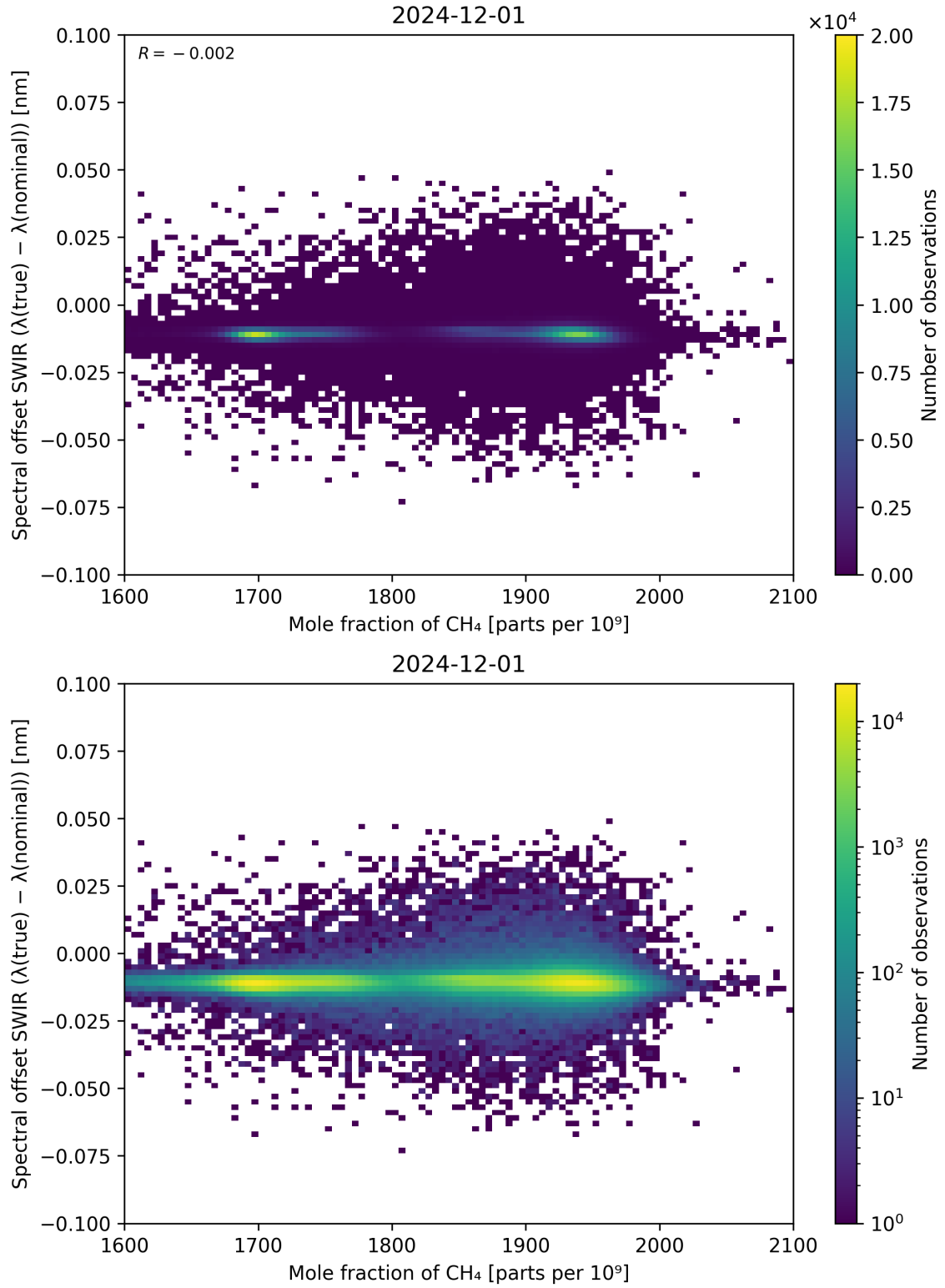
Figure 86: Scatter density plot of “Mole fraction of CH 4 ” against “Spectral offset SWIR ( \lambda_{\text{true}} - \lambda_{\text{nominal}} )” for 2024-11-30 to 2024-12-02.
