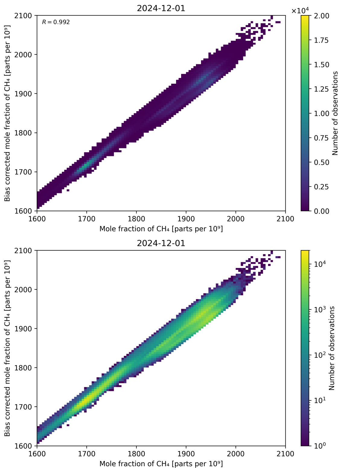
Figure 74: Scatter density plot of “Mole fraction of CH 4 ” against “Bias corrected mole fraction of CH 4 ” for 2024-11-30 to 2024-12-02.
