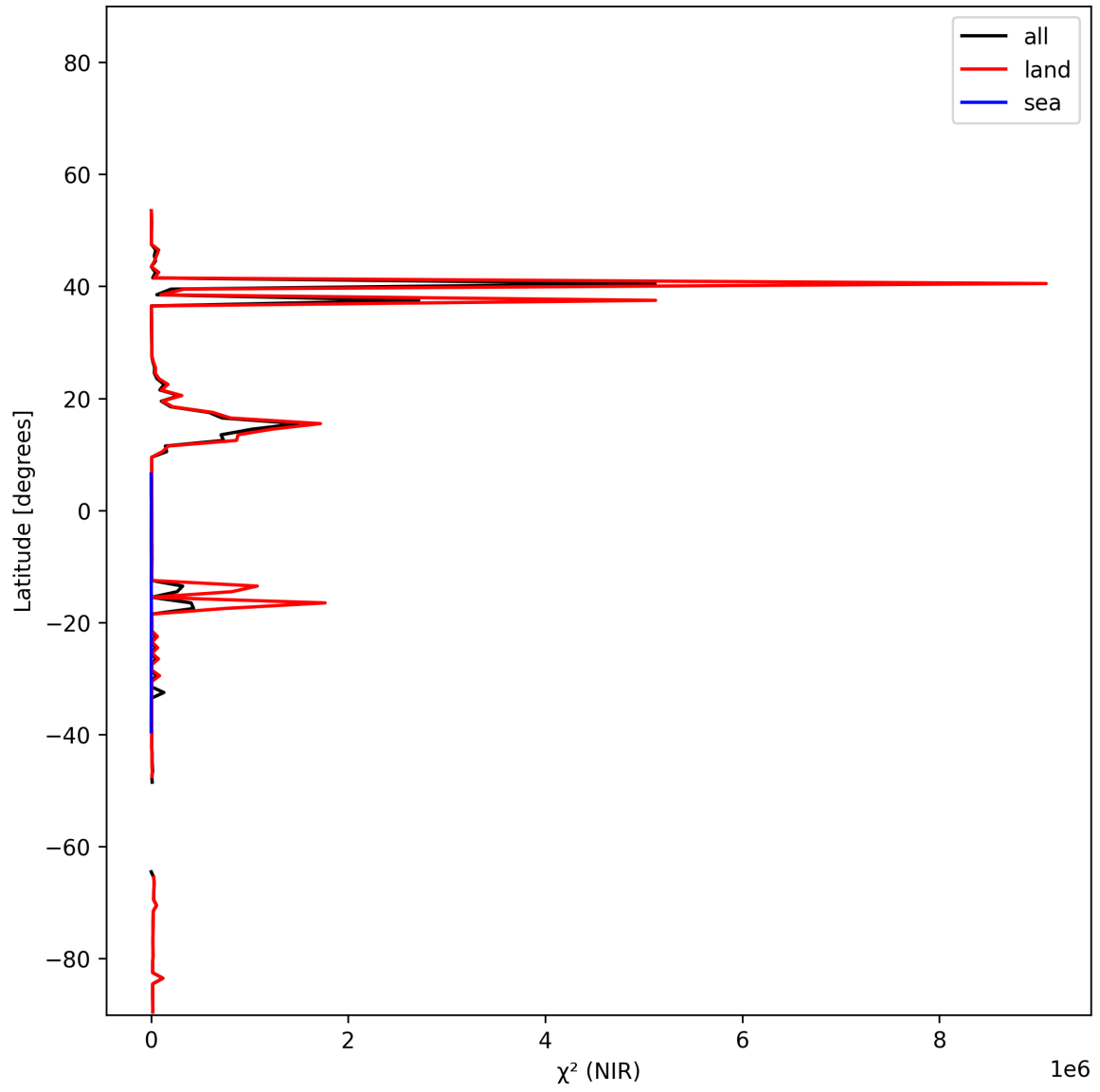
Figure 18: Zonal average of “ \chi^2 (NIR)” for 2024-11-30 to 2024-12-02.
