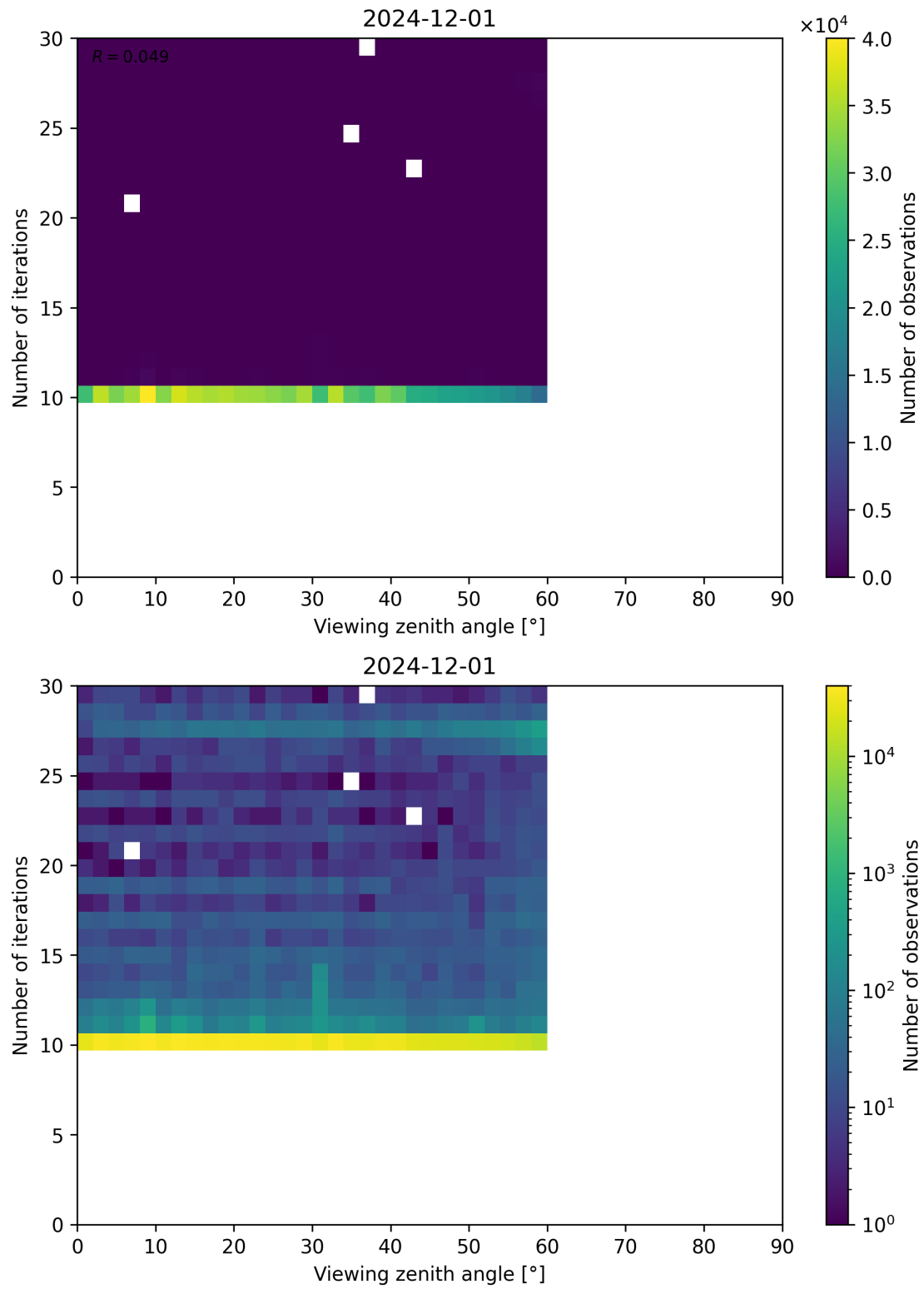
Figure 113: Scatter density plot of “Viewing zenith angle” against “Number of iterations” for 2024-11-30 to 2024-12-02.
