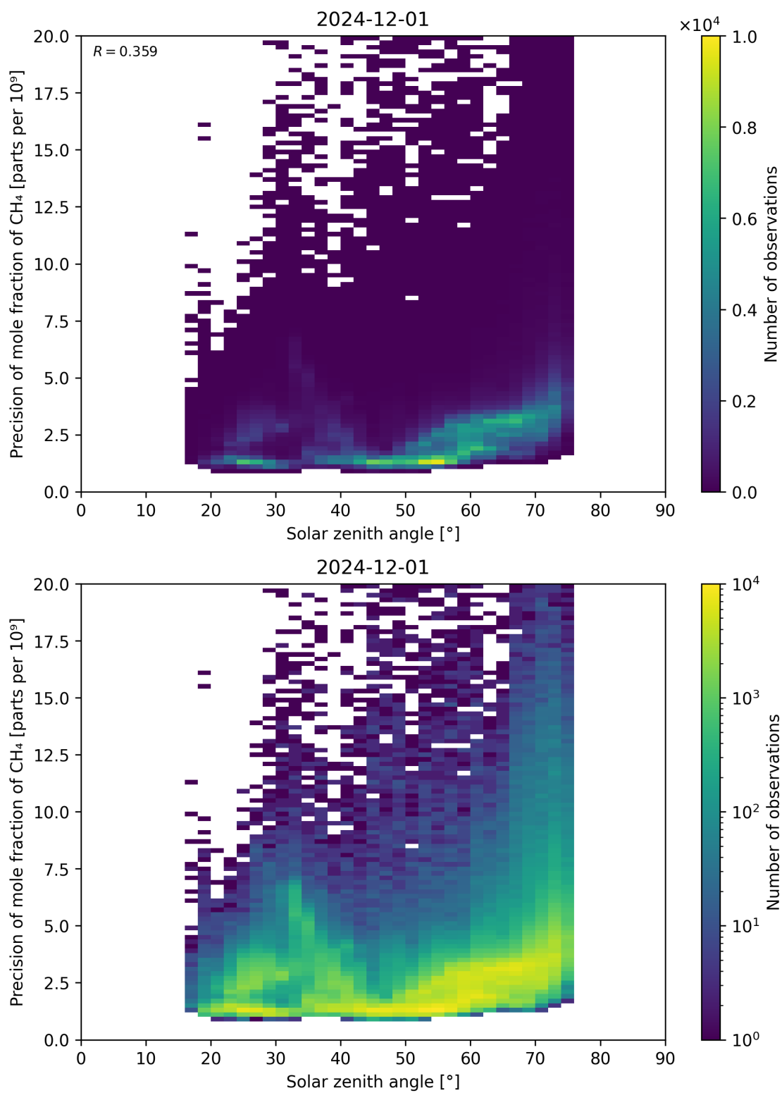
Figure 101: Scatter density plot of “Solar zenith angle” against “Precision of mole fraction of CH 4 ” for 2024-11-30 to 2024-12-02.
