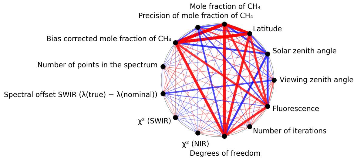
Figure 1: Map of correlation graph for 2024-11-30 to 2024-12-02.
