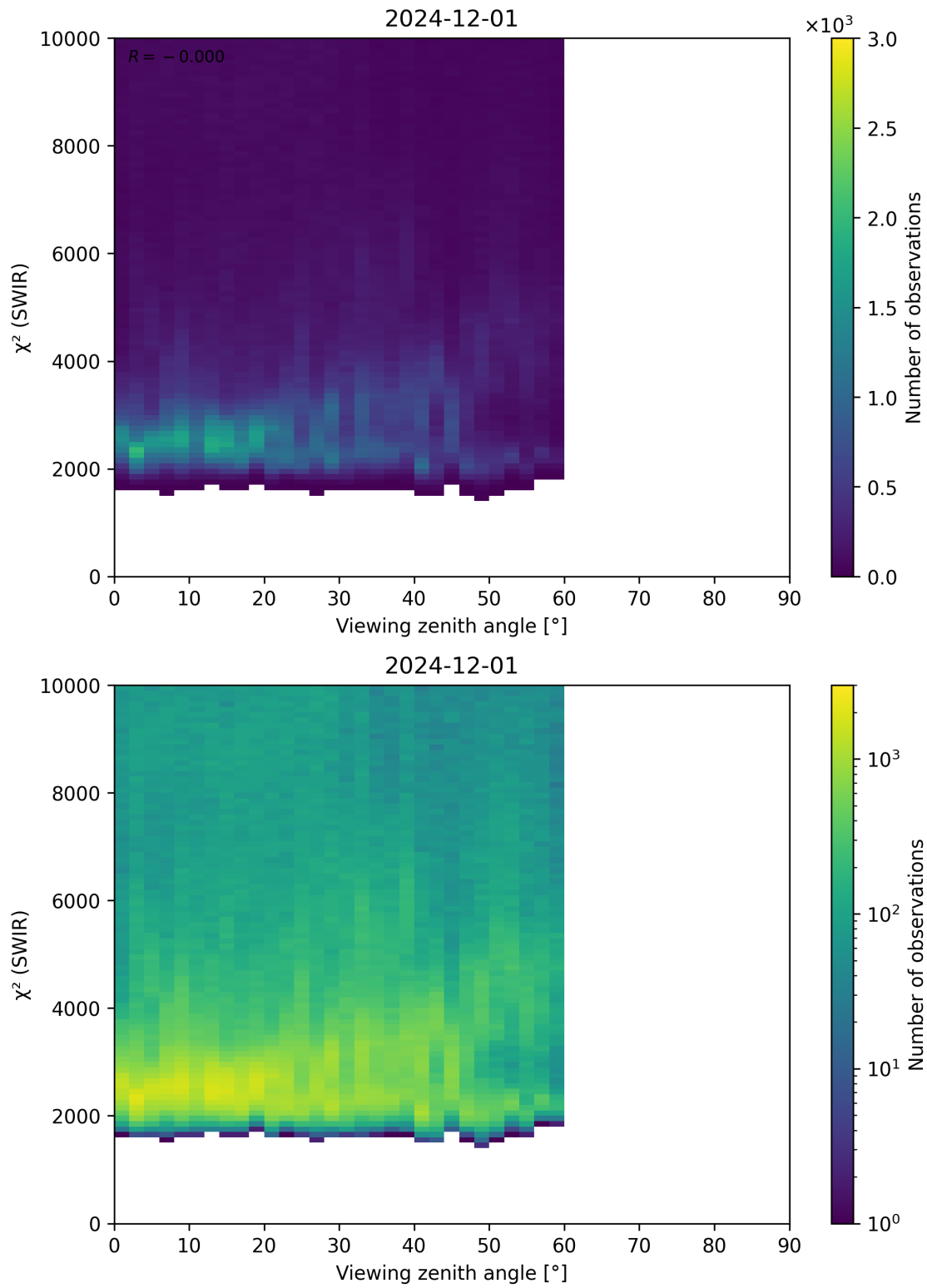
Figure 106: Scatter density plot of “Viewing zenith angle” against “ \chi^2 (SWIR)” for 2024-11-30 to 2024-12-02.
