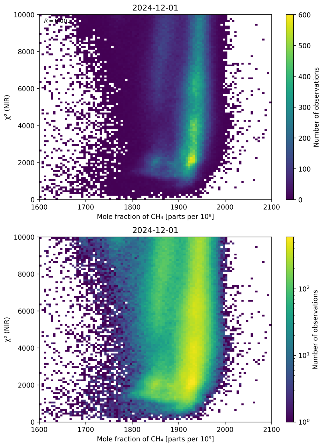
Figure 70: Scatter density plot of “Mole fraction of \text{CH}_4 ” against “ \chi^2 (NIR)” for 2024-11-30 to 2024-12-02.
