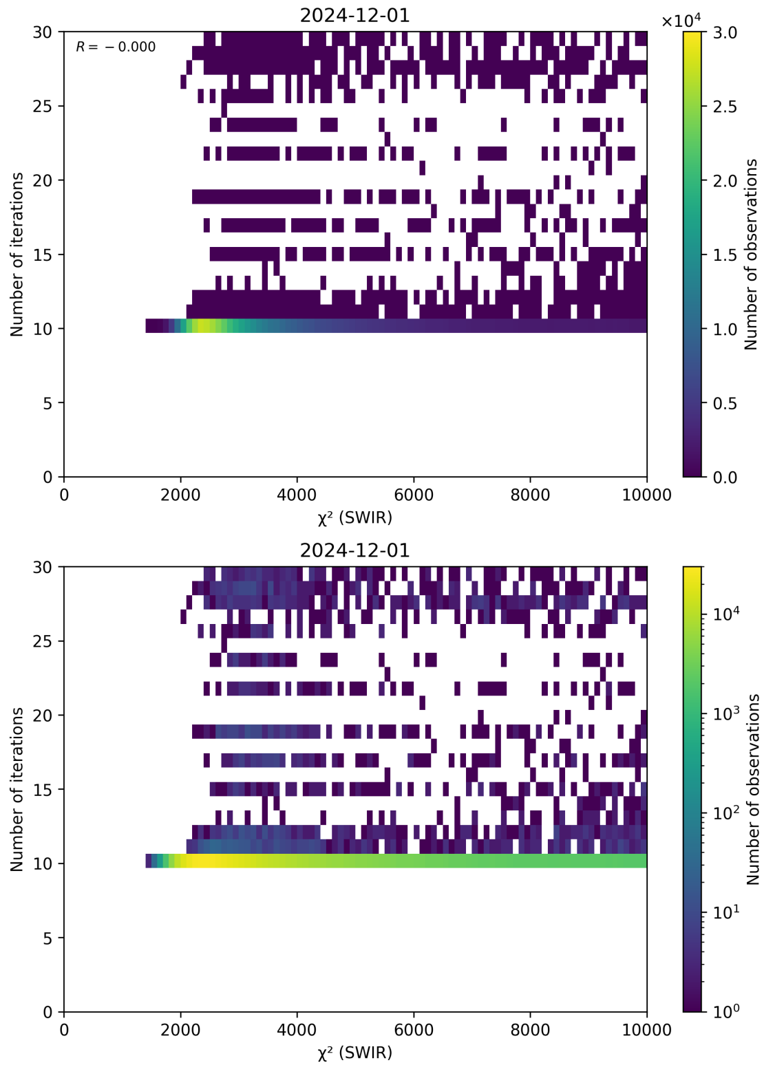
Figure 50: Scatter density plot of “ \chi^2 (SWIR)” against “Number of iterations” for 2024-11-30 to 2024-12-02.
