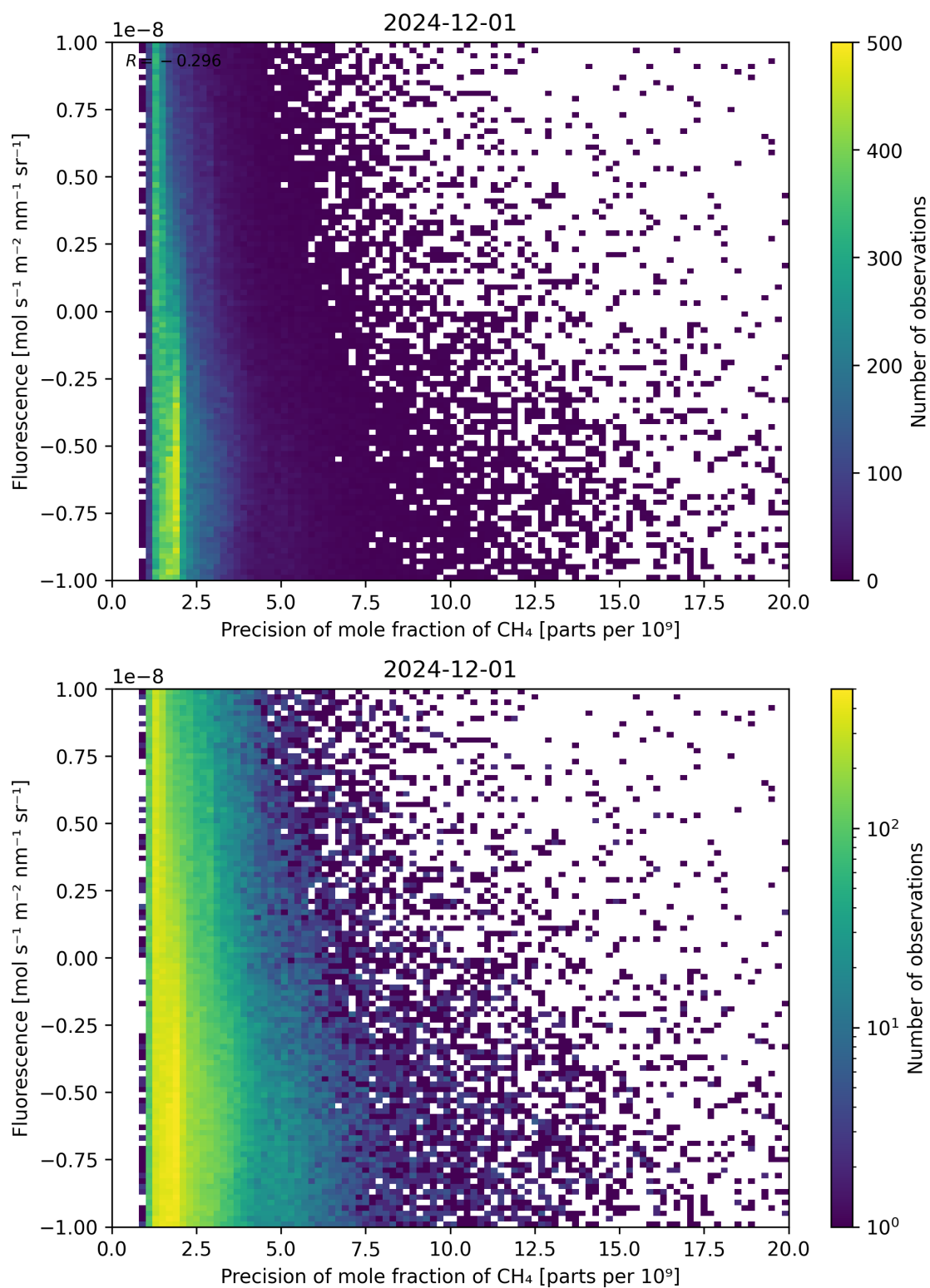
Figure 81: Scatter density plot of “Precision of mole fraction of \text{CH}_4 ” against “Fluorescence” for 2024-11-30 to 2024-12-02.
