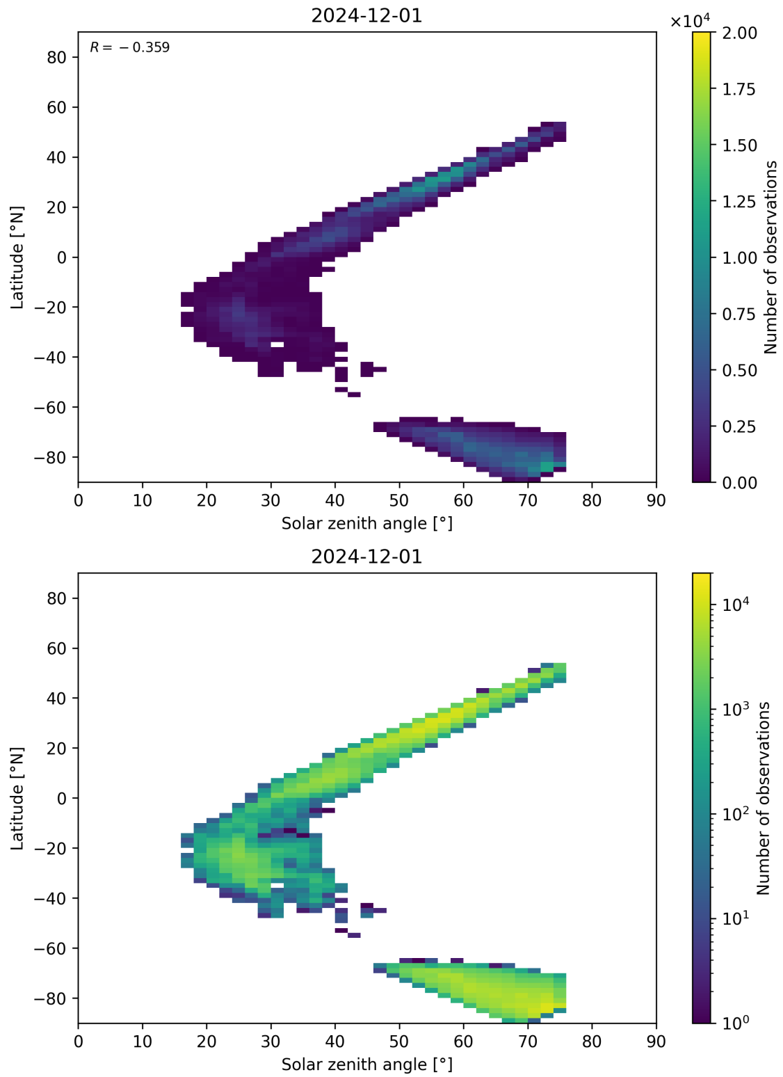
Figure 98: Scatter density plot of “Solar zenith angle” against “Latitude” for 2024-11-30 to 2024-12-02.
