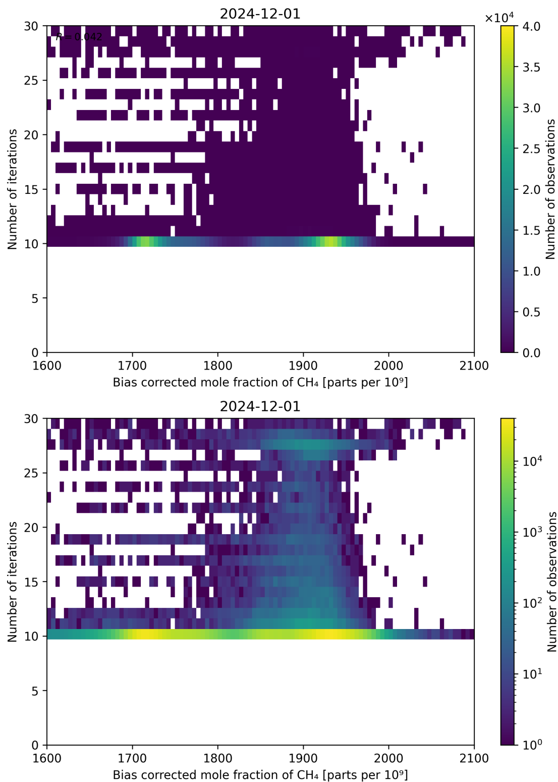
Figure 67: Scatter density plot of “Bias corrected mole fraction of CH 4 ” against “Number of iterations” for 2024-11-30 to 2024-12-02.
