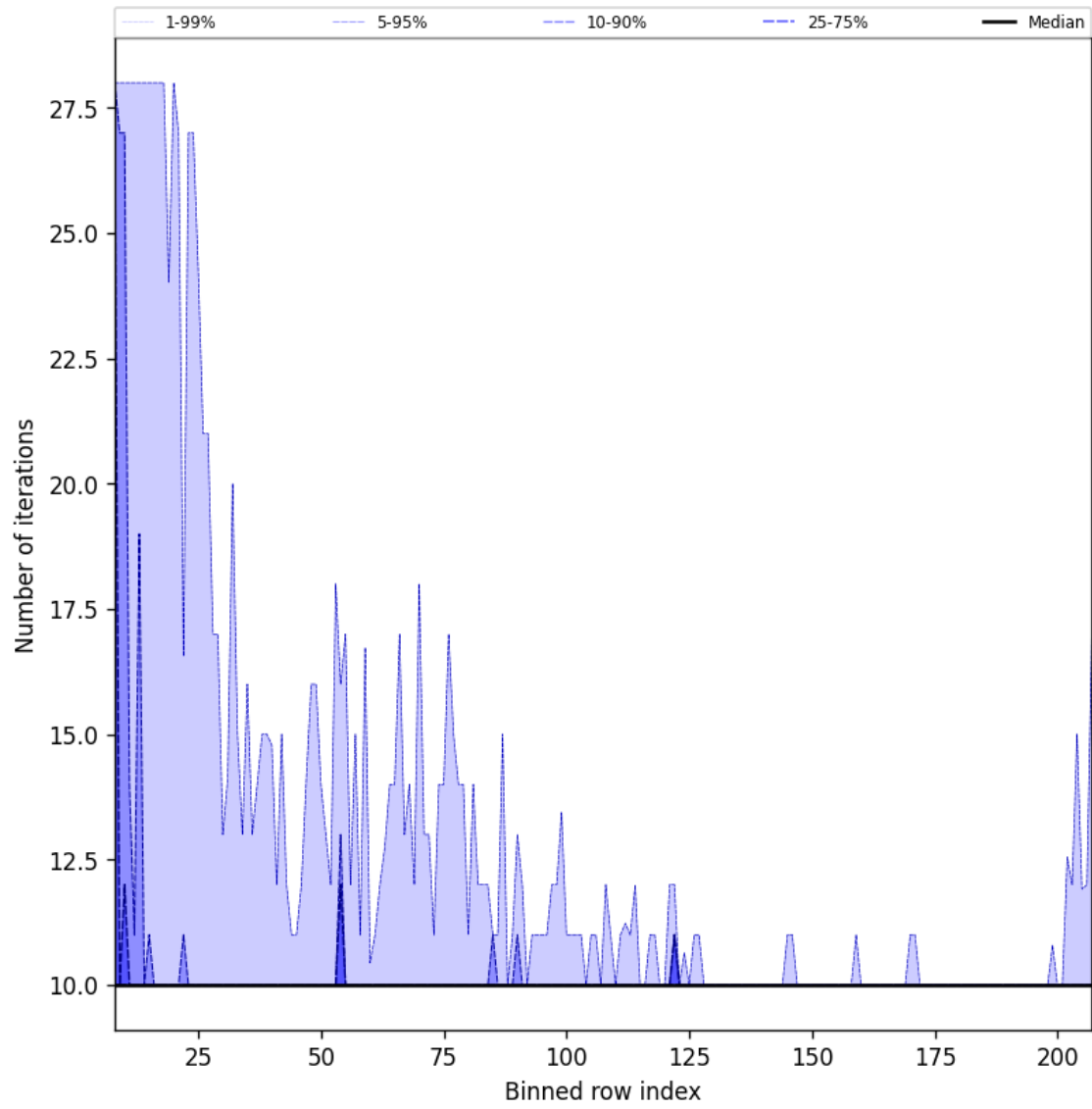
Figure 42: Along track statistics of “Number of iterations” for 2024-11-30 to 2024-12-02
