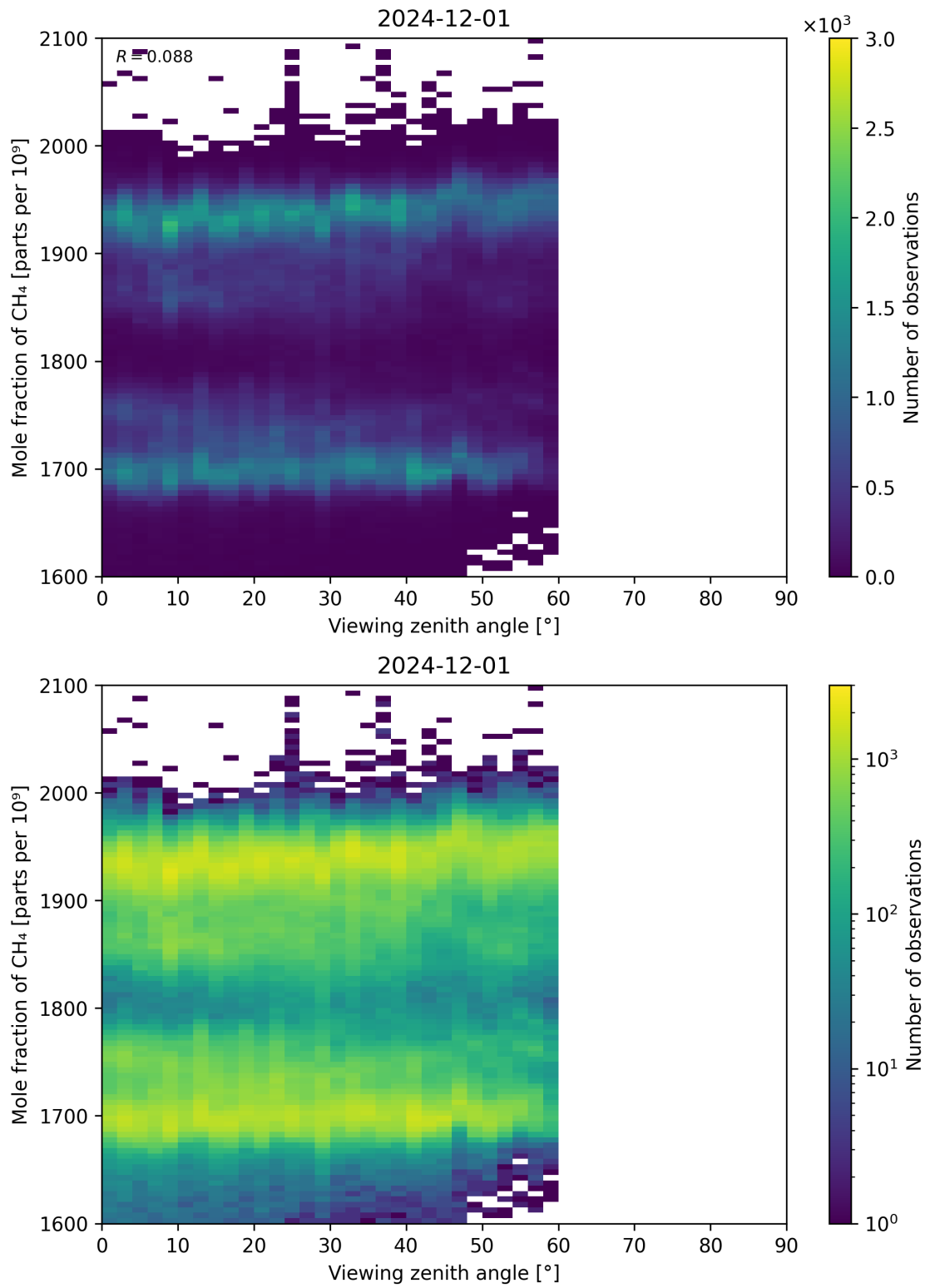
Figure 110: Scatter density plot of “Viewing zenith angle” against “Mole fraction of CH 4 ” for 2024-11-30 to 2024-12-02.
