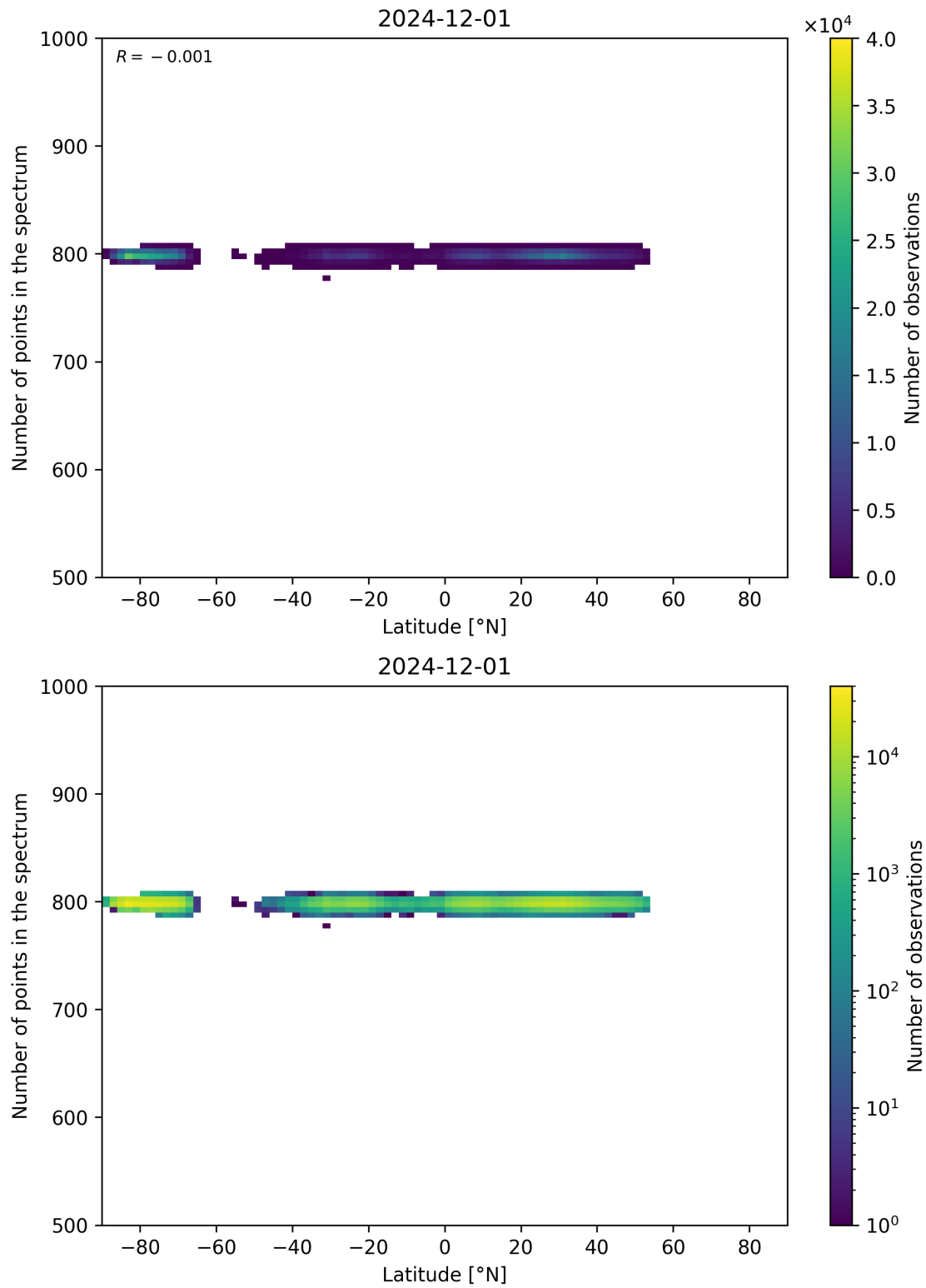
Figure 61: Scatter density plot of “Latitude” against “Number of points in the spectrum” for 2024-11-30 to 2024-12-02.
