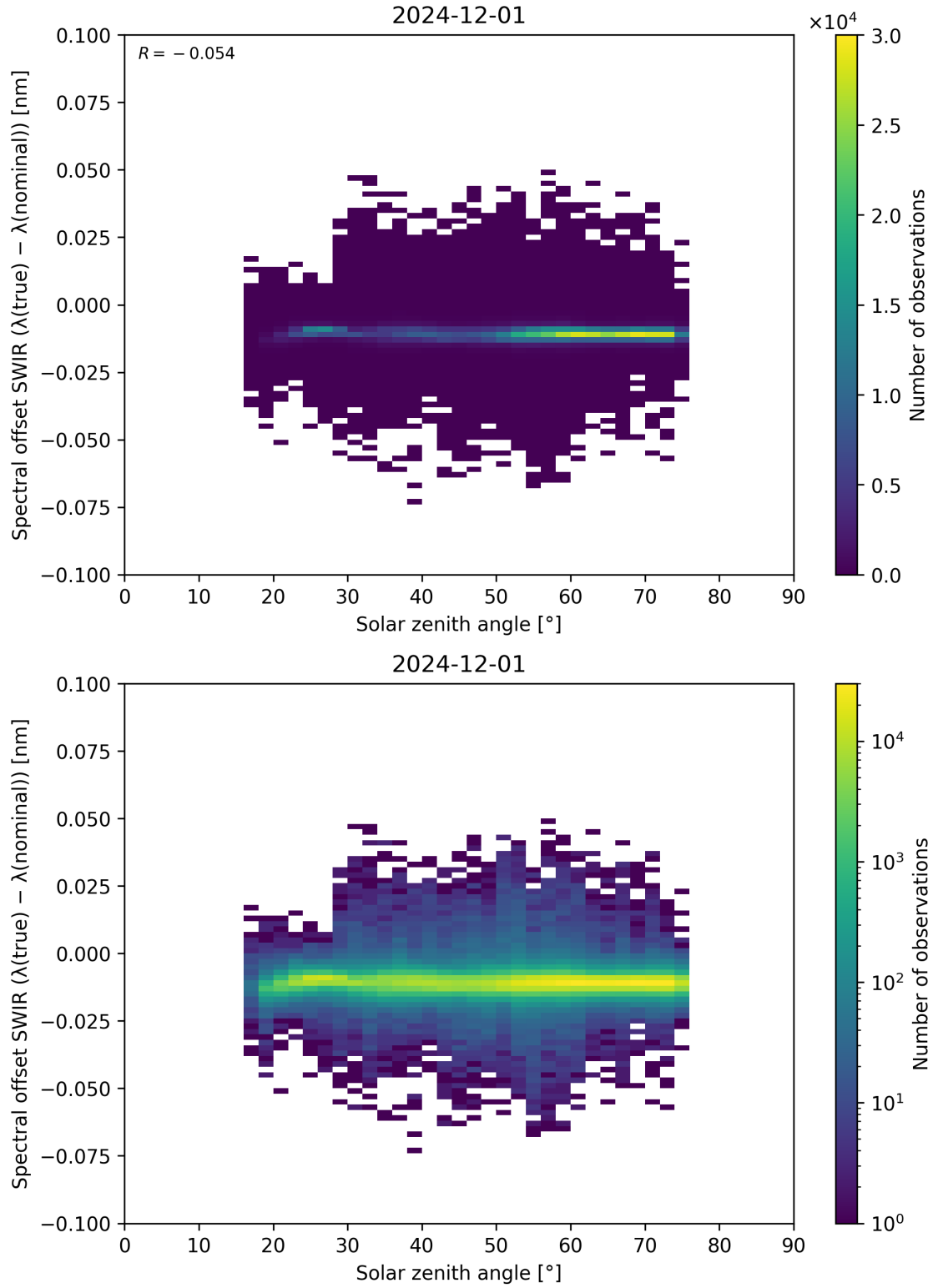
Figure 104: Scatter density plot of “Solar zenith angle” against “Spectral offset SWIR ( \lambda_{\text{true}} - \lambda_{\text{nominal}} )” for 2024-11-30 to 2024-12-02.
