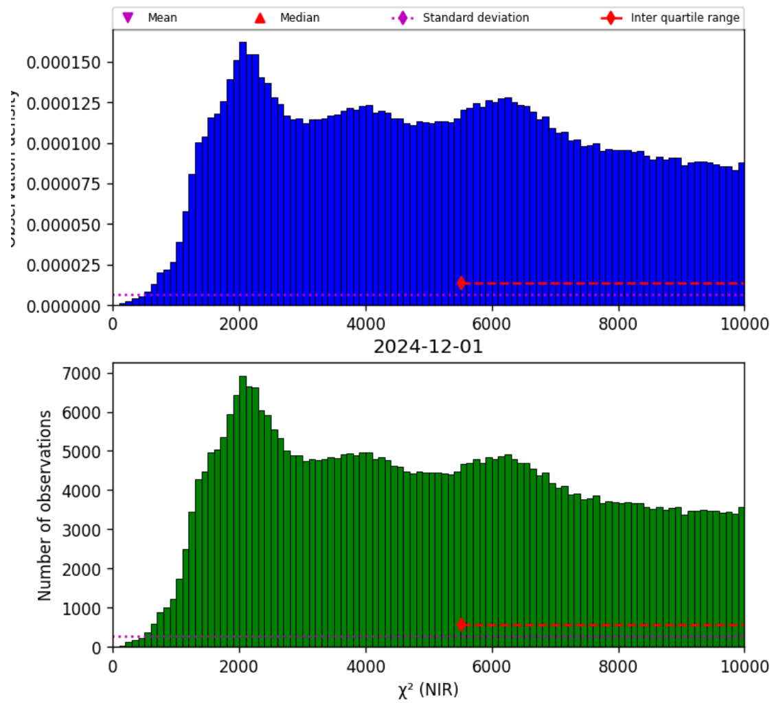
Figure 29: Histogram of “ \chi^2 (NIR)” for 2024-11-30 to 2024-12-02
