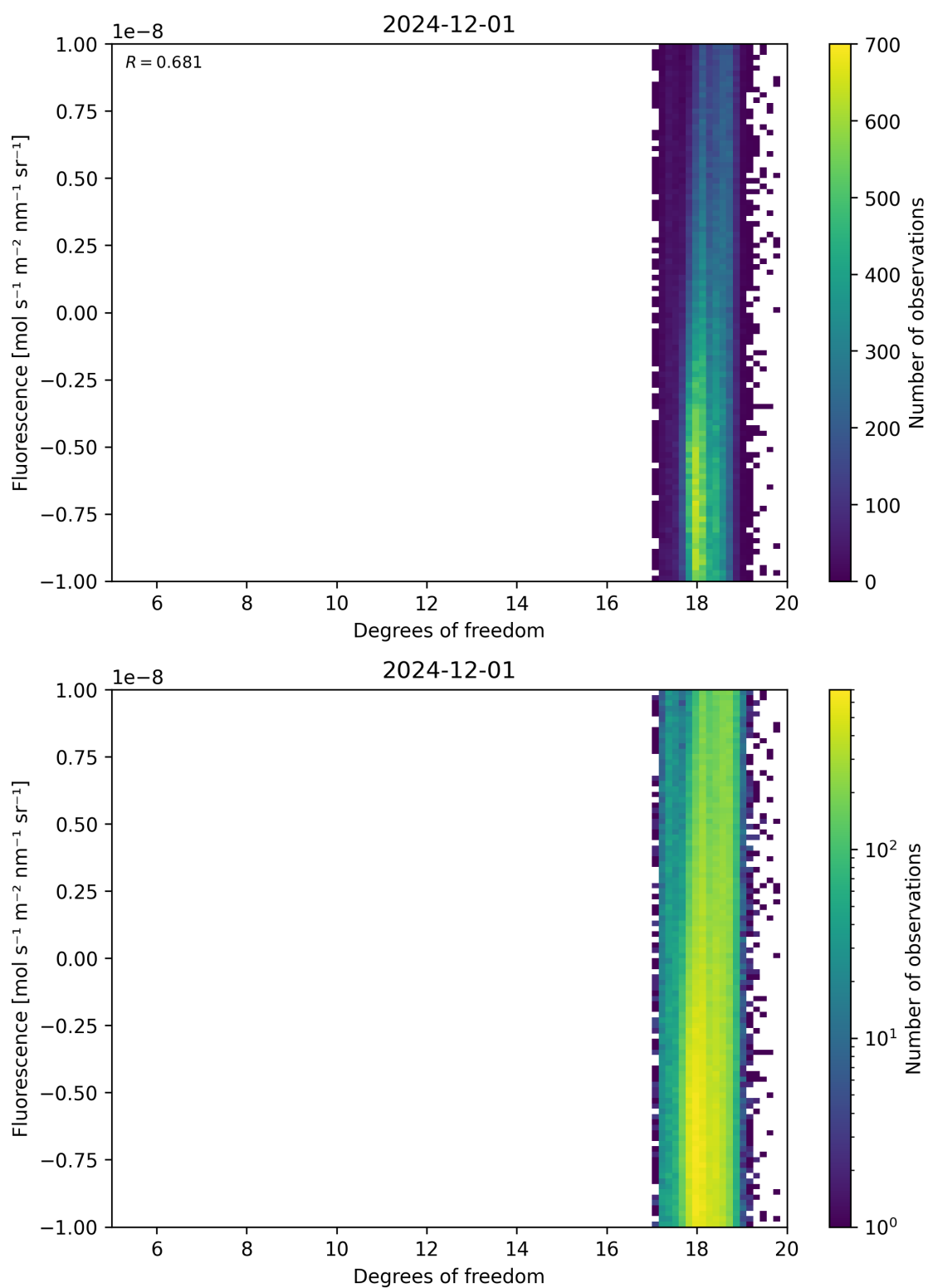
Figure 51: Scatter density plot of “Degrees of freedom” against “Fluorescence” for 2024-11-30 to 2024-12-02.
