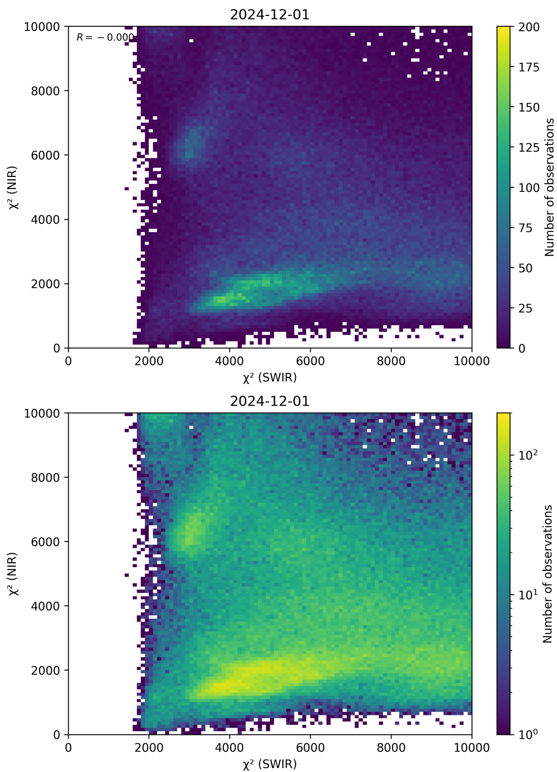
Figure 47: Scatter density plot of “ \chi^2 (SWIR)” against “ \chi^2 (NIR)” for 2024-11-30 to 2024-12-02.
