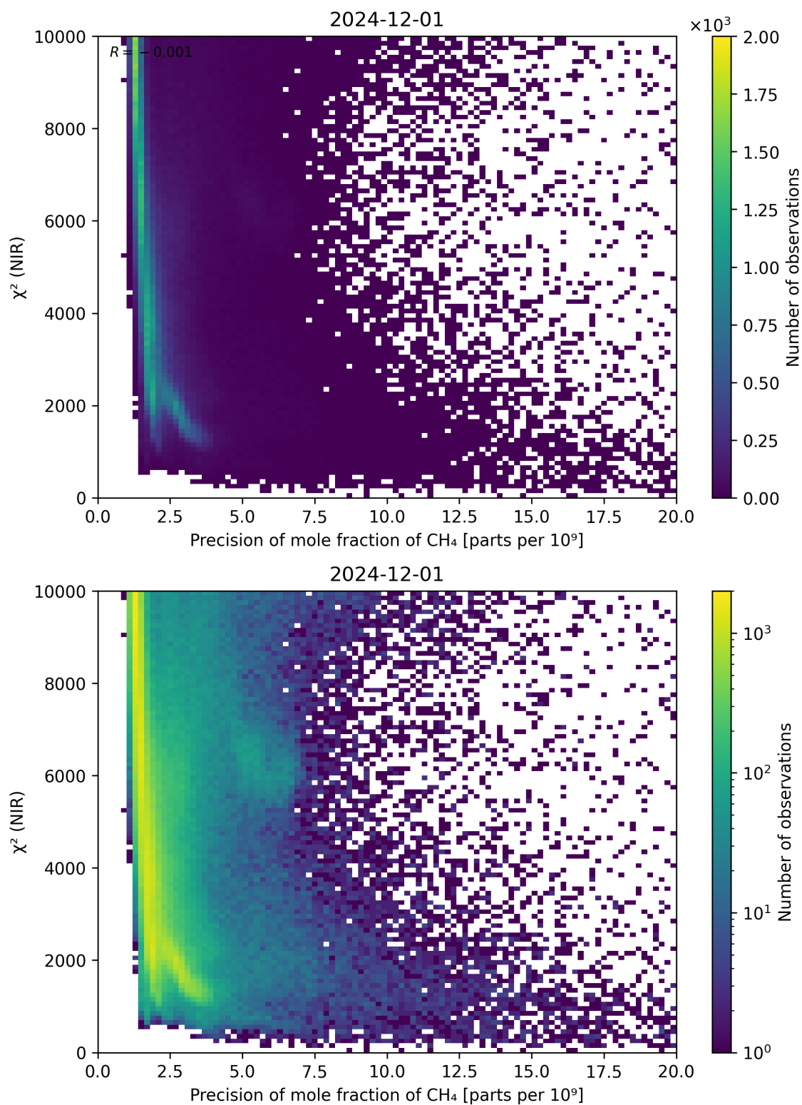
Figure 78: Scatter density plot of “Precision of mole fraction of \text{CH}_4 ” against “ \chi^2 (NIR)” for 2024-11-30 to 2024-12-02.
