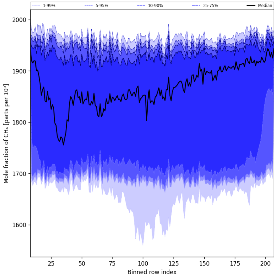
Figure 34: Along track statistics of “Mole fraction of CH 4 ” for 2024-11-30 to 2024-12-02
