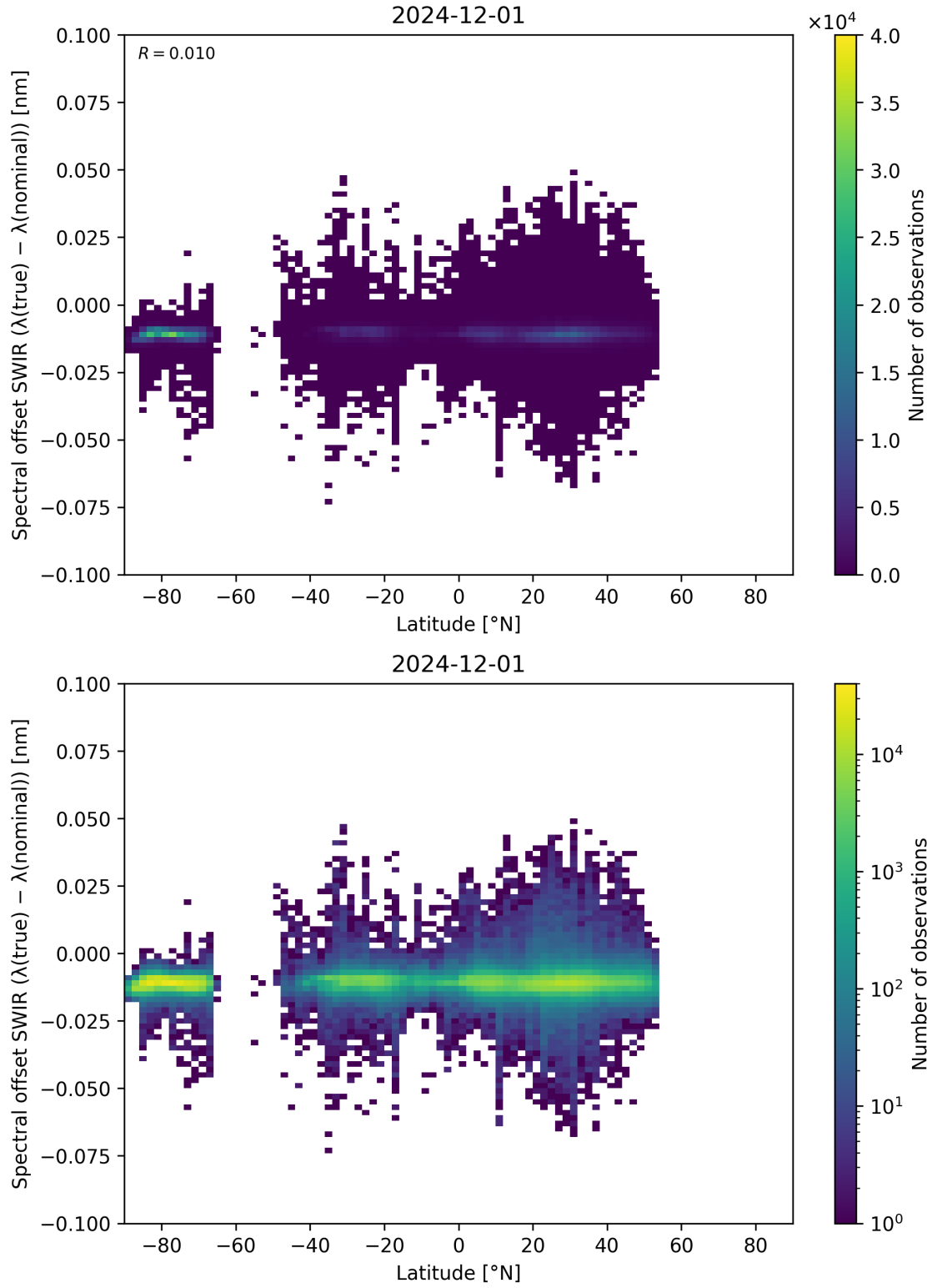
Figure 62: Scatter density plot of “Latitude” against “Spectral offset SWIR ( \lambda_{\text{true}} - \lambda_{\text{nominal}} )” for 2024-11-30 to 2024-12-02.
