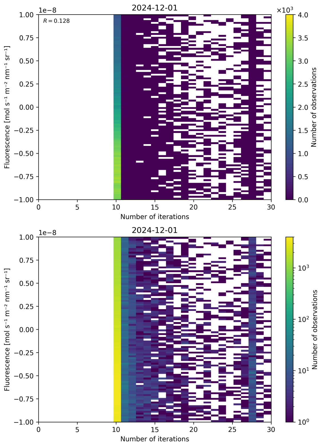
Figure 87: Scatter density plot of “Number of iterations” against “Fluorescence” for 2024-11-30 to 2024-12-02.
