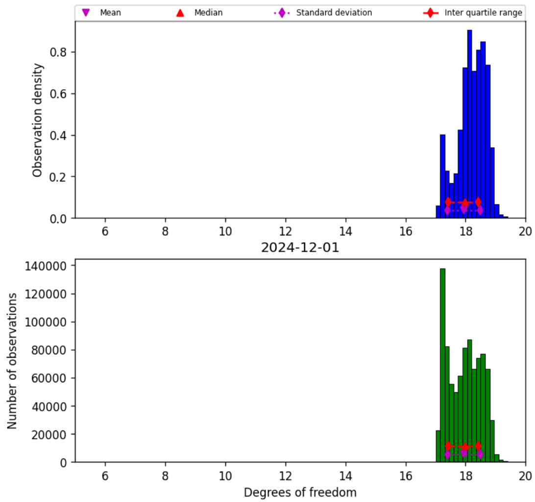
Figure 30: Histogram of “Degrees of freedom” for 2024-11-30 to 2024-12-02
