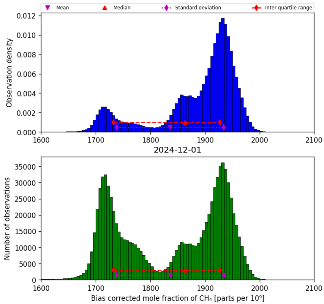
Figure 25: Histogram of “Bias corrected mole fraction of CH 4 ” for 2024-11-30 to 2024-12-02
