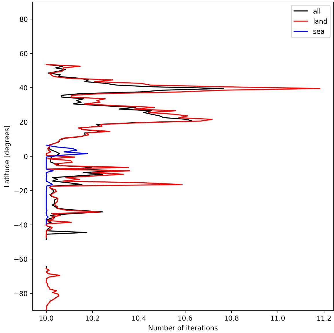
Figure 20: Zonal average of “Number of iterations” for 2024-11-30 to 2024-12-02.
