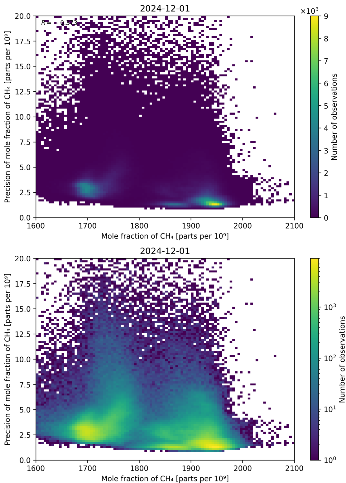
Figure 75: Scatter density plot of “Mole fraction of CH 4 ” against “Precision of mole fraction of CH 4 ” for 2024-11-30 to 2024-12-02.
