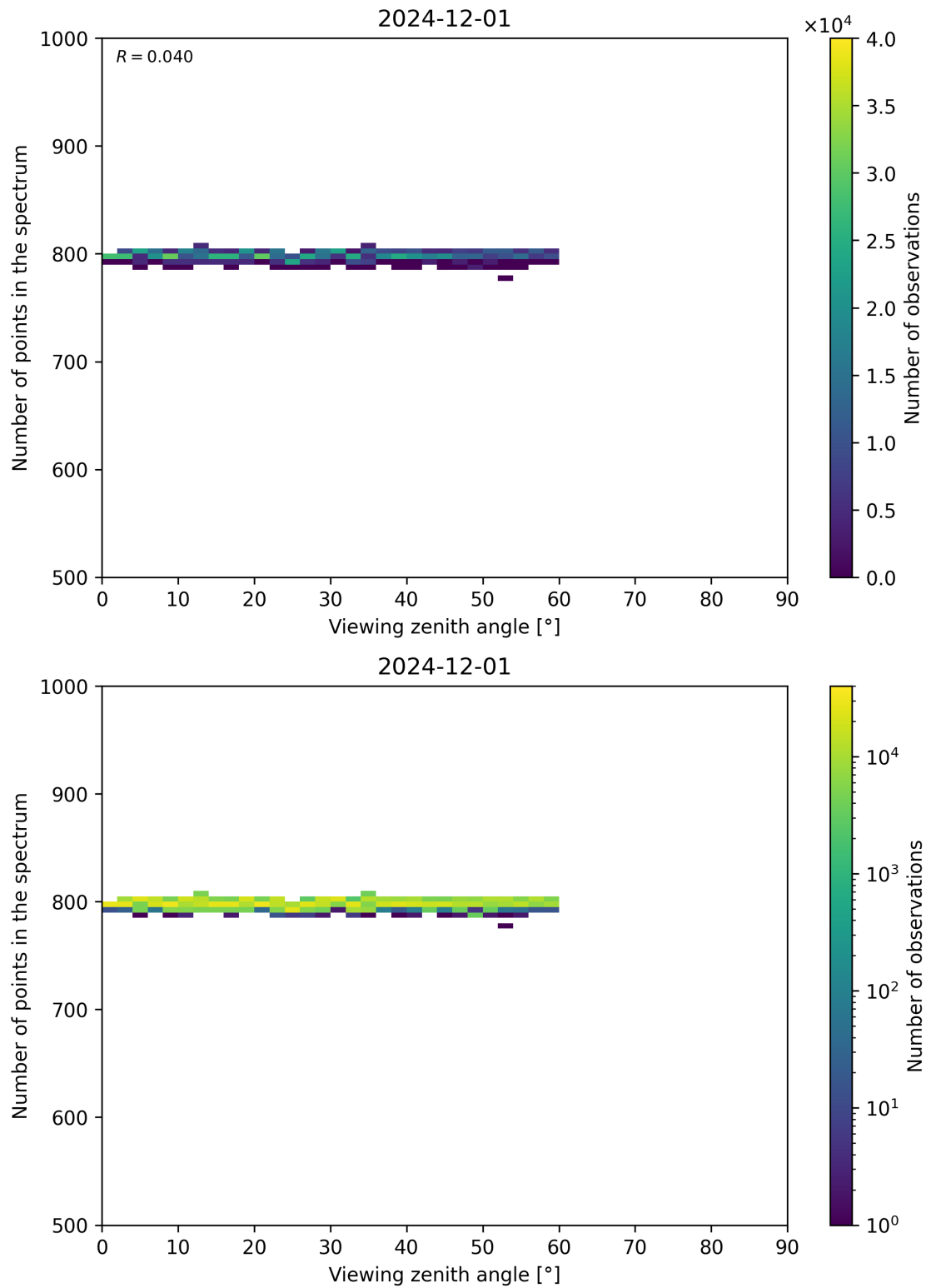
Figure 114: Scatter density plot of “Viewing zenith angle” against “Number of points in the spectrum” for 2024-11-30 to 2024-12-02.
