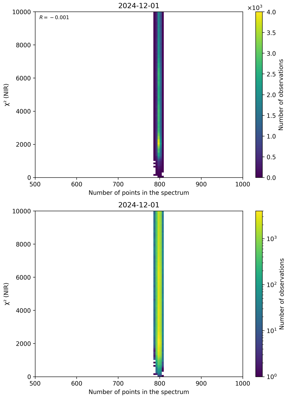
Figure 88: Scatter density plot of “Number of points in the spectrum” against “ \chi^2 (NIR)” for 2024-11-30 to 2024-12-02.
