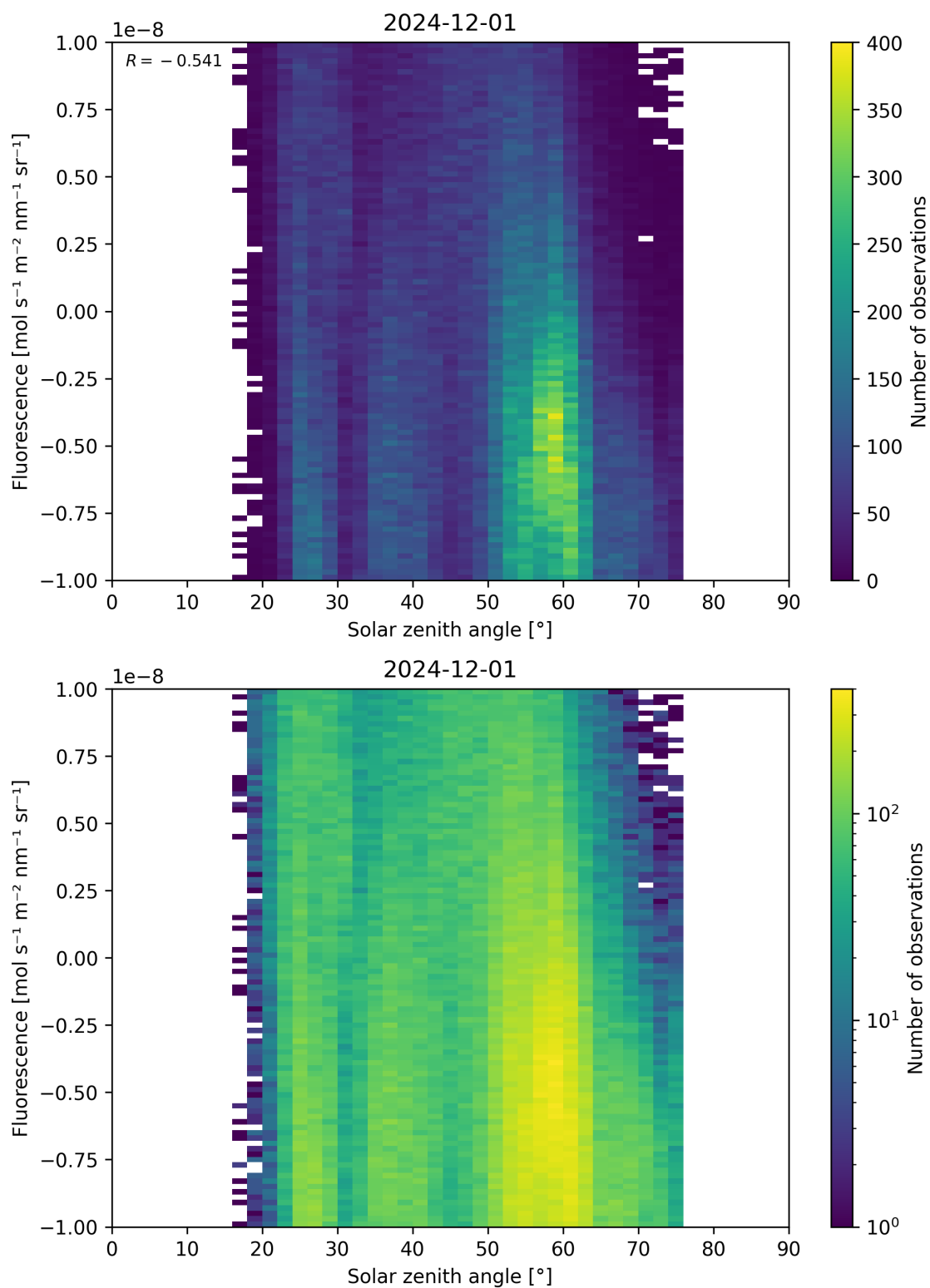
Figure 97: Scatter density plot of “Solar zenith angle” against “Fluorescence” for 2024-11-30 to 2024-12-02.
