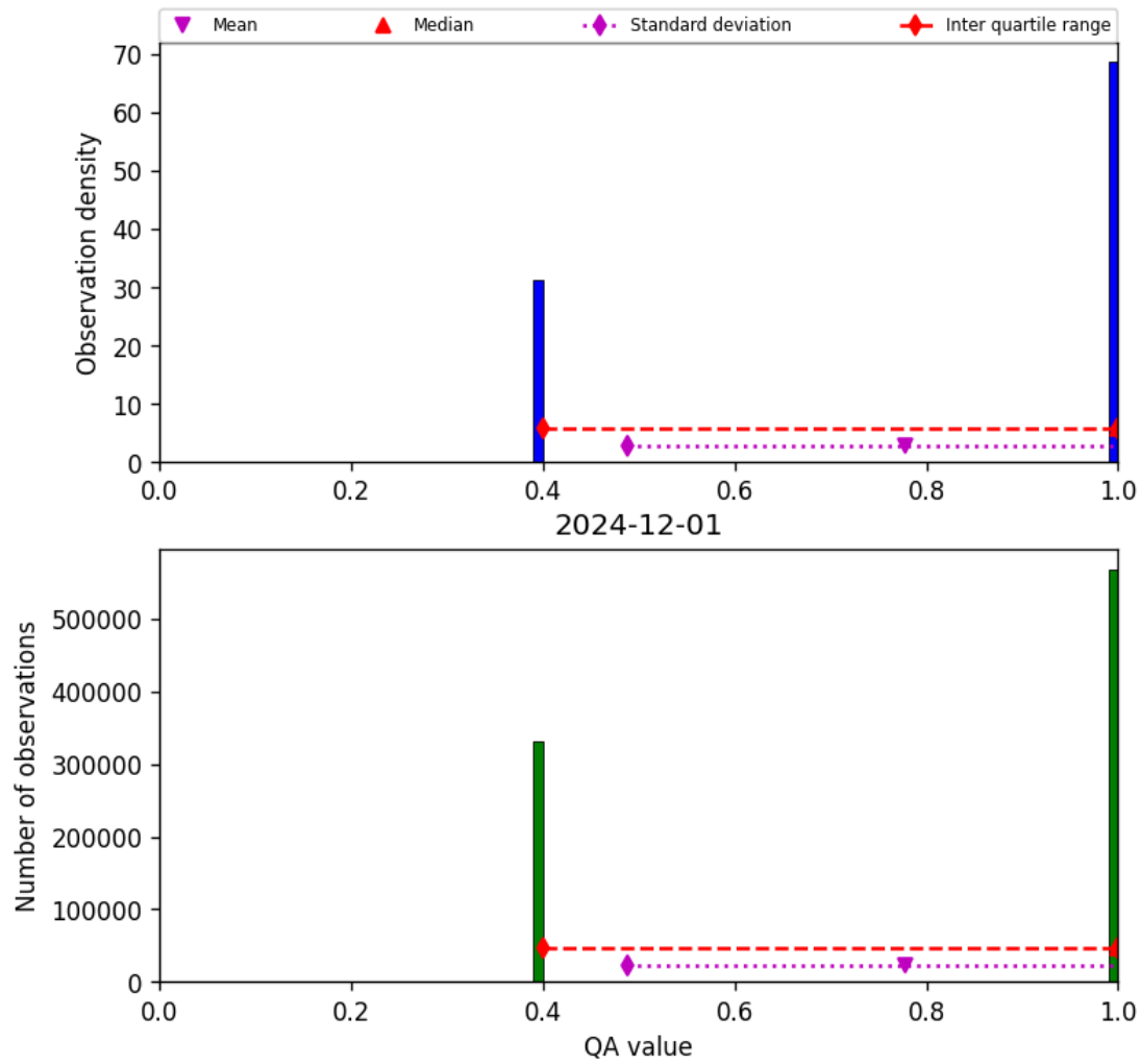
Figure 22: Histogram of “QA value” for 2024-11-30 to 2024-12-02
