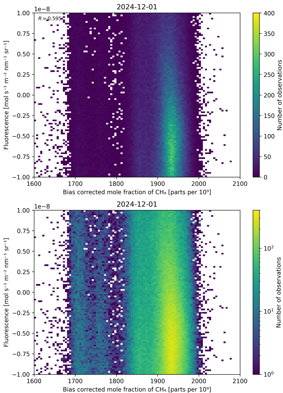
Figure 66: Scatter density plot of “Bias corrected mole fraction of \text{CH}_4 ” against “Fluorescence” for 2024-11-30 to 2024-12-02.
