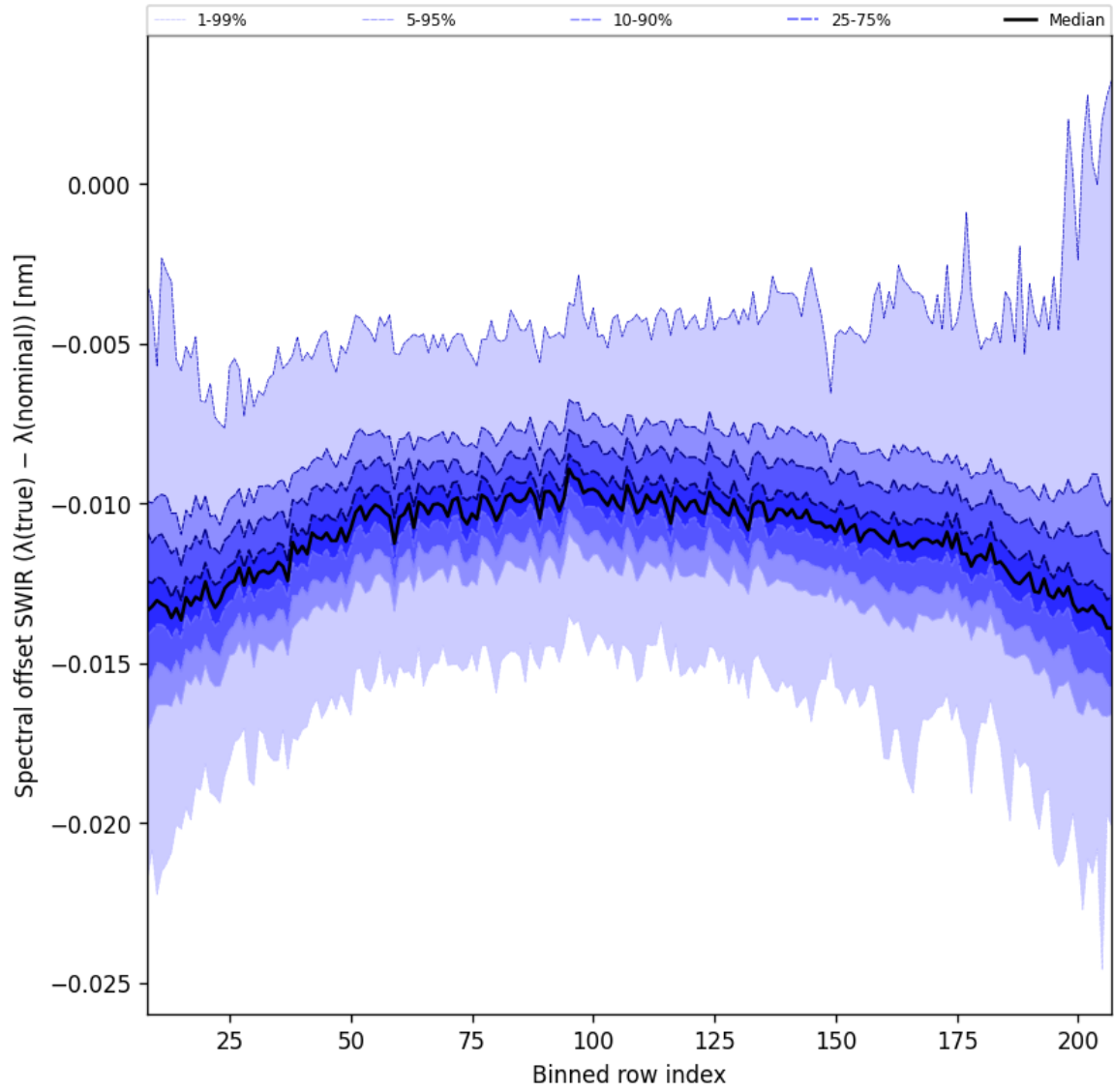
Figure 38: Along track statistics of “Spectral offset SWIR ( \lambda_{\text{true}} - \lambda_{\text{nominal}} )” for 2024-11-30 to 2024-12-02
