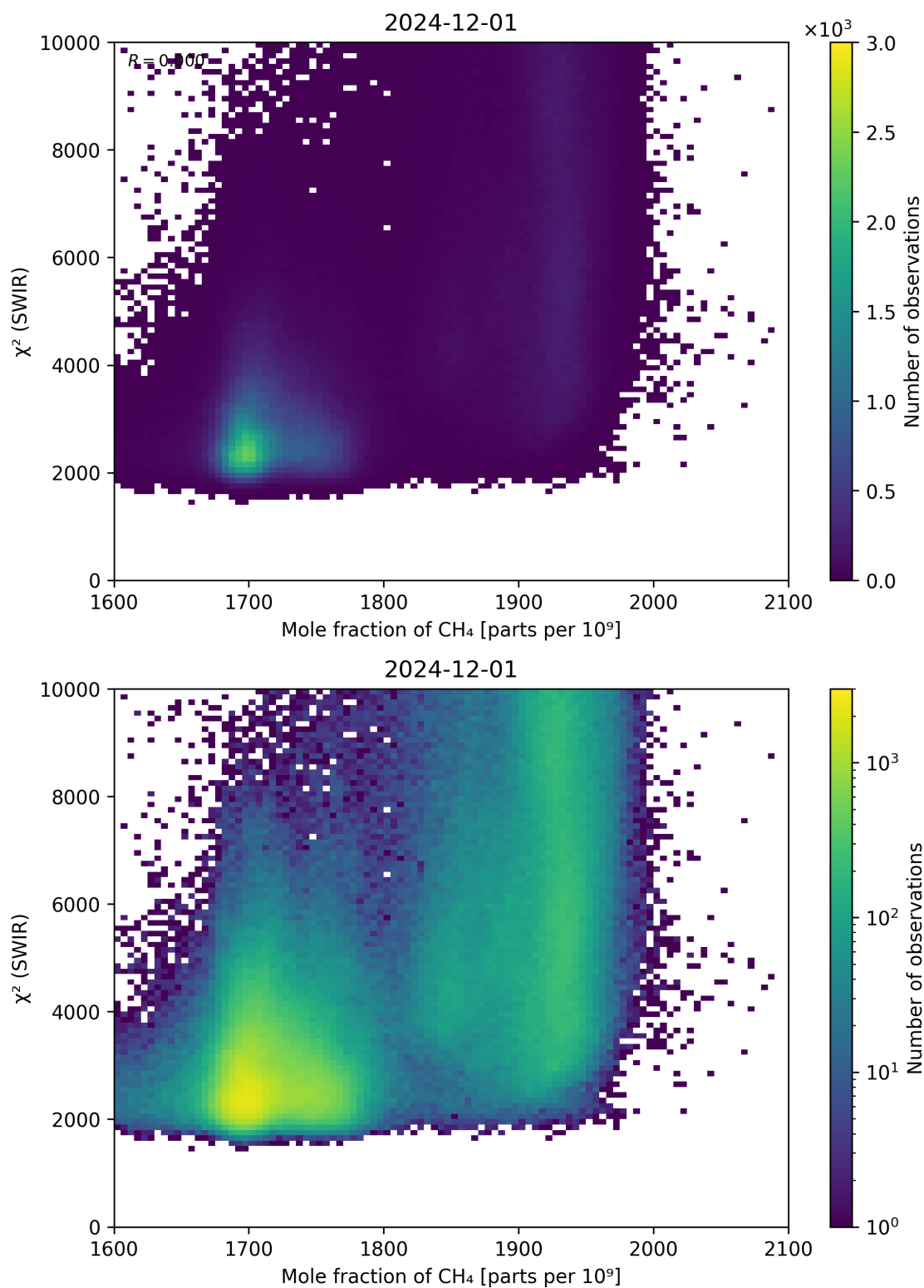
Figure 71: Scatter density plot of “Mole fraction of CH 4 ” against “ \chi^2 (SWIR)” for 2024-11-30 to 2024-12-02.
