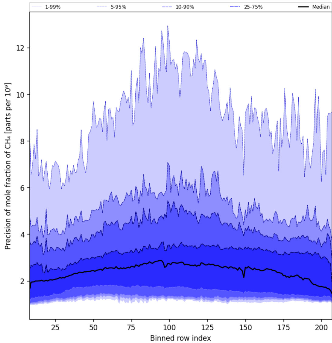
Figure 35: Along track statistics of “Precision of mole fraction of CH 4 ” for 2024-11-30 to 2024-12-02
