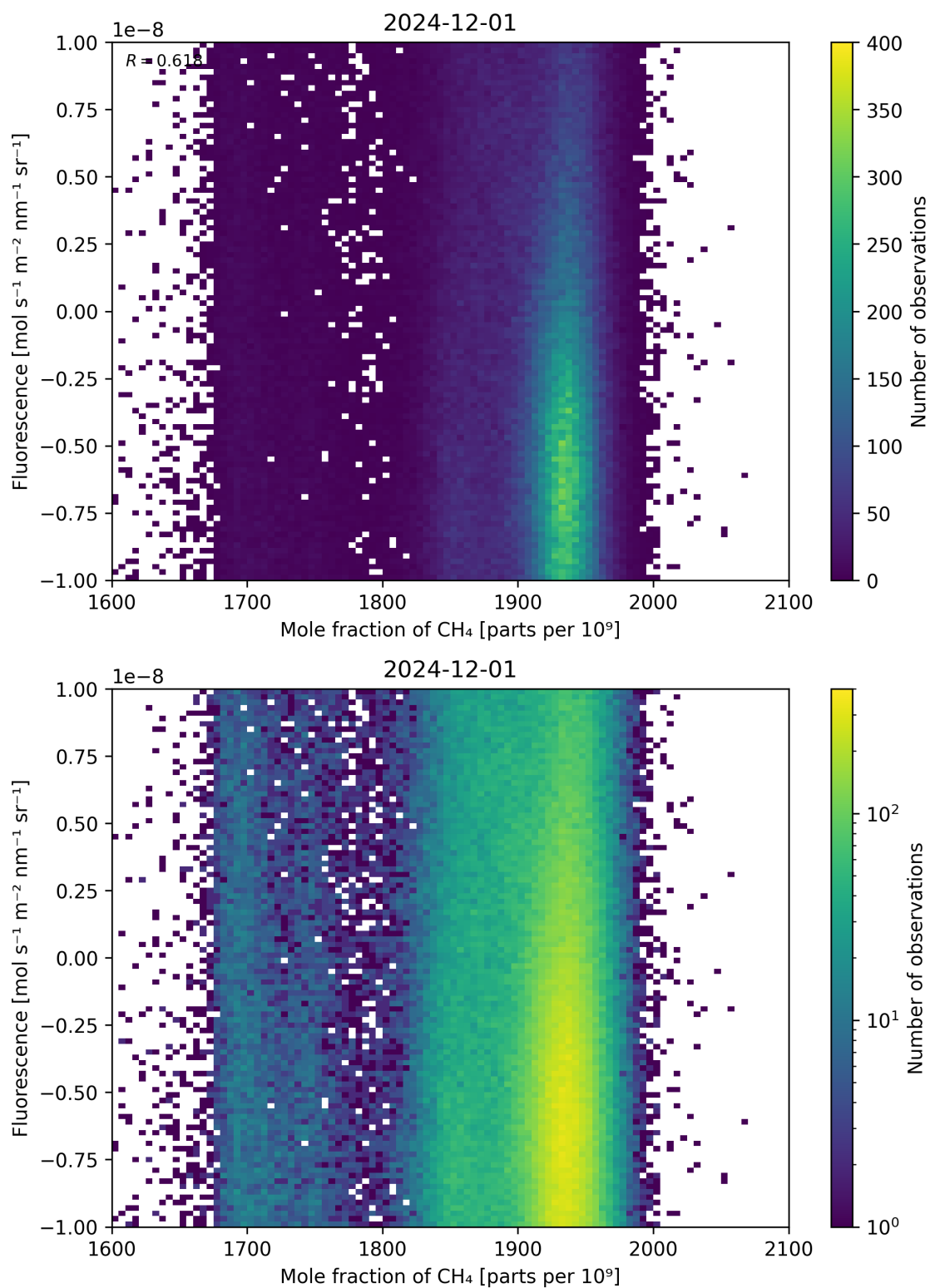
Figure 73: Scatter density plot of “Mole fraction of CH 4 ” against “Fluorescence” for 2024-11-30 to 2024-12-02.
