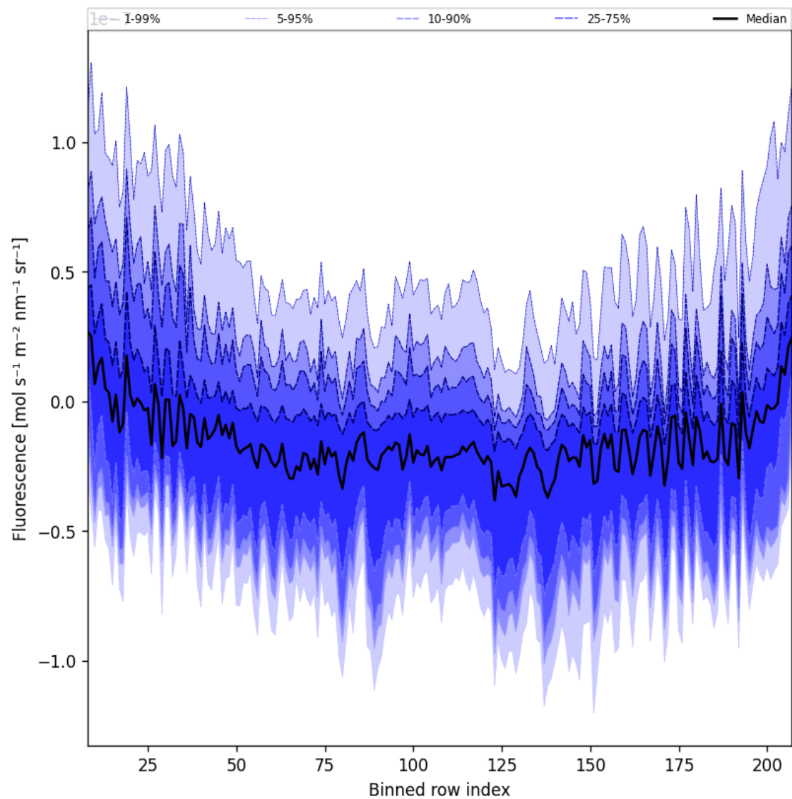
Figure 43: Along track statistics of “Fluorescence” for 2024-11-30 to 2024-12-02
