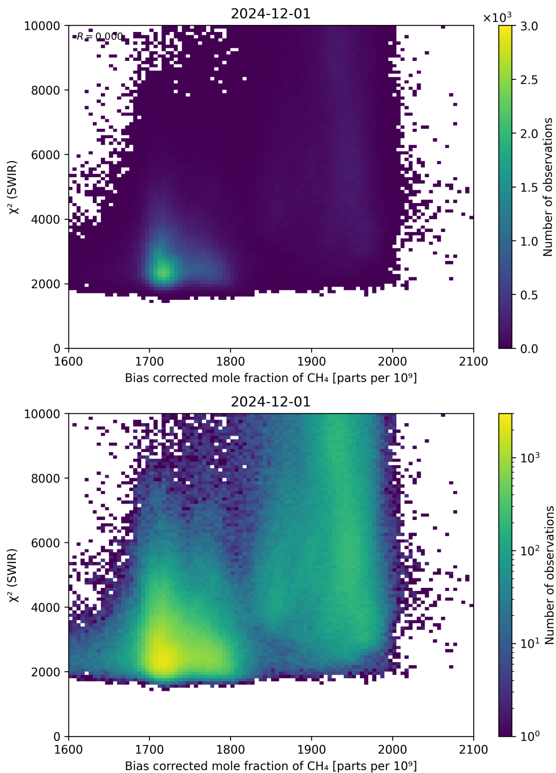
Figure 64: Scatter density plot of “Bias corrected mole fraction of \text{CH}_4 ” against “ \chi^2 (SWIR)” for 2024-11-30 to 2024-12-02.
