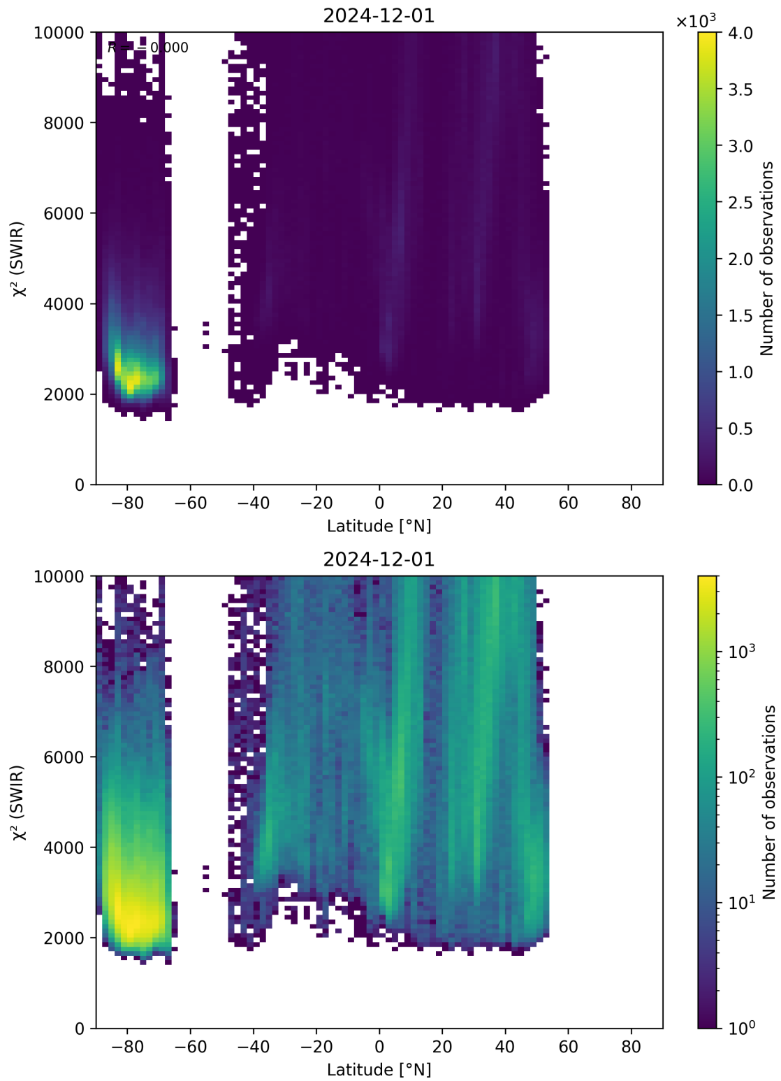
Figure 54: Scatter density plot of “Latitude” against “ \chi^2 (SWIR)” for 2024-11-30 to 2024-12-02.
