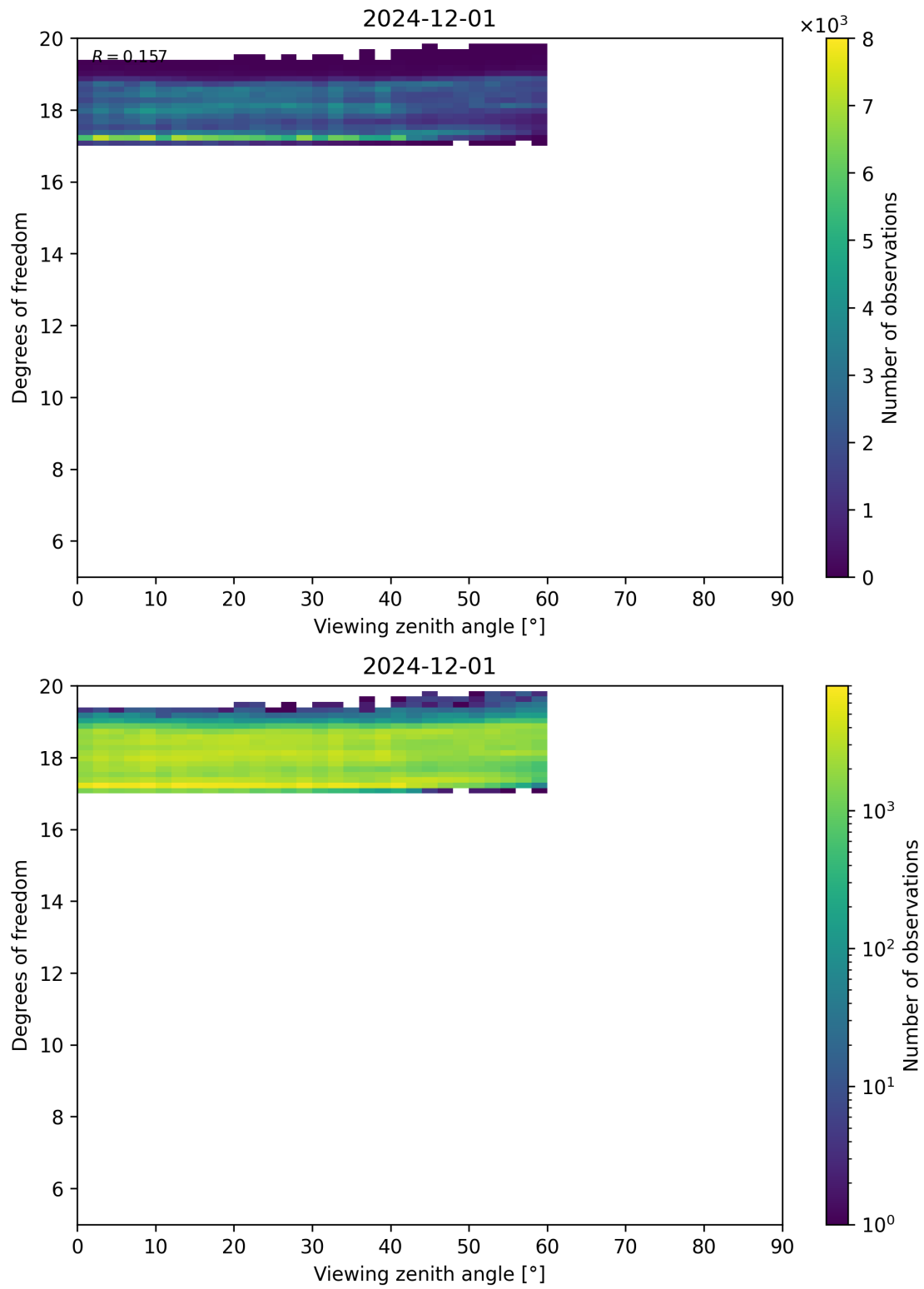
Figure 107: Scatter density plot of “Viewing zenith angle” against “Degrees of freedom” for 2024-11-30 to 2024-12-02.
