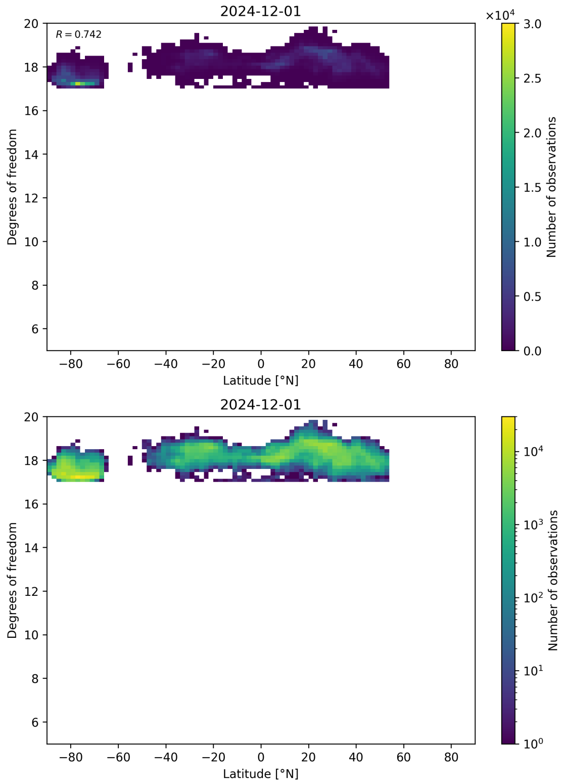
Figure 55: Scatter density plot of “Latitude” against “Degrees of freedom” for 2024-11-30 to 2024-12-02.
