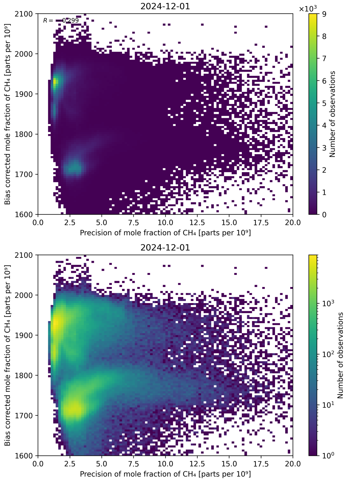
Figure 82: Scatter density plot of “Precision of mole fraction of CH 4 ” against “Bias corrected mole fraction of CH 4 ” for 2024-11-30 to 2024-12-02.
