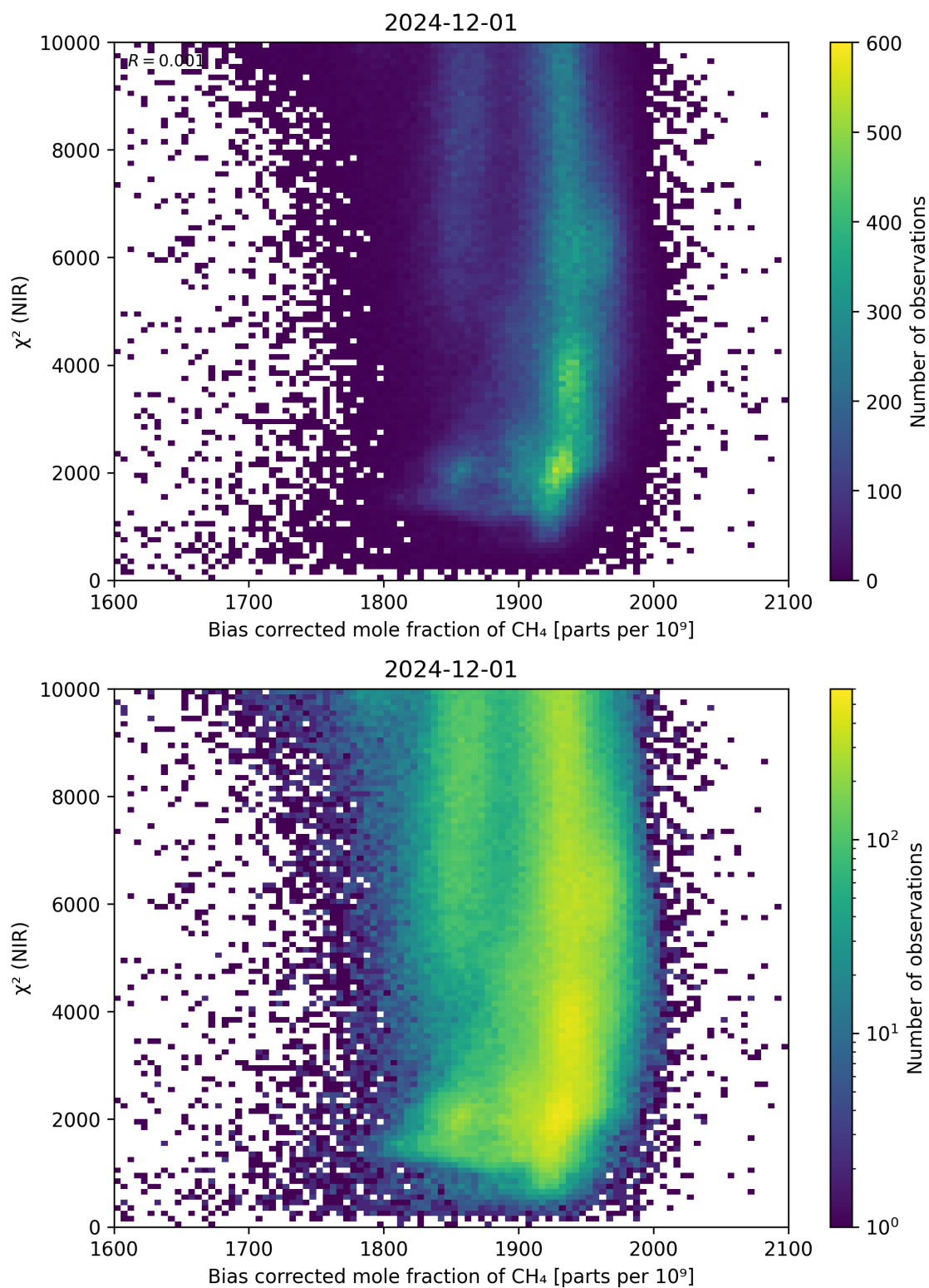
Figure 63: Scatter density plot of “Bias corrected mole fraction of \text{CH}_4 ” against “ \chi^2 (NIR)” for 2024-11-30 to 2024-12-02.
