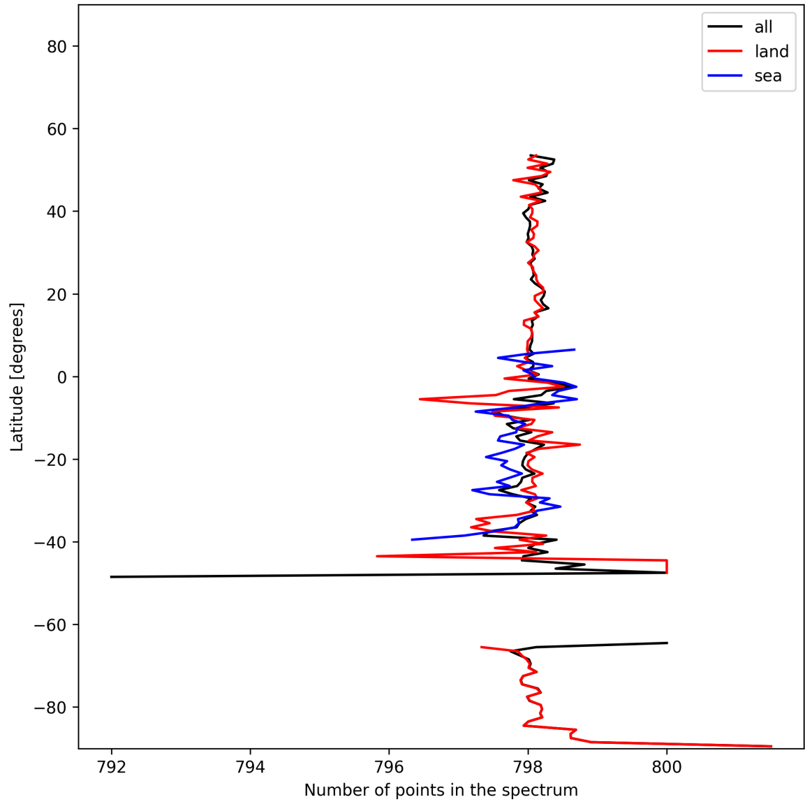
Figure 15: Zonal average of “Number of points in the spectrum” for 2024-11-30 to 2024-12-02.
