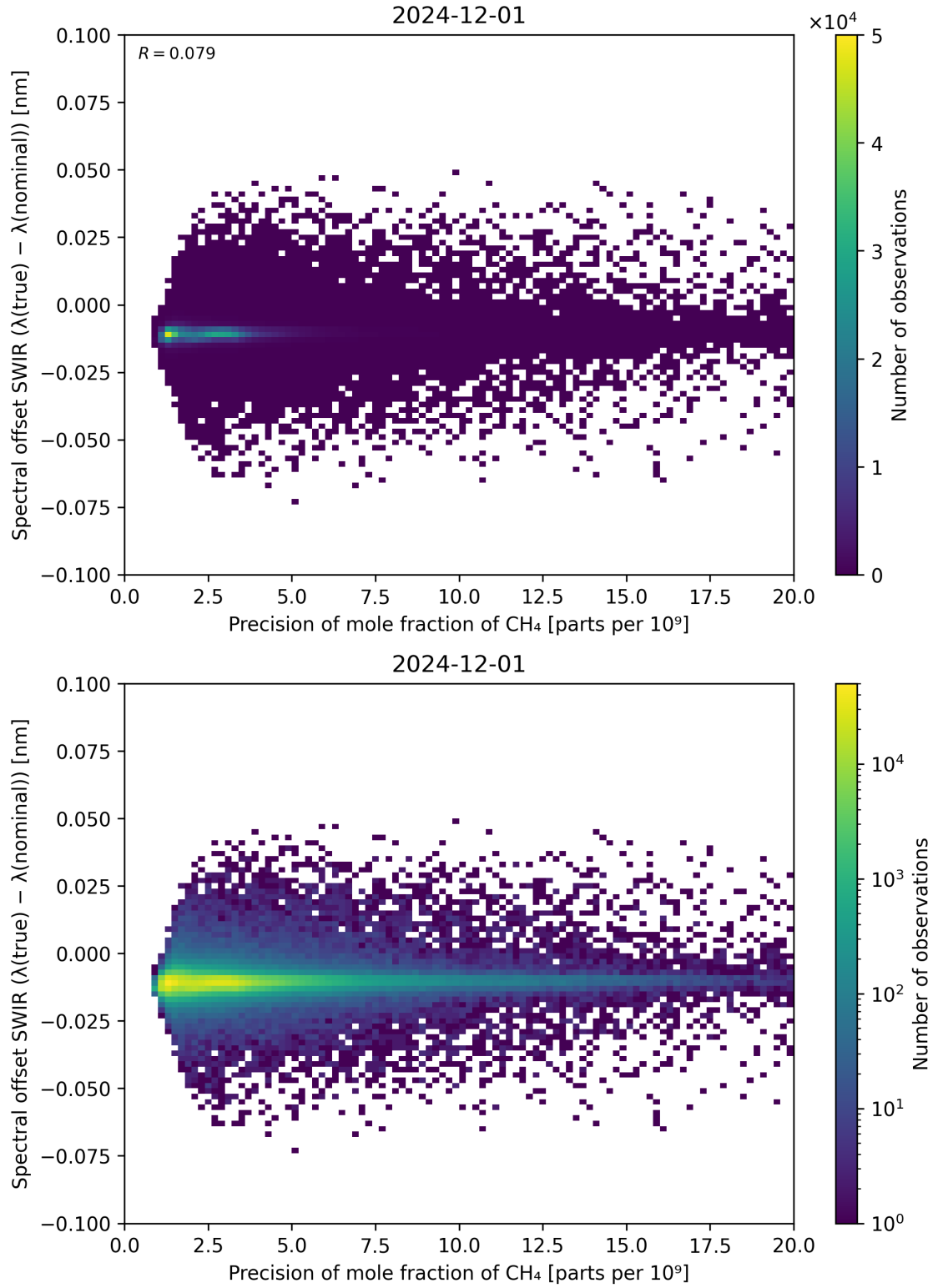
Figure 85: Scatter density plot of “Precision of mole fraction of \text{CH}_4 ” against “Spectral offset SWIR ( \lambda_{\text{true}} - \lambda_{\text{nominal}} )” for 2024-11-30 to 2024-12-02.
