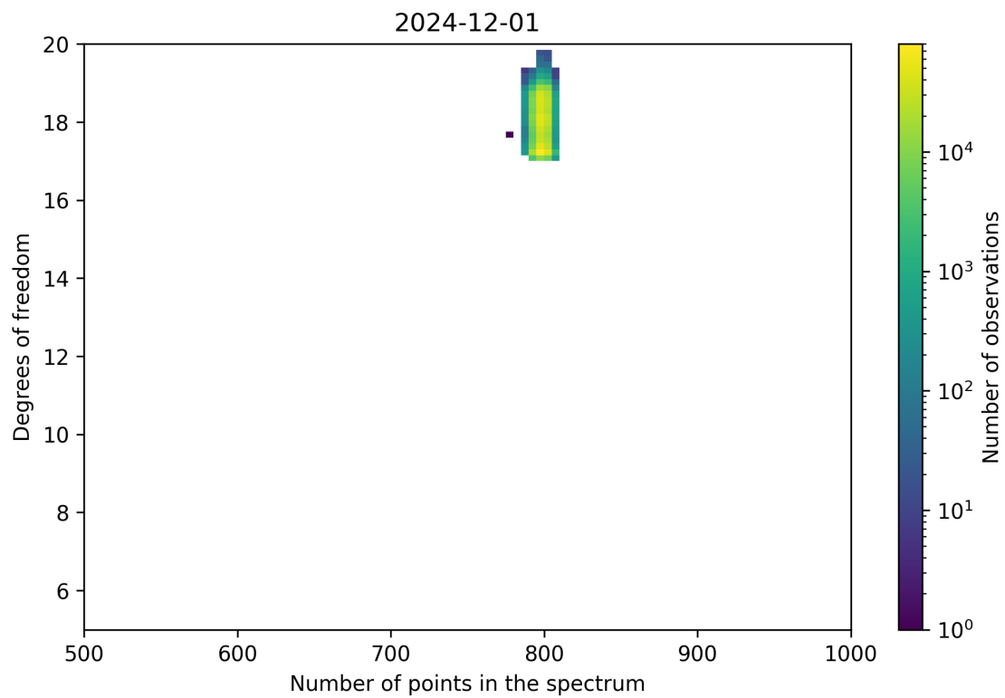
Figure 90: Scatter density plot of “Number of points in the spectrum” against “Degrees of freedom” for 2024-11-30 to 2024-12-02.
