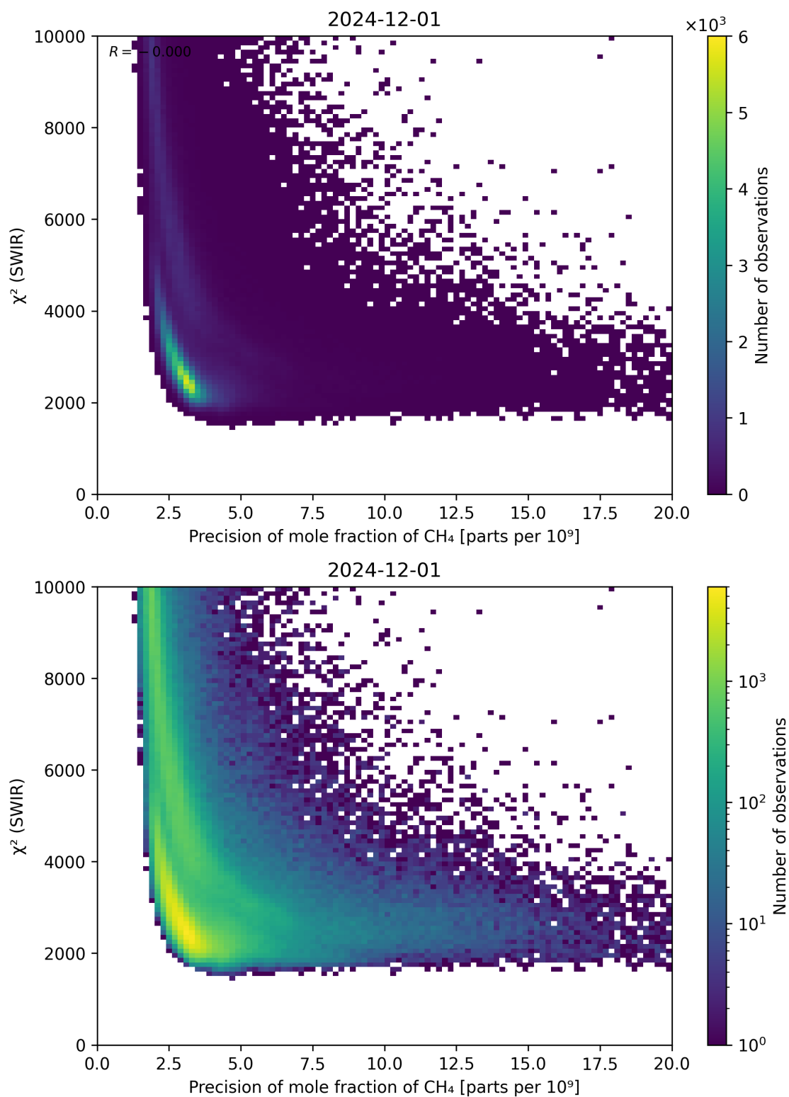
Figure 79: Scatter density plot of “Precision of mole fraction of \text{CH}_4 ” against “ \chi^2 (SWIR)” for 2024-11-30 to 2024-12-02.
