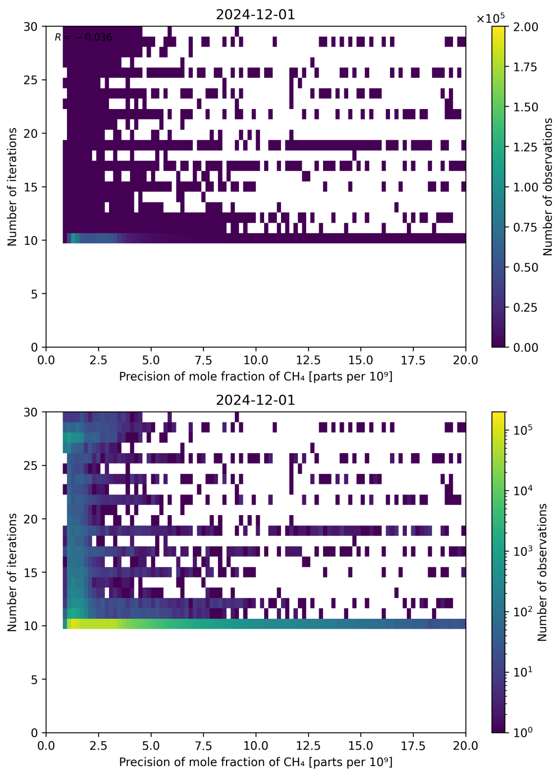
Figure 83: Scatter density plot of “Precision of mole fraction of CH 4 ” against “Number of iterations” for 2024-11-30 to 2024-12-02.
