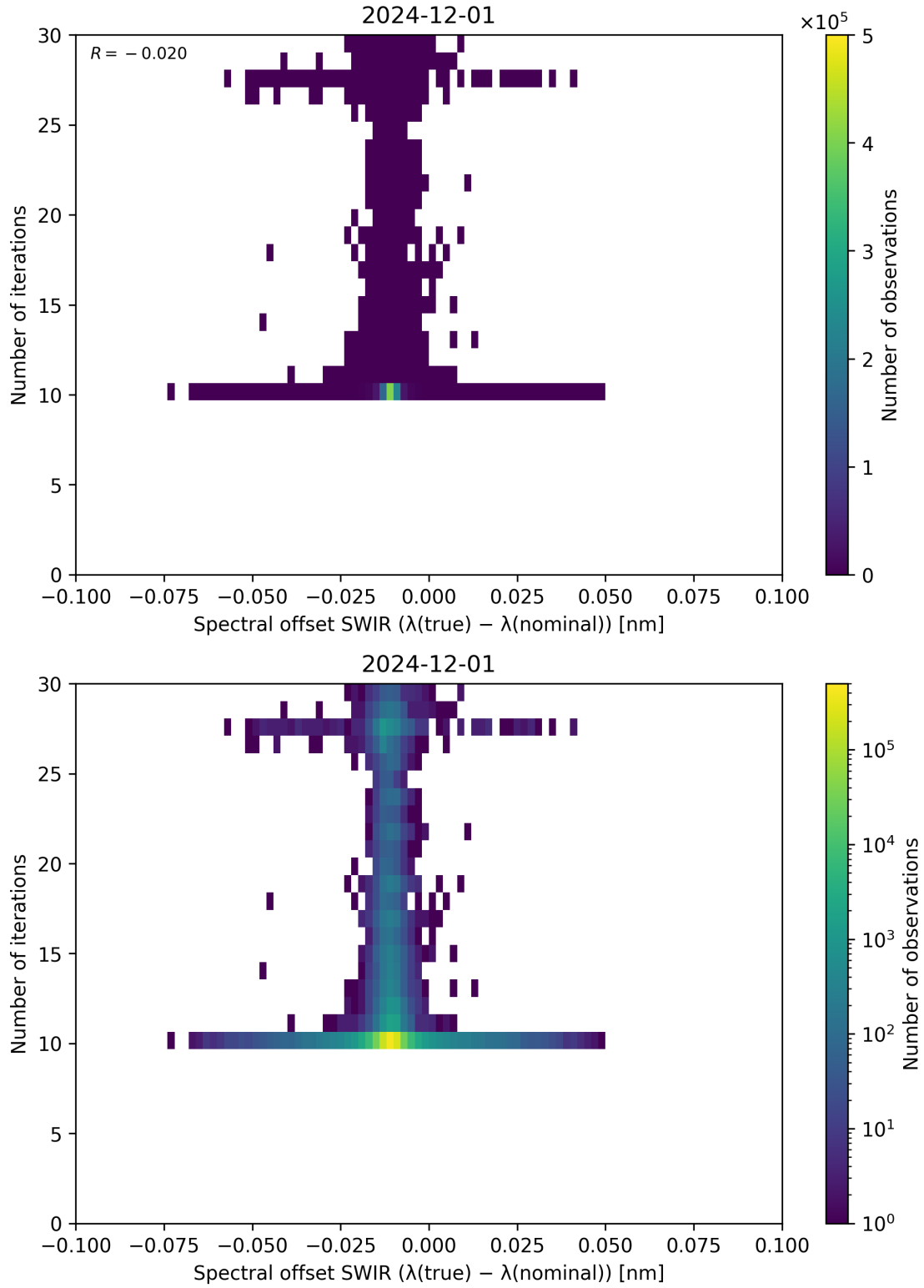
Figure 121: Scatter density plot of “Spectral offset SWIR ( \lambda_{\text{true}} - \lambda_{\text{nominal}} )” against “Number of iterations” for 2024-11-30 to 2024-12-02.
