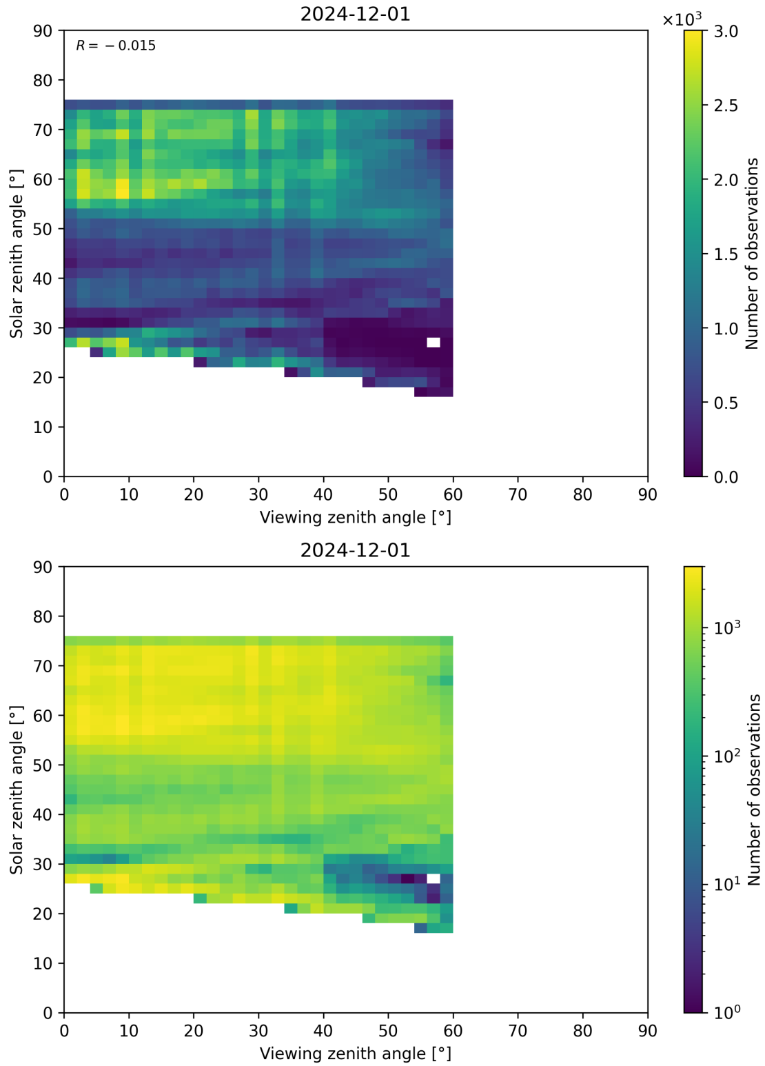
Figure 115: Scatter density plot of “Viewing zenith angle” against “Solar zenith angle” for 2024-11-30 to 2024-12-02.
