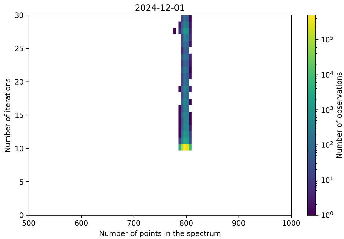
Figure 92: Scatter density plot of “Number of points in the spectrum” against “Number of iterations” for 2024-11-30 to 2024-12-02.
