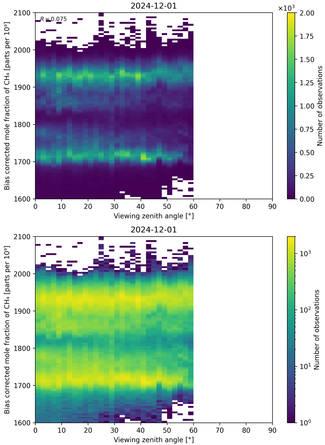
Figure 111: Scatter density plot of “Viewing zenith angle” against “Bias corrected mole fraction of CH 4 ” for 2024-11-30 to 2024-12-02.
