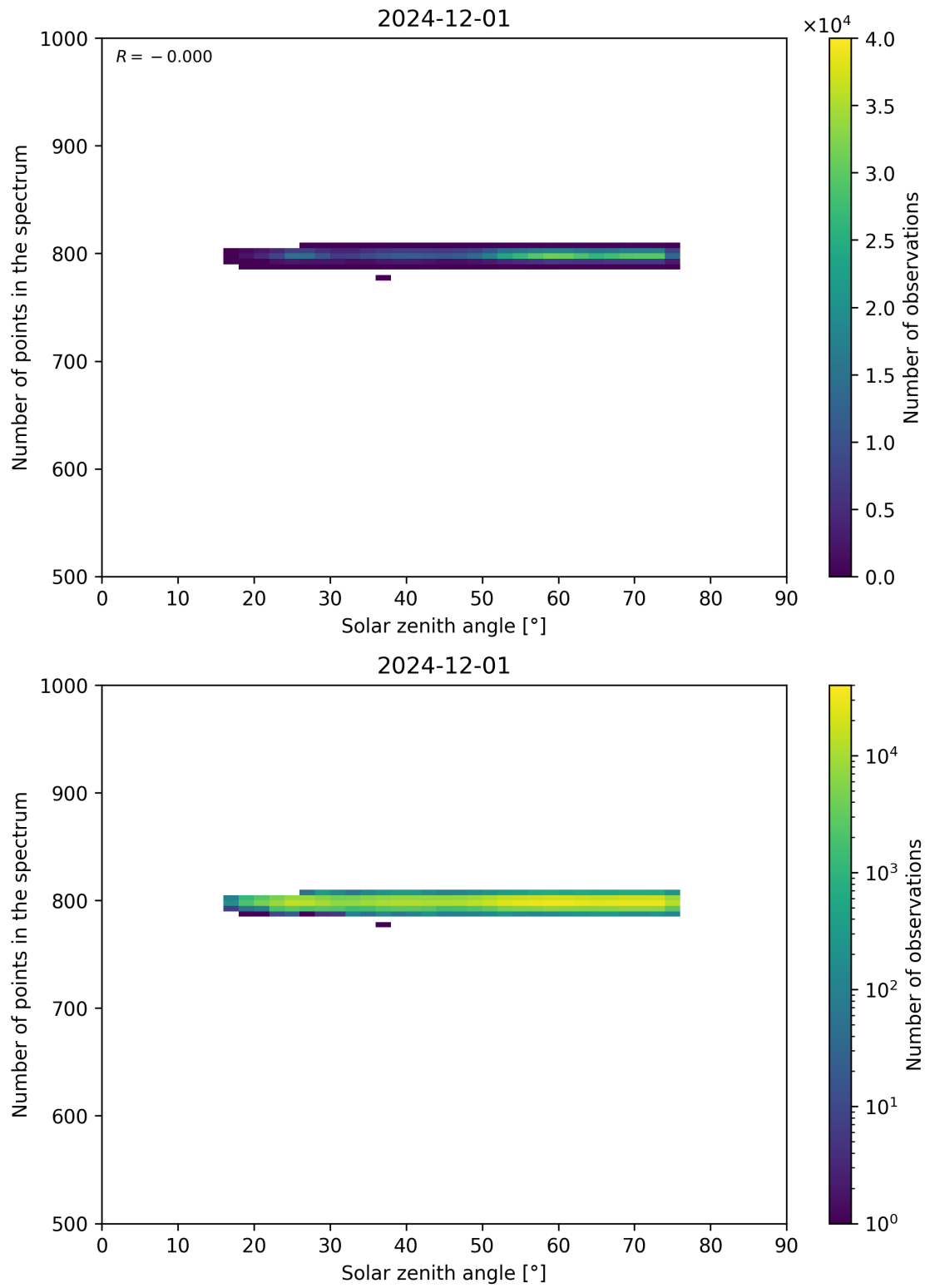
Figure 103: Scatter density plot of “Solar zenith angle” against “Number of points in the spectrum” for 2024-11-30 to 2024-12-02.
