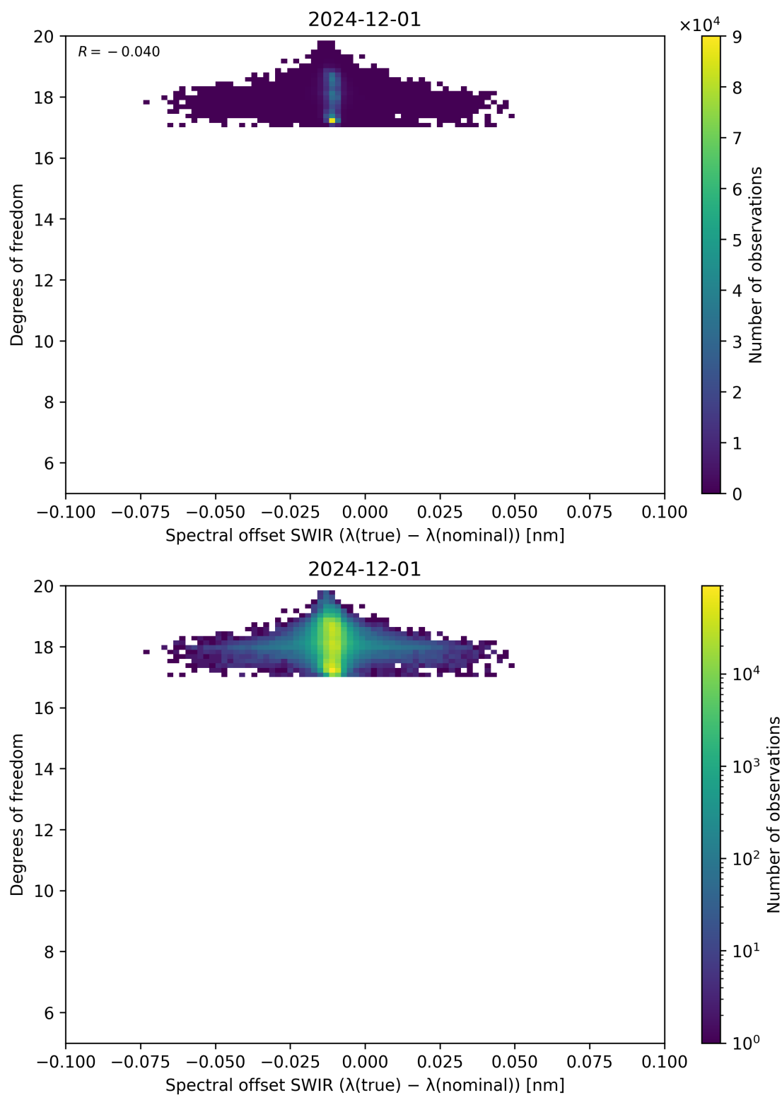
Figure 119: Scatter density plot of “Spectral offset SWIR ( \lambda_{\text{true}} - \lambda_{\text{nominal}} )” against “Degrees of freedom” for 2024-11-30 to 2024-12-02.
