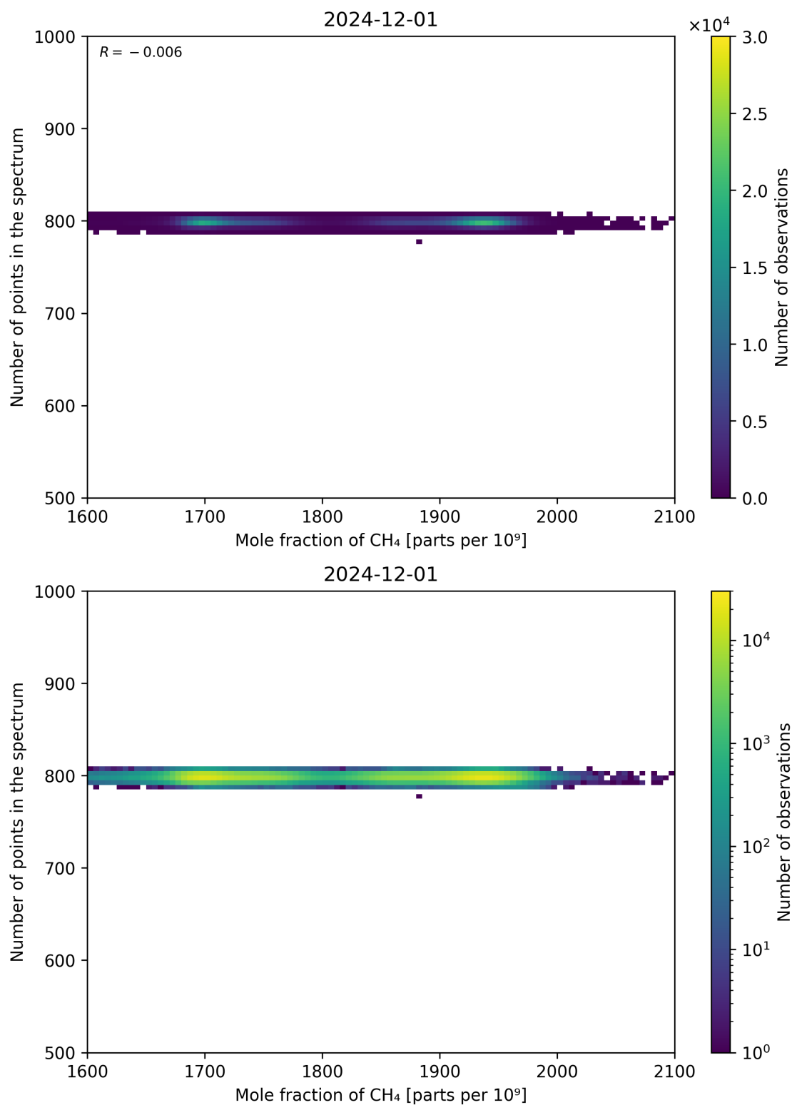
Figure 77: Scatter density plot of “Mole fraction of CH 4 ” against “Number of points in the spectrum” for 2024-11-30 to 2024-12-02.
