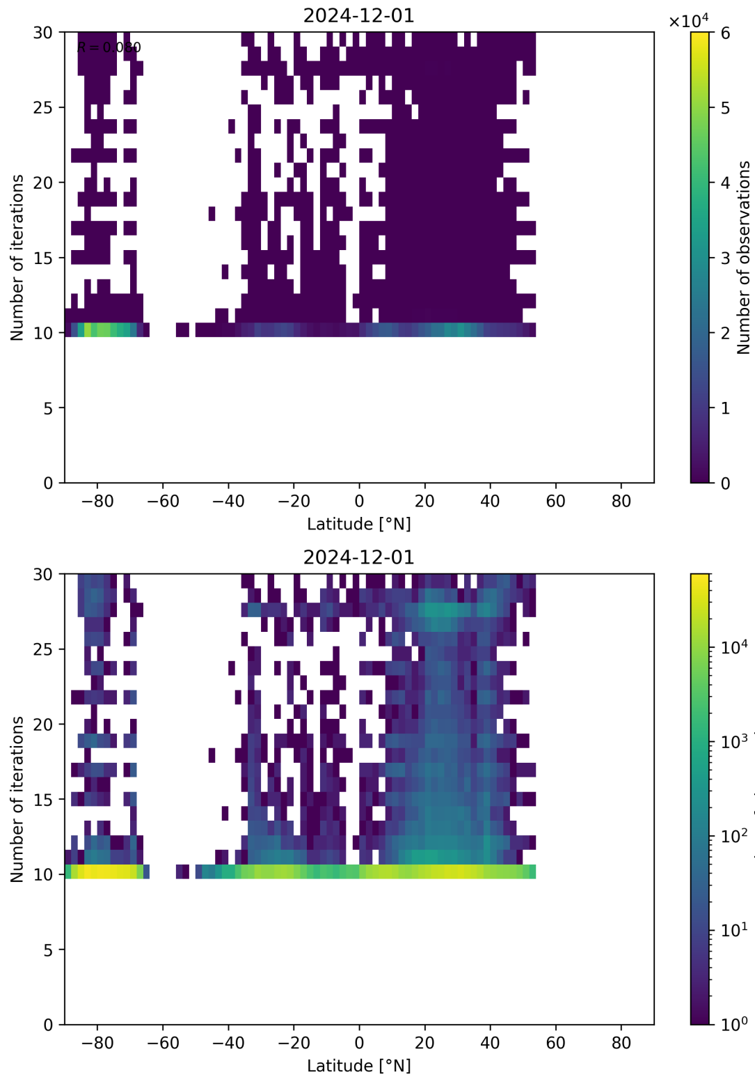
Figure 60: Scatter density plot of “Latitude” against “Number of iterations” for 2024-11-30 to 2024-12-02.
