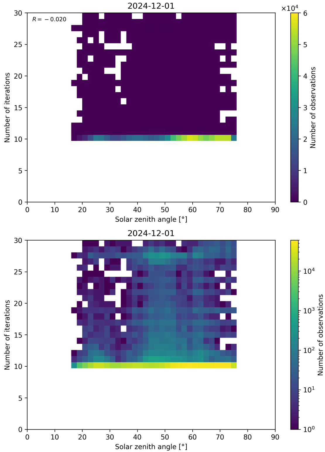
Figure 102: Scatter density plot of “Solar zenith angle” against “Number of iterations” for 2024-11-30 to 2024-12-02.
