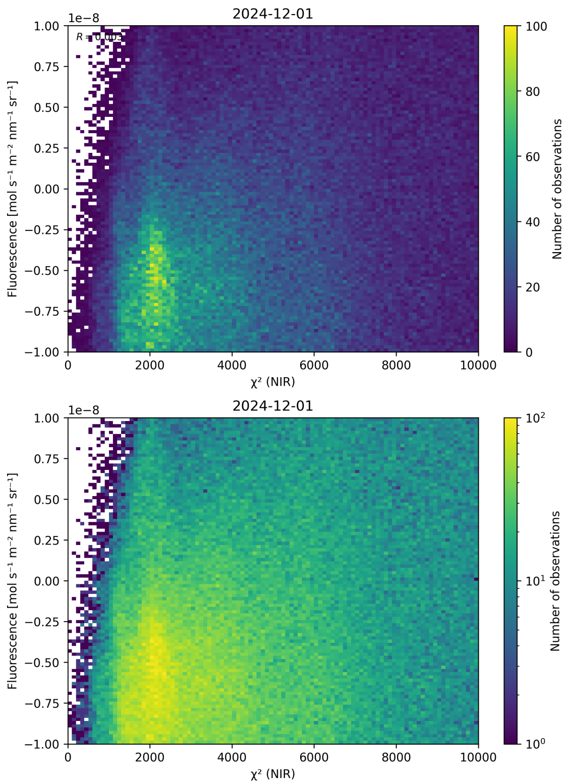
Figure 45: Scatter density plot of “ \chi^2 (NIR)” against “Fluorescence” for 2024-11-30 to 2024-12-02.
