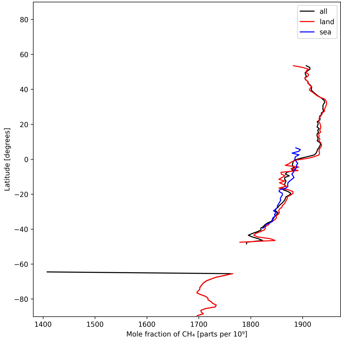
Figure 12: Zonal average of “Mole fraction of \text{CH}_4 ” for 2024-11-30 to 2024-12-02.
