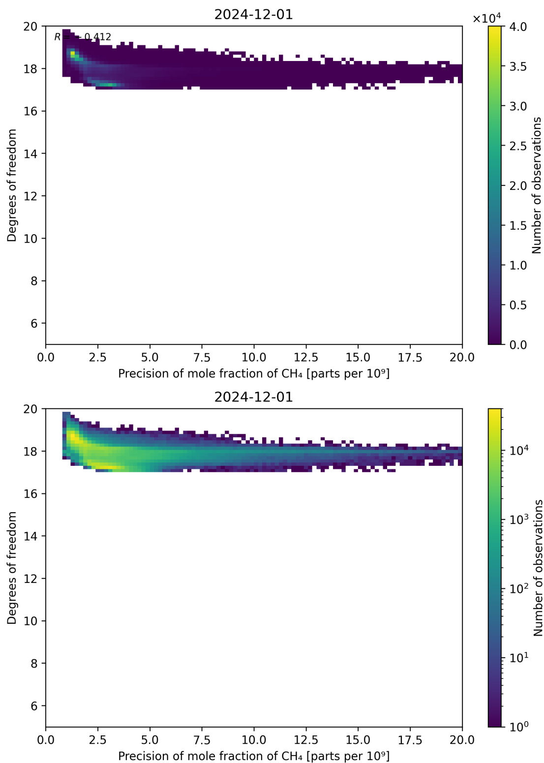
Figure 80: Scatter density plot of “Precision of mole fraction of CH 4 ” against “Degrees of freedom” for 2024-11-30 to 2024-12-02.
