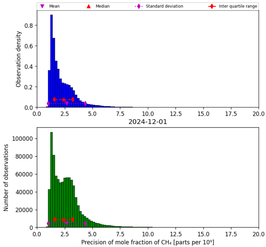
Figure 24: Histogram of “Precision of mole fraction of CH 4 ” for 2024-11-30 to 2024-12-02
