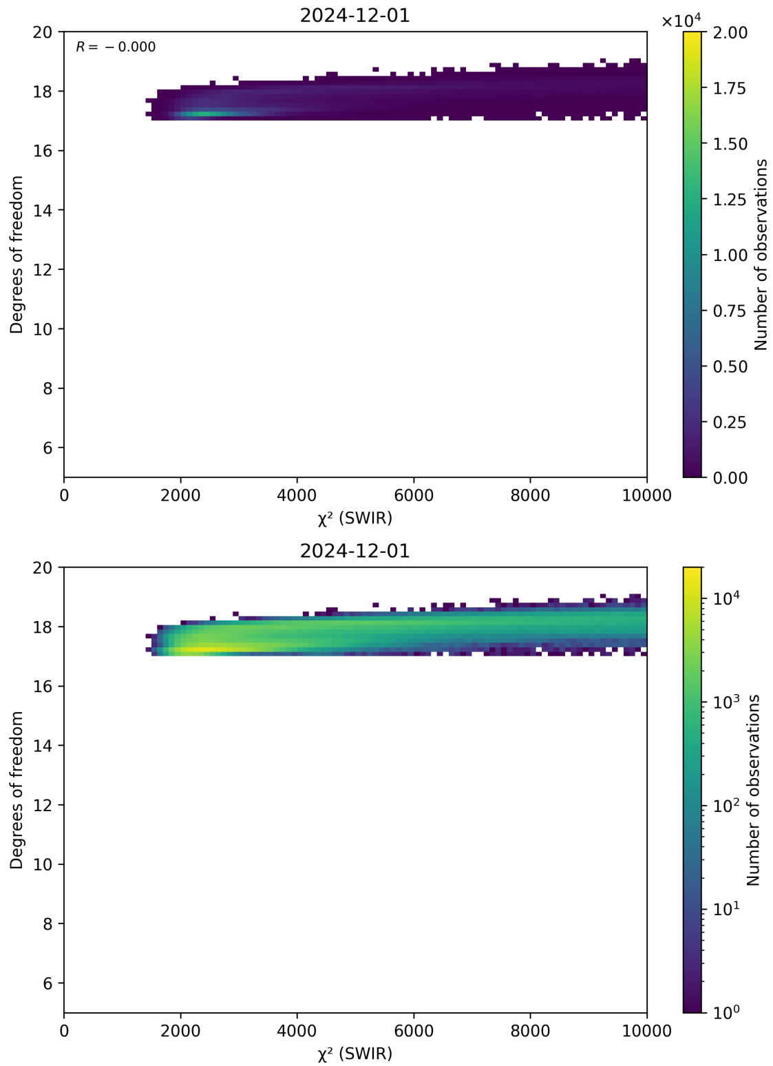
Figure 48: Scatter density plot of “ \chi^2 (SWIR)” against “Degrees of freedom” for 2024-11-30 to 2024-12-02.
