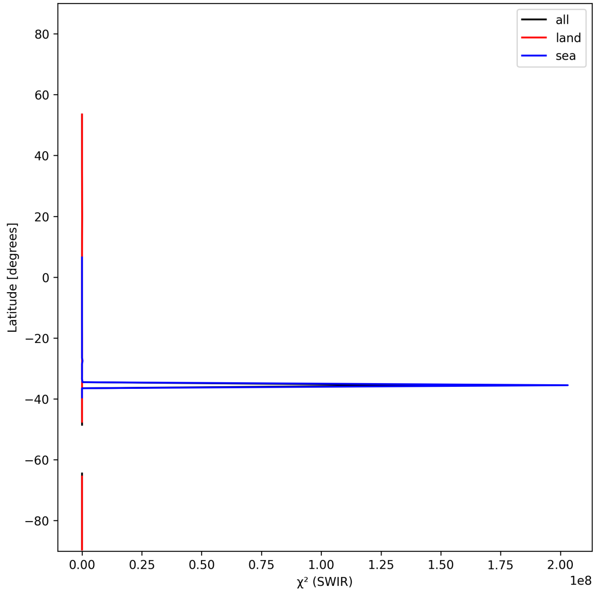
Figure 17: Zonal average of “ \chi^2 (SWIR)” for 2024-11-30 to 2024-12-02.
