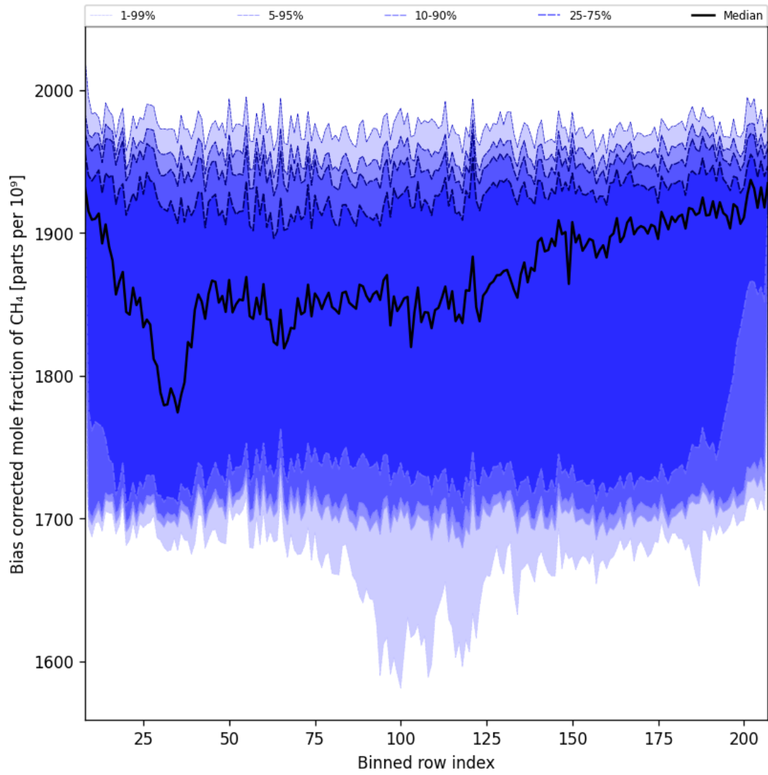
Figure 36: Along track statistics of “Bias corrected mole fraction of CH 4 ” for 2024-11-30 to 2024-12-02
