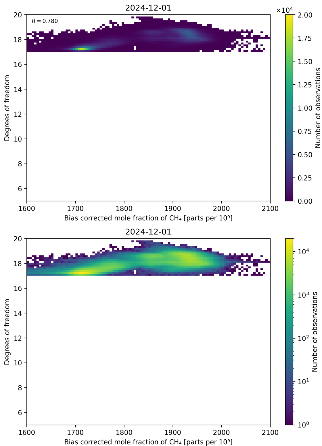
Figure 65: Scatter density plot of “Bias corrected mole fraction of CH 4 ” against “Degrees of freedom” for 2024-11-30 to 2024-12-02.
