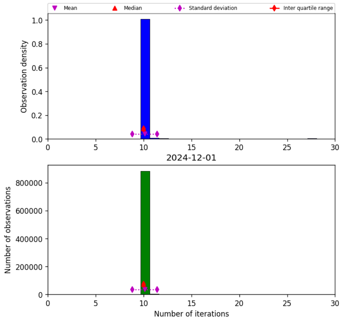
Figure 31: Histogram of “Number of iterations” for 2024-11-30 to 2024-12-02
