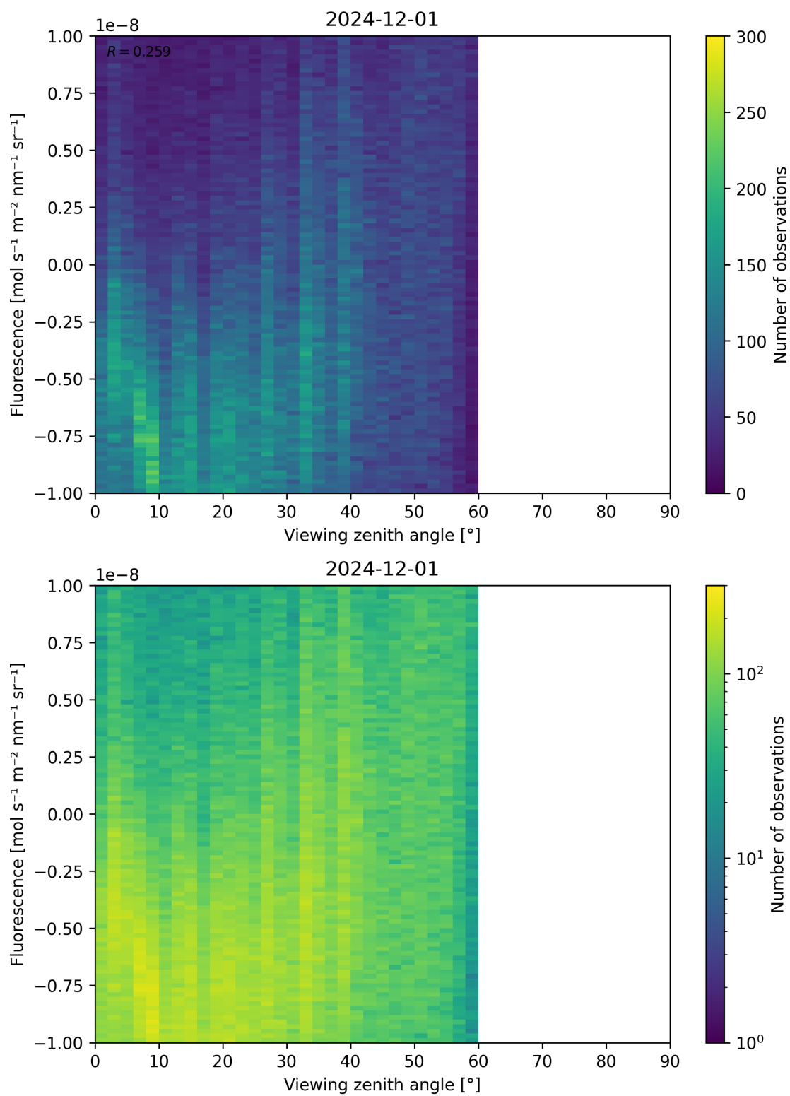
Figure 108: Scatter density plot of “Viewing zenith angle” against “Fluorescence” for 2024-11-30 to 2024-12-02.
