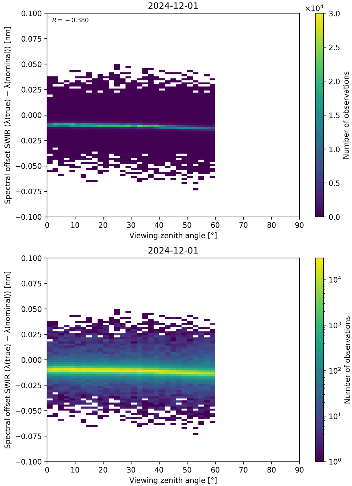
Figure 116: Scatter density plot of “Viewing zenith angle” against “Spectral offset SWIR ( \lambda_{\text{true}} - \lambda_{\text{nominal}} )” for 2024-11-30 to 2024-12-02.
