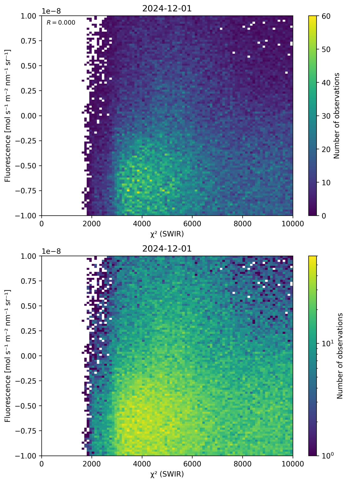
Figure 49: Scatter density plot of “ \chi^2 (SWIR)” against “Fluorescence” for 2024-11-30 to 2024-12-02.
