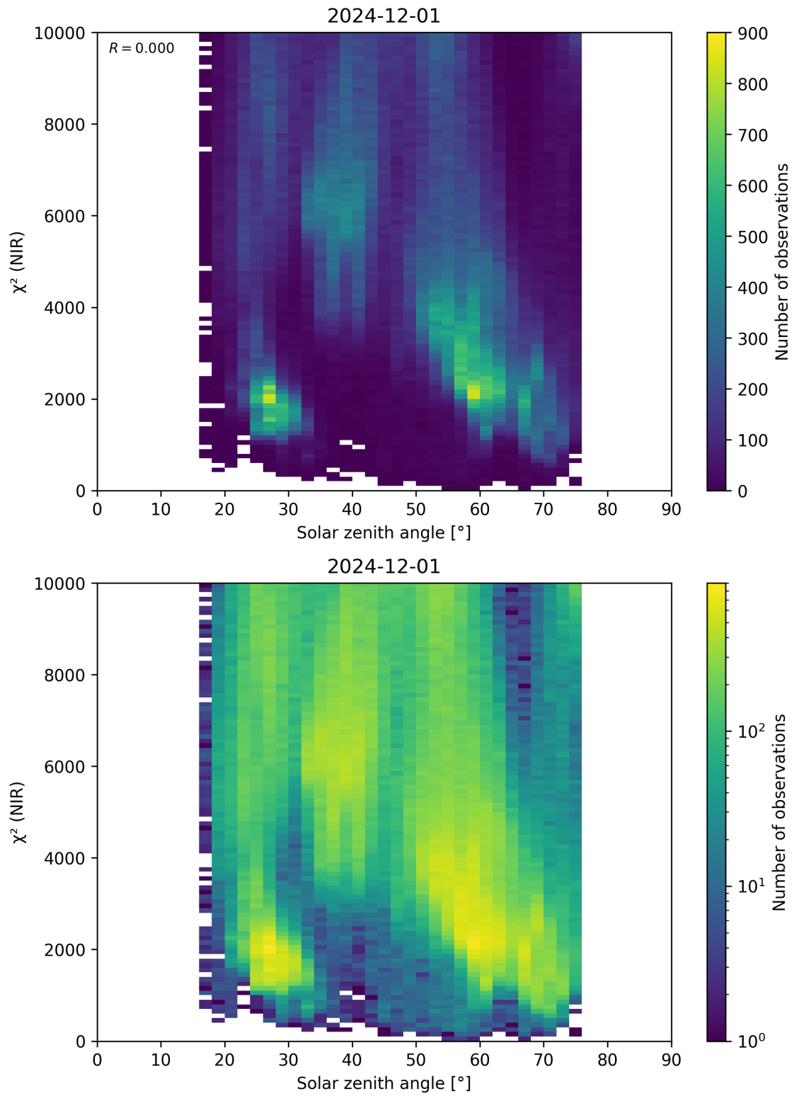
Figure 94: Scatter density plot of “Solar zenith angle” against “ \chi^2 (NIR)” for 2024-11-30 to 2024-12-02.
