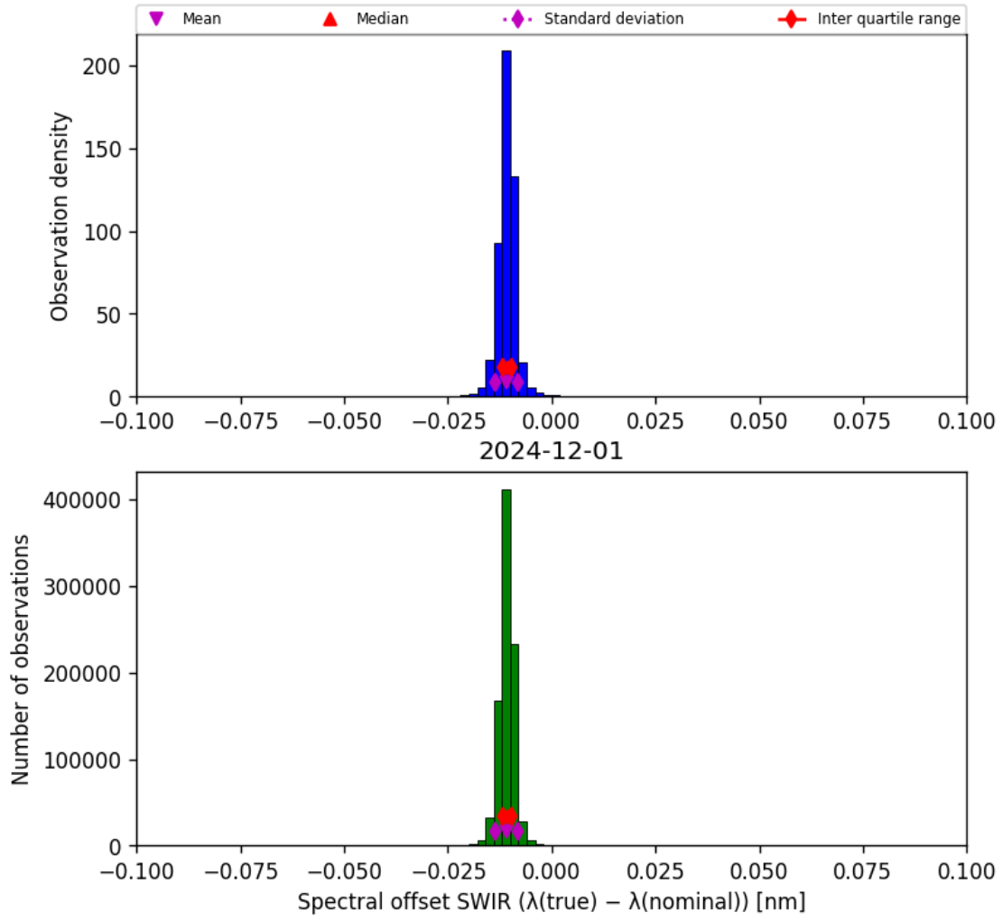
Figure 27: Histogram of “Spectral offset SWIR ( \lambda_{\text{true}} - \lambda_{\text{nominal}} )” for 2024-11-30 to 2024-12-02
