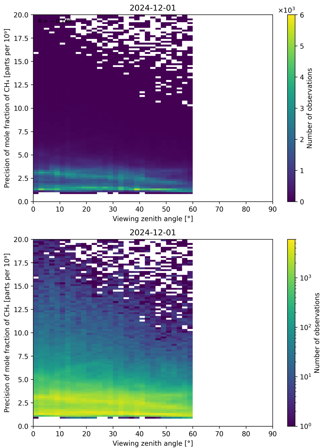
Figure 112: Scatter density plot of “Viewing zenith angle” against “Precision of mole fraction of CH 4 ” for 2024-11-30 to 2024-12-02.
