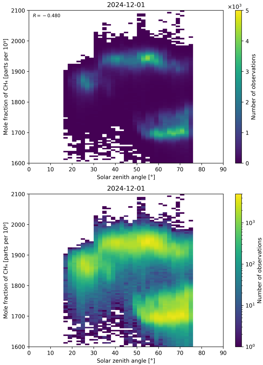
Figure 99: Scatter density plot of “Solar zenith angle” against “Mole fraction of CH 4 ” for 2024-11-30 to 2024-12-02.
