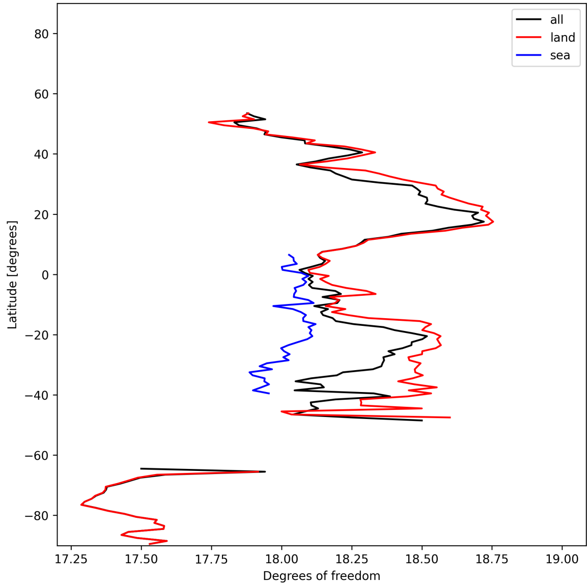
Figure 19: Zonal average of “Degrees of freedom” for 2024-11-30 to 2024-12-02.
