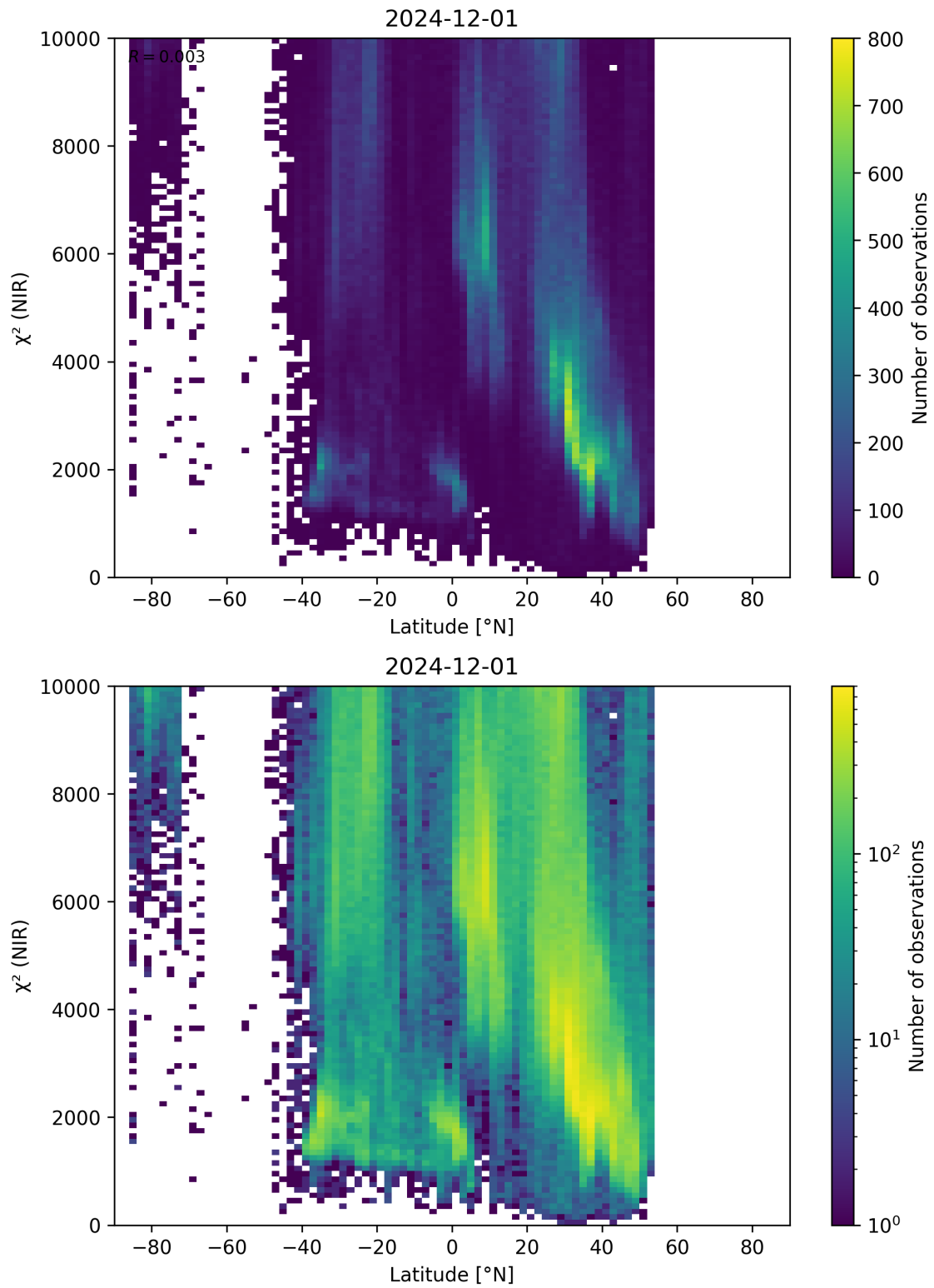
Figure 53: Scatter density plot of “Latitude” against “ \chi^2 (NIR)” for 2024-11-30 to 2024-12-02.
