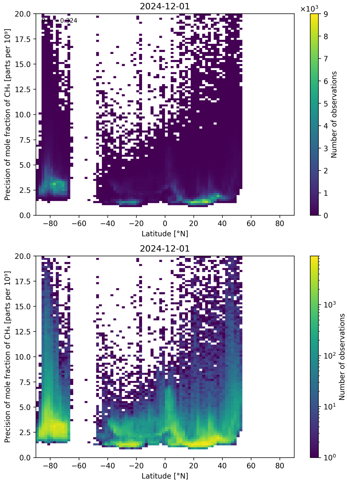
Figure 59: Scatter density plot of “Latitude” against “Precision of mole fraction of CH 4 ” for 2024-11-30 to 2024-12-02.
