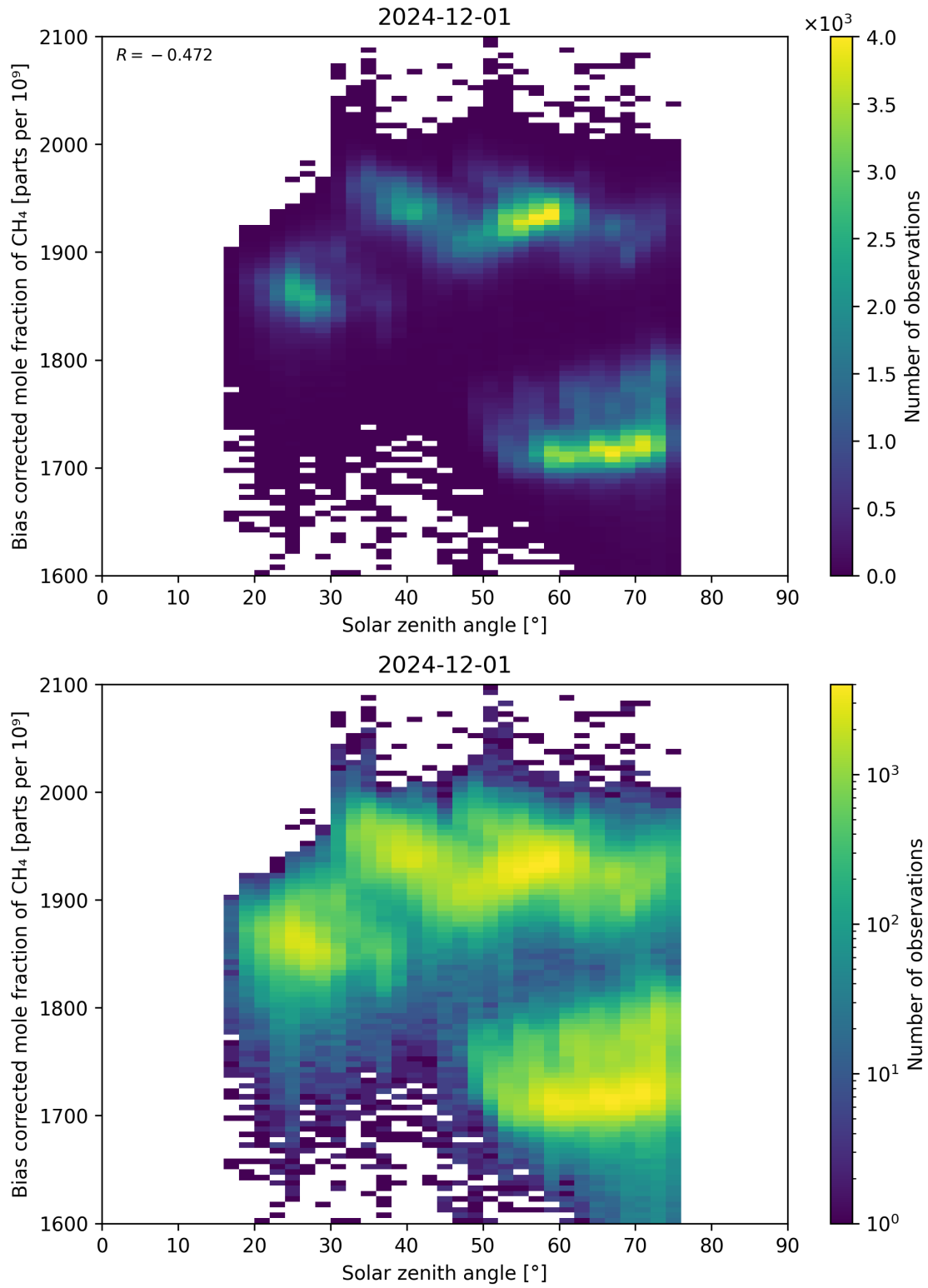
Figure 100: Scatter density plot of “Solar zenith angle” against “Bias corrected mole fraction of CH 4 ” for 2024-11-30 to 2024-12-02.
