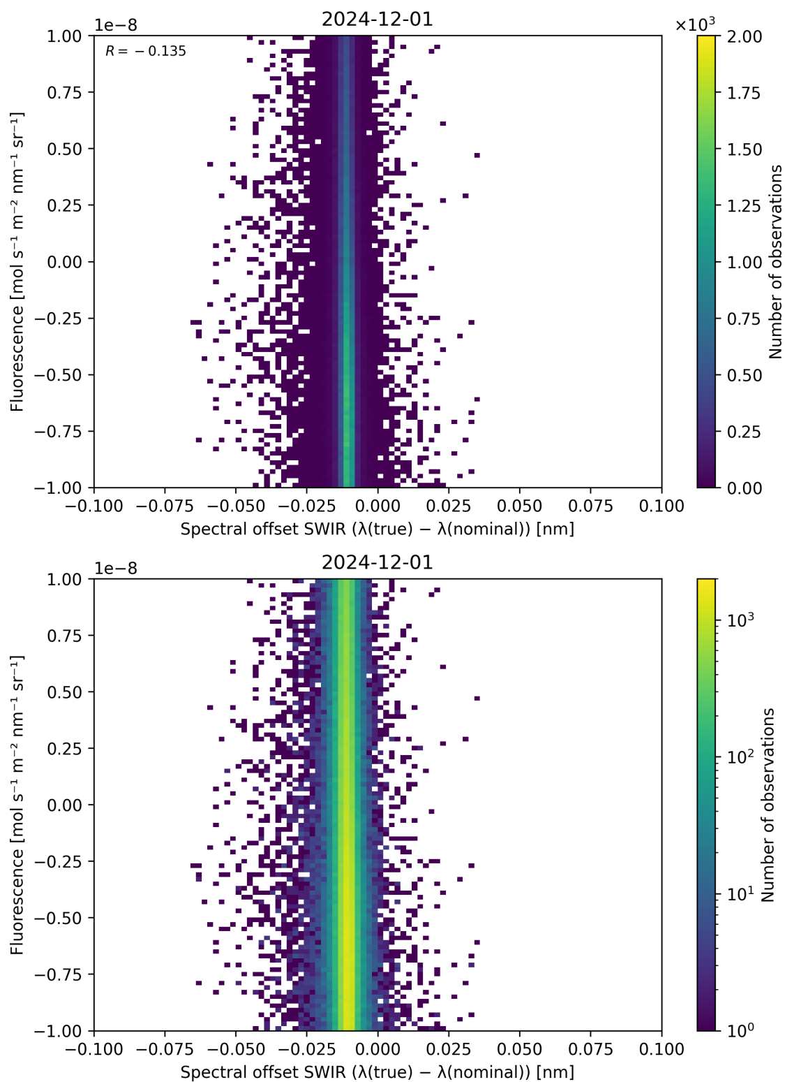
Figure 120: Scatter density plot of “Spectral offset SWIR ( \lambda_{\text{true}} - \lambda_{\text{nominal}} )” against “Fluorescence” for 2024-11-30 to 2024-12-02.
