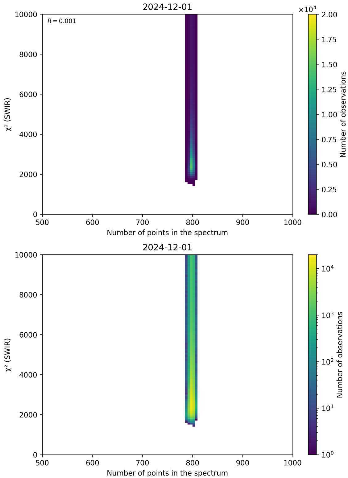
Figure 89: Scatter density plot of “Number of points in the spectrum” against “ \chi^2 (SWIR)” for 2024-11-30 to 2024-12-02.
