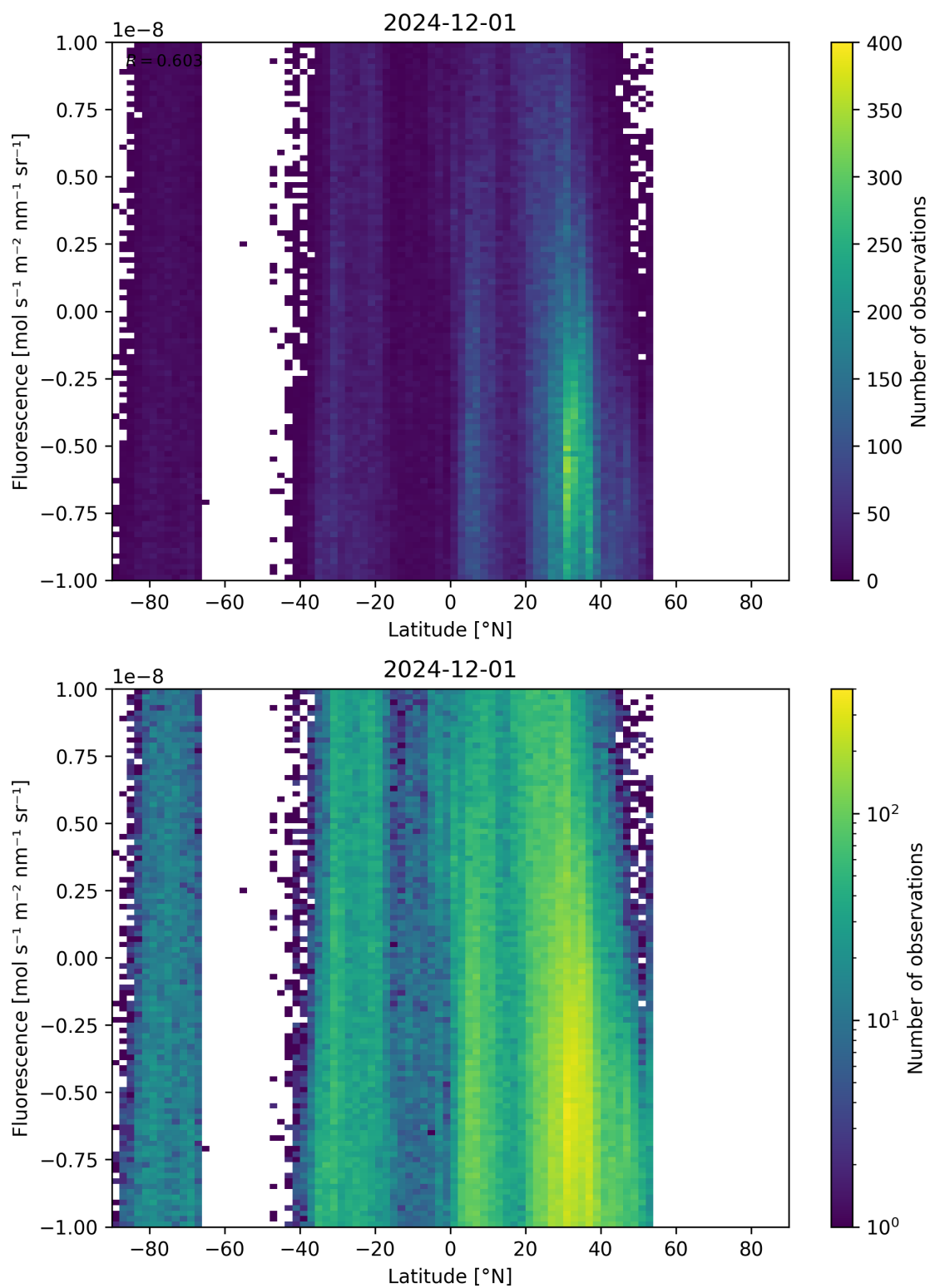
Figure 56: Scatter density plot of “Latitude” against “Fluorescence” for 2024-11-30 to 2024-12-02.
