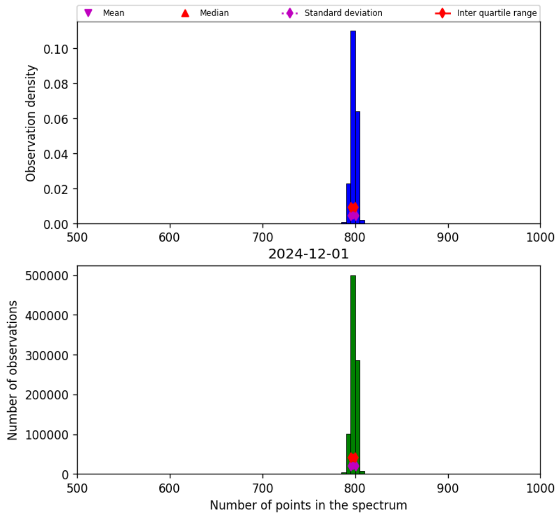
Figure 26: Histogram of “Number of points in the spectrum” for 2024-11-30 to 2024-12-02
