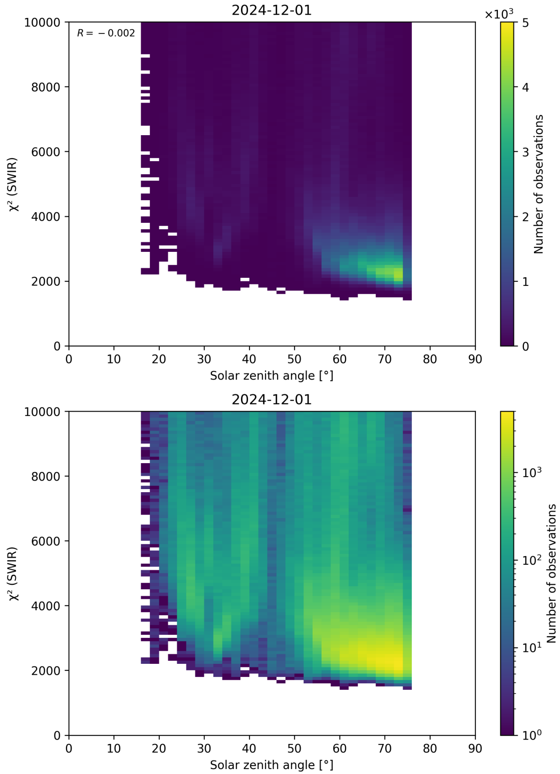
Figure 95: Scatter density plot of “Solar zenith angle” against “ \chi^2 (SWIR)” for 2024-11-30 to 2024-12-02.
