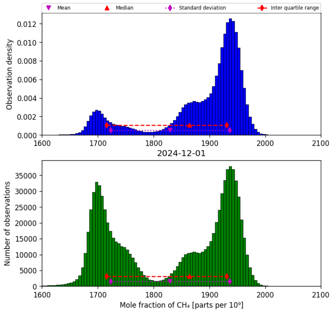
Figure 23: Histogram of “Mole fraction of CH 4 ” for 2024-11-30 to 2024-12-02
