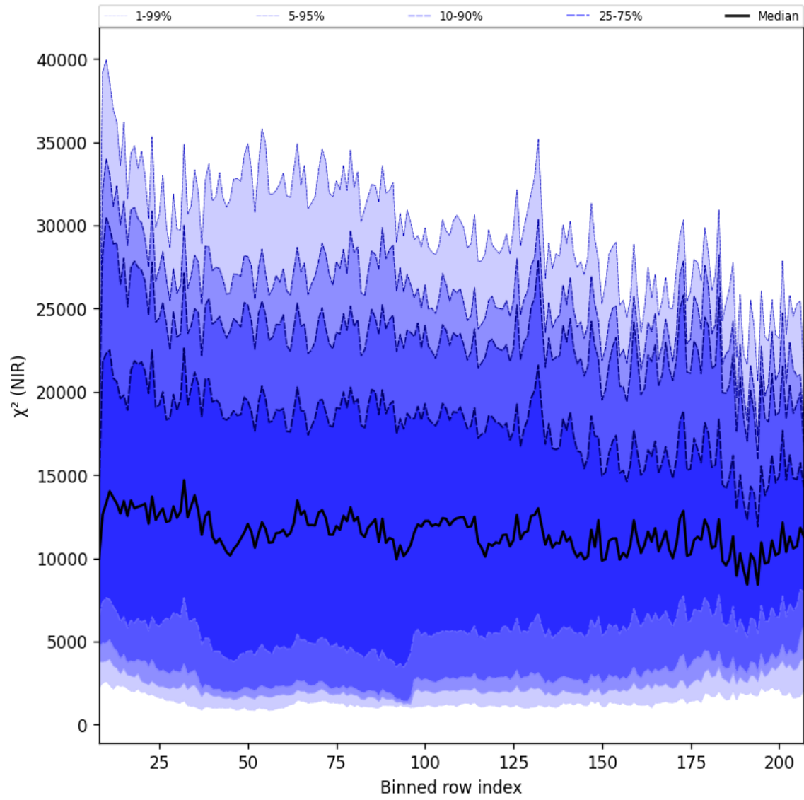
Figure 40: Along track statistics of “ \chi^2 (NIR)” for 2024-11-30 to 2024-12-02
