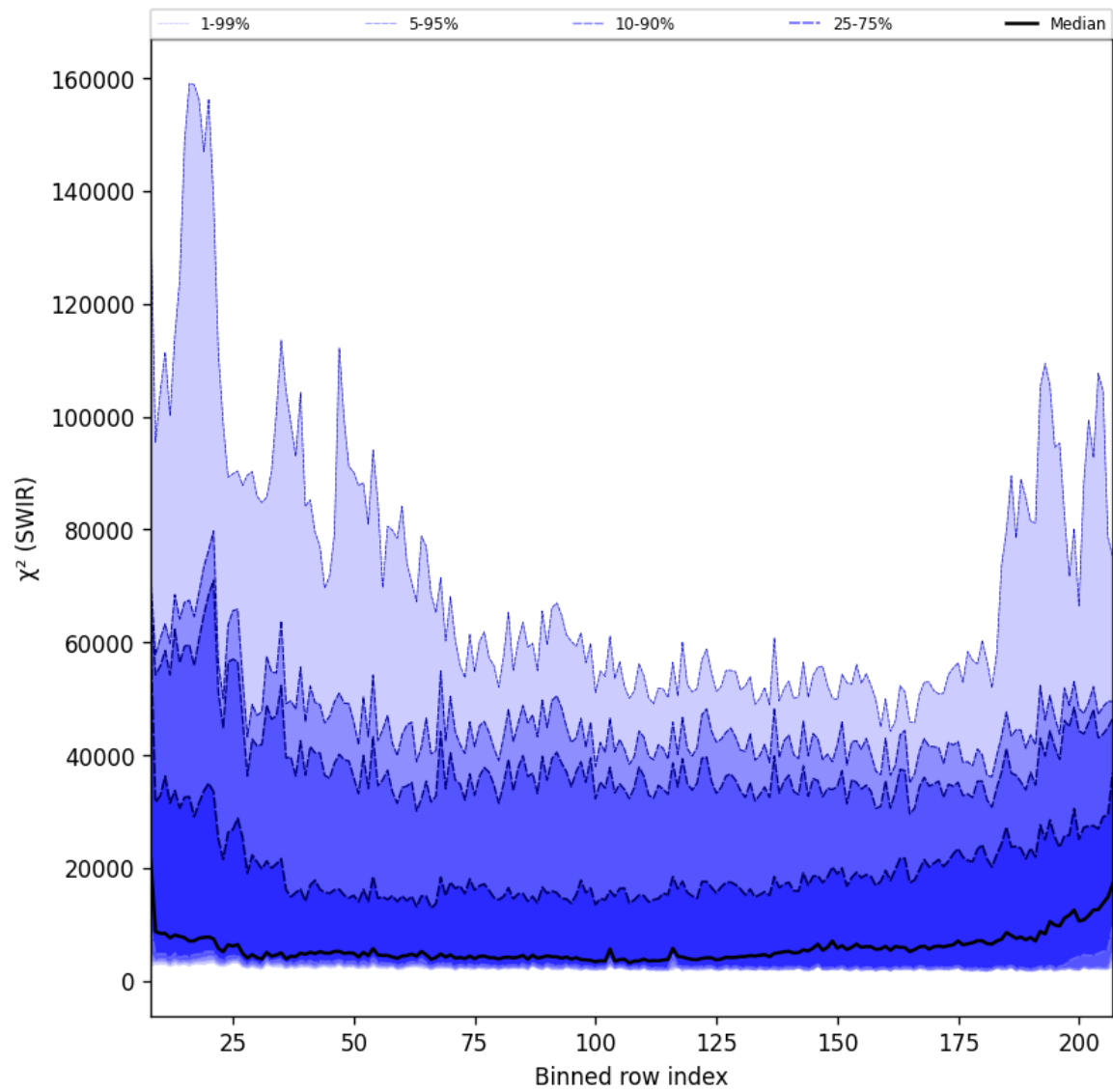
Figure 39: Along track statistics of “ \chi^2 (SWIR)” for 2024-11-30 to 2024-12-02
