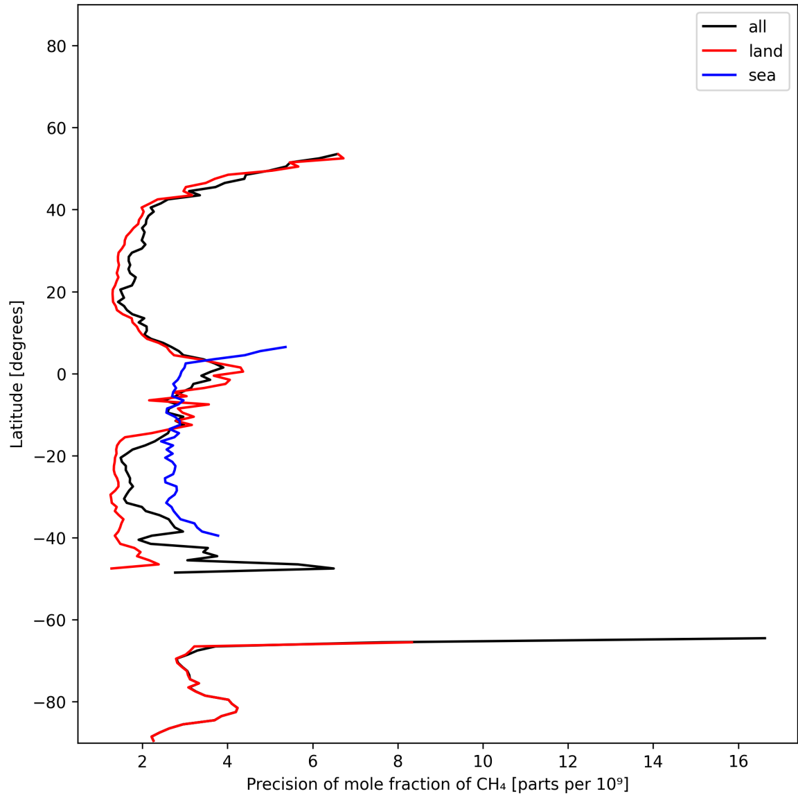
Figure 13: Zonal average of “Precision of mole fraction of CH 4 ” for 2024-11-30 to 2024-12-02.
