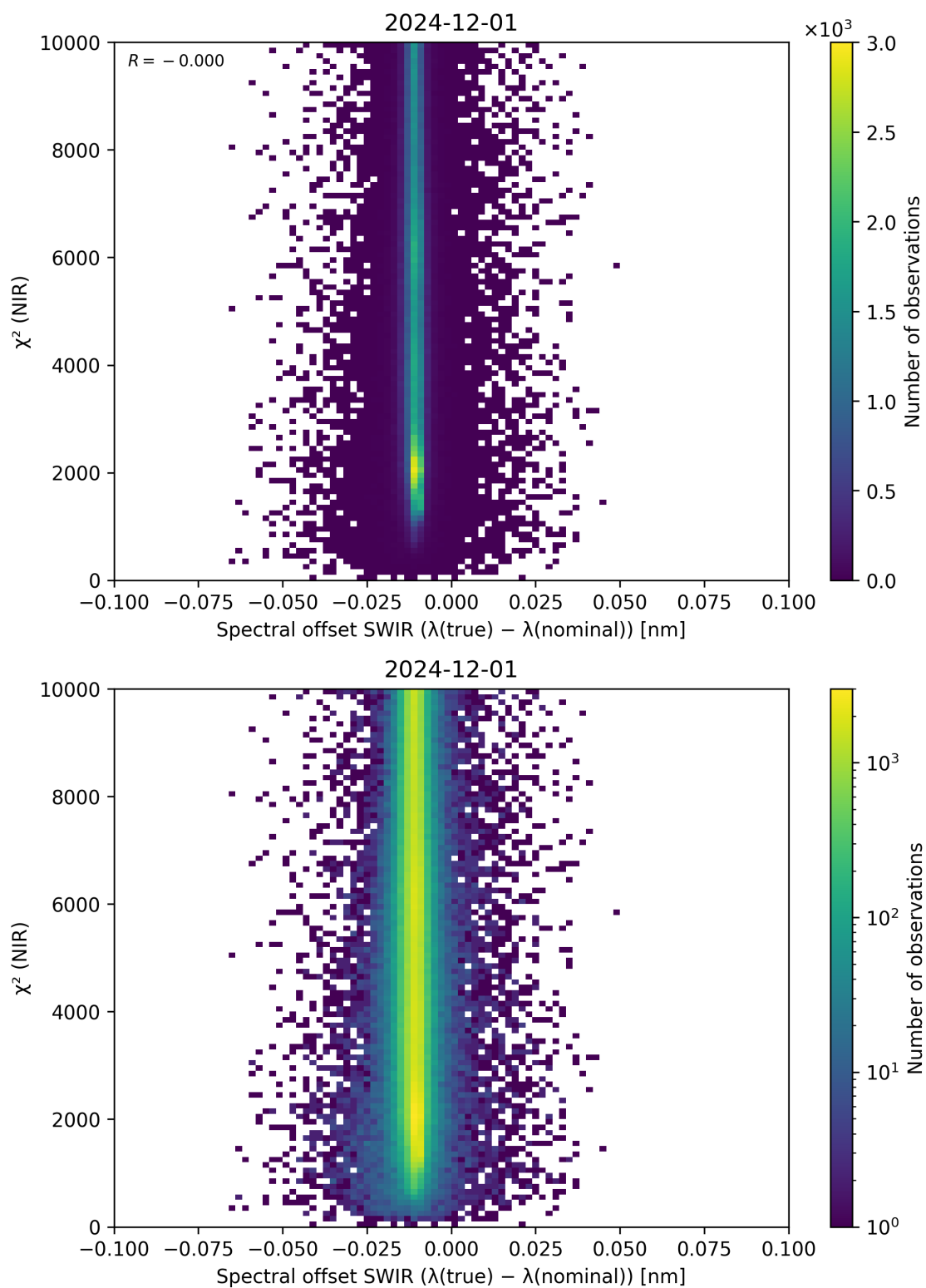
Figure 117: Scatter density plot of “Spectral offset SWIR ( \lambda_{\text{true}} - \lambda_{\text{nominal}} )” against “ \chi^2 (NIR)” for 2024-11-30 to 2024-12-02.
