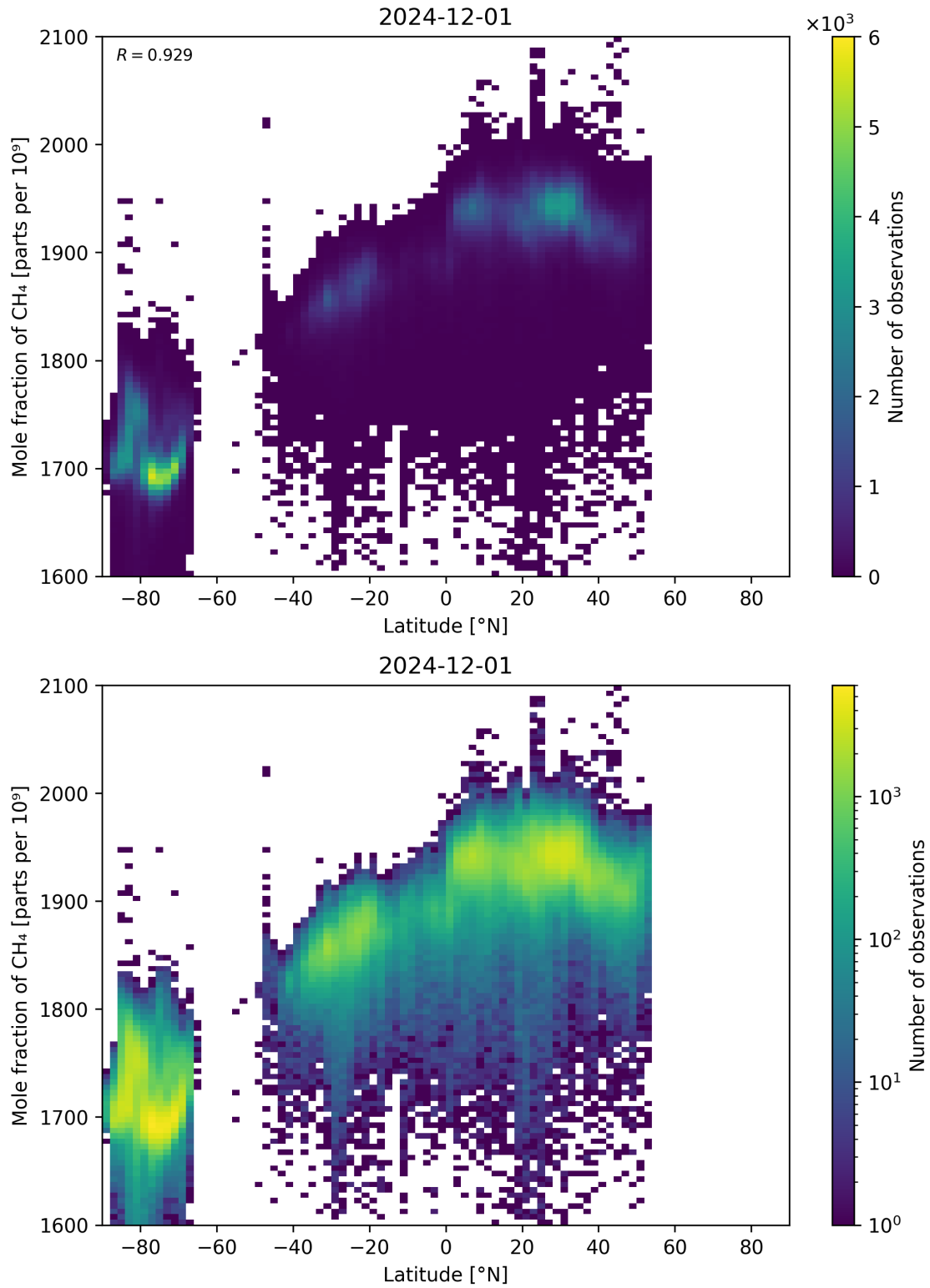
Figure 57: Scatter density plot of “Latitude” against “Mole fraction of CH 4 ” for 2024-11-30 to 2024-12-02.
