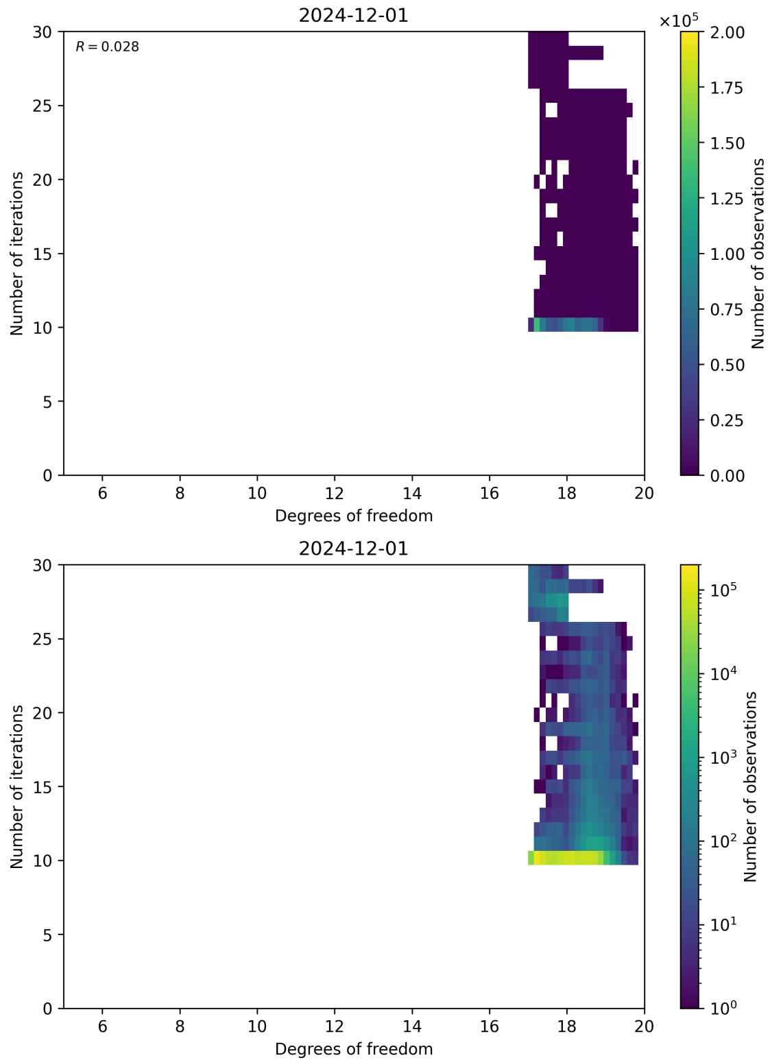
Figure 52: Scatter density plot of “Degrees of freedom” against “Number of iterations” for 2024-11-30 to 2024-12-02.
