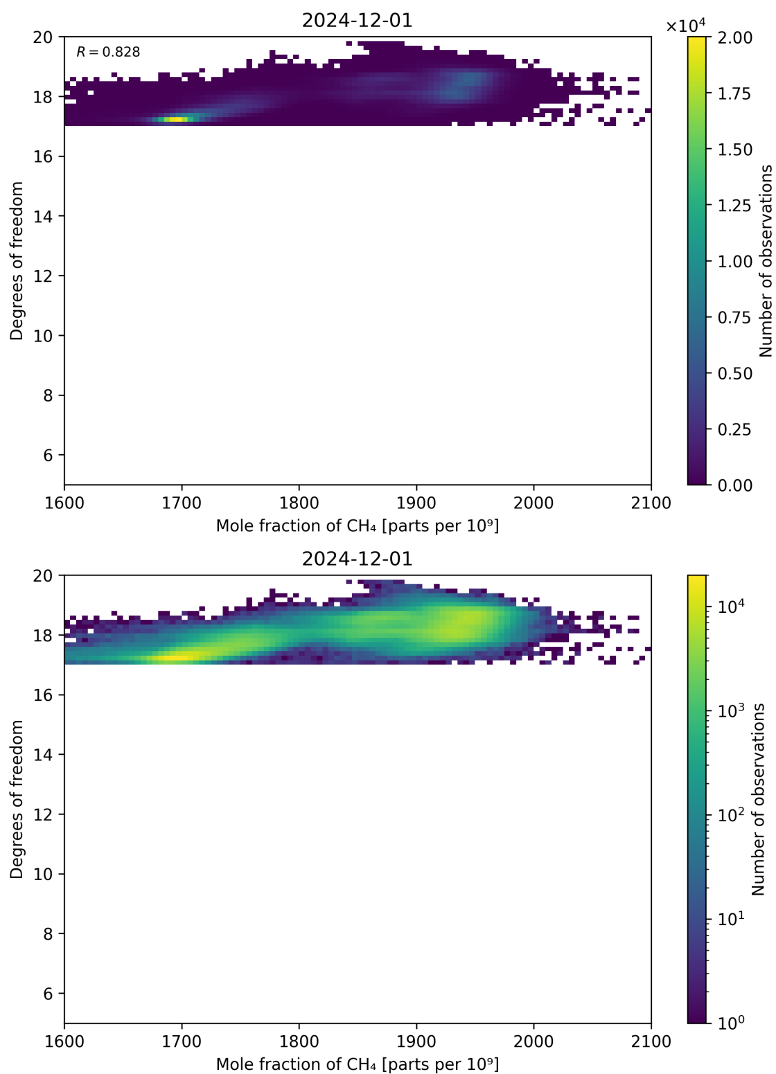
Figure 72: Scatter density plot of “Mole fraction of CH 4 ” against “Degrees of freedom” for 2024-11-30 to 2024-12-02.
