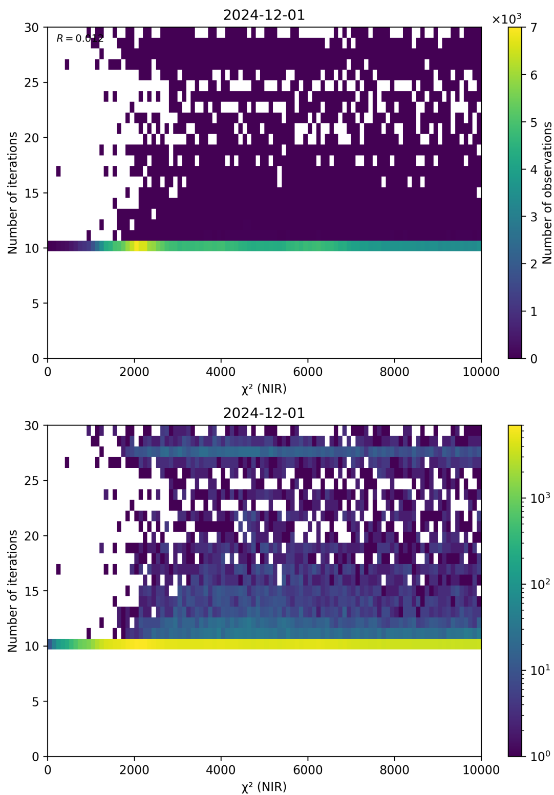
Figure 46: Scatter density plot of “ \chi^2 (NIR)” against “Number of iterations” for 2024-11-30 to 2024-12-02.
