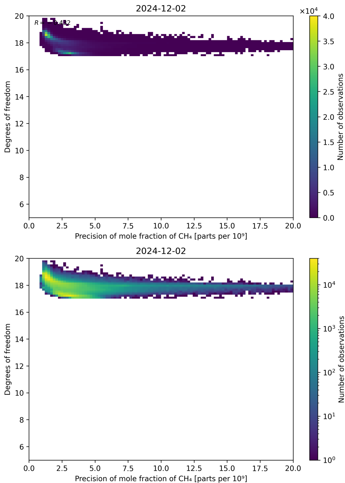
Figure 80: Scatter density plot of “Precision of mole fraction of CH 4 ” against “Degrees of freedom” for 2024-12-01 to 2024-12-03.
