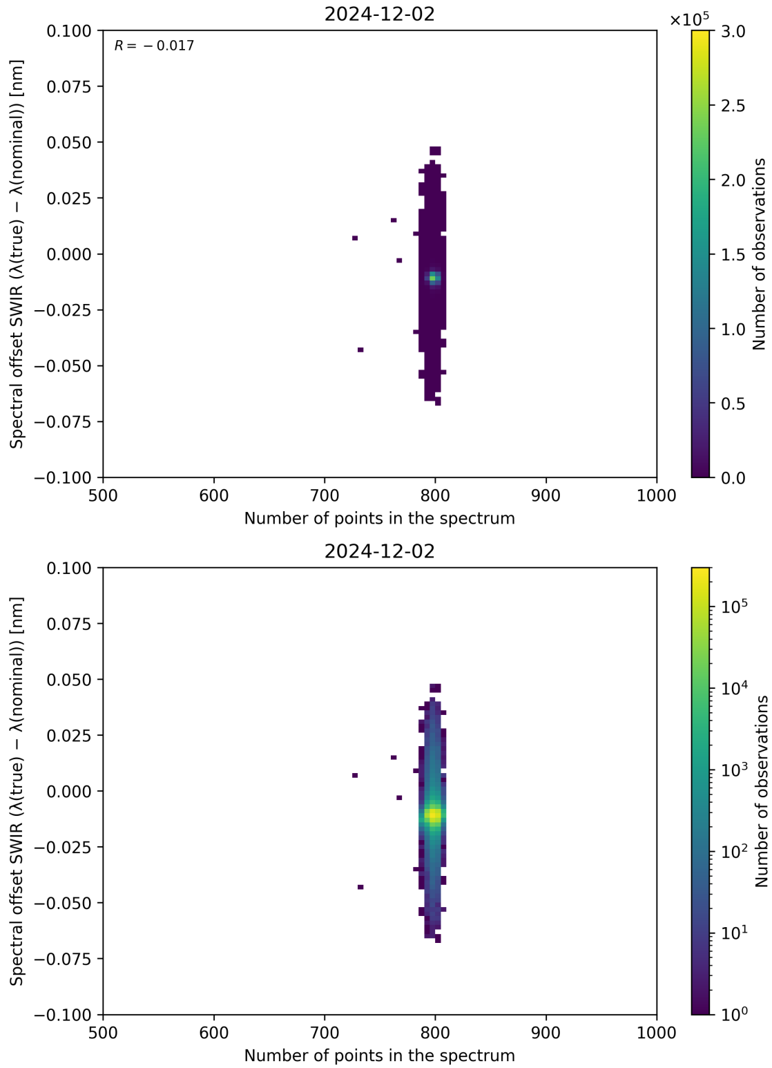
Figure 93: Scatter density plot of “Number of points in the spectrum” against “Spectral offset SWIR ( \lambda_{\text{true}} - \lambda_{\text{nominal}} )” for 2024-12-01 to 2024-12-03.
