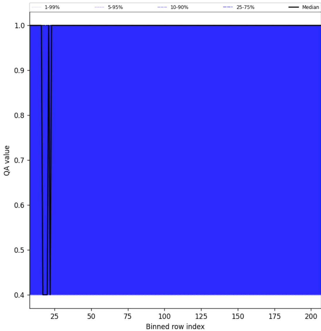
Figure 33: Along track statistics of “QA value” for 2024-12-01 to 2024-12-03
