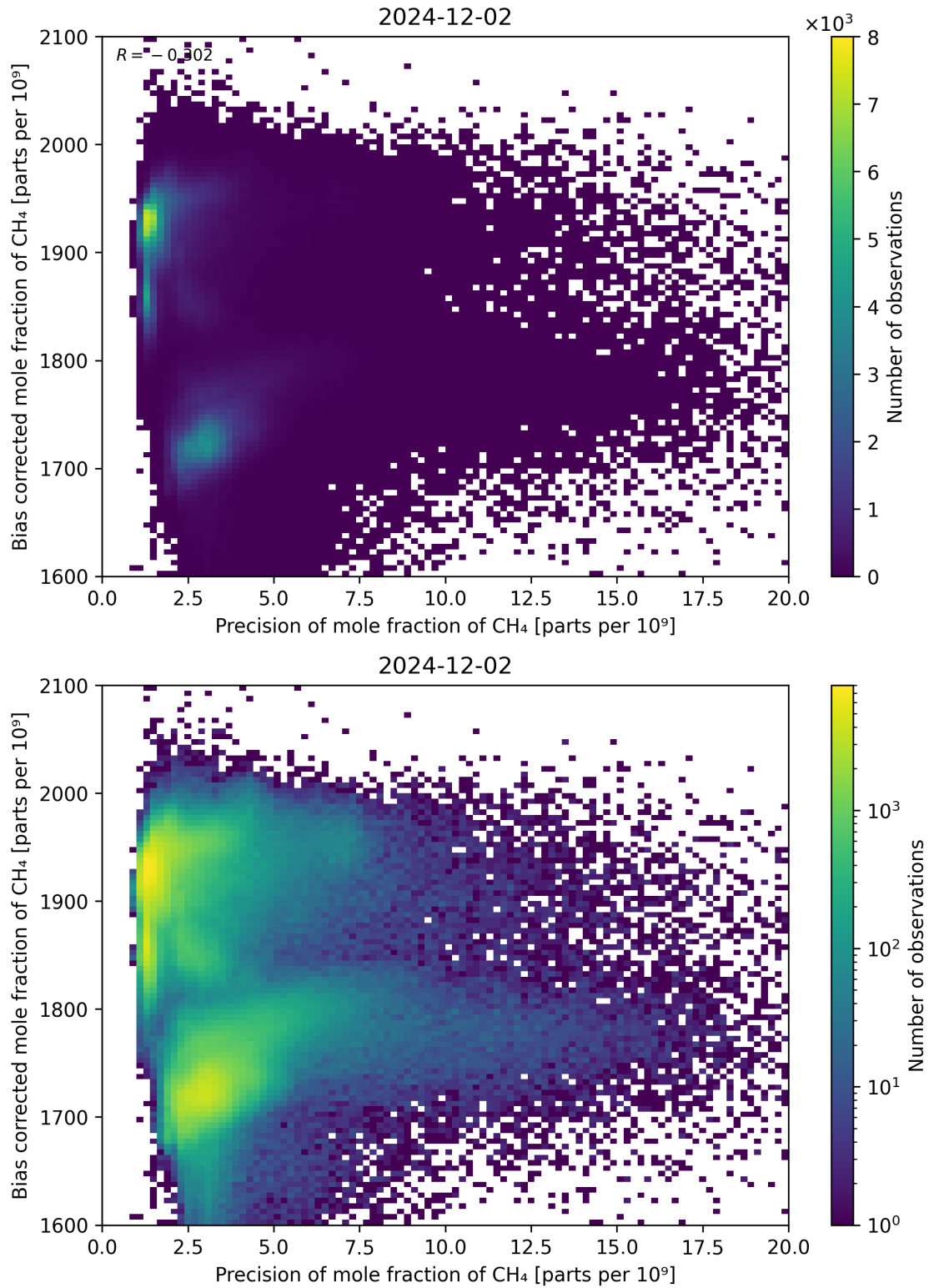
Figure 82: Scatter density plot of “Precision of mole fraction of CH 4 ” against “Bias corrected mole fraction of CH 4 ” for 2024-12-01 to 2024-12-03.
