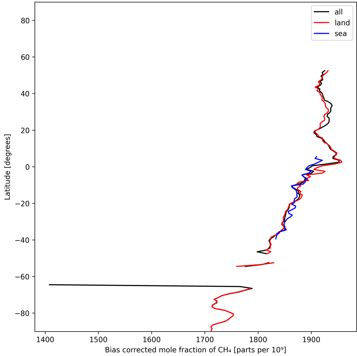
Figure 14: Zonal average of “Bias corrected mole fraction of CH 4 ” for 2024-12-01 to 2024-12-03.
