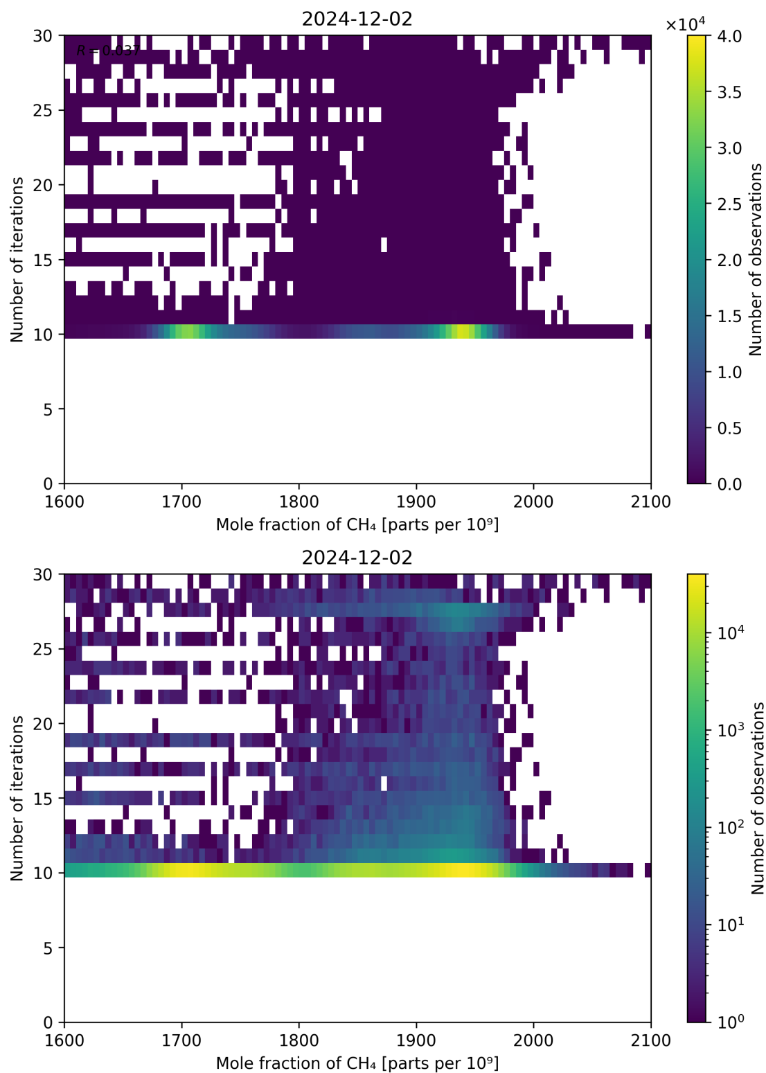
Figure 76: Scatter density plot of “Mole fraction of CH 4 ” against “Number of iterations” for 2024-12-01 to 2024-12-03.
