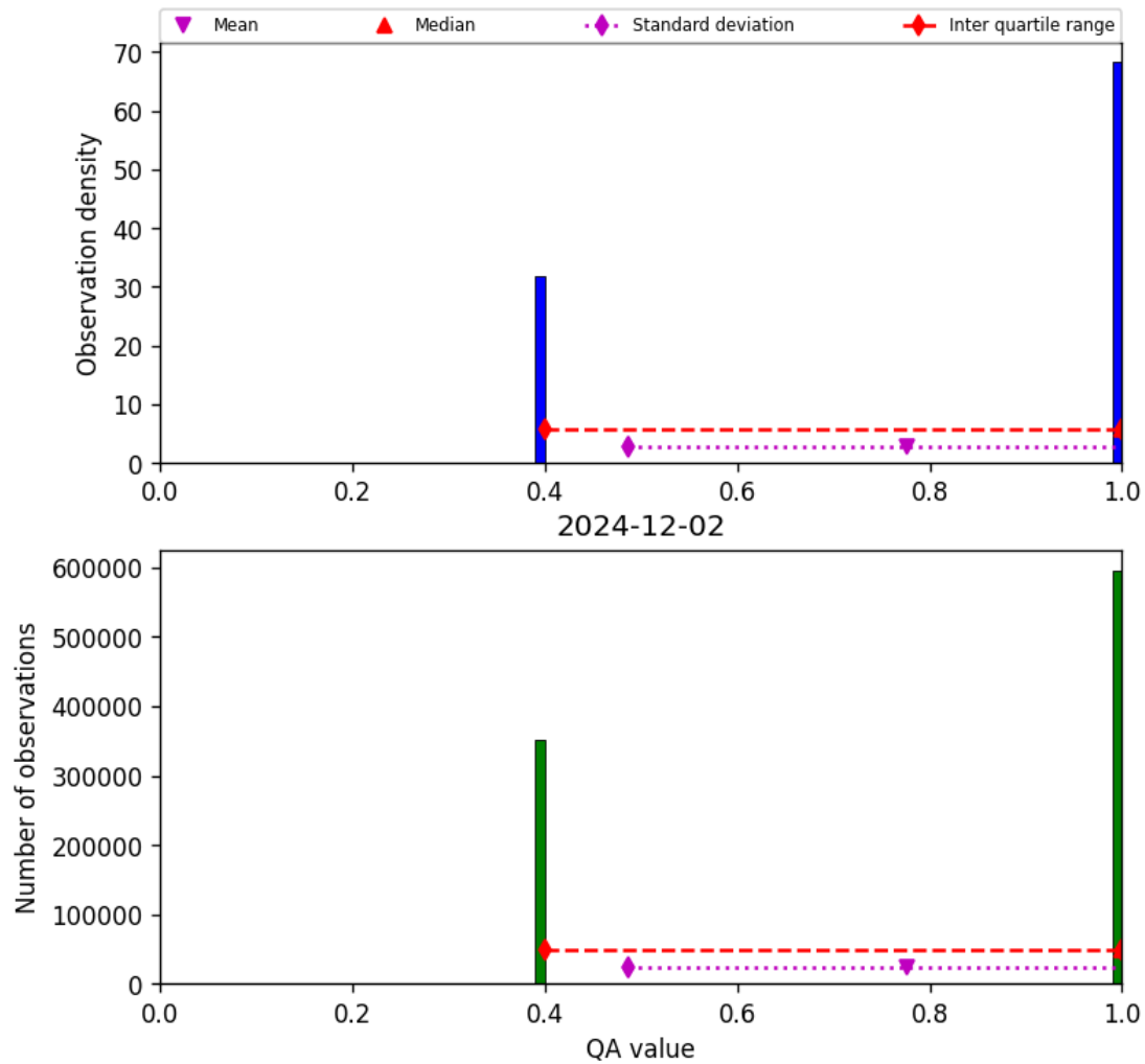
Figure 22: Histogram of “QA value” for 2024-12-01 to 2024-12-03
