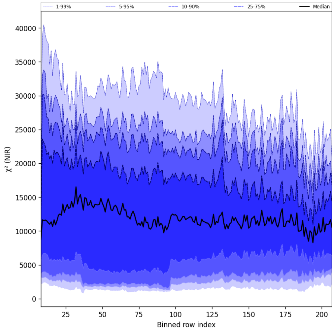
Figure 40: Along track statistics of “ \chi^2 (NIR)” for 2024-12-01 to 2024-12-03
