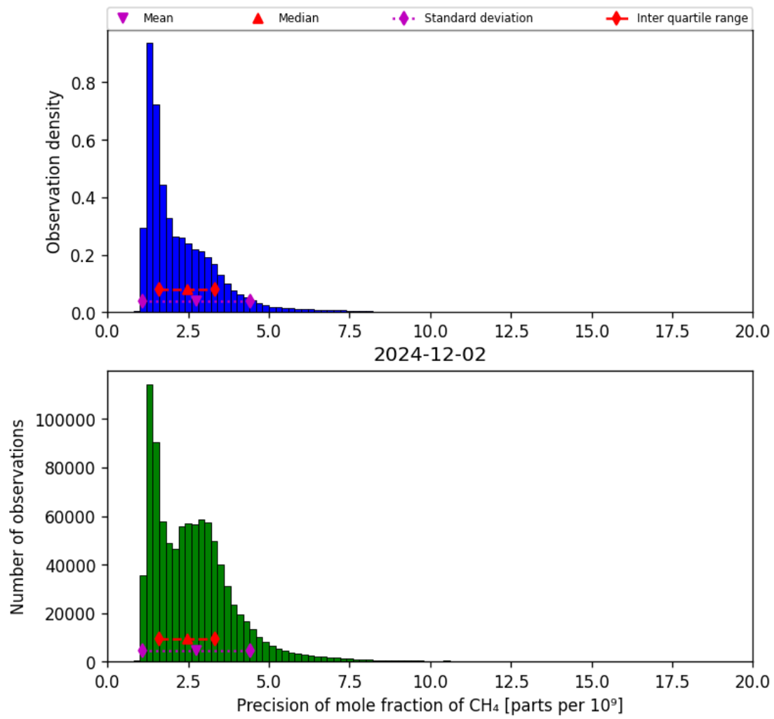
Figure 24: Histogram of “Precision of mole fraction of CH 4 ” for 2024-12-01 to 2024-12-03
