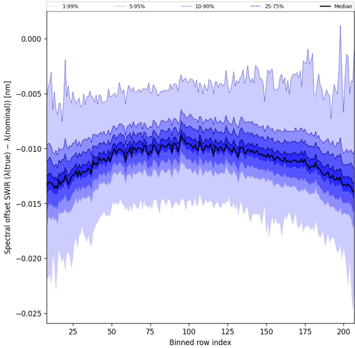
Figure 38: Along track statistics of “Spectral offset SWIR ( \lambda_{\text{true}} - \lambda_{\text{nominal}} )” for 2024-12-01 to 2024-12-03
