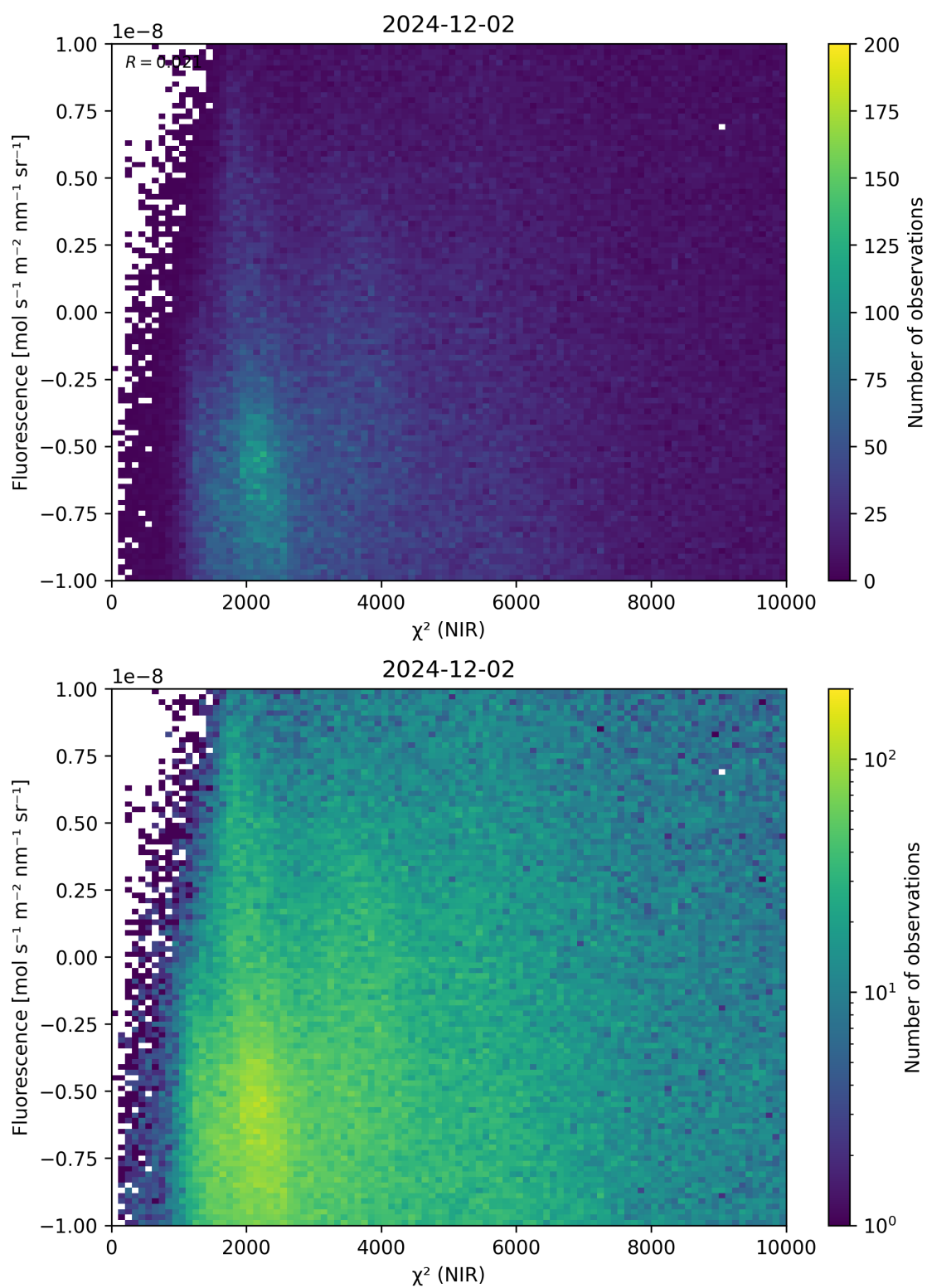
Figure 45: Scatter density plot of “ \chi^2 (NIR)” against “Fluorescence” for 2024-12-01 to 2024-12-03.
