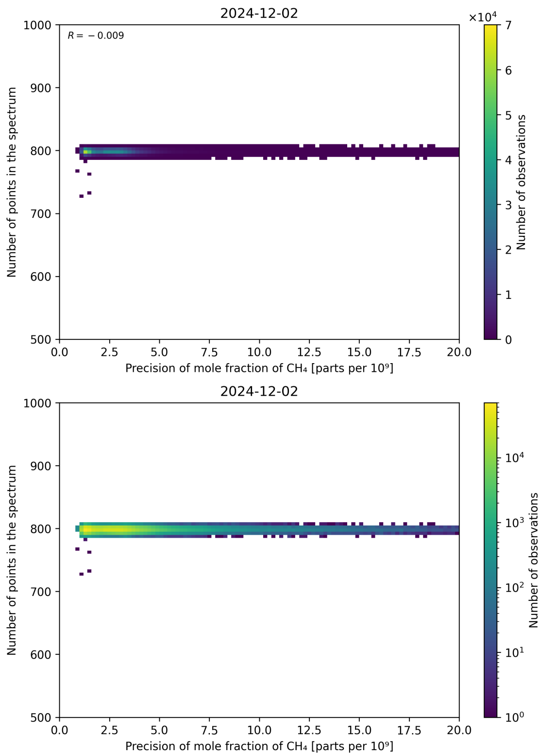
Figure 84: Scatter density plot of “Precision of mole fraction of CH 4 ” against “Number of points in the spectrum” for 2024-12-01 to 2024-12-03.
