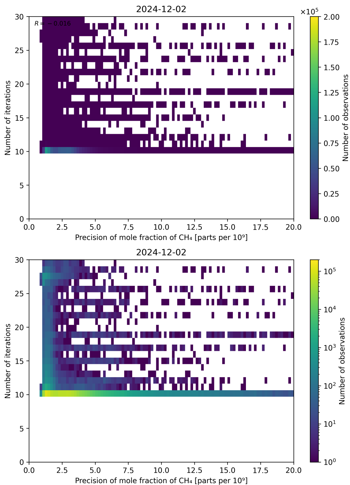
Figure 83: Scatter density plot of “Precision of mole fraction of CH 4 ” against “Number of iterations” for 2024-12-01 to 2024-12-03.
