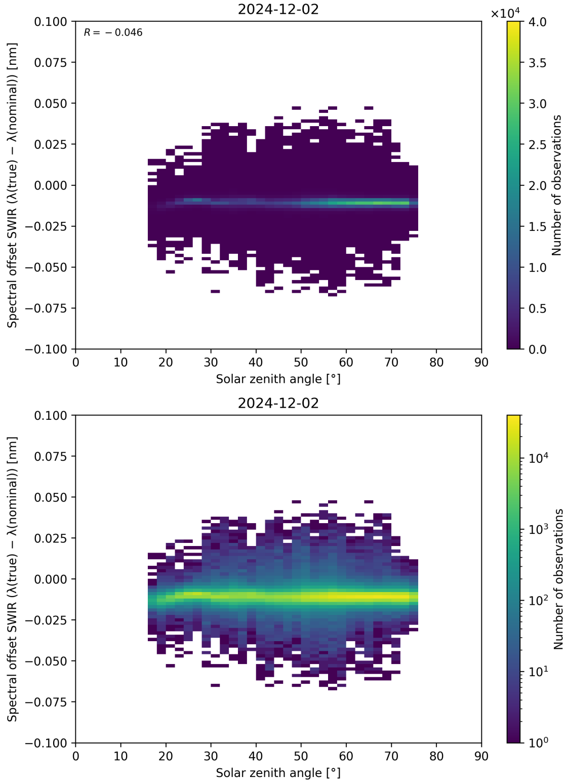
Figure 104: Scatter density plot of “Solar zenith angle” against “Spectral offset SWIR ( \lambda_{\text{true}} - \lambda_{\text{nominal}} )” for 2024-12-01 to 2024-12-03.
