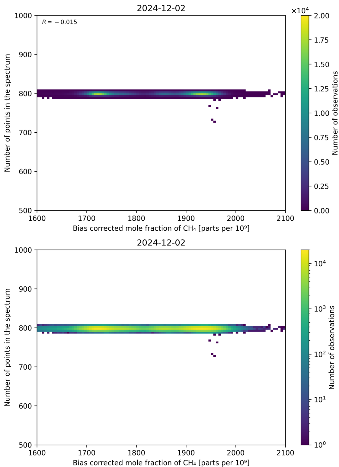
Figure 68: Scatter density plot of “Bias corrected mole fraction of CH 4 ” against “Number of points in the spectrum” for 2024-12-01 to 2024-12-03.
