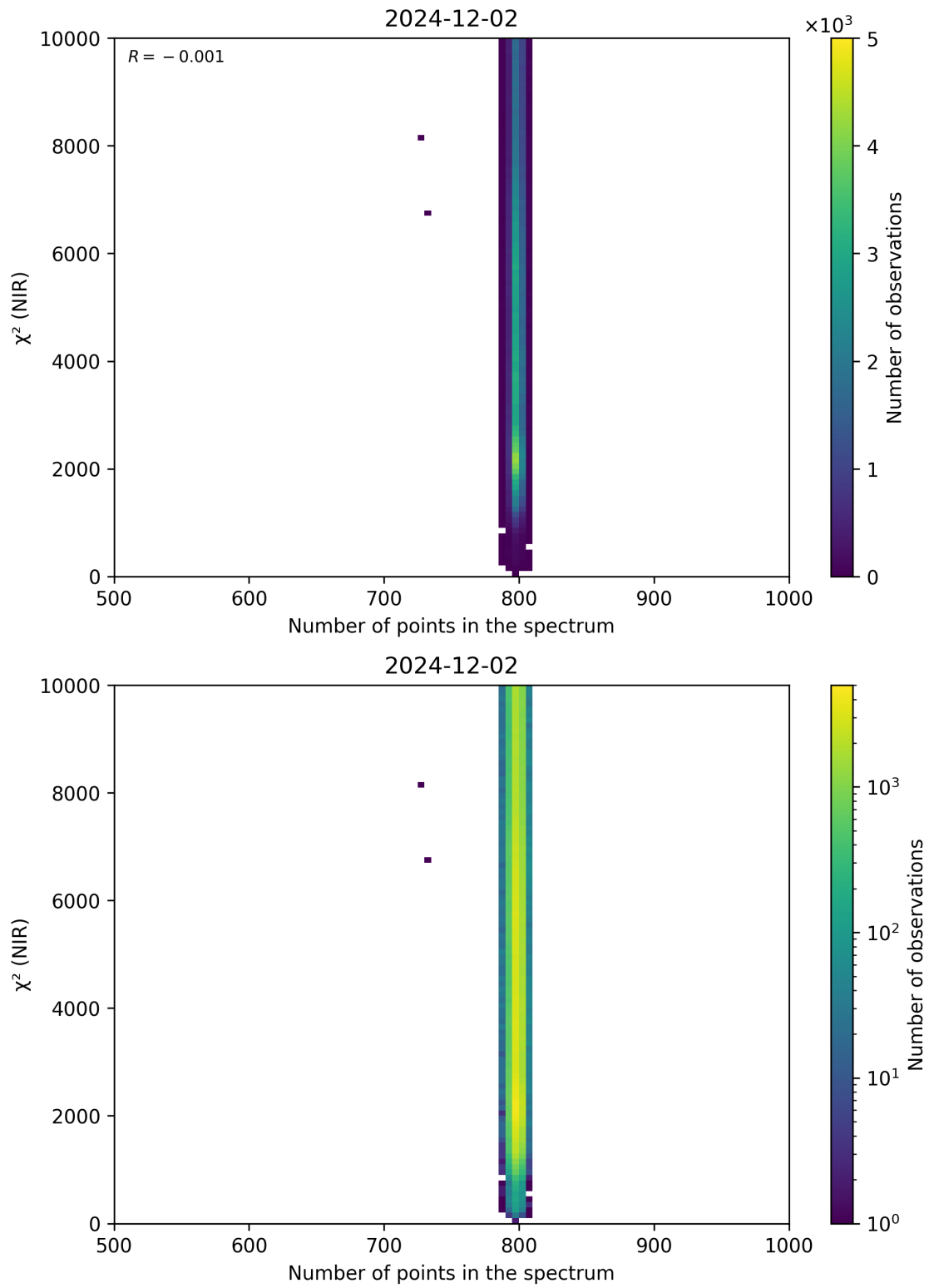
Figure 88: Scatter density plot of “Number of points in the spectrum” against “ \chi^2 (NIR)” for 2024-12-01 to 2024-12-03.
