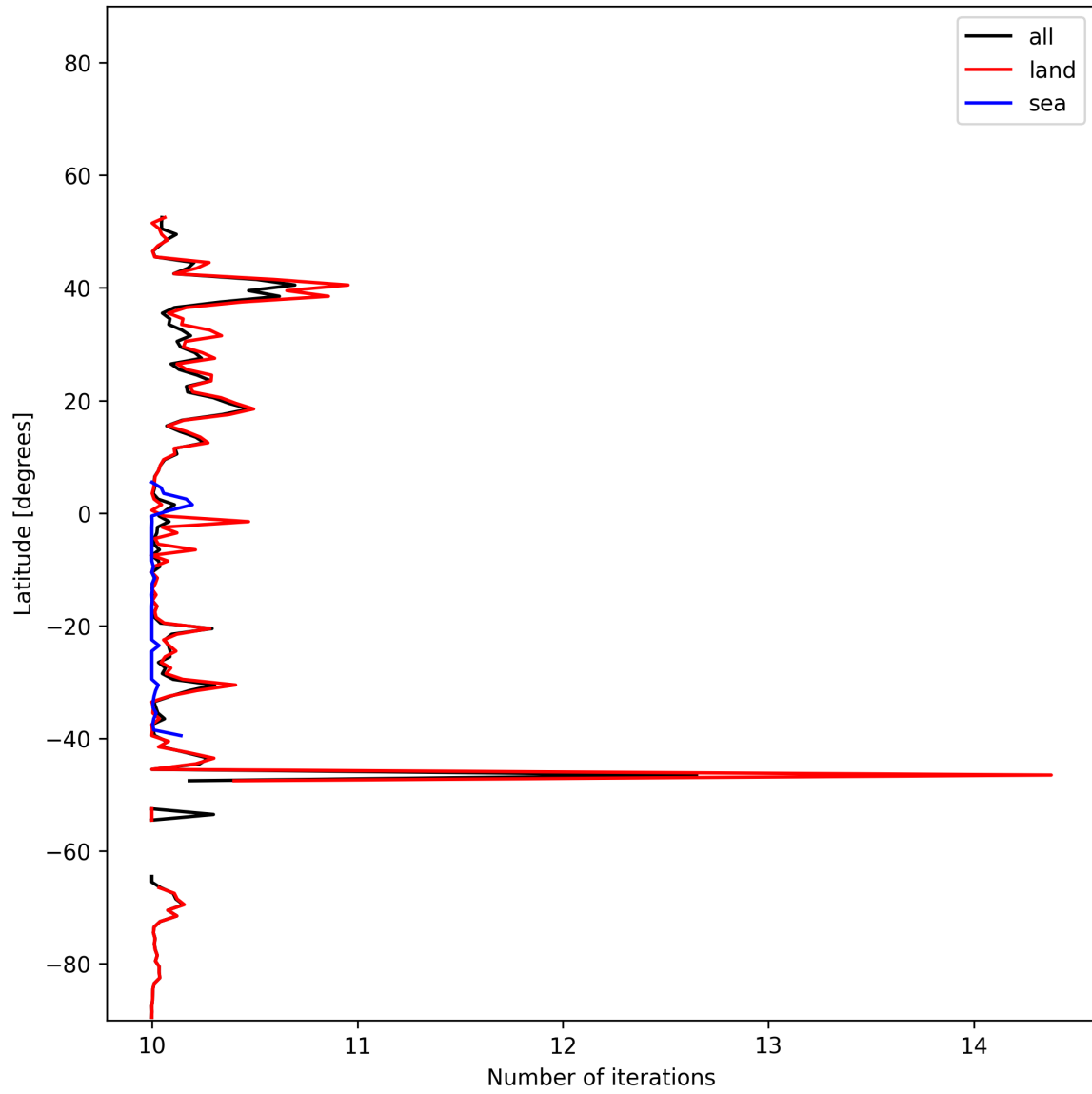
Figure 20: Zonal average of “Number of iterations” for 2024-12-01 to 2024-12-03.
