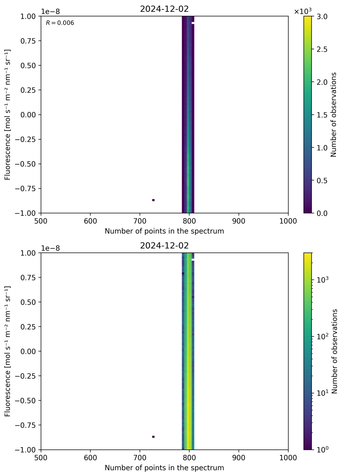
Figure 91: Scatter density plot of “Number of points in the spectrum” against “Fluorescence” for 2024-12-01 to 2024-12-03.
