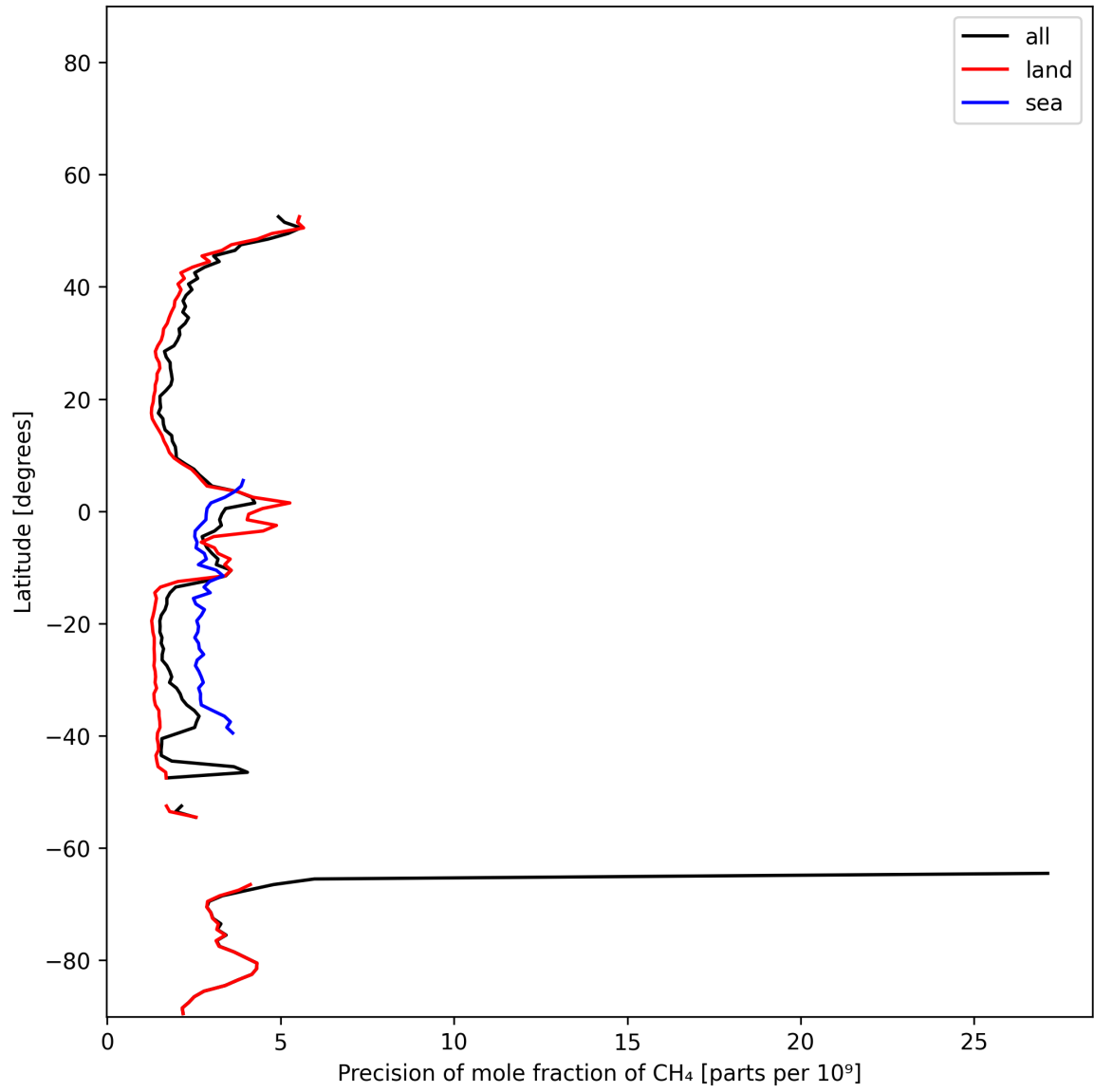
Figure 13: Zonal average of “Precision of mole fraction of \text{CH}_4 ” for 2024-12-01 to 2024-12-03.
