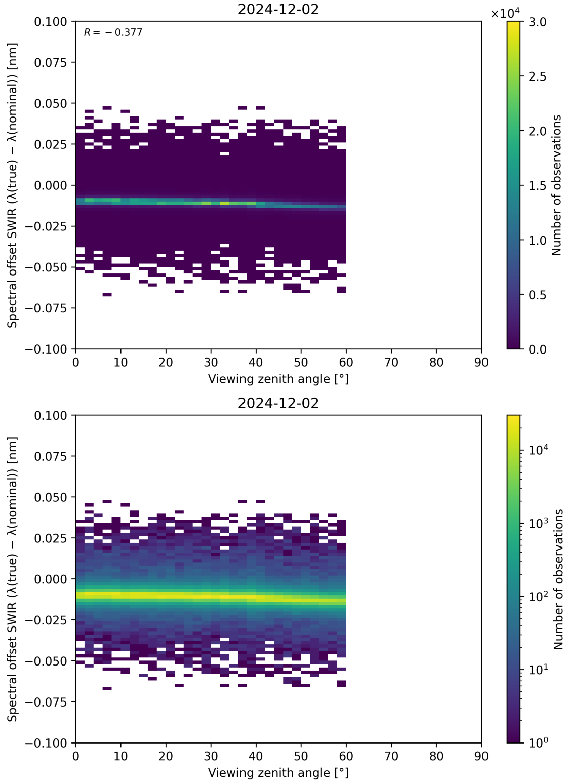
Figure 116: Scatter density plot of “Viewing zenith angle” against “Spectral offset SWIR ( \lambda_{\text{true}} - \lambda_{\text{nominal}} )” for 2024-12-01 to 2024-12-03.
