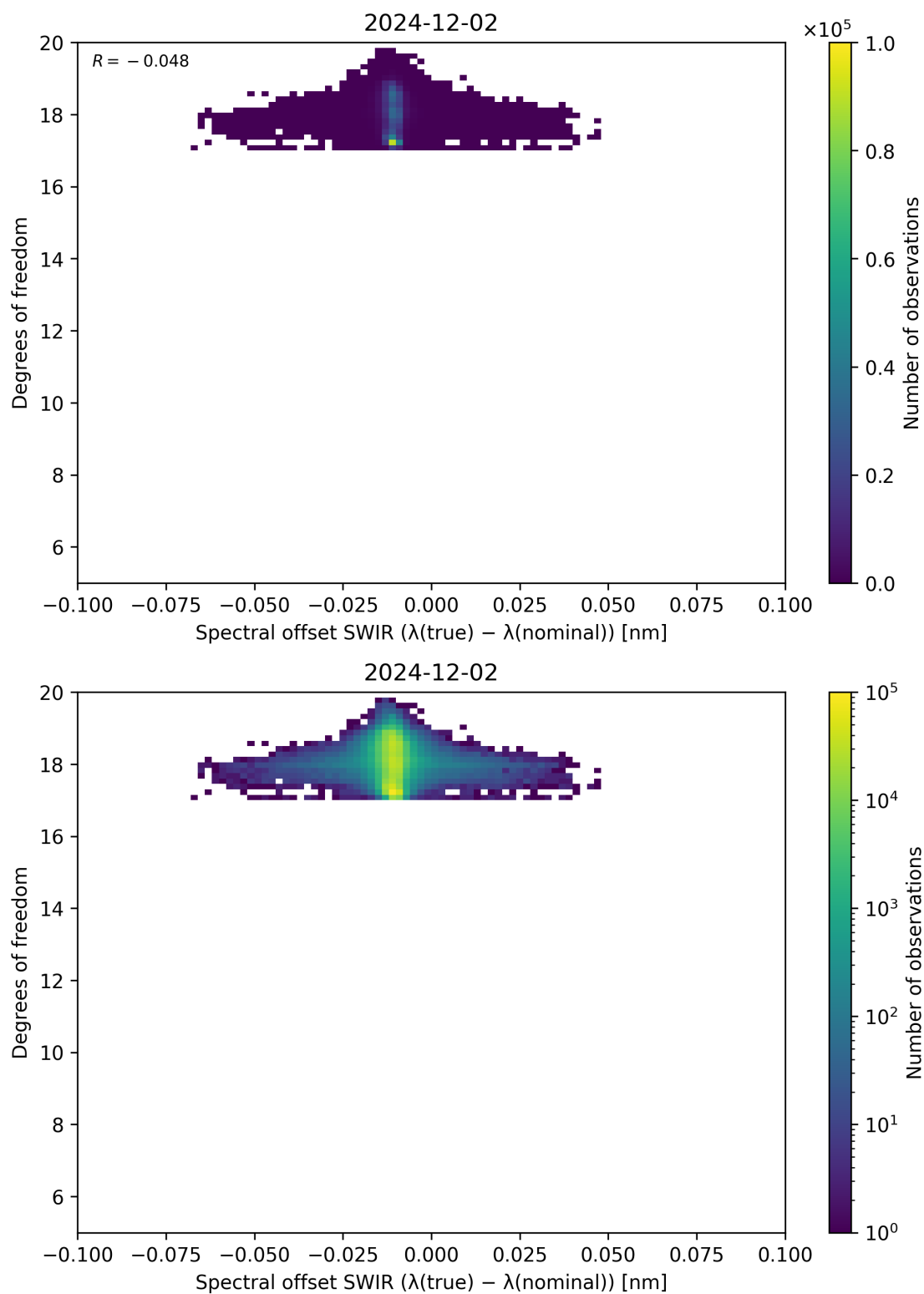
Figure 119: Scatter density plot of “Spectral offset SWIR ( \lambda_{\text{true}} - \lambda_{\text{nominal}} )” against “Degrees of freedom” for 2024-12-01 to 2024-12-03.
