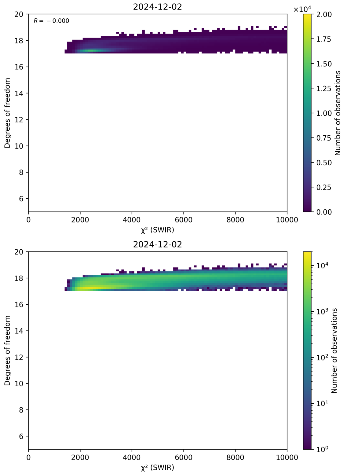
Figure 48: Scatter density plot of “ \chi^2 (SWIR)” against “Degrees of freedom” for 2024-12-01 to 2024-12-03.
