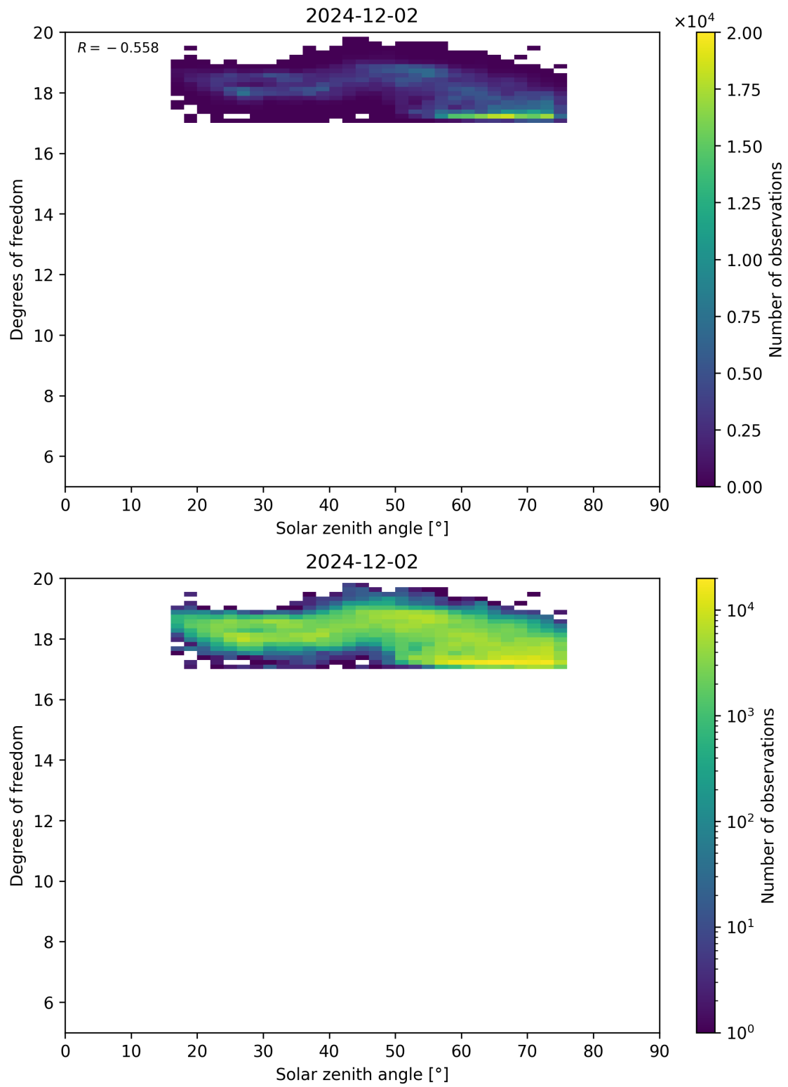
Figure 96: Scatter density plot of “Solar zenith angle” against “Degrees of freedom” for 2024-12-01 to 2024-12-03.
