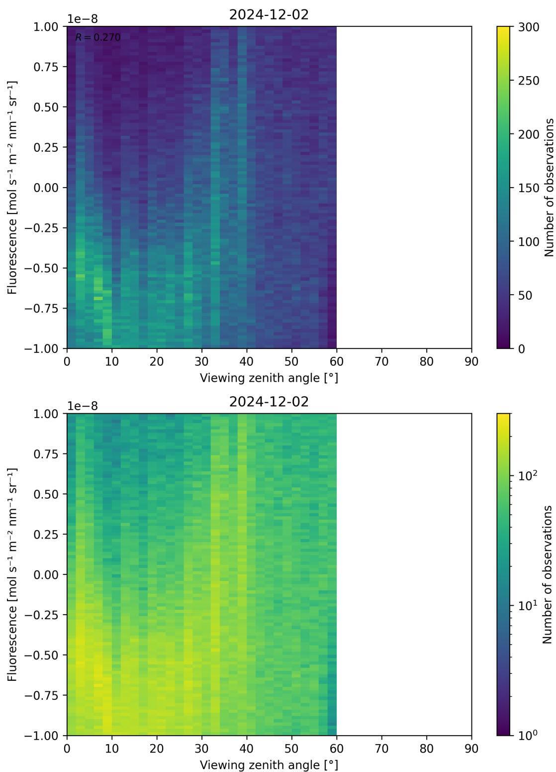
Figure 108: Scatter density plot of “Viewing zenith angle” against “Fluorescence” for 2024-12-01 to 2024-12-03.
