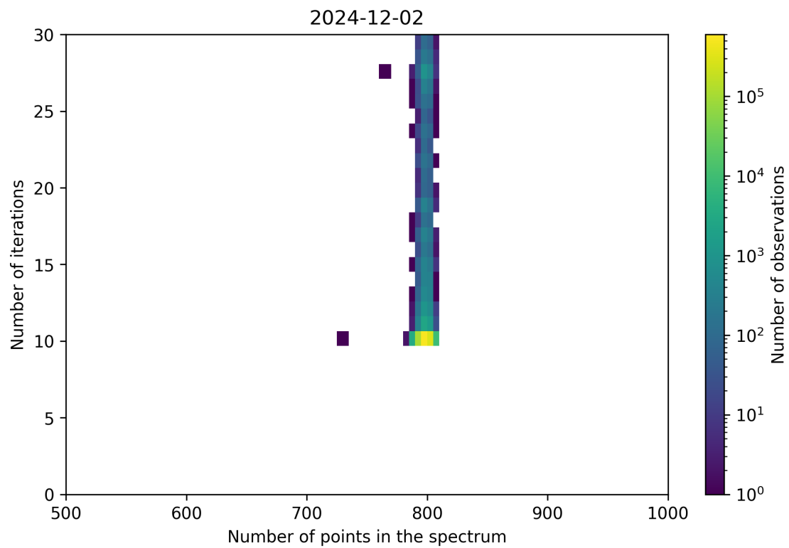
Figure 92: Scatter density plot of “Number of points in the spectrum” against “Number of iterations” for 2024-12-01 to 2024-12-03.
