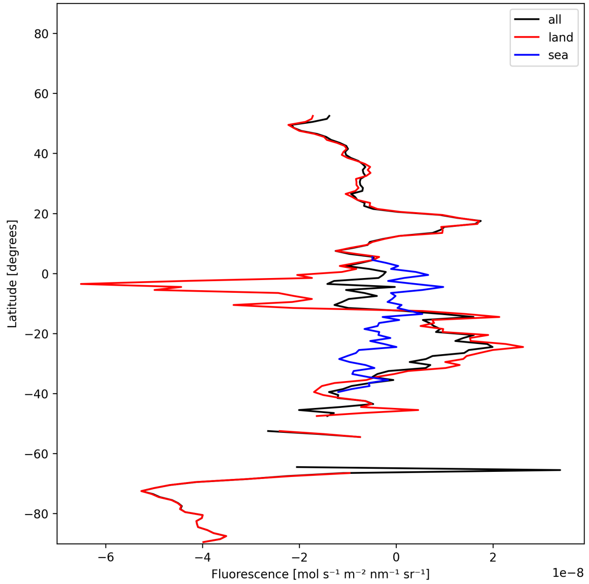
Figure 21: Zonal average of “Fluorescence” for 2024-12-01 to 2024-12-03.
