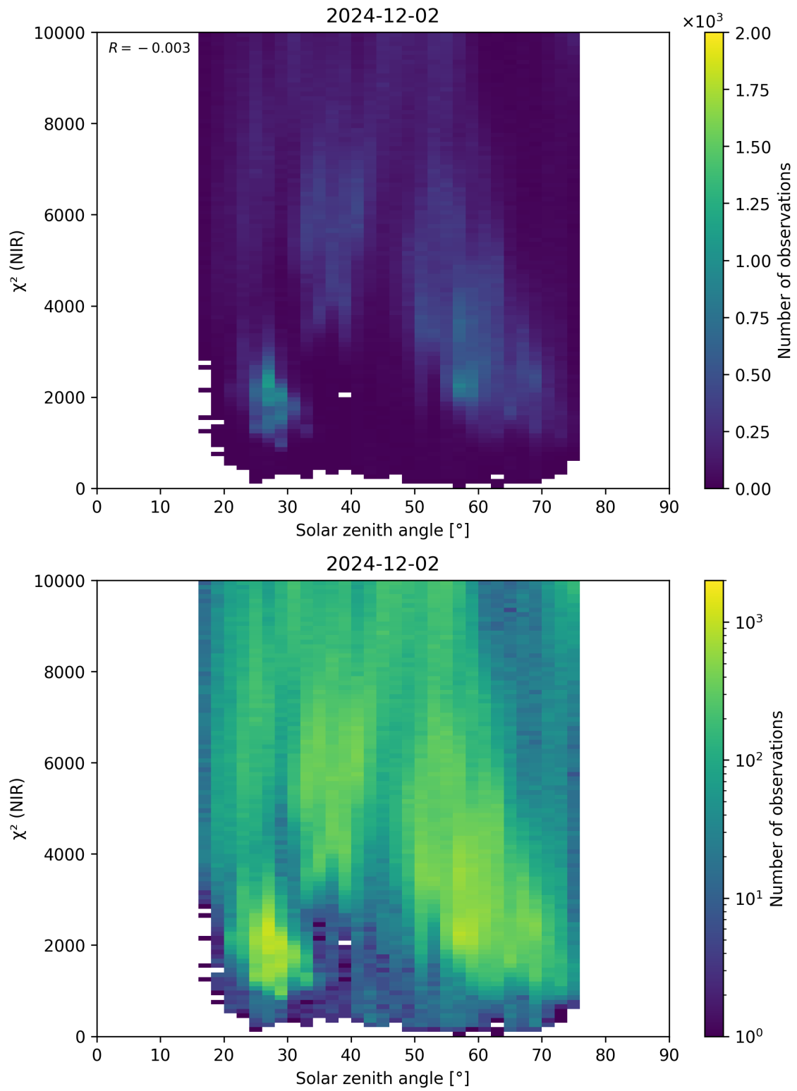
Figure 94: Scatter density plot of “Solar zenith angle” against “ \chi^2 (NIR)” for 2024-12-01 to 2024-12-03.
