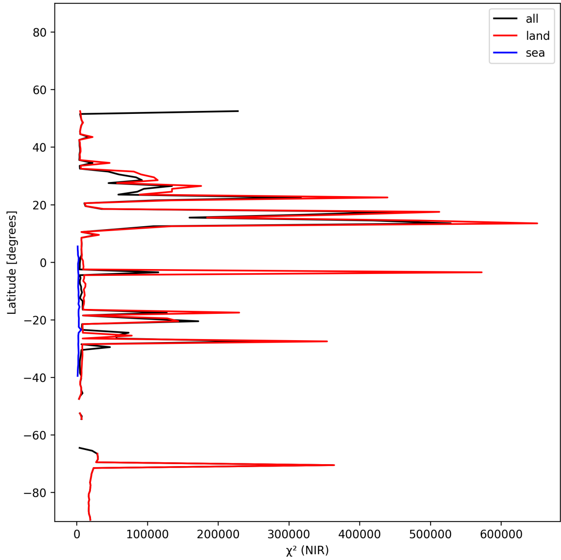
Figure 18: Zonal average of “ \chi^2 (NIR)” for 2024-12-01 to 2024-12-03.
