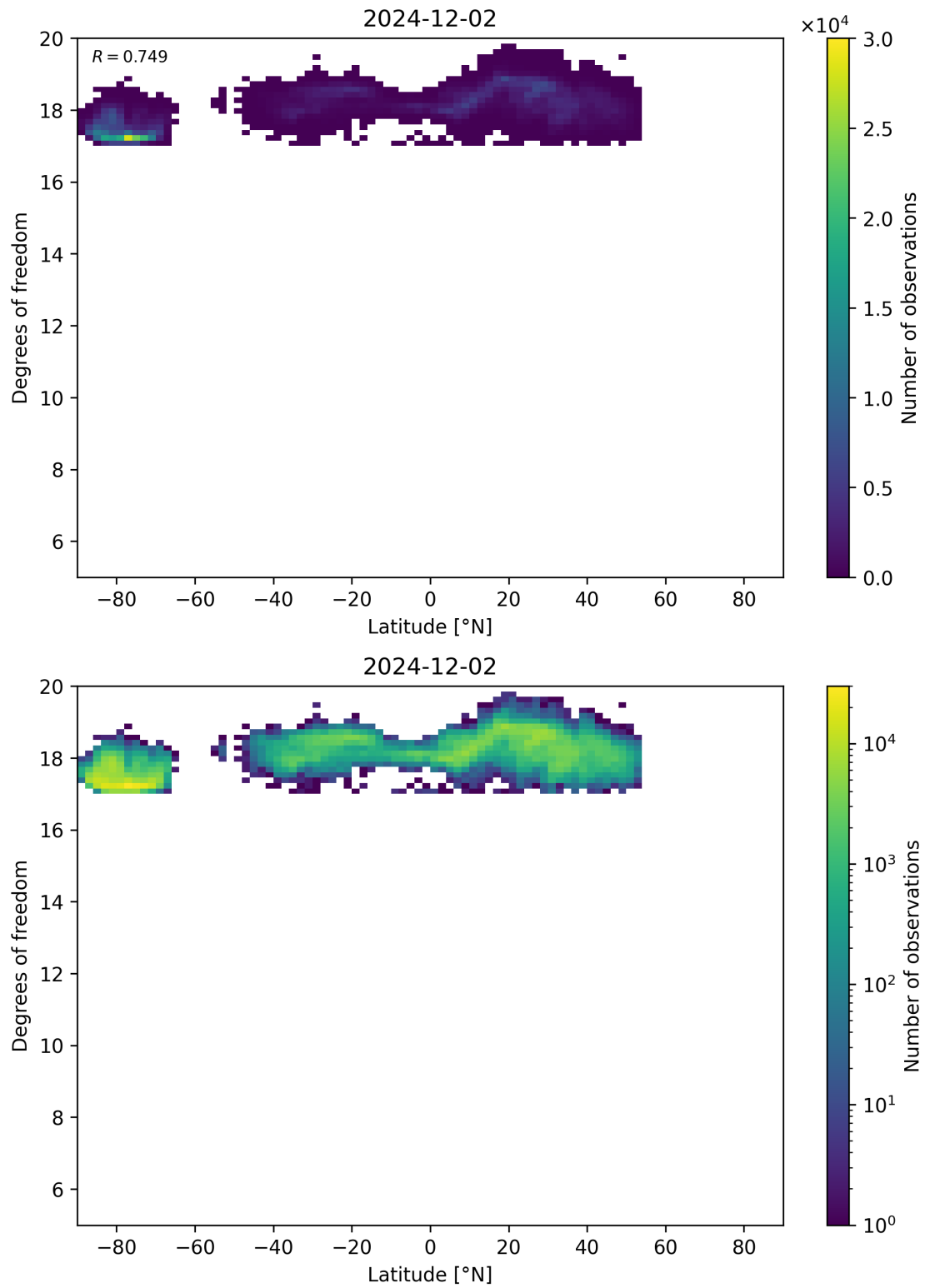
Figure 55: Scatter density plot of “Latitude” against “Degrees of freedom” for 2024-12-01 to 2024-12-03.
