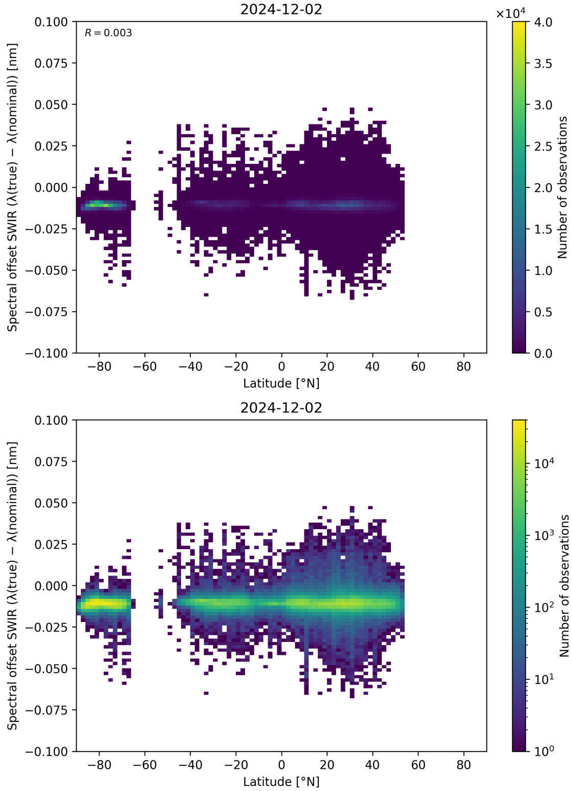
Figure 62: Scatter density plot of “Latitude” against “Spectral offset SWIR ( \lambda_{\text{true}} - \lambda_{\text{nominal}} )” for 2024-12-01 to 2024-12-03.
