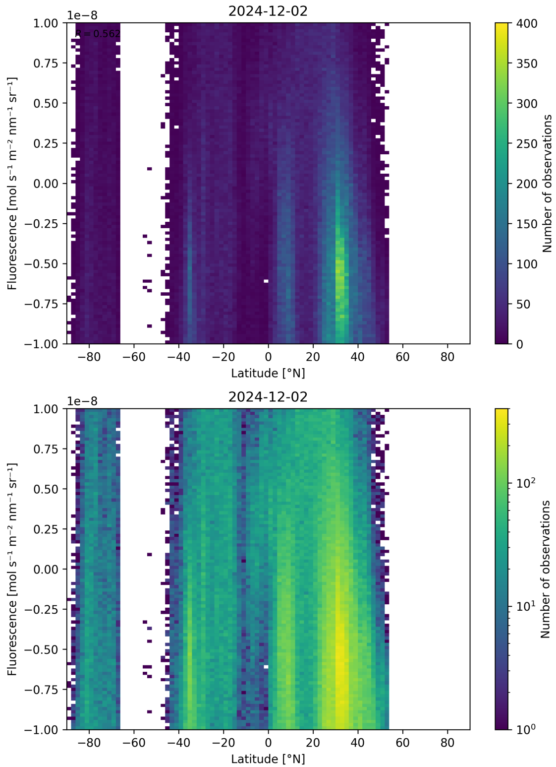
Figure 56: Scatter density plot of “Latitude” against “Fluorescence” for 2024-12-01 to 2024-12-03.
