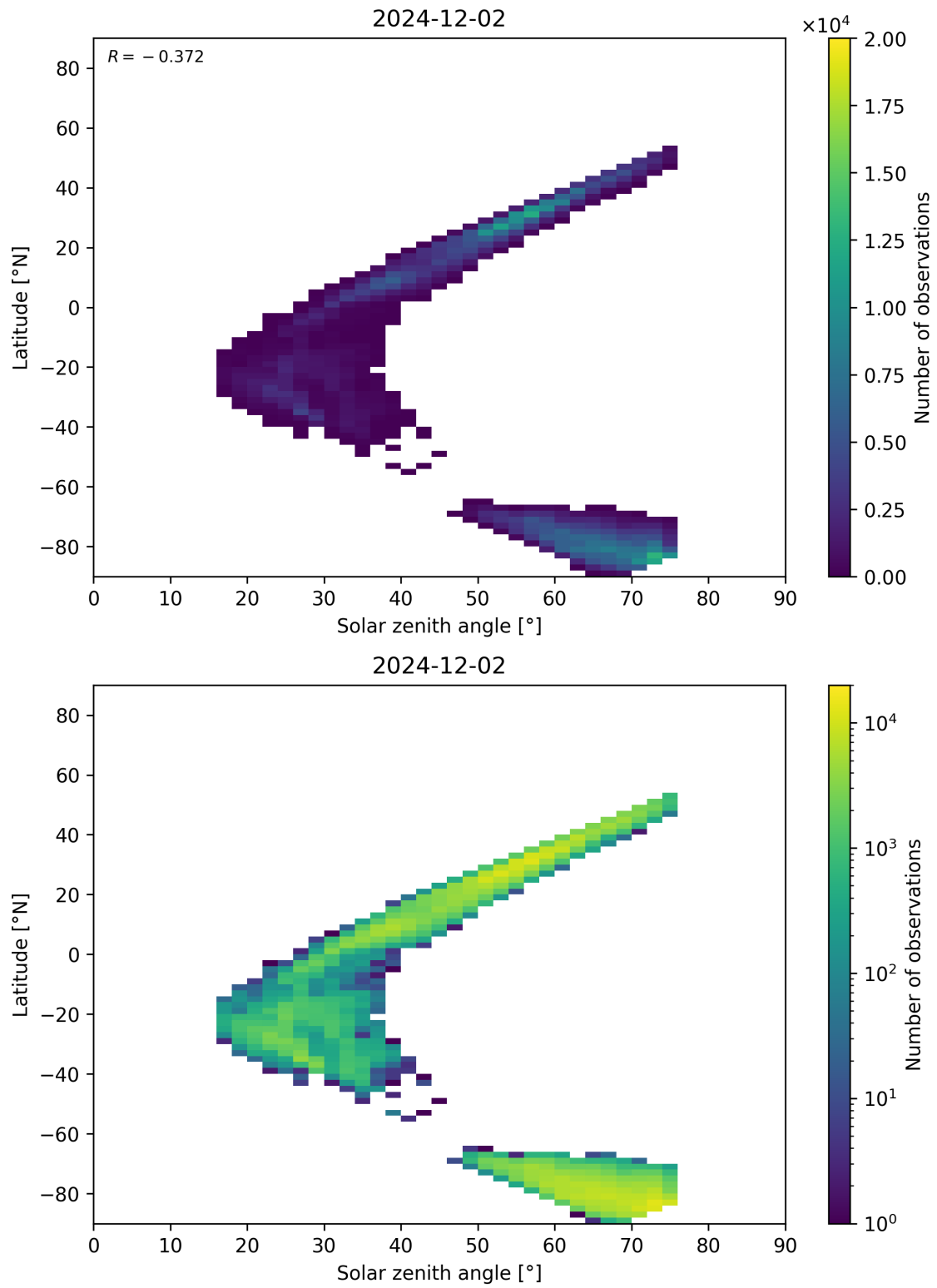
Figure 98: Scatter density plot of “Solar zenith angle” against “Latitude” for 2024-12-01 to 2024-12-03.
