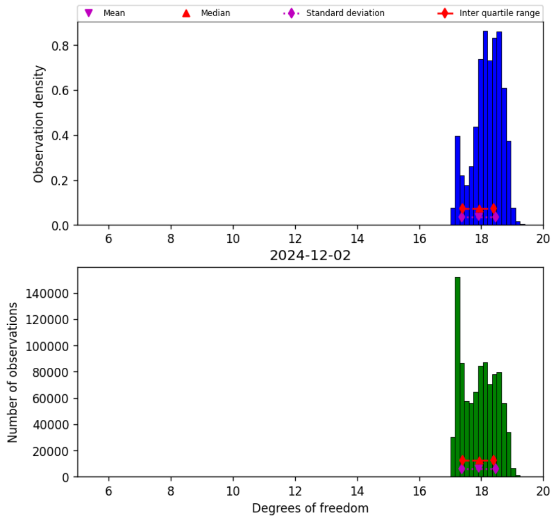
Figure 30: Histogram of “Degrees of freedom” for 2024-12-01 to 2024-12-03
