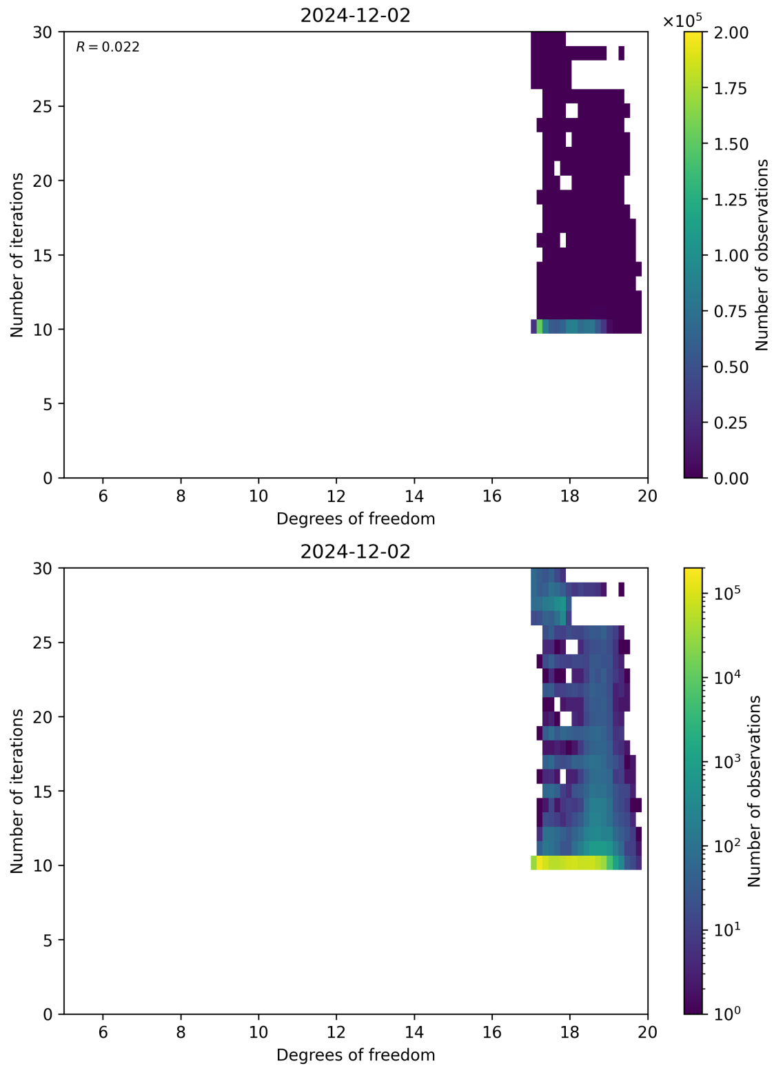
Figure 52: Scatter density plot of “Degrees of freedom” against “Number of iterations” for 2024-12-01 to 2024-12-03.
