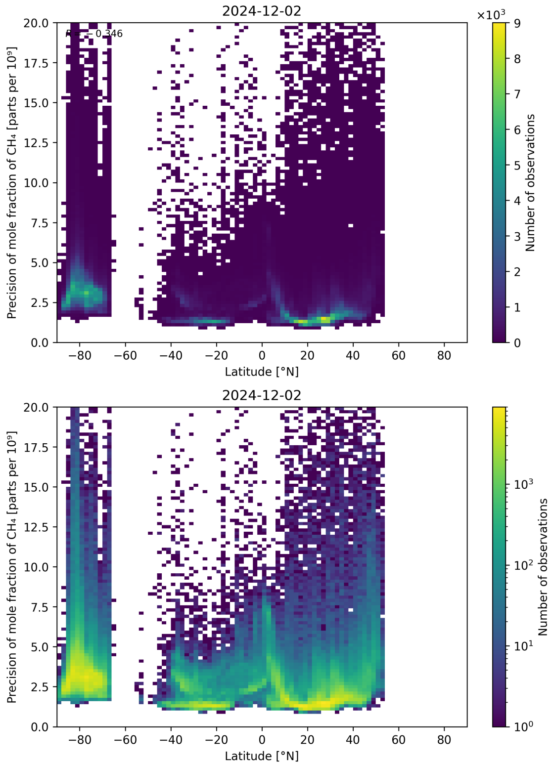
Figure 59: Scatter density plot of “Latitude” against “Precision of mole fraction of CH 4 ” for 2024-12-01 to 2024-12-03.
