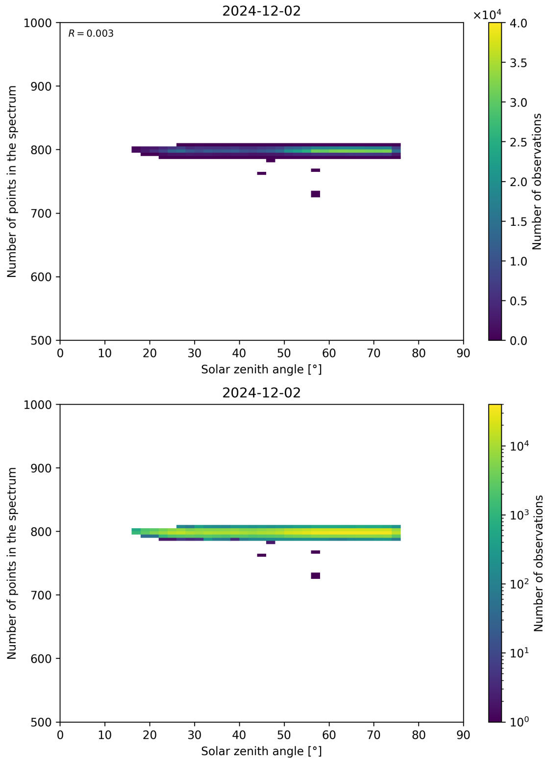
Figure 103: Scatter density plot of “Solar zenith angle” against “Number of points in the spectrum” for 2024-12-01 to 2024-12-03.
