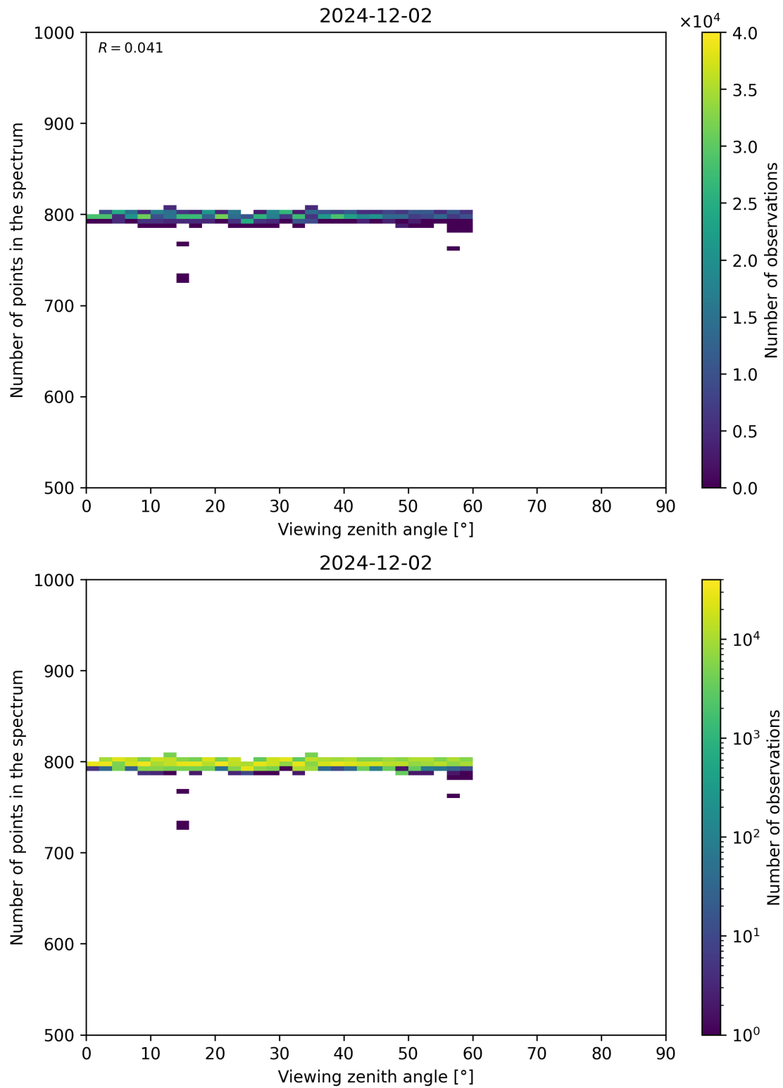
Figure 114: Scatter density plot of “Viewing zenith angle” against “Number of points in the spectrum” for 2024-12-01 to 2024-12-03.
