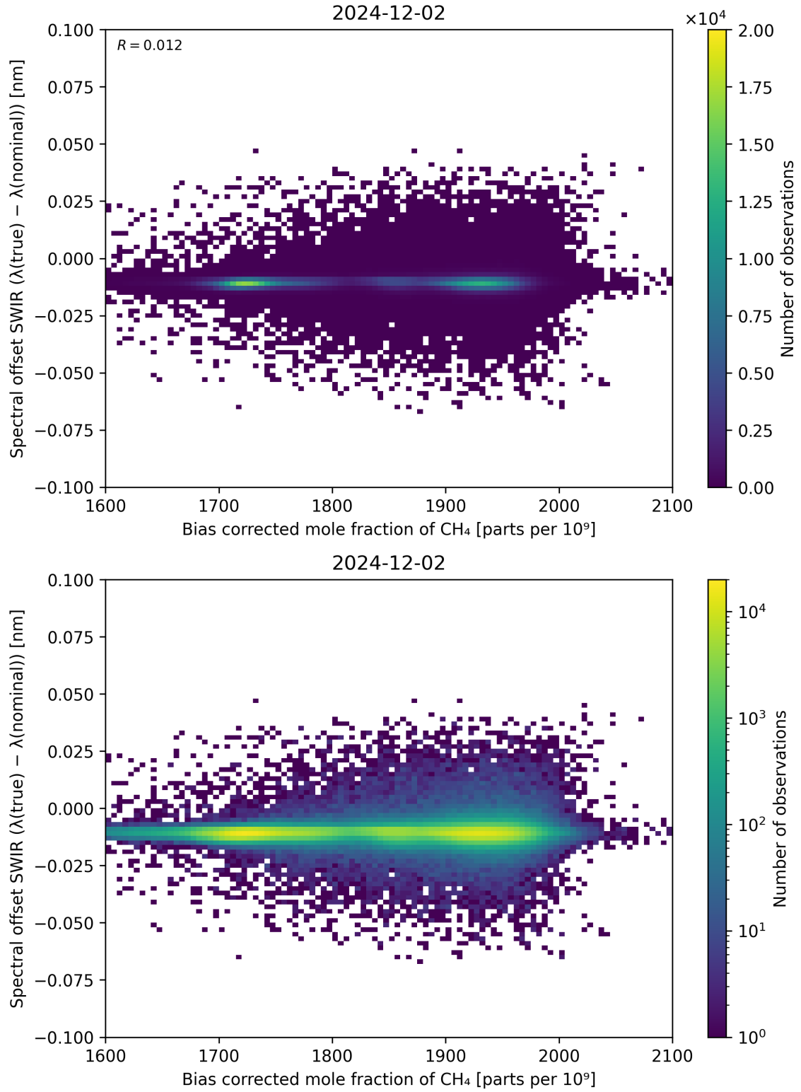
Figure 69: Scatter density plot of “Bias corrected mole fraction of \text{CH}_4 ” against “Spectral offset SWIR ( \lambda_{\text{true}} - \lambda_{\text{nominal}} )” for 2024-12-01 to 2024-12-03.
