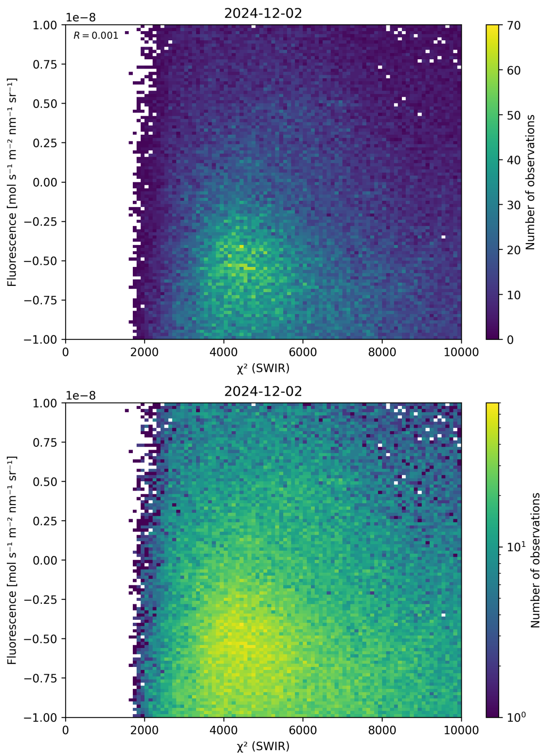
Figure 49: Scatter density plot of “ \chi^2 (SWIR)” against “Fluorescence” for 2024-12-01 to 2024-12-03.
