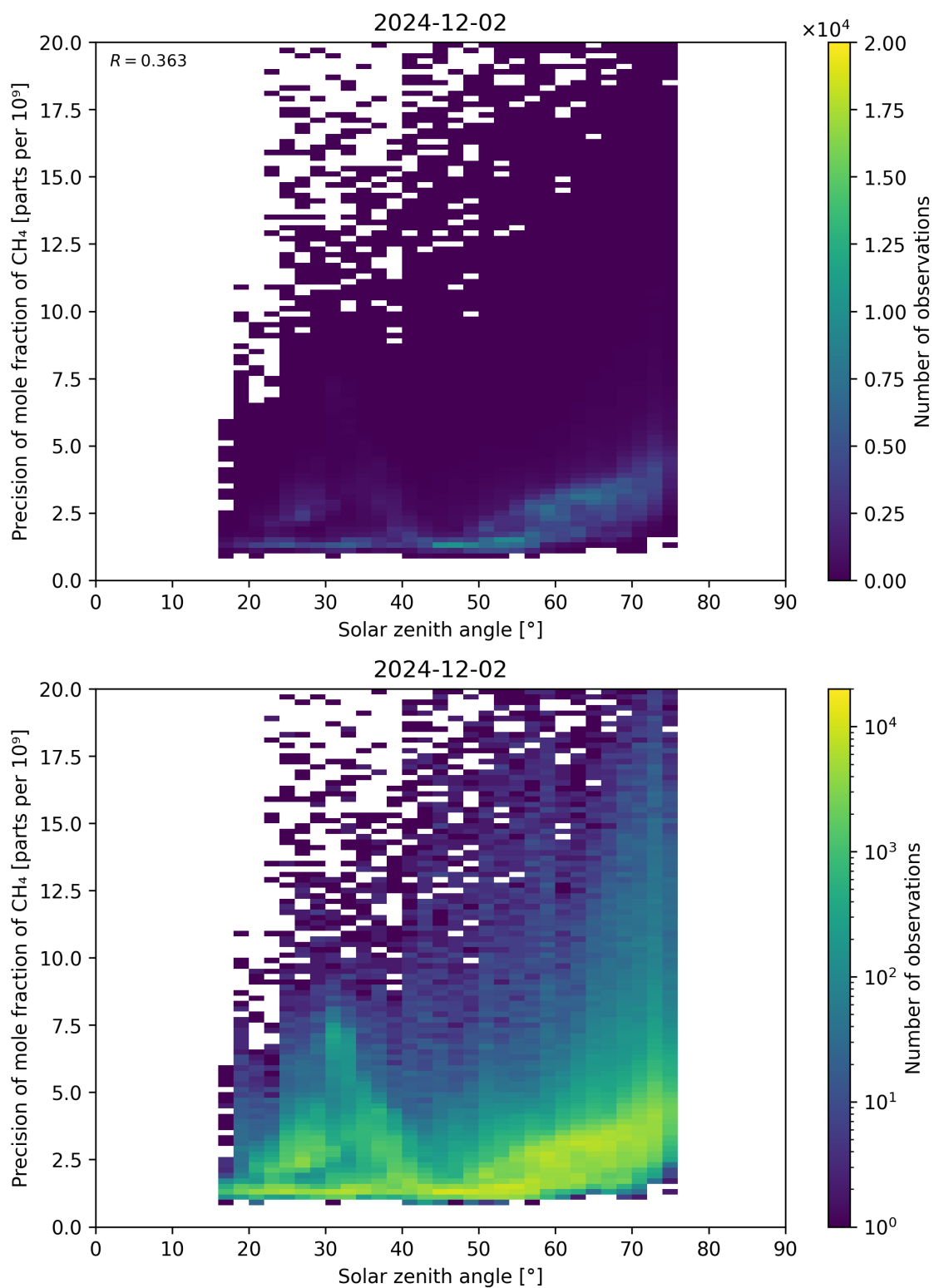
Figure 101: Scatter density plot of “Solar zenith angle” against “Precision of mole fraction of \text{CH}_4 ” for 2024-12-01 to 2024-12-03.
