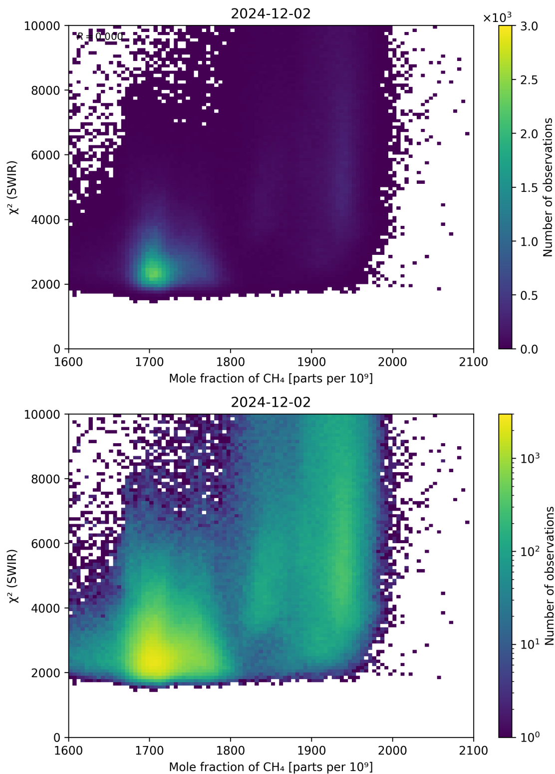
Figure 71: Scatter density plot of “Mole fraction of CH 4 ” against “ \chi^2 (SWIR)” for 2024-12-01 to 2024-12-03.
