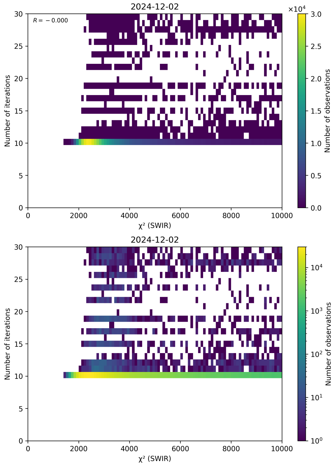
Figure 50: Scatter density plot of “ \chi^2 (SWIR)” against “Number of iterations” for 2024-12-01 to 2024-12-03.
