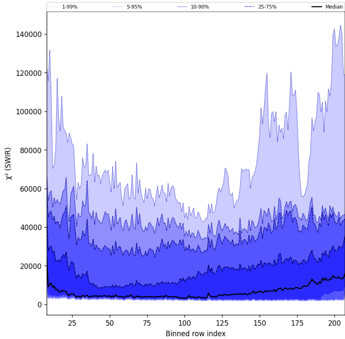
Figure 39: Along track statistics of “ \chi^2 (SWIR)” for 2024-12-01 to 2024-12-03
