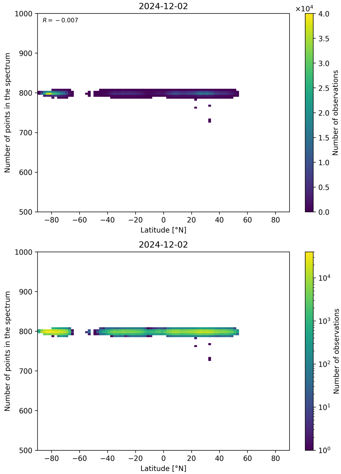
Figure 61: Scatter density plot of “Latitude” against “Number of points in the spectrum” for 2024-12-01 to 2024-12-03.
