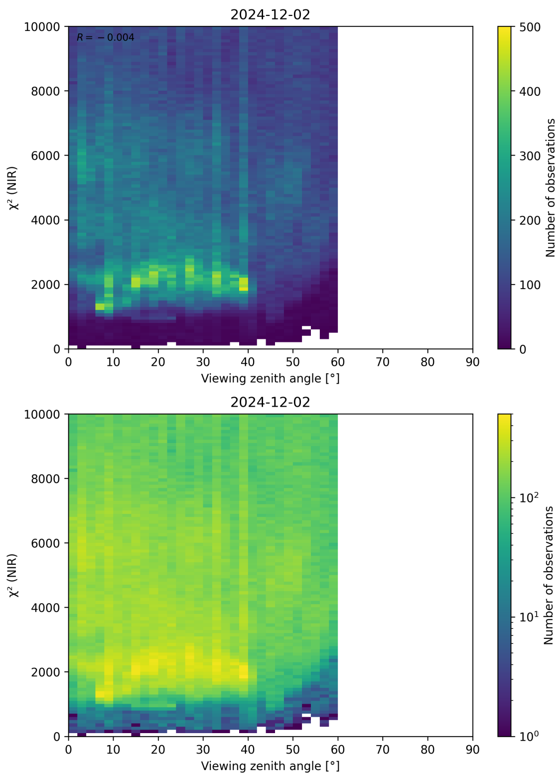
Figure 105: Scatter density plot of “Viewing zenith angle” against “ \chi^2 (NIR)” for 2024-12-01 to 2024-12-03.
