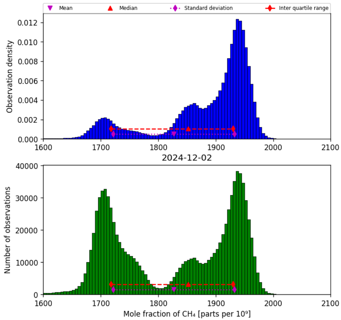
Figure 23: Histogram of “Mole fraction of CH 4 ” for 2024-12-01 to 2024-12-03
