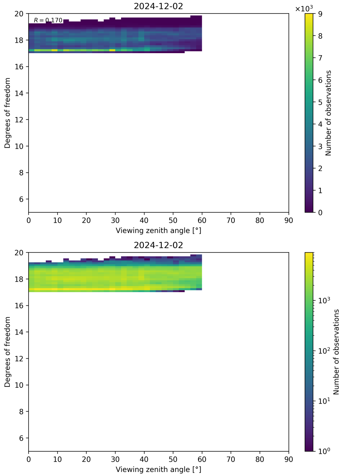
Figure 107: Scatter density plot of “Viewing zenith angle” against “Degrees of freedom” for 2024-12-01 to 2024-12-03.
