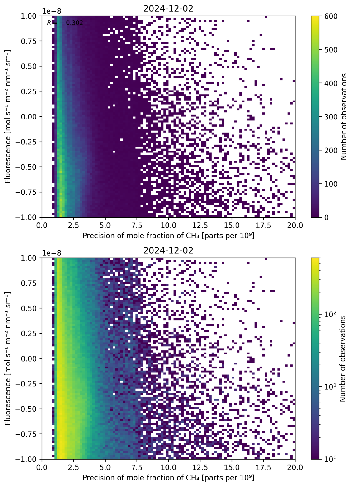
Figure 81: Scatter density plot of “Precision of mole fraction of \text{CH}_4 ” against “Fluorescence” for 2024-12-01 to 2024-12-03.
