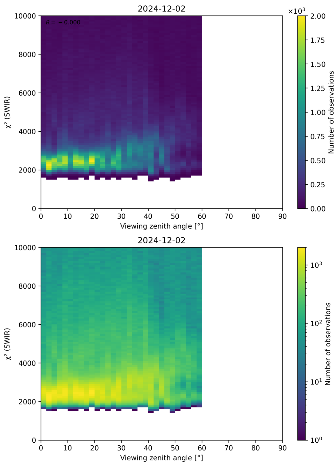
Figure 106: Scatter density plot of “Viewing zenith angle” against “ \chi^2 (SWIR)” for 2024-12-01 to 2024-12-03.
