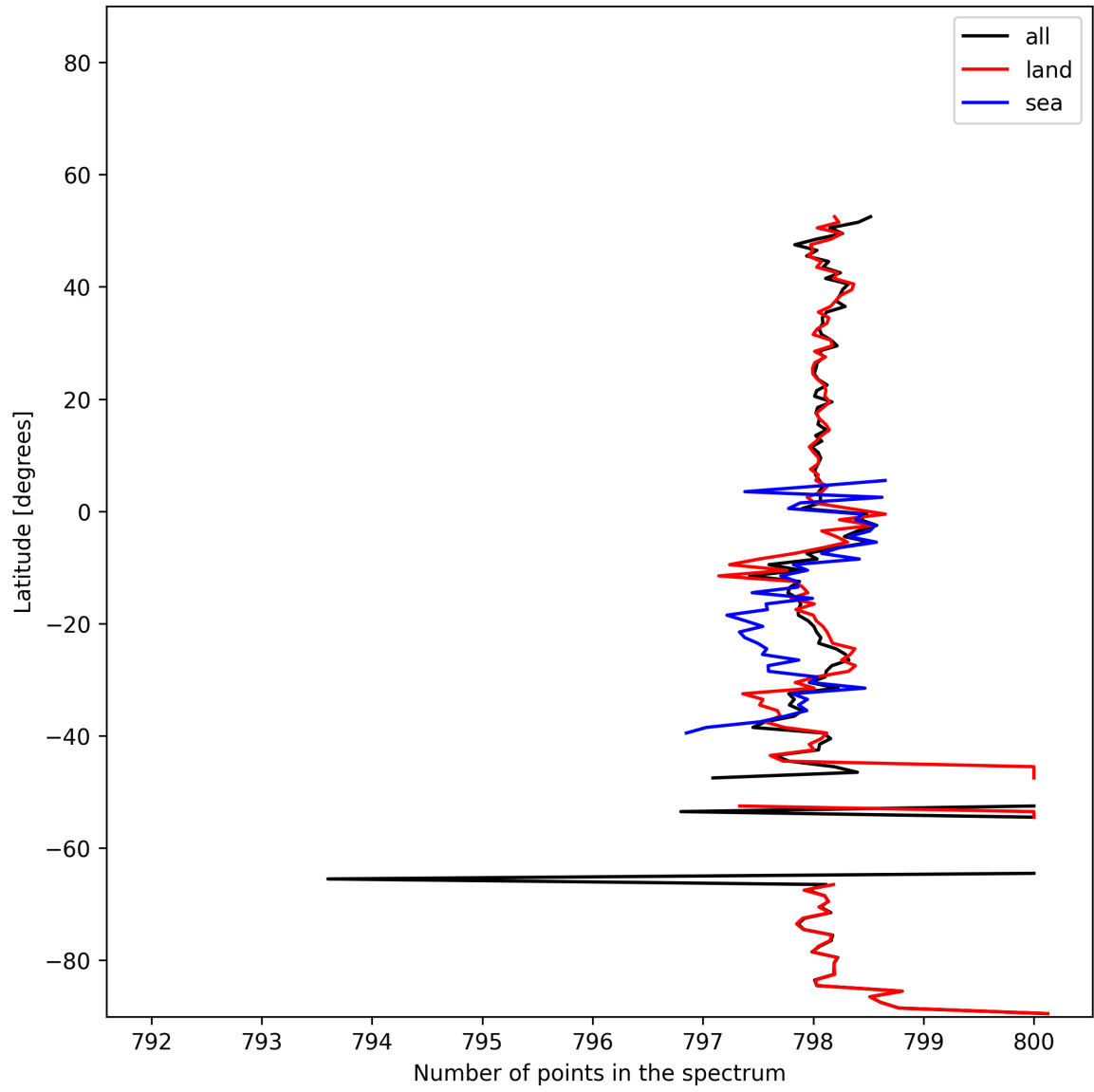
Figure 15: Zonal average of “Number of points in the spectrum” for 2024-12-01 to 2024-12-03.
