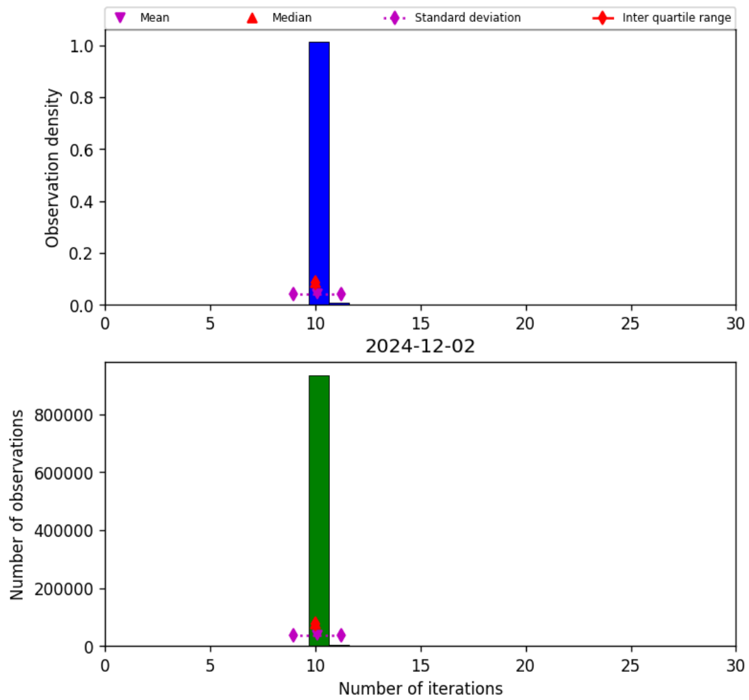
Figure 31: Histogram of “Number of iterations” for 2024-12-01 to 2024-12-03
