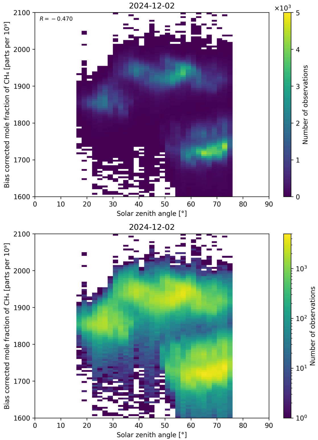
Figure 100: Scatter density plot of “Solar zenith angle” against “Bias corrected mole fraction of CH 4 ” for 2024-12-01 to 2024-12-03.
