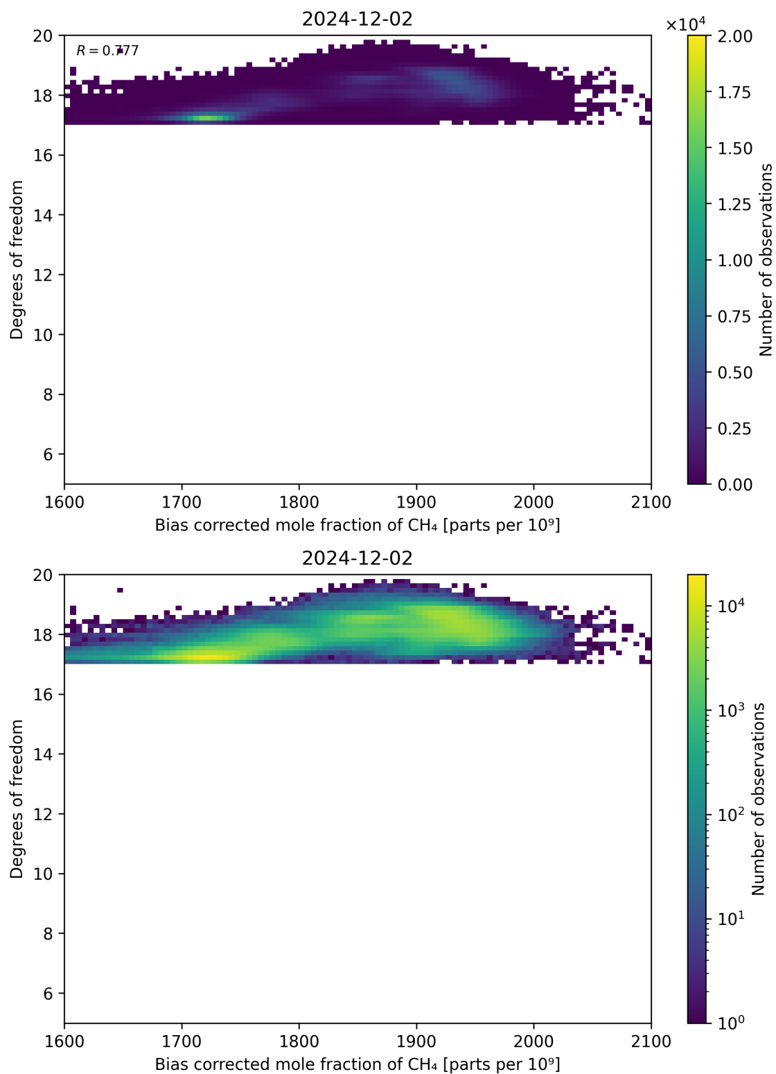
Figure 65: Scatter density plot of “Bias corrected mole fraction of CH 4 ” against “Degrees of freedom” for 2024-12-01 to 2024-12-03.
