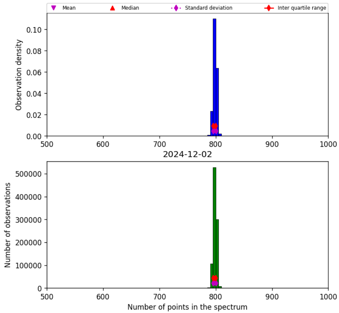
Figure 26: Histogram of “Number of points in the spectrum” for 2024-12-01 to 2024-12-03
