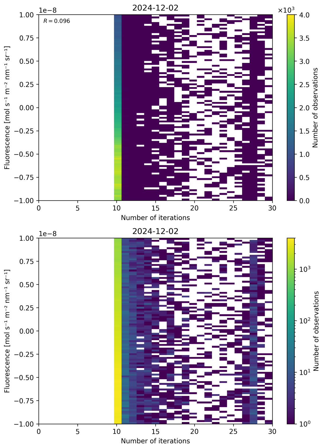
Figure 87: Scatter density plot of “Number of iterations” against “Fluorescence” for 2024-12-01 to 2024-12-03.
