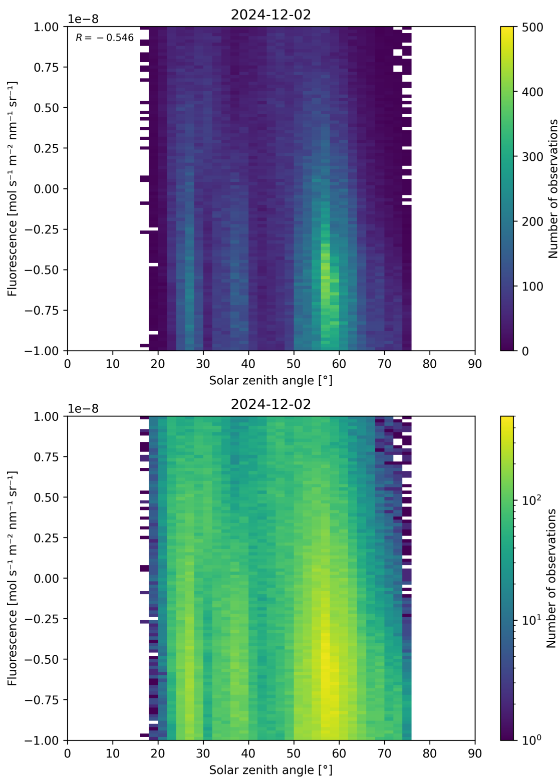
Figure 97: Scatter density plot of “Solar zenith angle” against “Fluorescence” for 2024-12-01 to 2024-12-03.
