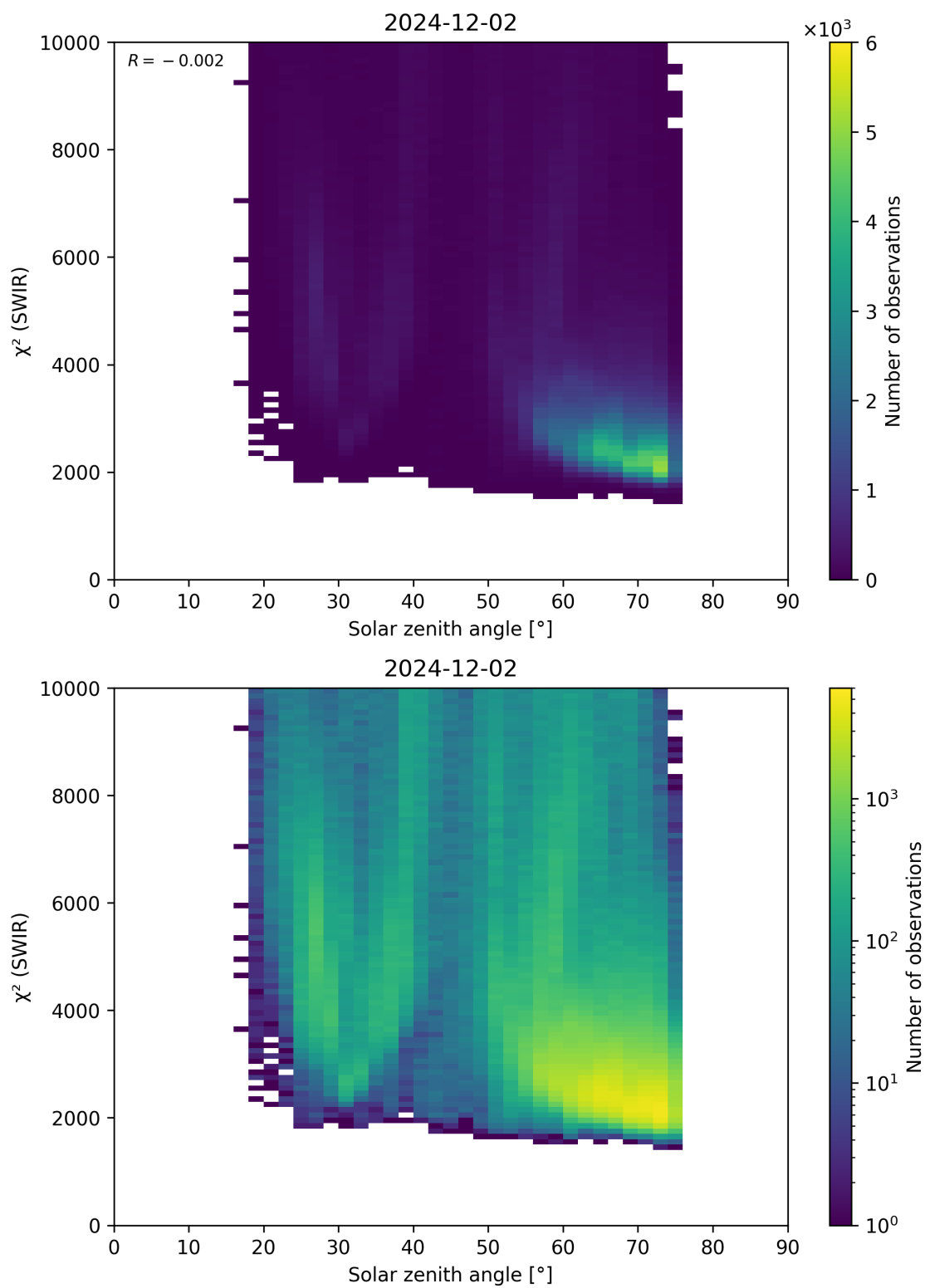
Figure 95: Scatter density plot of “Solar zenith angle” against “ \chi^2 (SWIR)” for 2024-12-01 to 2024-12-03.
