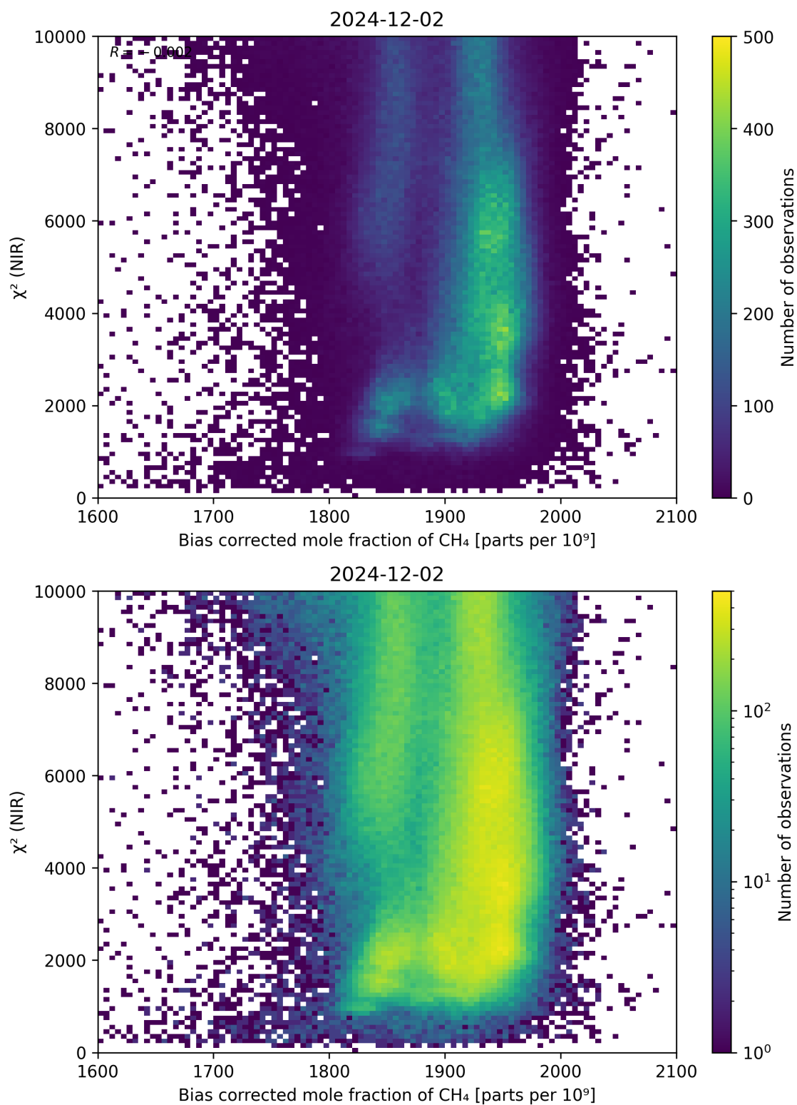
Figure 63: Scatter density plot of “Bias corrected mole fraction of CH 4 ” against “ \chi^2 (NIR)” for 2024-12-01 to 2024-12-03.
