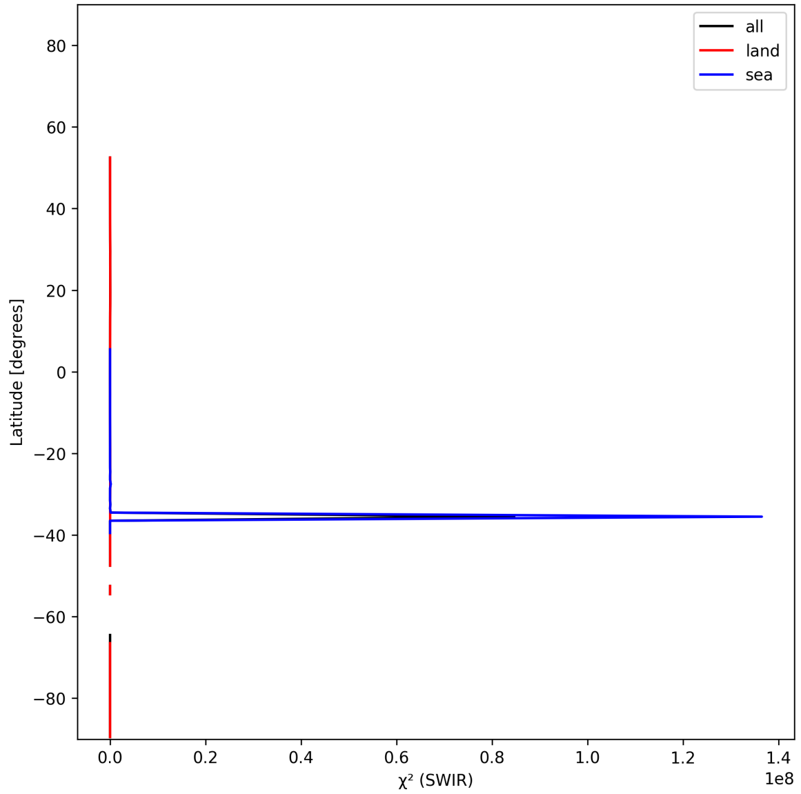
Figure 17: Zonal average of “ \chi^2 (SWIR)” for 2024-12-01 to 2024-12-03.
