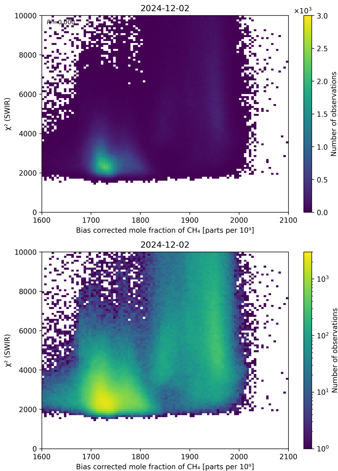
Figure 64: Scatter density plot of “Bias corrected mole fraction of \text{CH}_4 ” against “ \chi^2 (SWIR)” for 2024-12-01 to 2024-12-03.
