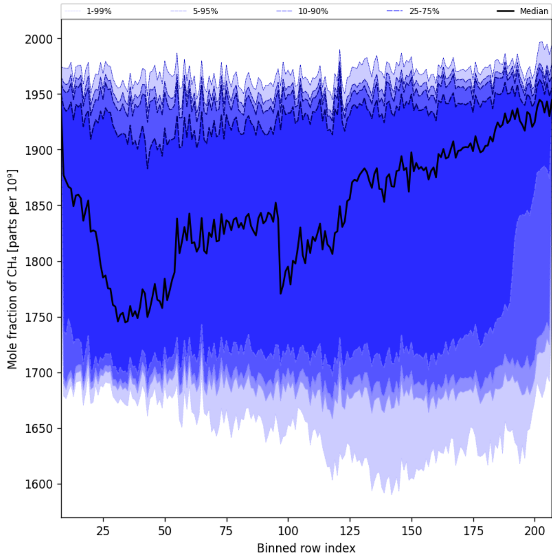
Figure 34: Along track statistics of “Mole fraction of CH 4 ” for 2024-12-01 to 2024-12-03
