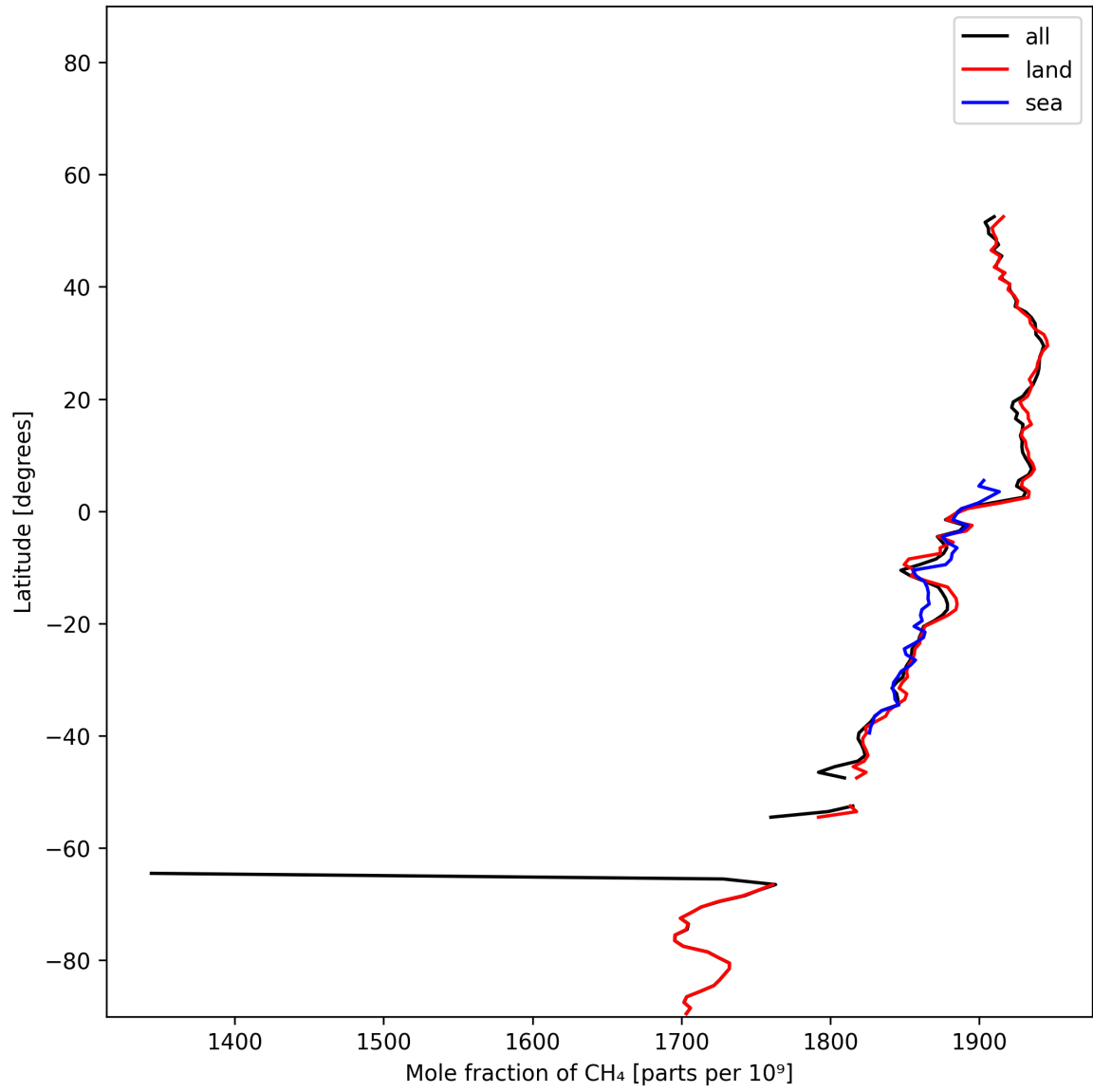
Figure 12: Zonal average of “Mole fraction of CH 4 ” for 2024-12-01 to 2024-12-03.
