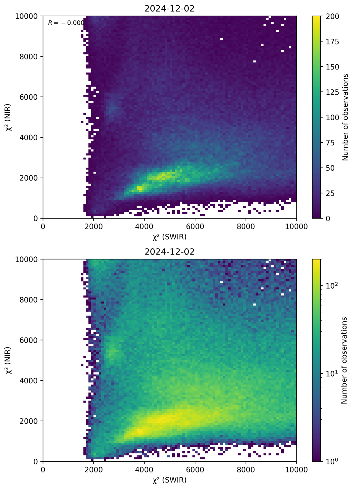
Figure 47: Scatter density plot of “ \chi^2 (SWIR)” against “ \chi^2 (NIR)” for 2024-12-01 to 2024-12-03.
