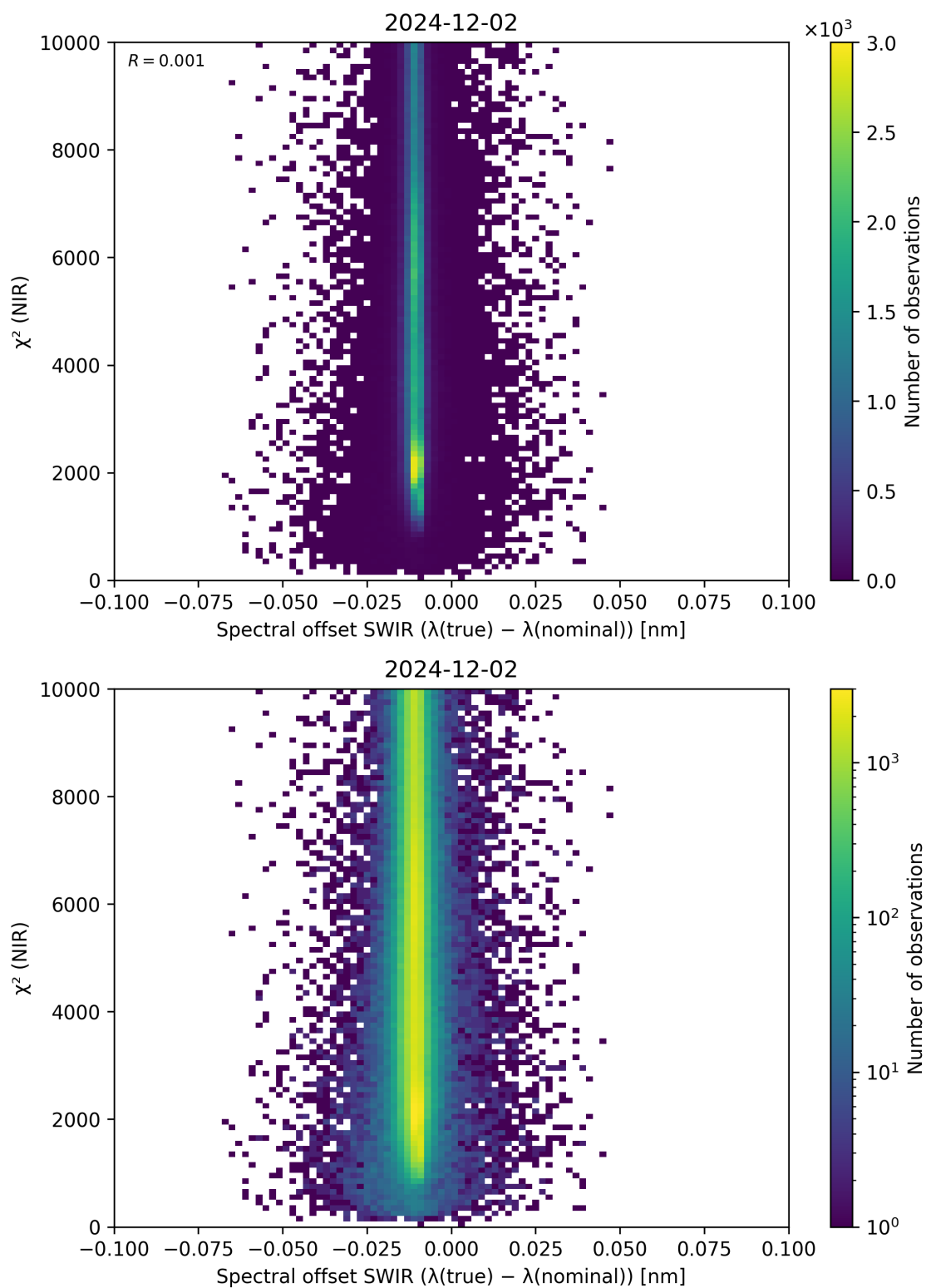
Figure 117: Scatter density plot of “Spectral offset SWIR ( \lambda_{\text{true}} - \lambda_{\text{nominal}} )” against “ \chi^2 (NIR)” for 2024-12-01 to 2024-12-03.
