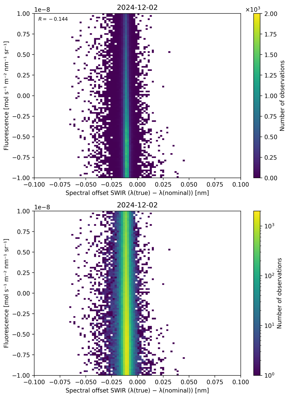
Figure 120: Scatter density plot of “Spectral offset SWIR ( \lambda_{\text{true}} - \lambda_{\text{nominal}} )” against “Fluorescence” for 2024-12-01 to 2024-12-03.
