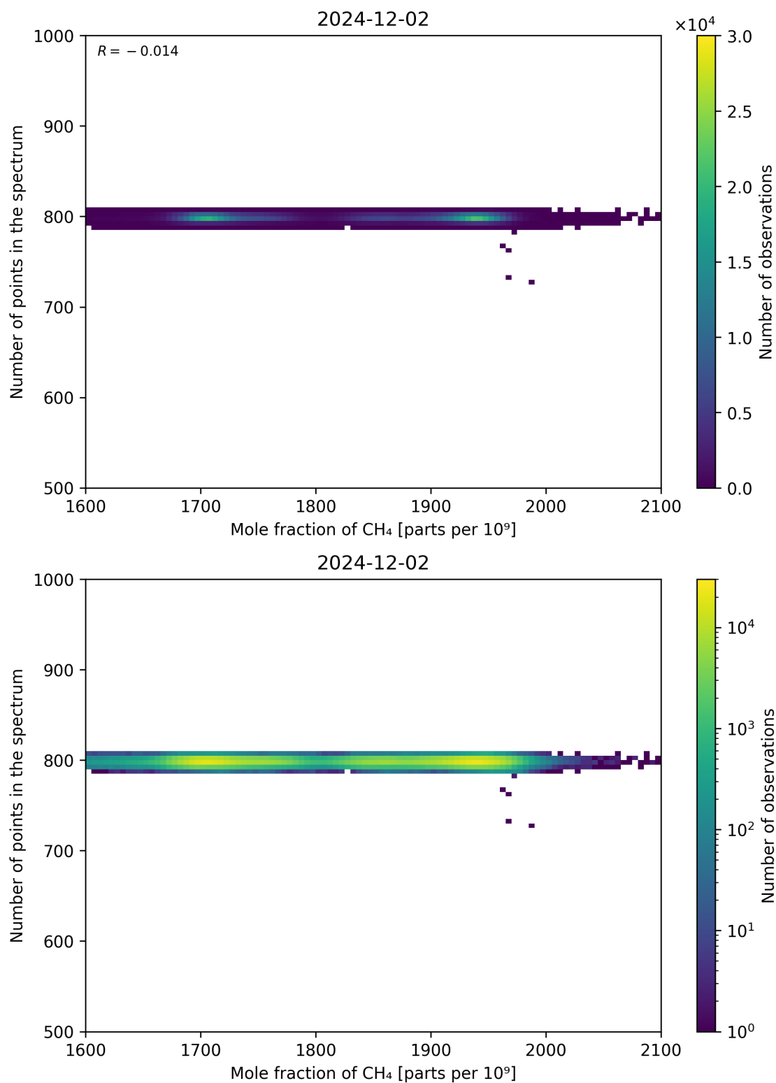
Figure 77: Scatter density plot of “Mole fraction of CH 4 ” against “Number of points in the spectrum” for 2024-12-01 to 2024-12-03.
