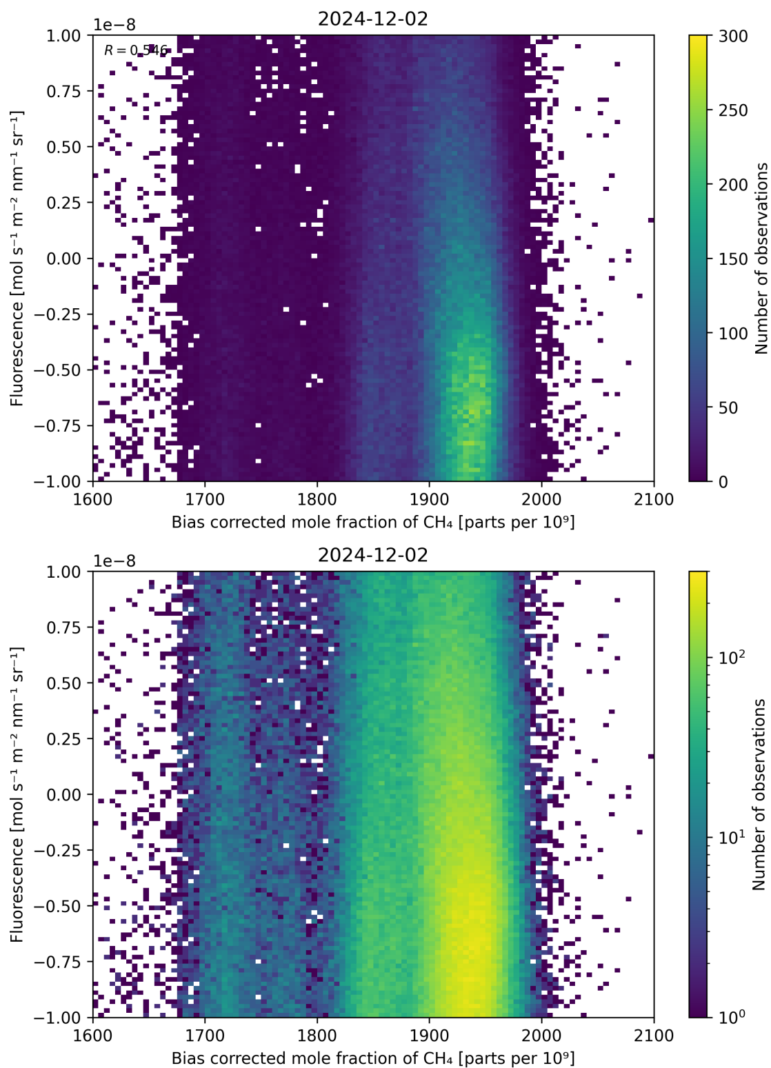
Figure 66: Scatter density plot of “Bias corrected mole fraction of \text{CH}_4 ” against “Fluorescence” for 2024-12-01 to 2024-12-03.
