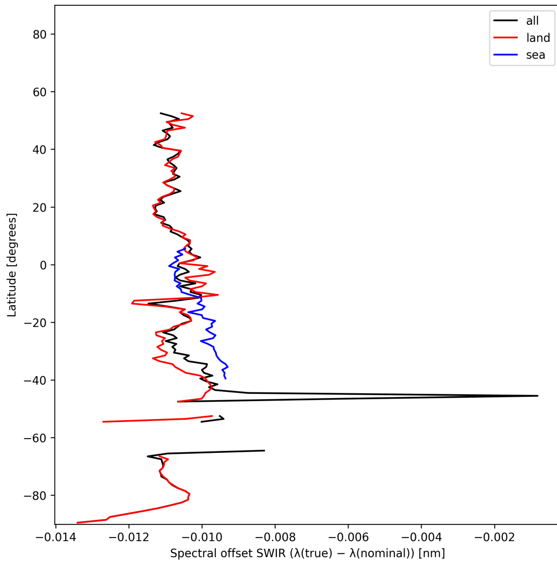
Figure 16: Zonal average of “Spectral offset SWIR ( \lambda_{\text{true}} - \lambda_{\text{nominal}} )” for 2024-12-01 to 2024-12-03.
