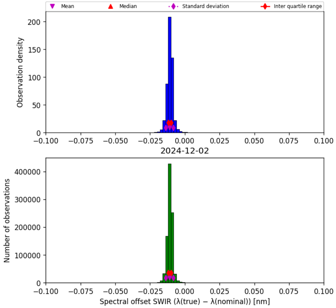
Figure 27: Histogram of “Spectral offset SWIR ( \lambda_{\text{true}} - \lambda_{\text{nominal}} )” for 2024-12-01 to 2024-12-03
