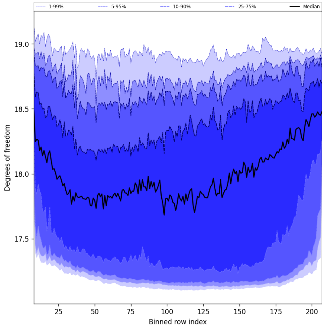
Figure 41: Along track statistics of “Degrees of freedom” for 2024-12-01 to 2024-12-03
