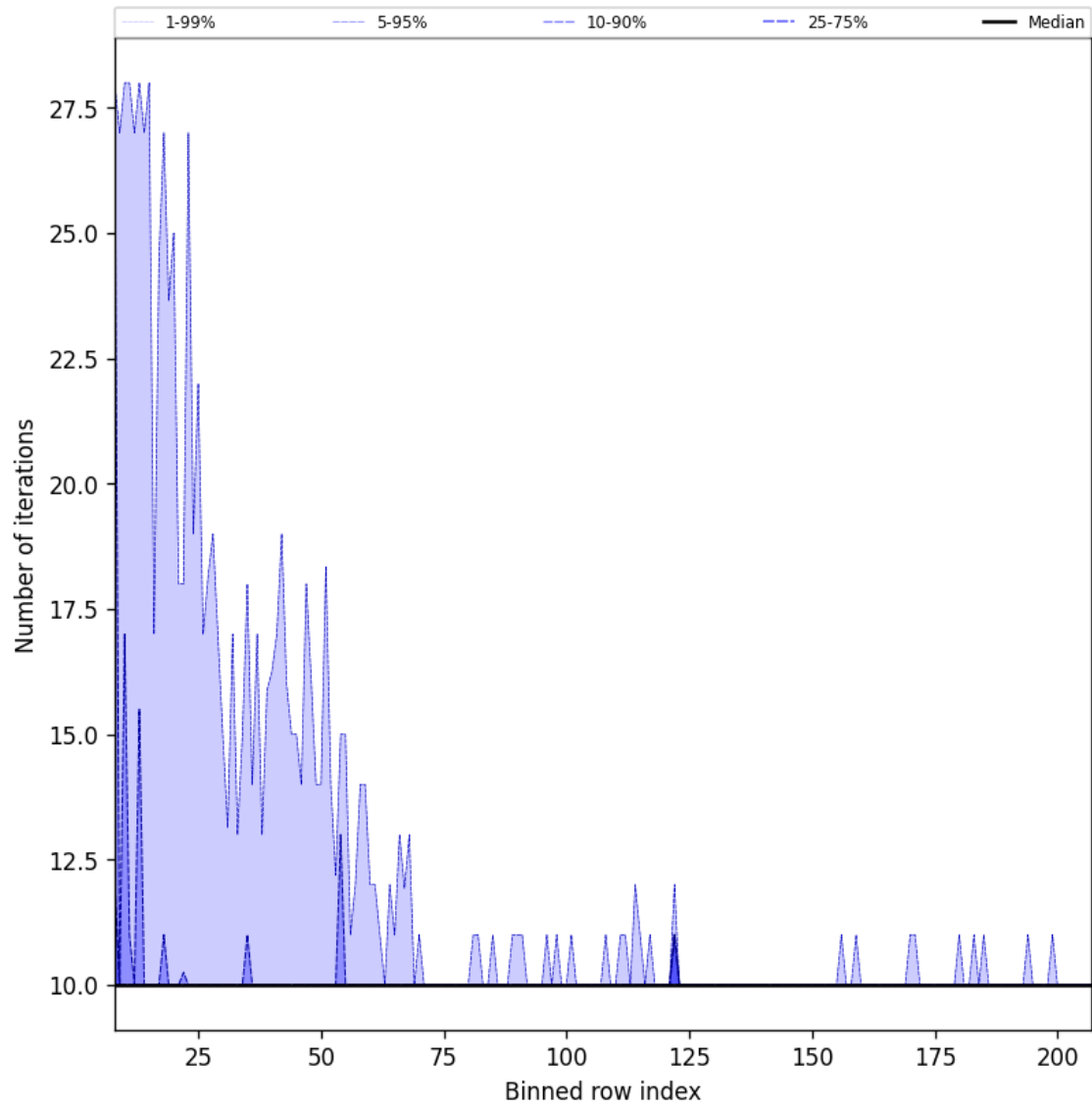
Figure 42: Along track statistics of “Number of iterations” for 2024-12-01 to 2024-12-03
