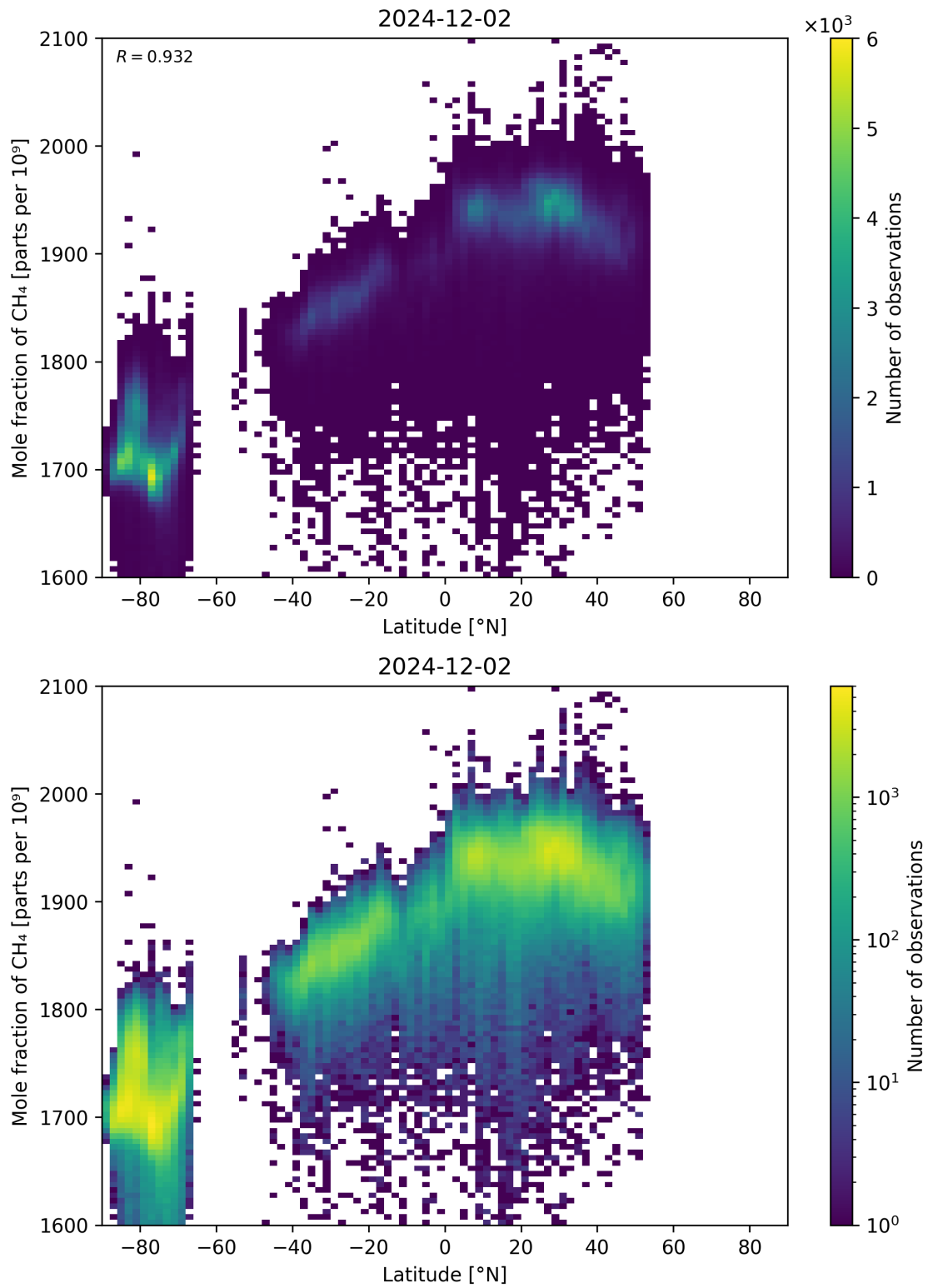
Figure 57: Scatter density plot of “Latitude” against “Mole fraction of CH 4 ” for 2024-12-01 to 2024-12-03.
