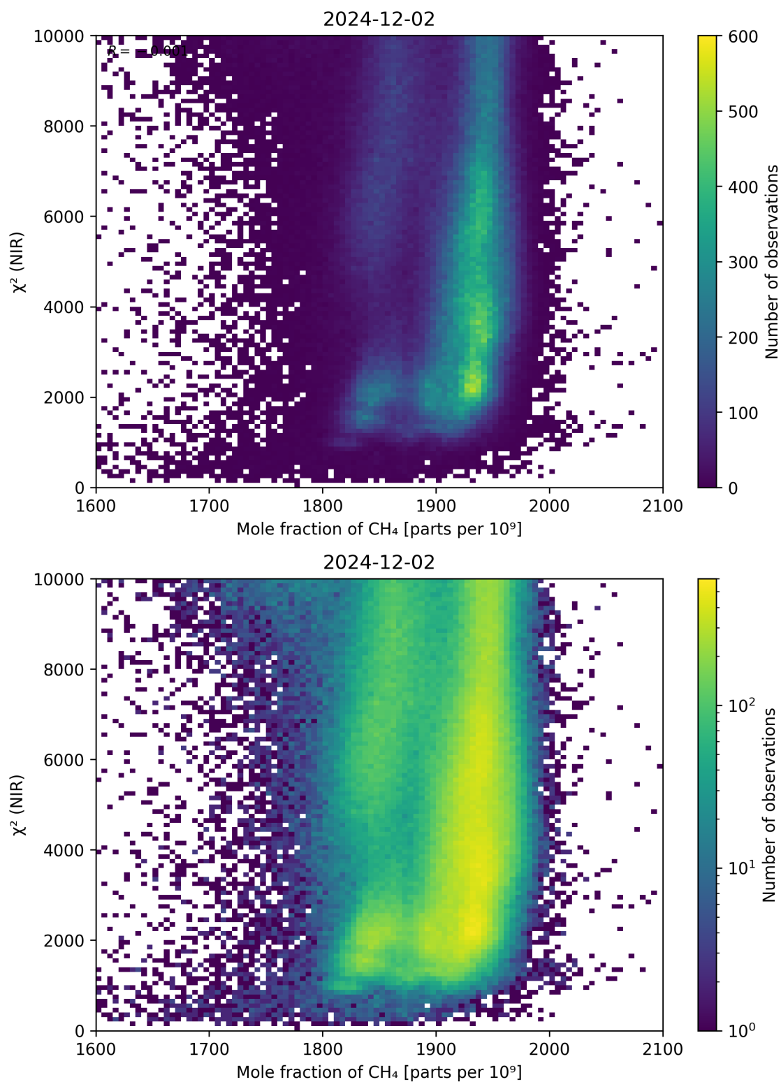
Figure 70: Scatter density plot of “Mole fraction of CH 4 ” against “ \chi^2 (NIR)” for 2024-12-01 to 2024-12-03.
