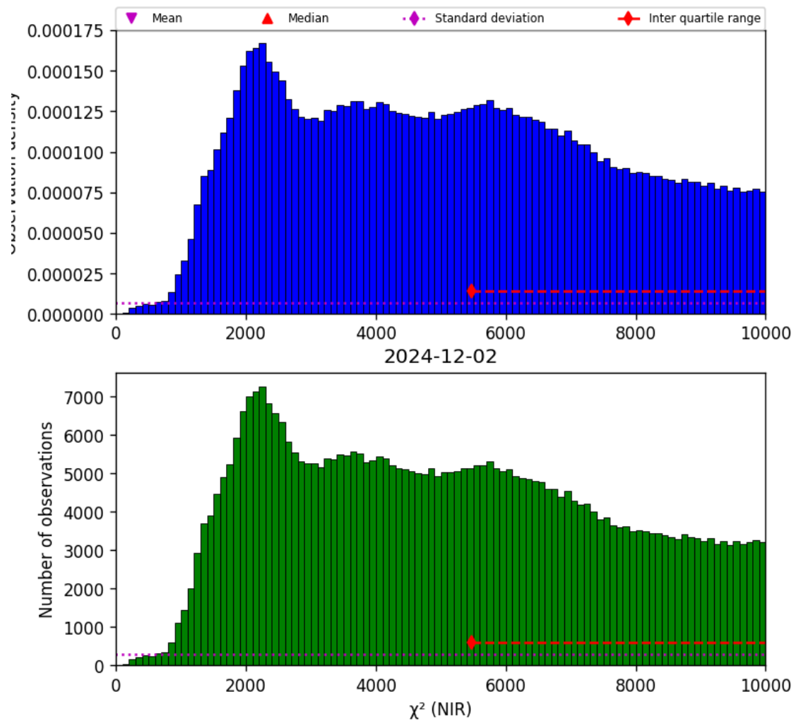
Figure 29: Histogram of “ \chi^2 (NIR)” for 2024-12-01 to 2024-12-03
