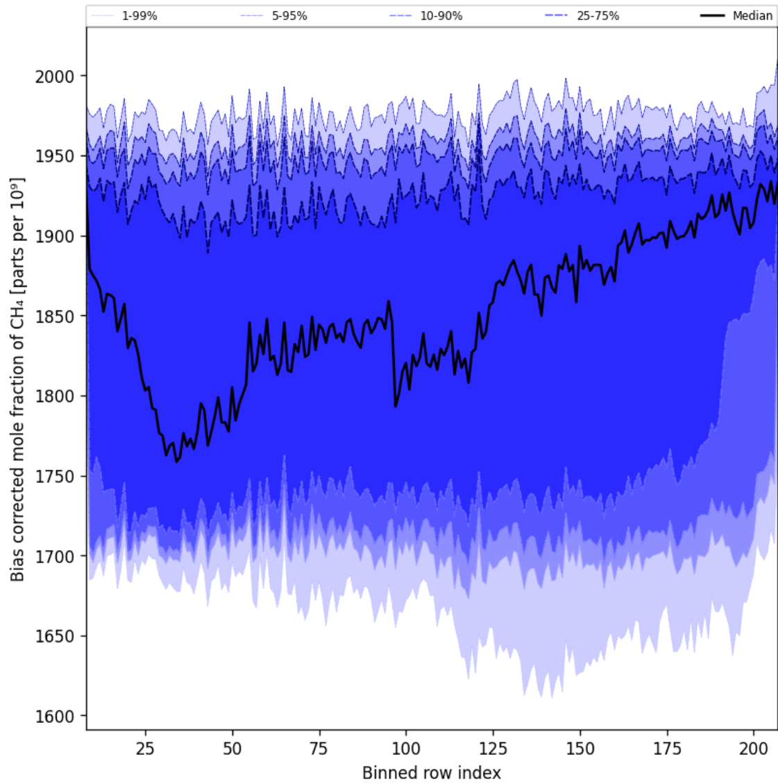
Figure 36: Along track statistics of “Bias corrected mole fraction of CH 4 ” for 2024-12-01 to 2024-12-03
