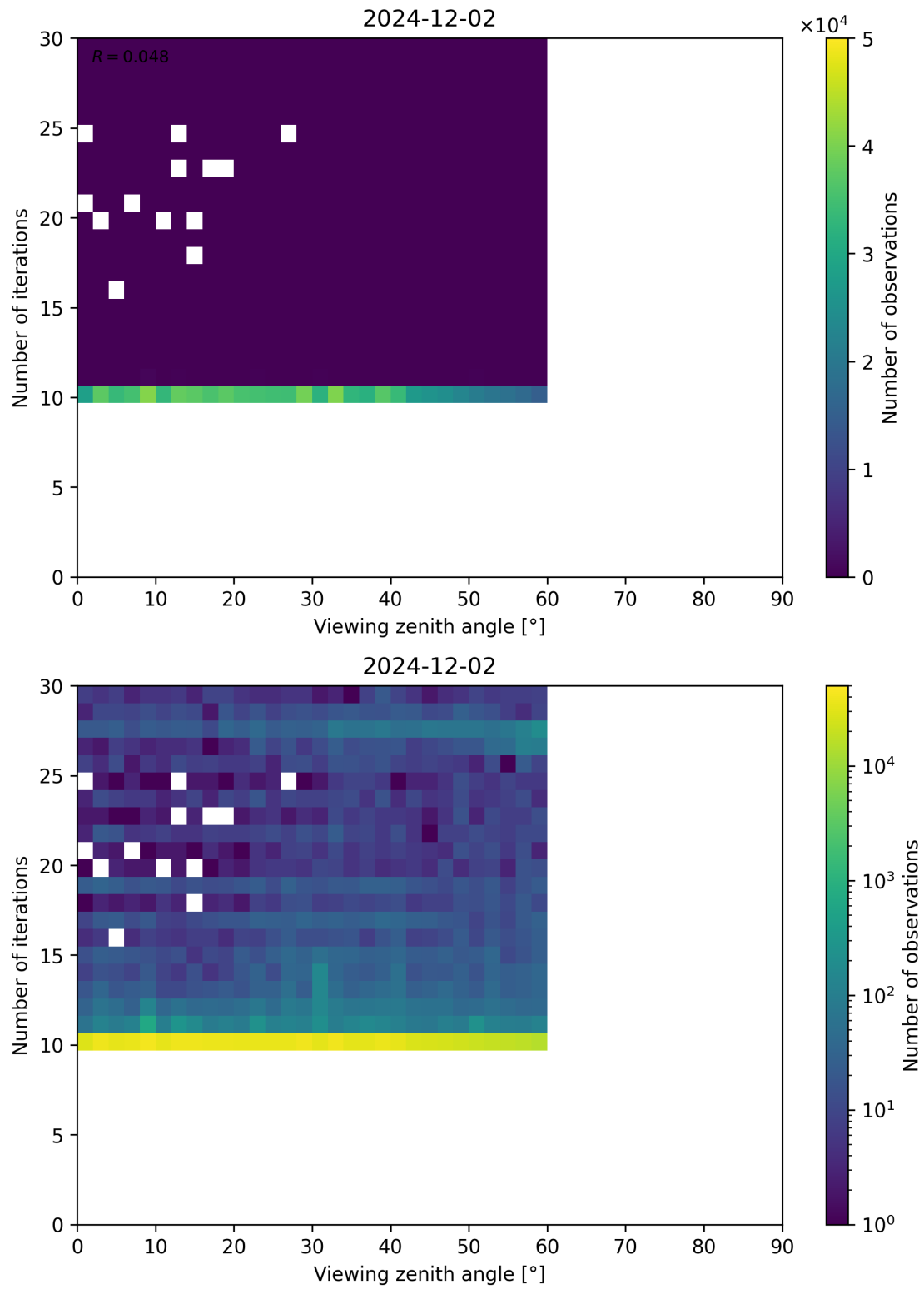
Figure 113: Scatter density plot of “Viewing zenith angle” against “Number of iterations” for 2024-12-01 to 2024-12-03.
