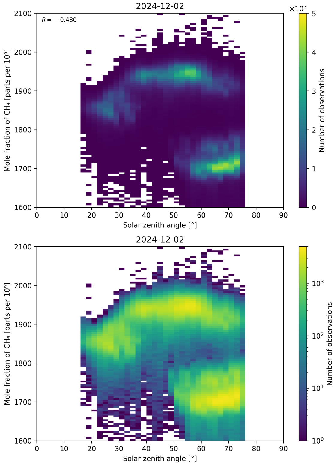
Figure 99: Scatter density plot of “Solar zenith angle” against “Mole fraction of CH 4 ” for 2024-12-01 to 2024-12-03.
