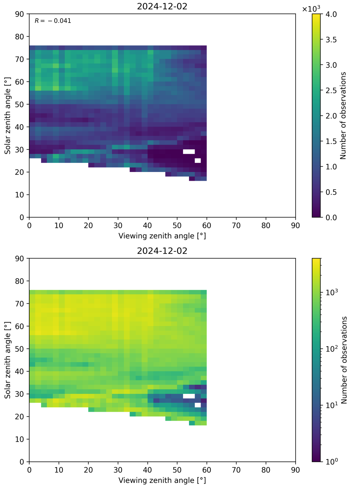
Figure 115: Scatter density plot of “Viewing zenith angle” against “Solar zenith angle” for 2024-12-01 to 2024-12-03.
