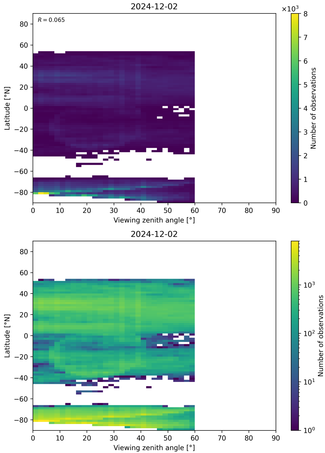
Figure 109: Scatter density plot of “Viewing zenith angle” against “Latitude” for 2024-12-01 to 2024-12-03.
