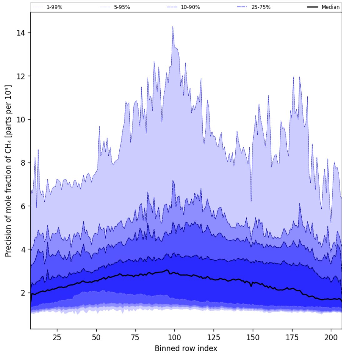
Figure 35: Along track statistics of “Precision of mole fraction of CH 4 ” for 2024-12-01 to 2024-12-03
