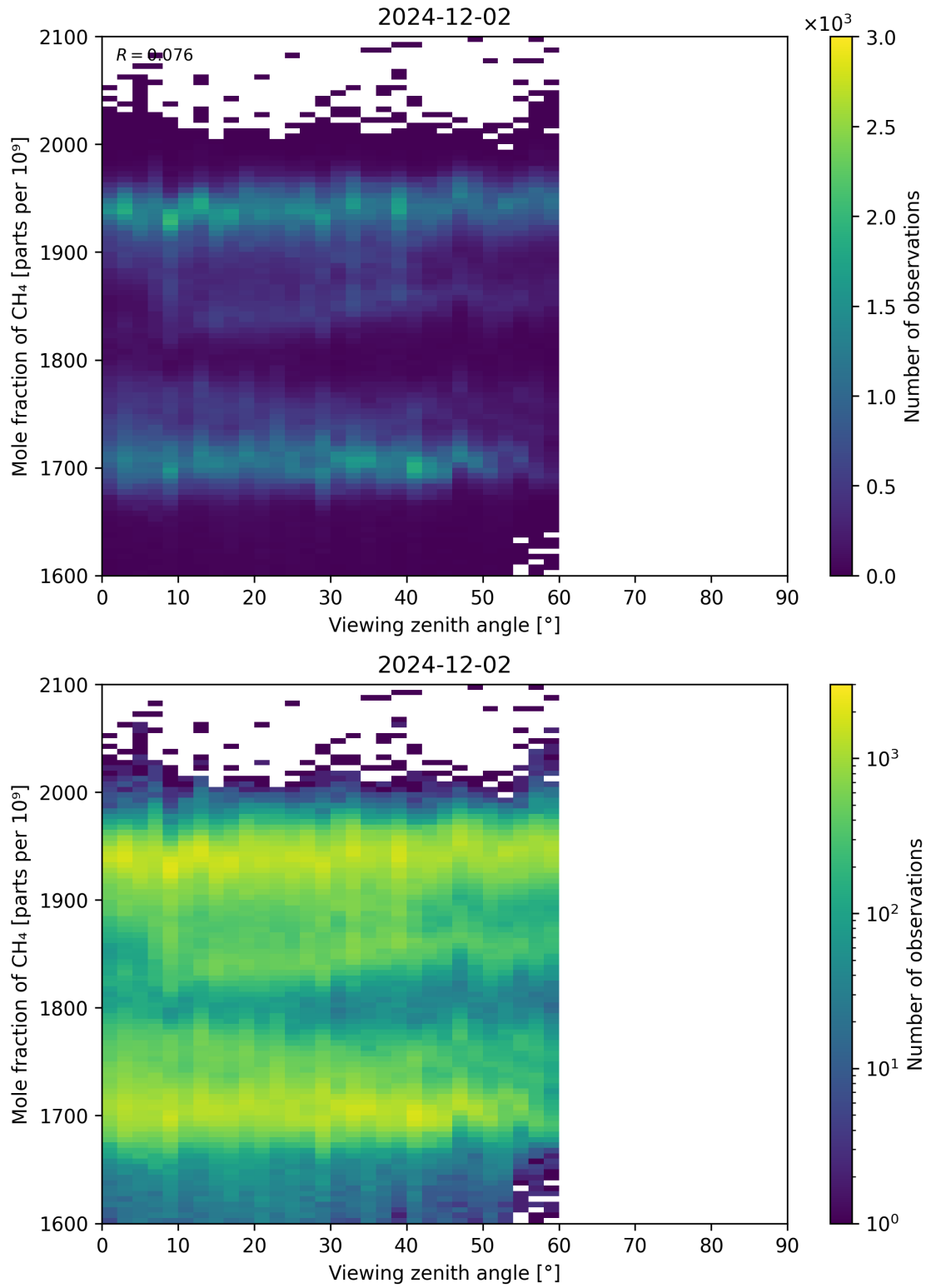
Figure 110: Scatter density plot of “Viewing zenith angle” against “Mole fraction of CH 4 ” for 2024-12-01 to 2024-12-03.
