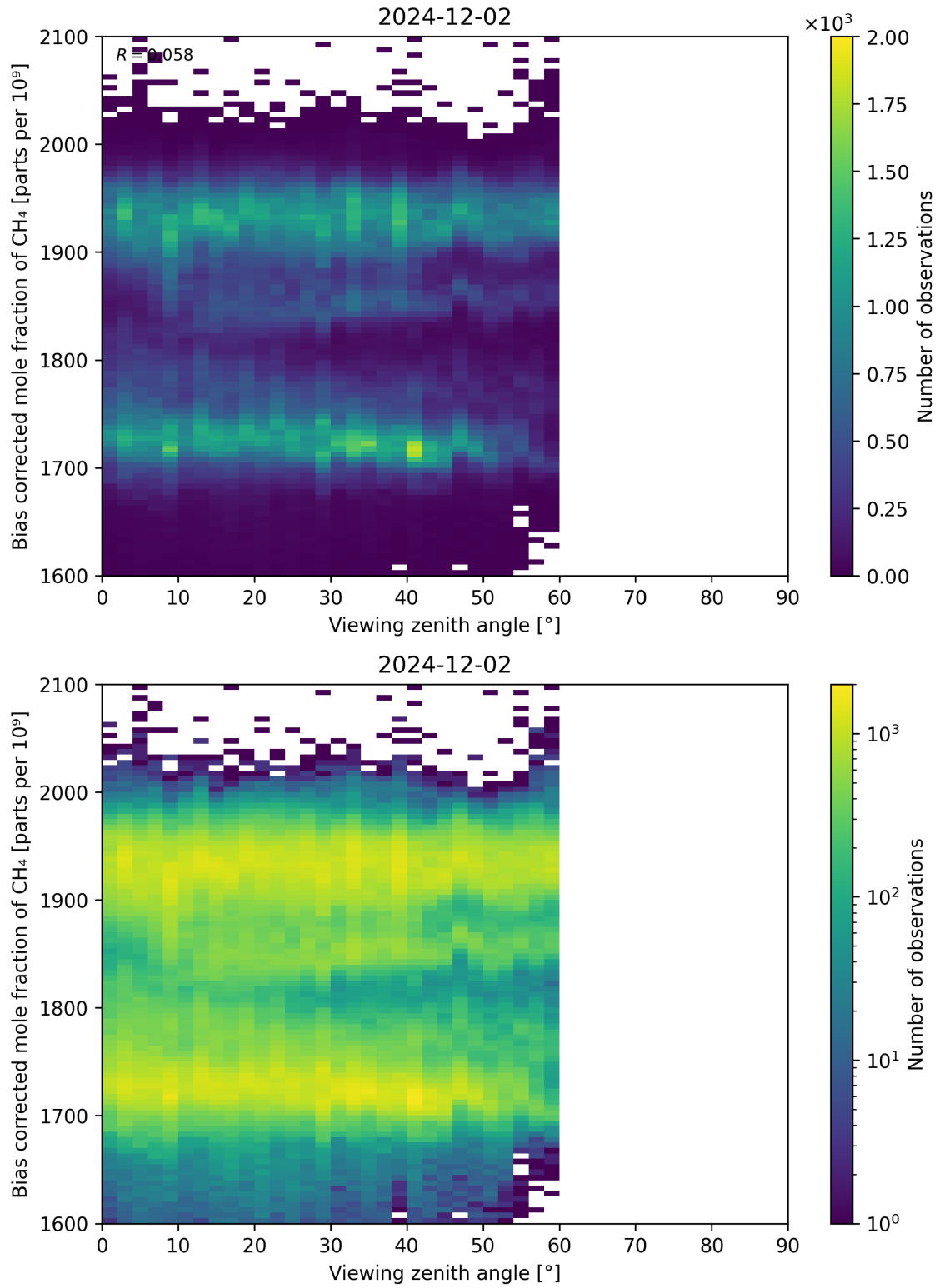
Figure 111: Scatter density plot of “Viewing zenith angle” against “Bias corrected mole fraction of CH 4 ” for 2024-12-01 to 2024-12-03.
