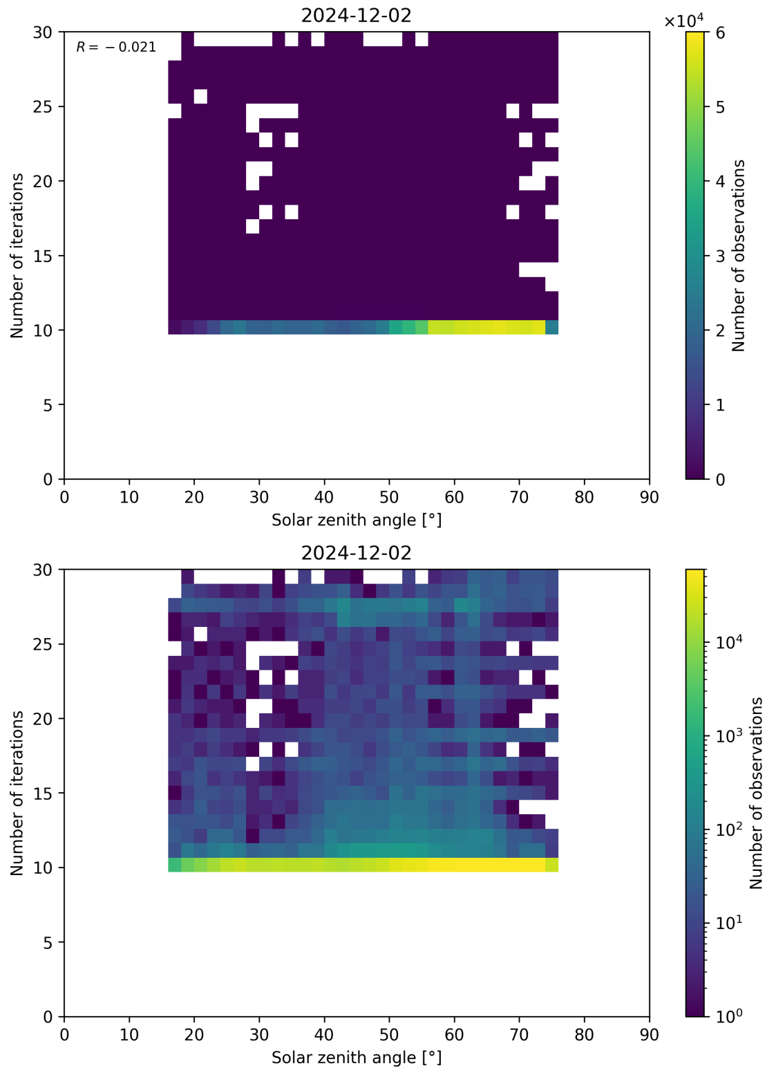
Figure 102: Scatter density plot of “Solar zenith angle” against “Number of iterations” for 2024-12-01 to 2024-12-03.
