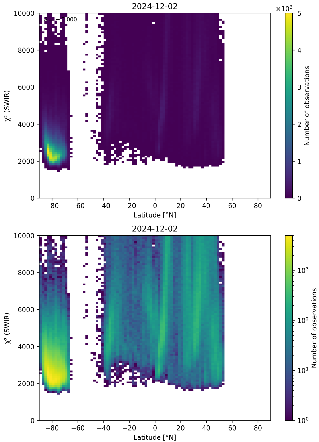
Figure 54: Scatter density plot of “Latitude” against “ \chi^2 (SWIR)” for 2024-12-01 to 2024-12-03.
