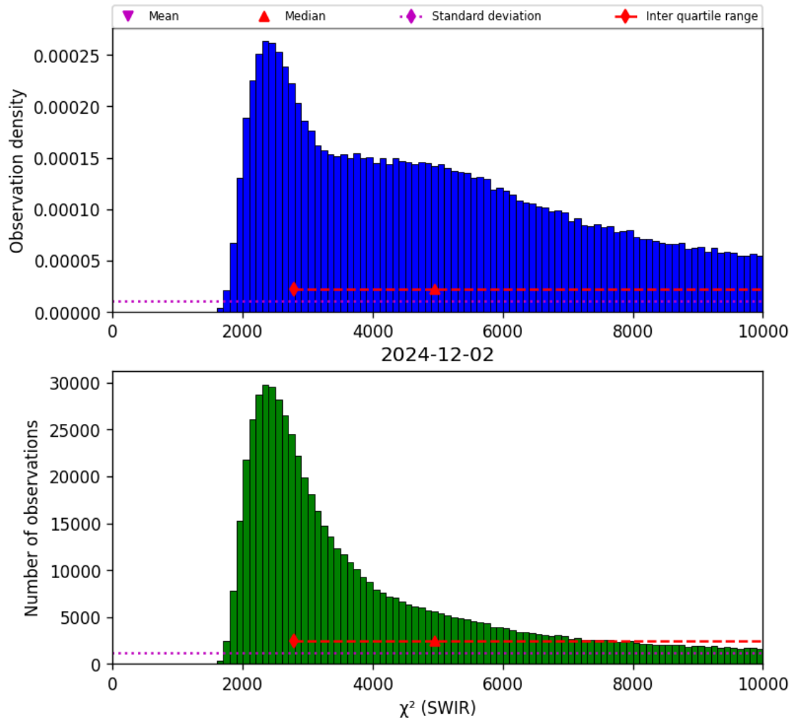
Figure 28: Histogram of “ \chi^2 (SWIR)” for 2024-12-01 to 2024-12-03
