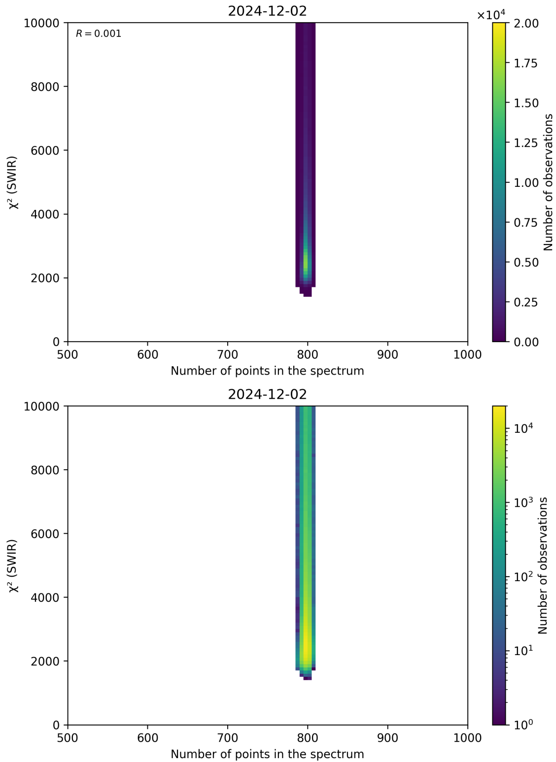
Figure 89: Scatter density plot of “Number of points in the spectrum” against “ \chi^2 (SWIR)” for 2024-12-01 to 2024-12-03.
