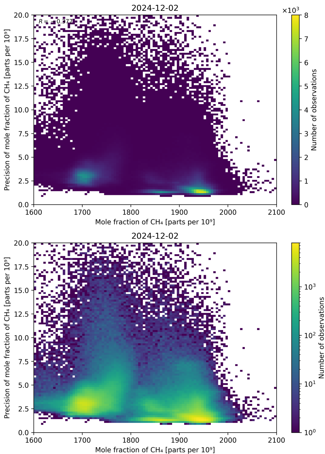
Figure 75: Scatter density plot of “Mole fraction of CH 4 ” against “Precision of mole fraction of CH 4 ” for 2024-12-01 to 2024-12-03.
