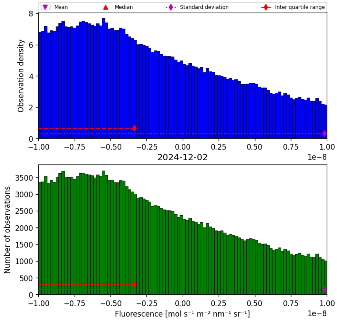
Figure 32: Histogram of “Fluorescence” for 2024-12-01 to 2024-12-03
