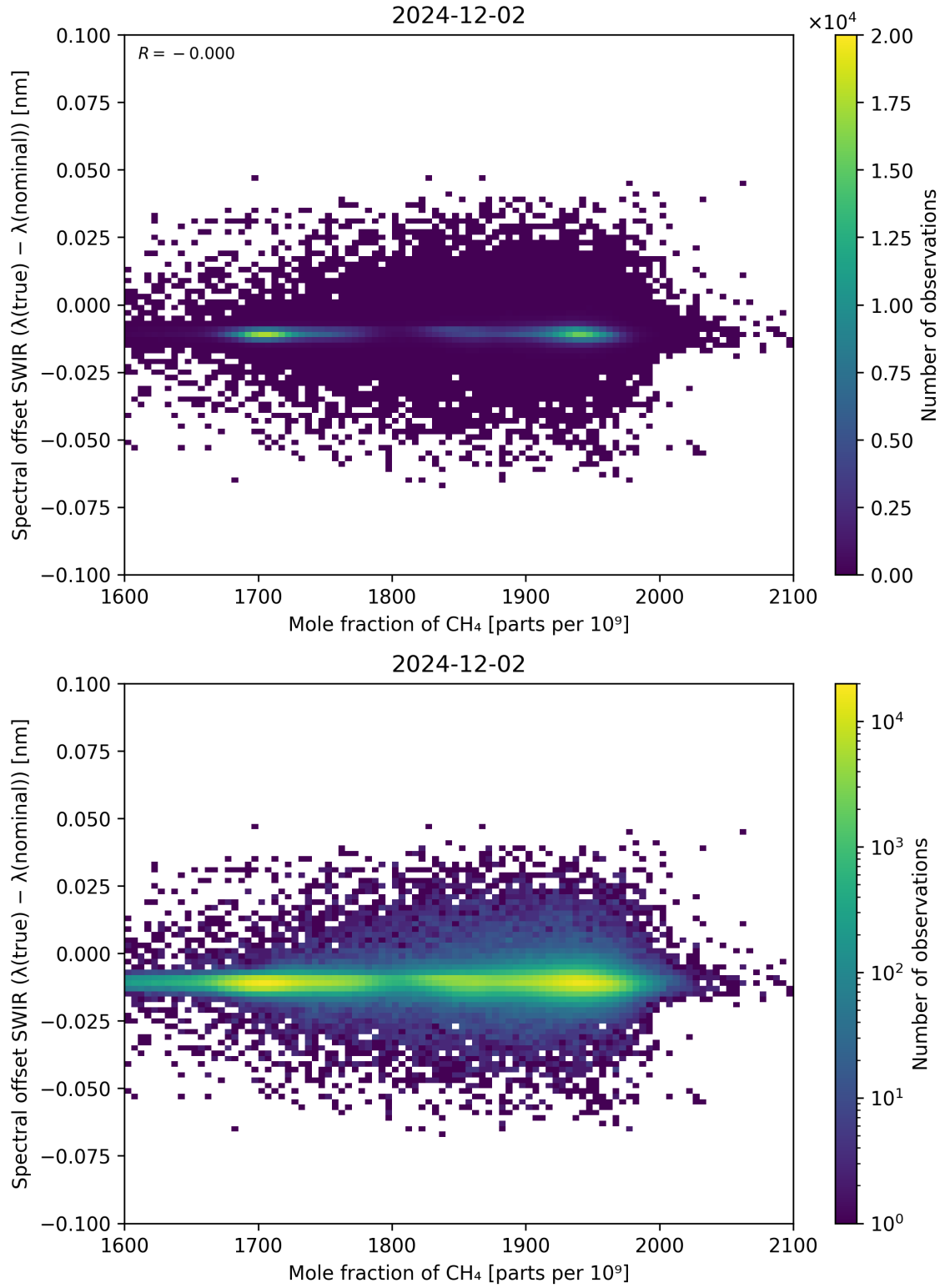
Figure 86: Scatter density plot of “Mole fraction of \text{CH}_4 ” against “Spectral offset SWIR ( \lambda_{\text{true}} - \lambda_{\text{nominal}} )” for 2024-12-01 to 2024-12-03.
