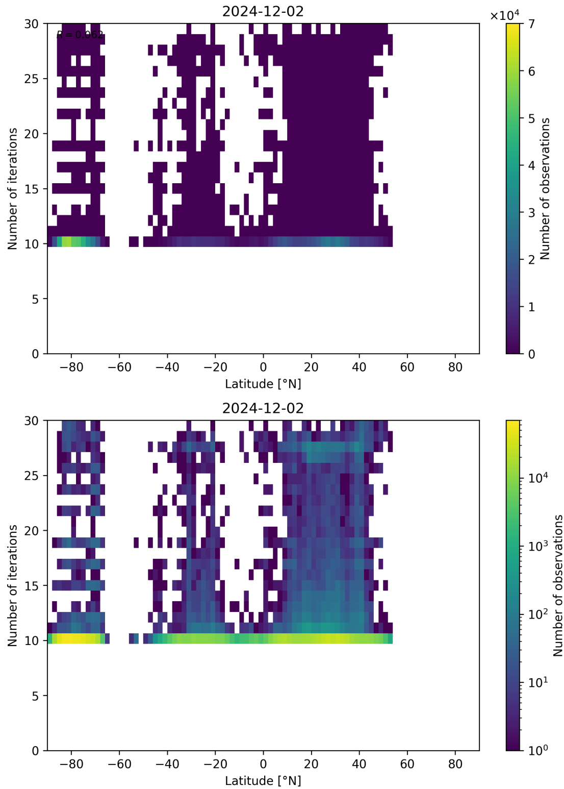
Figure 60: Scatter density plot of “Latitude” against “Number of iterations” for 2024-12-01 to 2024-12-03.
