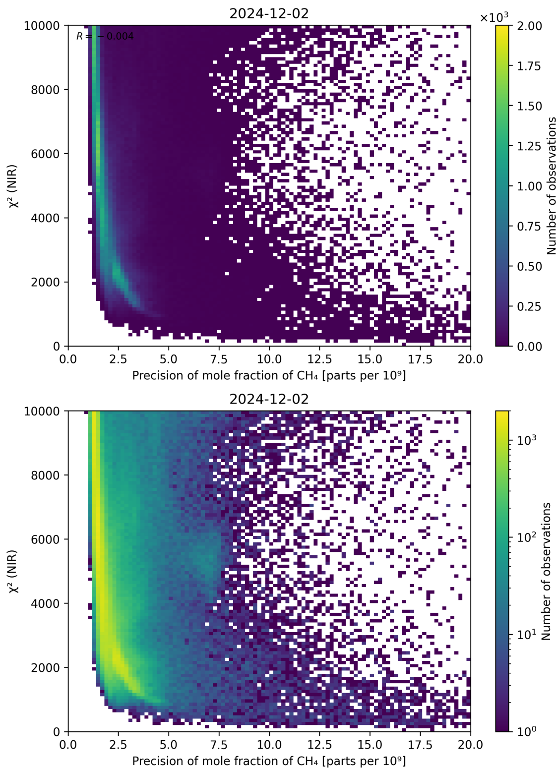
Figure 78: Scatter density plot of “Precision of mole fraction of CH 4 ” against “ \chi^2 (NIR)” for 2024-12-01 to 2024-12-03.
