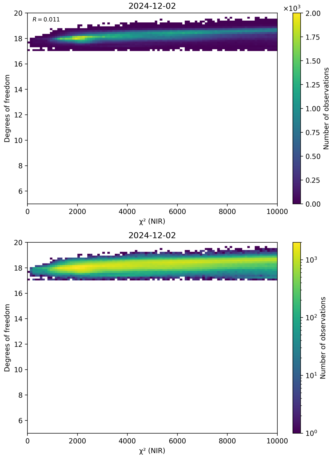
Figure 44: Scatter density plot of “ \chi^2 (NIR)” against “Degrees of freedom” for 2024-12-01 to 2024-12-03.
