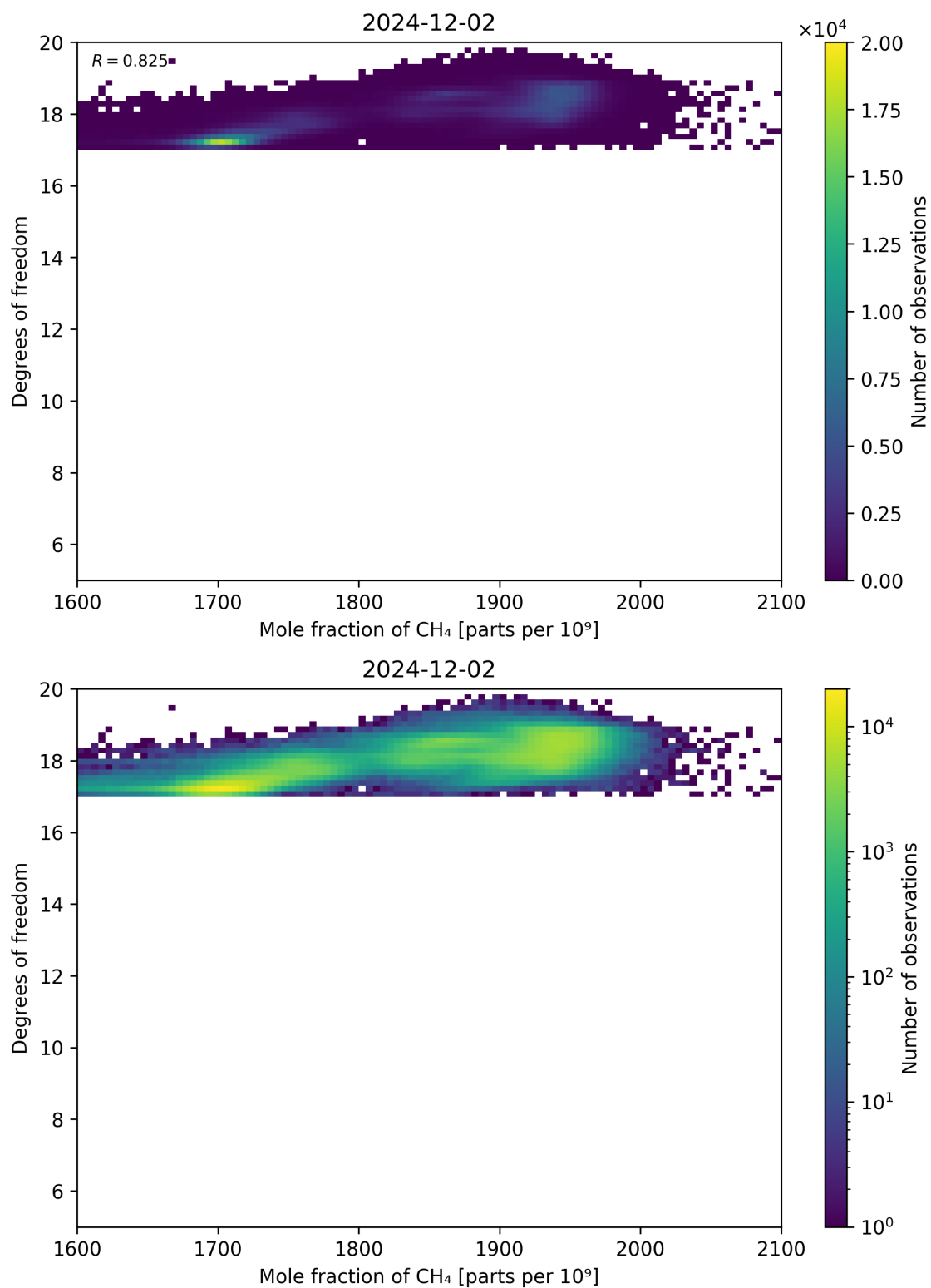
Figure 72: Scatter density plot of “Mole fraction of CH 4 ” against “Degrees of freedom” for 2024-12-01 to 2024-12-03.
