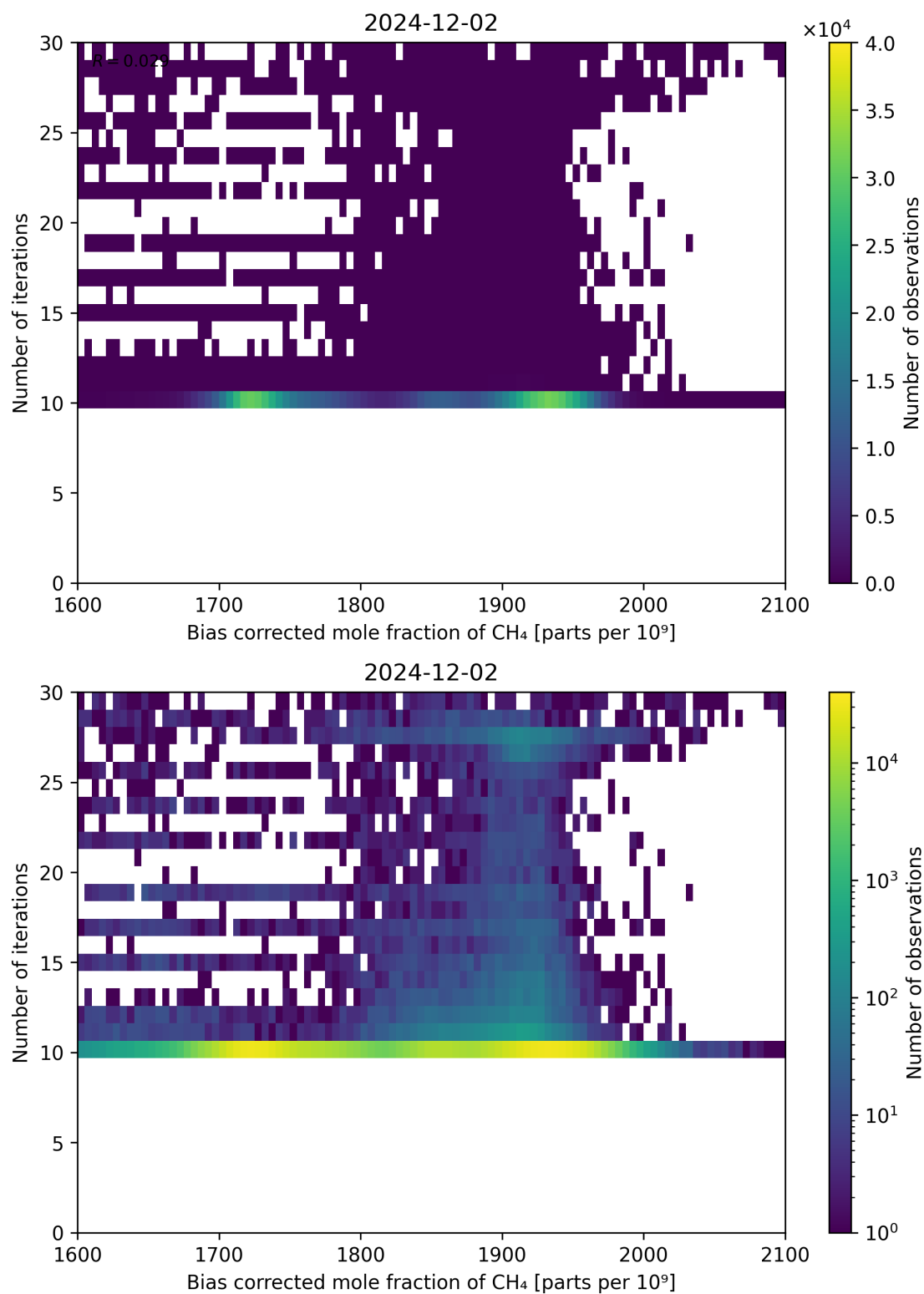
Figure 67: Scatter density plot of “Bias corrected mole fraction of \text{CH}_4 ” against “Number of iterations” for 2024-12-01 to 2024-12-03.
