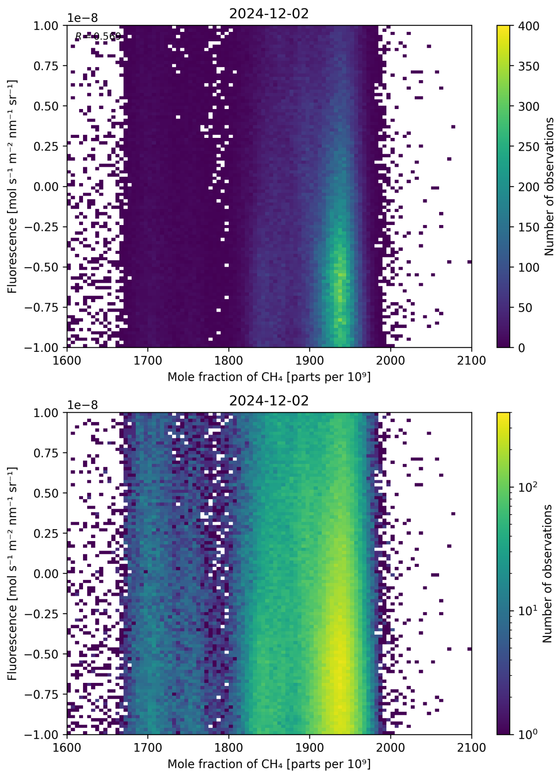
Figure 73: Scatter density plot of “Mole fraction of \text{CH}_4 ” against “Fluorescence” for 2024-12-01 to 2024-12-03.
