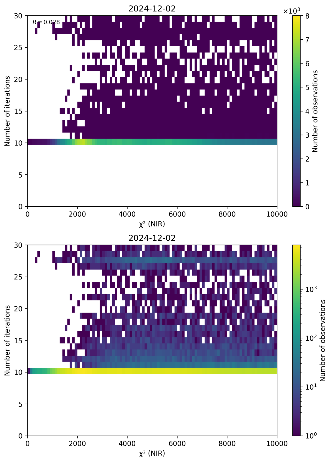
Figure 46: Scatter density plot of “ \chi^2 (NIR)” against “Number of iterations” for 2024-12-01 to 2024-12-03.
