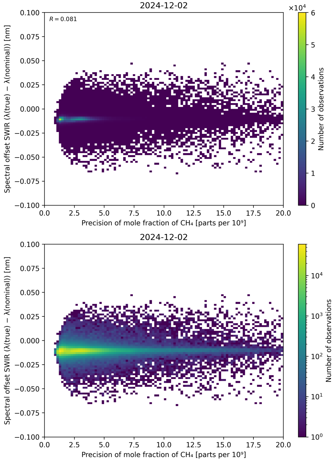
Figure 85: Scatter density plot of “Precision of mole fraction of \text{CH}_4 ” against “Spectral offset SWIR ( \lambda_{\text{true}} - \lambda_{\text{nominal}} )” for 2024-12-01 to 2024-12-03.
