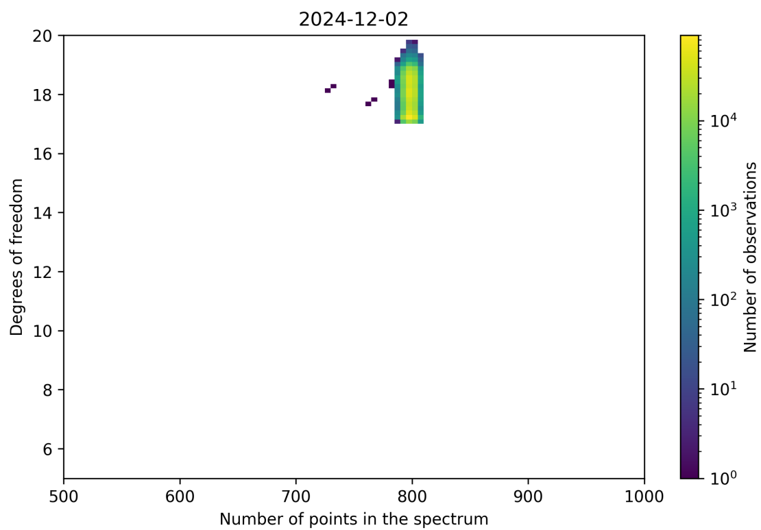
Figure 90: Scatter density plot of “Number of points in the spectrum” against “Degrees of freedom” for 2024-12-01 to 2024-12-03.
