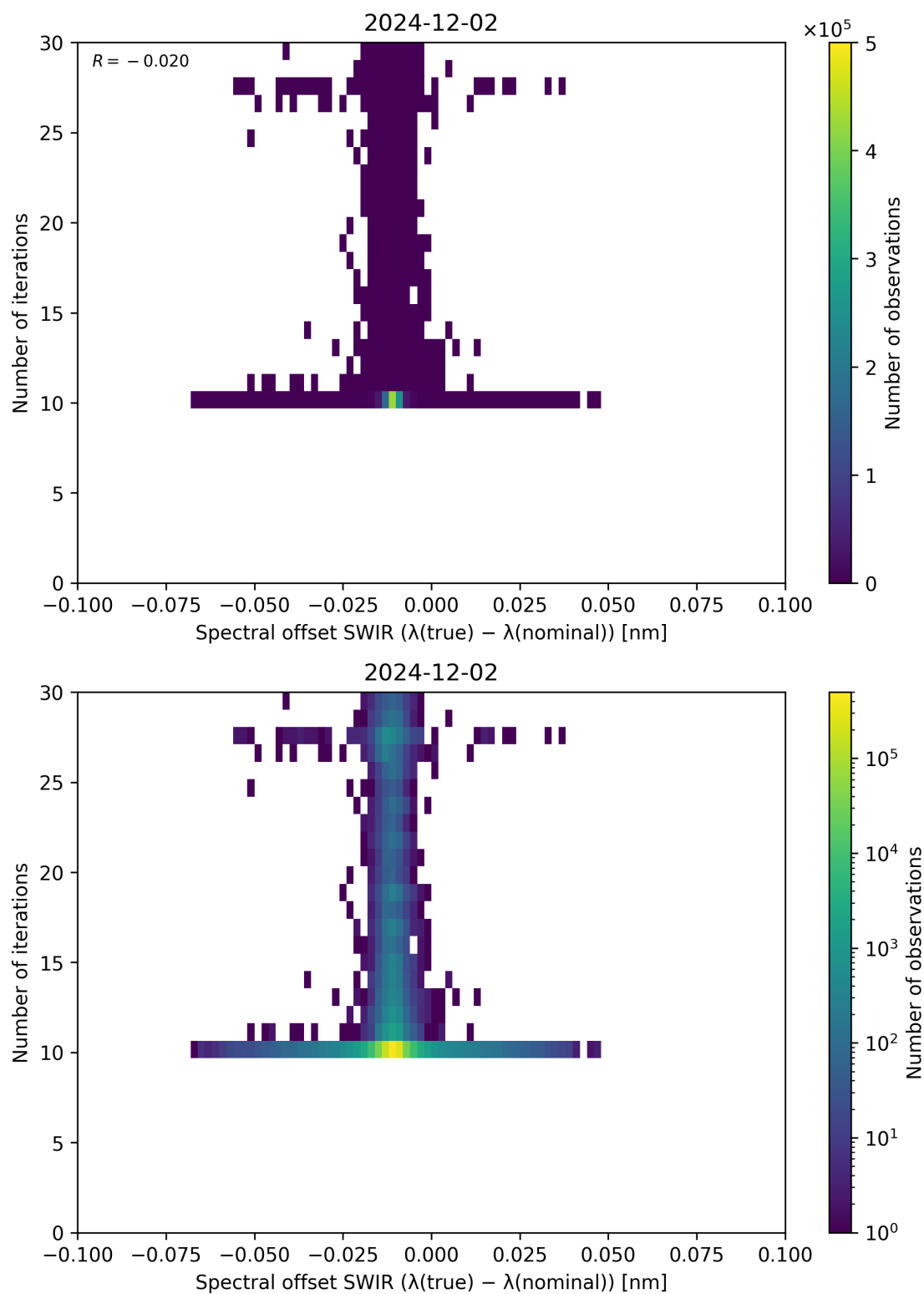
Figure 121: Scatter density plot of “Spectral offset SWIR ( \lambda_{\text{true}} - \lambda_{\text{nominal}} )” against “Number of iterations” for 2024-12-01 to 2024-12-03.
