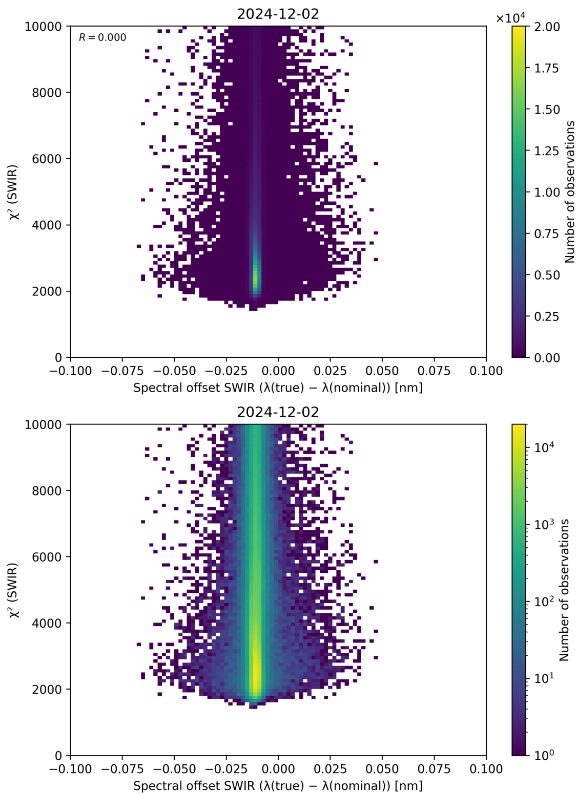
Figure 118: Scatter density plot of “Spectral offset SWIR ( \lambda_{\text{true}} - \lambda_{\text{nominal}} )” against “ \chi^2 (SWIR)” for 2024-12-01 to 2024-12-03.
