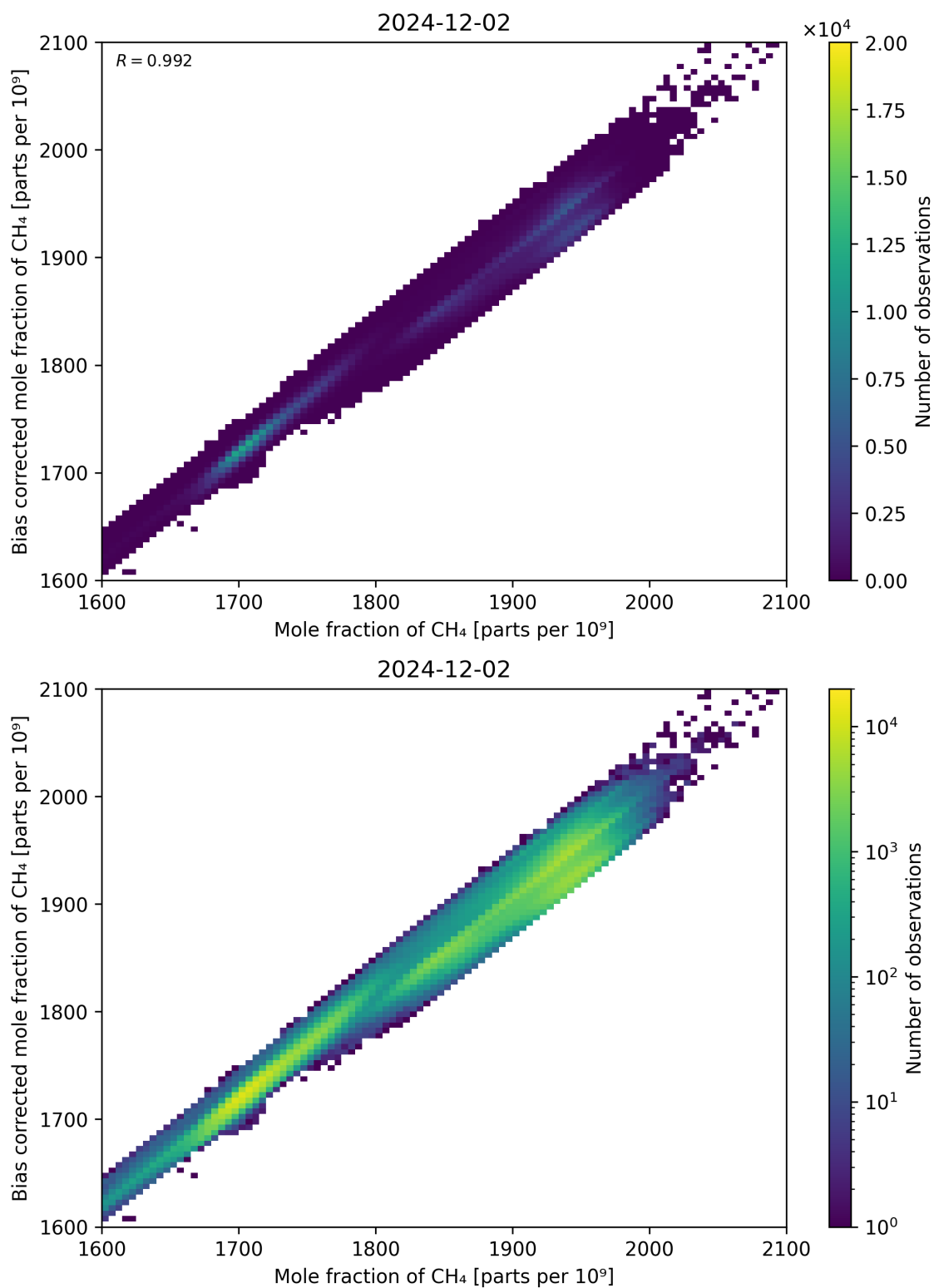
Figure 74: Scatter density plot of “Mole fraction of CH 4 ” against “Bias corrected mole fraction of CH 4 ” for 2024-12-01 to 2024-12-03.
