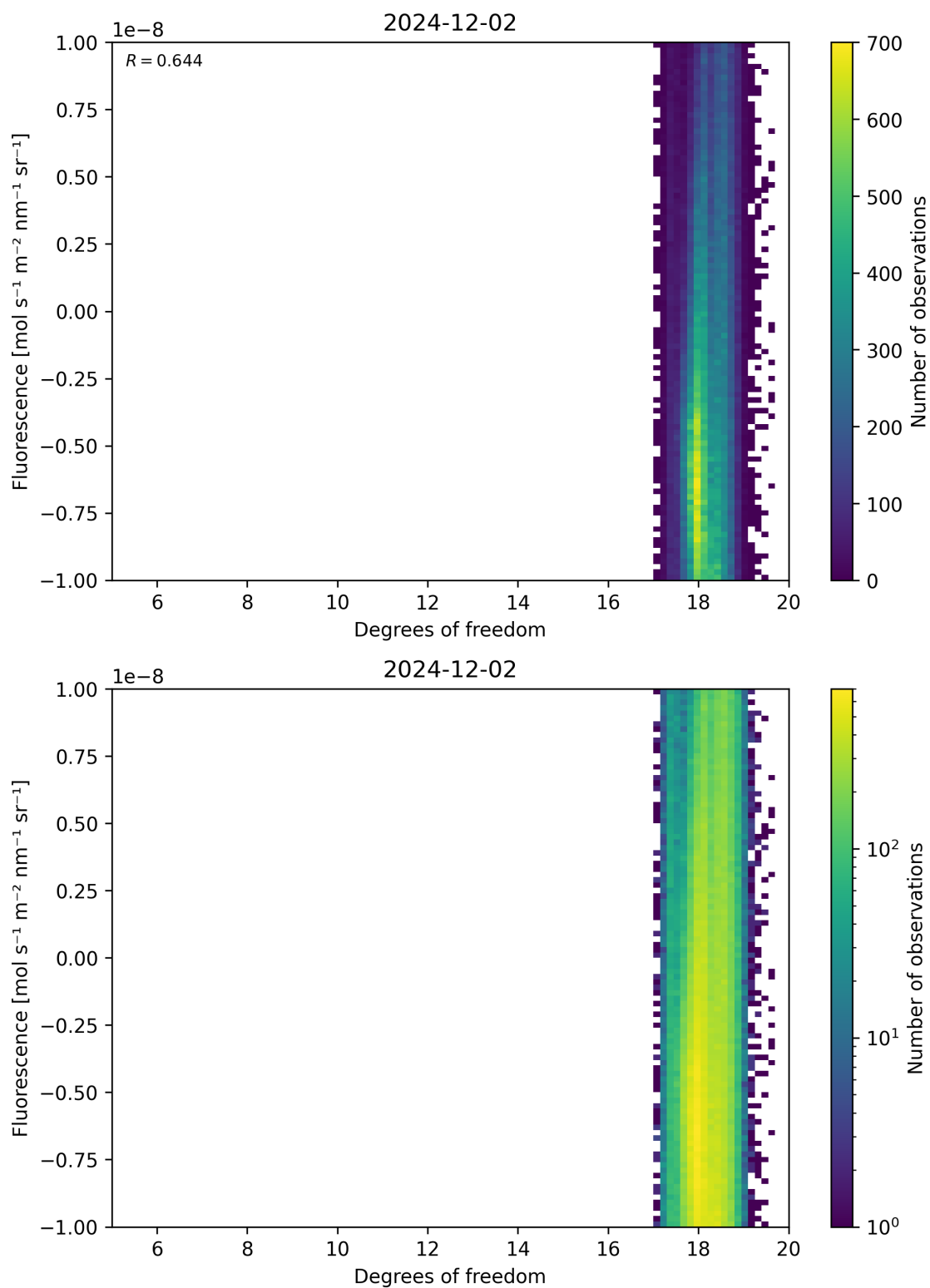
Figure 51: Scatter density plot of “Degrees of freedom” against “Fluorescence” for 2024-12-01 to 2024-12-03.
