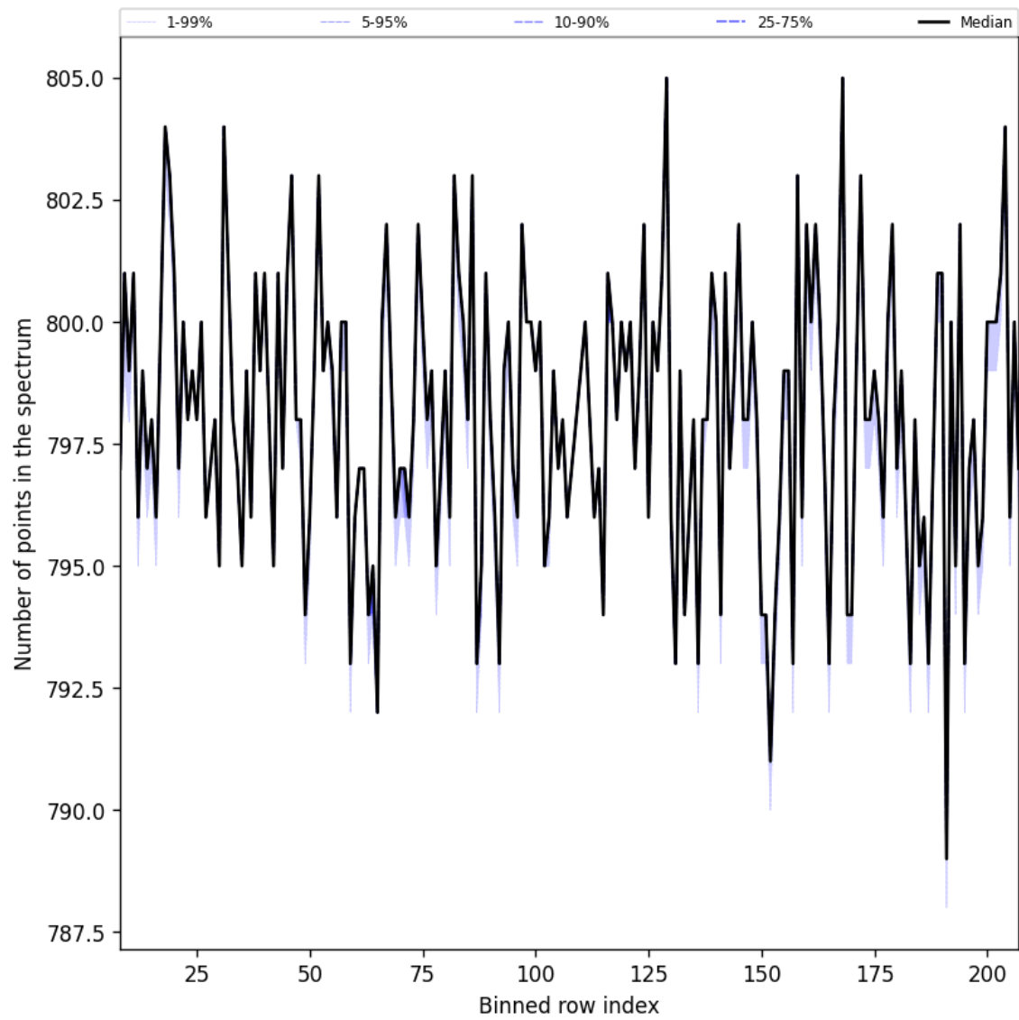
Figure 37: Along track statistics of “Number of points in the spectrum” for 2024-12-01 to 2024-12-03
