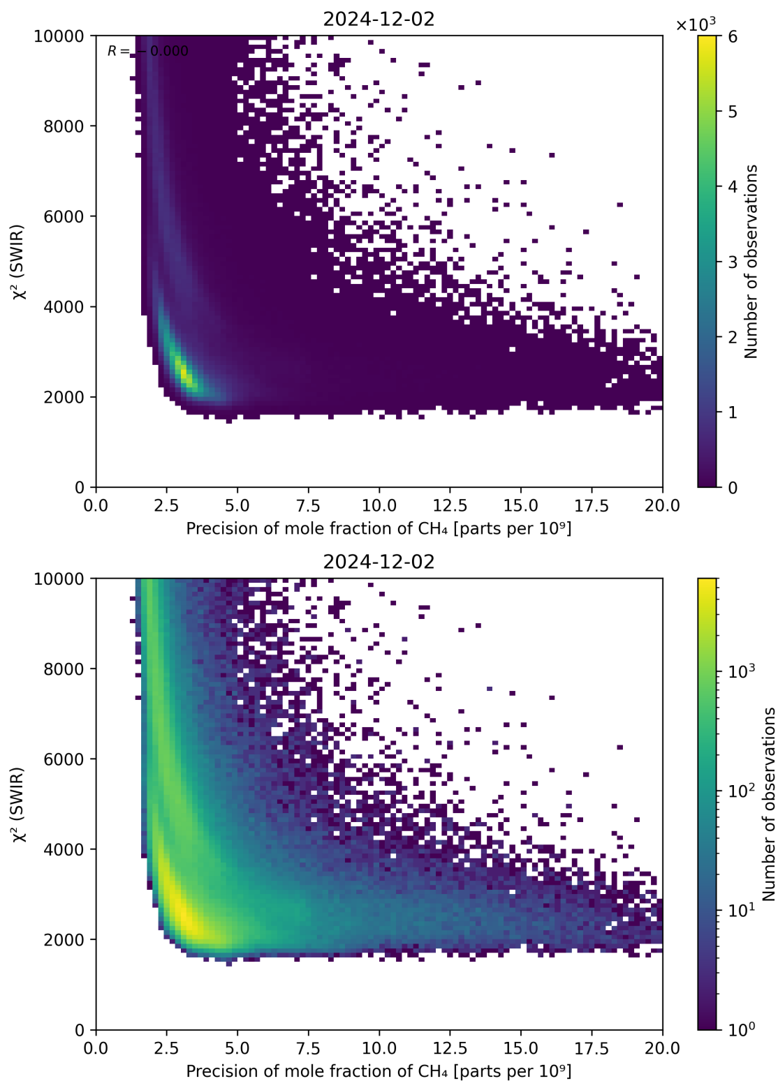
Figure 79: Scatter density plot of “Precision of mole fraction of \text{CH}_4 ” against “ \chi^2 (SWIR)” for 2024-12-01 to 2024-12-03.
