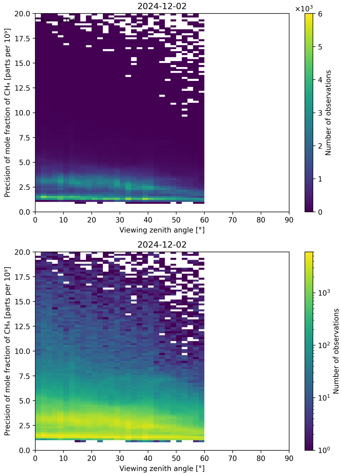
Figure 112: Scatter density plot of “Viewing zenith angle” against “Precision of mole fraction of CH 4 ” for 2024-12-01 to 2024-12-03.
