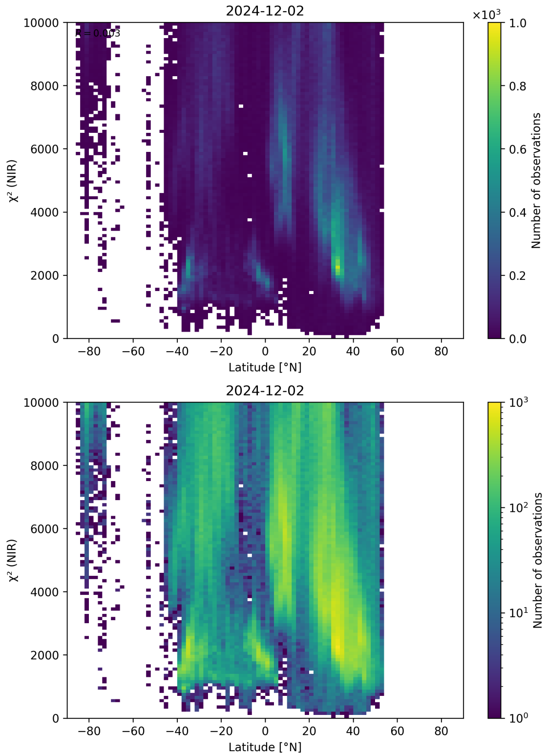
Figure 53: Scatter density plot of “Latitude” against “ \chi^2 (NIR)” for 2024-12-01 to 2024-12-03.
