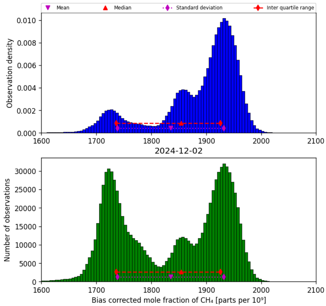
Figure 25: Histogram of “Bias corrected mole fraction of CH 4 ” for 2024-12-01 to 2024-12-03
