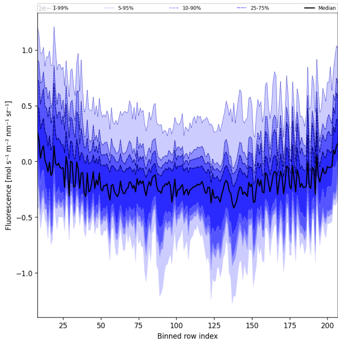
Figure 43: Along track statistics of “Fluorescence” for 2024-12-01 to 2024-12-03
