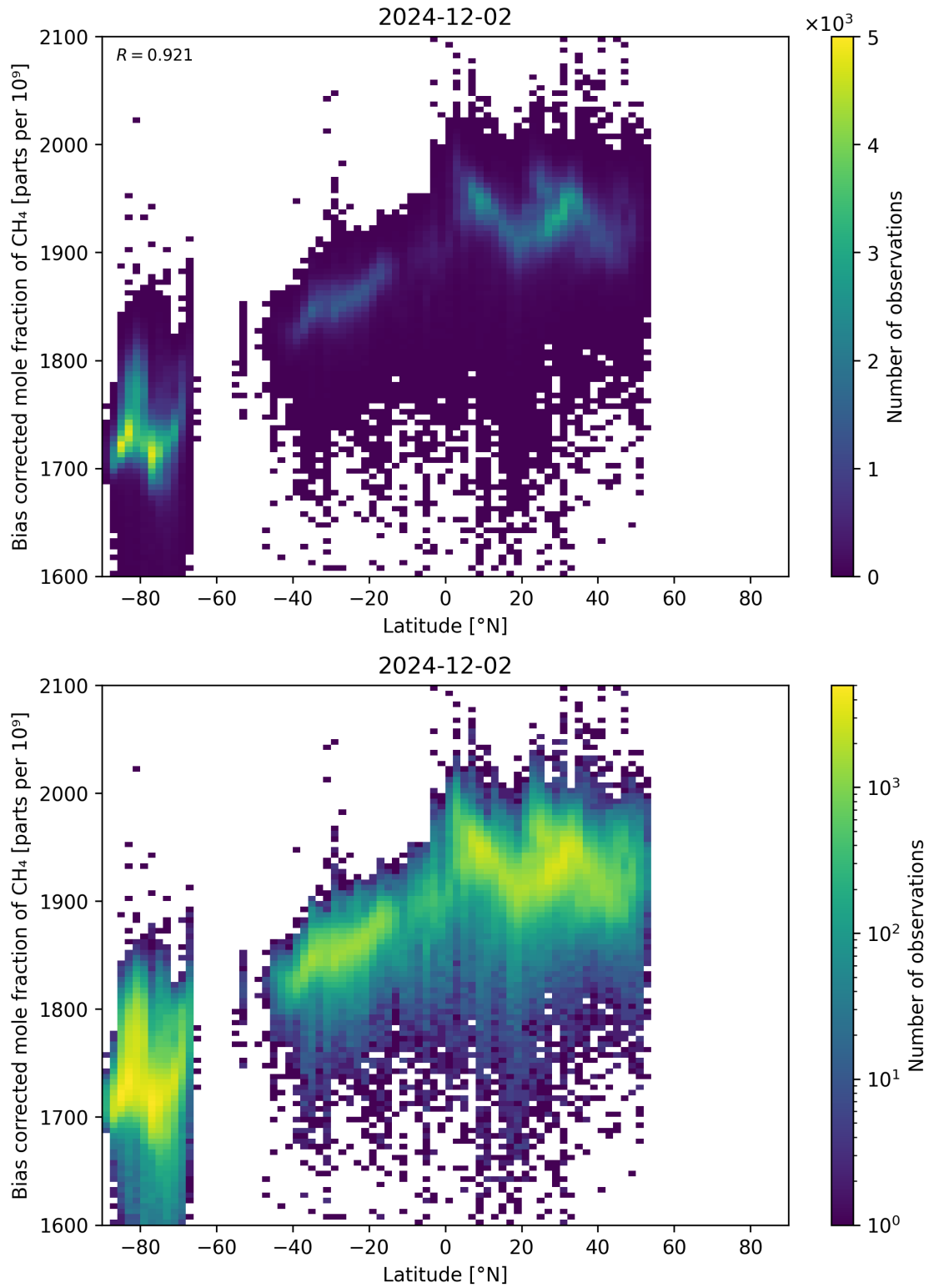
Figure 58: Scatter density plot of “Latitude” against “Bias corrected mole fraction of CH 4 ” for 2024-12-01 to 2024-12-03.
