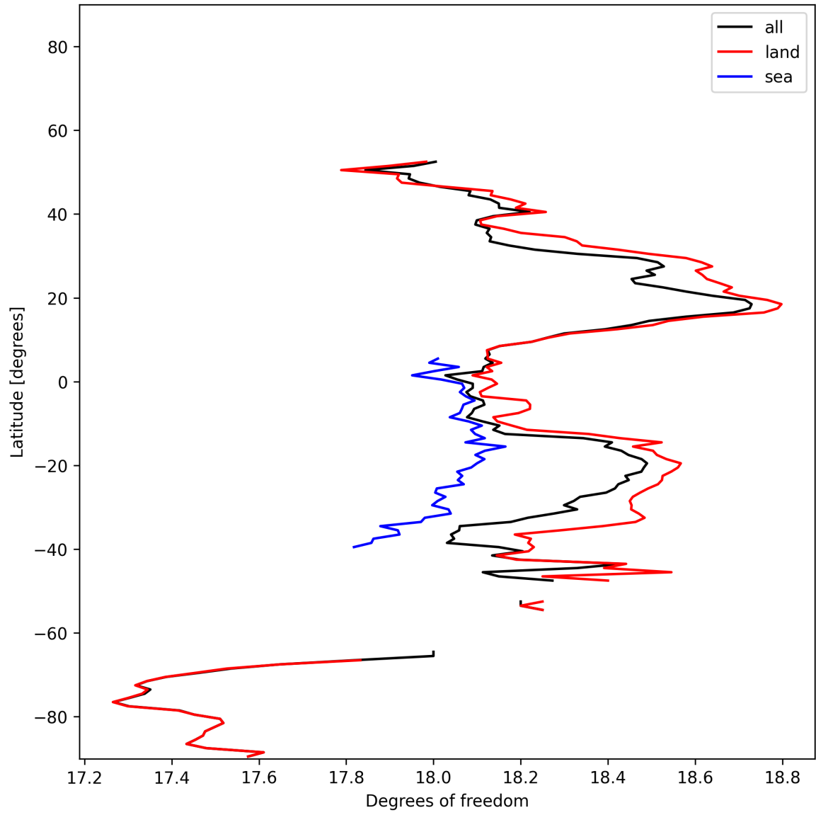
Figure 19: Zonal average of “Degrees of freedom” for 2024-12-01 to 2024-12-03.
