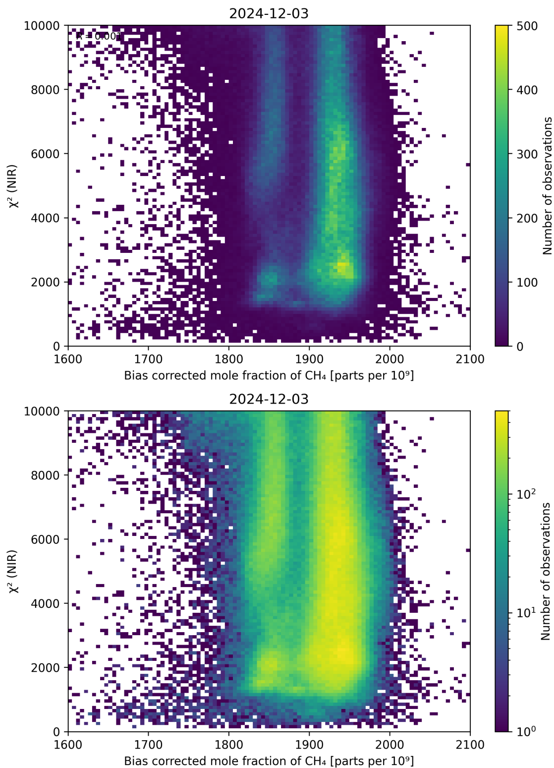
Figure 63: Scatter density plot of “Bias corrected mole fraction of CH 4 ” against “ \chi^2 (NIR)” for 2024-12-02 to 2024-12-04.
