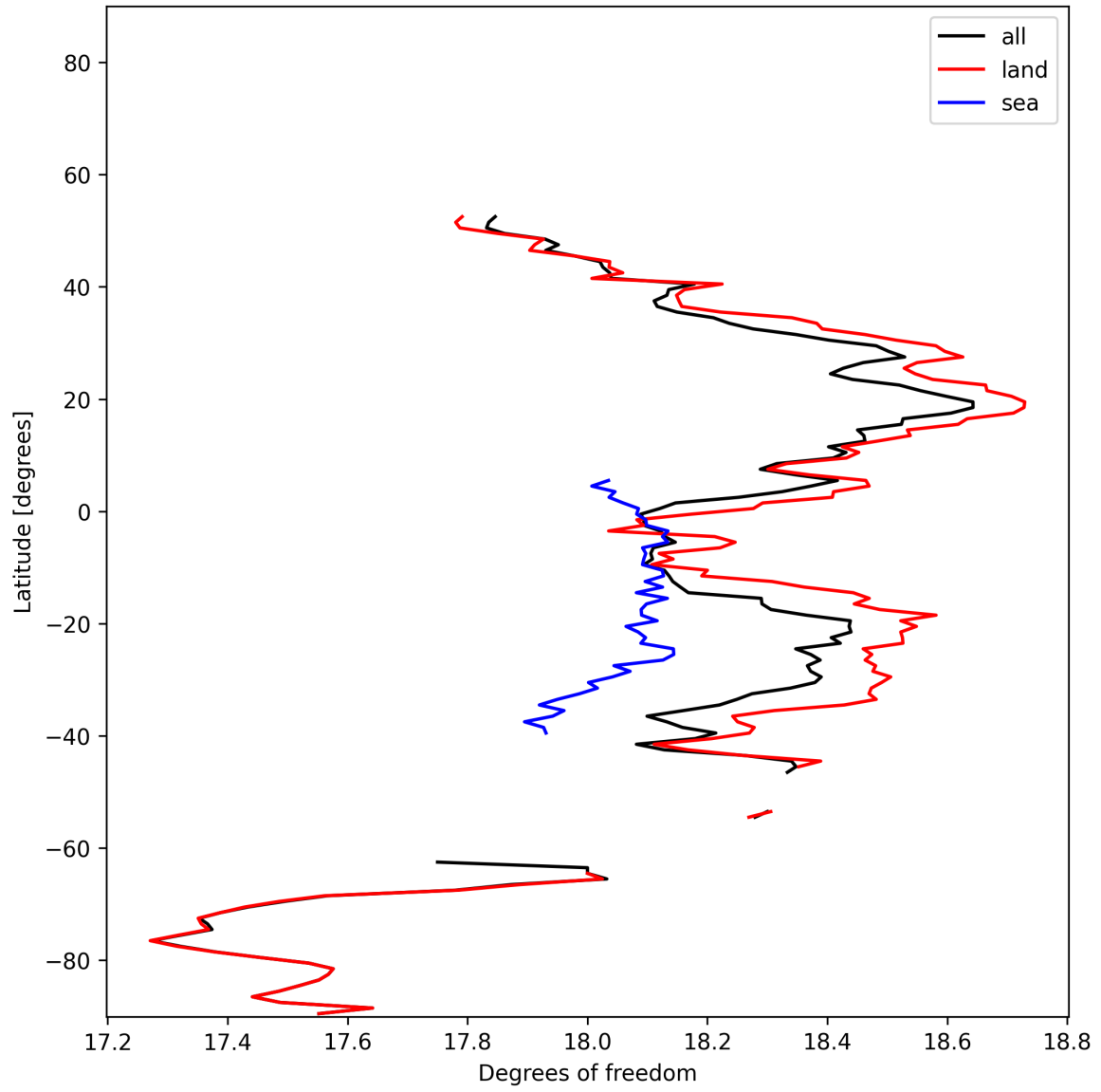
Figure 19: Zonal average of “Degrees of freedom” for 2024-12-02 to 2024-12-04.
