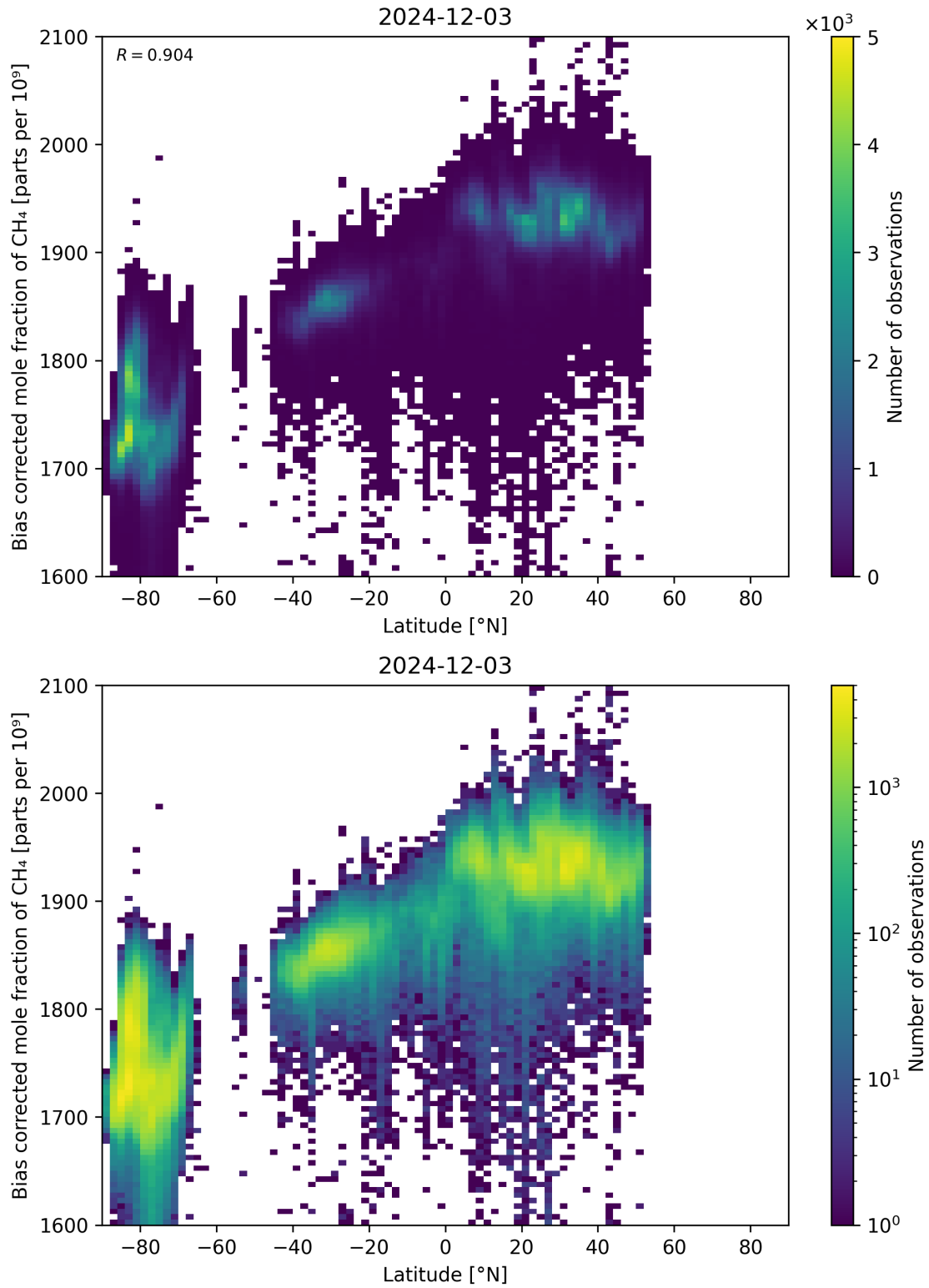
Figure 58: Scatter density plot of “Latitude” against “Bias corrected mole fraction of \text{CH}_4 ” for 2024-12-02 to 2024-12-04.
