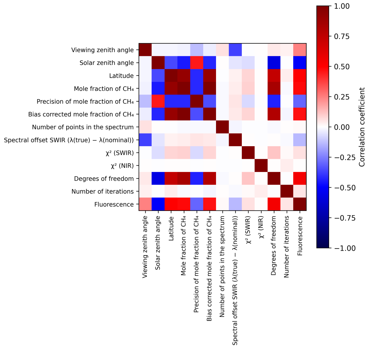
Figure 2: Map of correlation matrix for 2024-12-02 to 2024-12-04.
