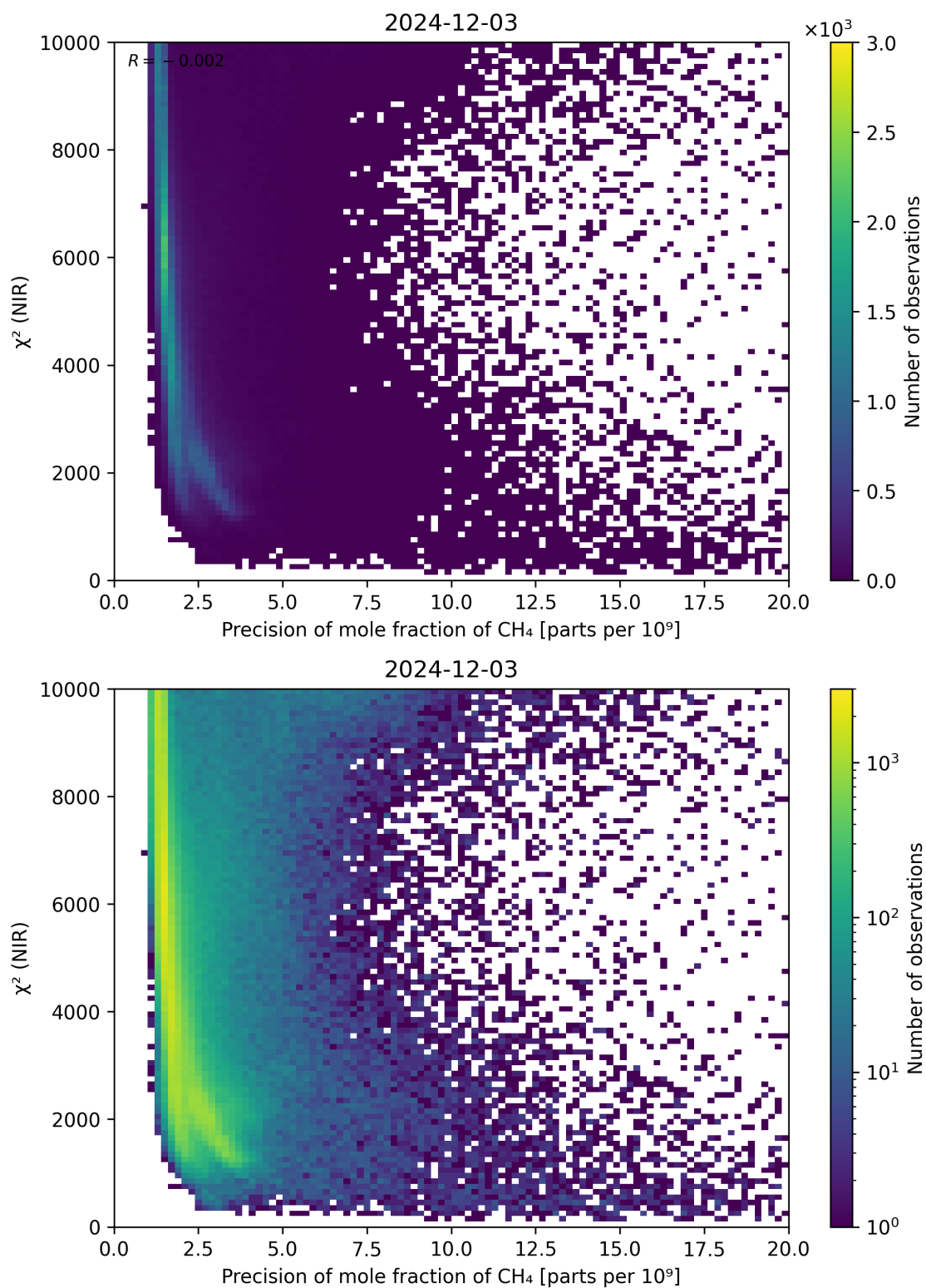
Figure 78: Scatter density plot of “Precision of mole fraction of CH 4 ” against “ \chi^2 (NIR)” for 2024-12-02 to 2024-12-04.
