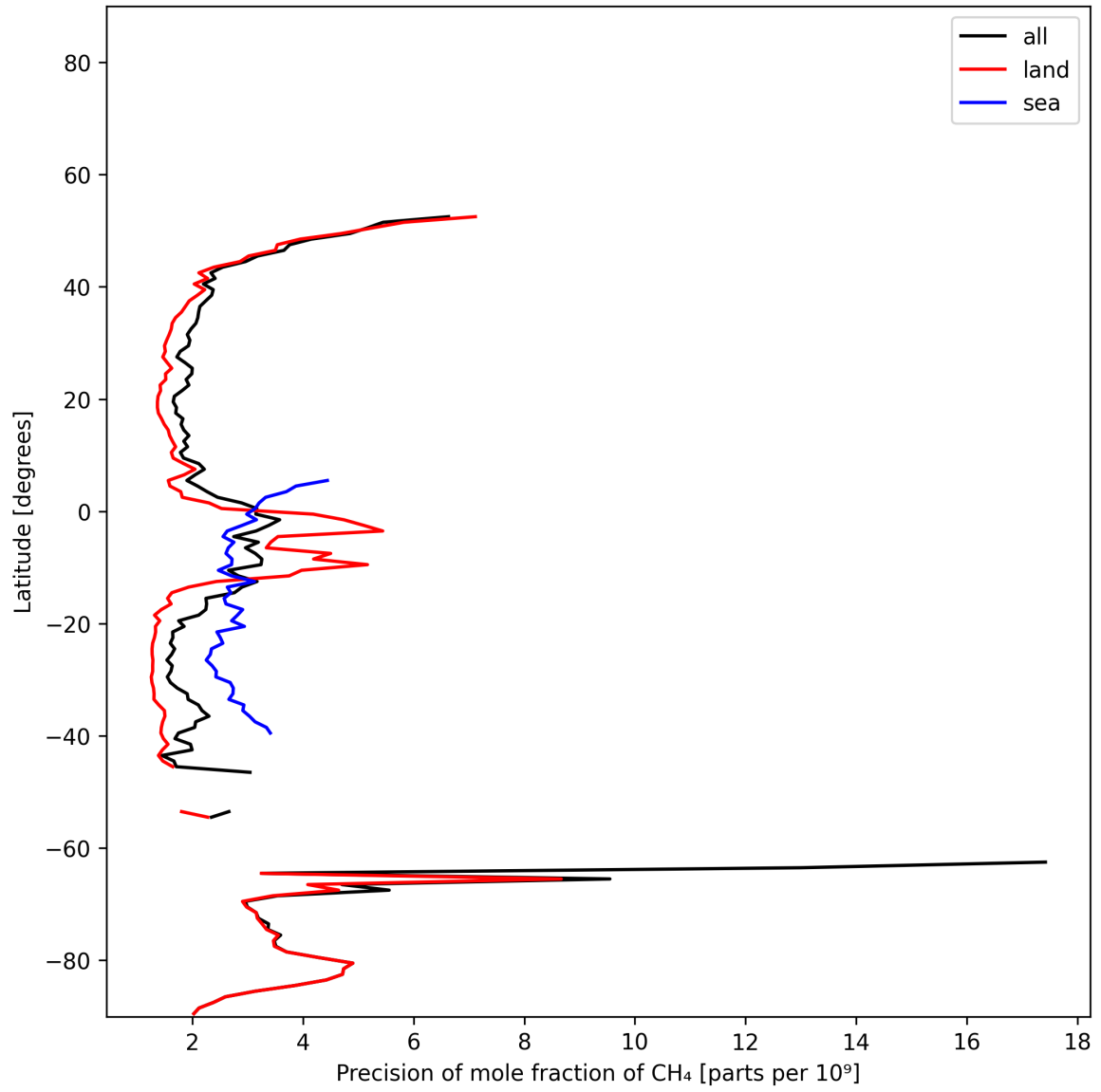
Figure 13: Zonal average of “Precision of mole fraction of CH 4 ” for 2024-12-02 to 2024-12-04.
