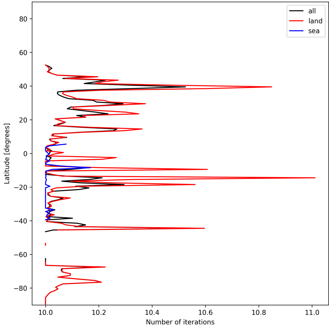
Figure 20: Zonal average of “Number of iterations” for 2024-12-02 to 2024-12-04.
