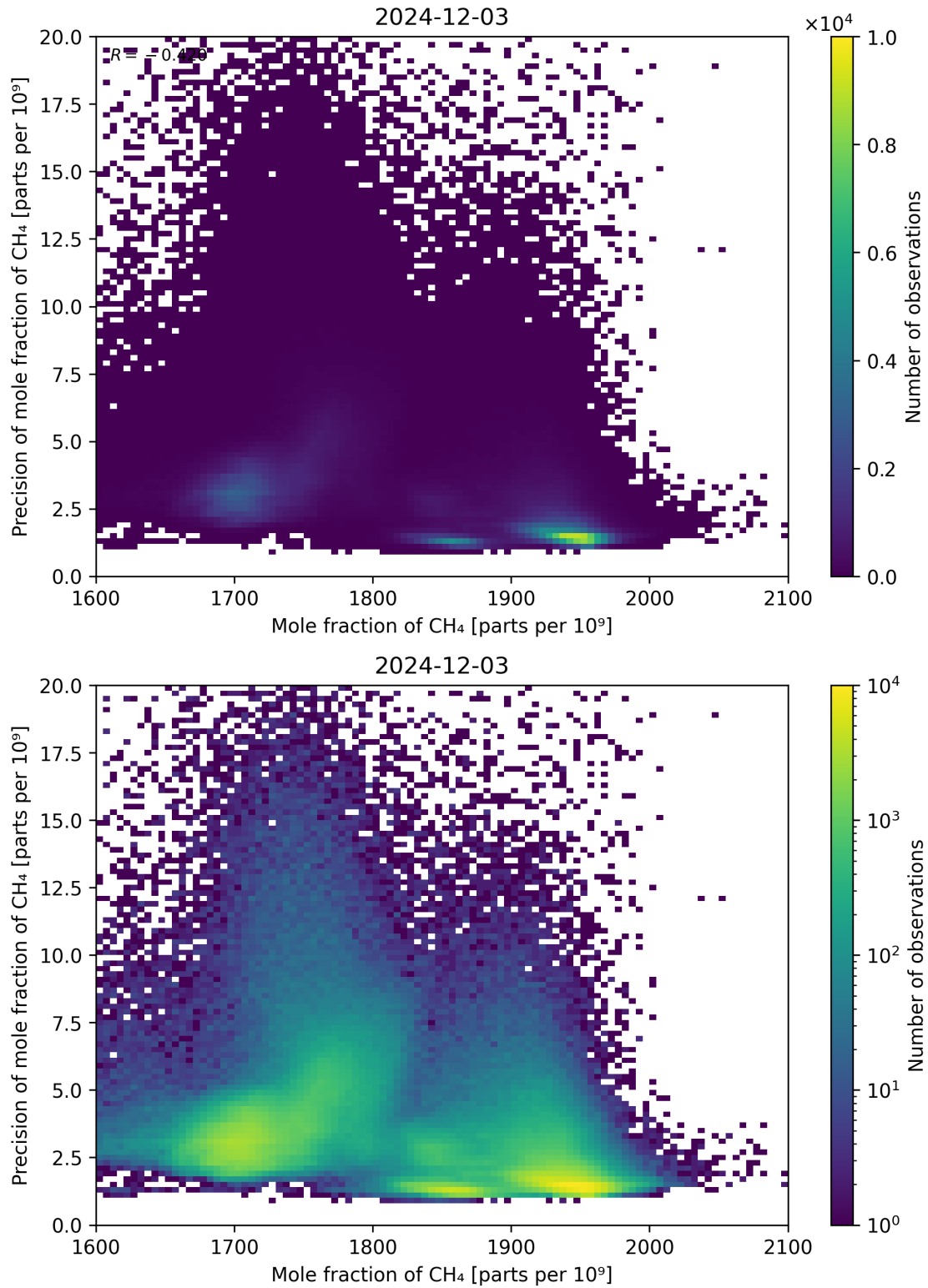
Figure 75: Scatter density plot of “Mole fraction of CH 4 ” against “Precision of mole fraction of CH 4 ” for 2024-12-02 to 2024-12-04.
