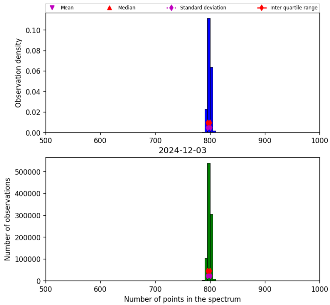
Figure 26: Histogram of “Number of points in the spectrum” for 2024-12-02 to 2024-12-04
