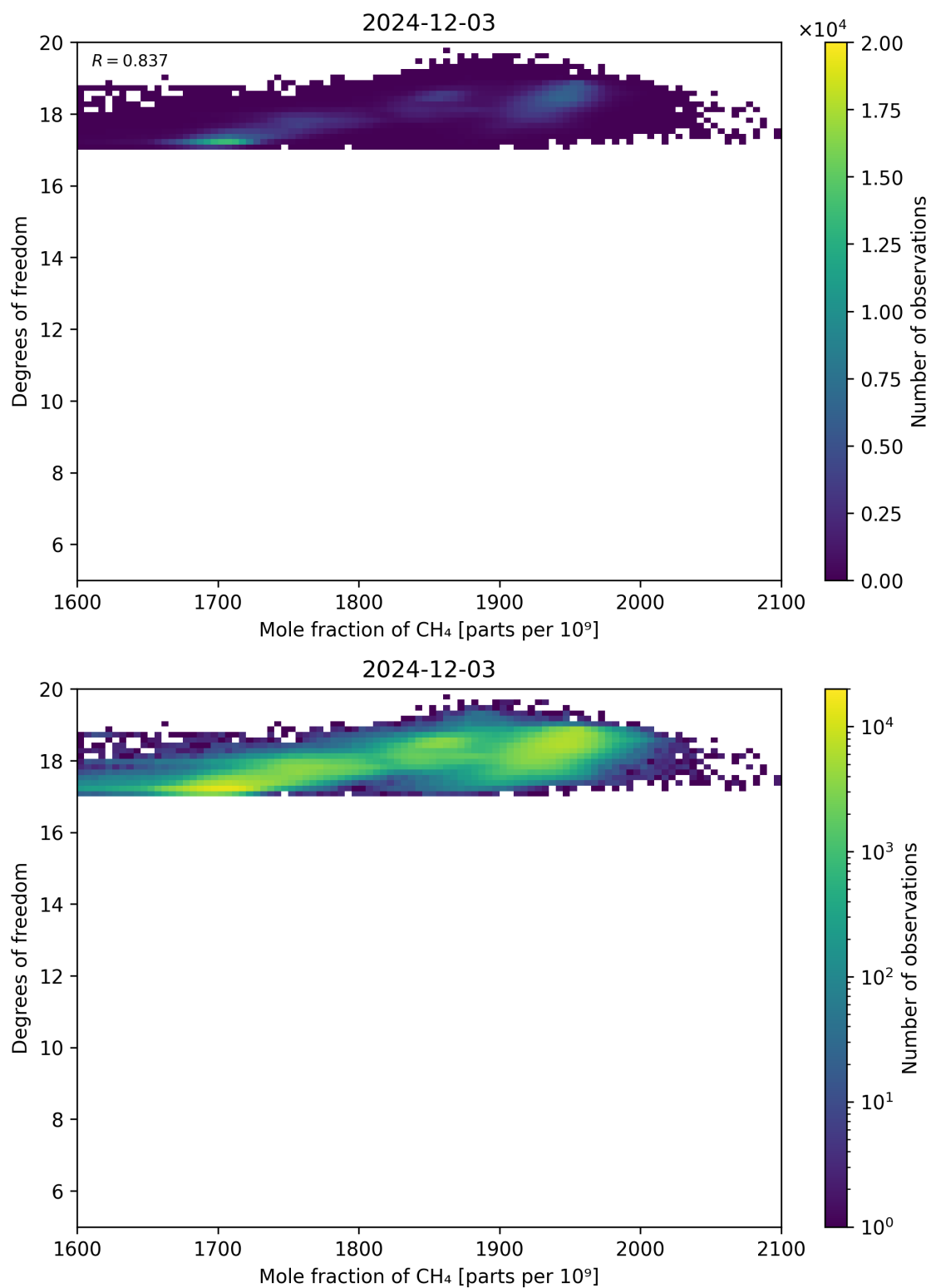
Figure 72: Scatter density plot of “Mole fraction of CH 4 ” against “Degrees of freedom” for 2024-12-02 to 2024-12-04.
