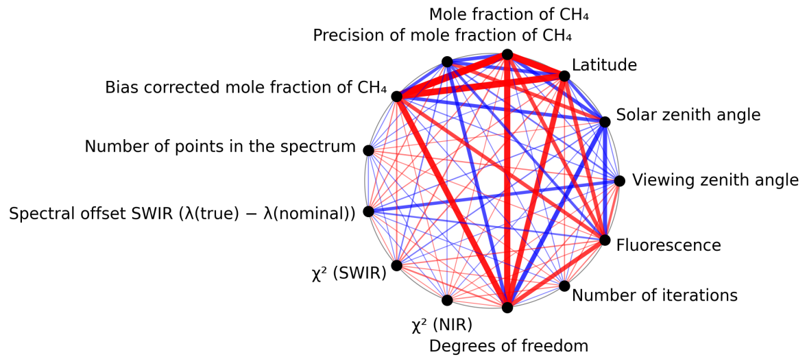
Figure 1: Map of correlation graph for 2024-12-02 to 2024-12-04.
