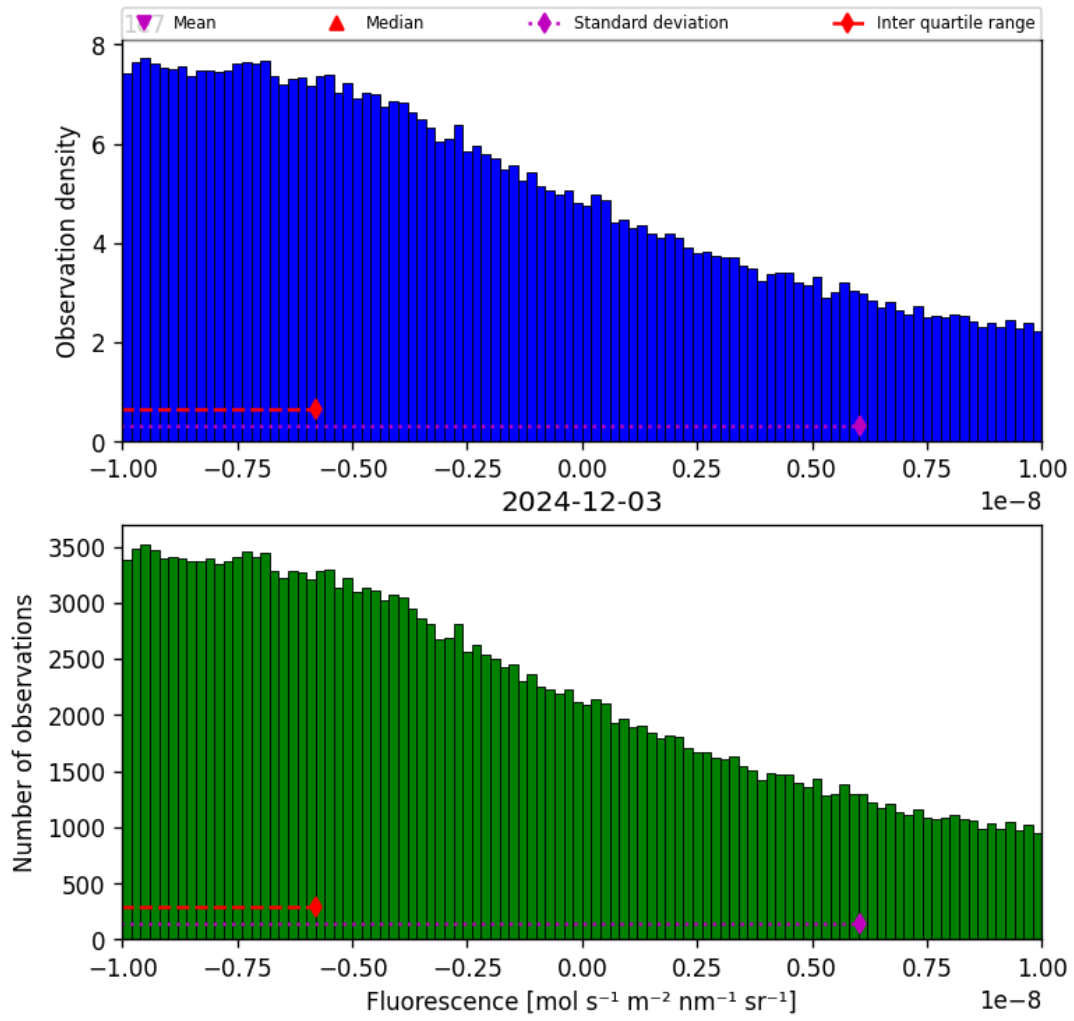
Figure 32: Histogram of “Fluorescence” for 2024-12-02 to 2024-12-04
