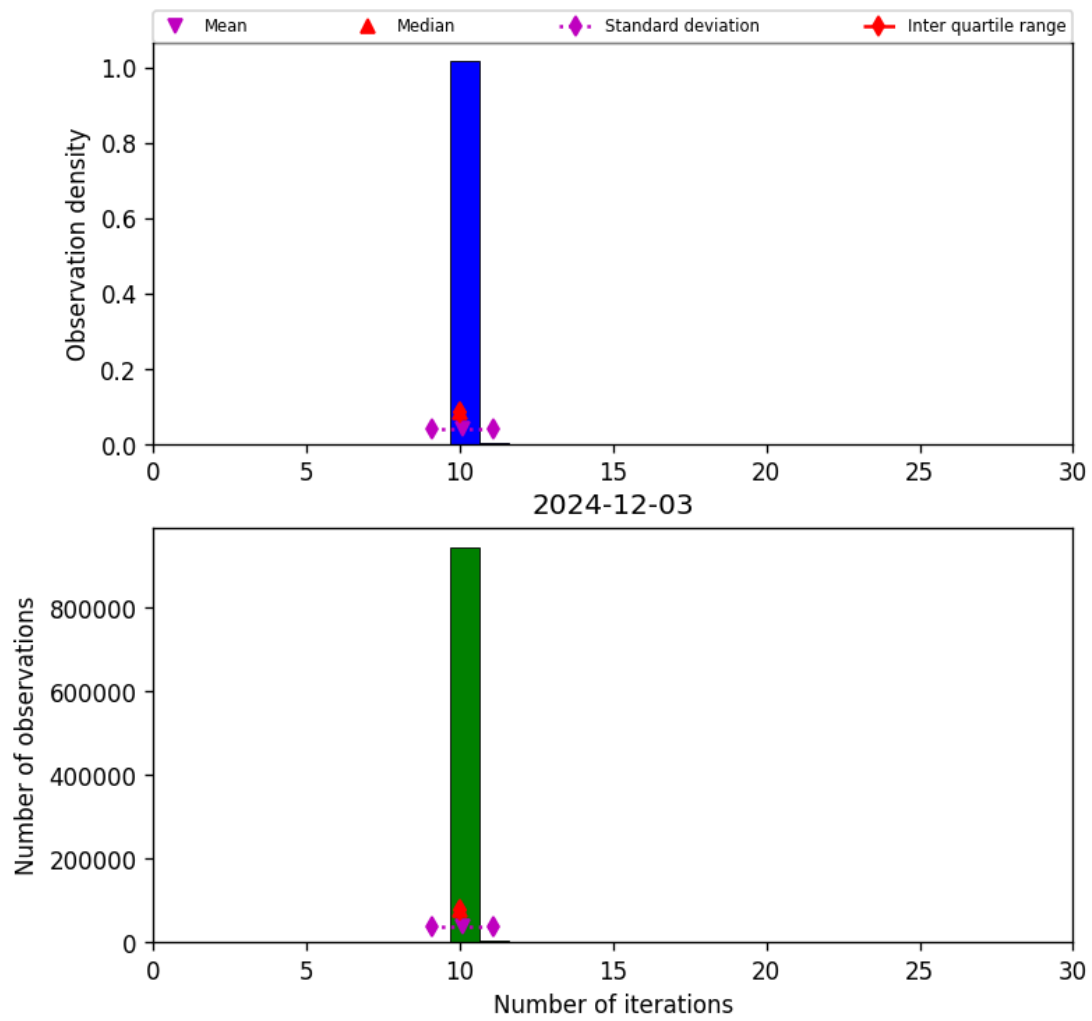
Figure 31: Histogram of “Number of iterations” for 2024-12-02 to 2024-12-04
