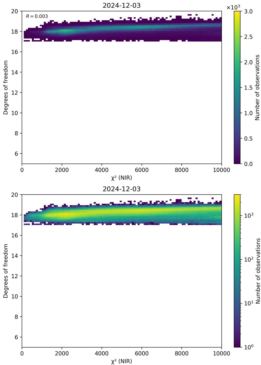
Figure 44: Scatter density plot of “ \chi^2 (NIR)” against “Degrees of freedom” for 2024-12-02 to 2024-12-04.
