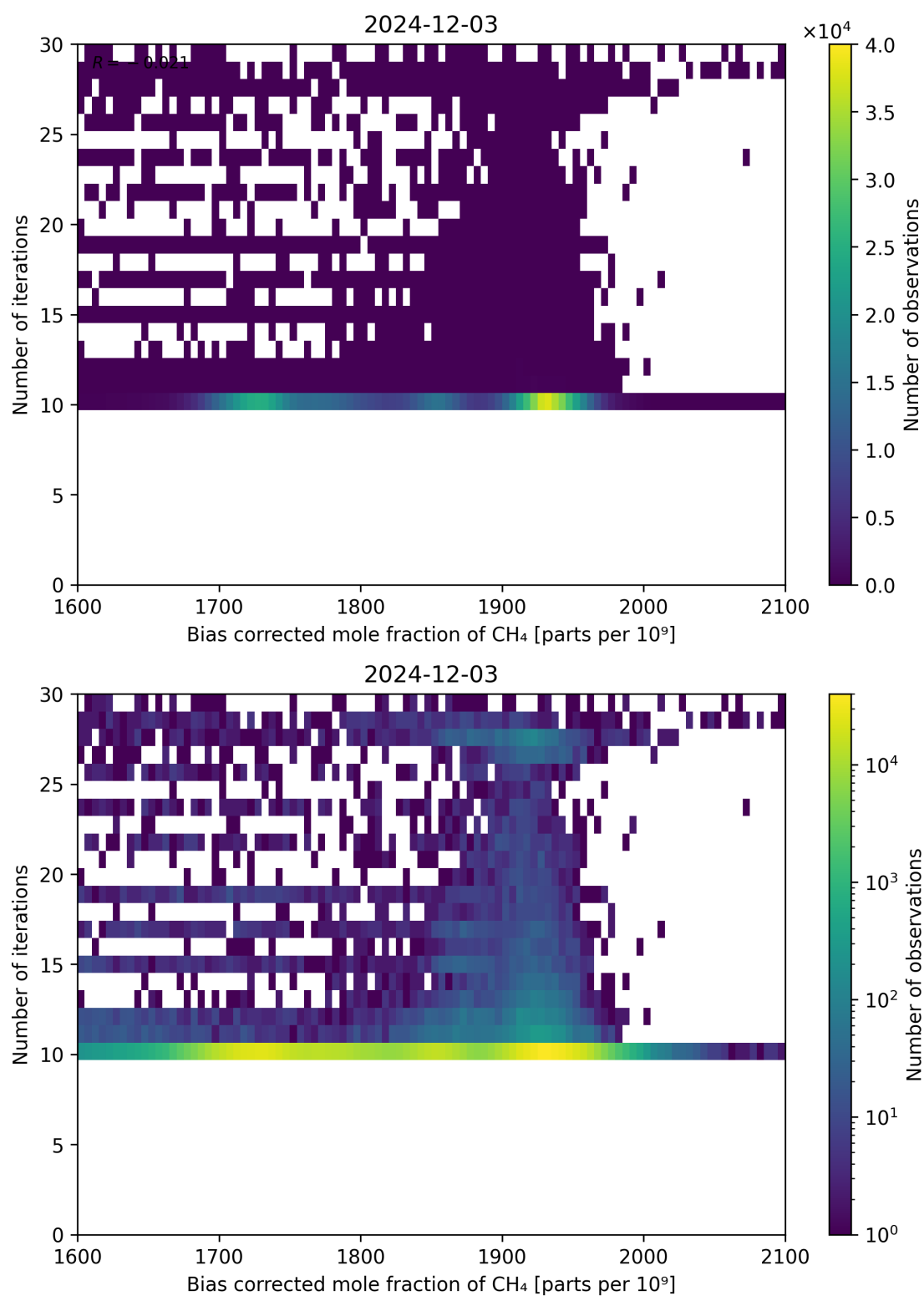
Figure 67: Scatter density plot of “Bias corrected mole fraction of CH 4 ” against “Number of iterations” for 2024-12-02 to 2024-12-04.
