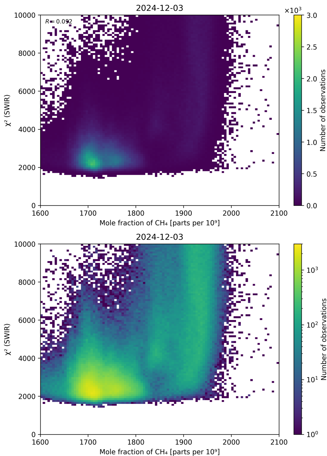
Figure 71: Scatter density plot of “Mole fraction of \text{CH}_4 ” against “ \chi^2 (SWIR)” for 2024-12-02 to 2024-12-04.
