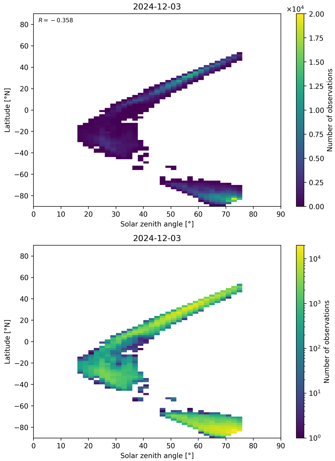
Figure 98: Scatter density plot of “Solar zenith angle” against “Latitude” for 2024-12-02 to 2024-12-04.
