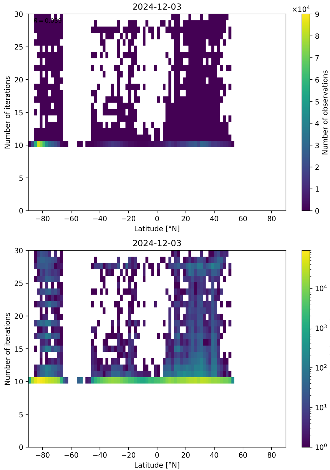
Figure 60: Scatter density plot of “Latitude” against “Number of iterations” for 2024-12-02 to 2024-12-04.
