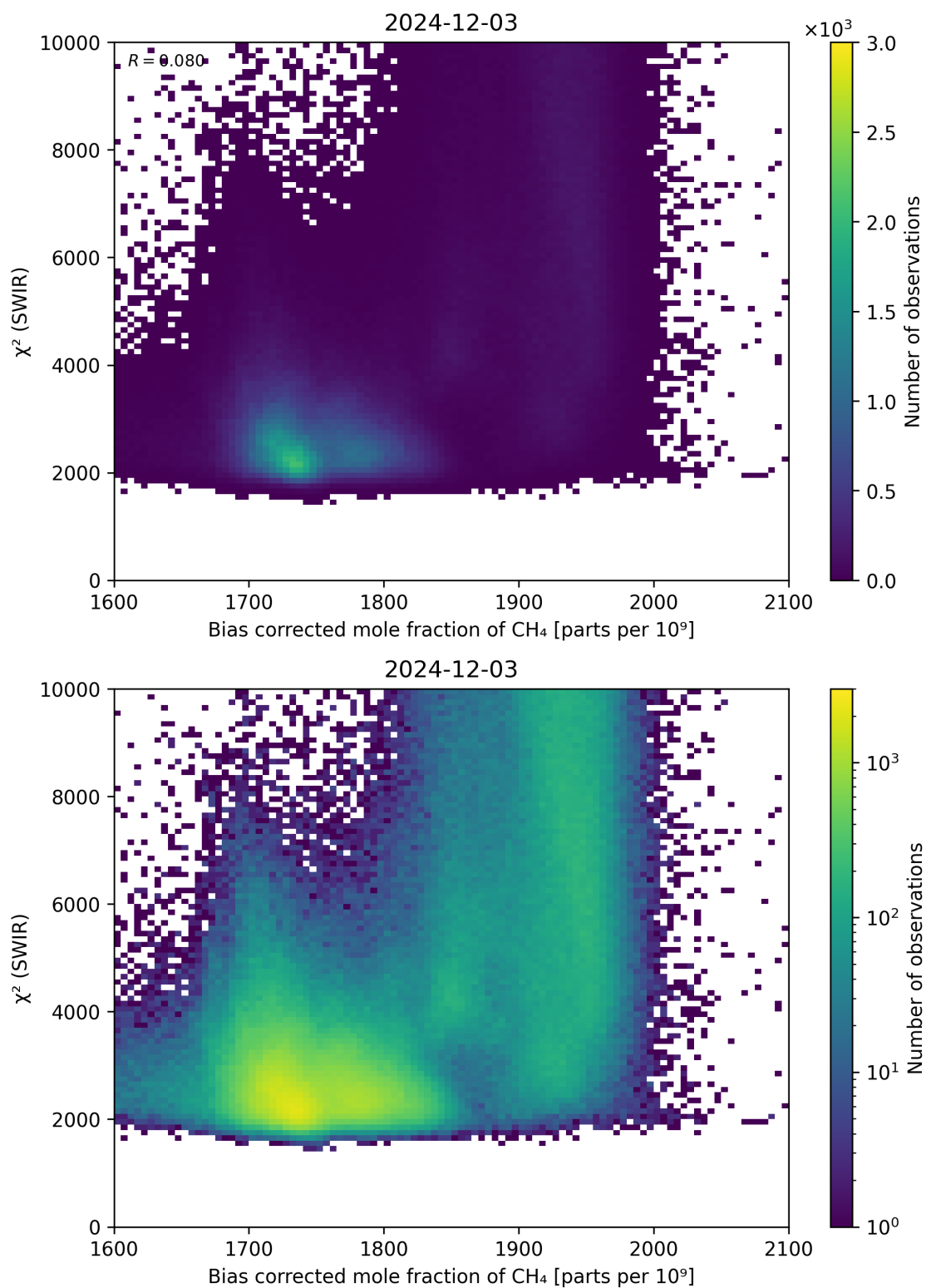
Figure 64: Scatter density plot of “Bias corrected mole fraction of \text{CH}_4 ” against “ \chi^2 (SWIR)” for 2024-12-02 to 2024-12-04.
