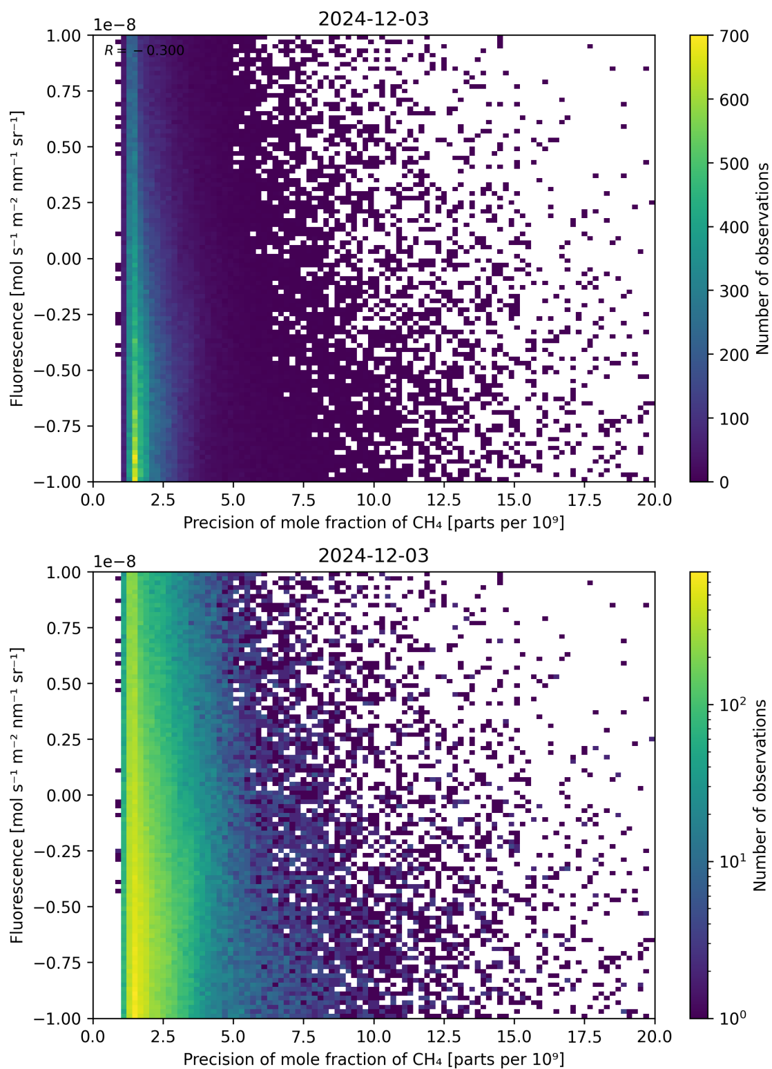
Figure 81: Scatter density plot of “Precision of mole fraction of \text{CH}_4 ” against “Fluorescence” for 2024-12-02 to 2024-12-04.
