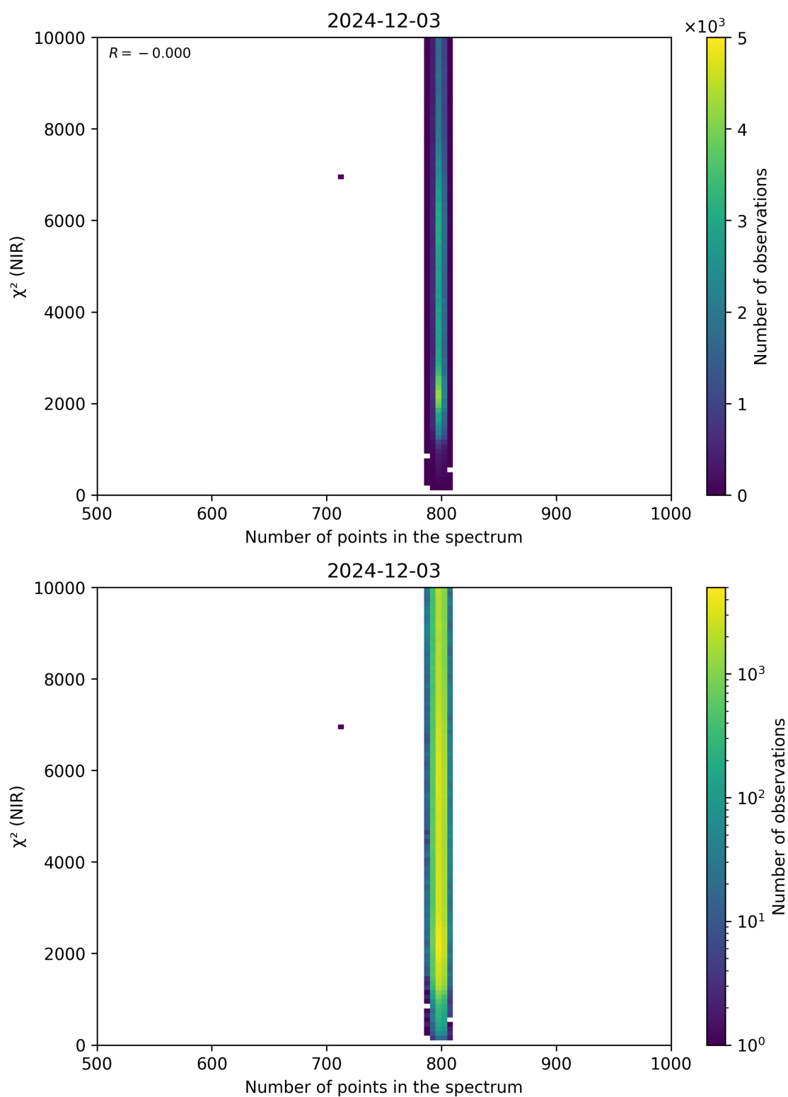
Figure 88: Scatter density plot of “Number of points in the spectrum” against “ \chi^2 (NIR)” for 2024-12-02 to 2024-12-04.
