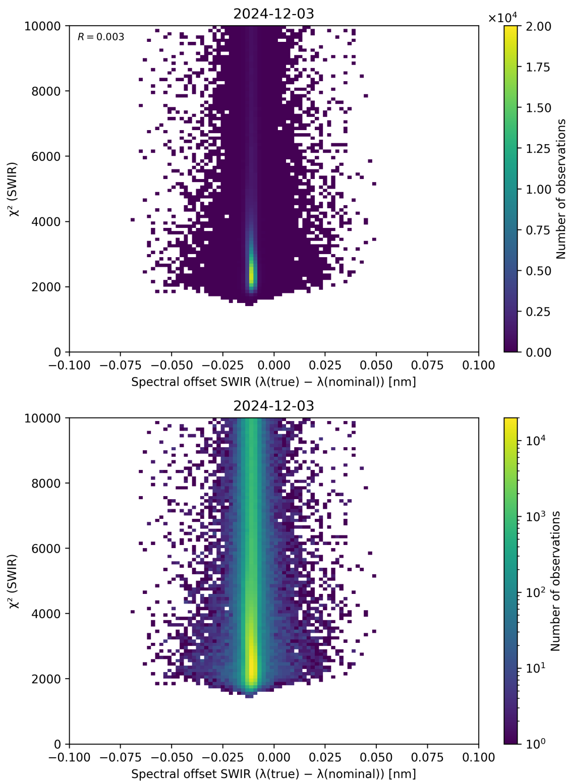
Figure 118: Scatter density plot of “Spectral offset SWIR ( \lambda_{\text{true}} - \lambda_{\text{nominal}} )” against “ \chi^2 (SWIR)” for 2024-12-02 to 2024-12-04.
