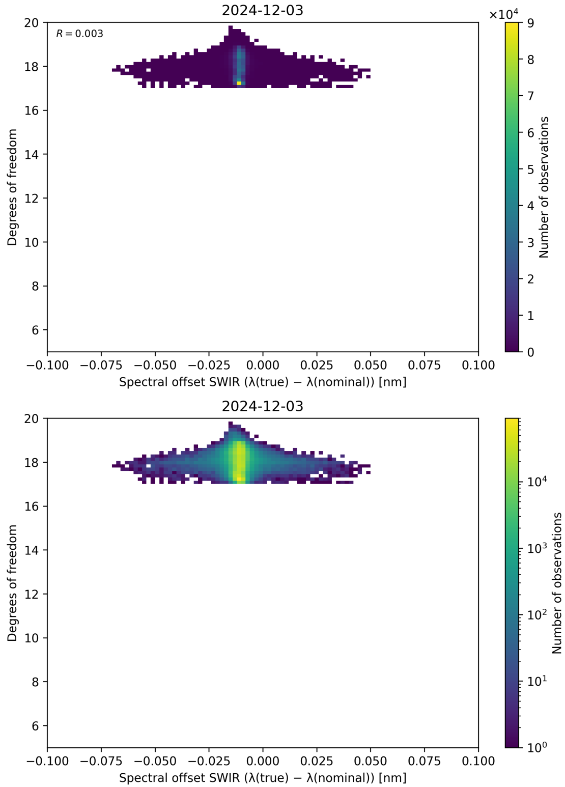
Figure 119: Scatter density plot of “Spectral offset SWIR ( \lambda_{\text{true}} - \lambda_{\text{nominal}} )” against “Degrees of freedom” for 2024-12-02 to 2024-12-04.
