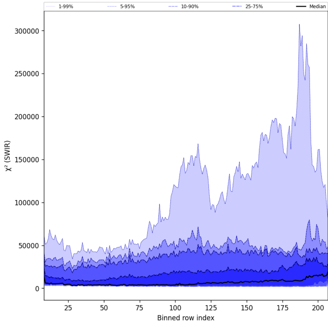
Figure 39: Along track statistics of “ \chi^2 (SWIR)” for 2024-12-02 to 2024-12-04
