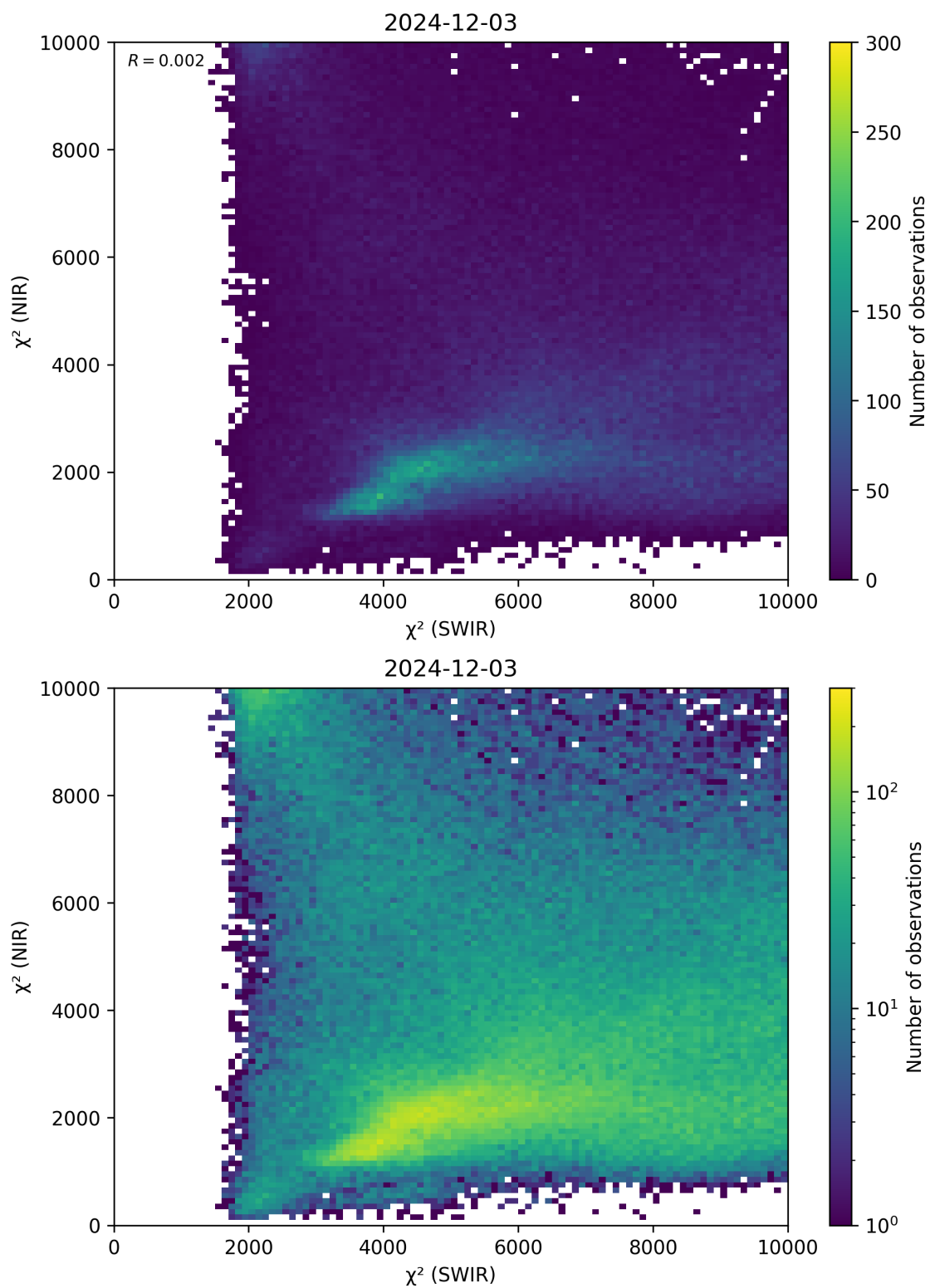
Figure 47: Scatter density plot of “ \chi^2 (SWIR)” against “ \chi^2 (NIR)” for 2024-12-02 to 2024-12-04.
