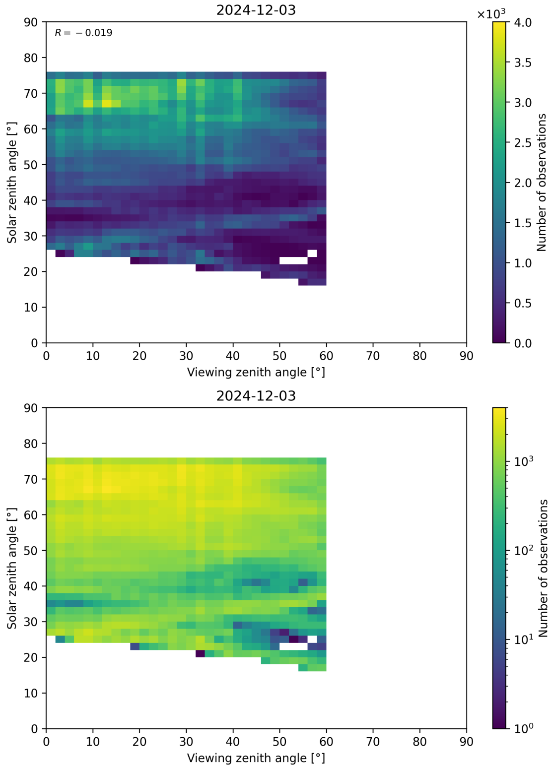
Figure 115: Scatter density plot of “Viewing zenith angle” against “Solar zenith angle” for 2024-12-02 to 2024-12-04.
