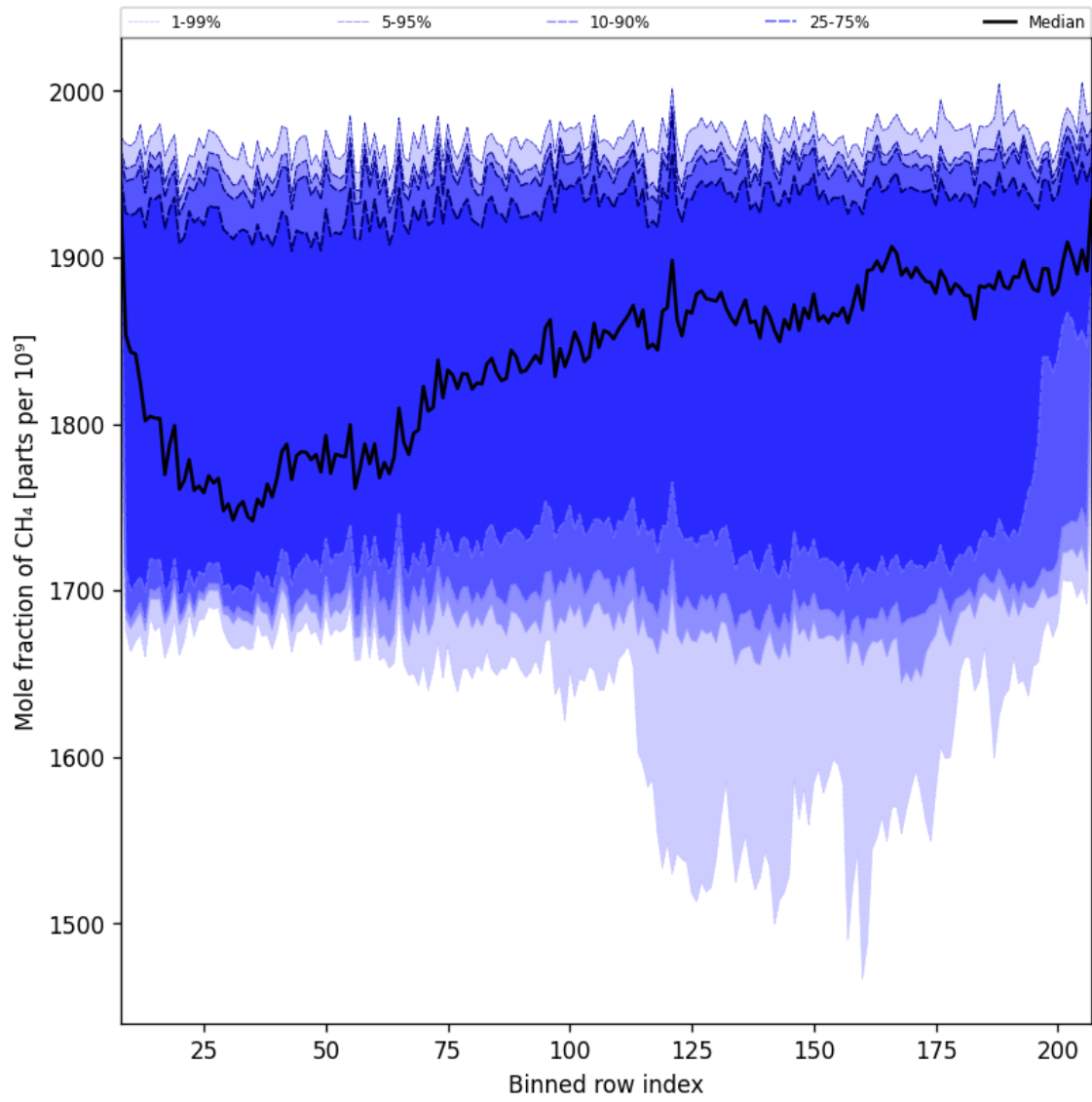
Figure 34: Along track statistics of “Mole fraction of CH 4 ” for 2024-12-02 to 2024-12-04
