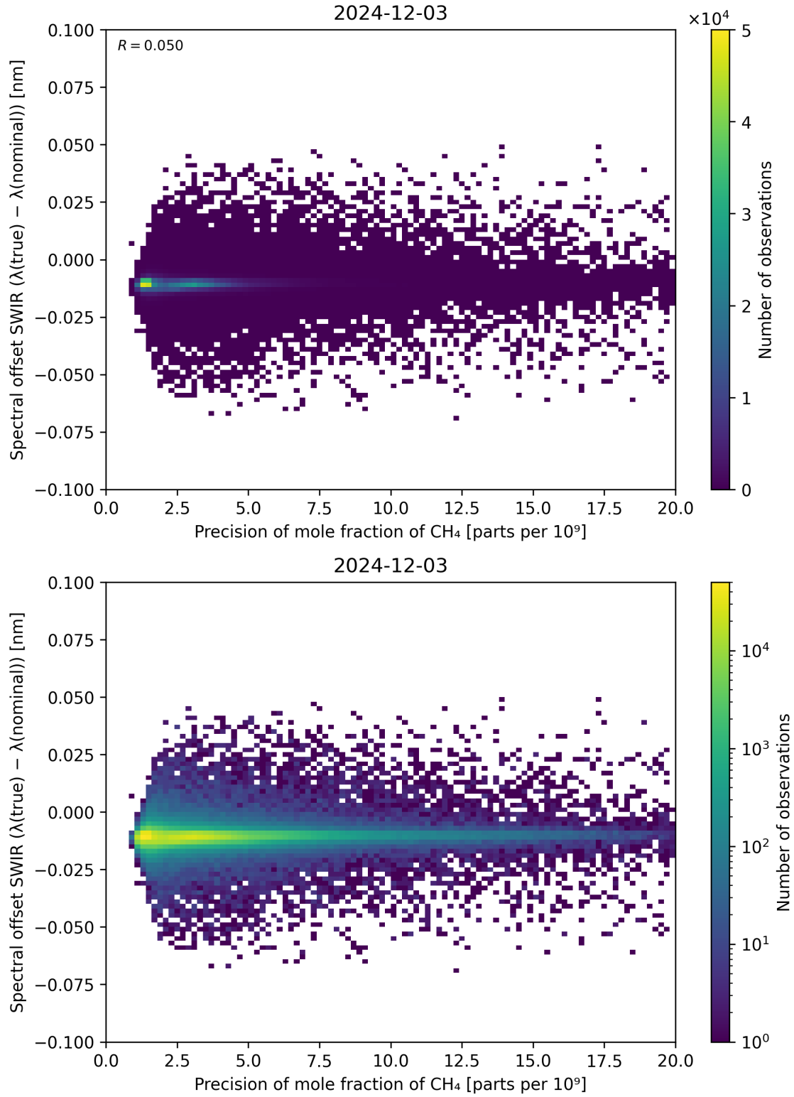
Figure 85: Scatter density plot of “Precision of mole fraction of \text{CH}_4 ” against “Spectral offset SWIR ( \lambda_{\text{true}} - \lambda_{\text{nominal}} )” for 2024-12-02 to 2024-12-04.
