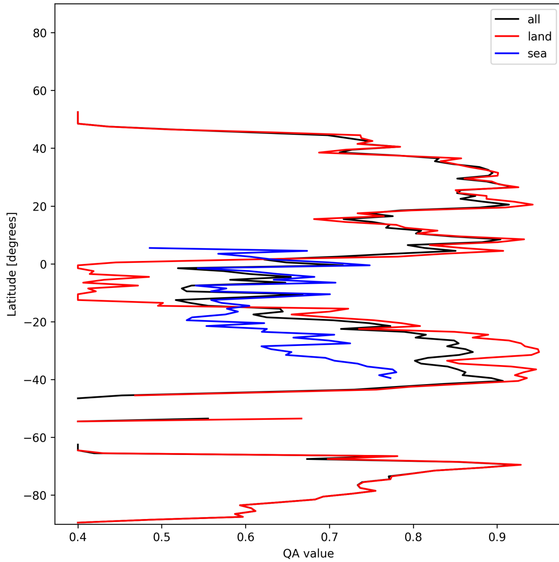
Figure 11: Zonal average of “QA value” for 2024-12-02 to 2024-12-04.
