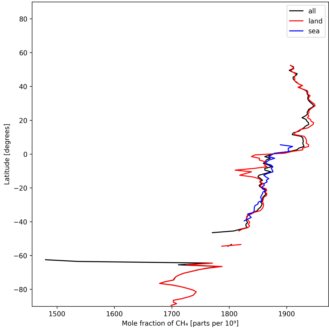
Figure 12: Zonal average of “Mole fraction of CH 4 ” for 2024-12-02 to 2024-12-04.
