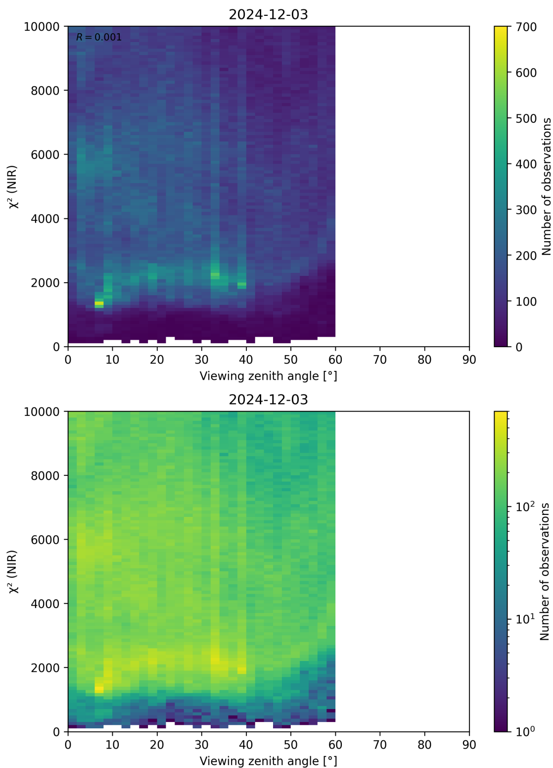
Figure 105: Scatter density plot of “Viewing zenith angle” against “ \chi^2 (NIR)” for 2024-12-02 to 2024-12-04.
