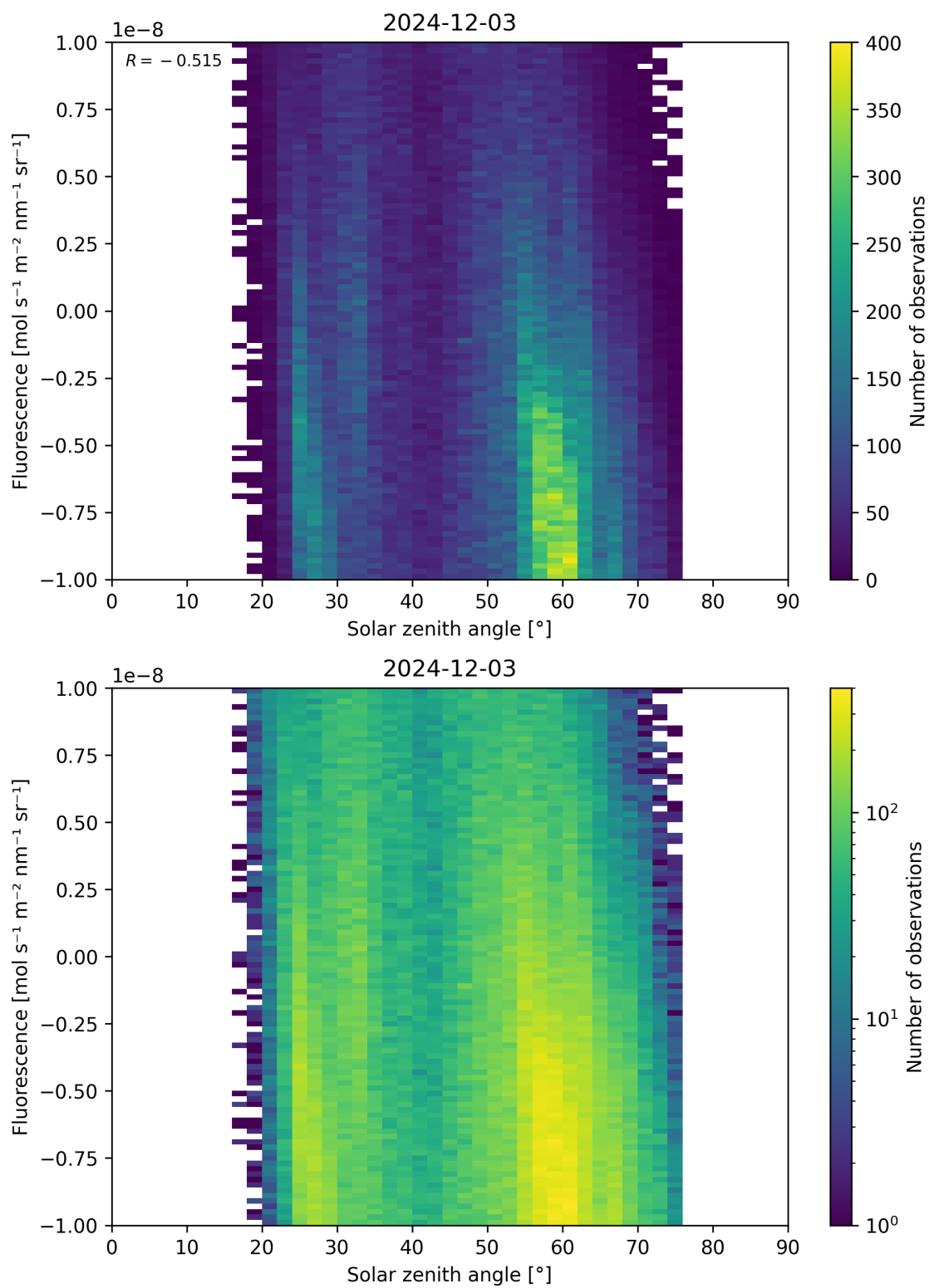
Figure 97: Scatter density plot of “Solar zenith angle” against “Fluorescence” for 2024-12-02 to 2024-12-04.
