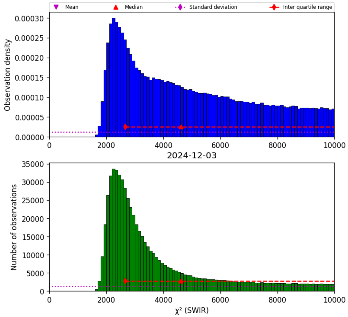
Figure 28: Histogram of “ \chi^2 (SWIR)” for 2024-12-02 to 2024-12-04
