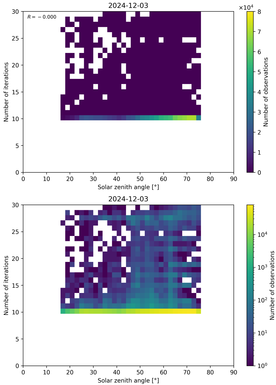
Figure 102: Scatter density plot of “Solar zenith angle” against “Number of iterations” for 2024-12-02 to 2024-12-04.
