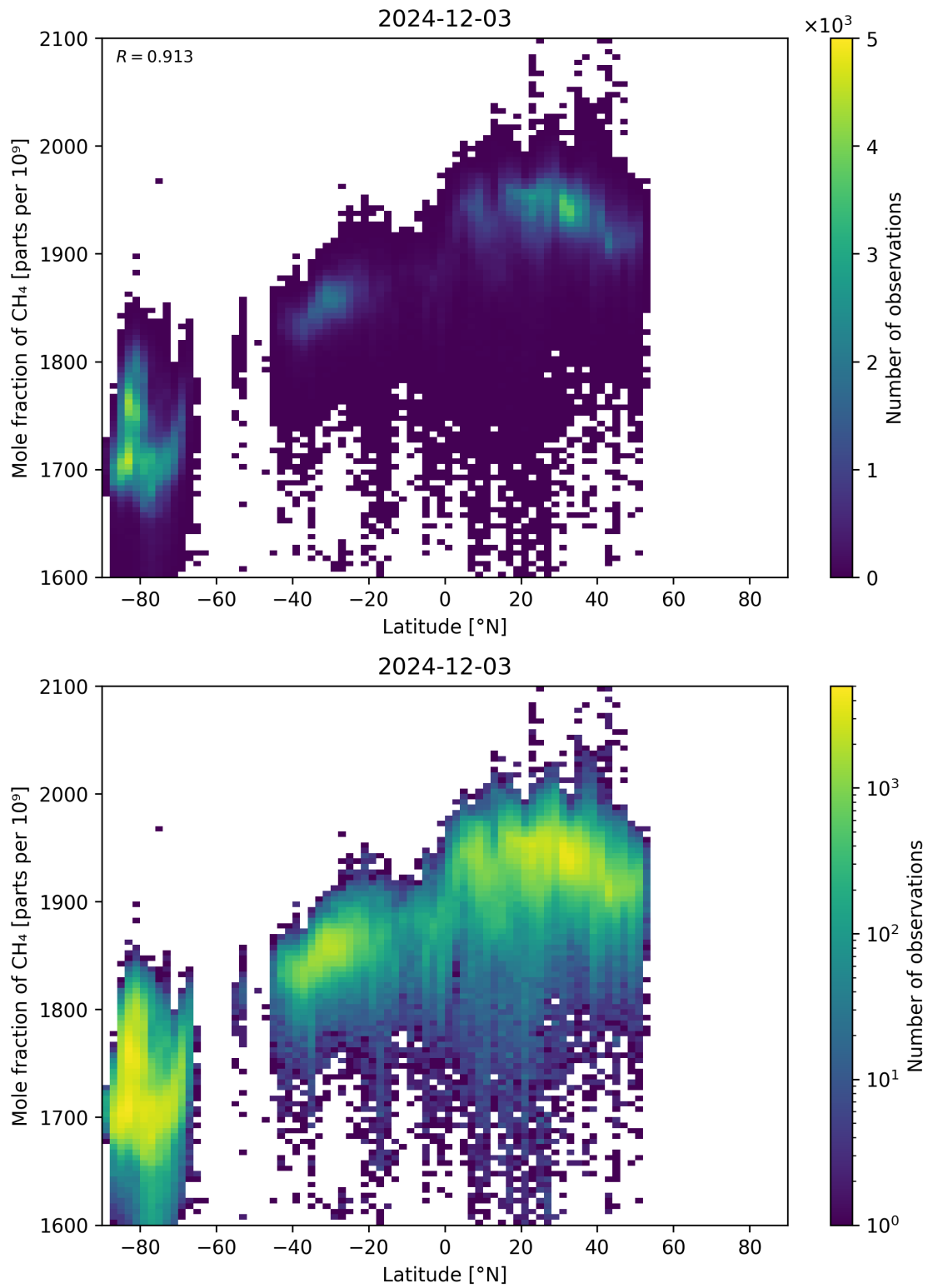
Figure 57: Scatter density plot of “Latitude” against “Mole fraction of CH 4 ” for 2024-12-02 to 2024-12-04.
