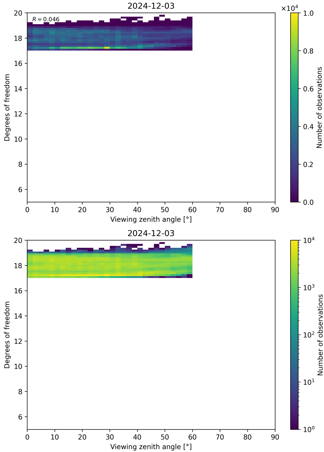
Figure 107: Scatter density plot of “Viewing zenith angle” against “Degrees of freedom” for 2024-12-02 to 2024-12-04.
