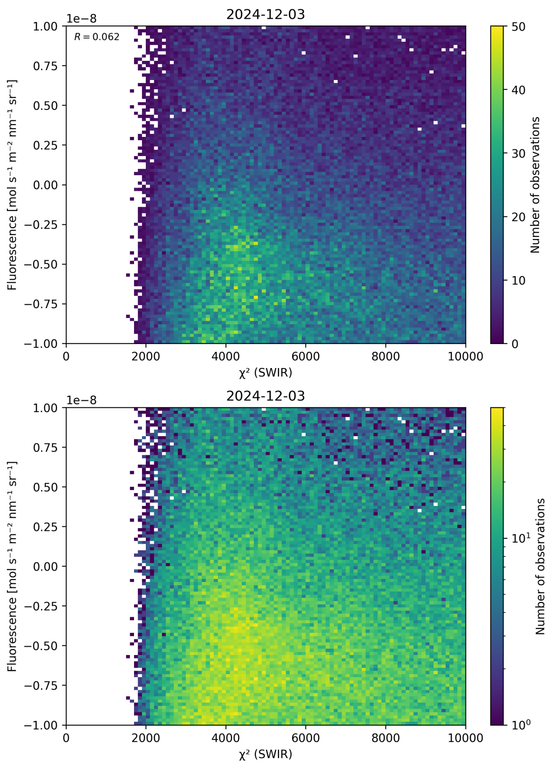
Figure 49: Scatter density plot of “ \chi^2 (SWIR)” against “Fluorescence” for 2024-12-02 to 2024-12-04.
