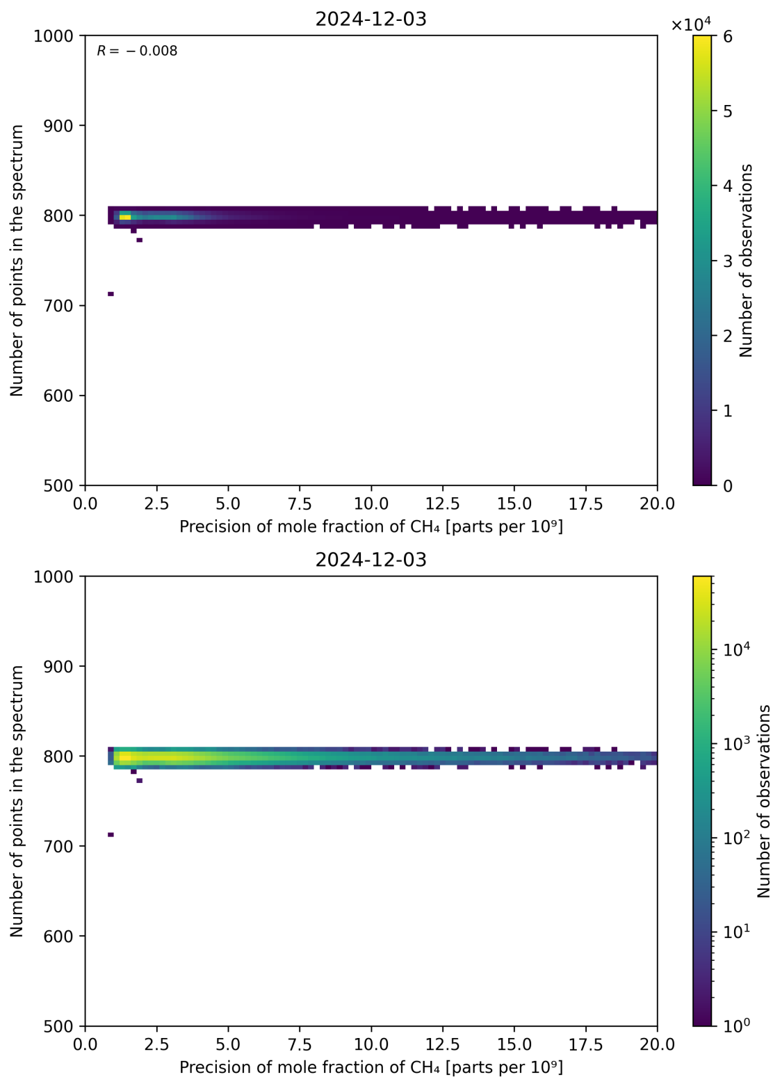
Figure 84: Scatter density plot of “Precision of mole fraction of CH 4 ” against “Number of points in the spectrum” for 2024-12-02 to 2024-12-04.
