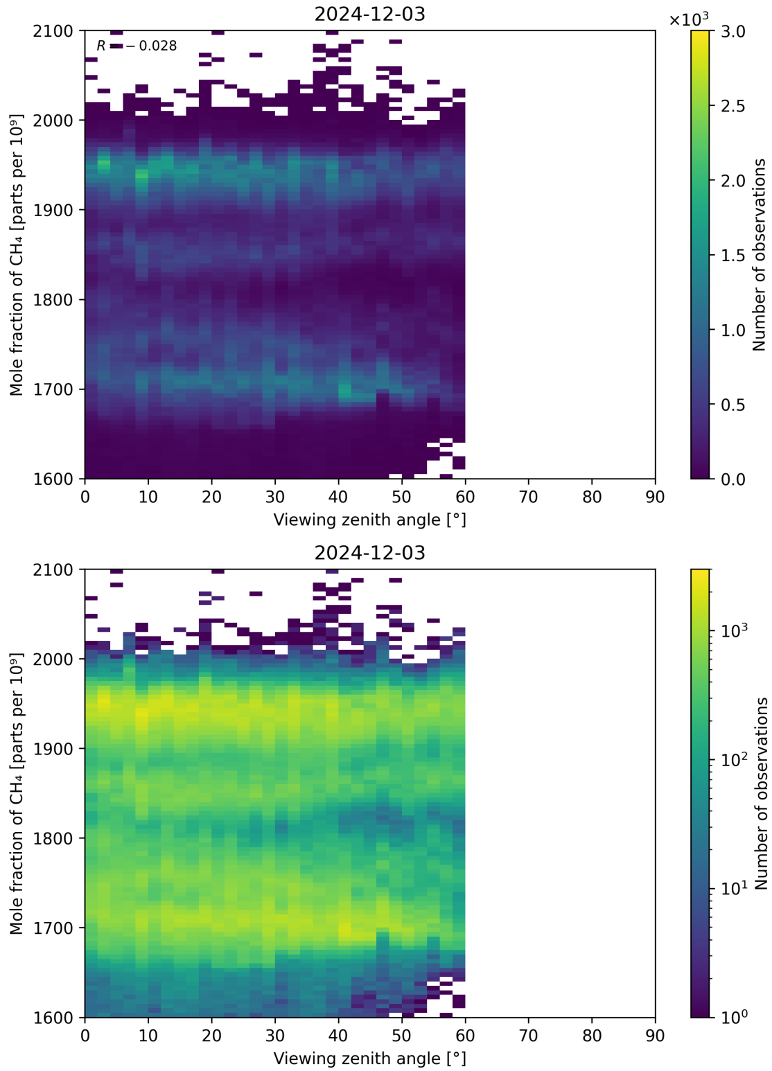
Figure 110: Scatter density plot of “Viewing zenith angle” against “Mole fraction of CH 4 ” for 2024-12-02 to 2024-12-04.
