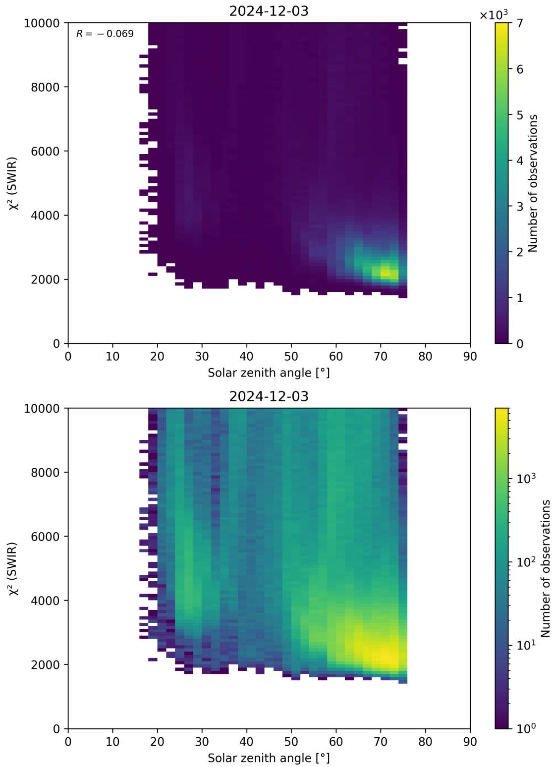
Figure 95: Scatter density plot of “Solar zenith angle” against “ \chi^2 (SWIR)” for 2024-12-02 to 2024-12-04.
