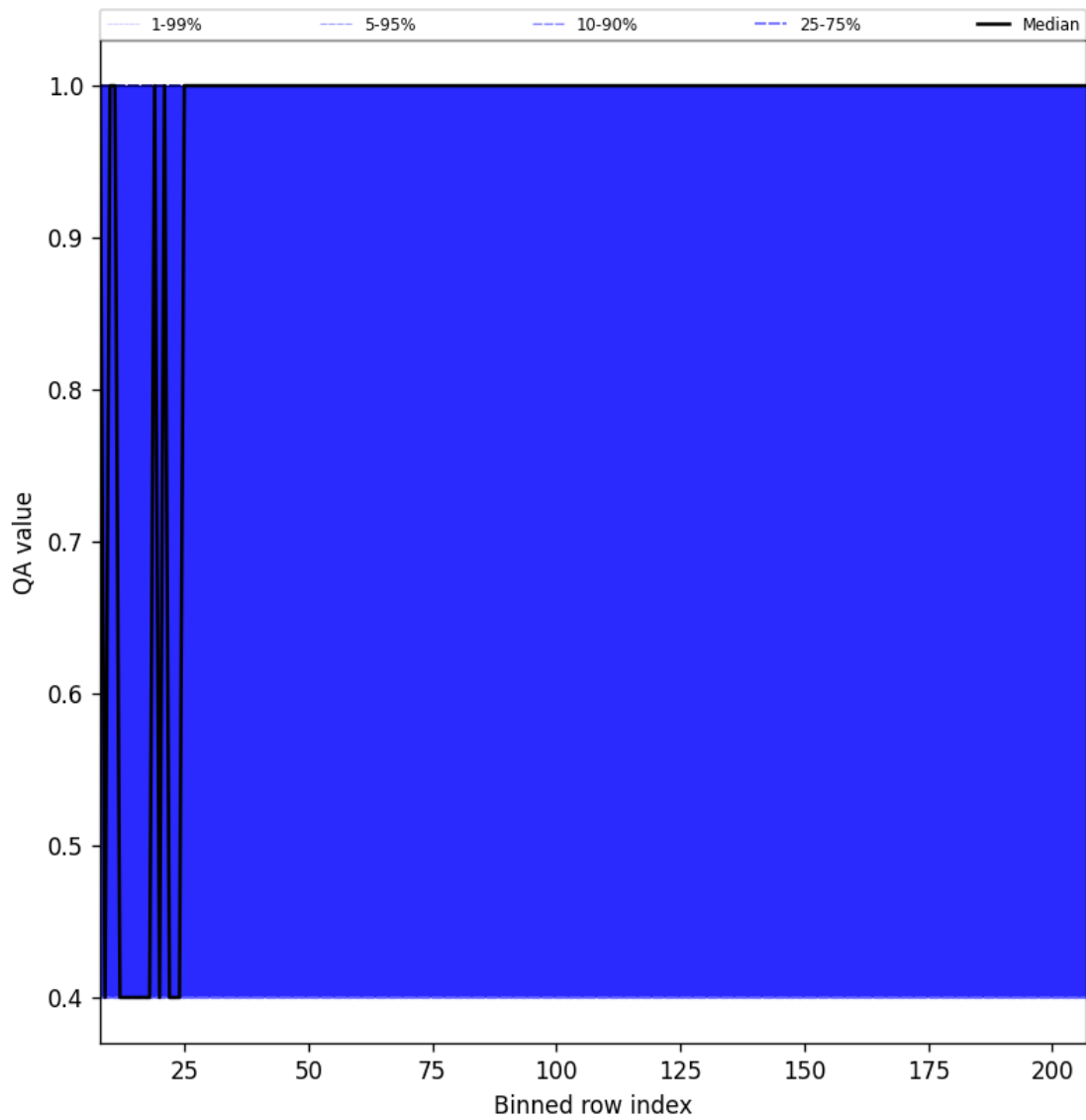
Figure 33: Along track statistics of “QA value” for 2024-12-02 to 2024-12-04
