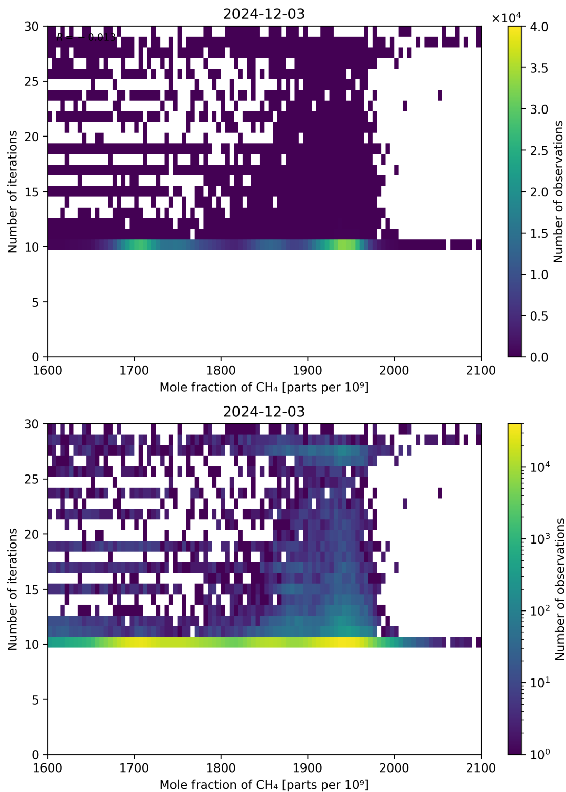
Figure 76: Scatter density plot of “Mole fraction of CH 4 ” against “Number of iterations” for 2024-12-02 to 2024-12-04.
