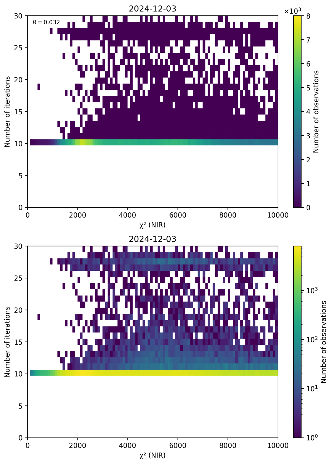
Figure 46: Scatter density plot of “ \chi^2 (NIR)” against “Number of iterations” for 2024-12-02 to 2024-12-04.
