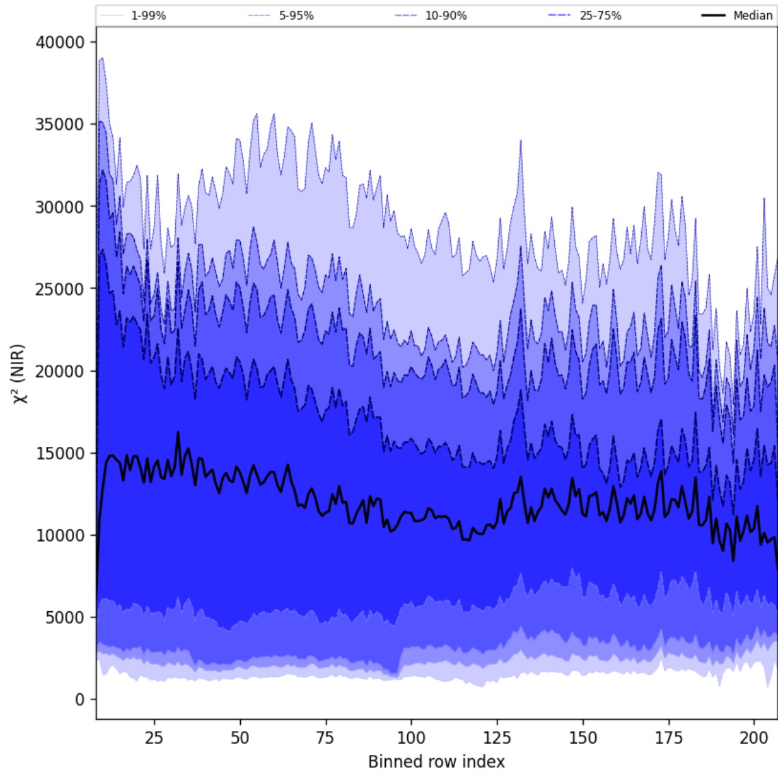
Figure 40: Along track statistics of “ \chi^2 (NIR)” for 2024-12-02 to 2024-12-04
