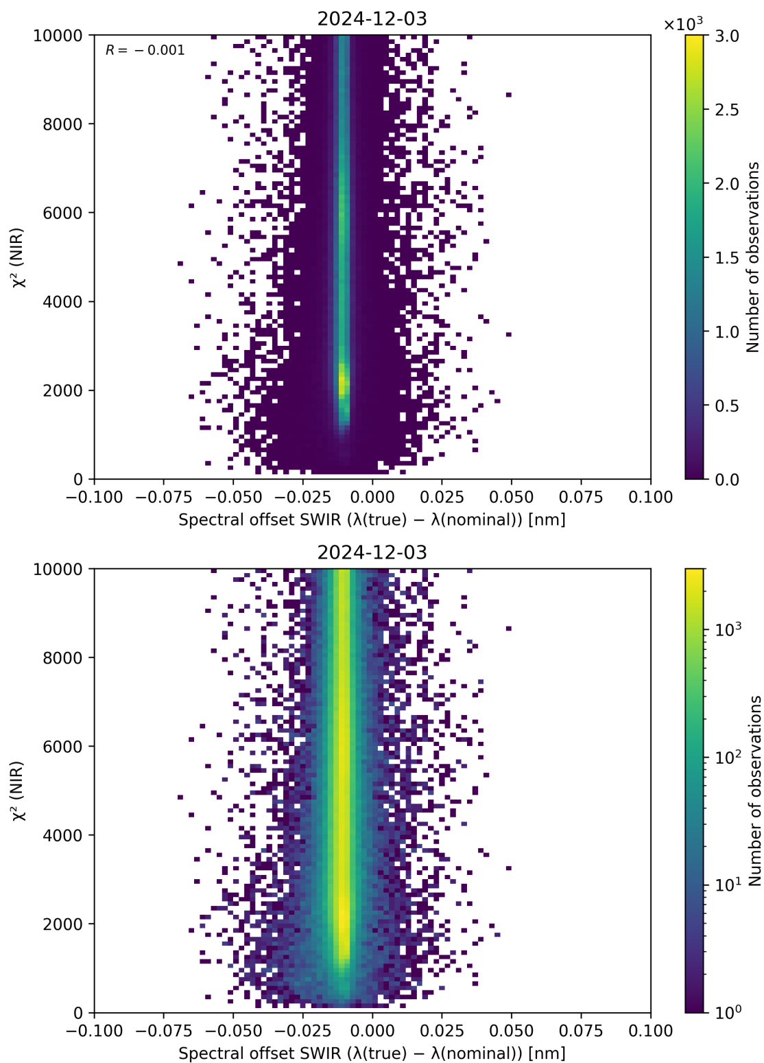
Figure 117: Scatter density plot of “Spectral offset SWIR ( \lambda_{\text{true}} - \lambda_{\text{nominal}} )” against “ \chi^2 (NIR)” for 2024-12-02 to 2024-12-04.
