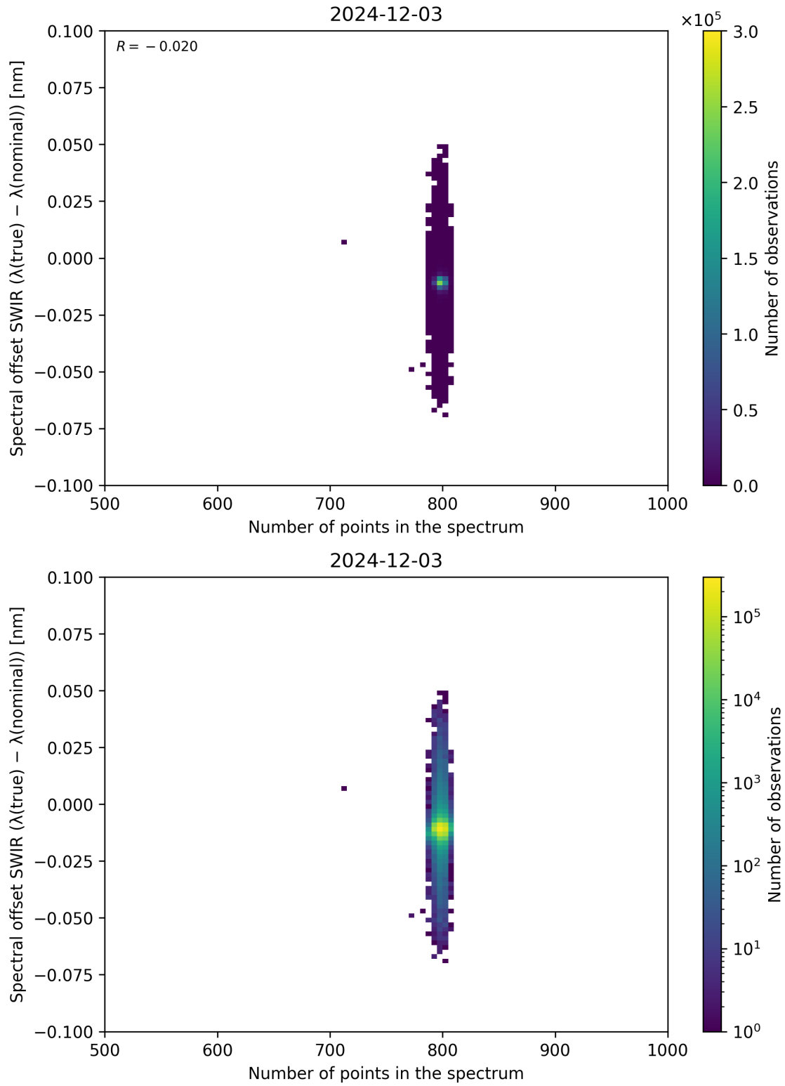
Figure 93: Scatter density plot of “Number of points in the spectrum” against “Spectral offset SWIR ( \lambda_{\text{true}} - \lambda_{\text{nominal}} )” for 2024-12-02 to 2024-12-04.
