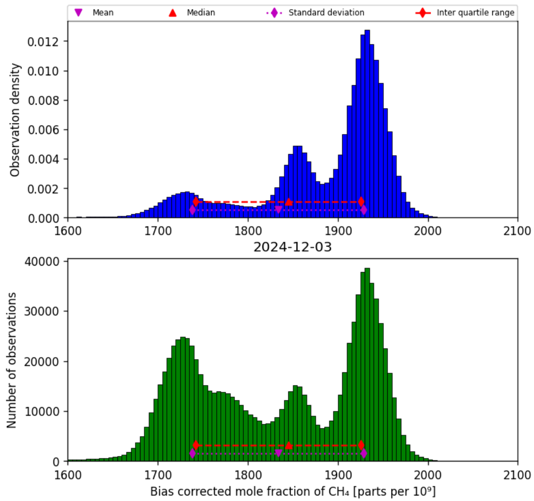
Figure 25: Histogram of “Bias corrected mole fraction of CH 4 ” for 2024-12-02 to 2024-12-04
