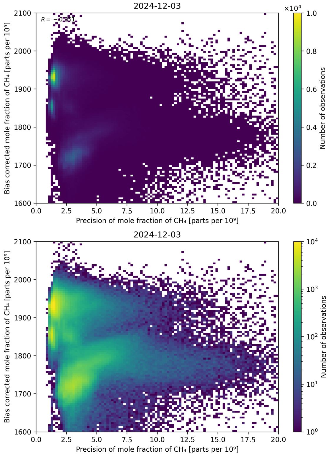
Figure 82: Scatter density plot of “Precision of mole fraction of \text{CH}_4 ” against “Bias corrected mole fraction of \text{CH}_4 ” for 2024-12-02 to 2024-12-04.
