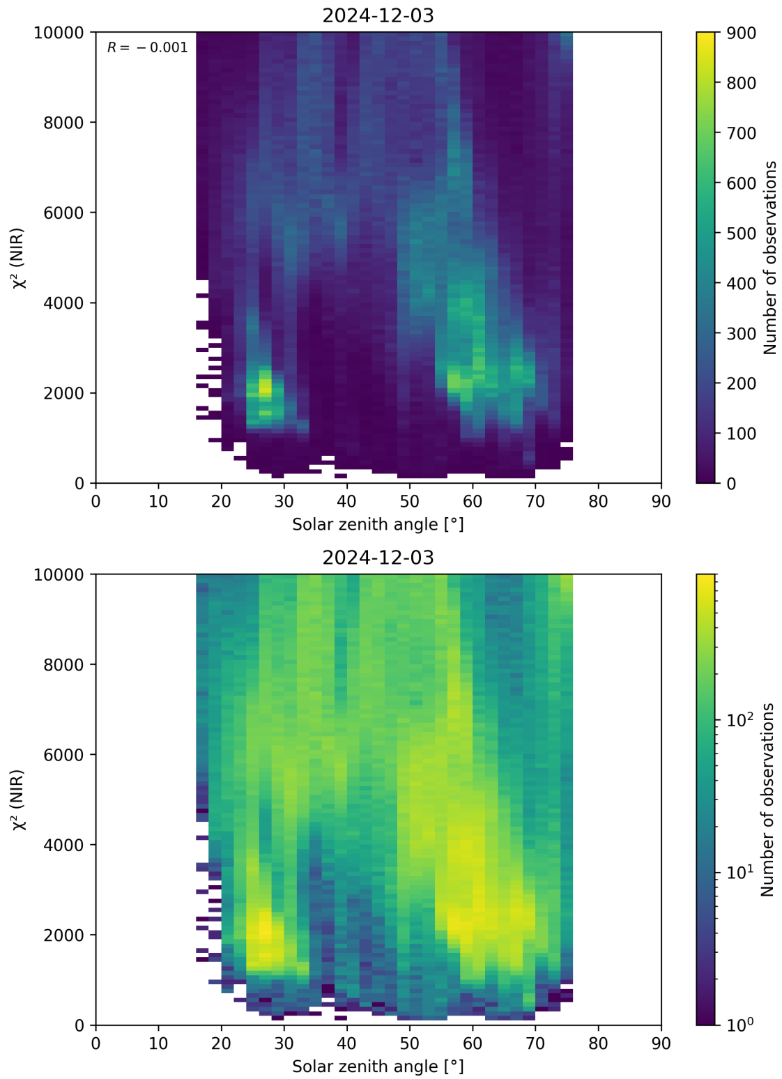
Figure 94: Scatter density plot of “Solar zenith angle” against “ \chi^2 (NIR)” for 2024-12-02 to 2024-12-04.
