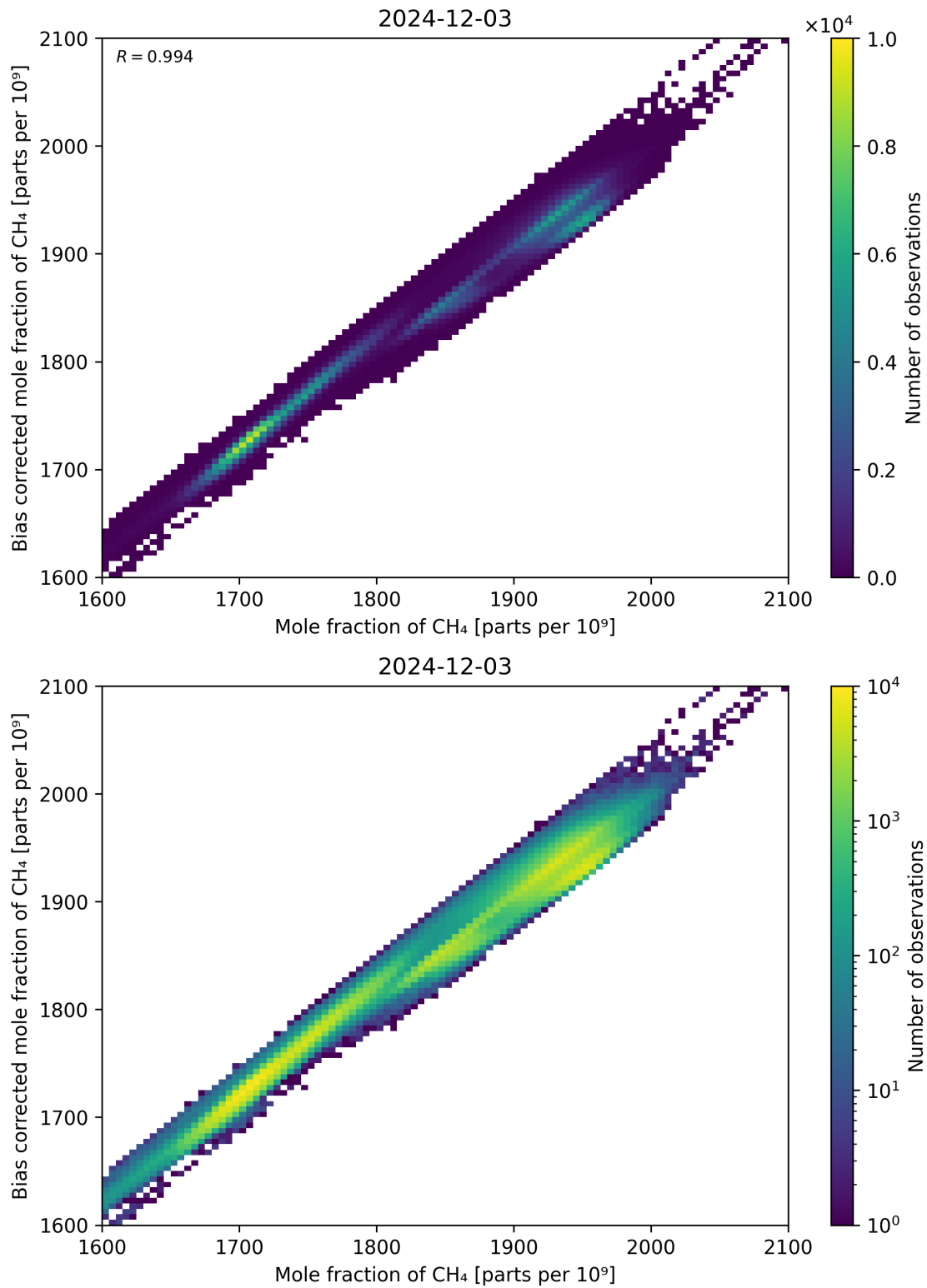
Figure 74: Scatter density plot of “Mole fraction of CH 4 ” against “Bias corrected mole fraction of CH 4 ” for 2024-12-02 to 2024-12-04.
