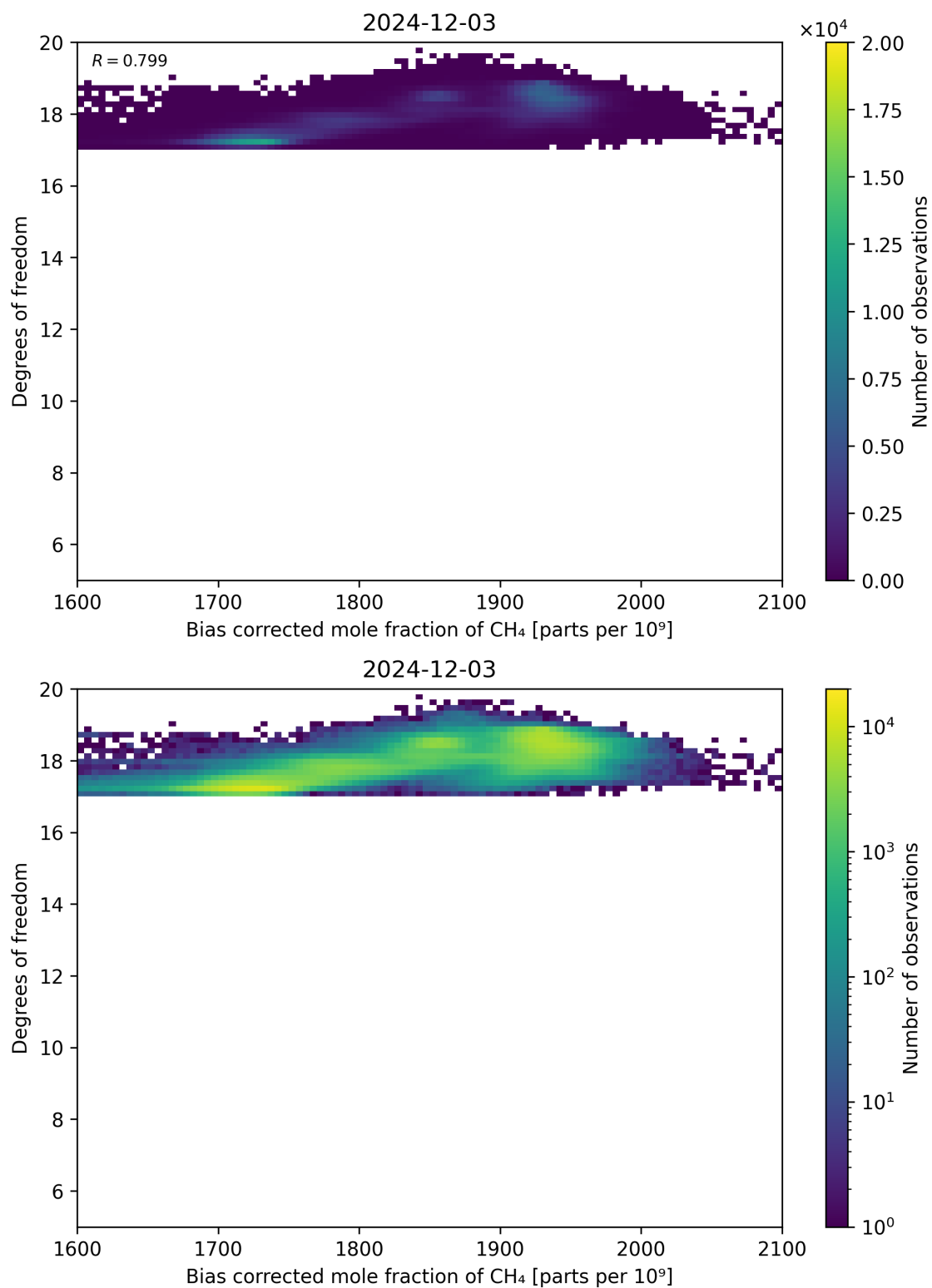
Figure 65: Scatter density plot of “Bias corrected mole fraction of CH 4 ” against “Degrees of freedom” for 2024-12-02 to 2024-12-04.
