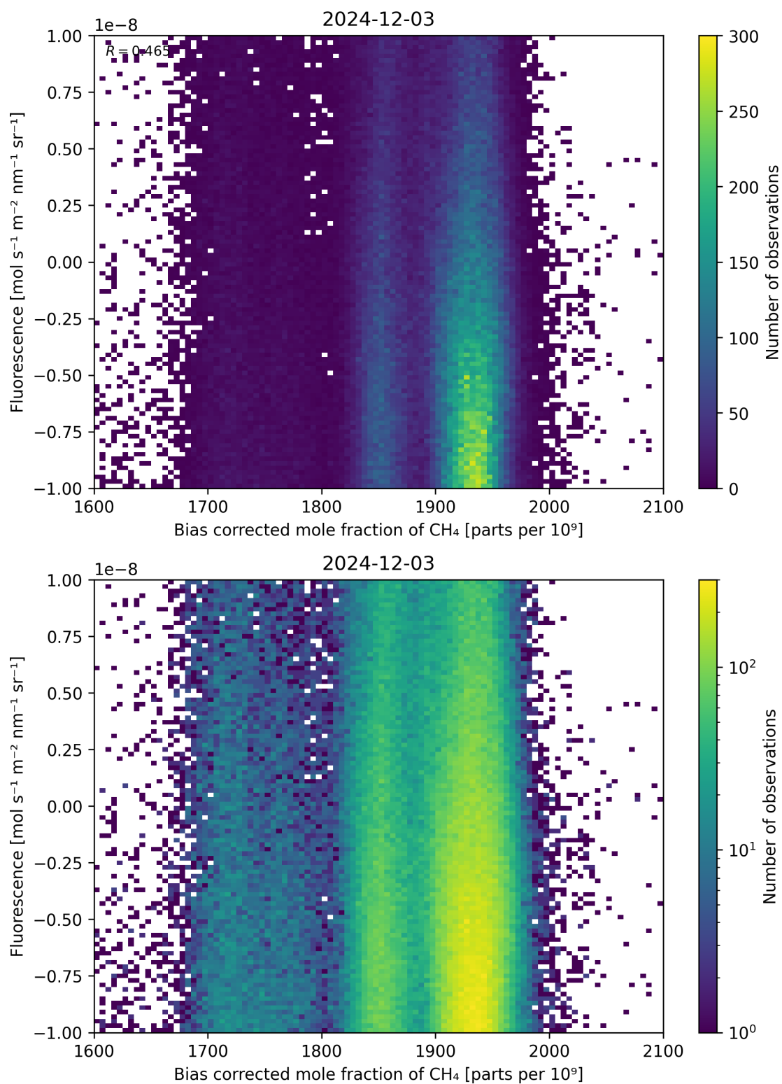
Figure 66: Scatter density plot of “Bias corrected mole fraction of \text{CH}_4 ” against “Fluorescence” for 2024-12-02 to 2024-12-04.
