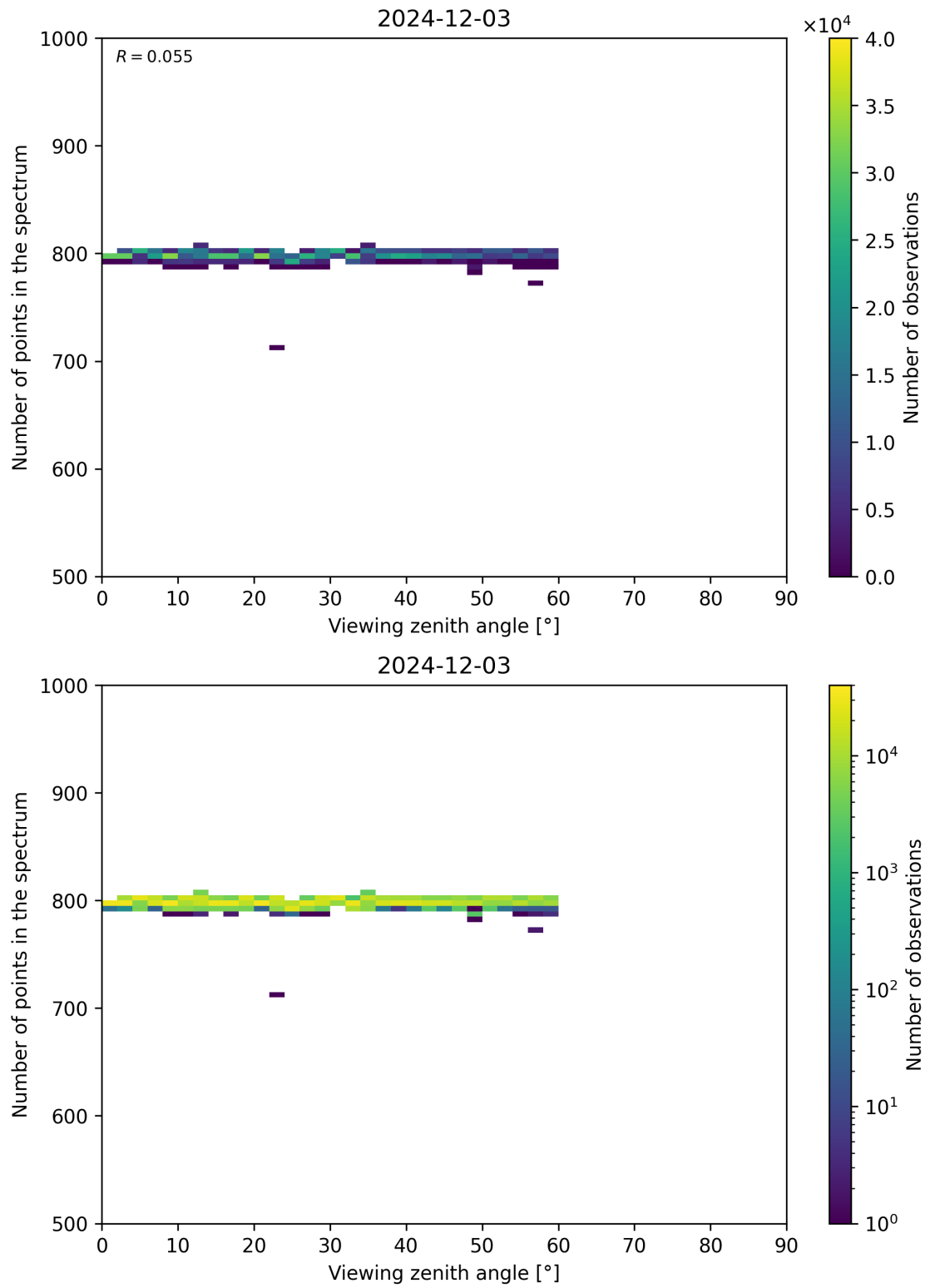
Figure 114: Scatter density plot of “Viewing zenith angle” against “Number of points in the spectrum” for 2024-12-02 to 2024-12-04.
