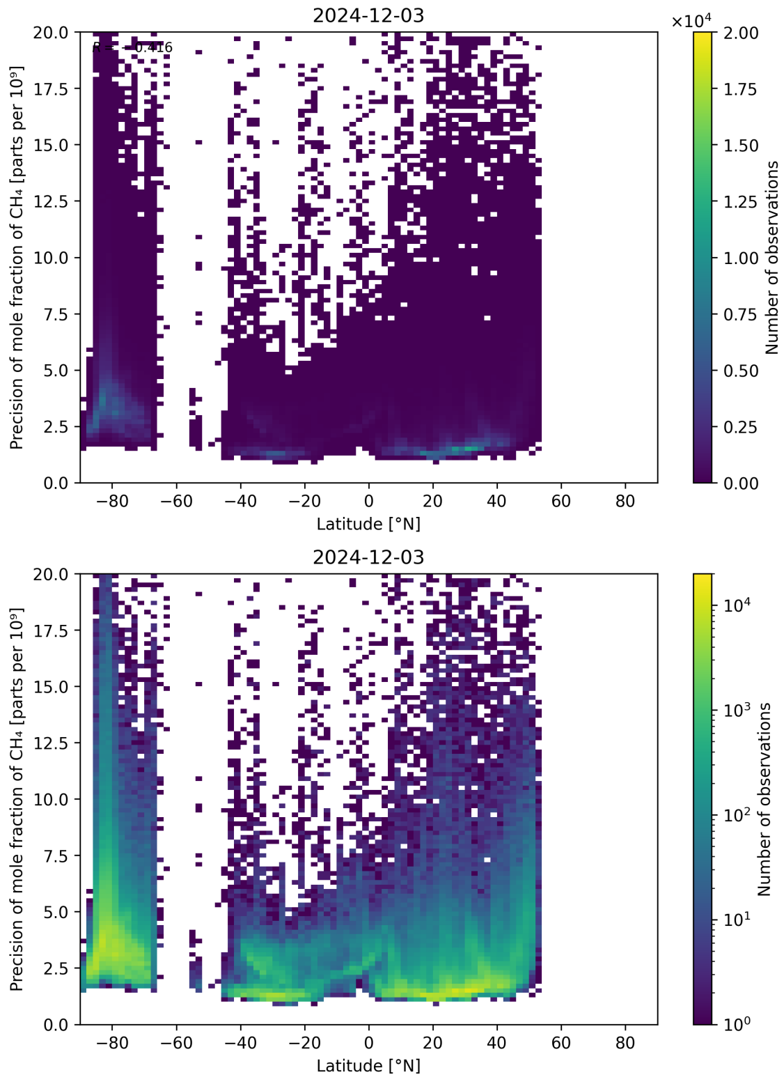
Figure 59: Scatter density plot of “Latitude” against “Precision of mole fraction of CH 4 ” for 2024-12-02 to 2024-12-04.
