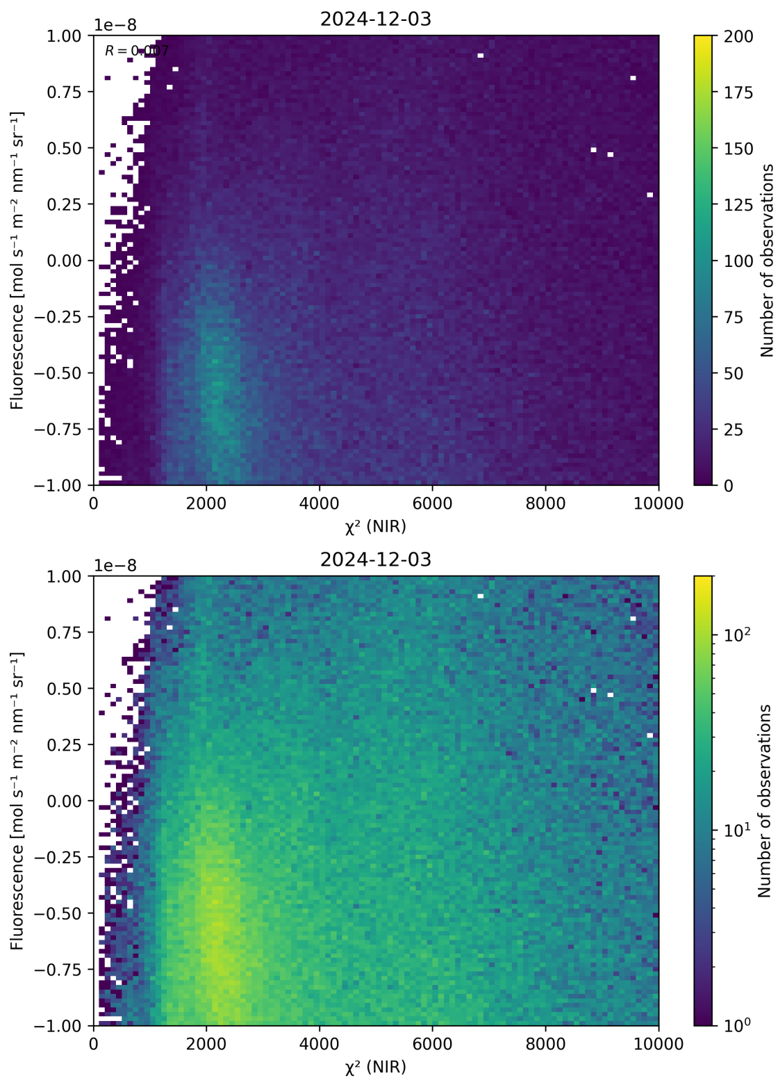
Figure 45: Scatter density plot of “ \chi^2 (NIR)” against “Fluorescence” for 2024-12-02 to 2024-12-04.
