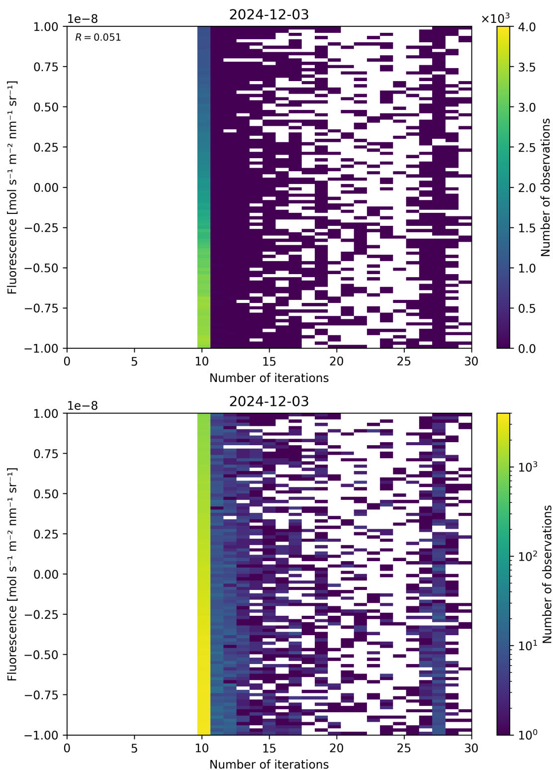
Figure 87: Scatter density plot of “Number of iterations” against “Fluorescence” for 2024-12-02 to 2024-12-04.
