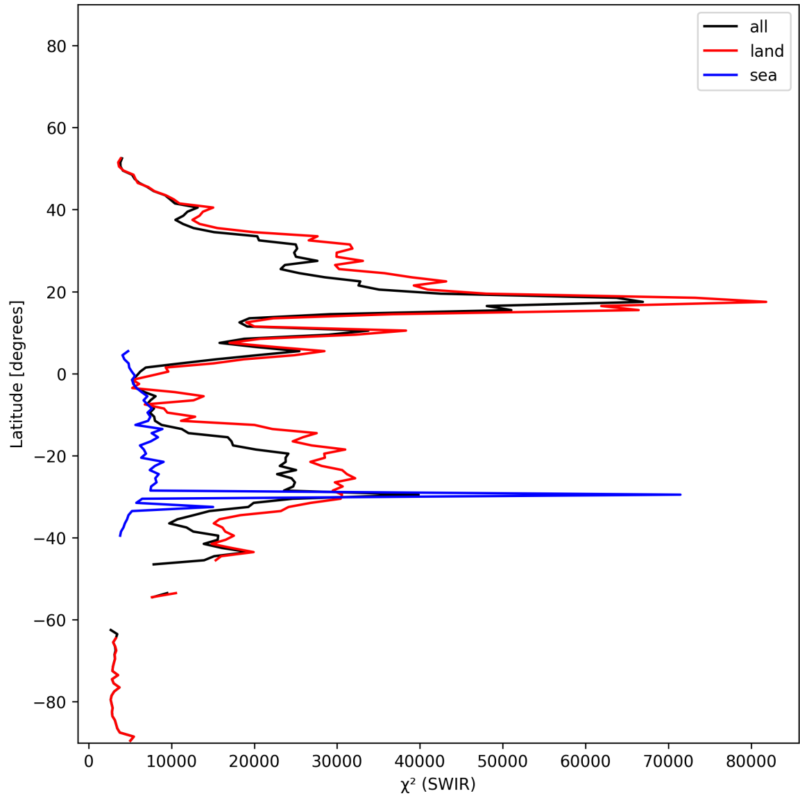
Figure 17: Zonal average of “ \chi^2 (SWIR)” for 2024-12-02 to 2024-12-04.
