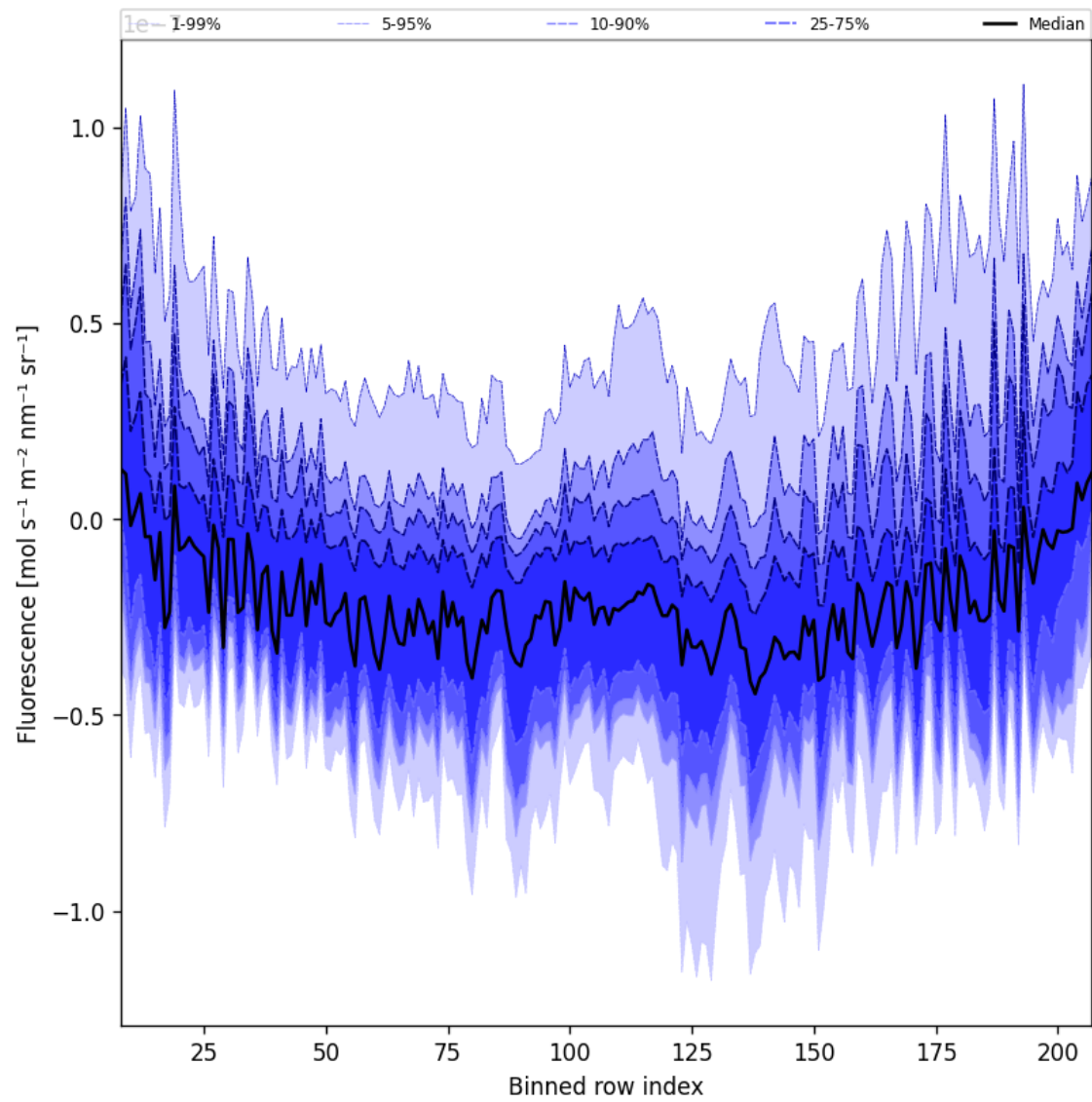
Figure 43: Along track statistics of “Fluorescence” for 2024-12-02 to 2024-12-04
