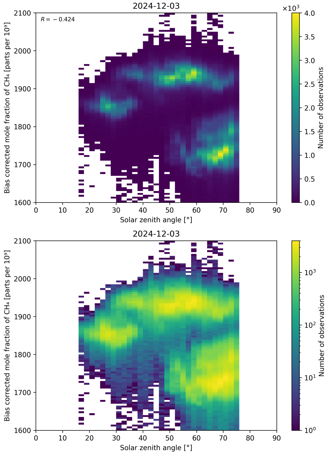
Figure 100: Scatter density plot of “Solar zenith angle” against “Bias corrected mole fraction of CH 4 ” for 2024-12-02 to 2024-12-04.
