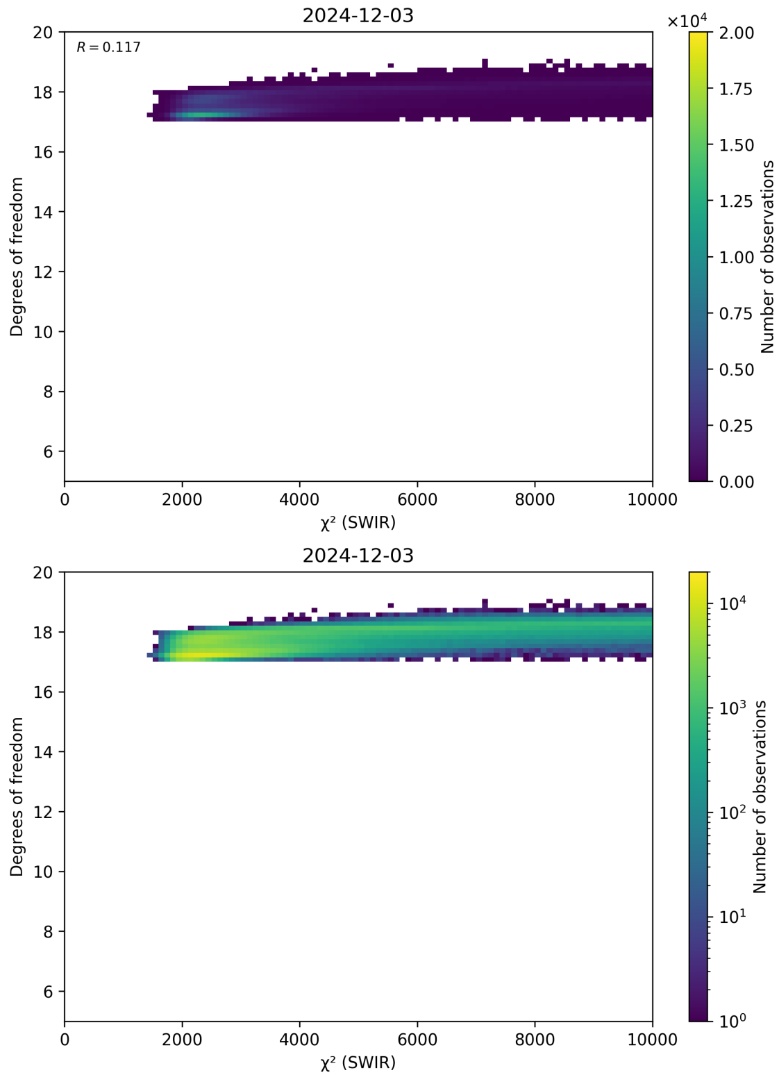
Figure 48: Scatter density plot of “ \chi^2 (SWIR)” against “Degrees of freedom” for 2024-12-02 to 2024-12-04.
