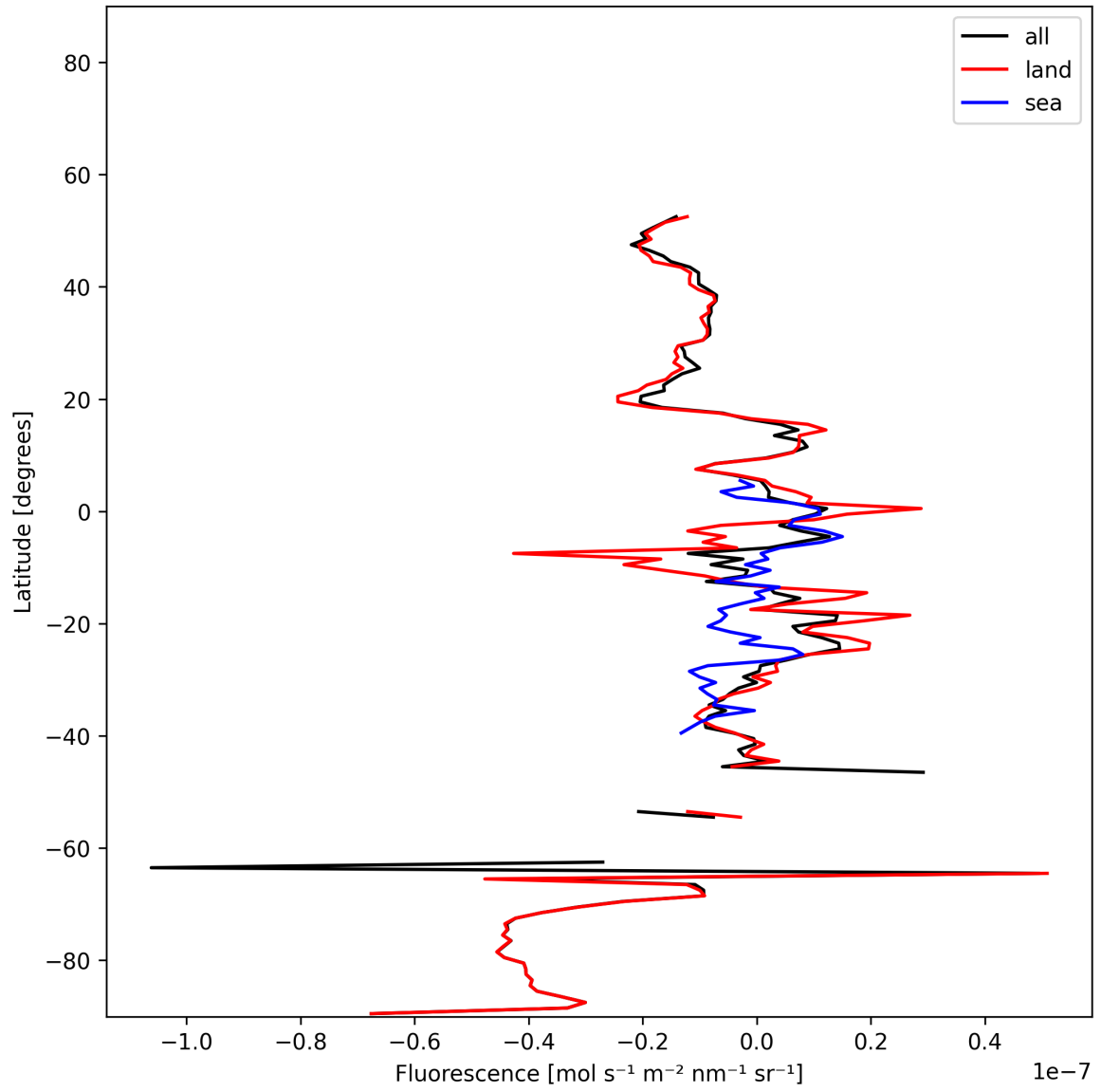
Figure 21: Zonal average of “Fluorescence” for 2024-12-02 to 2024-12-04.
