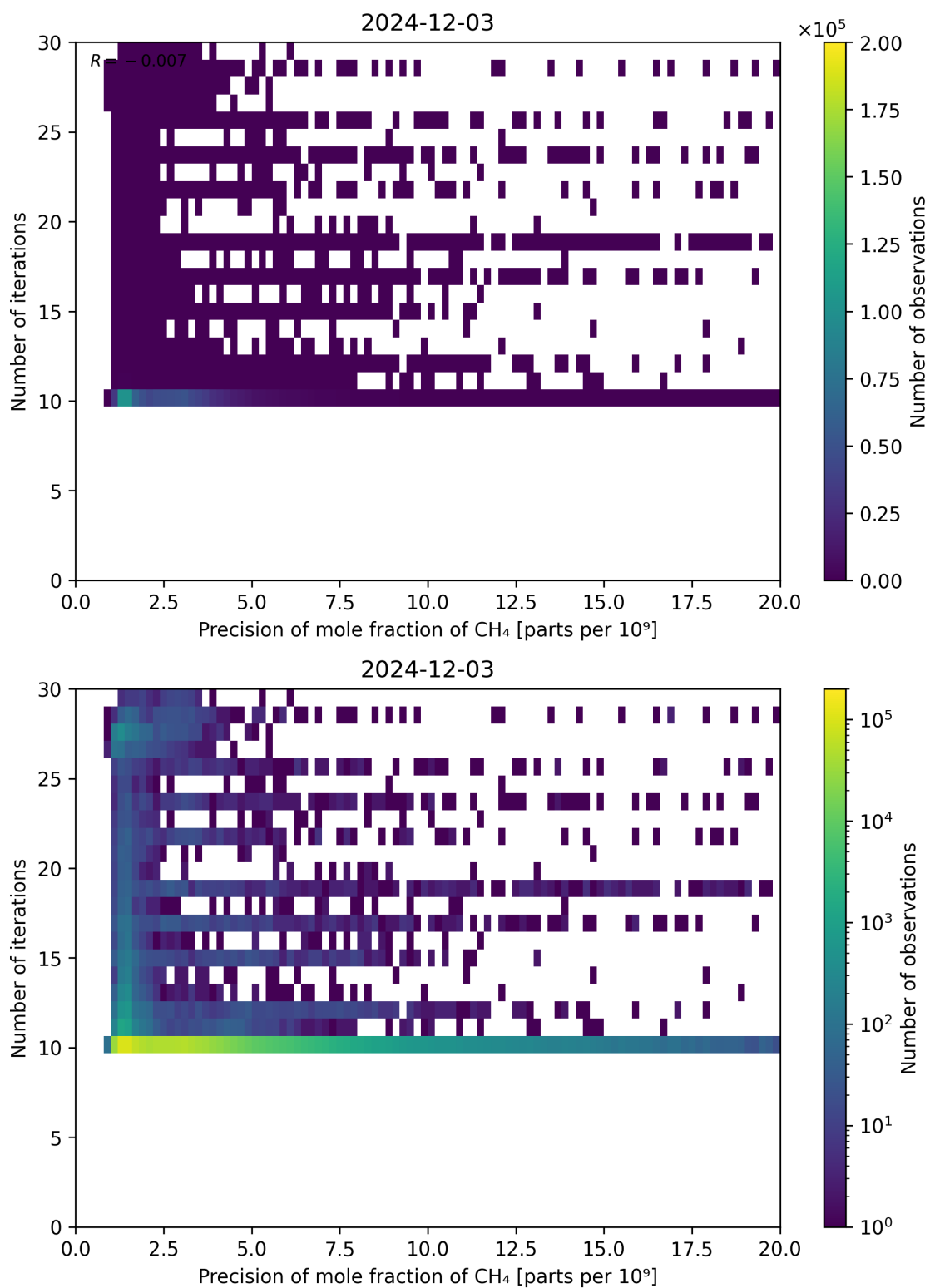
Figure 83: Scatter density plot of “Precision of mole fraction of CH 4 ” against “Number of iterations” for 2024-12-02 to 2024-12-04.
