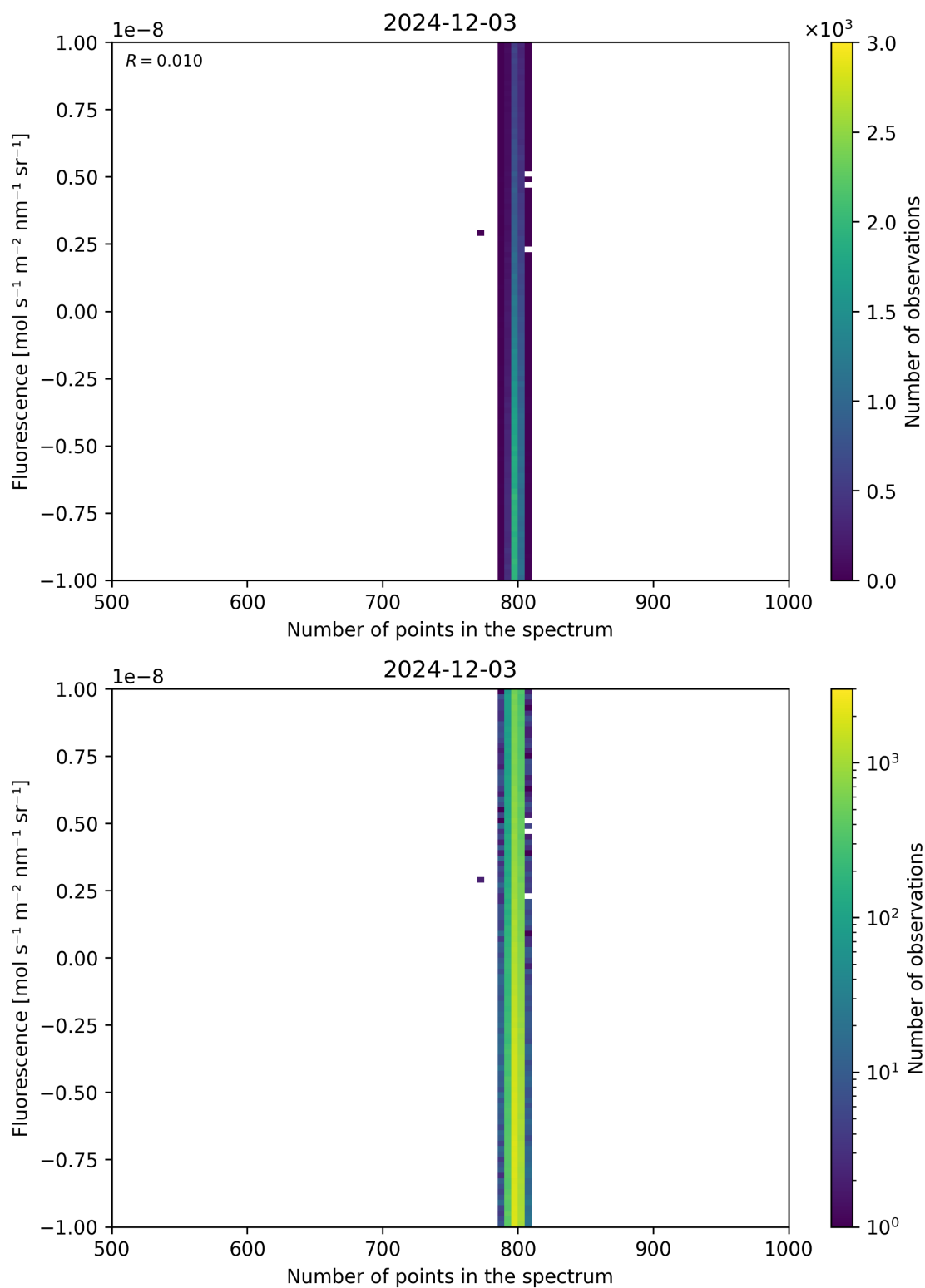
Figure 91: Scatter density plot of “Number of points in the spectrum” against “Fluorescence” for 2024-12-02 to 2024-12-04.
