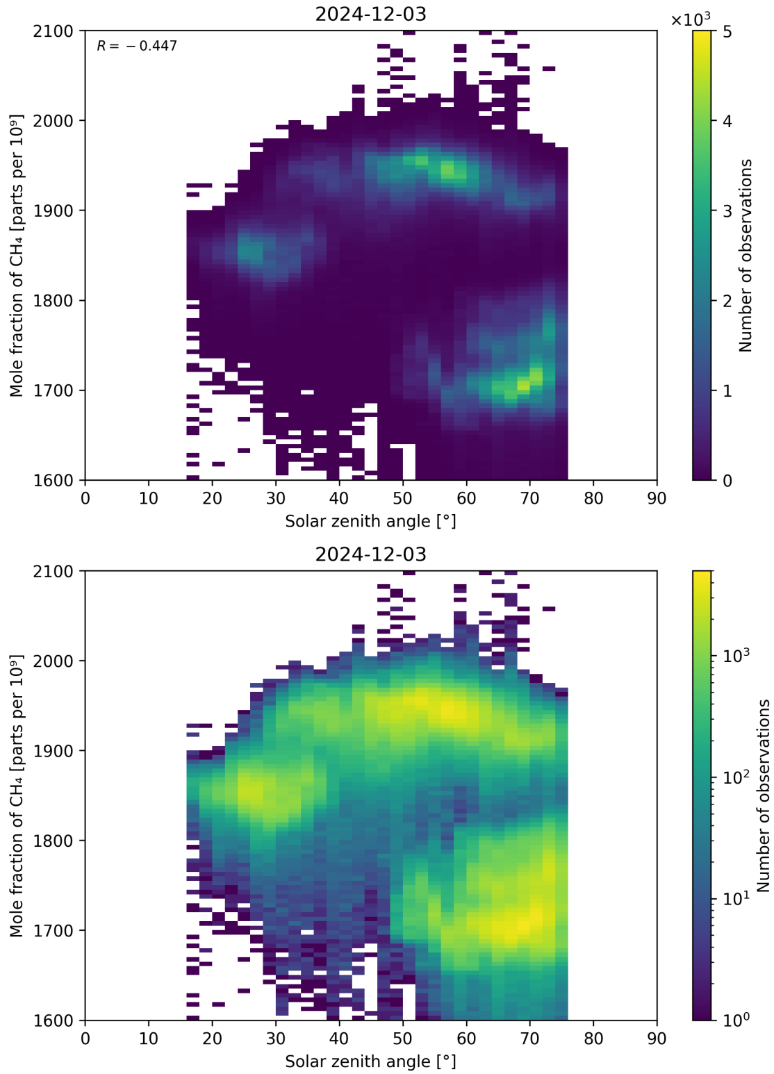
Figure 99: Scatter density plot of “Solar zenith angle” against “Mole fraction of CH 4 ” for 2024-12-02 to 2024-12-04.
