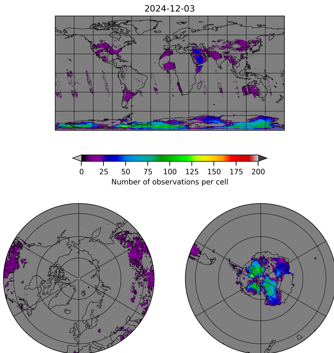
Figure 10: Map of the number of observations for 2024-12-02 to 2024-12-04
