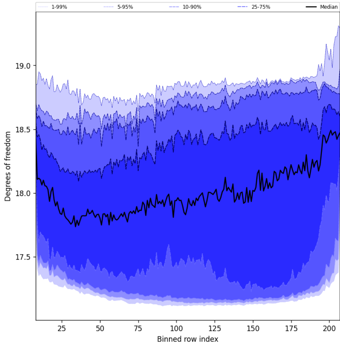
Figure 41: Along track statistics of “Degrees of freedom” for 2024-12-02 to 2024-12-04
