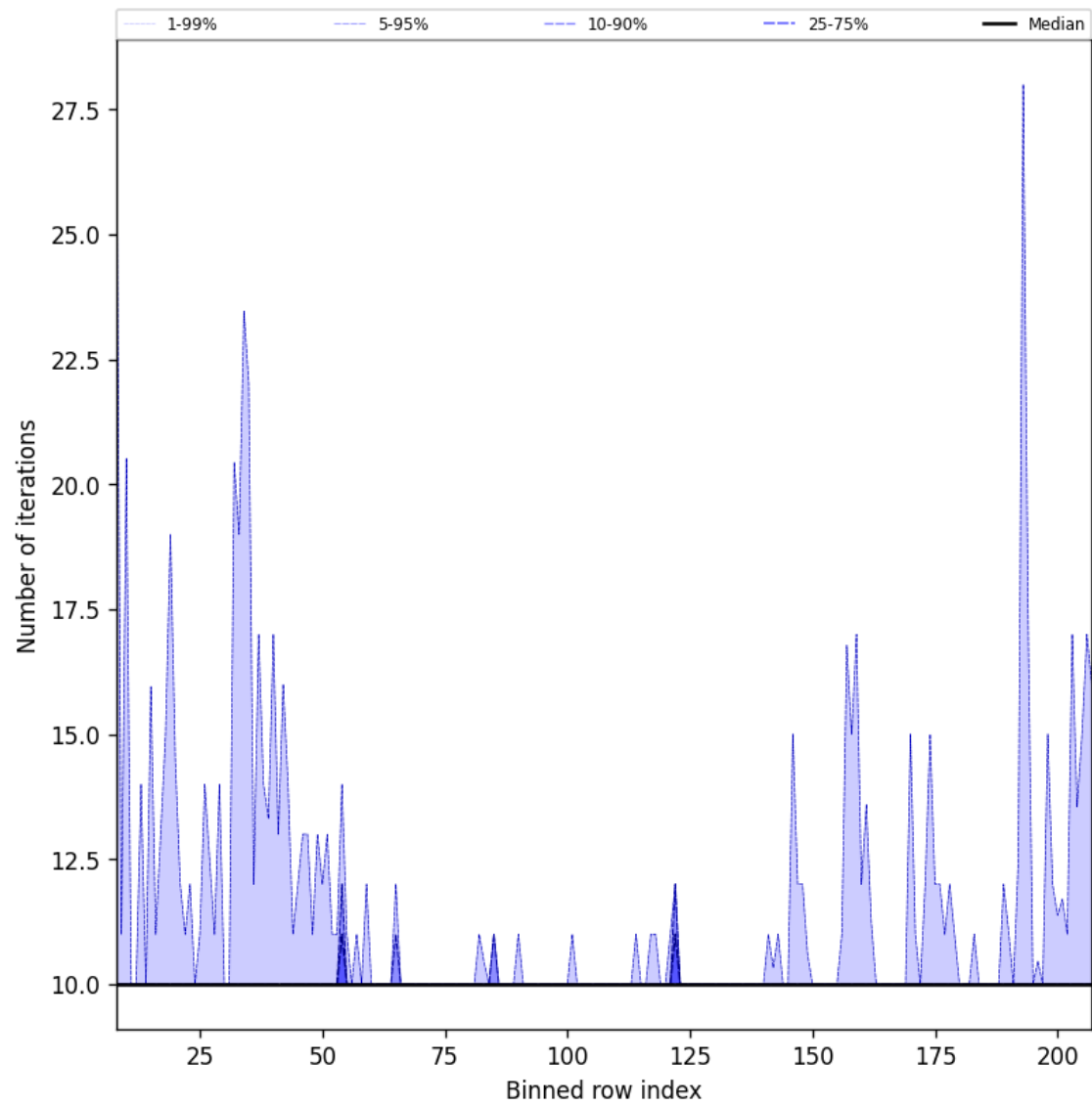
Figure 42: Along track statistics of “Number of iterations” for 2024-12-02 to 2024-12-04
