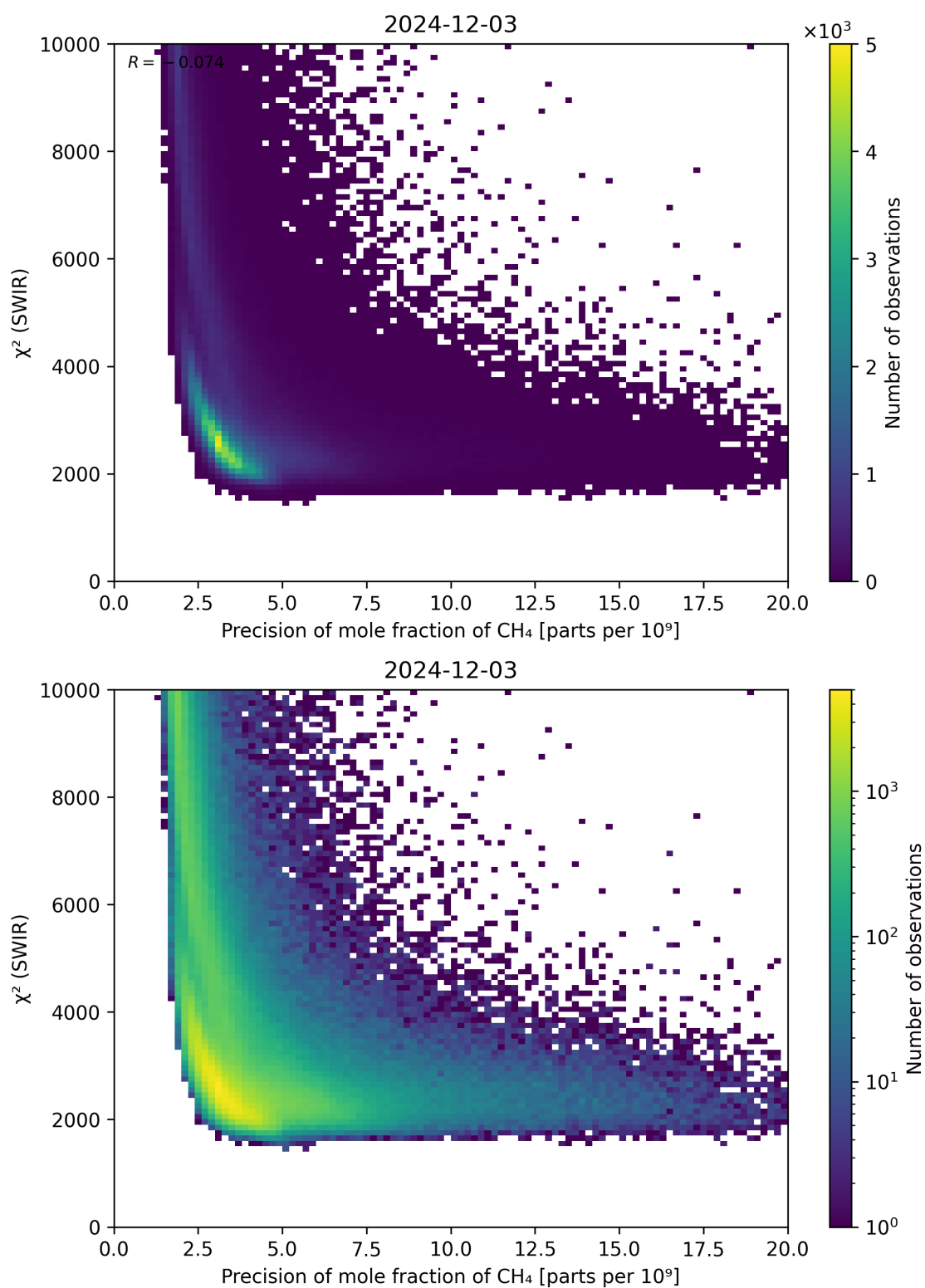
Figure 79: Scatter density plot of “Precision of mole fraction of \text{CH}_4 ” against “ \chi^2 (SWIR)” for 2024-12-02 to 2024-12-04.
