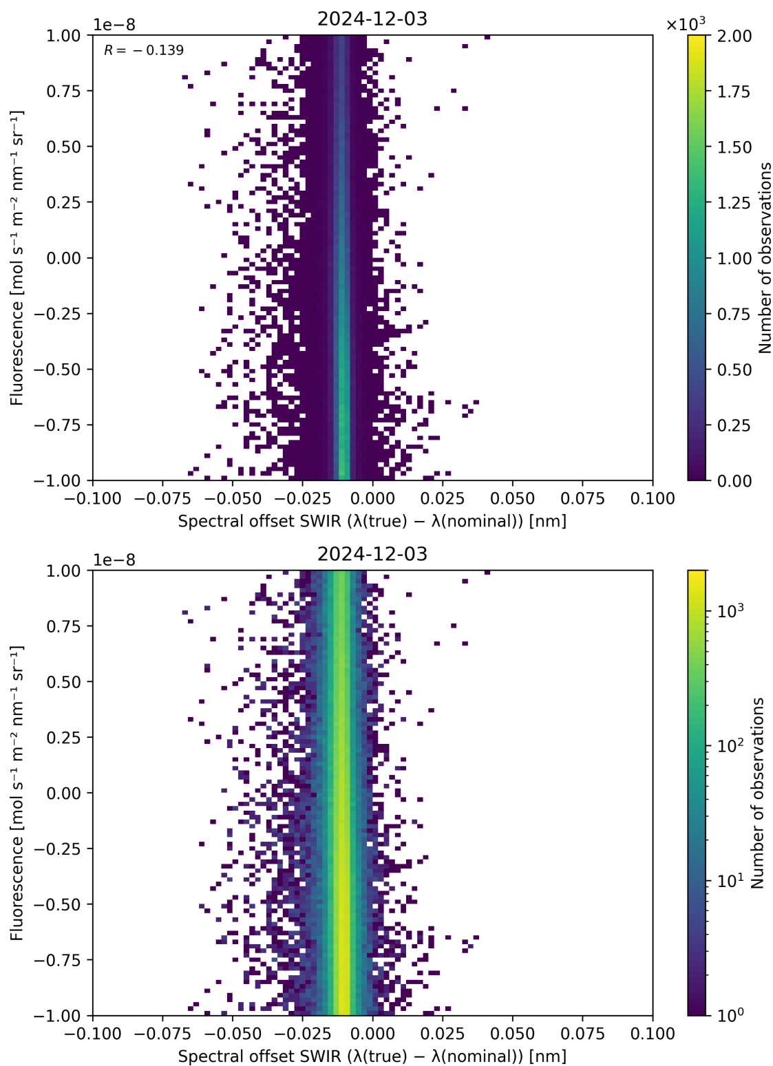
Figure 120: Scatter density plot of “Spectral offset SWIR ( \lambda_{\text{true}} - \lambda_{\text{nominal}} )” against “Fluorescence” for 2024-12-02 to 2024-12-04.
