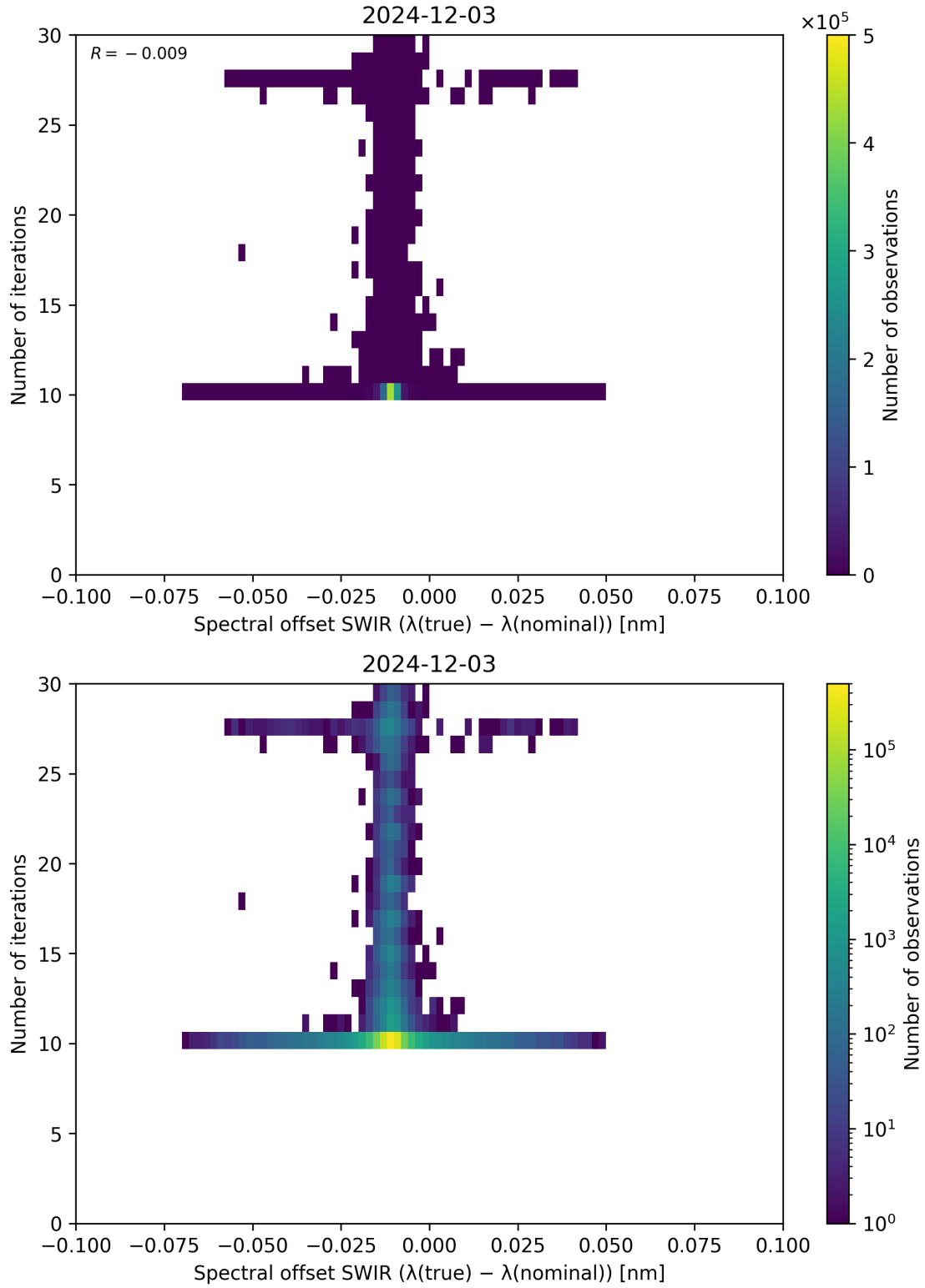
Figure 121: Scatter density plot of “Spectral offset SWIR ( \lambda_{\text{true}} - \lambda_{\text{nominal}} )” against “Number of iterations” for 2024-12-02 to 2024-12-04.
