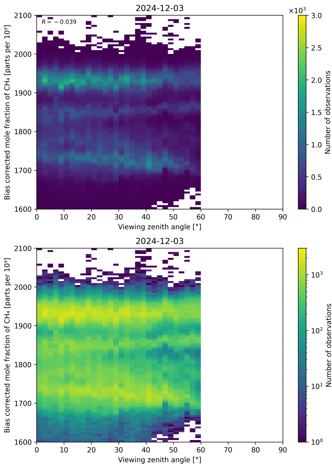
Figure 111: Scatter density plot of “Viewing zenith angle” against “Bias corrected mole fraction of CH 4 ” for 2024-12-02 to 2024-12-04.
