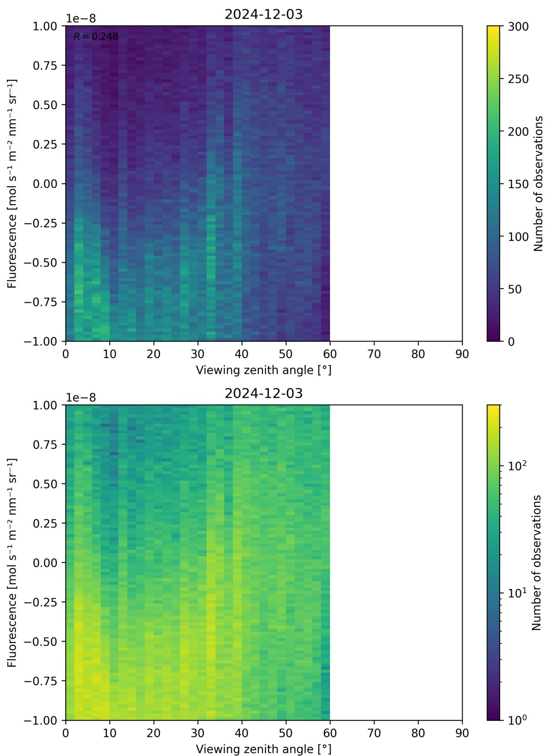
Figure 108: Scatter density plot of “Viewing zenith angle” against “Fluorescence” for 2024-12-02 to 2024-12-04.
