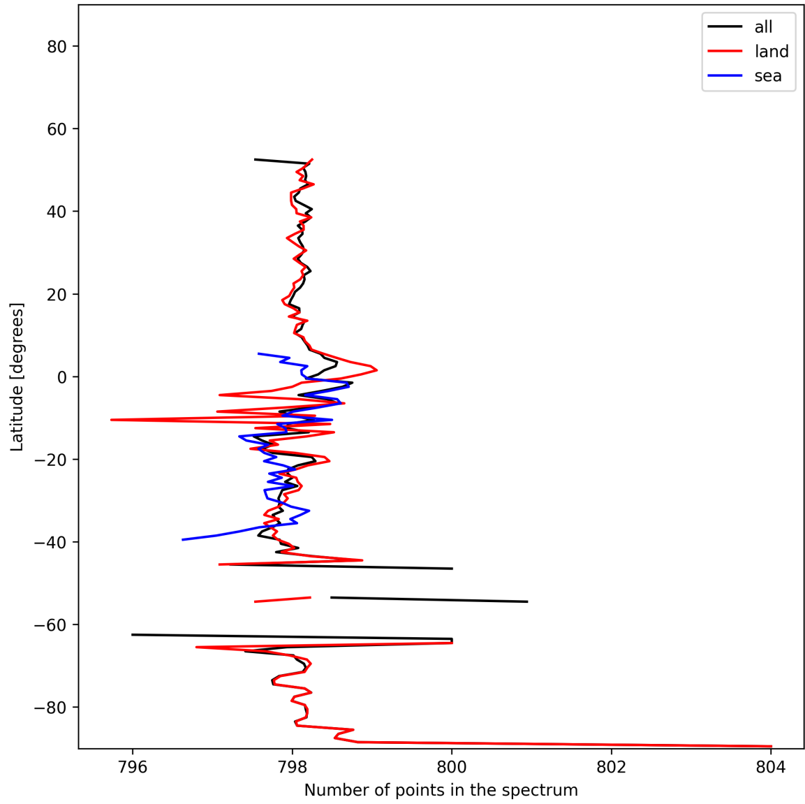
Figure 15: Zonal average of “Number of points in the spectrum” for 2024-12-02 to 2024-12-04.
