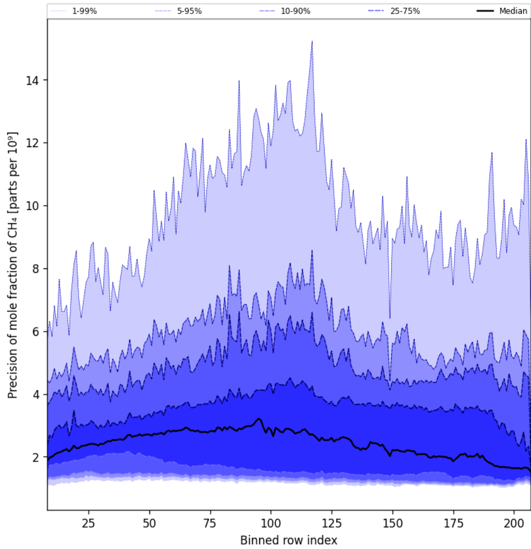
Figure 35: Along track statistics of “Precision of mole fraction of CH 4 ” for 2024-12-02 to 2024-12-04
