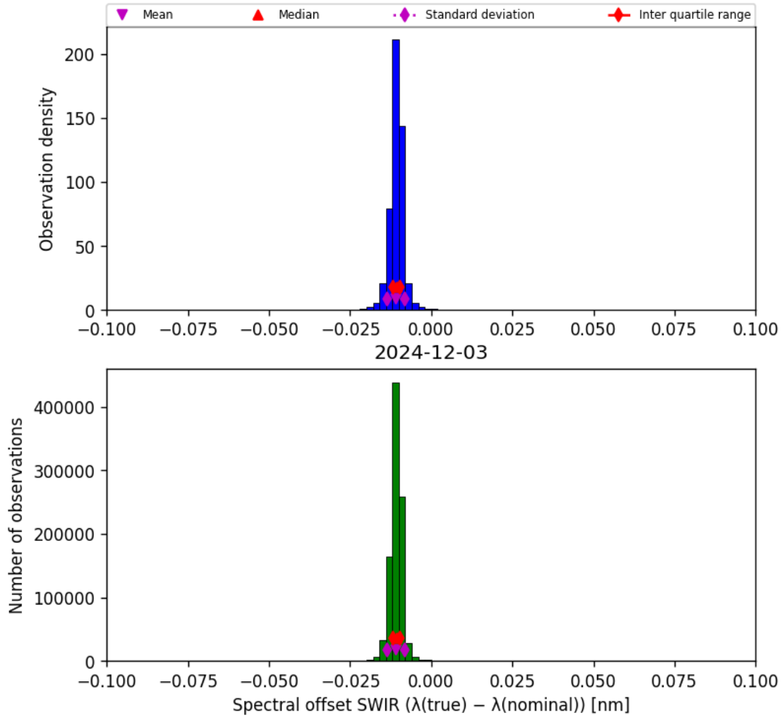
Figure 27: Histogram of “Spectral offset SWIR ( \lambda_{\text{true}} - \lambda_{\text{nominal}} )” for 2024-12-02 to 2024-12-04
