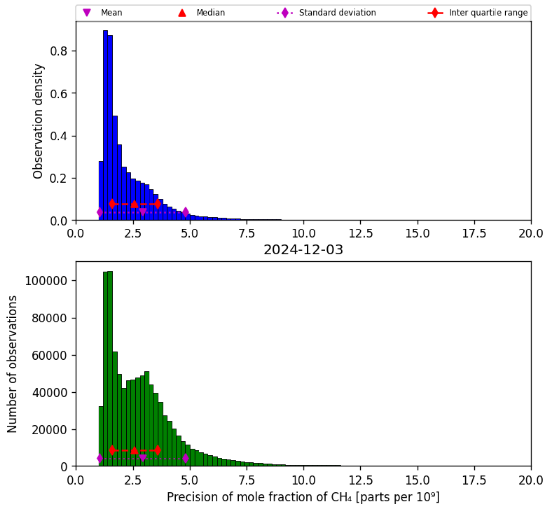
Figure 24: Histogram of “Precision of mole fraction of CH 4 ” for 2024-12-02 to 2024-12-04
