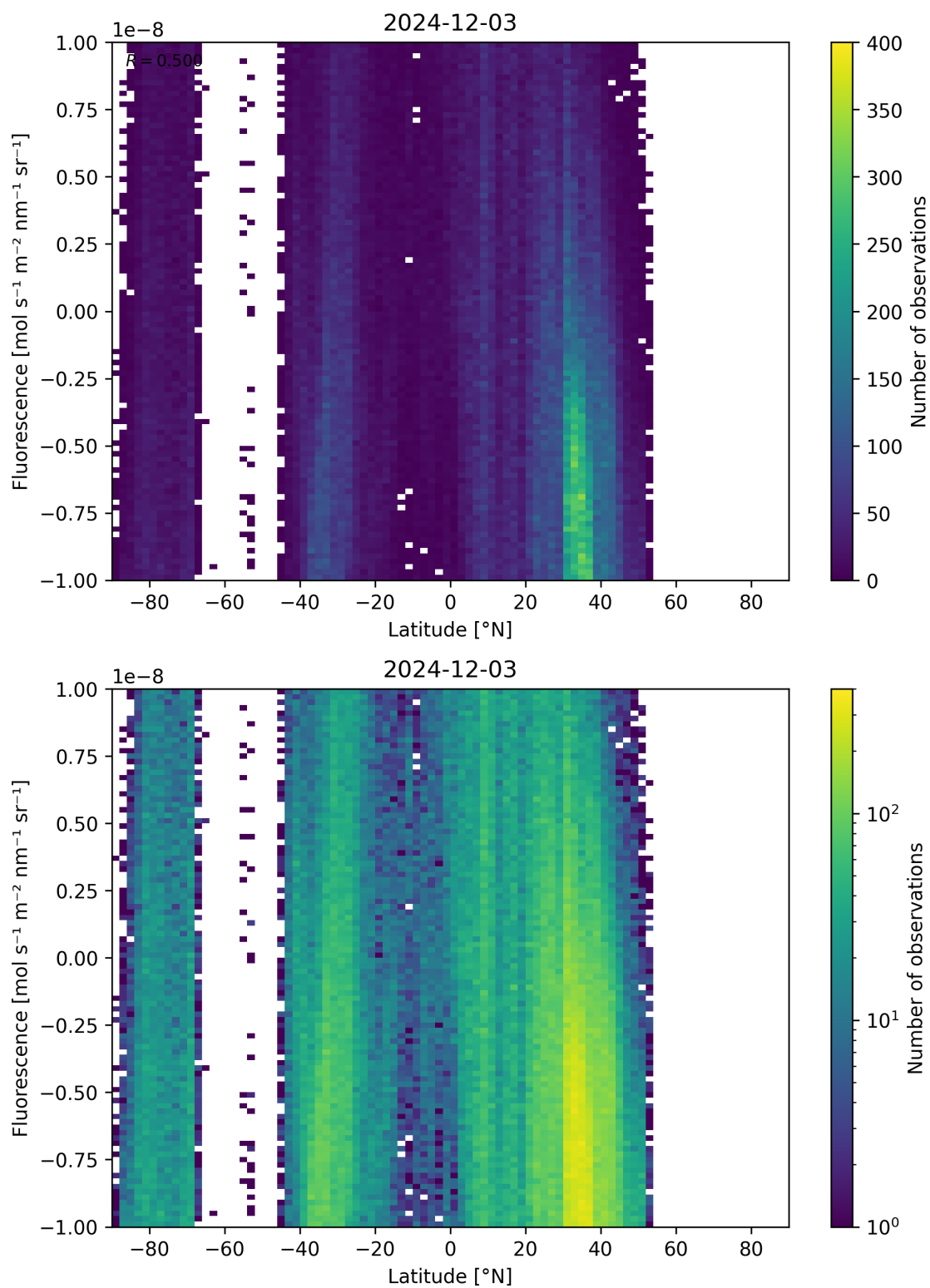
Figure 56: Scatter density plot of “Latitude” against “Fluorescence” for 2024-12-02 to 2024-12-04.
