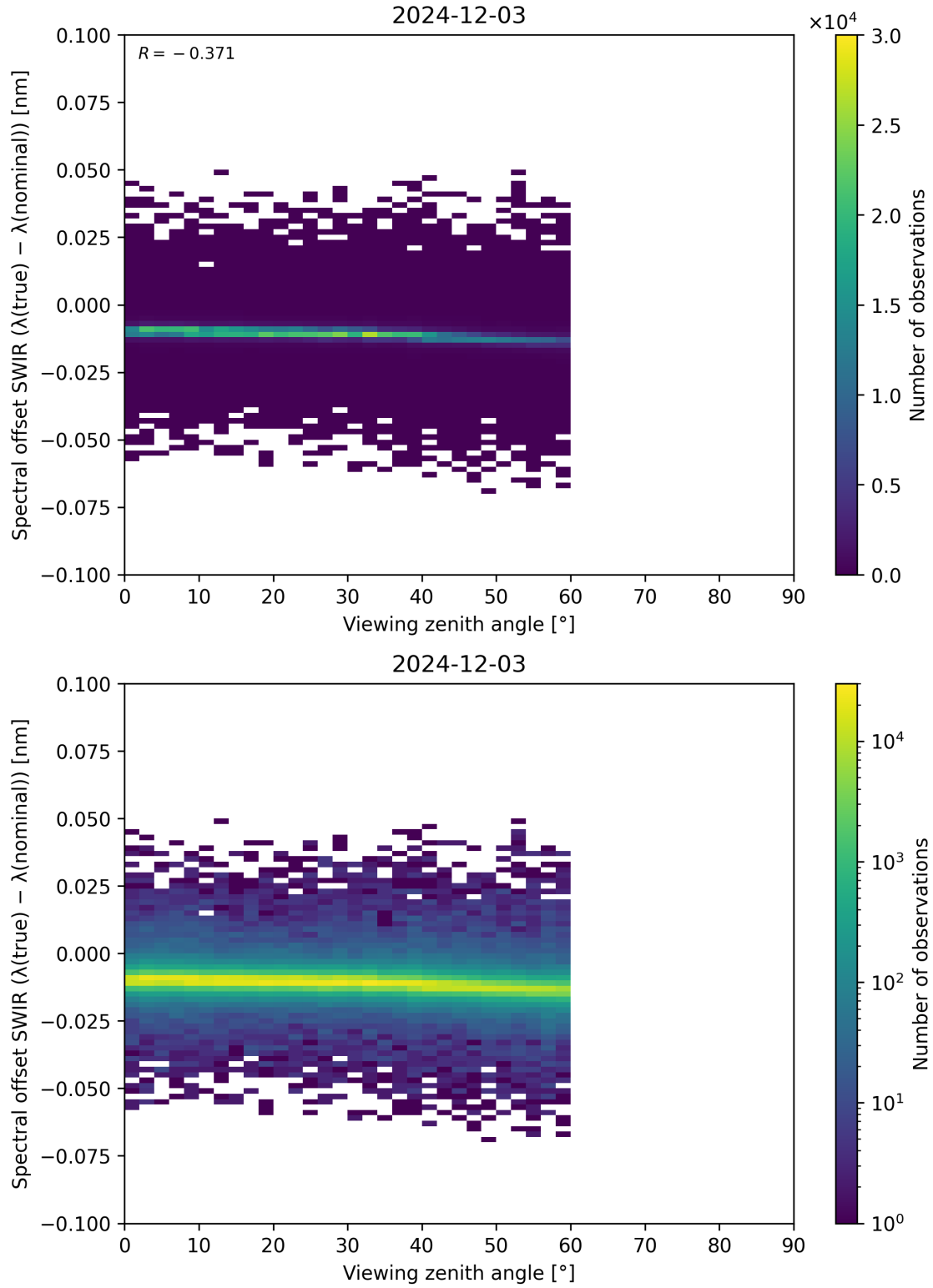
Figure 116: Scatter density plot of “Viewing zenith angle” against “Spectral offset SWIR ( \lambda_{\text{true}} - \lambda_{\text{nominal}} )” for 2024-12-02 to 2024-12-04.
