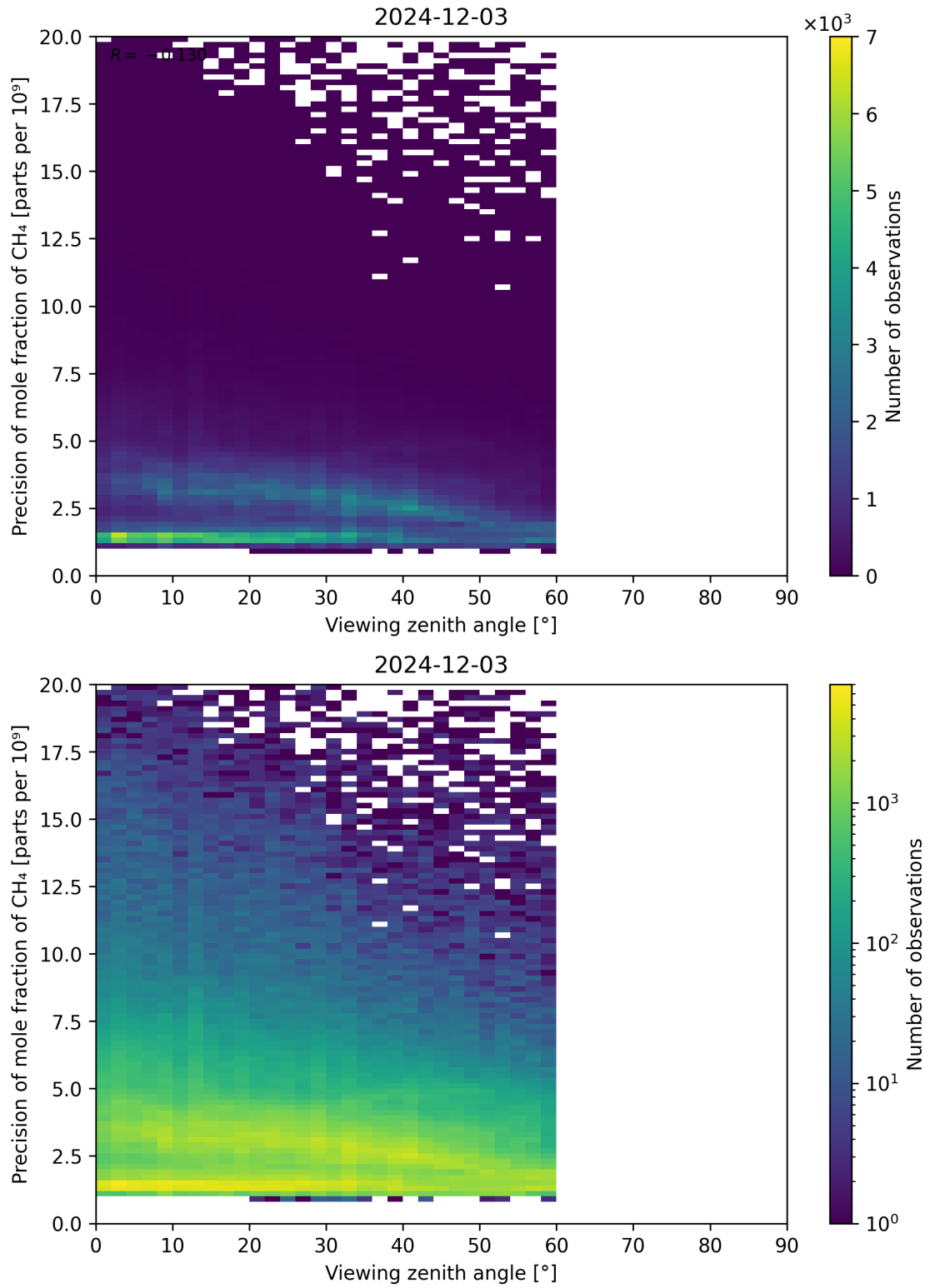
Figure 112: Scatter density plot of “Viewing zenith angle” against “Precision of mole fraction of CH 4 ” for 2024-12-02 to 2024-12-04.
