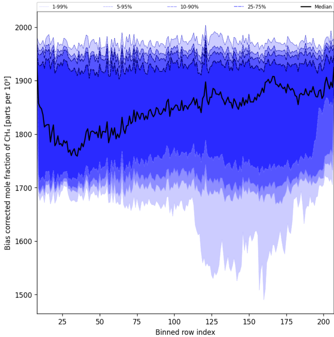
Figure 36: Along track statistics of “Bias corrected mole fraction of CH 4 ” for 2024-12-02 to 2024-12-04
