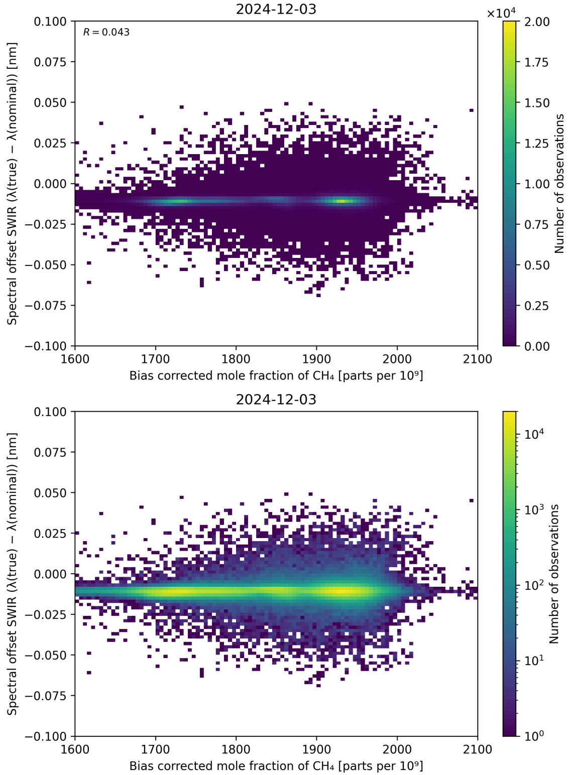
Figure 69: Scatter density plot of “Bias corrected mole fraction of \text{CH}_4 ” against “Spectral offset SWIR ( \lambda_{\text{true}} - \lambda_{\text{nominal}} )” for 2024-12-02 to 2024-12-04.
