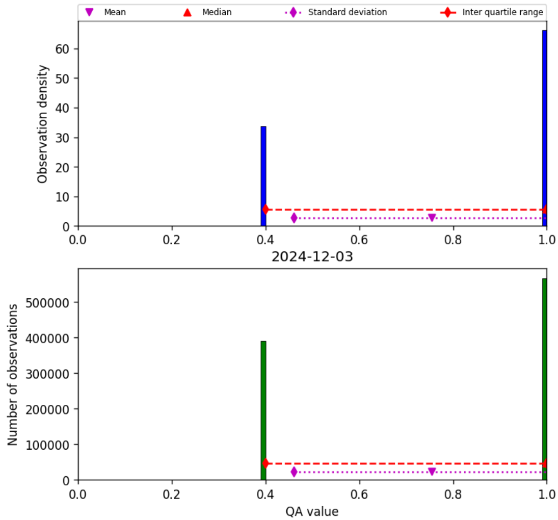
Figure 22: Histogram of “QA value” for 2024-12-02 to 2024-12-04
