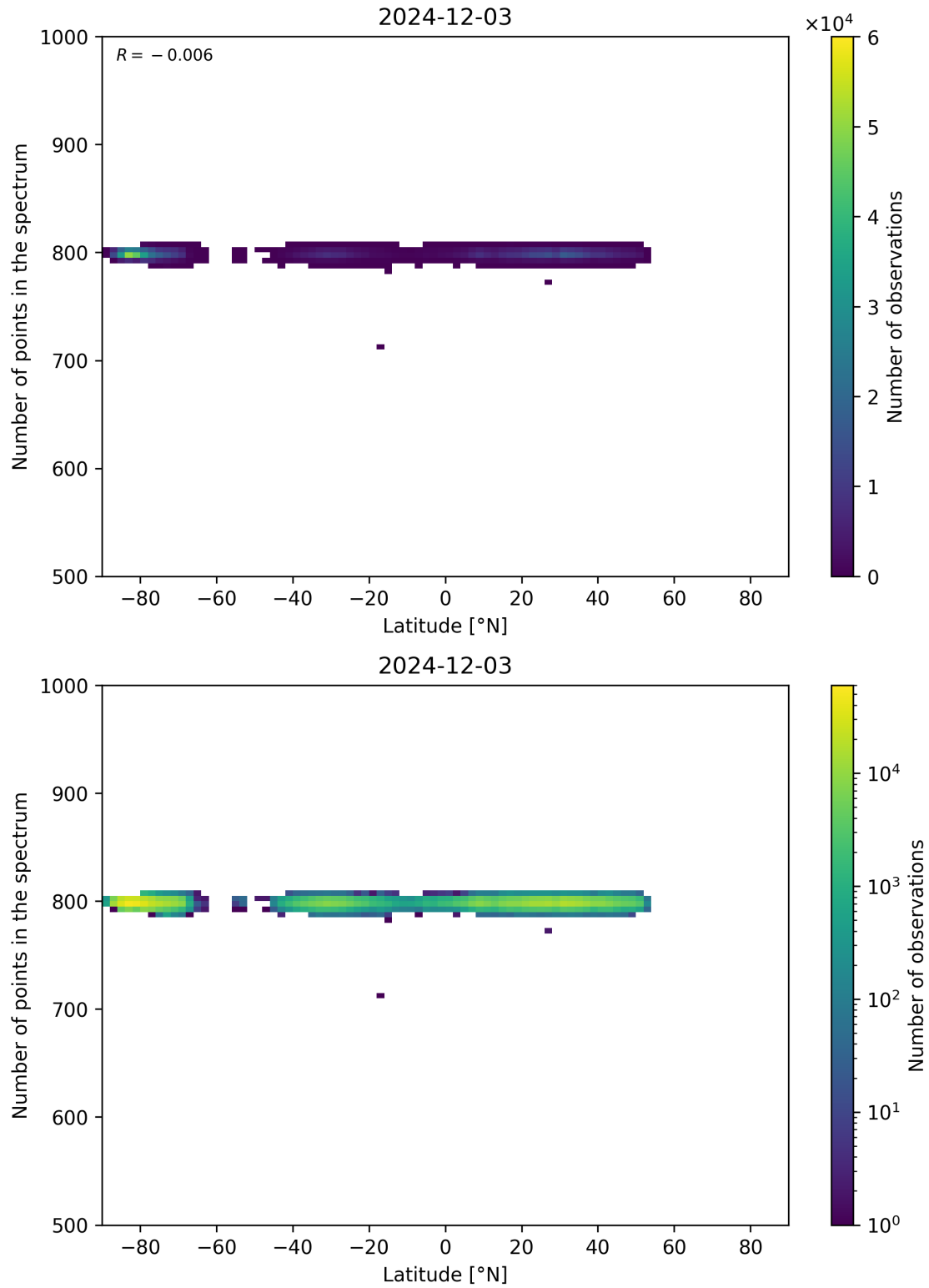
Figure 61: Scatter density plot of “Latitude” against “Number of points in the spectrum” for 2024-12-02 to 2024-12-04.
