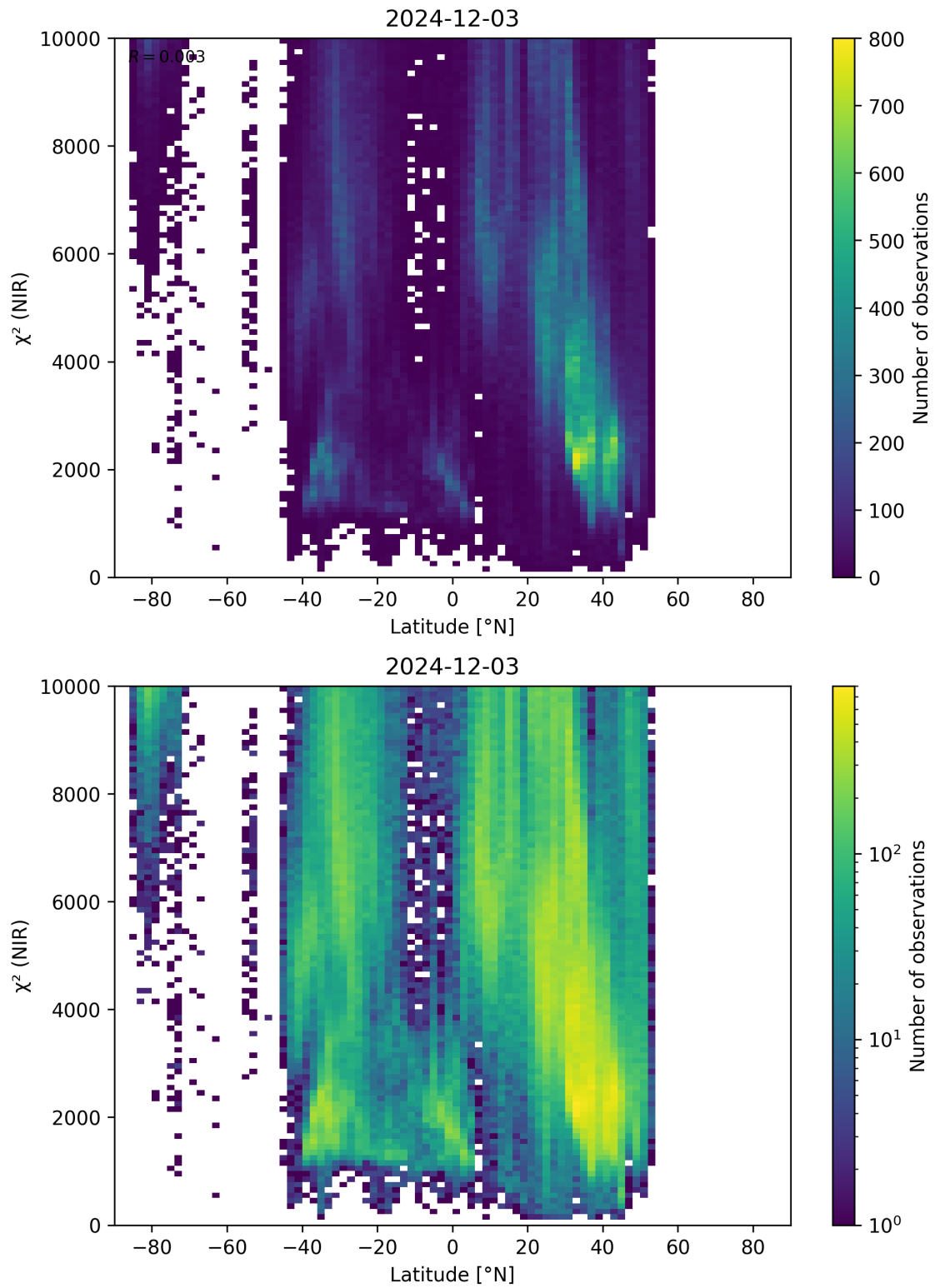
Figure 53: Scatter density plot of “Latitude” against “ \chi^2 (NIR)” for 2024-12-02 to 2024-12-04.
