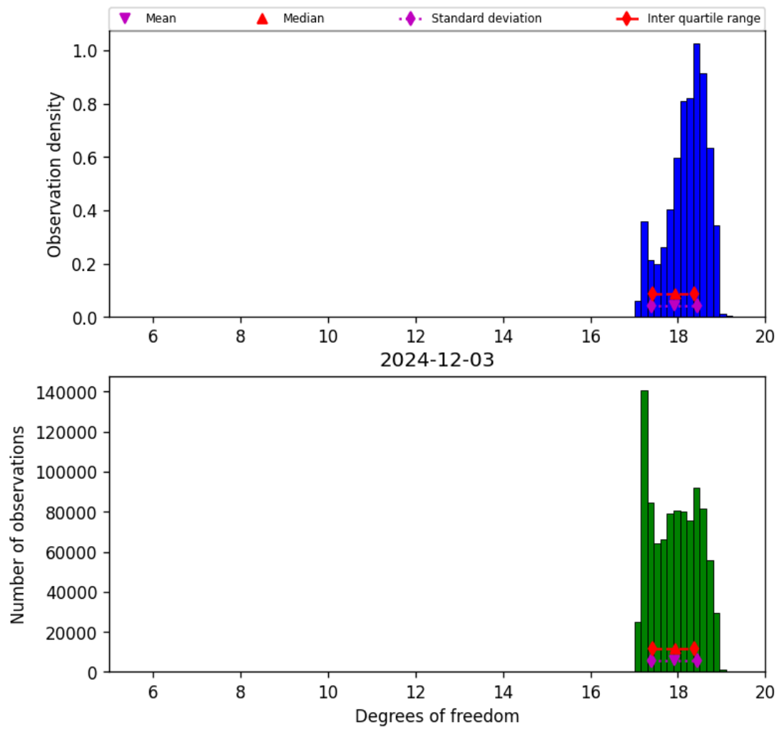
Figure 30: Histogram of “Degrees of freedom” for 2024-12-02 to 2024-12-04
