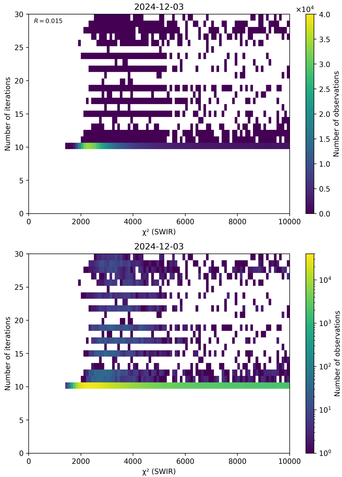
Figure 50: Scatter density plot of “ \chi^2 (SWIR)” against “Number of iterations” for 2024-12-02 to 2024-12-04.
