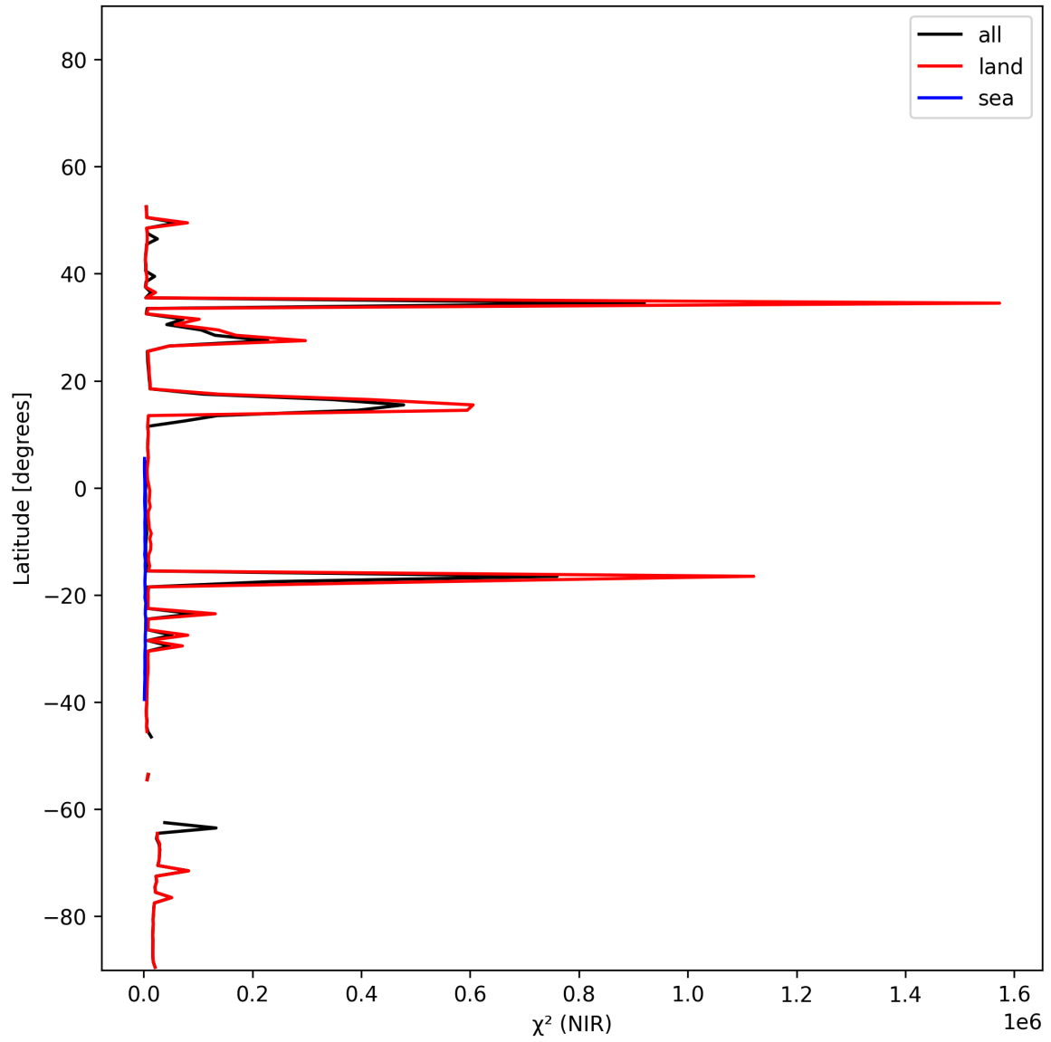
Figure 18: Zonal average of “ \chi^2 (NIR)” for 2024-12-02 to 2024-12-04.
