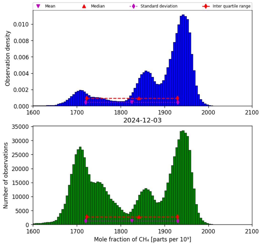
Figure 23: Histogram of “Mole fraction of CH 4 ” for 2024-12-02 to 2024-12-04
