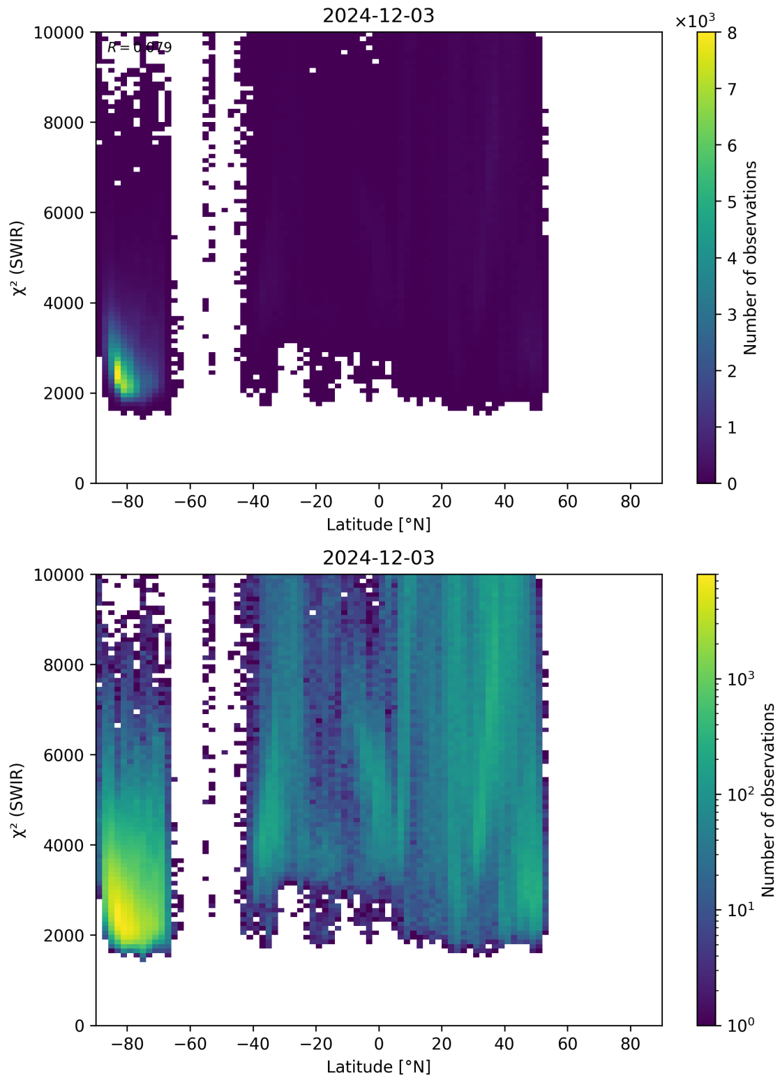
Figure 54: Scatter density plot of “Latitude” against “ \chi^2 (SWIR)” for 2024-12-02 to 2024-12-04.
