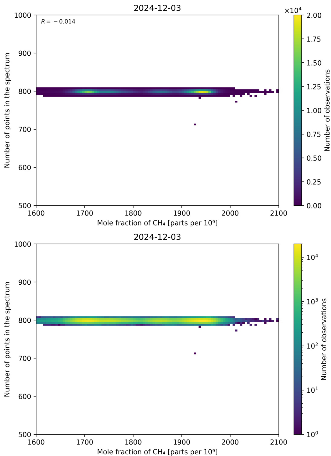
Figure 77: Scatter density plot of “Mole fraction of CH 4 ” against “Number of points in the spectrum” for 2024-12-02 to 2024-12-04.
