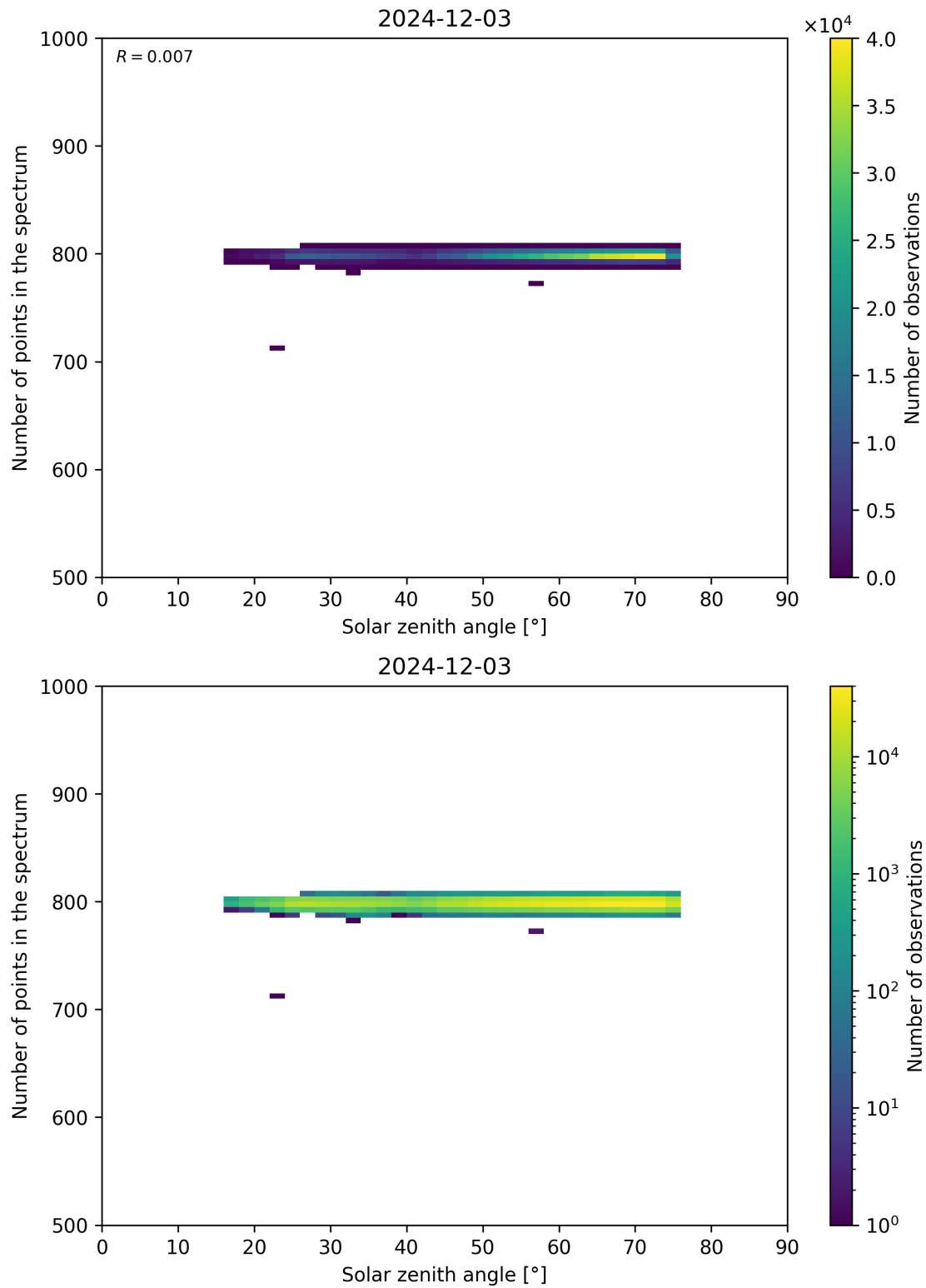
Figure 103: Scatter density plot of “Solar zenith angle” against “Number of points in the spectrum” for 2024-12-02 to 2024-12-04.
