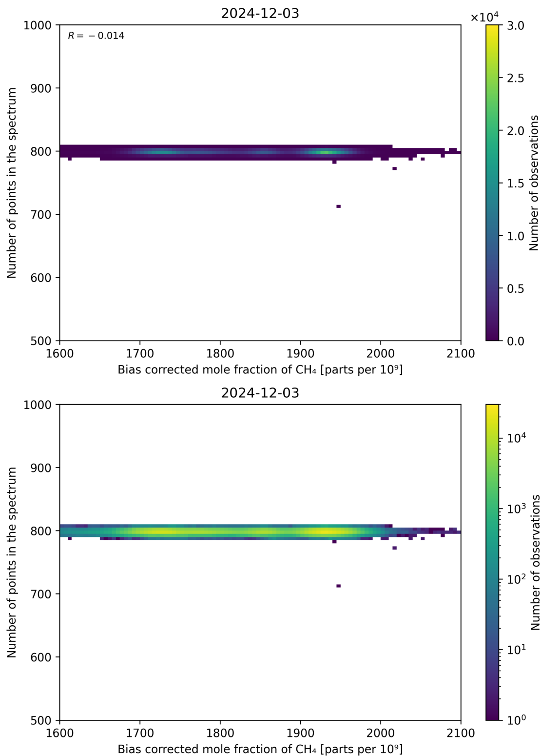
Figure 68: Scatter density plot of “Bias corrected mole fraction of CH 4 ” against “Number of points in the spectrum” for 2024-12-02 to 2024-12-04.
