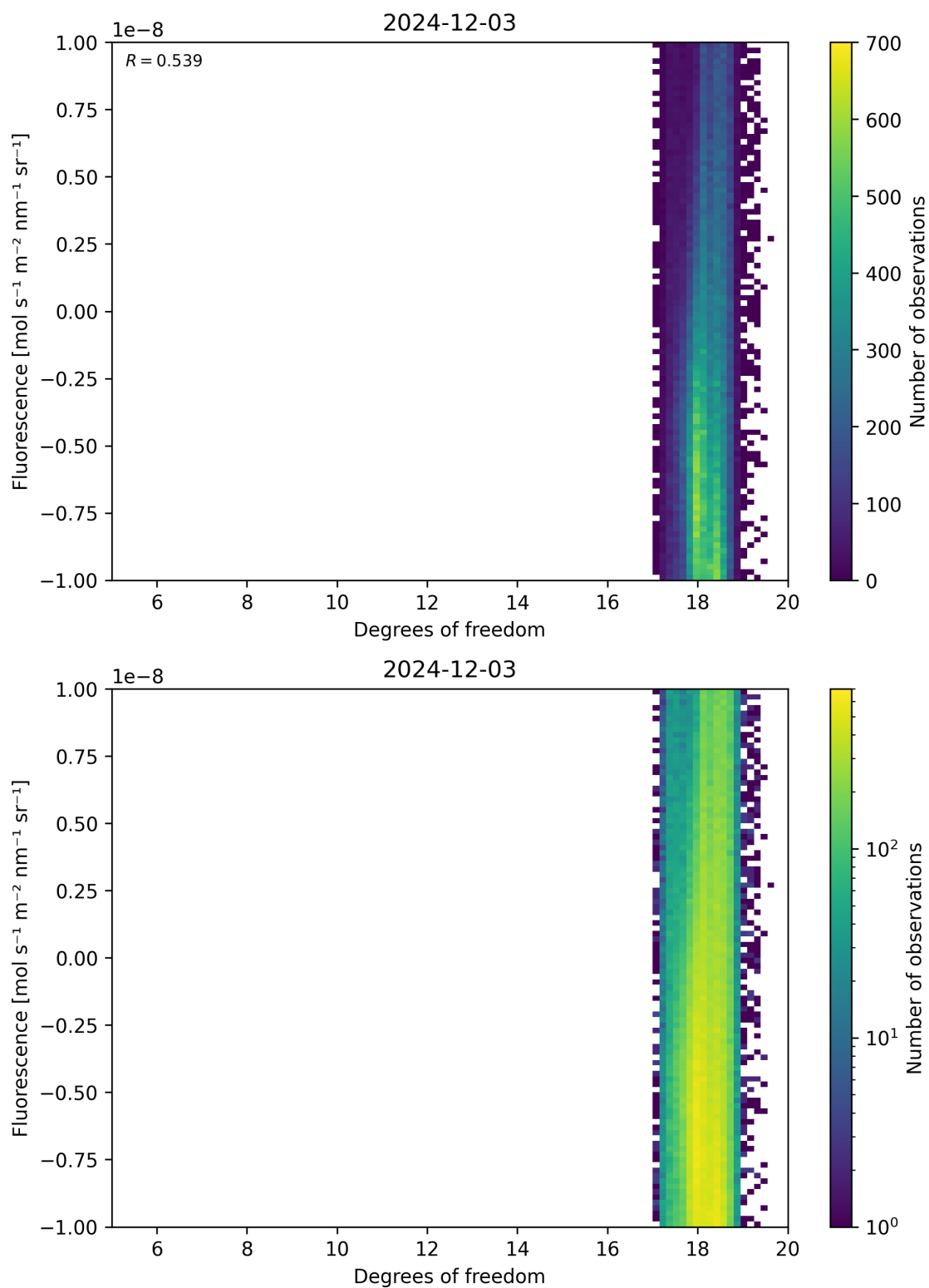
Figure 51: Scatter density plot of “Degrees of freedom” against “Fluorescence” for 2024-12-02 to 2024-12-04.
