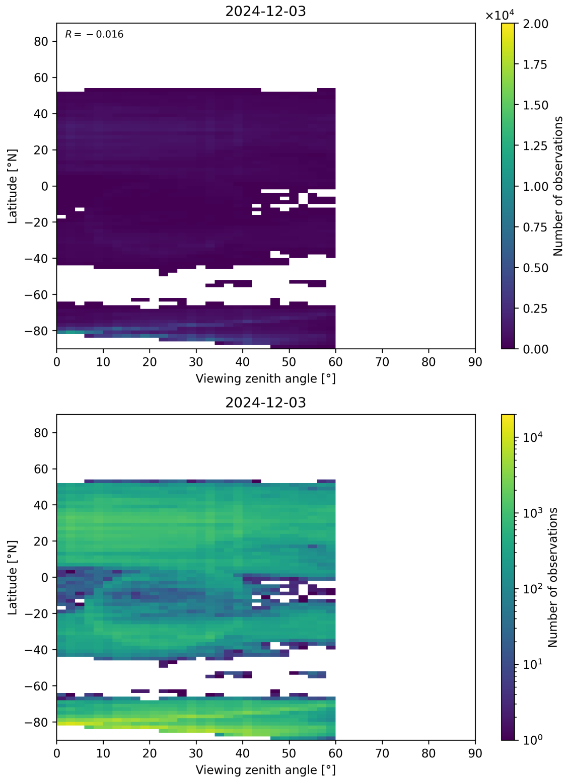
Figure 109: Scatter density plot of “Viewing zenith angle” against “Latitude” for 2024-12-02 to 2024-12-04.
