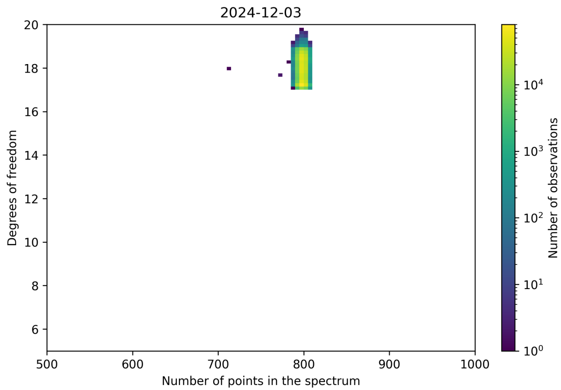
Figure 90: Scatter density plot of “Number of points in the spectrum” against “Degrees of freedom” for 2024-12-02 to 2024-12-04.
