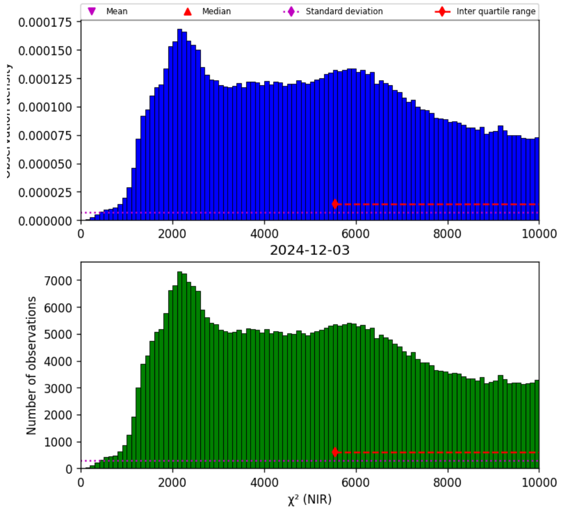
Figure 29: Histogram of “ \chi^2 (NIR)” for 2024-12-02 to 2024-12-04
