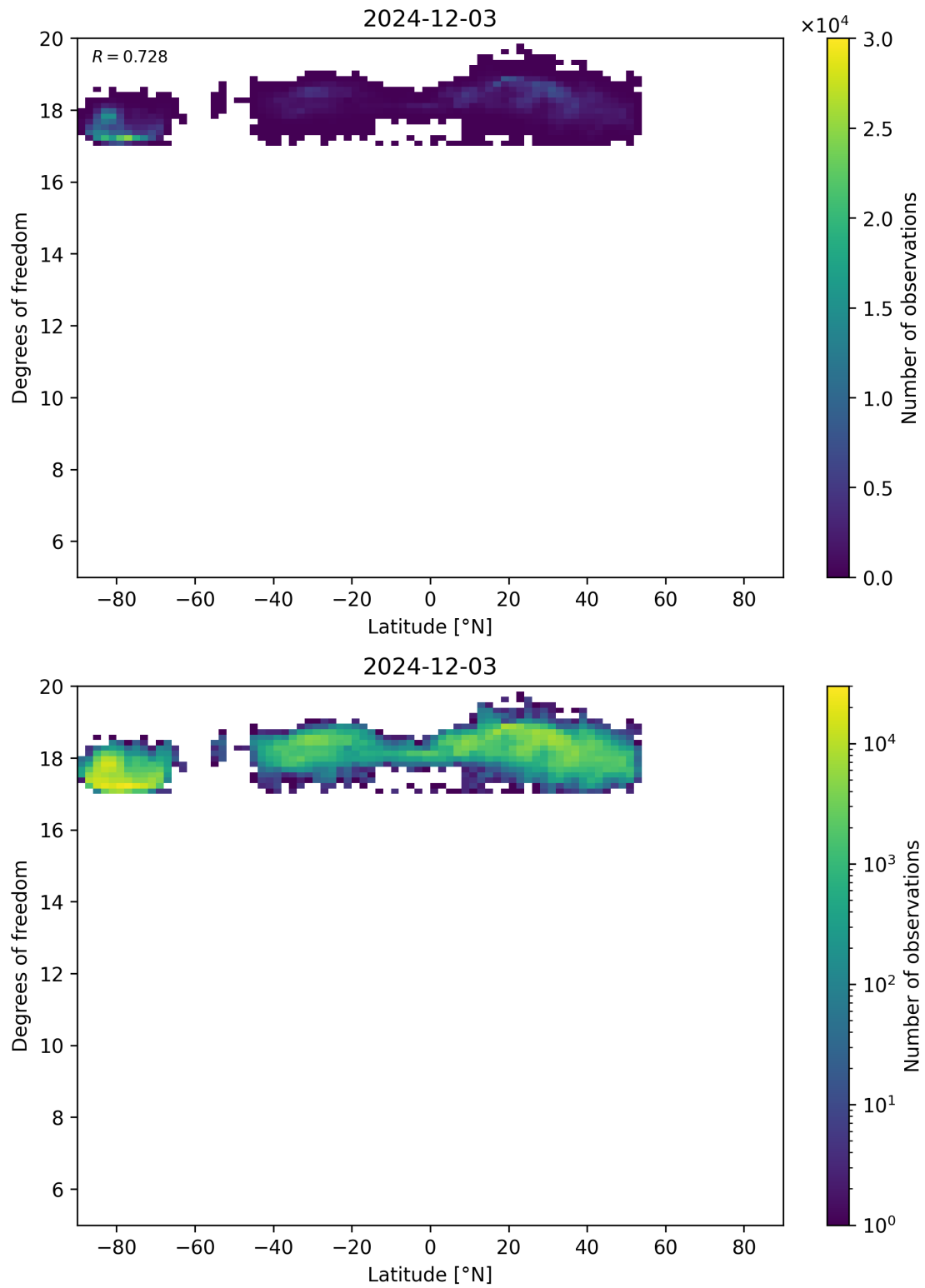
Figure 55: Scatter density plot of “Latitude” against “Degrees of freedom” for 2024-12-02 to 2024-12-04.
