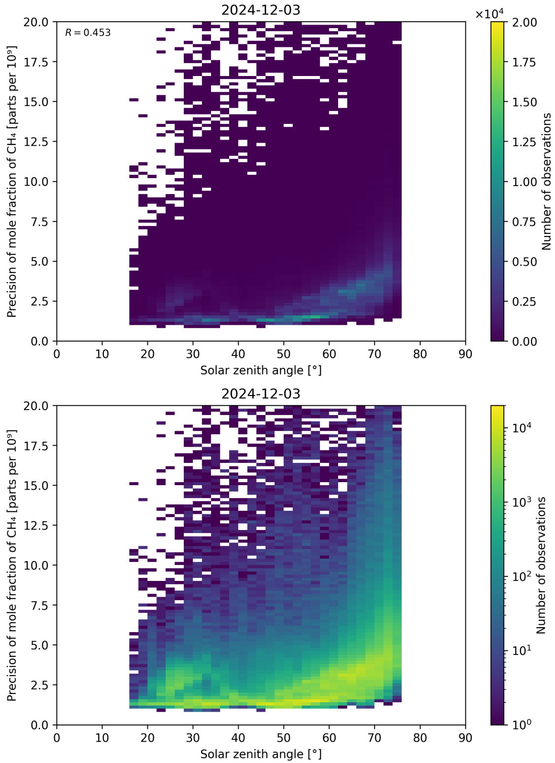
Figure 101: Scatter density plot of “Solar zenith angle” against “Precision of mole fraction of \text{CH}_4 ” for 2024-12-02 to 2024-12-04.
