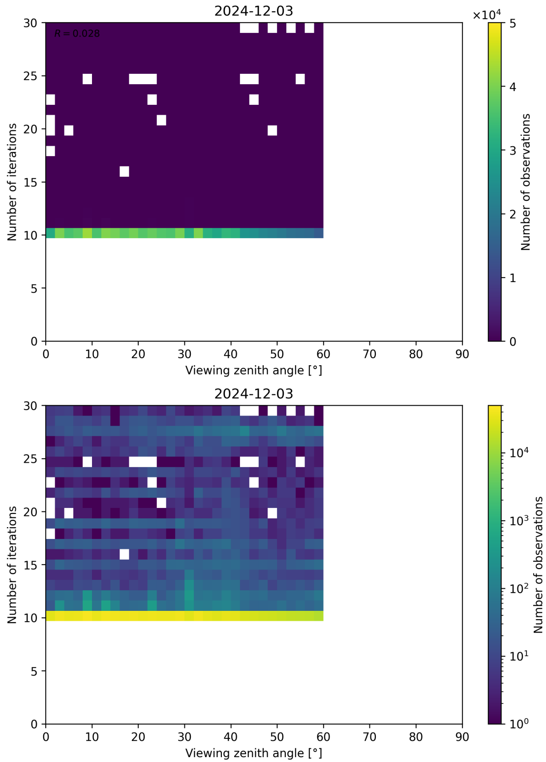
Figure 113: Scatter density plot of “Viewing zenith angle” against “Number of iterations” for 2024-12-02 to 2024-12-04.
