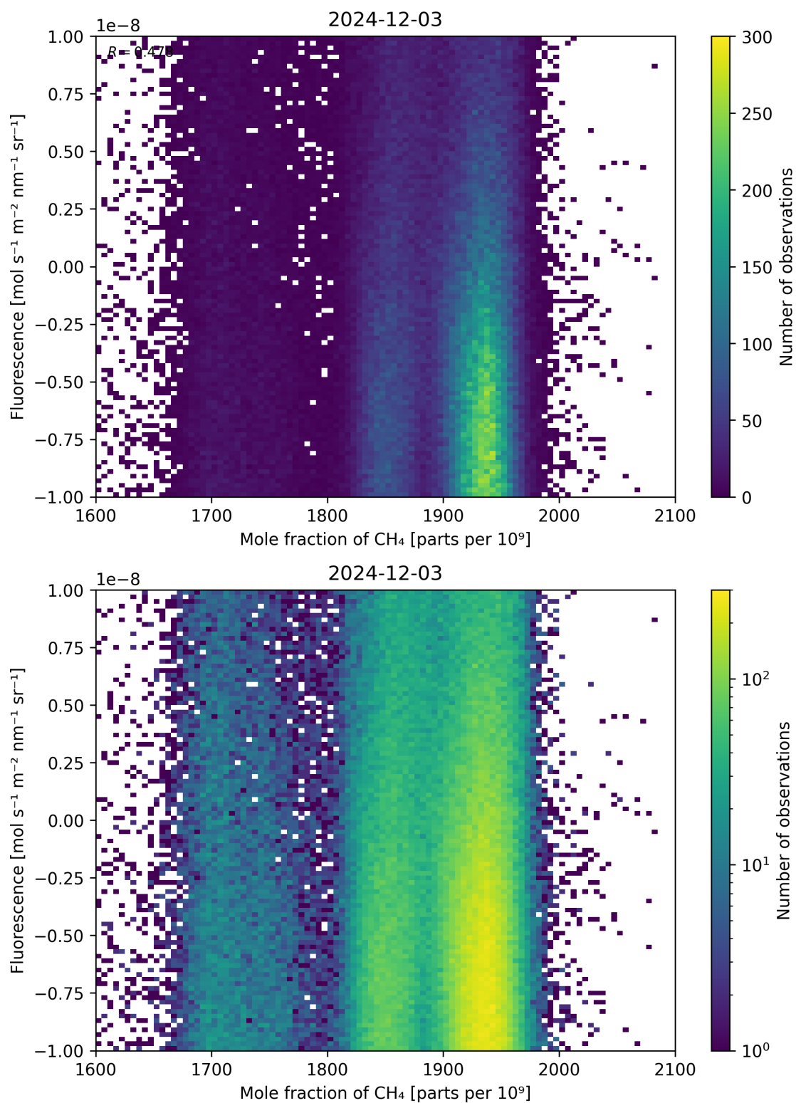
Figure 73: Scatter density plot of “Mole fraction of \text{CH}_4 ” against “Fluorescence” for 2024-12-02 to 2024-12-04.
