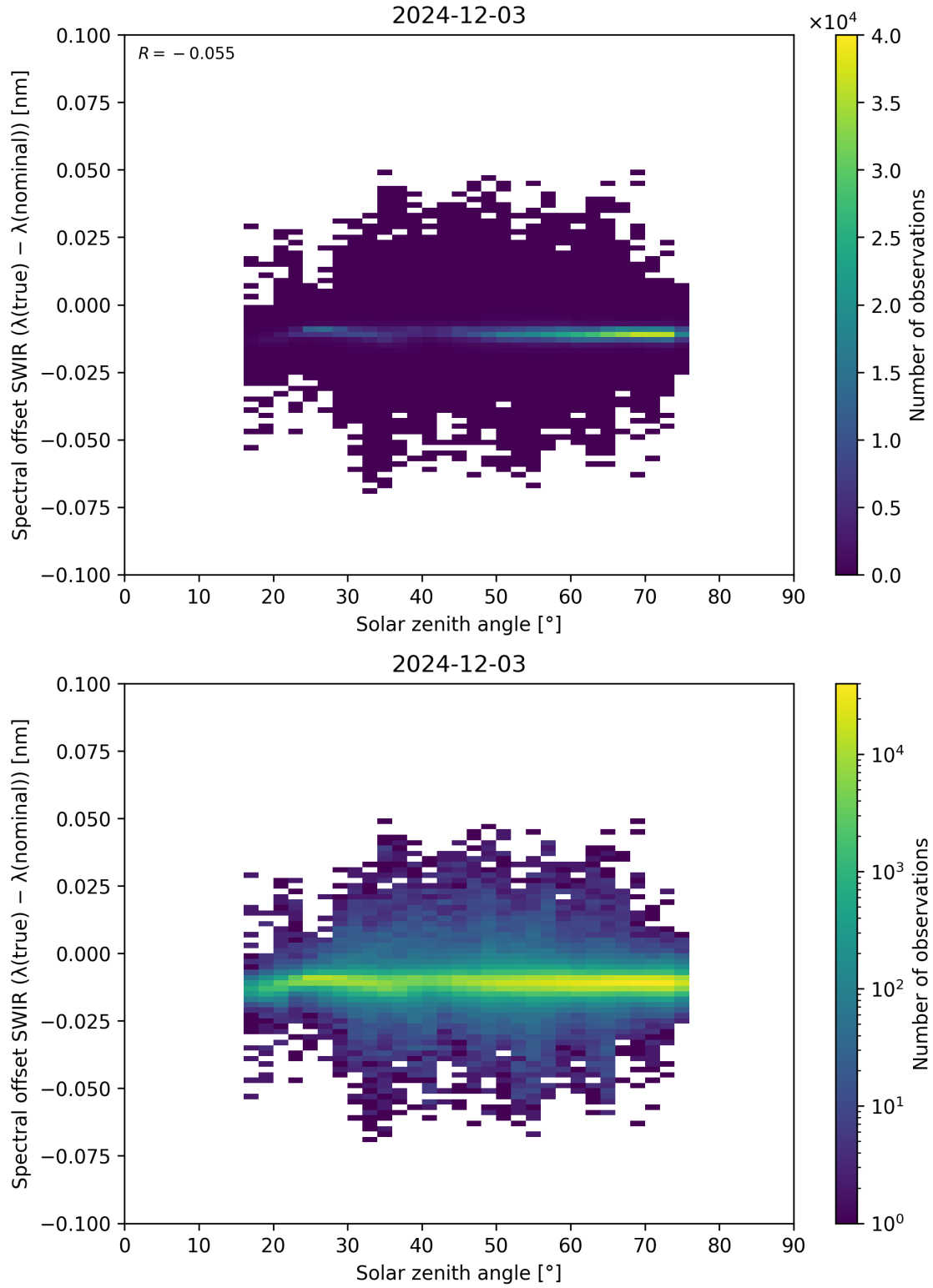
Figure 104: Scatter density plot of “Solar zenith angle” against “Spectral offset SWIR ( \lambda_{\text{true}} - \lambda_{\text{nominal}} )” for 2024-12-02 to 2024-12-04.
