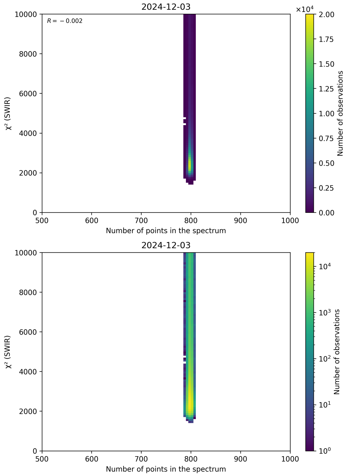
Figure 89: Scatter density plot of “Number of points in the spectrum” against “ \chi^2 (SWIR)” for 2024-12-02 to 2024-12-04.
