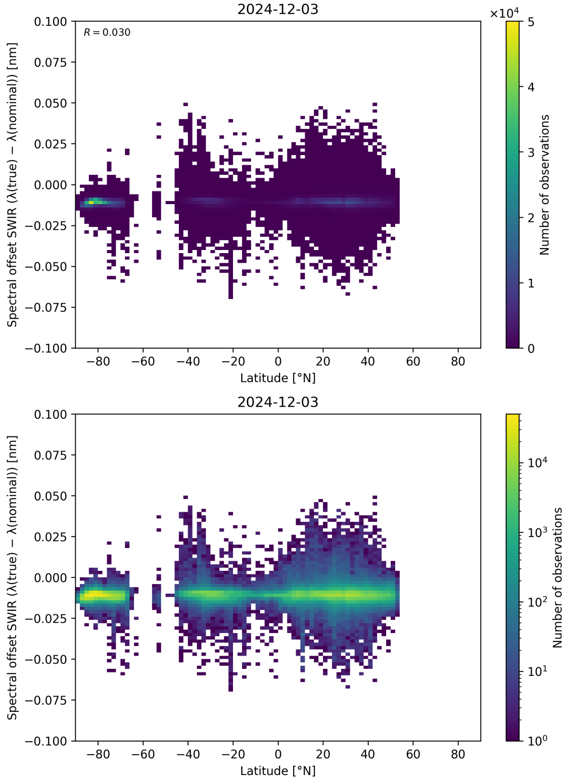
Figure 62: Scatter density plot of “Latitude” against “Spectral offset SWIR ( \lambda_{\text{true}} - \lambda_{\text{nominal}} )” for 2024-12-02 to 2024-12-04.
