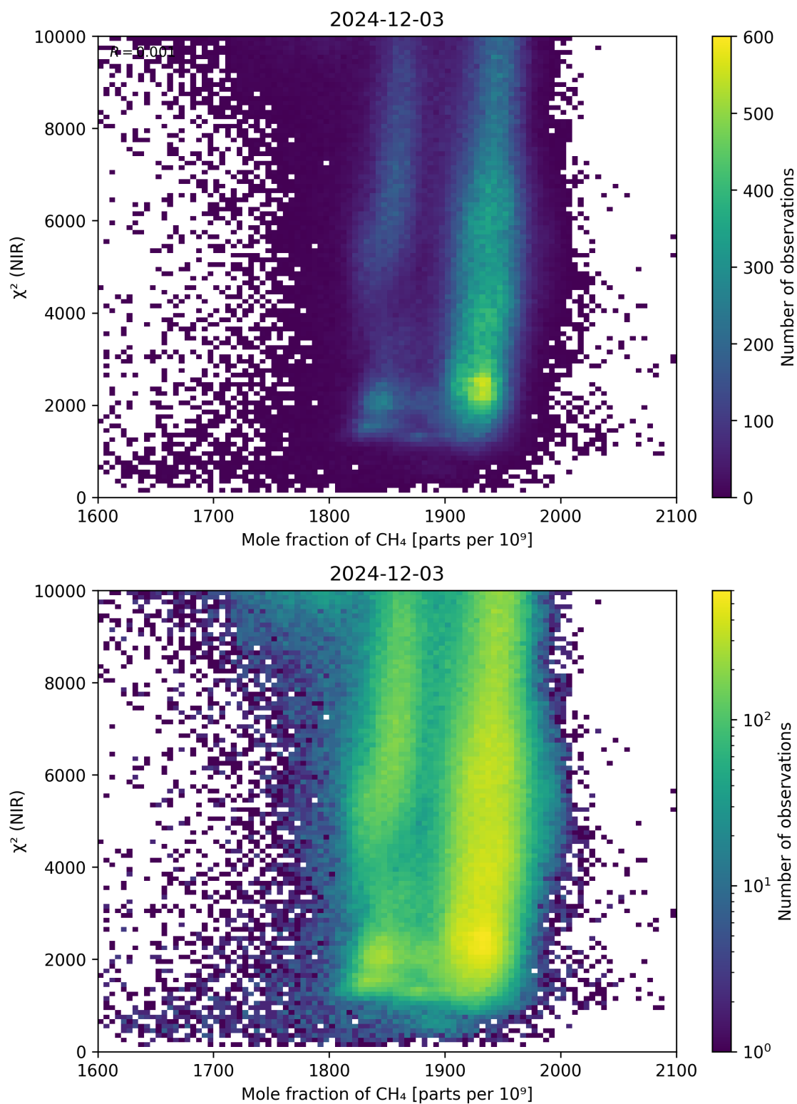
Figure 70: Scatter density plot of “Mole fraction of CH 4 ” against “ \chi^2 (NIR)” for 2024-12-02 to 2024-12-04.
