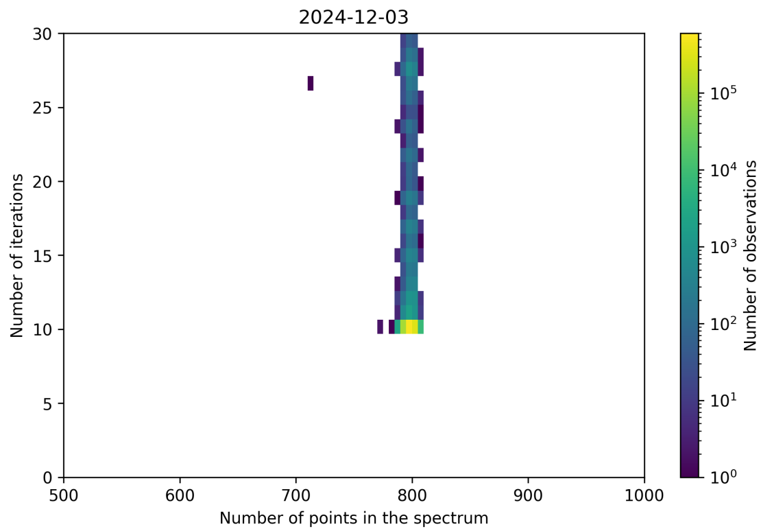
Figure 92: Scatter density plot of “Number of points in the spectrum” against “Number of iterations” for 2024-12-02 to 2024-12-04.
