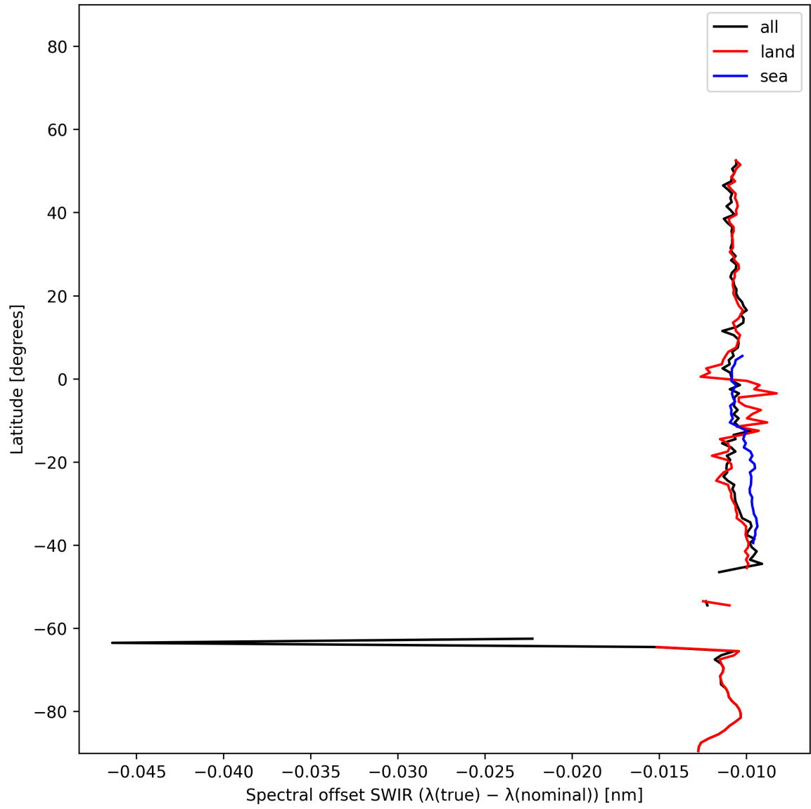
Figure 16: Zonal average of “Spectral offset SWIR ( \lambda_{\text{true}} - \lambda_{\text{nominal}} )” for 2024-12-02 to 2024-12-04.
