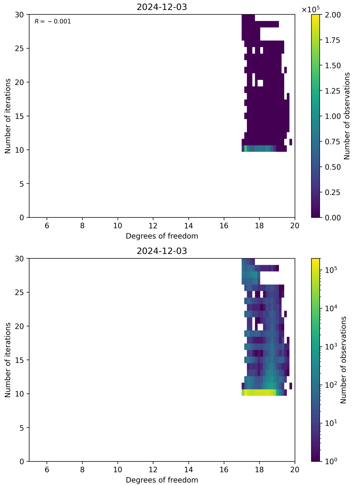
Figure 52: Scatter density plot of “Degrees of freedom” against “Number of iterations” for 2024-12-02 to 2024-12-04.
