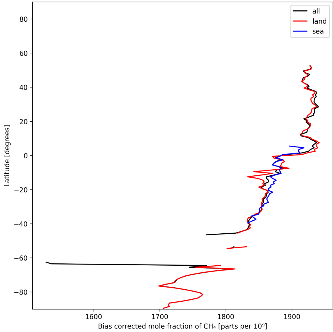
Figure 14: Zonal average of “Bias corrected mole fraction of CH 4 ” for 2024-12-02 to 2024-12-04.
