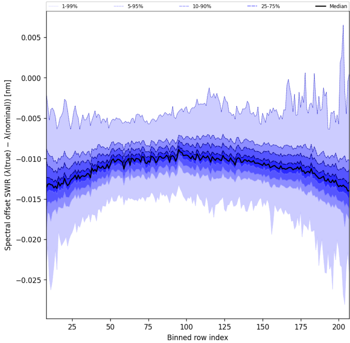
Figure 38: Along track statistics of “Spectral offset SWIR ( \lambda_{\text{true}} - \lambda_{\text{nominal}} )” for 2024-12-02 to 2024-12-04
