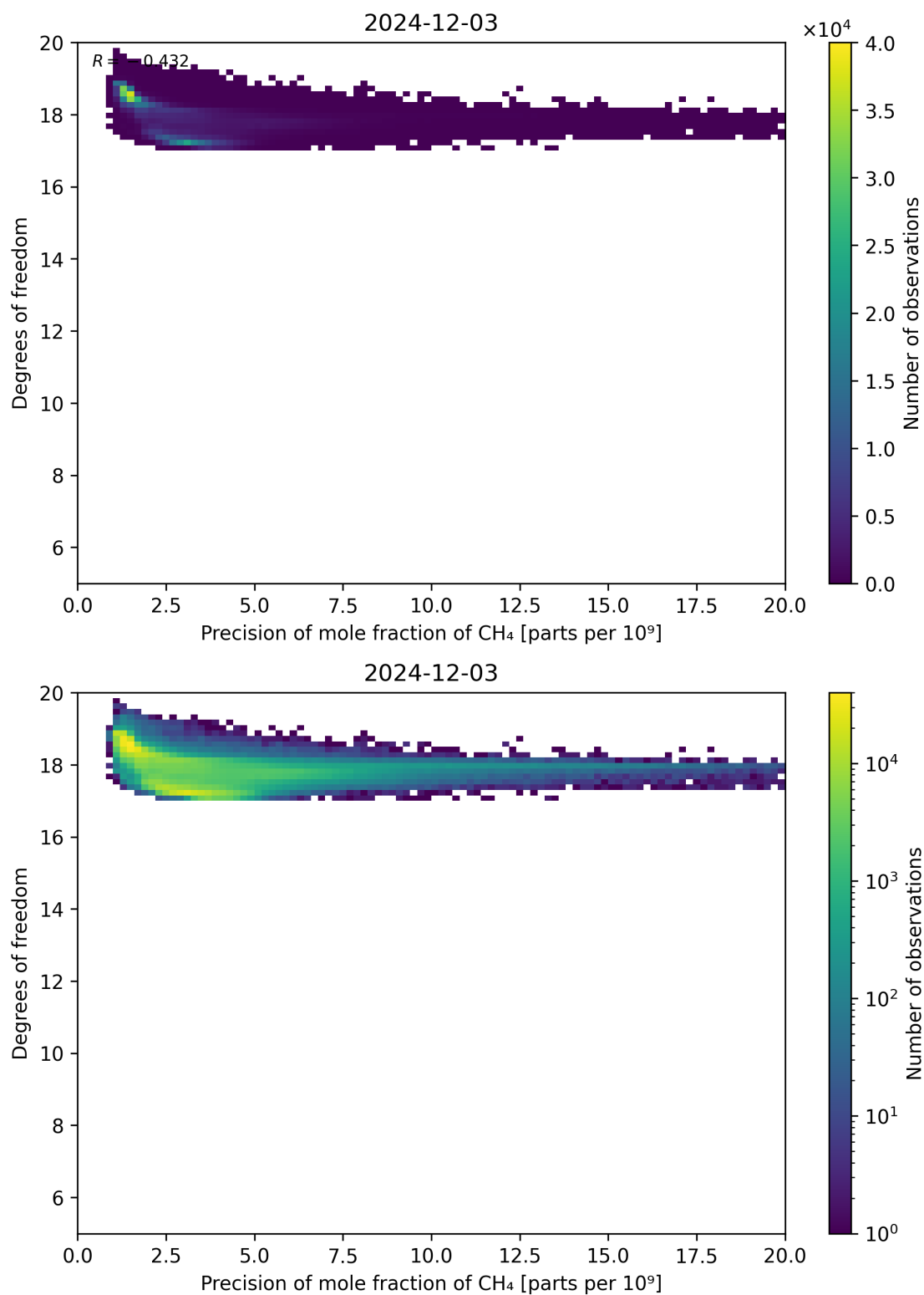
Figure 80: Scatter density plot of “Precision of mole fraction of CH 4 ” against “Degrees of freedom” for 2024-12-02 to 2024-12-04.
