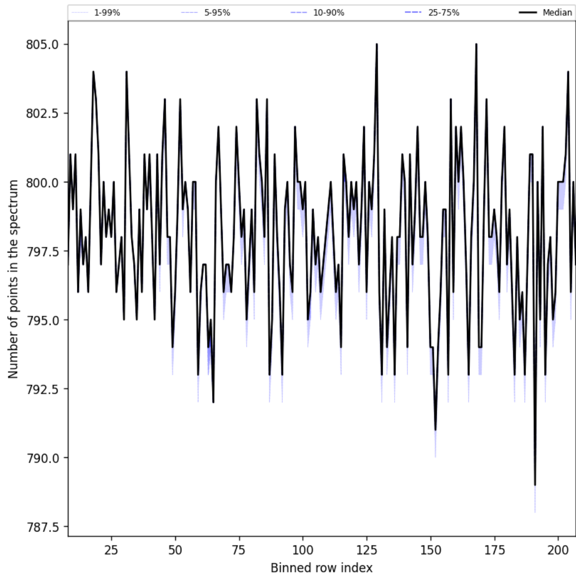
Figure 37: Along track statistics of “Number of points in the spectrum” for 2024-12-02 to 2024-12-04
