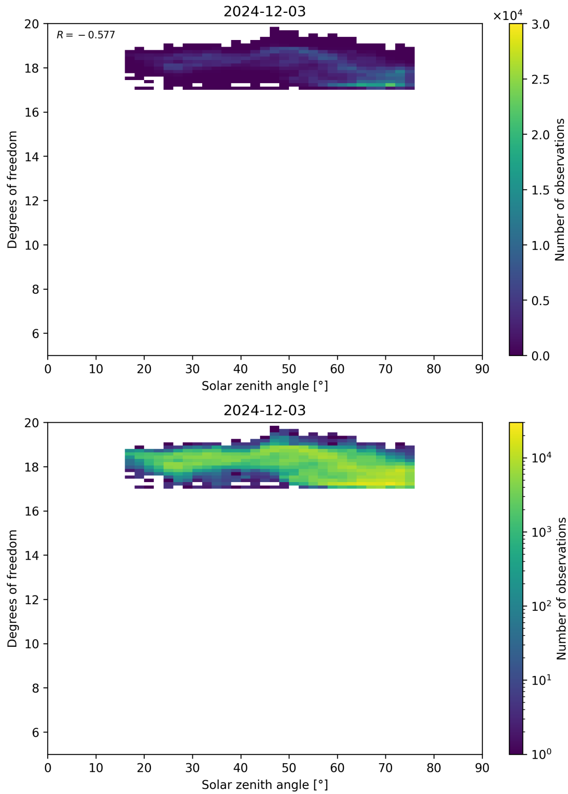
Figure 96: Scatter density plot of “Solar zenith angle” against “Degrees of freedom” for 2024-12-02 to 2024-12-04.
