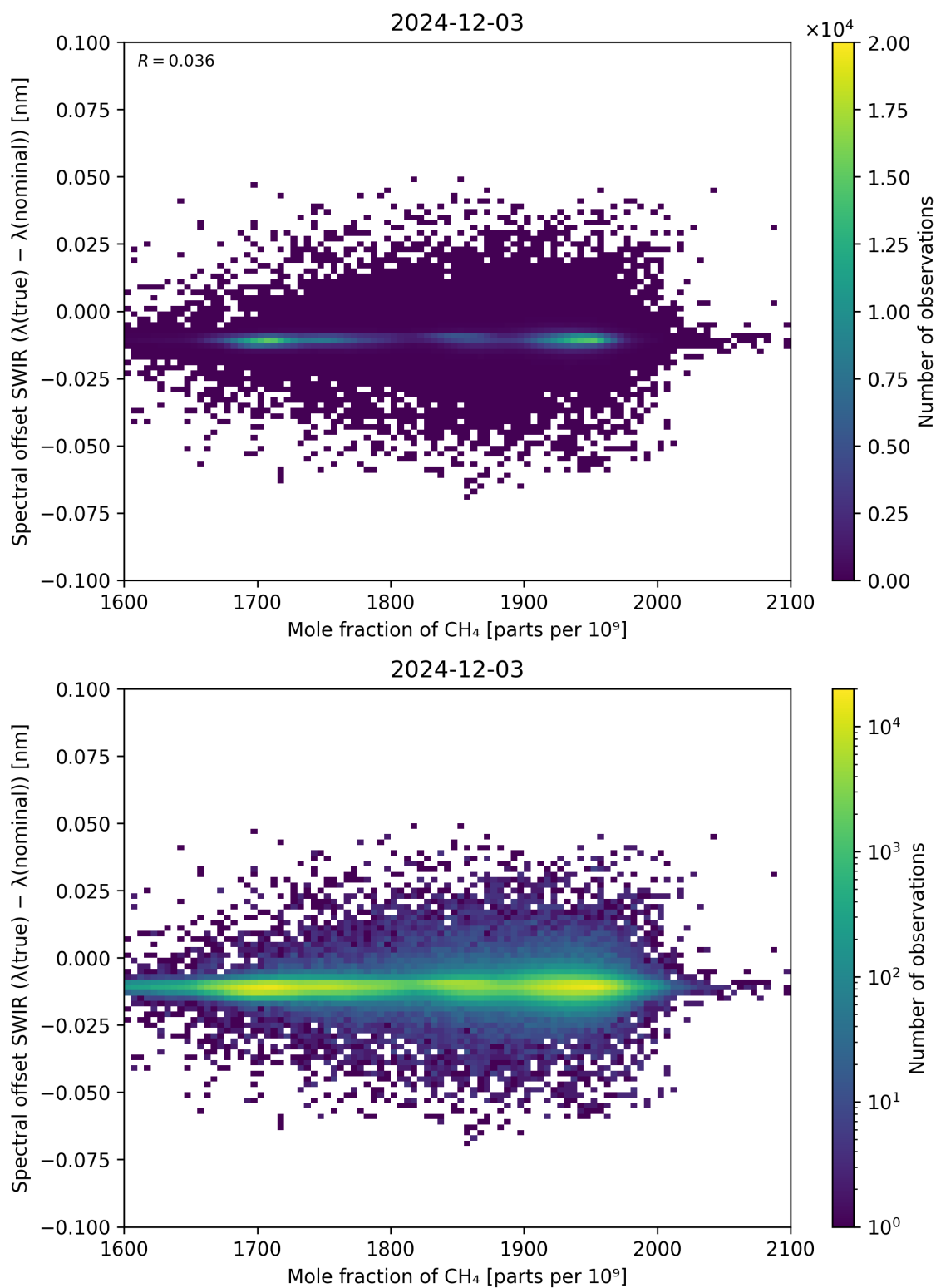
Figure 86: Scatter density plot of “Mole fraction of \text{CH}_4 ” against “Spectral offset SWIR ( \lambda_{\text{true}} - \lambda_{\text{nominal}} )” for 2024-12-02 to 2024-12-04.
