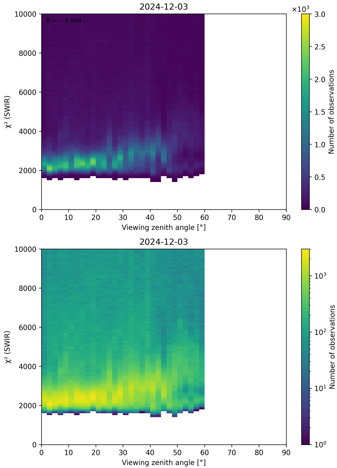
Figure 106: Scatter density plot of “Viewing zenith angle” against “ \chi^2 (SWIR)” for 2024-12-02 to 2024-12-04.
