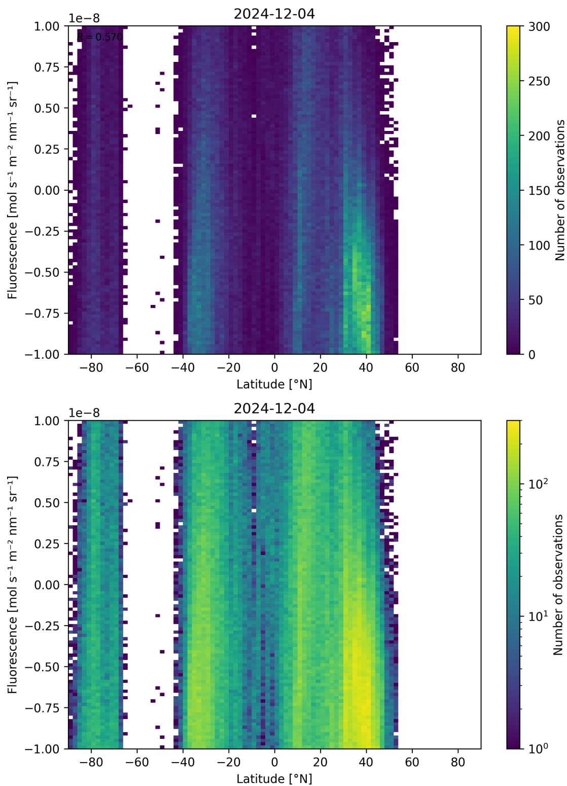
Figure 56: Scatter density plot of “Latitude” against “Fluorescence” for 2024-12-03 to 2024-12-05.
