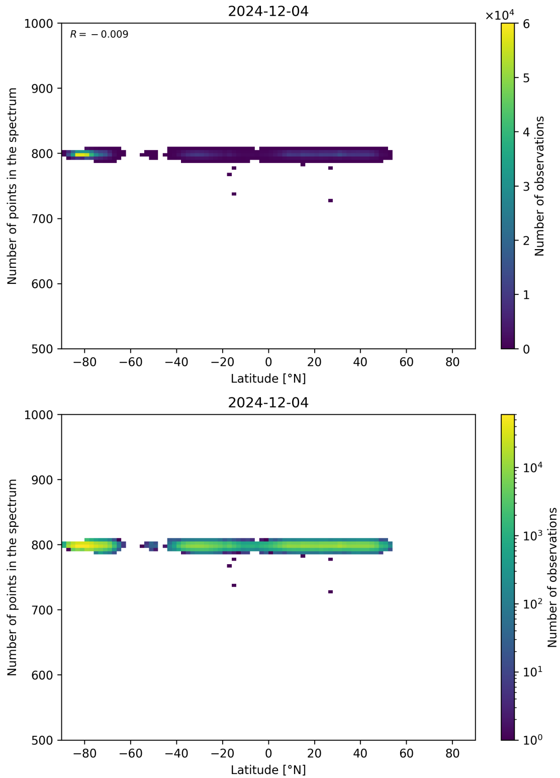
Figure 61: Scatter density plot of “Latitude” against “Number of points in the spectrum” for 2024-12-03 to 2024-12-05.
