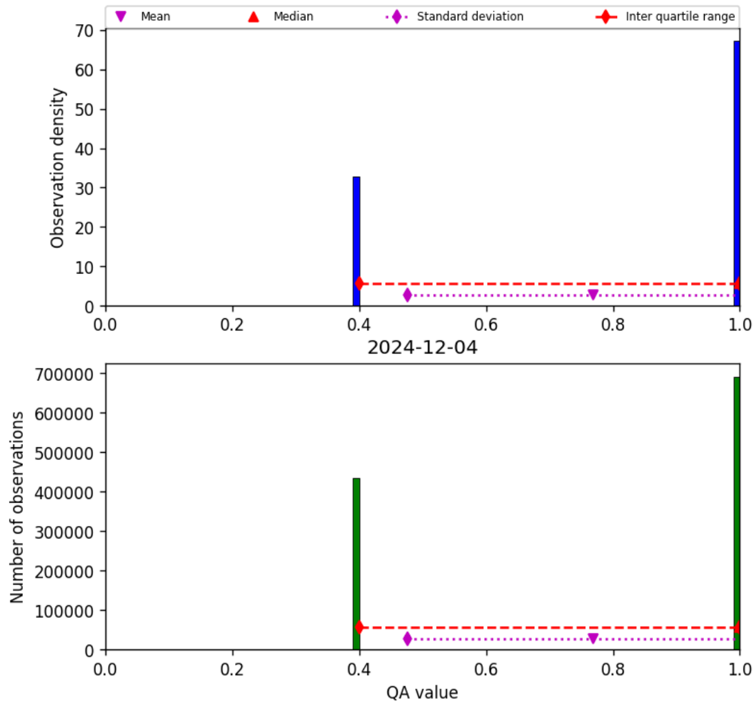
Figure 22: Histogram of “QA value” for 2024-12-03 to 2024-12-05
