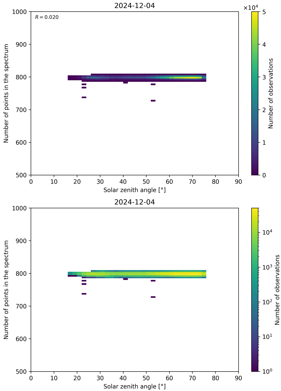
Figure 103: Scatter density plot of “Solar zenith angle” against “Number of points in the spectrum” for 2024-12-03 to 2024-12-05.
