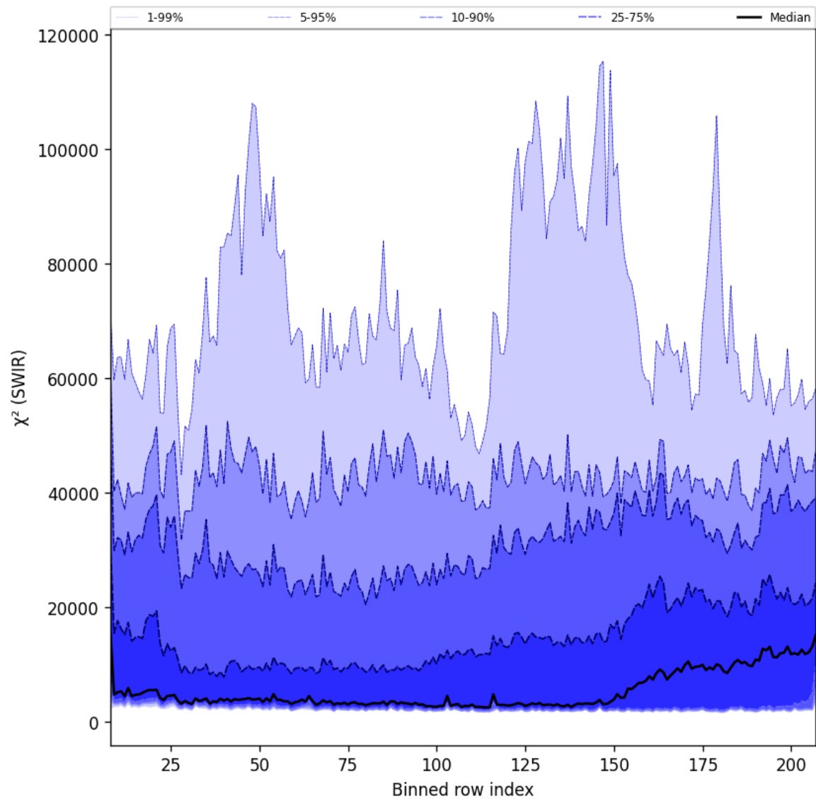
Figure 39: Along track statistics of “ \chi^2 (SWIR)” for 2024-12-03 to 2024-12-05
