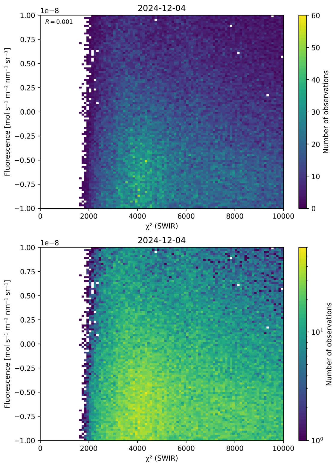
Figure 49: Scatter density plot of “ \chi^2 (SWIR)” against “Fluorescence” for 2024-12-03 to 2024-12-05.
