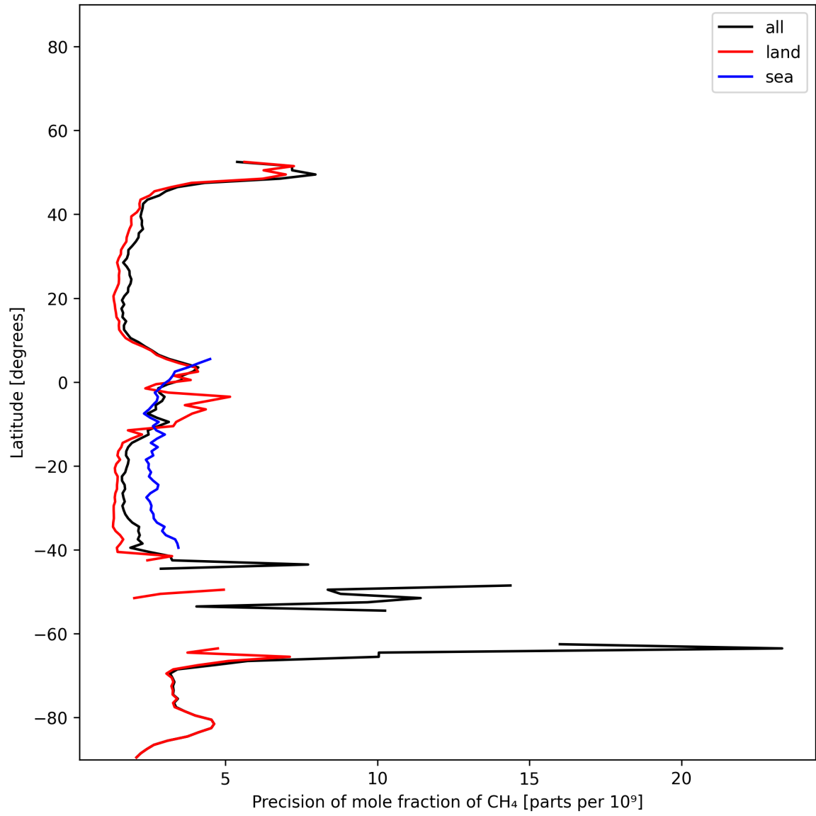
Figure 13: Zonal average of “Precision of mole fraction of CH 4 ” for 2024-12-03 to 2024-12-05.
