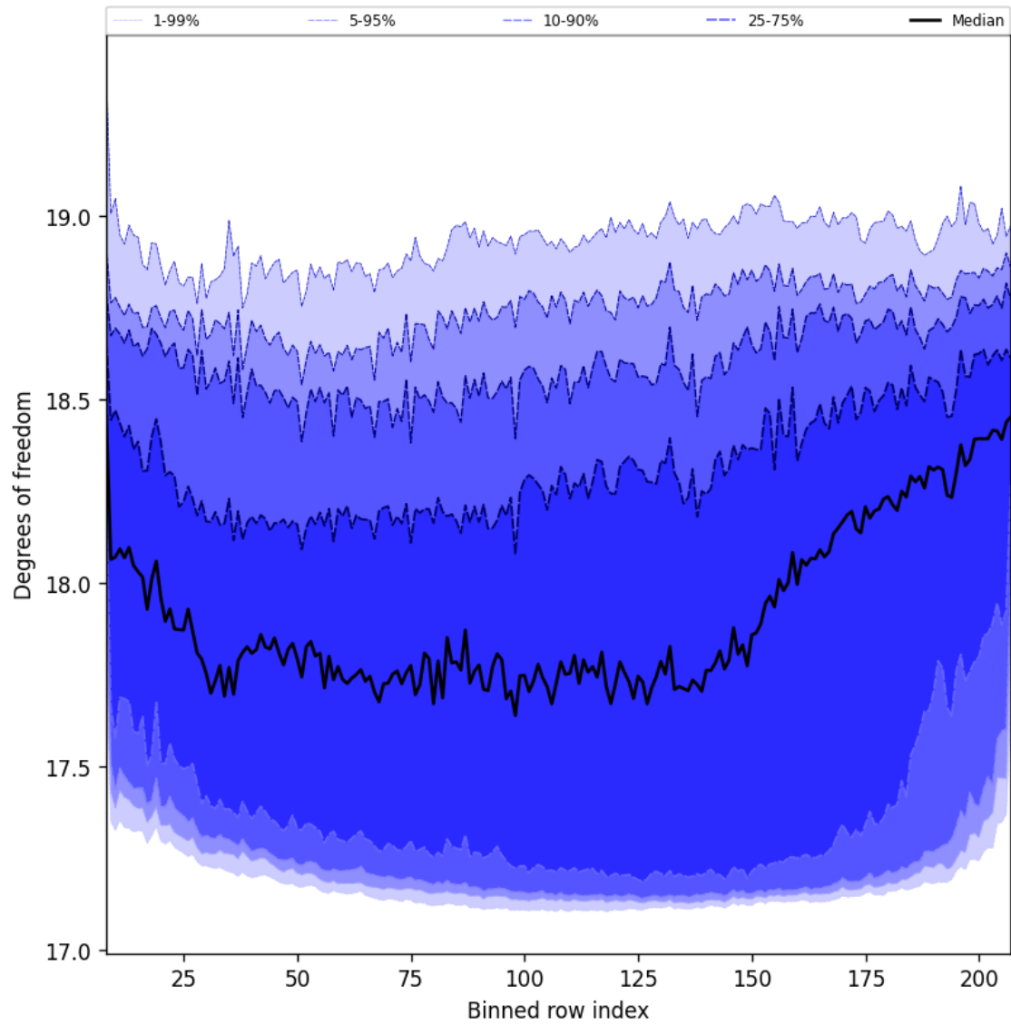
Figure 41: Along track statistics of “Degrees of freedom” for 2024-12-03 to 2024-12-05
