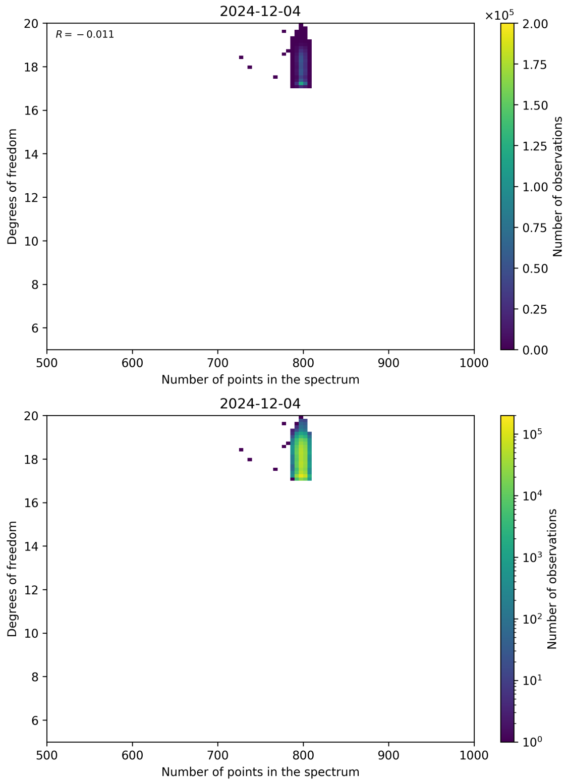
Figure 90: Scatter density plot of “Number of points in the spectrum” against “Degrees of freedom” for 2024-12-03 to 2024-12-05.
