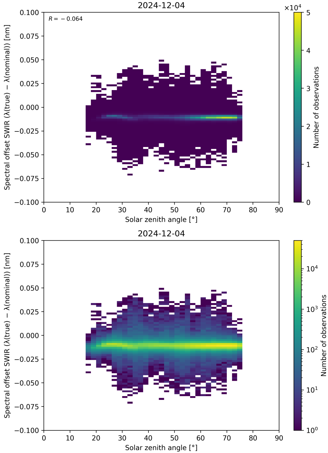
Figure 104: Scatter density plot of “Solar zenith angle” against “Spectral offset SWIR ( \lambda_{\text{true}} - \lambda_{\text{nominal}} )” for 2024-12-03 to 2024-12-05.
