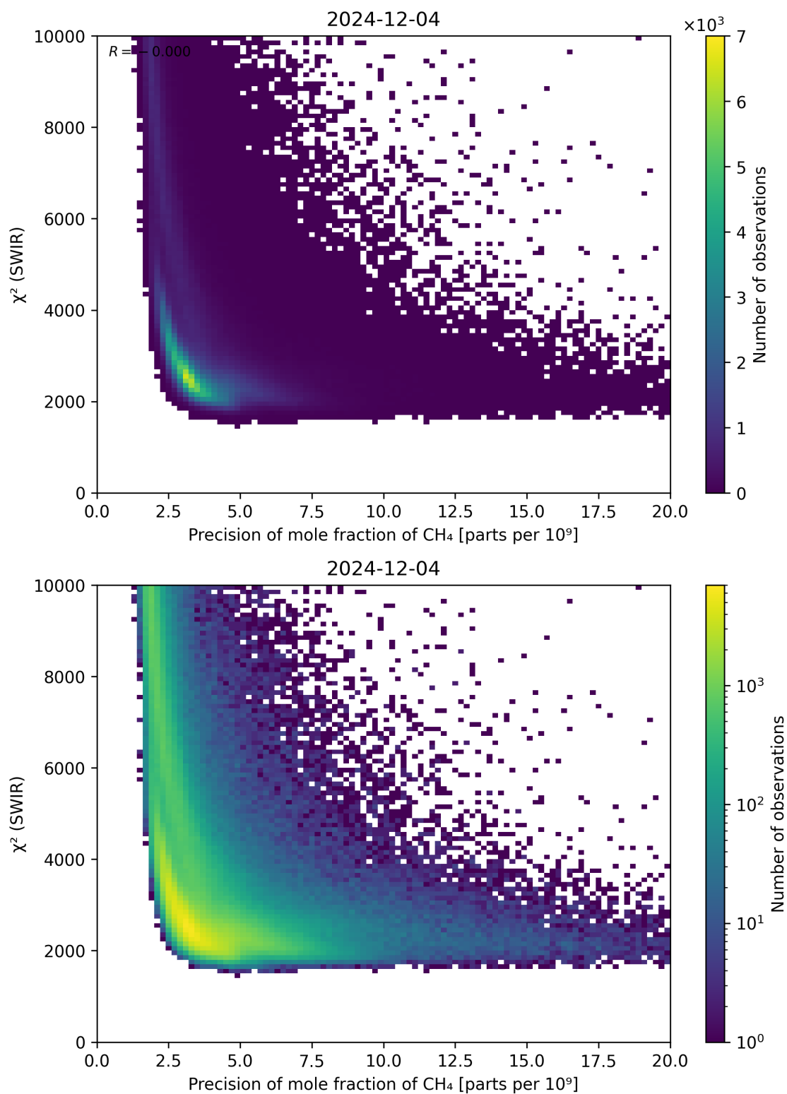
Figure 79: Scatter density plot of “Precision of mole fraction of CH 4 ” against “ \chi^2 (SWIR)” for 2024-12-03 to 2024-12-05.
