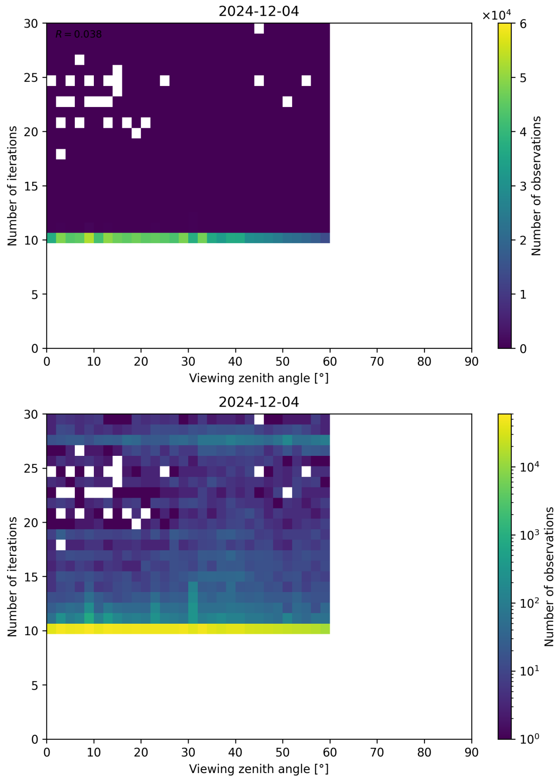
Figure 113: Scatter density plot of “Viewing zenith angle” against “Number of iterations” for 2024-12-03 to 2024-12-05.
