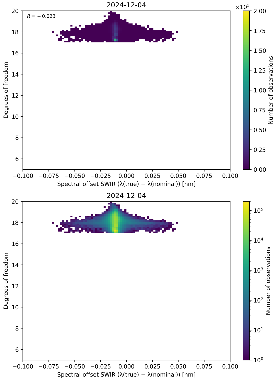
Figure 119: Scatter density plot of “Spectral offset SWIR ( \lambda_{\text{true}} - \lambda_{\text{nominal}} )” against “Degrees of freedom” for 2024-12-03 to 2024-12-05.
