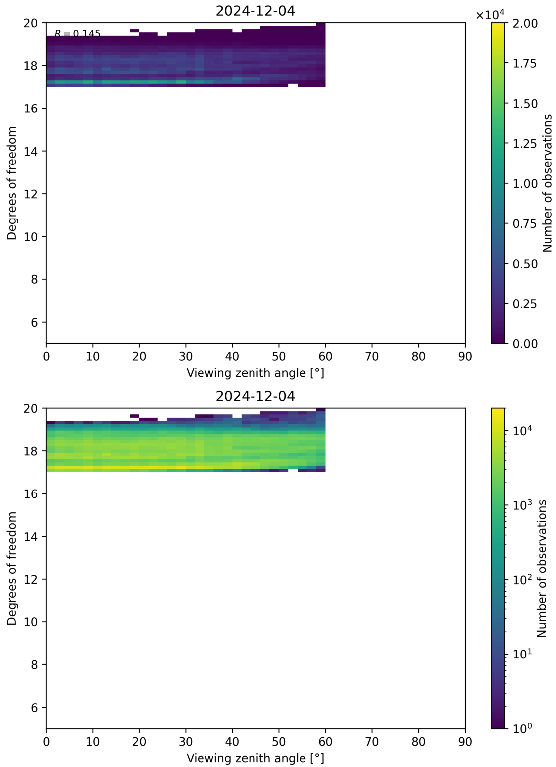
Figure 107: Scatter density plot of “Viewing zenith angle” against “Degrees of freedom” for 2024-12-03 to 2024-12-05.
