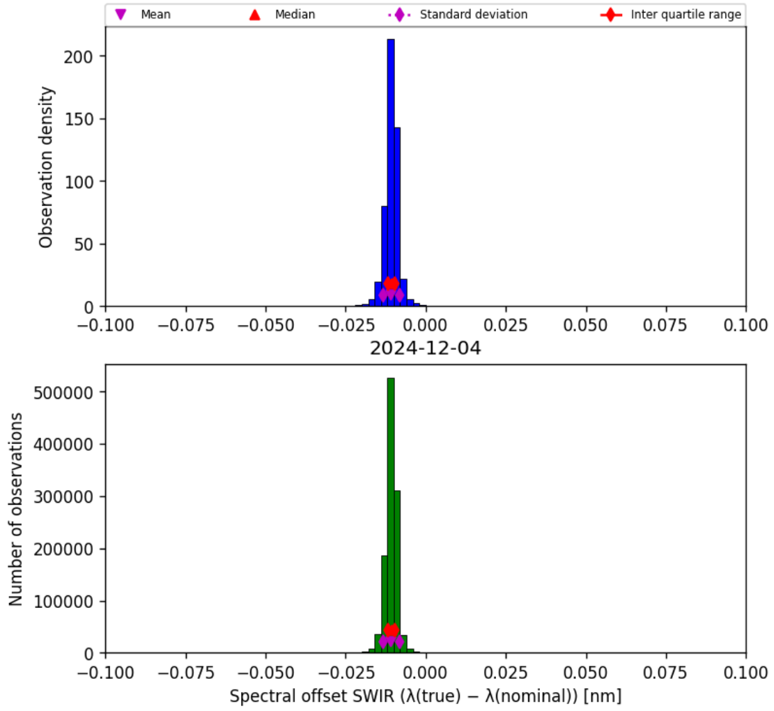
Figure 27: Histogram of “Spectral offset SWIR ( \lambda_{\text{true}} - \lambda_{\text{nominal}} )” for 2024-12-03 to 2024-12-05
