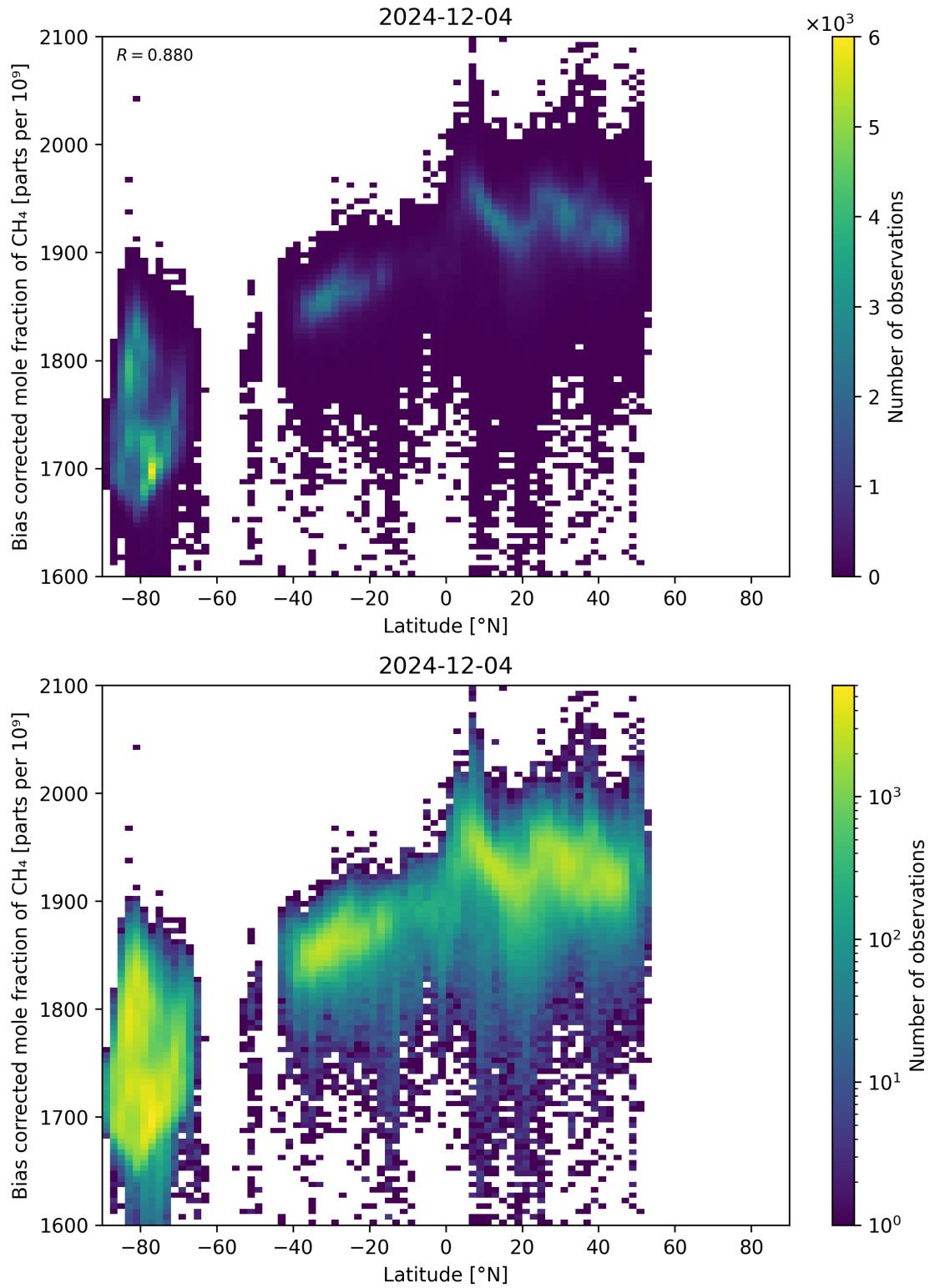
Figure 58: Scatter density plot of “Latitude” against “Bias corrected mole fraction of \text{CH}_4 ” for 2024-12-03 to 2024-12-05.
