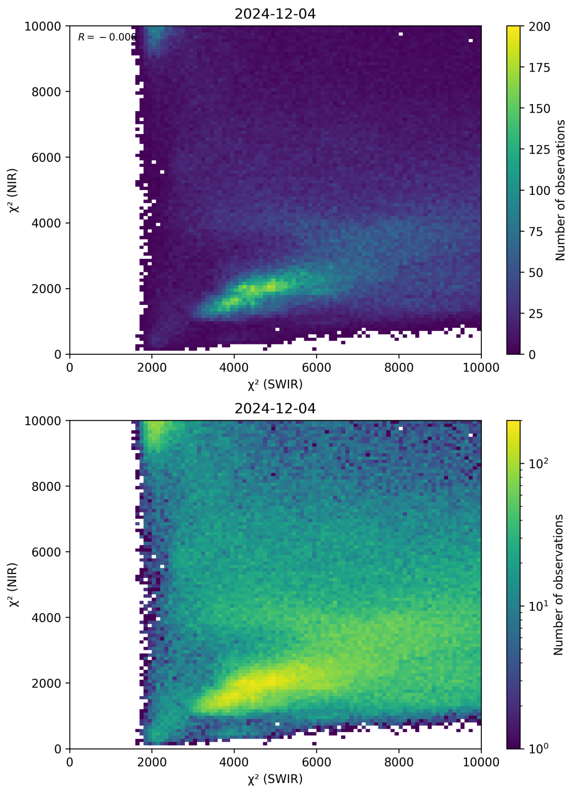
Figure 47: Scatter density plot of “ \chi^2 (SWIR)” against “ \chi^2 (NIR)” for 2024-12-03 to 2024-12-05.
