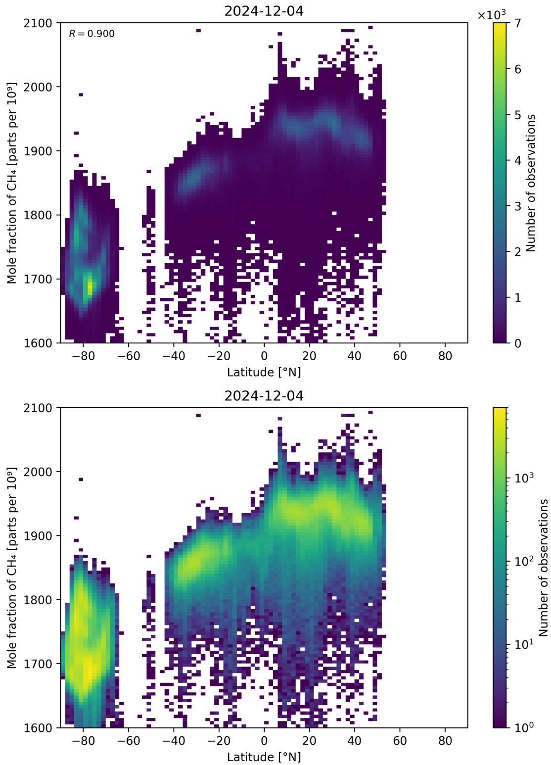
Figure 57: Scatter density plot of “Latitude” against “Mole fraction of CH 4 ” for 2024-12-03 to 2024-12-05.
