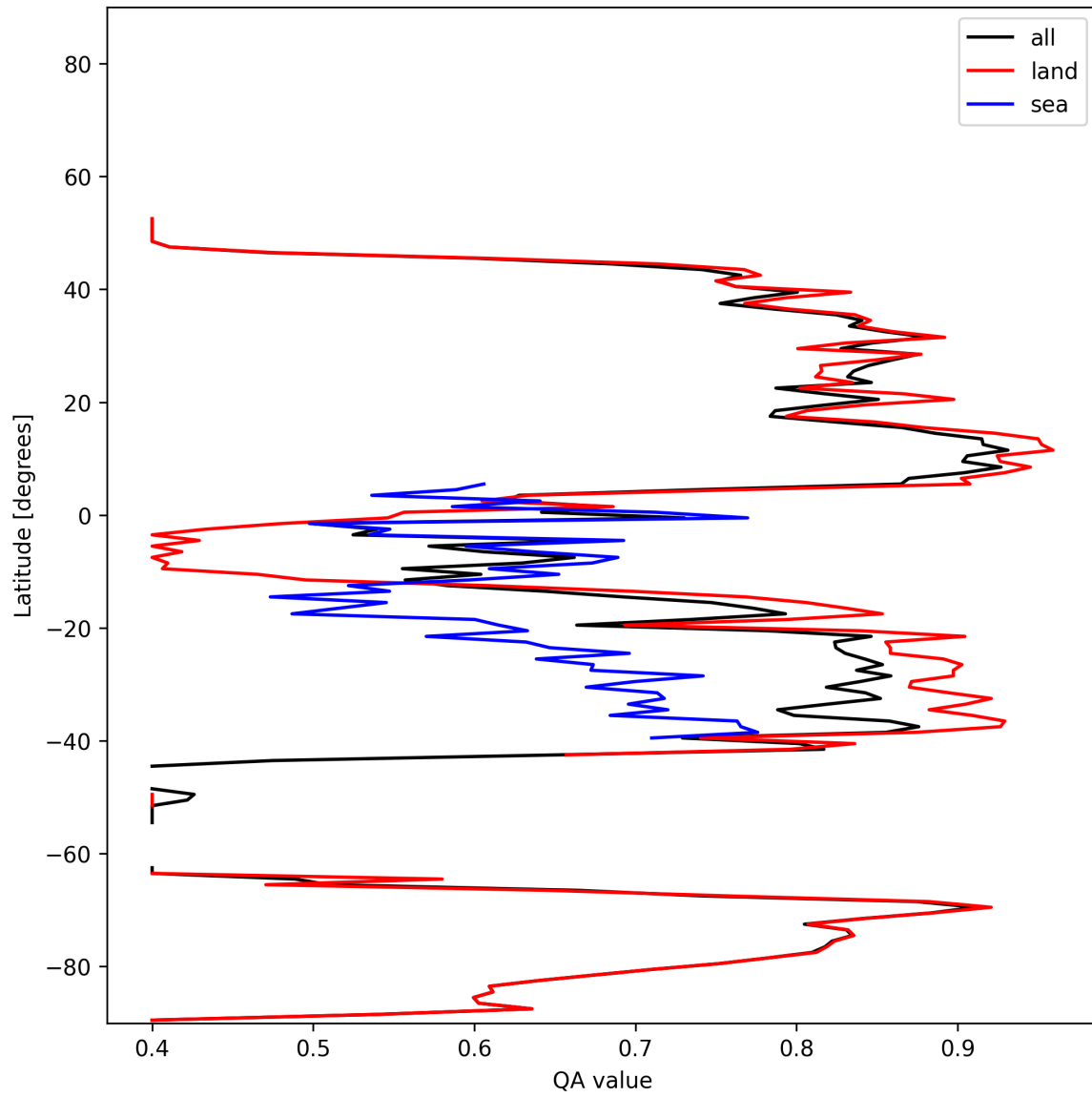
Figure 11: Zonal average of “QA value” for 2024-12-03 to 2024-12-05.
