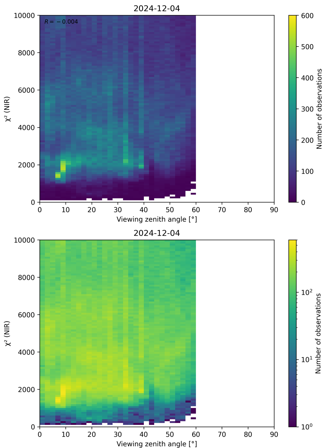
Figure 105: Scatter density plot of “Viewing zenith angle” against “ \chi^2 (NIR)” for 2024-12-03 to 2024-12-05.
