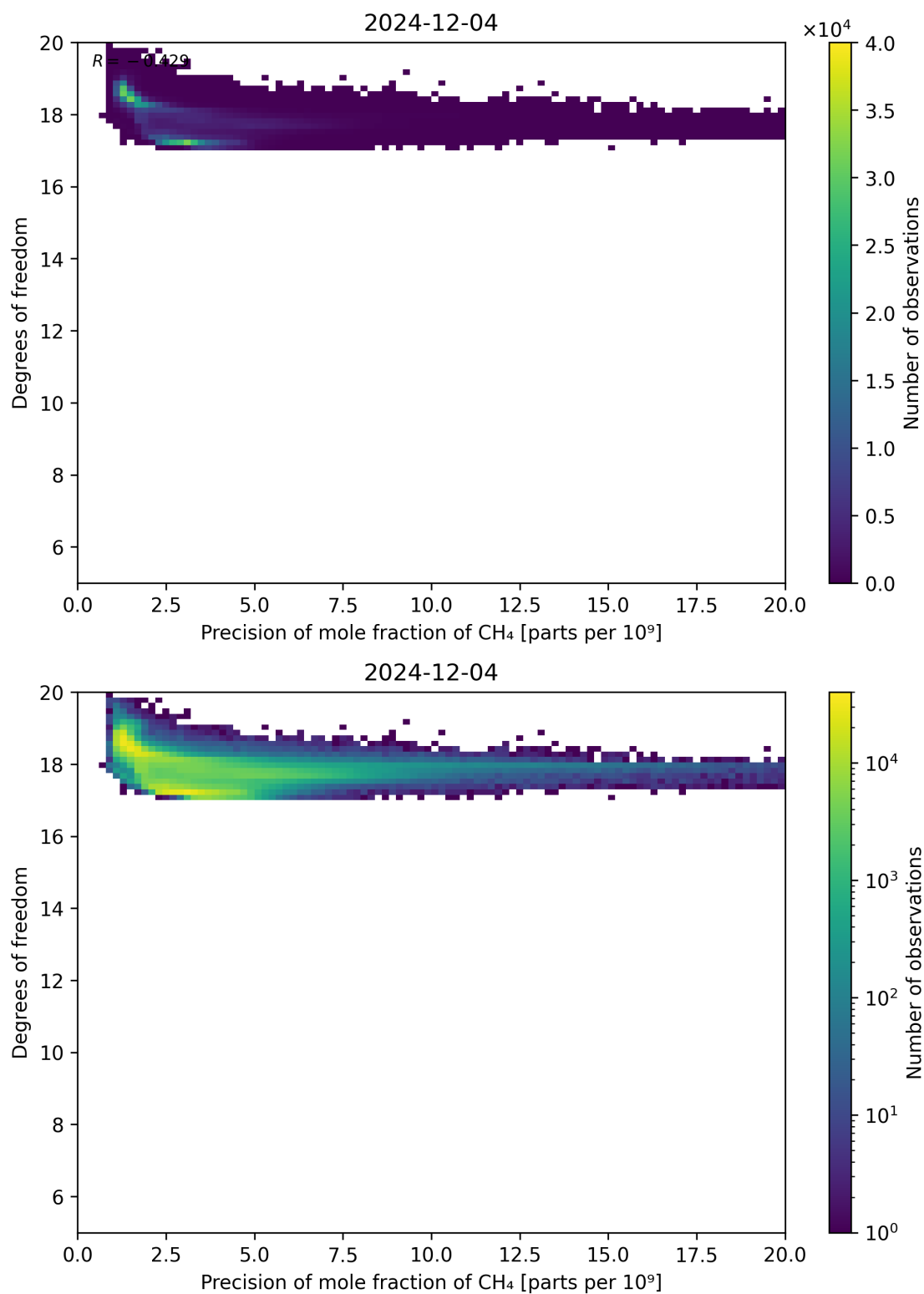
Figure 80: Scatter density plot of “Precision of mole fraction of CH 4 ” against “Degrees of freedom” for 2024-12-03 to 2024-12-05.
