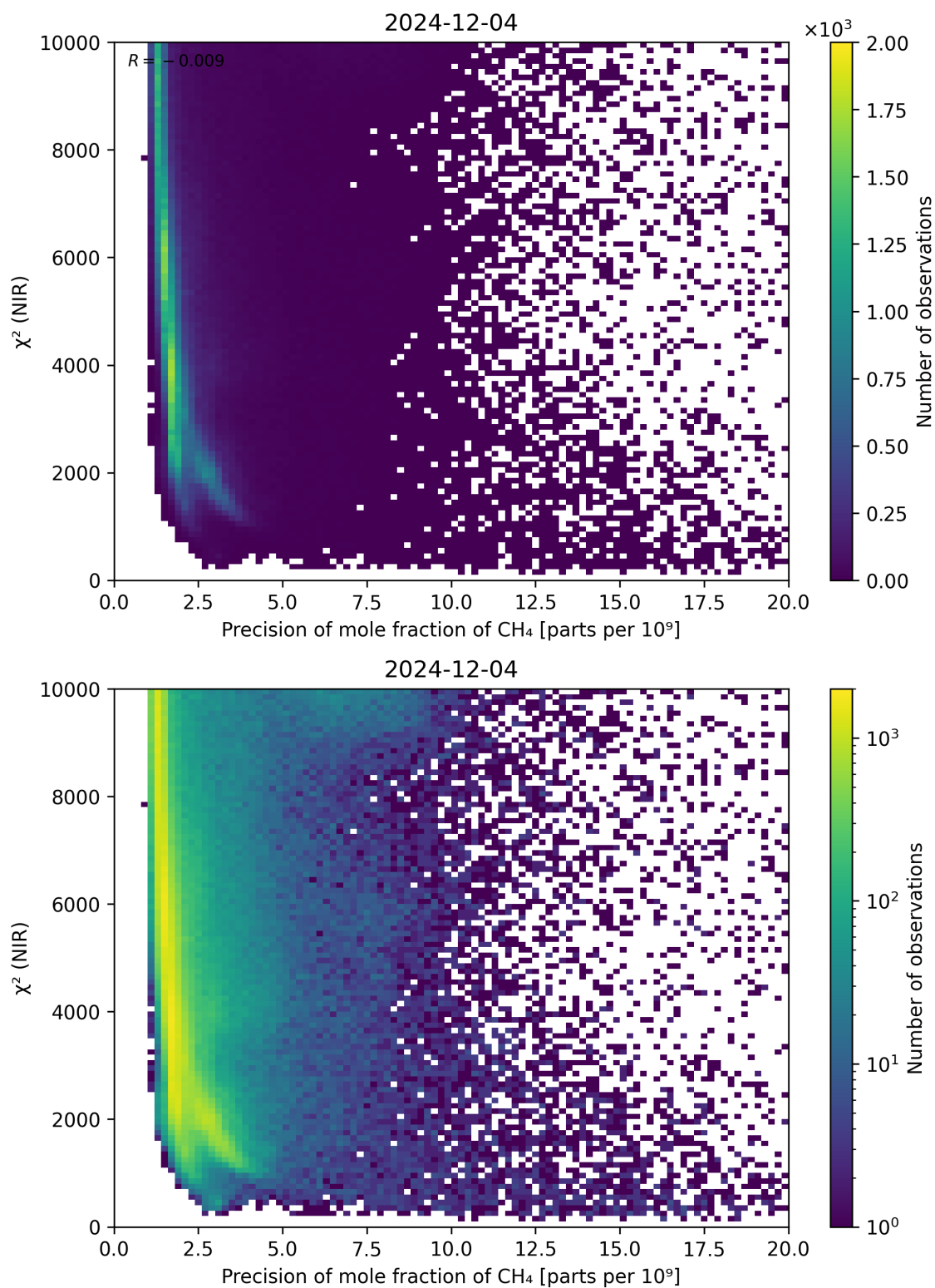
Figure 78: Scatter density plot of “Precision of mole fraction of CH 4 ” against “ \chi^2 (NIR)” for 2024-12-03 to 2024-12-05.
