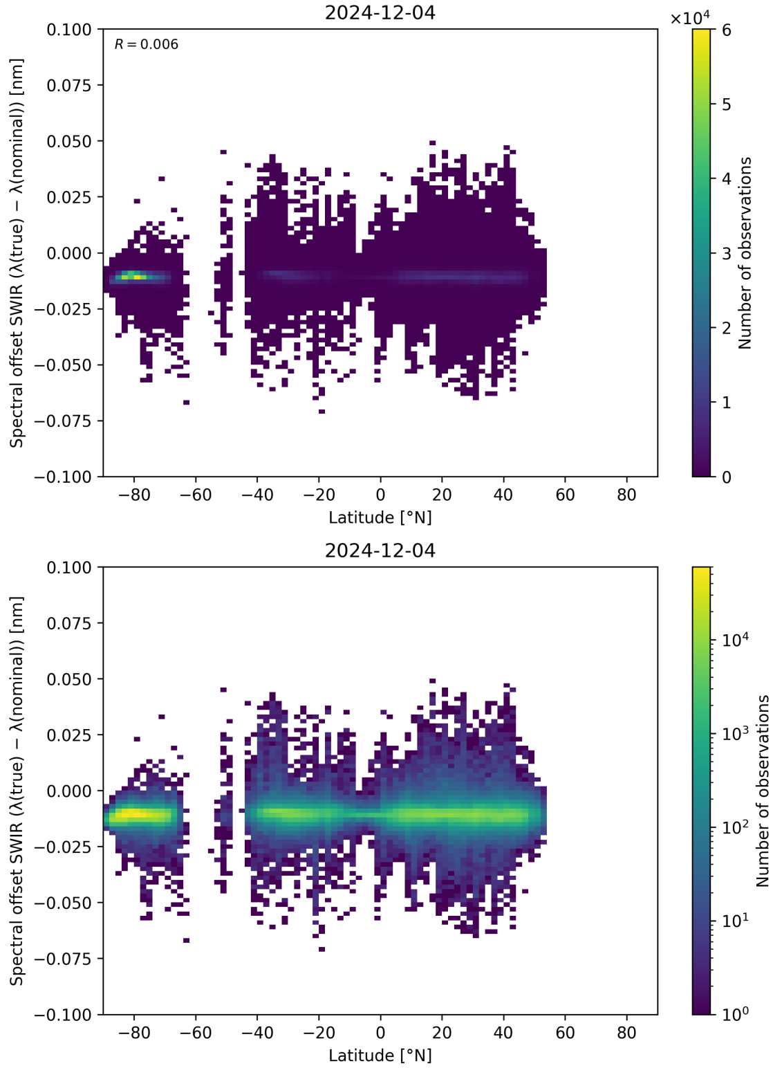
Figure 62: Scatter density plot of “Latitude” against “Spectral offset SWIR ( \lambda_{\text{true}} - \lambda_{\text{nominal}} )” for 2024-12-03 to 2024-12-05.
