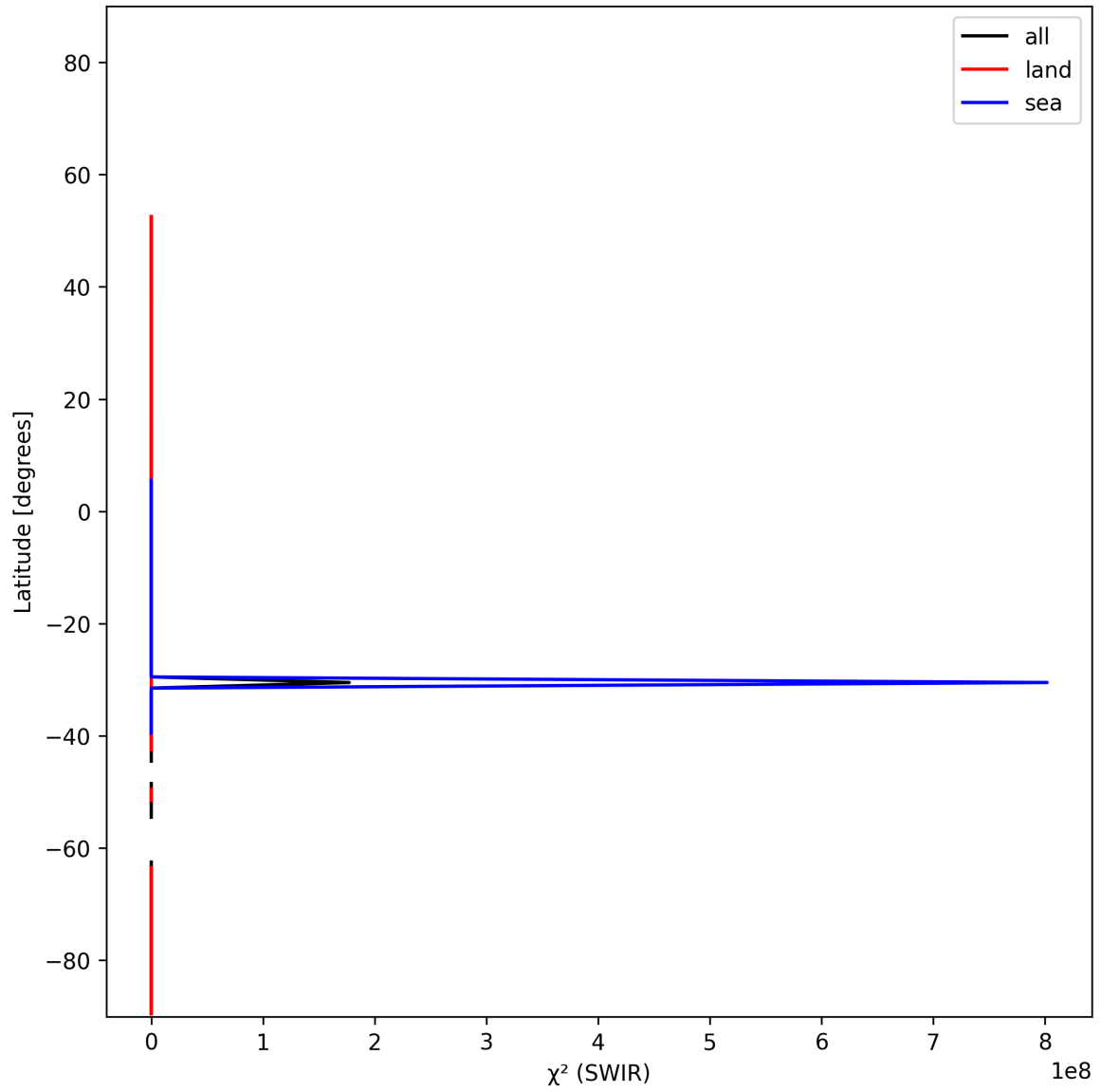
Figure 17: Zonal average of “ \chi^2 (SWIR)” for 2024-12-03 to 2024-12-05.
