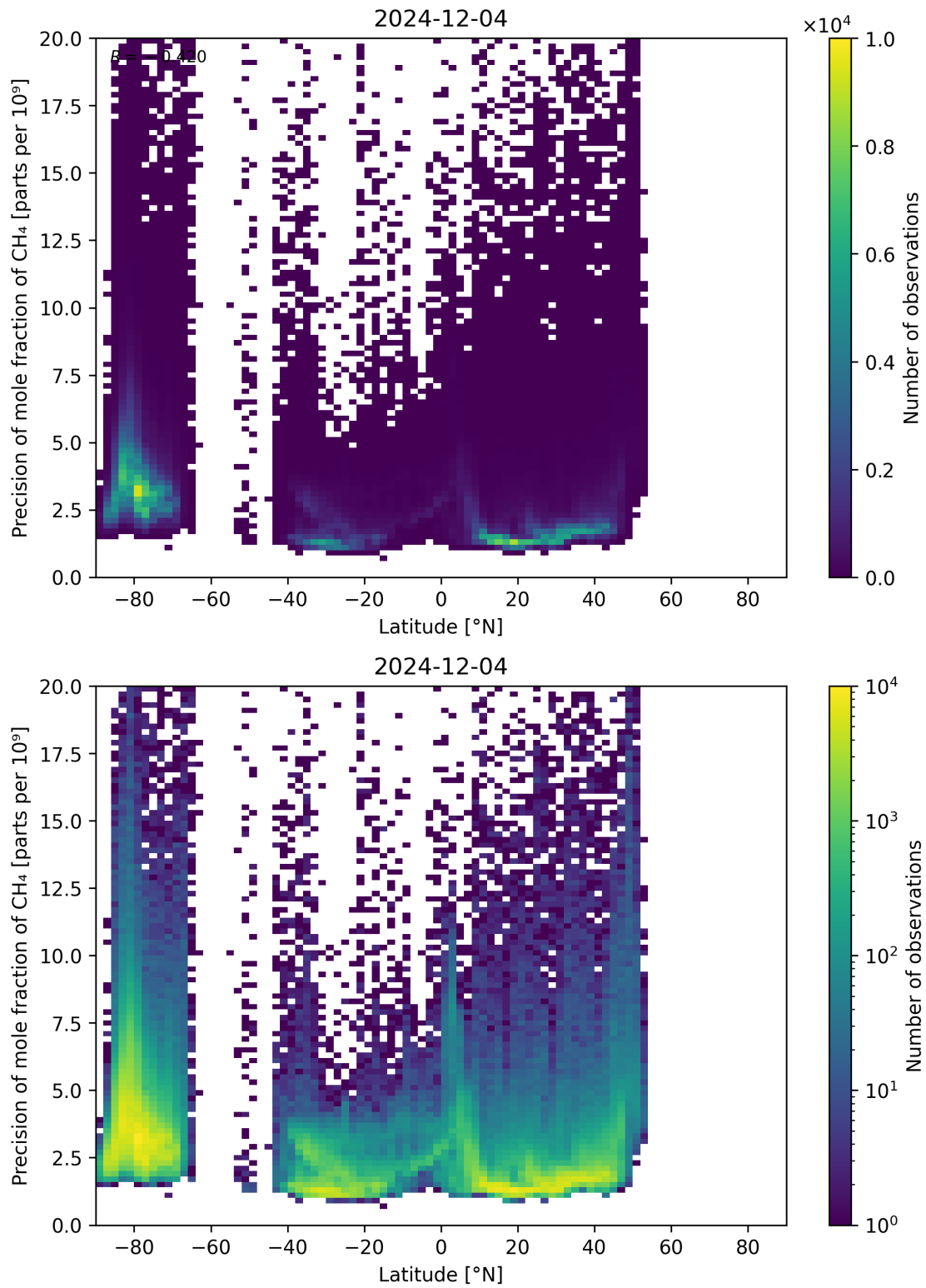
Figure 59: Scatter density plot of “Latitude” against “Precision of mole fraction of CH 4 ” for 2024-12-03 to 2024-12-05.
