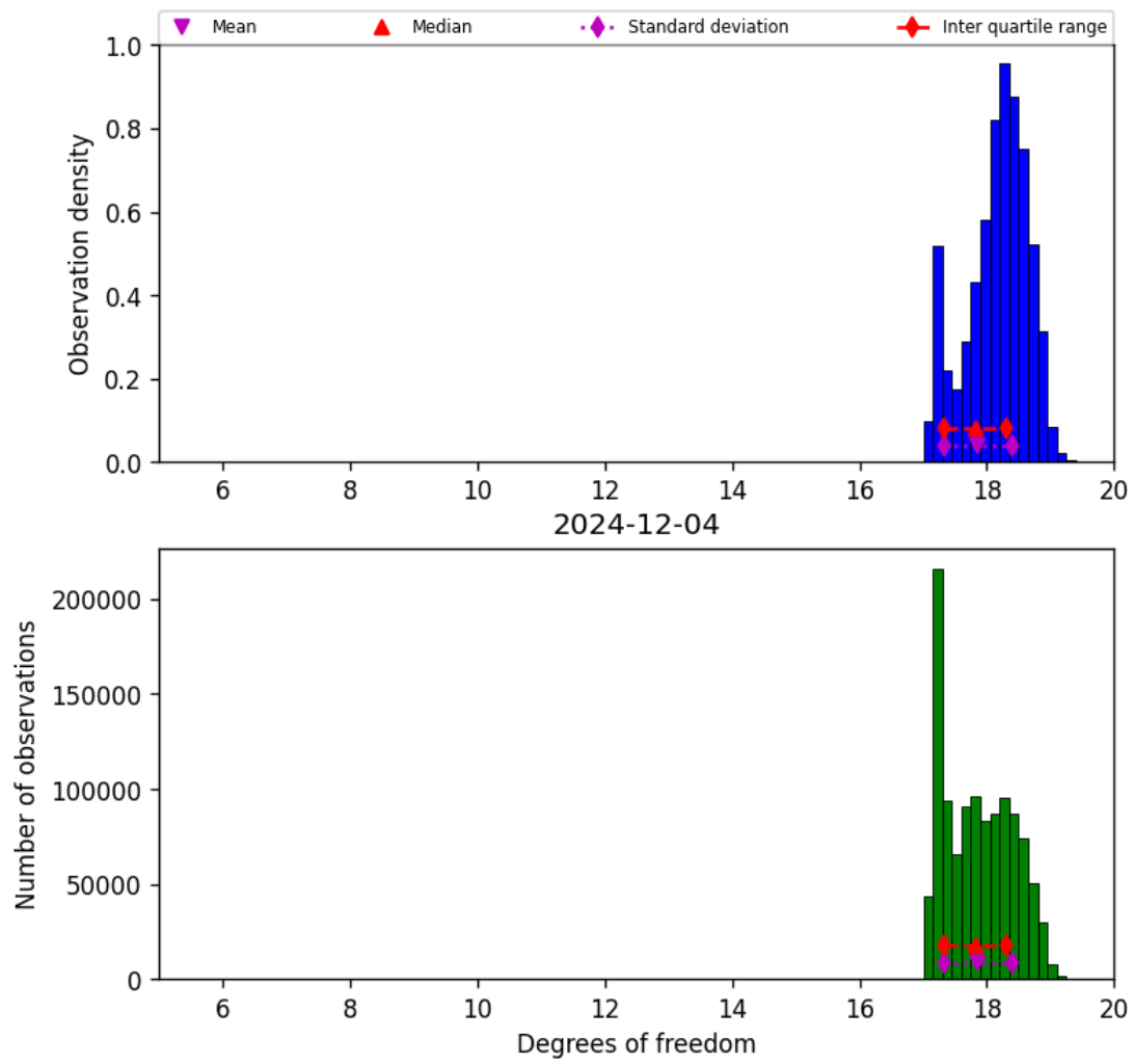
Figure 30: Histogram of “Degrees of freedom” for 2024-12-03 to 2024-12-05
