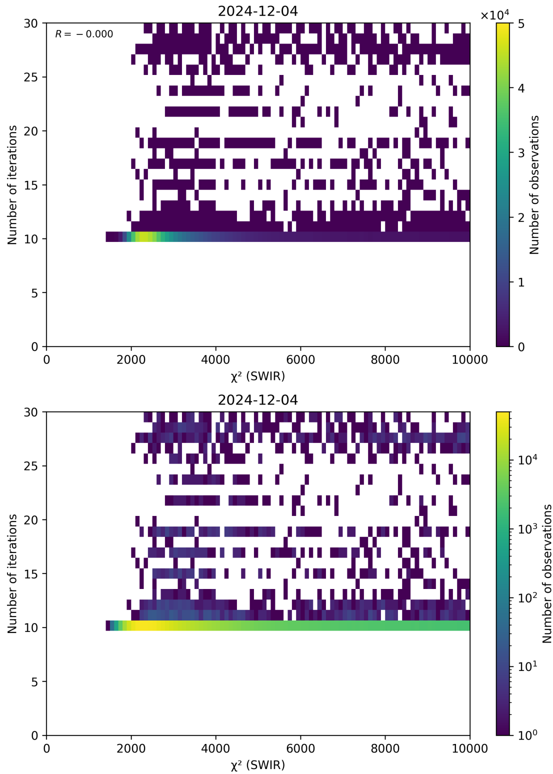
Figure 50: Scatter density plot of “ \chi^2 (SWIR)” against “Number of iterations” for 2024-12-03 to 2024-12-05.
