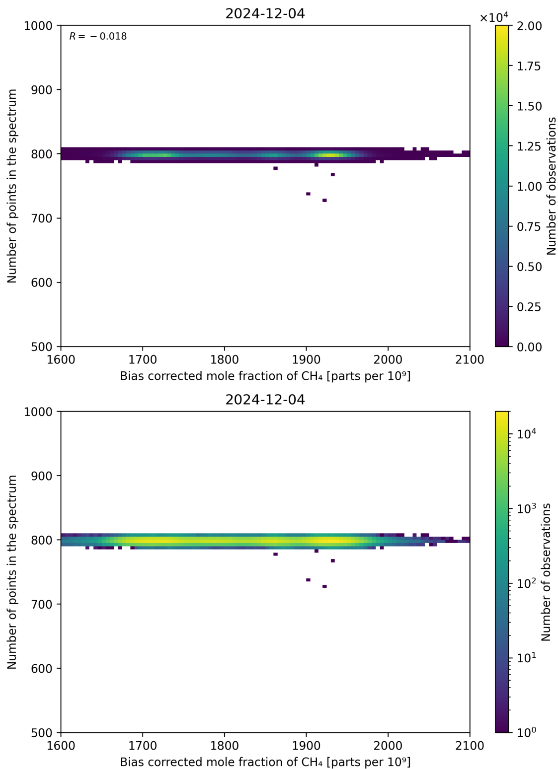
Figure 68: Scatter density plot of “Bias corrected mole fraction of CH 4 ” against “Number of points in the spectrum” for 2024-12-03 to 2024-12-05.
