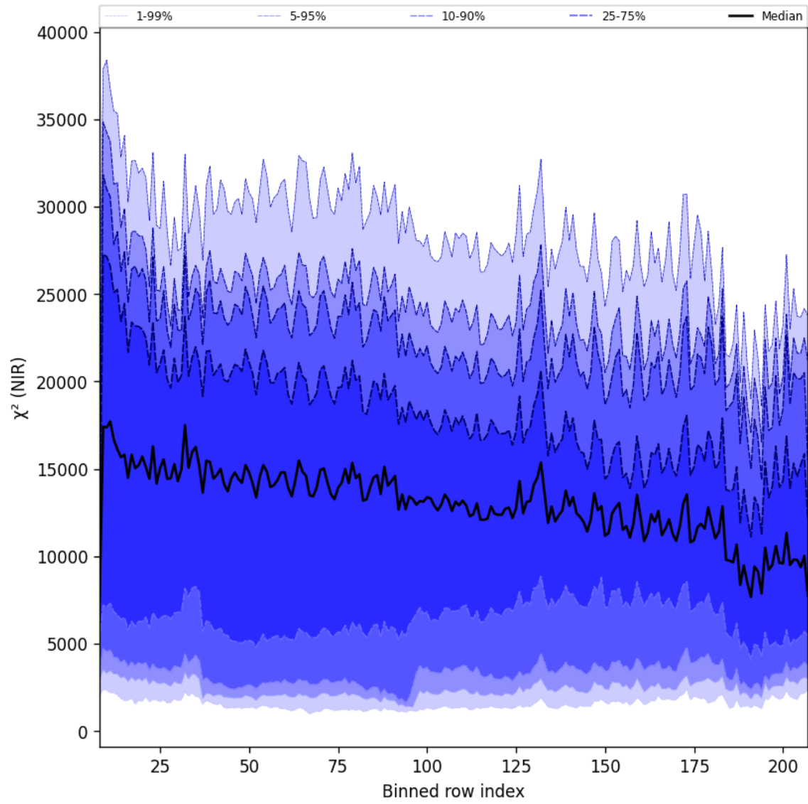
Figure 40: Along track statistics of “ \chi^2 (NIR)” for 2024-12-03 to 2024-12-05
