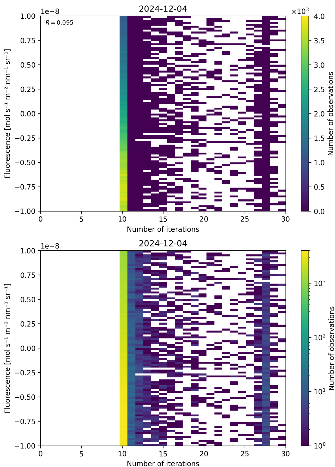
Figure 87: Scatter density plot of “Number of iterations” against “Fluorescence” for 2024-12-03 to 2024-12-05.
