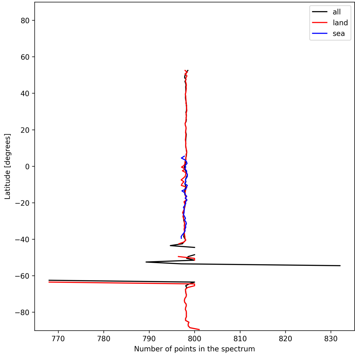
Figure 15: Zonal average of “Number of points in the spectrum” for 2024-12-03 to 2024-12-05.
