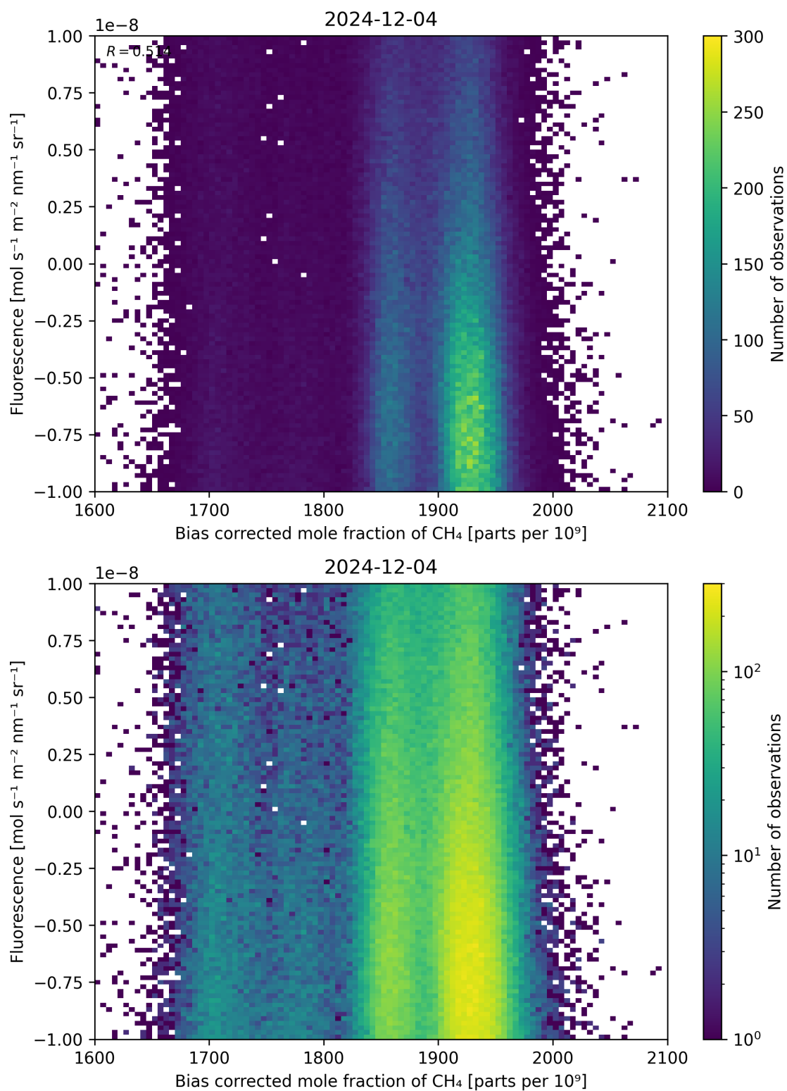
Figure 66: Scatter density plot of “Bias corrected mole fraction of \text{CH}_4 ” against “Fluorescence” for 2024-12-03 to 2024-12-05.
