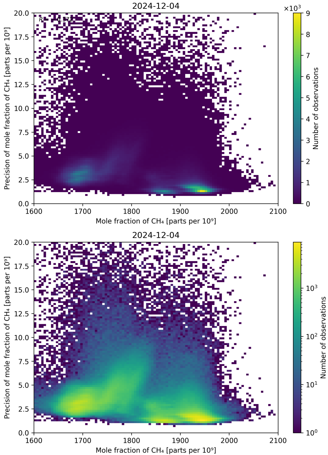
Figure 75: Scatter density plot of “Mole fraction of CH 4 ” against “Precision of mole fraction of CH 4 ” for 2024-12-03 to 2024-12-05.
