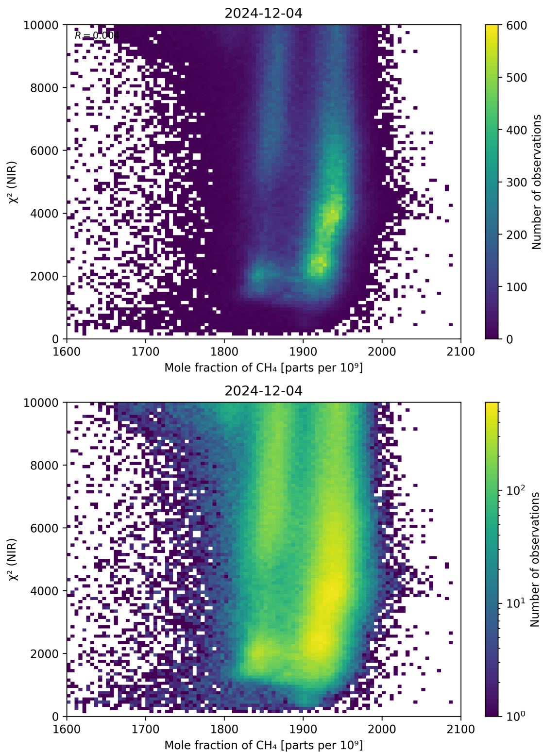
Figure 70: Scatter density plot of “Mole fraction of \text{CH}_4 ” against “ \chi^2 (NIR)” for 2024-12-03 to 2024-12-05.
