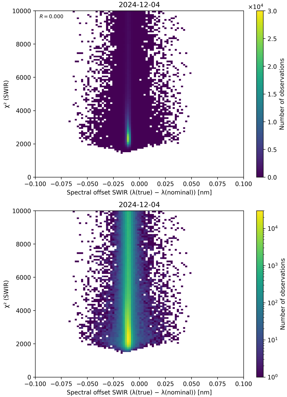
Figure 118: Scatter density plot of “Spectral offset SWIR ( \lambda_{\text{true}} - \lambda_{\text{nominal}} )” against “ \chi^2 (SWIR)” for 2024-12-03 to 2024-12-05.
