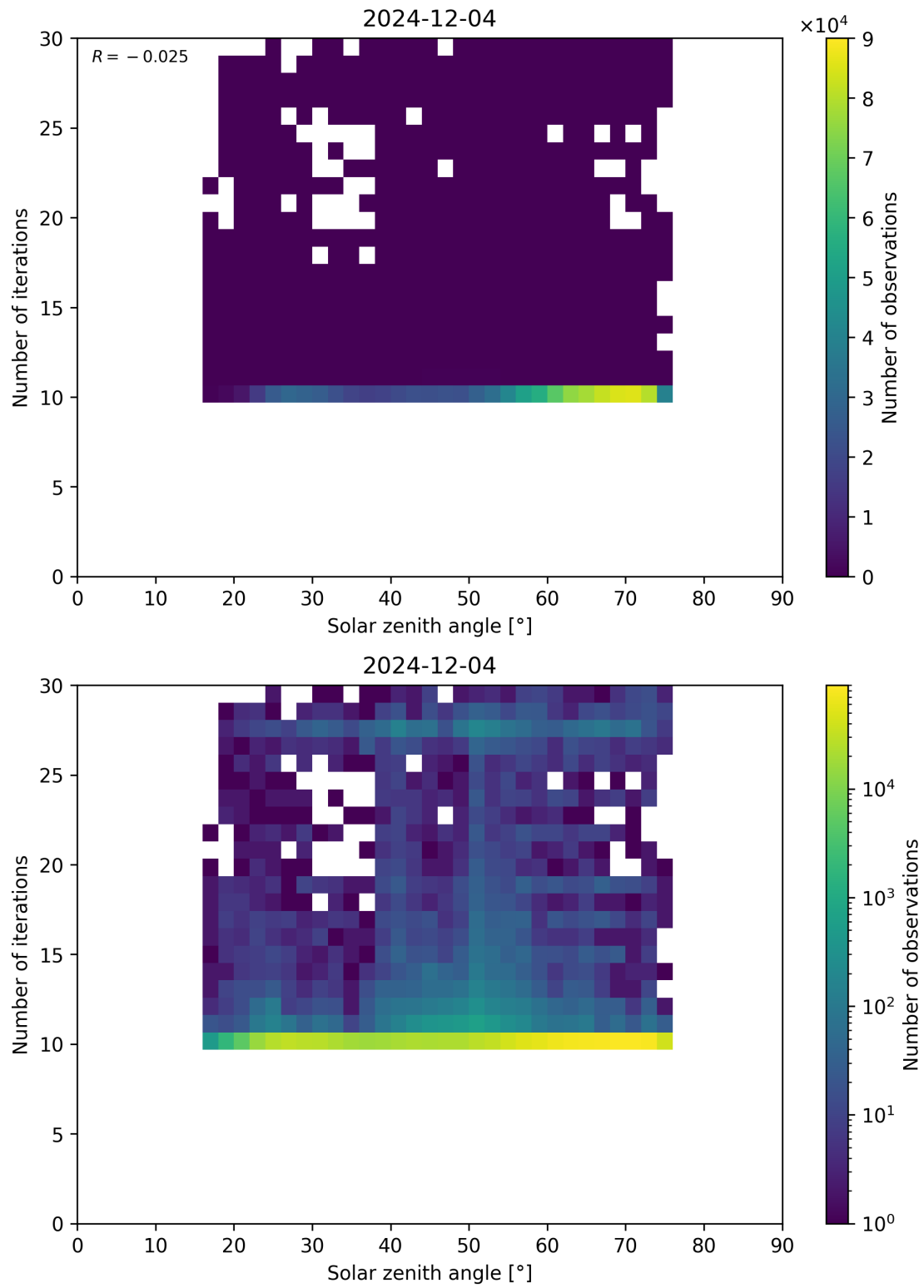
Figure 102: Scatter density plot of “Solar zenith angle” against “Number of iterations” for 2024-12-03 to 2024-12-05.
