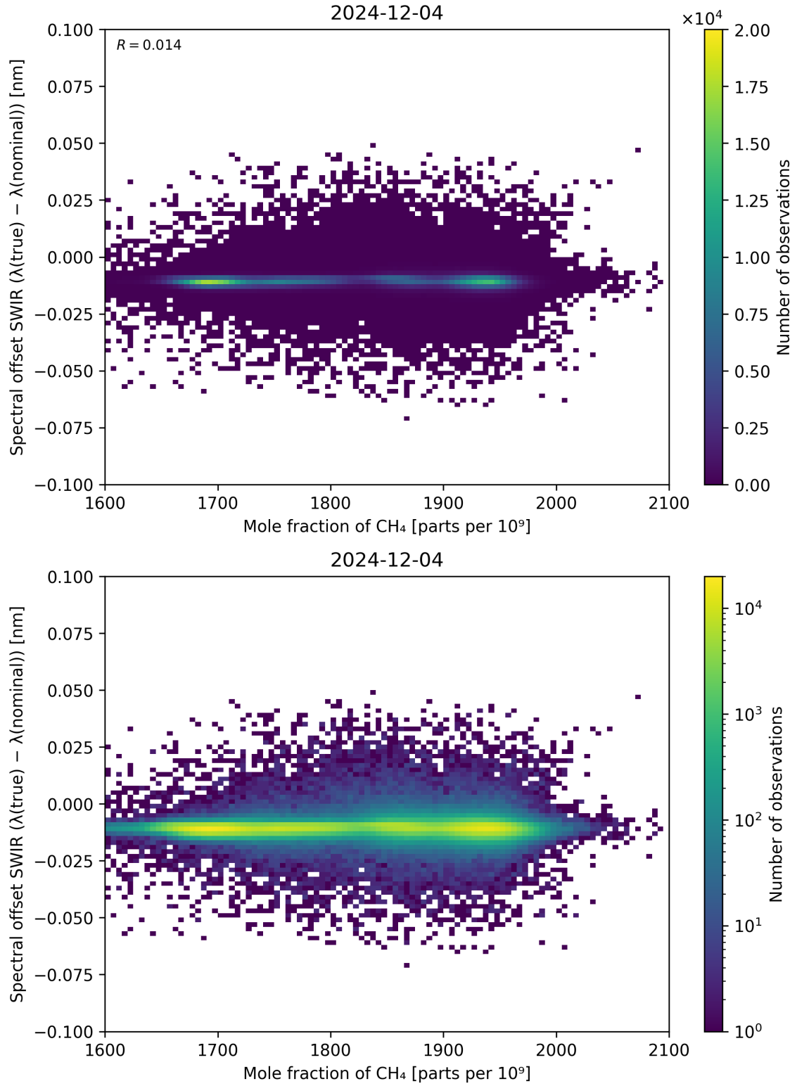
Figure 86: Scatter density plot of “Mole fraction of CH 4 ” against “Spectral offset SWIR ( \lambda_{\text{true}} - \lambda_{\text{nominal}} )” for 2024-12-03 to 2024-12-05.
