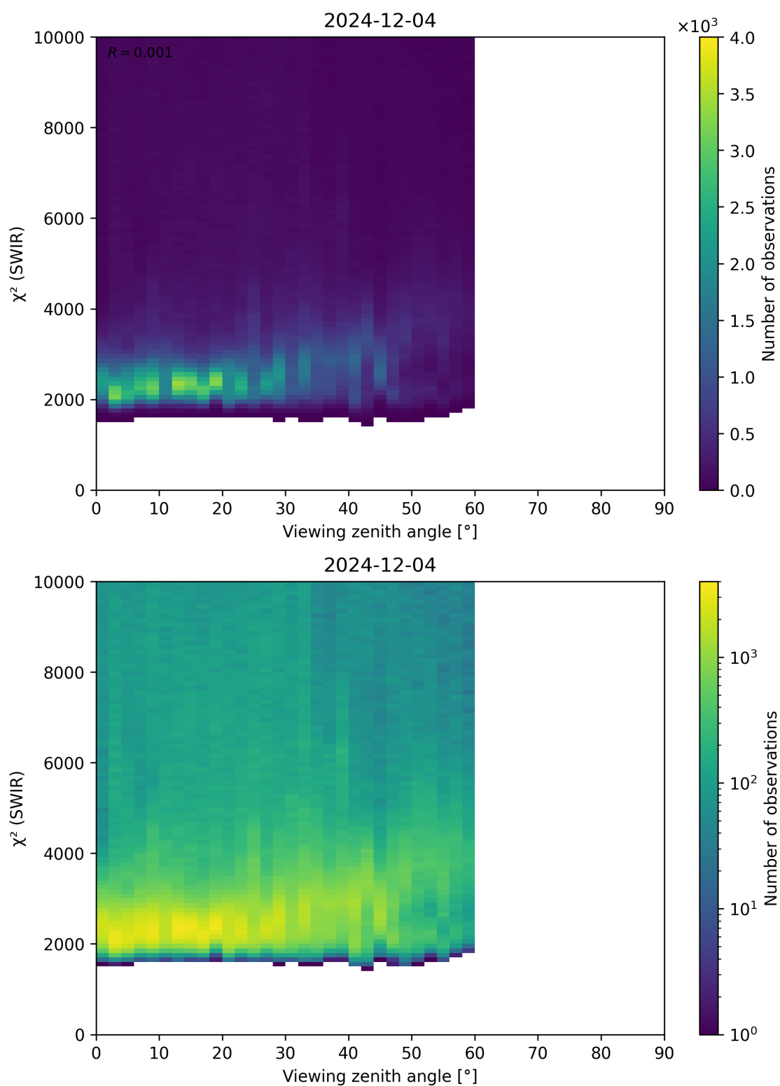
Figure 106: Scatter density plot of “Viewing zenith angle” against “ \chi^2 (SWIR)” for 2024-12-03 to 2024-12-05.
