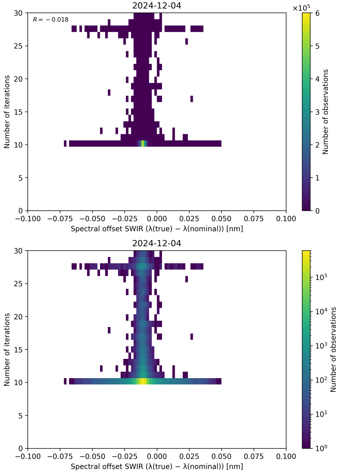
Figure 121: Scatter density plot of “Spectral offset SWIR ( \lambda_{\text{true}} - \lambda_{\text{nominal}} )” against “Number of iterations” for 2024-12-03 to 2024-12-05.
