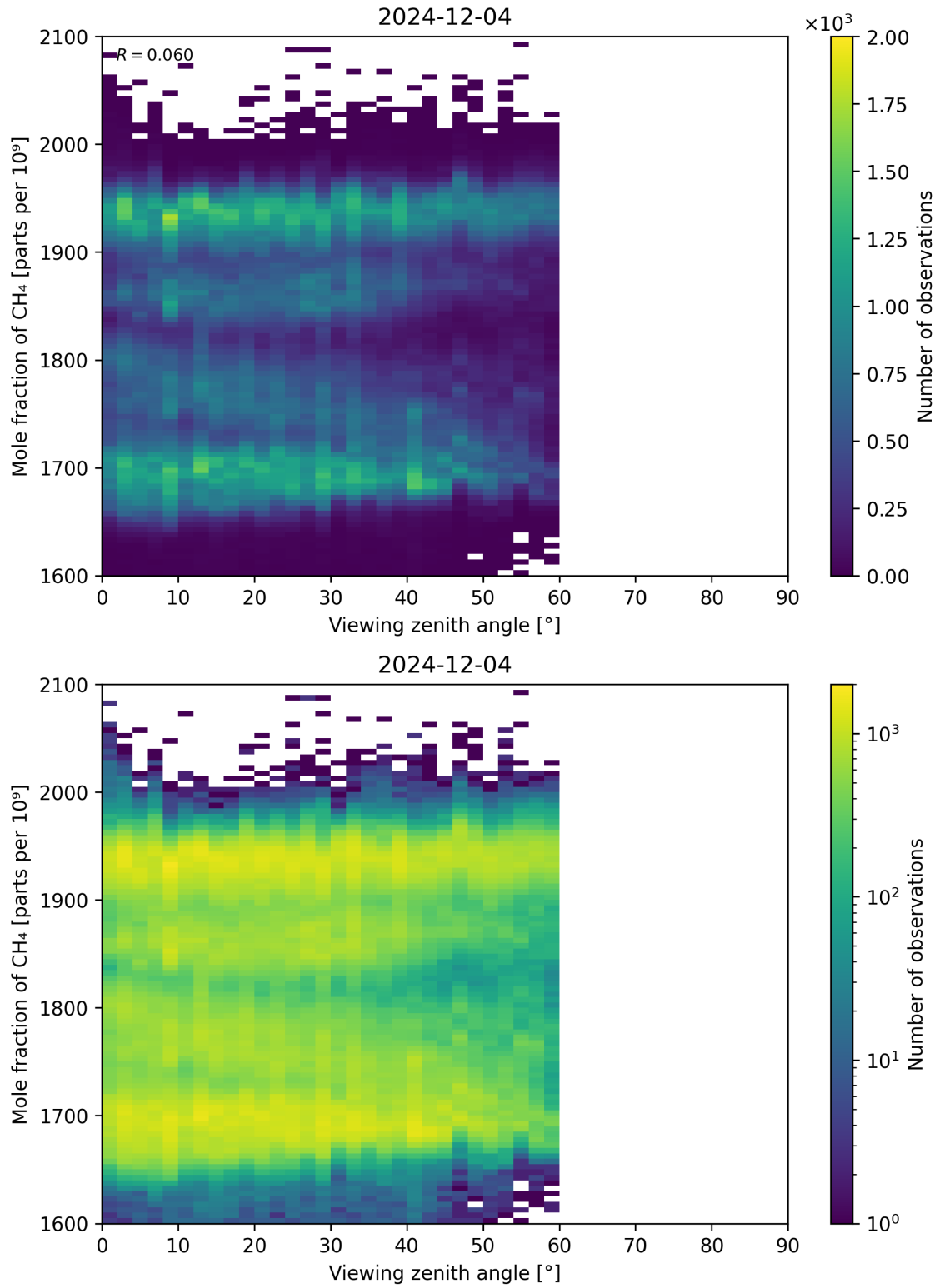
Figure 110: Scatter density plot of “Viewing zenith angle” against “Mole fraction of CH 4 ” for 2024-12-03 to 2024-12-05.
