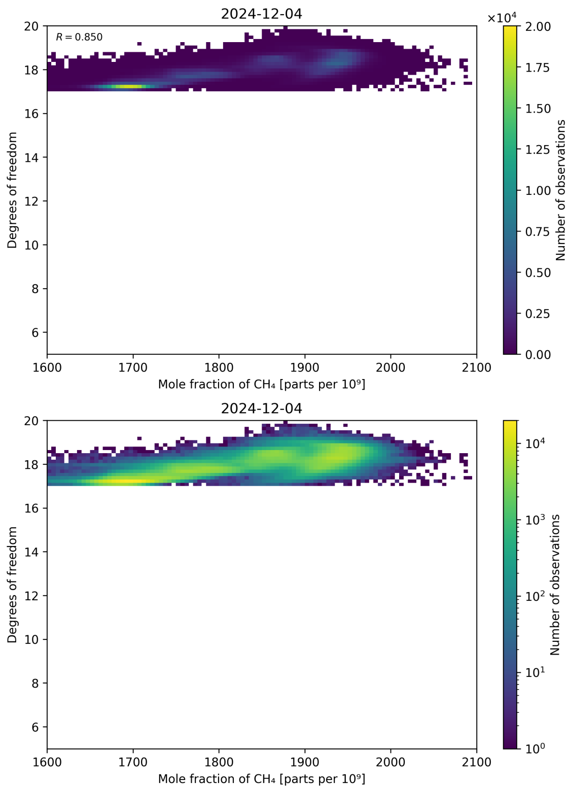
Figure 72: Scatter density plot of “Mole fraction of CH 4 ” against “Degrees of freedom” for 2024-12-03 to 2024-12-05.
