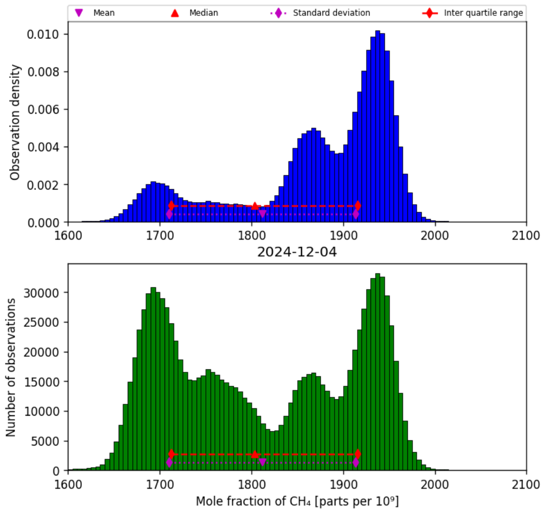
Figure 23: Histogram of “Mole fraction of CH 4 ” for 2024-12-03 to 2024-12-05
