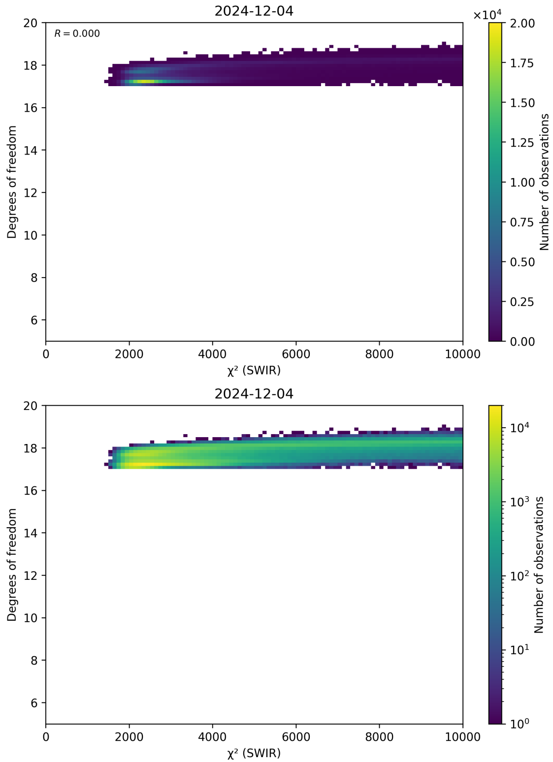
Figure 48: Scatter density plot of “ \chi^2 (SWIR)” against “Degrees of freedom” for 2024-12-03 to 2024-12-05.
