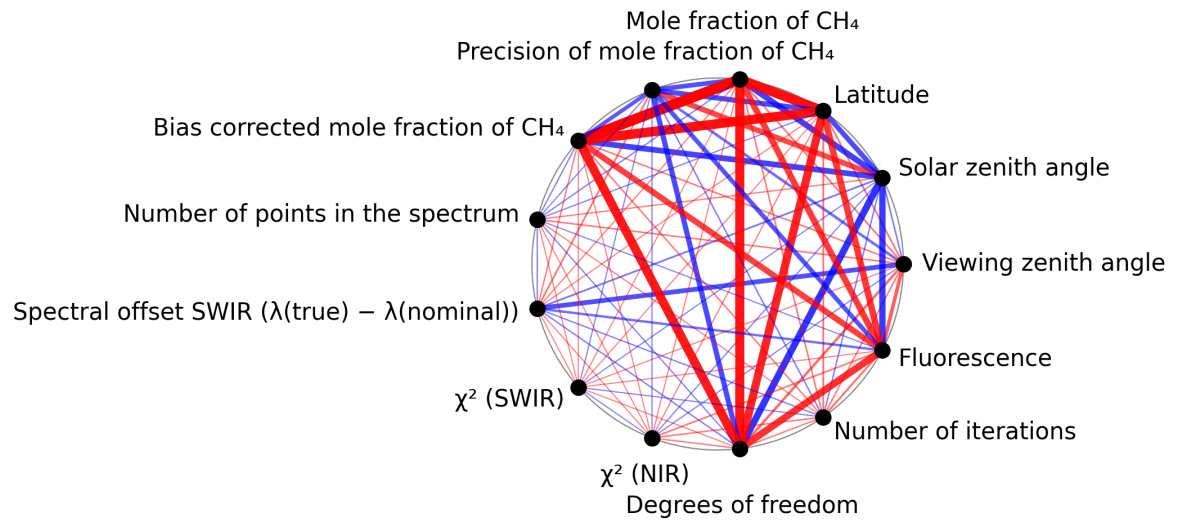
Figure 1: Map of correlation graph for 2024-12-03 to 2024-12-05.
