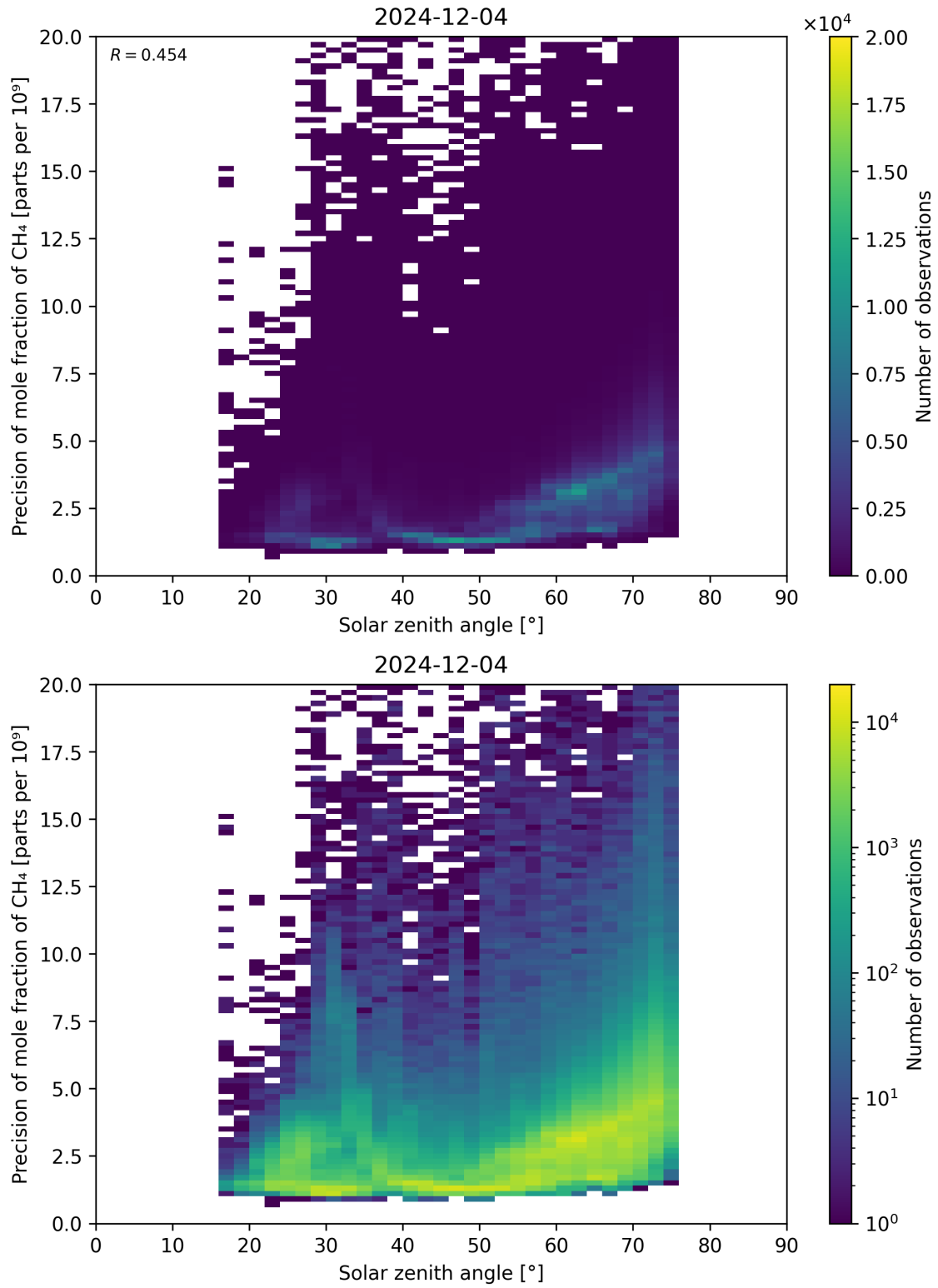
Figure 101: Scatter density plot of “Solar zenith angle” against “Precision of mole fraction of \text{CH}_4 ” for 2024-12-03 to 2024-12-05.
