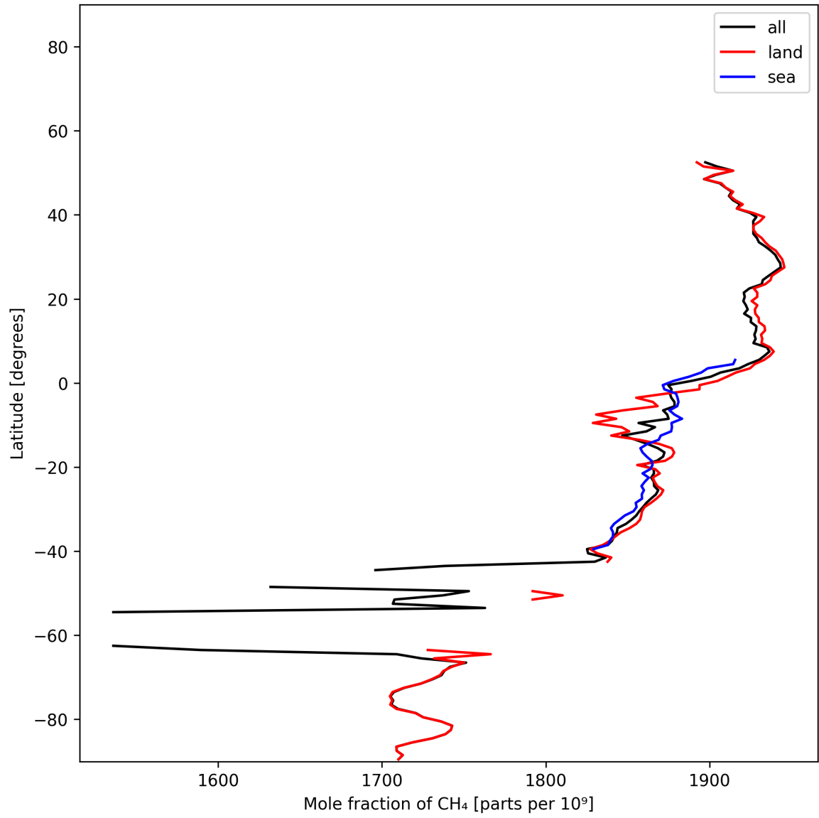
Figure 12: Zonal average of “Mole fraction of \text{CH}_4 ” for 2024-12-03 to 2024-12-05.
