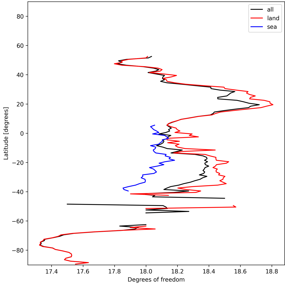
Figure 19: Zonal average of “Degrees of freedom” for 2024-12-03 to 2024-12-05.
