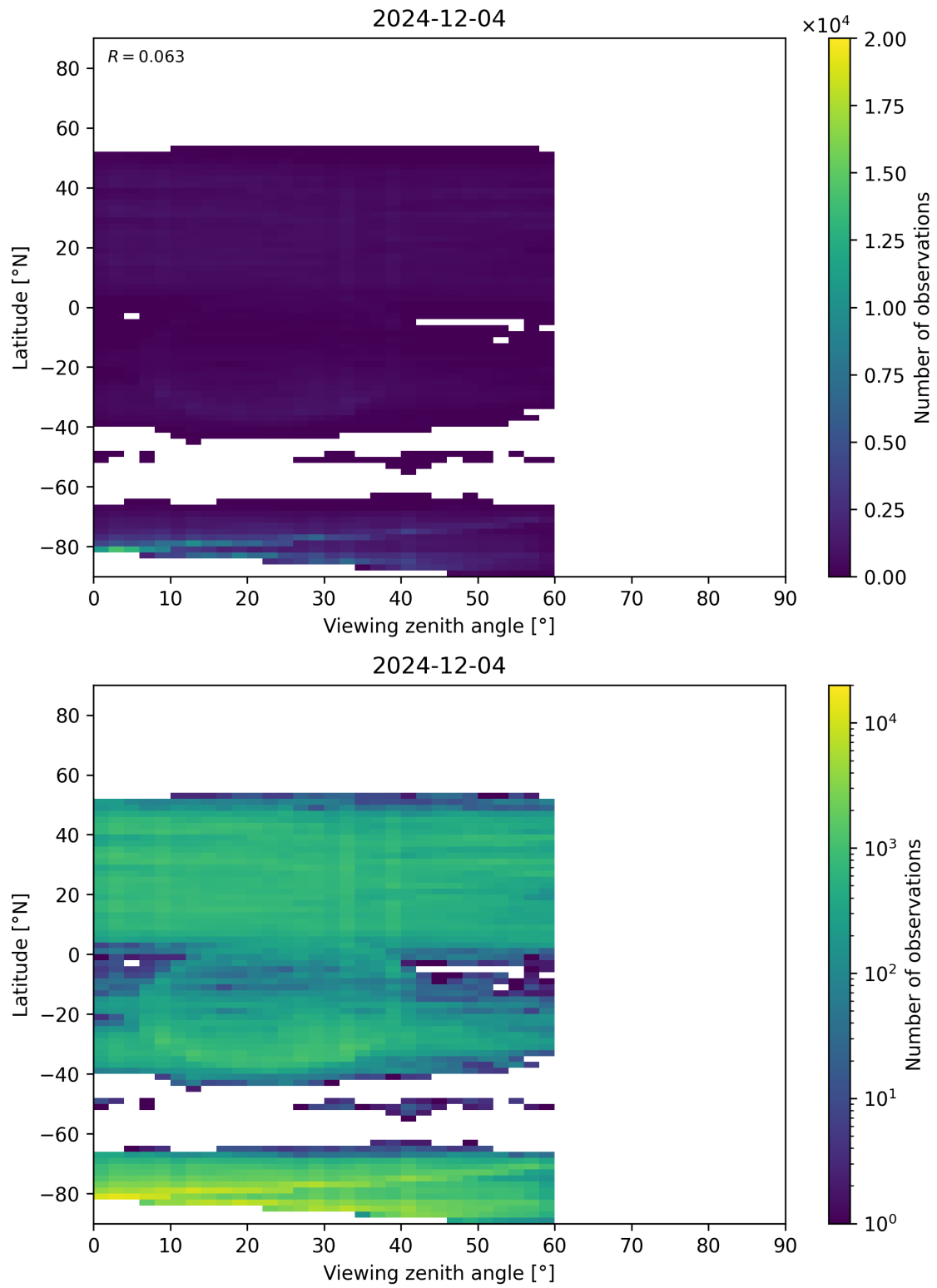
Figure 109: Scatter density plot of “Viewing zenith angle” against “Latitude” for 2024-12-03 to 2024-12-05.
