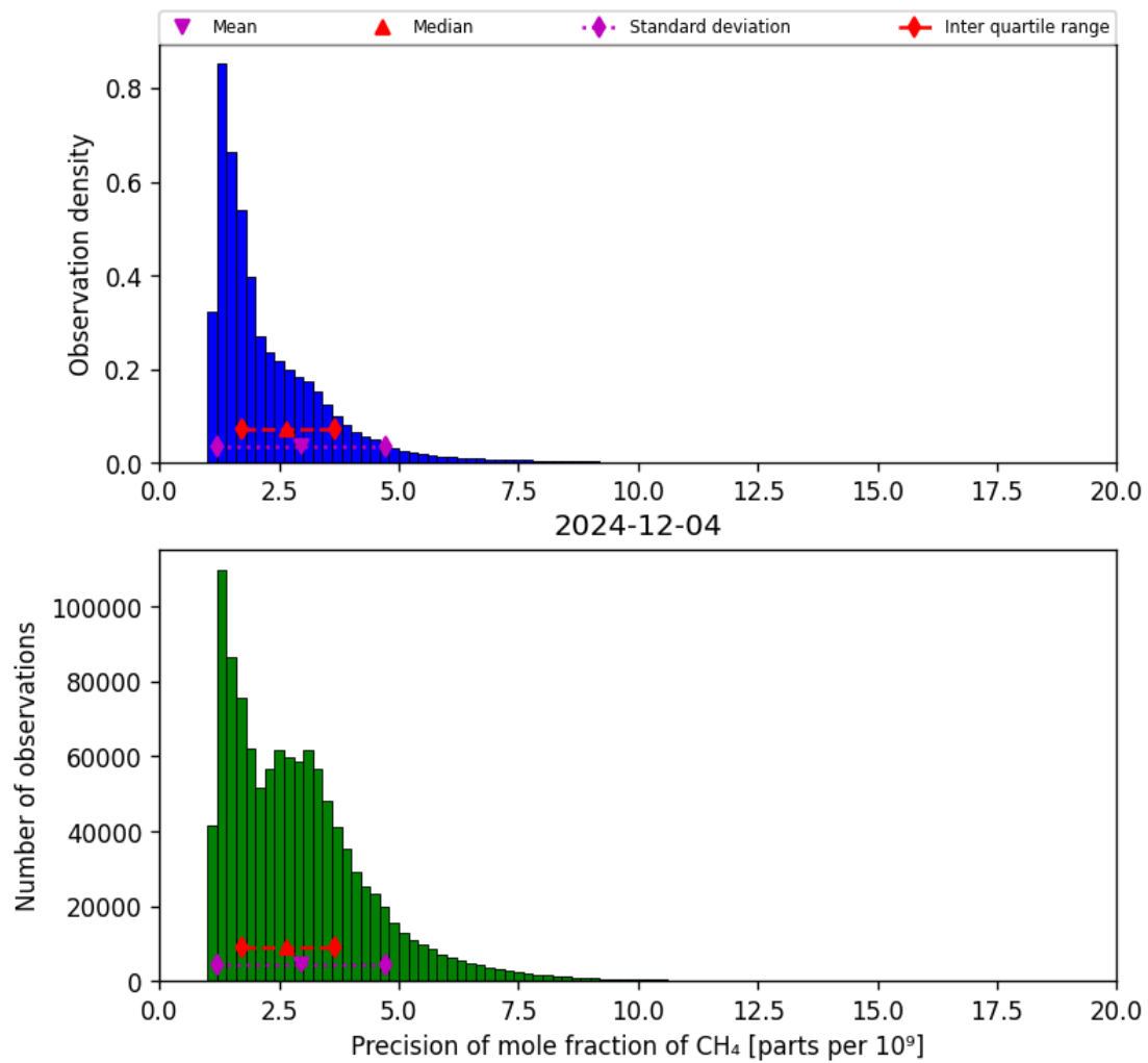
Figure 24: Histogram of “Precision of mole fraction of CH 4 ” for 2024-12-03 to 2024-12-05
