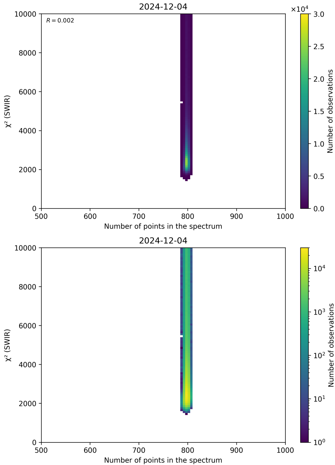
Figure 89: Scatter density plot of “Number of points in the spectrum” against “ \chi^2 (SWIR)” for 2024-12-03 to 2024-12-05.
