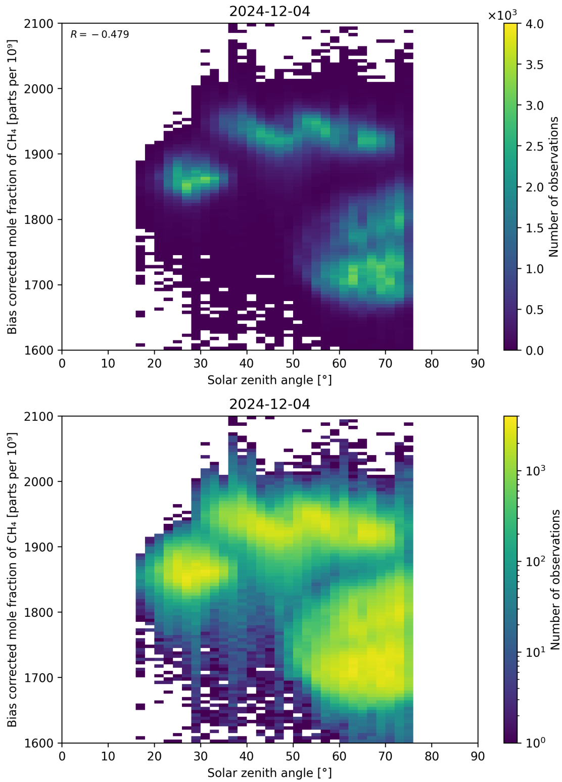
Figure 100: Scatter density plot of “Solar zenith angle” against “Bias corrected mole fraction of CH 4 ” for 2024-12-03 to 2024-12-05.
