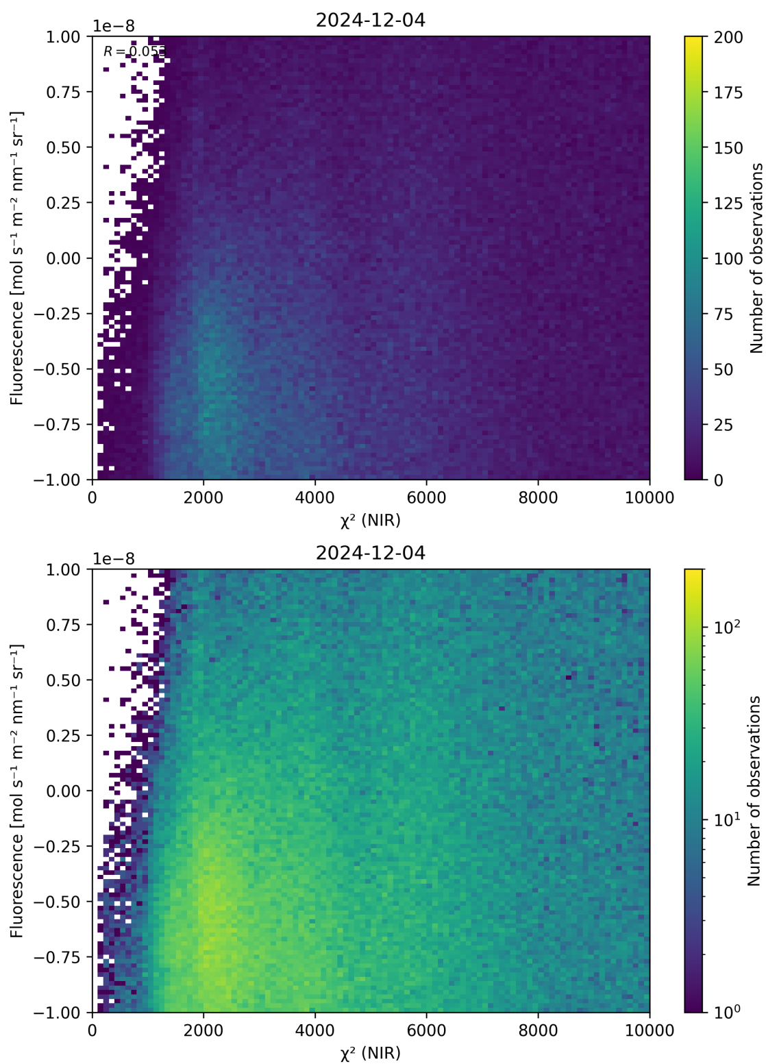
Figure 45: Scatter density plot of “ \chi^2 (NIR)” against “Fluorescence” for 2024-12-03 to 2024-12-05.
