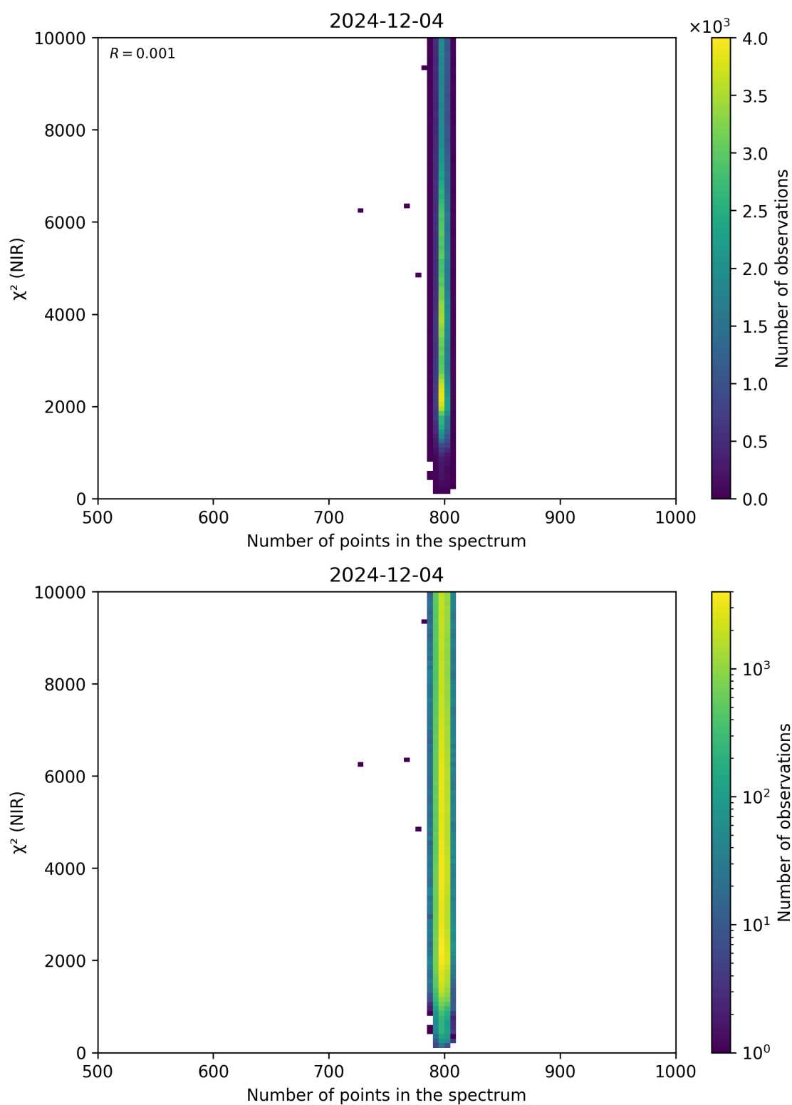
Figure 88: Scatter density plot of “Number of points in the spectrum” against “ \chi^2 (NIR)” for 2024-12-03 to 2024-12-05.
