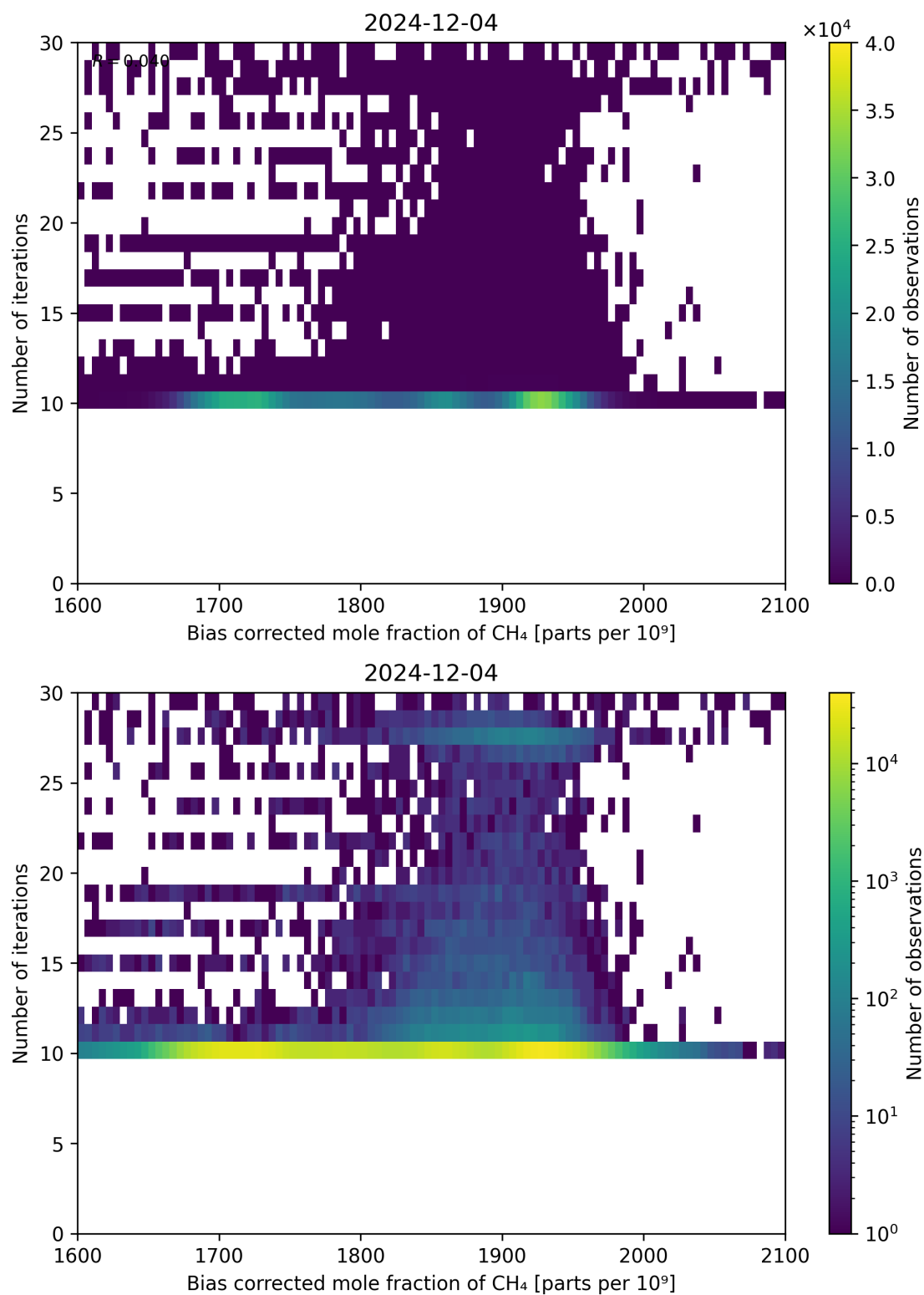
Figure 67: Scatter density plot of “Bias corrected mole fraction of \text{CH}_4 ” against “Number of iterations” for 2024-12-03 to 2024-12-05.
