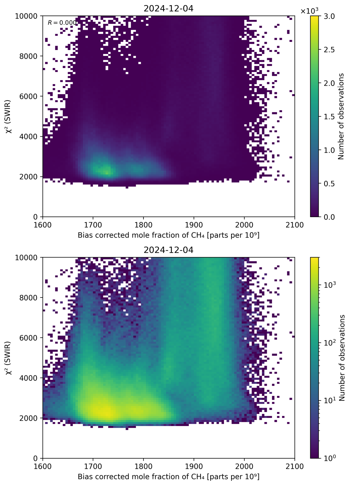
Figure 64: Scatter density plot of “Bias corrected mole fraction of \text{CH}_4 ” against “ \chi^2 (SWIR)” for 2024-12-03 to 2024-12-05.
