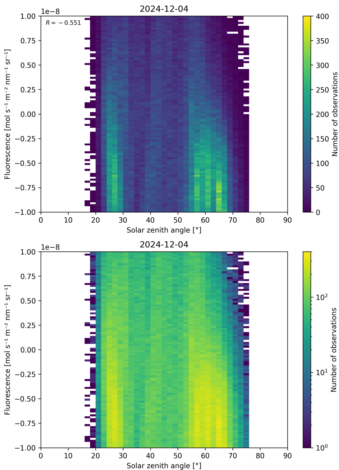
Figure 97: Scatter density plot of “Solar zenith angle” against “Fluorescence” for 2024-12-03 to 2024-12-05.
