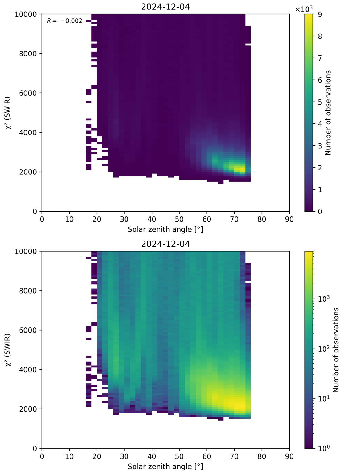
Figure 95: Scatter density plot of “Solar zenith angle” against “ \chi^2 (SWIR)” for 2024-12-03 to 2024-12-05.
