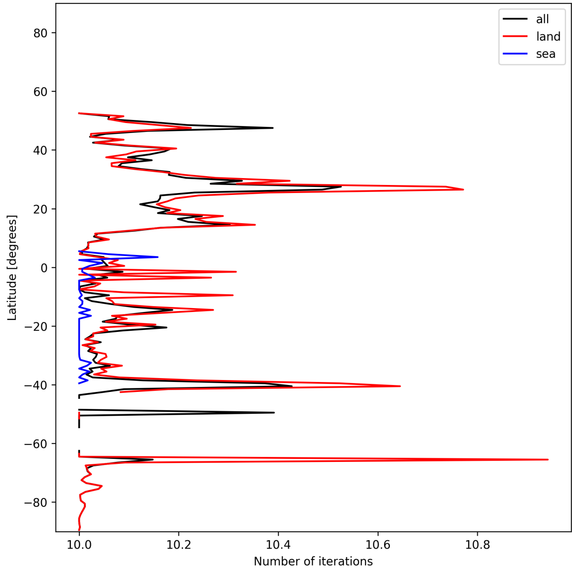
Figure 20: Zonal average of “Number of iterations” for 2024-12-03 to 2024-12-05.
