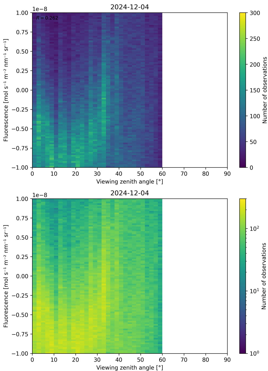
Figure 108: Scatter density plot of “Viewing zenith angle” against “Fluorescence” for 2024-12-03 to 2024-12-05.
