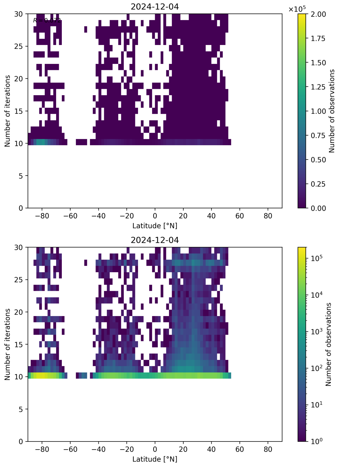
Figure 60: Scatter density plot of “Latitude” against “Number of iterations” for 2024-12-03 to 2024-12-05.
