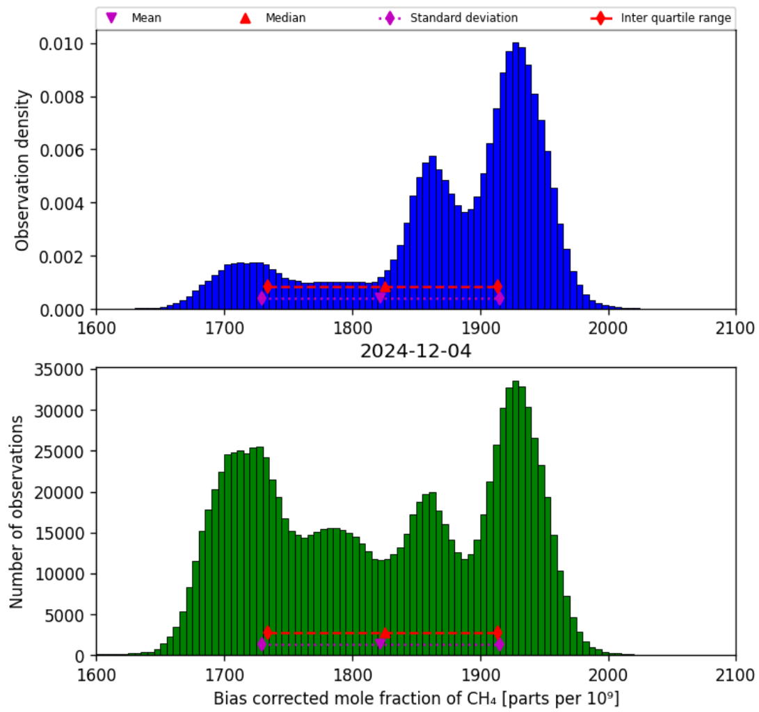
Figure 25: Histogram of “Bias corrected mole fraction of CH 4 ” for 2024-12-03 to 2024-12-05
