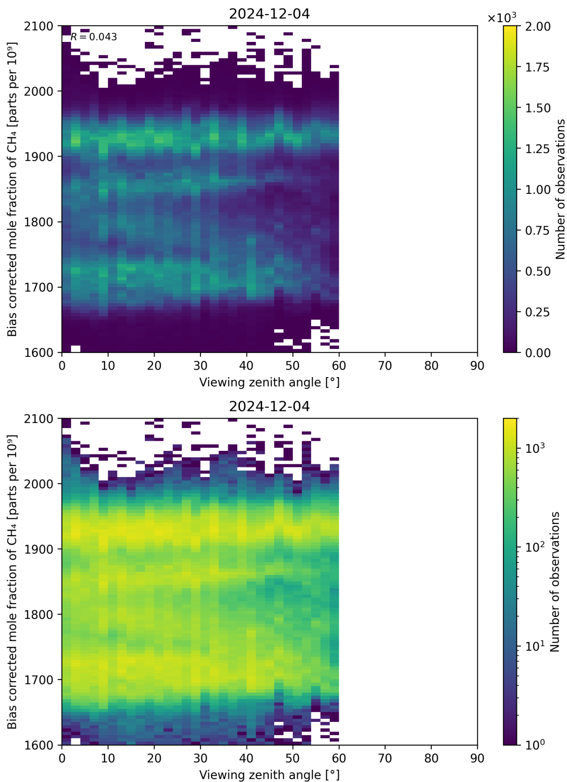
Figure 111: Scatter density plot of “Viewing zenith angle” against “Bias corrected mole fraction of CH 4 ” for 2024-12-03 to 2024-12-05.
