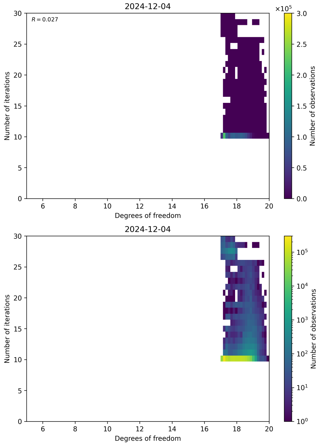
Figure 52: Scatter density plot of “Degrees of freedom” against “Number of iterations” for 2024-12-03 to 2024-12-05.
