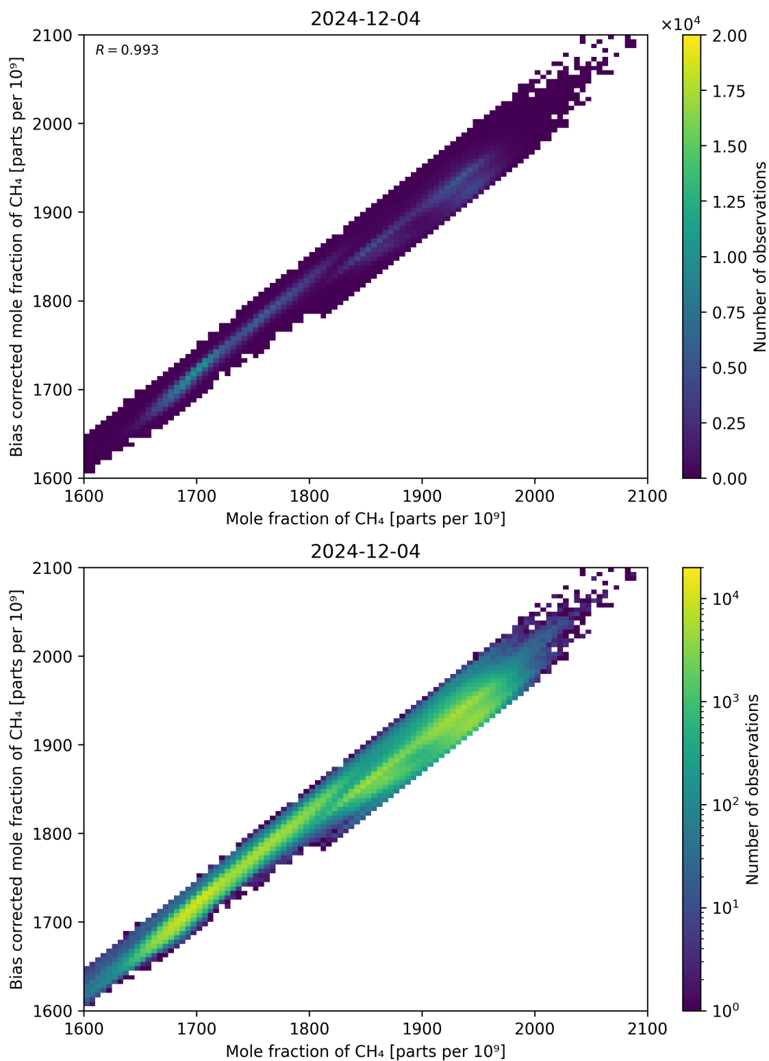
Figure 74: Scatter density plot of “Mole fraction of CH 4 ” against “Bias corrected mole fraction of CH 4 ” for 2024-12-03 to 2024-12-05.
