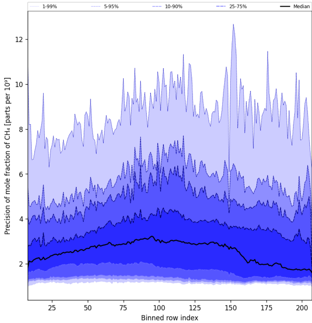
Figure 35: Along track statistics of “Precision of mole fraction of CH 4 ” for 2024-12-03 to 2024-12-05
