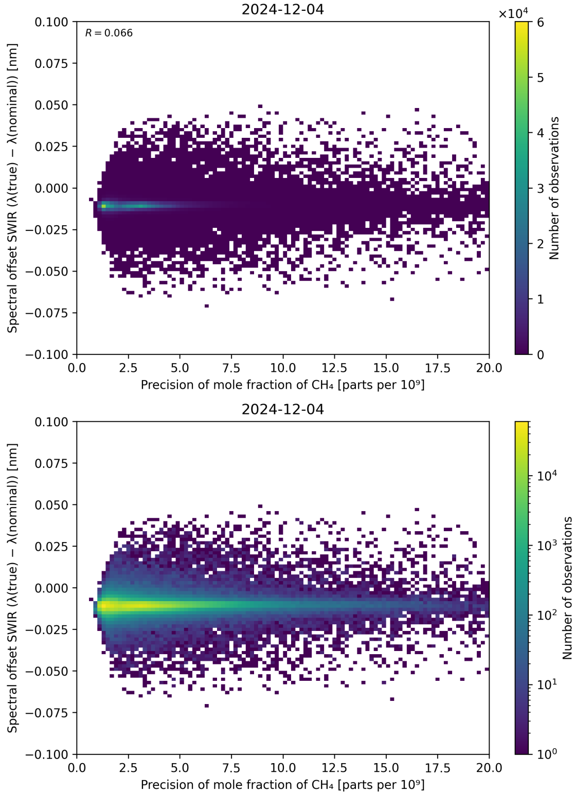
Figure 85: Scatter density plot of “Precision of mole fraction of CH 4 ” against “Spectral offset SWIR ( \lambda_{\text{true}} - \lambda_{\text{nominal}} )” for 2024-12-03 to 2024-12-05.
