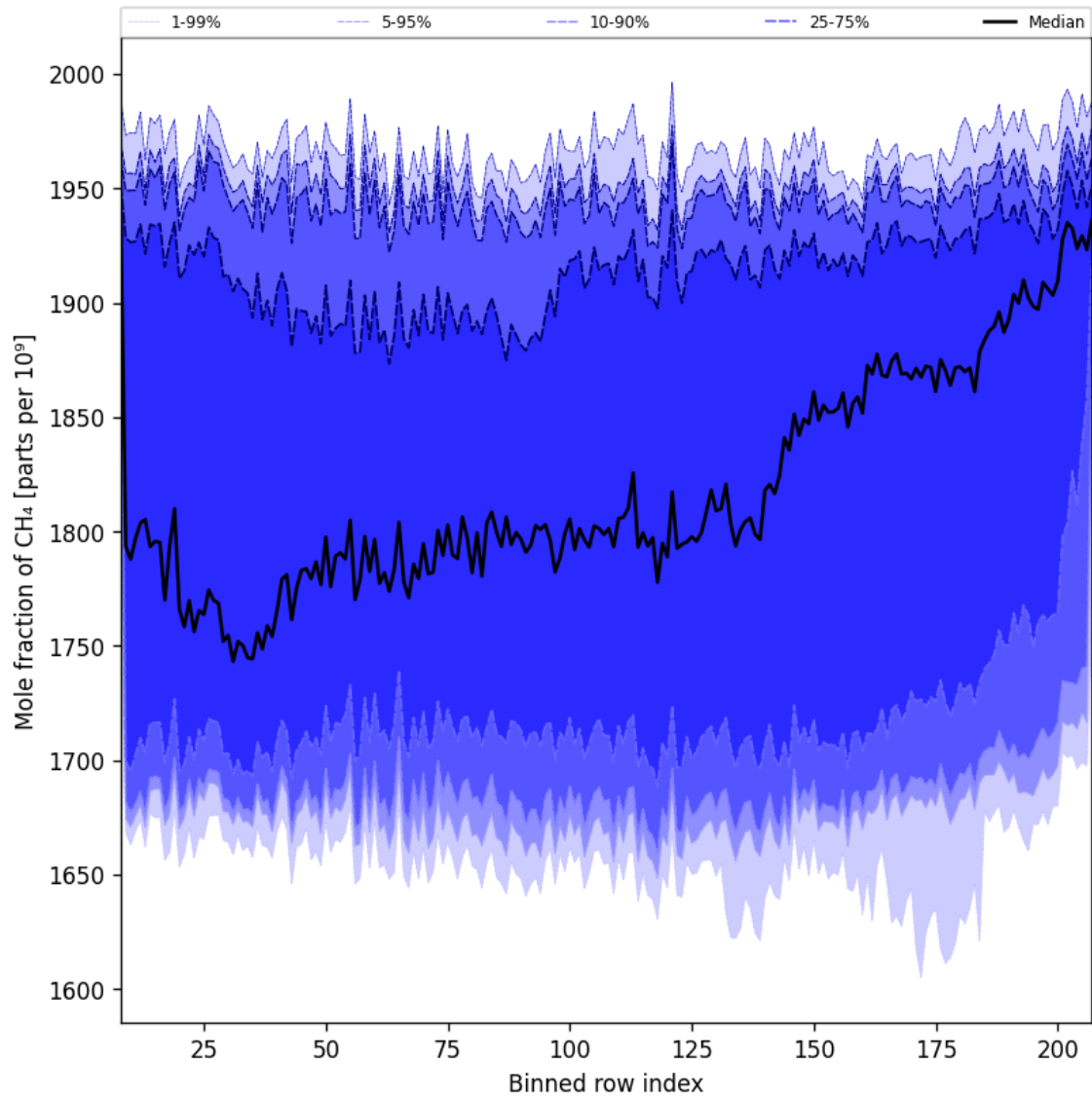
Figure 34: Along track statistics of “Mole fraction of CH 4 ” for 2024-12-03 to 2024-12-05
