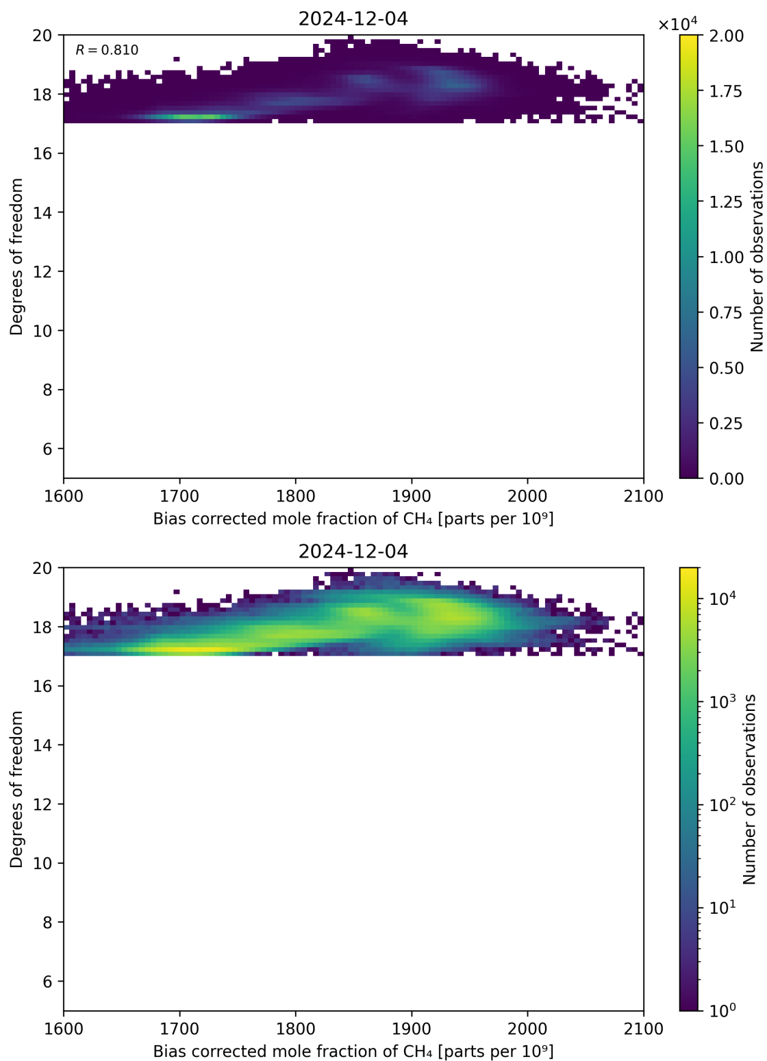
Figure 65: Scatter density plot of “Bias corrected mole fraction of CH 4 ” against “Degrees of freedom” for 2024-12-03 to 2024-12-05.
