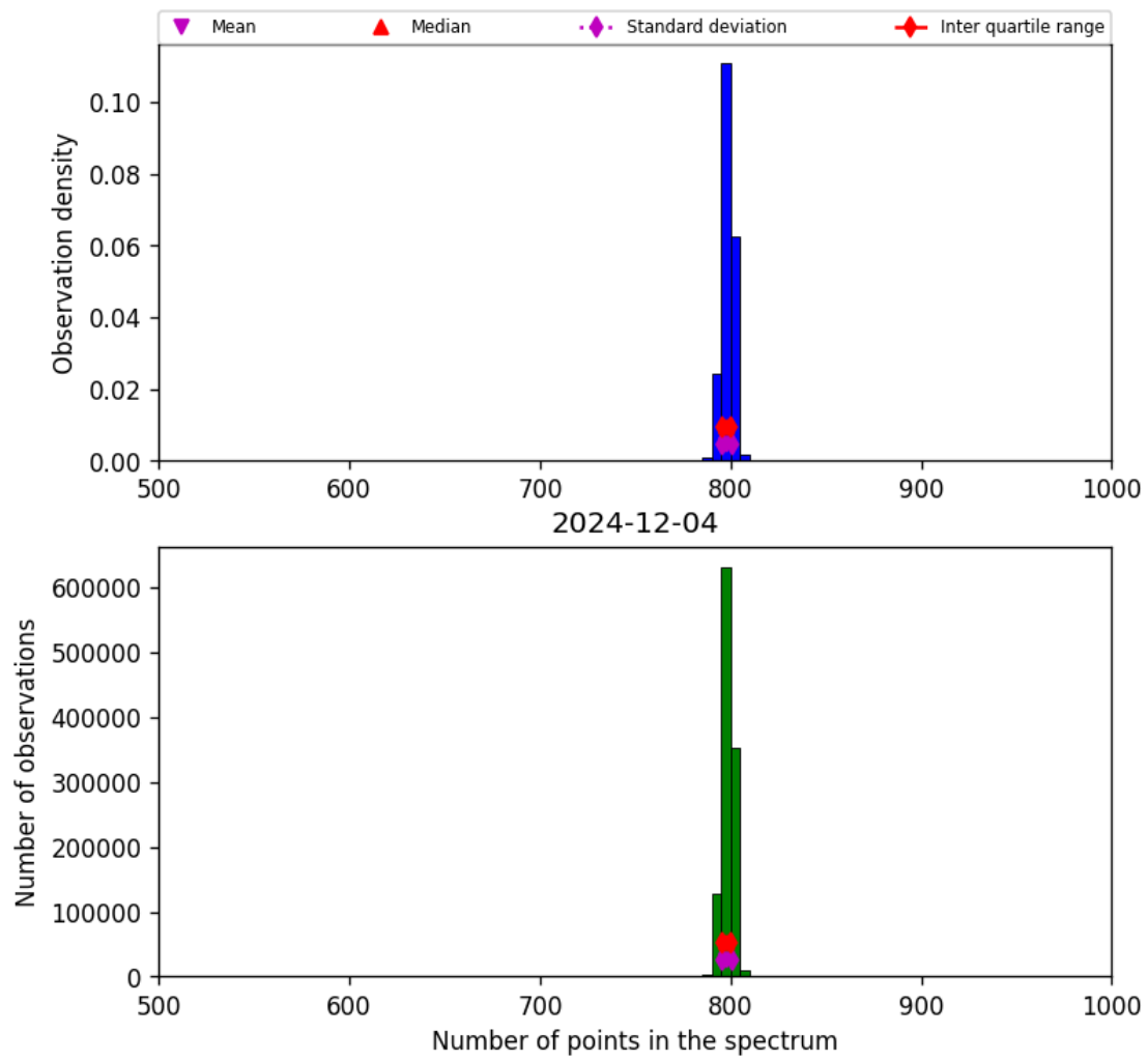
Figure 26: Histogram of “Number of points in the spectrum” for 2024-12-03 to 2024-12-05
