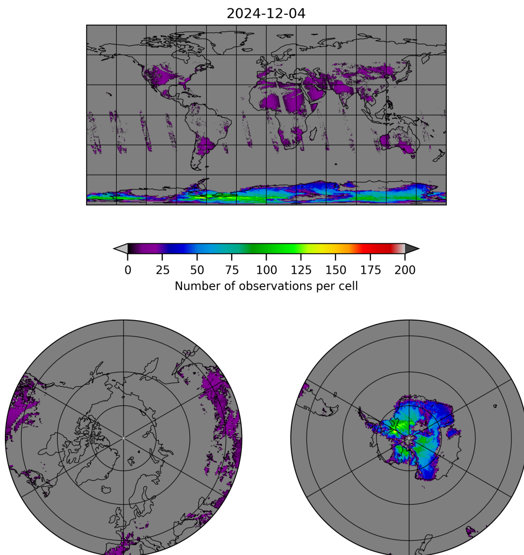
Figure 10: Map of the number of observations for 2024-12-03 to 2024-12-05
