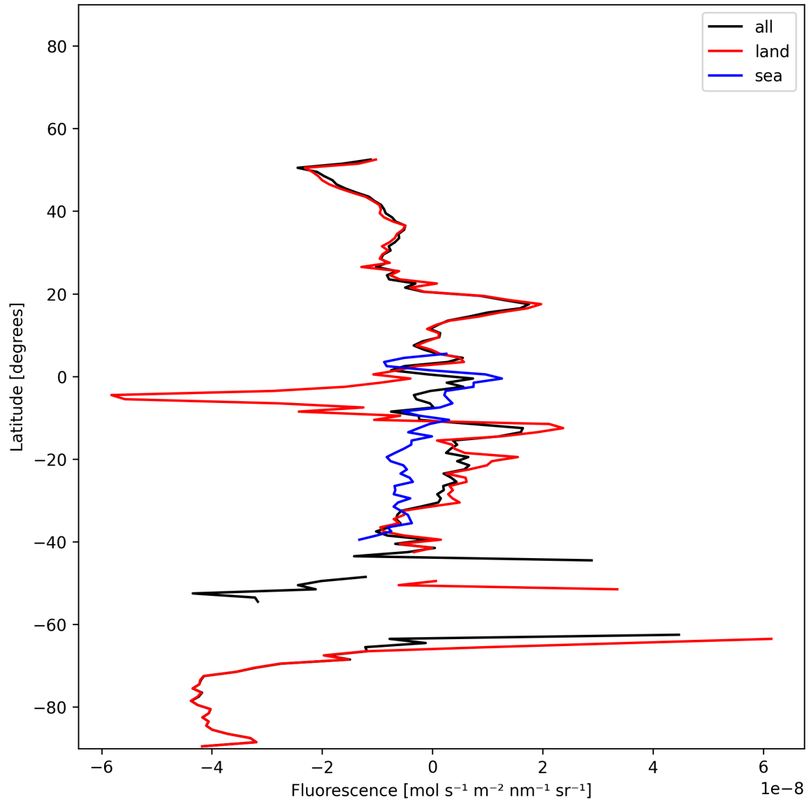
Figure 21: Zonal average of “Fluorescence” for 2024-12-03 to 2024-12-05.
