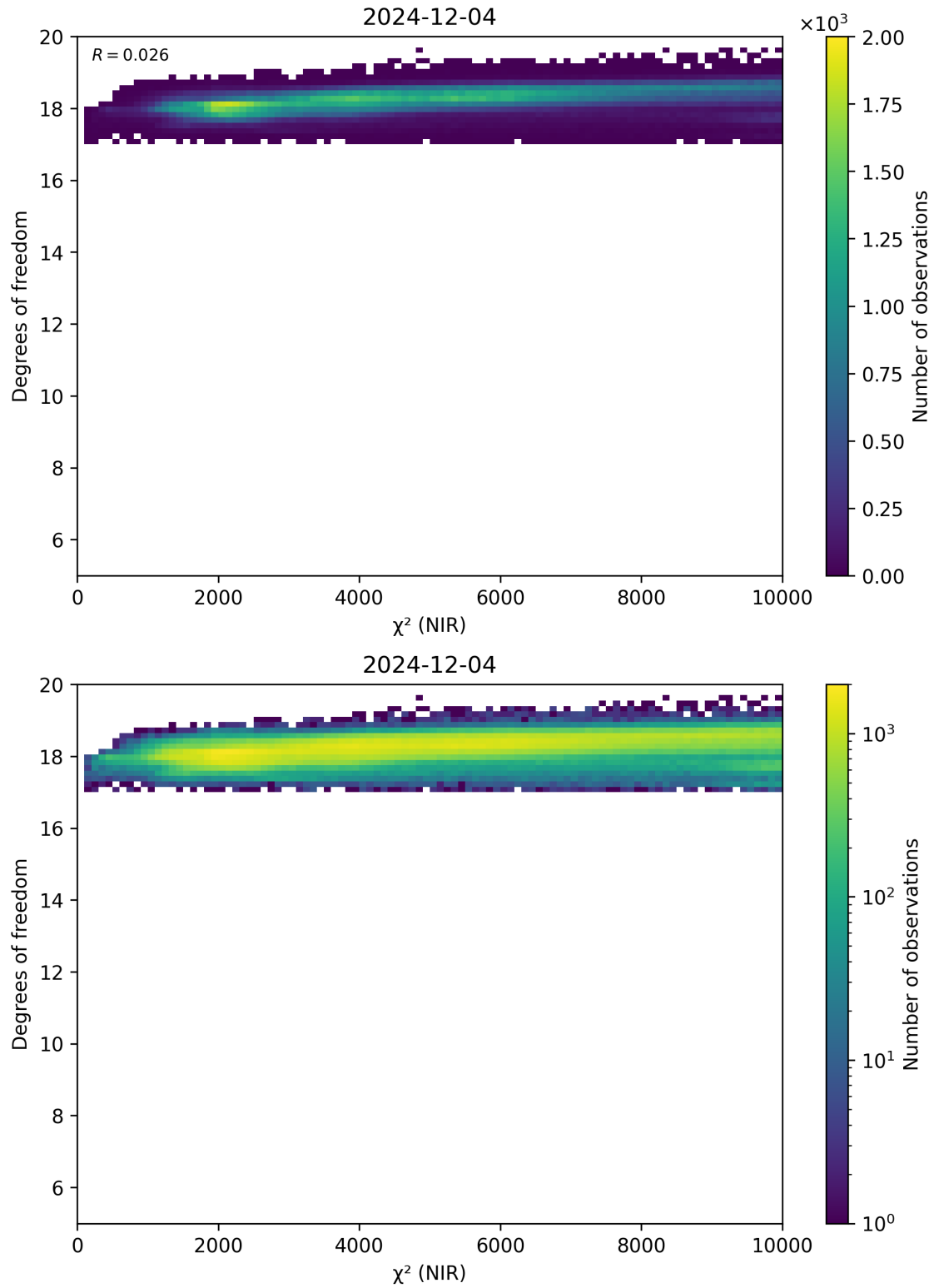
Figure 44: Scatter density plot of “ \chi^2 (NIR)” against “Degrees of freedom” for 2024-12-03 to 2024-12-05.
