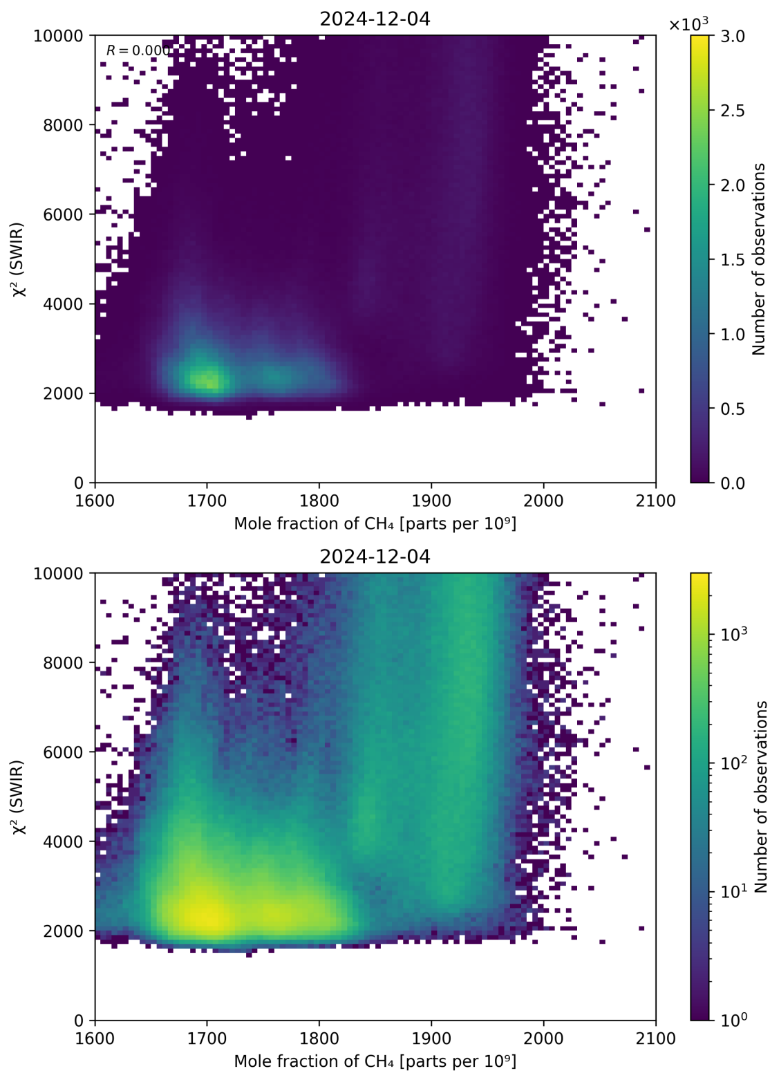
Figure 71: Scatter density plot of “Mole fraction of \text{CH}_4 ” against “ \chi^2 (SWIR)” for 2024-12-03 to 2024-12-05.
