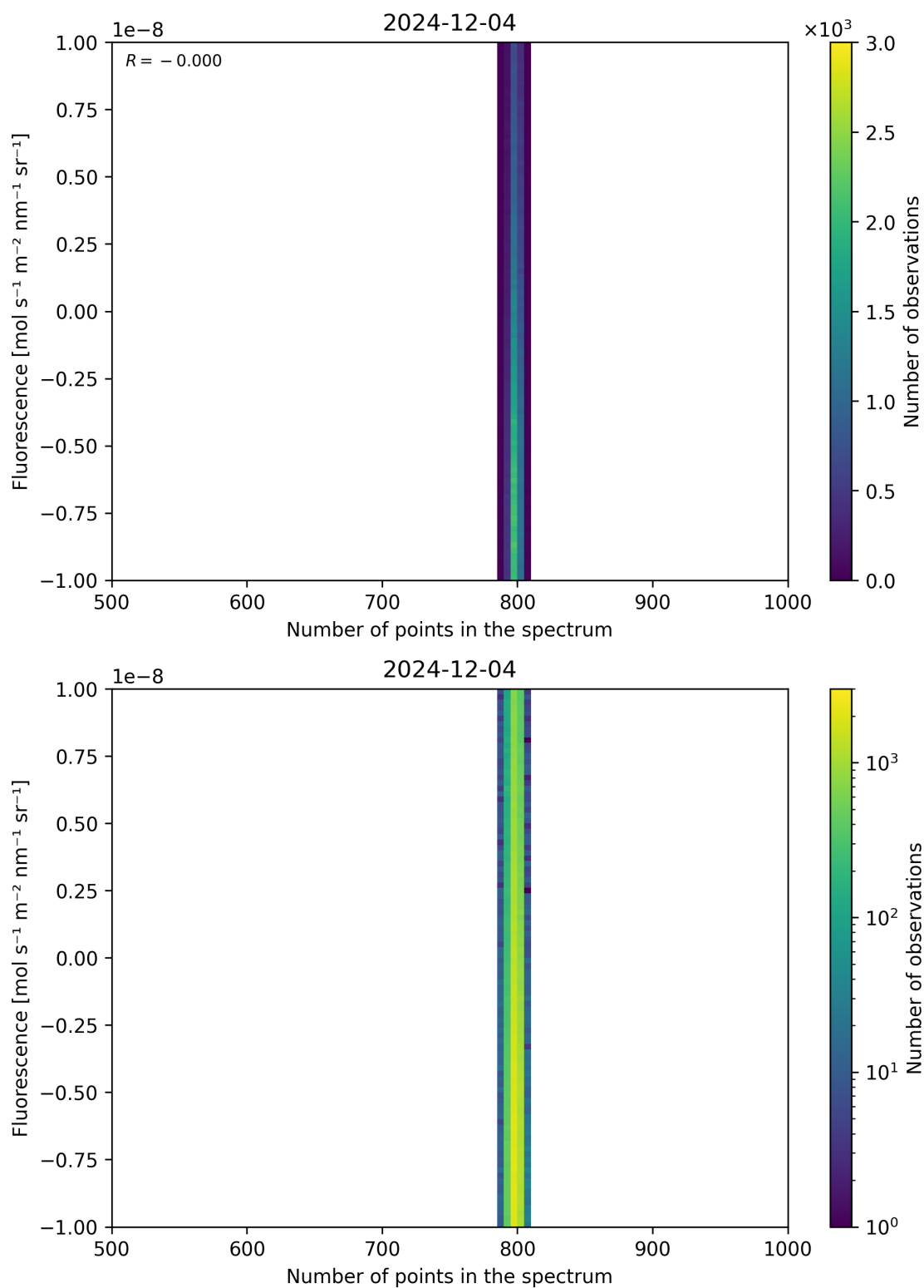
Figure 91: Scatter density plot of “Number of points in the spectrum” against “Fluorescence” for 2024-12-03 to 2024-12-05.
