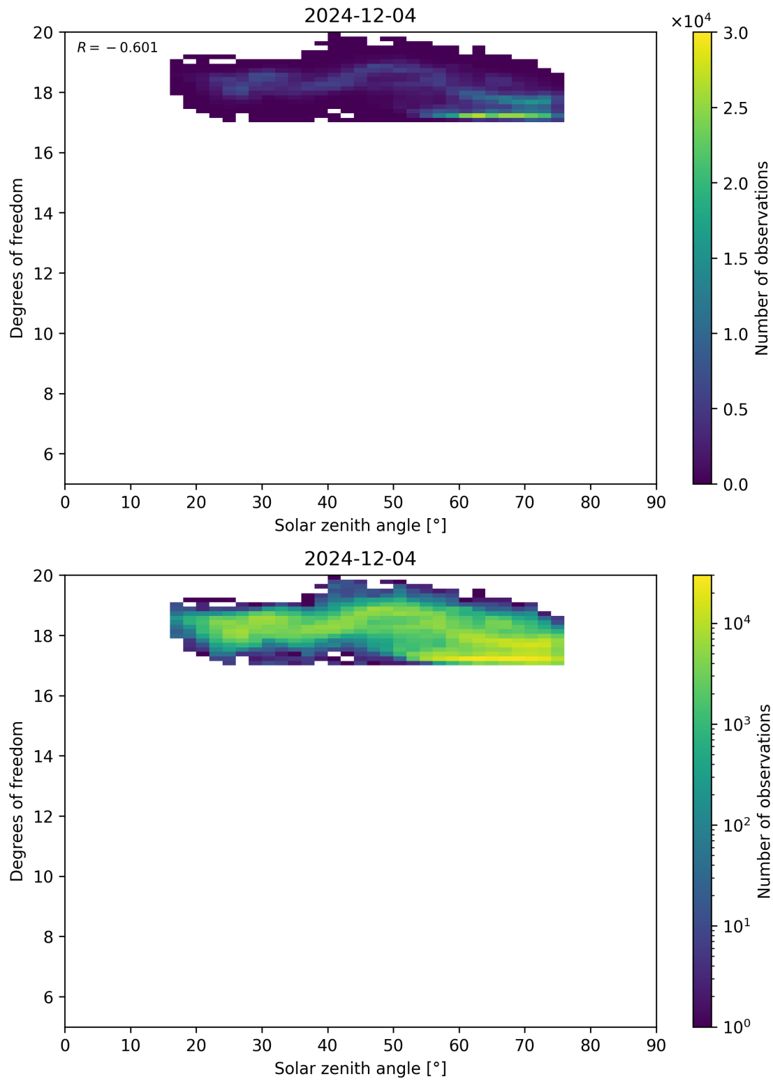
Figure 96: Scatter density plot of “Solar zenith angle” against “Degrees of freedom” for 2024-12-03 to 2024-12-05.
