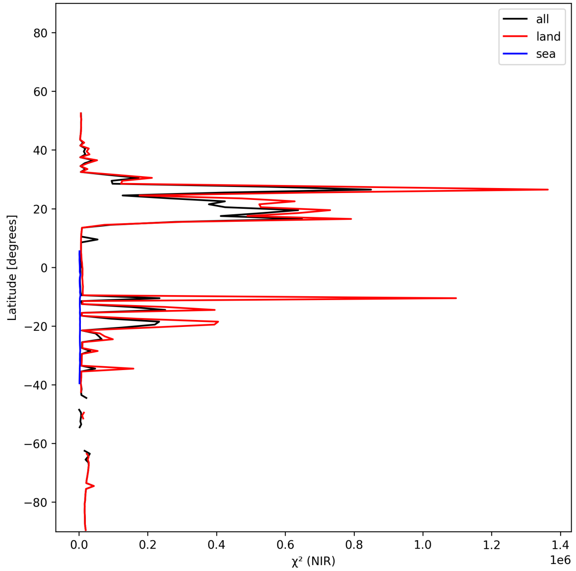
Figure 18: Zonal average of “ \chi^2 (NIR)” for 2024-12-03 to 2024-12-05.
