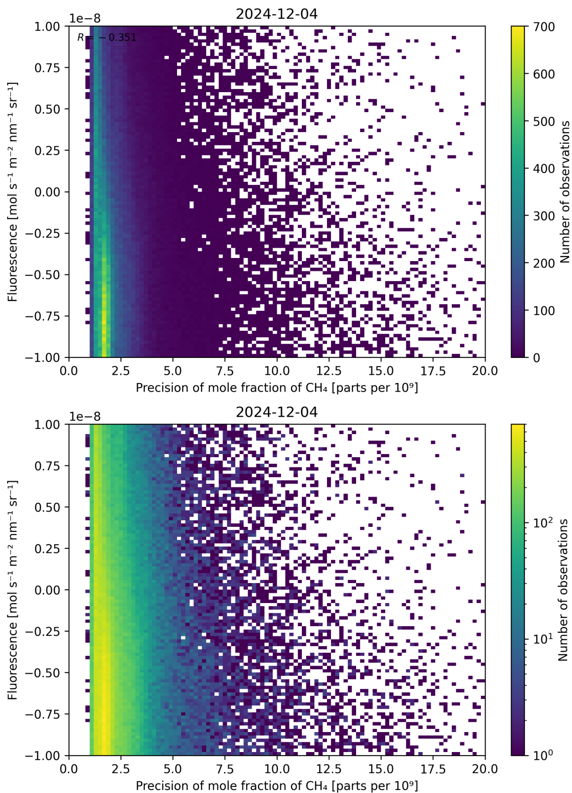
Figure 81: Scatter density plot of “Precision of mole fraction of \text{CH}_4 ” against “Fluorescence” for 2024-12-03 to 2024-12-05.
