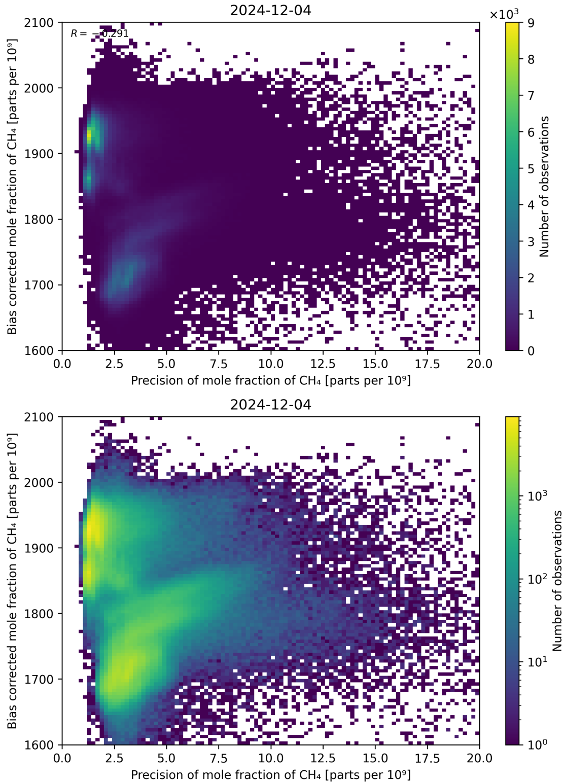
Figure 82: Scatter density plot of “Precision of mole fraction of CH 4 ” against “Bias corrected mole fraction of CH 4 ” for 2024-12-03 to 2024-12-05.
