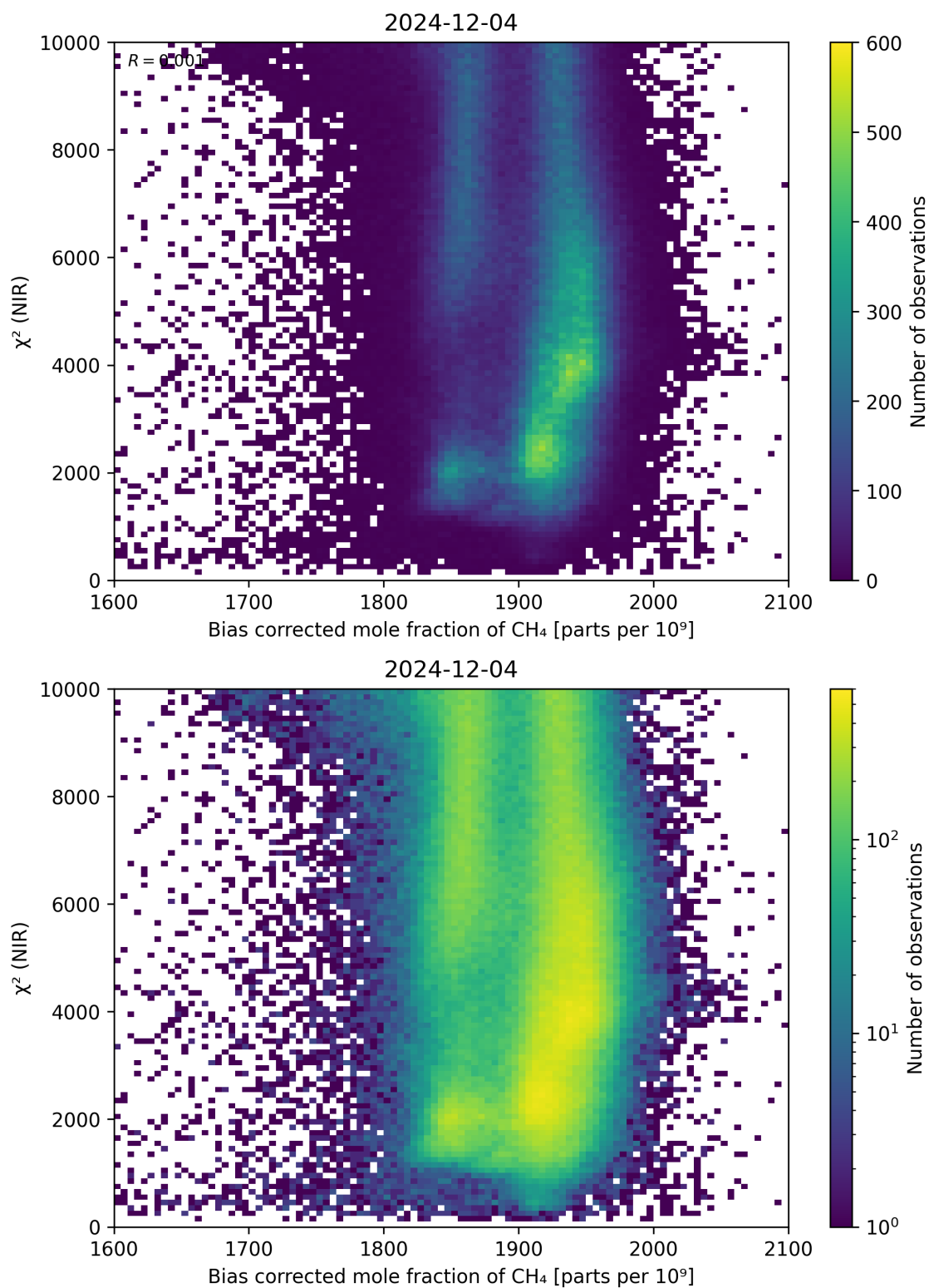
Figure 63: Scatter density plot of “Bias corrected mole fraction of CH 4 ” against “ \chi^2 (NIR)” for 2024-12-03 to 2024-12-05.
