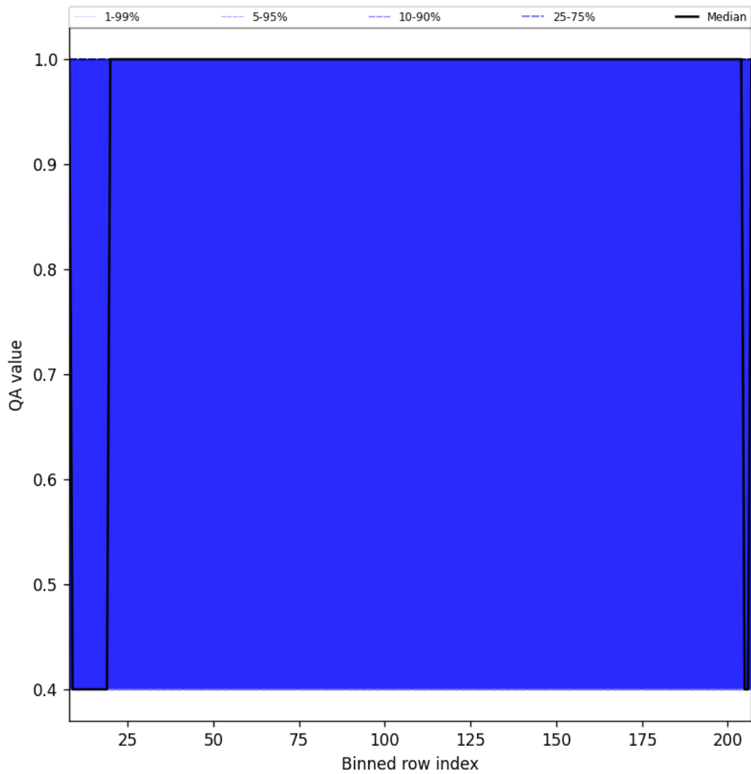
Figure 33: Along track statistics of “QA value” for 2024-12-03 to 2024-12-05
