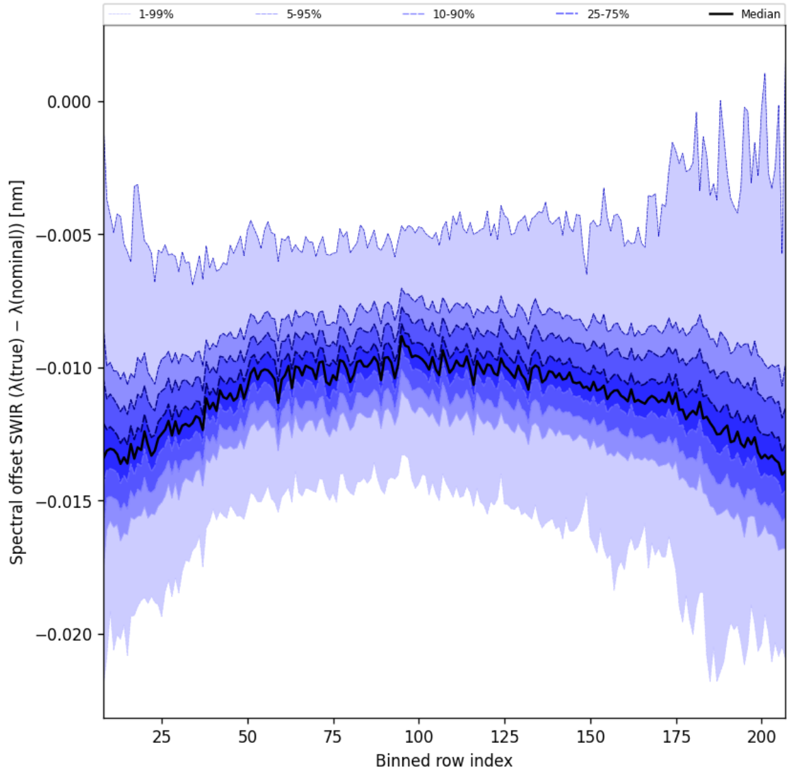
Figure 38: Along track statistics of “Spectral offset SWIR ( \lambda_{\text{true}} - \lambda_{\text{nominal}} )” for 2024-12-03 to 2024-12-05
