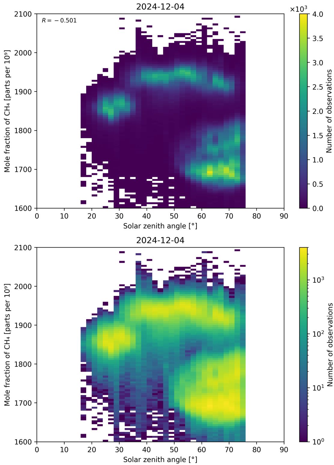
Figure 99: Scatter density plot of “Solar zenith angle” against “Mole fraction of CH 4 ” for 2024-12-03 to 2024-12-05.
