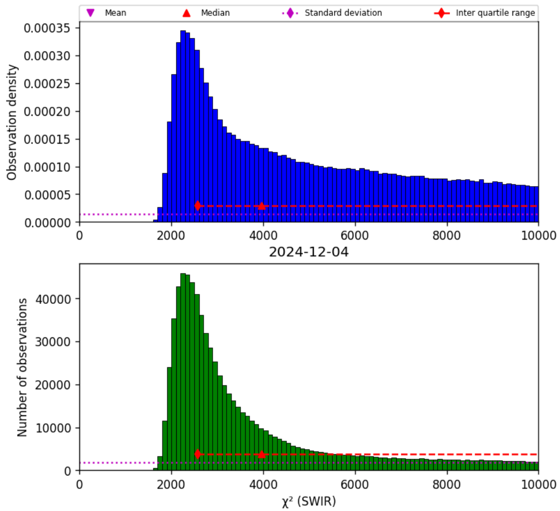
Figure 28: Histogram of “ \chi^2 (SWIR)” for 2024-12-03 to 2024-12-05
