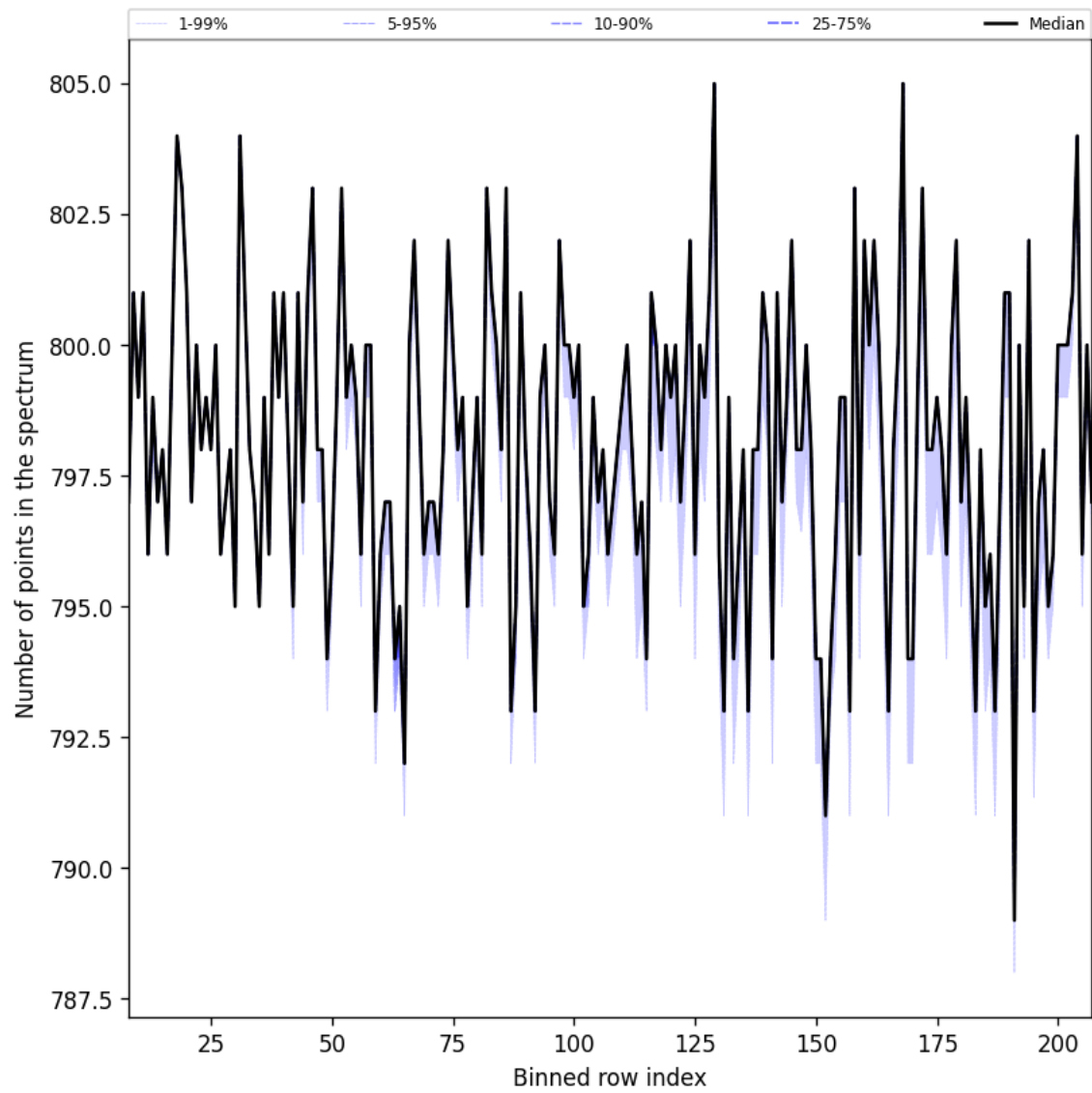
Figure 37: Along track statistics of “Number of points in the spectrum” for 2024-12-03 to 2024-12-05
