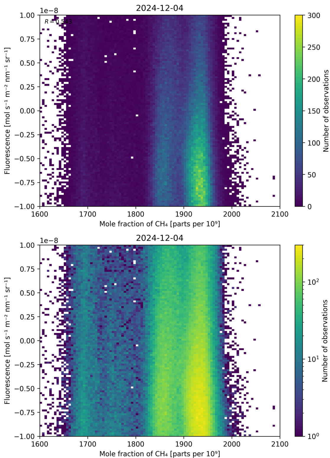
Figure 73: Scatter density plot of “Mole fraction of \text{CH}_4 ” against “Fluorescence” for 2024-12-03 to 2024-12-05.
