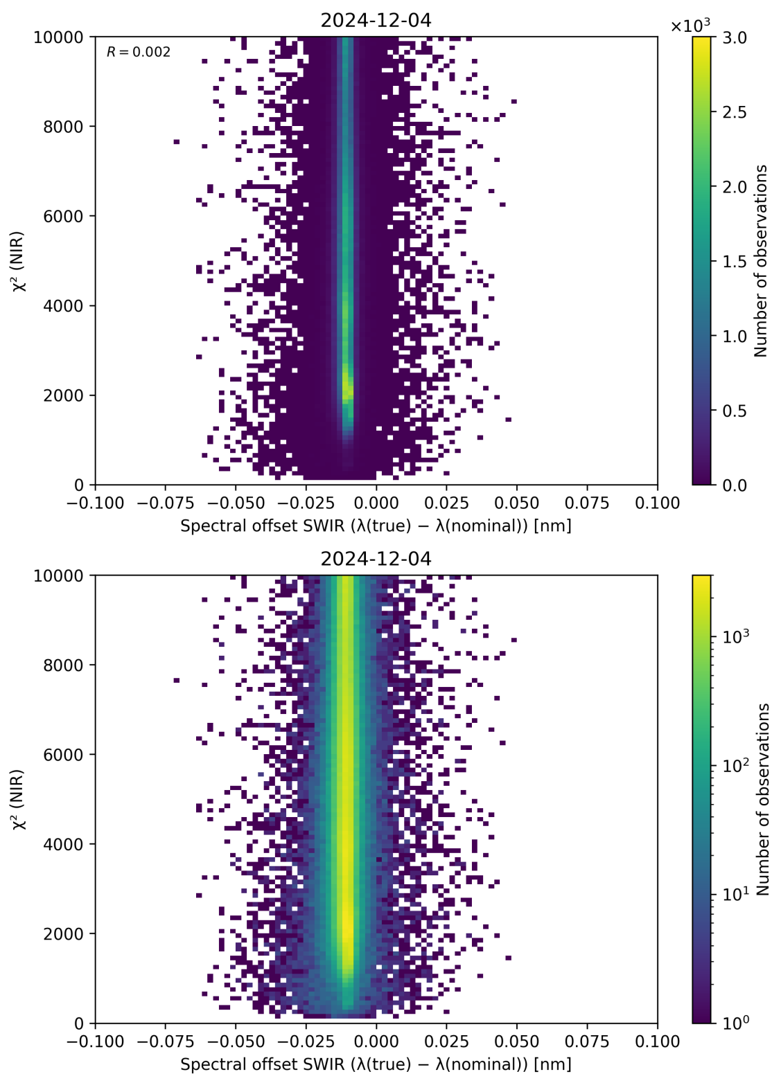
Figure 117: Scatter density plot of “Spectral offset SWIR ( \lambda_{\text{true}} - \lambda_{\text{nominal}} )” against “ \chi^2 (NIR)” for 2024-12-03 to 2024-12-05.
