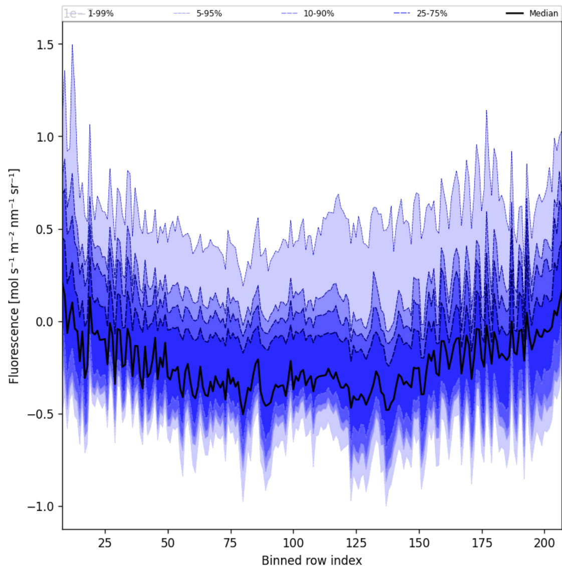
Figure 43: Along track statistics of “Fluorescence” for 2024-12-03 to 2024-12-05
