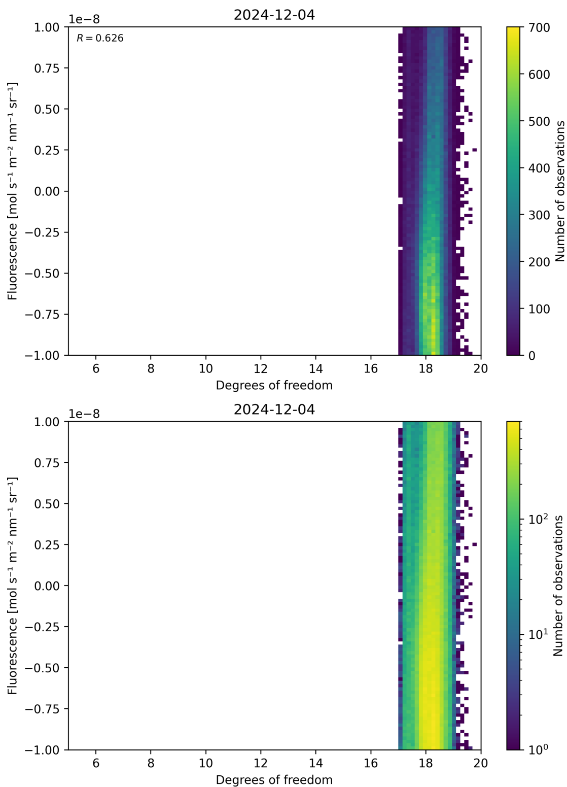
Figure 51: Scatter density plot of “Degrees of freedom” against “Fluorescence” for 2024-12-03 to 2024-12-05.
