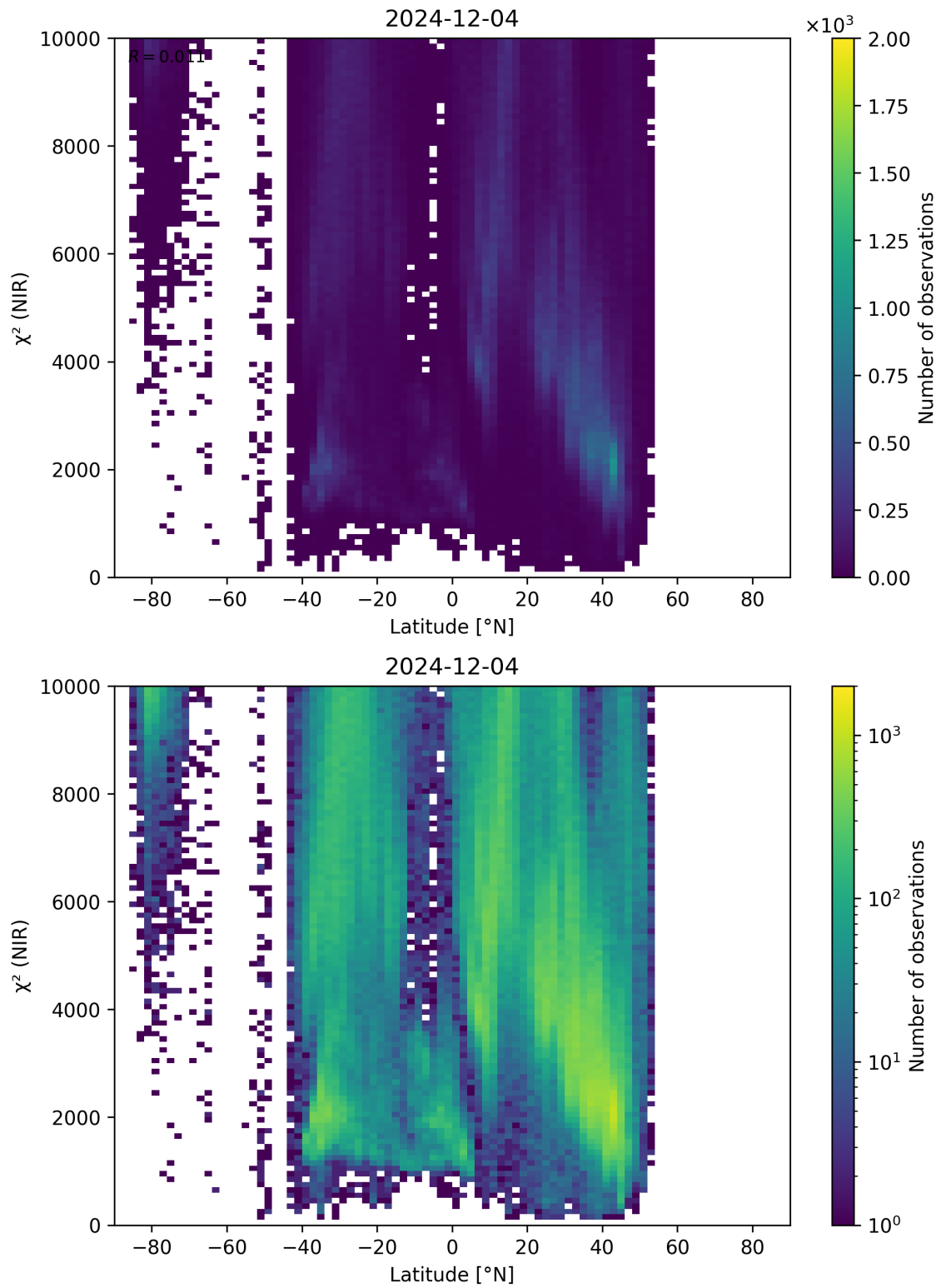
Figure 53: Scatter density plot of “Latitude” against “ \chi^2 (NIR)” for 2024-12-03 to 2024-12-05.
