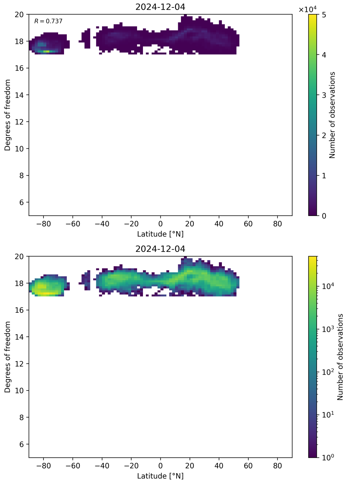
Figure 55: Scatter density plot of “Latitude” against “Degrees of freedom” for 2024-12-03 to 2024-12-05.
