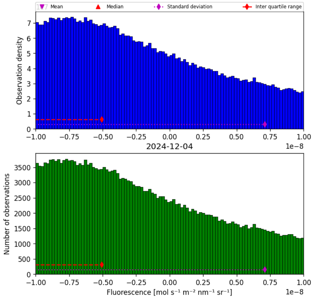
Figure 32: Histogram of “Fluorescence” for 2024-12-03 to 2024-12-05
