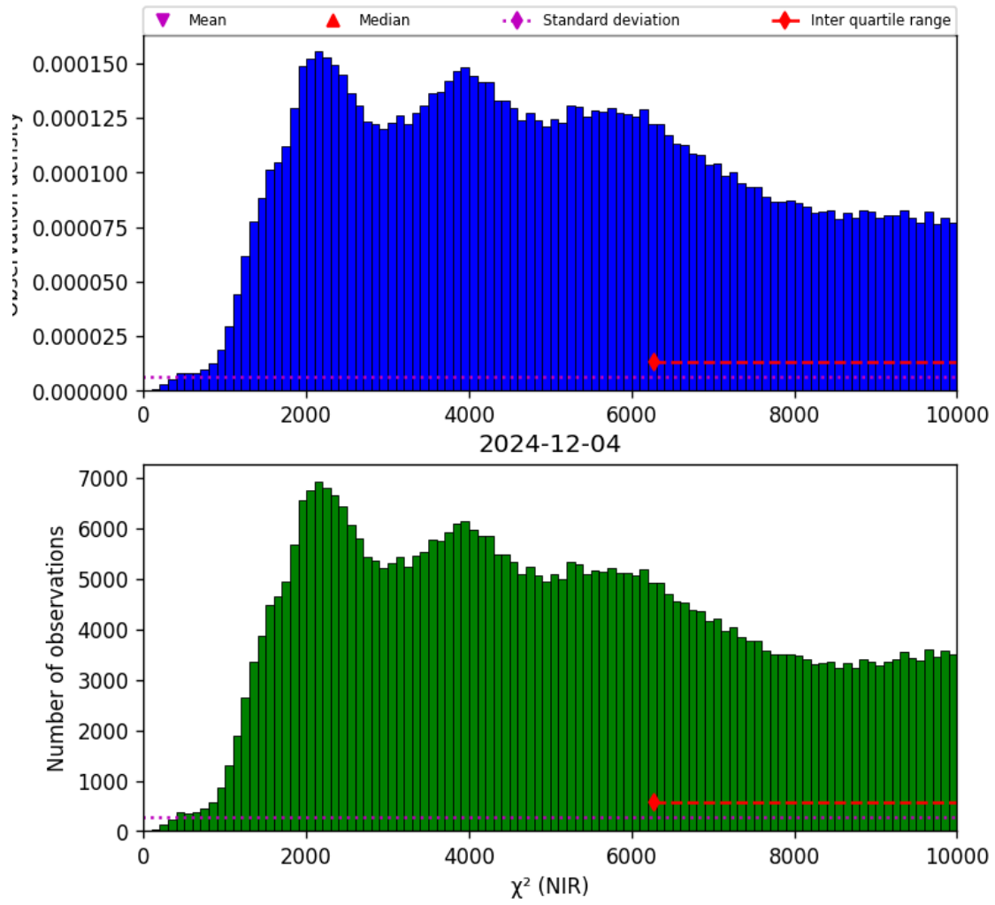
Figure 29: Histogram of “ \chi^2 (NIR)” for 2024-12-03 to 2024-12-05
