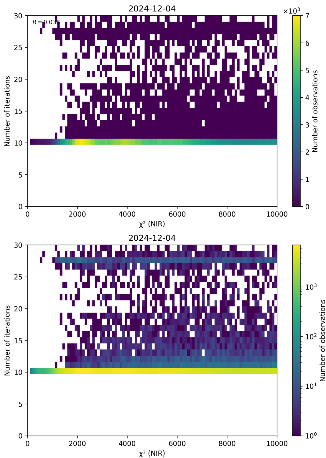
Figure 46: Scatter density plot of “ \chi^2 (NIR)” against “Number of iterations” for 2024-12-03 to 2024-12-05.
