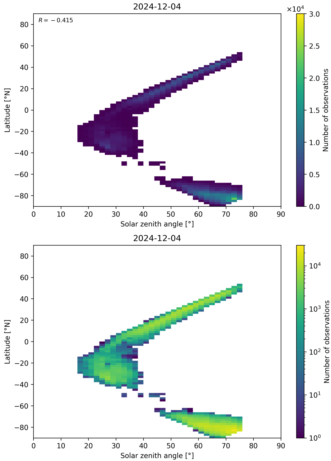
Figure 98: Scatter density plot of “Solar zenith angle” against “Latitude” for 2024-12-03 to 2024-12-05.
