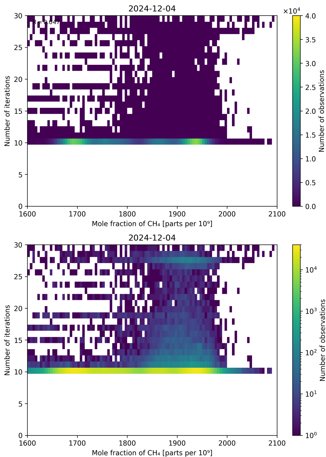
Figure 76: Scatter density plot of “Mole fraction of CH 4 ” against “Number of iterations” for 2024-12-03 to 2024-12-05.
