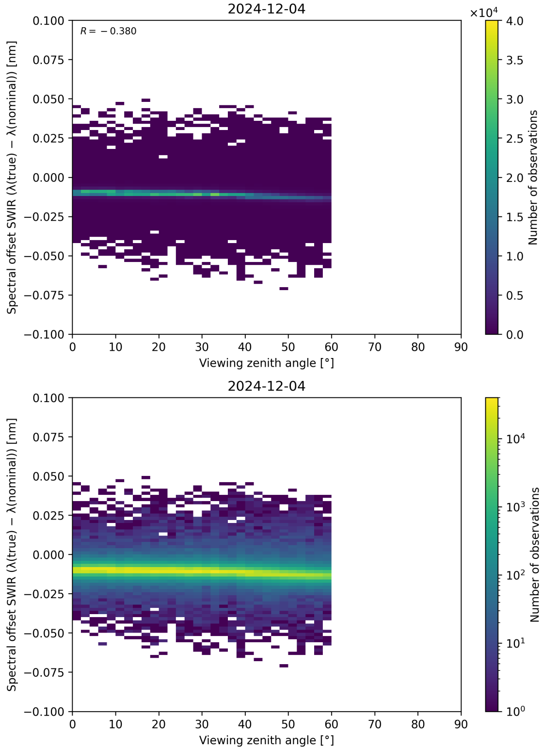
Figure 116: Scatter density plot of “Viewing zenith angle” against “Spectral offset SWIR ( \lambda_{\text{true}} - \lambda_{\text{nominal}} )” for 2024-12-03 to 2024-12-05.
