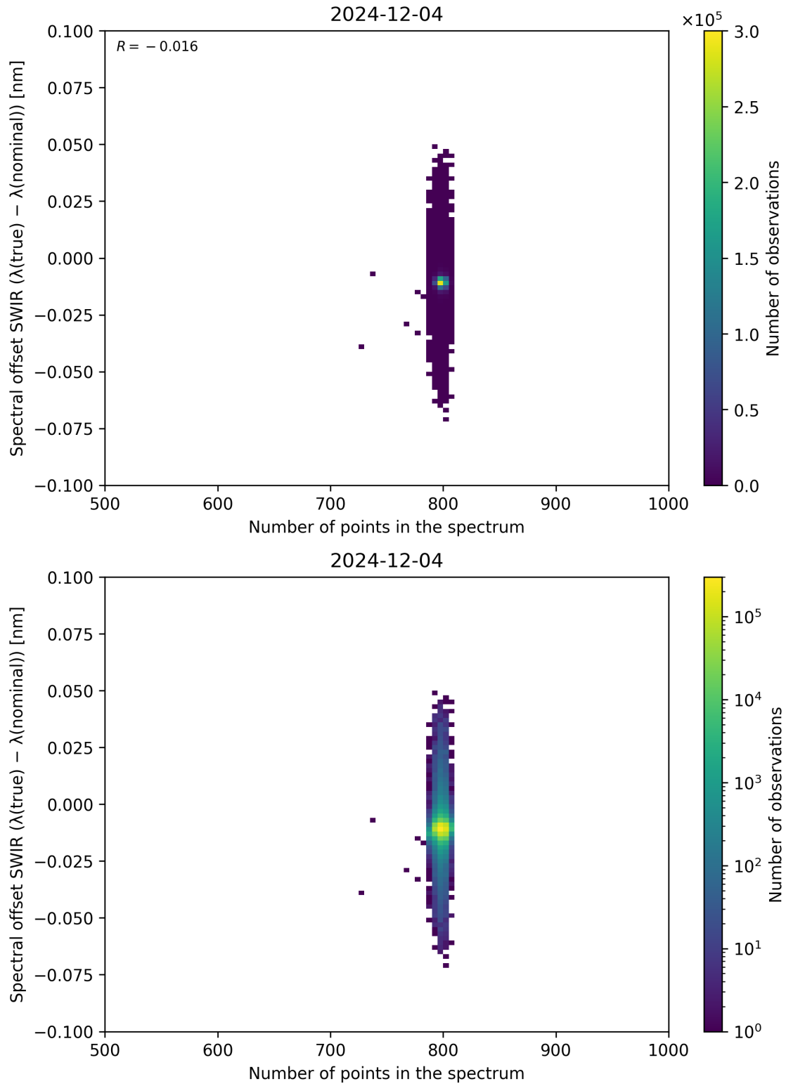
Figure 93: Scatter density plot of “Number of points in the spectrum” against “Spectral offset SWIR ( \lambda_{\text{true}} - \lambda_{\text{nominal}} )” for 2024-12-03 to 2024-12-05.
