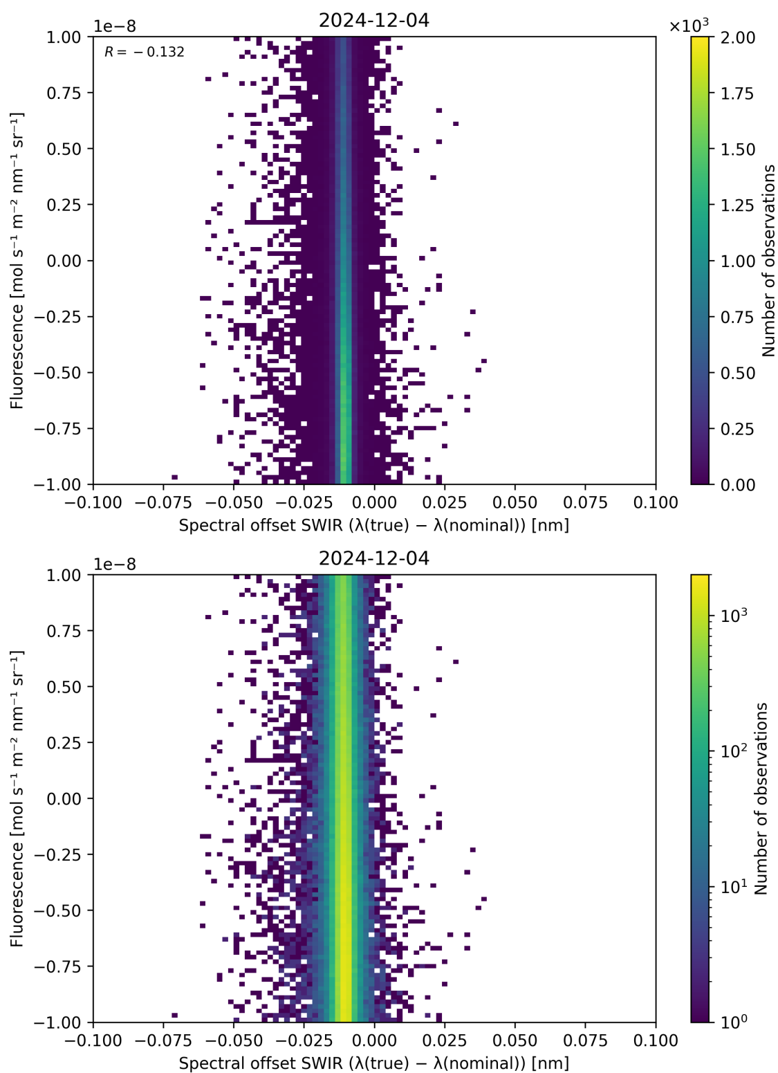
Figure 120: Scatter density plot of “Spectral offset SWIR ( \lambda_{\text{true}} - \lambda_{\text{nominal}} )” against “Fluorescence” for 2024-12-03 to 2024-12-05.
