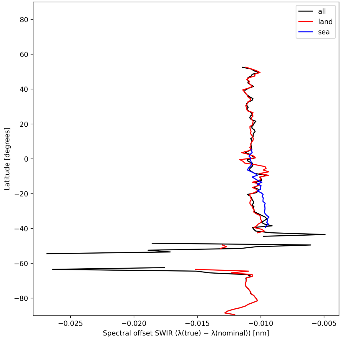
Figure 16: Zonal average of “Spectral offset SWIR ( \lambda_{\text{true}} - \lambda_{\text{nominal}} )” for 2024-12-03 to 2024-12-05.
