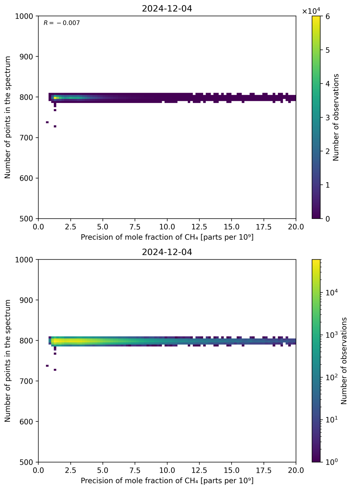
Figure 84: Scatter density plot of “Precision of mole fraction of CH 4 ” against “Number of points in the spectrum” for 2024-12-03 to 2024-12-05.
