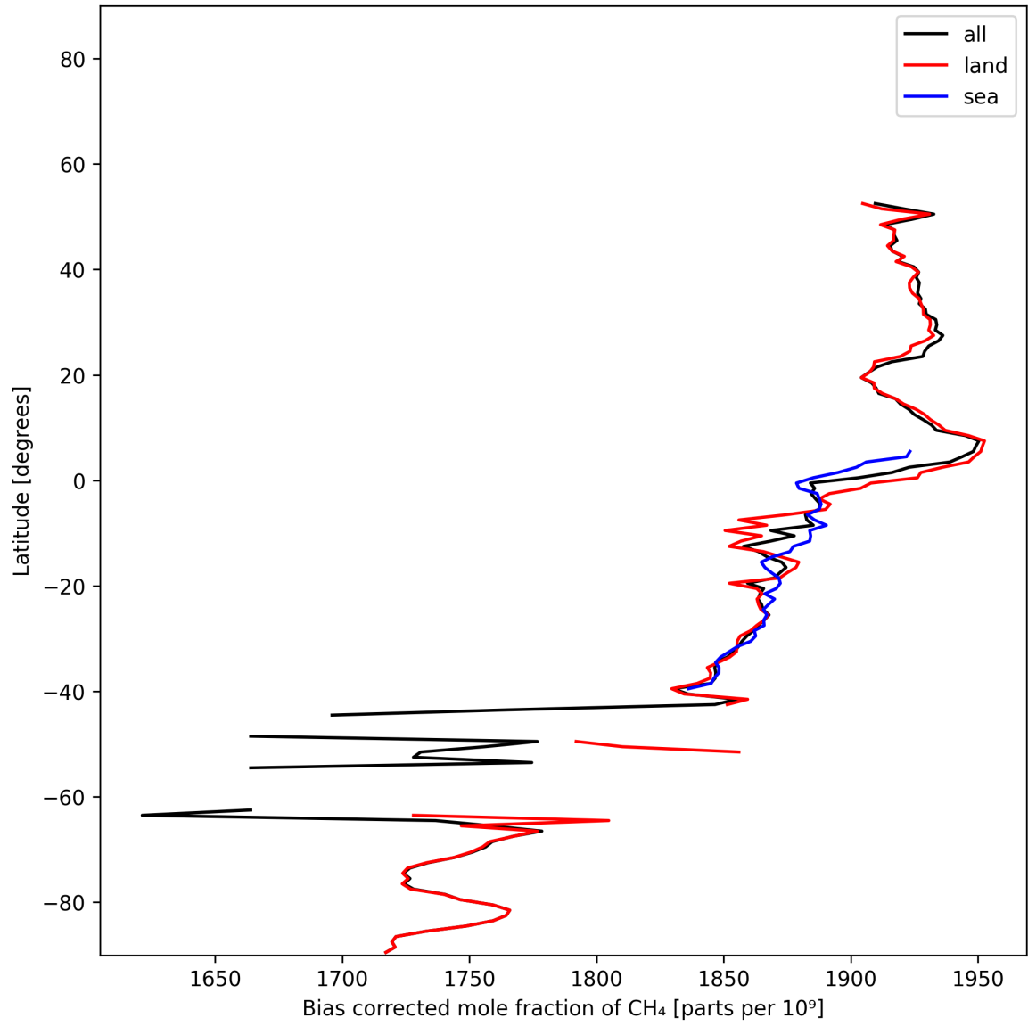
Figure 14: Zonal average of “Bias corrected mole fraction of CH 4 ” for 2024-12-03 to 2024-12-05.
