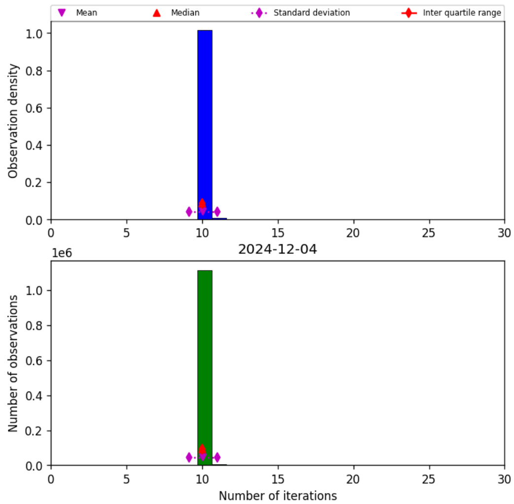
Figure 31: Histogram of “Number of iterations” for 2024-12-03 to 2024-12-05
