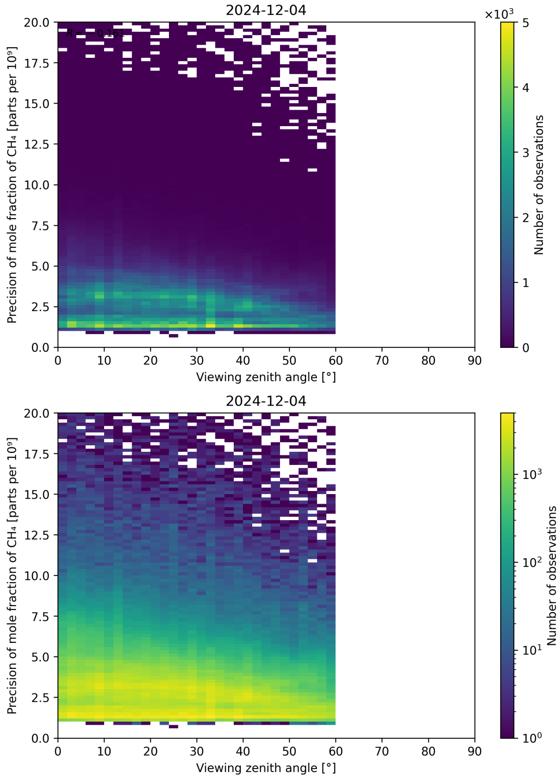
Figure 112: Scatter density plot of “Viewing zenith angle” against “Precision of mole fraction of CH 4 ” for 2024-12-03 to 2024-12-05.
