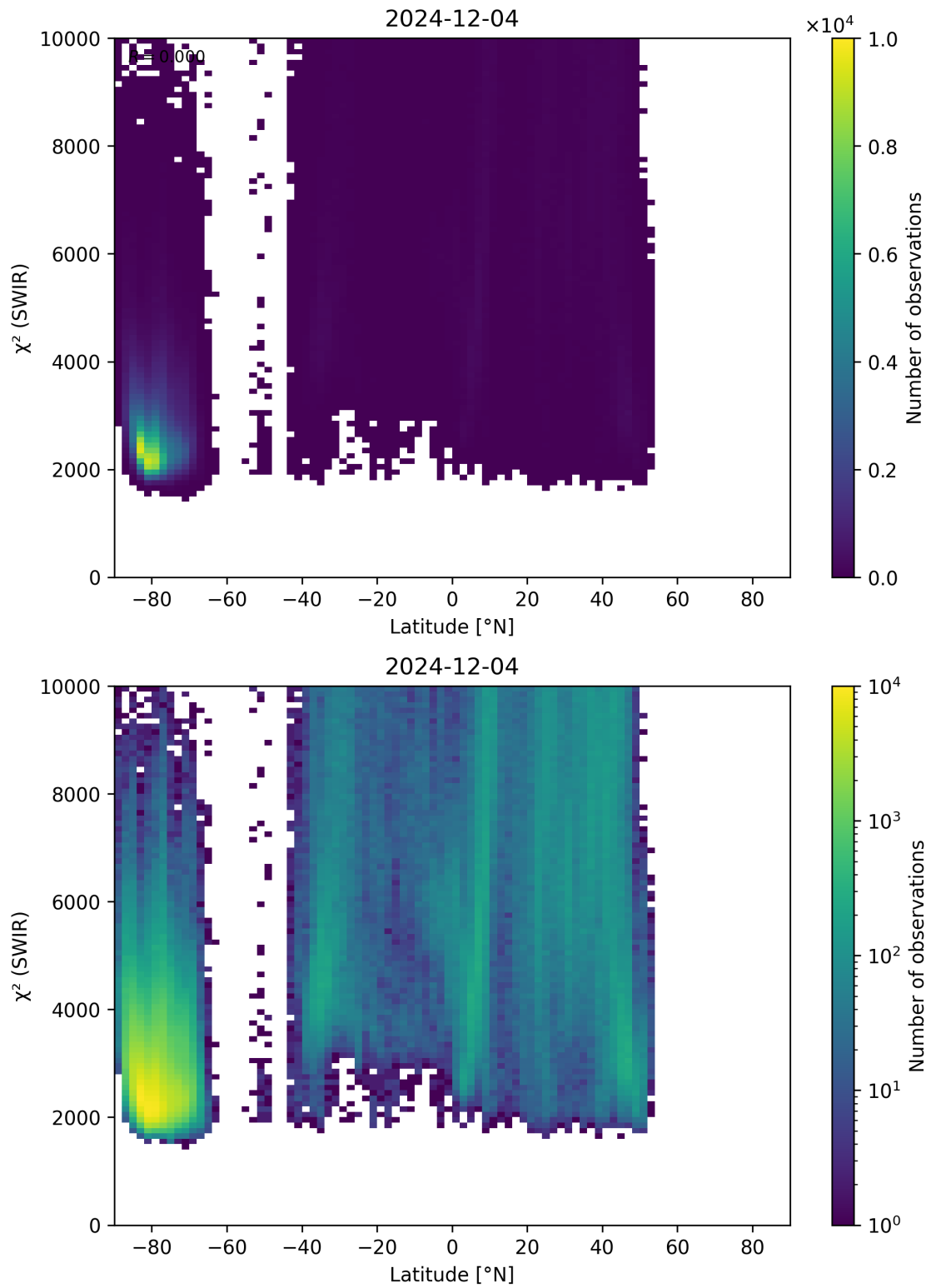
Figure 54: Scatter density plot of “Latitude” against “ \chi^2 (SWIR)” for 2024-12-03 to 2024-12-05.
