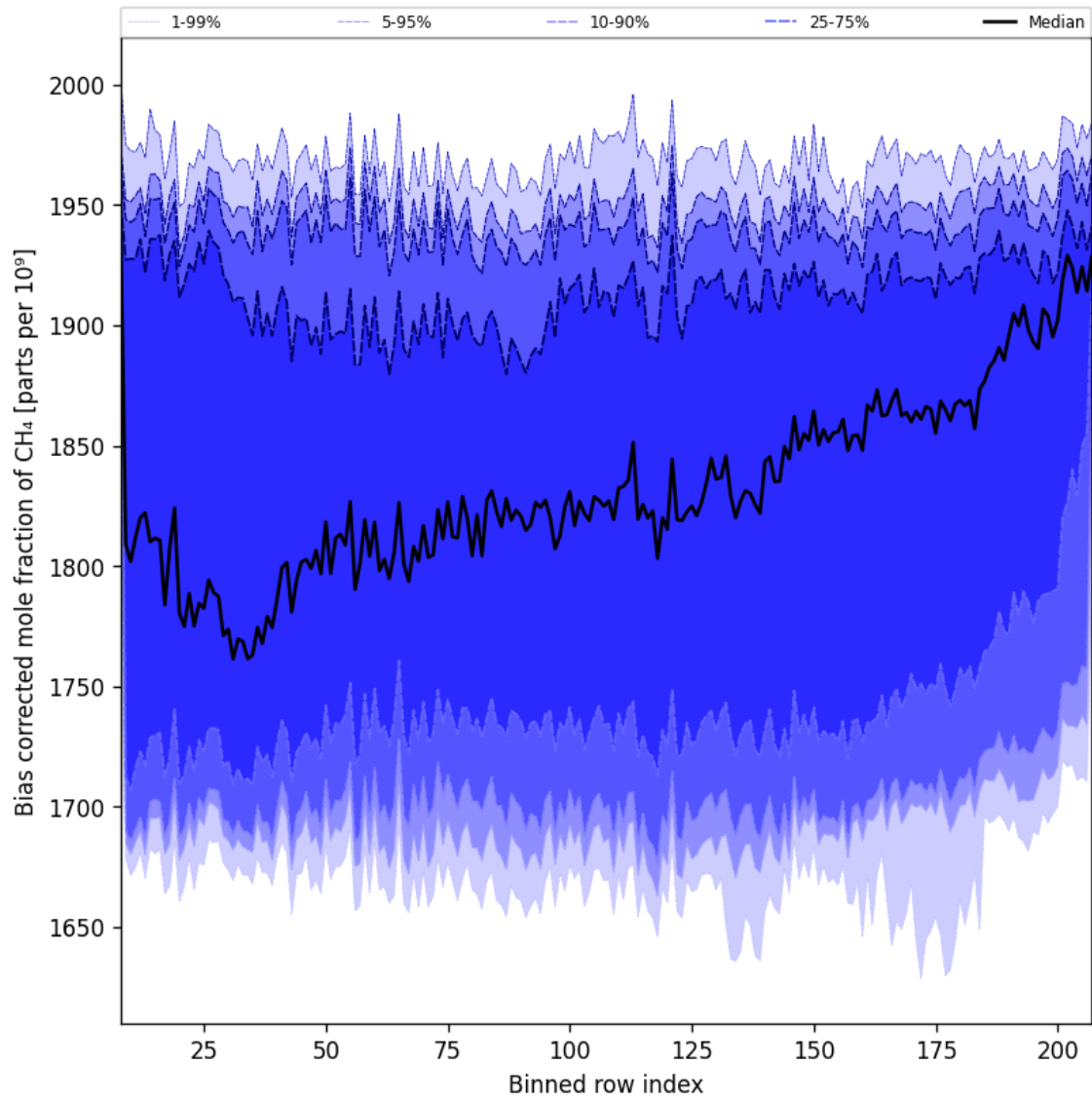
Figure 36: Along track statistics of “Bias corrected mole fraction of CH 4 ” for 2024-12-03 to 2024-12-05
