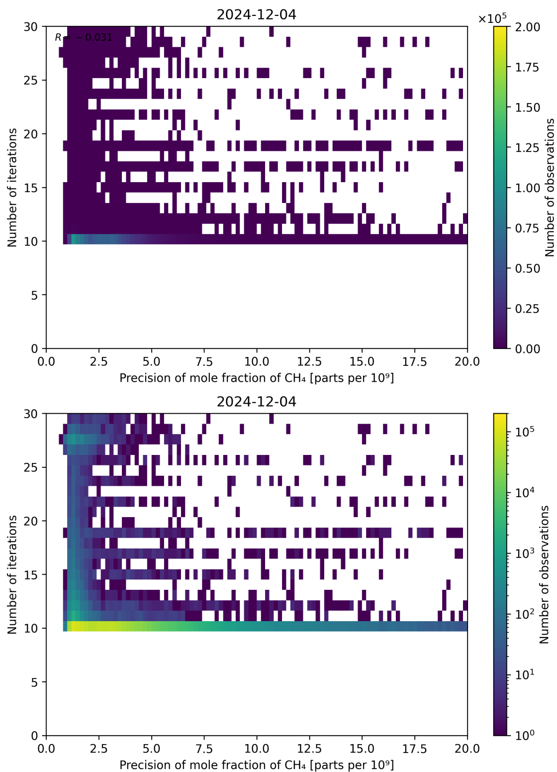
Figure 83: Scatter density plot of “Precision of mole fraction of CH 4 ” against “Number of iterations” for 2024-12-03 to 2024-12-05.
