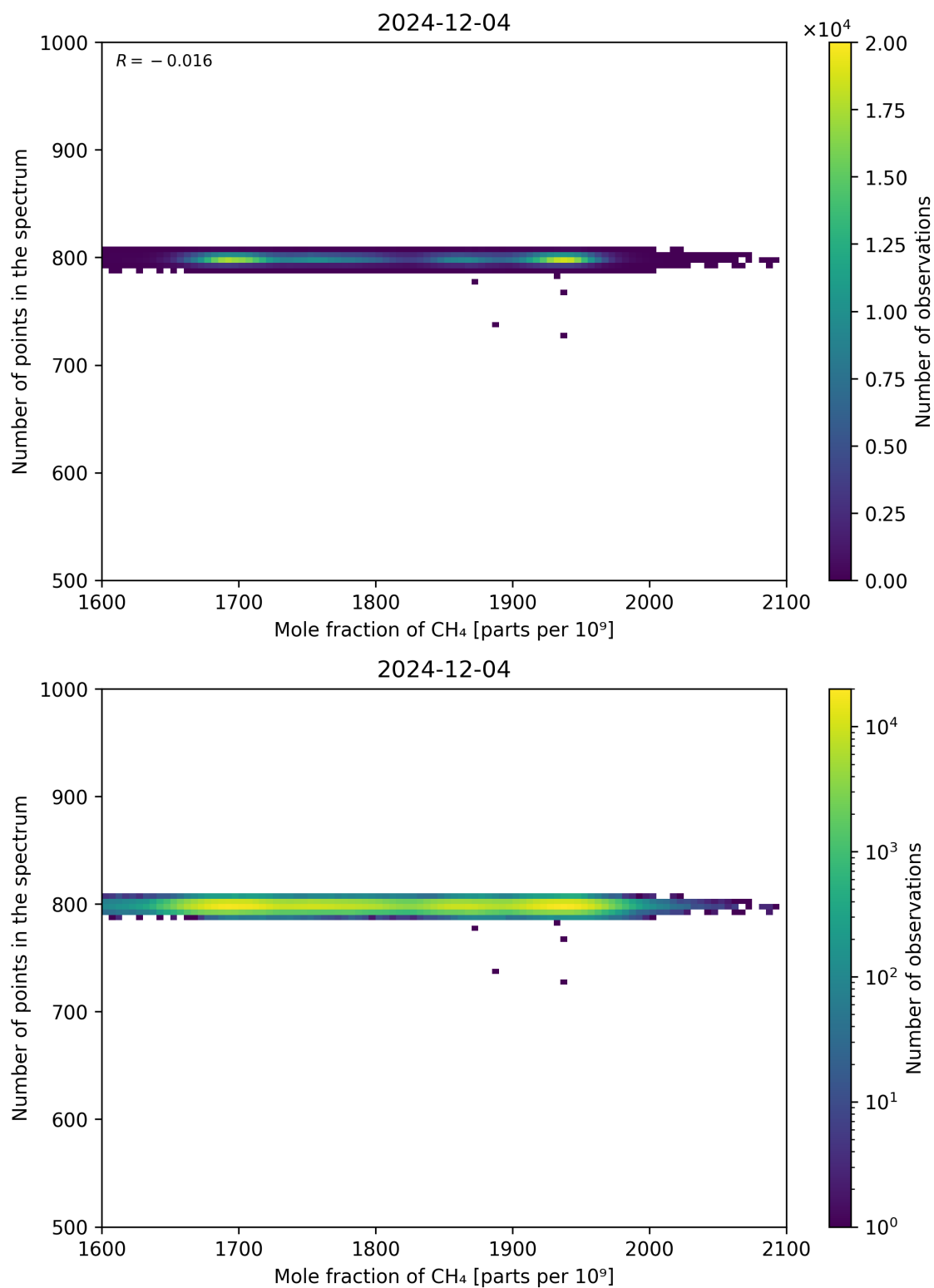
Figure 77: Scatter density plot of “Mole fraction of CH 4 ” against “Number of points in the spectrum” for 2024-12-03 to 2024-12-05.
