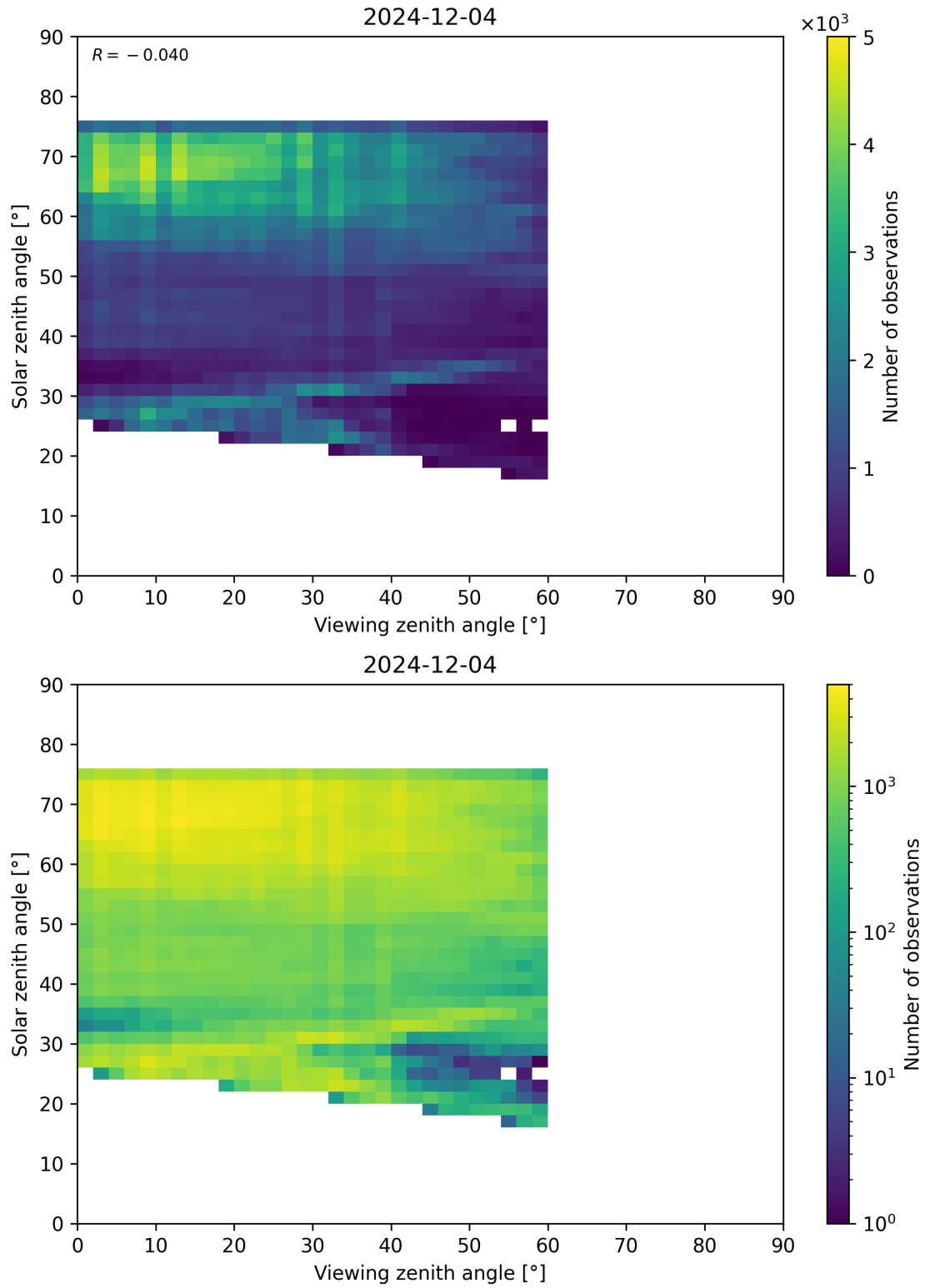
Figure 115: Scatter density plot of “Viewing zenith angle” against “Solar zenith angle” for 2024-12-03 to 2024-12-05.
