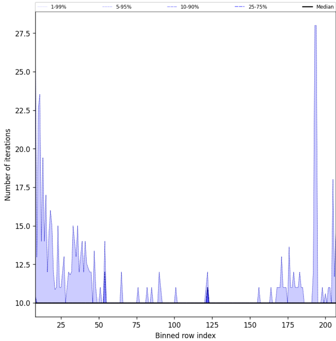
Figure 42: Along track statistics of “Number of iterations” for 2024-12-03 to 2024-12-05
