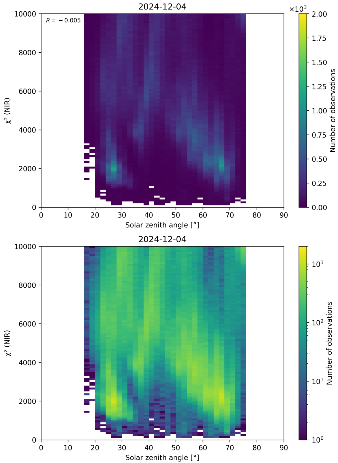
Figure 94: Scatter density plot of “Solar zenith angle” against “ \chi^2 (NIR)” for 2024-12-03 to 2024-12-05.
