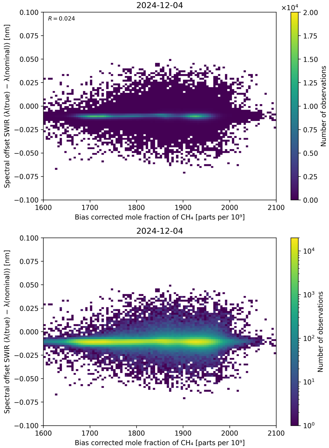
Figure 69: Scatter density plot of “Bias corrected mole fraction of \text{CH}_4 ” against “Spectral offset SWIR ( \lambda_{\text{true}} - \lambda_{\text{nominal}} )” for 2024-12-03 to 2024-12-05.
