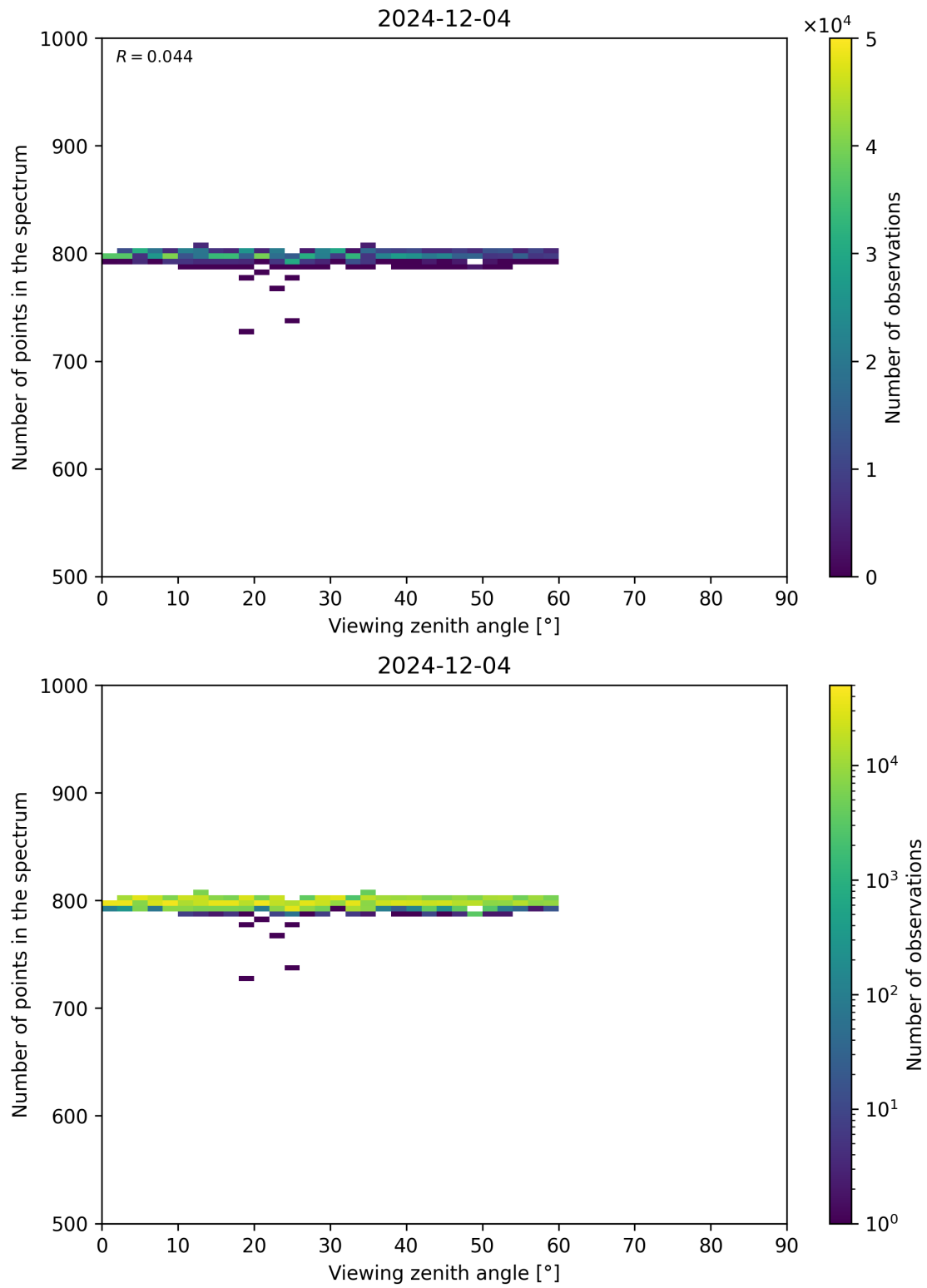
Figure 114: Scatter density plot of “Viewing zenith angle” against “Number of points in the spectrum” for 2024-12-03 to 2024-12-05.
