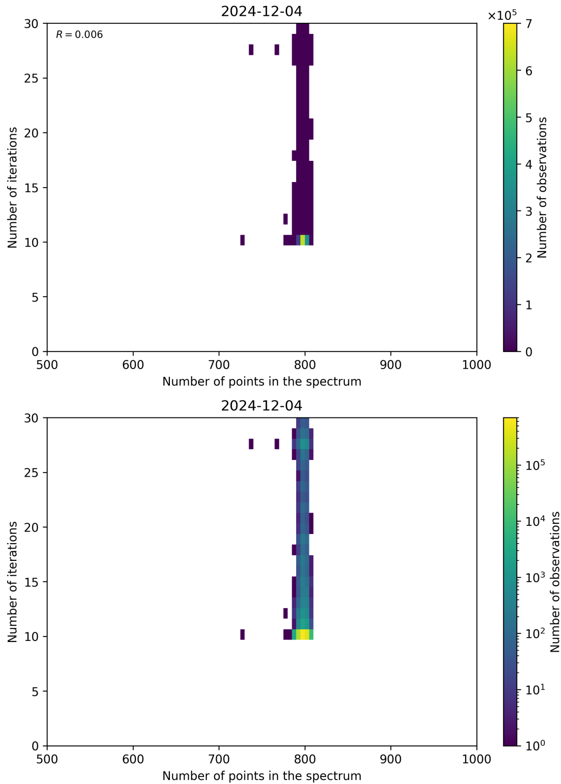
Figure 92: Scatter density plot of “Number of points in the spectrum” against “Number of iterations” for 2024-12-03 to 2024-12-05.
