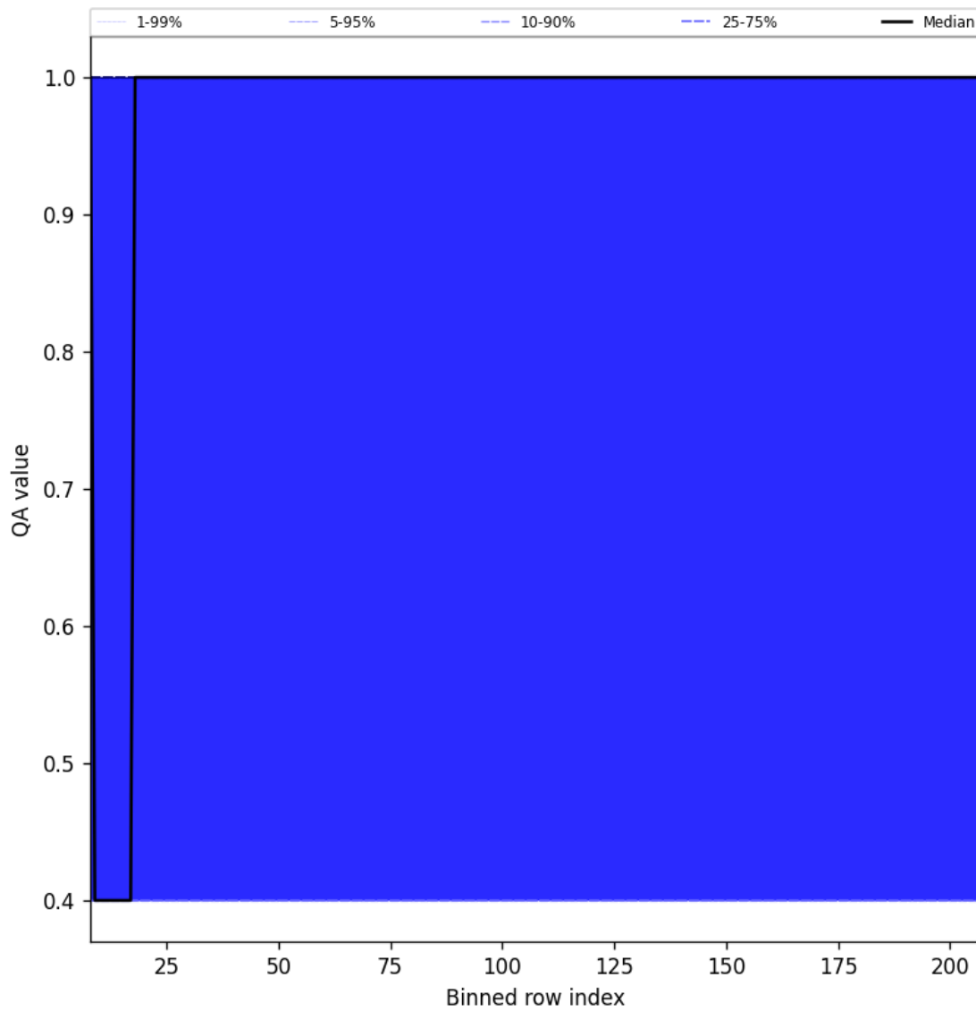
Figure 33: Along track statistics of “QA value” for 2024-12-04 to 2024-12-06
