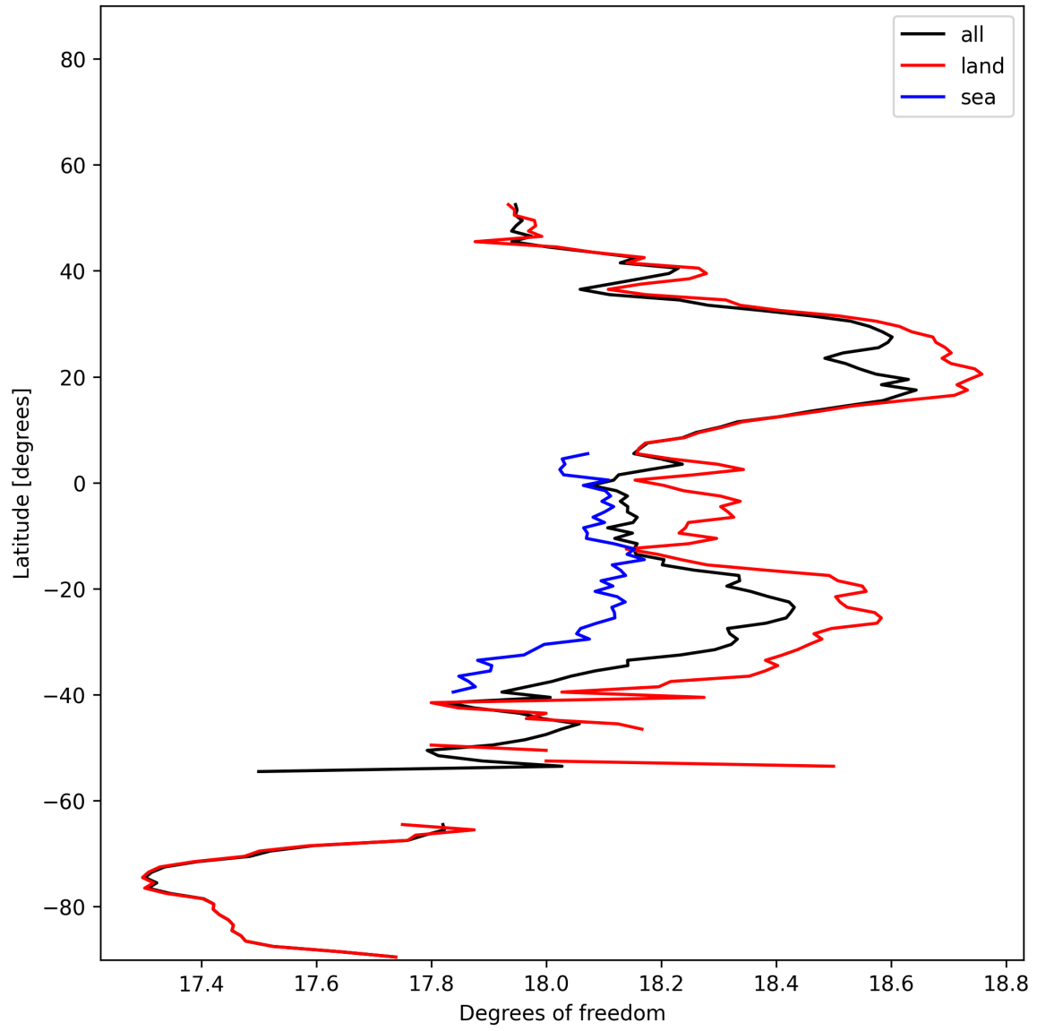
Figure 19: Zonal average of “Degrees of freedom” for 2024-12-04 to 2024-12-06.
