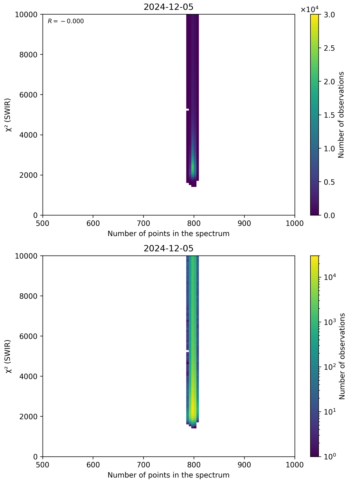
Figure 89: Scatter density plot of “Number of points in the spectrum” against “ \chi^2 (SWIR)” for 2024-12-04 to 2024-12-06.
