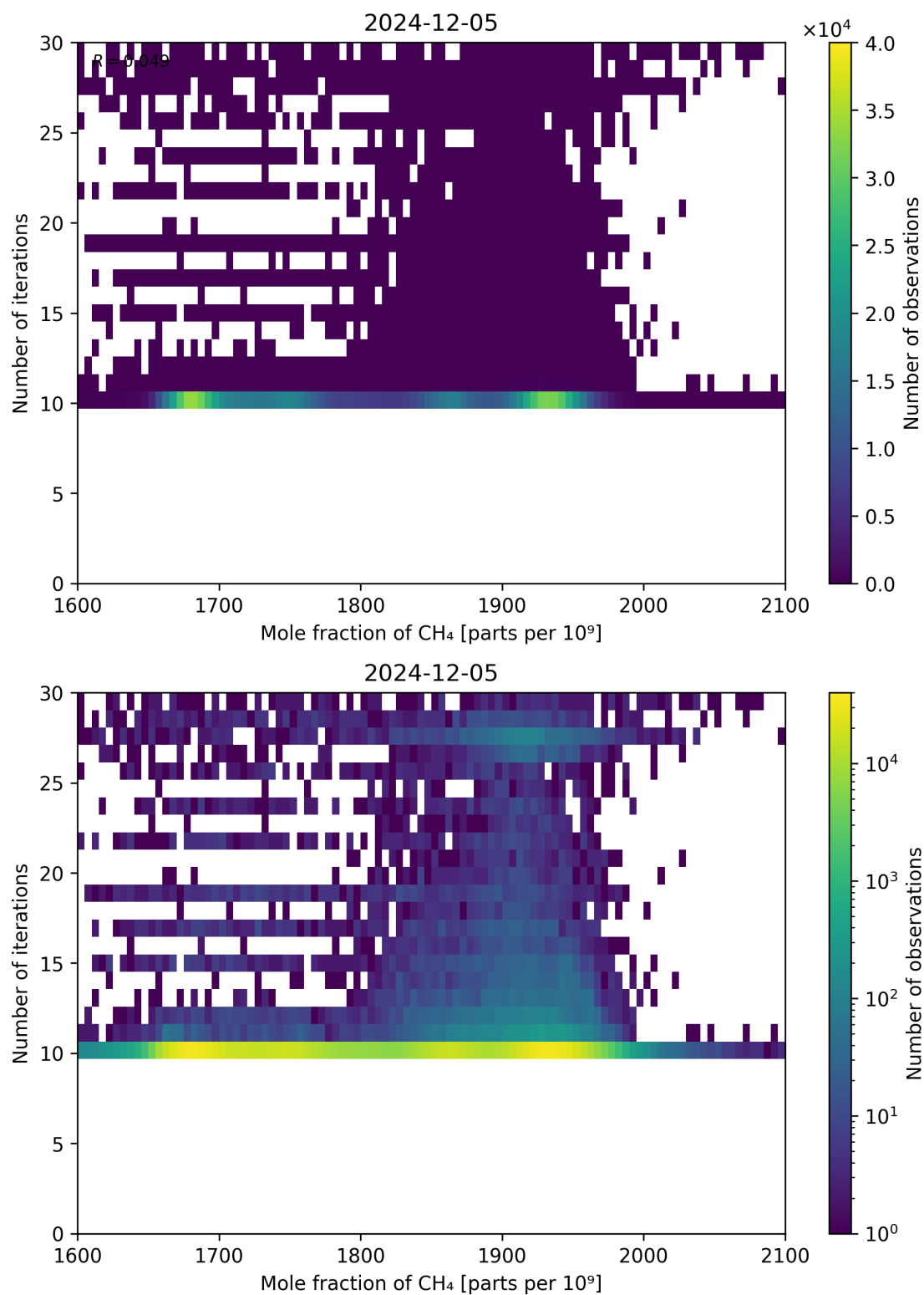
Figure 76: Scatter density plot of “Mole fraction of CH 4 ” against “Number of iterations” for 2024-12-04 to 2024-12-06.
