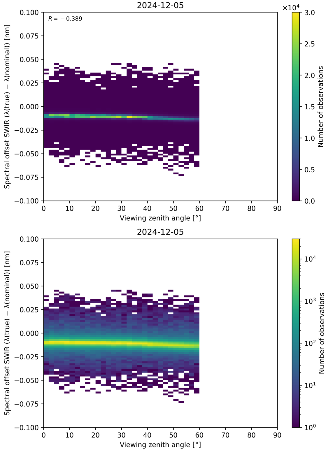
Figure 116: Scatter density plot of “Viewing zenith angle” against “Spectral offset SWIR ( \lambda_{\text{true}} - \lambda_{\text{nominal}} )” for 2024-12-04 to 2024-12-06.
