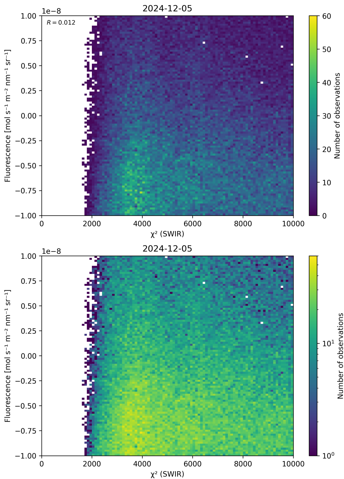
Figure 49: Scatter density plot of “ \chi^2 (SWIR)” against “Fluorescence” for 2024-12-04 to 2024-12-06.
