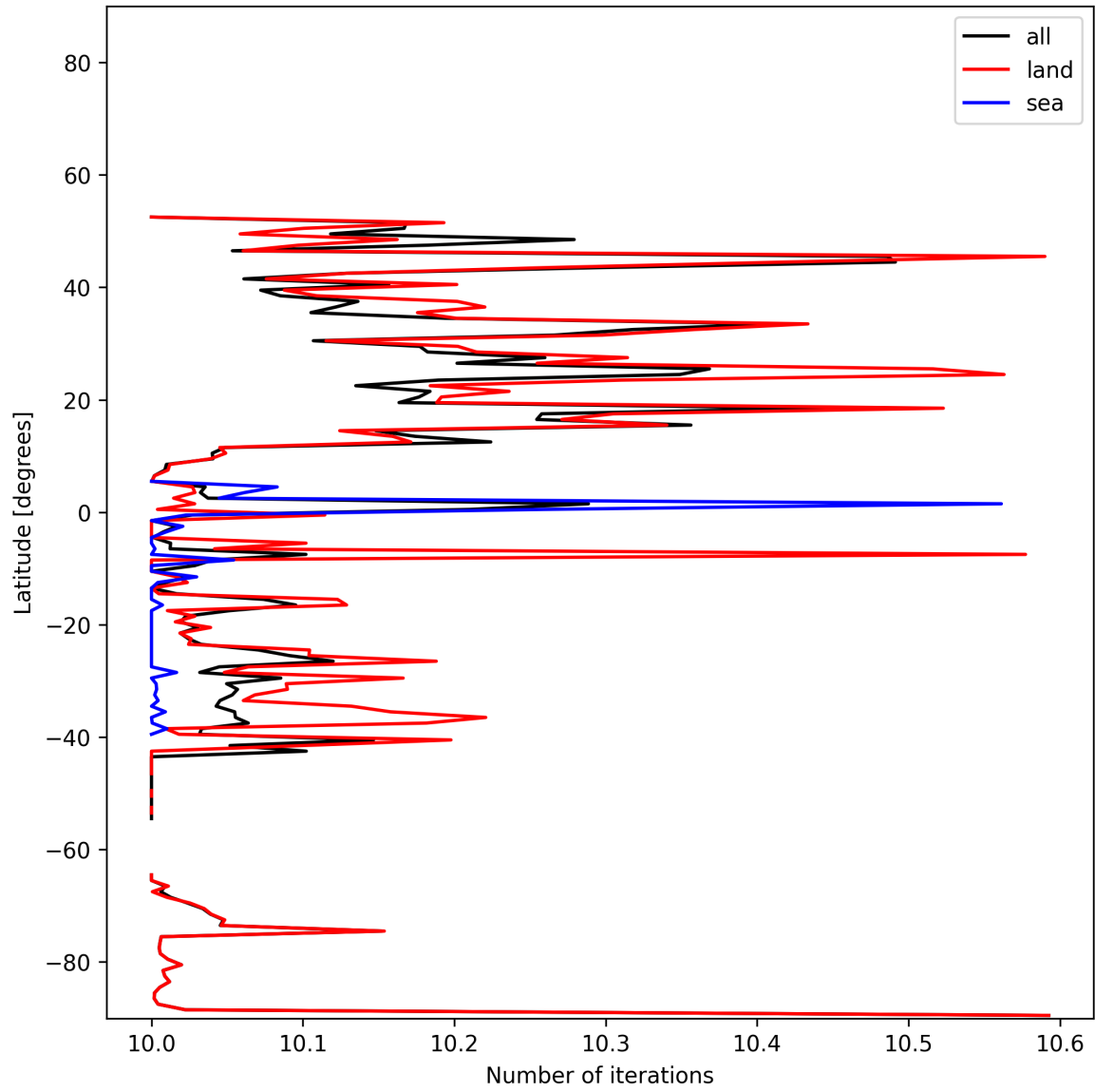
Figure 20: Zonal average of “Number of iterations” for 2024-12-04 to 2024-12-06.
