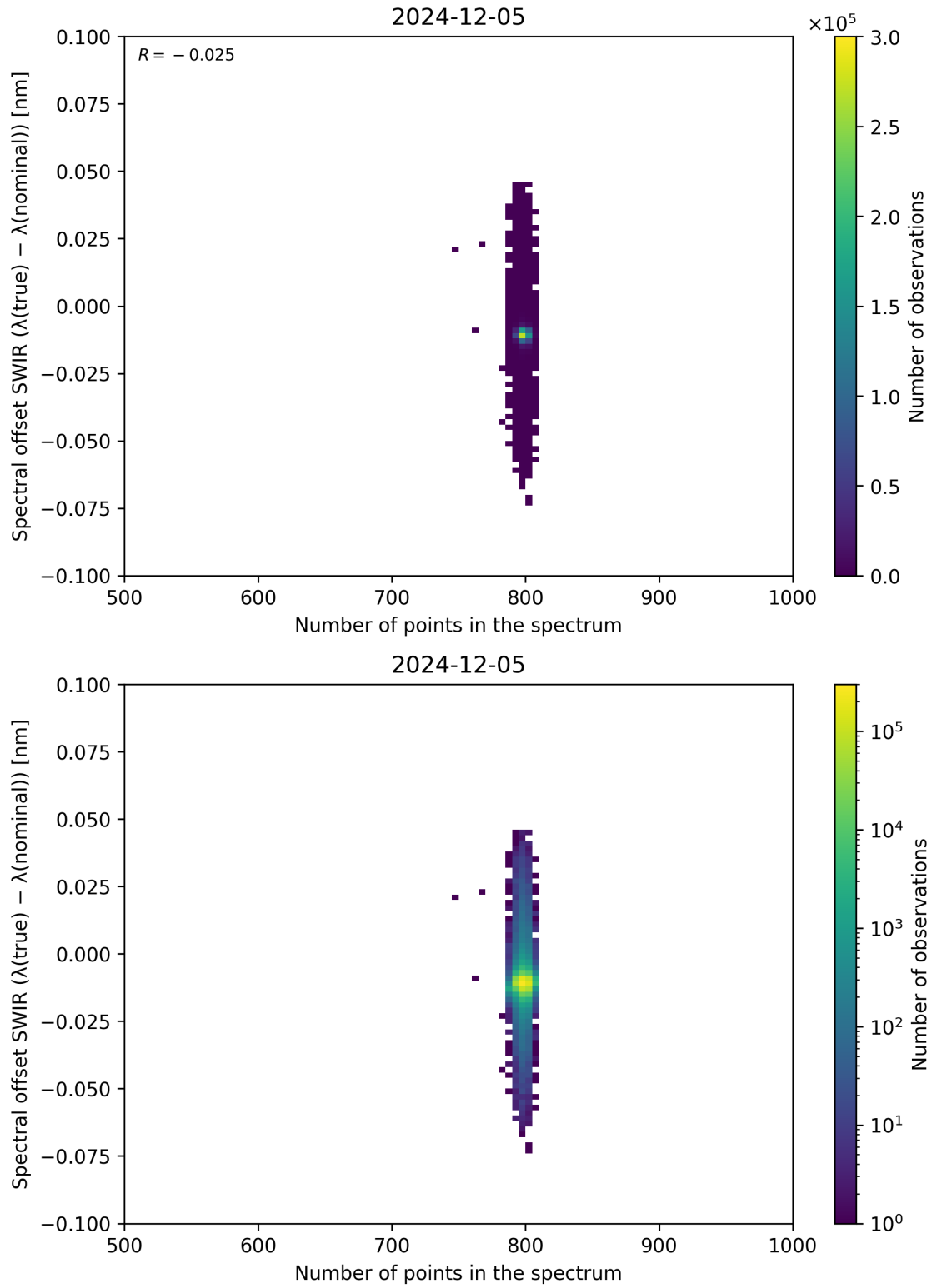
Figure 93: Scatter density plot of “Number of points in the spectrum” against “Spectral offset SWIR ( \lambda_{\text{true}} - \lambda_{\text{nominal}} )” for 2024-12-04 to 2024-12-06.
