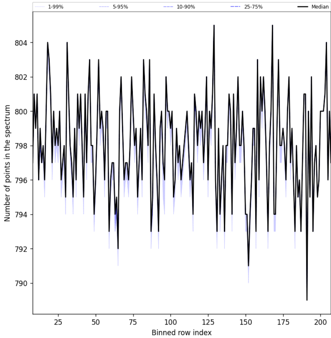
Figure 37: Along track statistics of “Number of points in the spectrum” for 2024-12-04 to 2024-12-06
