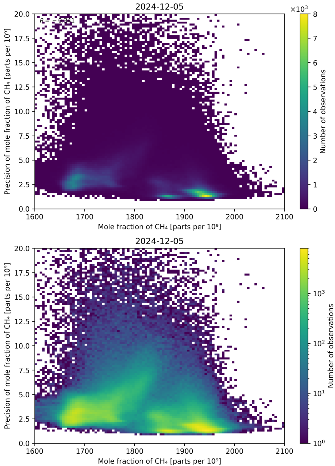
Figure 75: Scatter density plot of “Mole fraction of CH 4 ” against “Precision of mole fraction of CH 4 ” for 2024-12-04 to 2024-12-06.
