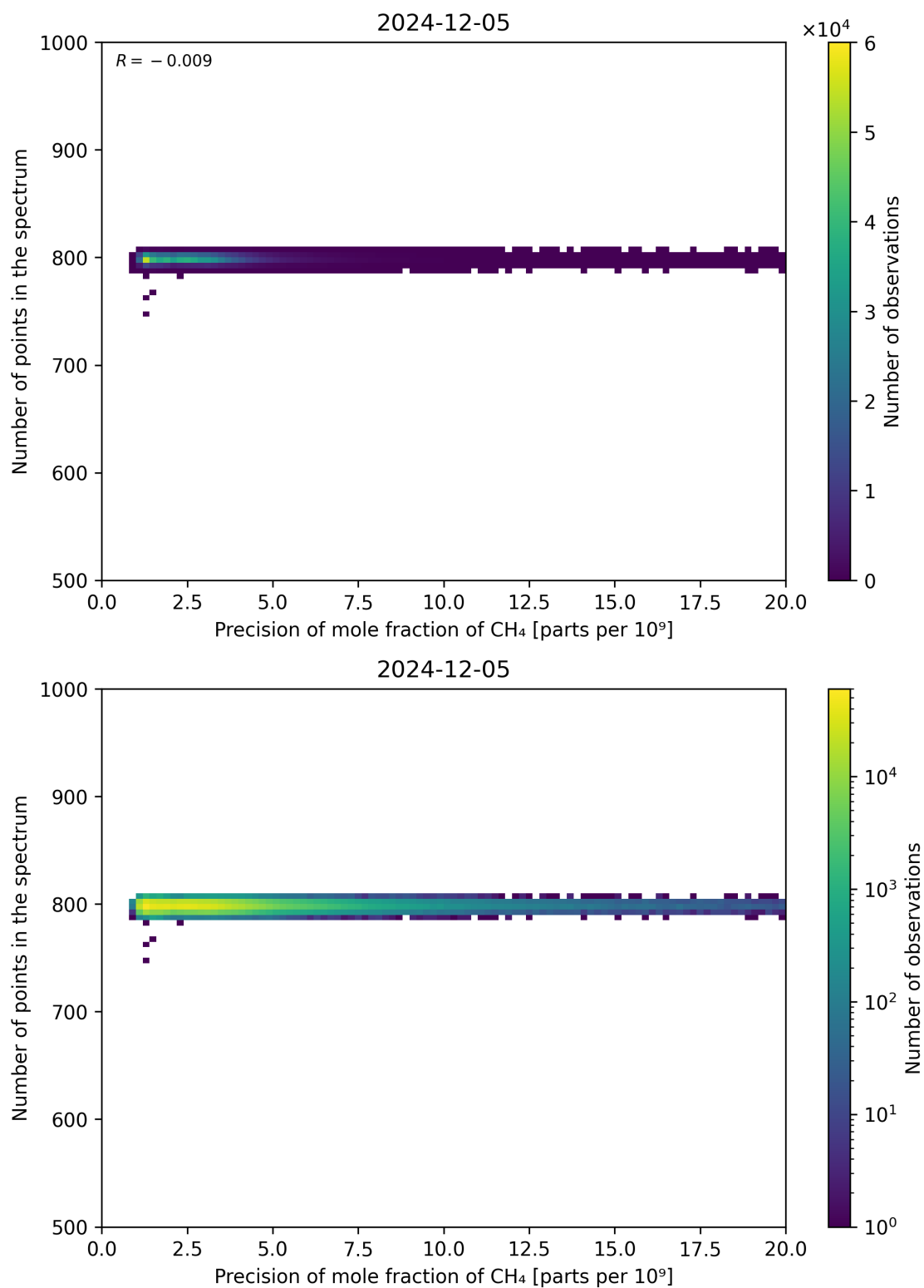
Figure 84: Scatter density plot of “Precision of mole fraction of CH 4 ” against “Number of points in the spectrum” for 2024-12-04 to 2024-12-06.
