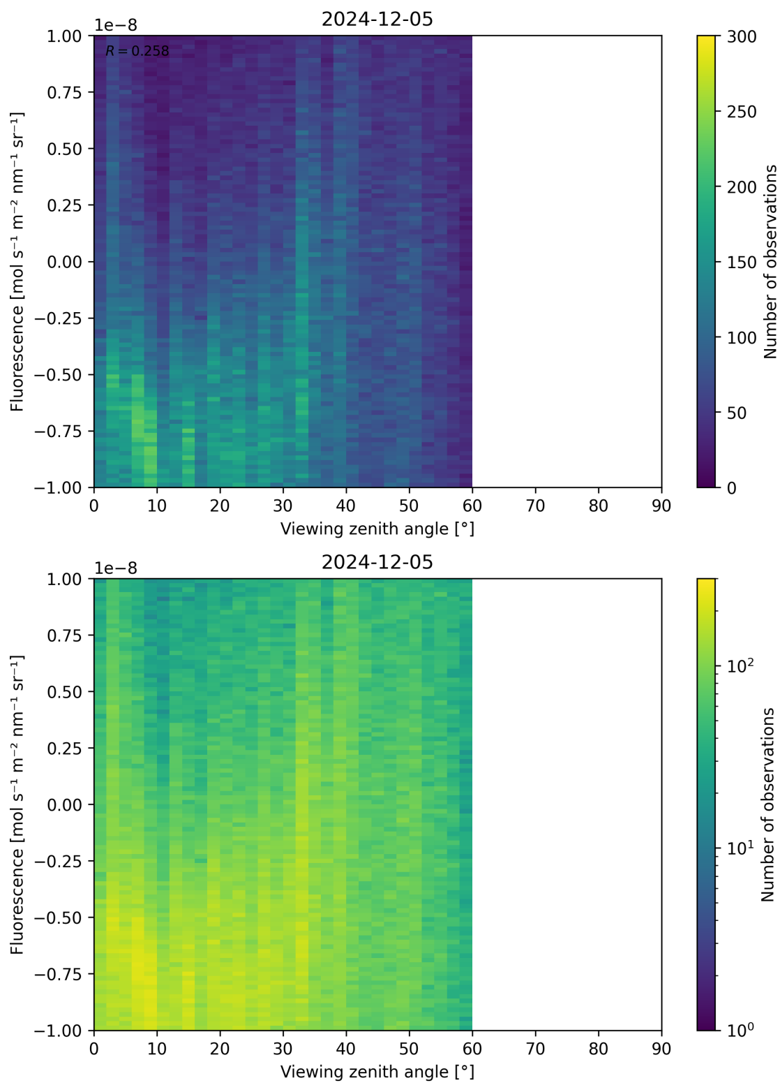
Figure 108: Scatter density plot of “Viewing zenith angle” against “Fluorescence” for 2024-12-04 to 2024-12-06.
