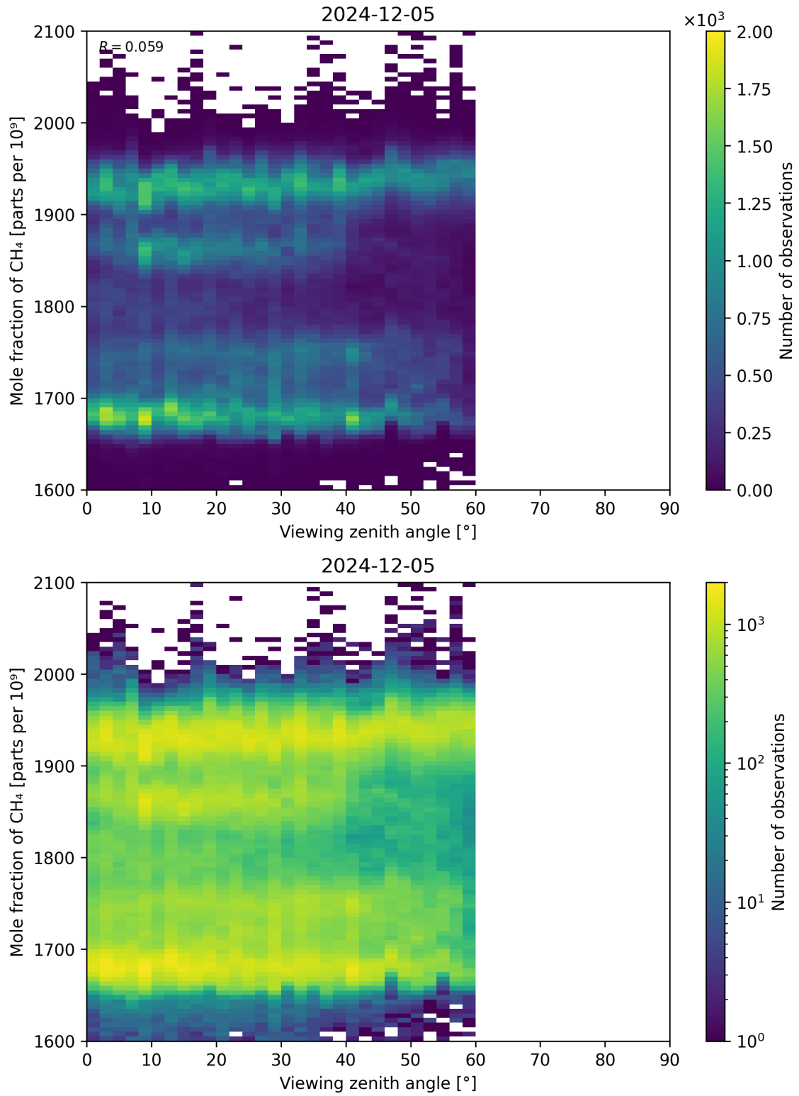
Figure 110: Scatter density plot of “Viewing zenith angle” against “Mole fraction of CH 4 ” for 2024-12-04 to 2024-12-06.
