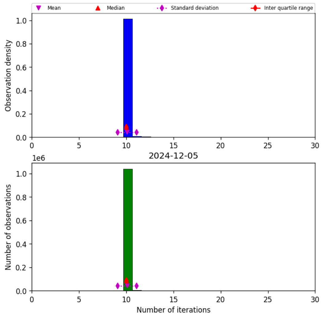
Figure 31: Histogram of “Number of iterations” for 2024-12-04 to 2024-12-06
