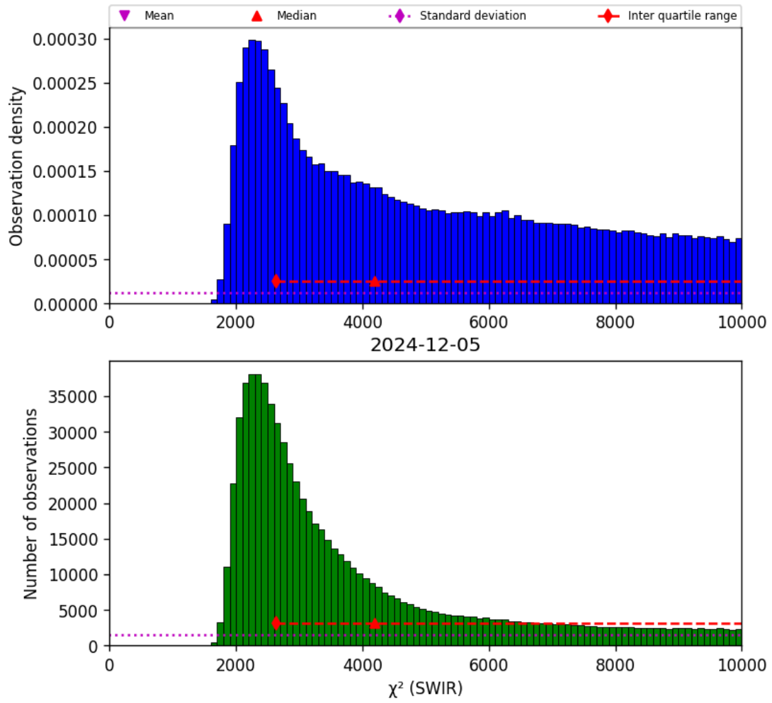
Figure 28: Histogram of “ \chi^2 (SWIR)” for 2024-12-04 to 2024-12-06
