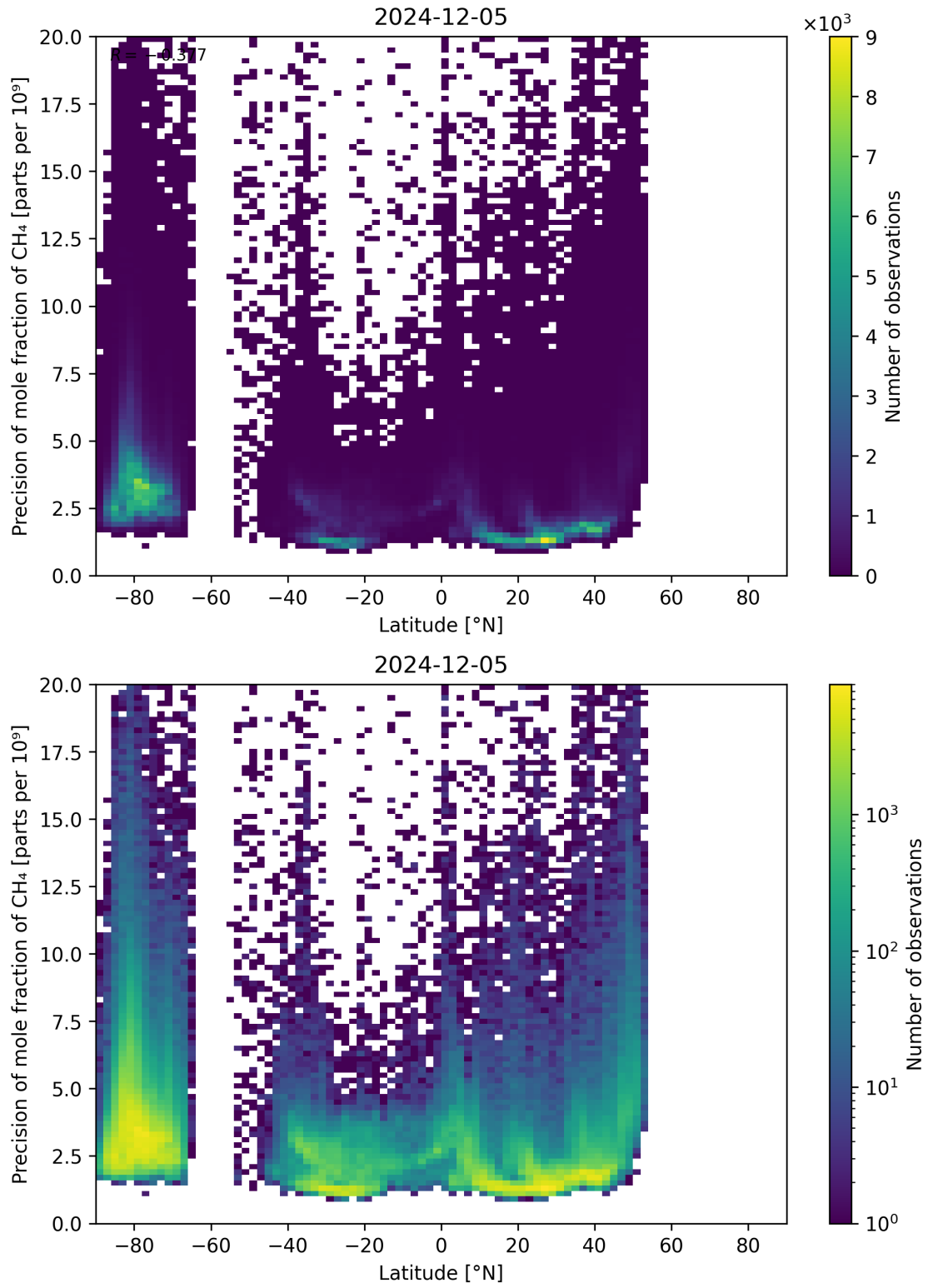
Figure 59: Scatter density plot of “Latitude” against “Precision of mole fraction of CH 4 ” for 2024-12-04 to 2024-12-06.
