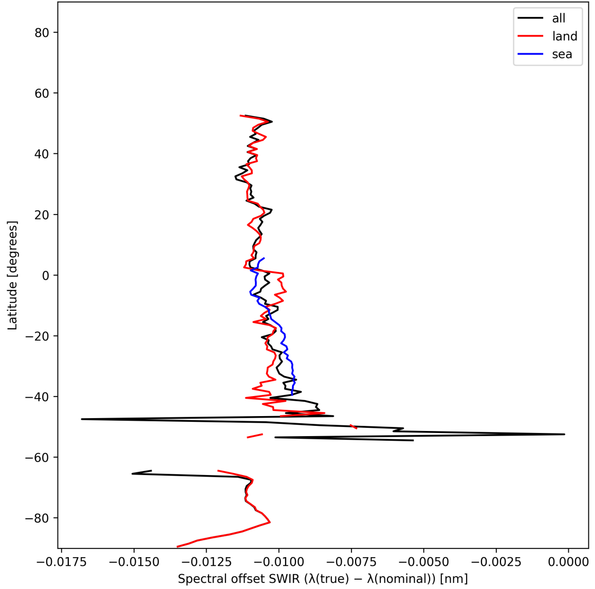
Figure 16: Zonal average of “Spectral offset SWIR ( \lambda_{\text{true}} - \lambda_{\text{nominal}} )” for 2024-12-04 to 2024-12-06.
