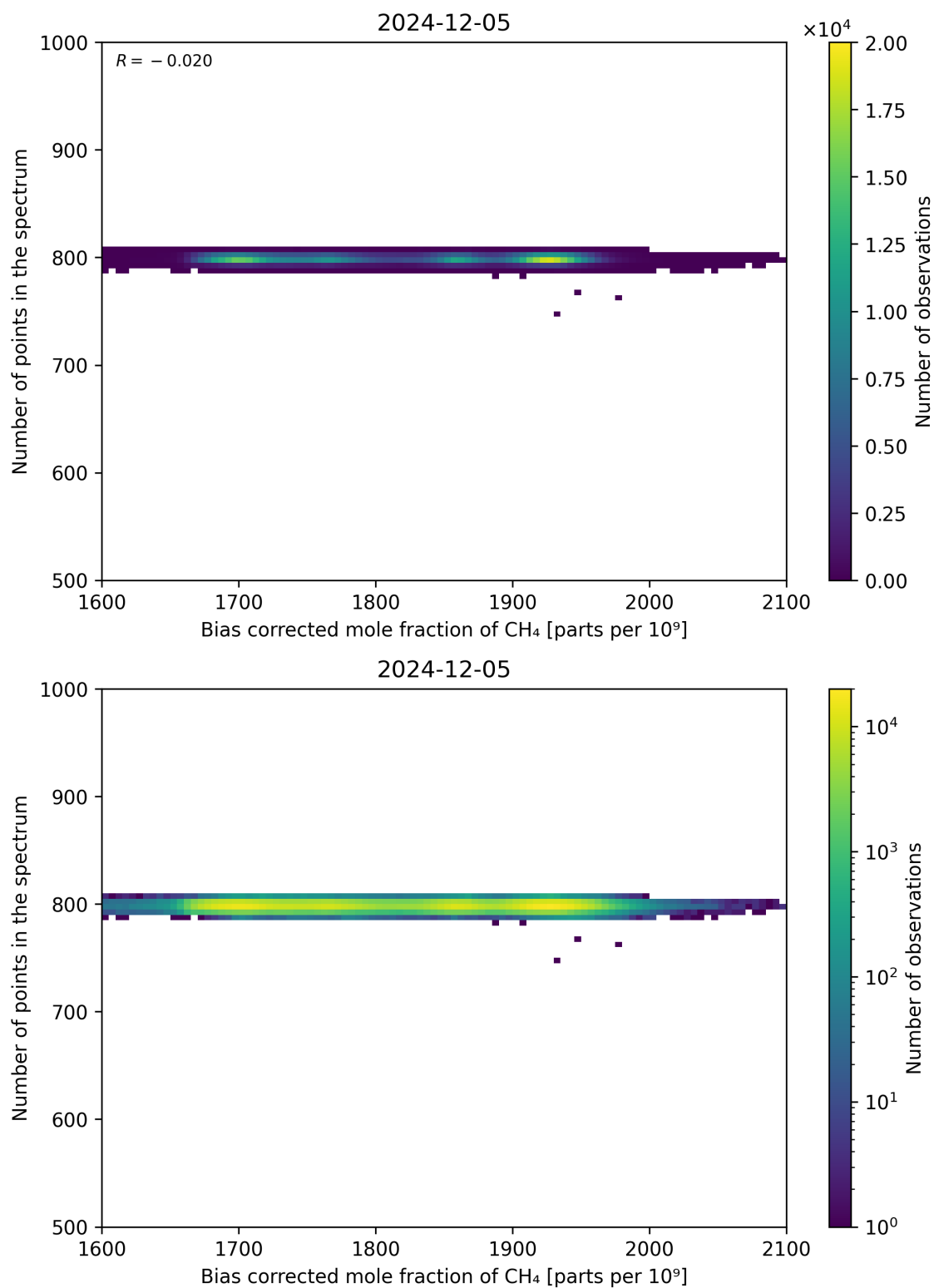
Figure 68: Scatter density plot of “Bias corrected mole fraction of CH 4 ” against “Number of points in the spectrum” for 2024-12-04 to 2024-12-06.
