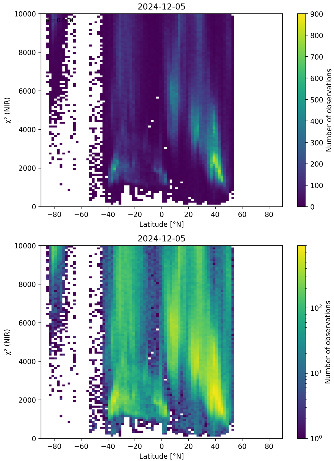
Figure 53: Scatter density plot of “Latitude” against “ \chi^2 (NIR)” for 2024-12-04 to 2024-12-06.
