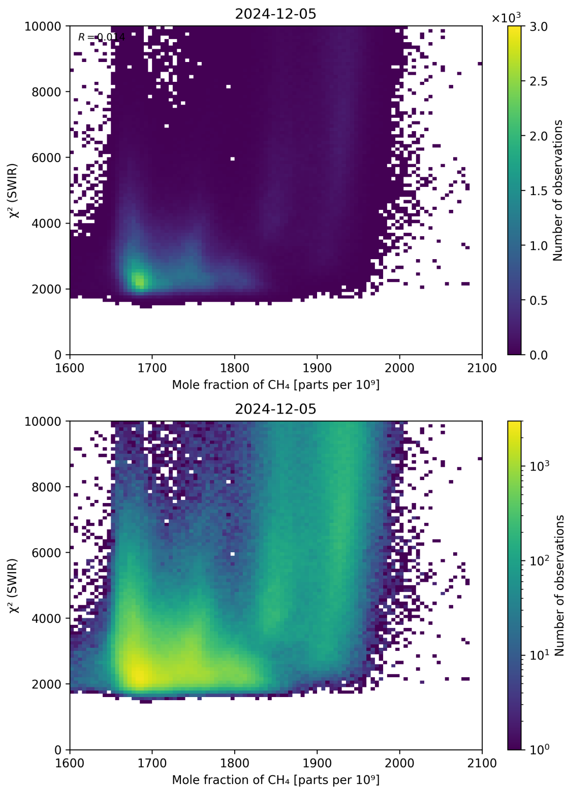
Figure 71: Scatter density plot of “Mole fraction of \text{CH}_4 ” against “ \chi^2 (SWIR)” for 2024-12-04 to 2024-12-06.
