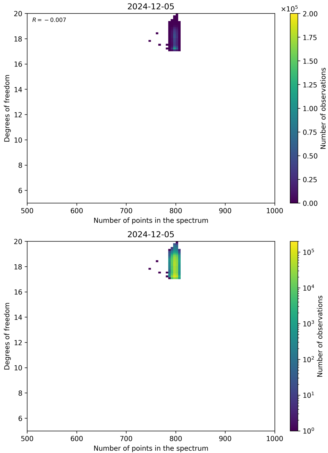
Figure 90: Scatter density plot of “Number of points in the spectrum” against “Degrees of freedom” for 2024-12-04 to 2024-12-06.
