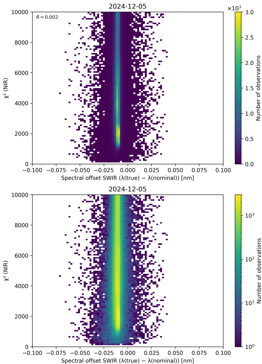
Figure 117: Scatter density plot of “Spectral offset SWIR ( \lambda_{\text{true}} - \lambda_{\text{nominal}} )” against “ \chi^2 (NIR)” for 2024-12-04 to 2024-12-06.
