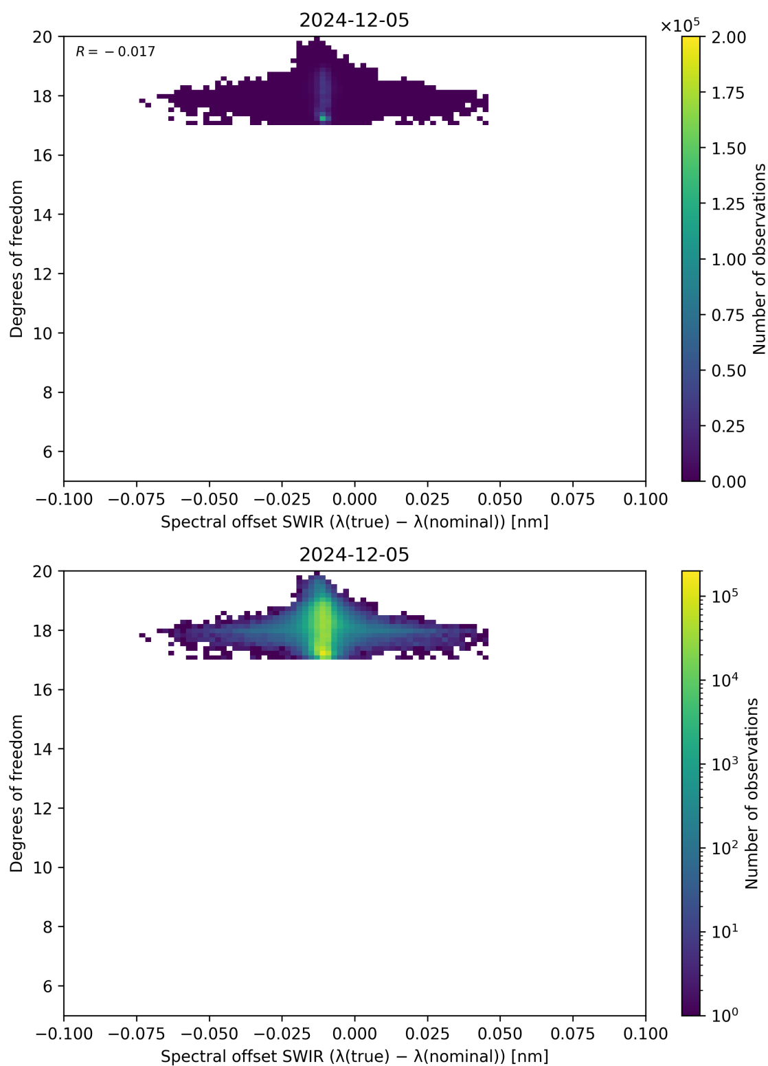
Figure 119: Scatter density plot of “Spectral offset SWIR ( \lambda_{\text{true}} - \lambda_{\text{nominal}} )” against “Degrees of freedom” for 2024-12-04 to 2024-12-06.
