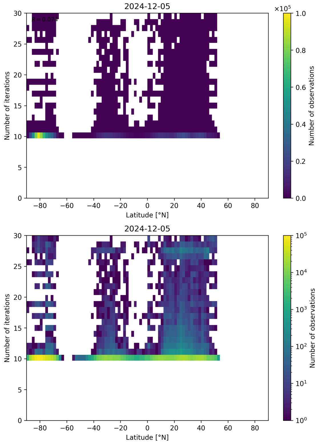
Figure 60: Scatter density plot of “Latitude” against “Number of iterations” for 2024-12-04 to 2024-12-06.
