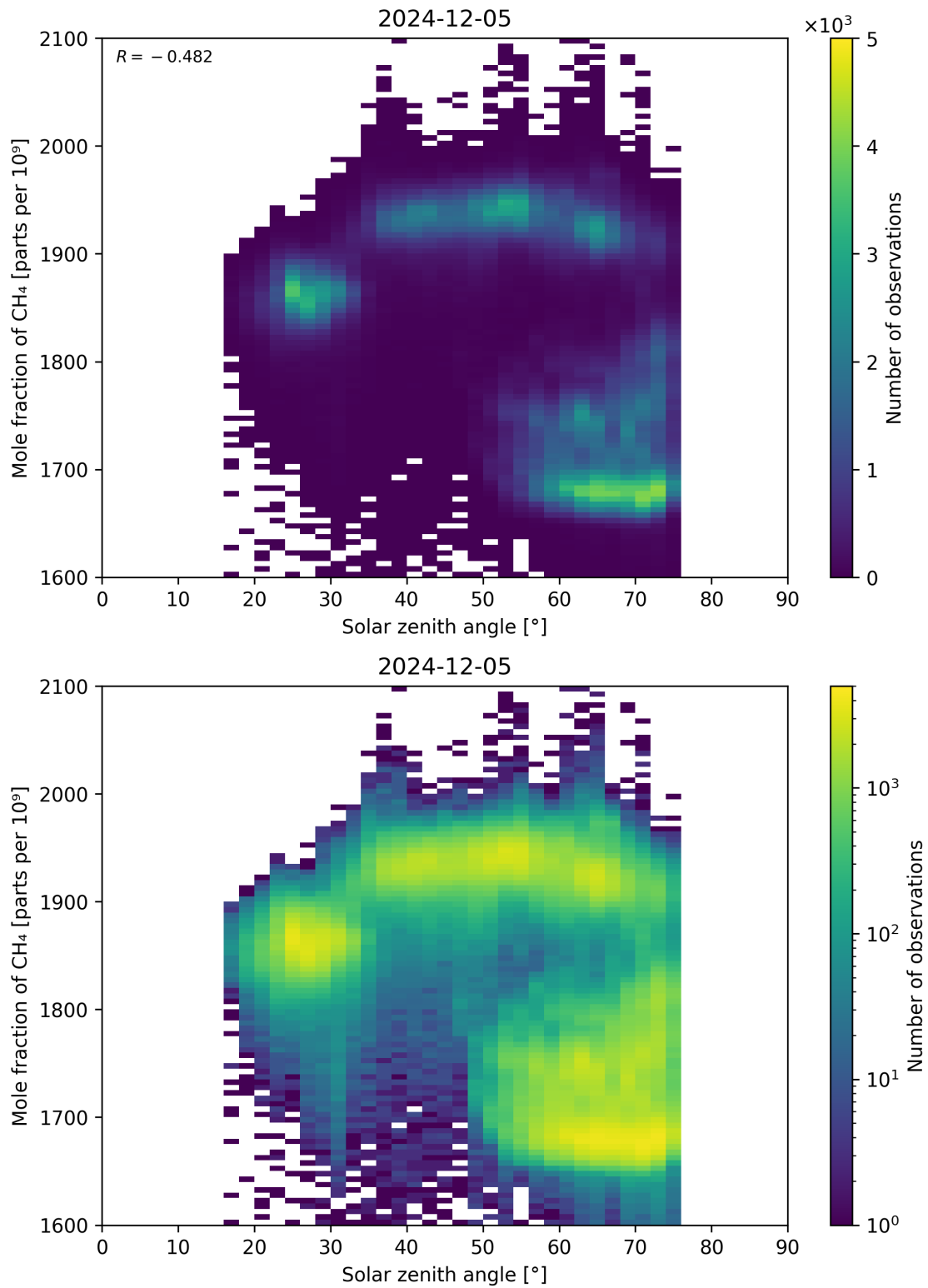
Figure 99: Scatter density plot of “Solar zenith angle” against “Mole fraction of CH 4 ” for 2024-12-04 to 2024-12-06.
