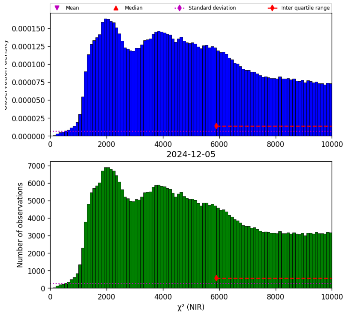
Figure 29: Histogram of “ \chi^2 (NIR)” for 2024-12-04 to 2024-12-06
