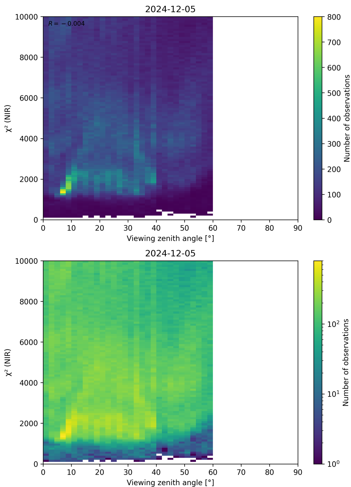
Figure 105: Scatter density plot of “Viewing zenith angle” against “ \chi^2 (NIR)” for 2024-12-04 to 2024-12-06.
