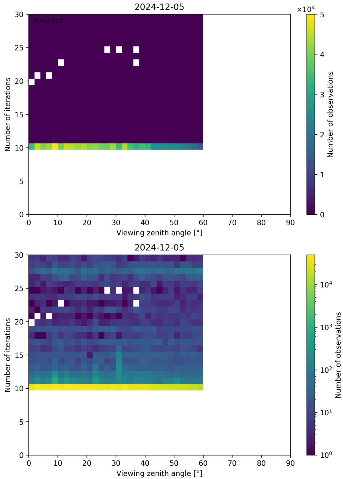
Figure 113: Scatter density plot of “Viewing zenith angle” against “Number of iterations” for 2024-12-04 to 2024-12-06.
