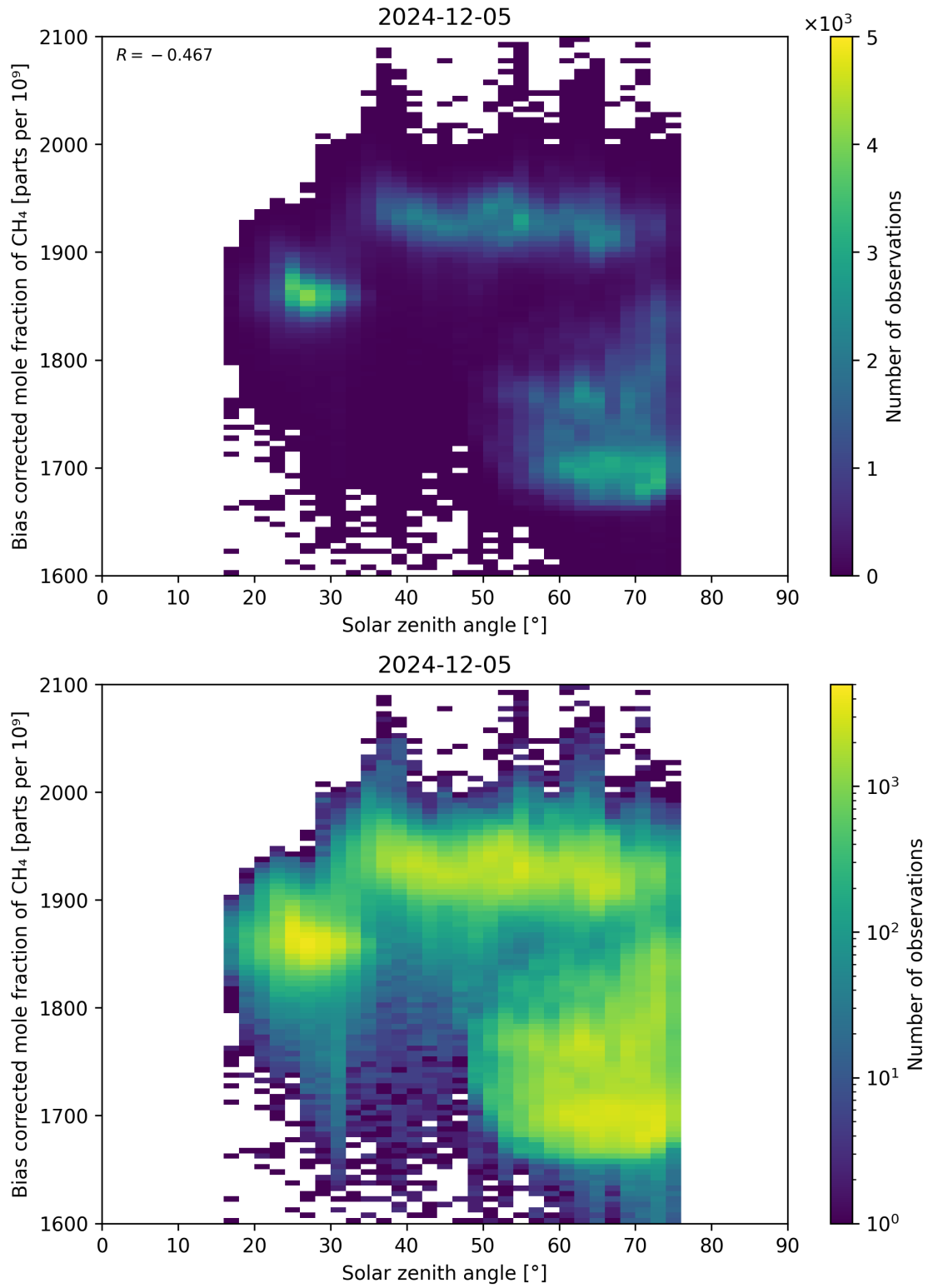
Figure 100: Scatter density plot of “Solar zenith angle” against “Bias corrected mole fraction of CH 4 ” for 2024-12-04 to 2024-12-06.
