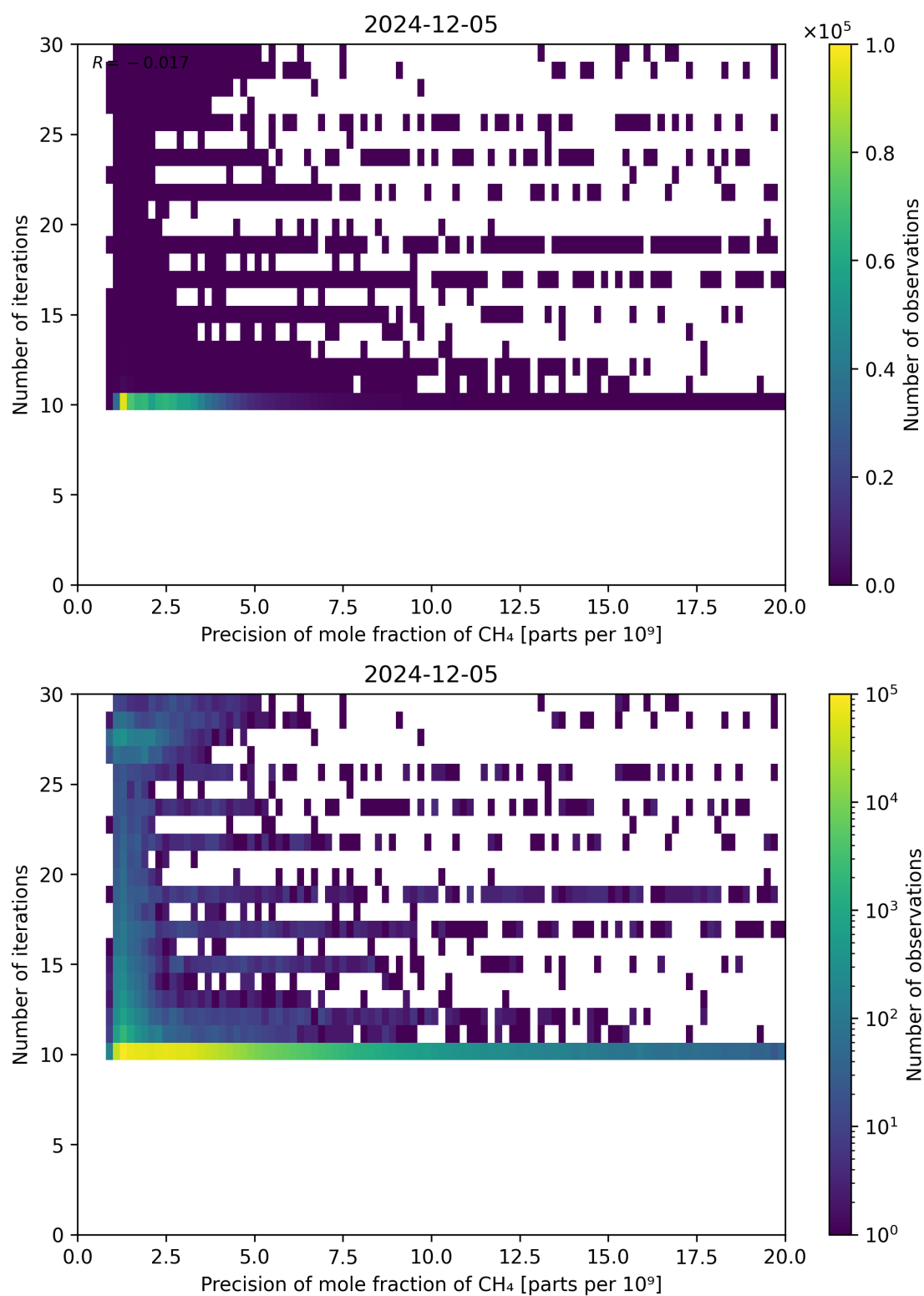
Figure 83: Scatter density plot of “Precision of mole fraction of CH 4 ” against “Number of iterations” for 2024-12-04 to 2024-12-06.
