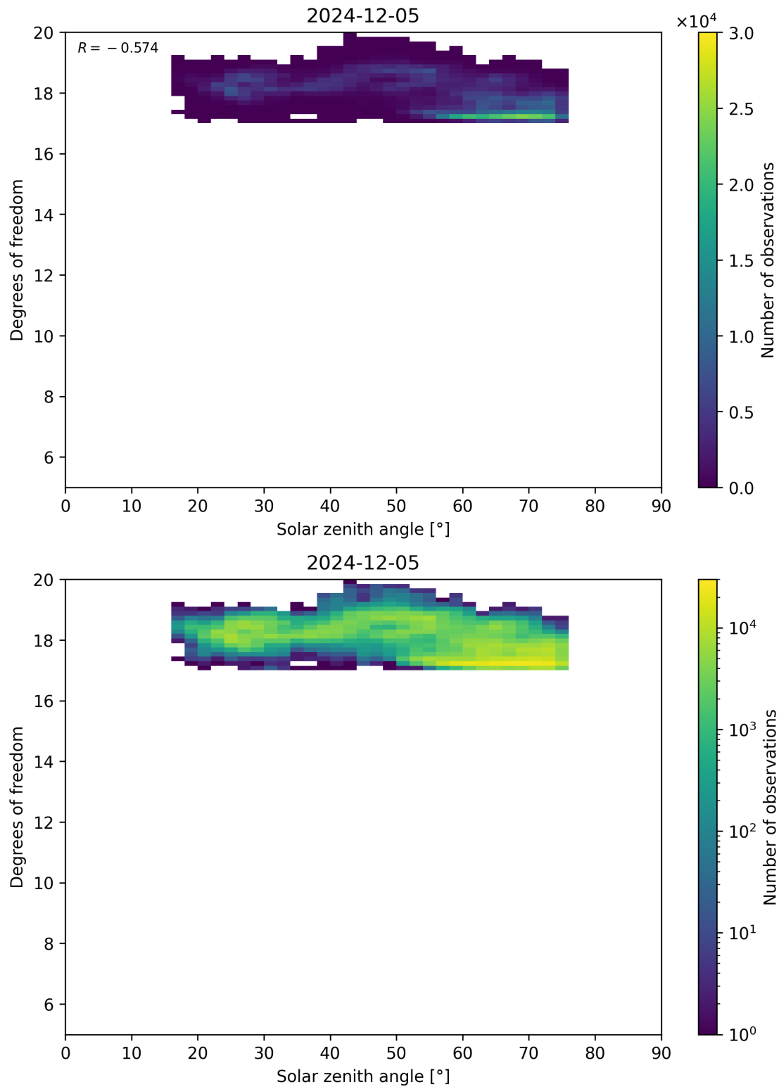
Figure 96: Scatter density plot of “Solar zenith angle” against “Degrees of freedom” for 2024-12-04 to 2024-12-06.
