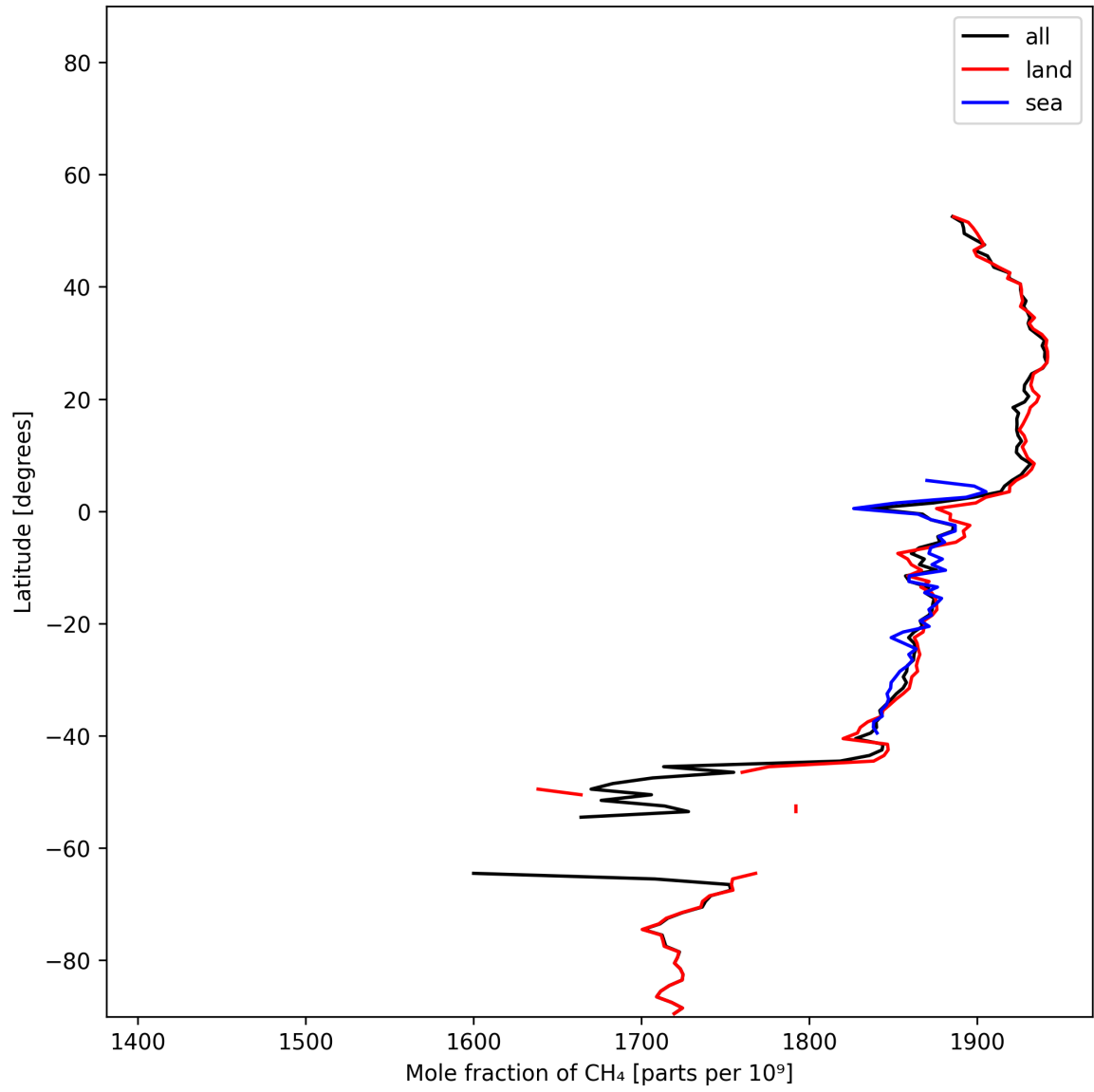
Figure 12: Zonal average of “Mole fraction of CH 4 ” for 2024-12-04 to 2024-12-06.
