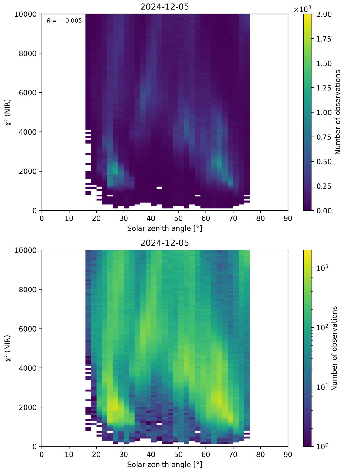
Figure 94: Scatter density plot of “Solar zenith angle” against “ \chi^2 (NIR)” for 2024-12-04 to 2024-12-06.
