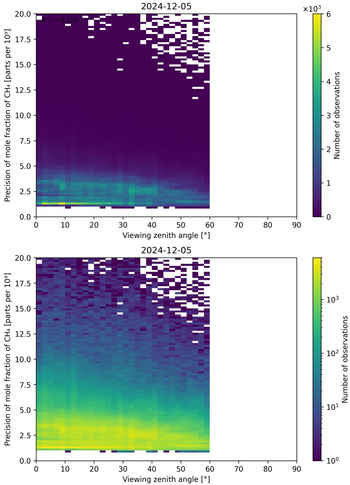
Figure 112: Scatter density plot of “Viewing zenith angle” against “Precision of mole fraction of \text{CH}_4 ” for 2024-12-04 to 2024-12-06.
