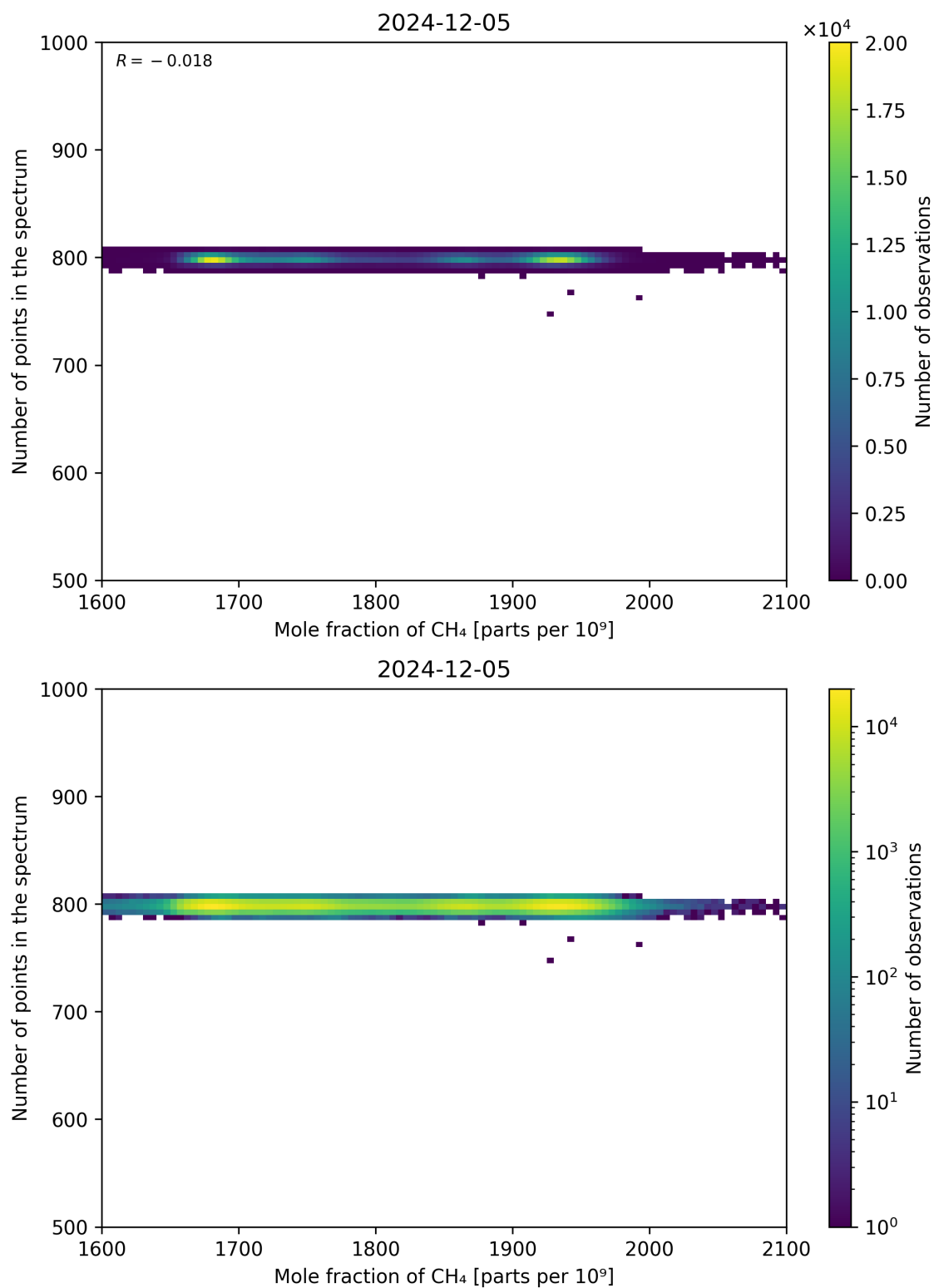
Figure 77: Scatter density plot of “Mole fraction of CH 4 ” against “Number of points in the spectrum” for 2024-12-04 to 2024-12-06.
