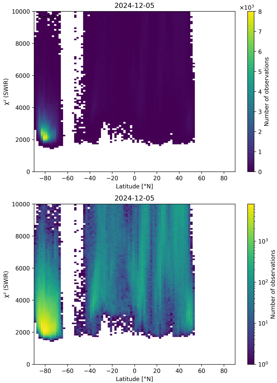
Figure 54: Scatter density plot of “Latitude” against “ \chi^2 (SWIR)” for 2024-12-04 to 2024-12-06.
