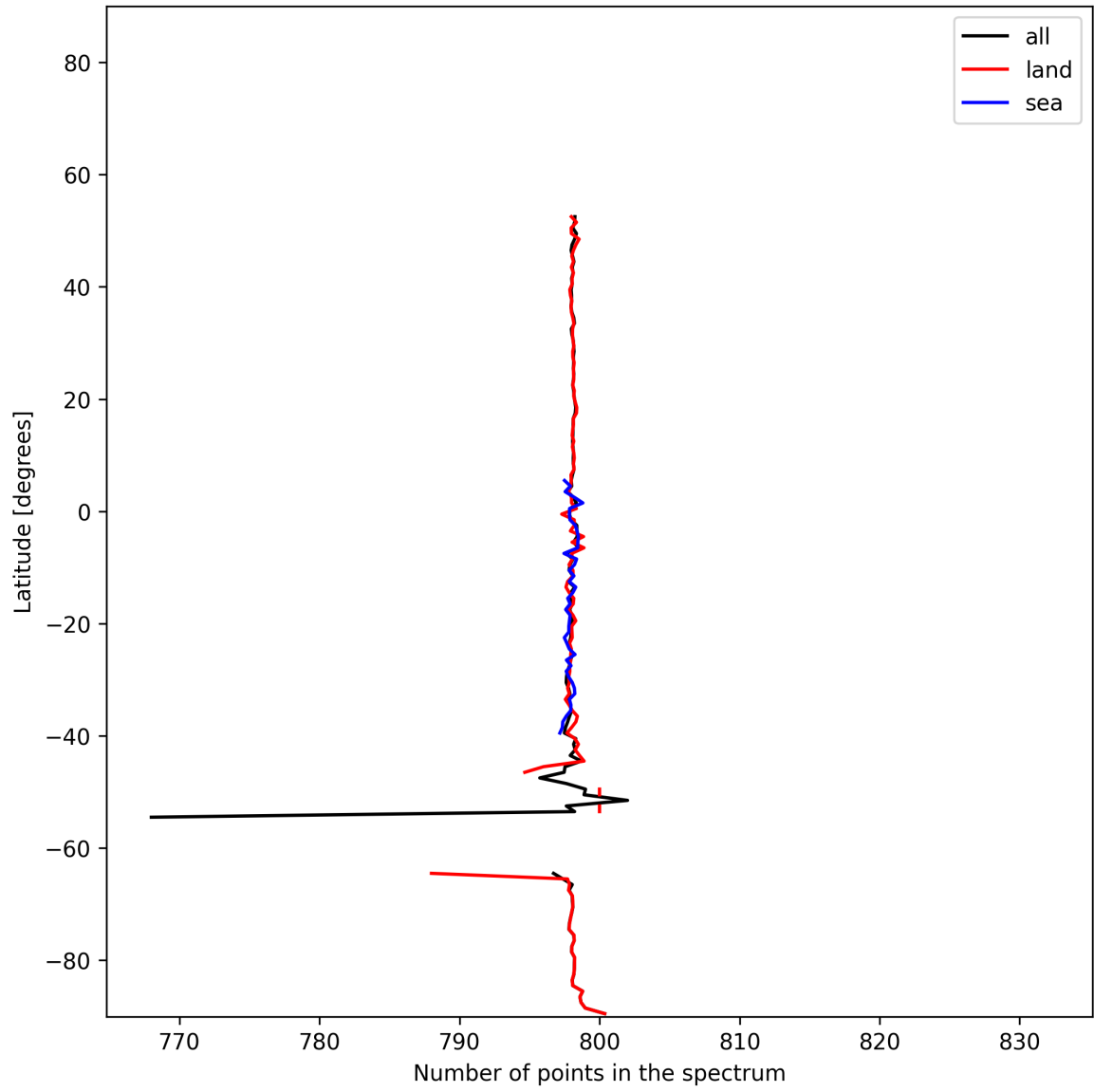
Figure 15: Zonal average of “Number of points in the spectrum” for 2024-12-04 to 2024-12-06.
