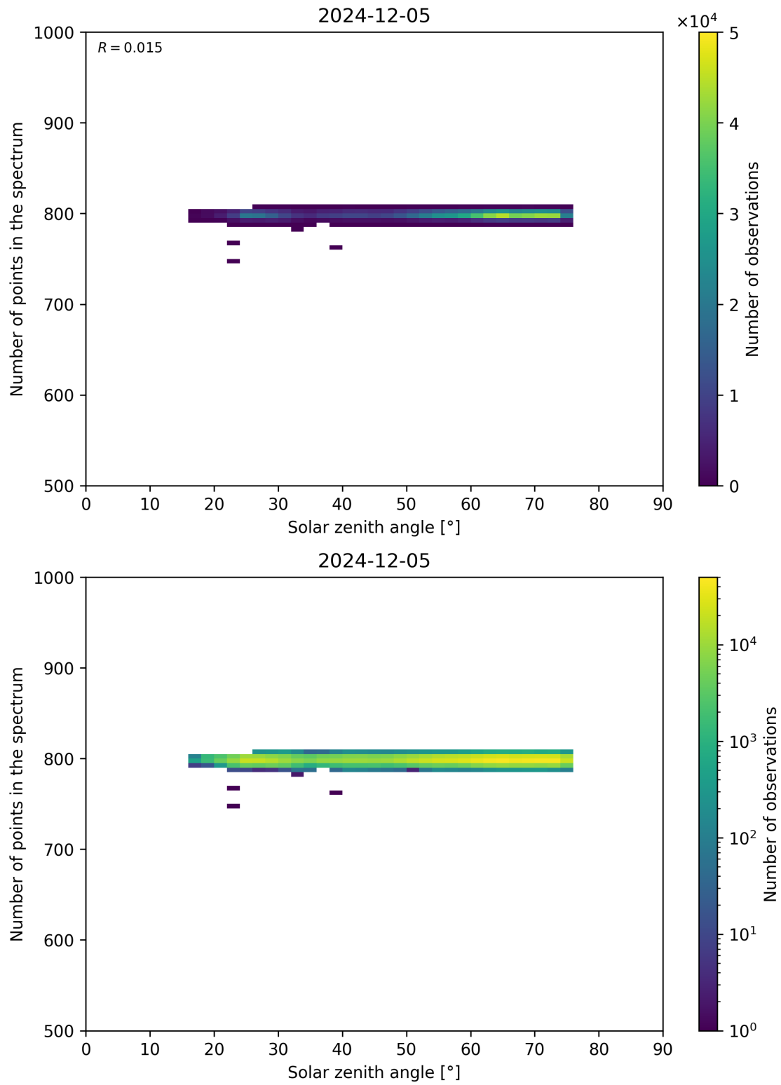
Figure 103: Scatter density plot of “Solar zenith angle” against “Number of points in the spectrum” for 2024-12-04 to 2024-12-06.
