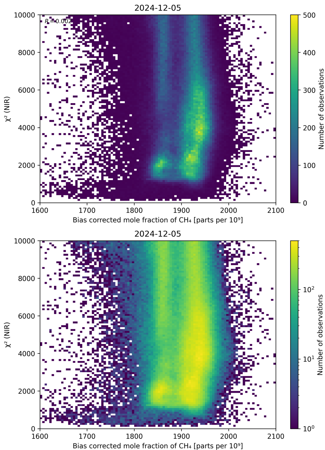
Figure 63: Scatter density plot of “Bias corrected mole fraction of \text{CH}_4 ” against “ \chi^2 (NIR)” for 2024-12-04 to 2024-12-06.
