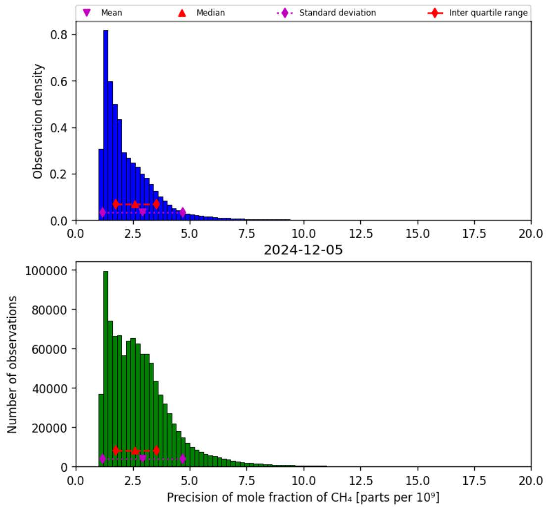
Figure 24: Histogram of “Precision of mole fraction of CH 4 ” for 2024-12-04 to 2024-12-06
