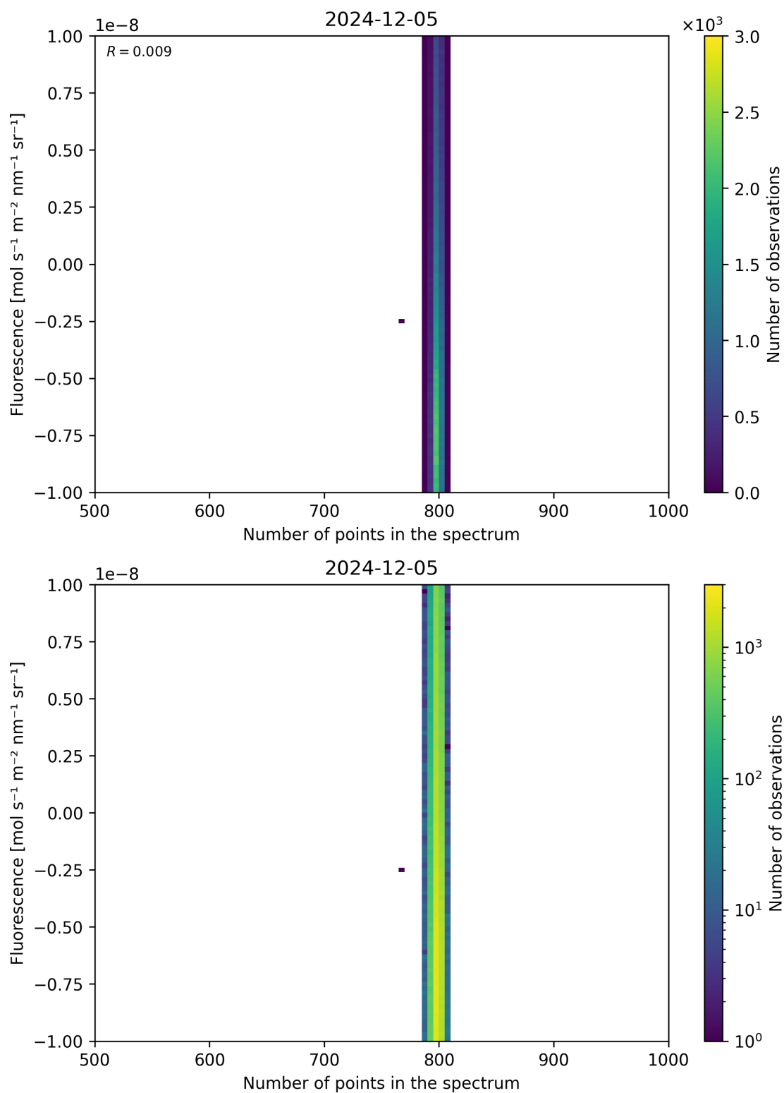
Figure 91: Scatter density plot of “Number of points in the spectrum” against “Fluorescence” for 2024-12-04 to 2024-12-06.
