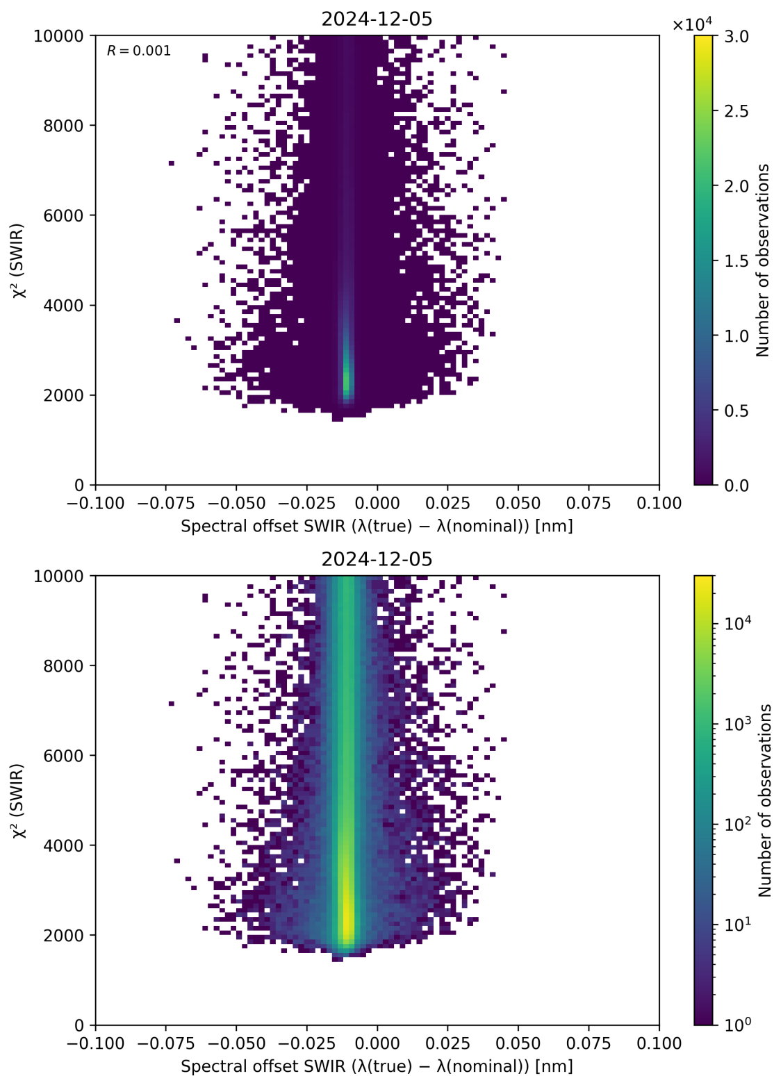
Figure 118: Scatter density plot of “Spectral offset SWIR ( \lambda_{\text{true}} - \lambda_{\text{nominal}} )” against “ \chi^2 (SWIR)” for 2024-12-04 to 2024-12-06.
