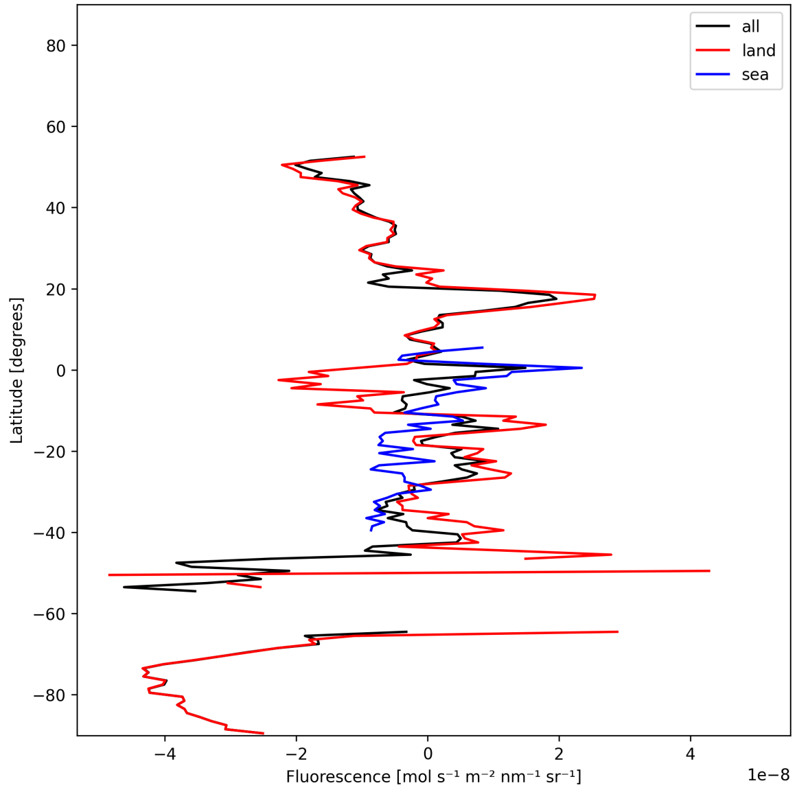
Figure 21: Zonal average of “Fluorescence” for 2024-12-04 to 2024-12-06.
