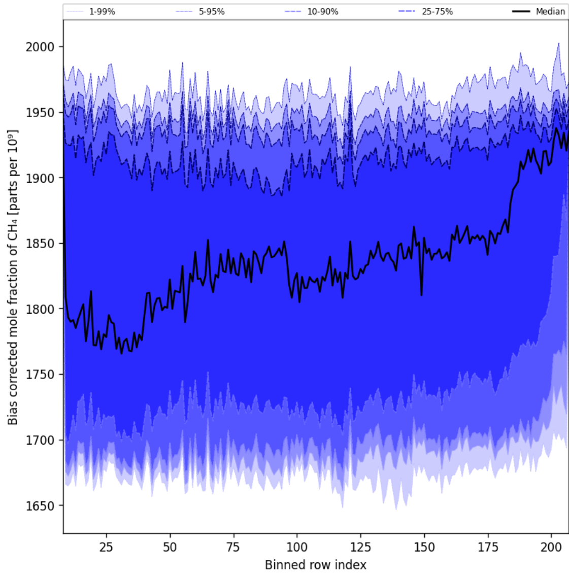
Figure 36: Along track statistics of “Bias corrected mole fraction of CH 4 ” for 2024-12-04 to 2024-12-06
