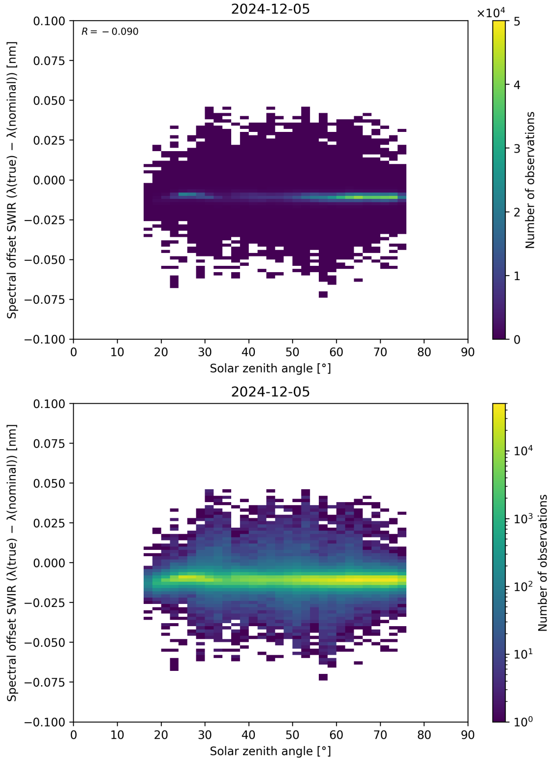
Figure 104: Scatter density plot of “Solar zenith angle” against “Spectral offset SWIR ( \lambda_{\text{true}} - \lambda_{\text{nominal}} )” for 2024-12-04 to 2024-12-06.
