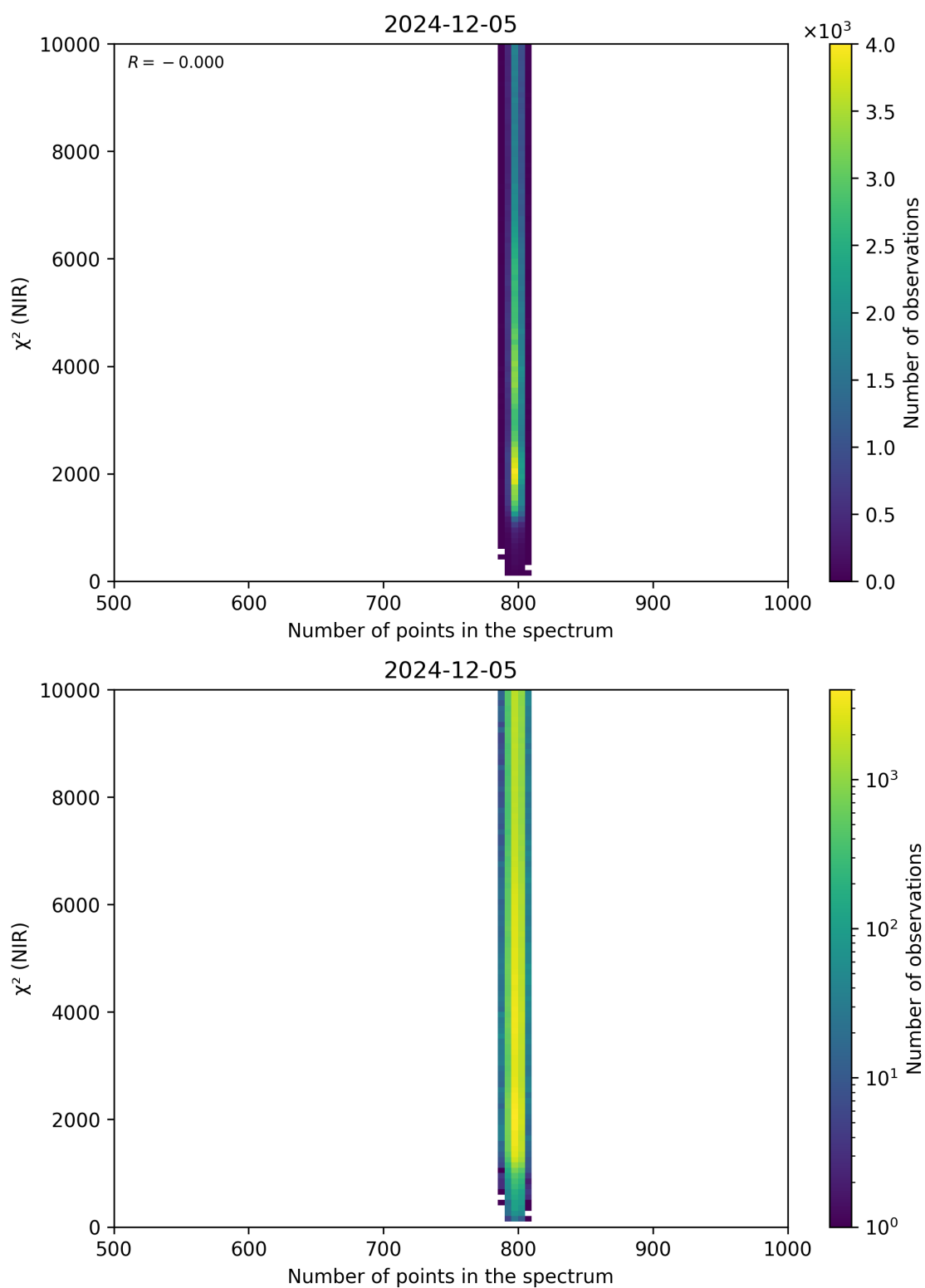
Figure 88: Scatter density plot of “Number of points in the spectrum” against “ \chi^2 (NIR)” for 2024-12-04 to 2024-12-06.
