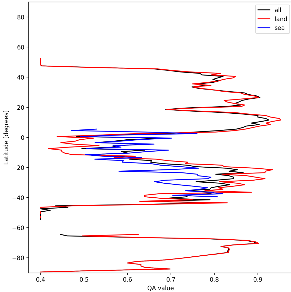
Figure 11: Zonal average of “QA value” for 2024-12-04 to 2024-12-06.
