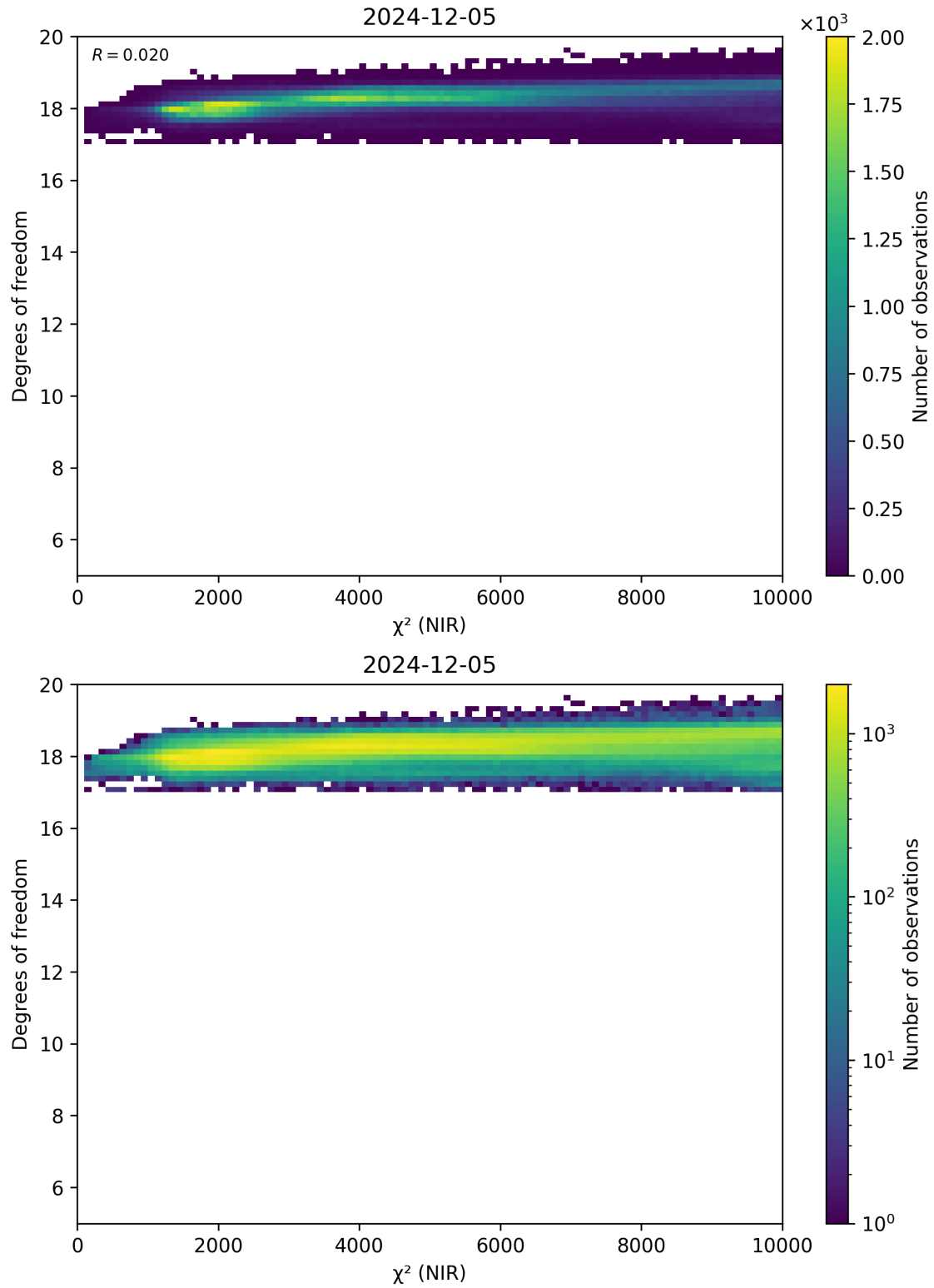
Figure 44: Scatter density plot of “ \chi^2 (NIR)” against “Degrees of freedom” for 2024-12-04 to 2024-12-06.
