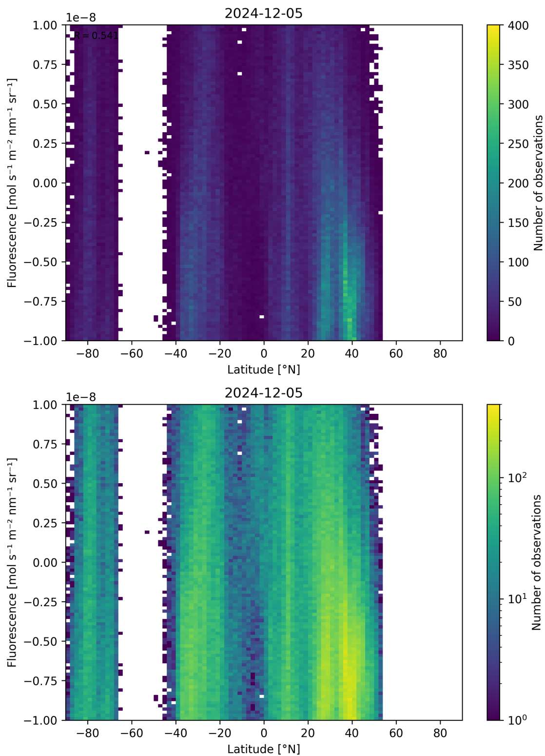
Figure 56: Scatter density plot of “Latitude” against “Fluorescence” for 2024-12-04 to 2024-12-06.
