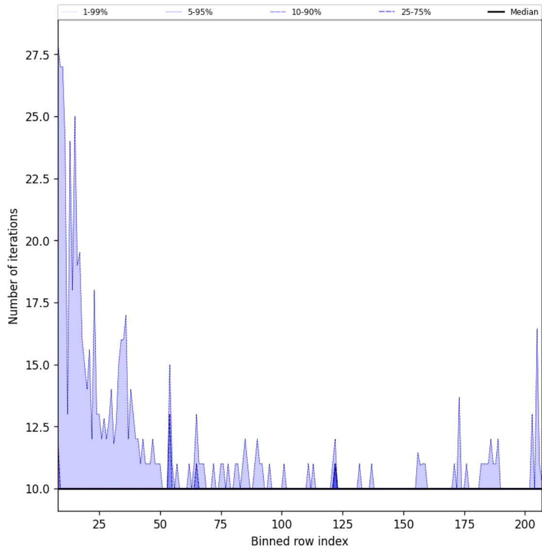
Figure 42: Along track statistics of “Number of iterations” for 2024-12-04 to 2024-12-06
