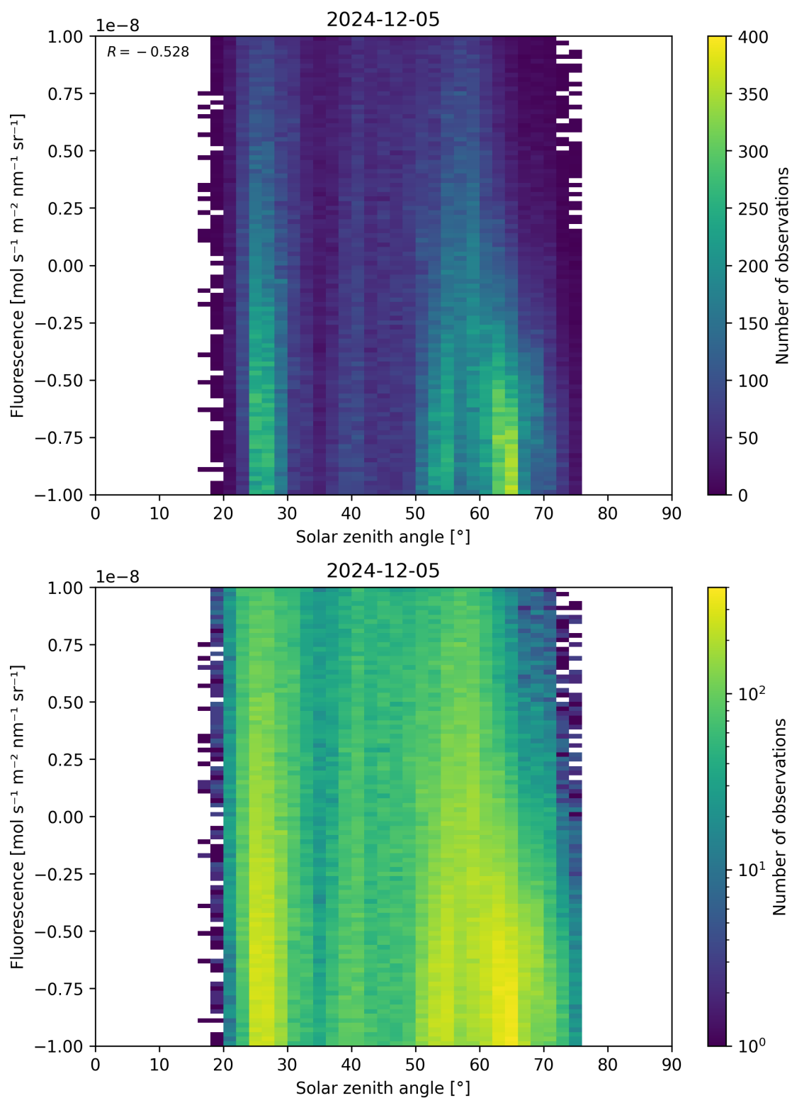
Figure 97: Scatter density plot of “Solar zenith angle” against “Fluorescence” for 2024-12-04 to 2024-12-06.
