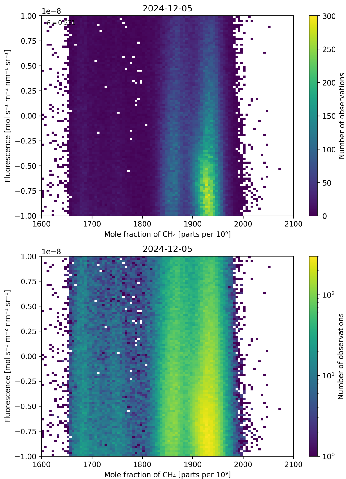
Figure 73: Scatter density plot of “Mole fraction of \text{CH}_4 ” against “Fluorescence” for 2024-12-04 to 2024-12-06.
