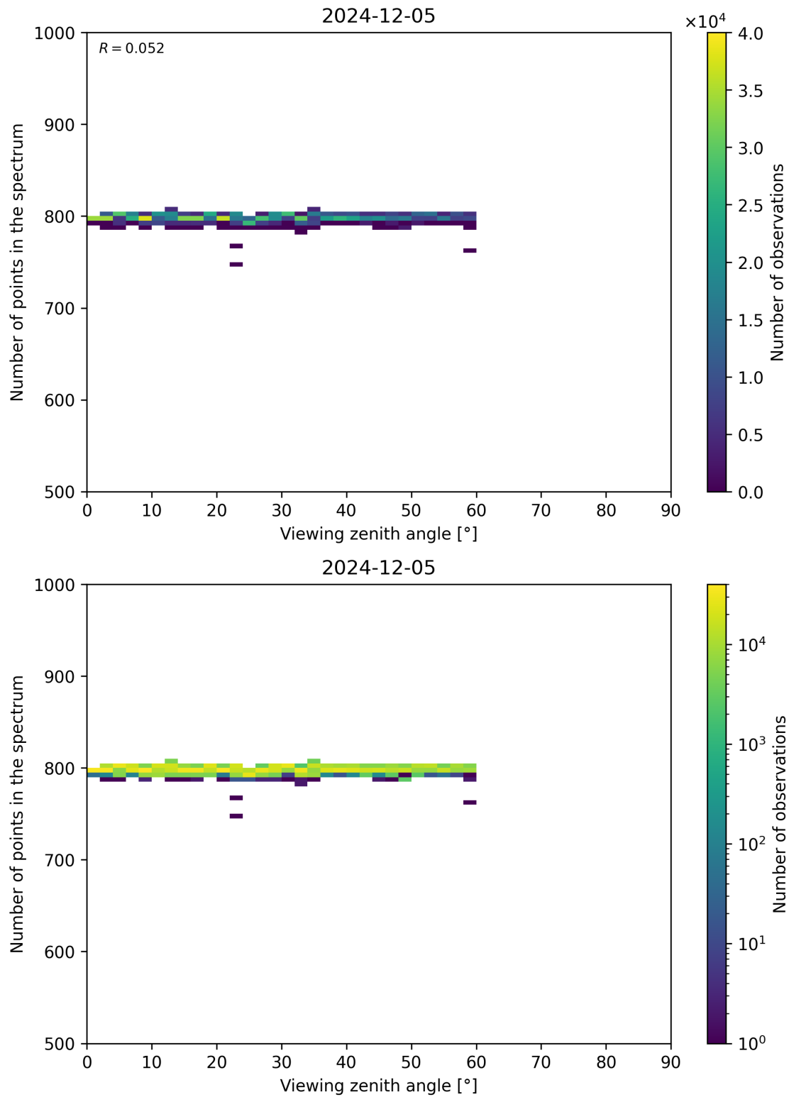
Figure 114: Scatter density plot of “Viewing zenith angle” against “Number of points in the spectrum” for 2024-12-04 to 2024-12-06.
