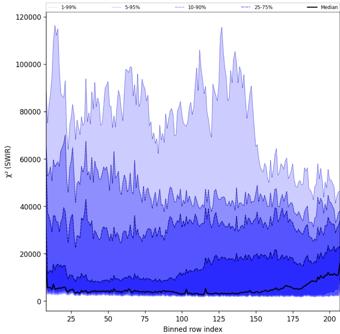
Figure 39: Along track statistics of “ \chi^2 (SWIR)” for 2024-12-04 to 2024-12-06
