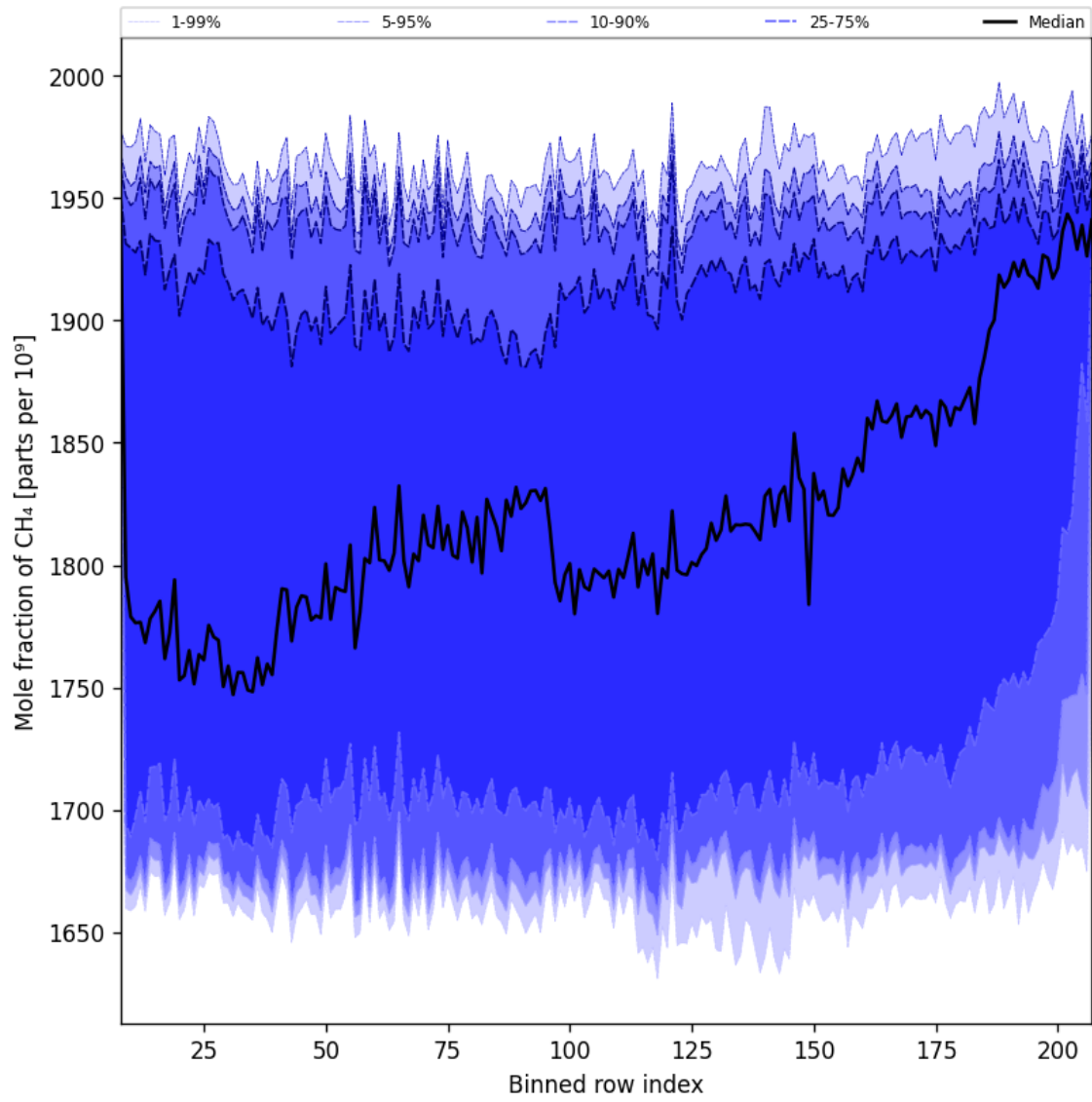
Figure 34: Along track statistics of “Mole fraction of CH 4 ” for 2024-12-04 to 2024-12-06
