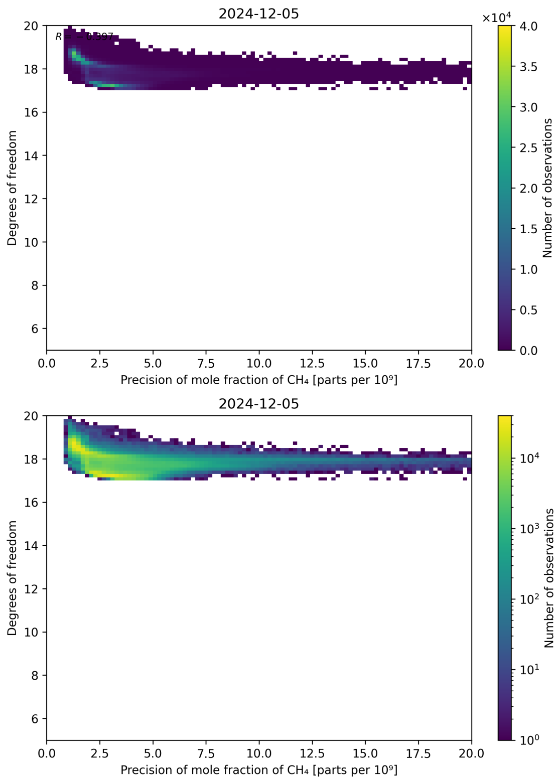
Figure 80: Scatter density plot of “Precision of mole fraction of CH 4 ” against “Degrees of freedom” for 2024-12-04 to 2024-12-06.
