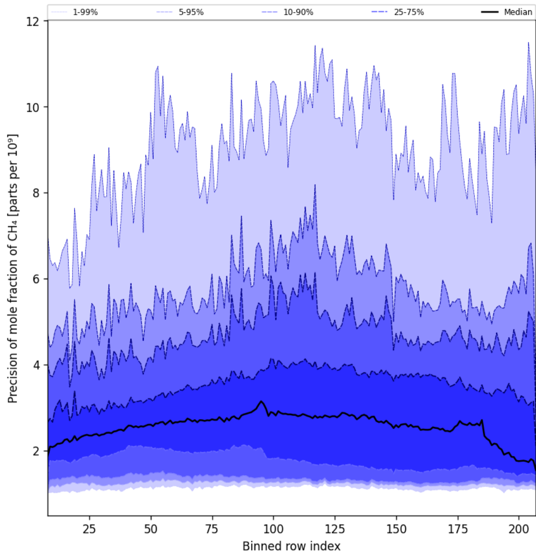
Figure 35: Along track statistics of “Precision of mole fraction of CH 4 ” for 2024-12-04 to 2024-12-06
