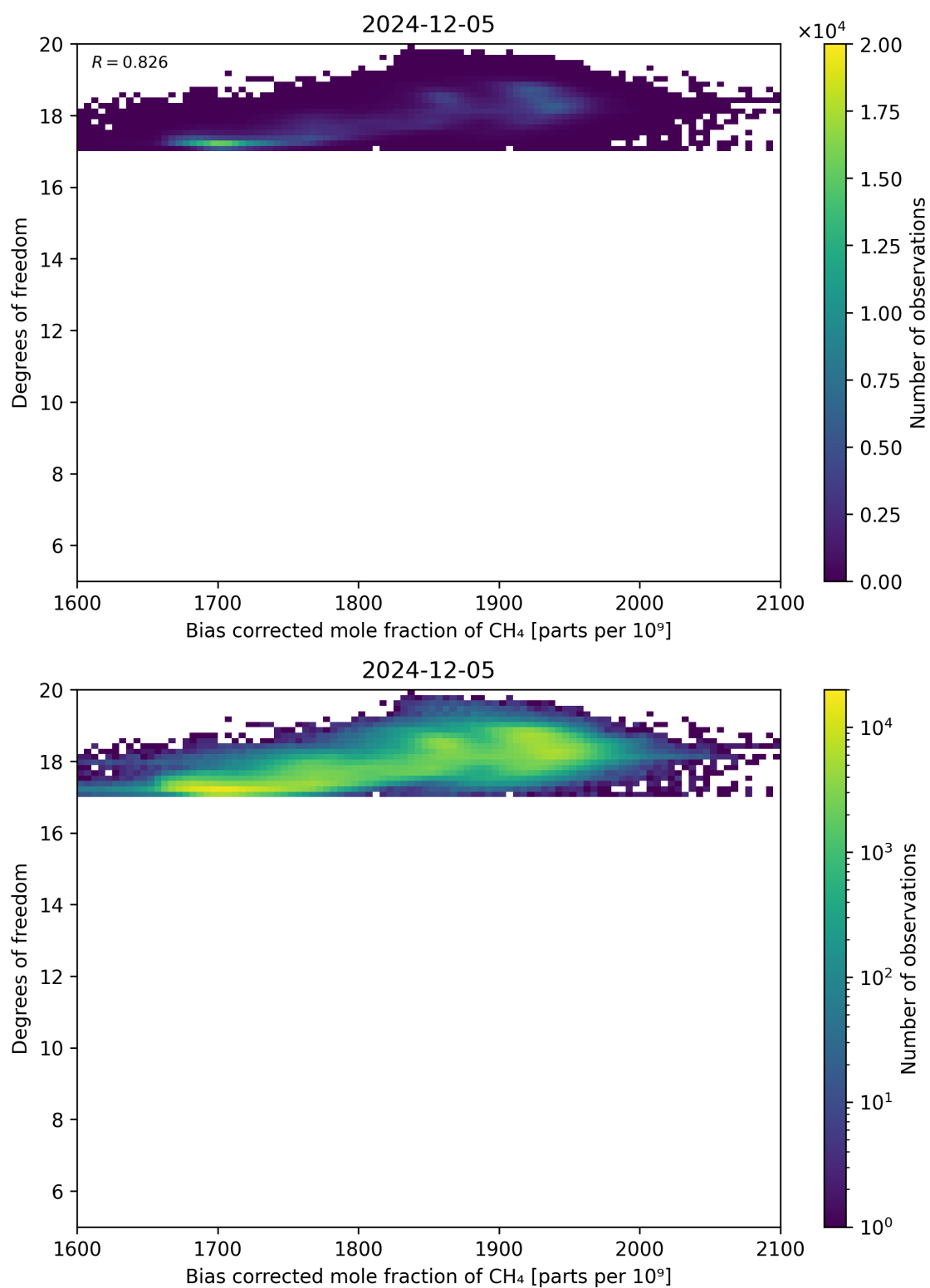
Figure 65: Scatter density plot of “Bias corrected mole fraction of CH 4 ” against “Degrees of freedom” for 2024-12-04 to 2024-12-06.
