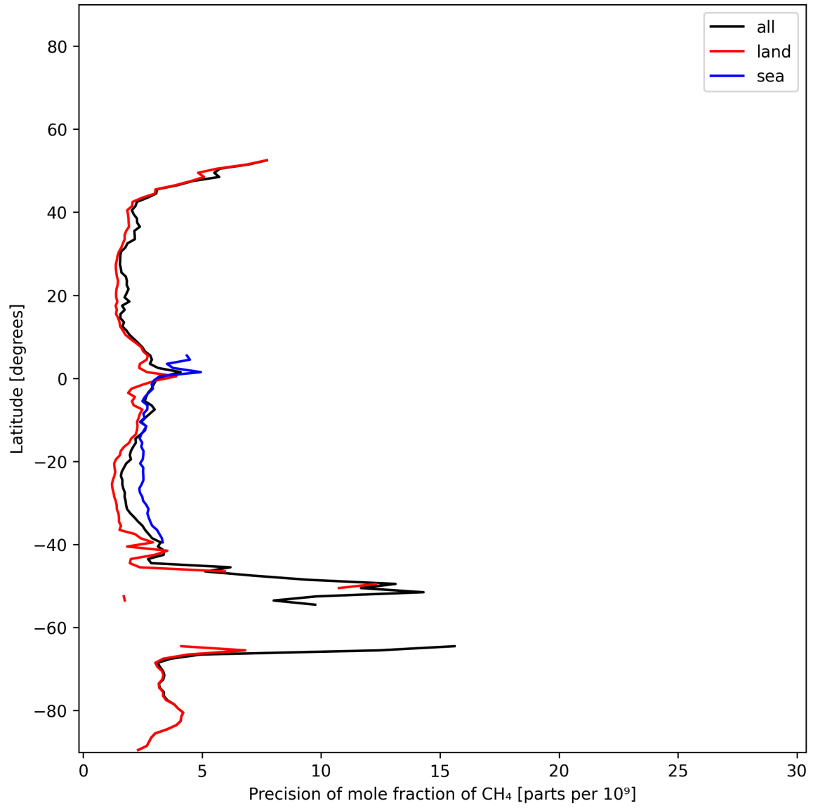
Figure 13: Zonal average of “Precision of mole fraction of CH 4 ” for 2024-12-04 to 2024-12-06.
