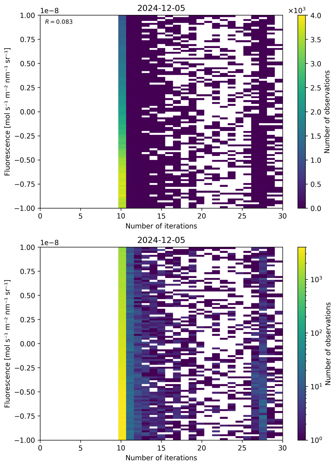
Figure 87: Scatter density plot of “Number of iterations” against “Fluorescence” for 2024-12-04 to 2024-12-06.
