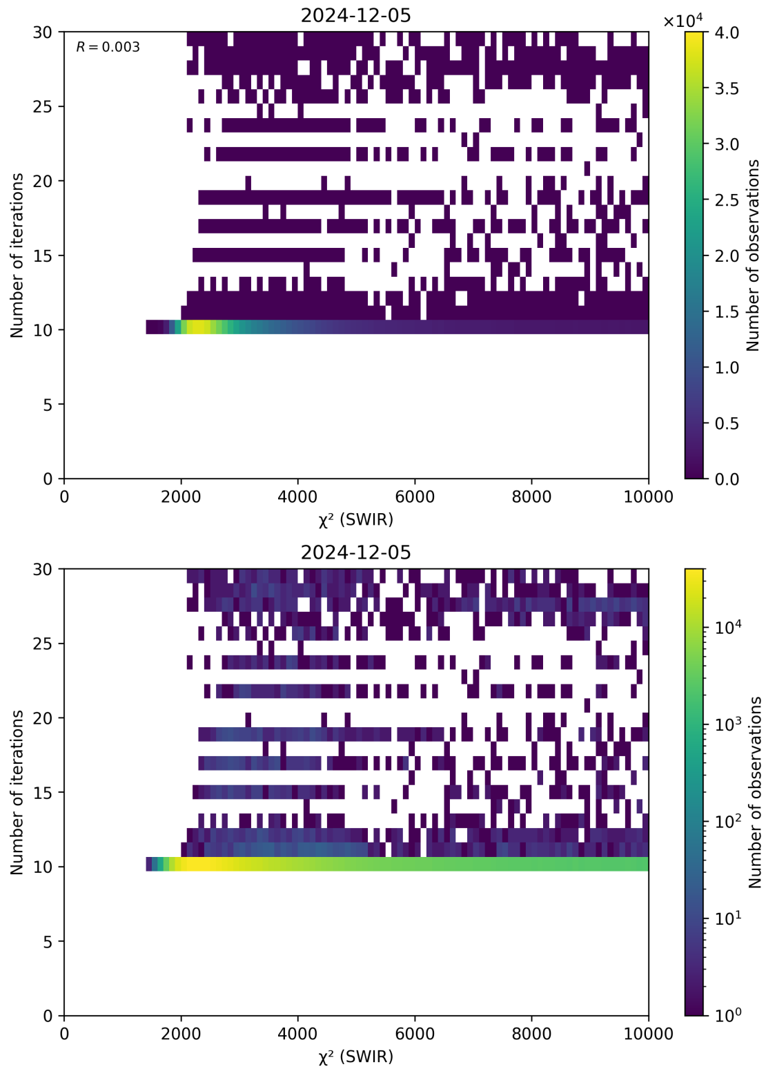
Figure 50: Scatter density plot of “ \chi^2 (SWIR)” against “Number of iterations” for 2024-12-04 to 2024-12-06.
