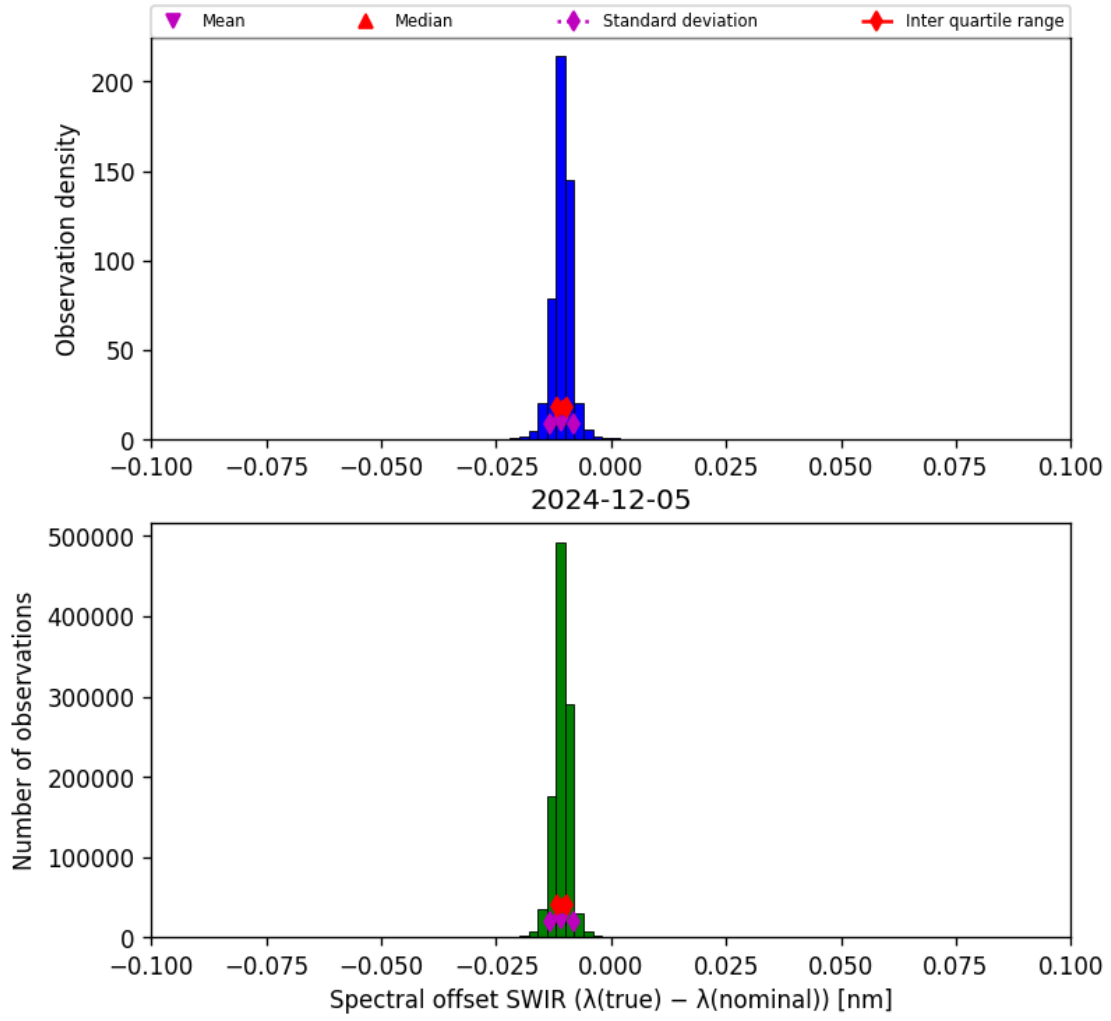
Figure 27: Histogram of “Spectral offset SWIR ( \lambda_{\text{true}} - \lambda_{\text{nominal}} )” for 2024-12-04 to 2024-12-06
