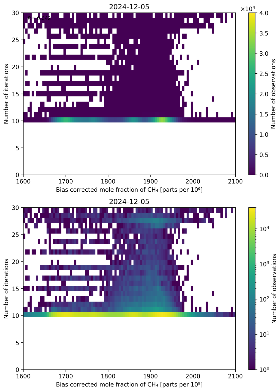
Figure 67: Scatter density plot of “Bias corrected mole fraction of CH 4 ” against “Number of iterations” for 2024-12-04 to 2024-12-06.
