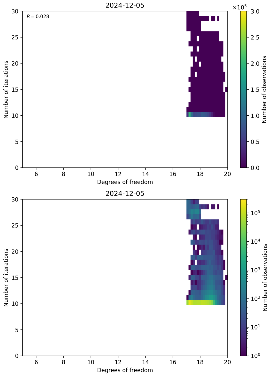
Figure 52: Scatter density plot of “Degrees of freedom” against “Number of iterations” for 2024-12-04 to 2024-12-06.
