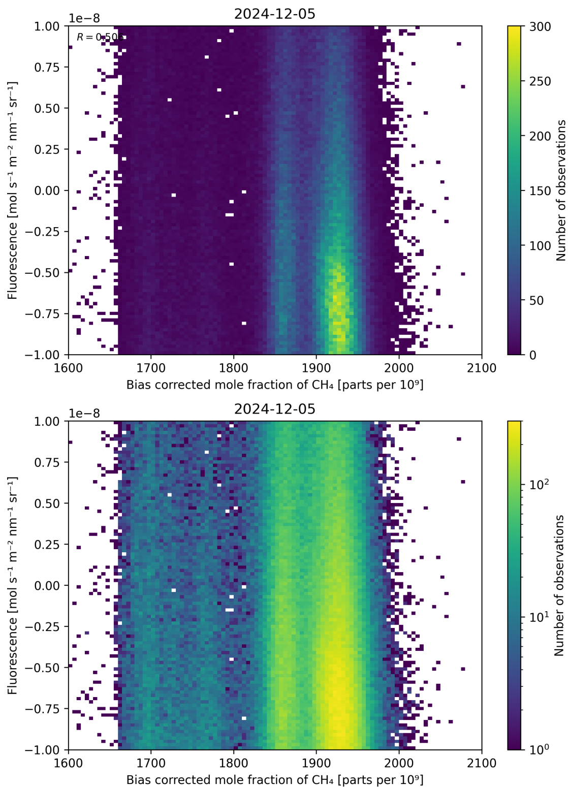
Figure 66: Scatter density plot of “Bias corrected mole fraction of \text{CH}_4 ” against “Fluorescence” for 2024-12-04 to 2024-12-06.
