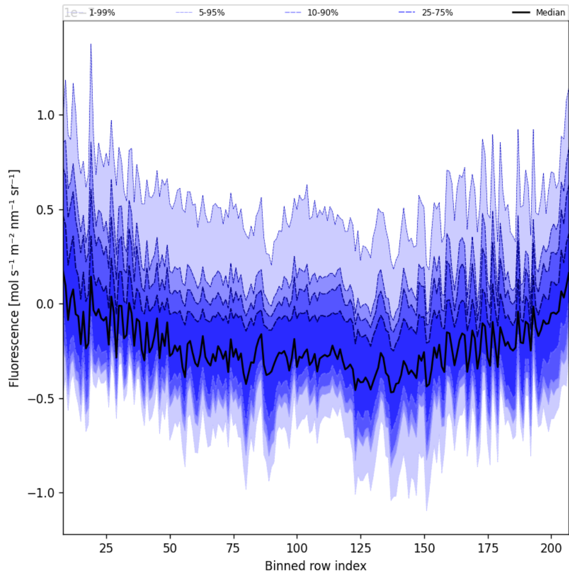
Figure 43: Along track statistics of “Fluorescence” for 2024-12-04 to 2024-12-06
