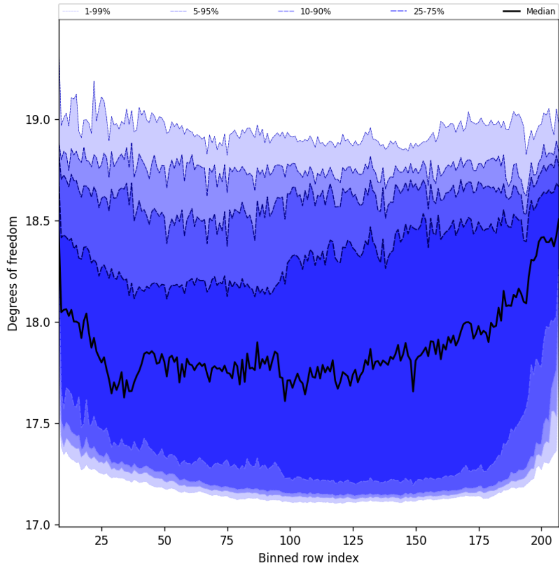
Figure 41: Along track statistics of “Degrees of freedom” for 2024-12-04 to 2024-12-06
