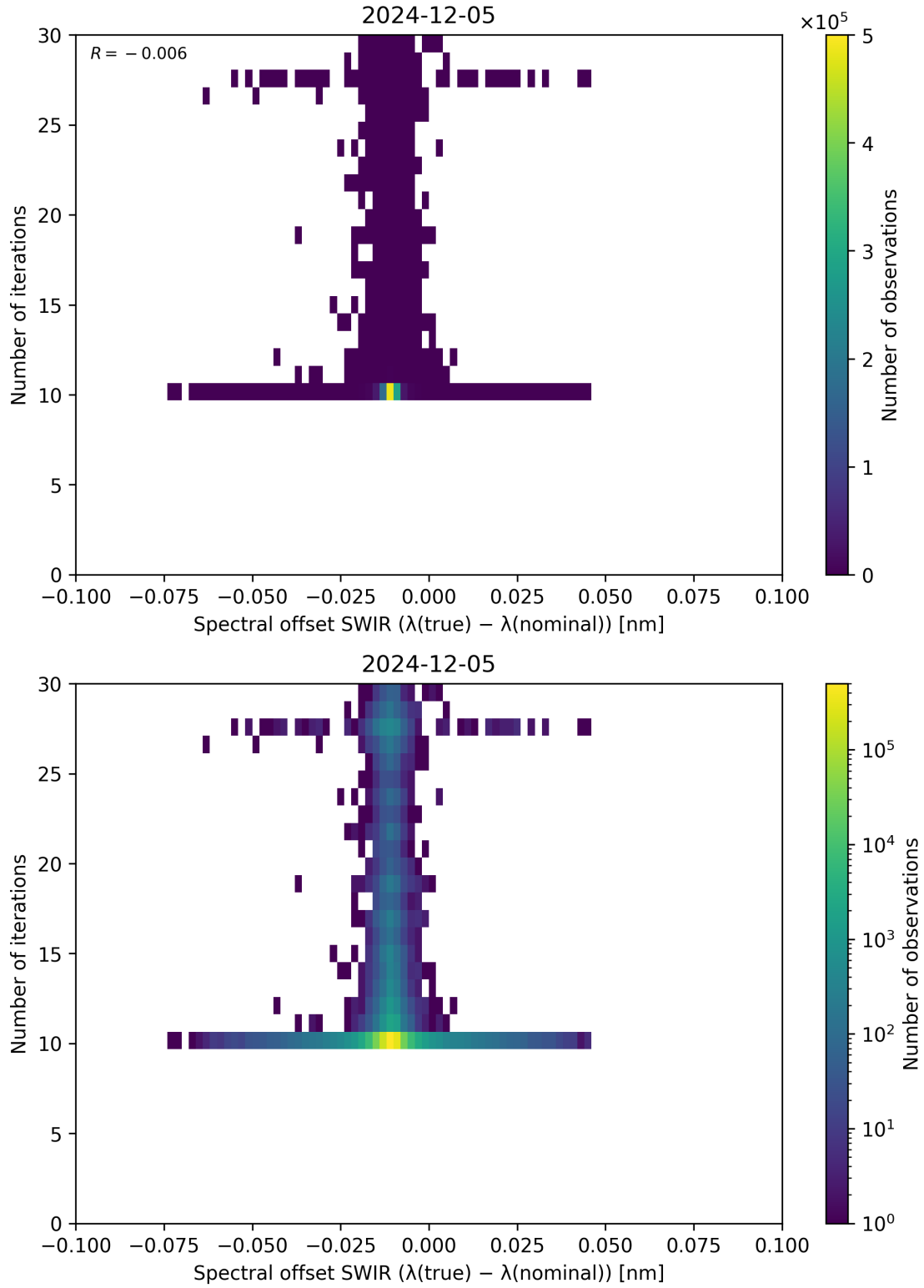
Figure 121: Scatter density plot of “Spectral offset SWIR ( \lambda_{\text{true}} - \lambda_{\text{nominal}} )” against “Number of iterations” for 2024-12-04 to 2024-12-06.
