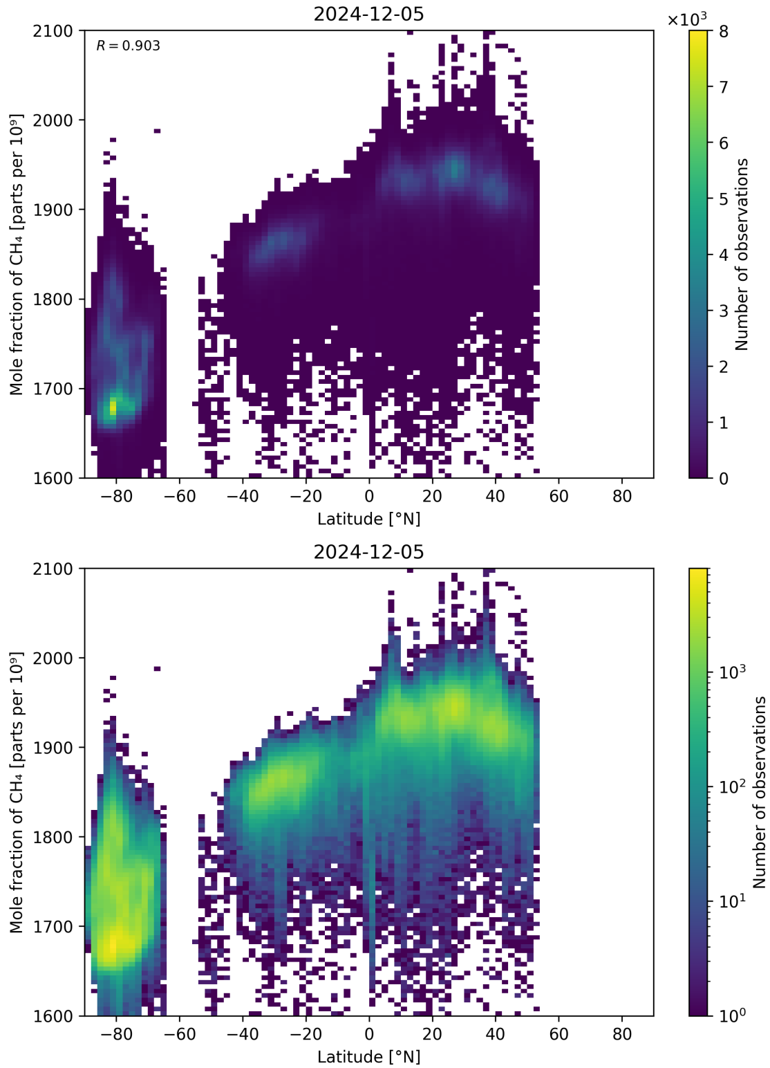
Figure 57: Scatter density plot of “Latitude” against “Mole fraction of CH 4 ” for 2024-12-04 to 2024-12-06.
