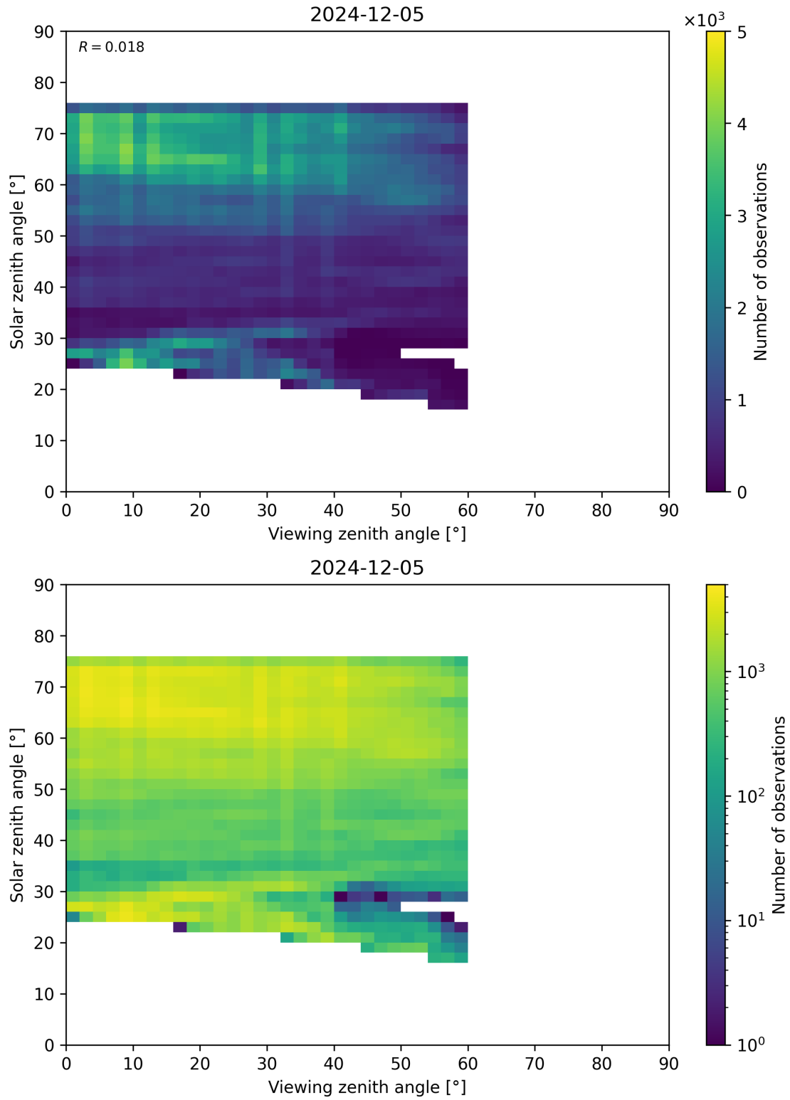
Figure 115: Scatter density plot of “Viewing zenith angle” against “Solar zenith angle” for 2024-12-04 to 2024-12-06.
