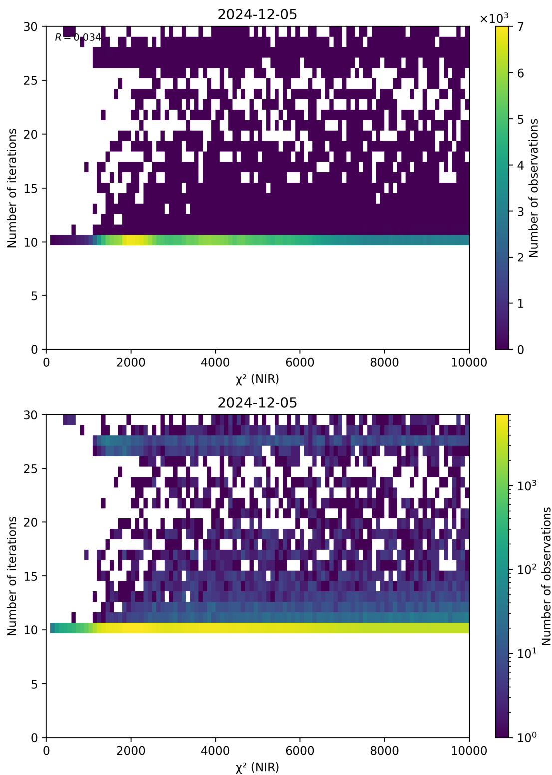
Figure 46: Scatter density plot of “ \chi^2 (NIR)” against “Number of iterations” for 2024-12-04 to 2024-12-06.
