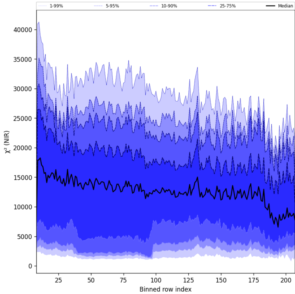
Figure 40: Along track statistics of " \chi^2 (NIR)" for 2024-12-04 to 2024-12-06
