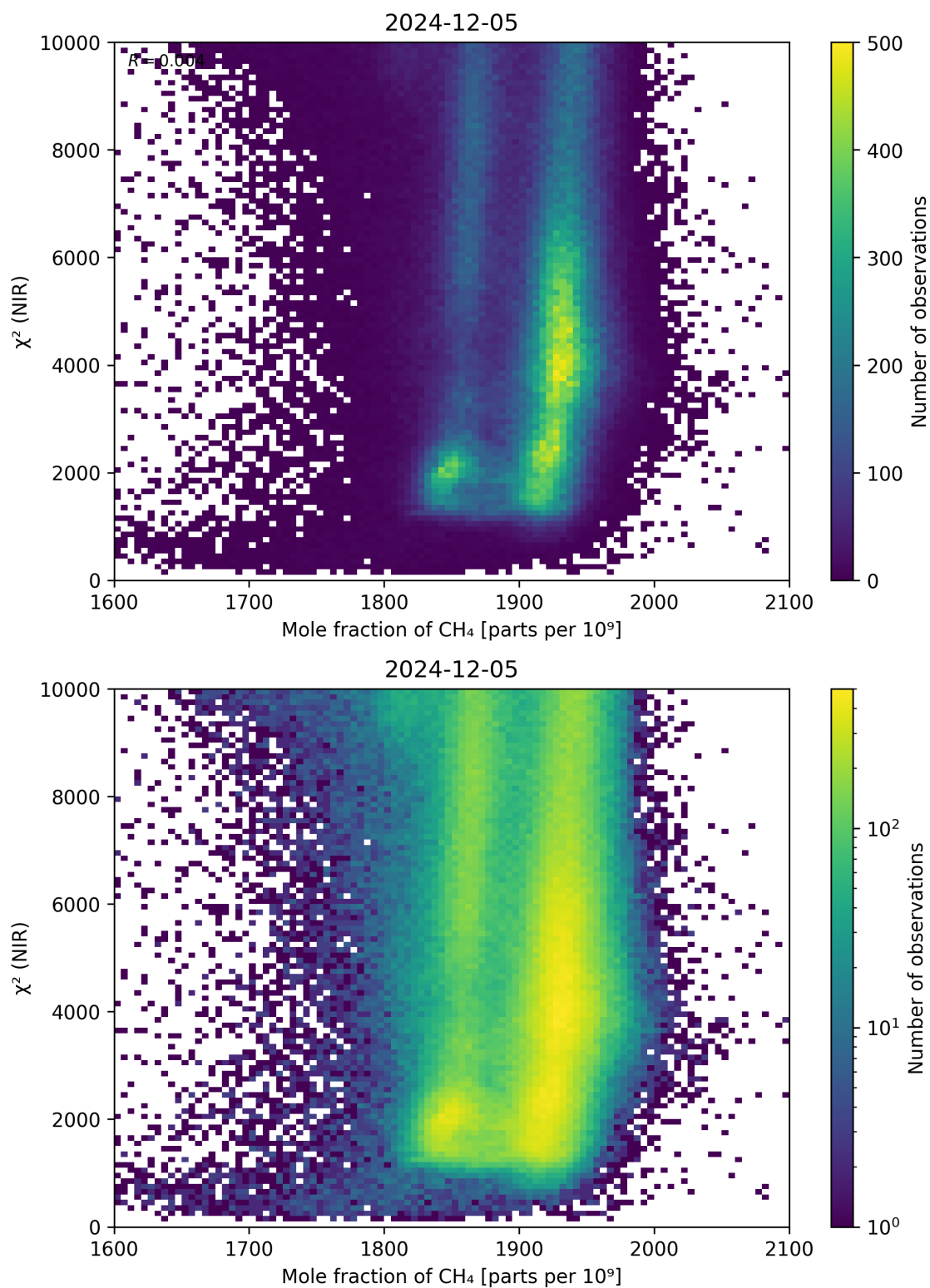
Figure 70: Scatter density plot of “Mole fraction of \text{CH}_4 ” against “ \chi^2 (NIR)” for 2024-12-04 to 2024-12-06.
