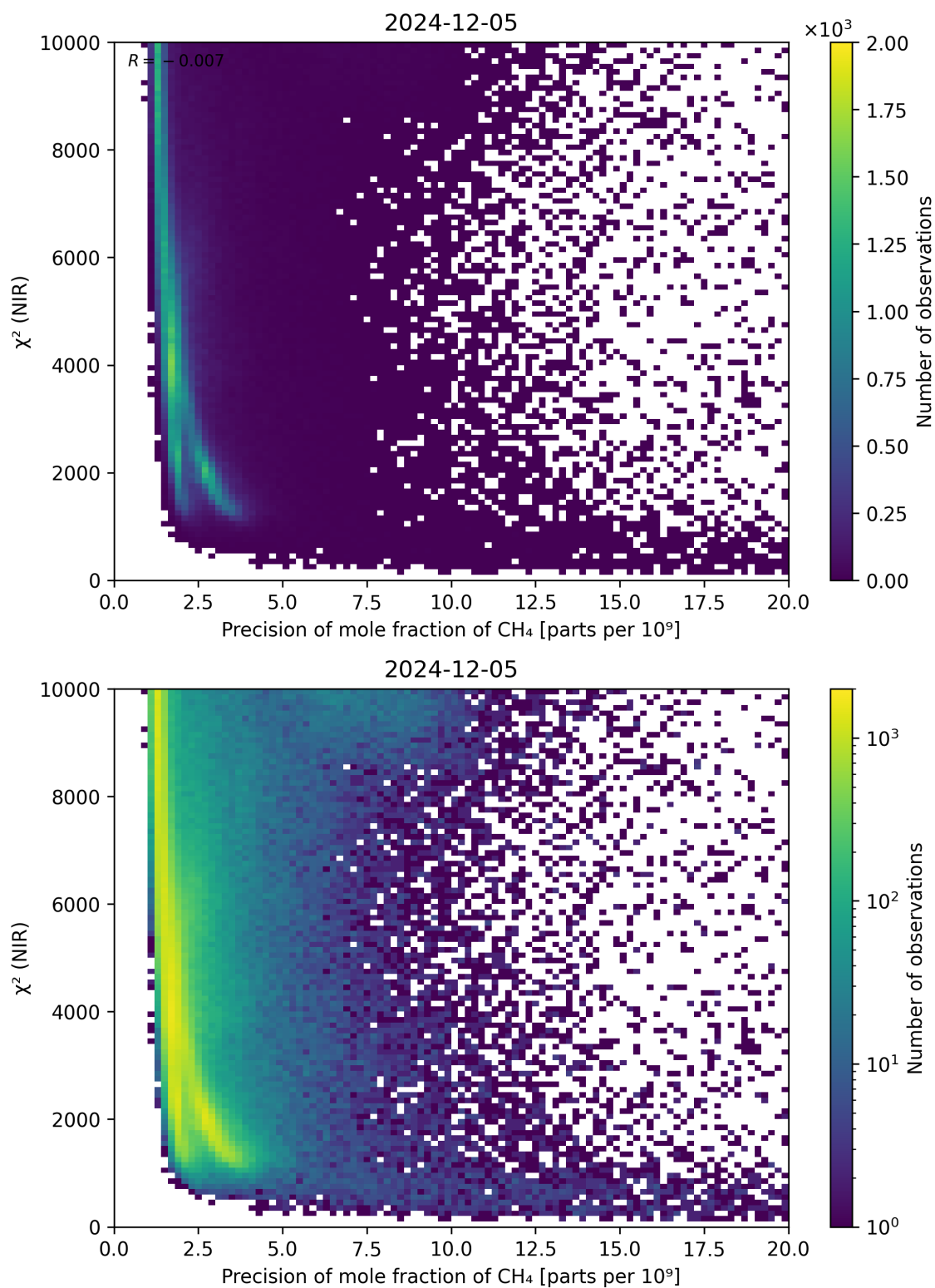
Figure 78: Scatter density plot of “Precision of mole fraction of CH 4 ” against “ \chi^2 (NIR)” for 2024-12-04 to 2024-12-06.
