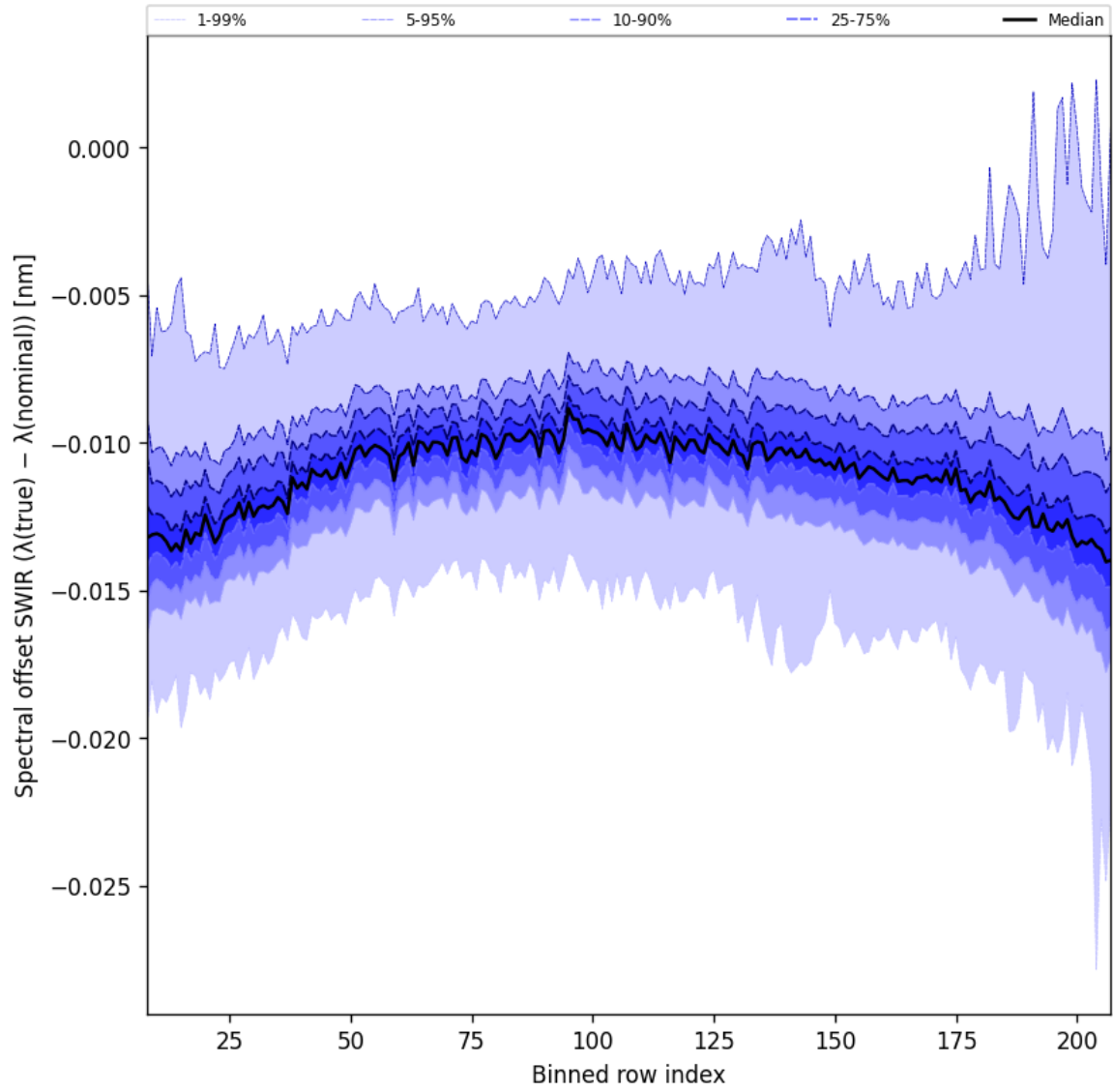
Figure 38: Along track statistics of “Spectral offset SWIR ( \lambda_{\text{true}} - \lambda_{\text{nominal}} )” for 2024-12-04 to 2024-12-06
