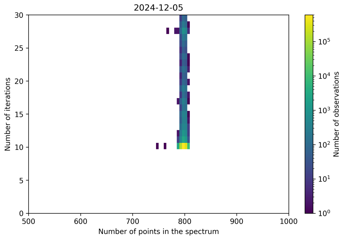
Figure 92: Scatter density plot of “Number of points in the spectrum” against “Number of iterations” for 2024-12-04 to 2024-12-06.
