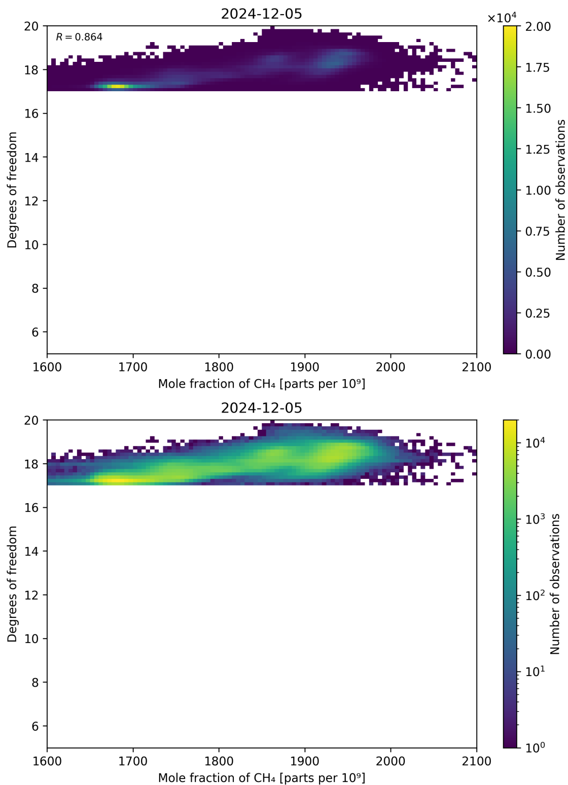
Figure 72: Scatter density plot of “Mole fraction of CH 4 ” against “Degrees of freedom” for 2024-12-04 to 2024-12-06.
