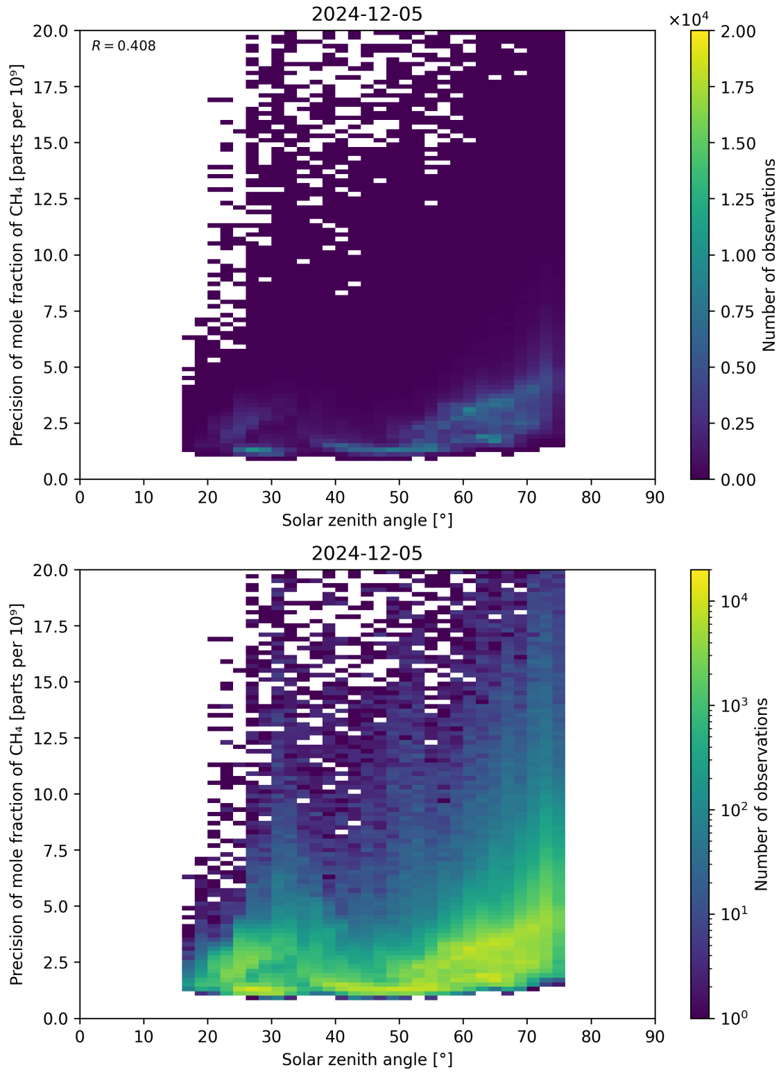
Figure 101: Scatter density plot of “Solar zenith angle” against “Precision of mole fraction of \text{CH}_4 ” for 2024-12-04 to 2024-12-06.
