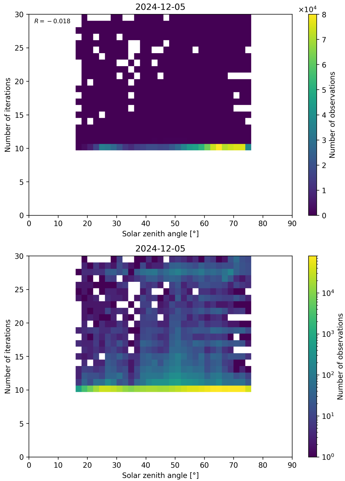
Figure 102: Scatter density plot of “Solar zenith angle” against “Number of iterations” for 2024-12-04 to 2024-12-06.
