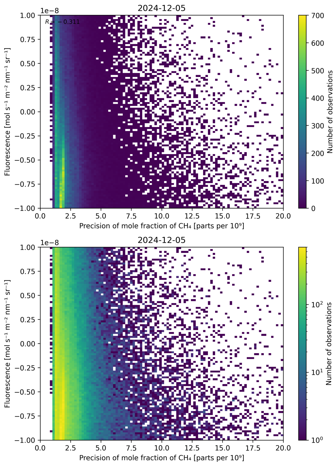
Figure 81: Scatter density plot of “Precision of mole fraction of CH 4 ” against “Fluorescence” for 2024-12-04 to 2024-12-06.
