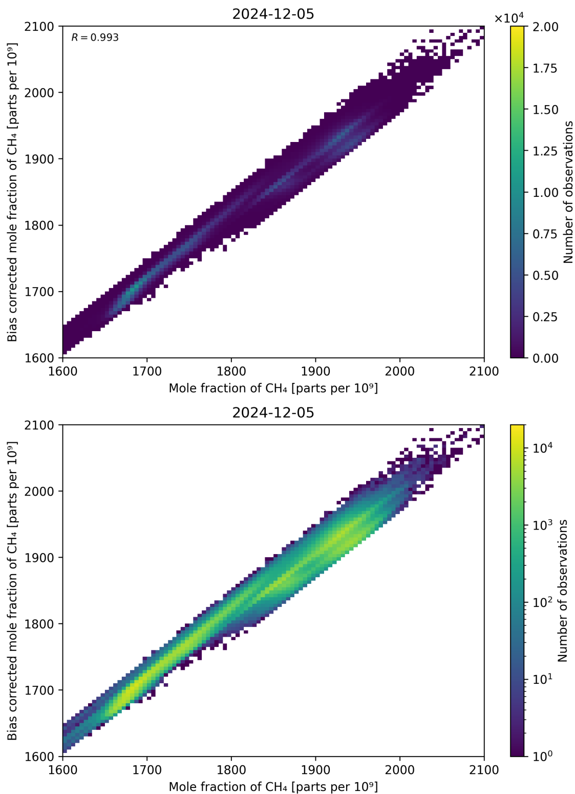
Figure 74: Scatter density plot of “Mole fraction of CH 4 ” against “Bias corrected mole fraction of CH 4 ” for 2024-12-04 to 2024-12-06.
