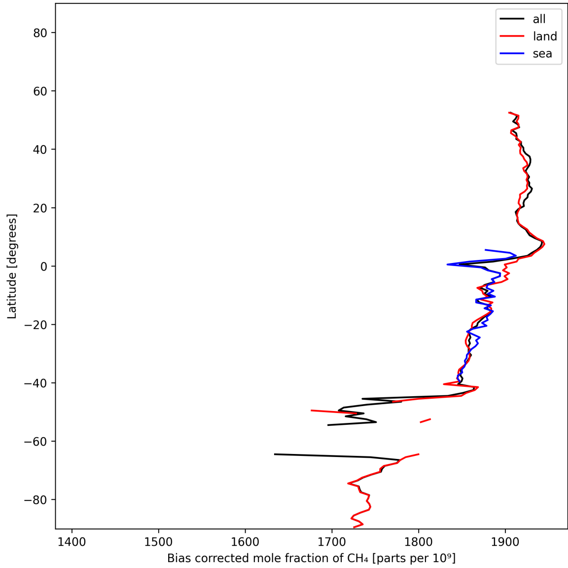
Figure 14: Zonal average of “Bias corrected mole fraction of CH 4 ” for 2024-12-04 to 2024-12-06.
