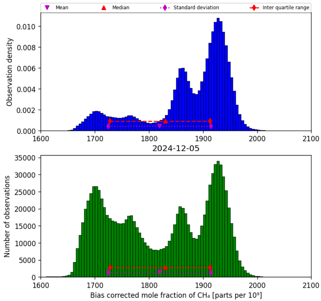
Figure 25: Histogram of “Bias corrected mole fraction of CH 4 ” for 2024-12-04 to 2024-12-06
