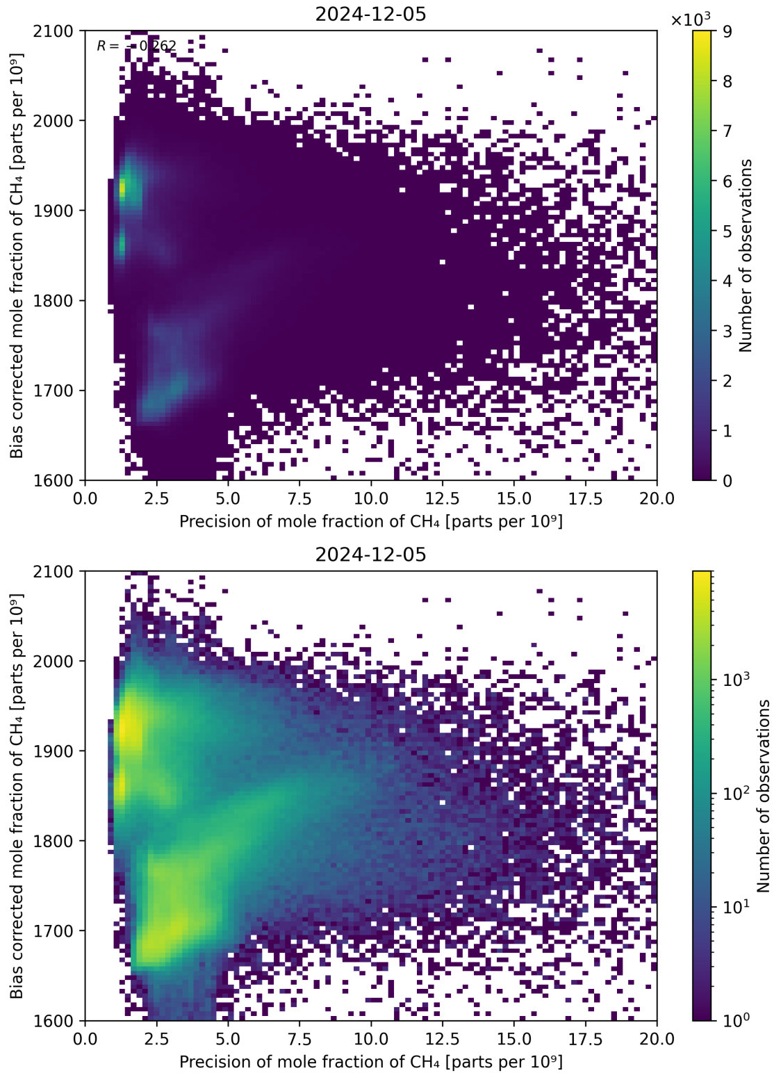
Figure 82: Scatter density plot of “Precision of mole fraction of \text{CH}_4 ” against “Bias corrected mole fraction of \text{CH}_4 ” for 2024-12-04 to 2024-12-06.
