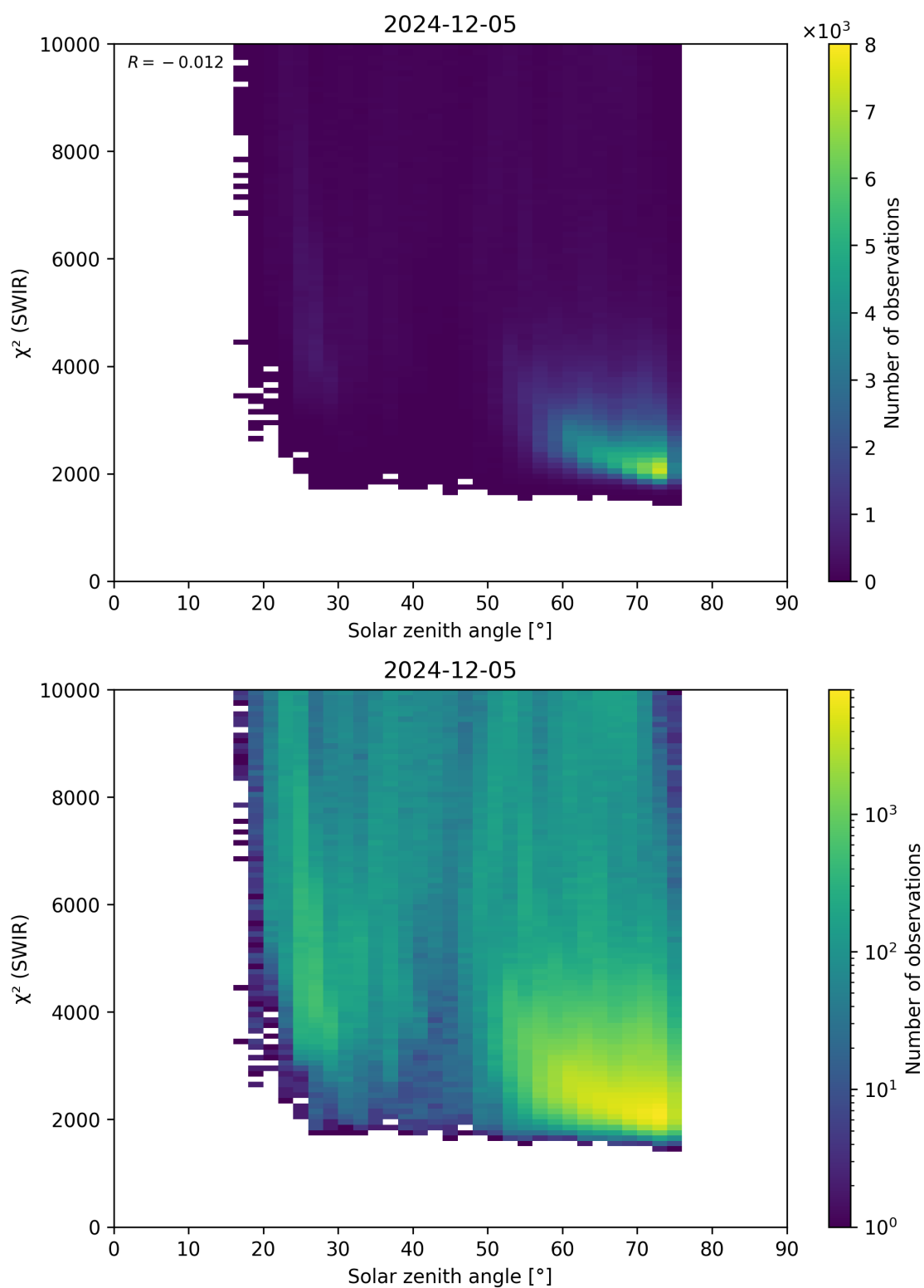
Figure 95: Scatter density plot of “Solar zenith angle” against “ \chi^2 (SWIR)” for 2024-12-04 to 2024-12-06.
