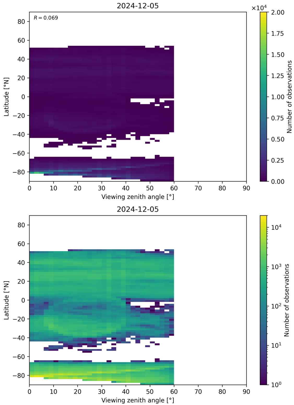
Figure 109: Scatter density plot of “Viewing zenith angle” against “Latitude” for 2024-12-04 to 2024-12-06.
