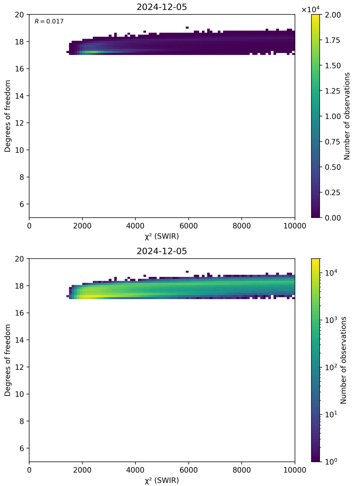
Figure 48: Scatter density plot of “ \chi^2 (SWIR)” against “Degrees of freedom” for 2024-12-04 to 2024-12-06.
