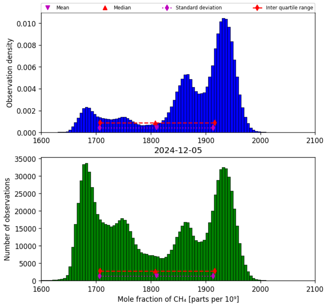
Figure 23: Histogram of “Mole fraction of CH 4 ” for 2024-12-04 to 2024-12-06
