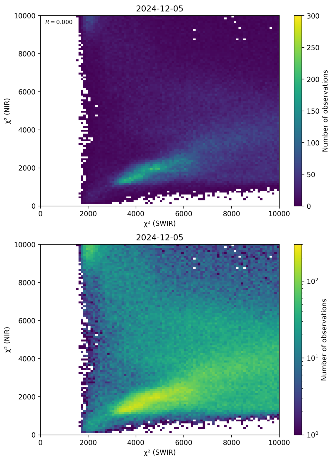
Figure 47: Scatter density plot of “ \chi^2 (SWIR)” against “ \chi^2 (NIR)” for 2024-12-04 to 2024-12-06.
