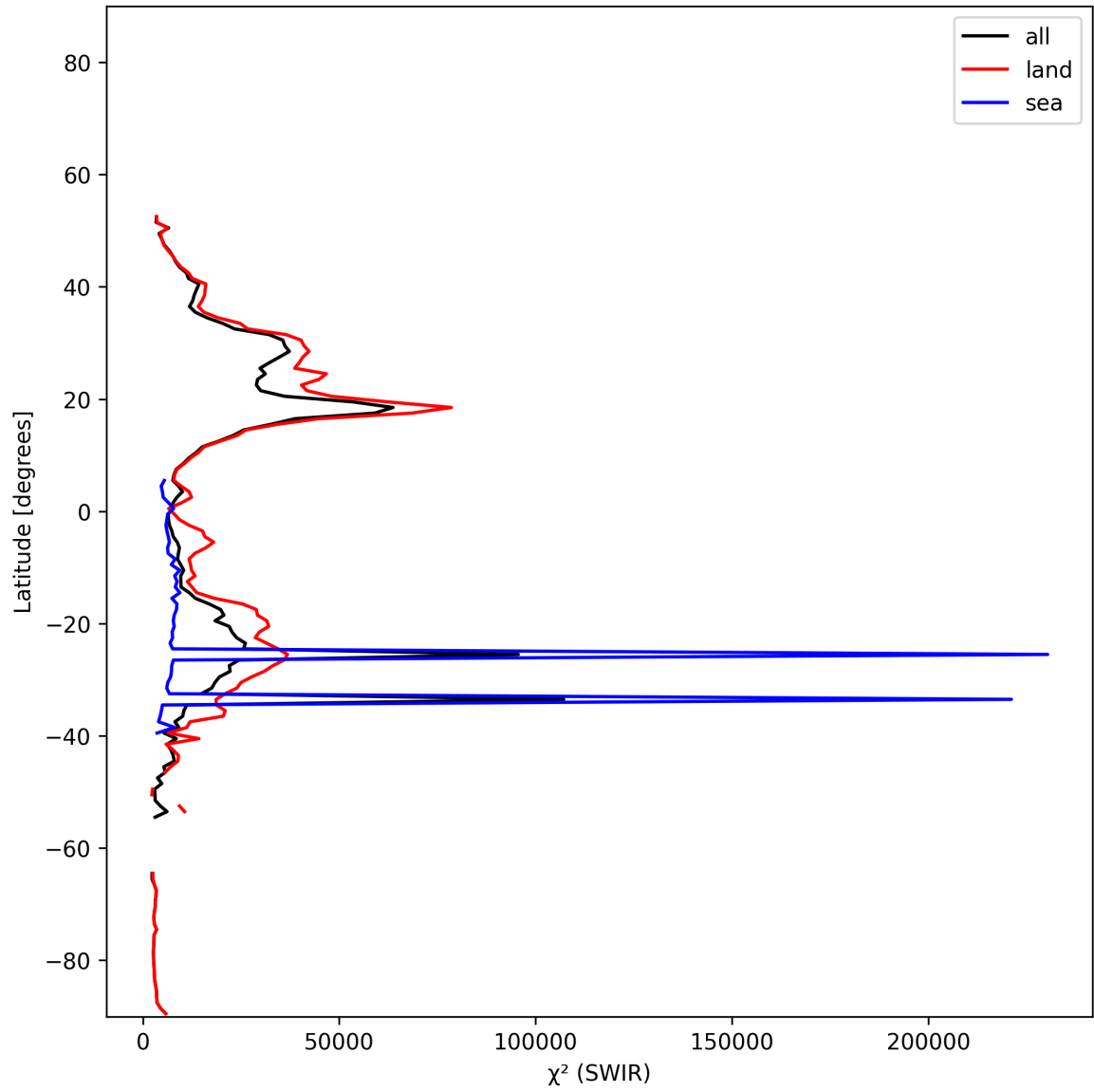
Figure 17: Zonal average of “ \chi^2 (SWIR)” for 2024-12-04 to 2024-12-06.
