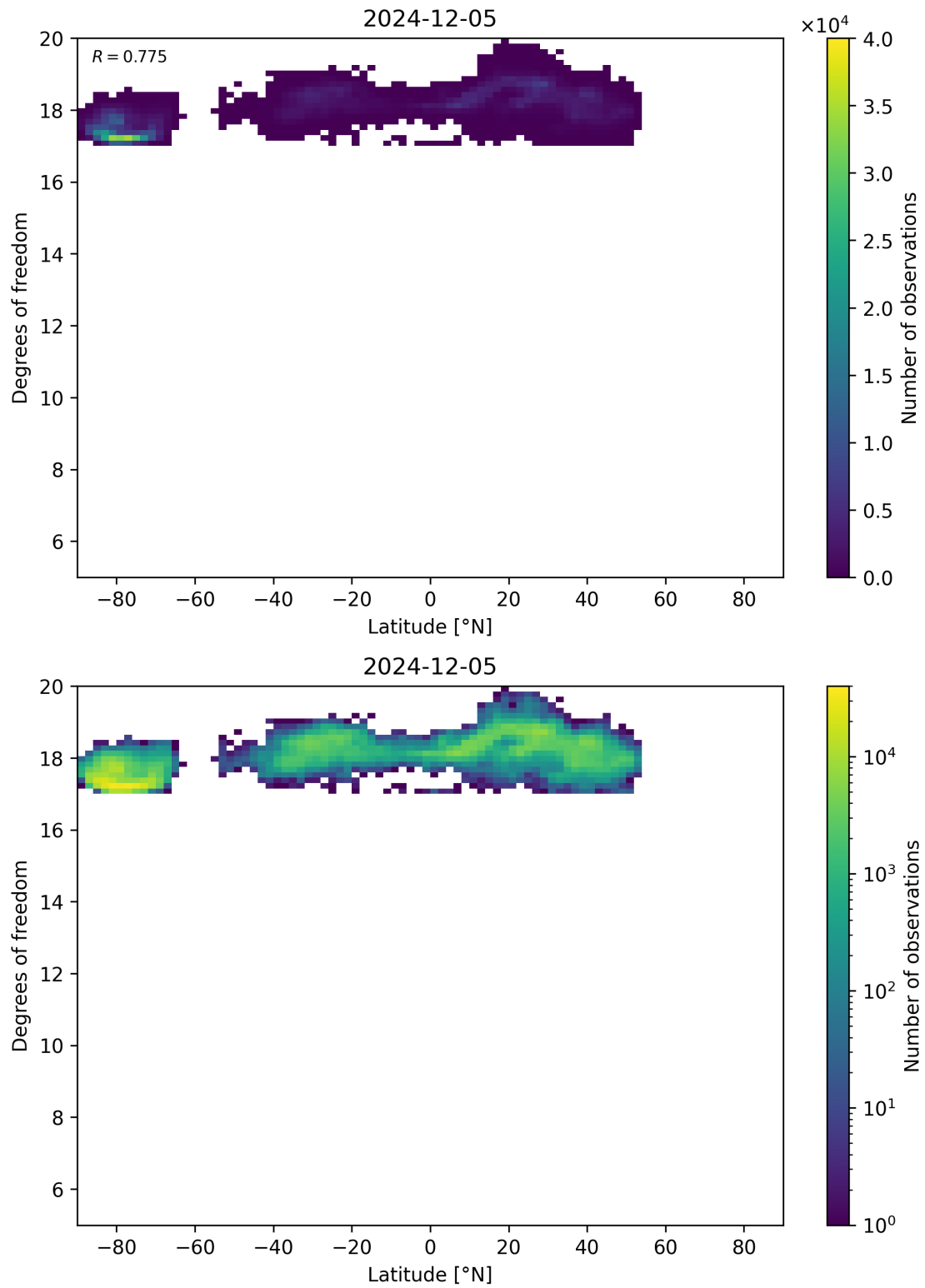
Figure 55: Scatter density plot of “Latitude” against “Degrees of freedom” for 2024-12-04 to 2024-12-06.
