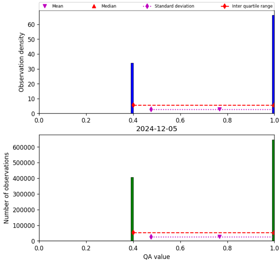
Figure 22: Histogram of “QA value” for 2024-12-04 to 2024-12-06
