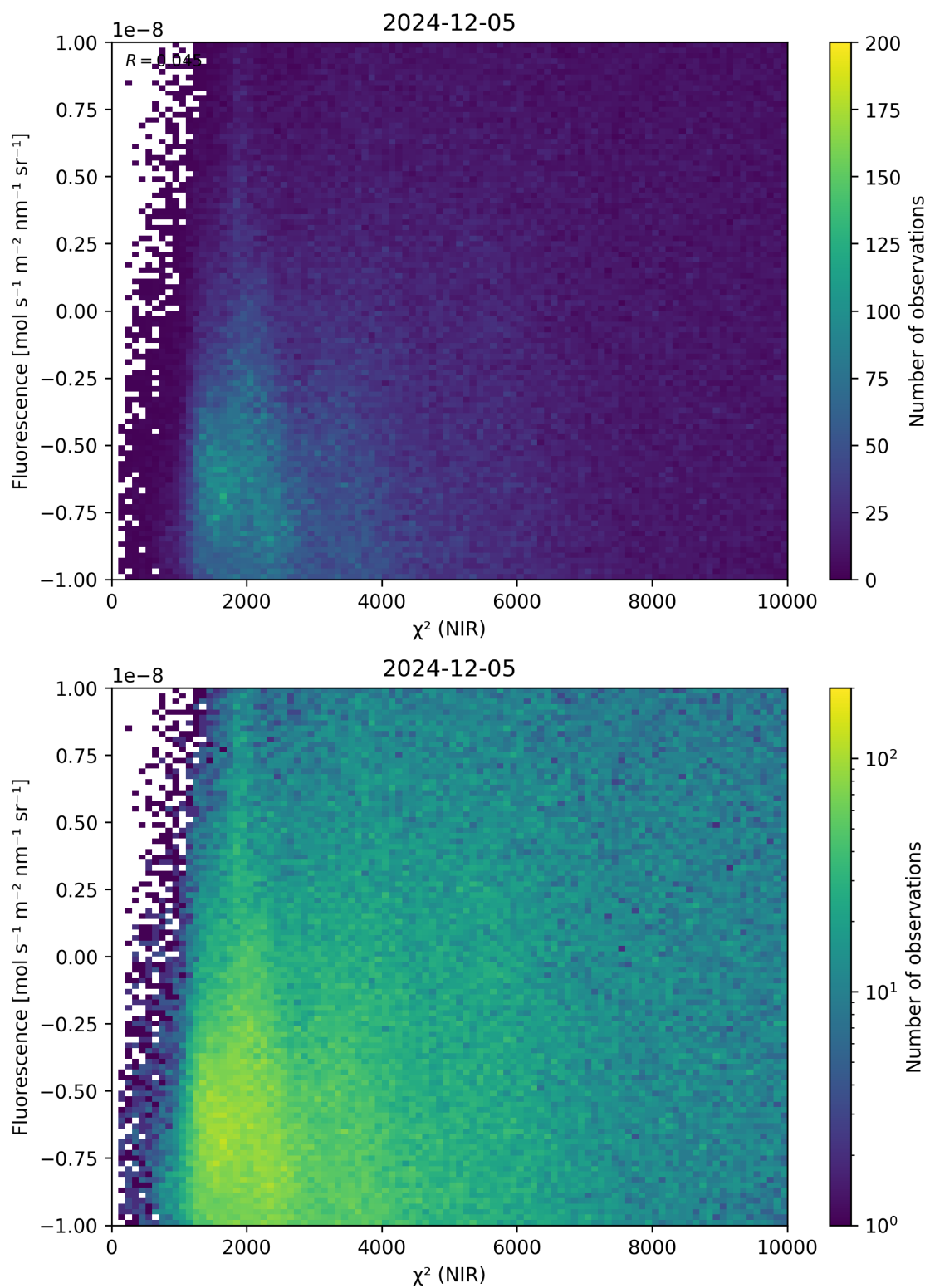
Figure 45: Scatter density plot of “ \chi^2 (NIR)” against “Fluorescence” for 2024-12-04 to 2024-12-06.
