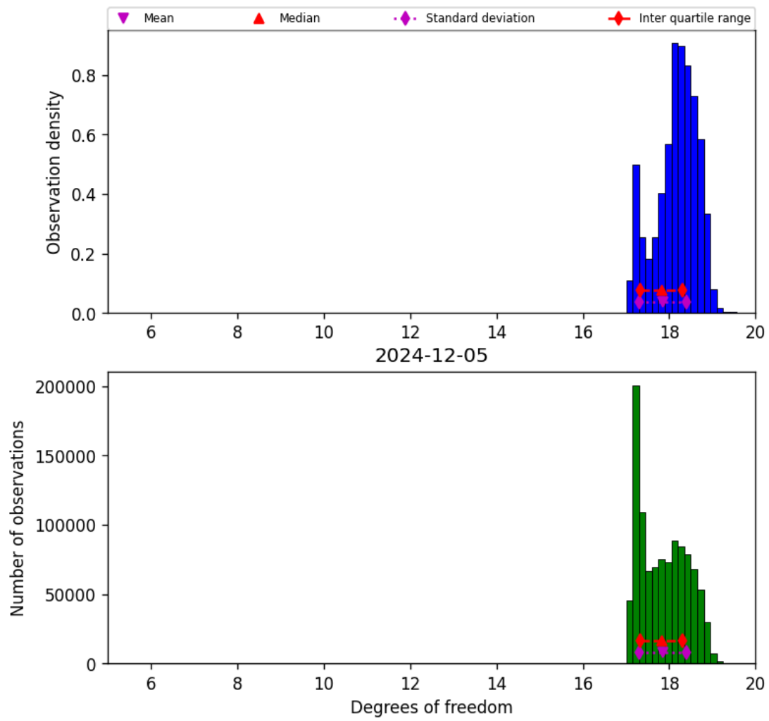
Figure 30: Histogram of “Degrees of freedom” for 2024-12-04 to 2024-12-06
