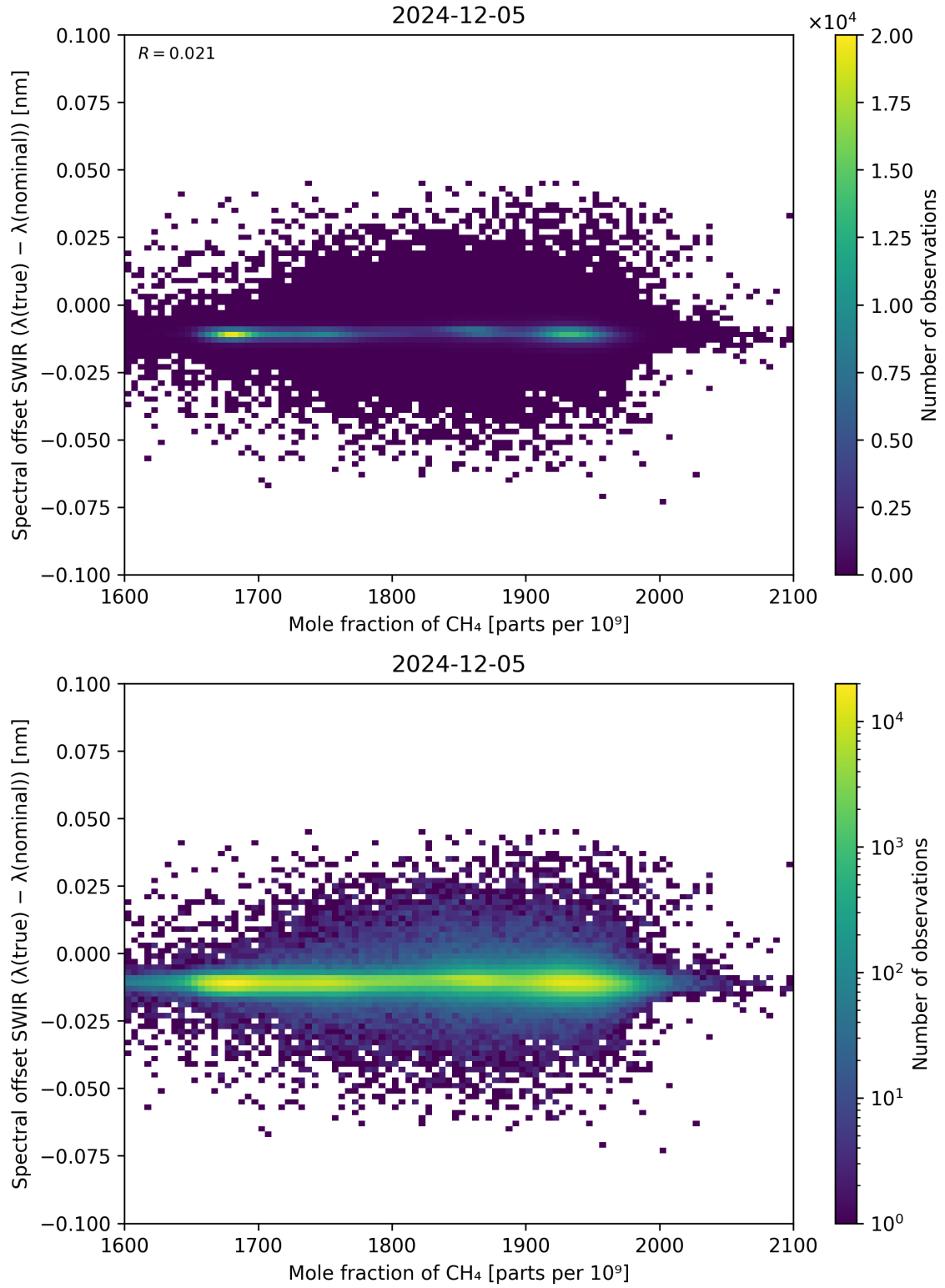
Figure 86: Scatter density plot of “Mole fraction of \text{CH}_4 ” against “Spectral offset SWIR ( \lambda_{\text{true}} - \lambda_{\text{nominal}} )” for 2024-12-04 to 2024-12-06.
