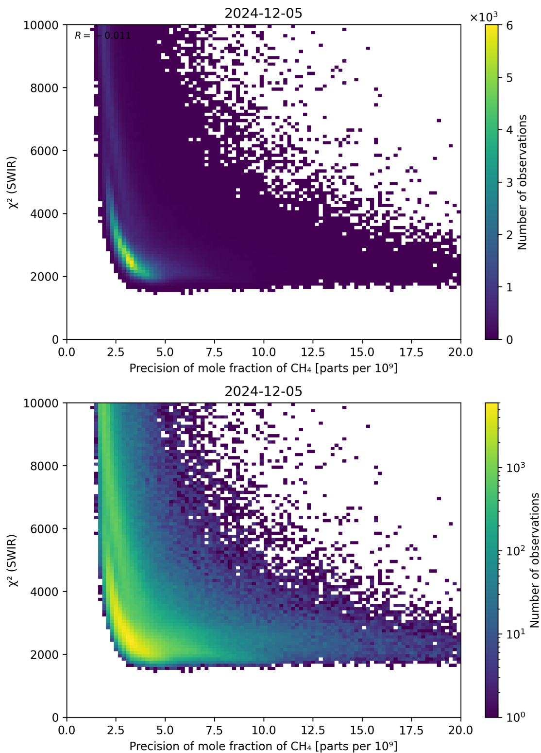
Figure 79: Scatter density plot of “Precision of mole fraction of \text{CH}_4 ” against “ \chi^2 (SWIR)” for 2024-12-04 to 2024-12-06.
