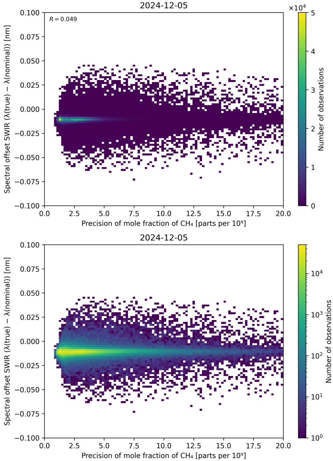
Figure 85: Scatter density plot of “Precision of mole fraction of CH 4 ” against “Spectral offset SWIR ( \lambda_{\text{true}} - \lambda_{\text{nominal}} )” for 2024-12-04 to 2024-12-06.
