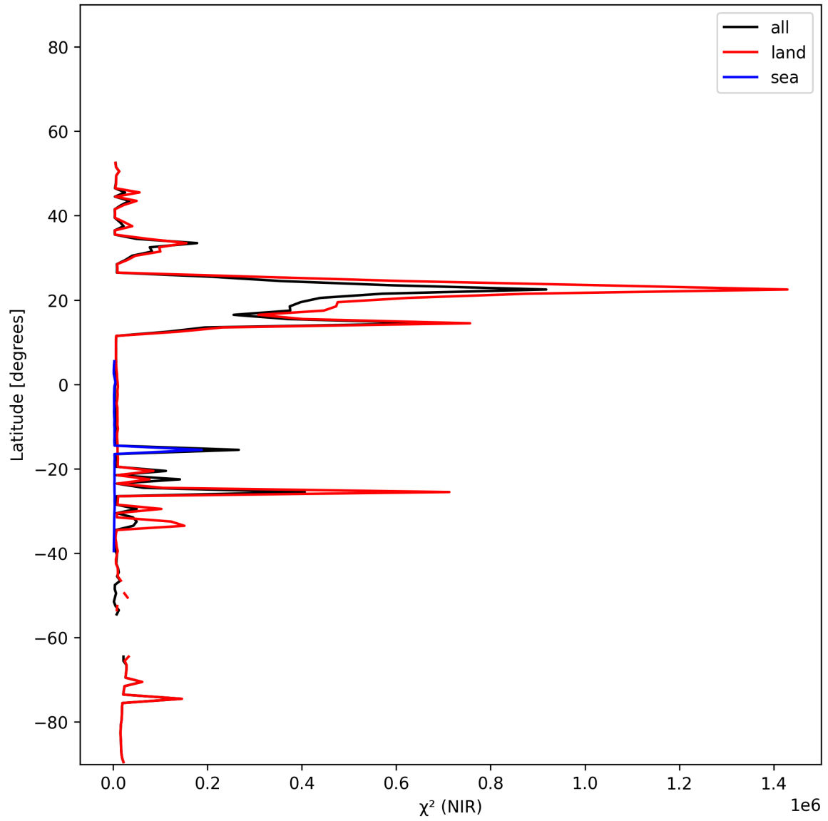
Figure 18: Zonal average of “ \chi^2 (NIR)” for 2024-12-04 to 2024-12-06.
