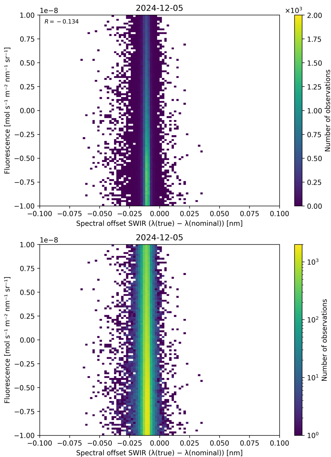
Figure 120: Scatter density plot of “Spectral offset SWIR ( \lambda_{\text{true}} - \lambda_{\text{nominal}} )” against “Fluorescence” for 2024-12-04 to 2024-12-06.
