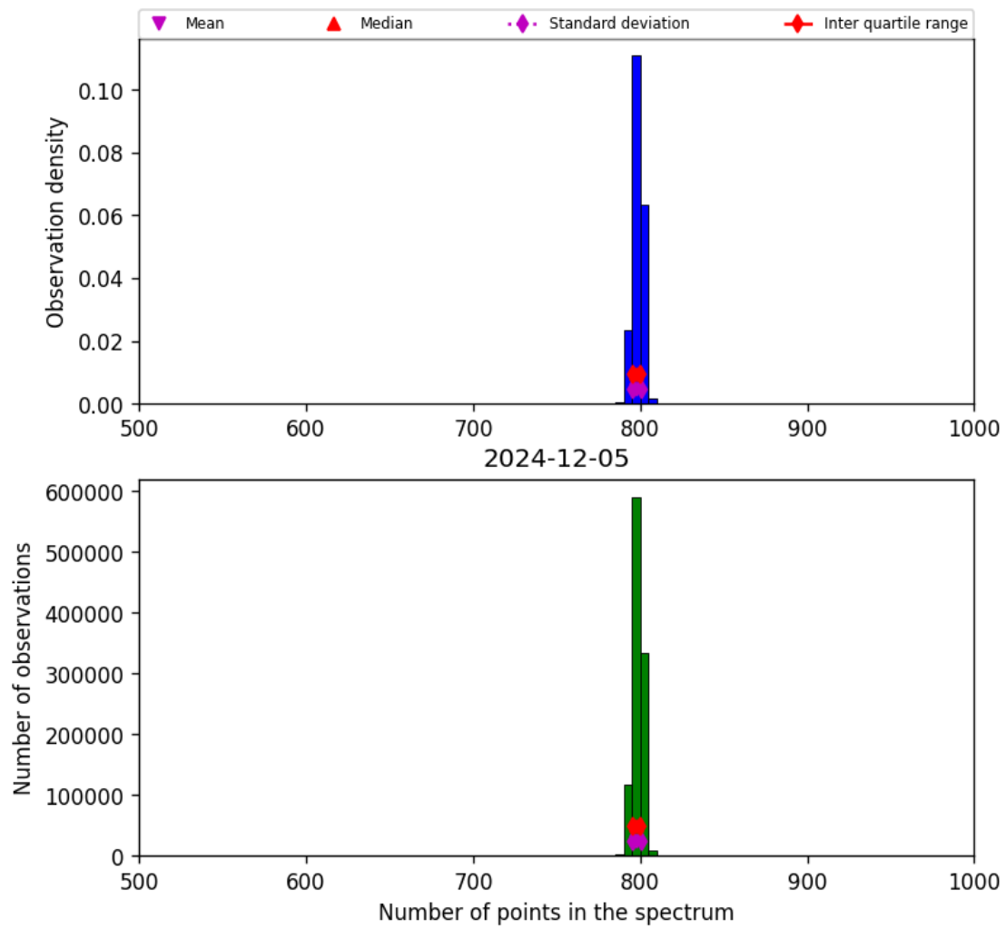
Figure 26: Histogram of “Number of points in the spectrum” for 2024-12-04 to 2024-12-06
