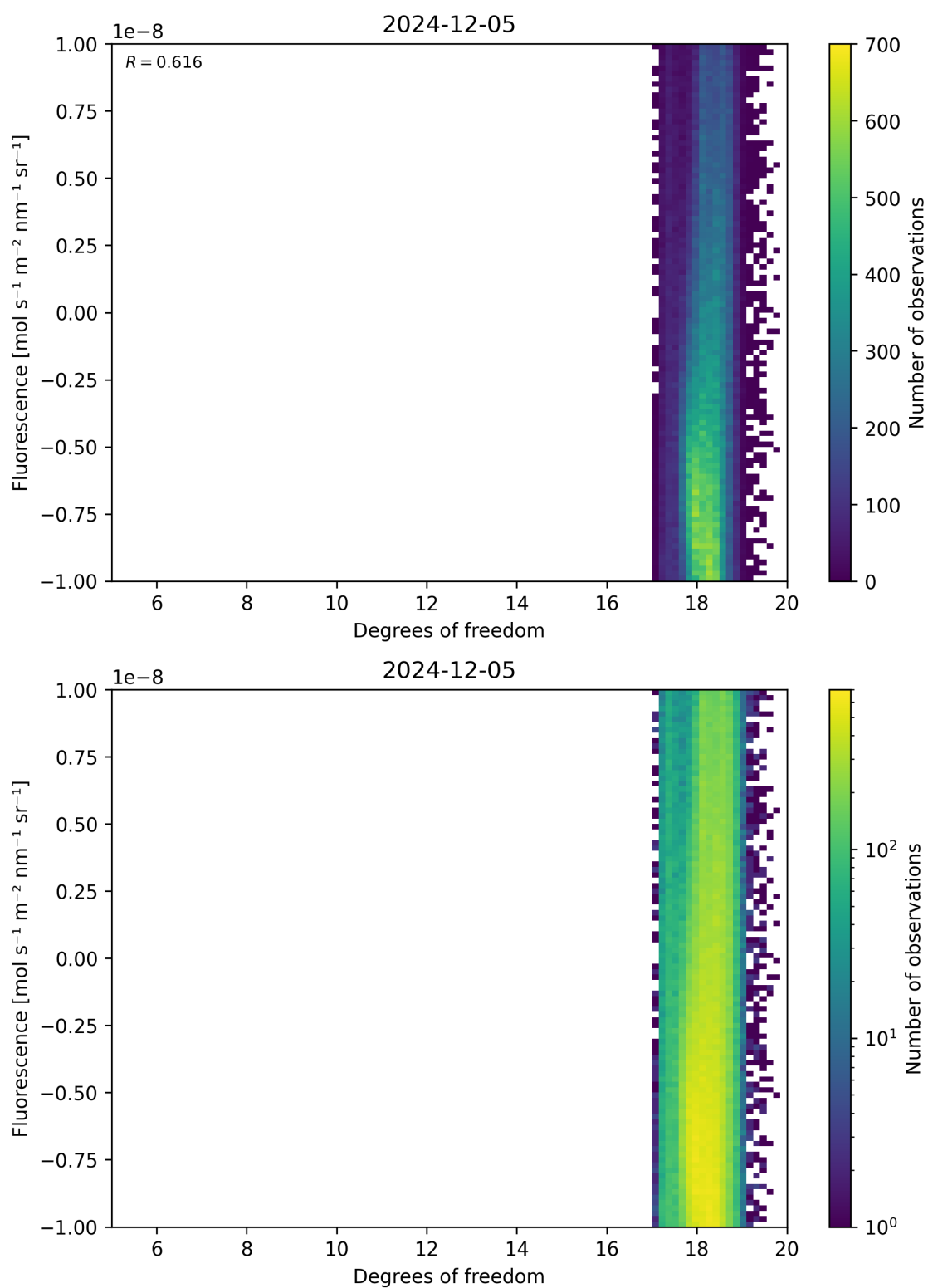
Figure 51: Scatter density plot of “Degrees of freedom” against “Fluorescence” for 2024-12-04 to 2024-12-06.
