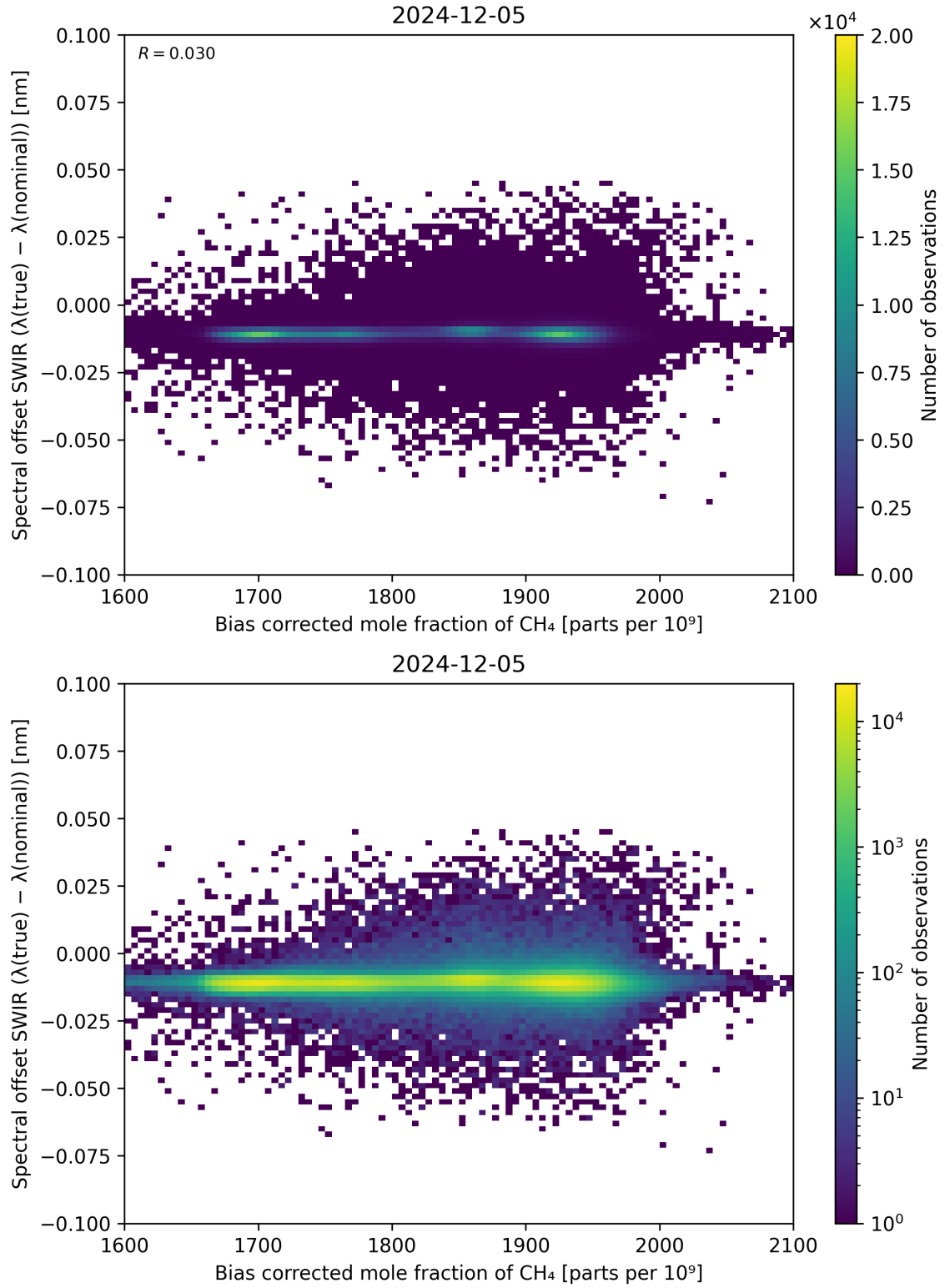
Figure 69: Scatter density plot of “Bias corrected mole fraction of \text{CH}_4 ” against “Spectral offset SWIR ( \lambda_{\text{true}} - \lambda_{\text{nominal}} )” for 2024-12-04 to 2024-12-06.
