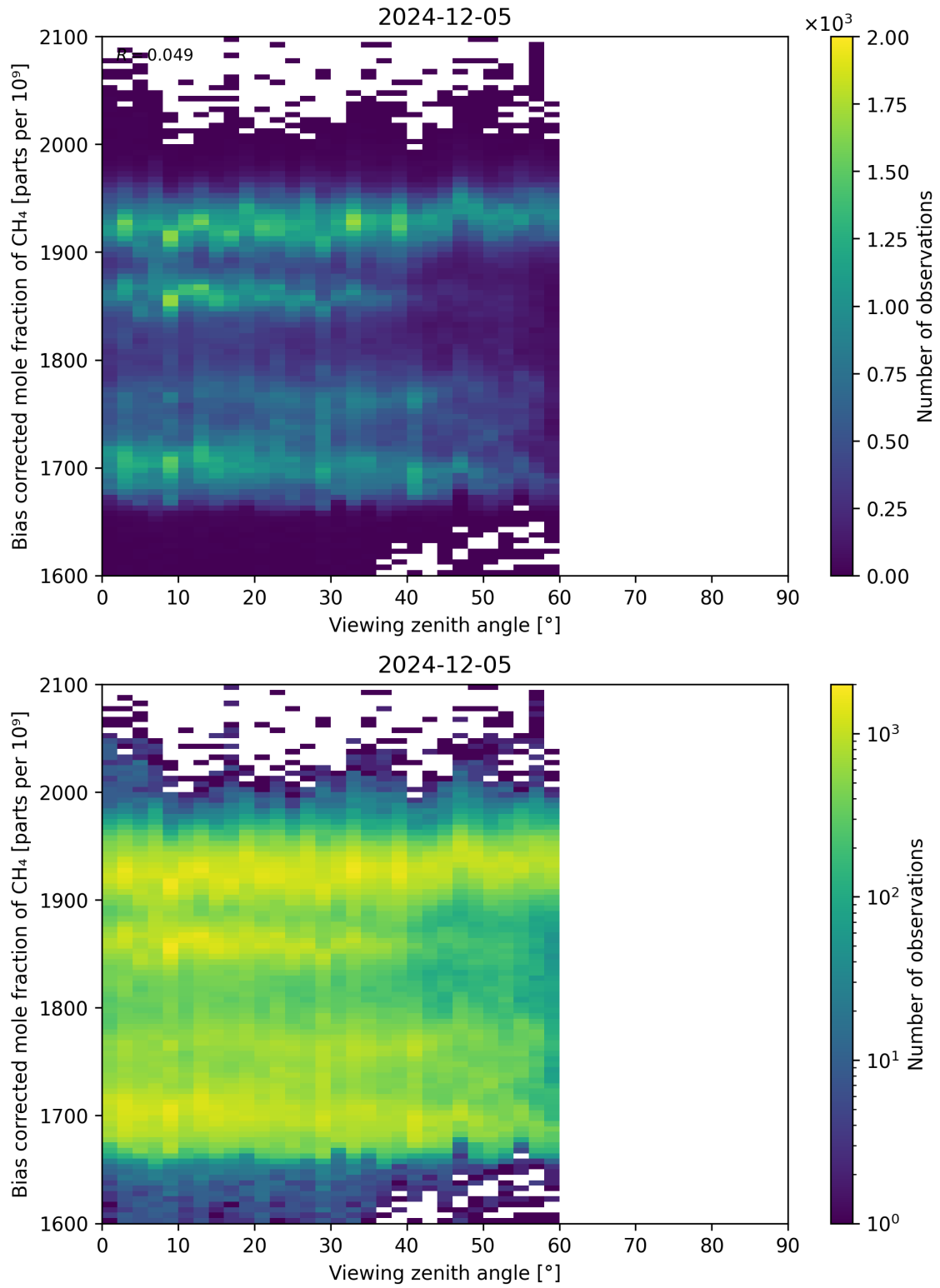
Figure 111: Scatter density plot of “Viewing zenith angle” against “Bias corrected mole fraction of CH 4 ” for 2024-12-04 to 2024-12-06.
