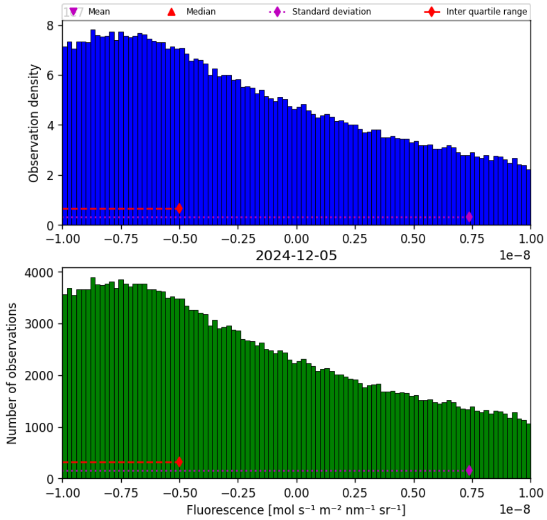
Figure 32: Histogram of “Fluorescence” for 2024-12-04 to 2024-12-06
