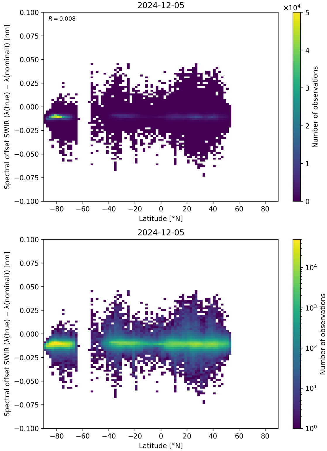
Figure 62: Scatter density plot of “Latitude” against “Spectral offset SWIR ( \lambda_{\text{true}} - \lambda_{\text{nominal}} )” for 2024-12-04 to 2024-12-06.
