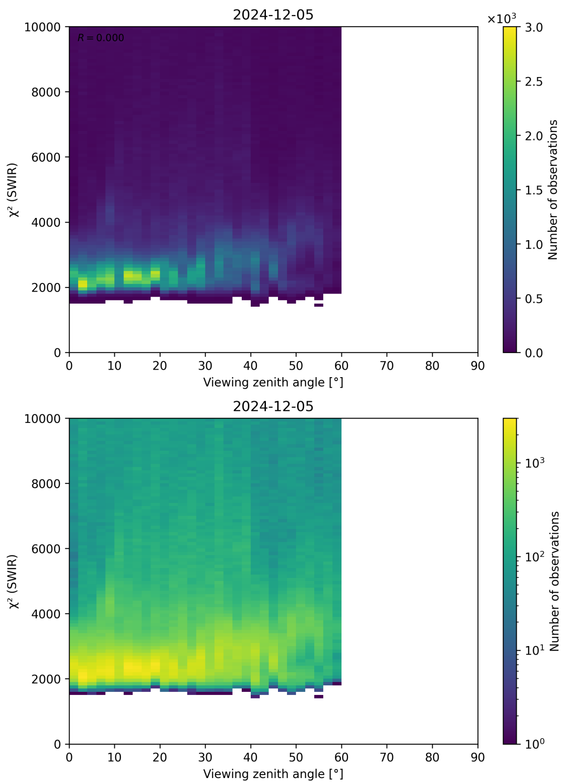
Figure 106: Scatter density plot of “Viewing zenith angle” against “ \chi^2 (SWIR)” for 2024-12-04 to 2024-12-06.
