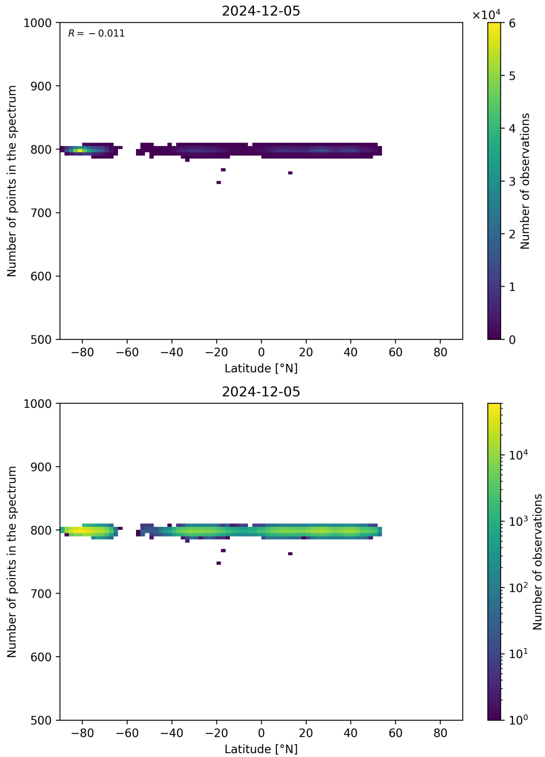
Figure 61: Scatter density plot of “Latitude” against “Number of points in the spectrum” for 2024-12-04 to 2024-12-06.
