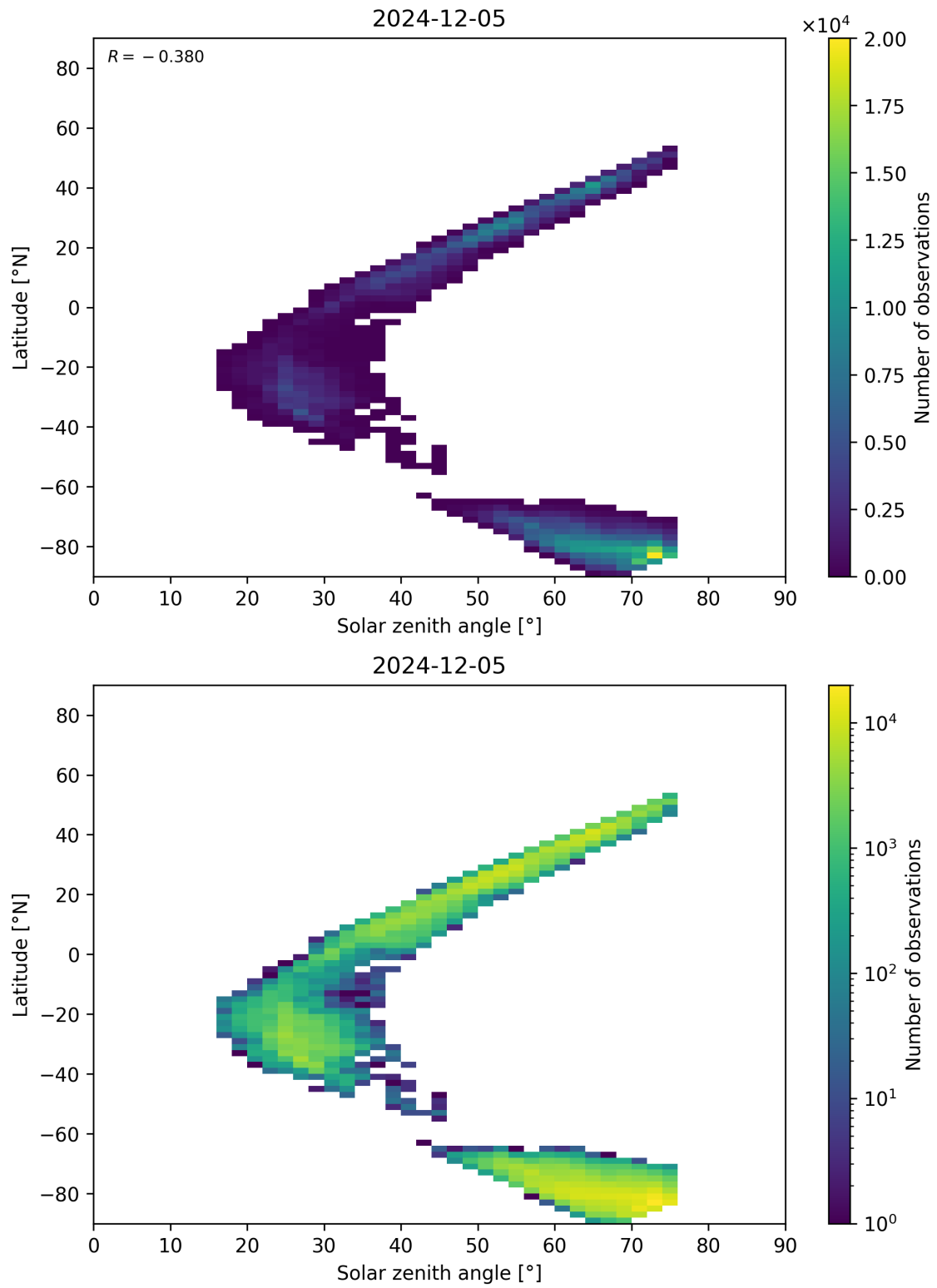
Figure 98: Scatter density plot of “Solar zenith angle” against “Latitude” for 2024-12-04 to 2024-12-06.
