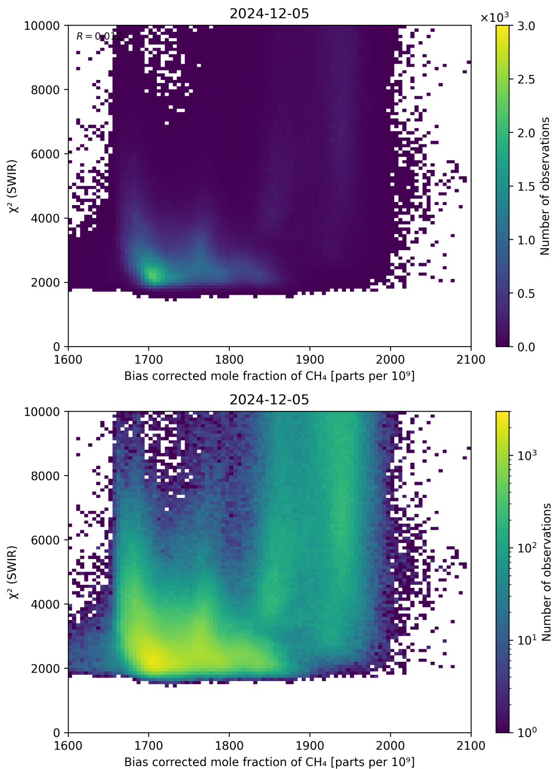
Figure 64: Scatter density plot of “Bias corrected mole fraction of \text{CH}_4 ” against “ \chi^2 (SWIR)” for 2024-12-04 to 2024-12-06.
