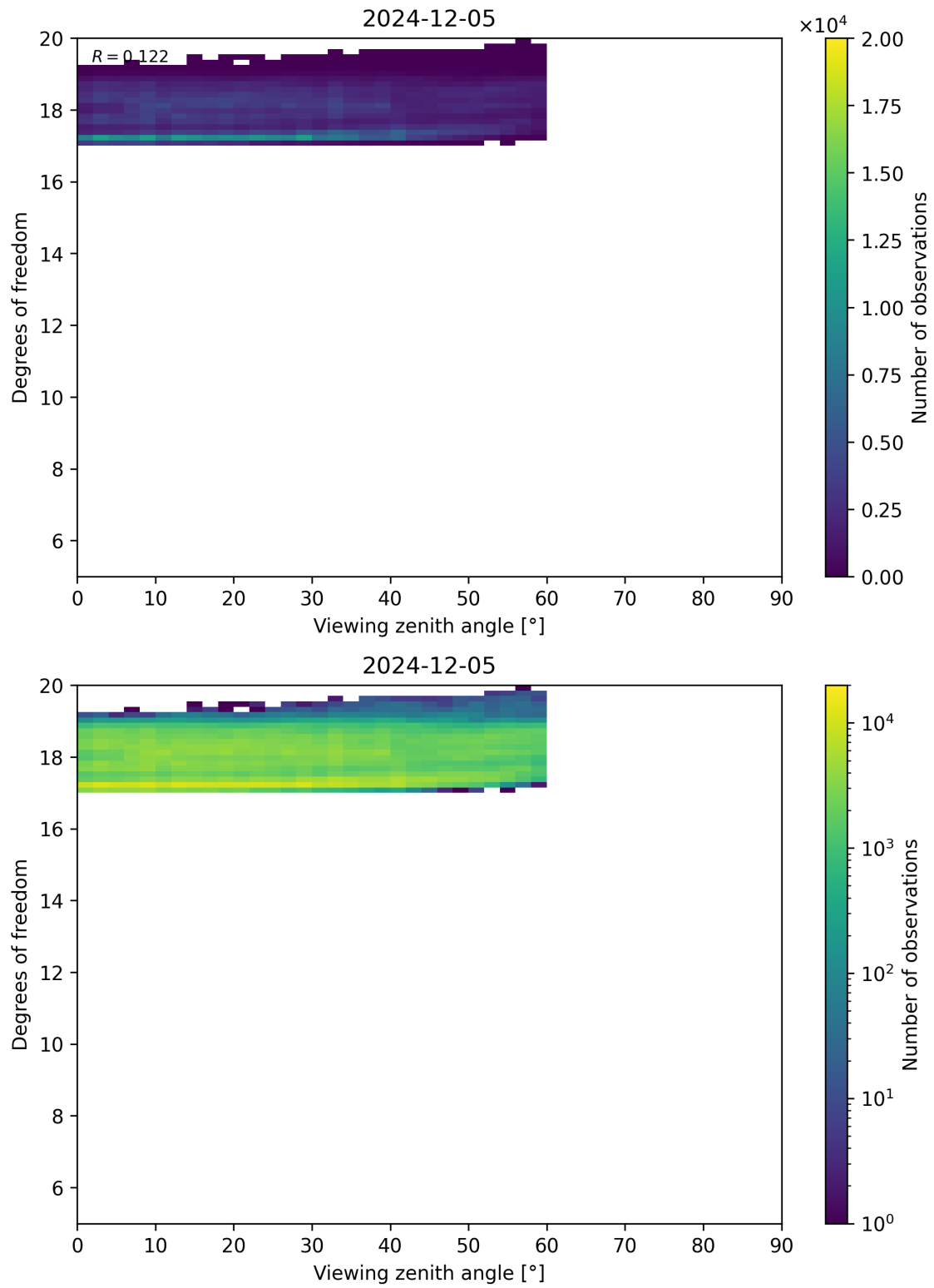
Figure 107: Scatter density plot of “Viewing zenith angle” against “Degrees of freedom” for 2024-12-04 to 2024-12-06.
