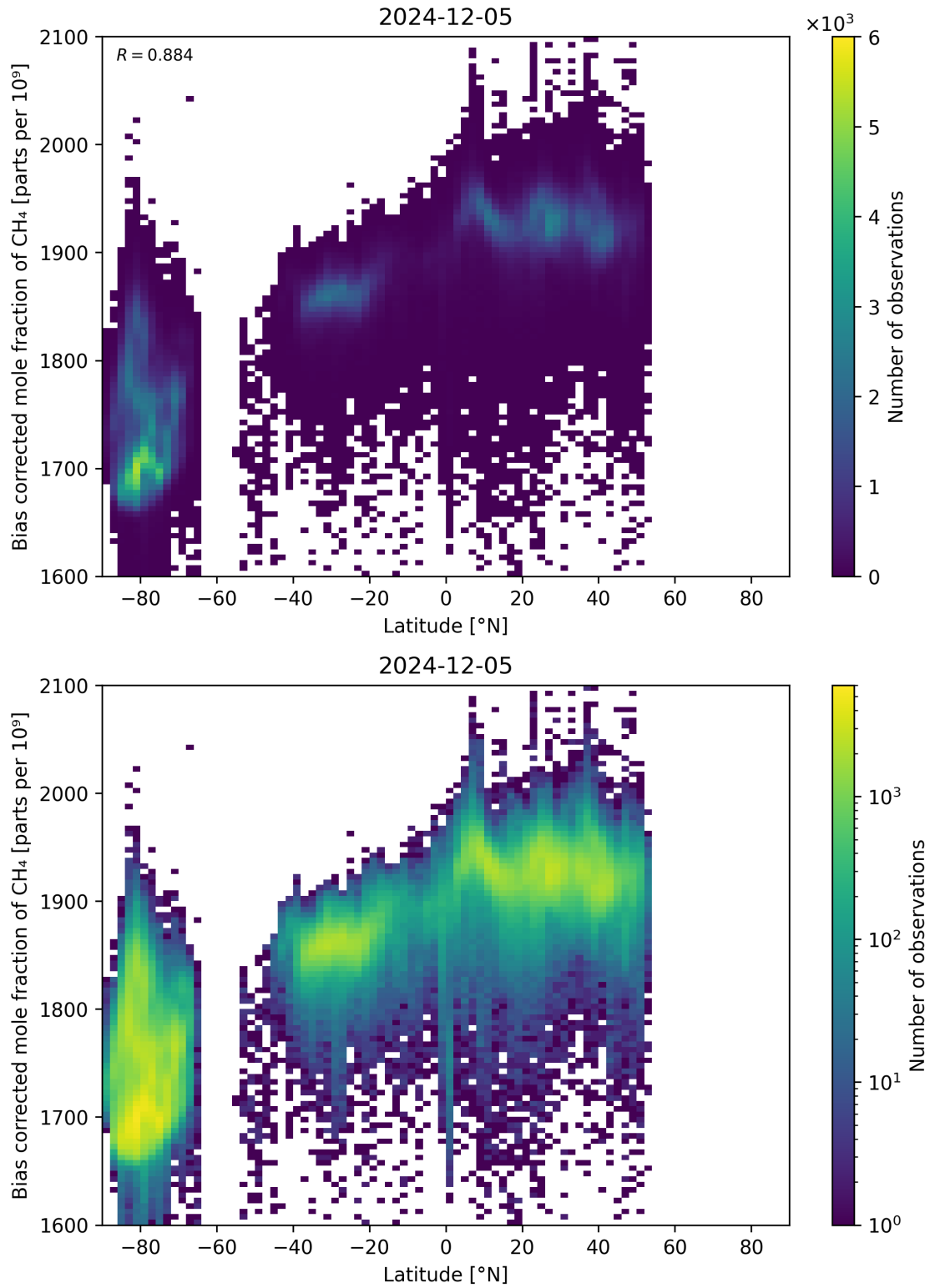
Figure 58: Scatter density plot of “Latitude” against “Bias corrected mole fraction of \text{CH}_4 ” for 2024-12-04 to 2024-12-06.
