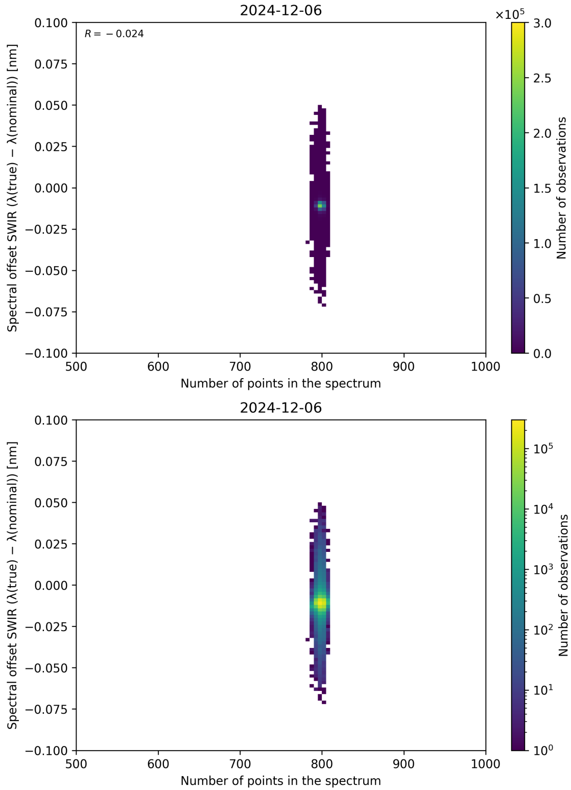
Figure 93: Scatter density plot of “Number of points in the spectrum” against “Spectral offset SWIR ( \lambda_{\text{true}} - \lambda_{\text{nominal}} )” for 2024-12-06 to 2024-12-07.
