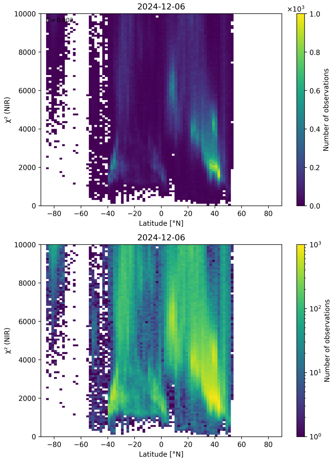
Figure 53: Scatter density plot of “Latitude” against “ \chi^2 (NIR)” for 2024-12-06 to 2024-12-07.
