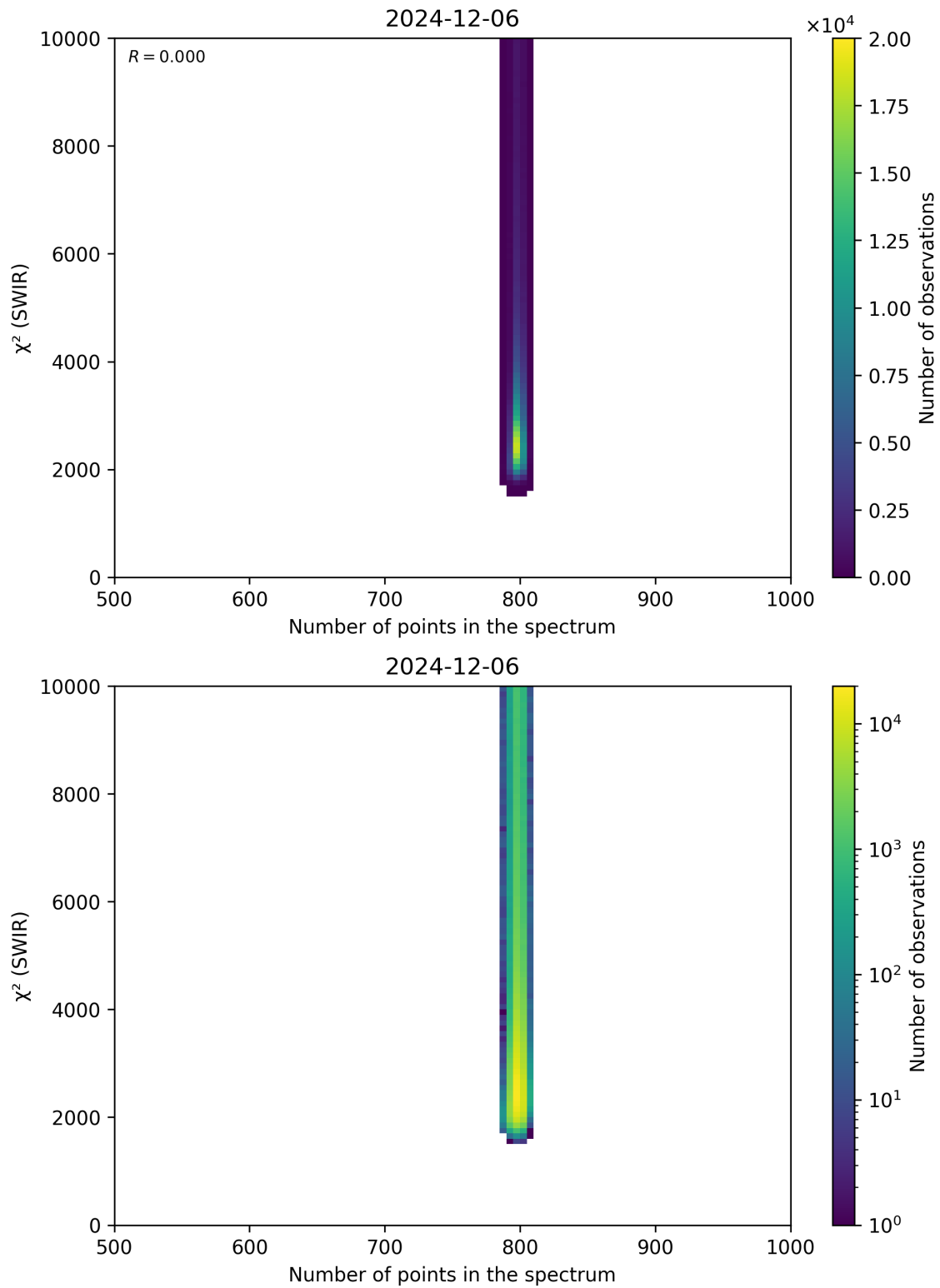
Figure 89: Scatter density plot of “Number of points in the spectrum” against “ \chi^2 (SWIR)” for 2024-12-06 to 2024-12-07.
