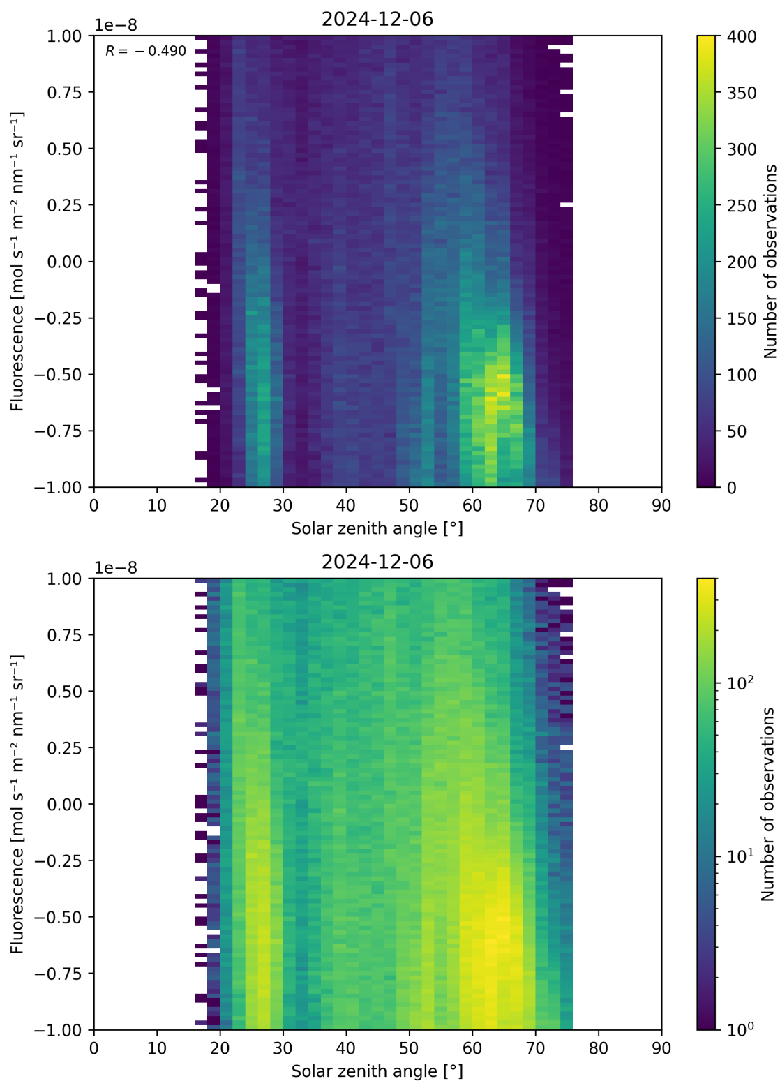
Figure 97: Scatter density plot of “Solar zenith angle” against “Fluorescence” for 2024-12-06 to 2024-12-07.
