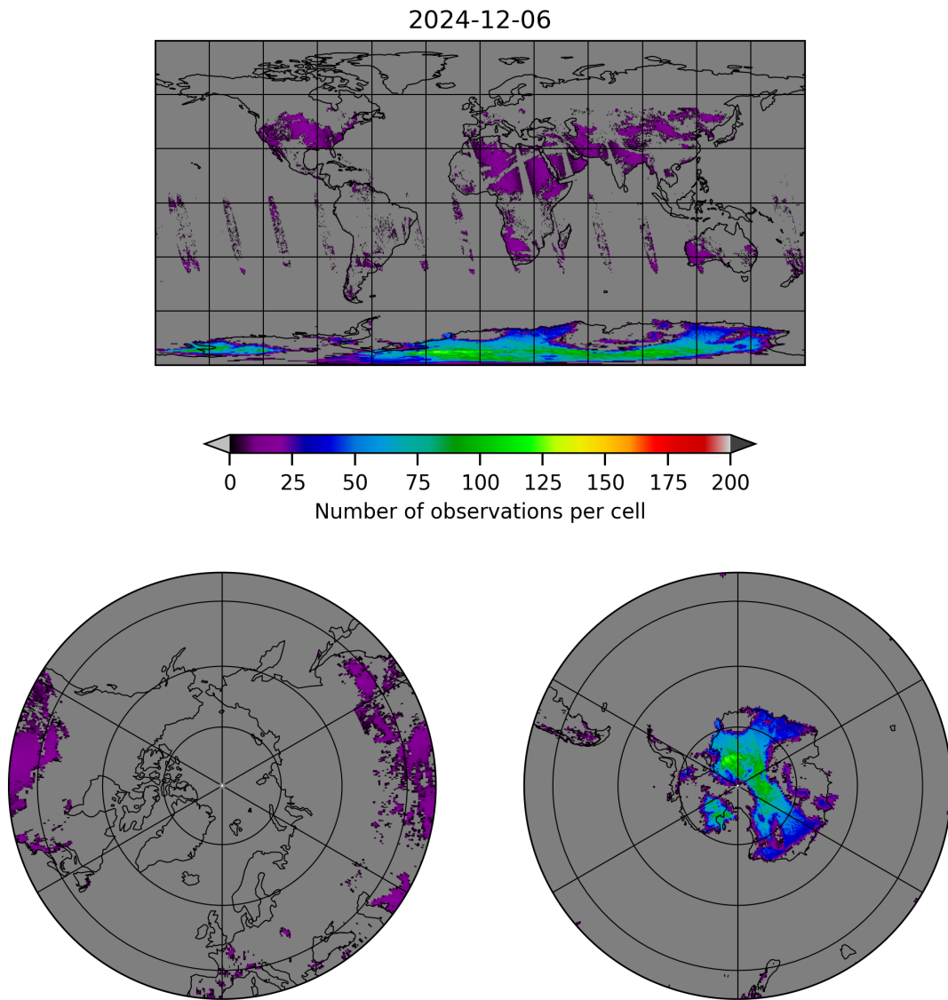
Figure 10: Map of the number of observations for 2024-12-06 to 2024-12-07
