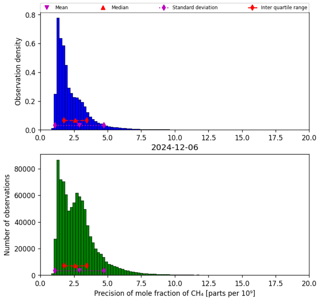
Figure 24: Histogram of “Precision of mole fraction of CH 4 ” for 2024-12-06 to 2024-12-07
