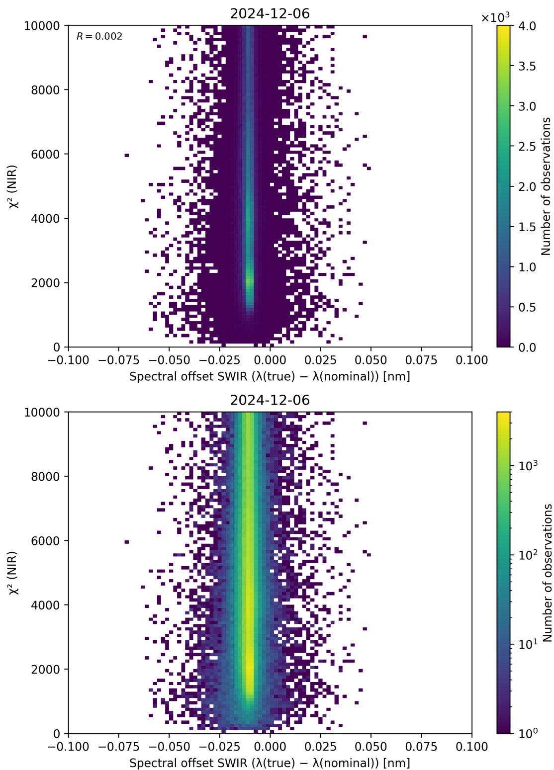
Figure 117: Scatter density plot of “Spectral offset SWIR ( \lambda_{\text{true}} - \lambda_{\text{nominal}} )” against “ \chi^2 (NIR)” for 2024-12-06 to 2024-12-07.
