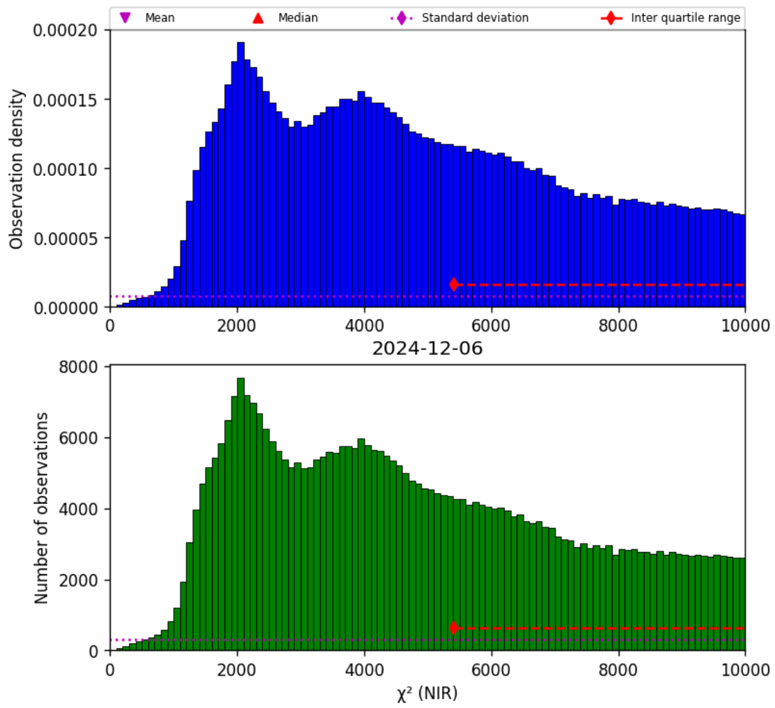
Figure 29: Histogram of “ \chi^2 (NIR)” for 2024-12-06 to 2024-12-07
