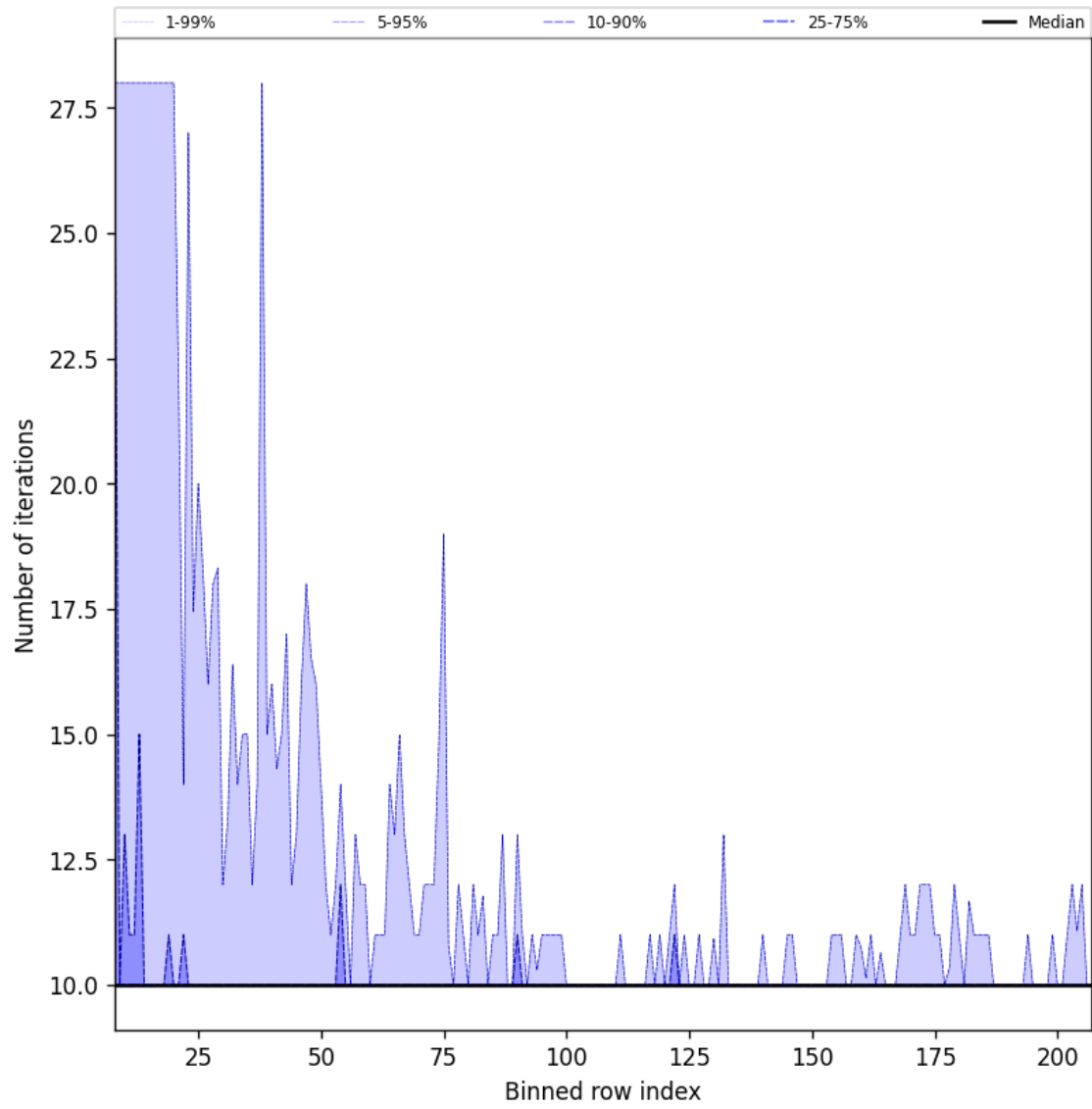
Figure 42: Along track statistics of “Number of iterations” for 2024-12-06 to 2024-12-07
