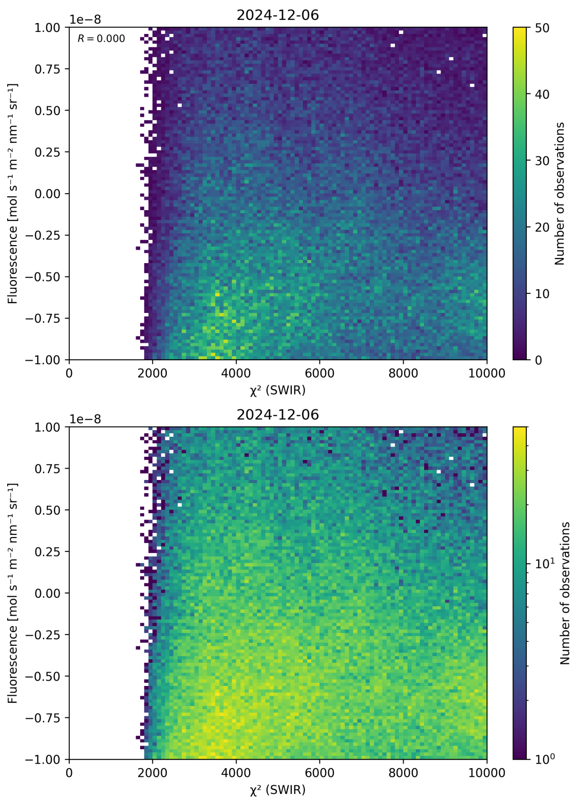
Figure 49: Scatter density plot of “ \chi^2 (SWIR)” against “Fluorescence” for 2024-12-06 to 2024-12-07.
