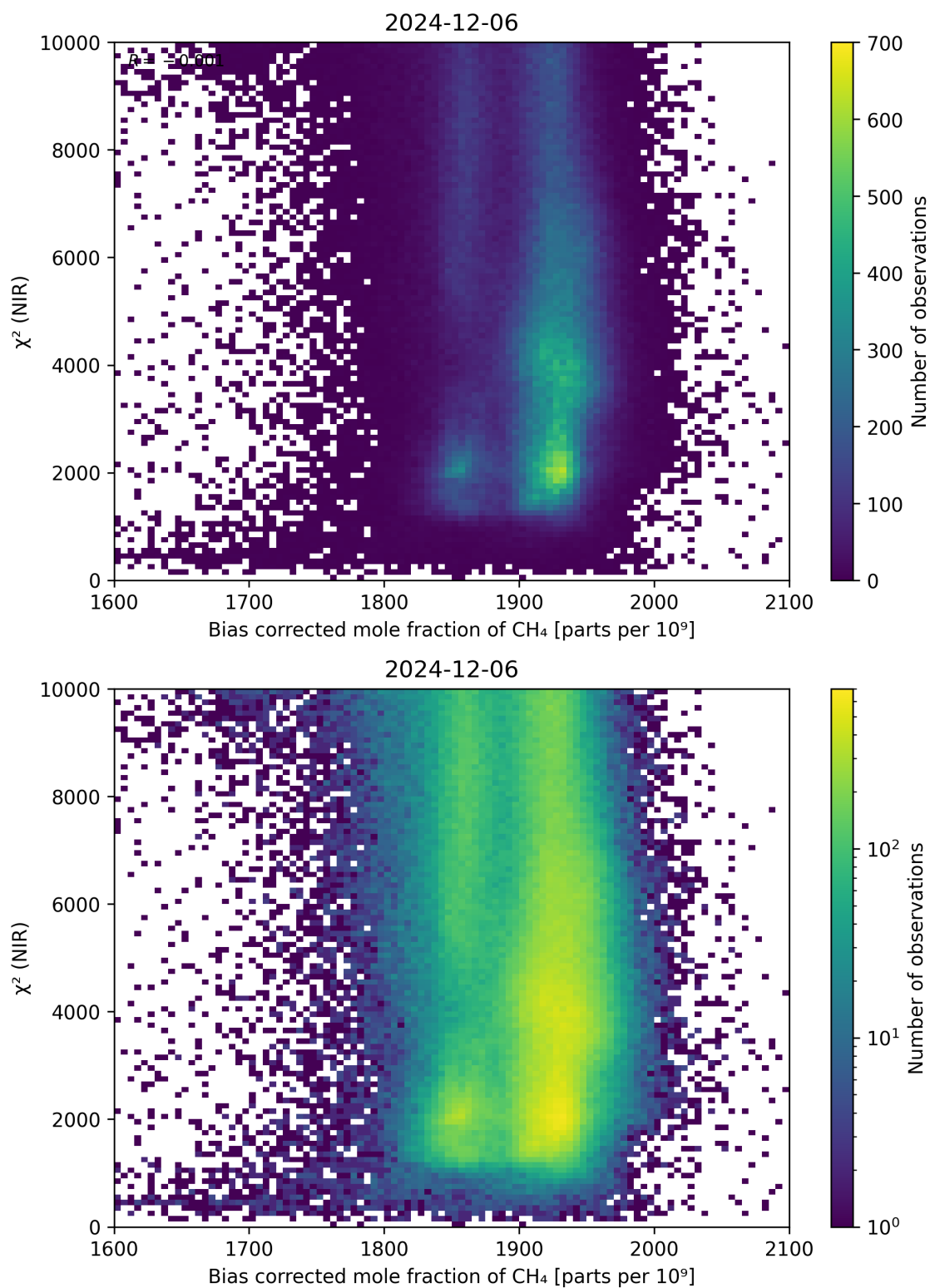
Figure 63: Scatter density plot of “Bias corrected mole fraction of \text{CH}_4 ” against “ \chi^2 (NIR)” for 2024-12-06 to 2024-12-07.
