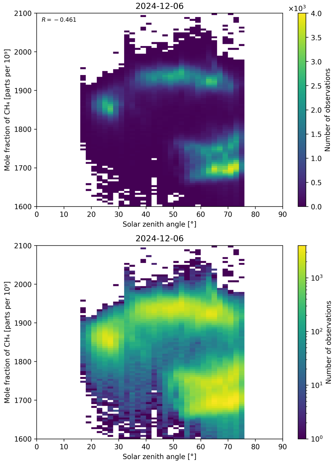
Figure 99: Scatter density plot of “Solar zenith angle” against “Mole fraction of \text{CH}_4 ” for 2024-12-06 to 2024-12-07.
