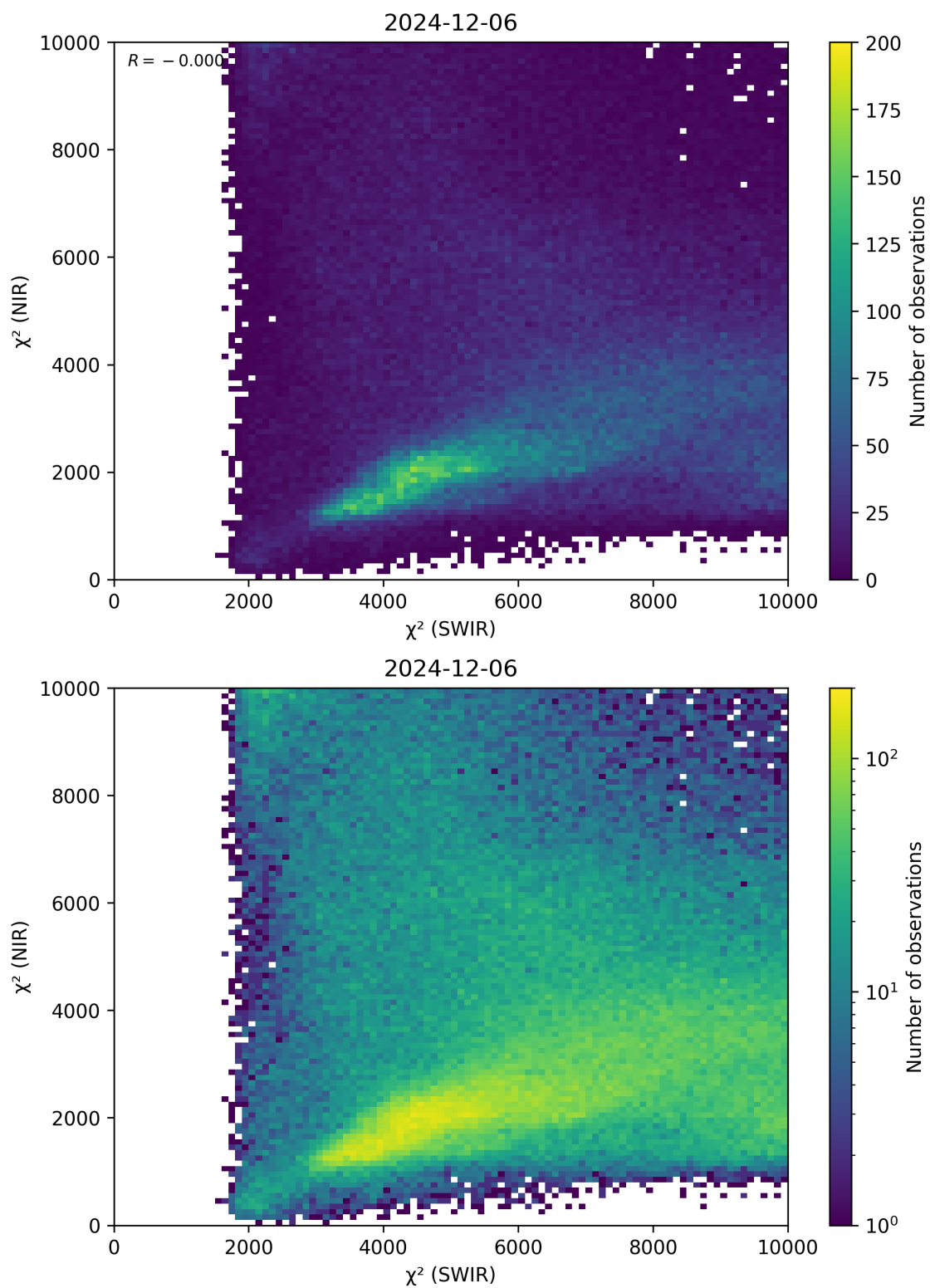
Figure 47: Scatter density plot of “ \chi^2 (SWIR)” against “ \chi^2 (NIR)” for 2024-12-06 to 2024-12-07.
