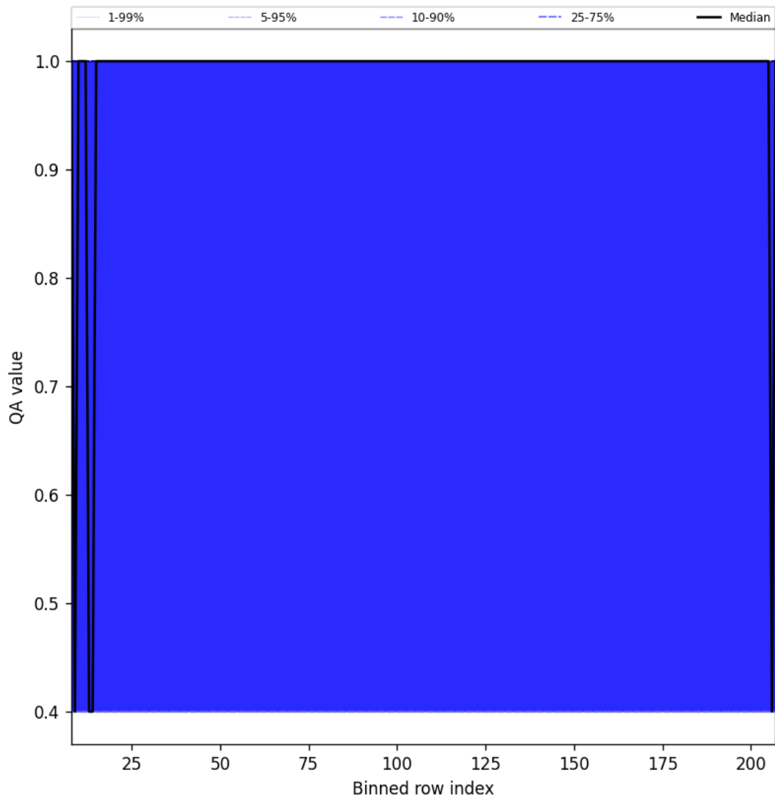
Figure 33: Along track statistics of “QA value” for 2024-12-06 to 2024-12-07
