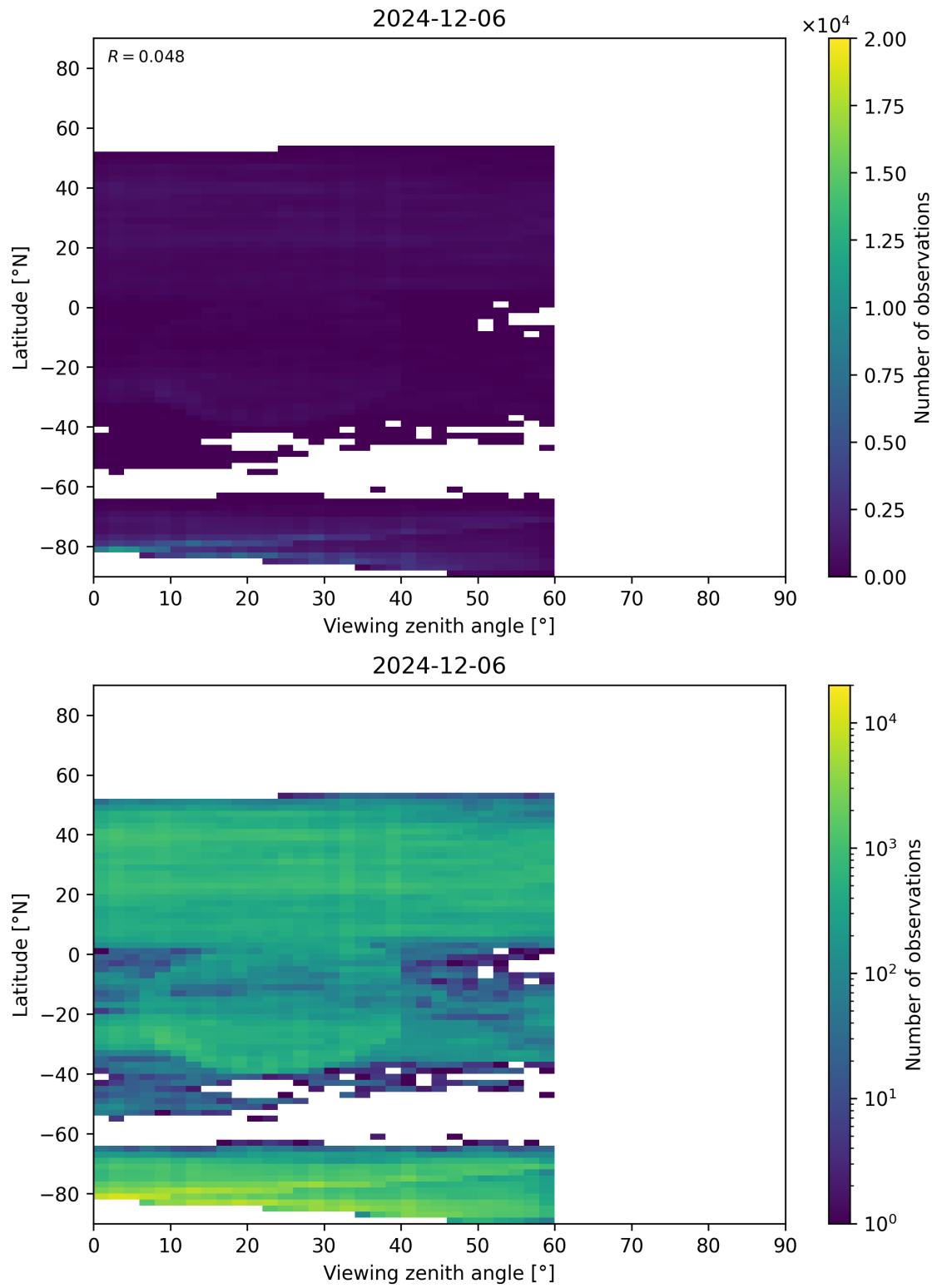
Figure 109: Scatter density plot of “Viewing zenith angle” against “Latitude” for 2024-12-06 to 2024-12-07.
