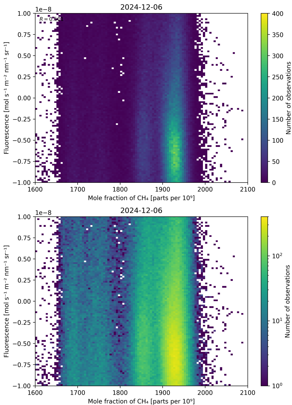
Figure 73: Scatter density plot of “Mole fraction of CH 4 ” against “Fluorescence” for 2024-12-06 to 2024-12-07.
