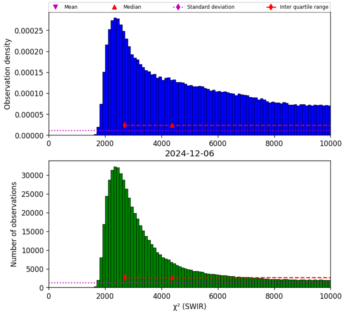
Figure 28: Histogram of “ \chi^2 (SWIR)” for 2024-12-06 to 2024-12-07
