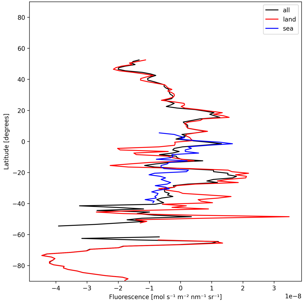
Figure 21: Zonal average of “Fluorescence” for 2024-12-06 to 2024-12-07.
