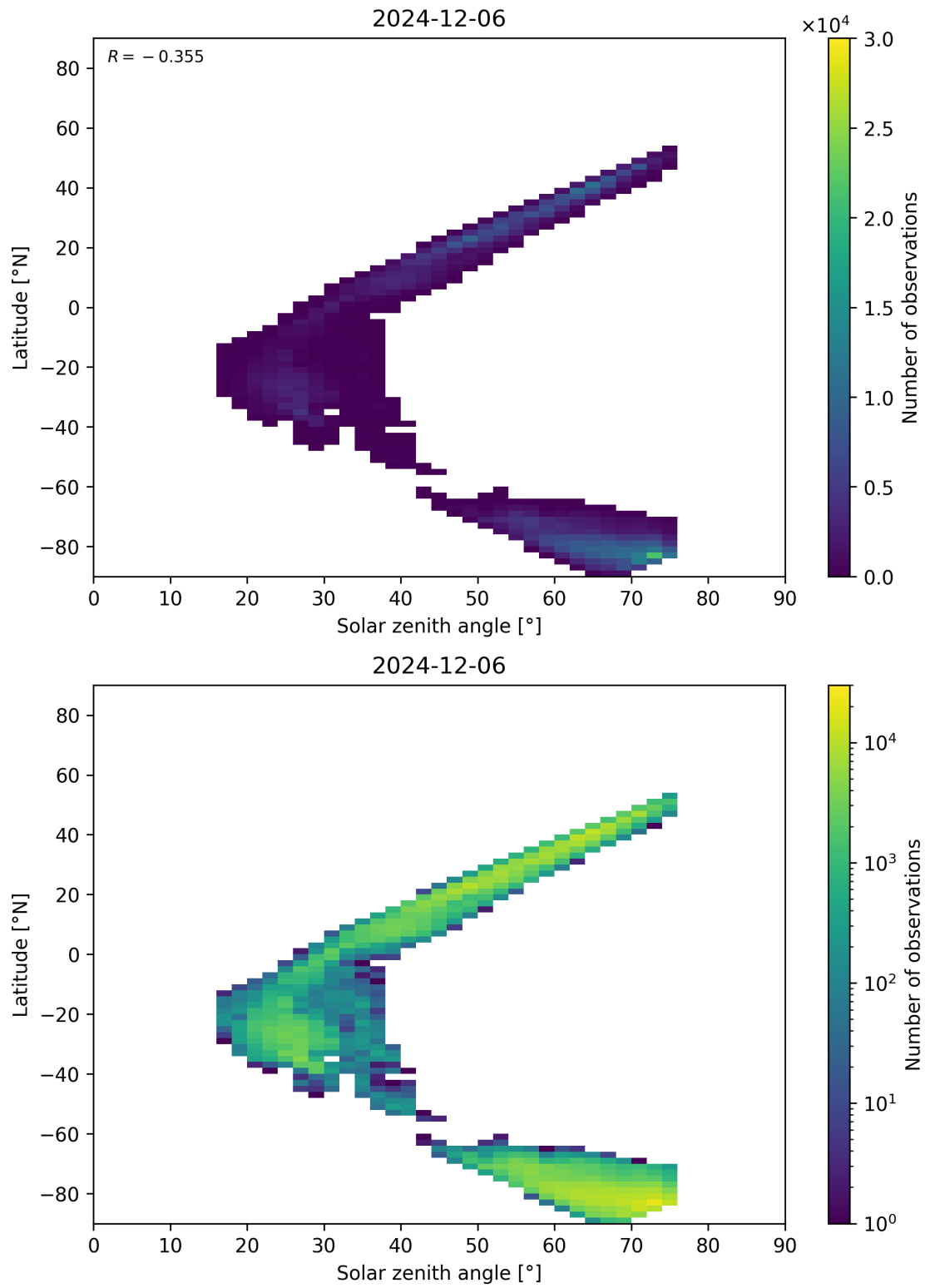
Figure 98: Scatter density plot of “Solar zenith angle” against “Latitude” for 2024-12-06 to 2024-12-07.
