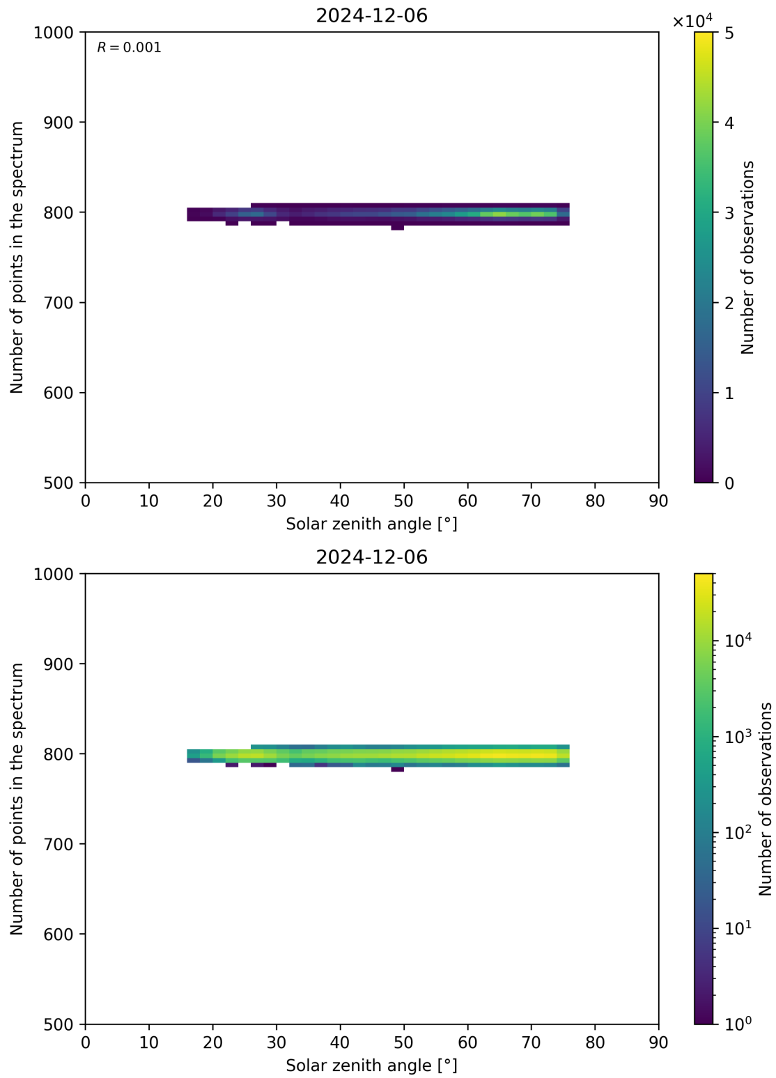
Figure 103: Scatter density plot of “Solar zenith angle” against “Number of points in the spectrum” for 2024-12-06 to 2024-12-07.
