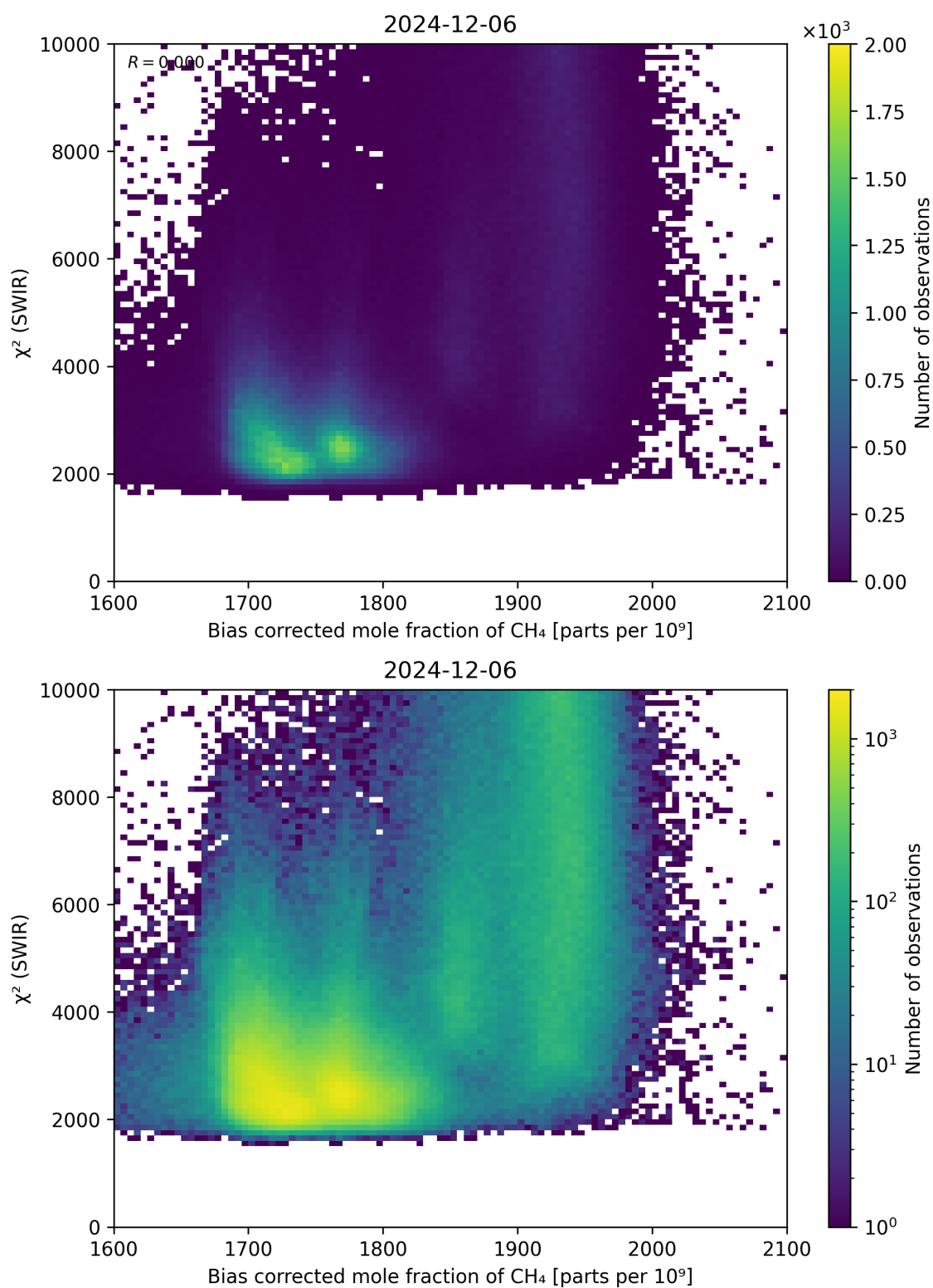
Figure 64: Scatter density plot of “Bias corrected mole fraction of \text{CH}_4 ” against “ \chi^2 (SWIR)” for 2024-12-06 to 2024-12-07.
