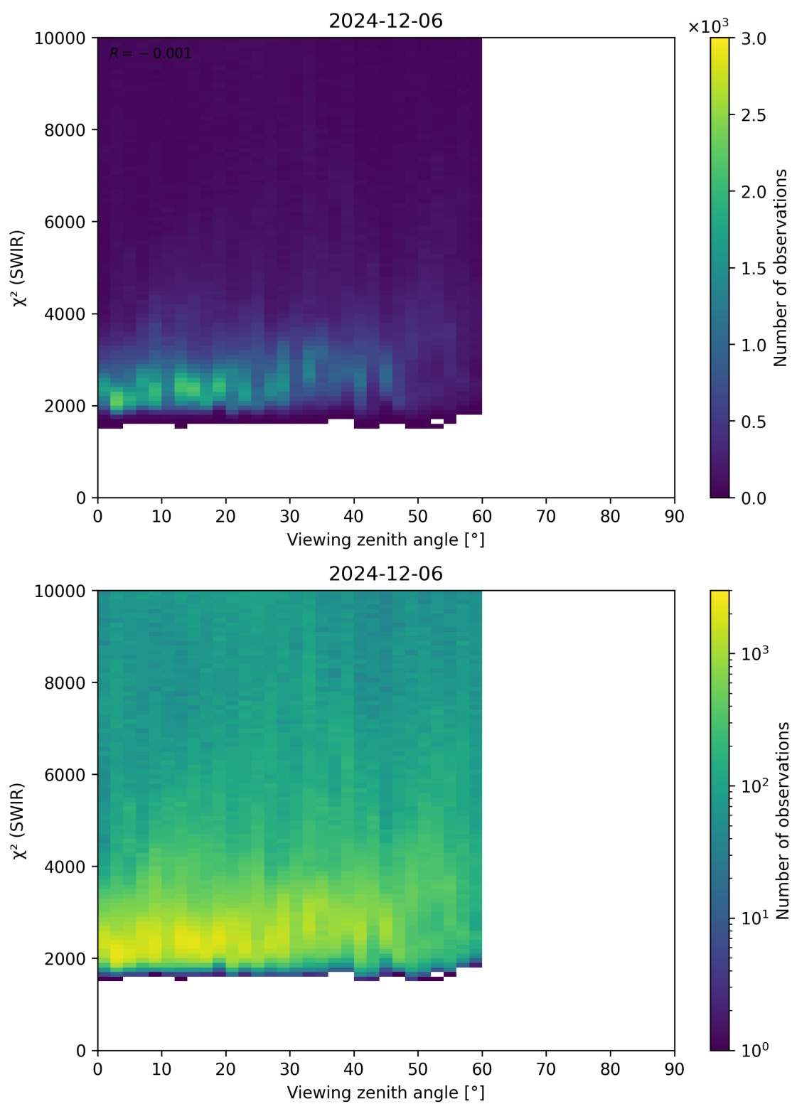
Figure 106: Scatter density plot of “Viewing zenith angle” against “ \chi^2 (SWIR)” for 2024-12-06 to 2024-12-07.
