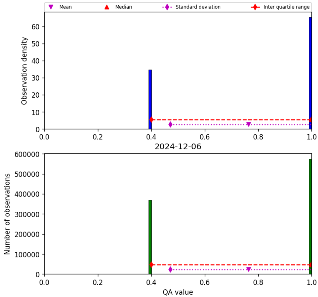
Figure 22: Histogram of “QA value” for 2024-12-06 to 2024-12-07
