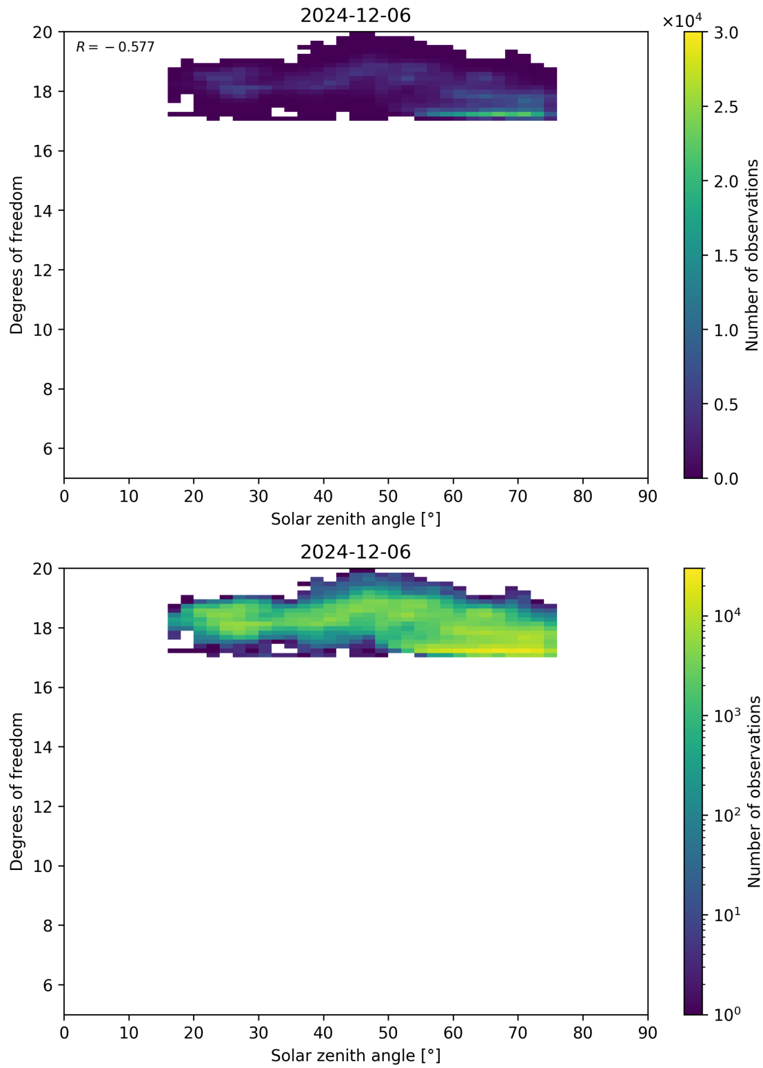
Figure 96: Scatter density plot of “Solar zenith angle” against “Degrees of freedom” for 2024-12-06 to 2024-12-07.
