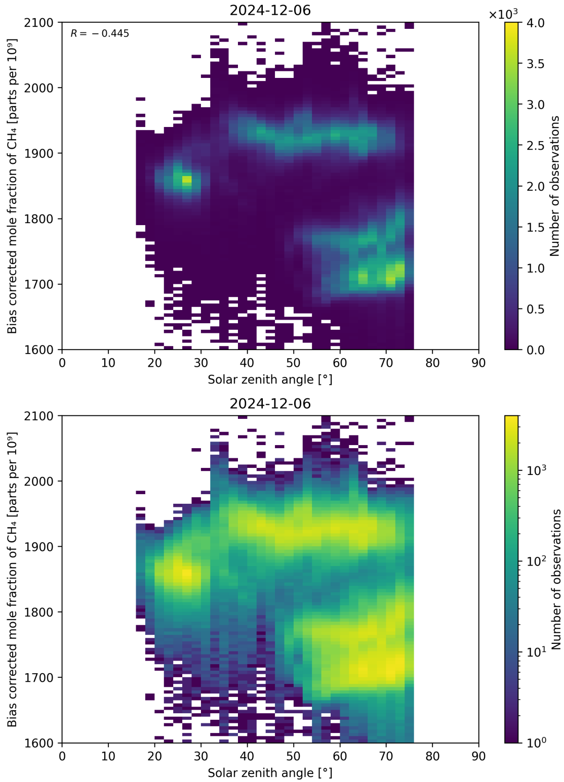
Figure 100: Scatter density plot of “Solar zenith angle” against “Bias corrected mole fraction of \text{CH}_4 ” for 2024-12-06 to 2024-12-07.
