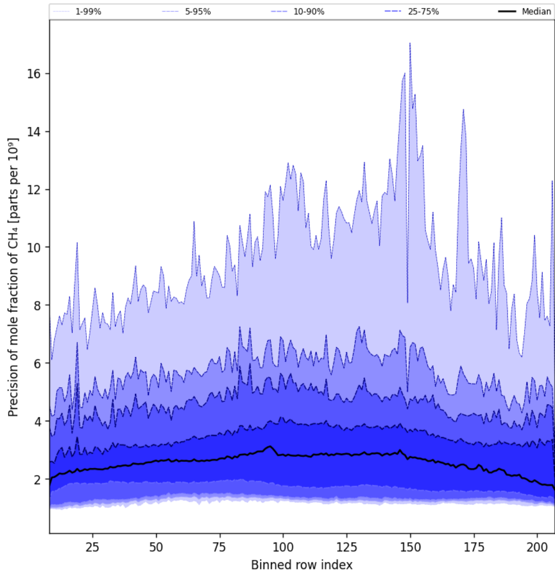
Figure 35: Along track statistics of “Precision of mole fraction of CH 4 ” for 2024-12-06 to 2024-12-07
