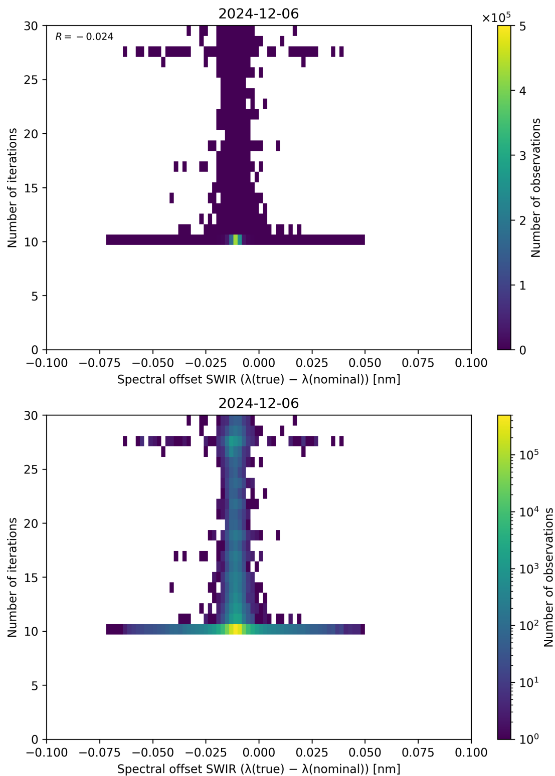
Figure 121: Scatter density plot of “Spectral offset SWIR ( \lambda_{\text{true}} - \lambda_{\text{nominal}} )” against “Number of iterations” for 2024-12-06 to 2024-12-07.
