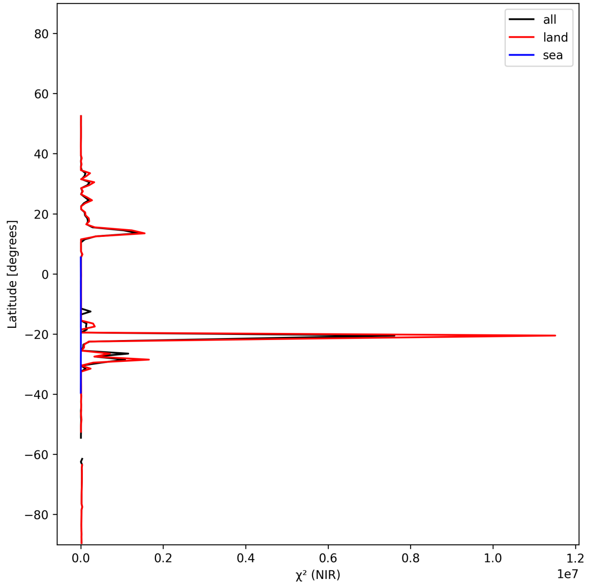
Figure 18: Zonal average of “ \chi^2 (NIR)” for 2024-12-06 to 2024-12-07.
