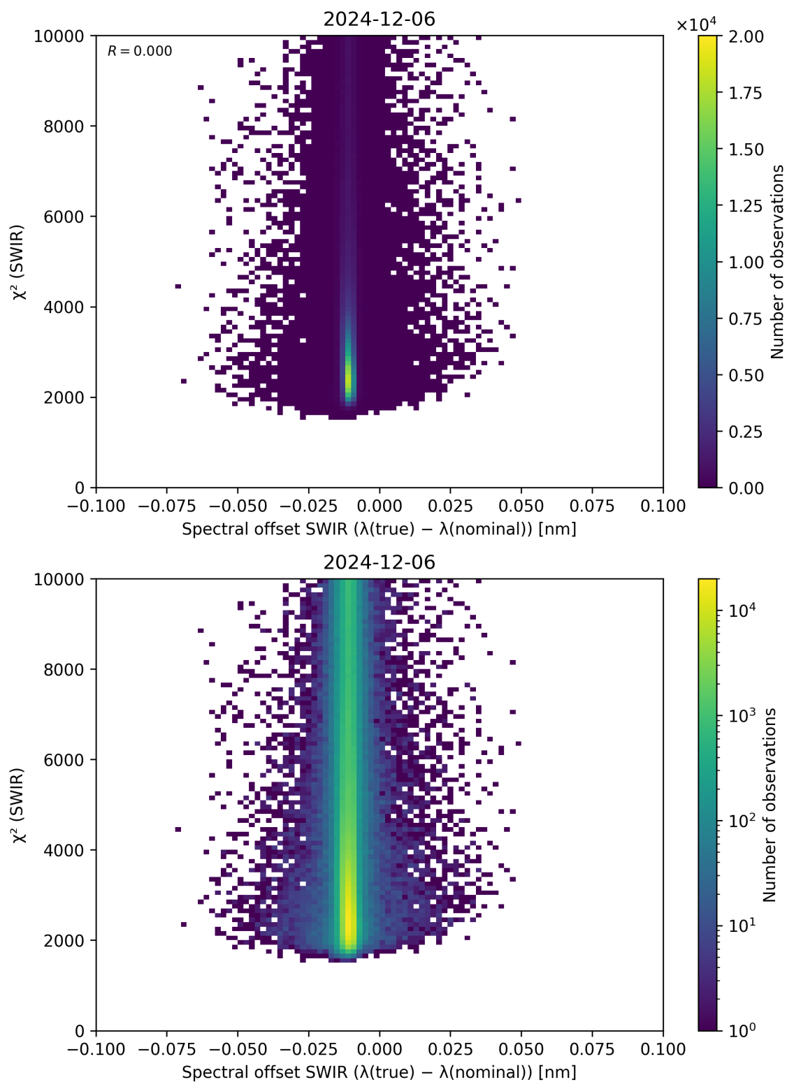
Figure 118: Scatter density plot of “Spectral offset SWIR ( \lambda_{\text{true}} - \lambda_{\text{nominal}} )” against “ \chi^2 (SWIR)” for 2024-12-06 to 2024-12-07.
