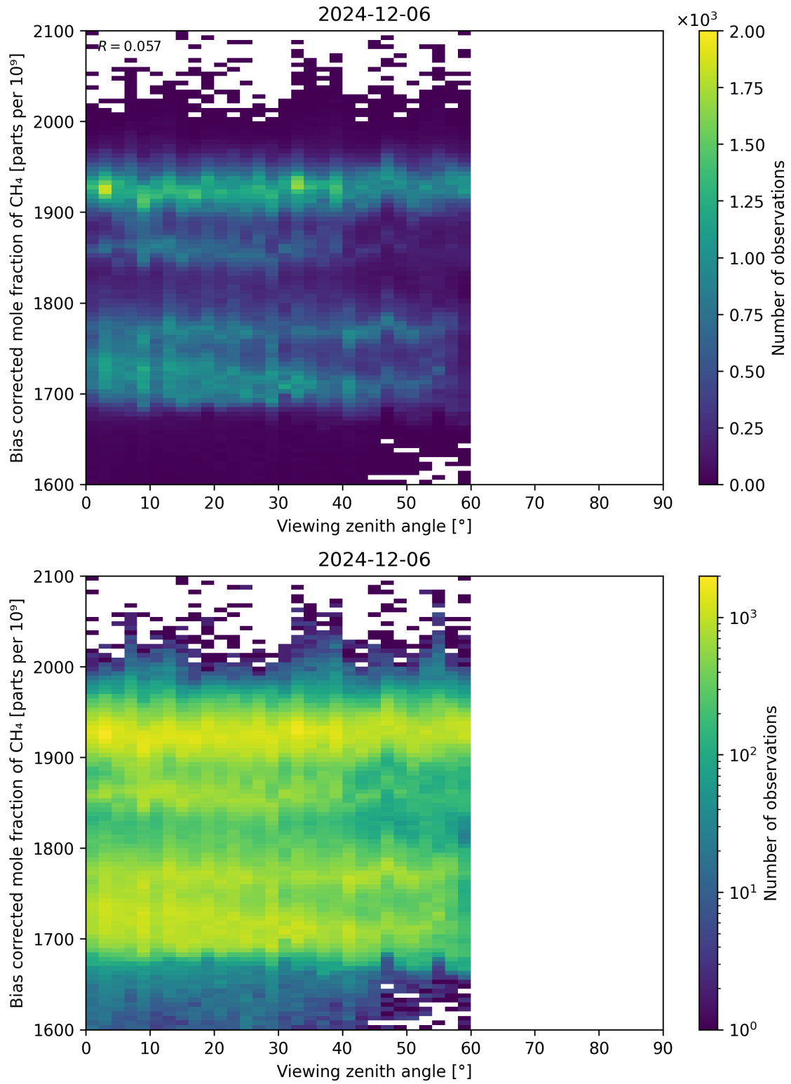
Figure 111: Scatter density plot of “Viewing zenith angle” against “Bias corrected mole fraction of CH 4 ” for 2024-12-06 to 2024-12-07.
