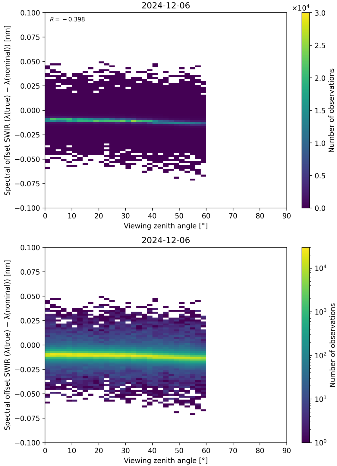
Figure 116: Scatter density plot of “Viewing zenith angle” against “Spectral offset SWIR ( \lambda_{\text{true}} - \lambda_{\text{nominal}} )” for 2024-12-06 to 2024-12-07.
