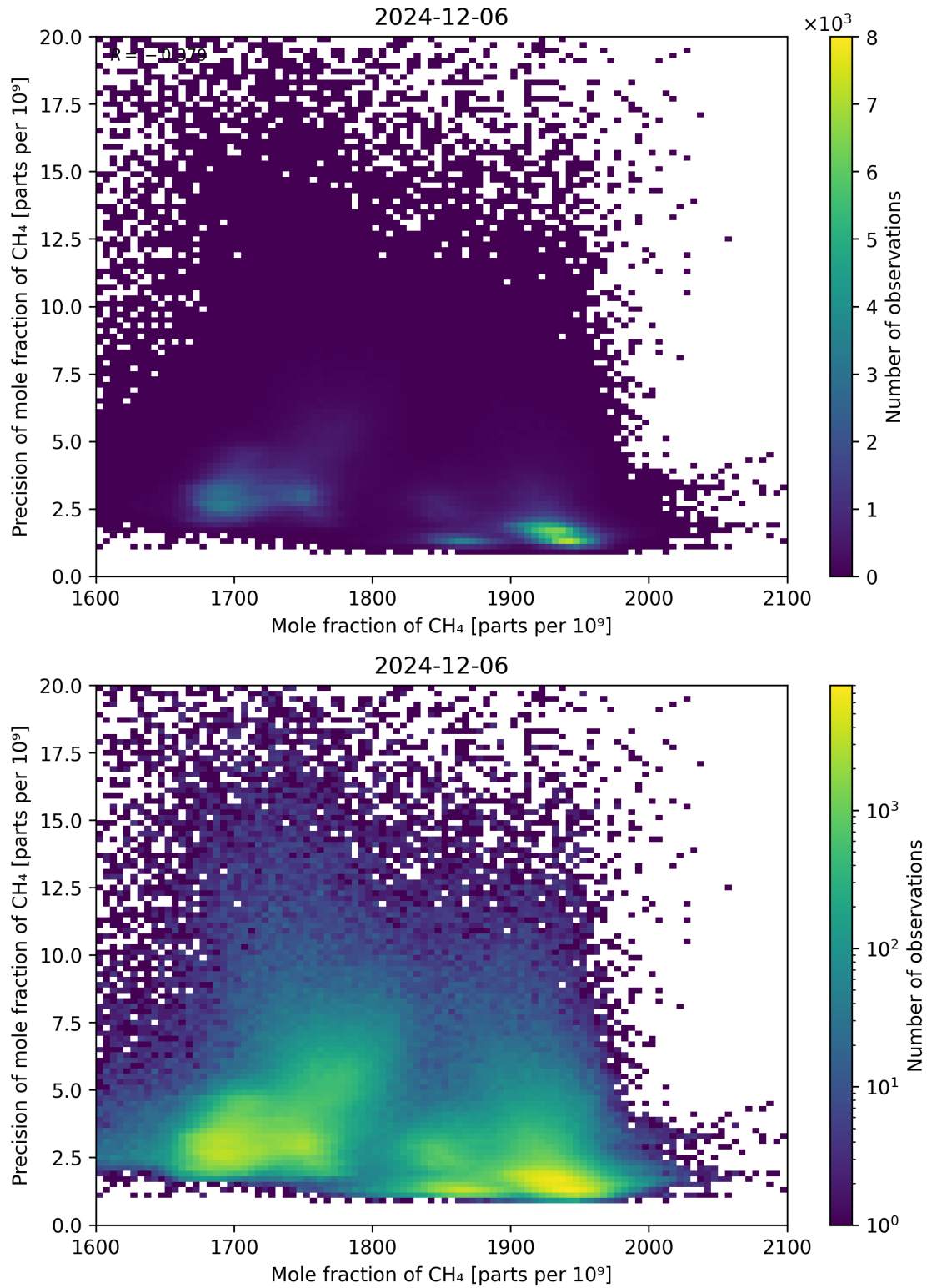
Figure 75: Scatter density plot of “Mole fraction of CH 4 ” against “Precision of mole fraction of CH 4 ” for 2024-12-06 to 2024-12-07.
