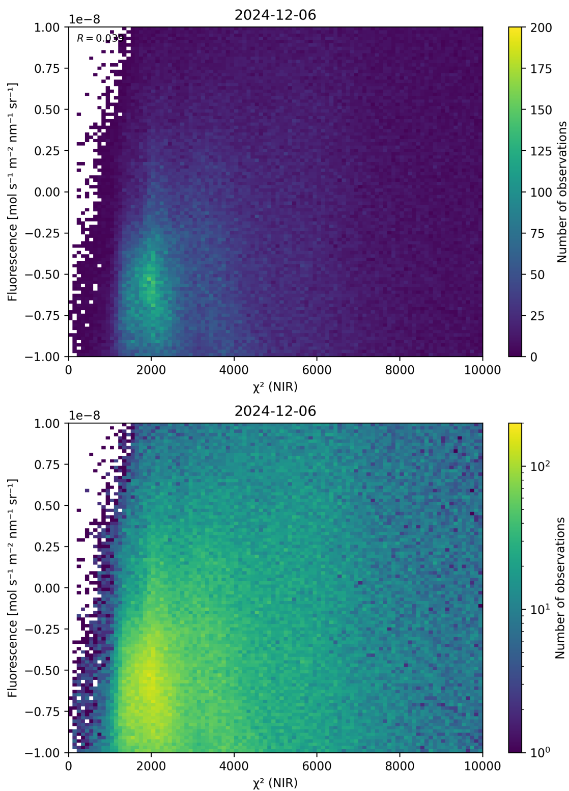
Figure 45: Scatter density plot of “ \chi^2 (NIR)” against “Fluorescence” for 2024-12-06 to 2024-12-07.
