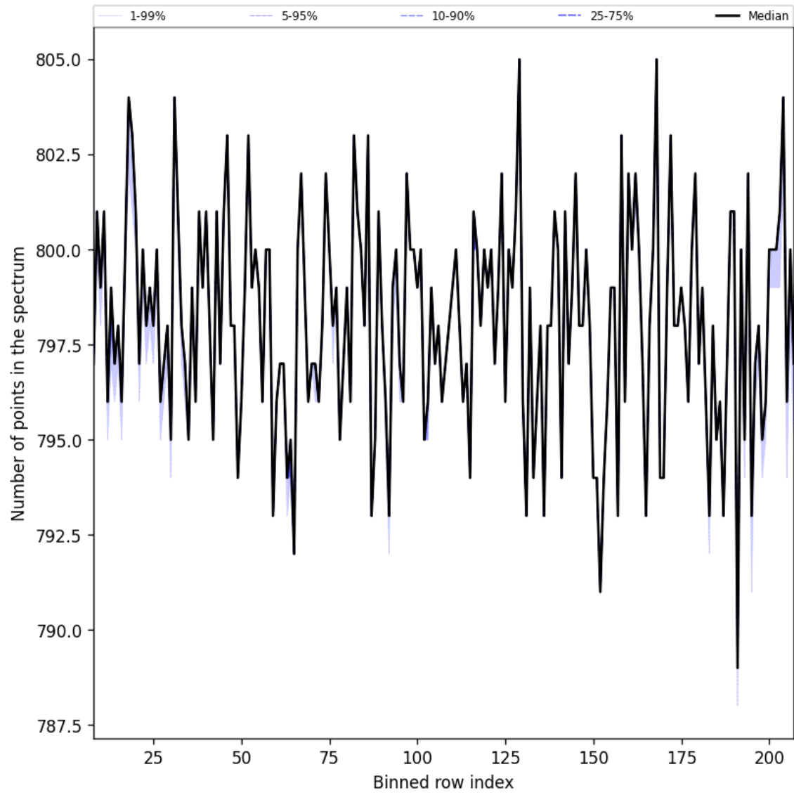
Figure 37: Along track statistics of “Number of points in the spectrum” for 2024-12-06 to 2024-12-07
