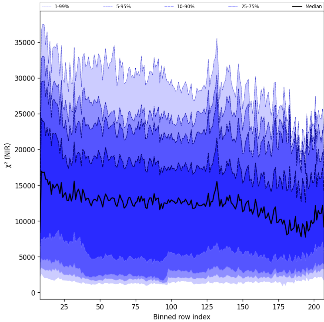
Figure 40: Along track statistics of “ \chi^2 (NIR)” for 2024-12-06 to 2024-12-07
