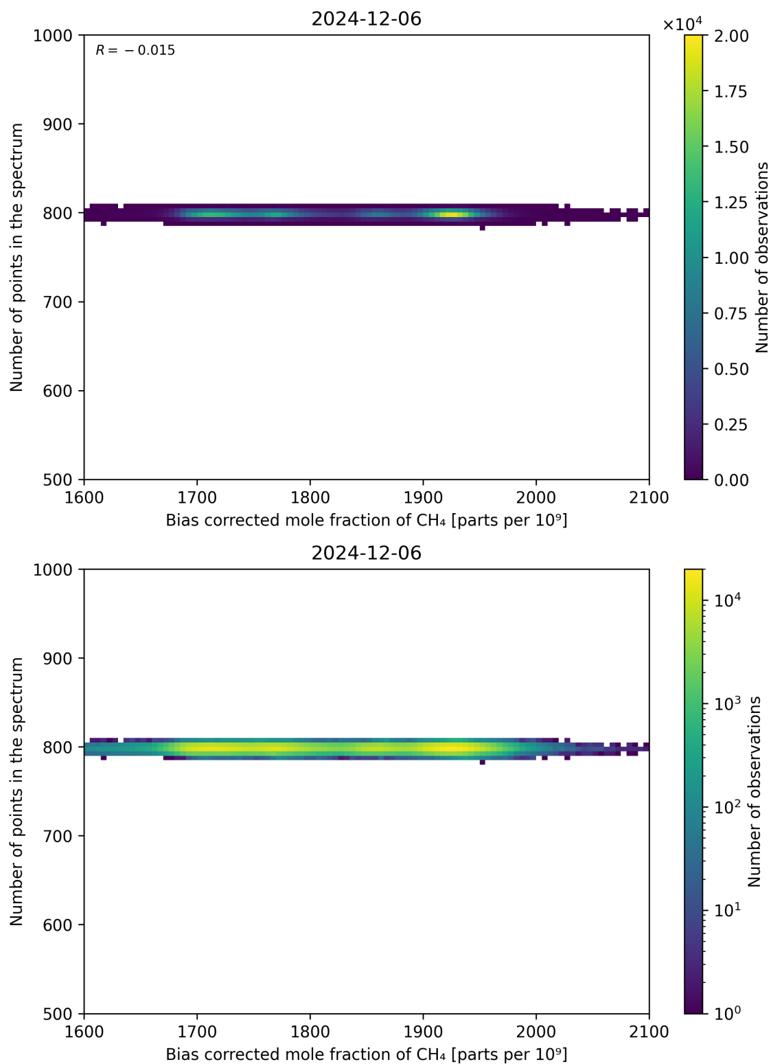
Figure 68: Scatter density plot of “Bias corrected mole fraction of CH 4 ” against “Number of points in the spectrum” for 2024-12-06 to 2024-12-07.
