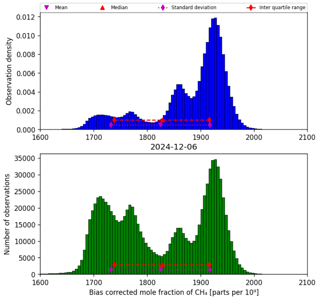
Figure 25: Histogram of “Bias corrected mole fraction of CH 4 ” for 2024-12-06 to 2024-12-07
