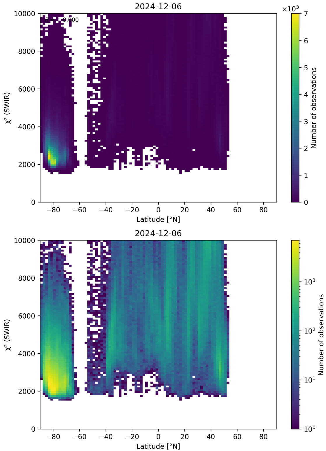
Figure 54: Scatter density plot of “Latitude” against “ \chi^2 (SWIR)” for 2024-12-06 to 2024-12-07.
