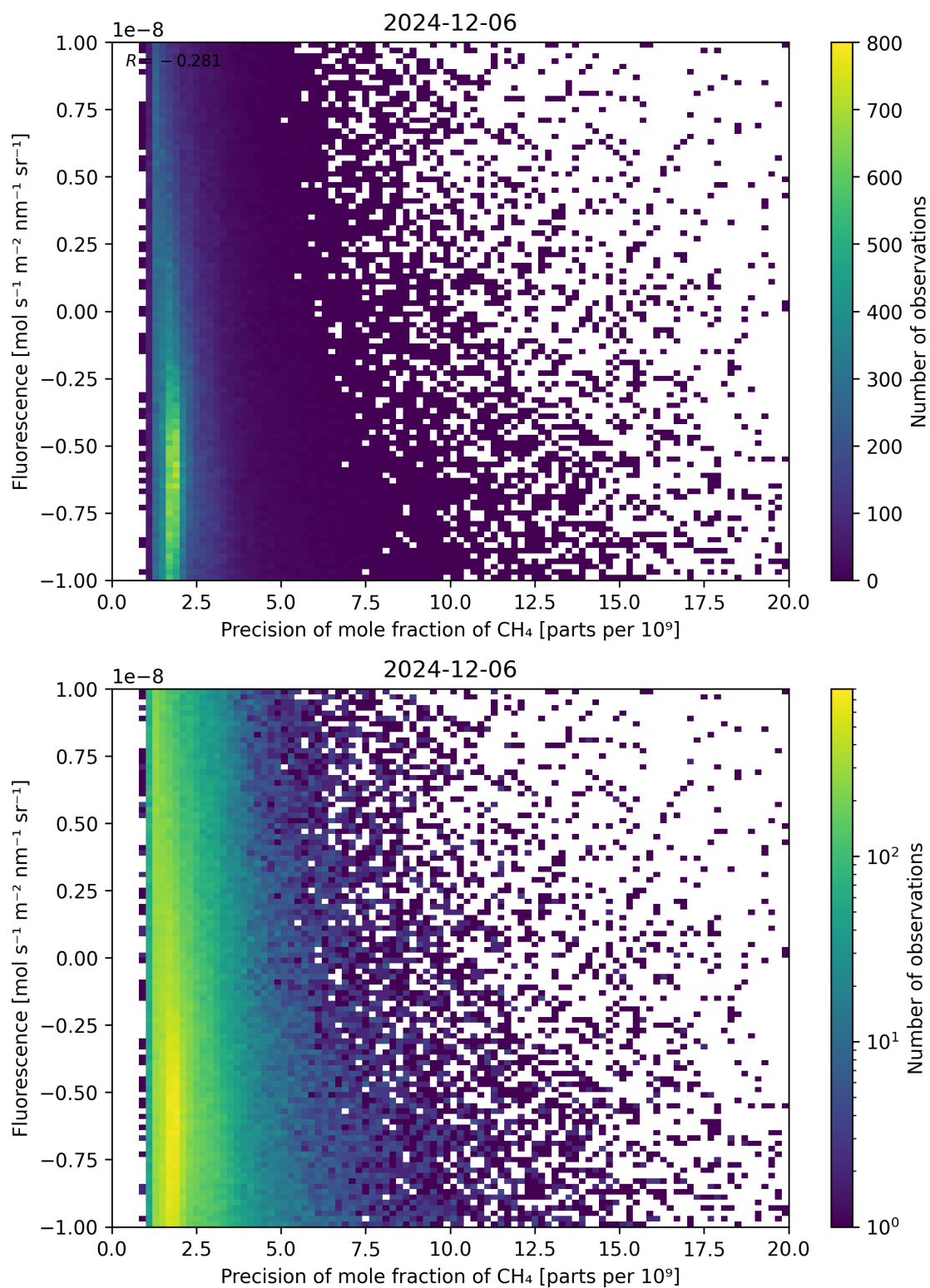
Figure 81: Scatter density plot of “Precision of mole fraction of \text{CH}_4 ” against “Fluorescence” for 2024-12-06 to 2024-12-07.
