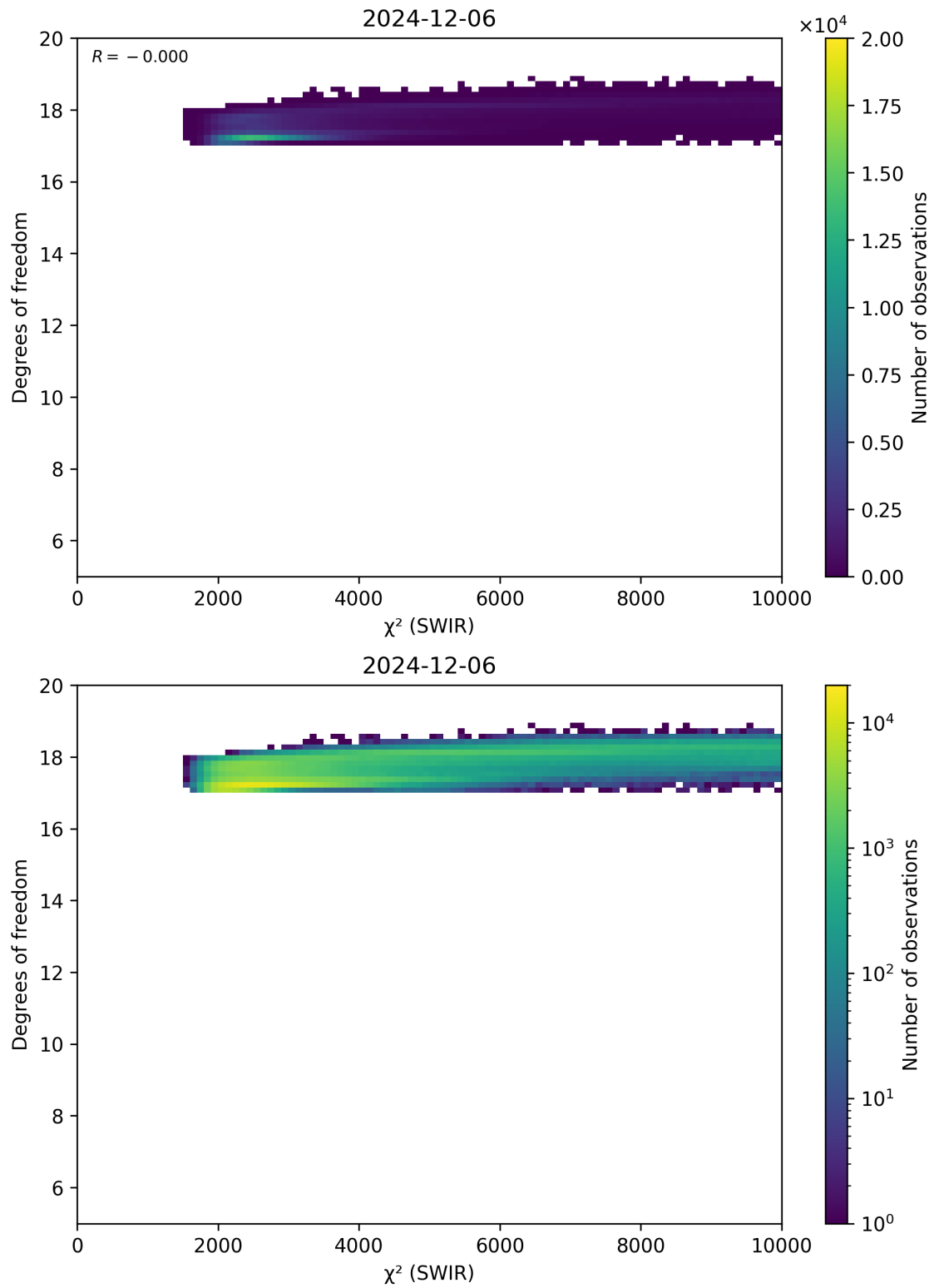
Figure 48: Scatter density plot of “ \chi^2 (SWIR)” against “Degrees of freedom” for 2024-12-06 to 2024-12-07.
