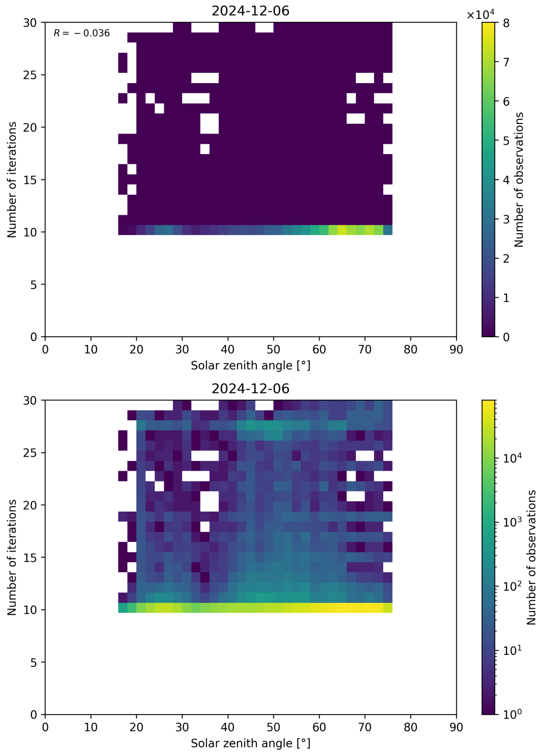
Figure 102: Scatter density plot of “Solar zenith angle” against “Number of iterations” for 2024-12-06 to 2024-12-07.
