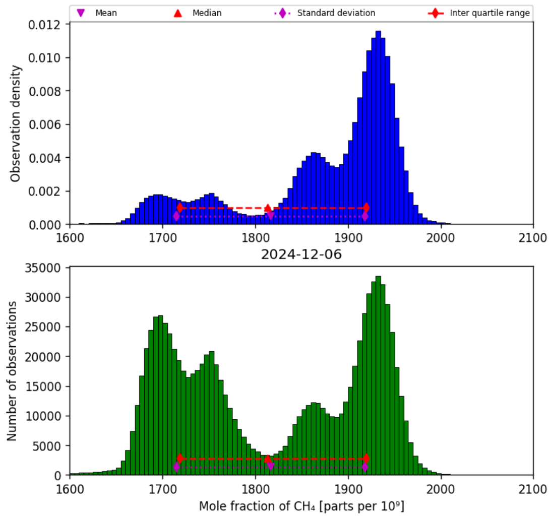
Figure 23: Histogram of “Mole fraction of CH 4 ” for 2024-12-06 to 2024-12-07
