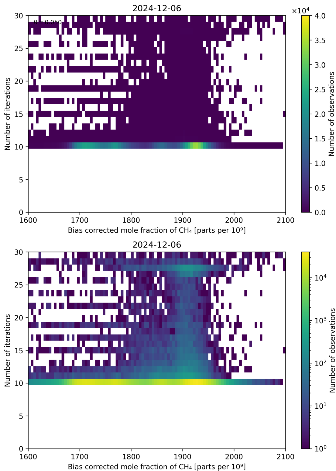
Figure 67: Scatter density plot of “Bias corrected mole fraction of CH 4 ” against “Number of iterations” for 2024-12-06 to 2024-12-07.
