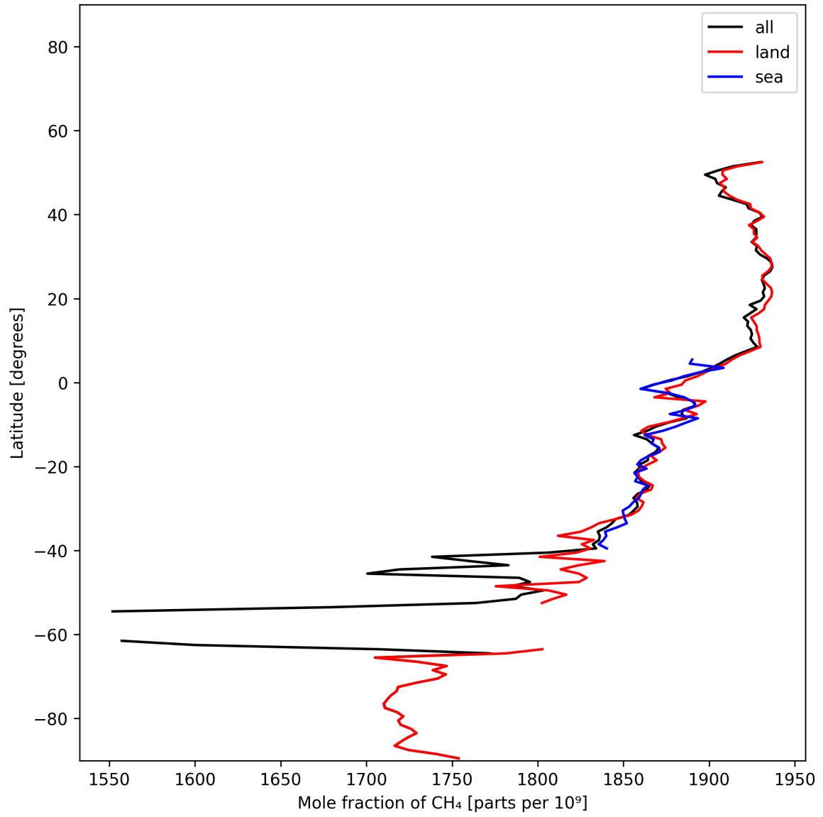
Figure 12: Zonal average of “Mole fraction of CH 4 ” for 2024-12-06 to 2024-12-07.
