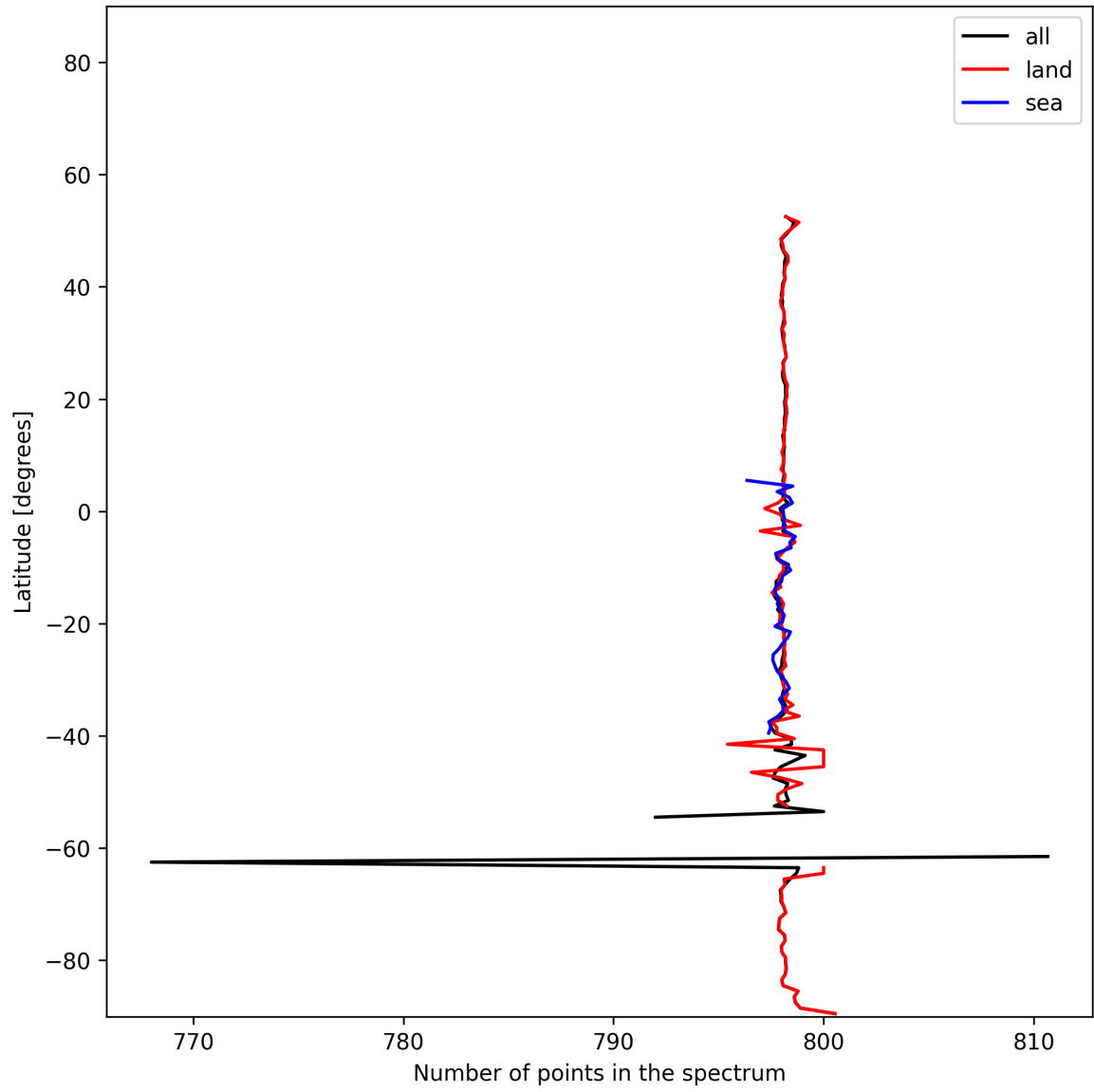
Figure 15: Zonal average of “Number of points in the spectrum” for 2024-12-06 to 2024-12-07.
