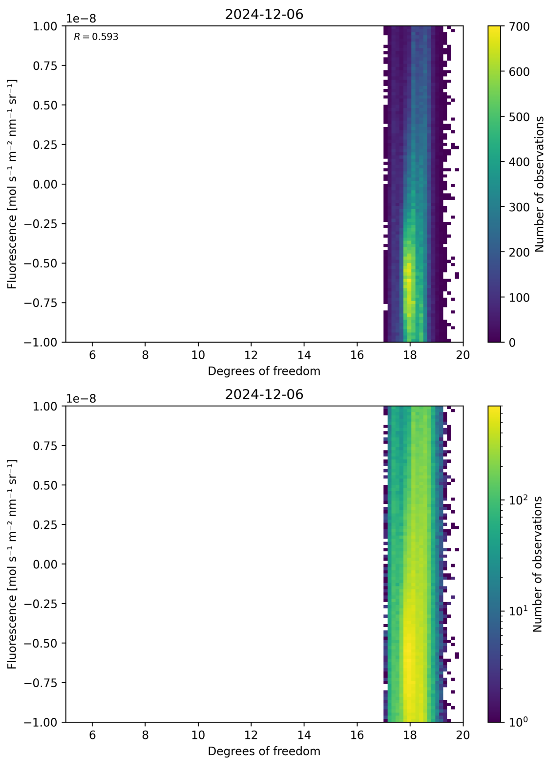
Figure 51: Scatter density plot of “Degrees of freedom” against “Fluorescence” for 2024-12-06 to 2024-12-07.
