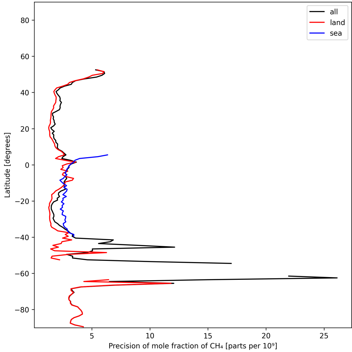
Figure 13: Zonal average of “Precision of mole fraction of CH 4 ” for 2024-12-06 to 2024-12-07.
