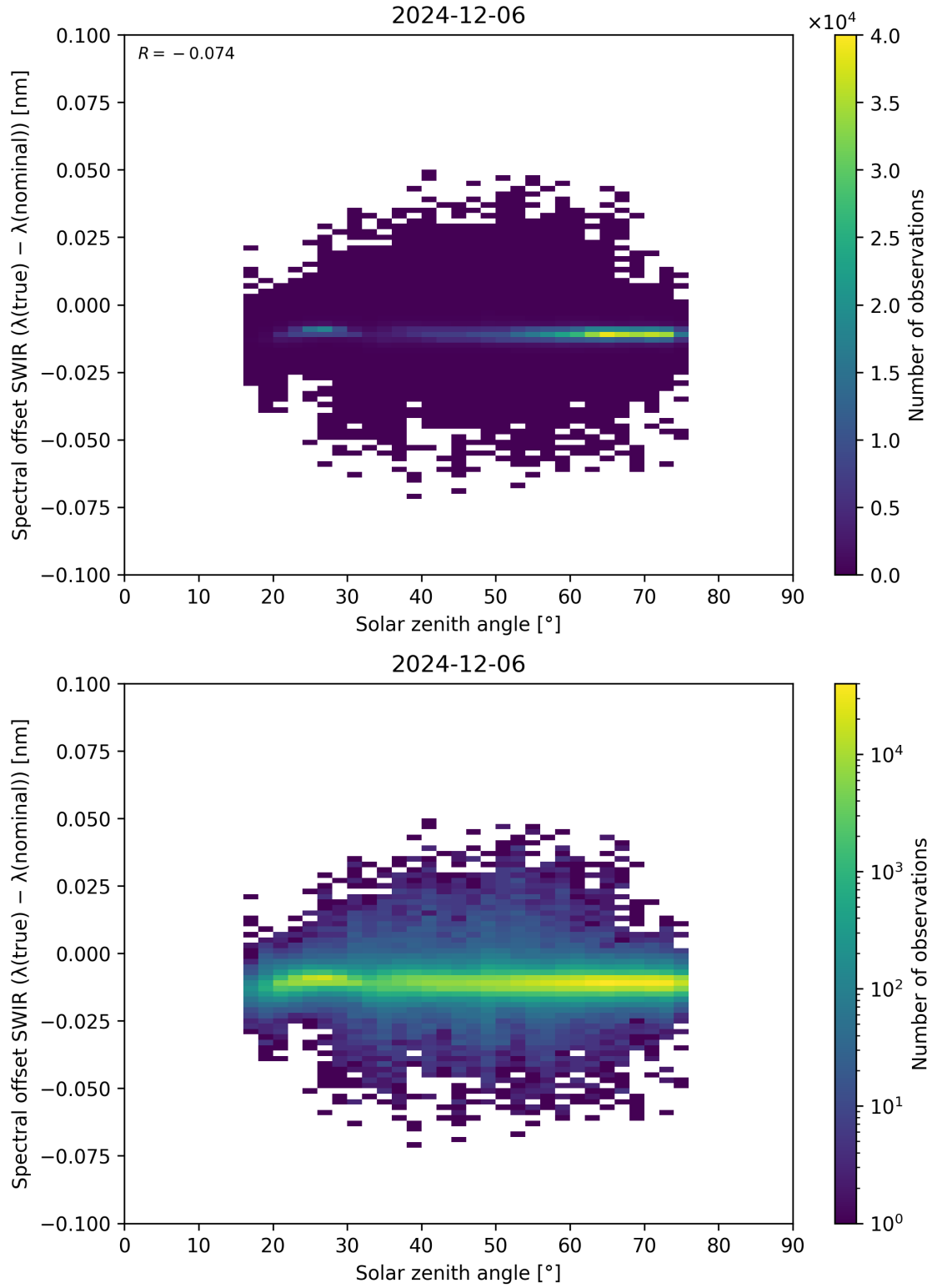
Figure 104: Scatter density plot of “Solar zenith angle” against “Spectral offset SWIR ( \lambda_{\text{true}} - \lambda_{\text{nominal}} )” for 2024-12-06 to 2024-12-07.
