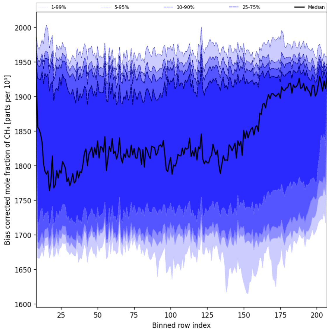
Figure 36: Along track statistics of “Bias corrected mole fraction of CH 4 ” for 2024-12-06 to 2024-12-07
