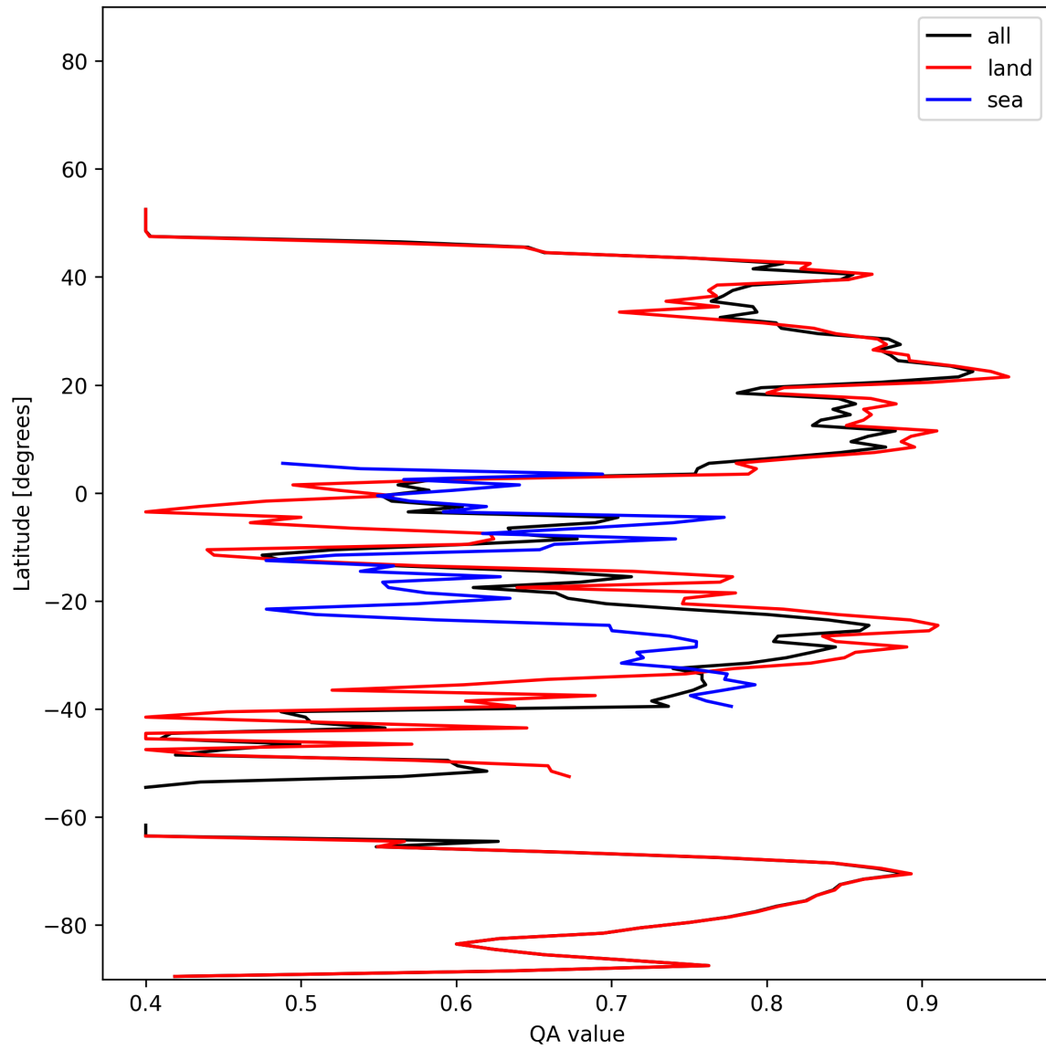
Figure 11: Zonal average of “QA value” for 2024-12-06 to 2024-12-07.
