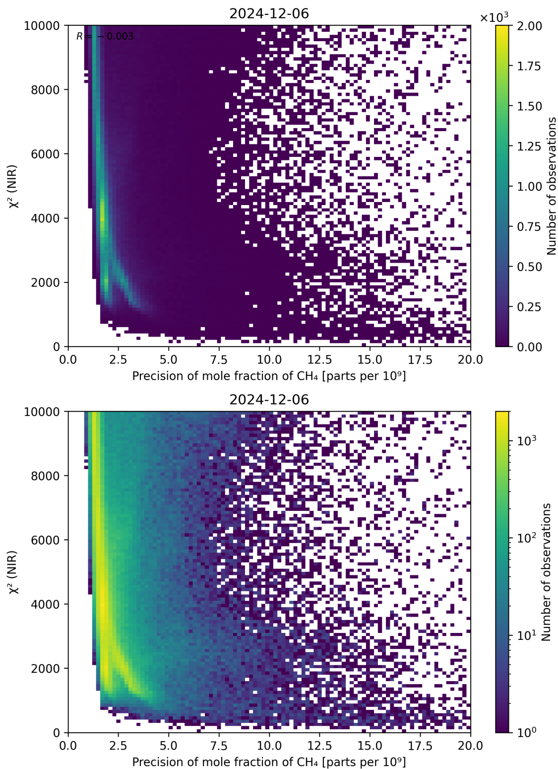
Figure 78: Scatter density plot of “Precision of mole fraction of CH 4 ” against “ \chi^2 (NIR)” for 2024-12-06 to 2024-12-07.
