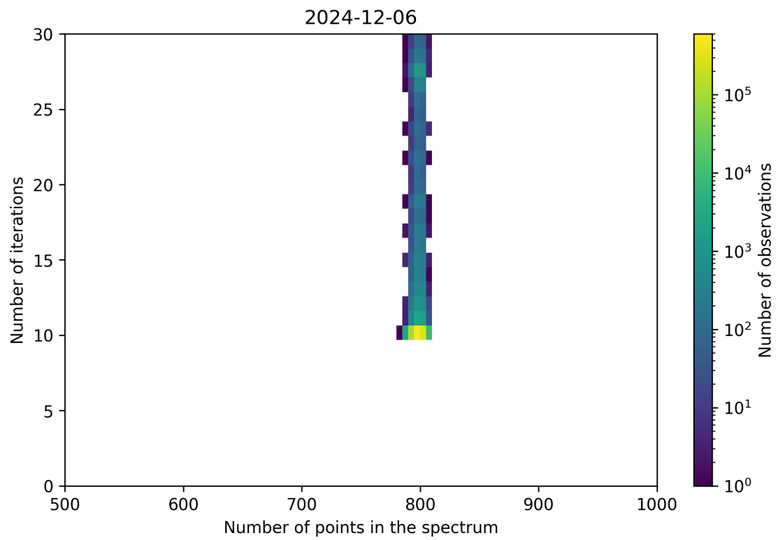
Figure 92: Scatter density plot of “Number of points in the spectrum” against “Number of iterations” for 2024-12-06 to 2024-12-07.
