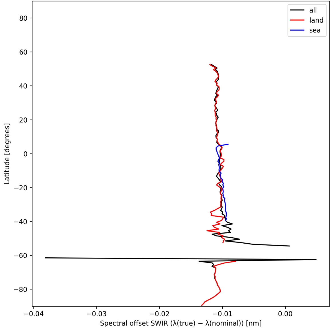
Figure 16: Zonal average of “Spectral offset SWIR ( \lambda_{\text{true}} - \lambda_{\text{nominal}} )” for 2024-12-06 to 2024-12-07.
