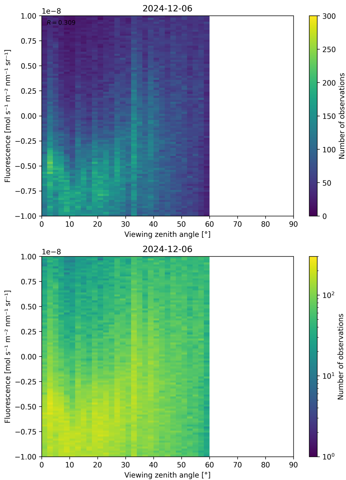
Figure 108: Scatter density plot of “Viewing zenith angle” against “Fluorescence” for 2024-12-06 to 2024-12-07.
