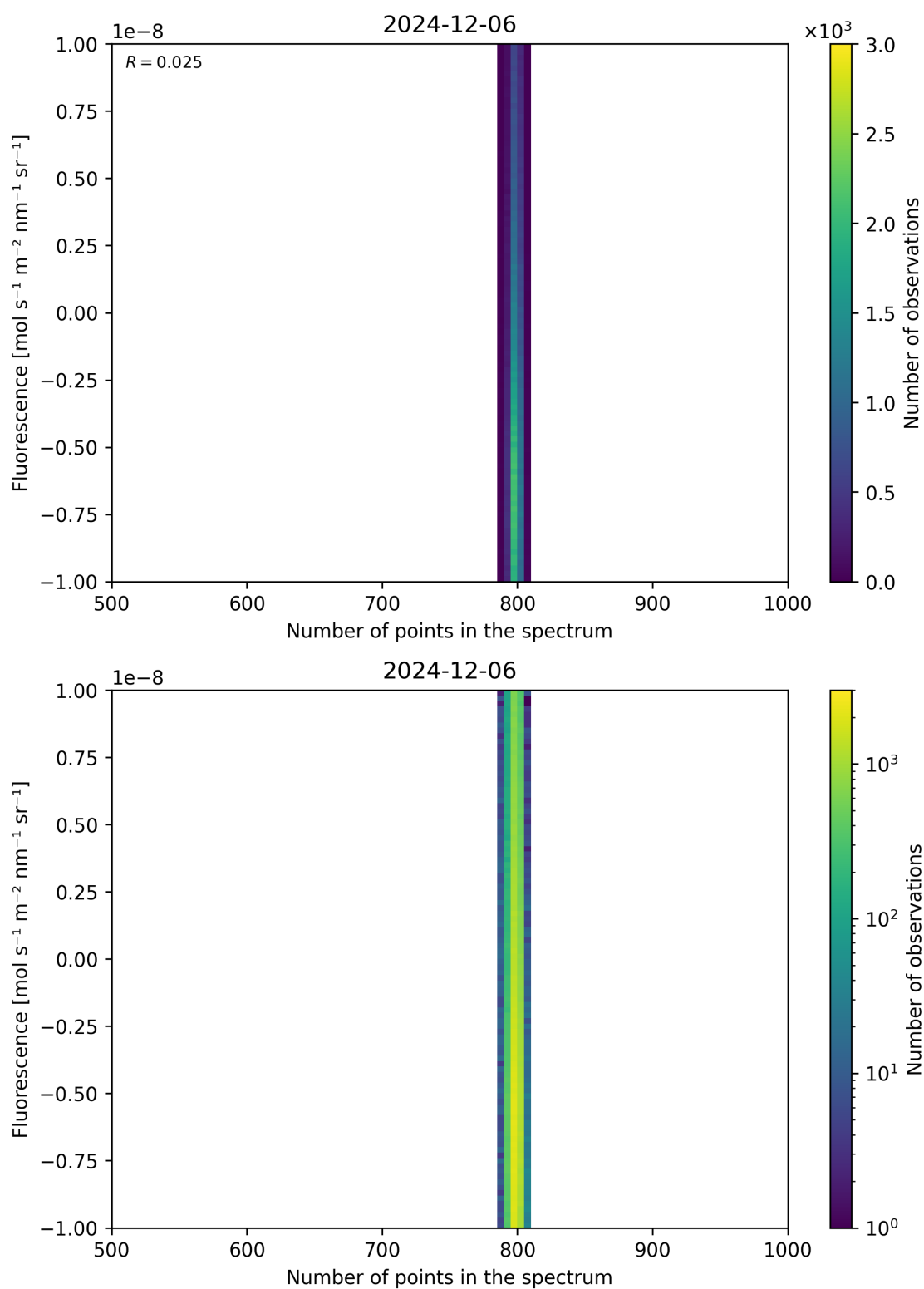
Figure 91: Scatter density plot of “Number of points in the spectrum” against “Fluorescence” for 2024-12-06 to 2024-12-07.
