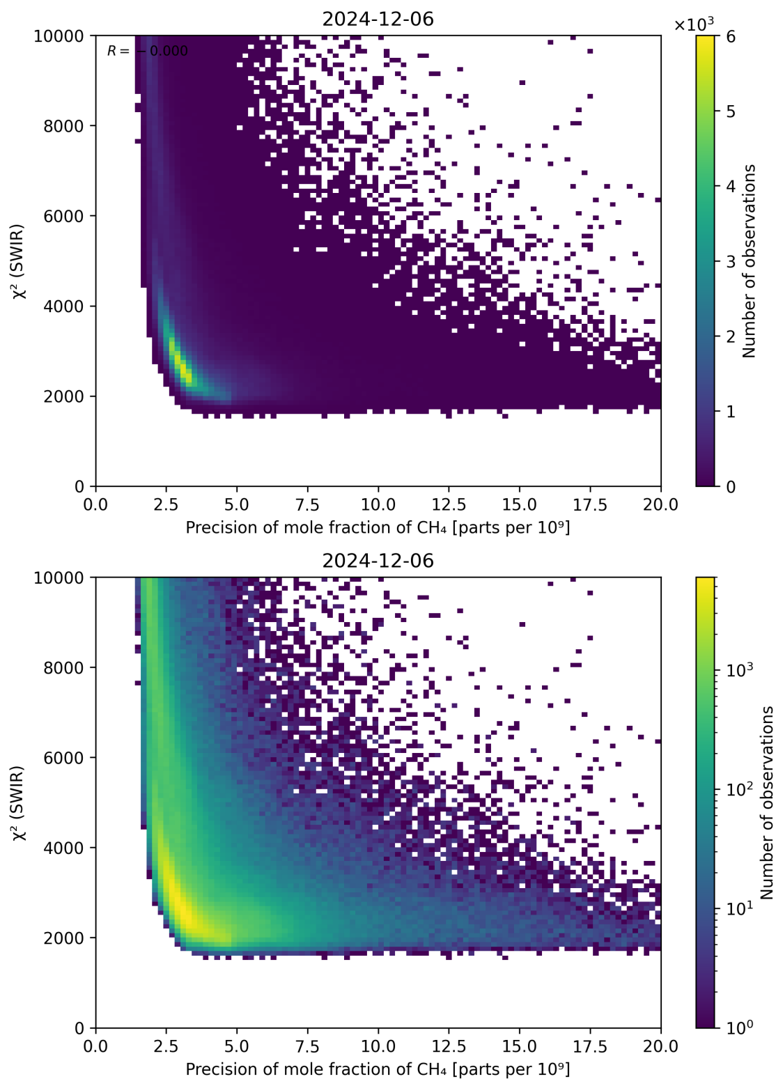
Figure 79: Scatter density plot of “Precision of mole fraction of CH 4 ” against “ \chi^2 (SWIR)” for 2024-12-06 to 2024-12-07.
