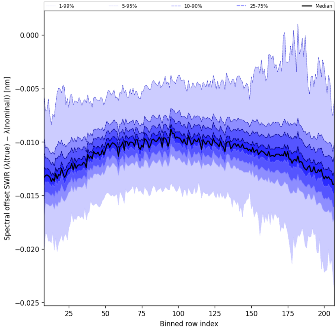
Figure 38: Along track statistics of “Spectral offset SWIR ( \lambda_{\text{true}} - \lambda_{\text{nominal}} )” for 2024-12-06 to 2024-12-07
