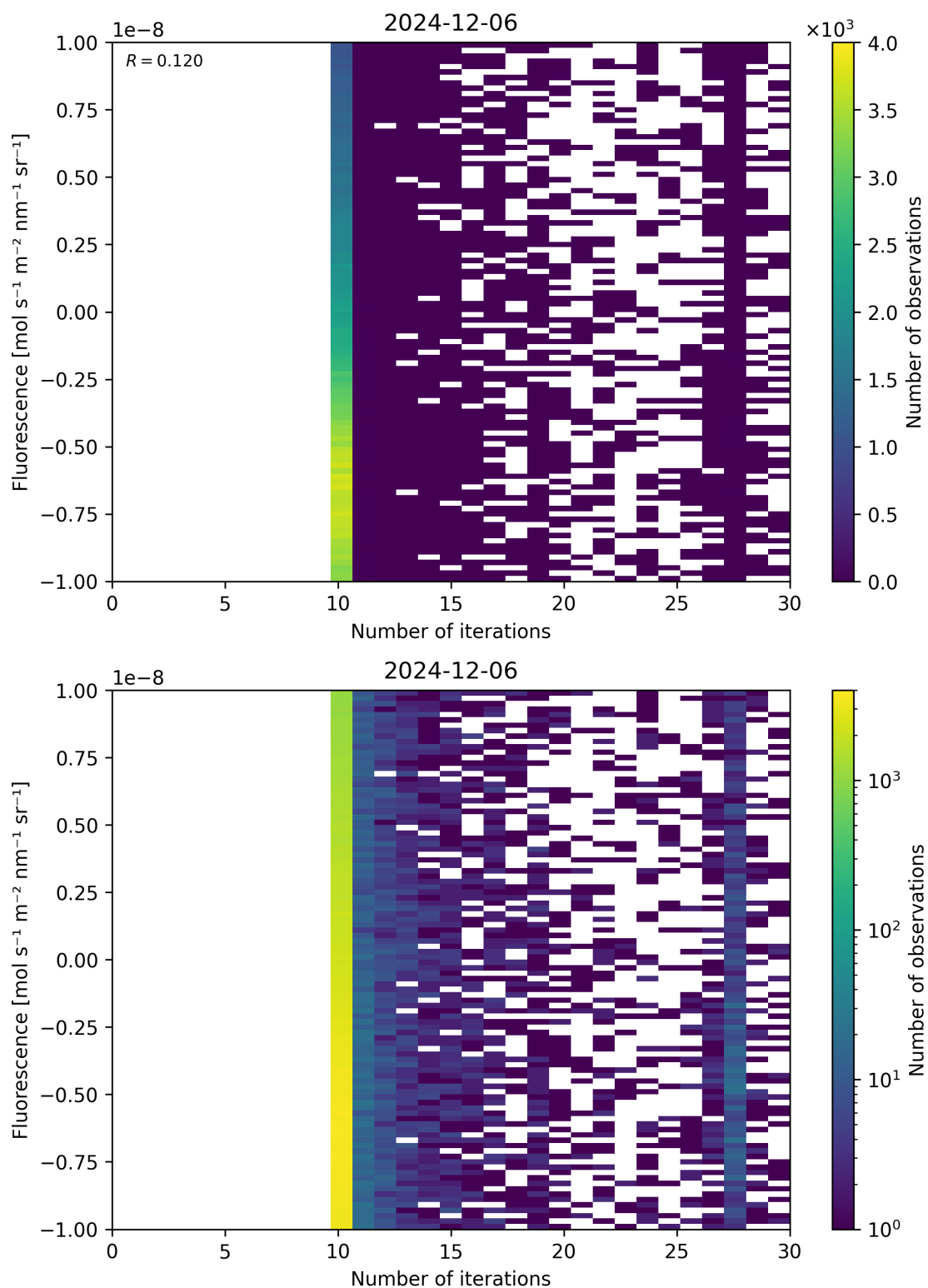
Figure 87: Scatter density plot of “Number of iterations” against “Fluorescence” for 2024-12-06 to 2024-12-07.
