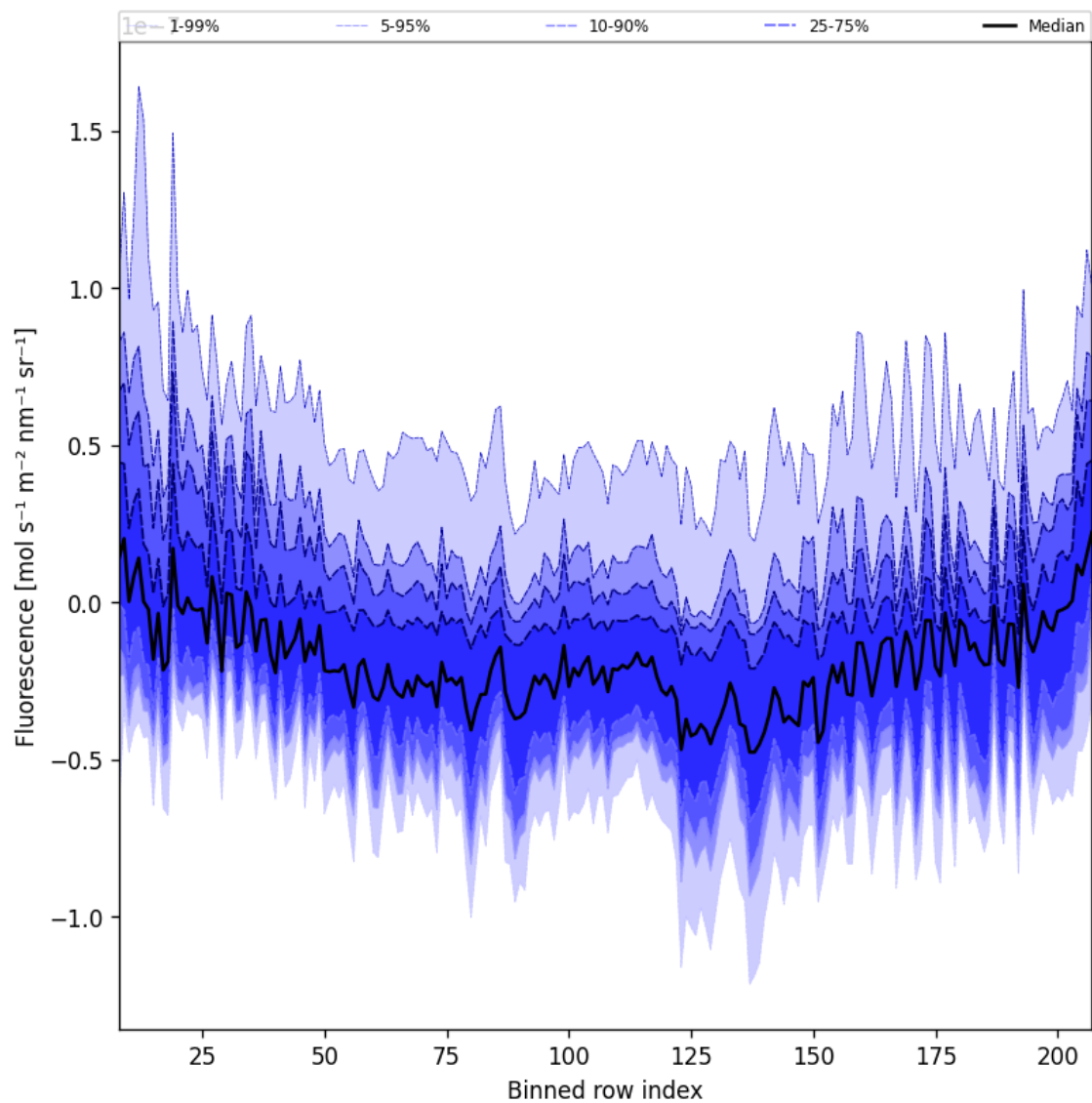
Figure 43: Along track statistics of “Fluorescence” for 2024-12-06 to 2024-12-07
