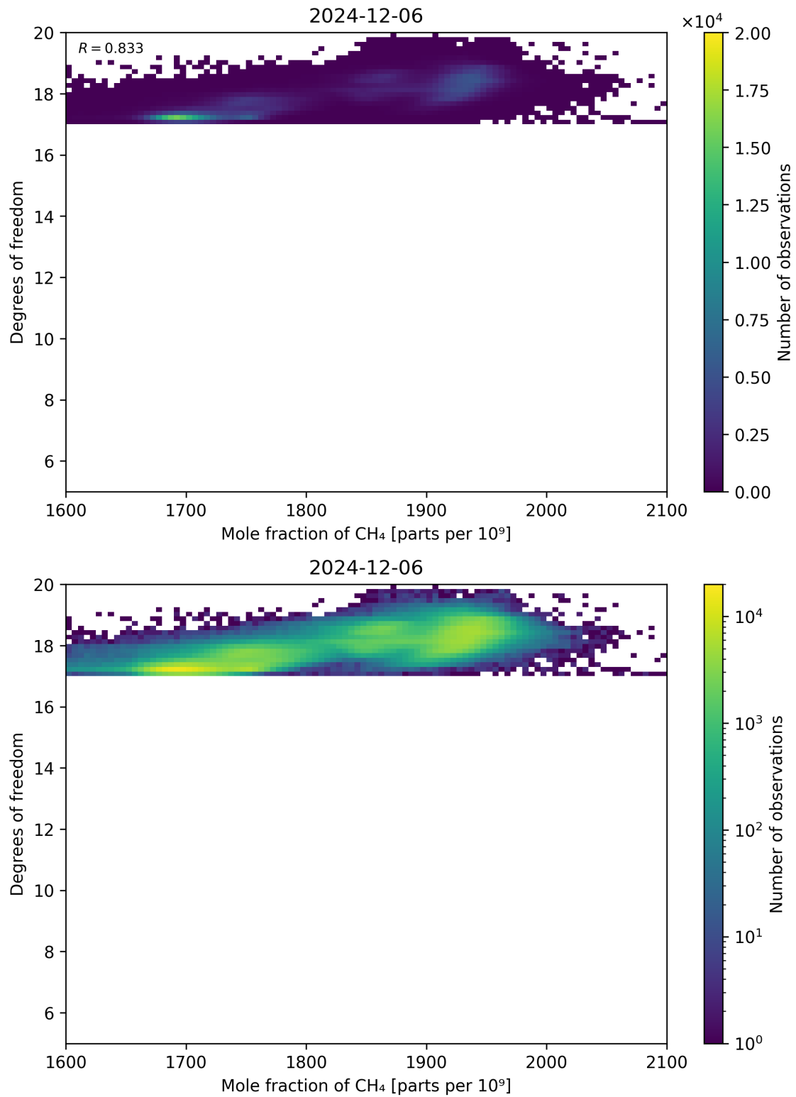
Figure 72: Scatter density plot of “Mole fraction of CH 4 ” against “Degrees of freedom” for 2024-12-06 to 2024-12-07.
