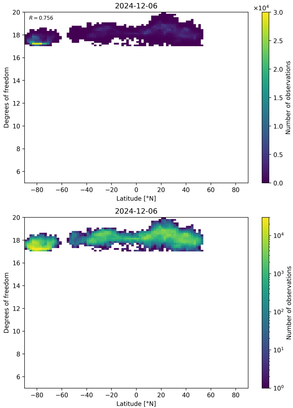
Figure 55: Scatter density plot of “Latitude” against “Degrees of freedom” for 2024-12-06 to 2024-12-07.
