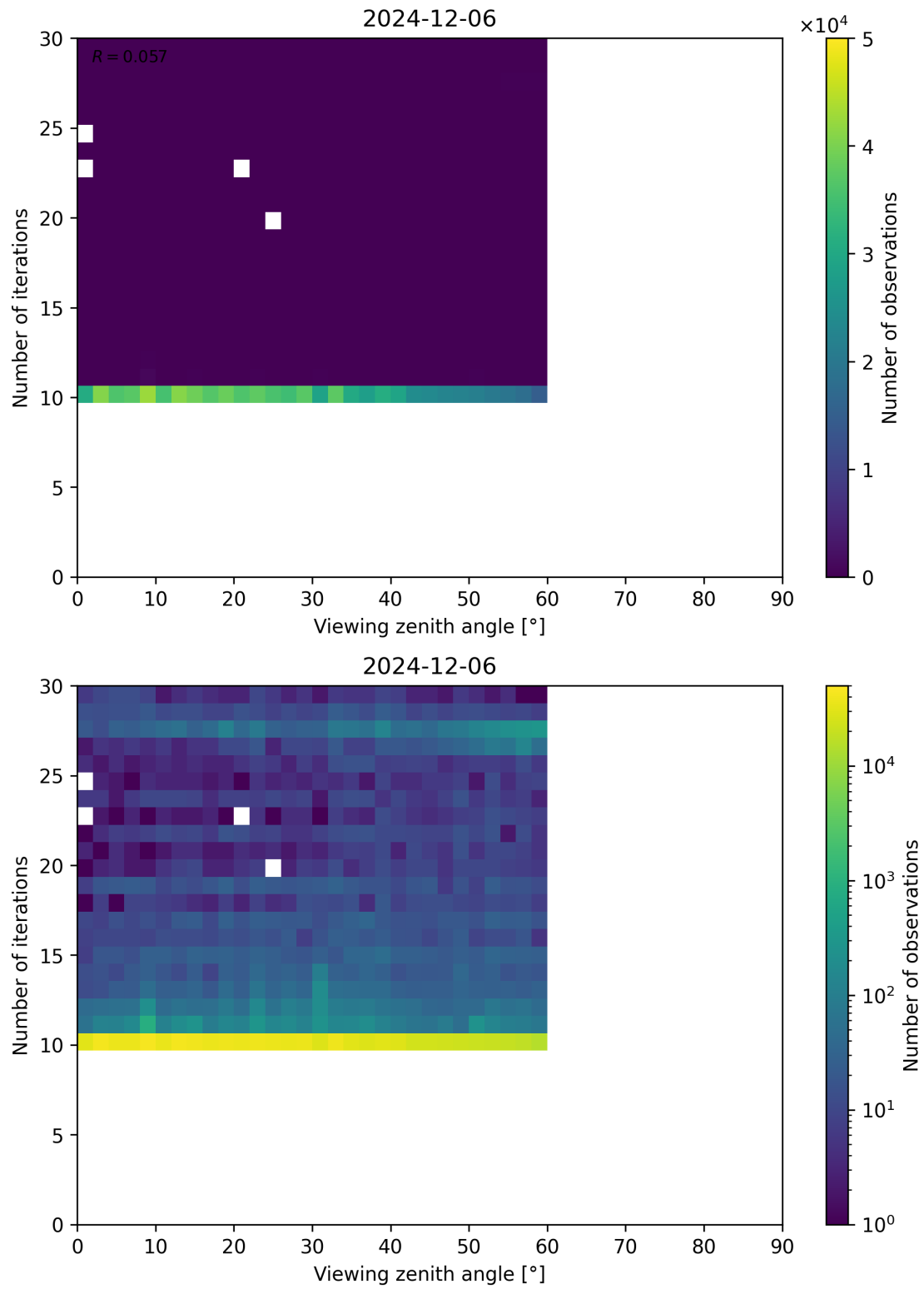
Figure 113: Scatter density plot of “Viewing zenith angle” against “Number of iterations” for 2024-12-06 to 2024-12-07.
