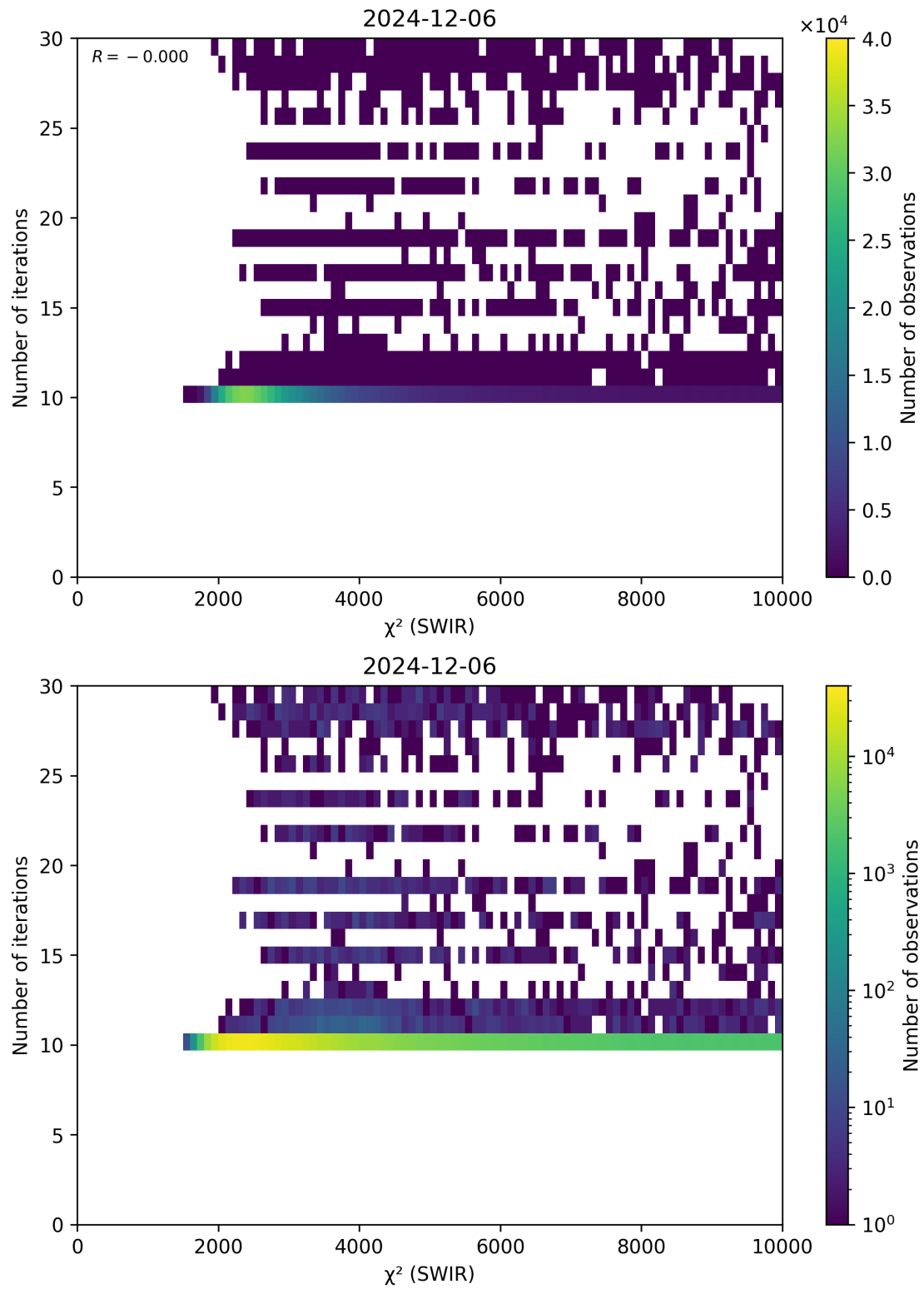
Figure 50: Scatter density plot of “ \chi^2 (SWIR)” against “Number of iterations” for 2024-12-06 to 2024-12-07.
