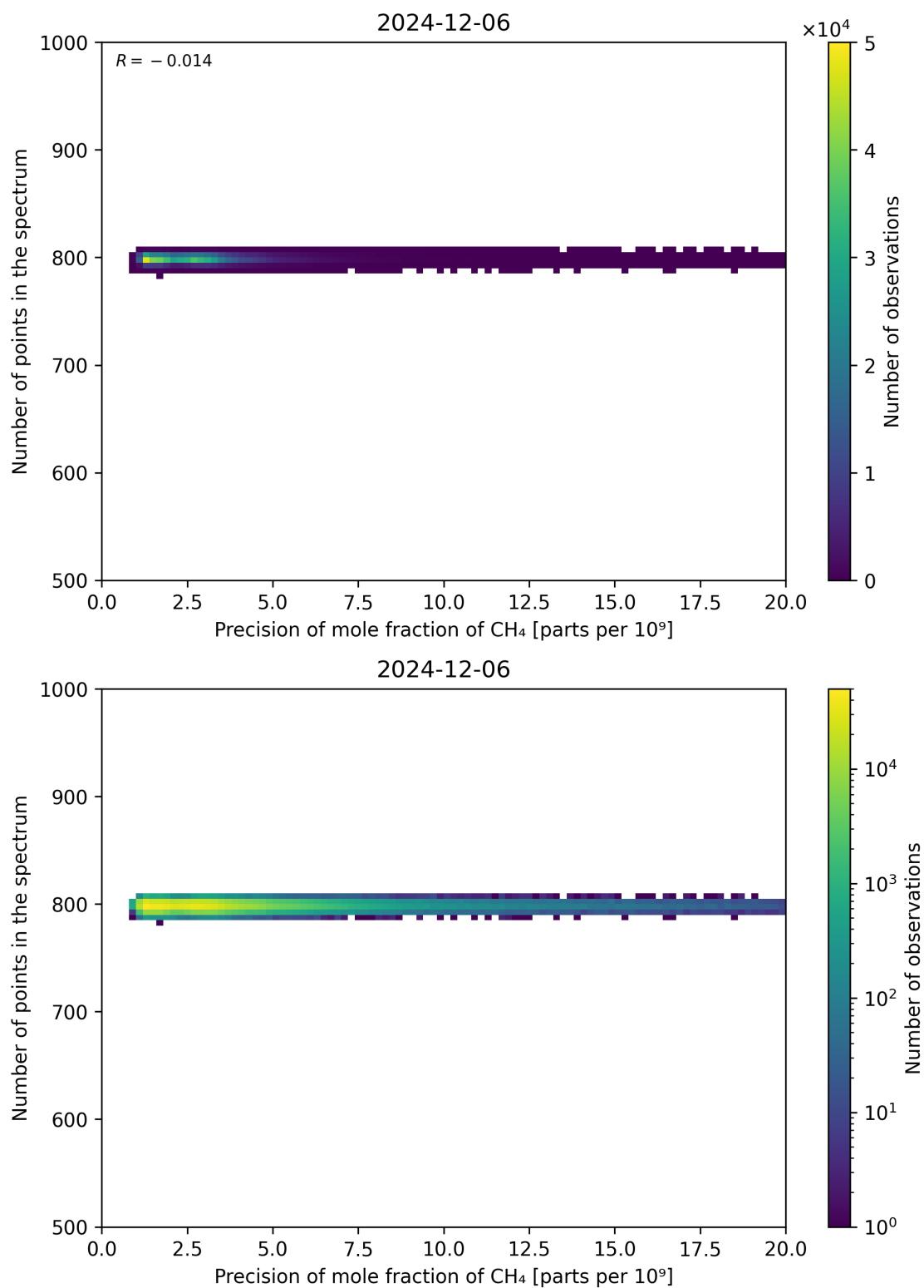
Figure 84: Scatter density plot of “Precision of mole fraction of CH 4 ” against “Number of points in the spectrum” for 2024-12-06 to 2024-12-07.
