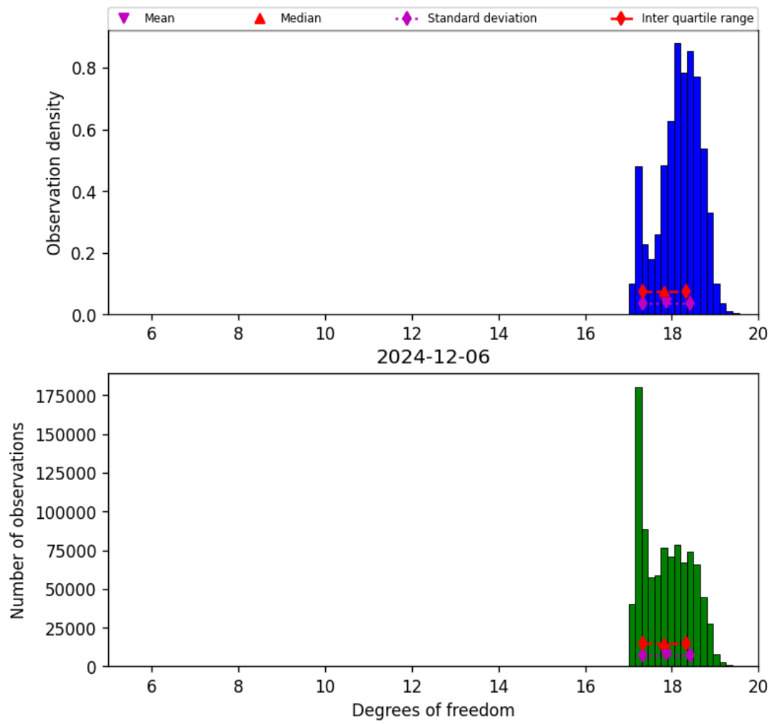
Figure 30: Histogram of “Degrees of freedom” for 2024-12-06 to 2024-12-07
