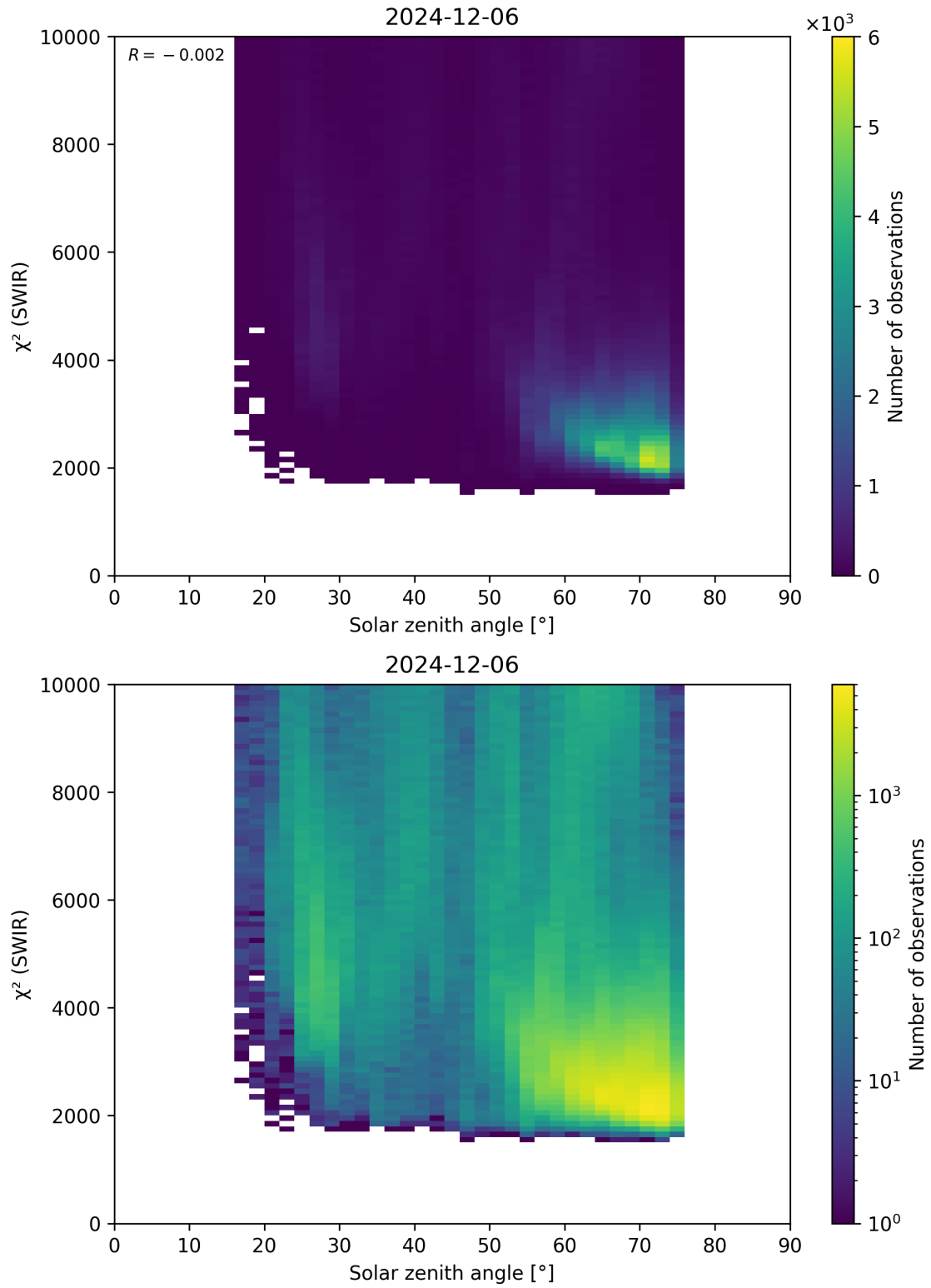
Figure 95: Scatter density plot of “Solar zenith angle” against “ \chi^2 (SWIR)” for 2024-12-06 to 2024-12-07.
