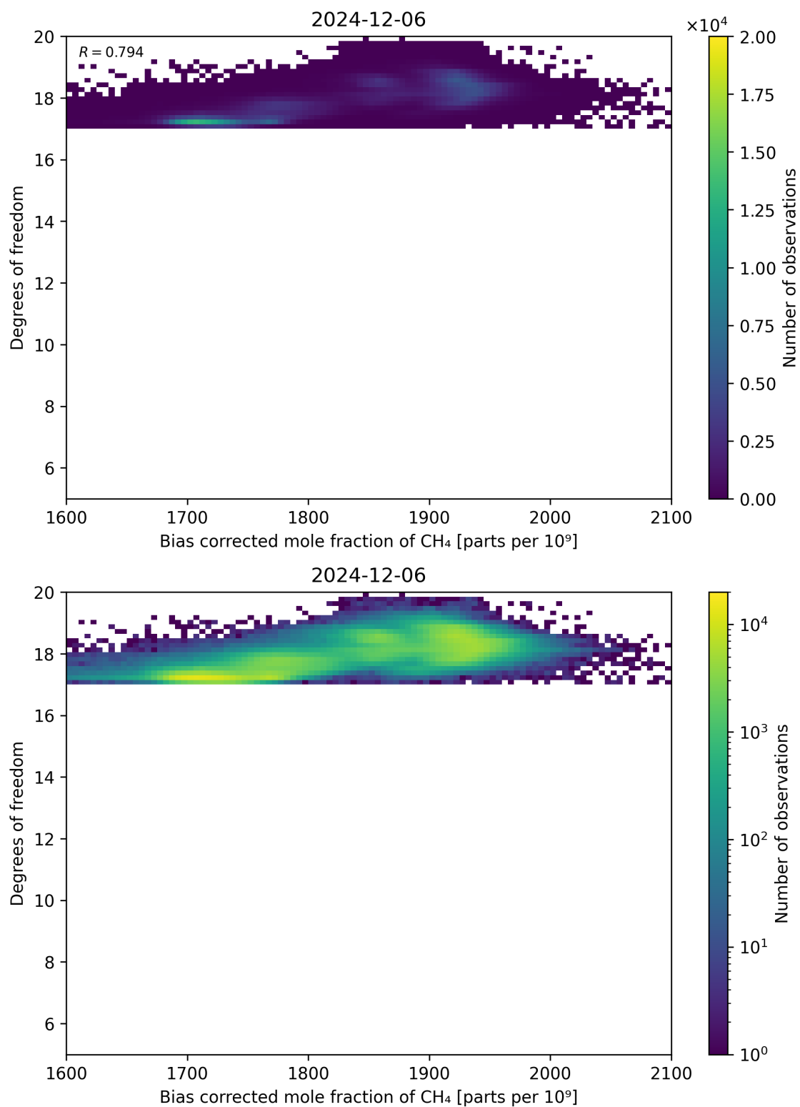
Figure 65: Scatter density plot of “Bias corrected mole fraction of CH 4 ” against “Degrees of freedom” for 2024-12-06 to 2024-12-07.
