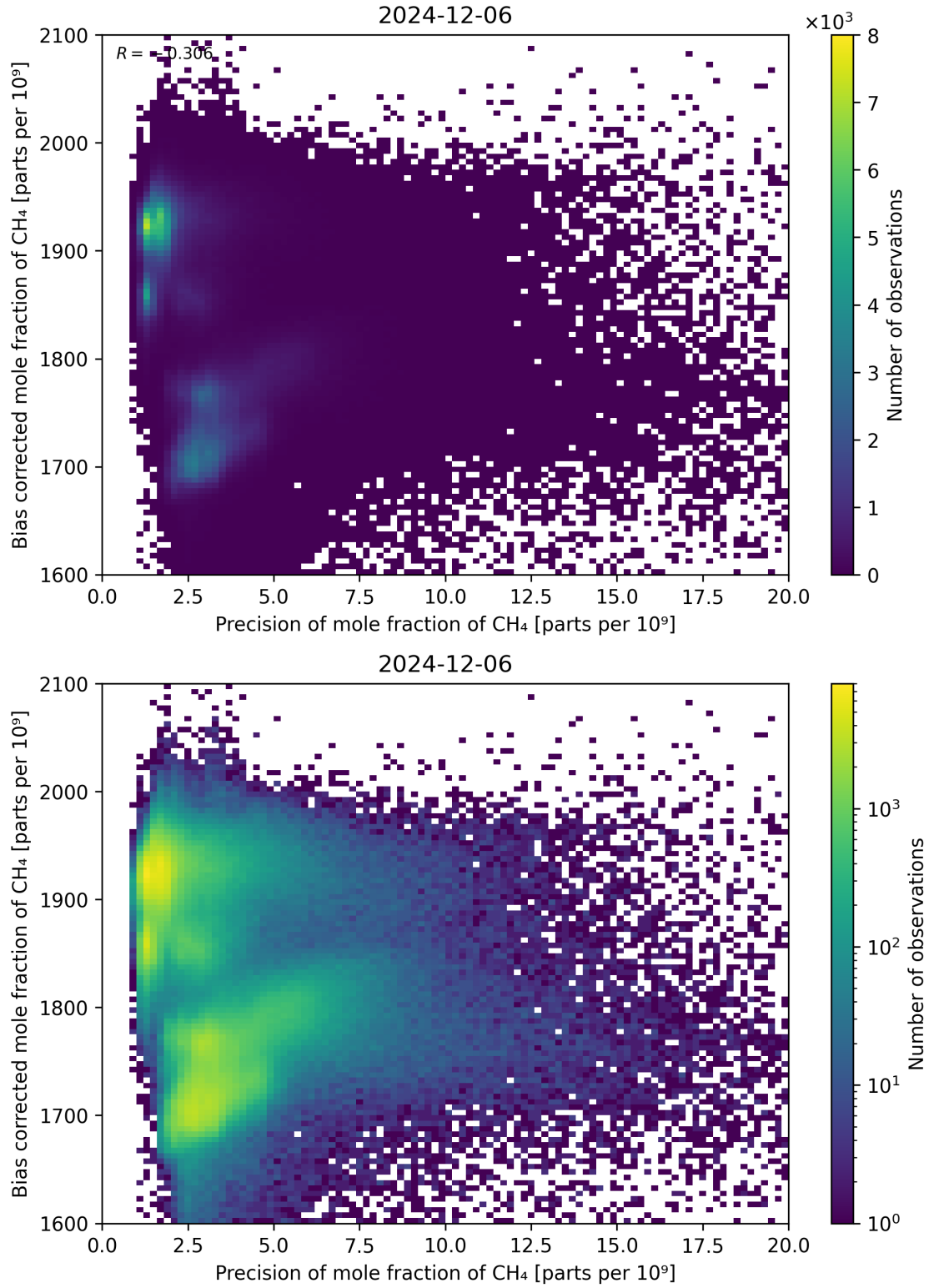
Figure 82: Scatter density plot of “Precision of mole fraction of CH 4 ” against “Bias corrected mole fraction of CH 4 ” for 2024-12-06 to 2024-12-07.
