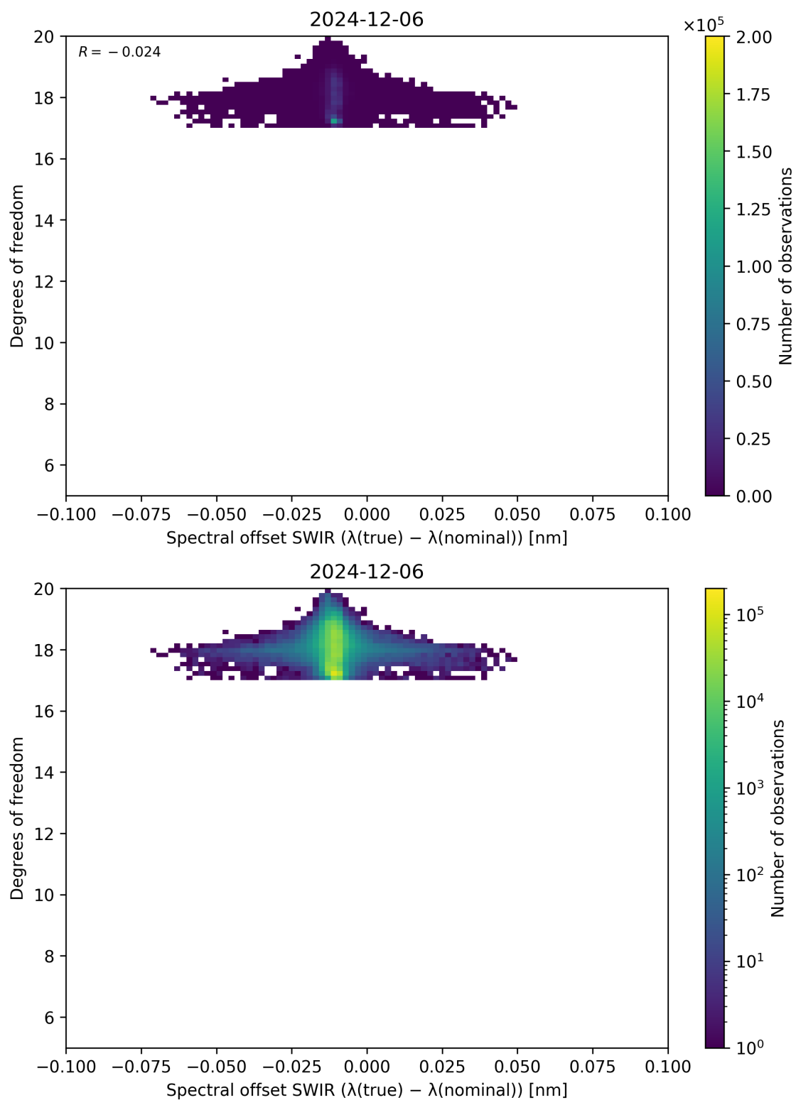
Figure 119: Scatter density plot of “Spectral offset SWIR ( \lambda_{\text{true}} - \lambda_{\text{nominal}} )” against “Degrees of freedom” for 2024-12-06 to 2024-12-07.
