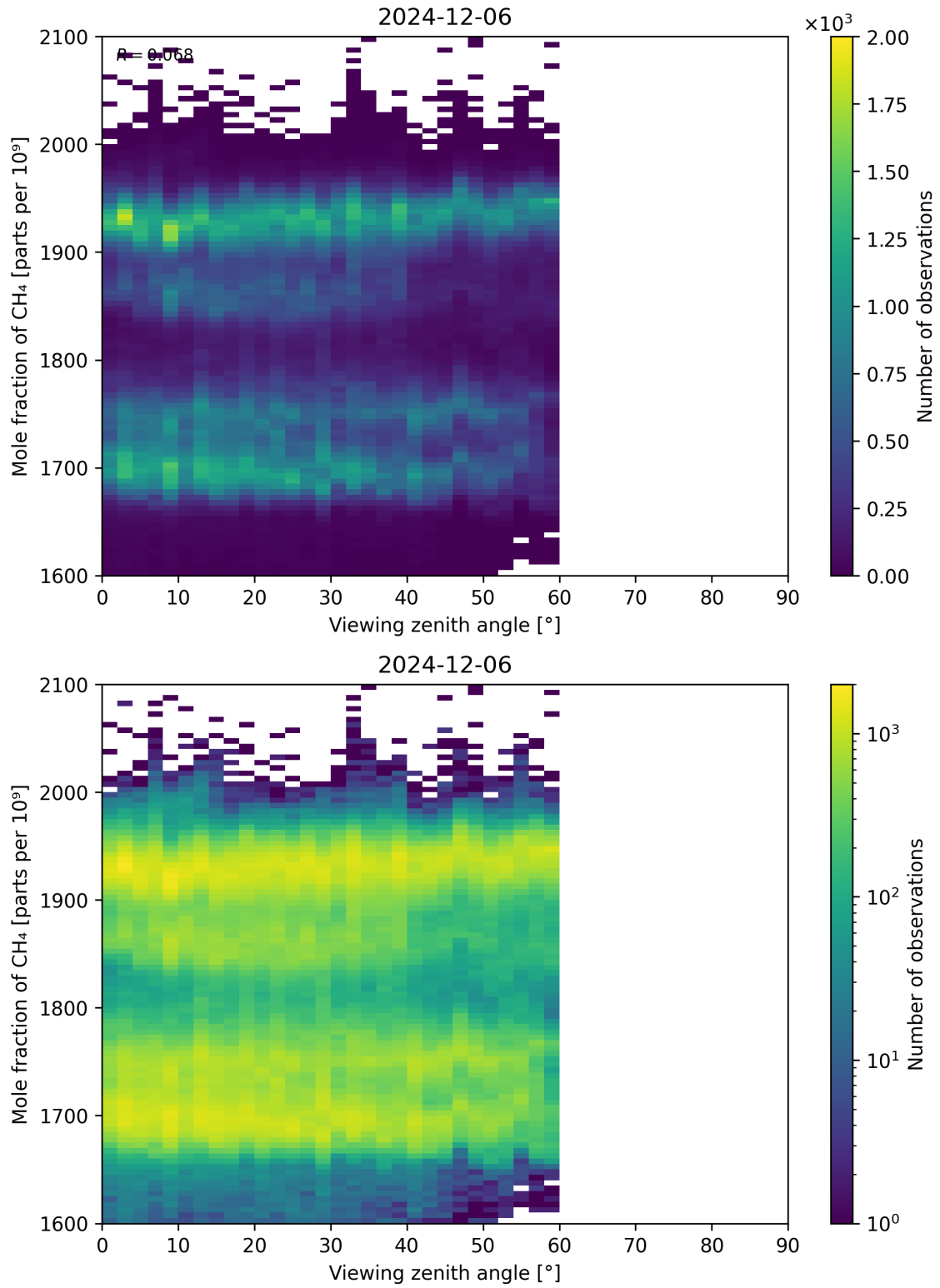
Figure 110: Scatter density plot of “Viewing zenith angle” against “Mole fraction of CH 4 ” for 2024-12-06 to 2024-12-07.
