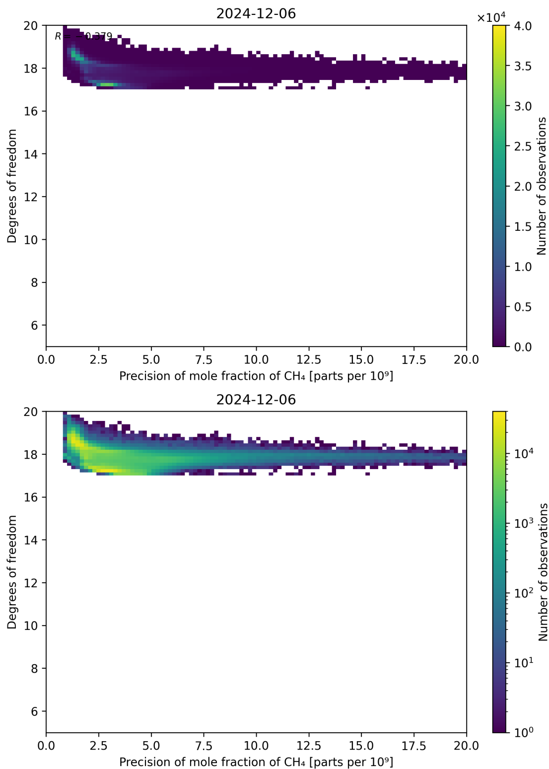
Figure 80: Scatter density plot of “Precision of mole fraction of CH 4 ” against “Degrees of freedom” for 2024-12-06 to 2024-12-07.
