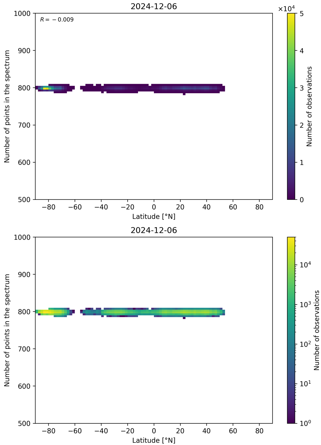
Figure 61: Scatter density plot of “Latitude” against “Number of points in the spectrum” for 2024-12-06 to 2024-12-07.
