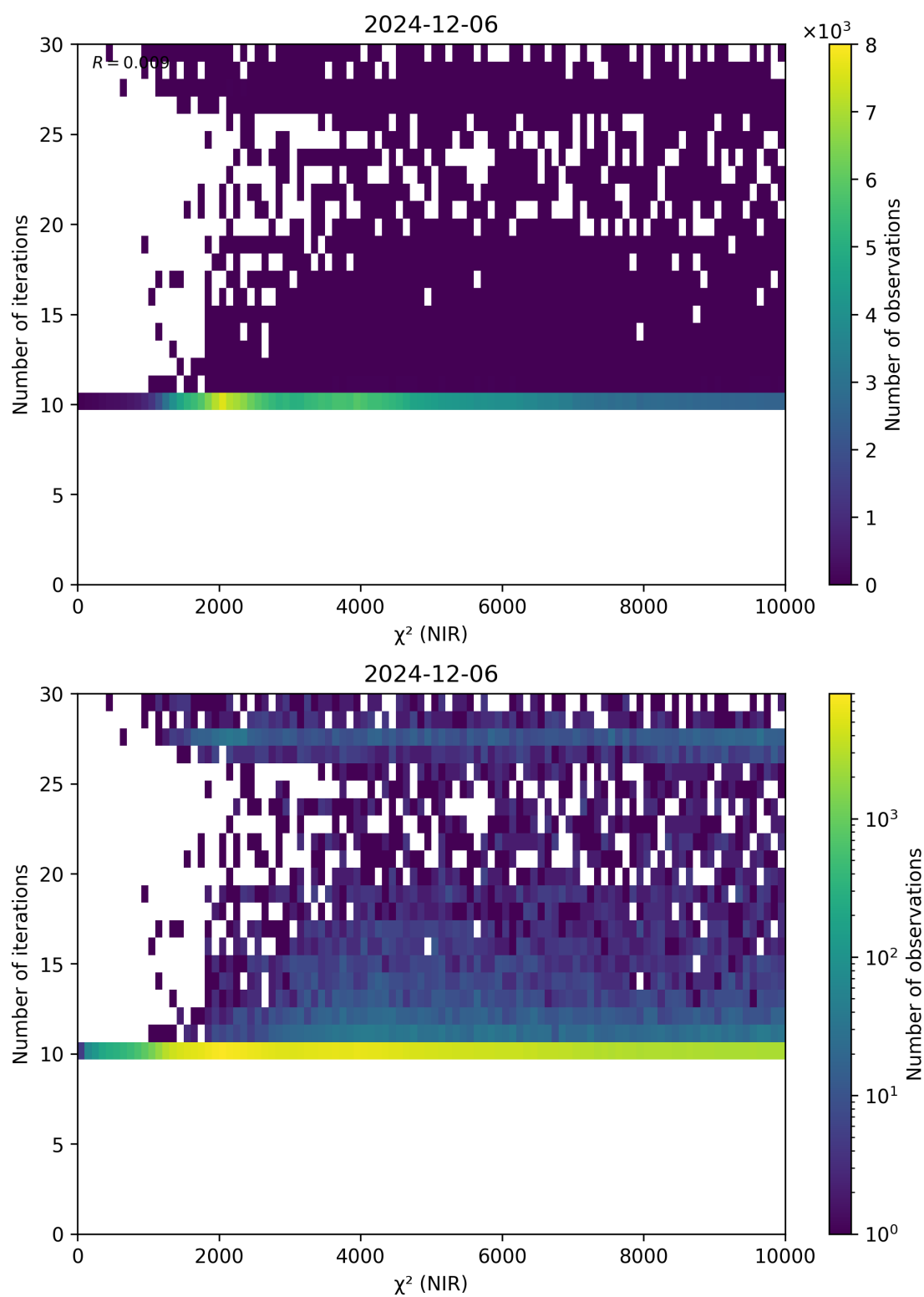
Figure 46: Scatter density plot of “ \chi^2 (NIR)” against “Number of iterations” for 2024-12-06 to 2024-12-07.
