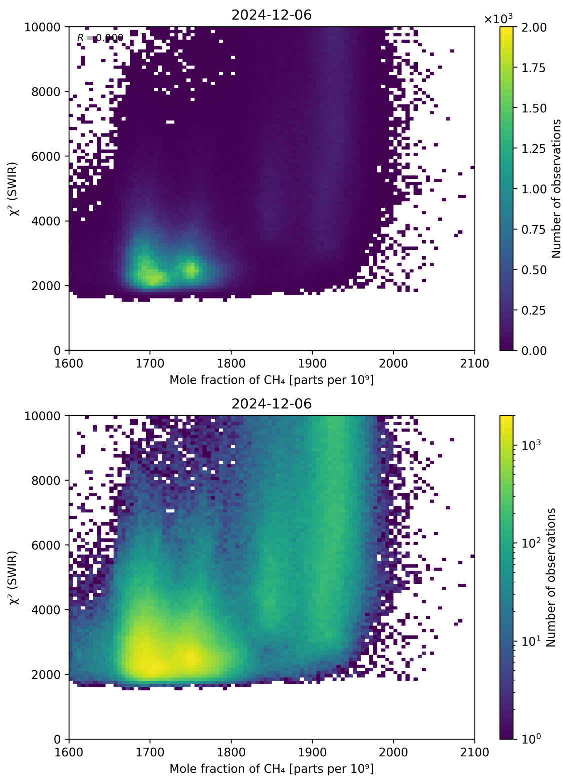
Figure 71: Scatter density plot of “Mole fraction of CH 4 ” against “ \chi^2 (SWIR)” for 2024-12-06 to 2024-12-07.
