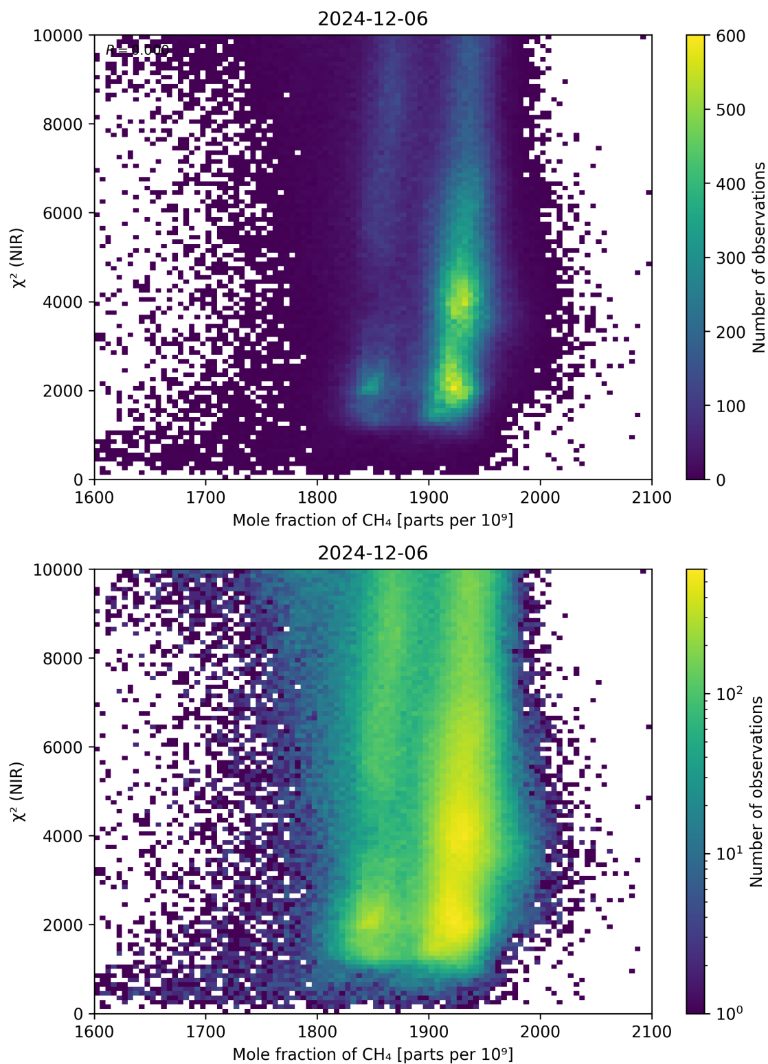
Figure 70: Scatter density plot of “Mole fraction of \text{CH}_4 ” against “ \chi^2 (NIR)” for 2024-12-06 to 2024-12-07.
