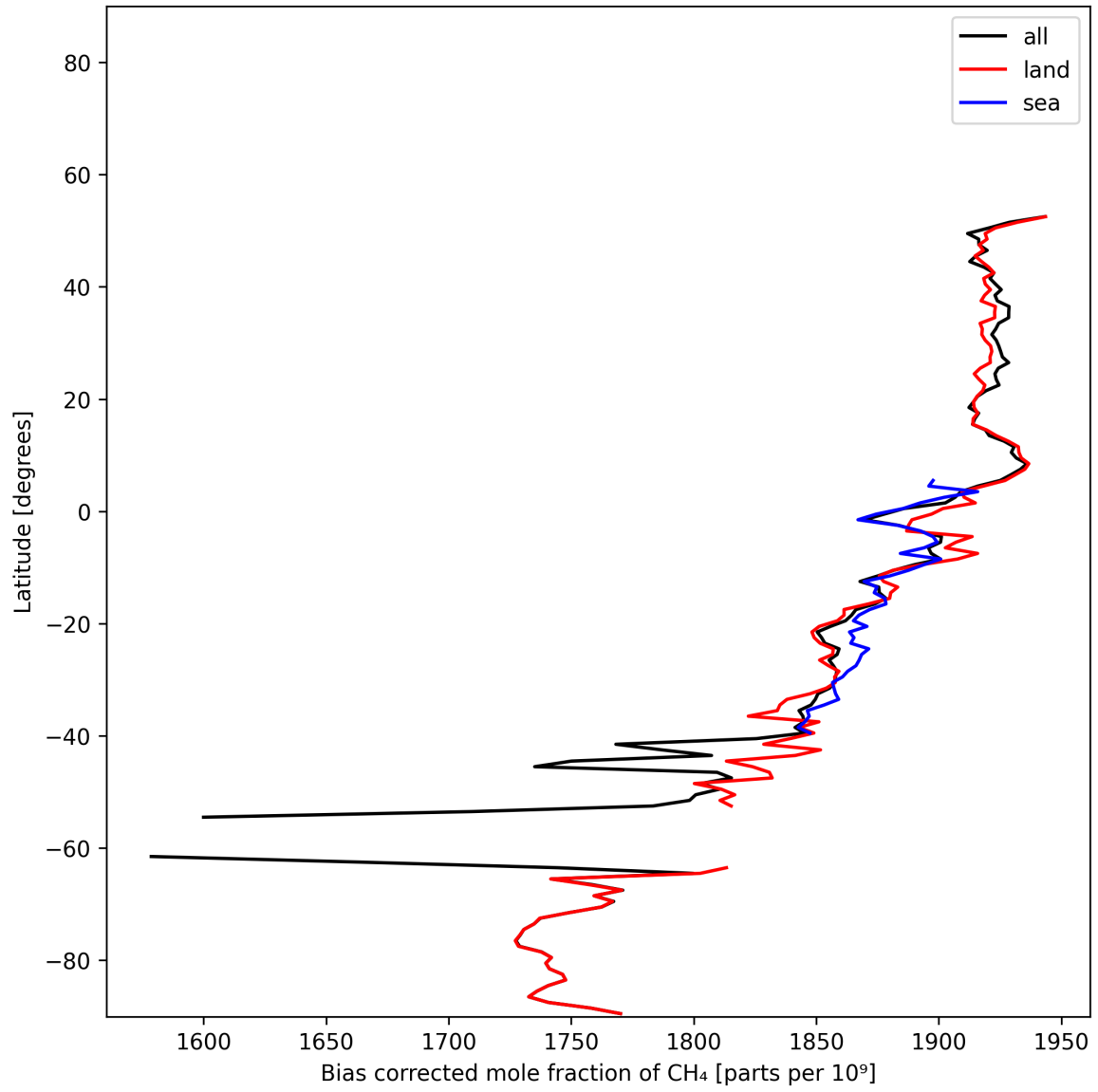
Figure 14: Zonal average of “Bias corrected mole fraction of CH 4 ” for 2024-12-06 to 2024-12-07.
