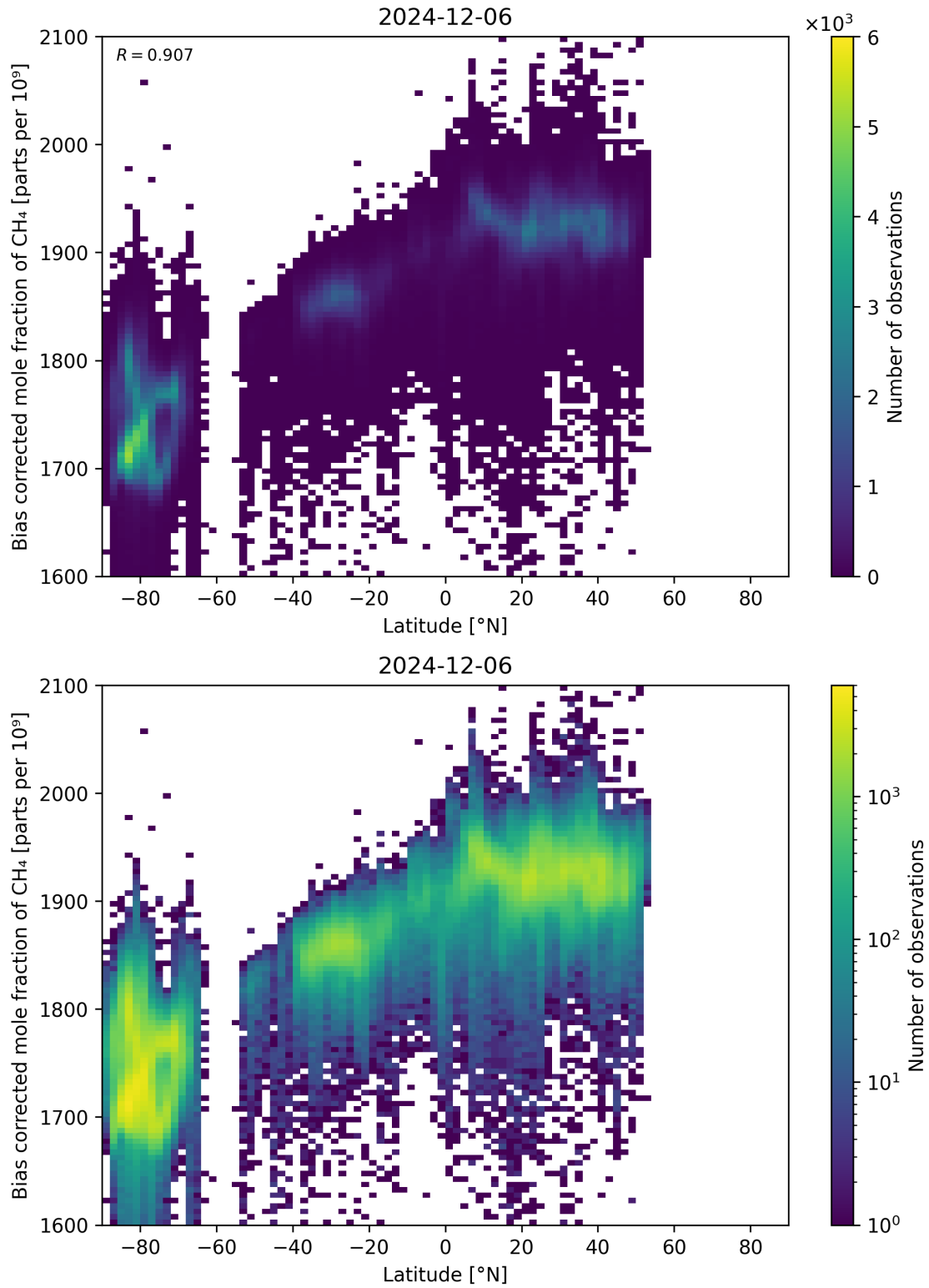
Figure 58: Scatter density plot of “Latitude” against “Bias corrected mole fraction of CH 4 ” for 2024-12-06 to 2024-12-07.
