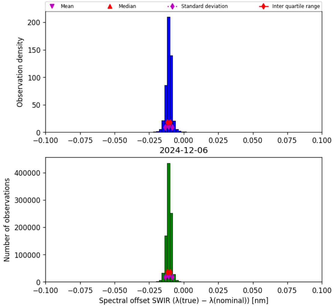
Figure 27: Histogram of “Spectral offset SWIR ( \lambda_{\text{true}} - \lambda_{\text{nominal}} )” for 2024-12-06 to 2024-12-07
