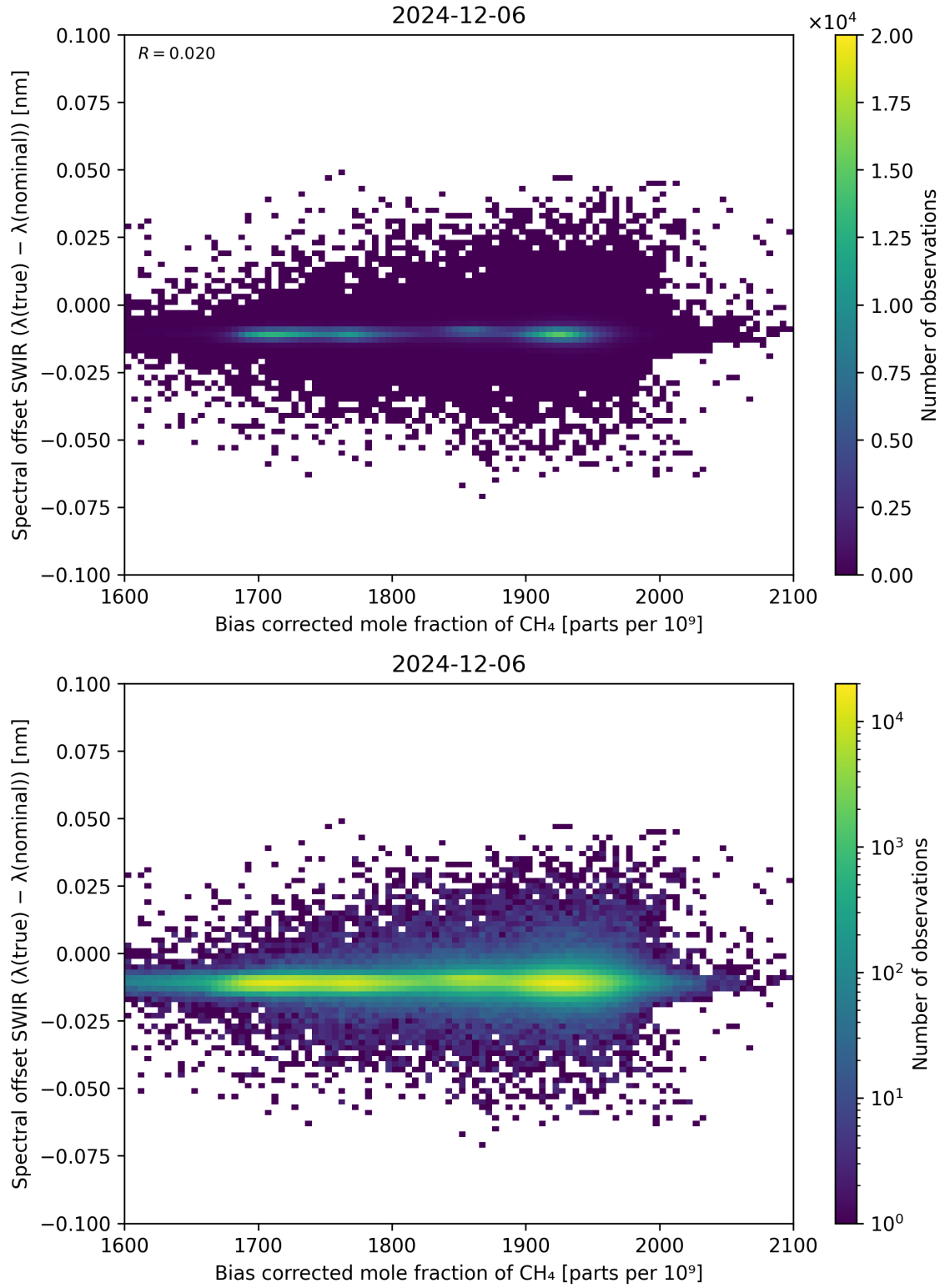
Figure 69: Scatter density plot of “Bias corrected mole fraction of \text{CH}_4 ” against “Spectral offset SWIR ( \lambda_{\text{true}} - \lambda_{\text{nominal}} )” for 2024-12-06 to 2024-12-07.
