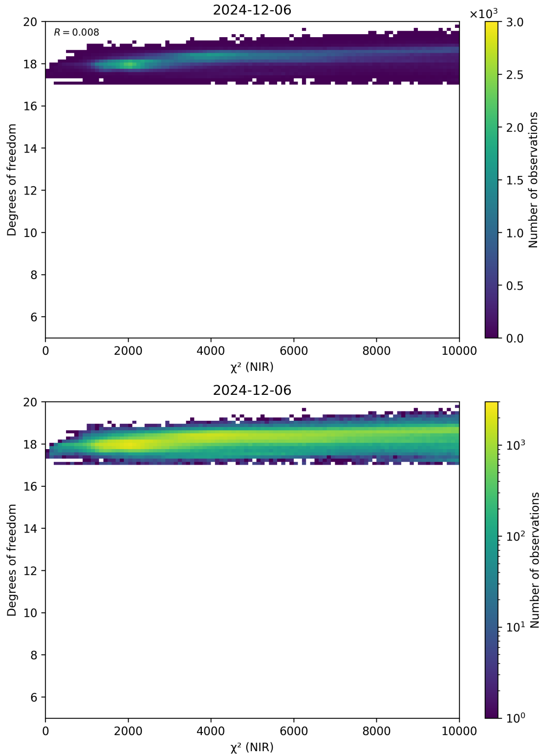
Figure 44: Scatter density plot of “ \chi^2 (NIR)” against “Degrees of freedom” for 2024-12-06 to 2024-12-07.
