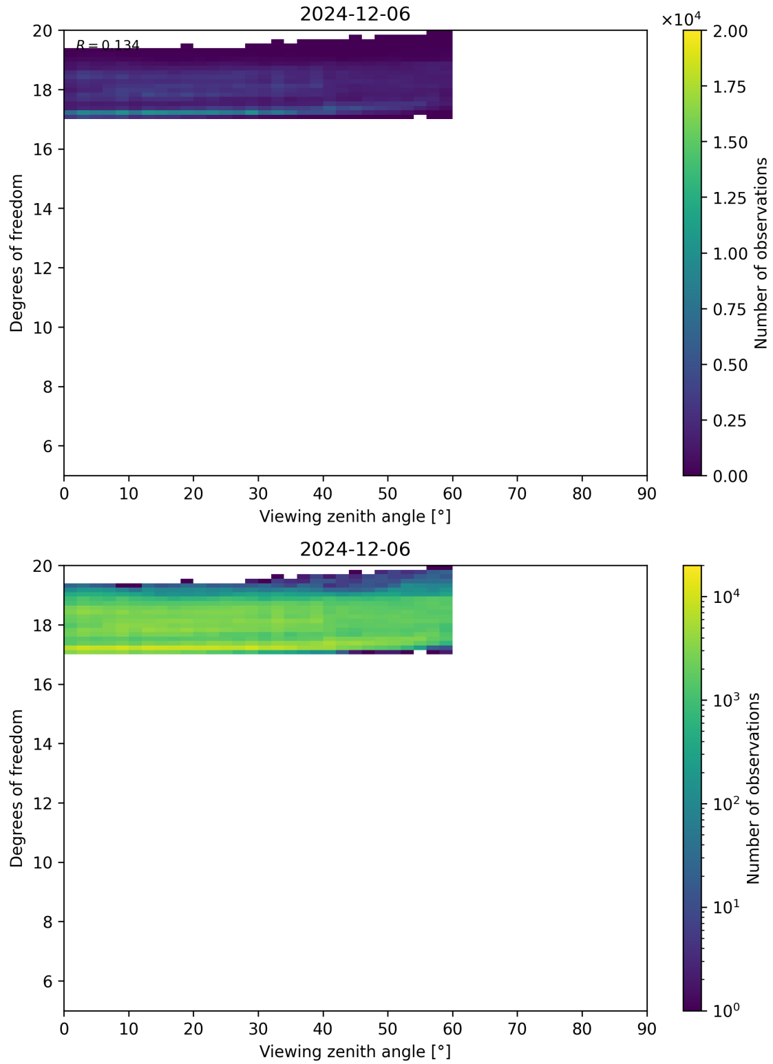
Figure 107: Scatter density plot of “Viewing zenith angle” against “Degrees of freedom” for 2024-12-06 to 2024-12-07.
