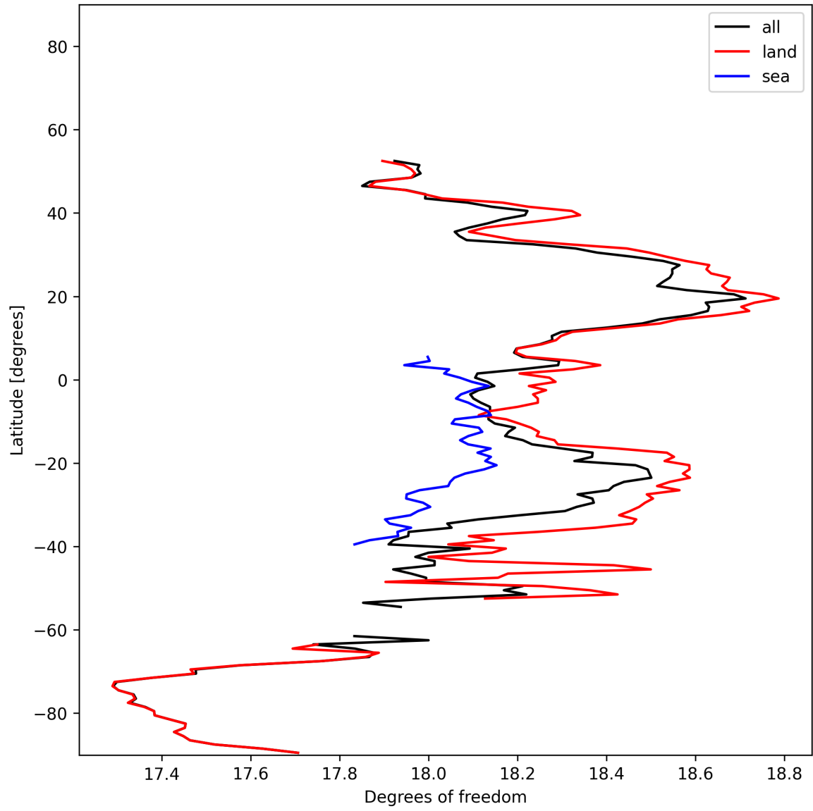
Figure 19: Zonal average of “Degrees of freedom” for 2024-12-06 to 2024-12-07.
