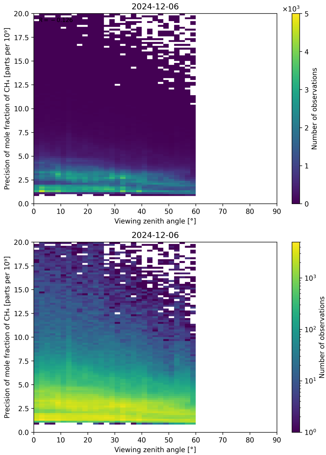
Figure 112: Scatter density plot of “Viewing zenith angle” against “Precision of mole fraction of \text{CH}_4 ” for 2024-12-06 to 2024-12-07.
