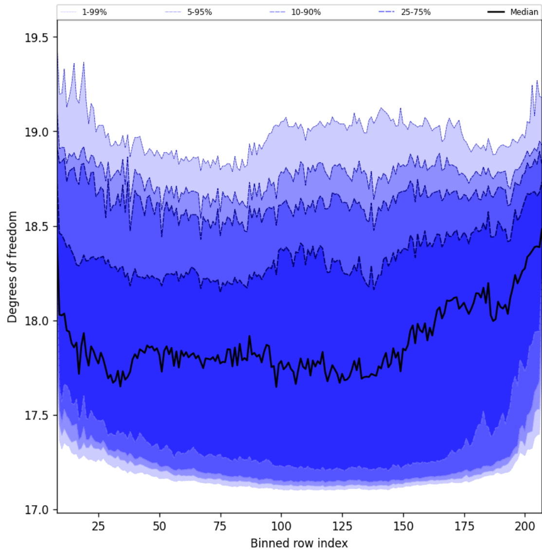
Figure 41: Along track statistics of “Degrees of freedom” for 2024-12-06 to 2024-12-07
