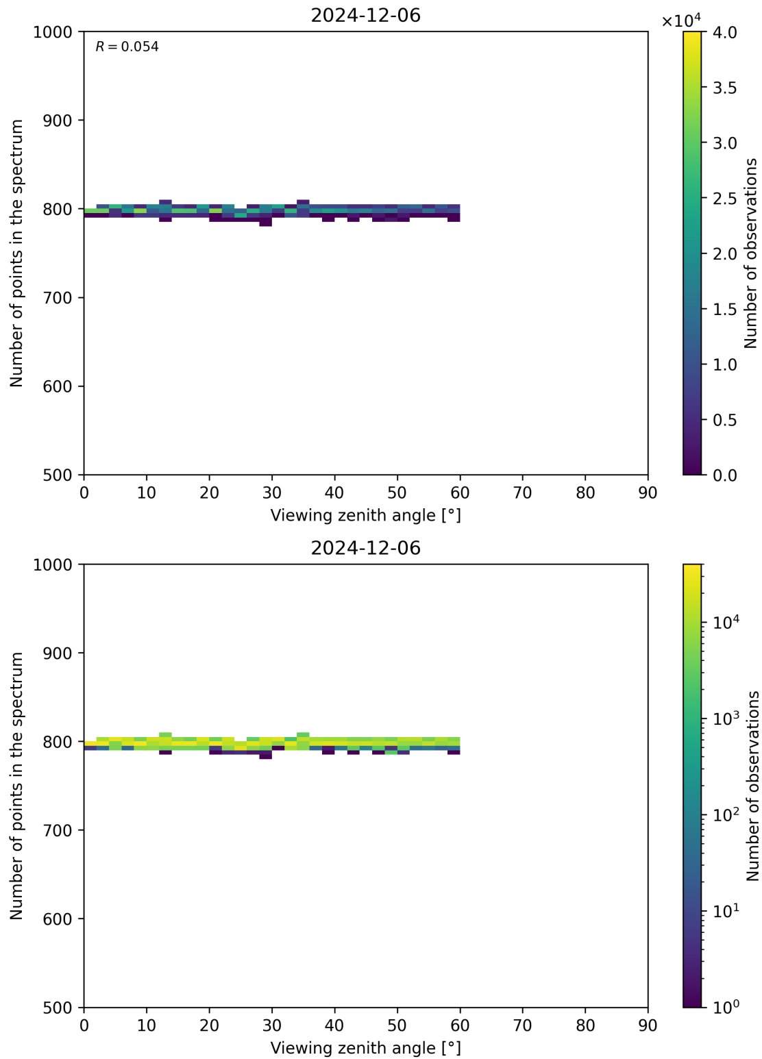
Figure 114: Scatter density plot of “Viewing zenith angle” against “Number of points in the spectrum” for 2024-12-06 to 2024-12-07.
