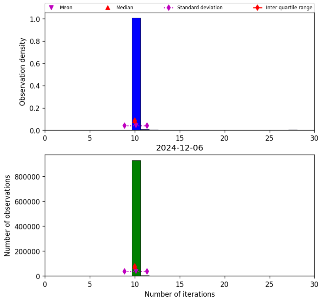
Figure 31: Histogram of “Number of iterations” for 2024-12-06 to 2024-12-07
