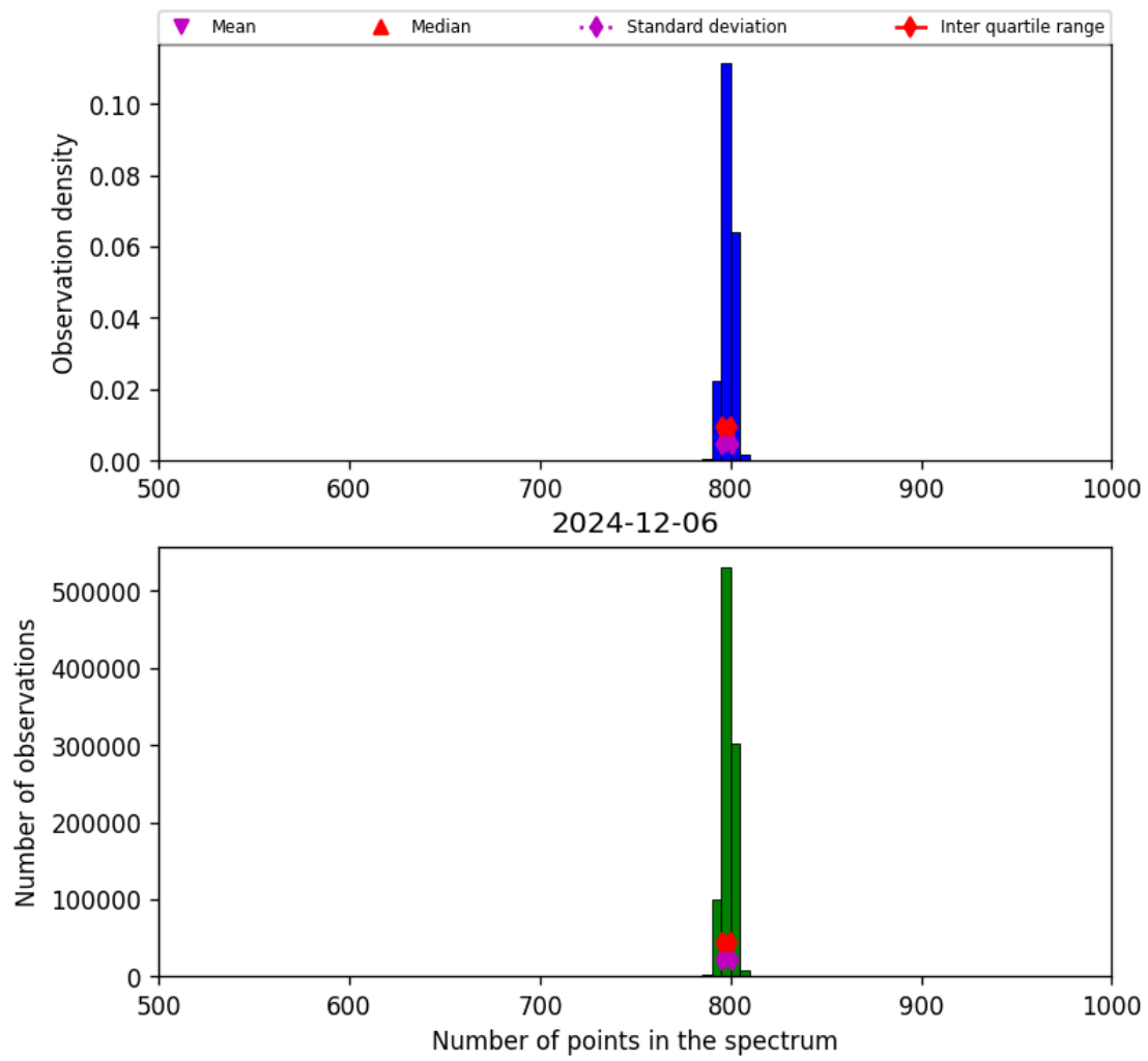
Figure 26: Histogram of “Number of points in the spectrum” for 2024-12-06 to 2024-12-07
