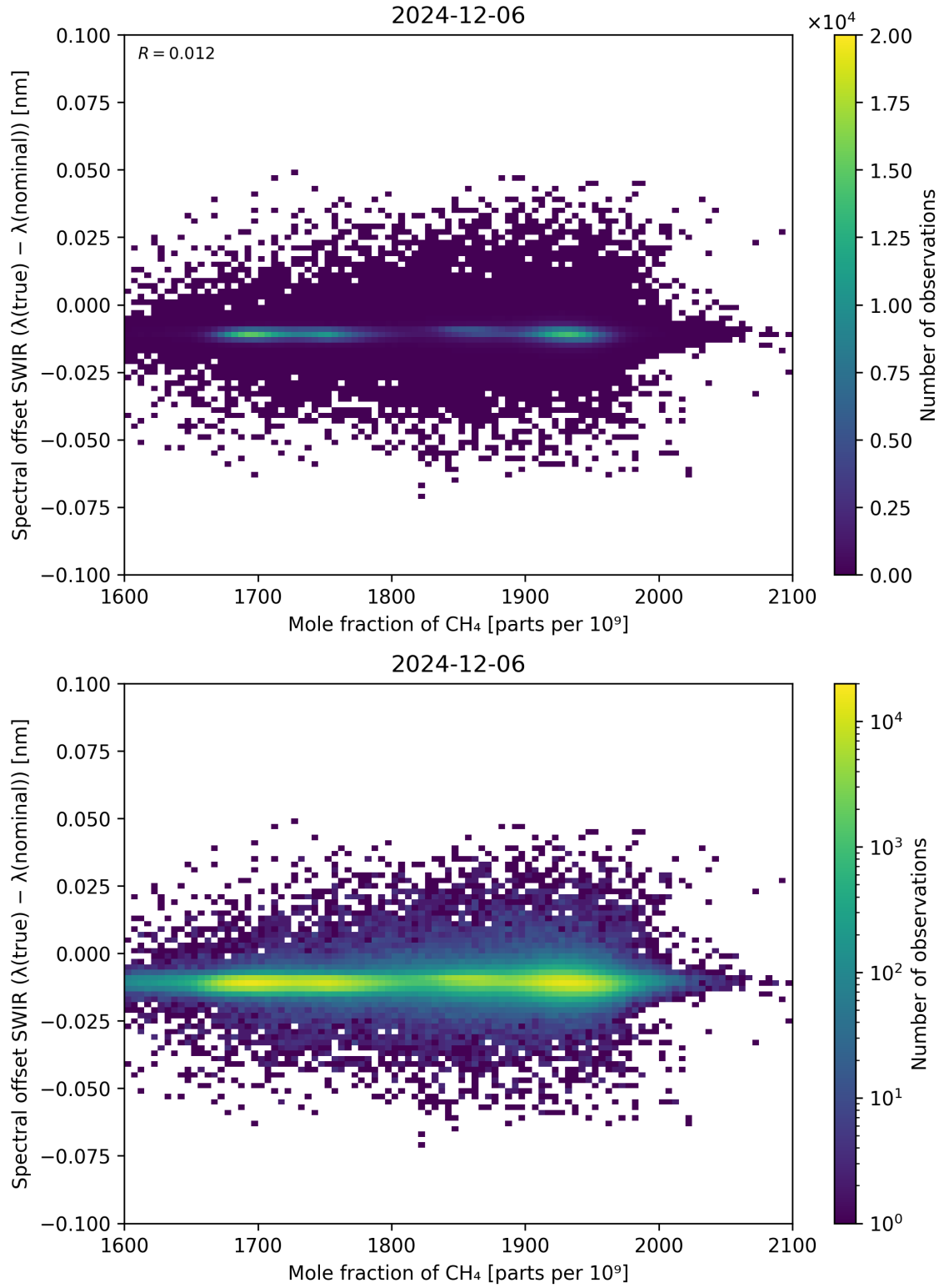
Figure 86: Scatter density plot of “Mole fraction of \text{CH}_4 ” against “Spectral offset SWIR ( \lambda_{\text{true}} - \lambda_{\text{nominal}} )” for 2024-12-06 to 2024-12-07.
