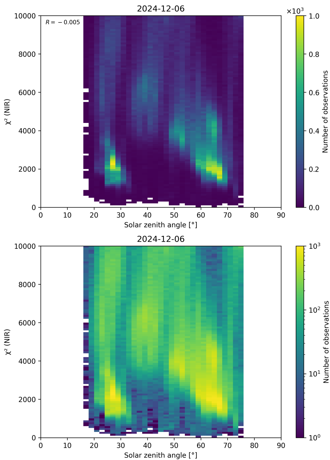
Figure 94: Scatter density plot of “Solar zenith angle” against “ \chi^2 (NIR)” for 2024-12-06 to 2024-12-07.
