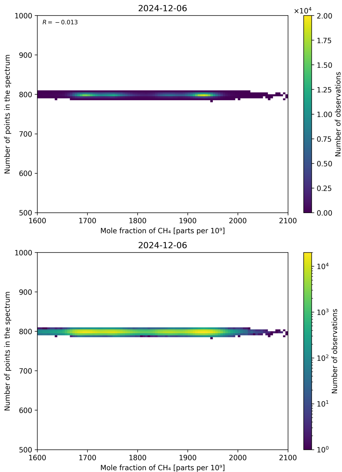
Figure 77: Scatter density plot of “Mole fraction of CH 4 ” against “Number of points in the spectrum” for 2024-12-06 to 2024-12-07.
