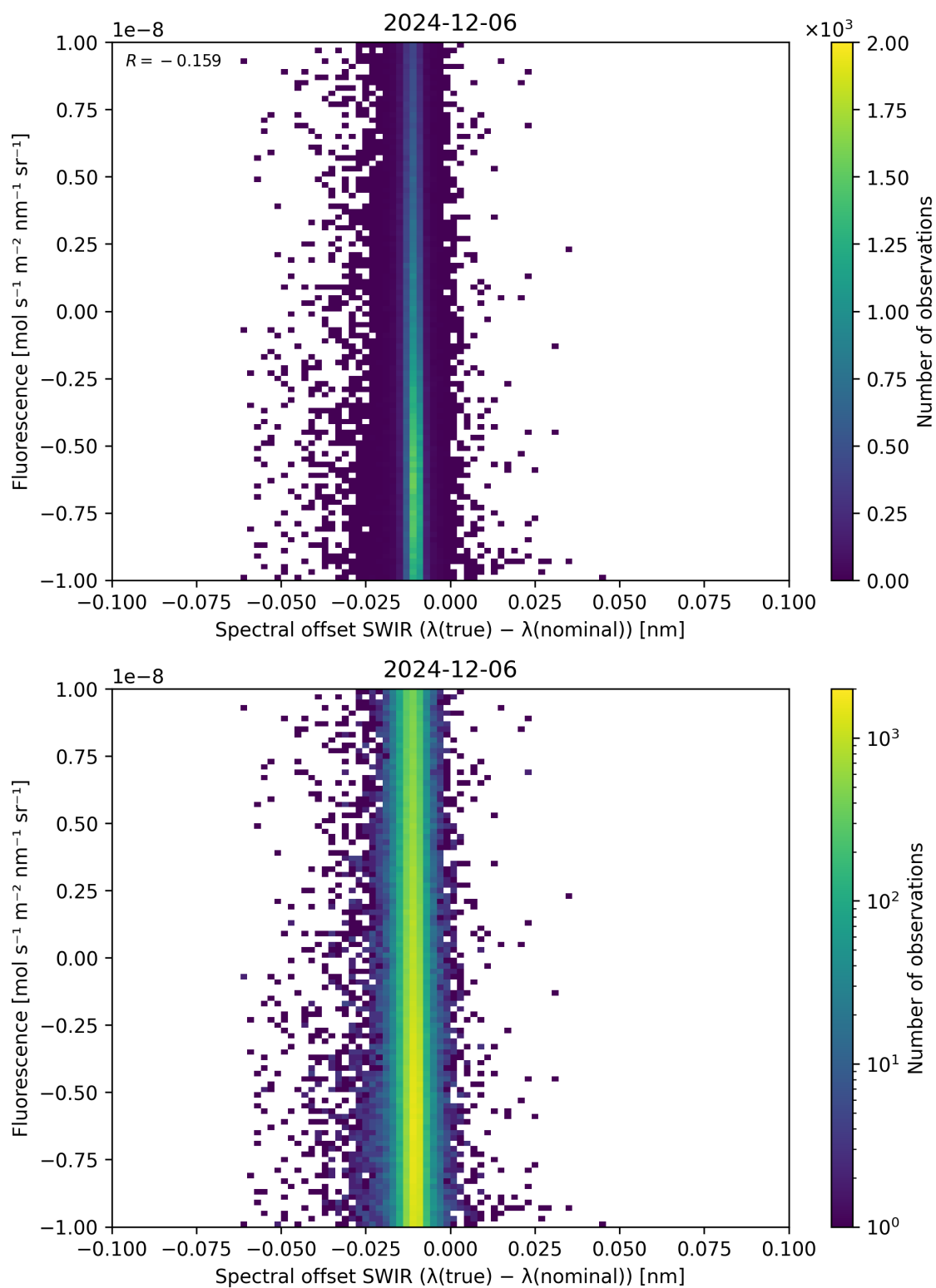
Figure 120: Scatter density plot of “Spectral offset SWIR ( \lambda_{\text{true}} - \lambda_{\text{nominal}} )” against “Fluorescence” for 2024-12-06 to 2024-12-07.
