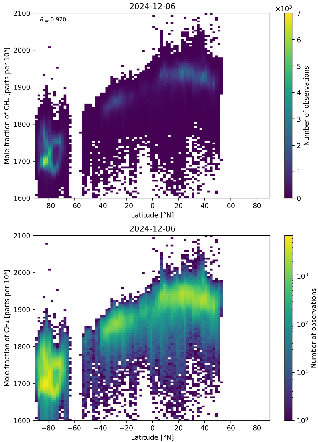
Figure 57: Scatter density plot of “Latitude” against “Mole fraction of CH 4 ” for 2024-12-06 to 2024-12-07.
