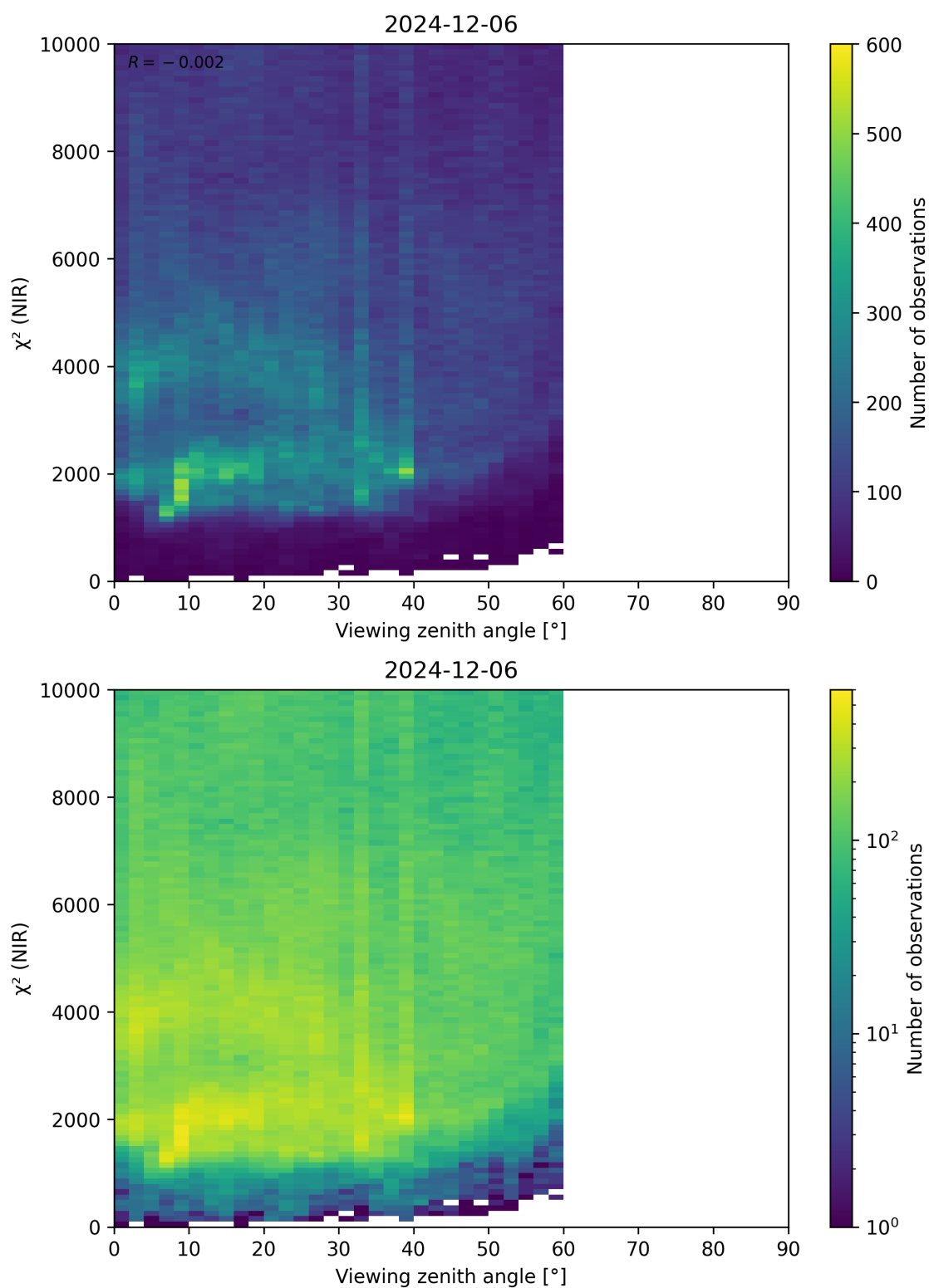
Figure 105: Scatter density plot of “Viewing zenith angle” against “ \chi^2 (NIR)” for 2024-12-06 to 2024-12-07.
