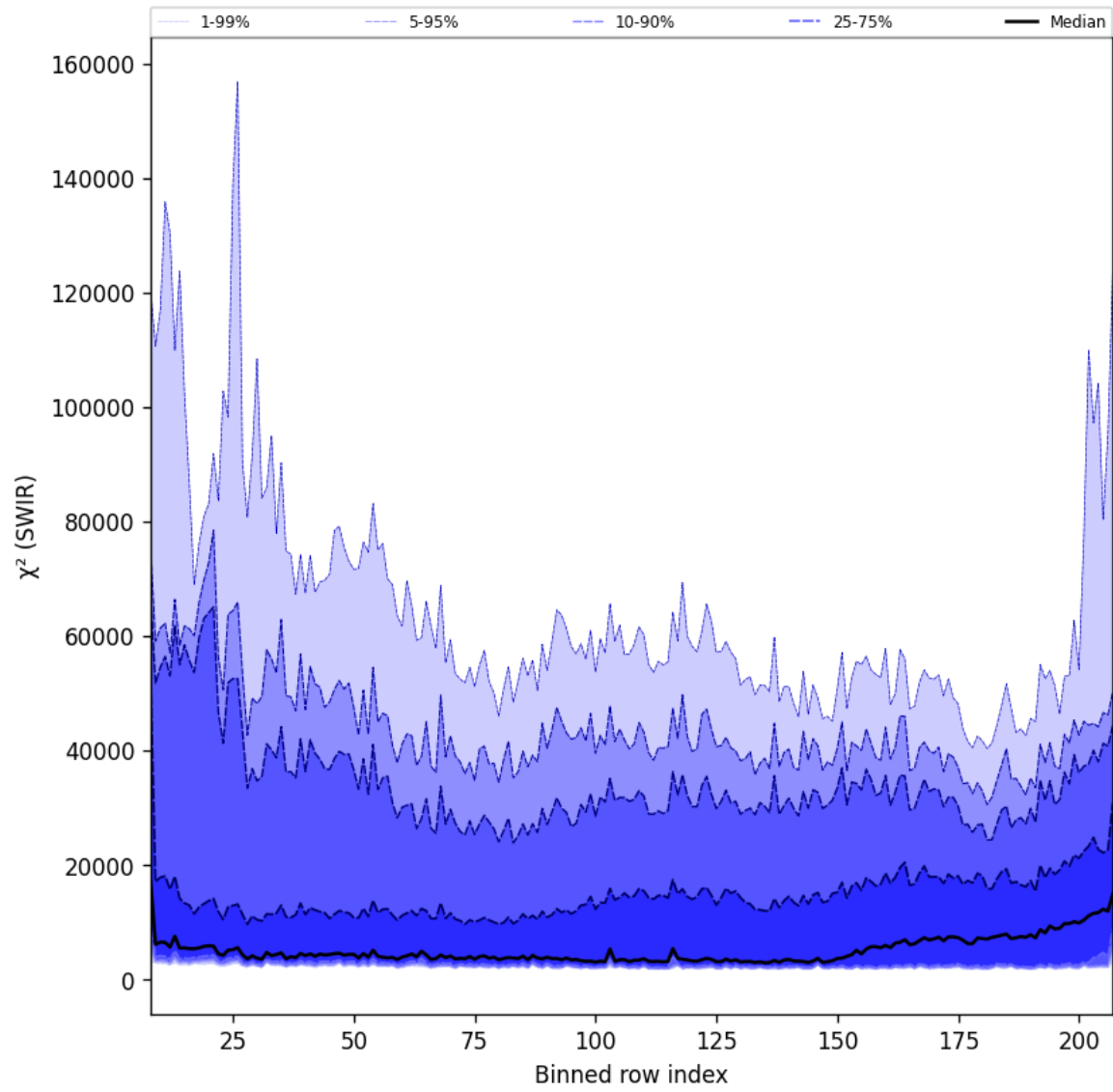
Figure 39: Along track statistics of “ \chi^2 (SWIR)” for 2024-12-06 to 2024-12-07
