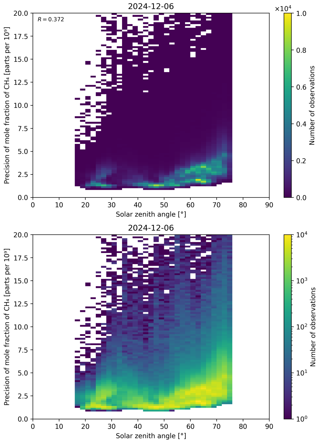
Figure 101: Scatter density plot of “Solar zenith angle” against “Precision of mole fraction of \text{CH}_4 ” for 2024-12-06 to 2024-12-07.
