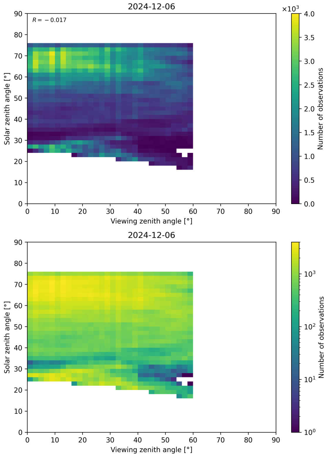
Figure 115: Scatter density plot of “Viewing zenith angle” against “Solar zenith angle” for 2024-12-06 to 2024-12-07.
