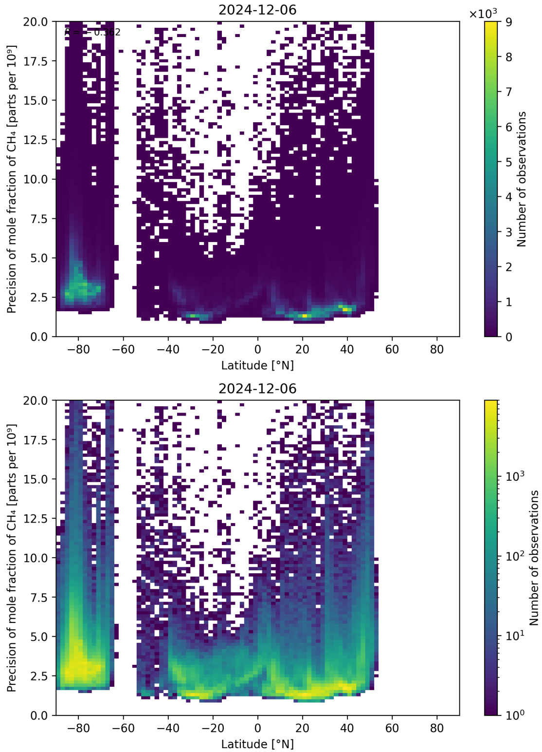
Figure 59: Scatter density plot of “Latitude” against “Precision of mole fraction of CH 4 ” for 2024-12-06 to 2024-12-07.
