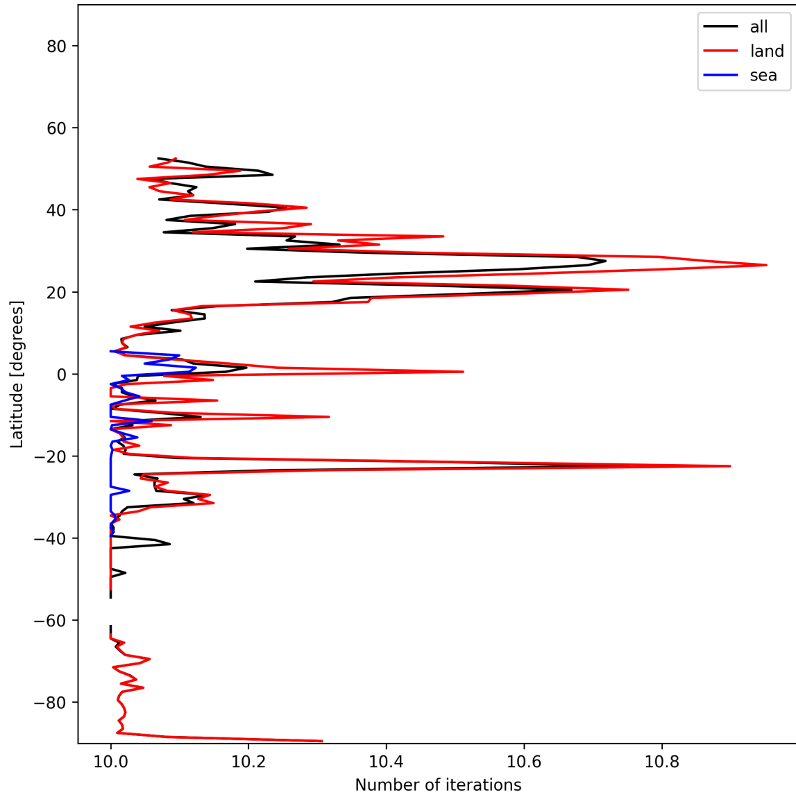
Figure 20: Zonal average of “Number of iterations” for 2024-12-06 to 2024-12-07.
