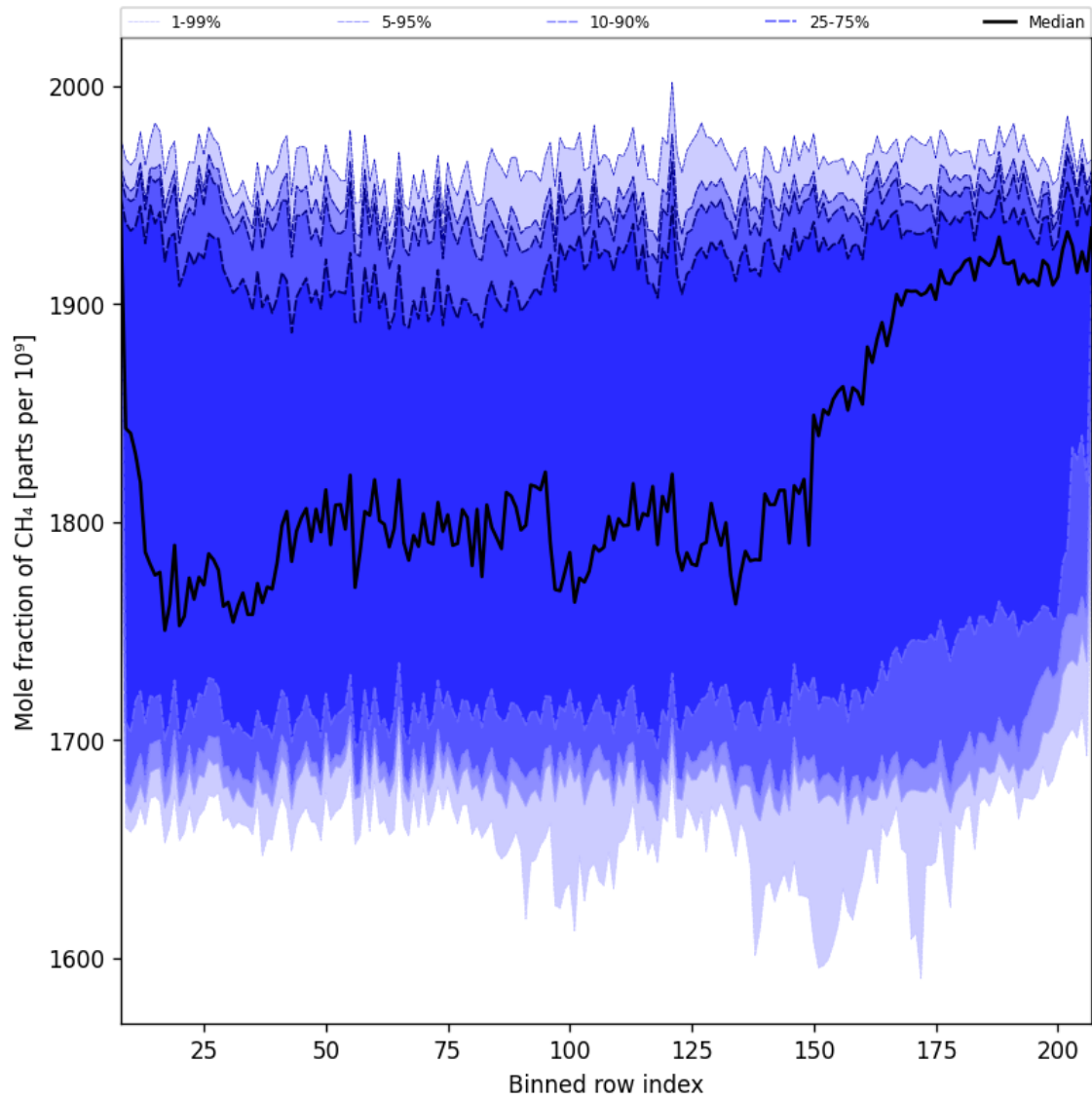
Figure 34: Along track statistics of “Mole fraction of CH 4 ” for 2024-12-06 to 2024-12-07
