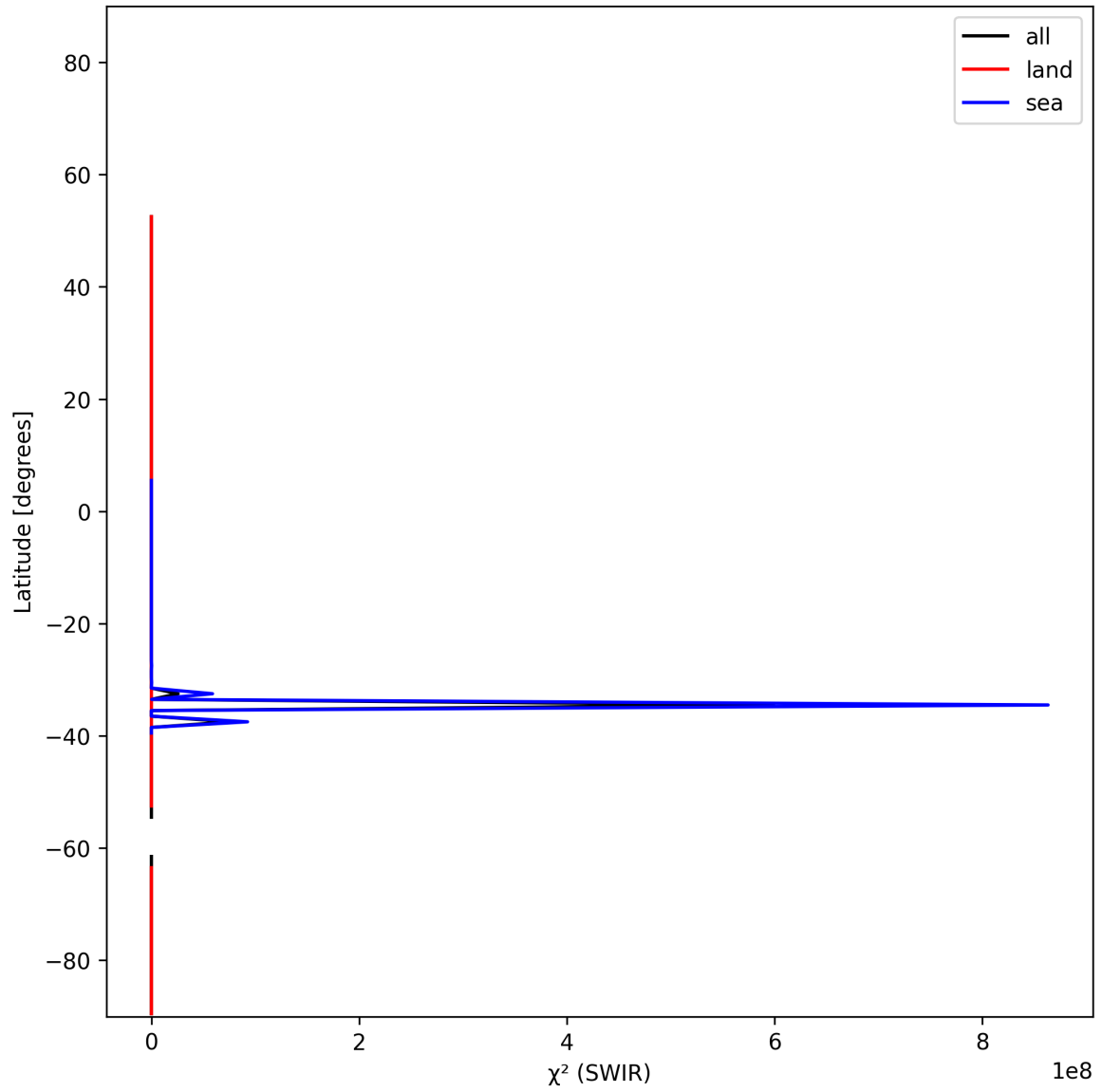
Figure 17: Zonal average of “ \chi^2 (SWIR)” for 2024-12-06 to 2024-12-07.
