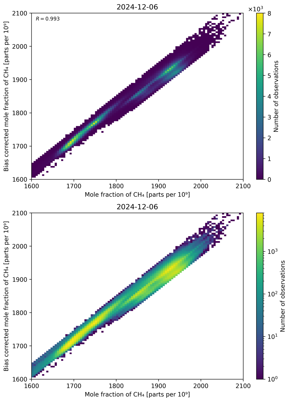
Figure 74: Scatter density plot of “Mole fraction of CH 4 ” against “Bias corrected mole fraction of CH 4 ” for 2024-12-06 to 2024-12-07.
