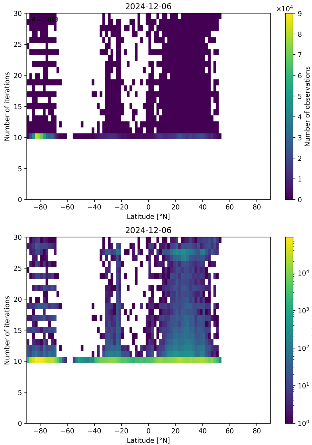
Figure 60: Scatter density plot of “Latitude” against “Number of iterations” for 2024-12-06 to 2024-12-07.
