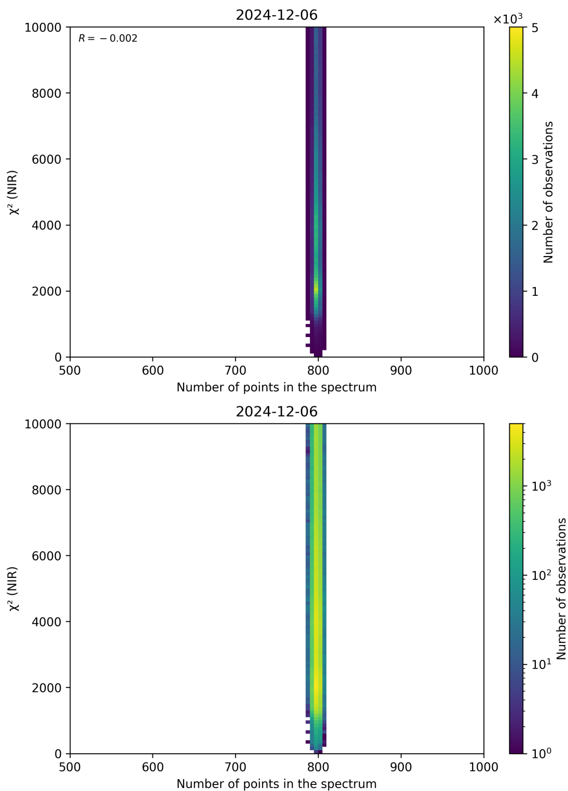
Figure 88: Scatter density plot of “Number of points in the spectrum” against “ \chi^2 (NIR)” for 2024-12-06 to 2024-12-07.
