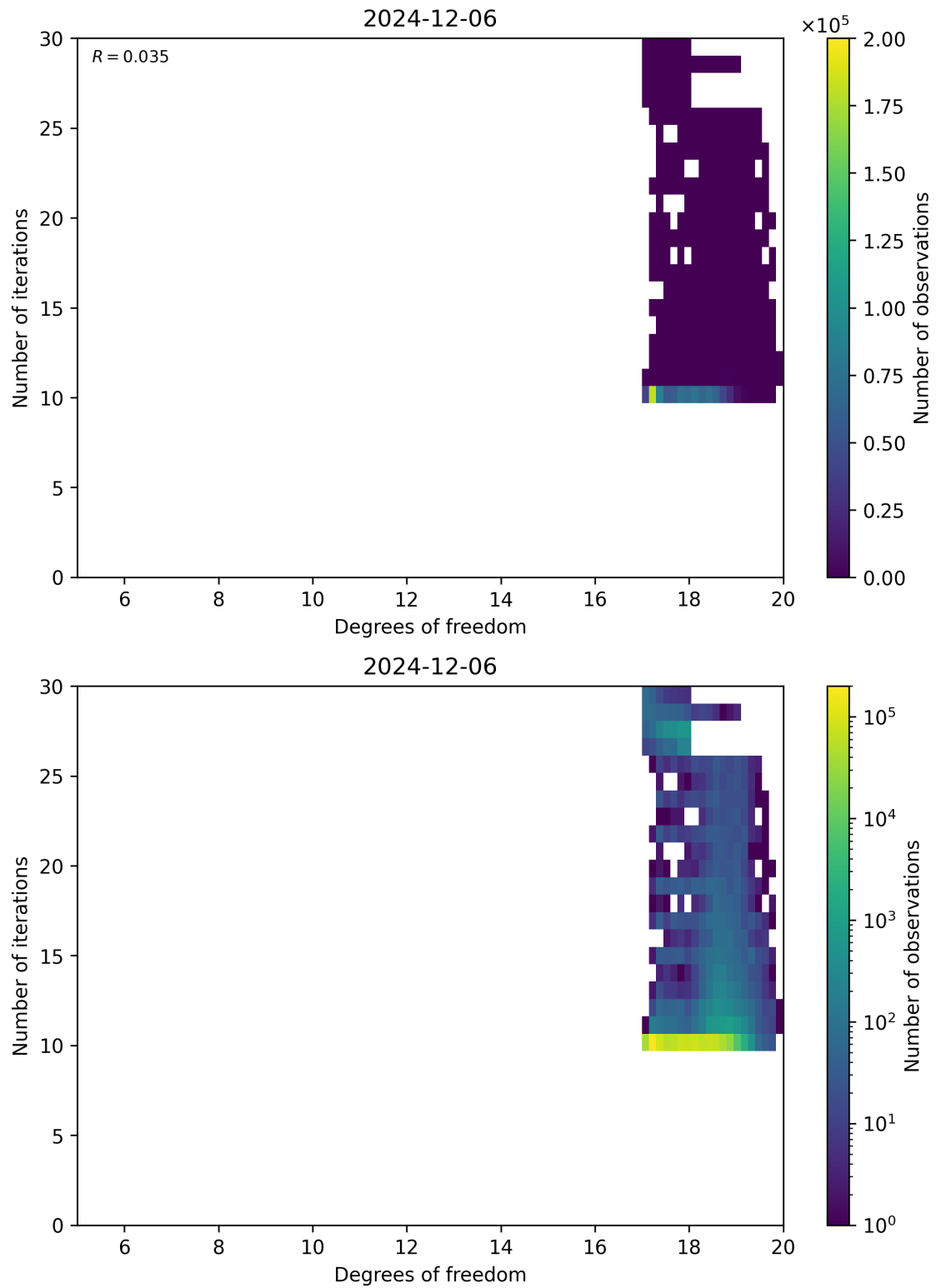
Figure 52: Scatter density plot of “Degrees of freedom” against “Number of iterations” for 2024-12-06 to 2024-12-07.
