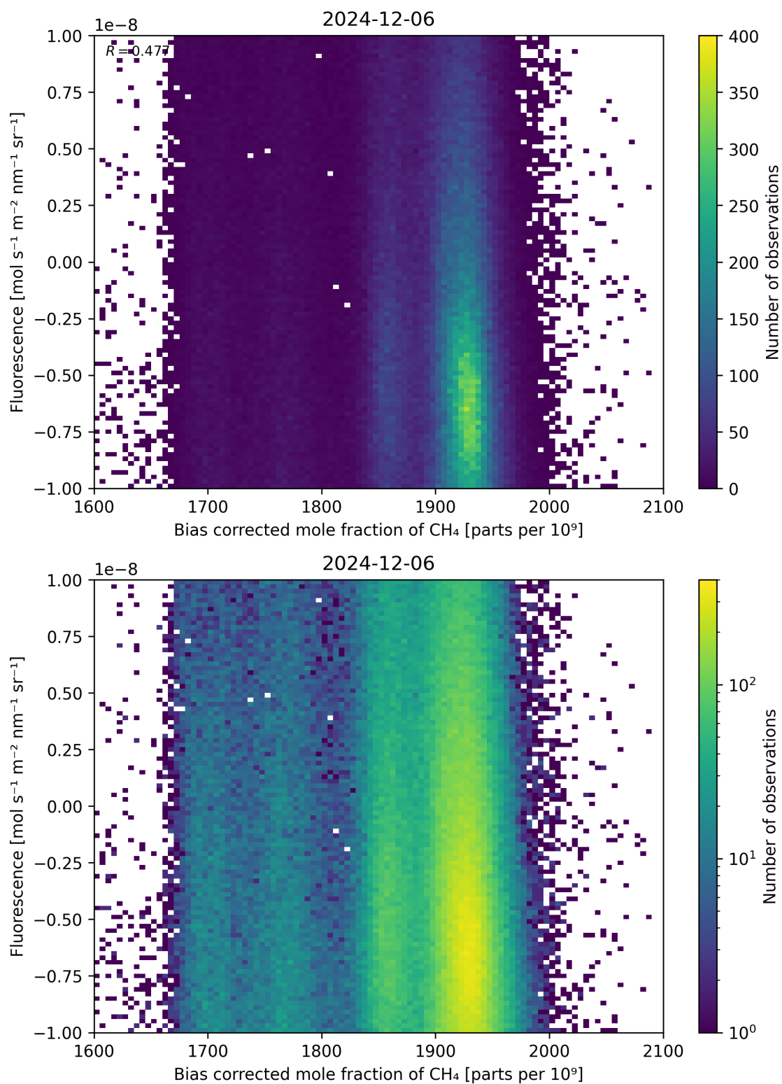
Figure 66: Scatter density plot of “Bias corrected mole fraction of \text{CH}_4 ” against “Fluorescence” for 2024-12-06 to 2024-12-07.
