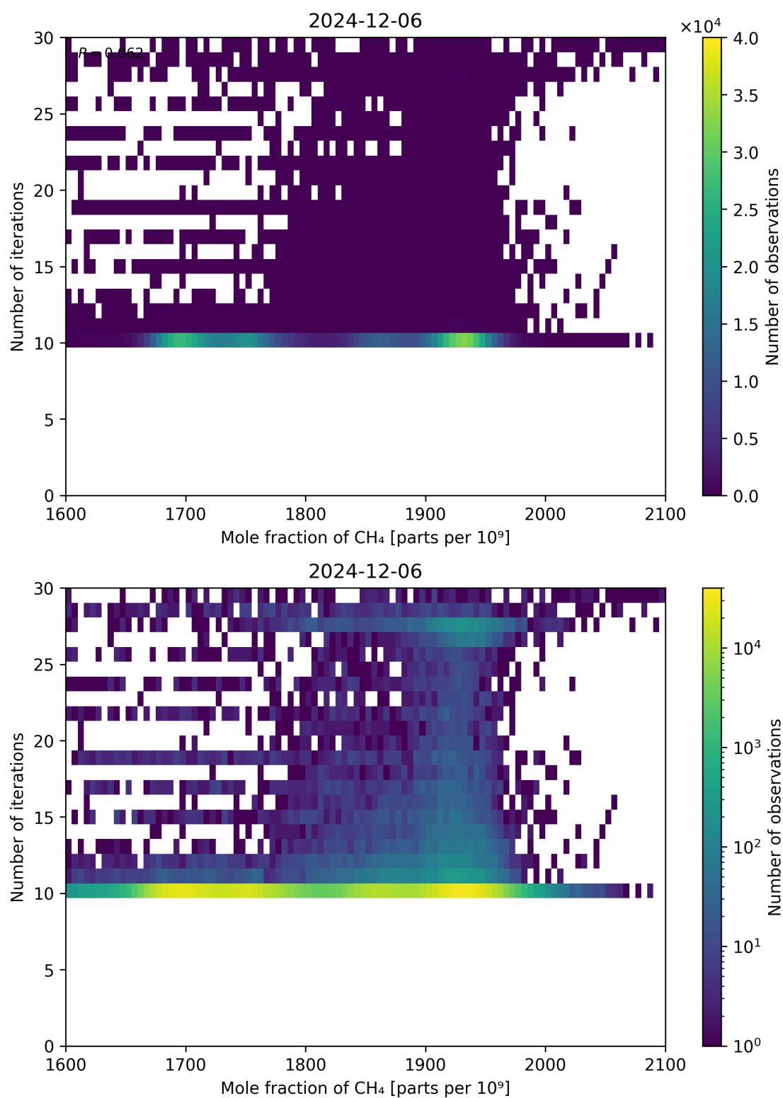
Figure 76: Scatter density plot of “Mole fraction of CH 4 ” against “Number of iterations” for 2024-12-06 to 2024-12-07.
