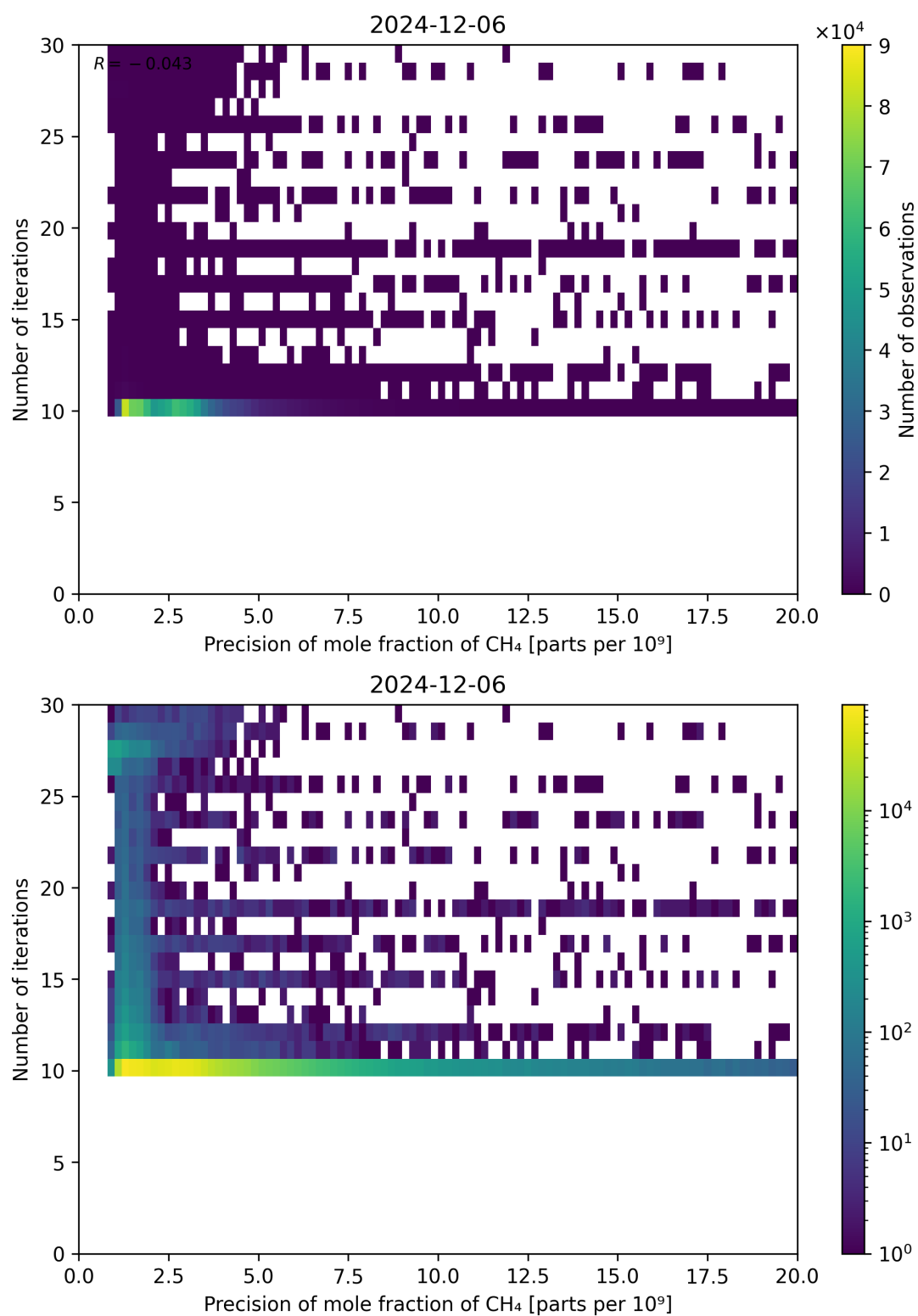
Figure 83: Scatter density plot of “Precision of mole fraction of CH 4 ” against “Number of iterations” for 2024-12-06 to 2024-12-07.
