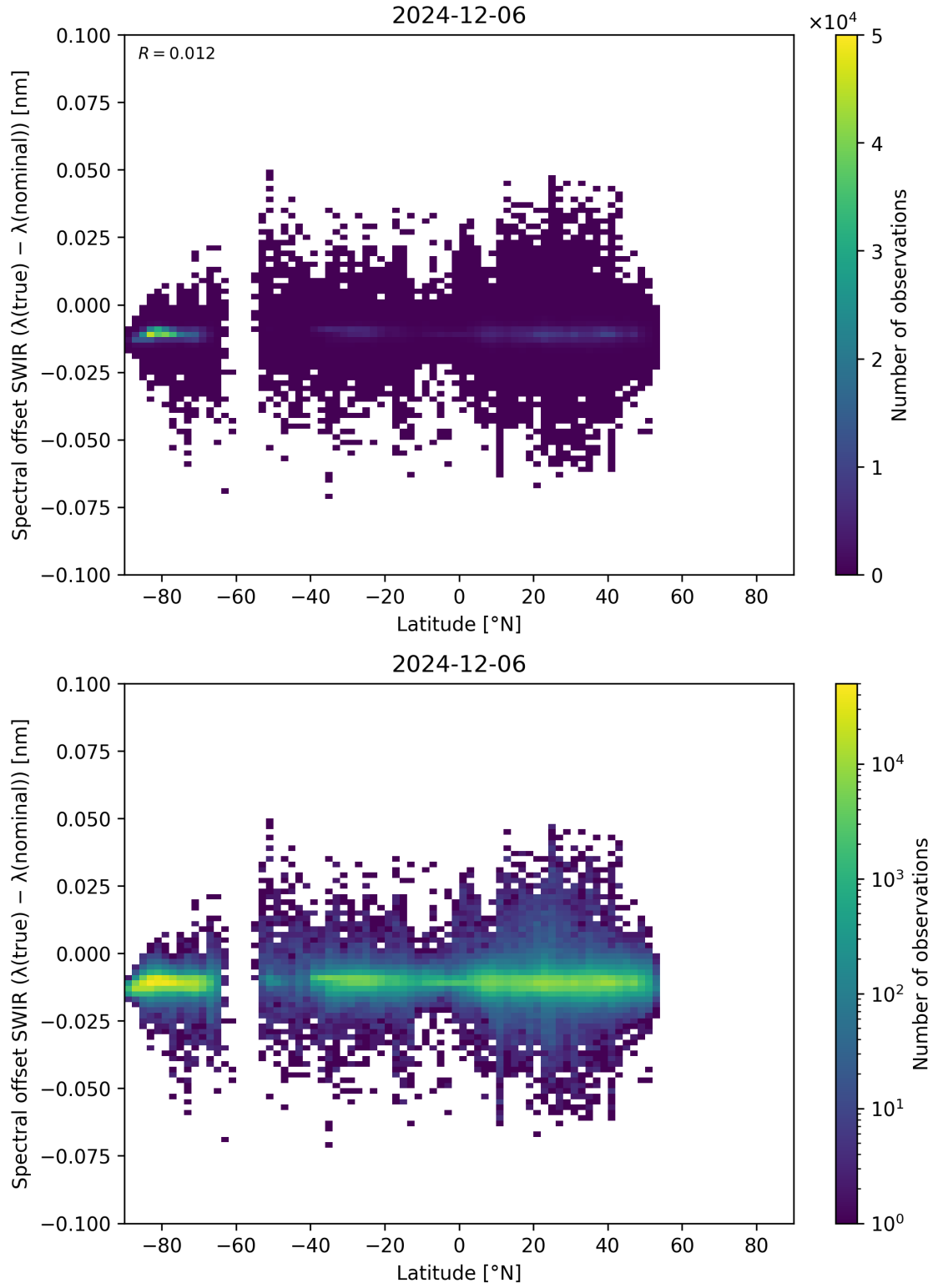
Figure 62: Scatter density plot of “Latitude” against “Spectral offset SWIR ( \lambda_{\text{true}} - \lambda_{\text{nominal}} )” for 2024-12-06 to 2024-12-07.
