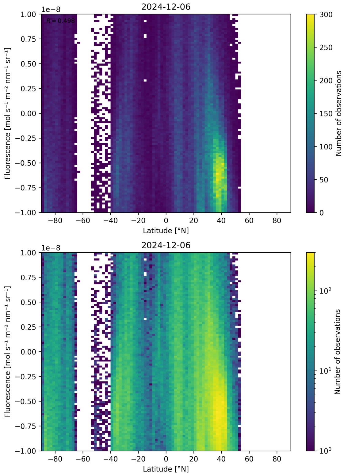
Figure 56: Scatter density plot of “Latitude” against “Fluorescence” for 2024-12-06 to 2024-12-07.
