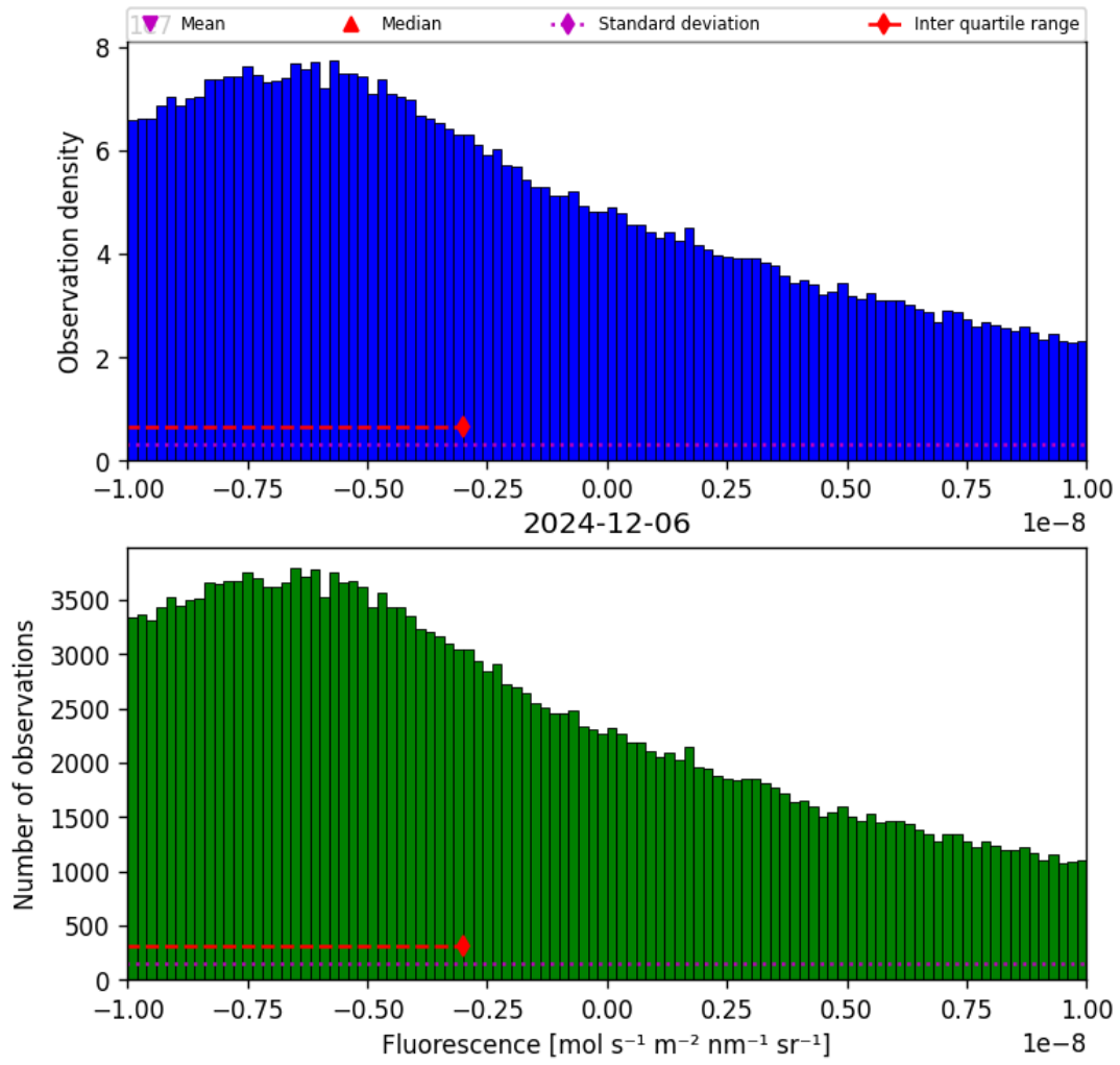
Figure 32: Histogram of “Fluorescence” for 2024-12-06 to 2024-12-07
