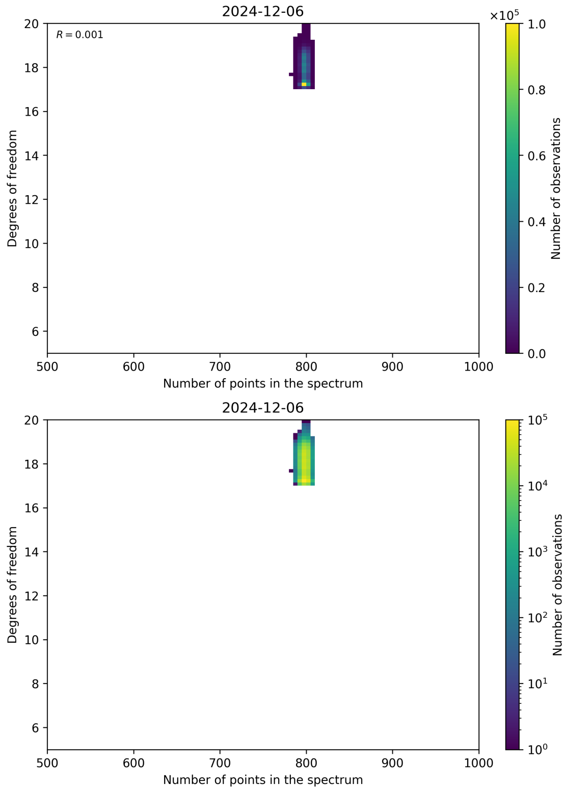
Figure 90: Scatter density plot of “Number of points in the spectrum” against “Degrees of freedom” for 2024-12-06 to 2024-12-07.
