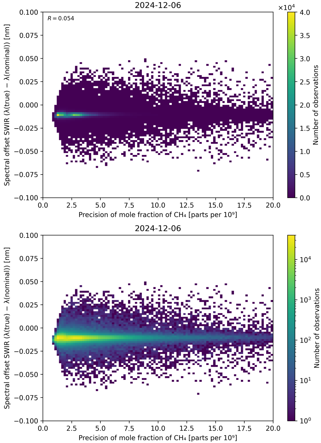
Figure 85: Scatter density plot of “Precision of mole fraction of \text{CH}_4 ” against “Spectral offset SWIR ( \lambda_{\text{true}} - \lambda_{\text{nominal}} )” for 2024-12-06 to 2024-12-07.
