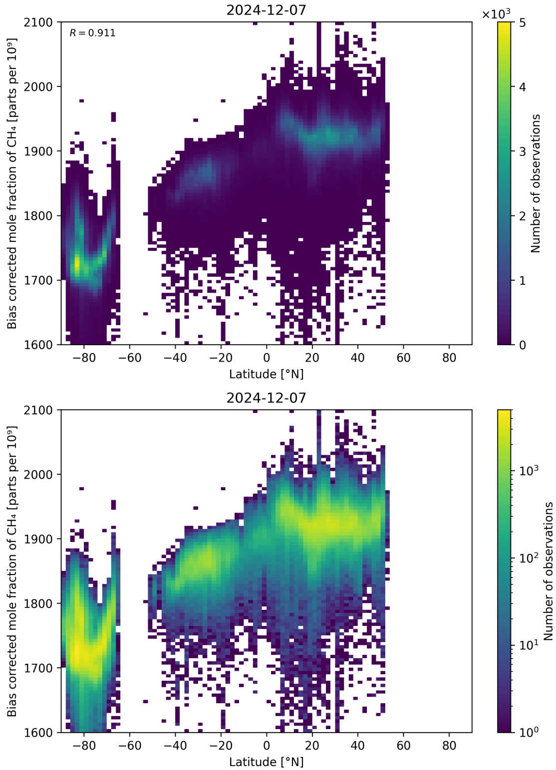
Figure 58: Scatter density plot of “Latitude” against “Bias corrected mole fraction of CH 4 ” for 2024-12-06 to 2024-12-08.
