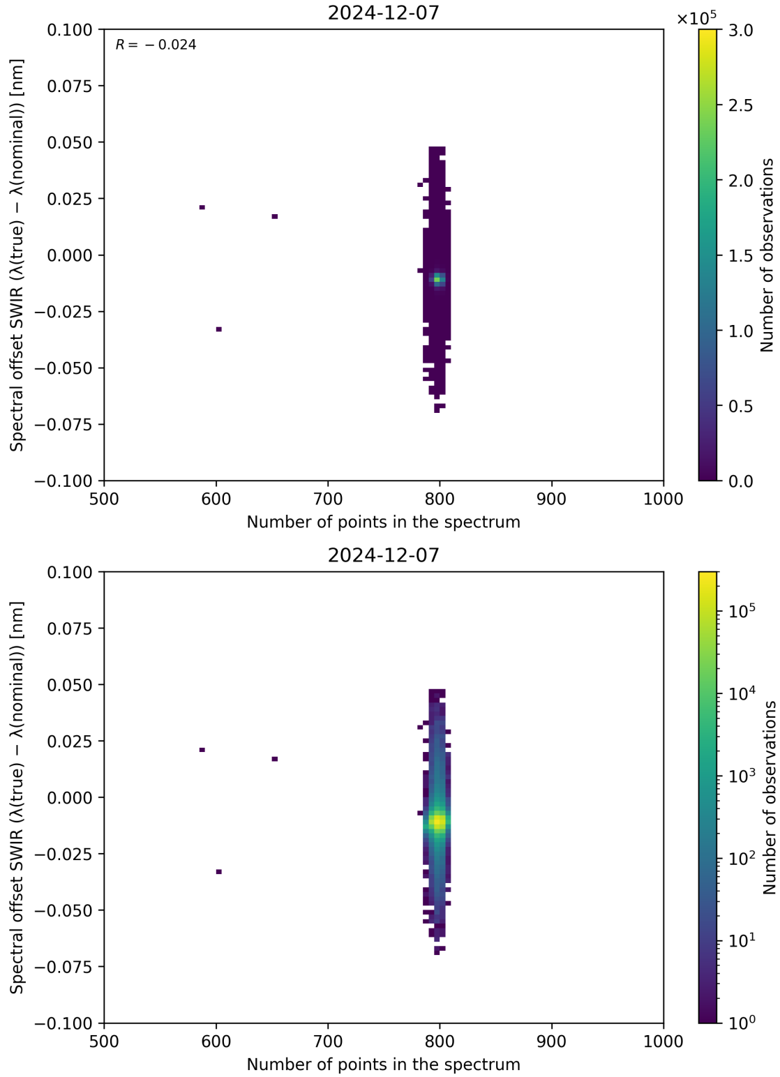
Figure 93: Scatter density plot of “Number of points in the spectrum” against “Spectral offset SWIR ( \lambda_{\text{true}} - \lambda_{\text{nominal}} )” for 2024-12-06 to 2024-12-08.
