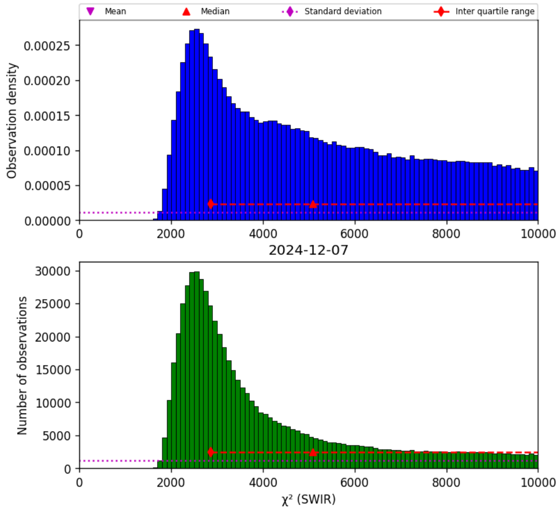
Figure 28: Histogram of “ \chi^2 (SWIR)” for 2024-12-06 to 2024-12-08
