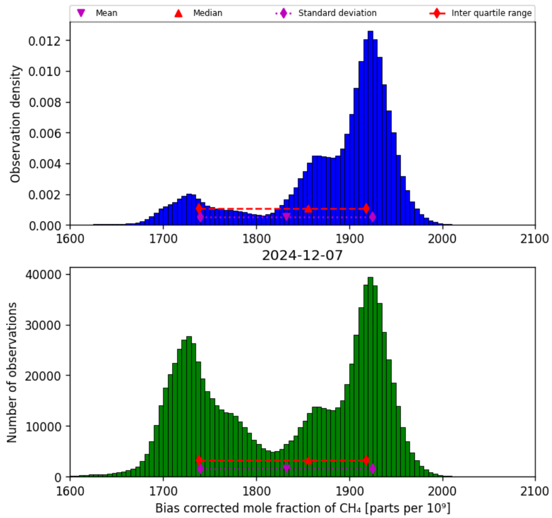
Figure 25: Histogram of “Bias corrected mole fraction of CH 4 ” for 2024-12-06 to 2024-12-08
