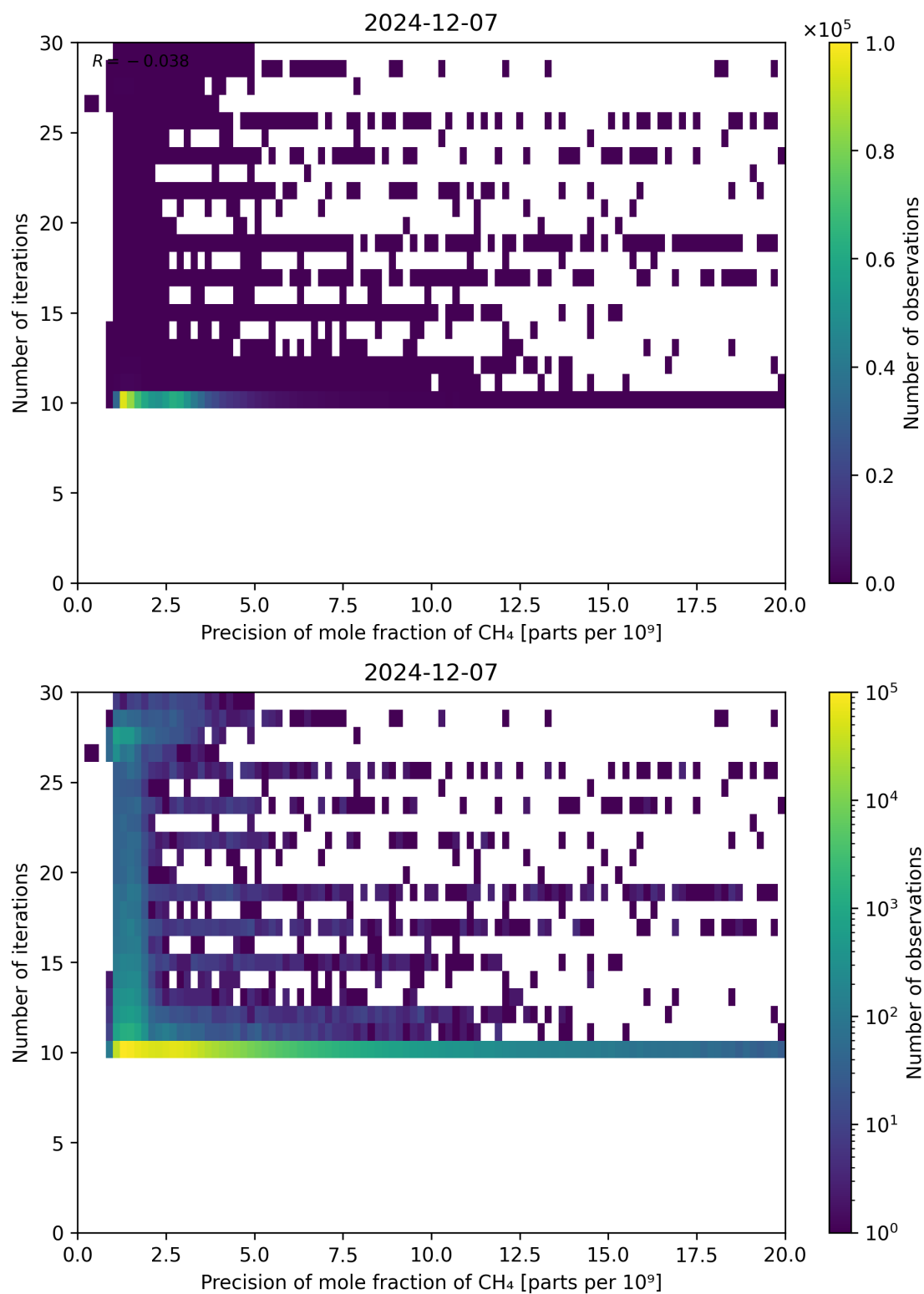
Figure 83: Scatter density plot of “Precision of mole fraction of \text{CH}_4 ” against “Number of iterations” for 2024-12-06 to 2024-12-08.
