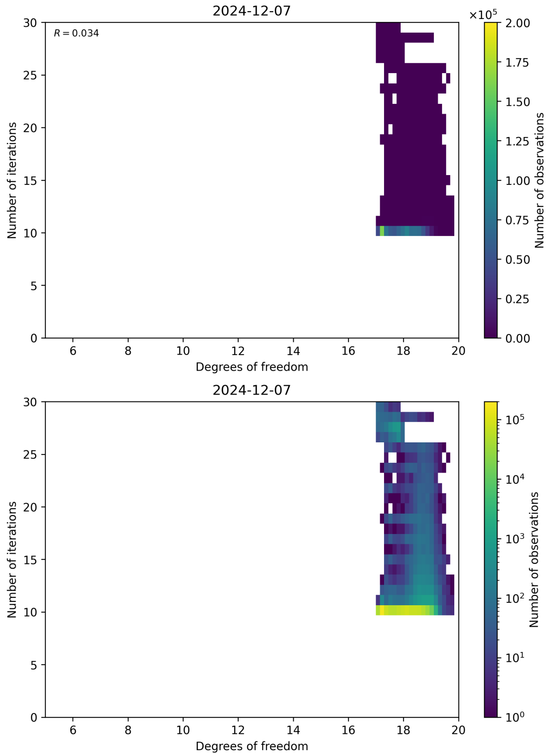
Figure 52: Scatter density plot of “Degrees of freedom” against “Number of iterations” for 2024-12-06 to 2024-12-08.
