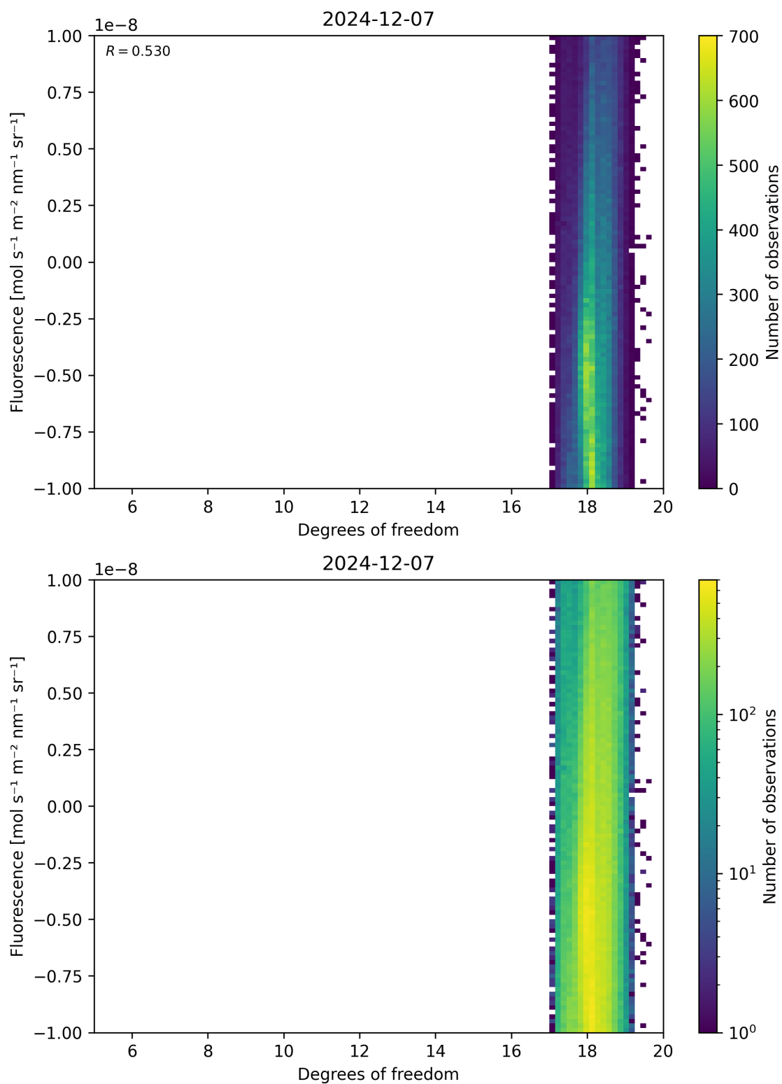
Figure 51: Scatter density plot of “Degrees of freedom” against “Fluorescence” for 2024-12-06 to 2024-12-08.
