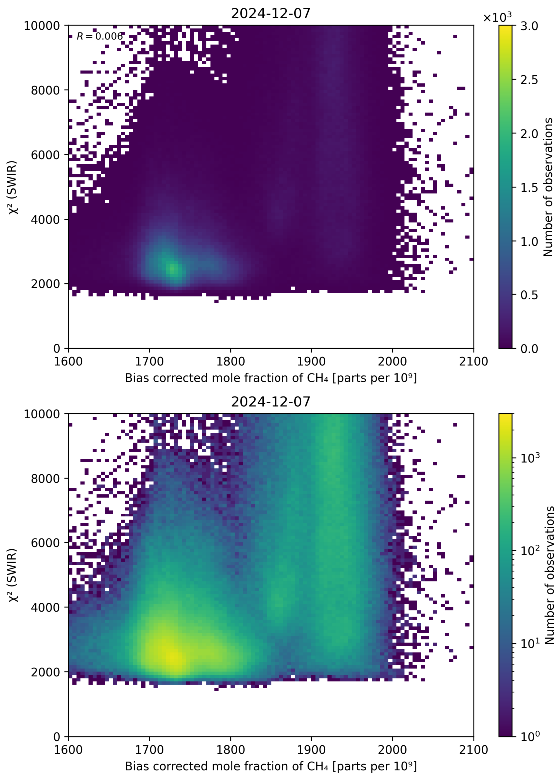
Figure 64: Scatter density plot of “Bias corrected mole fraction of \text{CH}_4 ” against “ \chi^2 (SWIR)” for 2024-12-06 to 2024-12-08.
