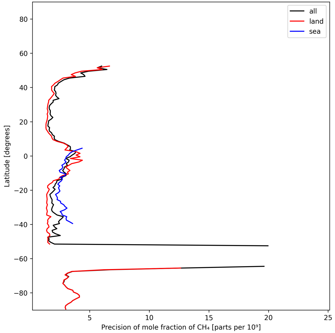
Figure 13: Zonal average of “Precision of mole fraction of CH 4 ” for 2024-12-06 to 2024-12-08.
