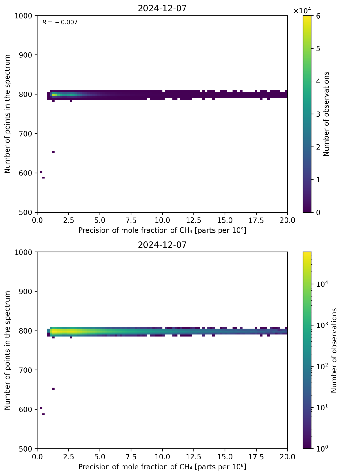
Figure 84: Scatter density plot of “Precision of mole fraction of CH 4 ” against “Number of points in the spectrum” for 2024-12-06 to 2024-12-08.
