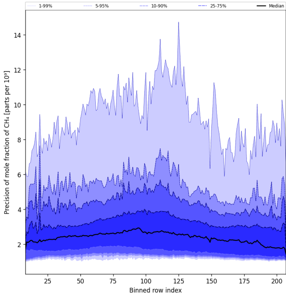
Figure 35: Along track statistics of “Precision of mole fraction of CH 4 ” for 2024-12-06 to 2024-12-08
