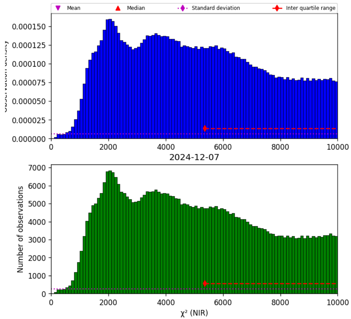
Figure 29: Histogram of “ \chi^2 (NIR)” for 2024-12-06 to 2024-12-08
