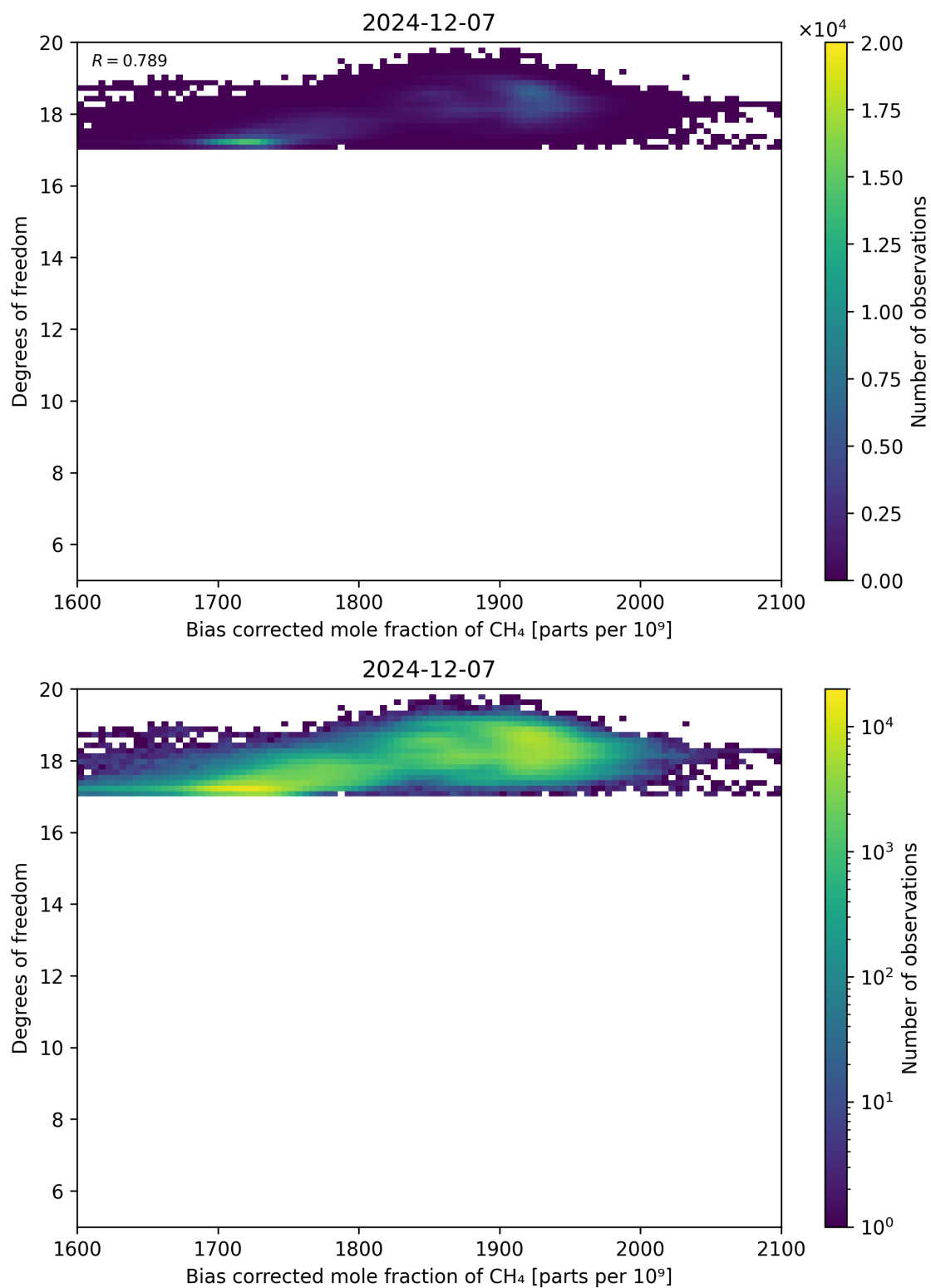
Figure 65: Scatter density plot of “Bias corrected mole fraction of CH 4 ” against “Degrees of freedom” for 2024-12-06 to 2024-12-08.
