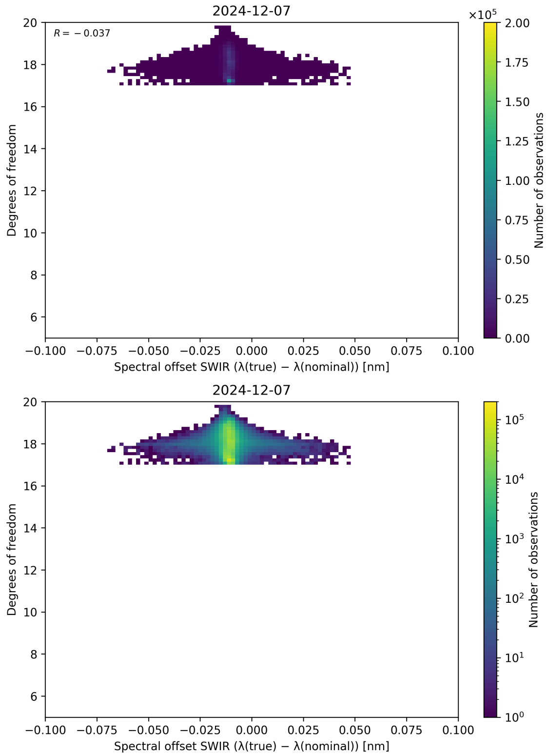
Figure 119: Scatter density plot of “Spectral offset SWIR ( \lambda_{\text{true}} - \lambda_{\text{nominal}} )” against “Degrees of freedom” for 2024-12-06 to 2024-12-08.
