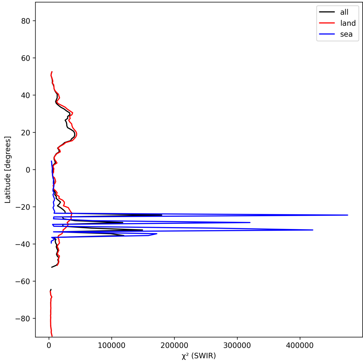
Figure 17: Zonal average of “ \chi^2 (SWIR)” for 2024-12-06 to 2024-12-08.
