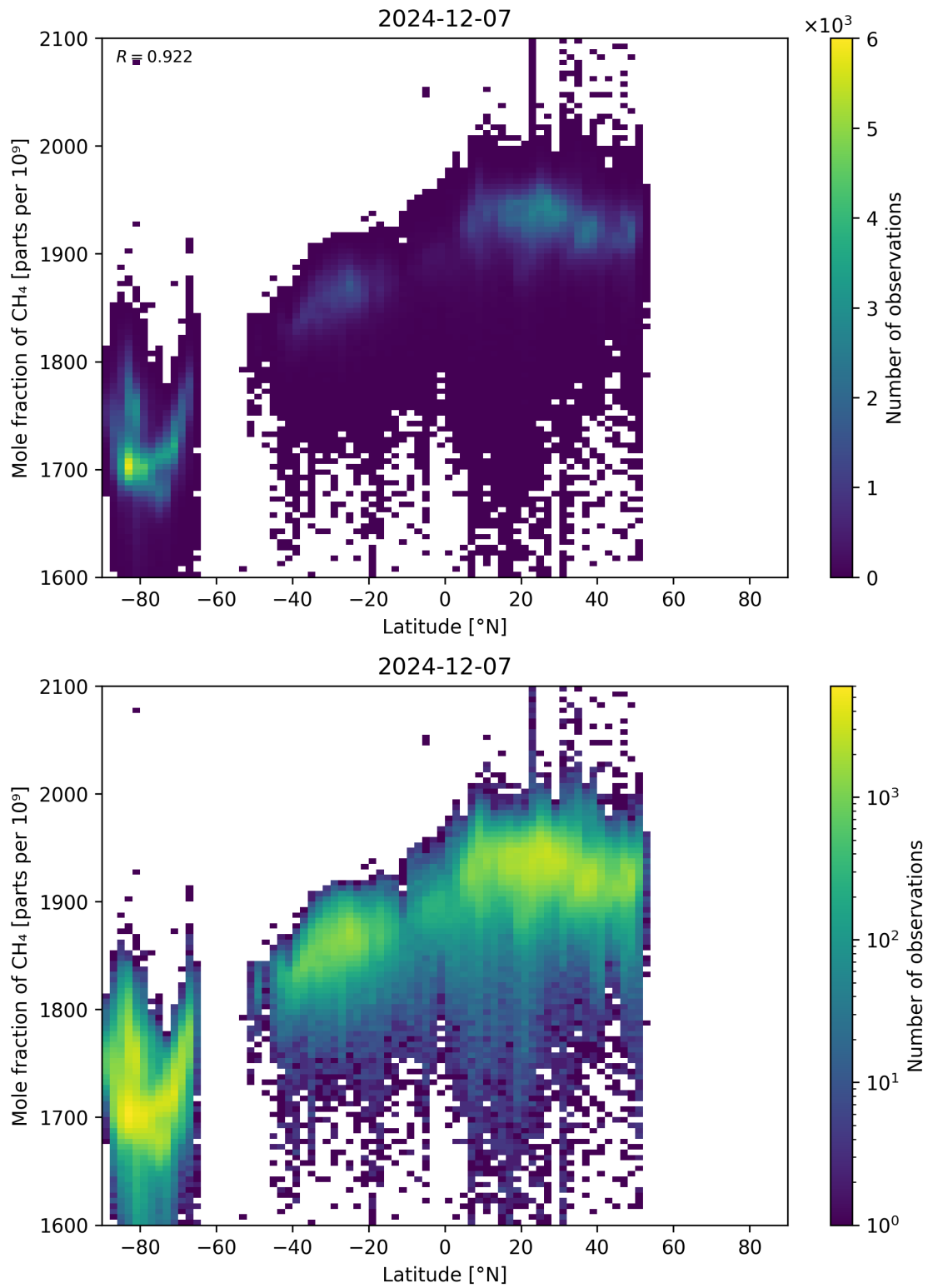
Figure 57: Scatter density plot of “Latitude” against “Mole fraction of CH 4 ” for 2024-12-06 to 2024-12-08.
