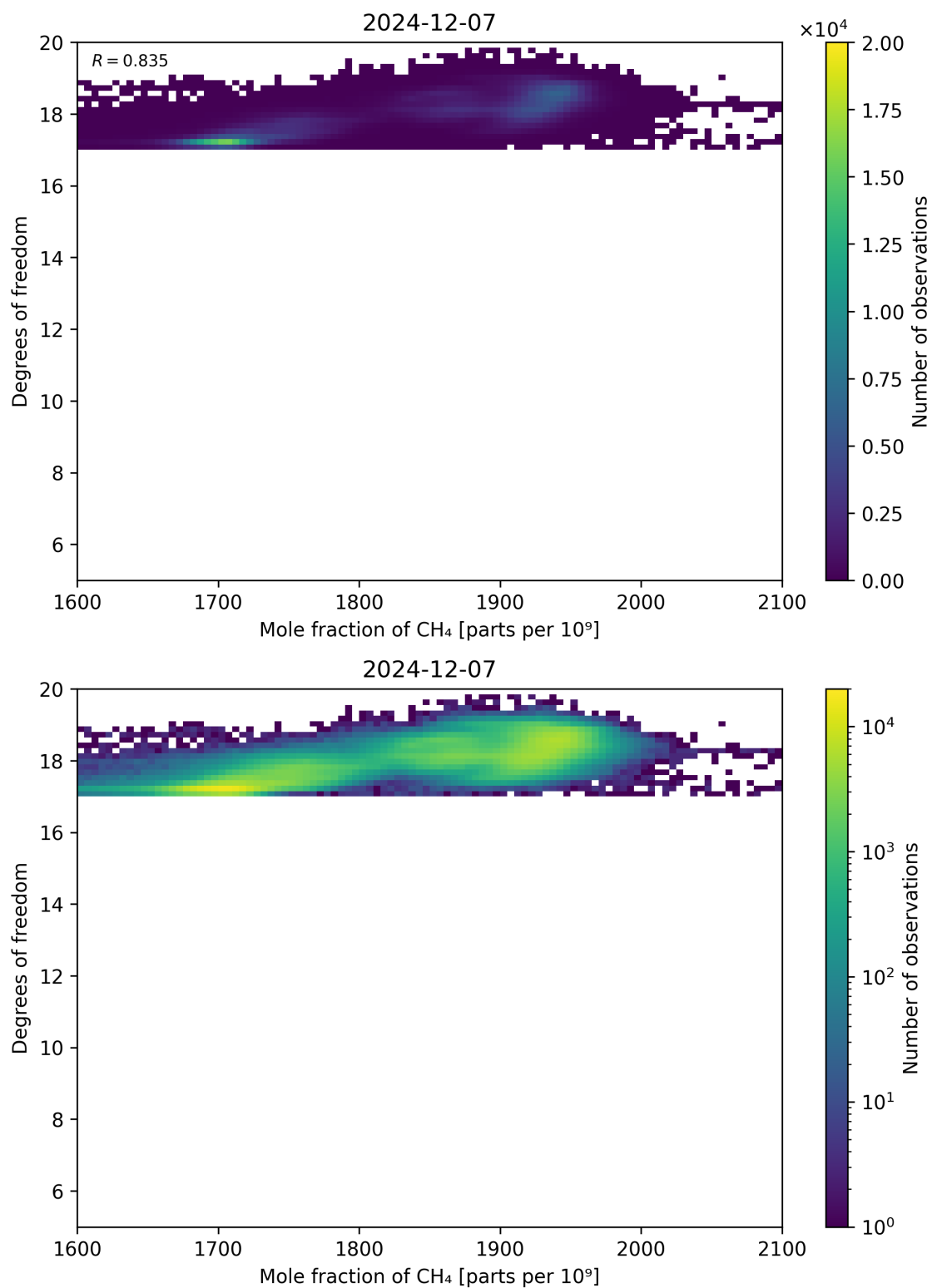
Figure 72: Scatter density plot of “Mole fraction of CH 4 ” against “Degrees of freedom” for 2024-12-06 to 2024-12-08.
