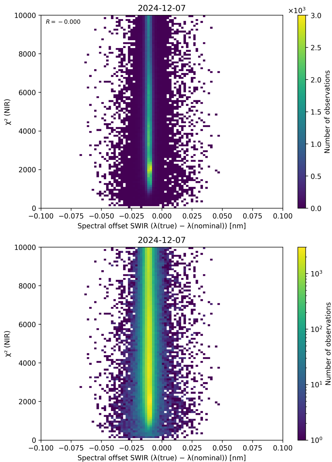
Figure 117: Scatter density plot of “Spectral offset SWIR ( \lambda_{\text{true}} - \lambda_{\text{nominal}} )” against “ \chi^2 (NIR)” for 2024-12-06 to 2024-12-08.
