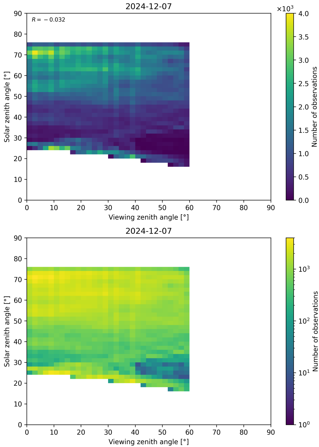
Figure 115: Scatter density plot of “Viewing zenith angle” against “Solar zenith angle” for 2024-12-06 to 2024-12-08.
