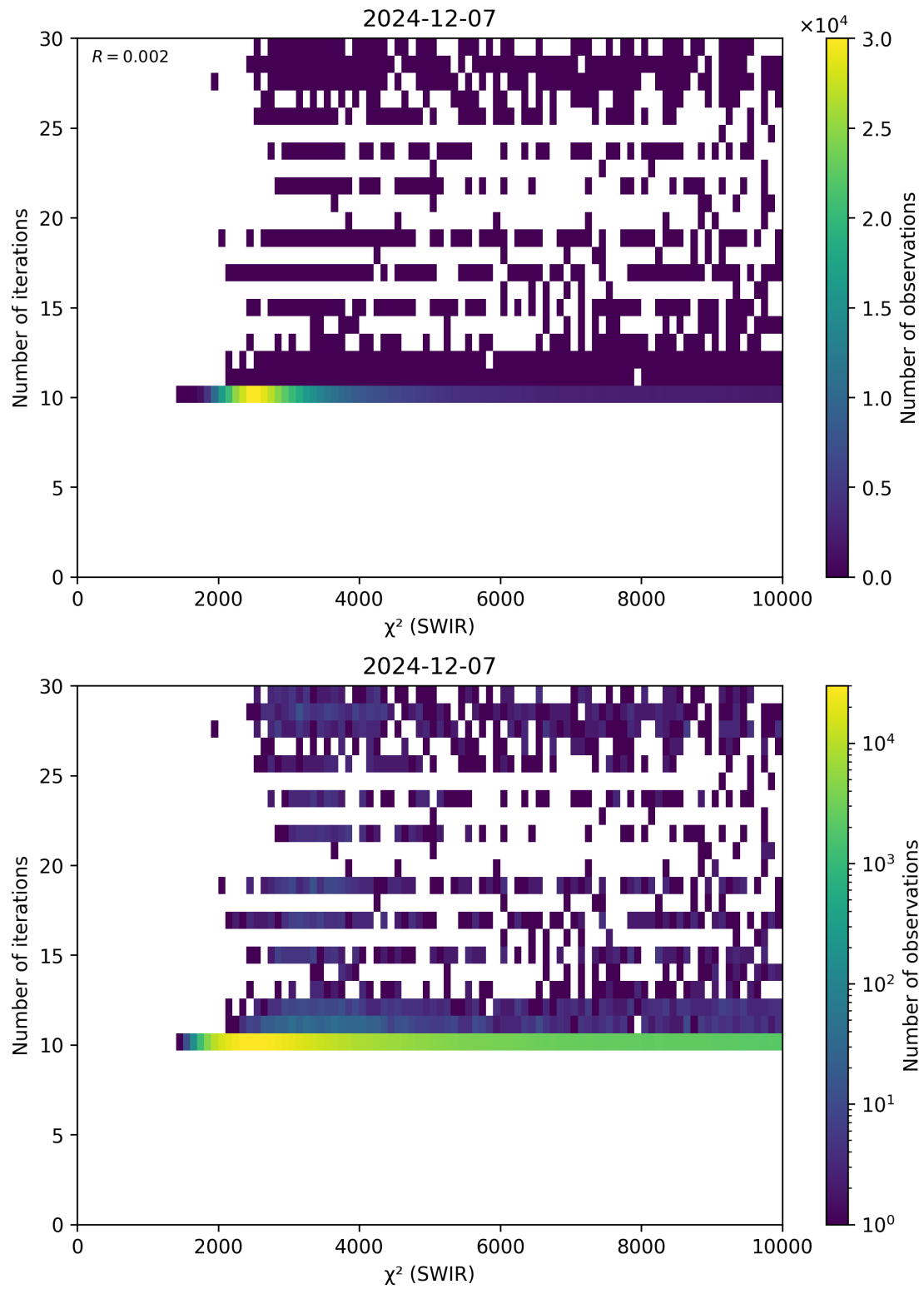
Figure 50: Scatter density plot of “ \chi^2 (SWIR)” against “Number of iterations” for 2024-12-06 to 2024-12-08.
