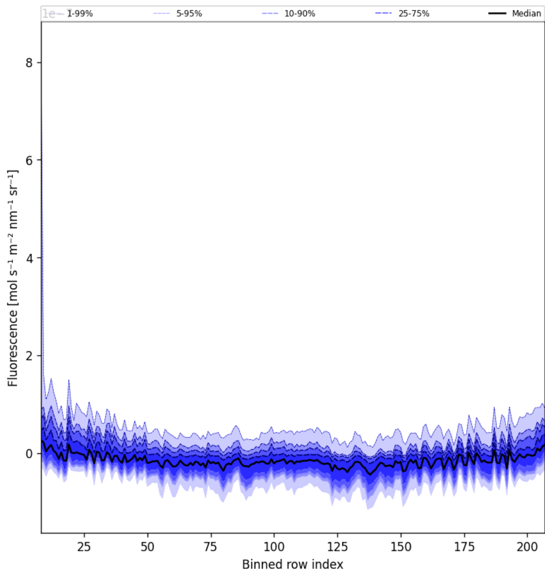
Figure 43: Along track statistics of “Fluorescence” for 2024-12-06 to 2024-12-08
