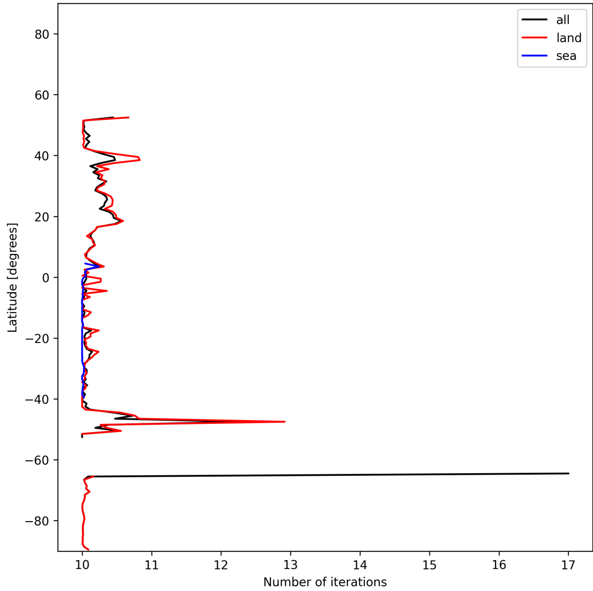
Figure 20: Zonal average of “Number of iterations” for 2024-12-06 to 2024-12-08.
