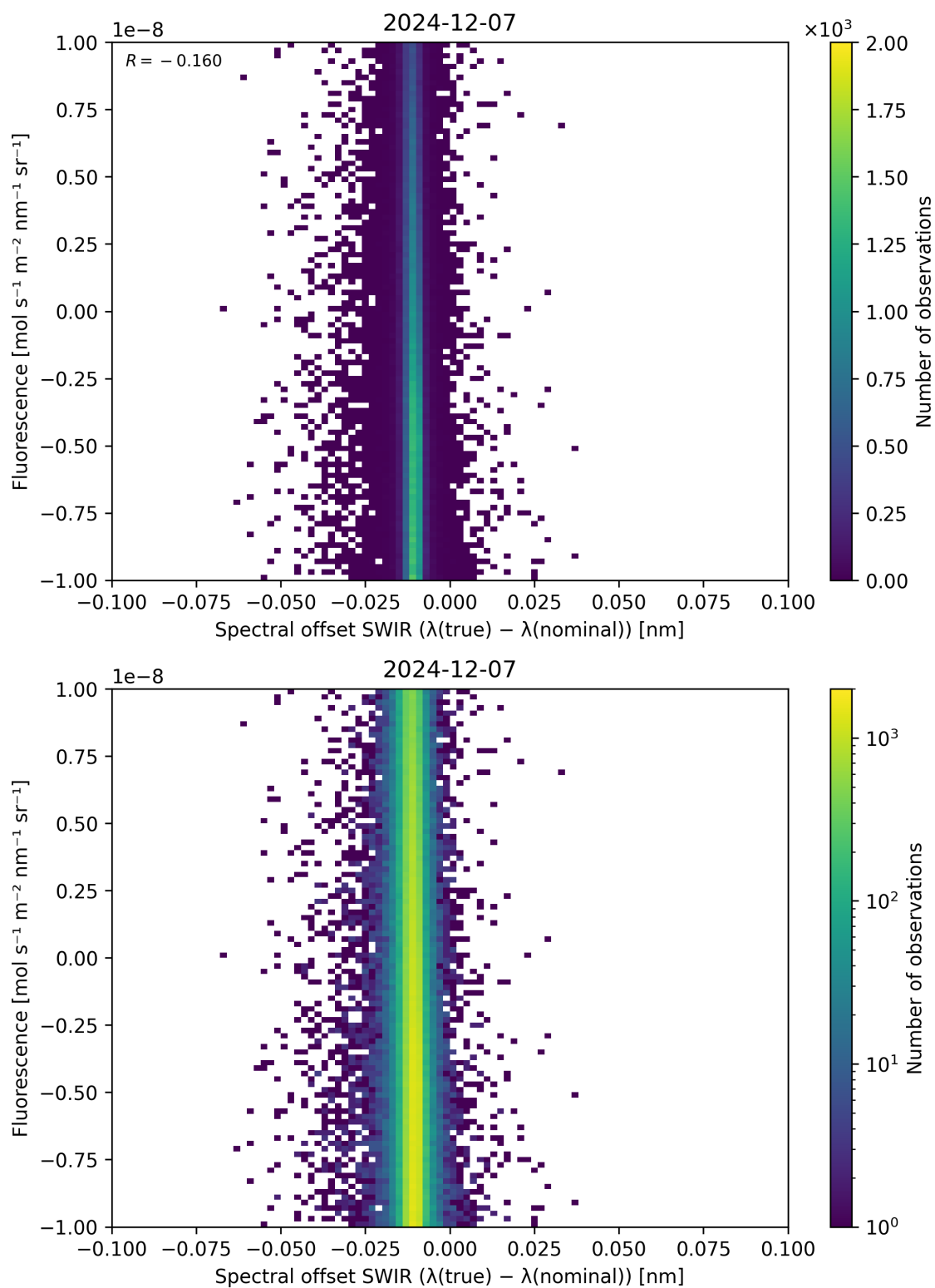
Figure 120: Scatter density plot of “Spectral offset SWIR ( \lambda_{\text{true}} - \lambda_{\text{nominal}} )” against “Fluorescence” for 2024-12-06 to 2024-12-08.
