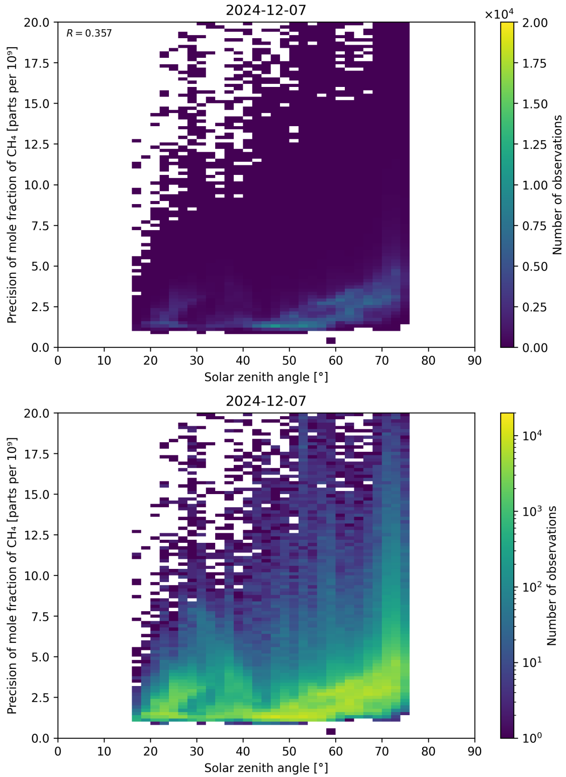
Figure 101: Scatter density plot of “Solar zenith angle” against “Precision of mole fraction of CH 4 ” for 2024-12-06 to 2024-12-08.
