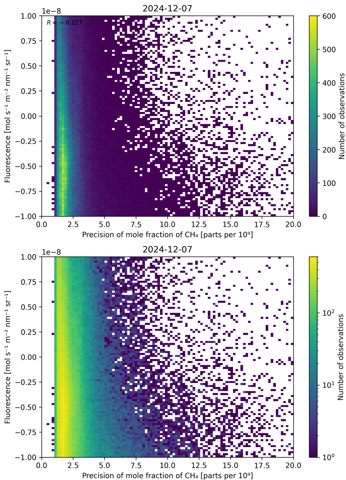
Figure 81: Scatter density plot of “Precision of mole fraction of CH 4 ” against “Fluorescence” for 2024-12-06 to 2024-12-08.
