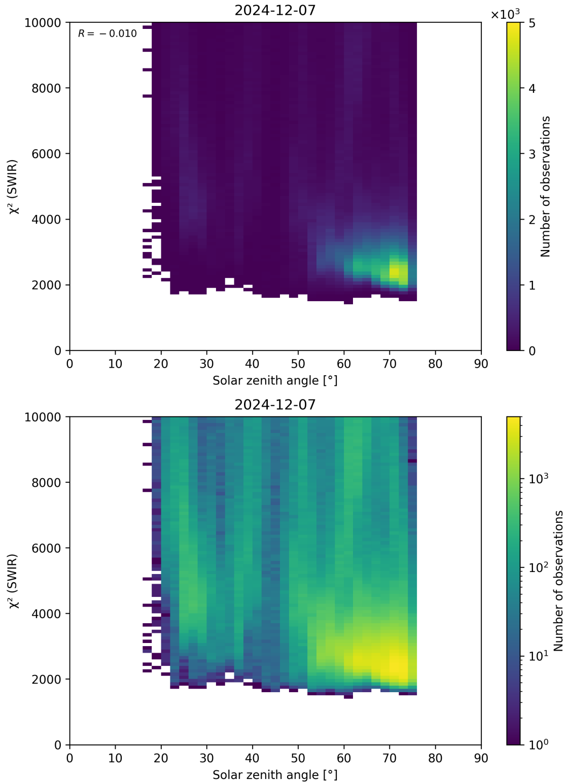
Figure 95: Scatter density plot of “Solar zenith angle” against “ \chi^2 (SWIR)” for 2024-12-06 to 2024-12-08.
