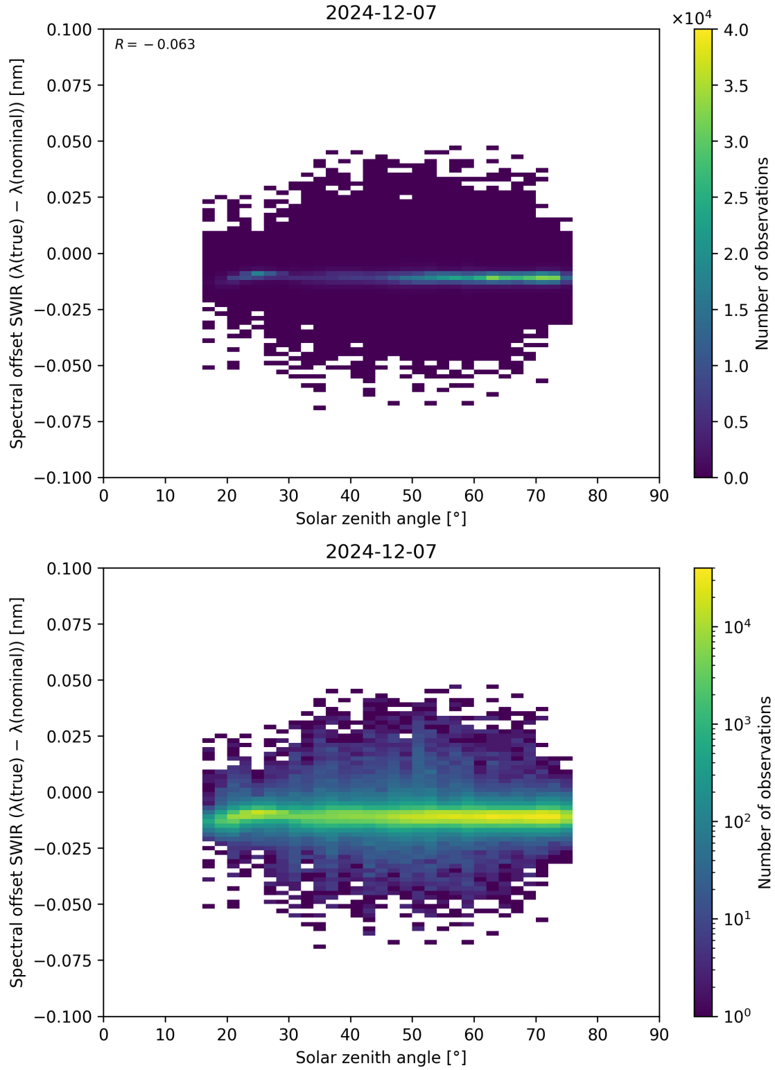
Figure 104: Scatter density plot of “Solar zenith angle” against “Spectral offset SWIR ( \lambda_{\text{true}} - \lambda_{\text{nominal}} )” for 2024-12-06 to 2024-12-08.
