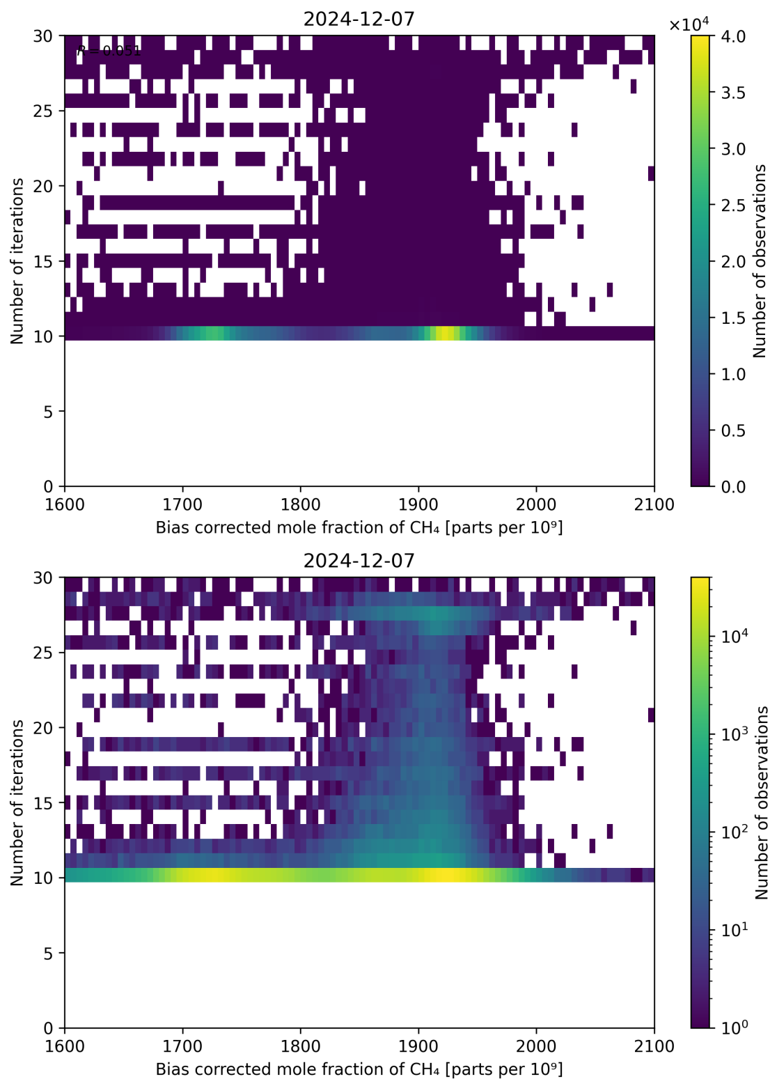
Figure 67: Scatter density plot of “Bias corrected mole fraction of CH 4 ” against “Number of iterations” for 2024-12-06 to 2024-12-08.
