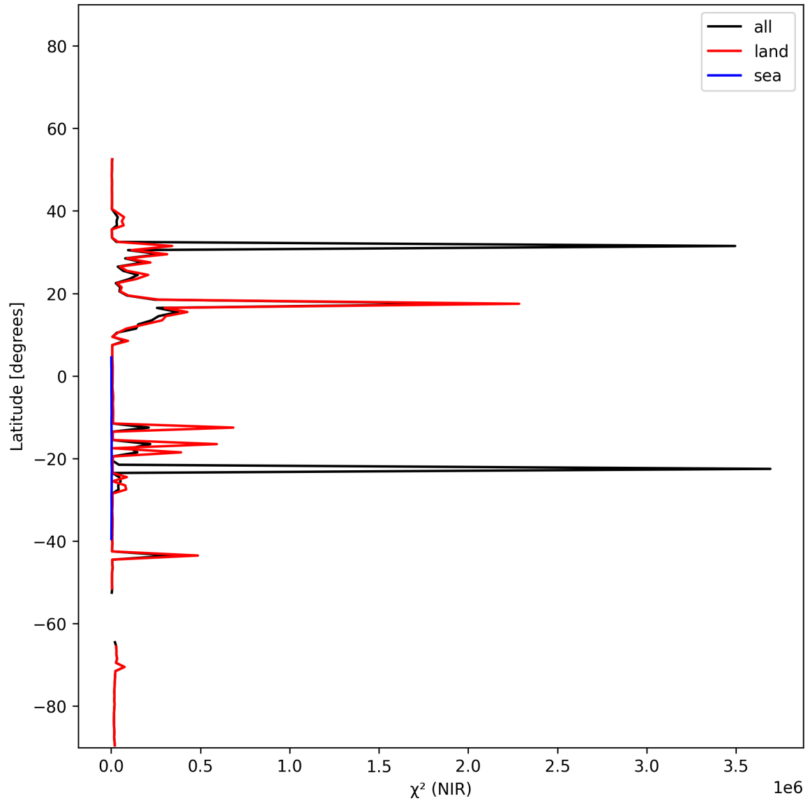
Figure 18: Zonal average of “ \chi^2 (NIR)” for 2024-12-06 to 2024-12-08.
