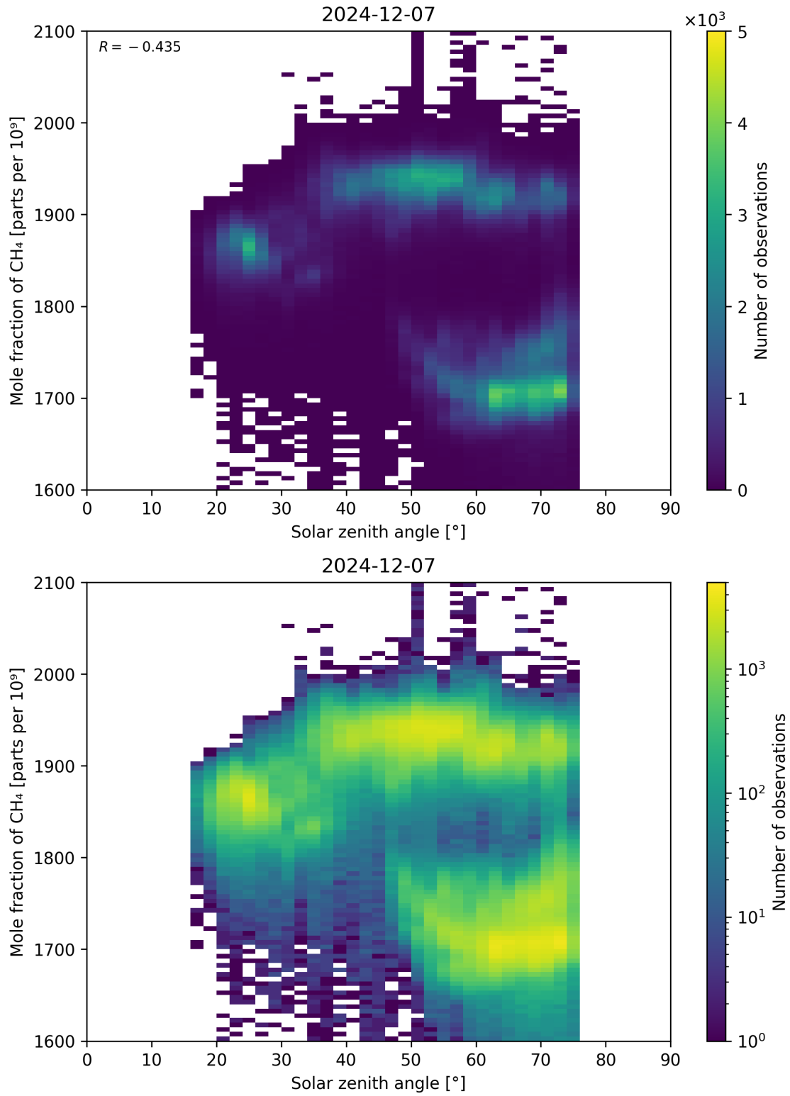
Figure 99: Scatter density plot of “Solar zenith angle” against “Mole fraction of CH 4 ” for 2024-12-06 to 2024-12-08.
