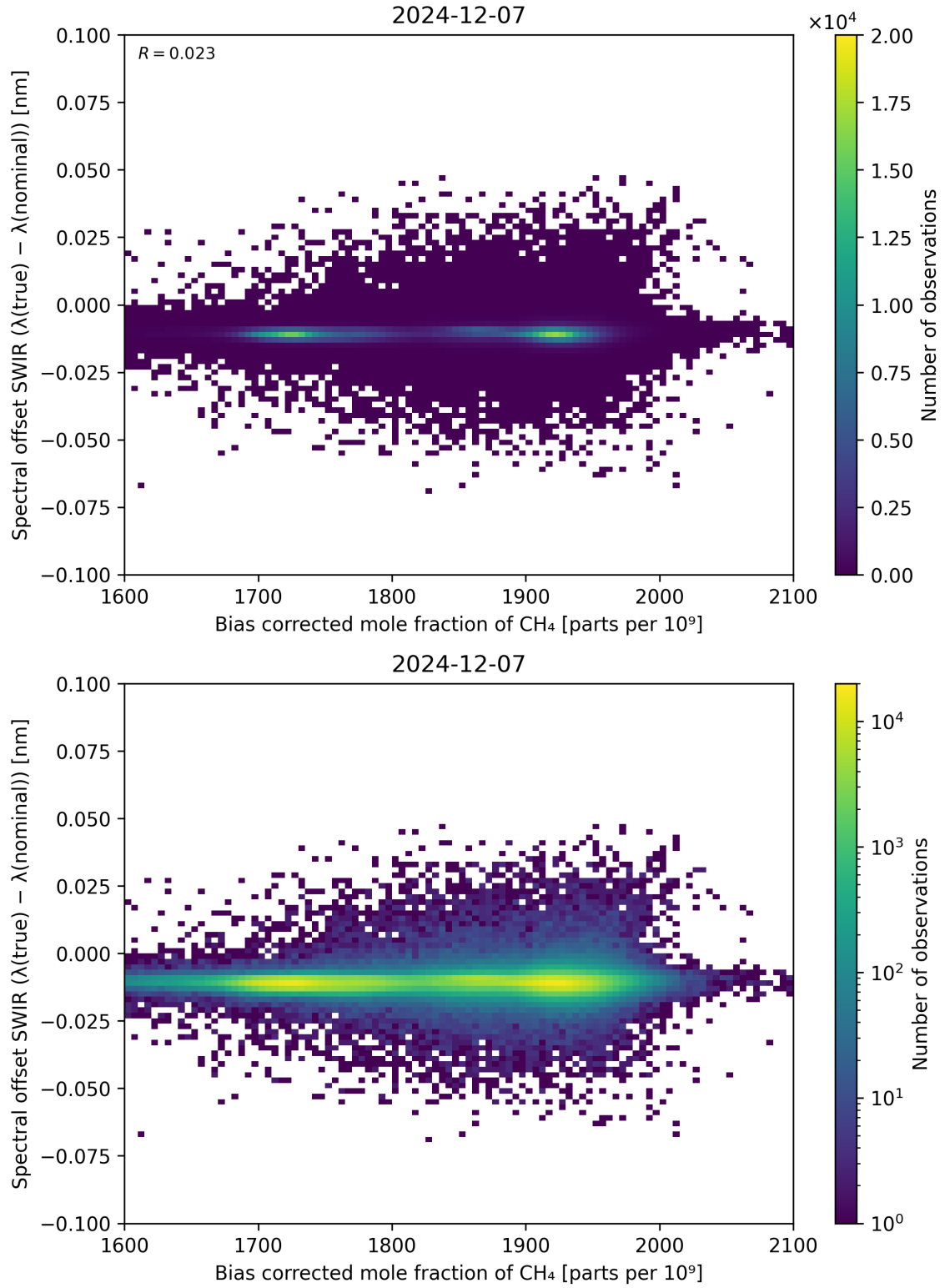
Figure 69: Scatter density plot of “Bias corrected mole fraction of \text{CH}_4 ” against “Spectral offset SWIR ( \lambda_{\text{true}} - \lambda_{\text{nominal}} )” for 2024-12-06 to 2024-12-08.
