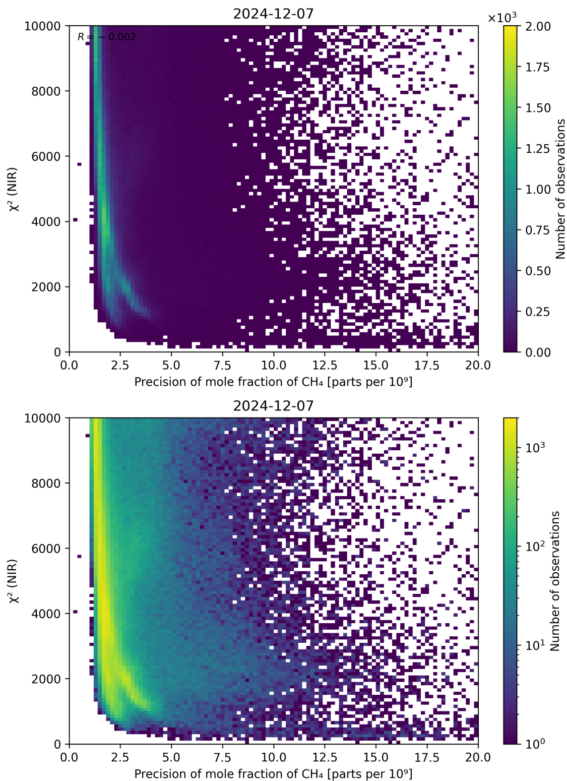
Figure 78: Scatter density plot of “Precision of mole fraction of \text{CH}_4 ” against “ \chi^2 (NIR)” for 2024-12-06 to 2024-12-08.
