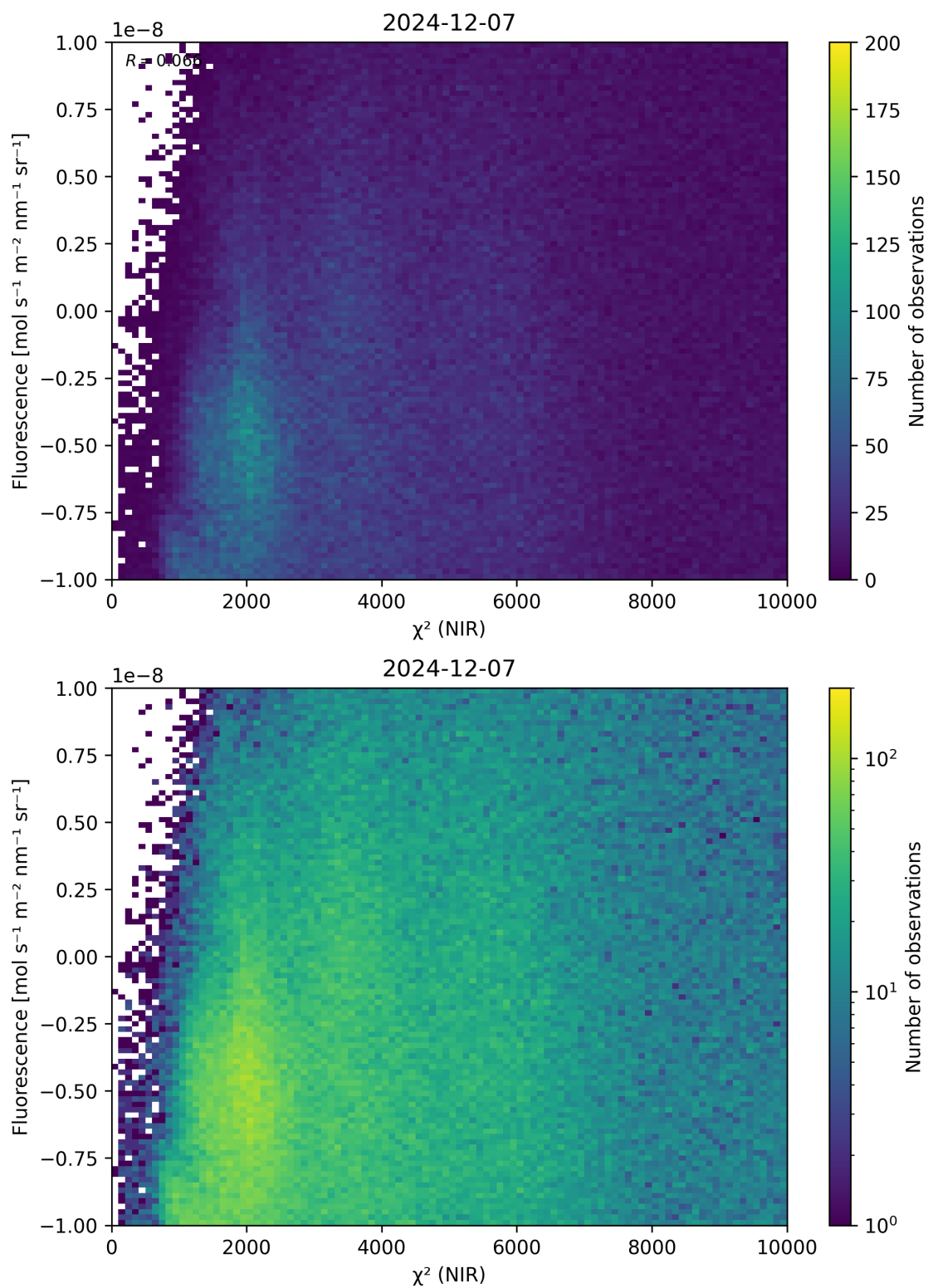
Figure 45: Scatter density plot of “ \chi^2 (NIR)” against “Fluorescence” for 2024-12-06 to 2024-12-08.
