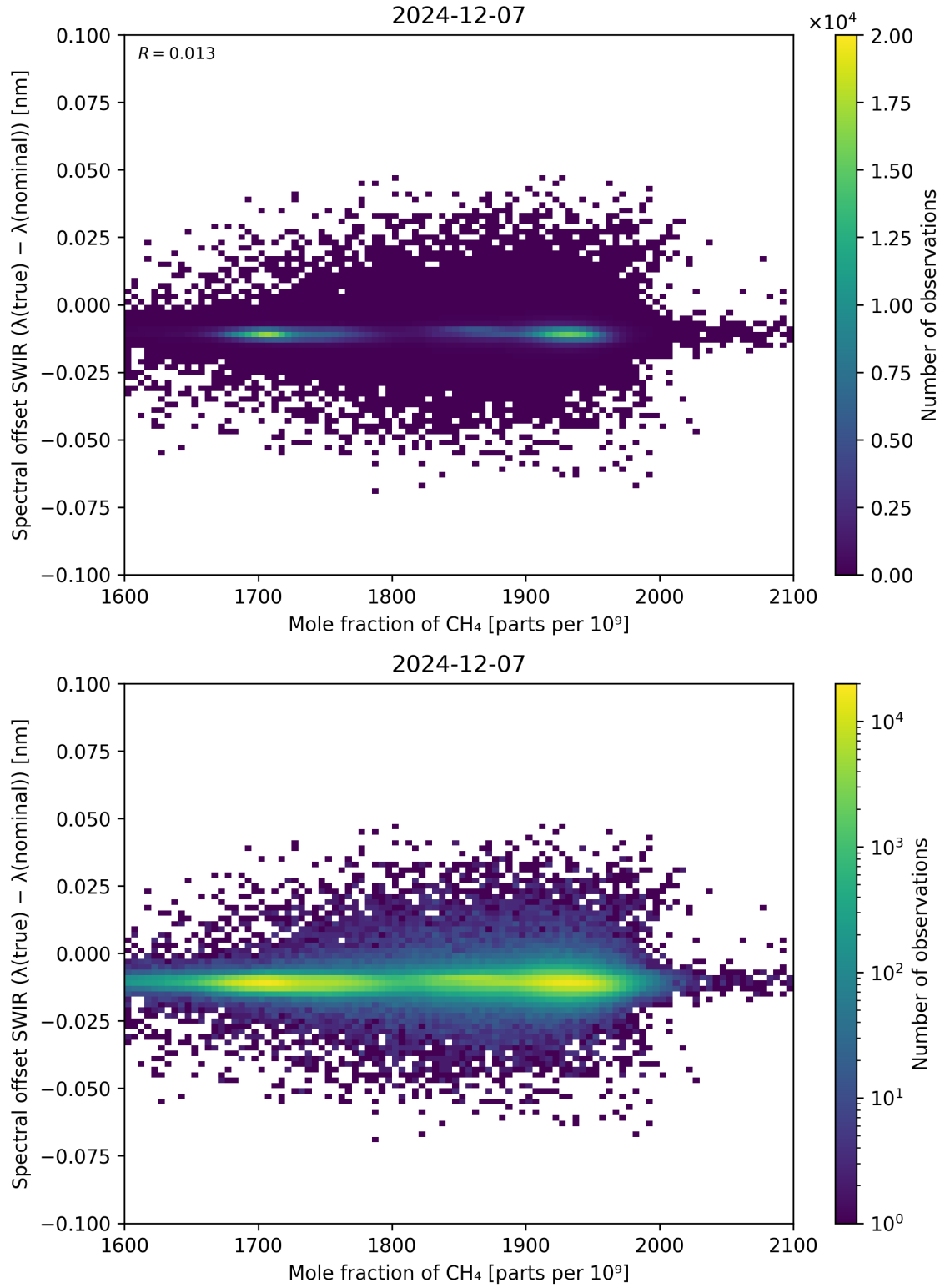
Figure 86: Scatter density plot of “Mole fraction of CH 4 ” against “Spectral offset SWIR ( \lambda_{\text{true}} - \lambda_{\text{nominal}} )” for 2024-12-06 to 2024-12-08.
