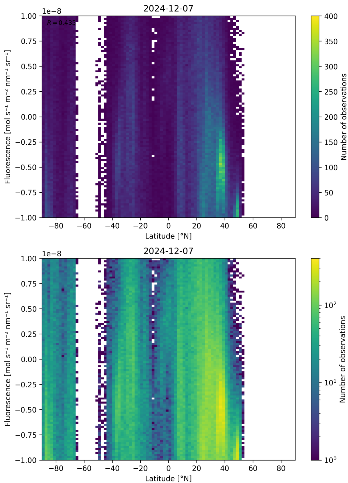
Figure 56: Scatter density plot of “Latitude” against “Fluorescence” for 2024-12-06 to 2024-12-08.
