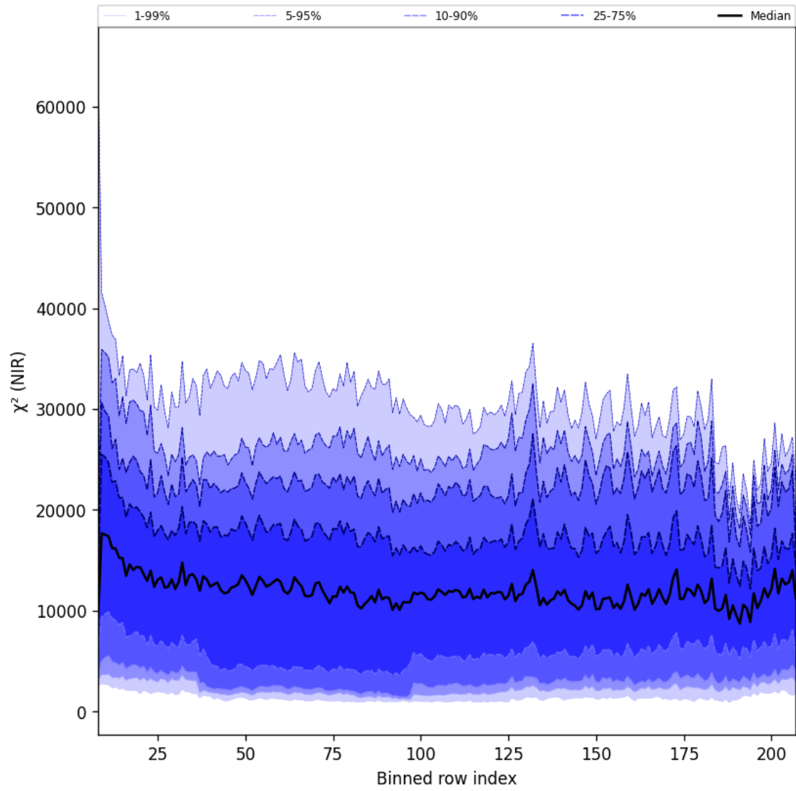
Figure 40: Along track statistics of “ \chi^2 (NIR)” for 2024-12-06 to 2024-12-08
