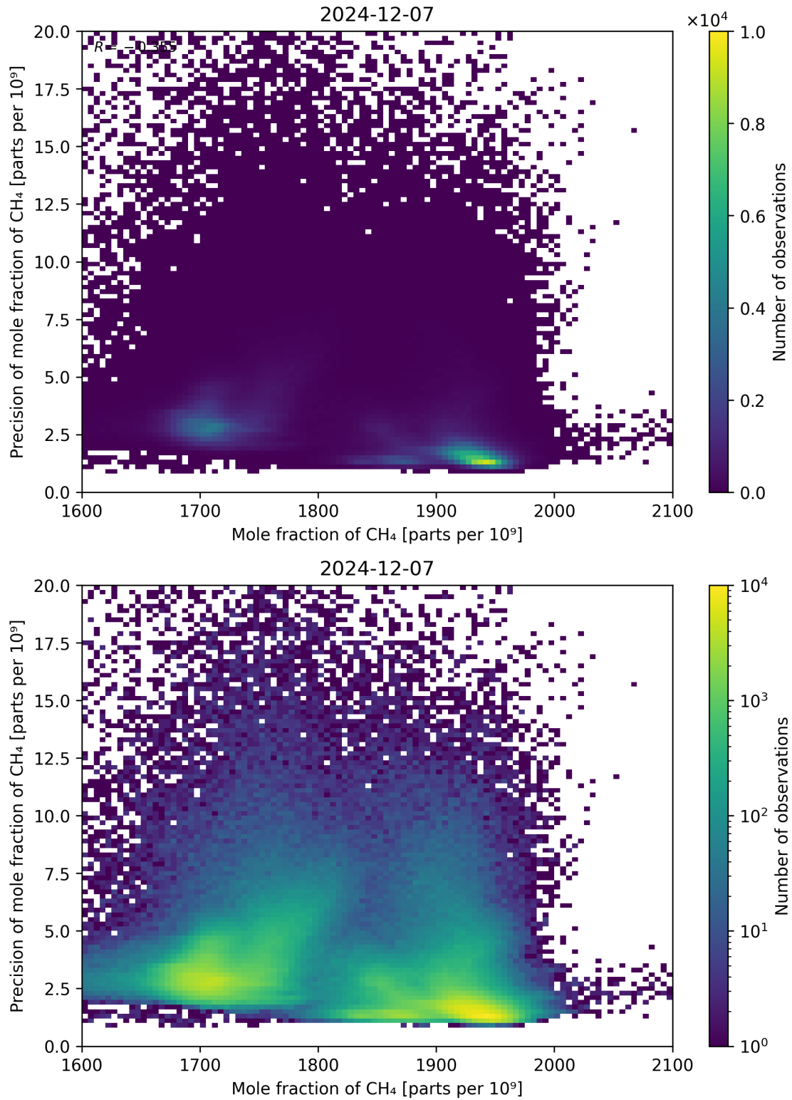
Figure 75: Scatter density plot of “Mole fraction of CH 4 ” against “Precision of mole fraction of CH 4 ” for 2024-12-06 to 2024-12-08.
