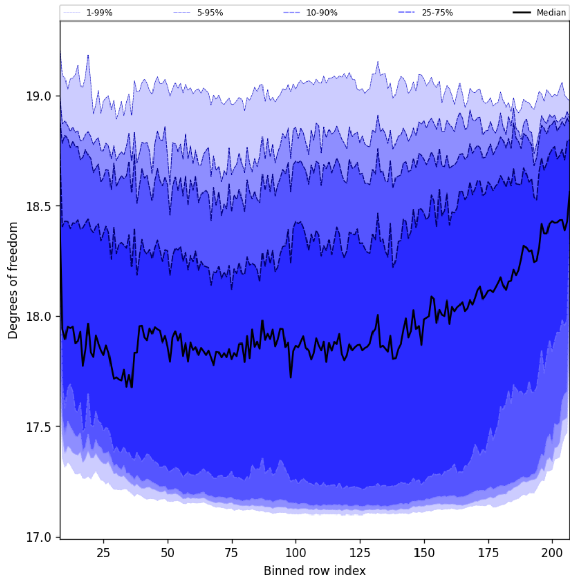
Figure 41: Along track statistics of “Degrees of freedom” for 2024-12-06 to 2024-12-08
