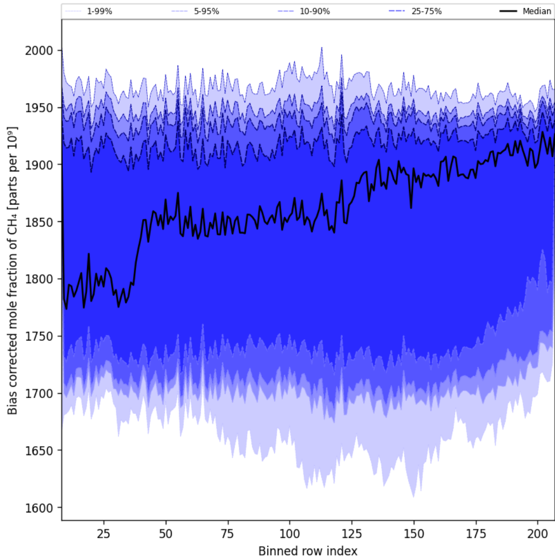
Figure 36: Along track statistics of “Bias corrected mole fraction of CH 4 ” for 2024-12-06 to 2024-12-08
