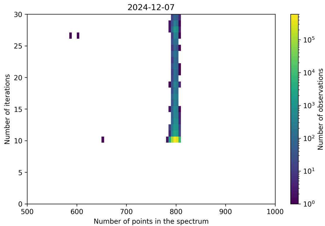
Figure 92: Scatter density plot of “Number of points in the spectrum” against “Number of iterations” for 2024-12-06 to 2024-12-08.
