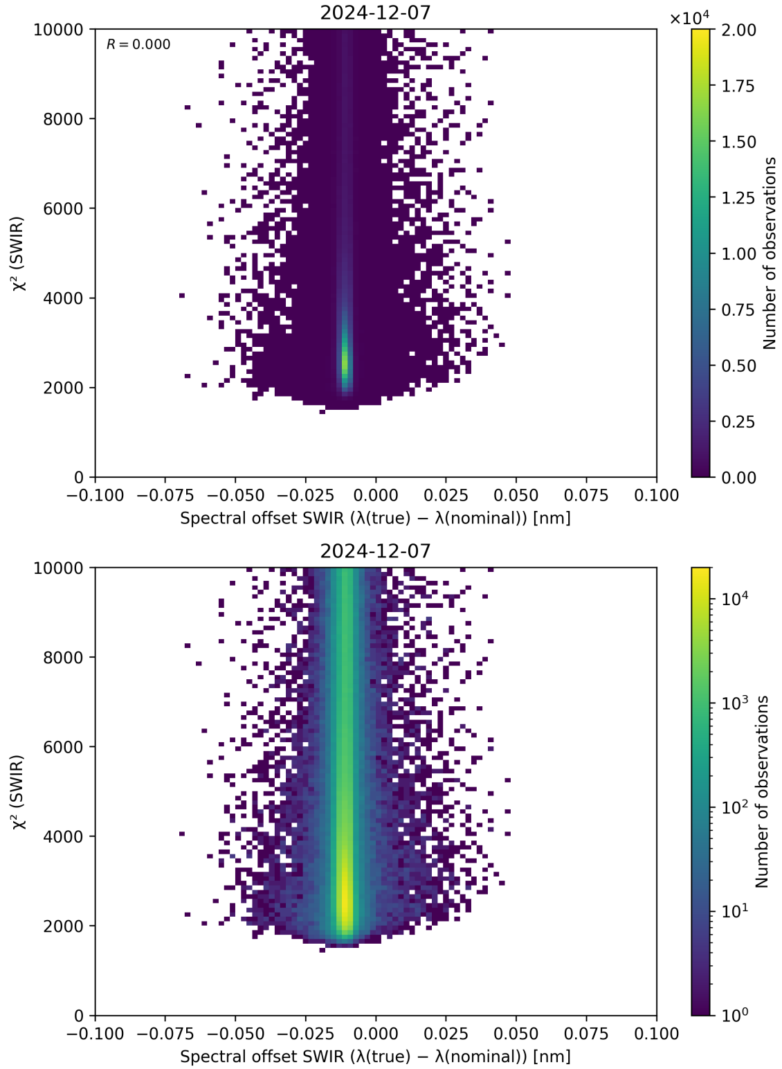
Figure 118: Scatter density plot of “Spectral offset SWIR ( \lambda_{\text{true}} - \lambda_{\text{nominal}} )” against “ \chi^2 (SWIR)” for 2024-12-06 to 2024-12-08.
