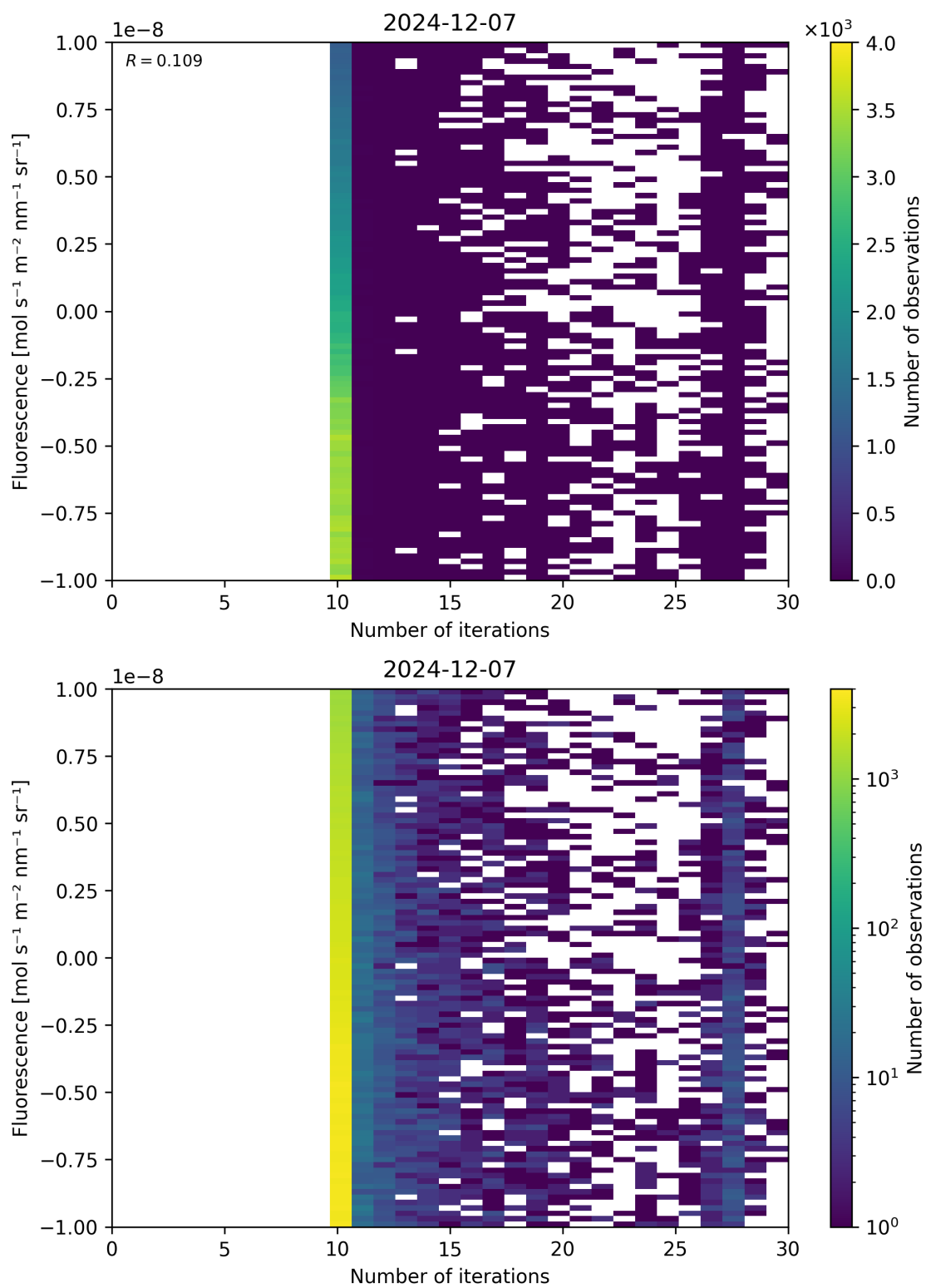
Figure 87: Scatter density plot of “Number of iterations” against “Fluorescence” for 2024-12-06 to 2024-12-08.
