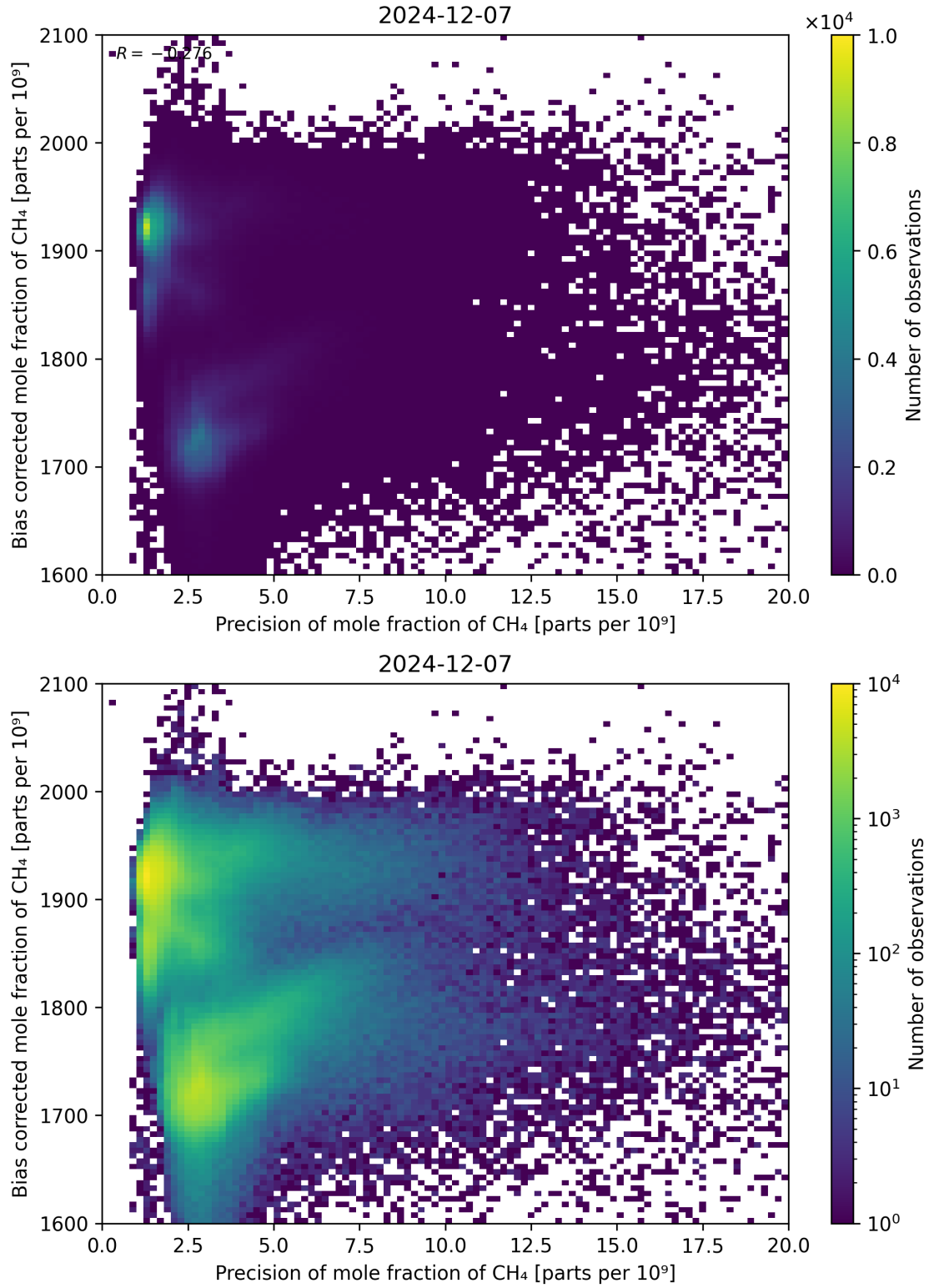
Figure 82: Scatter density plot of “Precision of mole fraction of CH 4 ” against “Bias corrected mole fraction of CH 4 ” for 2024-12-06 to 2024-12-08.
