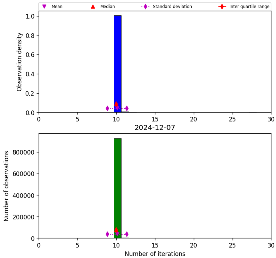
Figure 31: Histogram of “Number of iterations” for 2024-12-06 to 2024-12-08
