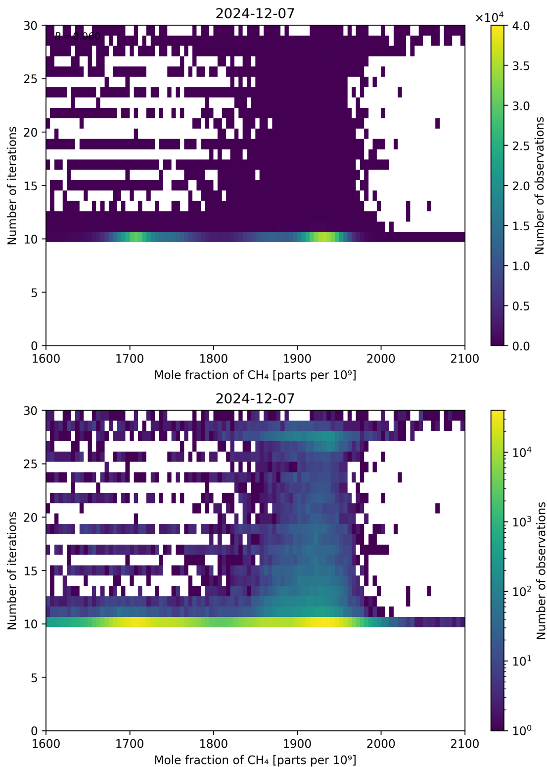
Figure 76: Scatter density plot of “Mole fraction of CH 4 ” against “Number of iterations” for 2024-12-06 to 2024-12-08.
