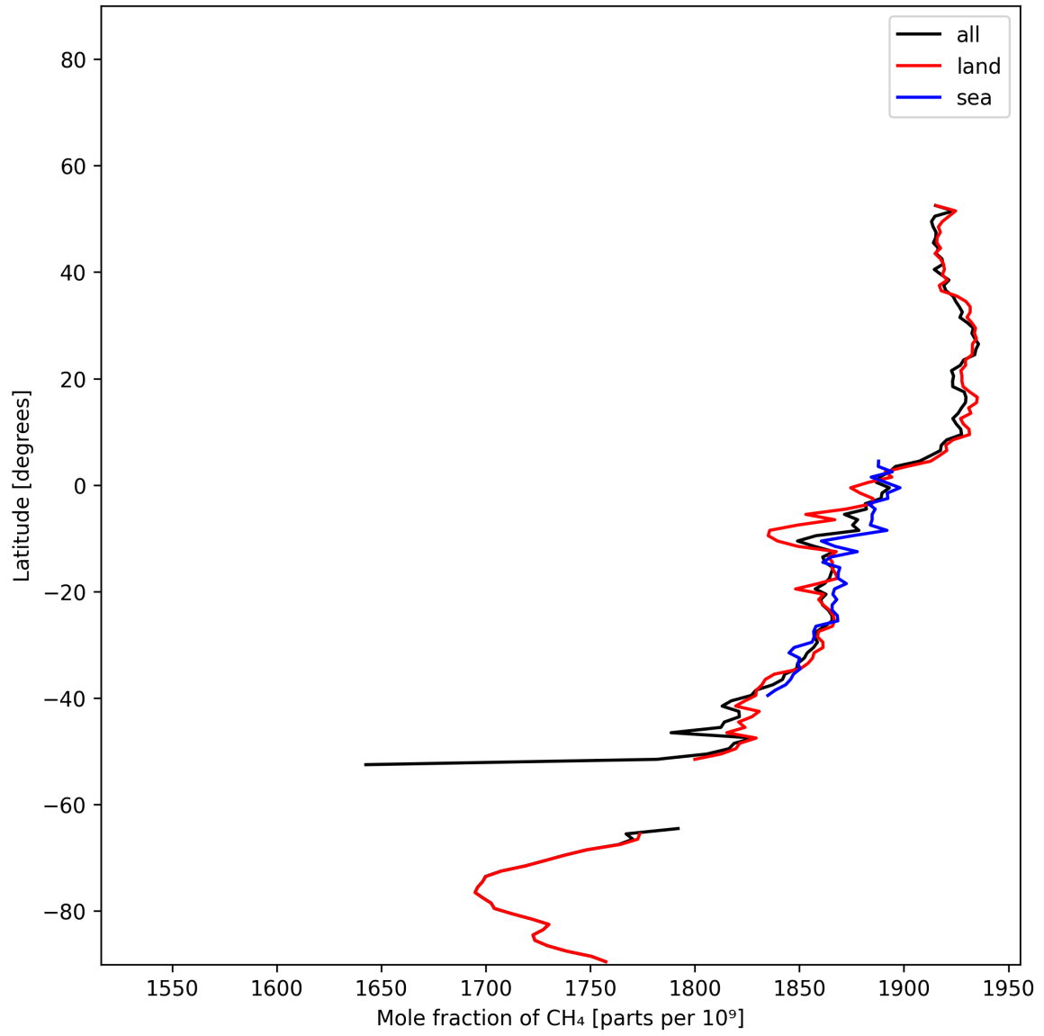
Figure 12: Zonal average of “Mole fraction of CH 4 ” for 2024-12-06 to 2024-12-08.
