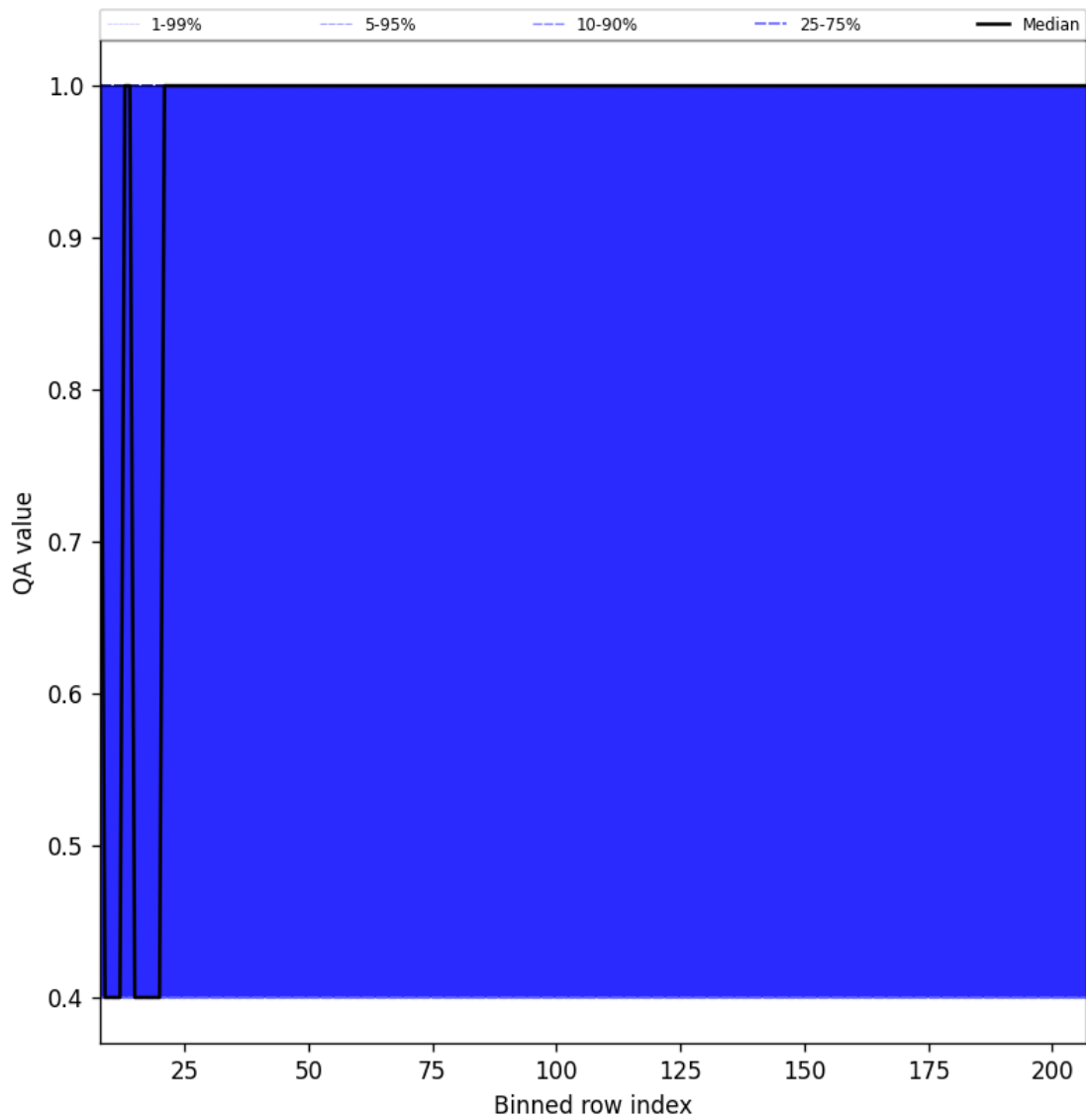
Figure 33: Along track statistics of “QA value” for 2024-12-06 to 2024-12-08
