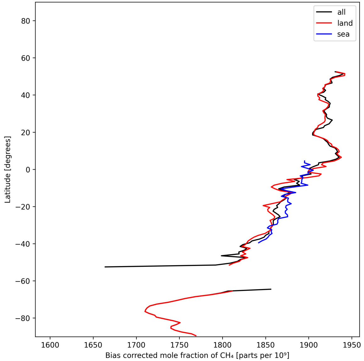
Figure 14: Zonal average of “Bias corrected mole fraction of CH 4 ” for 2024-12-06 to 2024-12-08.
