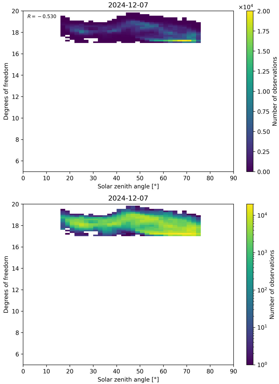
Figure 96: Scatter density plot of “Solar zenith angle” against “Degrees of freedom” for 2024-12-06 to 2024-12-08.
