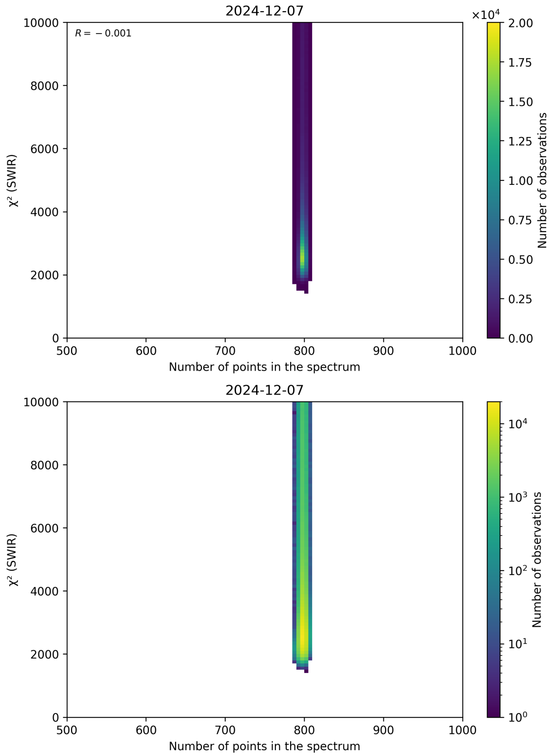
Figure 89: Scatter density plot of “Number of points in the spectrum” against “ \chi^2 (SWIR)” for 2024-12-06 to 2024-12-08.
