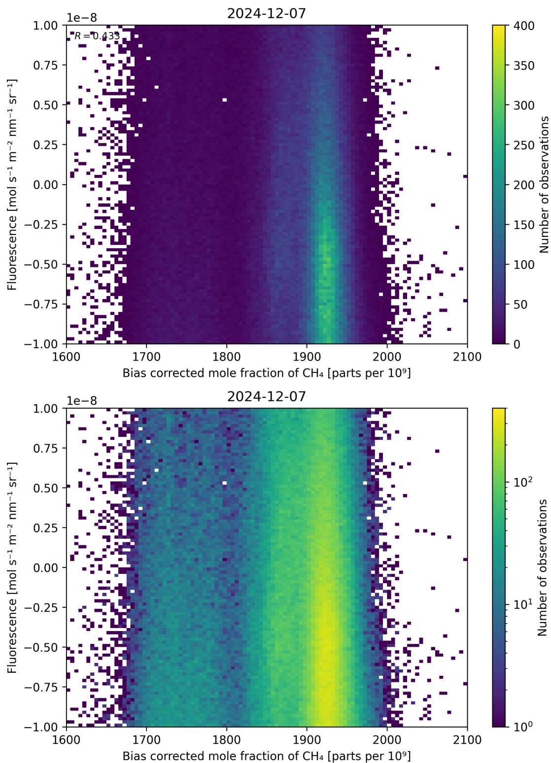
Figure 66: Scatter density plot of “Bias corrected mole fraction of \text{CH}_4 ” against “Fluorescence” for 2024-12-06 to 2024-12-08.
