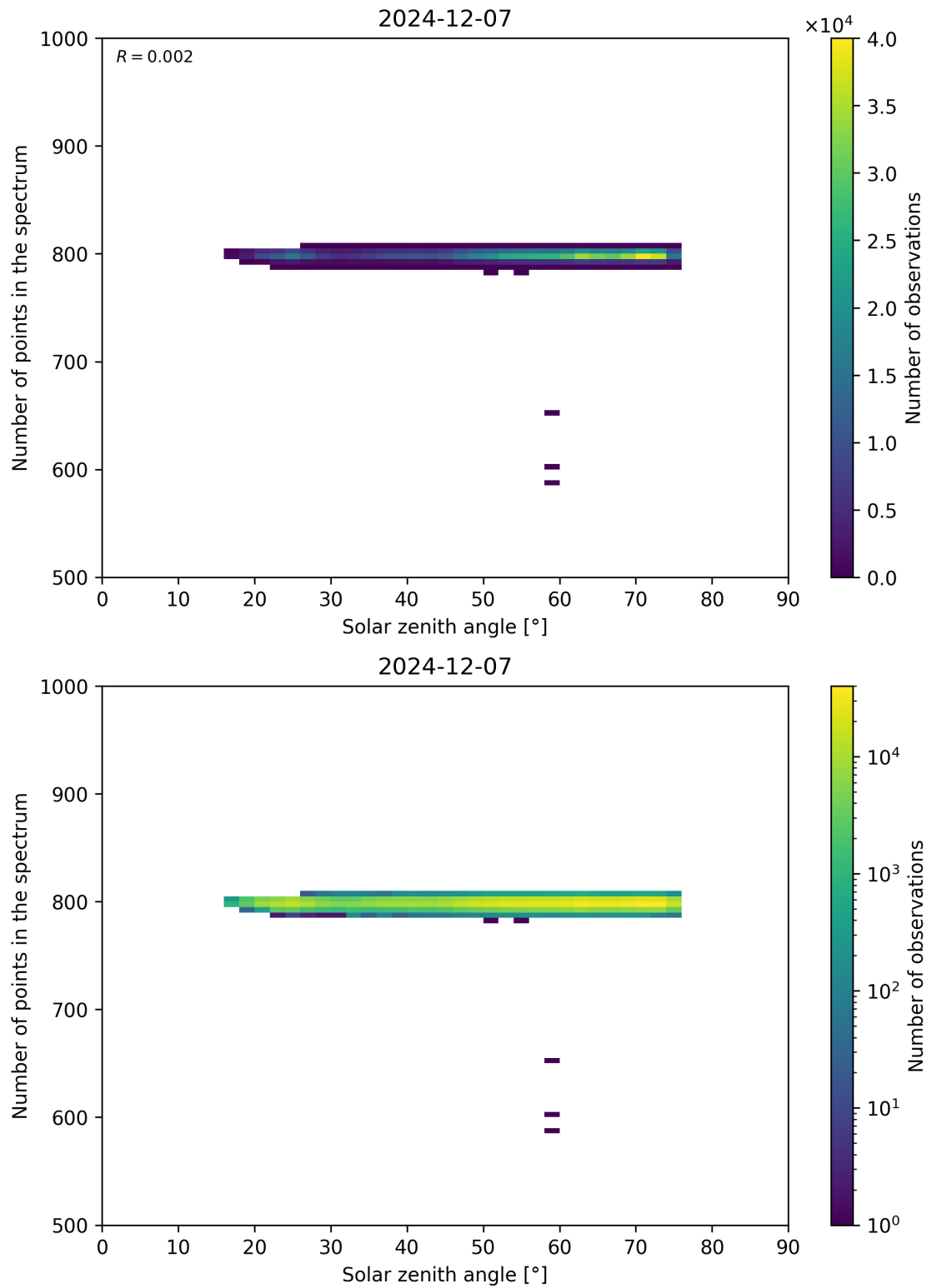
Figure 103: Scatter density plot of “Solar zenith angle” against “Number of points in the spectrum” for 2024-12-06 to 2024-12-08.
