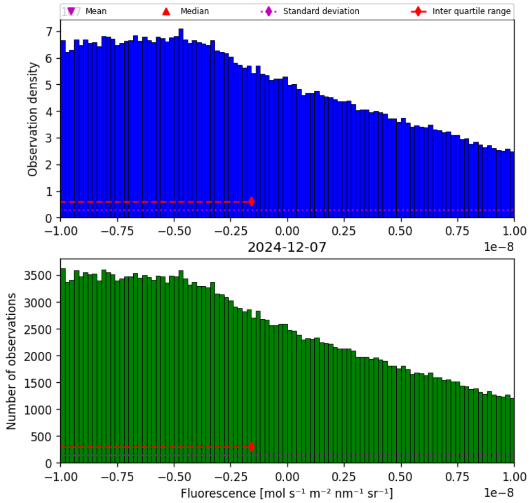
Figure 32: Histogram of “Fluorescence” for 2024-12-06 to 2024-12-08
