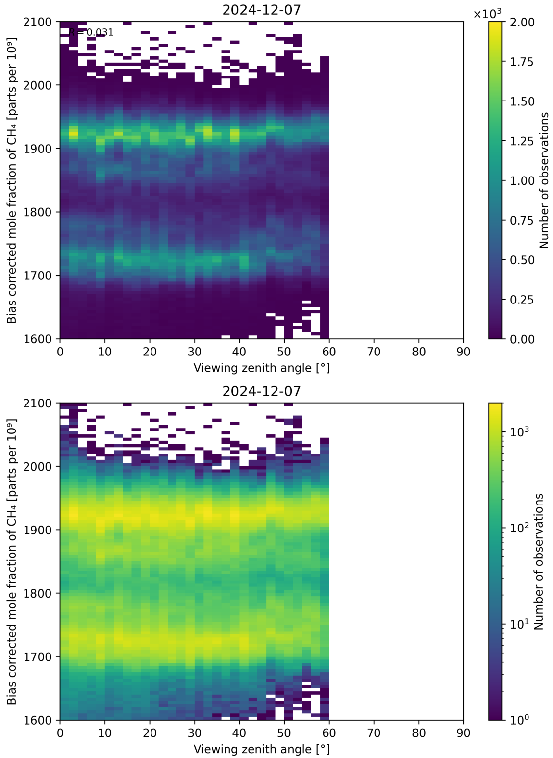
Figure 111: Scatter density plot of “Viewing zenith angle” against “Bias corrected mole fraction of CH 4 ” for 2024-12-06 to 2024-12-08.
