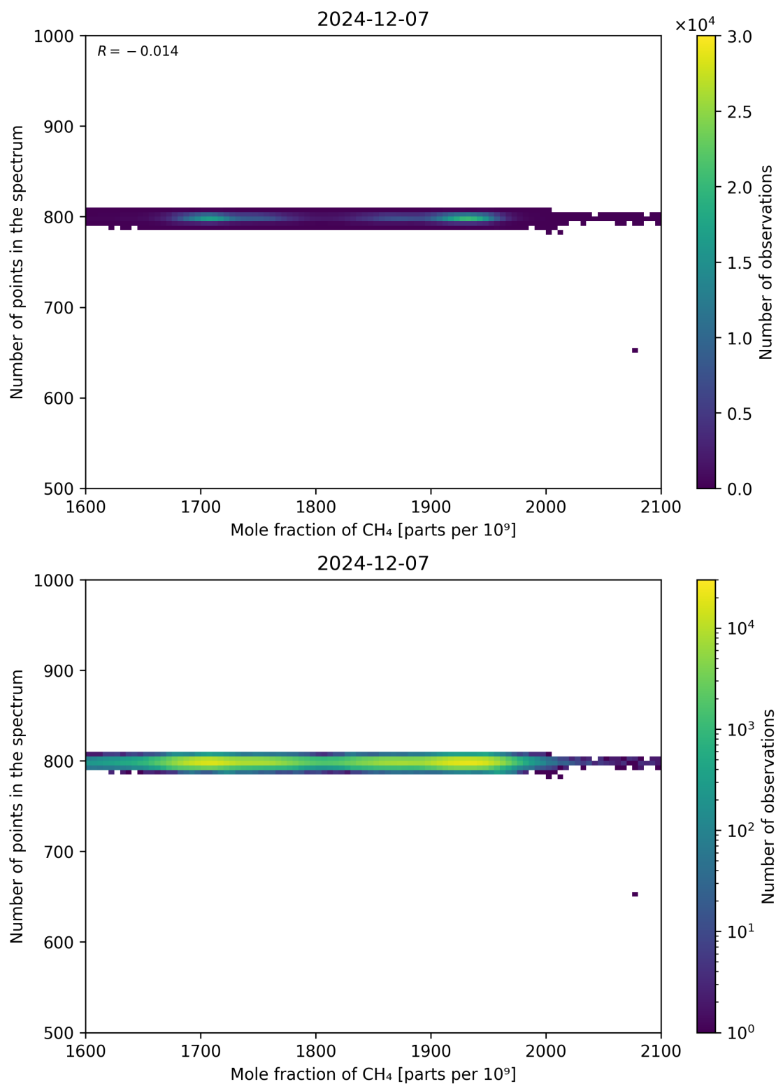
Figure 77: Scatter density plot of “Mole fraction of CH 4 ” against “Number of points in the spectrum” for 2024-12-06 to 2024-12-08.
