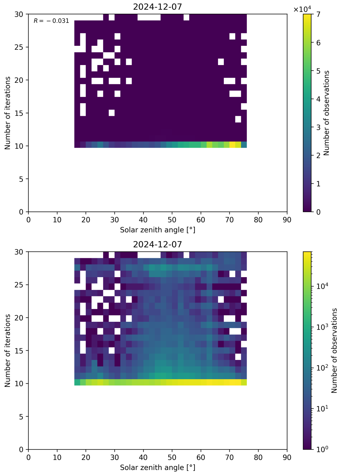
Figure 102: Scatter density plot of “Solar zenith angle” against “Number of iterations” for 2024-12-06 to 2024-12-08.
