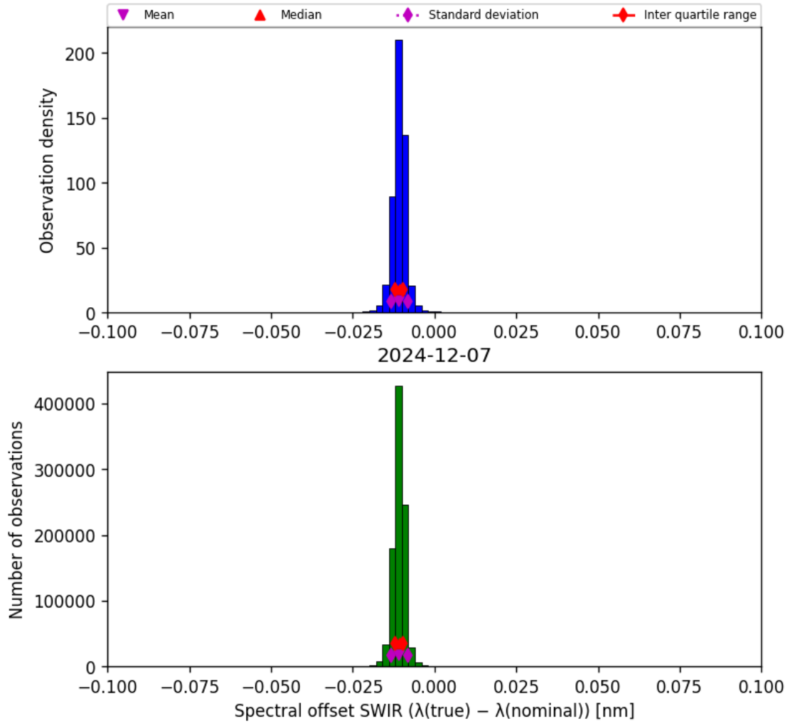
Figure 27: Histogram of “Spectral offset SWIR ( \lambda_{\text{true}} - \lambda_{\text{nominal}} )” for 2024-12-06 to 2024-12-08
