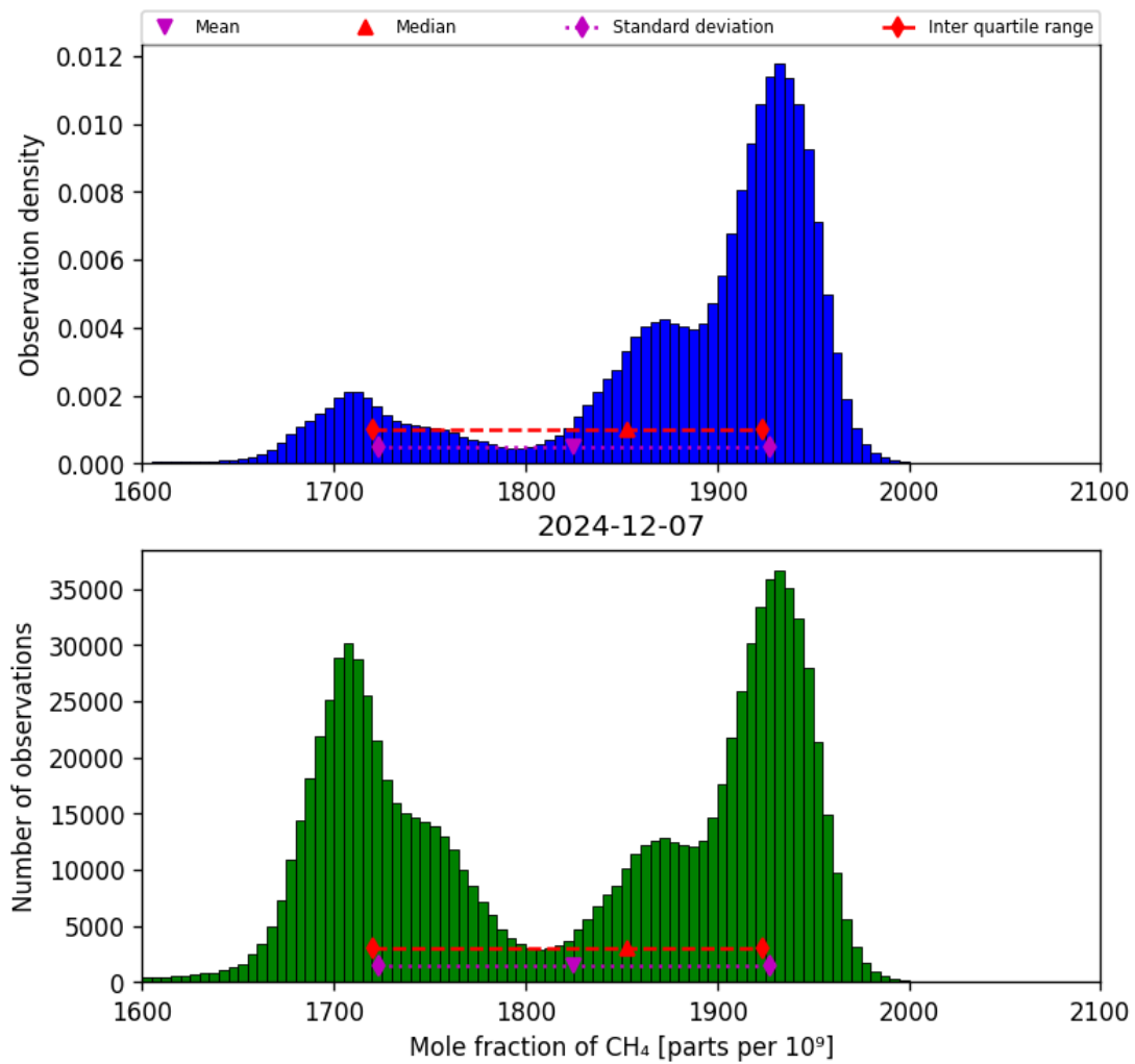
Figure 23: Histogram of “Mole fraction of CH 4 ” for 2024-12-06 to 2024-12-08
