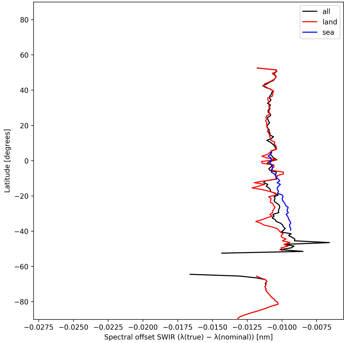
Figure 16: Zonal average of “Spectral offset SWIR ( \lambda_{\text{true}} - \lambda_{\text{nominal}} )” for 2024-12-06 to 2024-12-08.
