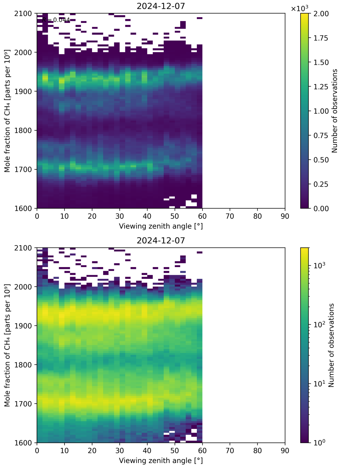
Figure 110: Scatter density plot of “Viewing zenith angle” against “Mole fraction of CH 4 ” for 2024-12-06 to 2024-12-08.
