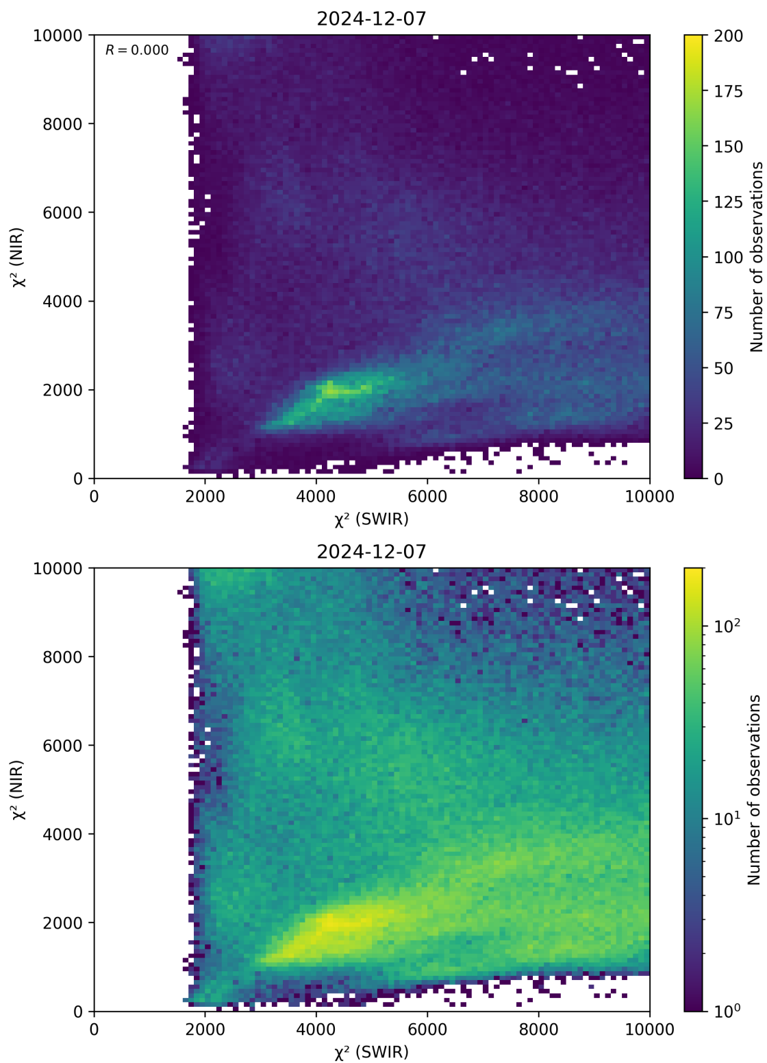
Figure 47: Scatter density plot of “ \chi^2 (SWIR)” against “ \chi^2 (NIR)” for 2024-12-06 to 2024-12-08.
