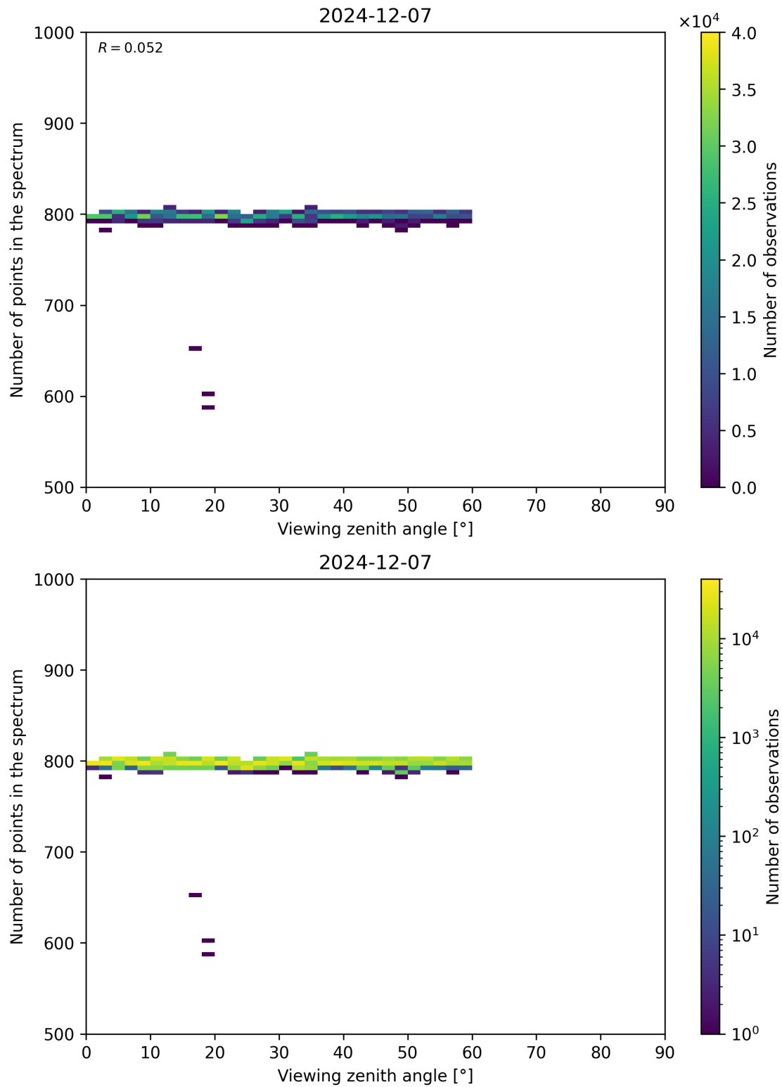
Figure 114: Scatter density plot of “Viewing zenith angle” against “Number of points in the spectrum” for 2024-12-06 to 2024-12-08.
