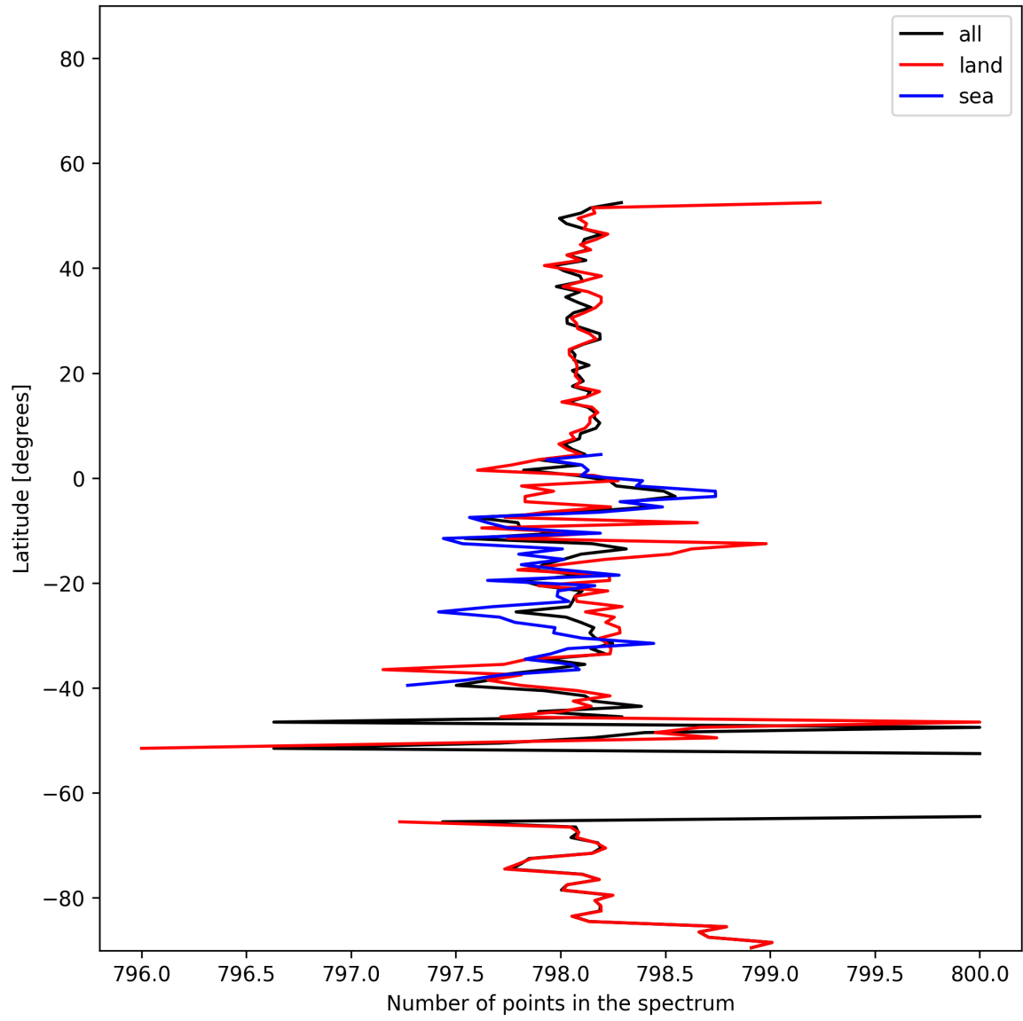
Figure 15: Zonal average of “Number of points in the spectrum” for 2024-12-06 to 2024-12-08.
