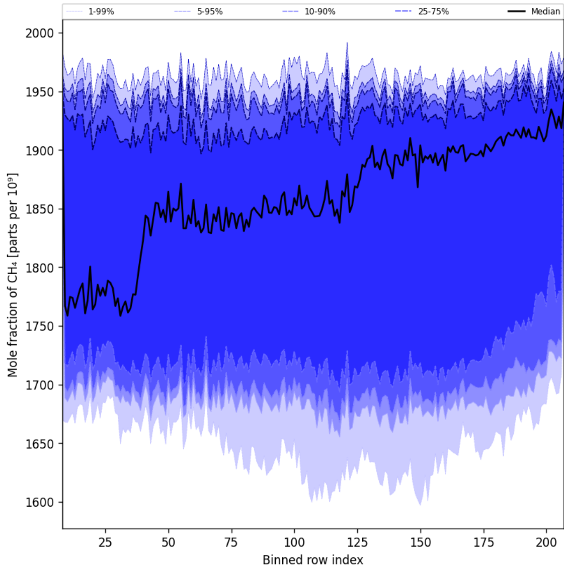
Figure 34: Along track statistics of “Mole fraction of CH 4 ” for 2024-12-06 to 2024-12-08
