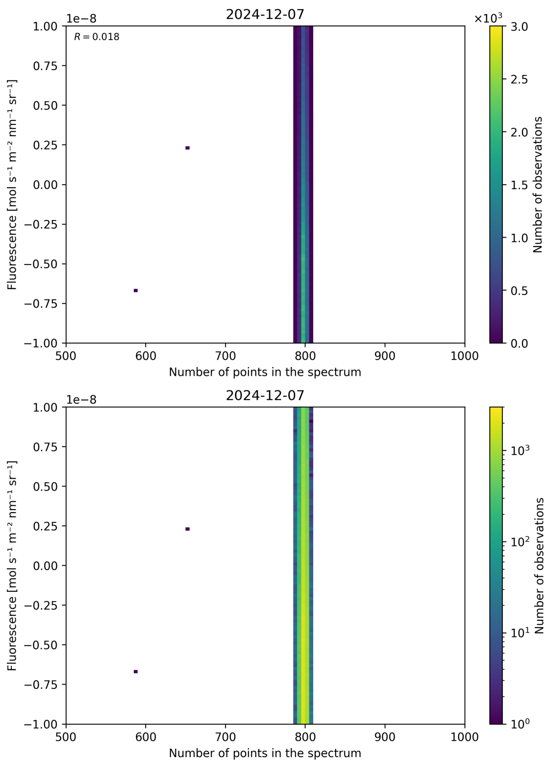
Figure 91: Scatter density plot of “Number of points in the spectrum” against “Fluorescence” for 2024-12-06 to 2024-12-08.
