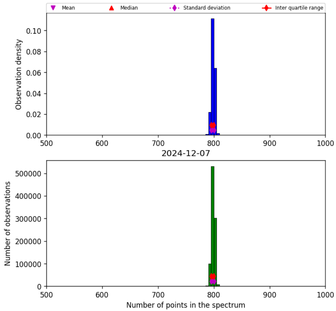
Figure 26: Histogram of “Number of points in the spectrum” for 2024-12-06 to 2024-12-08
