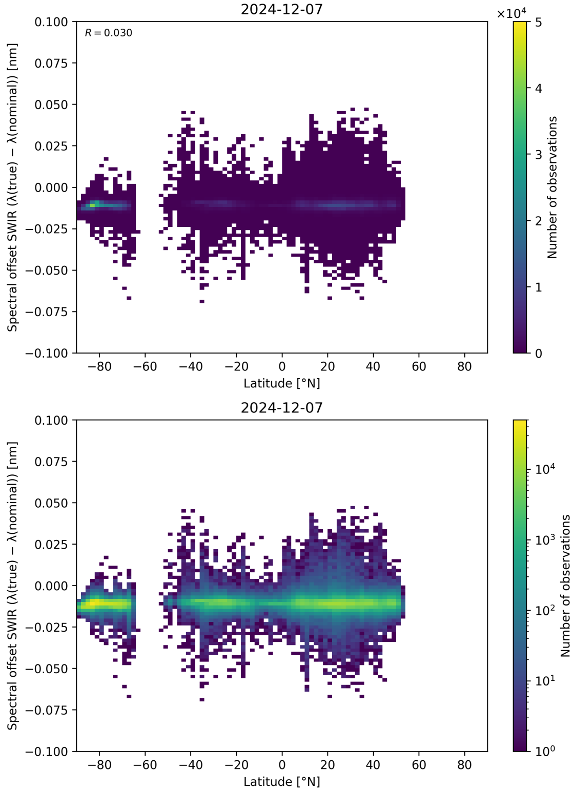
Figure 62: Scatter density plot of “Latitude” against “Spectral offset SWIR ( \lambda_{\text{true}} - \lambda_{\text{nominal}} )” for 2024-12-06 to 2024-12-08.
