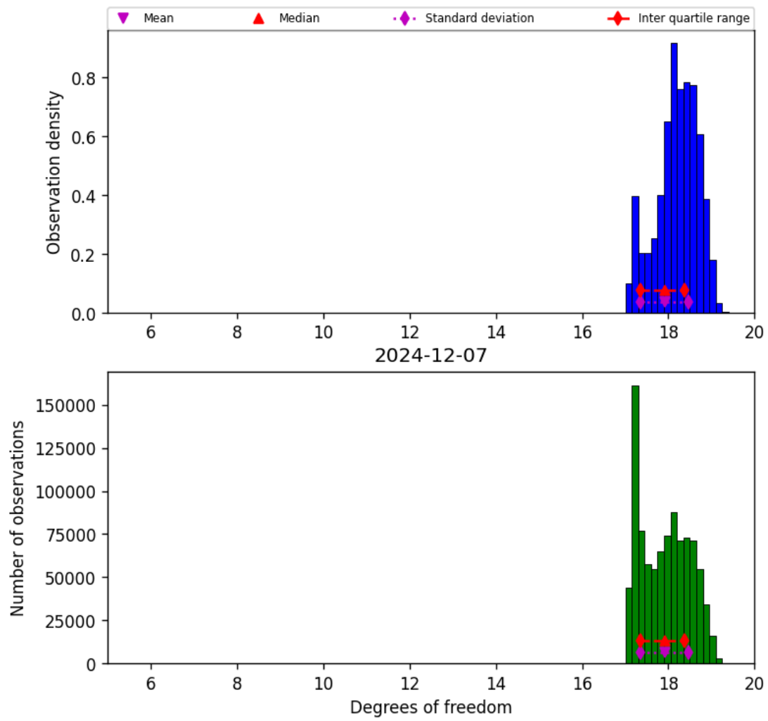
Figure 30: Histogram of “Degrees of freedom” for 2024-12-06 to 2024-12-08
