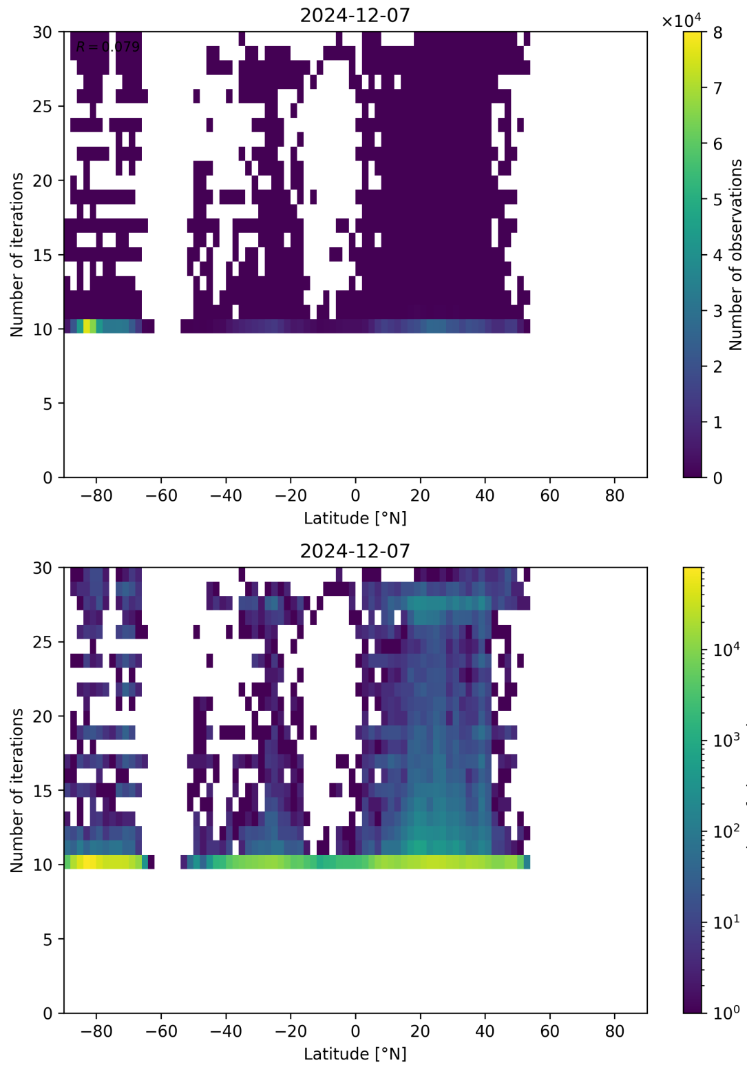
Figure 60: Scatter density plot of “Latitude” against “Number of iterations” for 2024-12-06 to 2024-12-08.
