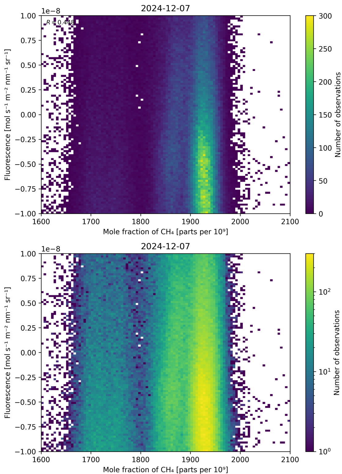
Figure 73: Scatter density plot of “Mole fraction of \text{CH}_4 ” against “Fluorescence” for 2024-12-06 to 2024-12-08.
