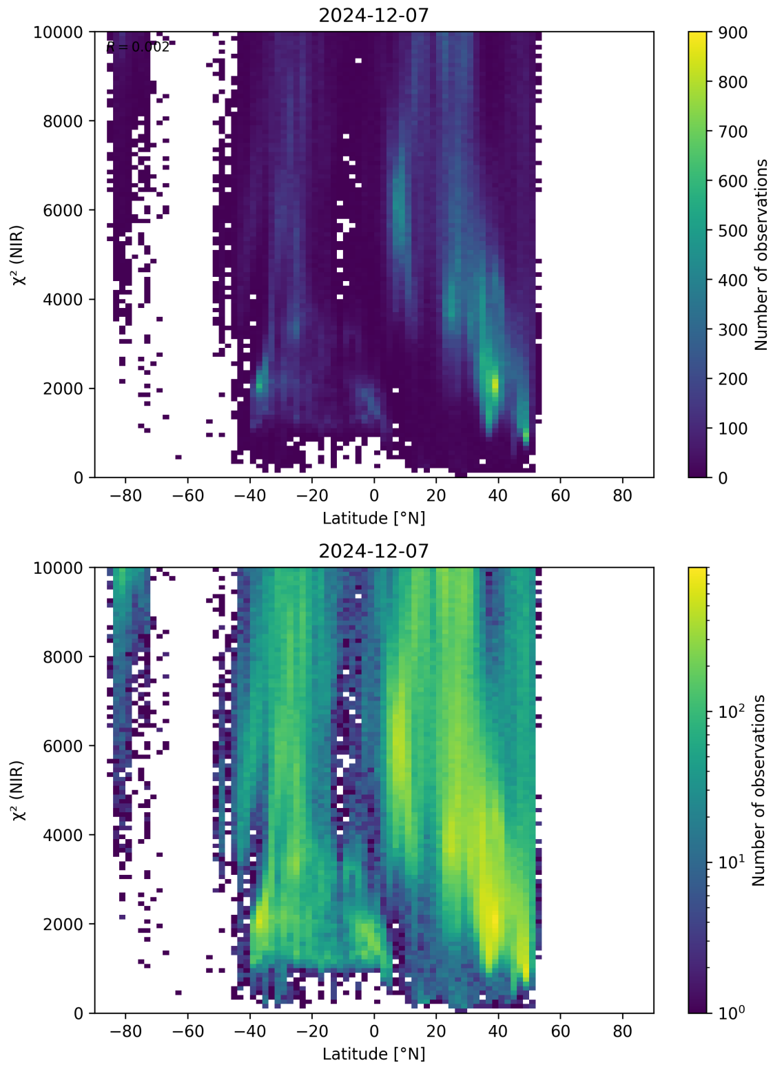
Figure 53: Scatter density plot of “Latitude” against “ \chi^2 (NIR)” for 2024-12-06 to 2024-12-08.
