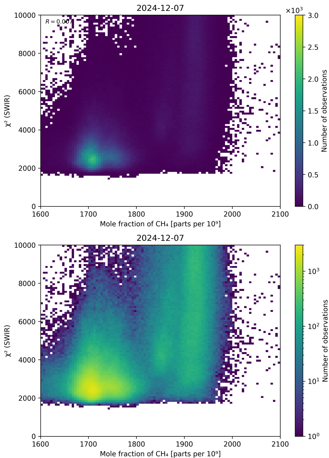
Figure 71: Scatter density plot of “Mole fraction of \text{CH}_4 ” against “ \chi^2 (SWIR)” for 2024-12-06 to 2024-12-08.
