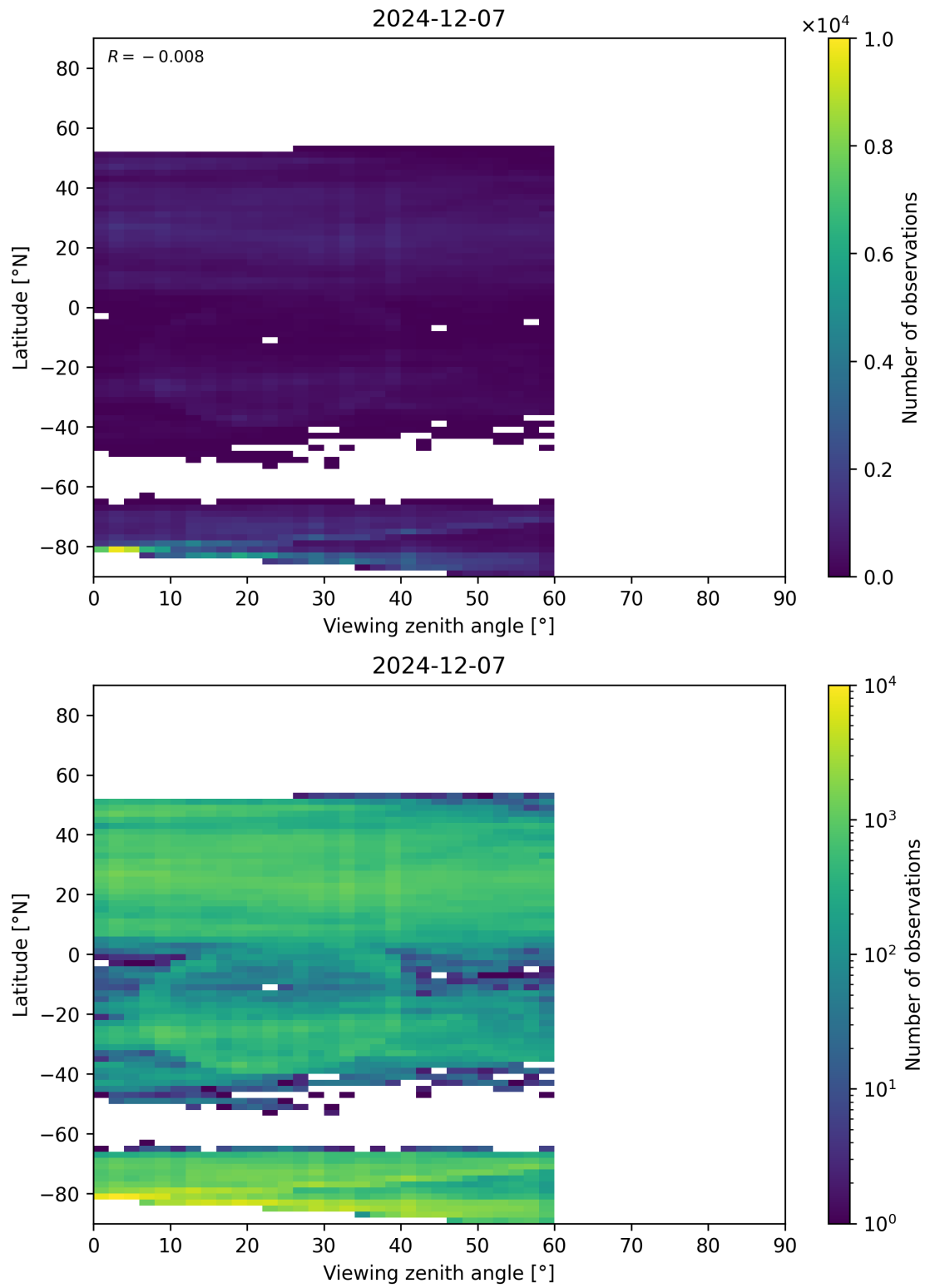
Figure 109: Scatter density plot of “Viewing zenith angle” against “Latitude” for 2024-12-06 to 2024-12-08.
