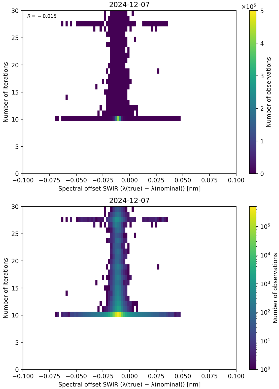
Figure 121: Scatter density plot of “Spectral offset SWIR ( \lambda_{\text{true}} - \lambda_{\text{nominal}} )” against “Number of iterations” for 2024-12-06 to 2024-12-08.
