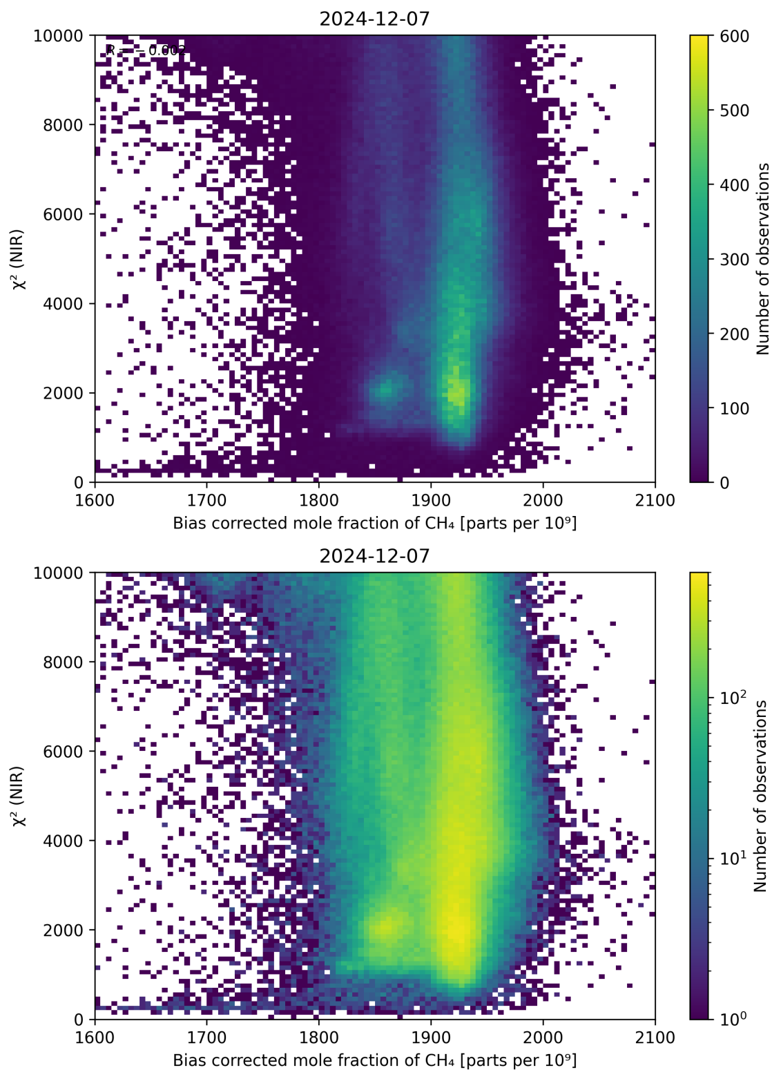
Figure 63: Scatter density plot of “Bias corrected mole fraction of \text{CH}_4 ” against “ \chi^2 (NIR)” for 2024-12-06 to 2024-12-08.
