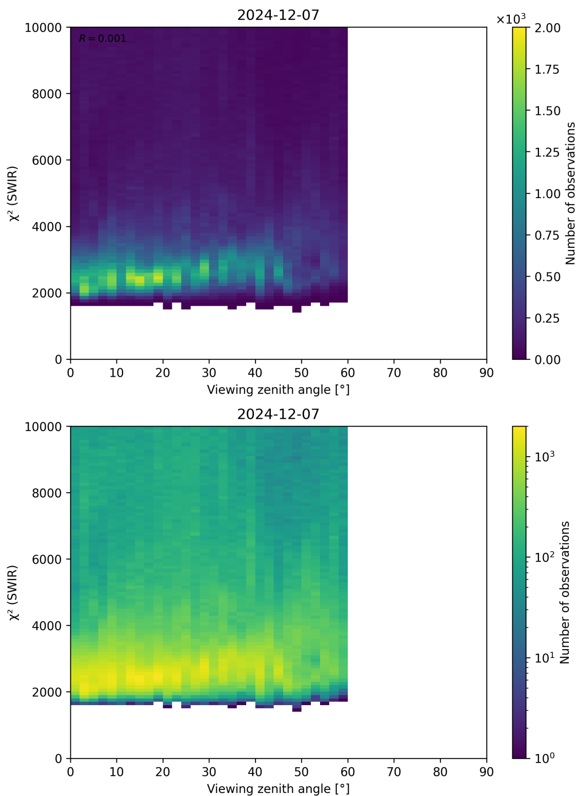
Figure 106: Scatter density plot of “Viewing zenith angle” against “ \chi^2 (SWIR)” for 2024-12-06 to 2024-12-08.
