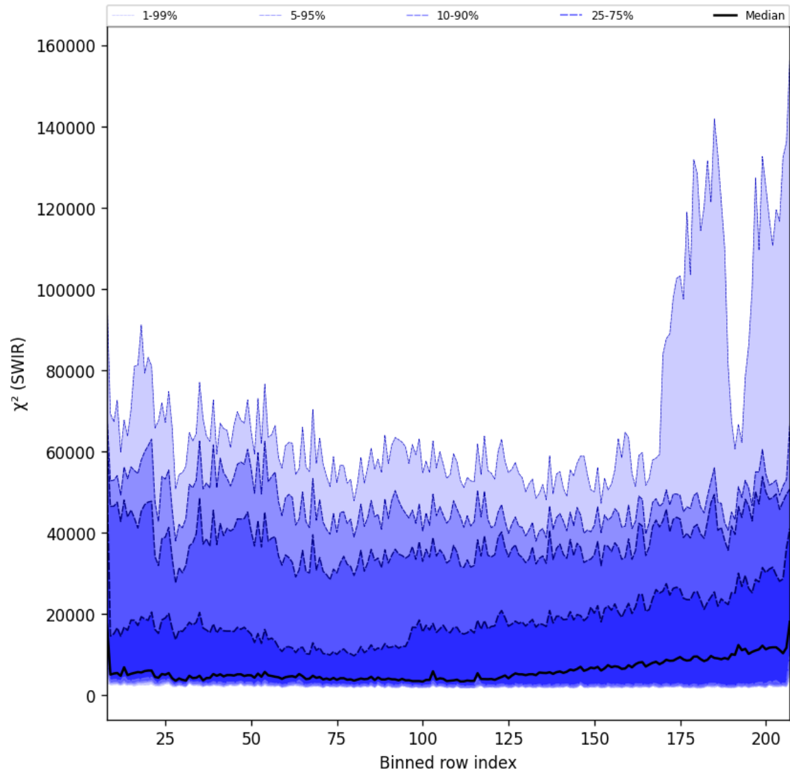
Figure 39: Along track statistics of “ \chi^2 (SWIR)” for 2024-12-06 to 2024-12-08
