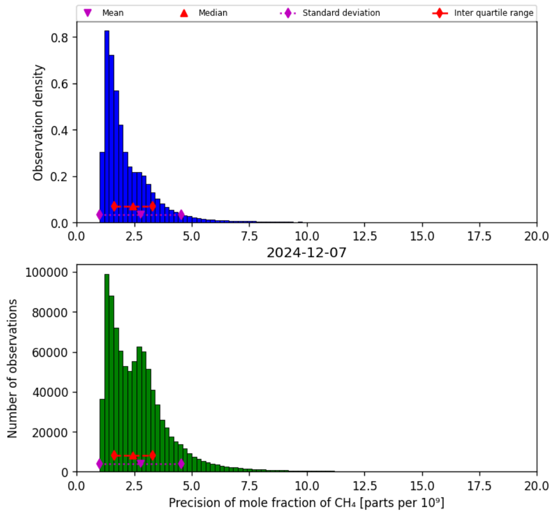
Figure 24: Histogram of “Precision of mole fraction of CH 4 ” for 2024-12-06 to 2024-12-08
