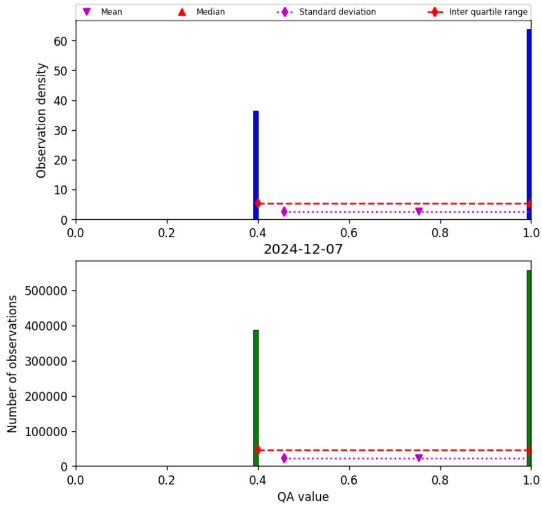
Figure 22: Histogram of “QA value” for 2024-12-06 to 2024-12-08
