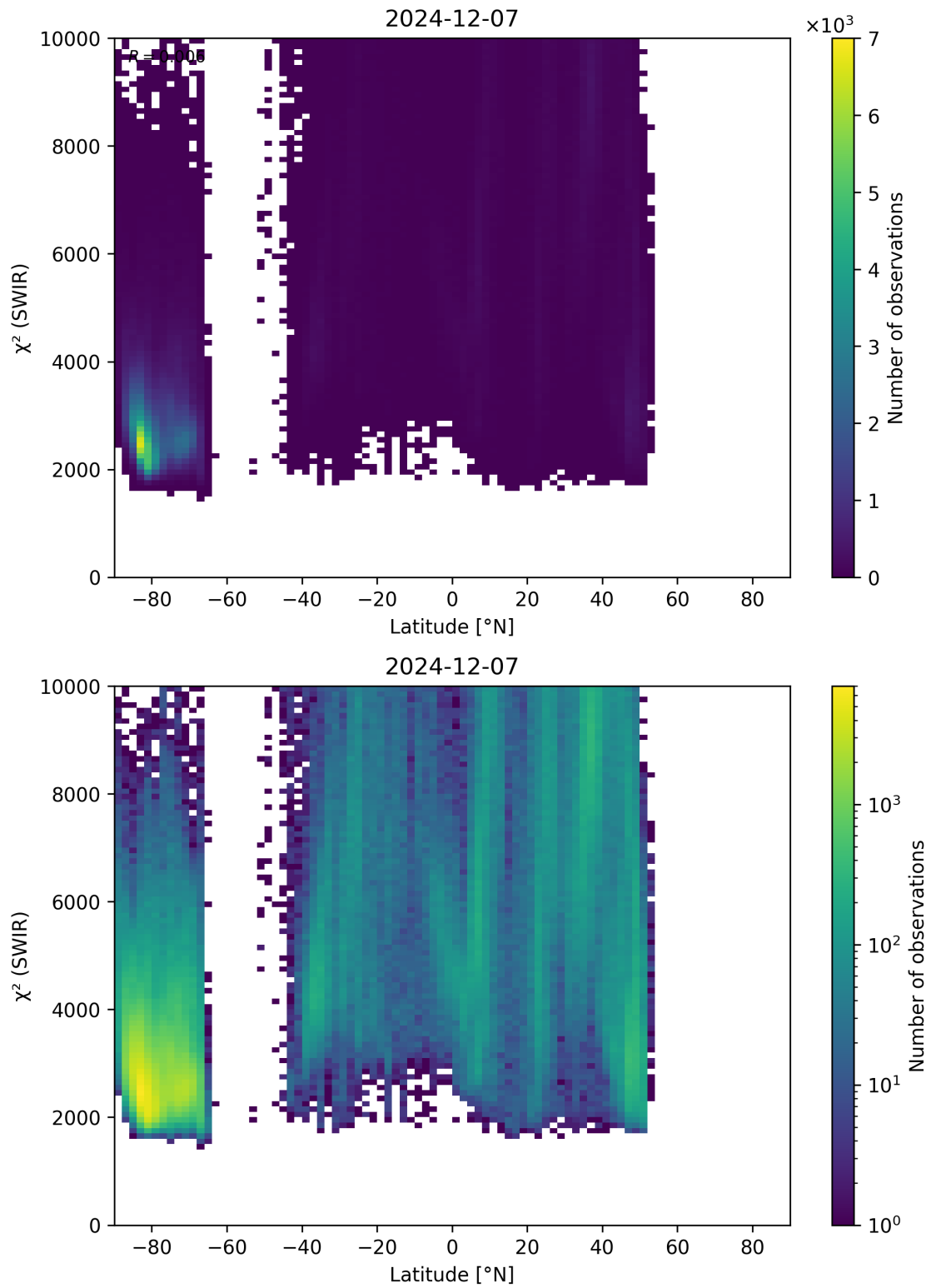
Figure 54: Scatter density plot of “Latitude” against “ \chi^2 (SWIR)” for 2024-12-06 to 2024-12-08.
