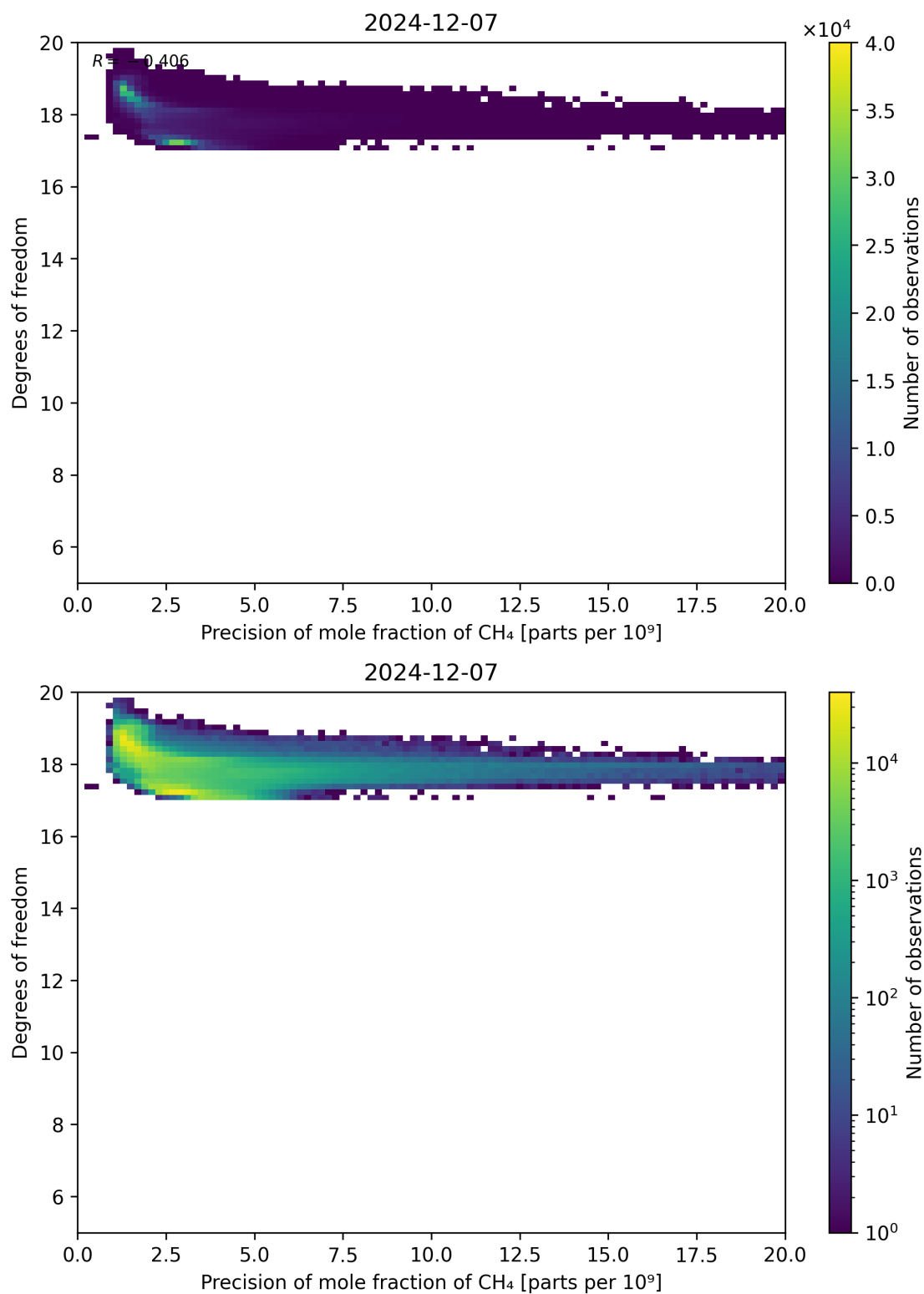
Figure 80: Scatter density plot of “Precision of mole fraction of CH 4 ” against “Degrees of freedom” for 2024-12-06 to 2024-12-08.
