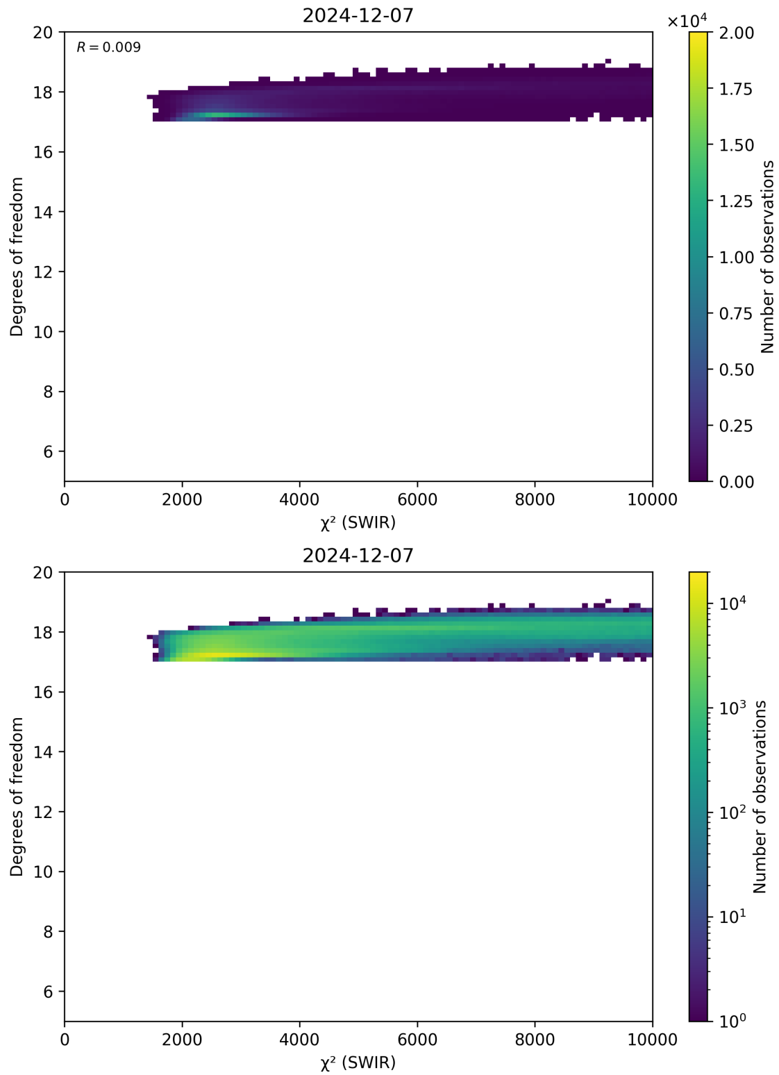
Figure 48: Scatter density plot of “ \chi^2 (SWIR)” against “Degrees of freedom” for 2024-12-06 to 2024-12-08.
