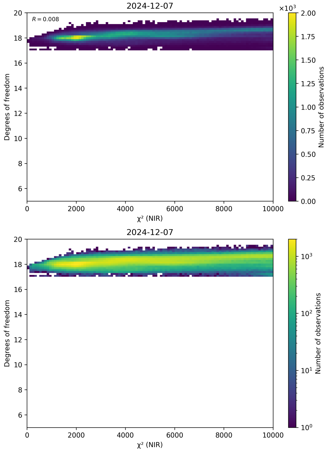
Figure 44: Scatter density plot of “ \chi^2 (NIR)” against “Degrees of freedom” for 2024-12-06 to 2024-12-08.
