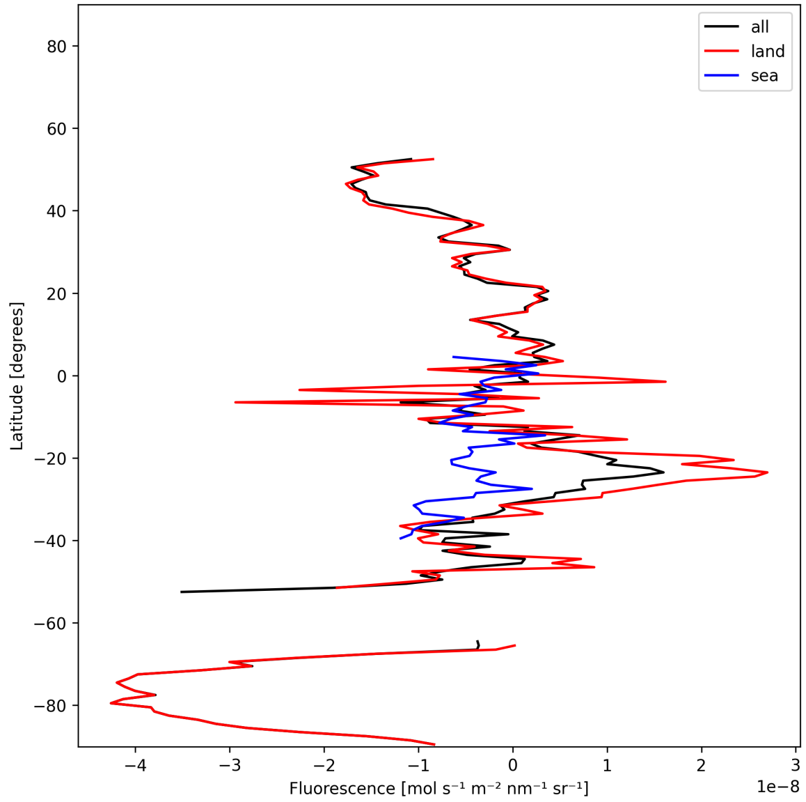
Figure 21: Zonal average of “Fluorescence” for 2024-12-06 to 2024-12-08.
