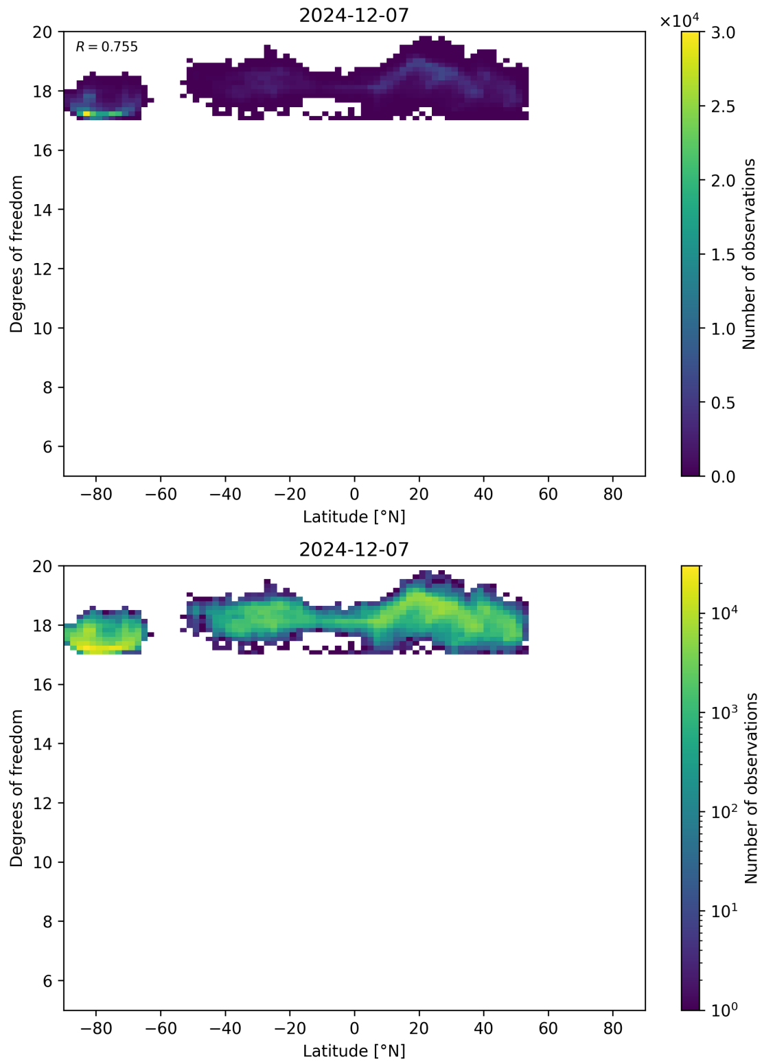
Figure 55: Scatter density plot of “Latitude” against “Degrees of freedom” for 2024-12-06 to 2024-12-08.
