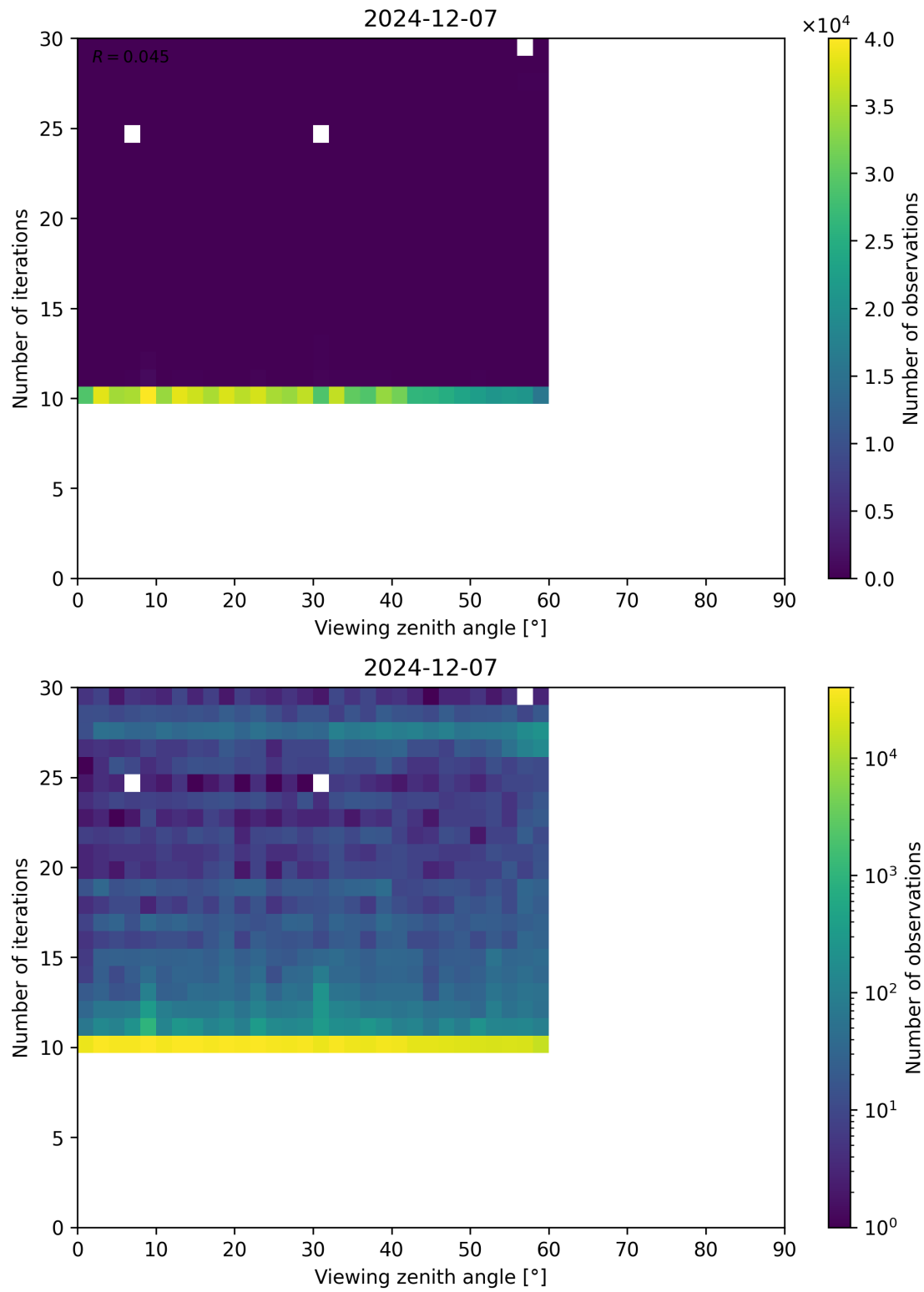
Figure 113: Scatter density plot of “Viewing zenith angle” against “Number of iterations” for 2024-12-06 to 2024-12-08.
