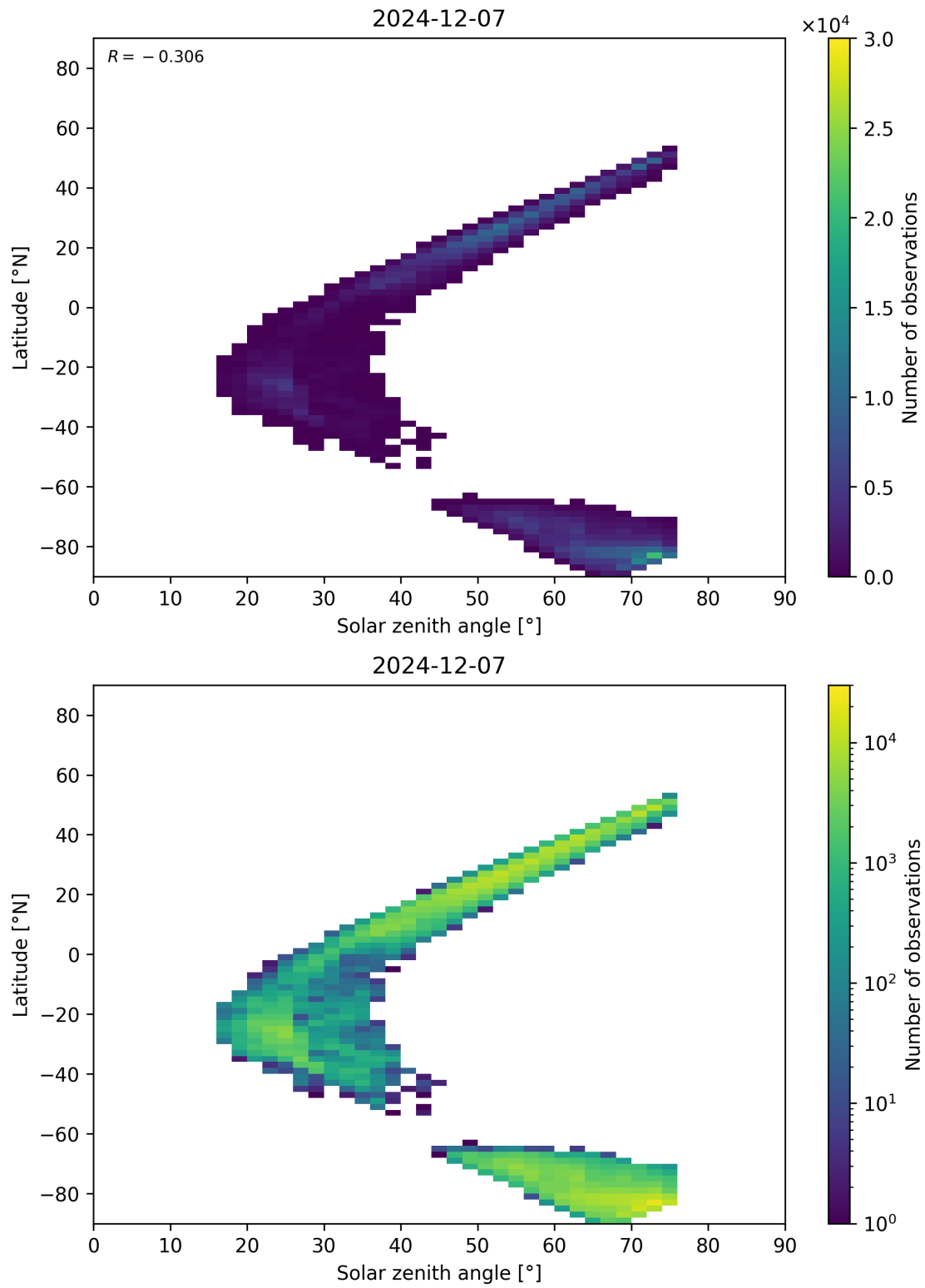
Figure 98: Scatter density plot of “Solar zenith angle” against “Latitude” for 2024-12-06 to 2024-12-08.
