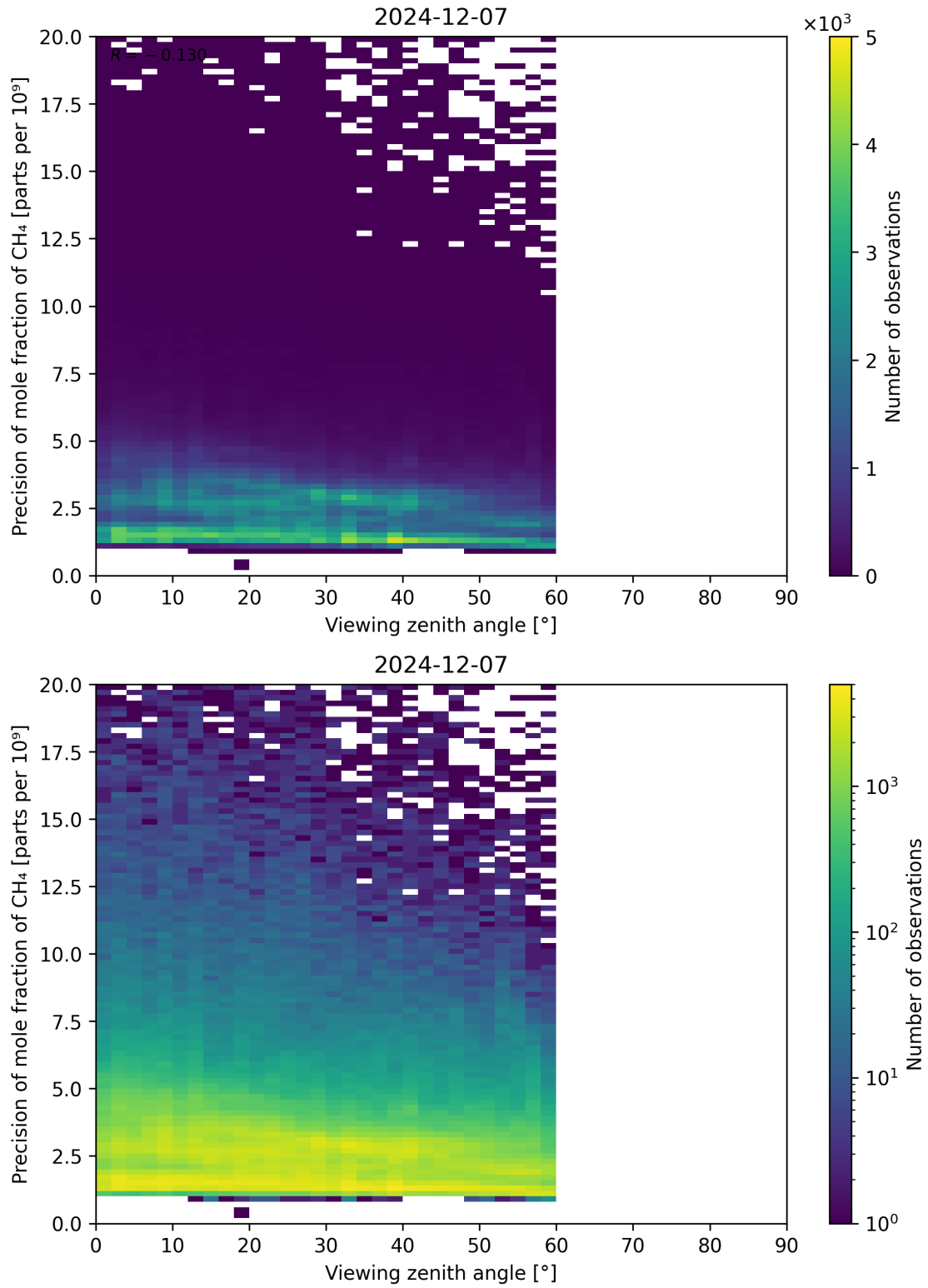
Figure 112: Scatter density plot of “Viewing zenith angle” against “Precision of mole fraction of CH 4 ” for 2024-12-06 to 2024-12-08.
