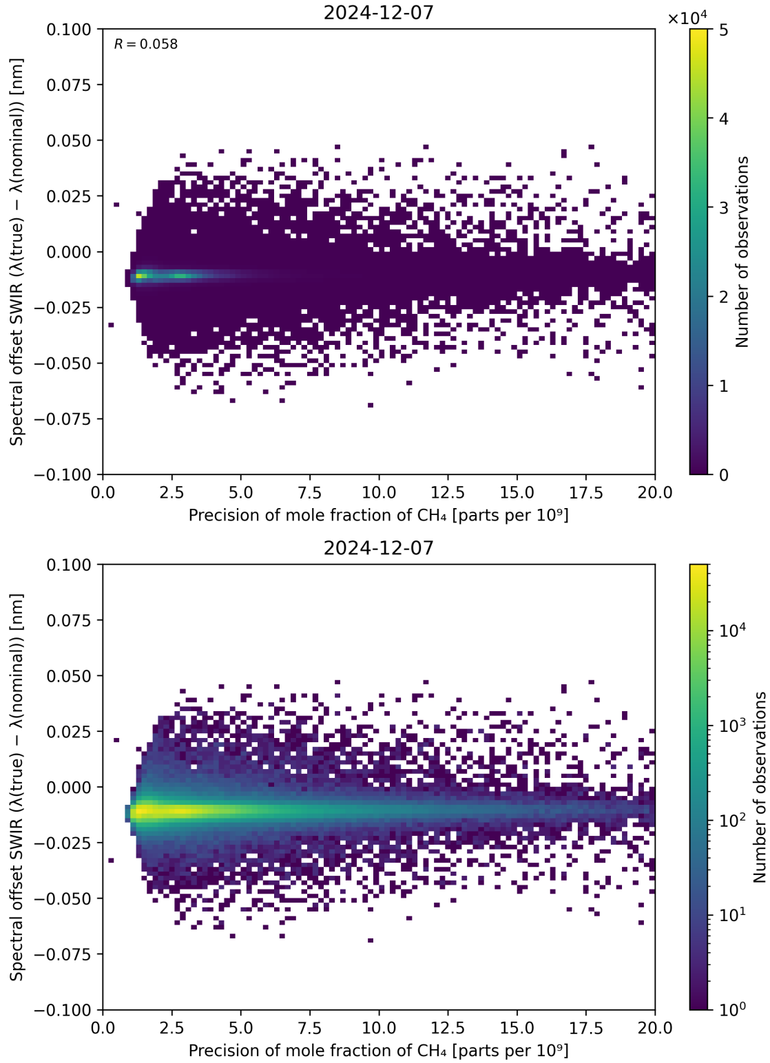
Figure 85: Scatter density plot of “Precision of mole fraction of CH 4 ” against “Spectral offset SWIR ( \lambda_{\text{true}} - \lambda_{\text{nominal}} )” for 2024-12-06 to 2024-12-08.
