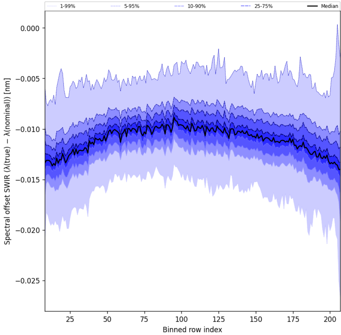
Figure 38: Along track statistics of “Spectral offset SWIR ( \lambda_{\text{true}} - \lambda_{\text{nominal}} )” for 2024-12-06 to 2024-12-08
