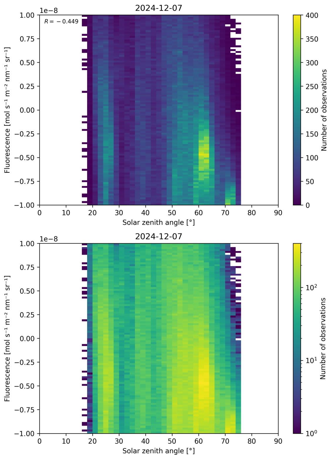
Figure 97: Scatter density plot of “Solar zenith angle” against “Fluorescence” for 2024-12-06 to 2024-12-08.
