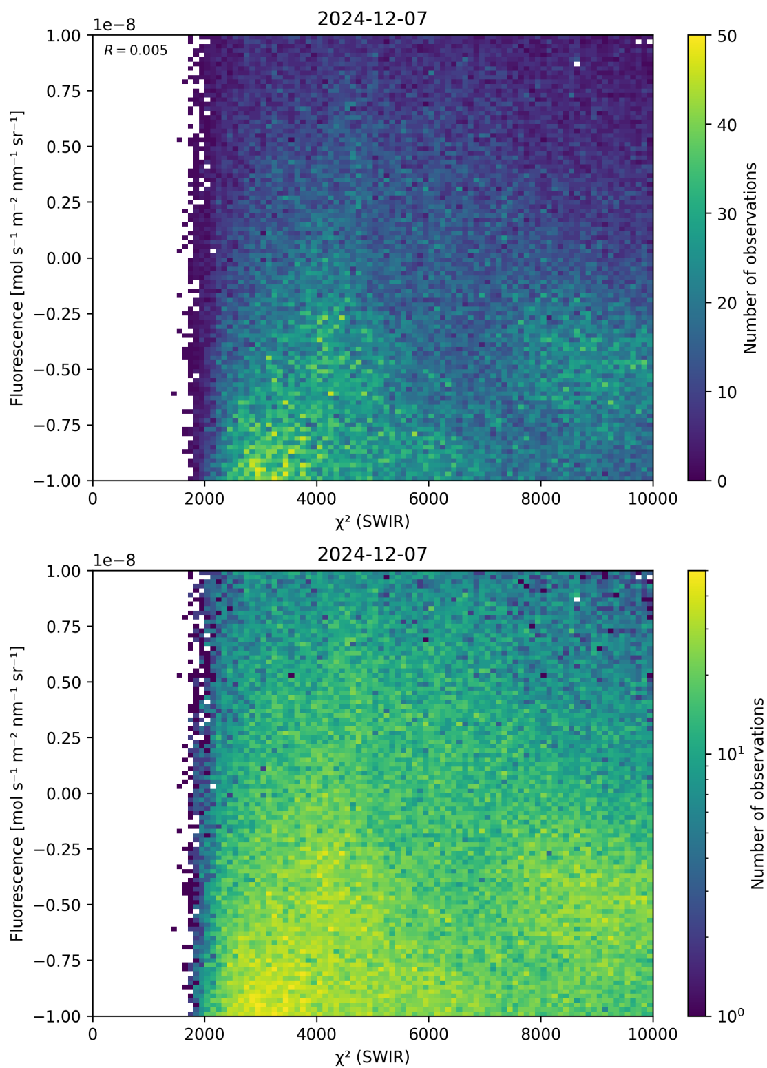
Figure 49: Scatter density plot of “ \chi^2 (SWIR)” against “Fluorescence” for 2024-12-06 to 2024-12-08.
