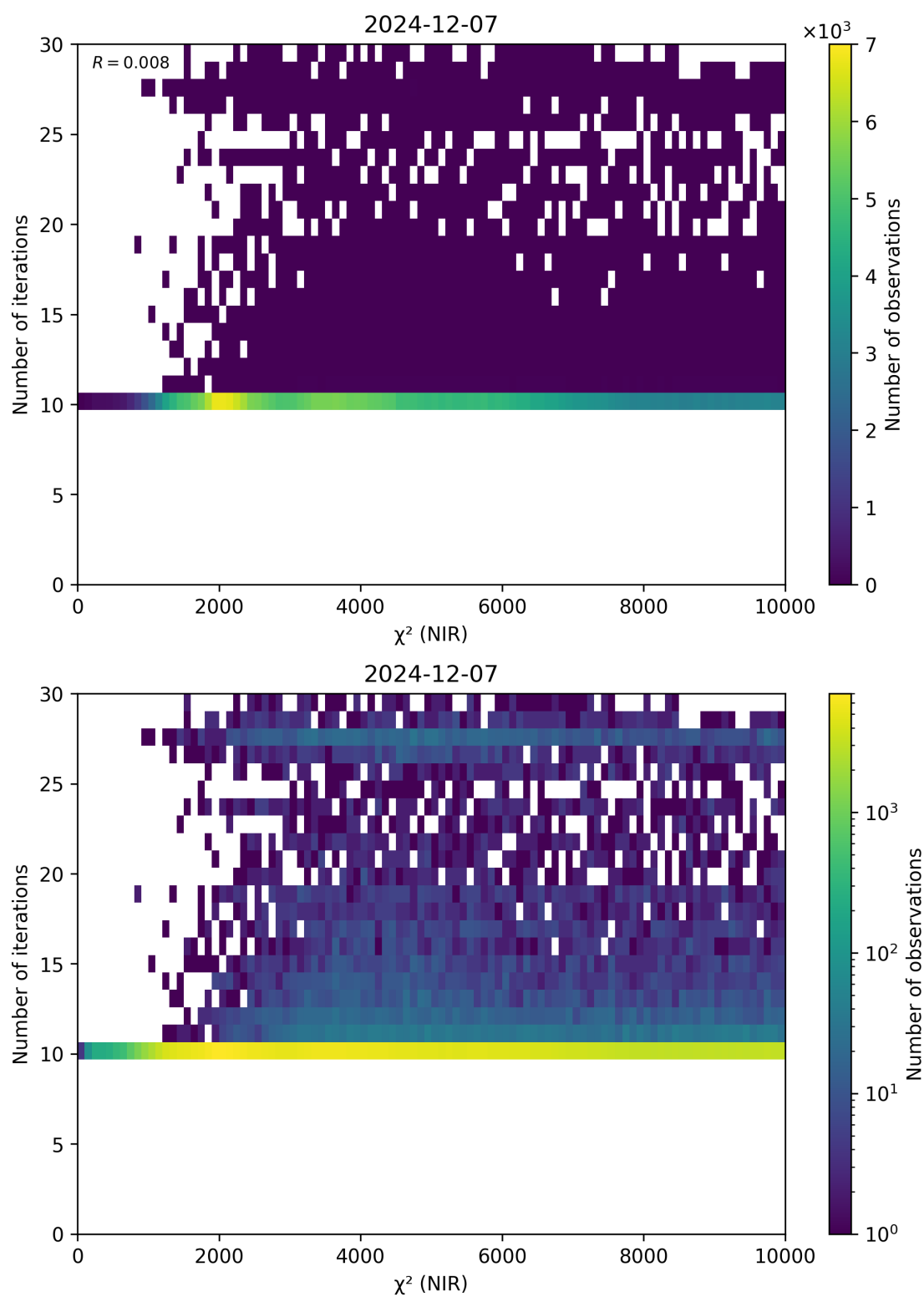
Figure 46: Scatter density plot of “ \chi^2 (NIR)” against “Number of iterations” for 2024-12-06 to 2024-12-08.
