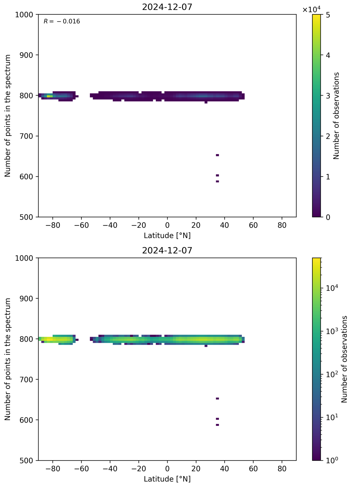
Figure 61: Scatter density plot of “Latitude” against “Number of points in the spectrum” for 2024-12-06 to 2024-12-08.
