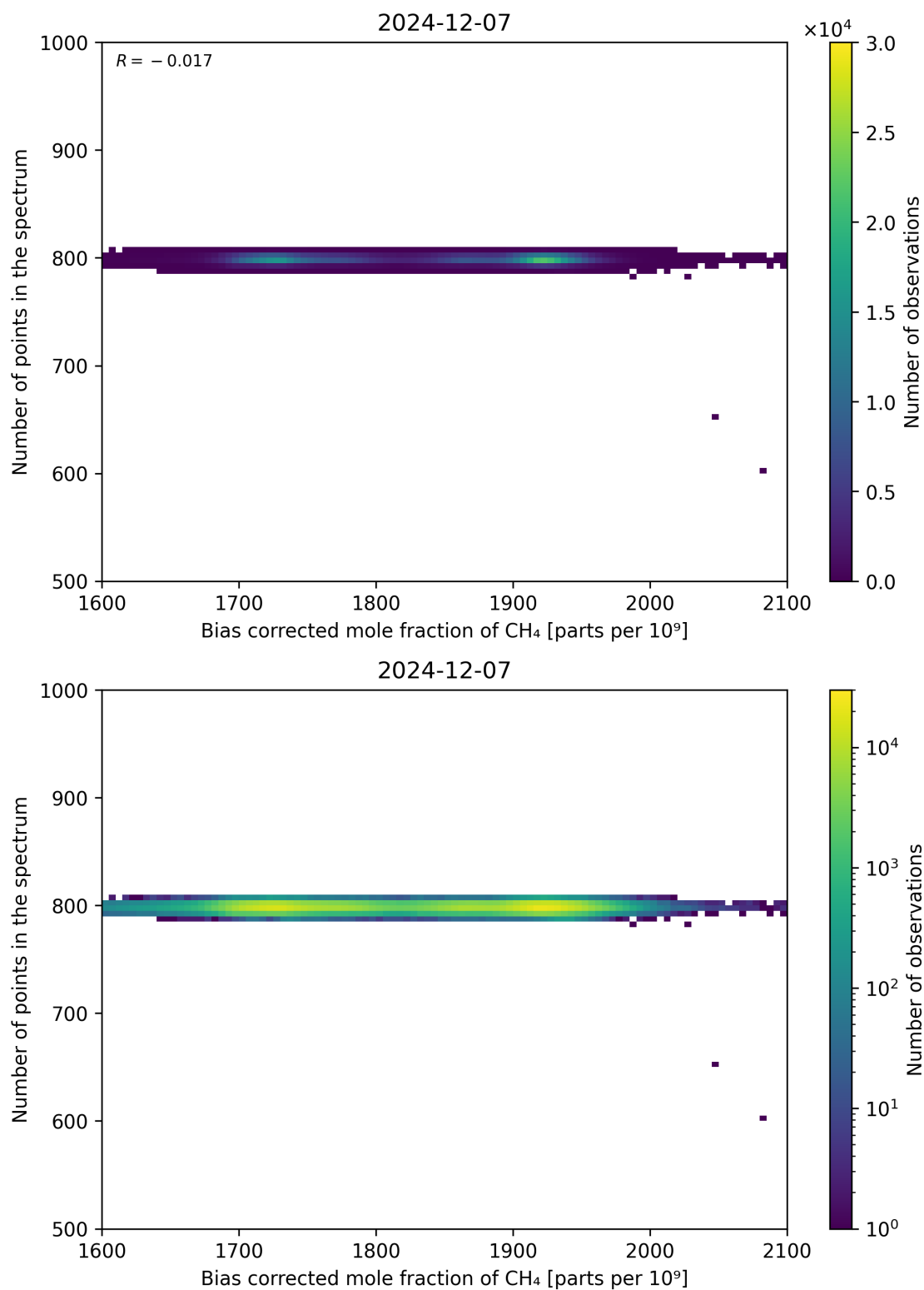
Figure 68: Scatter density plot of “Bias corrected mole fraction of CH 4 ” against “Number of points in the spectrum” for 2024-12-06 to 2024-12-08.
