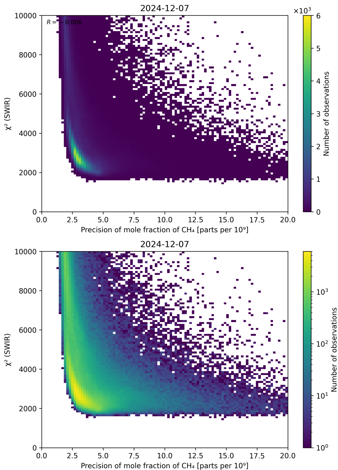
Figure 79: Scatter density plot of “Precision of mole fraction of CH 4 ” against “ \chi^2 (SWIR)” for 2024-12-06 to 2024-12-08.
