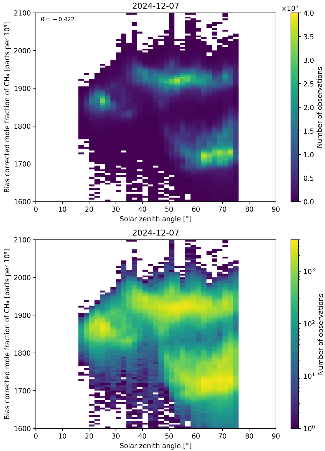
Figure 100: Scatter density plot of “Solar zenith angle” against “Bias corrected mole fraction of CH 4 ” for 2024-12-06 to 2024-12-08.
