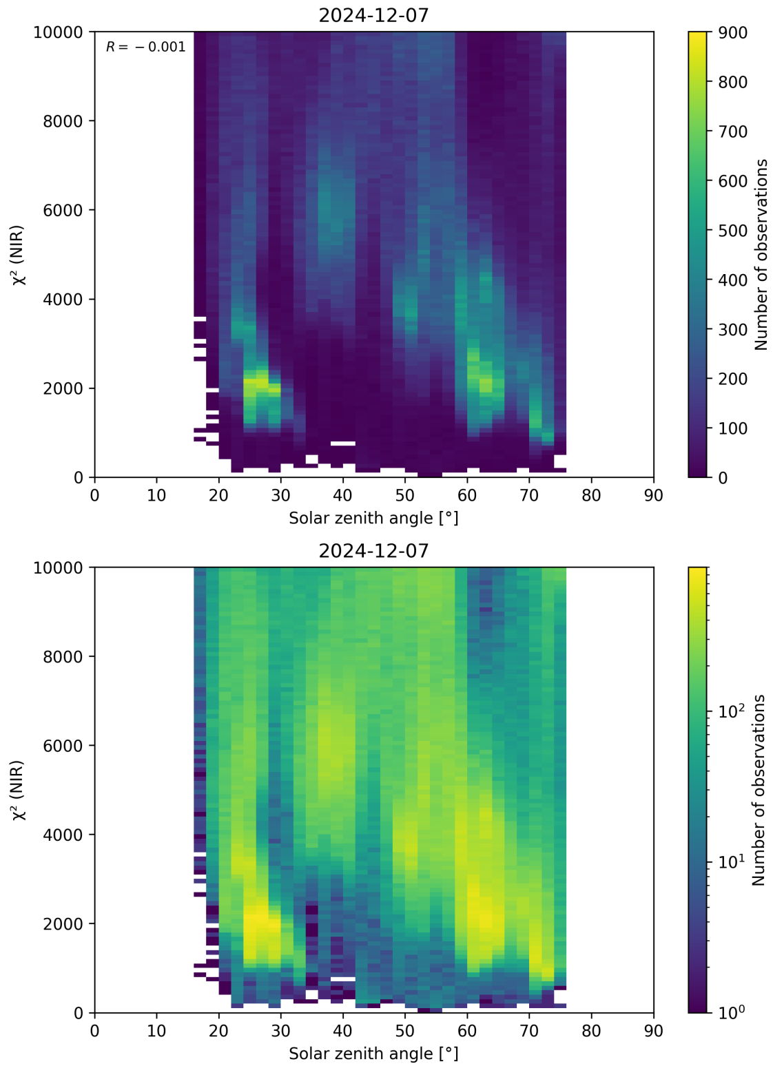
Figure 94: Scatter density plot of “Solar zenith angle” against “ \chi^2 (NIR)” for 2024-12-06 to 2024-12-08.
