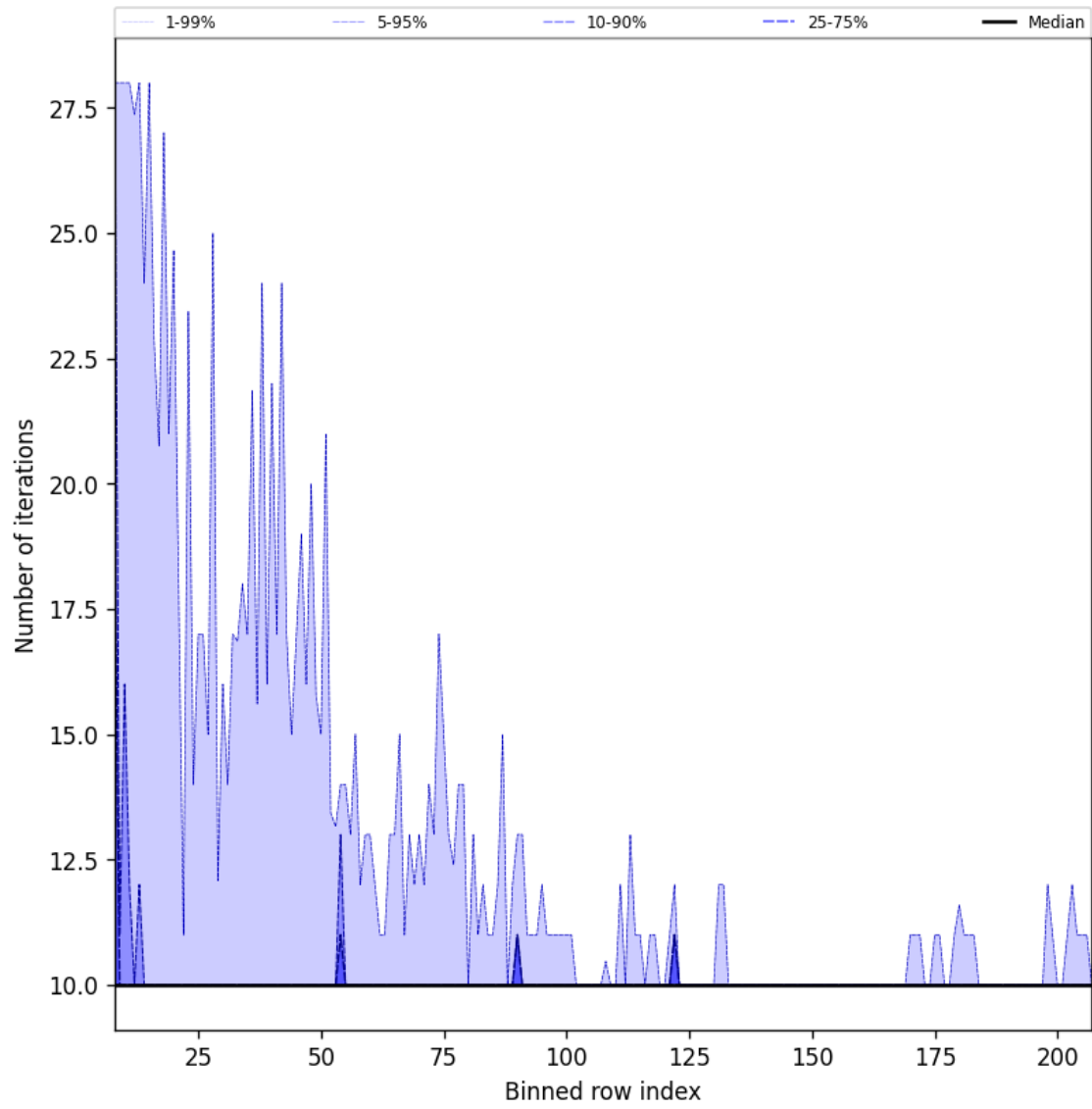
Figure 42: Along track statistics of “Number of iterations” for 2024-12-06 to 2024-12-08
