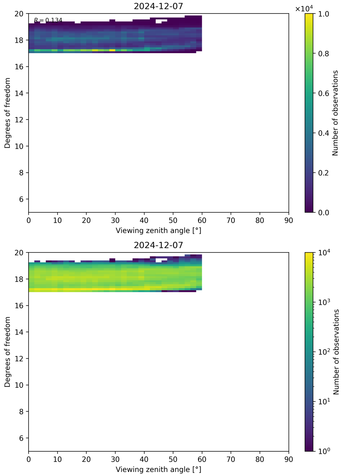
Figure 107: Scatter density plot of “Viewing zenith angle” against “Degrees of freedom” for 2024-12-06 to 2024-12-08.
