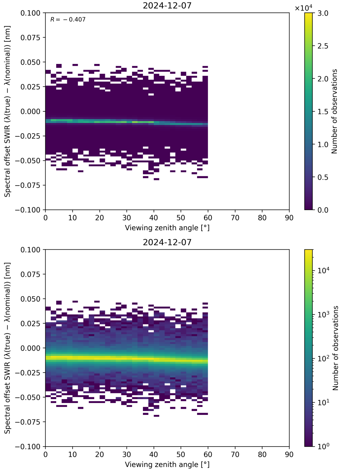
Figure 116: Scatter density plot of “Viewing zenith angle” against “Spectral offset SWIR ( \lambda_{\text{true}} - \lambda_{\text{nominal}} )” for 2024-12-06 to 2024-12-08.
