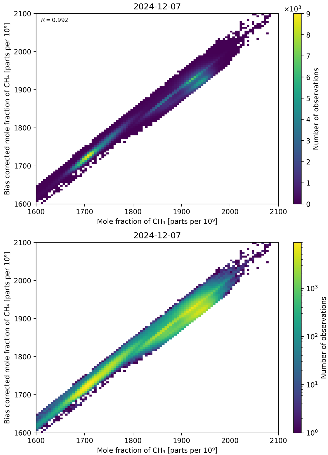
Figure 74: Scatter density plot of “Mole fraction of CH 4 ” against “Bias corrected mole fraction of CH 4 ” for 2024-12-06 to 2024-12-08.
