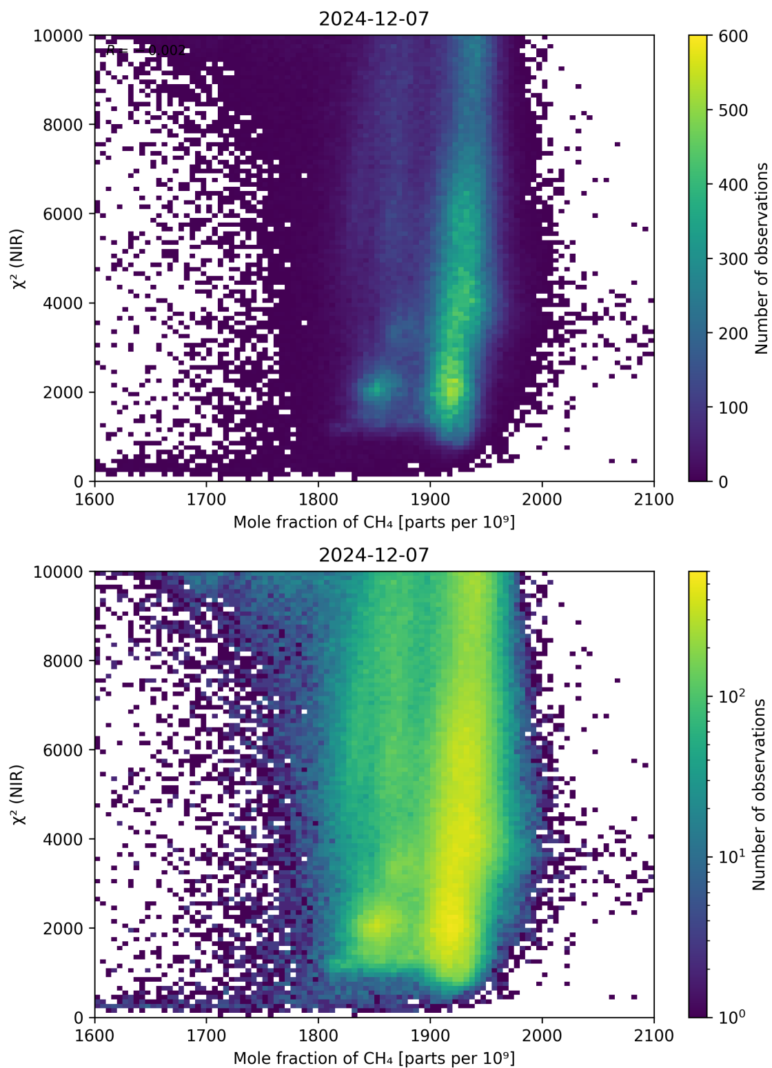
Figure 70: Scatter density plot of “Mole fraction of \text{CH}_4 ” against “ \chi^2 (NIR)” for 2024-12-06 to 2024-12-08.
