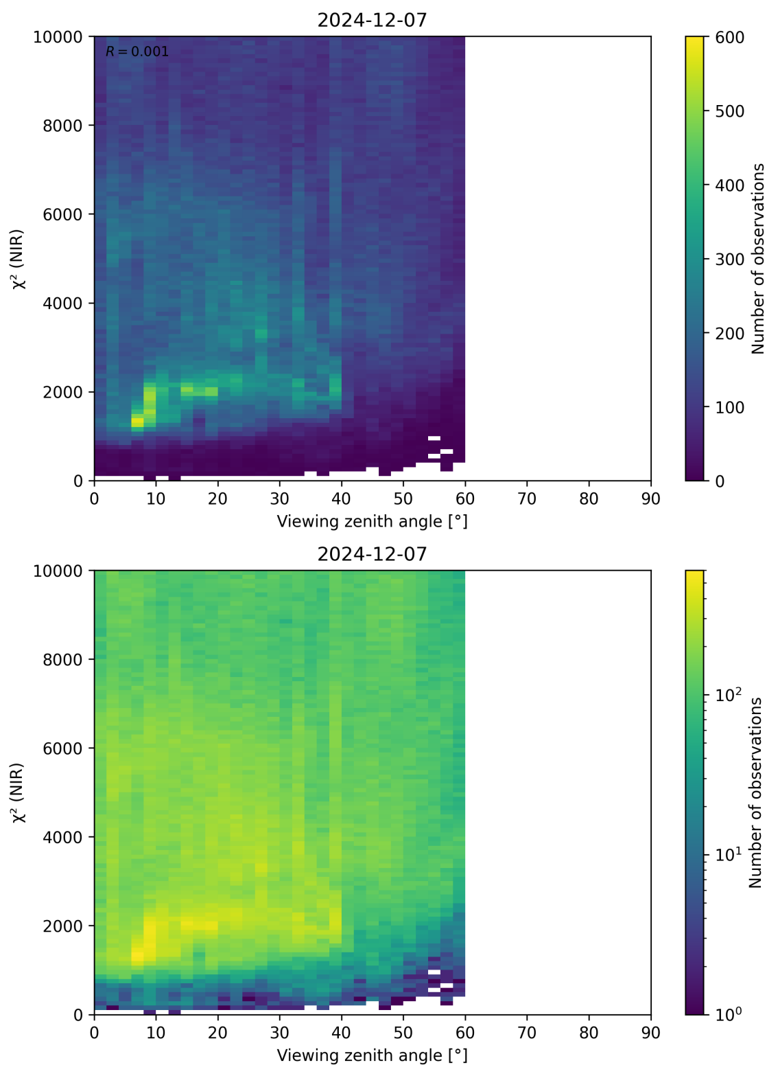
Figure 105: Scatter density plot of “Viewing zenith angle” against “ \chi^2 (NIR)” for 2024-12-06 to 2024-12-08.
