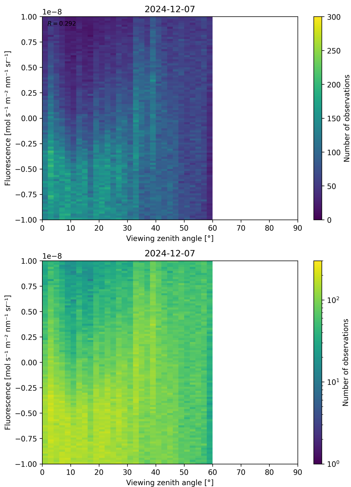
Figure 108: Scatter density plot of “Viewing zenith angle” against “Fluorescence” for 2024-12-06 to 2024-12-08.
