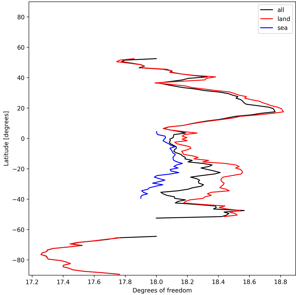
Figure 19: Zonal average of “Degrees of freedom” for 2024-12-06 to 2024-12-08.
