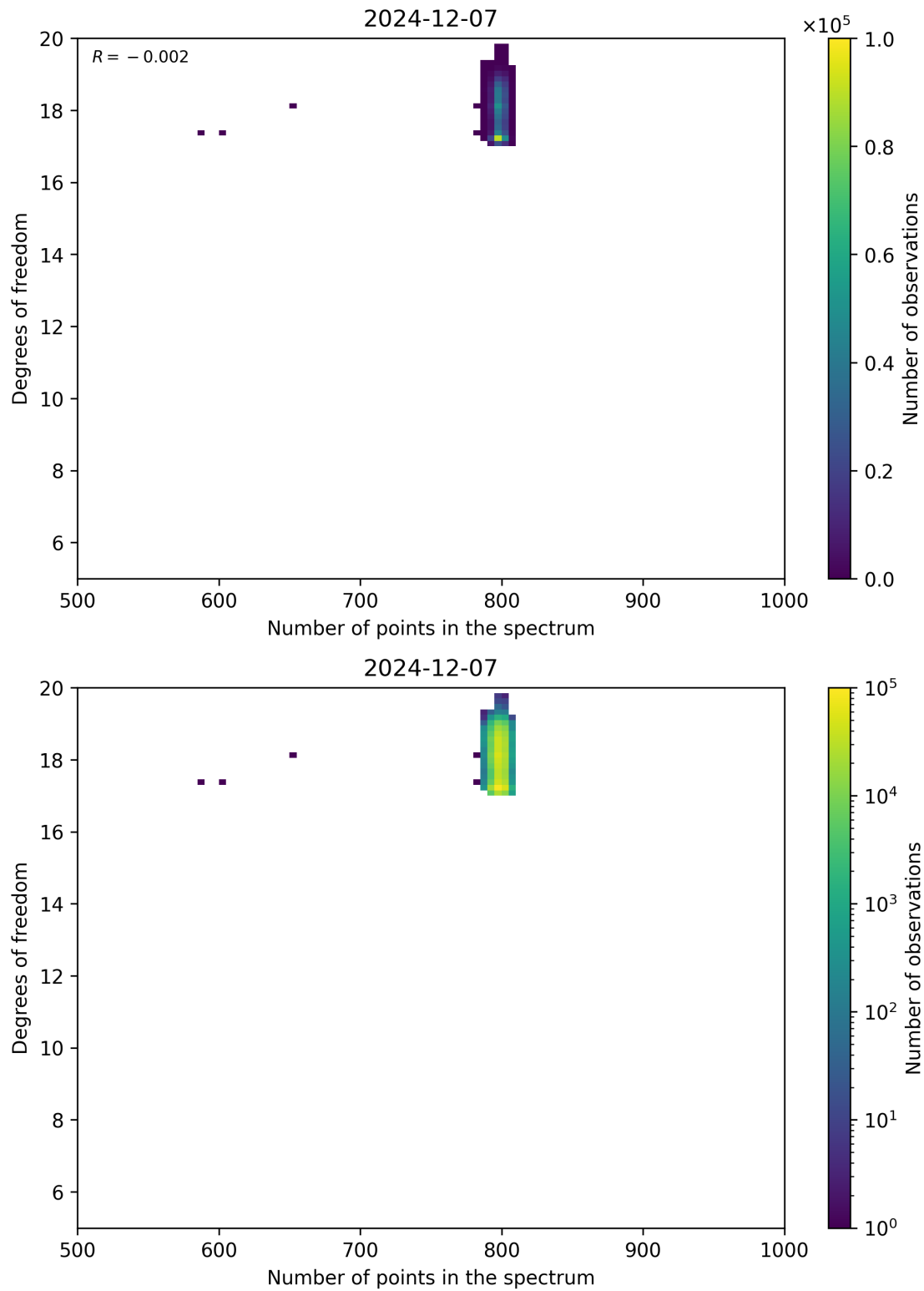
Figure 90: Scatter density plot of “Number of points in the spectrum” against “Degrees of freedom” for 2024-12-06 to 2024-12-08.
