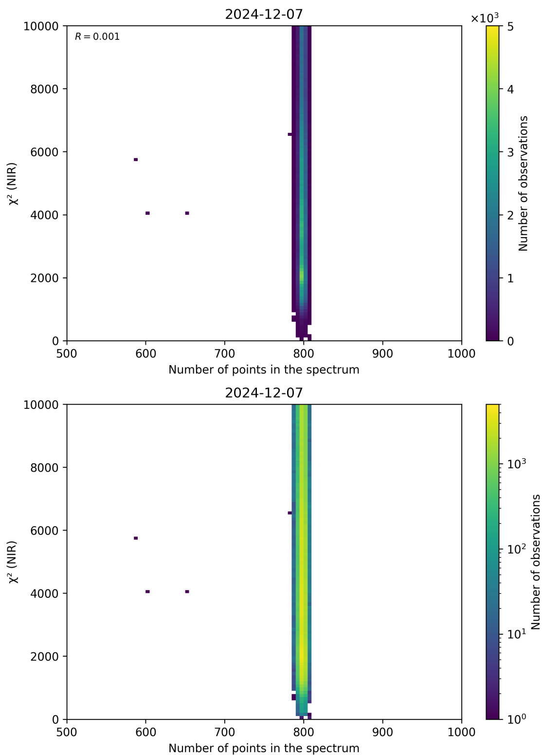
Figure 88: Scatter density plot of “Number of points in the spectrum” against “ \chi^2 (NIR)” for 2024-12-06 to 2024-12-08.
