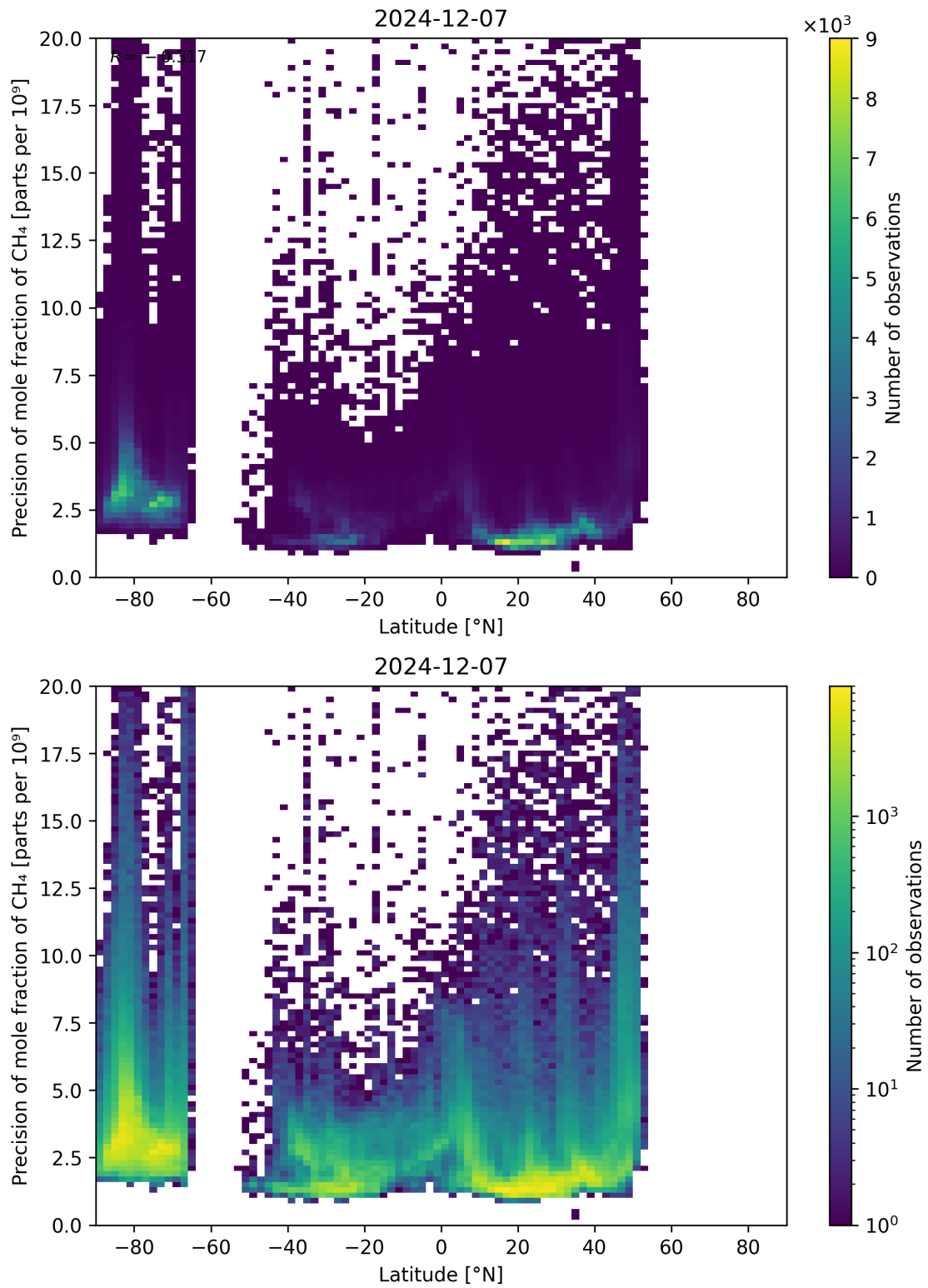
Figure 59: Scatter density plot of “Latitude” against “Precision of mole fraction of CH 4 ” for 2024-12-06 to 2024-12-08.
