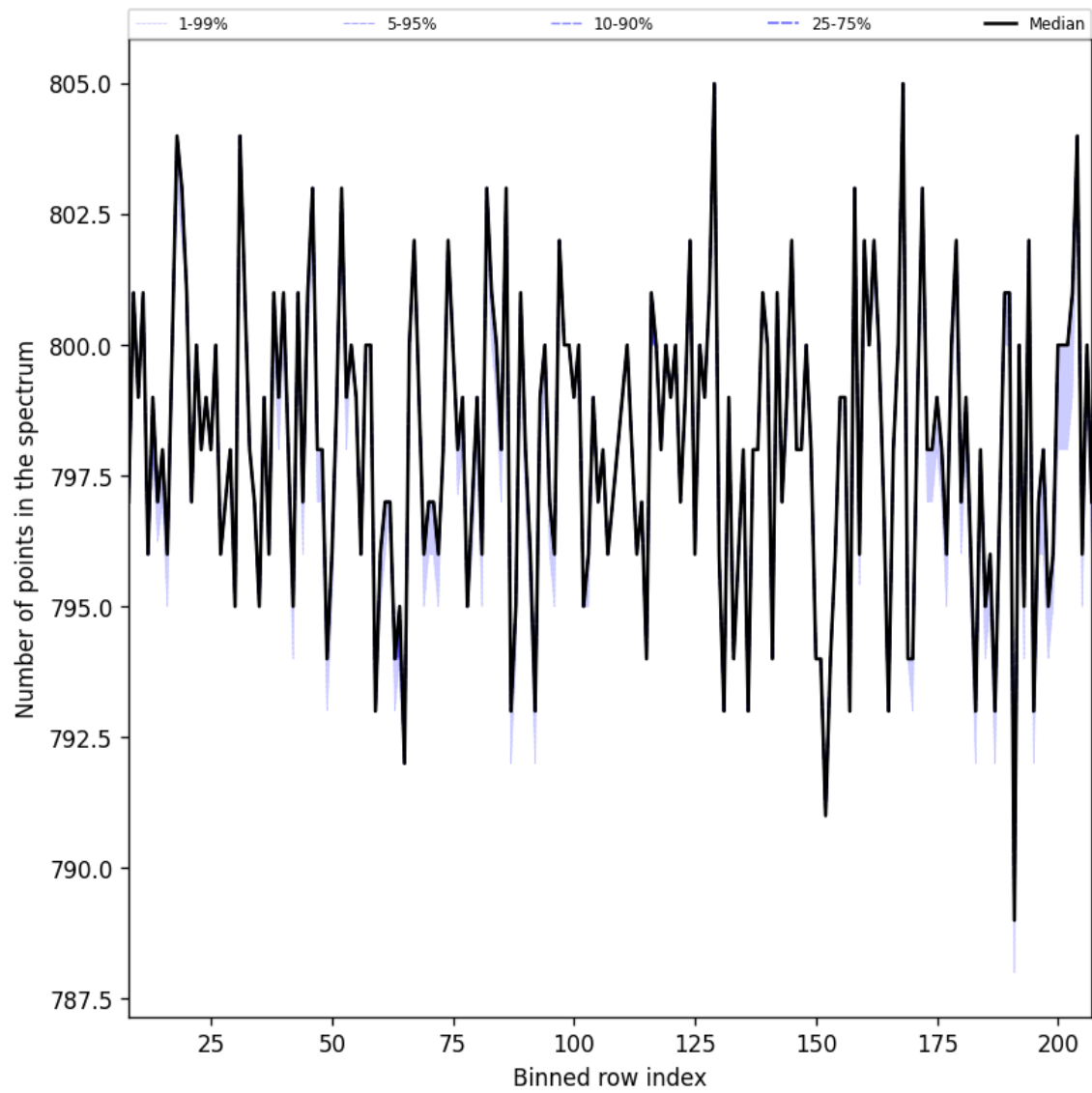
Figure 37: Along track statistics of “Number of points in the spectrum” for 2024-12-06 to 2024-12-08
