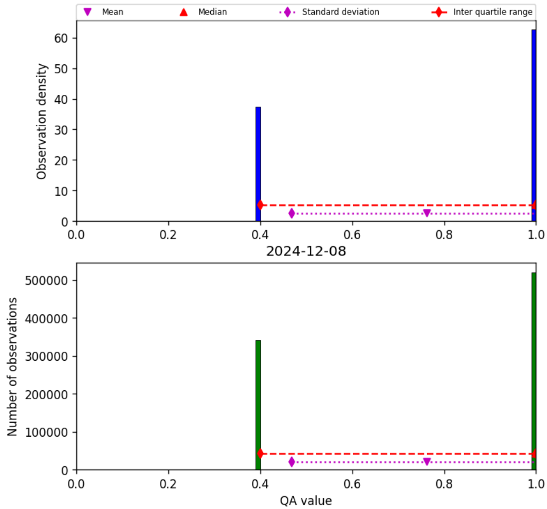
Figure 22: Histogram of “QA value” for 2024-12-07 to 2024-12-09
