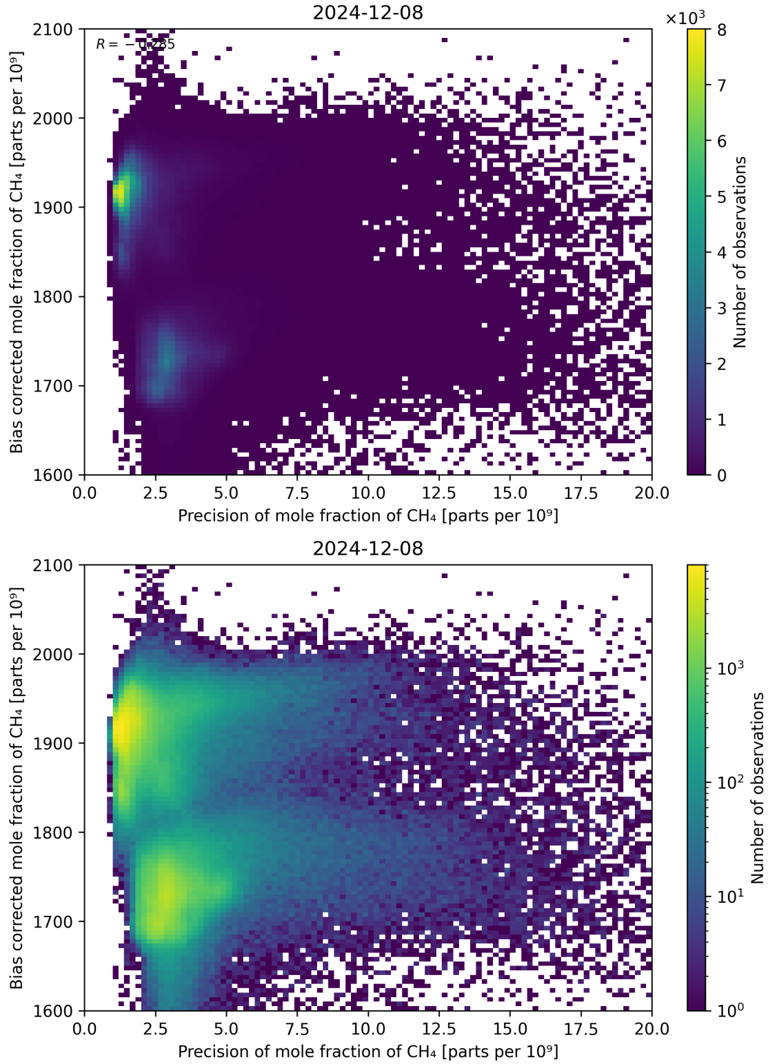
Figure 82: Scatter density plot of “Precision of mole fraction of CH 4 ” against “Bias corrected mole fraction of CH 4 ” for 2024-12-07 to 2024-12-09.
