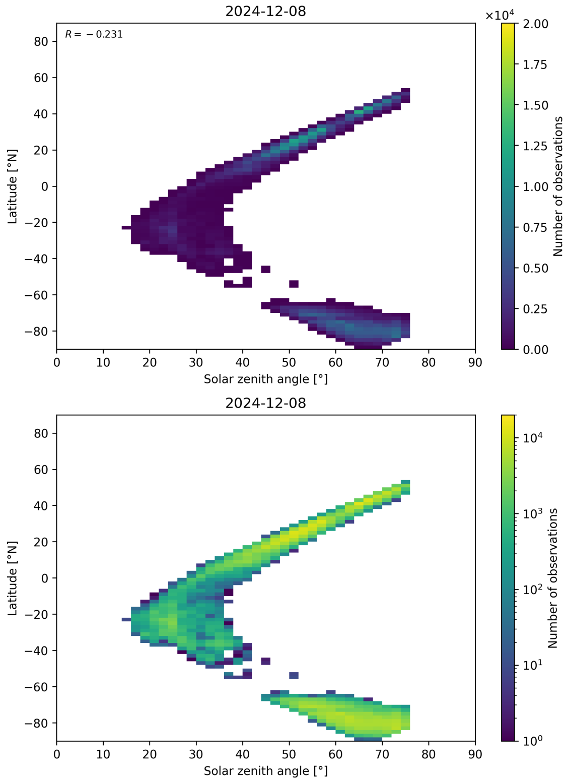
Figure 98: Scatter density plot of “Solar zenith angle” against “Latitude” for 2024-12-07 to 2024-12-09.
