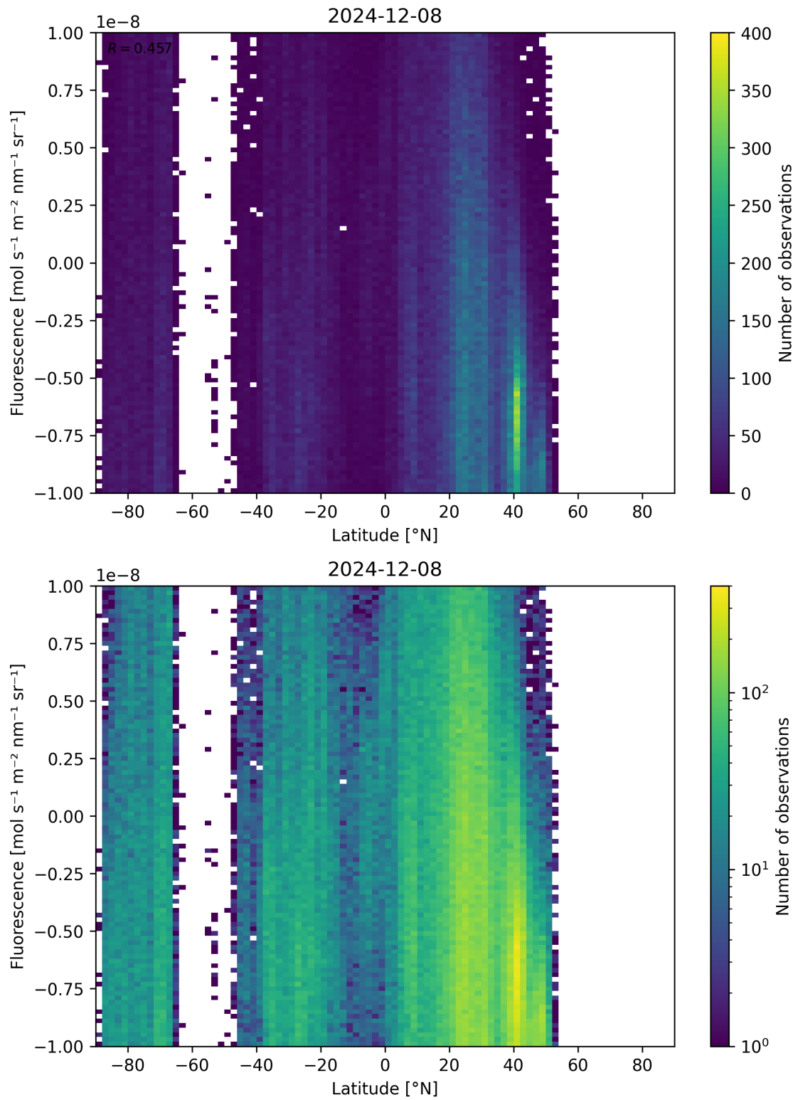
Figure 56: Scatter density plot of “Latitude” against “Fluorescence” for 2024-12-07 to 2024-12-09.
