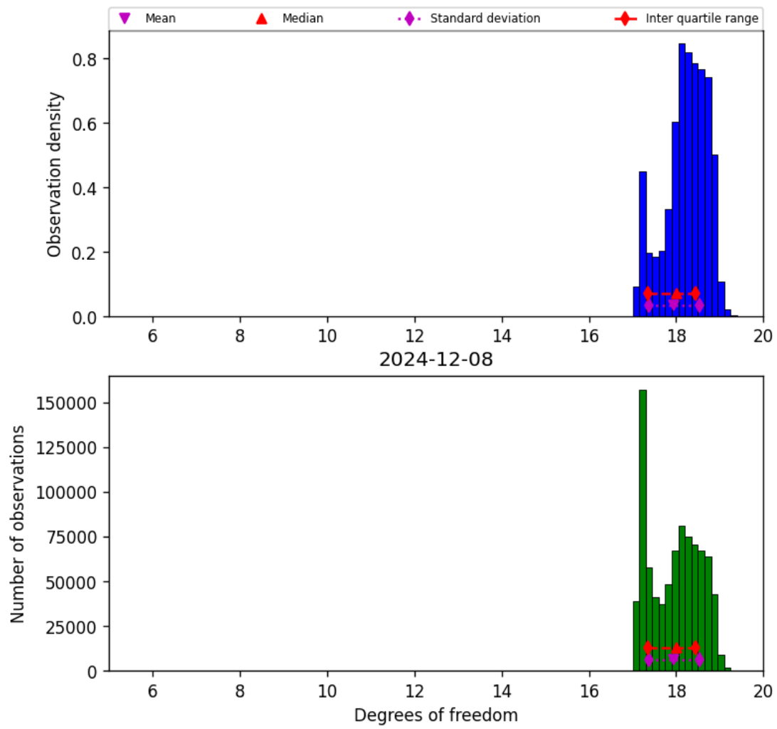
Figure 30: Histogram of “Degrees of freedom” for 2024-12-07 to 2024-12-09
