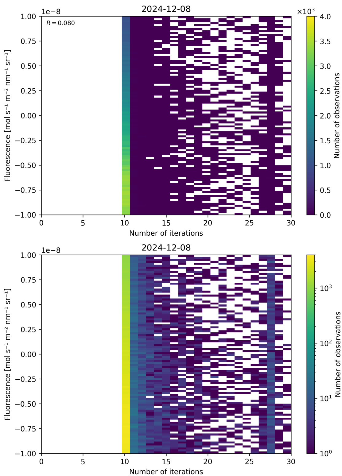
Figure 87: Scatter density plot of “Number of iterations” against “Fluorescence” for 2024-12-07 to 2024-12-09.
