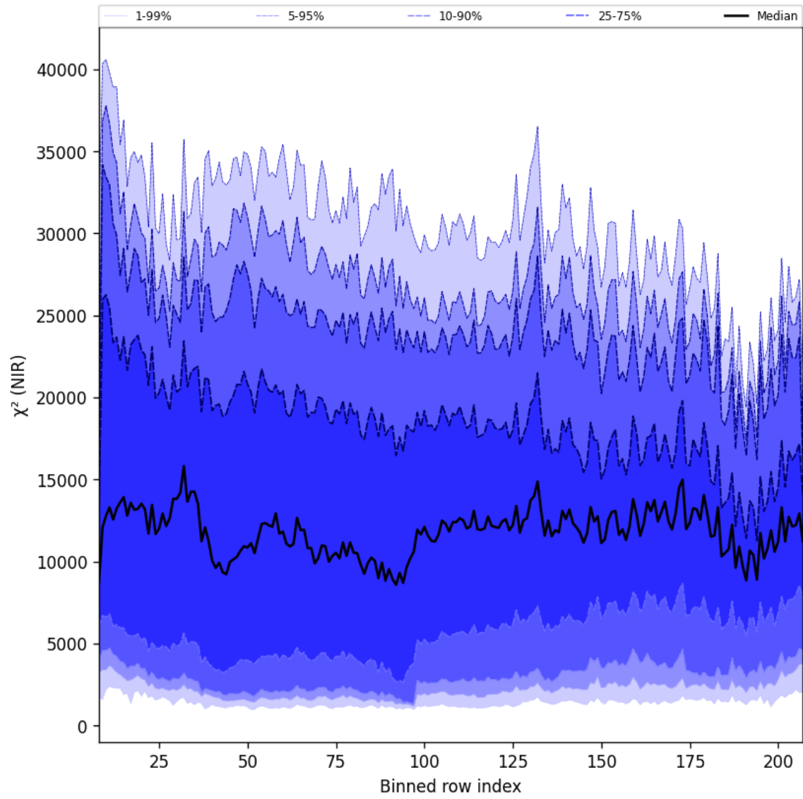
Figure 40: Along track statistics of “ \chi^2 (NIR)” for 2024-12-07 to 2024-12-09
