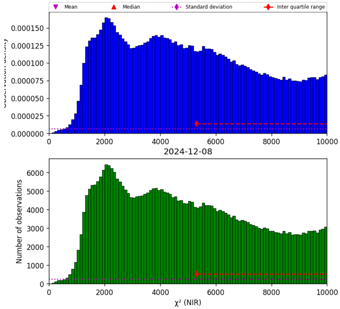
Figure 29: Histogram of “ \chi^2 (NIR)” for 2024-12-07 to 2024-12-09
