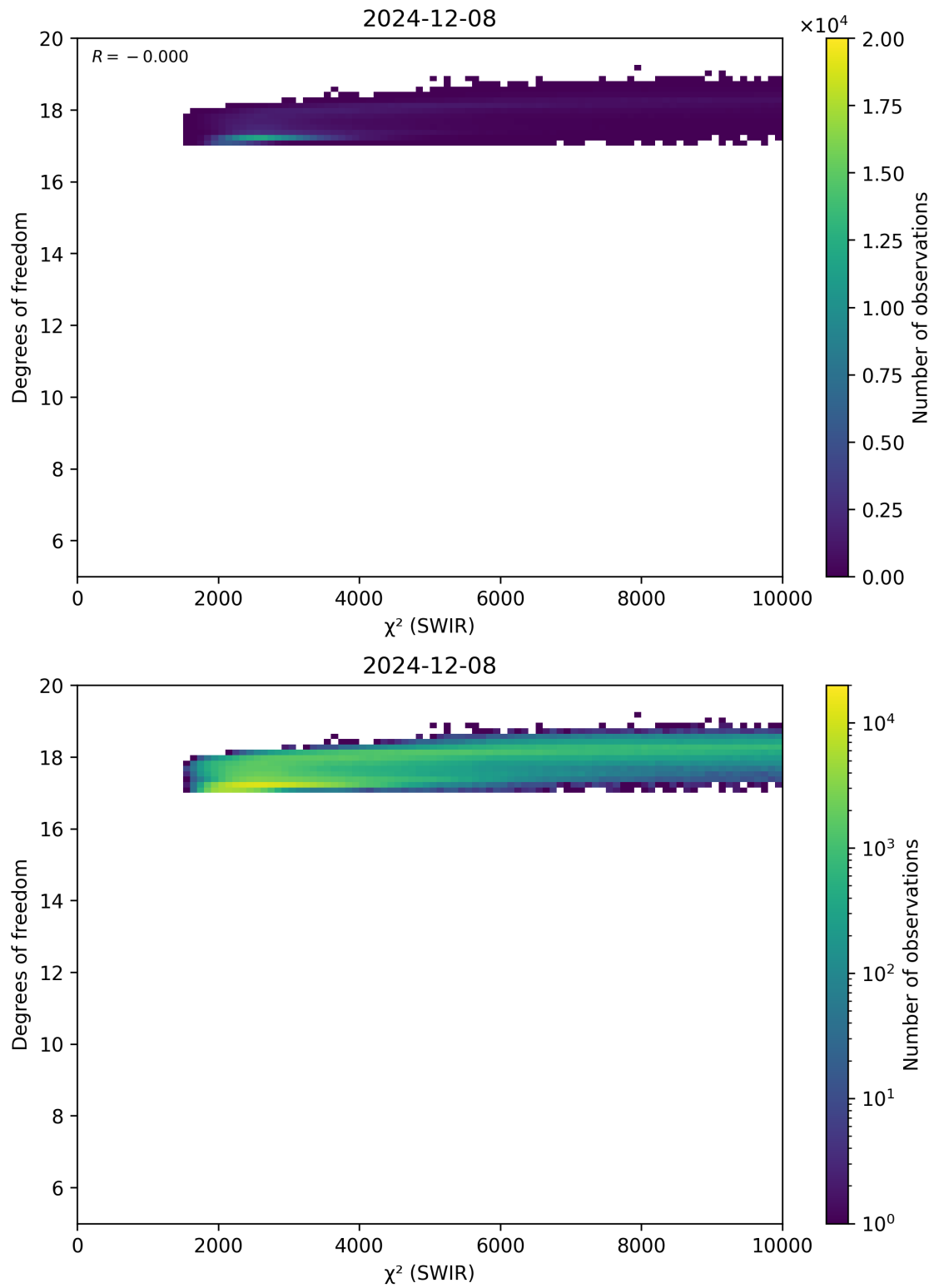
Figure 48: Scatter density plot of “ \chi^2 (SWIR)” against “Degrees of freedom” for 2024-12-07 to 2024-12-09.
