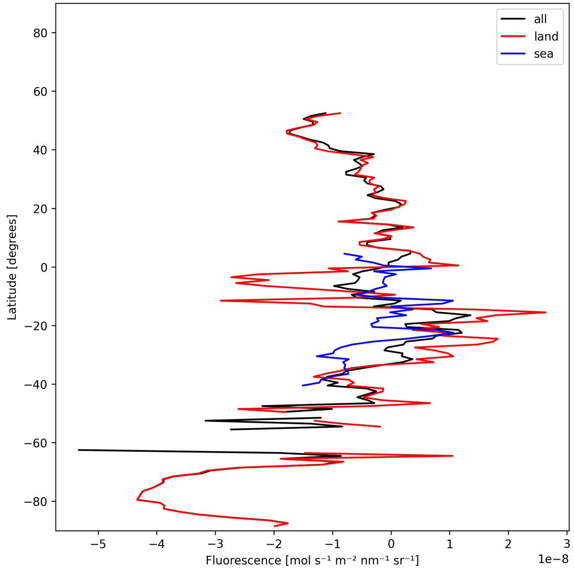
Figure 21: Zonal average of “Fluorescence” for 2024-12-07 to 2024-12-09.
