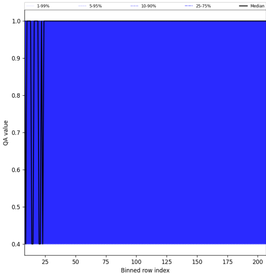
Figure 33: Along track statistics of “QA value” for 2024-12-07 to 2024-12-09
