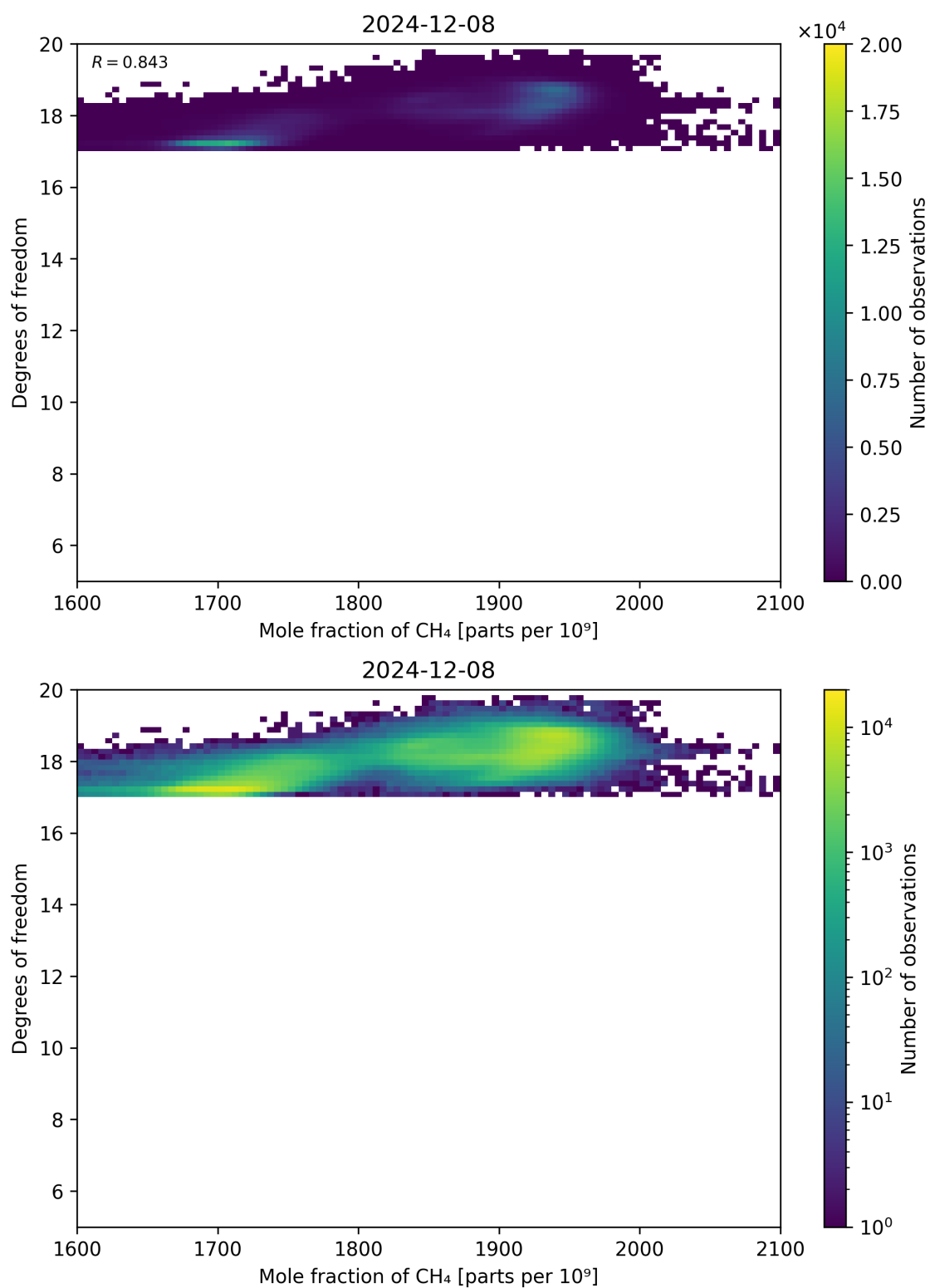
Figure 72: Scatter density plot of “Mole fraction of CH 4 ” against “Degrees of freedom” for 2024-12-07 to 2024-12-09.
