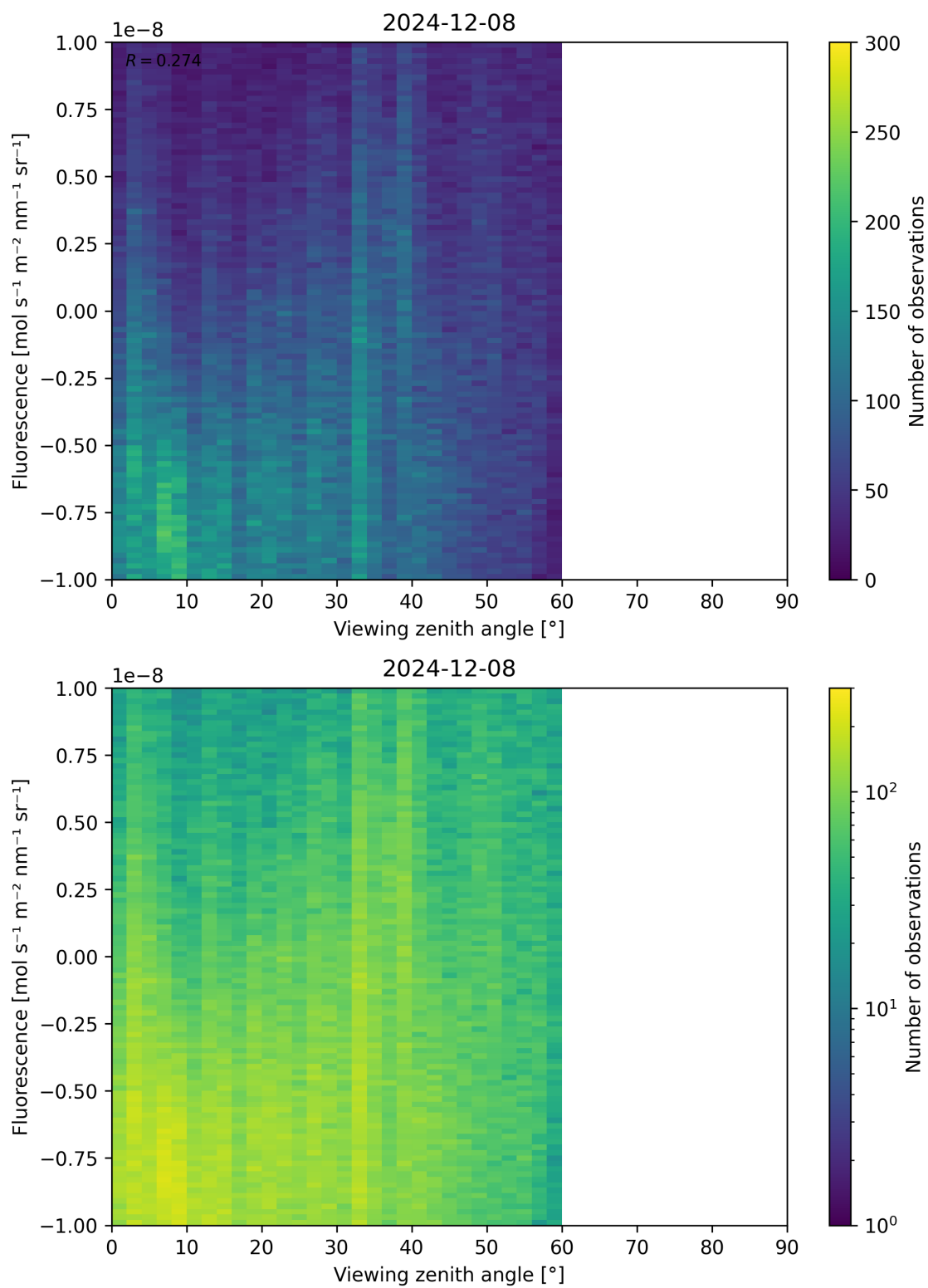
Figure 108: Scatter density plot of “Viewing zenith angle” against “Fluorescence” for 2024-12-07 to 2024-12-09.
