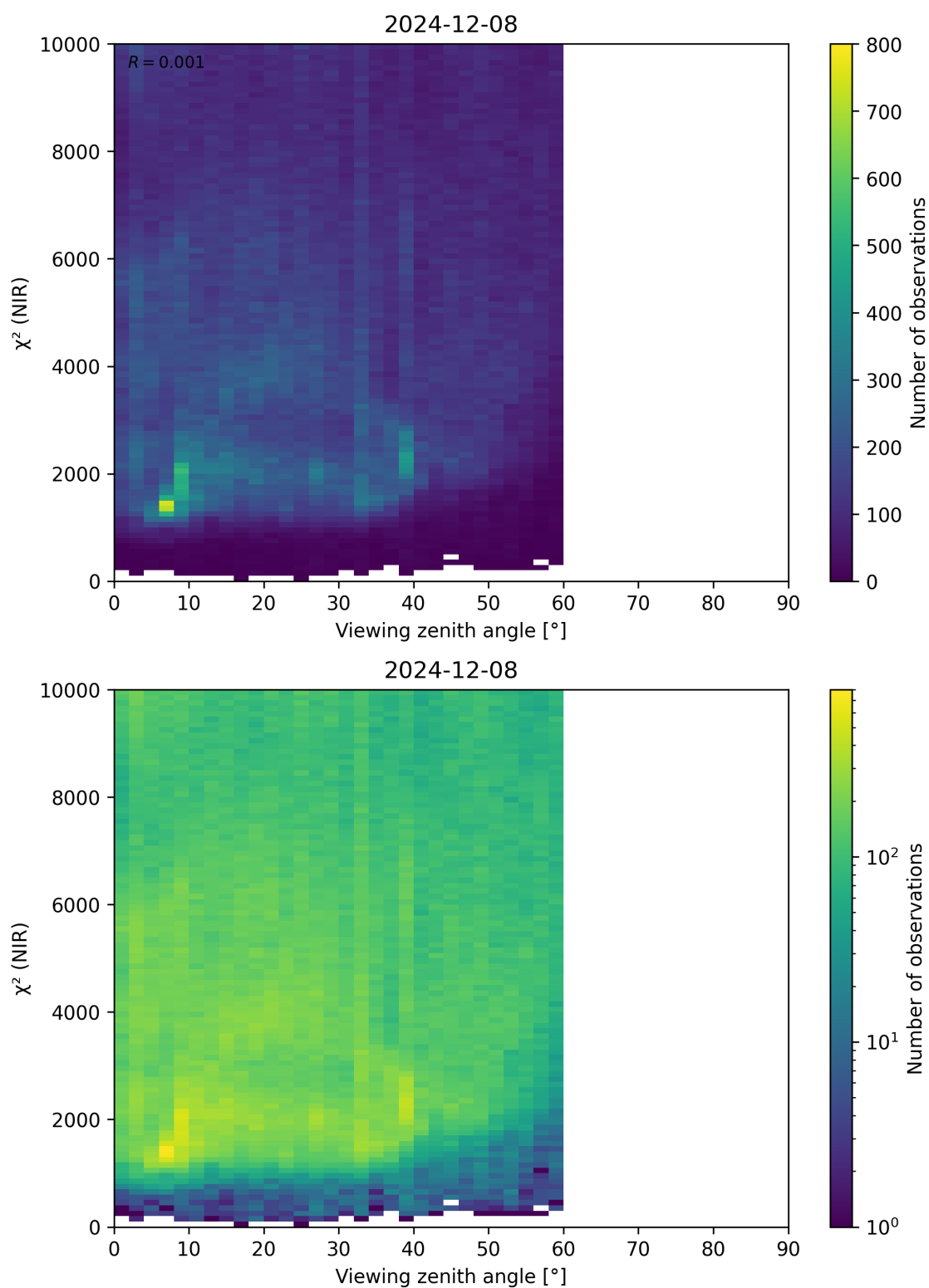
Figure 105: Scatter density plot of “Viewing zenith angle” against “ \chi^2 (NIR)” for 2024-12-07 to 2024-12-09.
