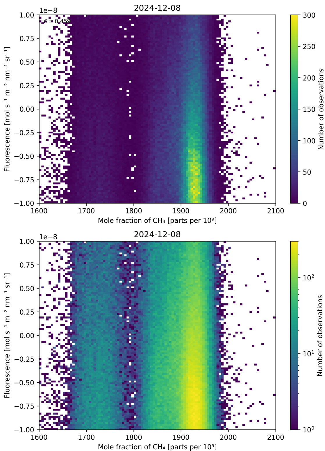
Figure 73: Scatter density plot of “Mole fraction of \text{CH}_4 ” against “Fluorescence” for 2024-12-07 to 2024-12-09.
