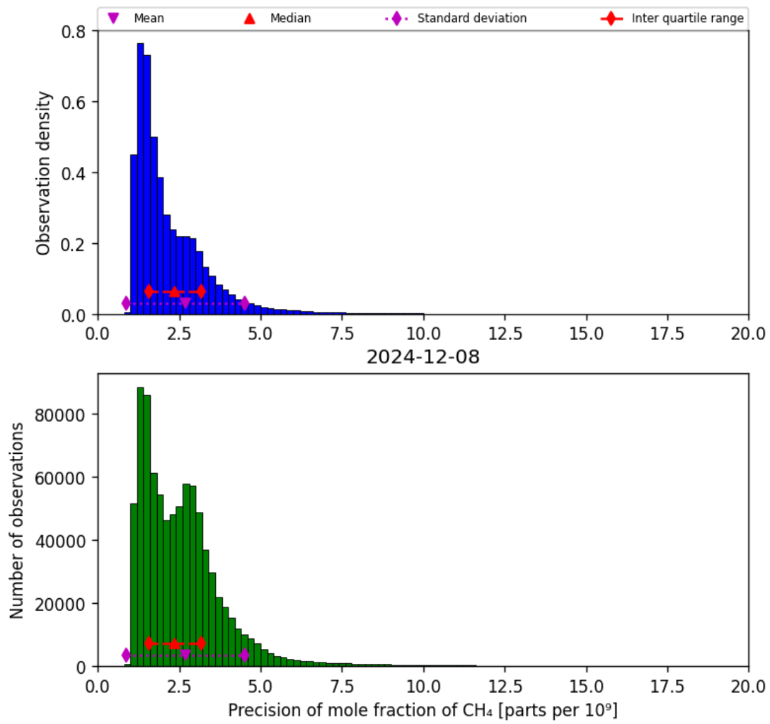
Figure 24: Histogram of “Precision of mole fraction of CH 4 ” for 2024-12-07 to 2024-12-09
