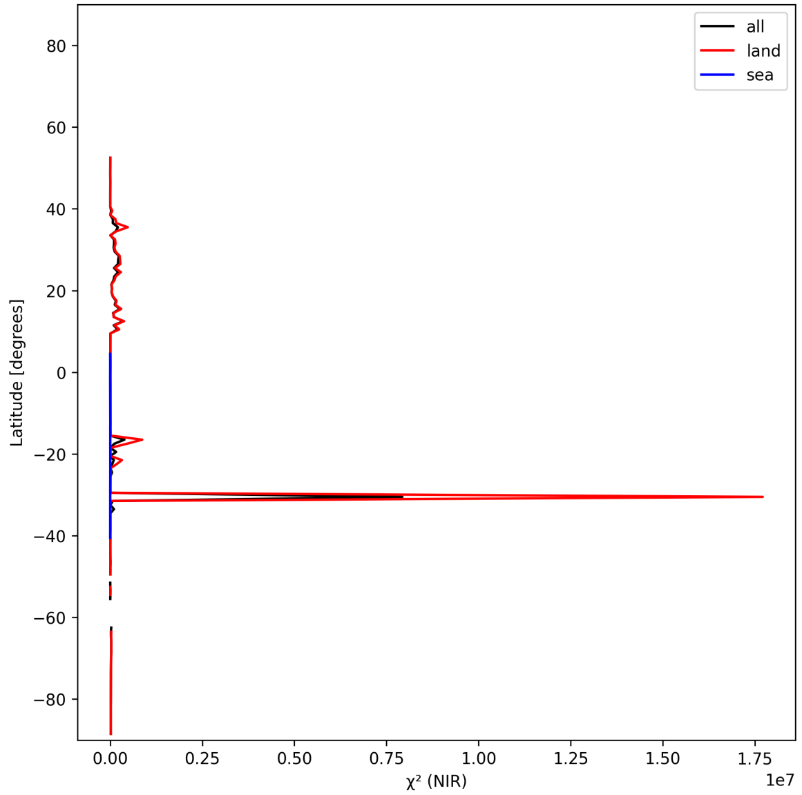
Figure 18: Zonal average of “ \chi^2 (NIR)” for 2024-12-07 to 2024-12-09.
