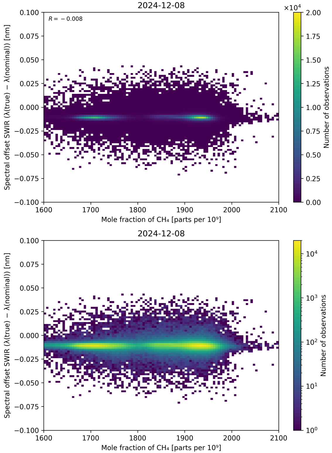
Figure 86: Scatter density plot of “Mole fraction of CH 4 ” against “Spectral offset SWIR ( \lambda_{\text{true}} - \lambda_{\text{nominal}} )” for 2024-12-07 to 2024-12-09.
