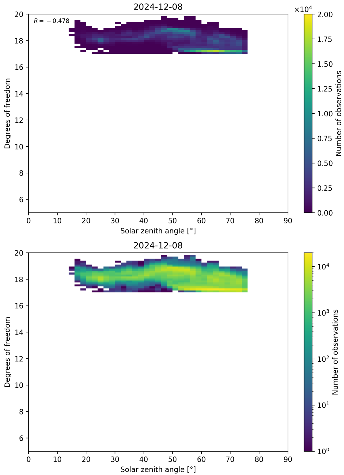
Figure 96: Scatter density plot of “Solar zenith angle” against “Degrees of freedom” for 2024-12-07 to 2024-12-09.
