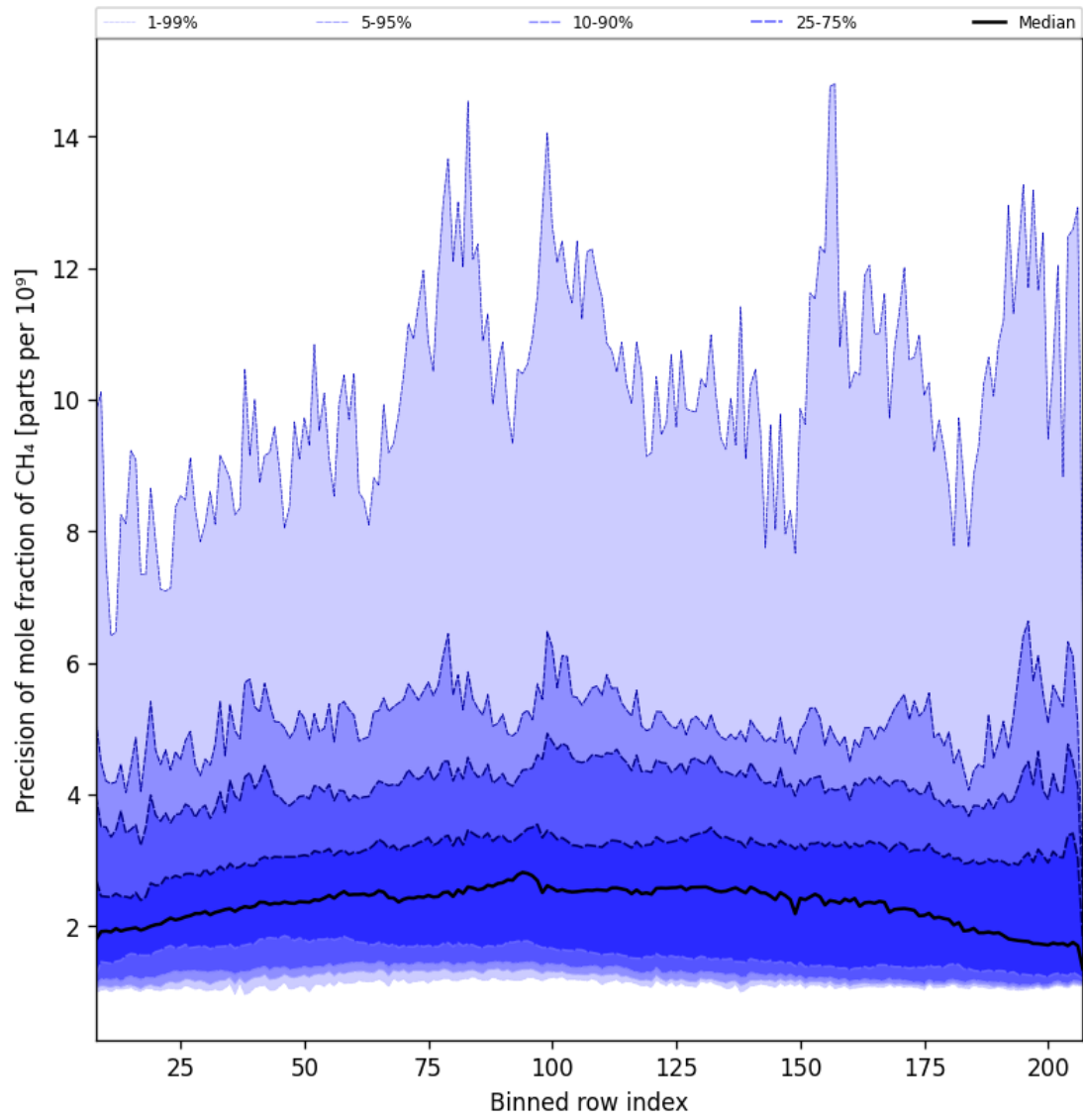
Figure 35: Along track statistics of “Precision of mole fraction of CH 4 ” for 2024-12-07 to 2024-12-09
