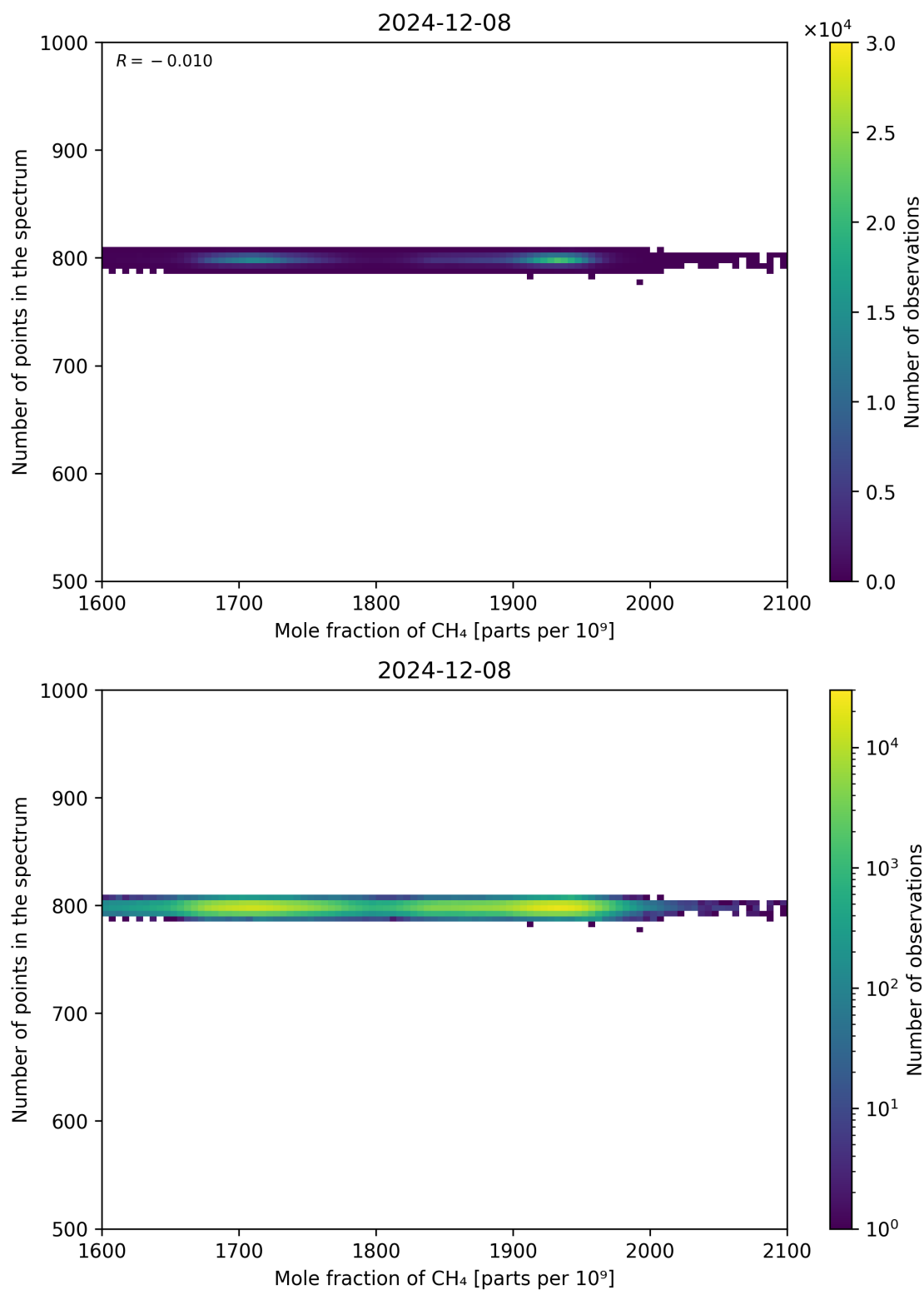
Figure 77: Scatter density plot of “Mole fraction of CH 4 ” against “Number of points in the spectrum” for 2024-12-07 to 2024-12-09.
