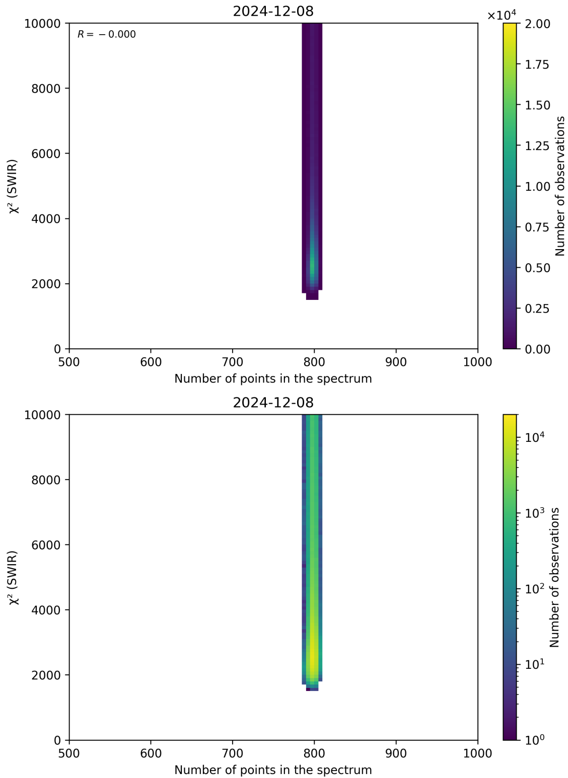
Figure 89: Scatter density plot of “Number of points in the spectrum” against “ \chi^2 (SWIR)” for 2024-12-07 to 2024-12-09.
