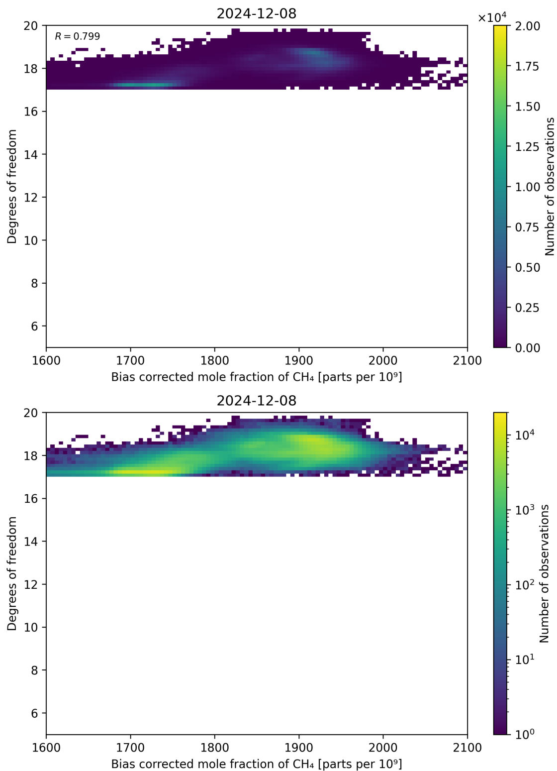
Figure 65: Scatter density plot of “Bias corrected mole fraction of \text{CH}_4 ” against “Degrees of freedom” for 2024-12-07 to 2024-12-09.
