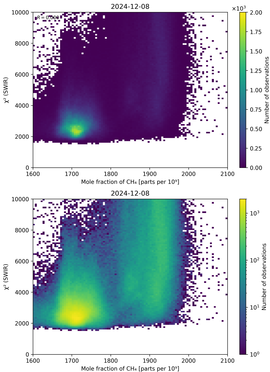
Figure 71: Scatter density plot of “Mole fraction of CH 4 ” against “ \chi^2 (SWIR)” for 2024-12-07 to 2024-12-09.
