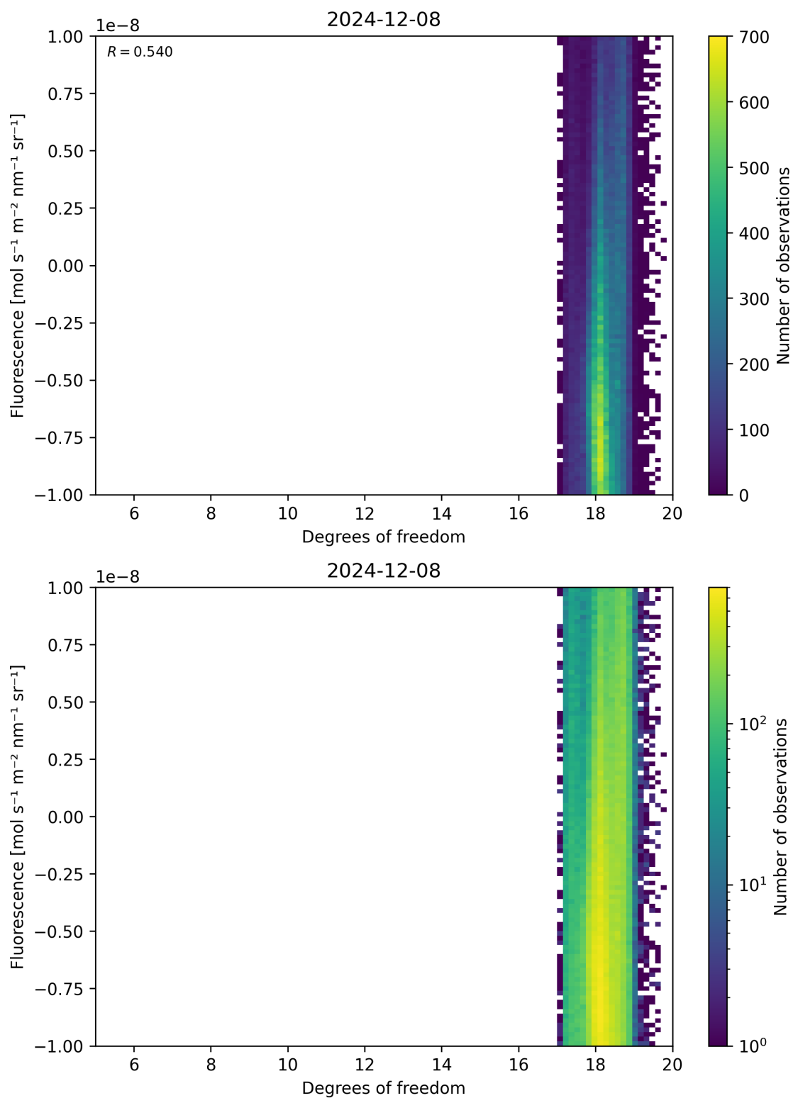
Figure 51: Scatter density plot of “Degrees of freedom” against “Fluorescence” for 2024-12-07 to 2024-12-09.
