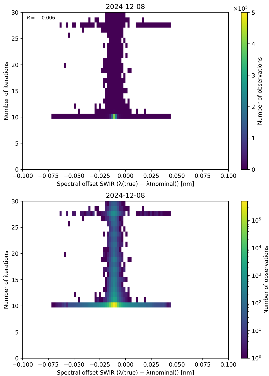
Figure 121: Scatter density plot of “Spectral offset SWIR ( \lambda_{\text{true}} - \lambda_{\text{nominal}} )” against “Number of iterations” for 2024-12-07 to 2024-12-09.
