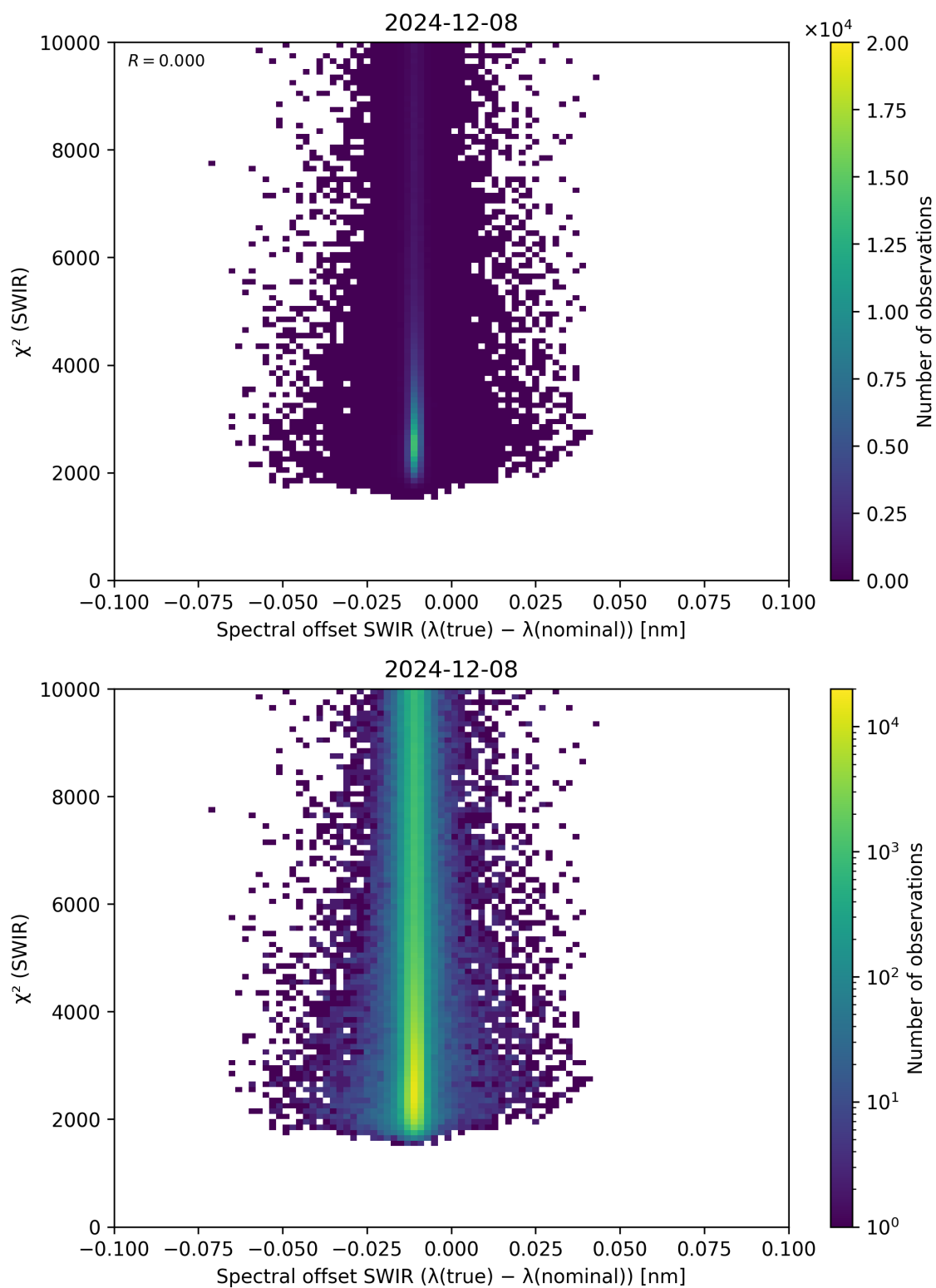
Figure 118: Scatter density plot of “Spectral offset SWIR ( \lambda_{\text{true}} - \lambda_{\text{nominal}} )” against “ \chi^2 (SWIR)” for 2024-12-07 to 2024-12-09.
