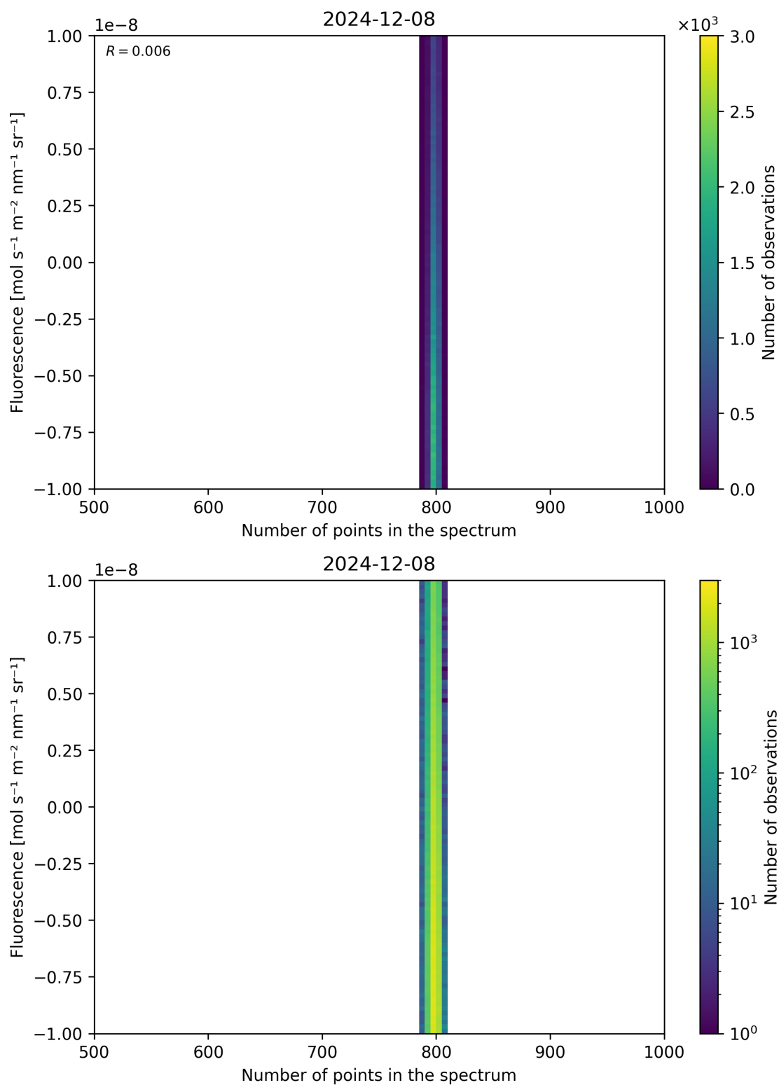
Figure 91: Scatter density plot of “Number of points in the spectrum” against “Fluorescence” for 2024-12-07 to 2024-12-09.
