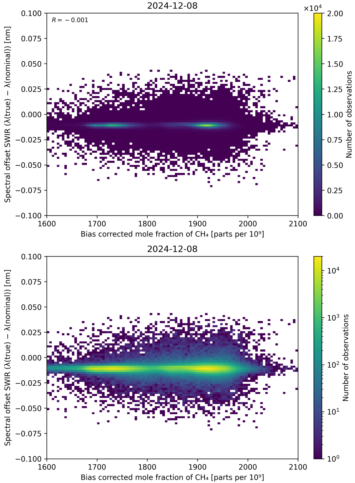
Figure 69: Scatter density plot of “Bias corrected mole fraction of \text{CH}_4 ” against “Spectral offset SWIR ( \lambda_{\text{true}} - \lambda_{\text{nominal}} )” for 2024-12-07 to 2024-12-09.
