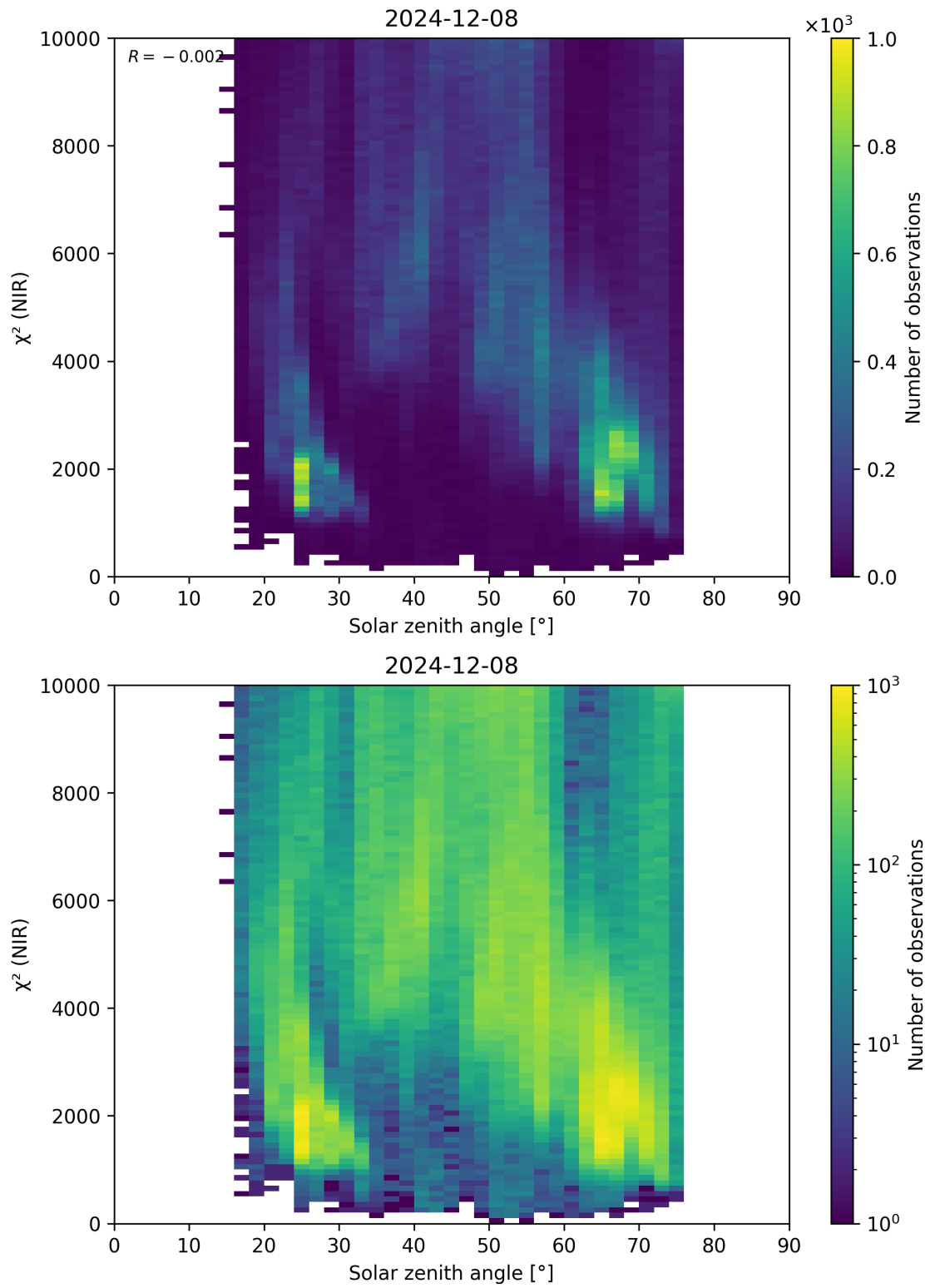
Figure 94: Scatter density plot of “Solar zenith angle” against “ \chi^2 (NIR)” for 2024-12-07 to 2024-12-09.
