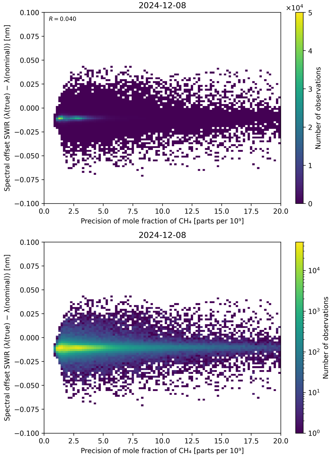
Figure 85: Scatter density plot of “Precision of mole fraction of \text{CH}_4 ” against “Spectral offset SWIR ( \lambda_{\text{true}} - \lambda_{\text{nominal}} )” for 2024-12-07 to 2024-12-09.
