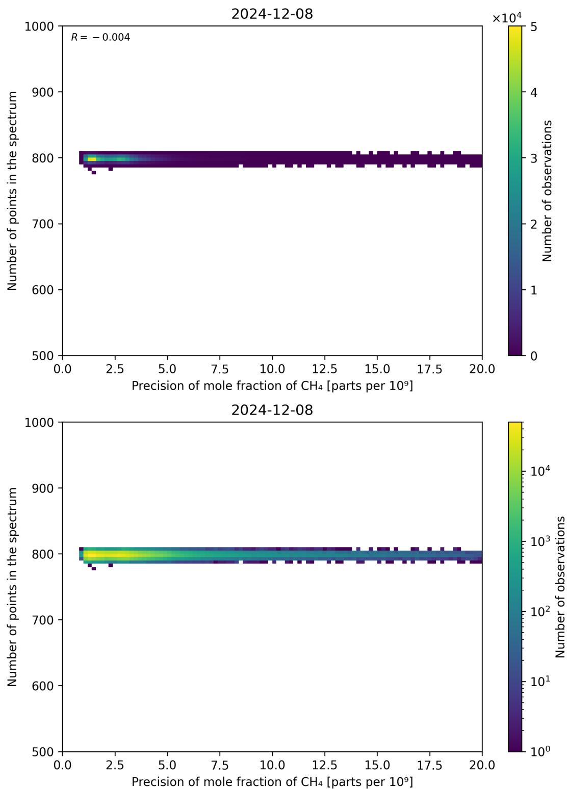
Figure 84: Scatter density plot of “Precision of mole fraction of CH 4 ” against “Number of points in the spectrum” for 2024-12-07 to 2024-12-09.
