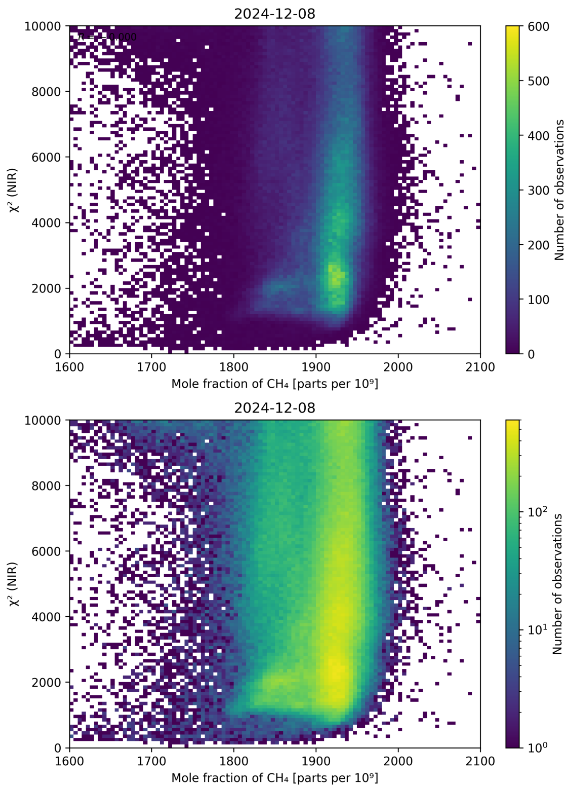
Figure 70: Scatter density plot of “Mole fraction of CH 4 ” against “ \chi^2 (NIR)” for 2024-12-07 to 2024-12-09.
