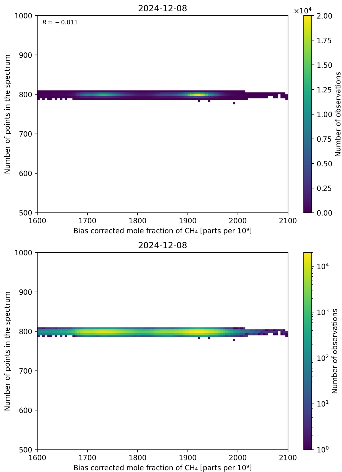
Figure 68: Scatter density plot of “Bias corrected mole fraction of CH 4 ” against “Number of points in the spectrum” for 2024-12-07 to 2024-12-09.
