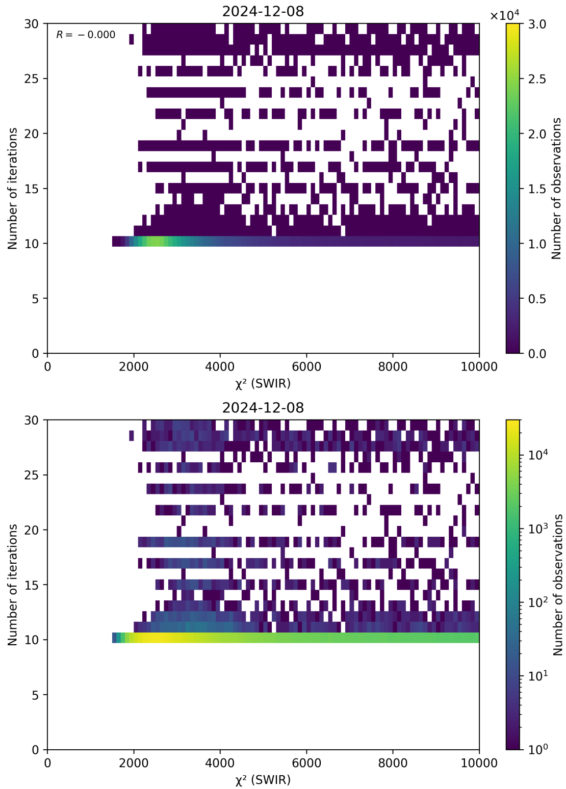
Figure 50: Scatter density plot of “ \chi^2 (SWIR)” against “Number of iterations” for 2024-12-07 to 2024-12-09.
