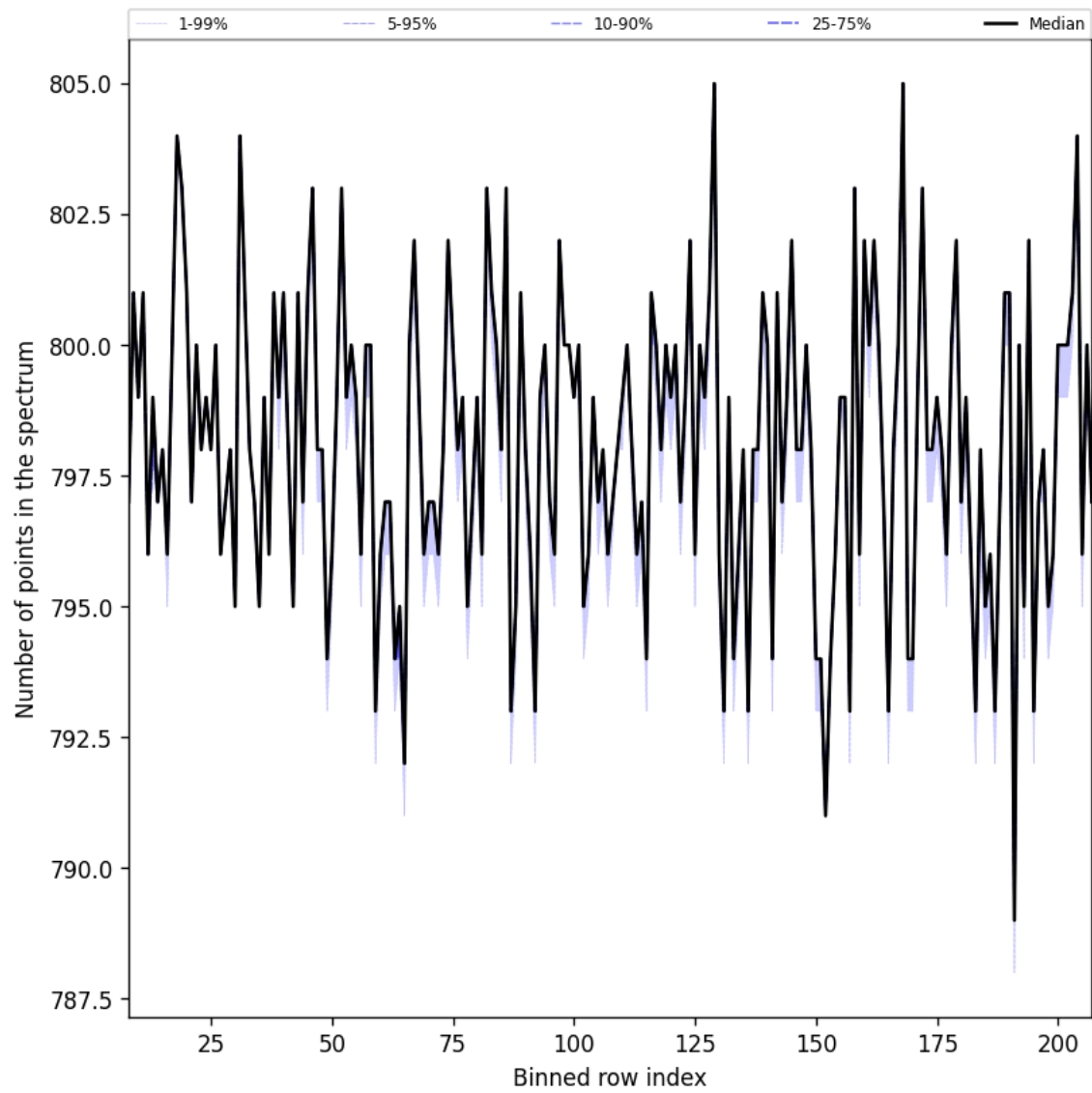
Figure 37: Along track statistics of “Number of points in the spectrum” for 2024-12-07 to 2024-12-09
