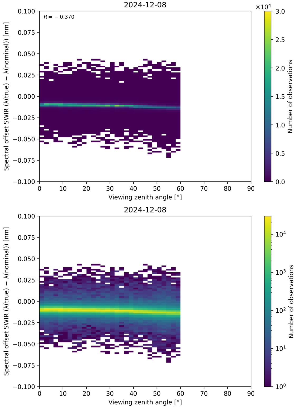
Figure 116: Scatter density plot of “Viewing zenith angle” against “Spectral offset SWIR ( \lambda_{\text{true}} - \lambda_{\text{nominal}} )” for 2024-12-07 to 2024-12-09.
