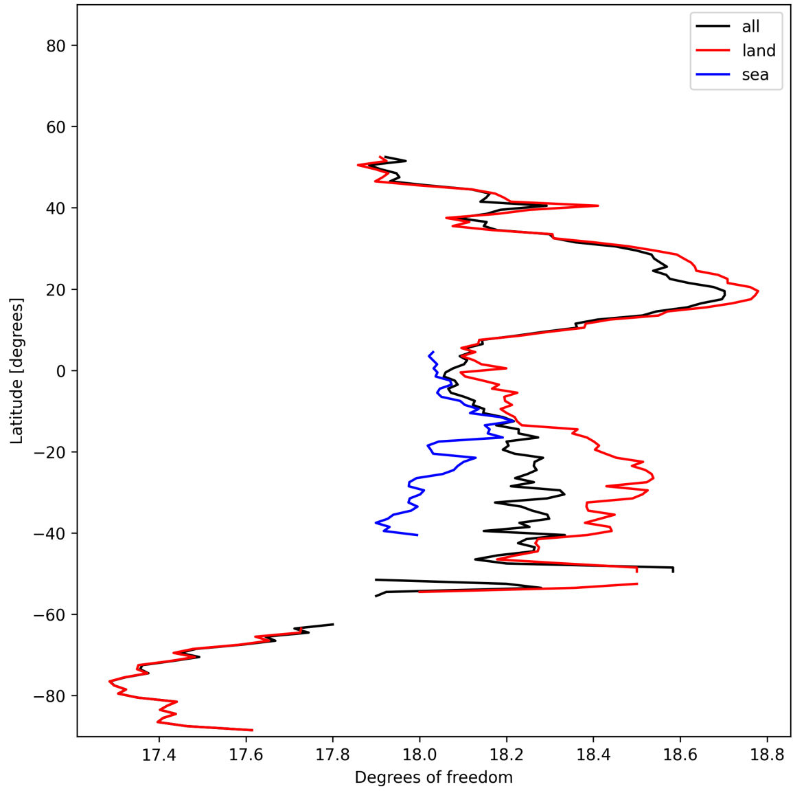
Figure 19: Zonal average of “Degrees of freedom” for 2024-12-07 to 2024-12-09.
