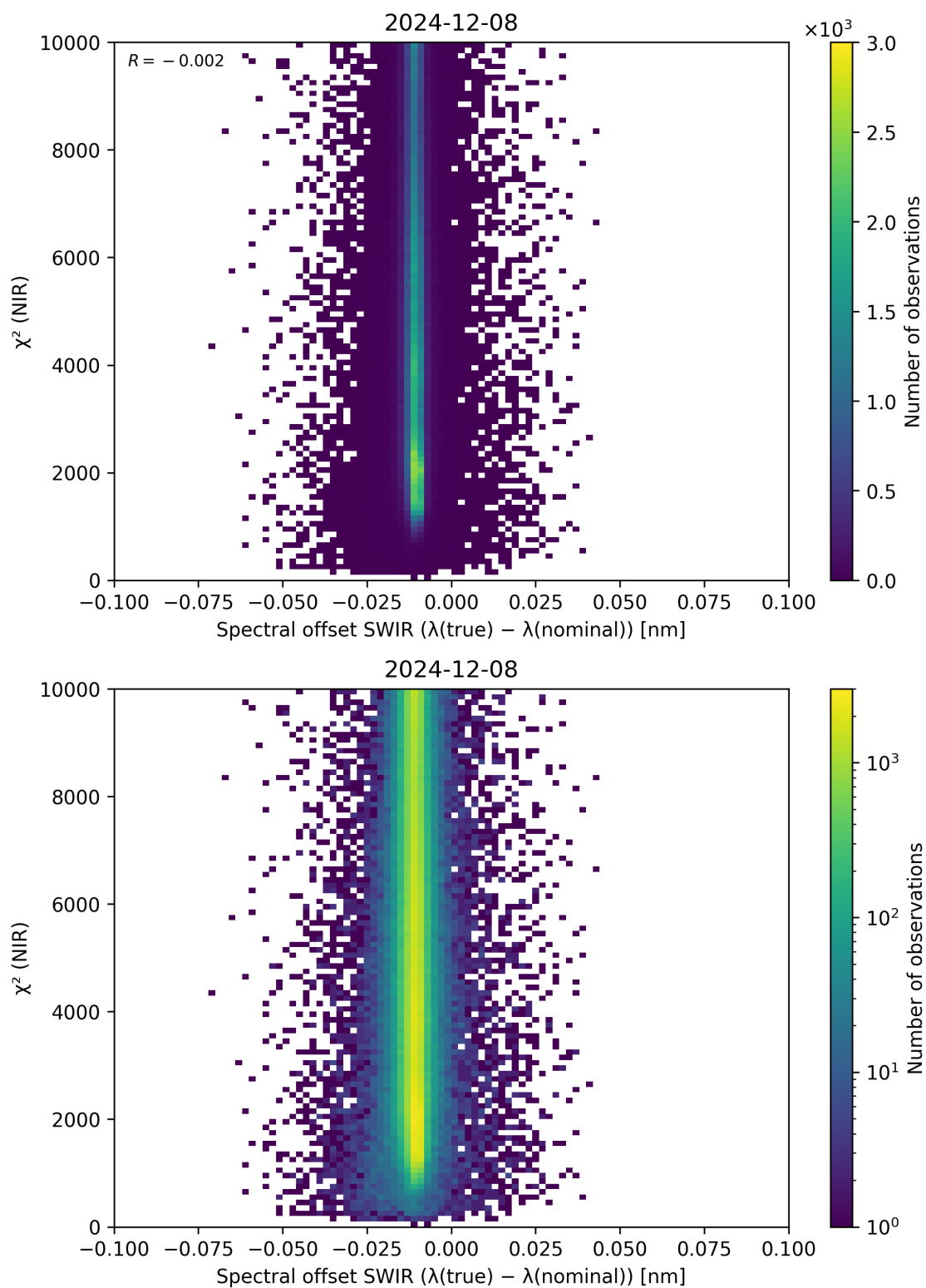
Figure 117: Scatter density plot of “Spectral offset SWIR ( \lambda_{\text{true}} - \lambda_{\text{nominal}} )” against “ \chi^2 (NIR)” for 2024-12-07 to 2024-12-09.
