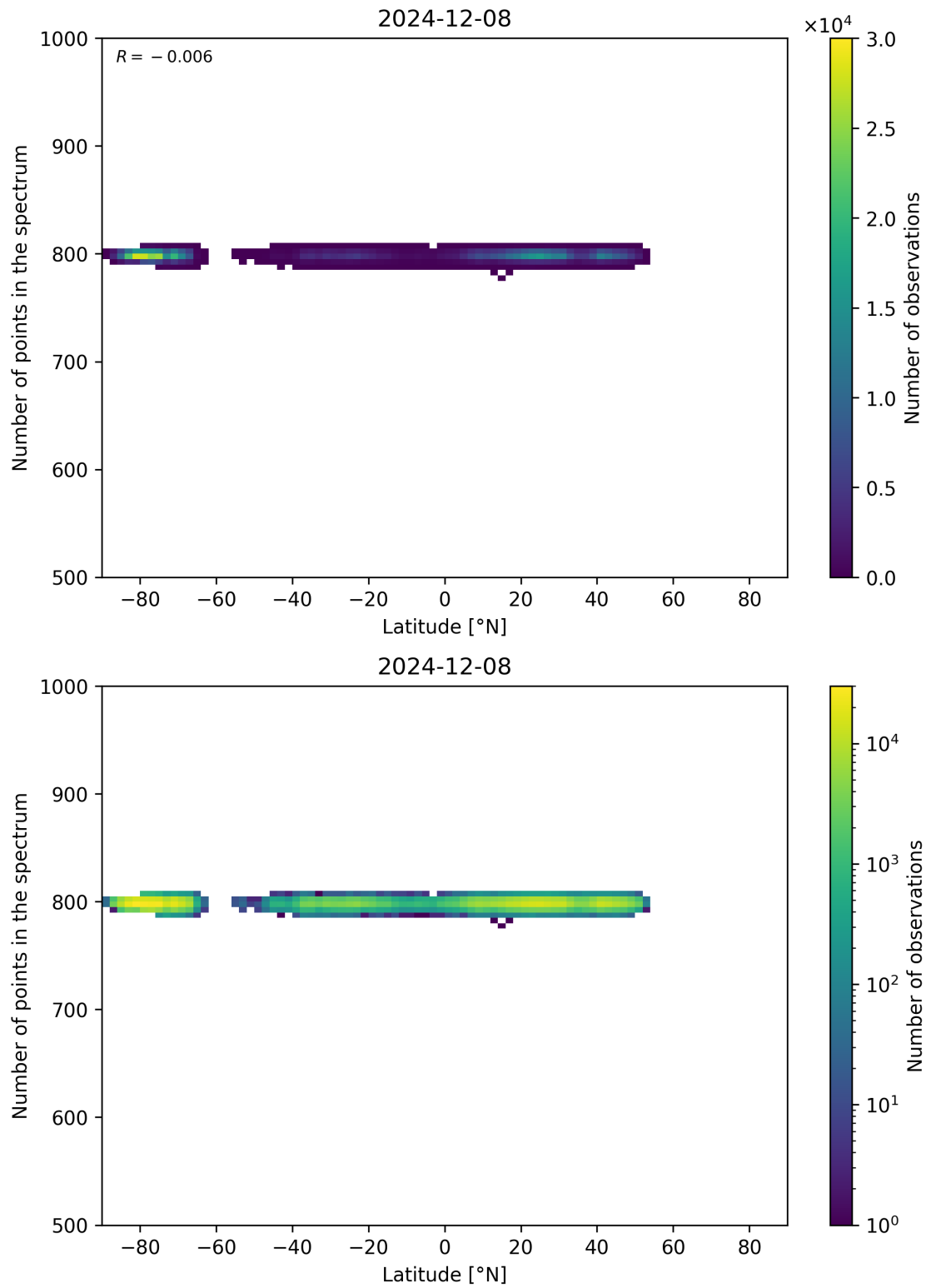
Figure 61: Scatter density plot of “Latitude” against “Number of points in the spectrum” for 2024-12-07 to 2024-12-09.
