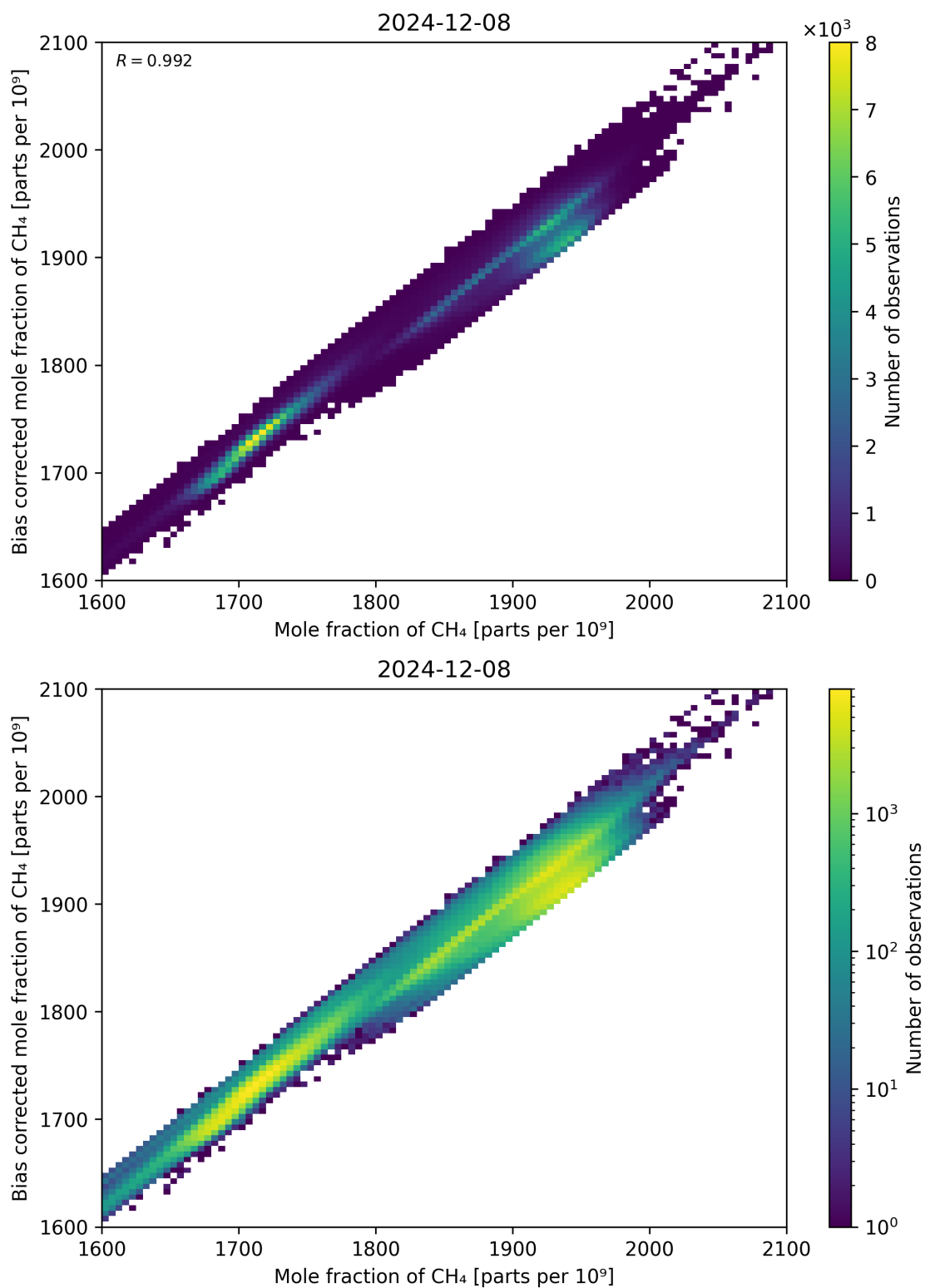
Figure 74: Scatter density plot of “Mole fraction of CH 4 ” against “Bias corrected mole fraction of CH 4 ” for 2024-12-07 to 2024-12-09.
