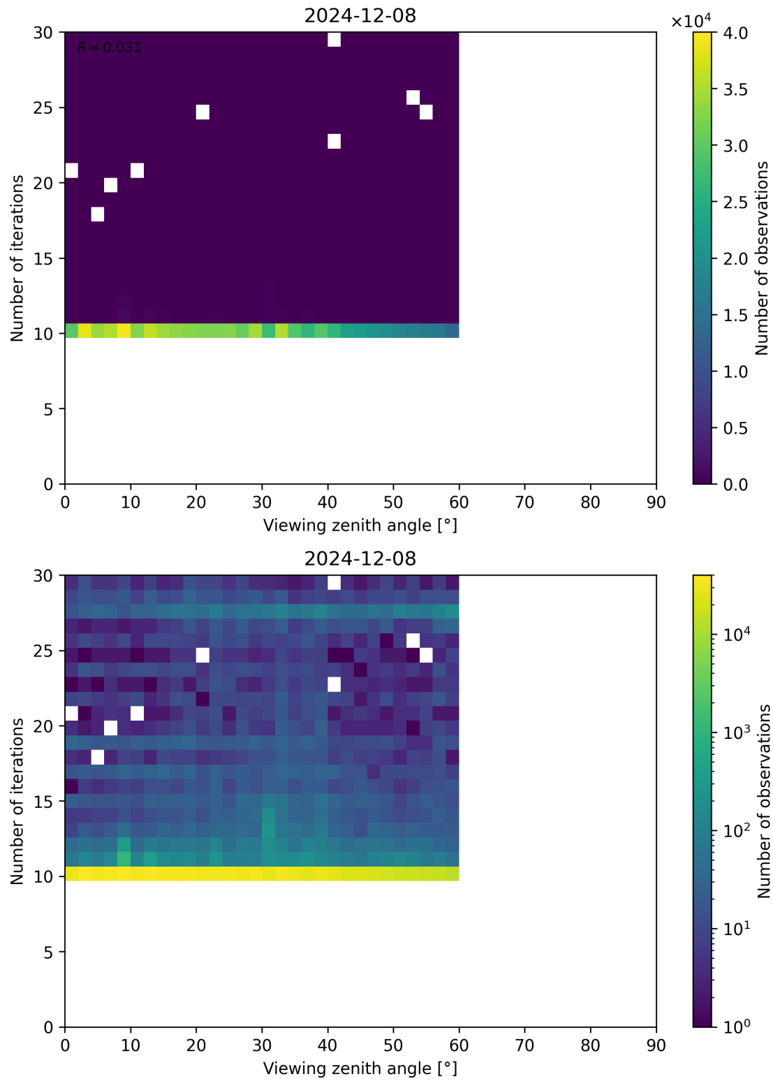
Figure 113: Scatter density plot of “Viewing zenith angle” against “Number of iterations” for 2024-12-07 to 2024-12-09.
