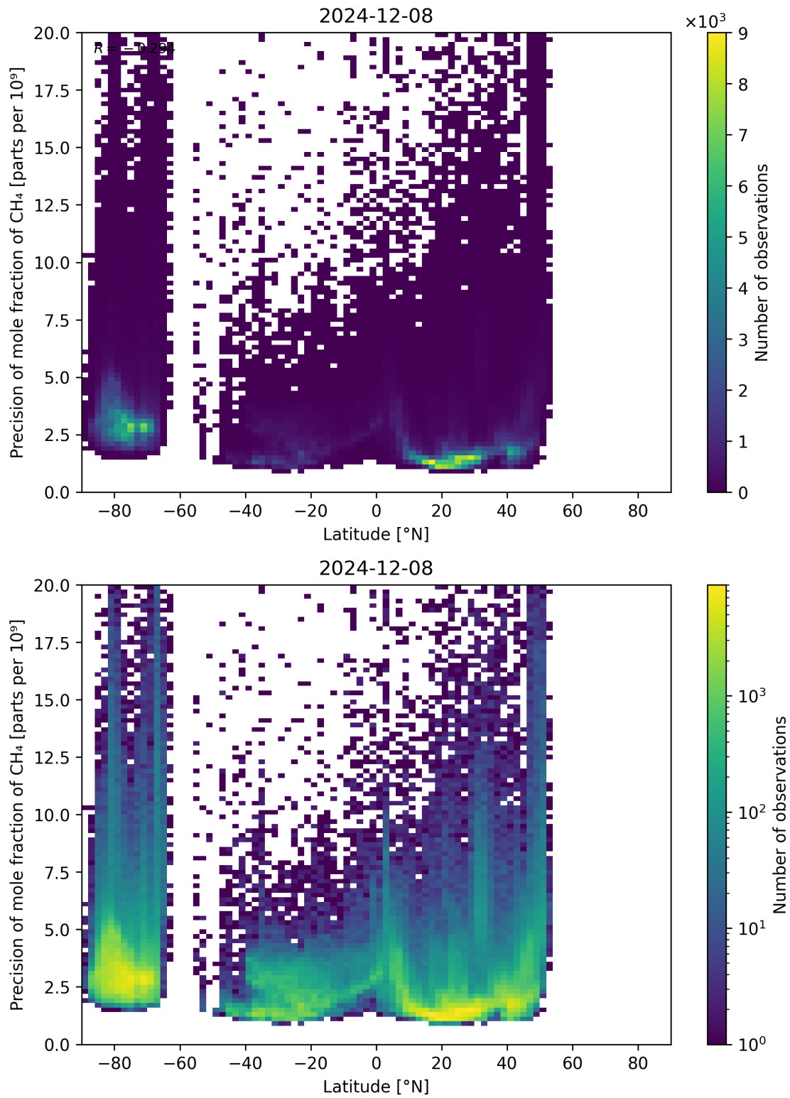
Figure 59: Scatter density plot of “Latitude” against “Precision of mole fraction of CH 4 ” for 2024-12-07 to 2024-12-09.
