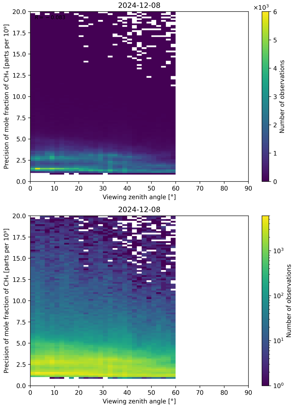
Figure 112: Scatter density plot of “Viewing zenith angle” against “Precision of mole fraction of CH 4 ” for 2024-12-07 to 2024-12-09.
