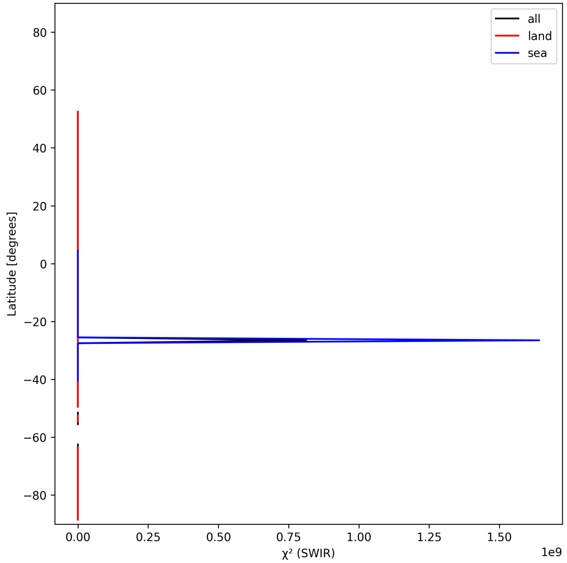
Figure 17: Zonal average of “ \chi^2 (SWIR)” for 2024-12-07 to 2024-12-09.
