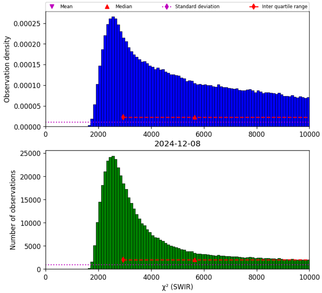
Figure 28: Histogram of “ \chi^2 (SWIR)” for 2024-12-07 to 2024-12-09
