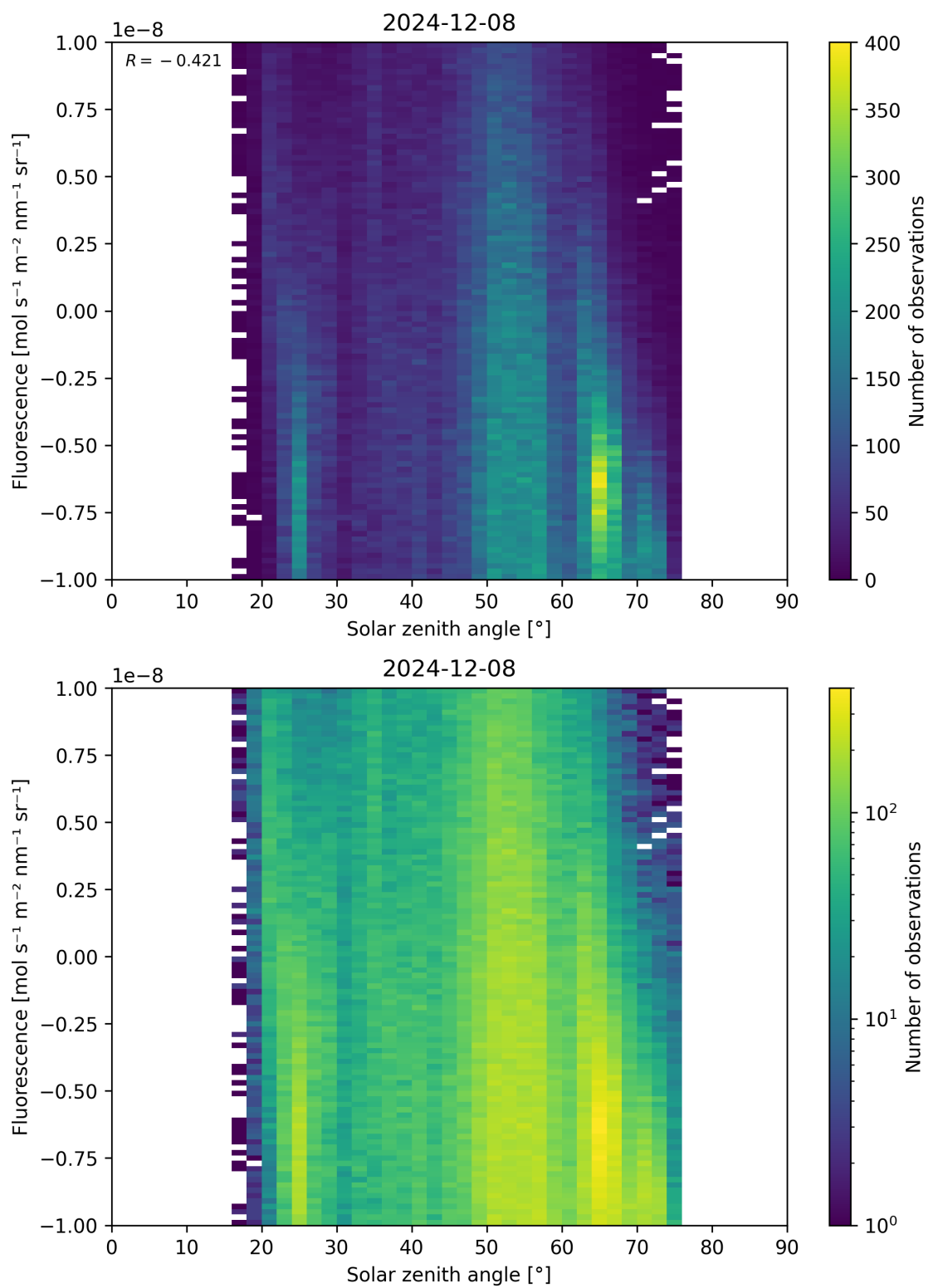
Figure 97: Scatter density plot of “Solar zenith angle” against “Fluorescence” for 2024-12-07 to 2024-12-09.
