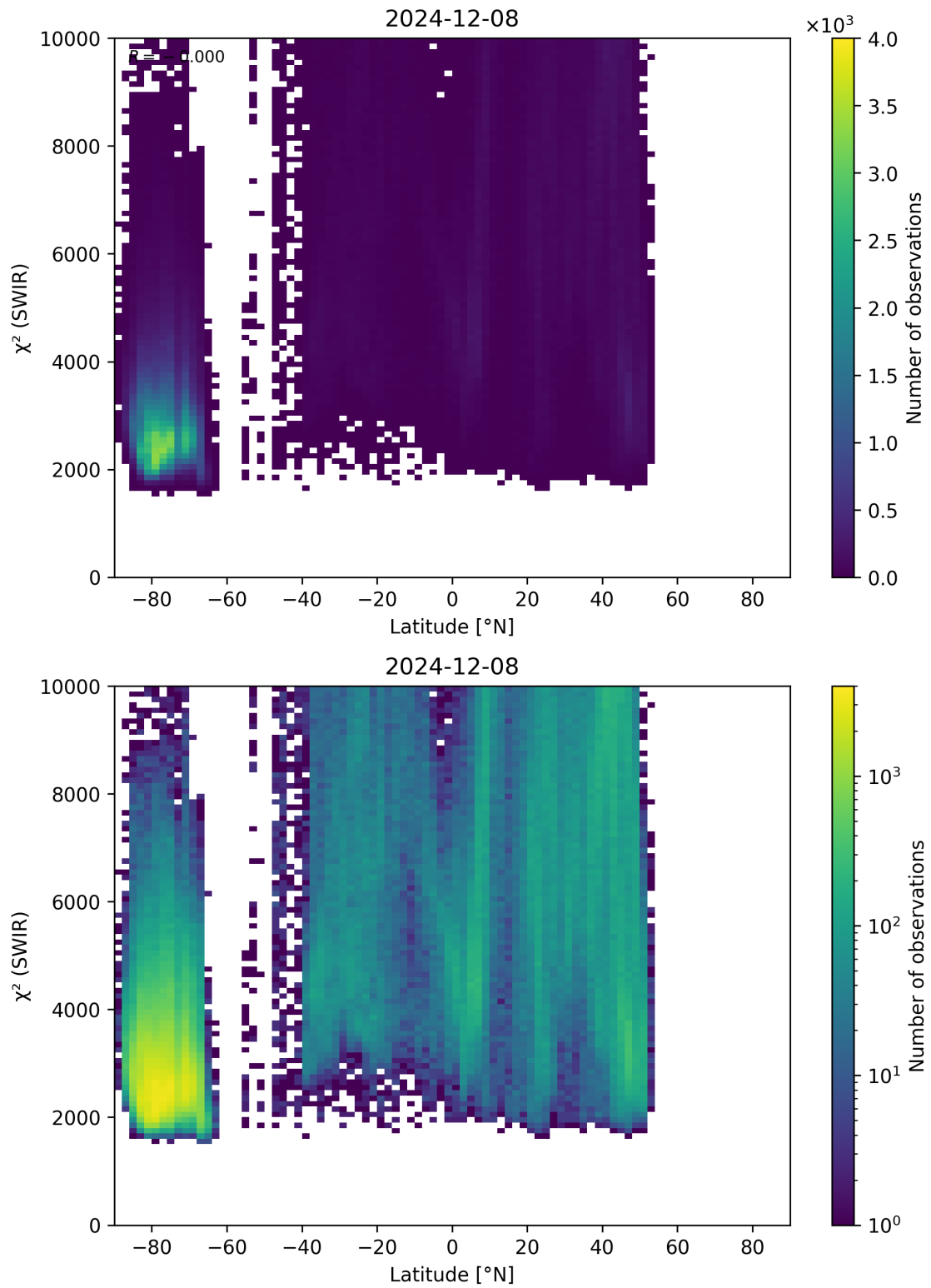
Figure 54: Scatter density plot of “Latitude” against “ \chi^2 (SWIR)” for 2024-12-07 to 2024-12-09.
