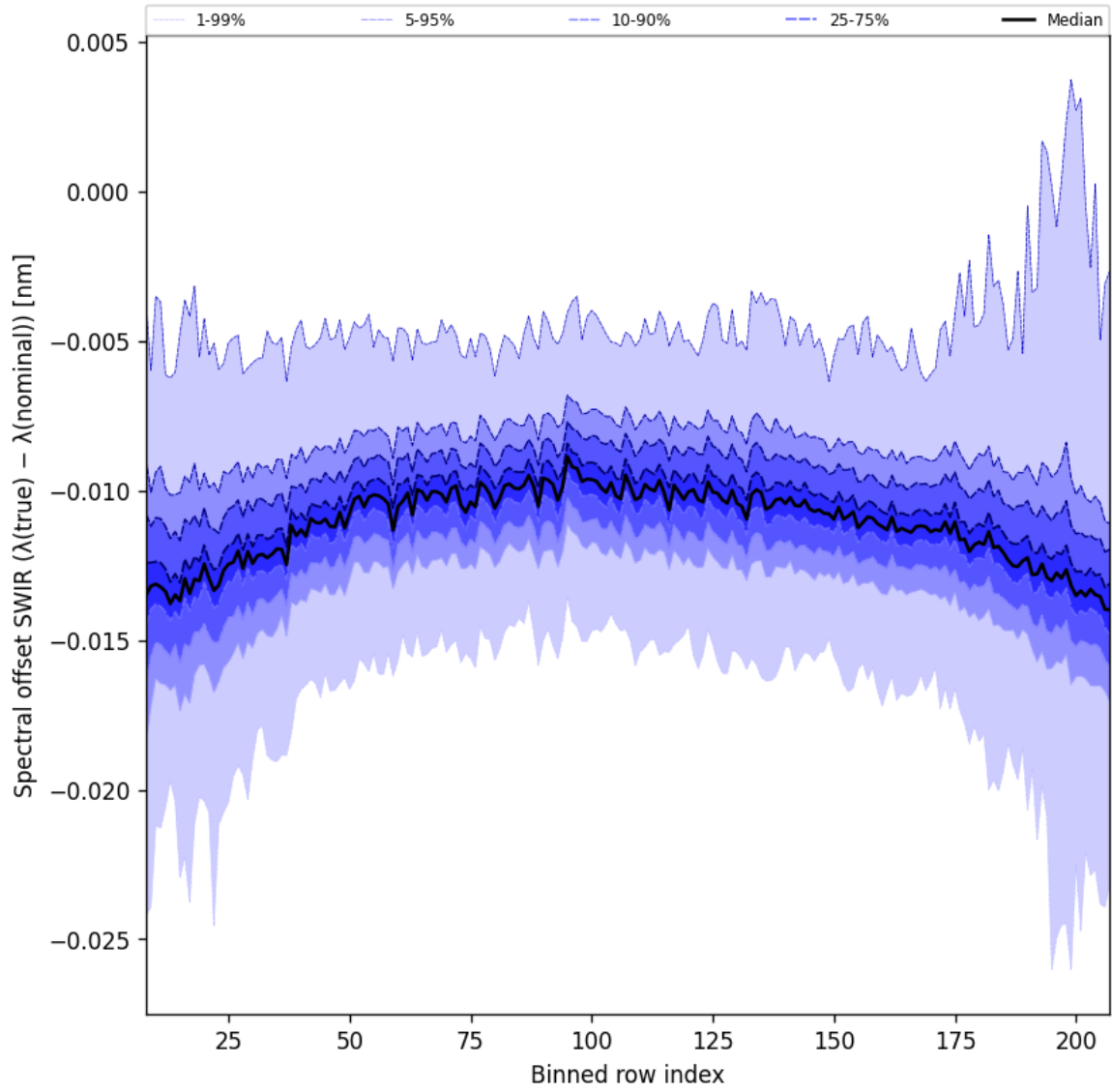
Figure 38: Along track statistics of “Spectral offset SWIR ( \lambda_{\text{true}} - \lambda_{\text{nominal}} )” for 2024-12-07 to 2024-12-09
