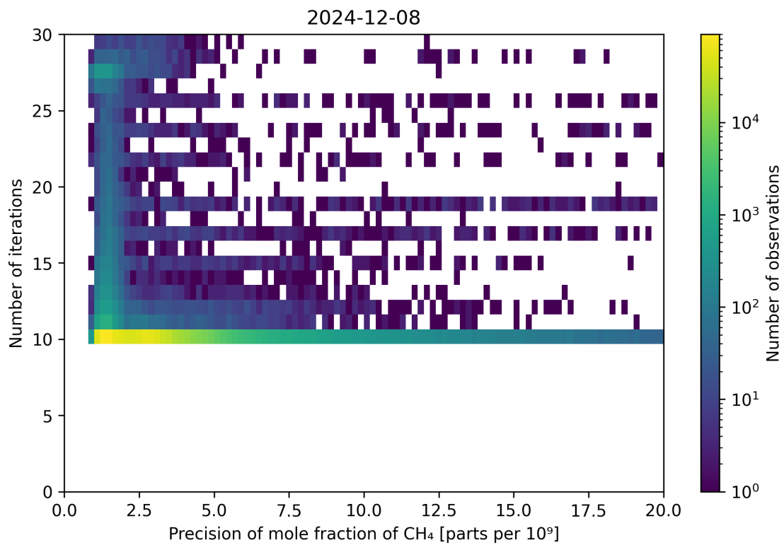
Figure 83: Scatter density plot of “Precision of mole fraction of \text{CH}_4 ” against “Number of iterations” for 2024-12-07 to 2024-12-09.
