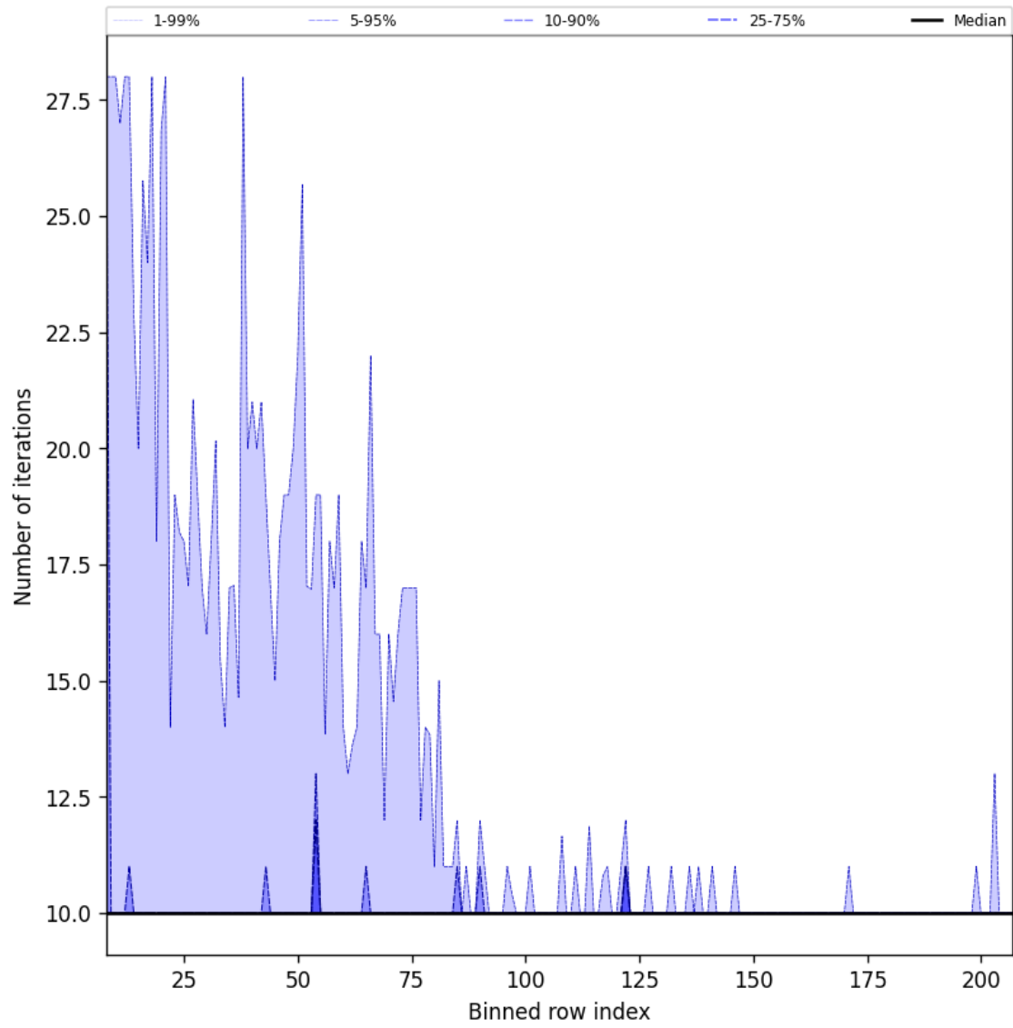
Figure 42: Along track statistics of “Number of iterations” for 2024-12-07 to 2024-12-09
