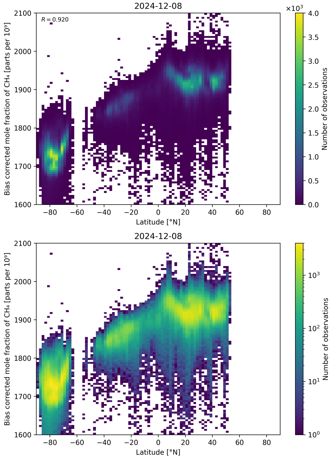
Figure 58: Scatter density plot of “Latitude” against “Bias corrected mole fraction of CH 4 ” for 2024-12-07 to 2024-12-09.
