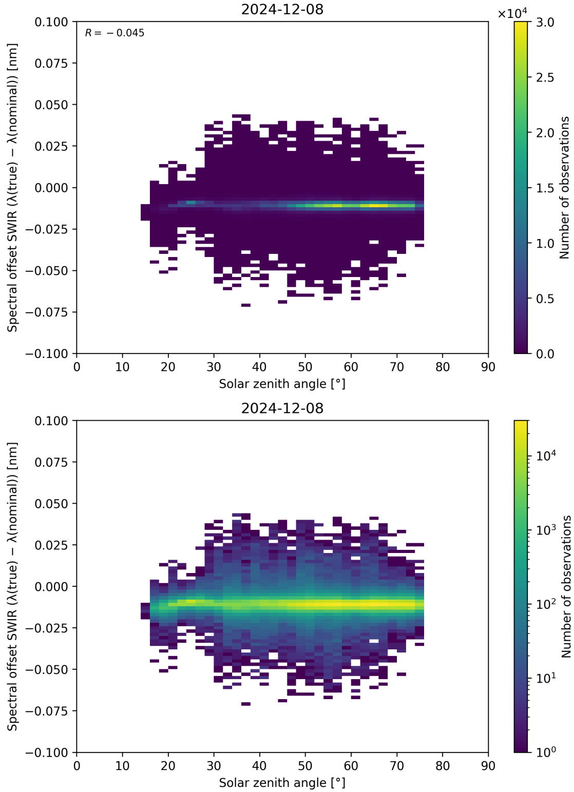
Figure 104: Scatter density plot of “Solar zenith angle” against “Spectral offset SWIR ( \lambda_{\text{true}} - \lambda_{\text{nominal}} )” for 2024-12-07 to 2024-12-09.
