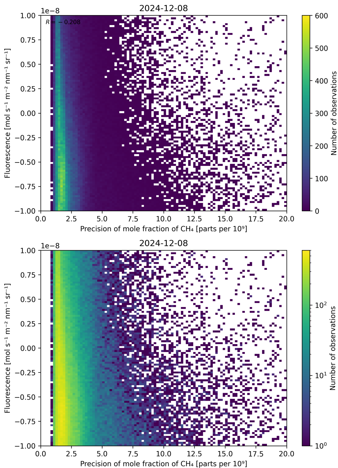
Figure 81: Scatter density plot of “Precision of mole fraction of \text{CH}_4 ” against “Fluorescence” for 2024-12-07 to 2024-12-09.
