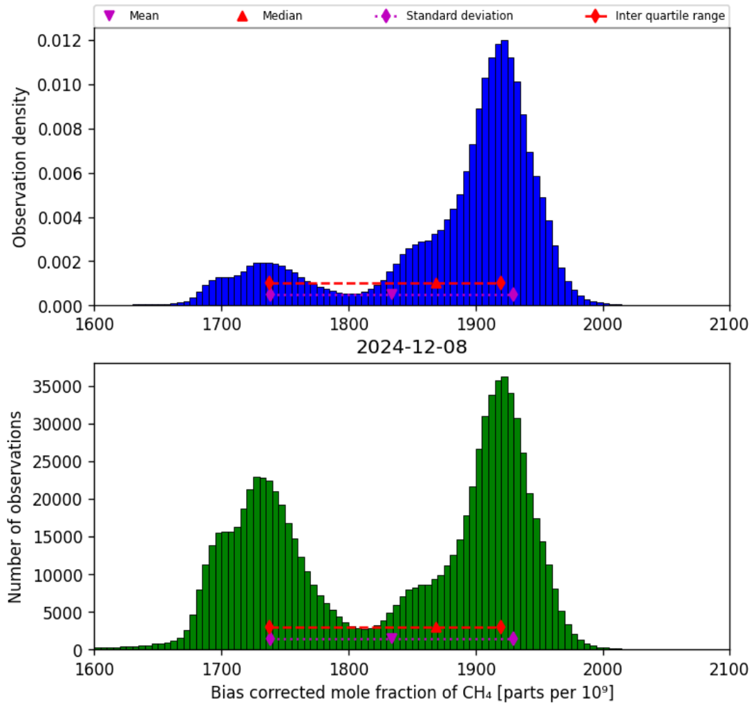
Figure 25: Histogram of “Bias corrected mole fraction of CH 4 ” for 2024-12-07 to 2024-12-09
