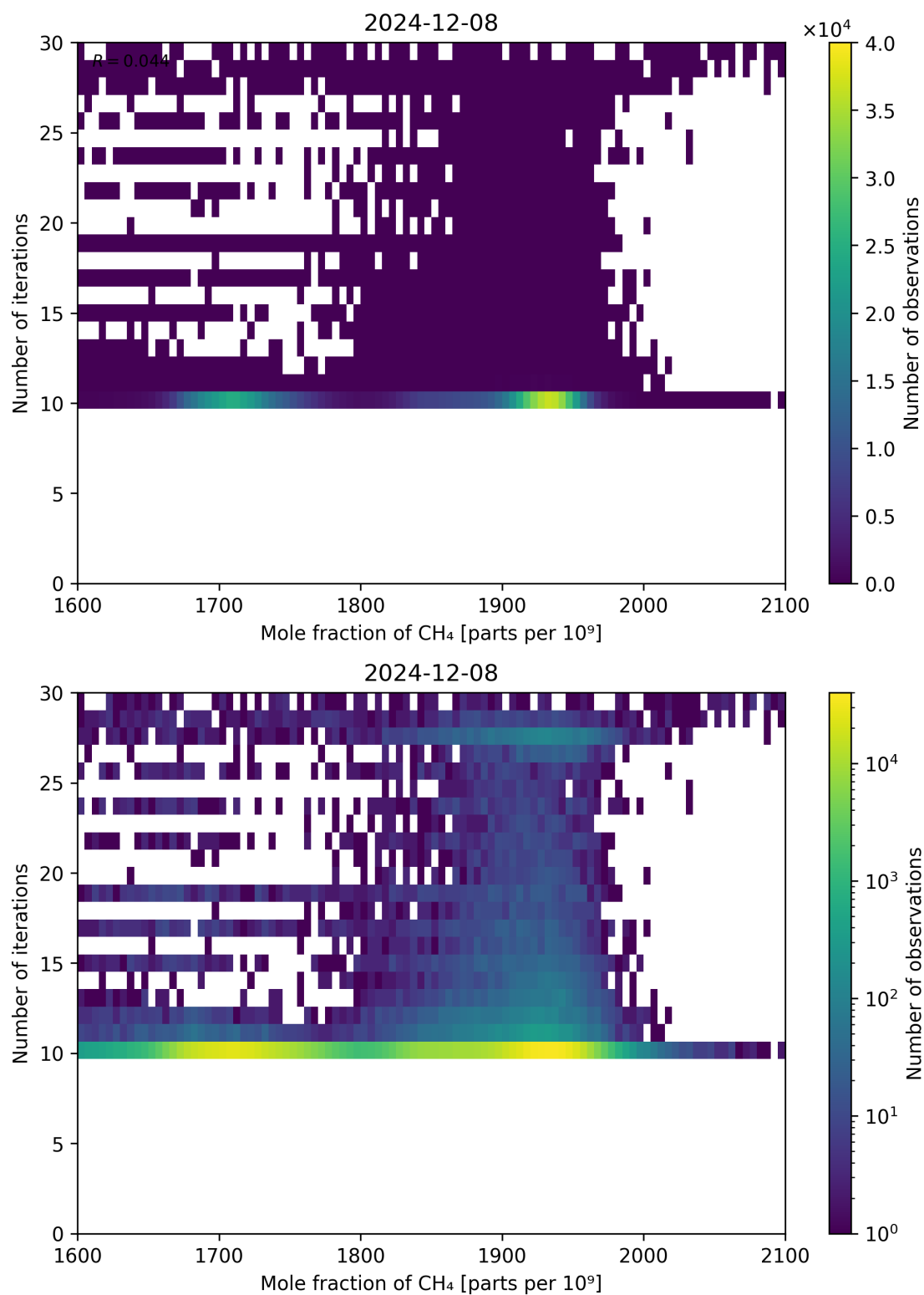
Figure 76: Scatter density plot of “Mole fraction of CH 4 ” against “Number of iterations” for 2024-12-07 to 2024-12-09.
