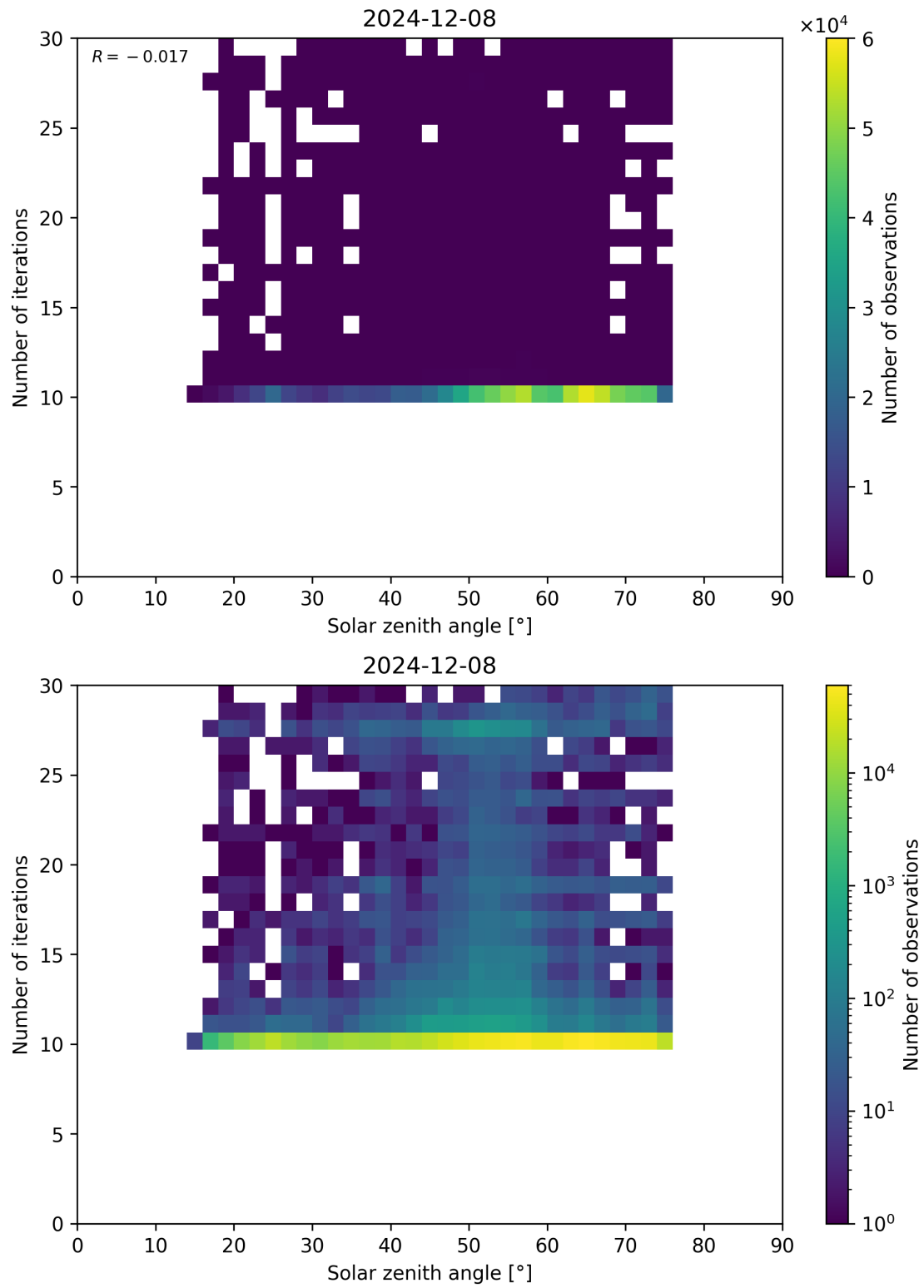
Figure 102: Scatter density plot of “Solar zenith angle” against “Number of iterations” for 2024-12-07 to 2024-12-09.
