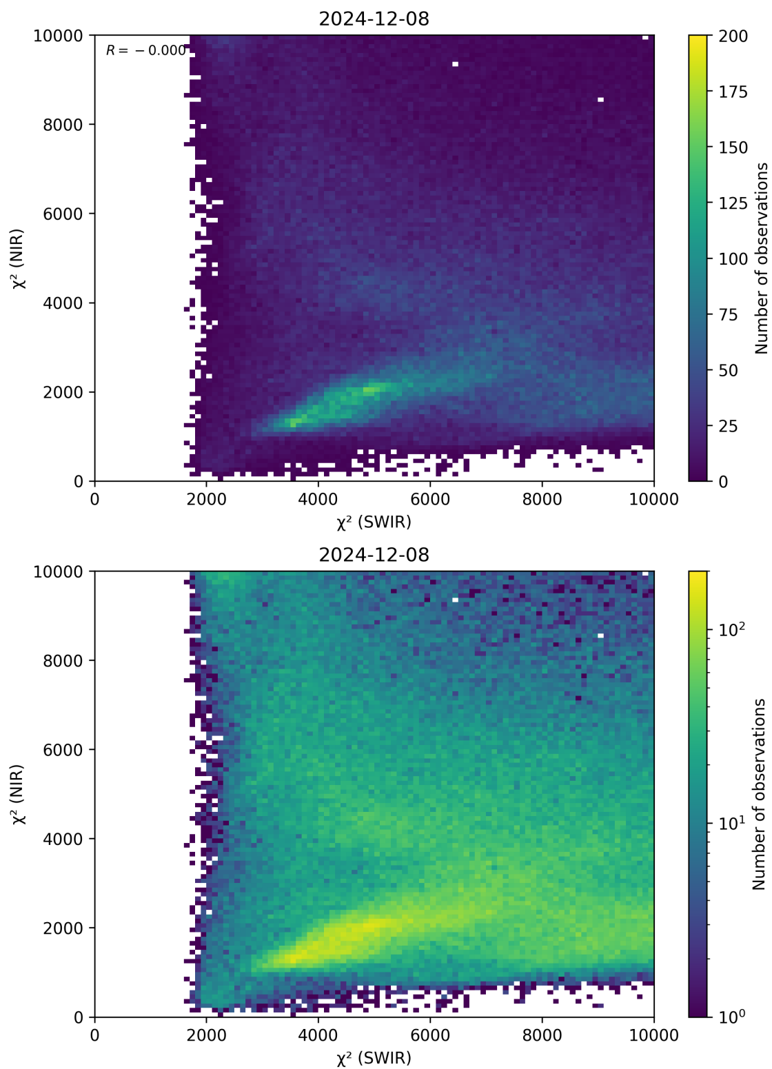
Figure 47: Scatter density plot of “ \chi^2 (SWIR)” against “ \chi^2 (NIR)” for 2024-12-07 to 2024-12-09.
