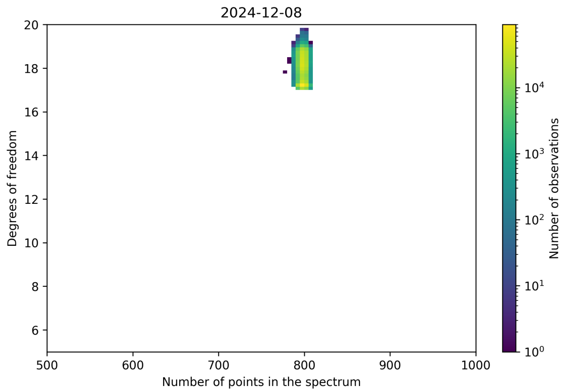
Figure 90: Scatter density plot of “Number of points in the spectrum” against “Degrees of freedom” for 2024-12-07 to 2024-12-09.
