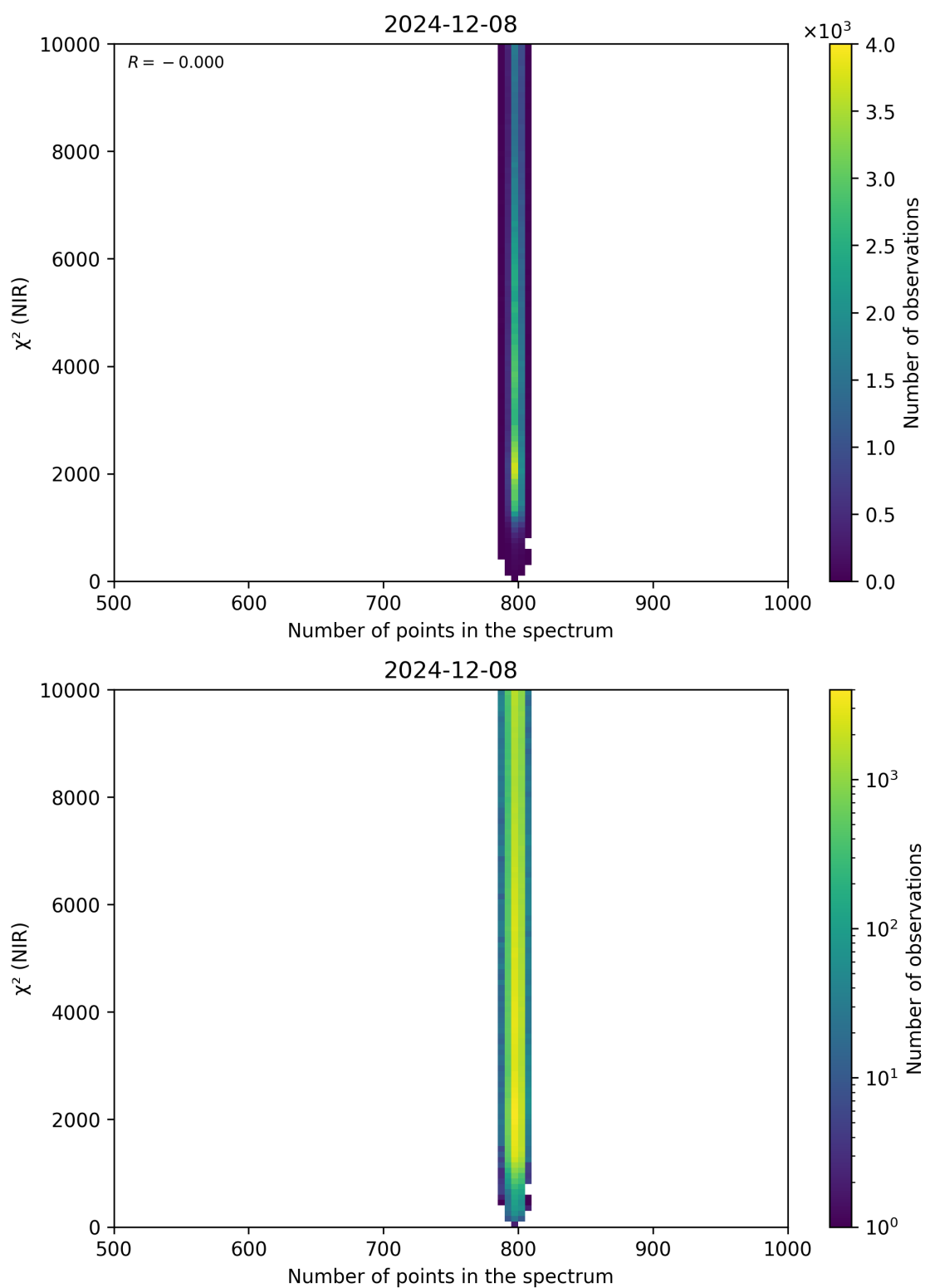
Figure 88: Scatter density plot of “Number of points in the spectrum” against “ \chi^2 (NIR)” for 2024-12-07 to 2024-12-09.
