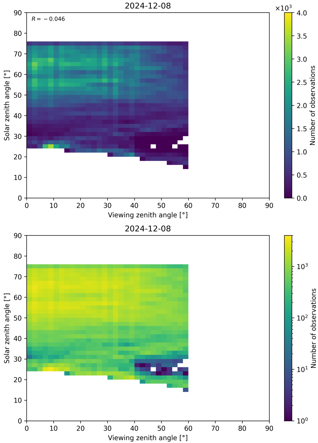
Figure 115: Scatter density plot of “Viewing zenith angle” against “Solar zenith angle” for 2024-12-07 to 2024-12-09.
