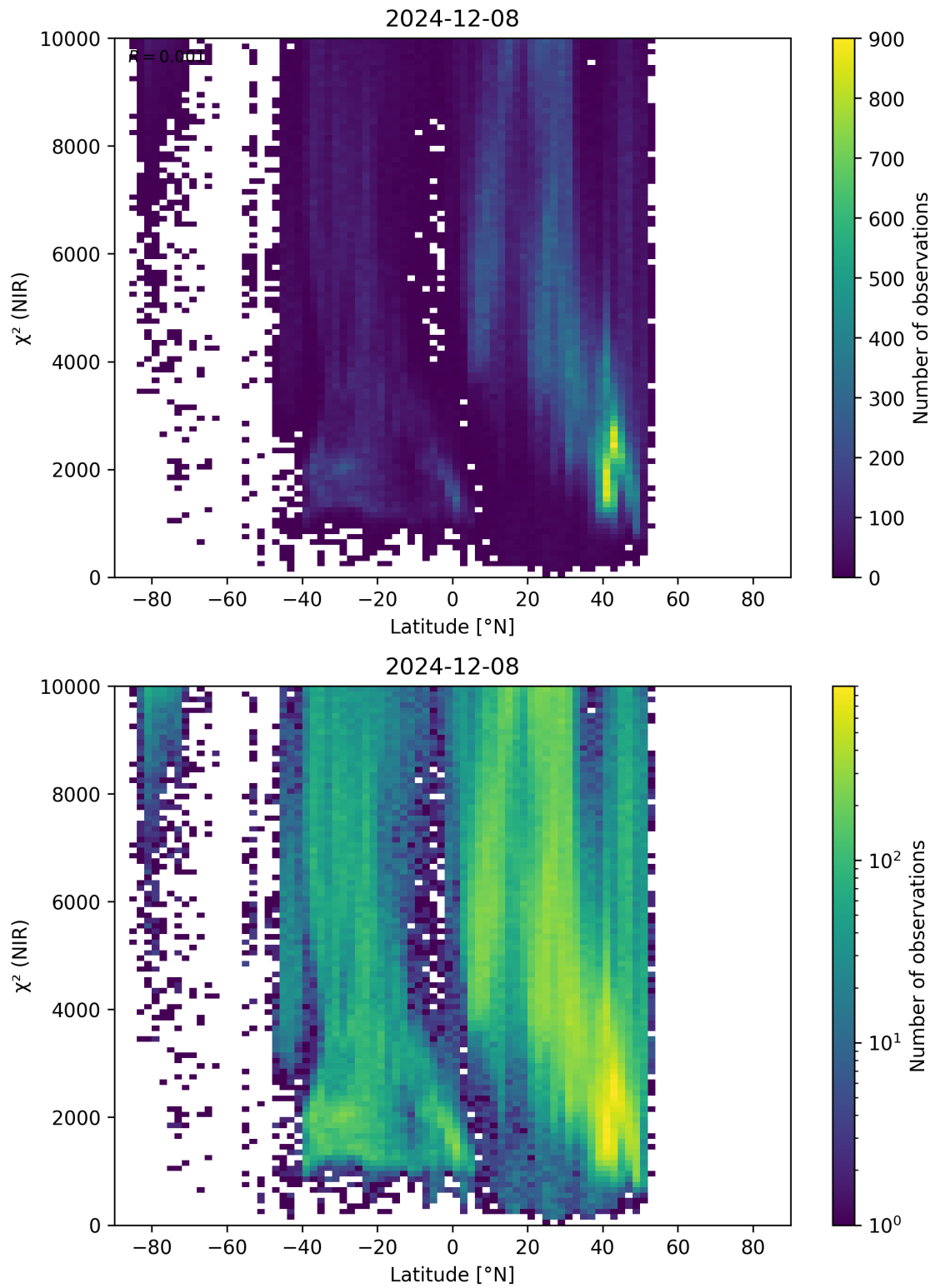
Figure 53: Scatter density plot of “Latitude” against “ \chi^2 (NIR)” for 2024-12-07 to 2024-12-09.
