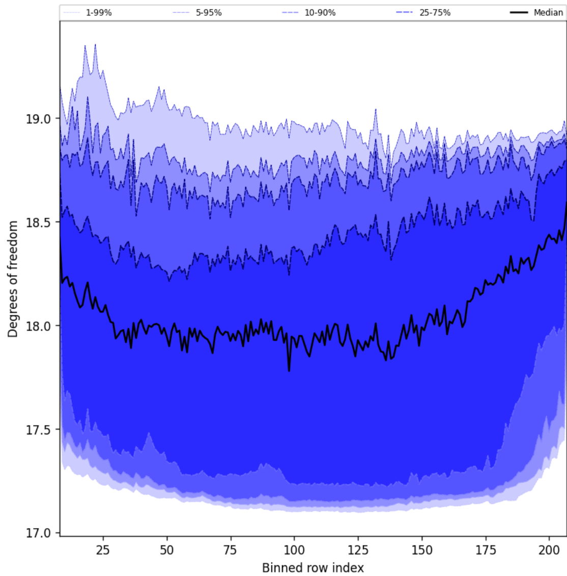
Figure 41: Along track statistics of “Degrees of freedom” for 2024-12-07 to 2024-12-09
