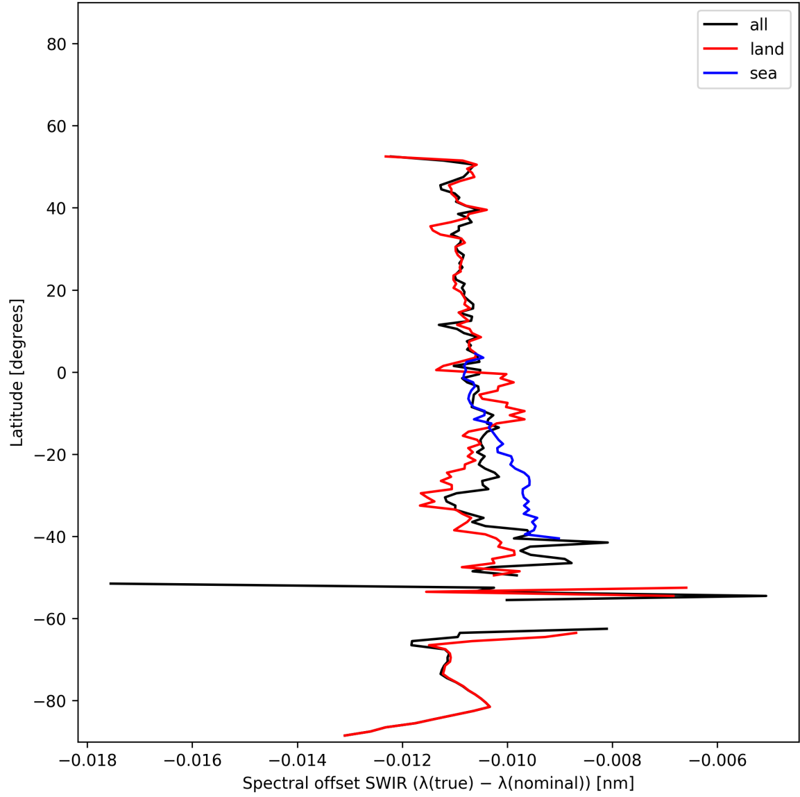
Figure 16: Zonal average of “Spectral offset SWIR ( \lambda_{\text{true}} - \lambda_{\text{nominal}} )” for 2024-12-07 to 2024-12-09.
