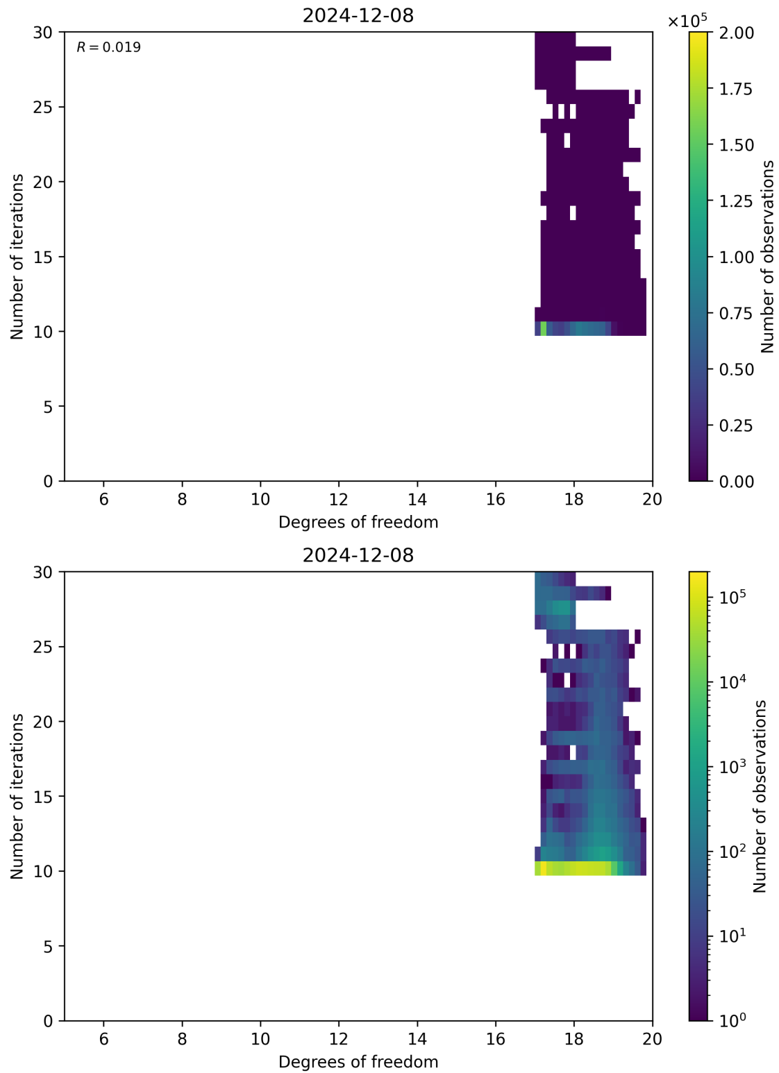
Figure 52: Scatter density plot of “Degrees of freedom” against “Number of iterations” for 2024-12-07 to 2024-12-09.
