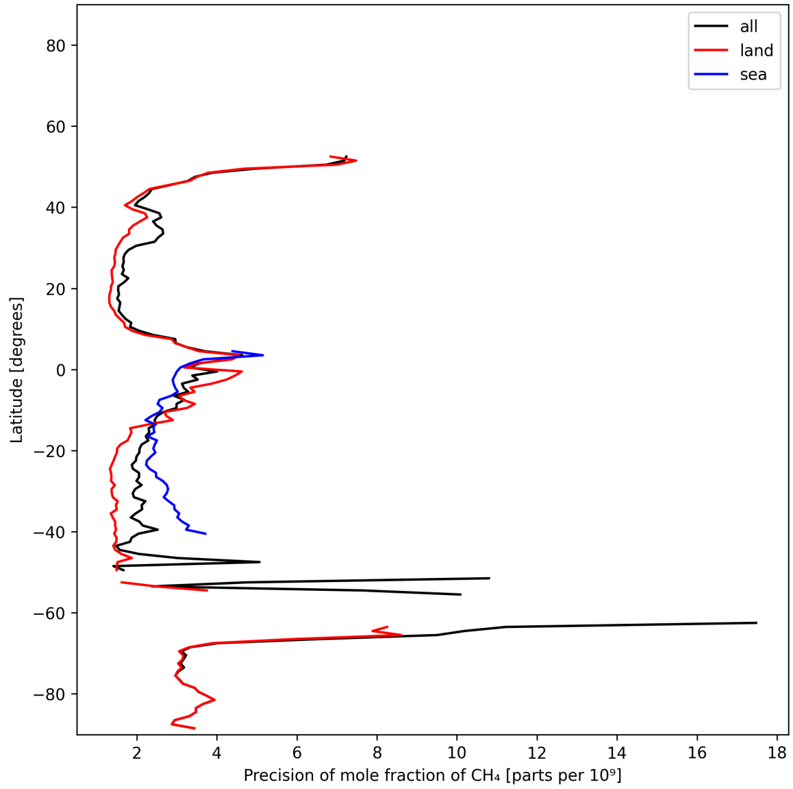
Figure 13: Zonal average of “Precision of mole fraction of CH 4 ” for 2024-12-07 to 2024-12-09.
