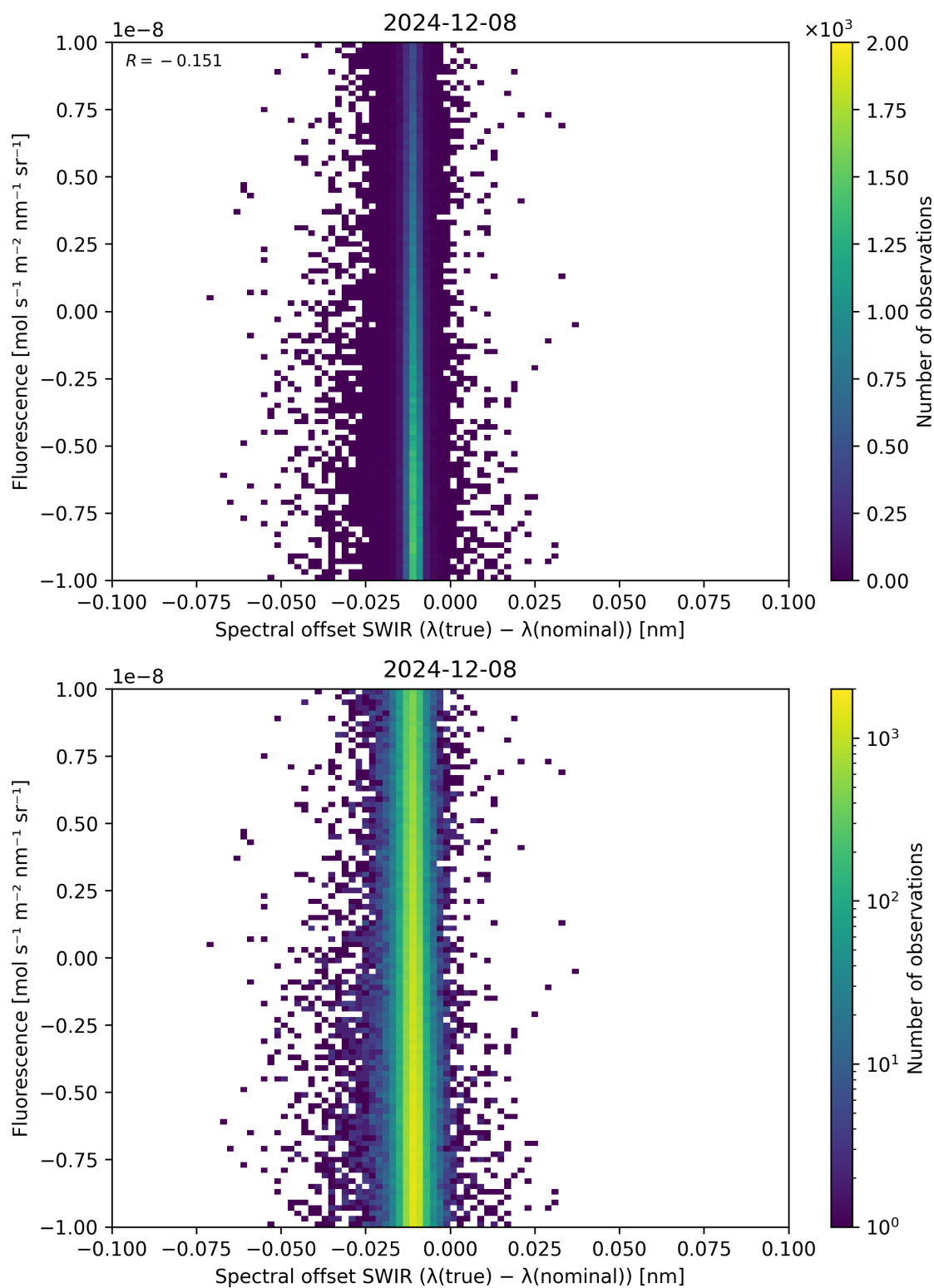
Figure 120: Scatter density plot of “Spectral offset SWIR ( \lambda_{\text{true}} - \lambda_{\text{nominal}} )” against “Fluorescence” for 2024-12-07 to 2024-12-09.
