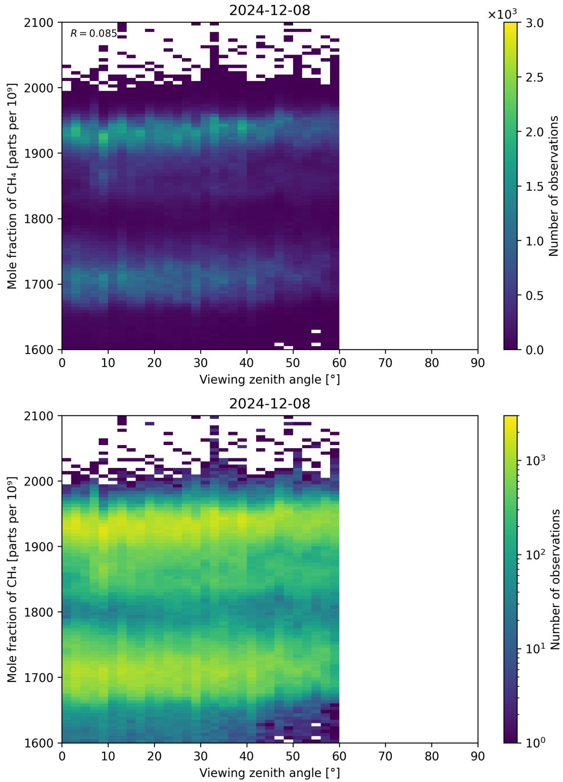
Figure 110: Scatter density plot of “Viewing zenith angle” against “Mole fraction of CH 4 ” for 2024-12-07 to 2024-12-09.
