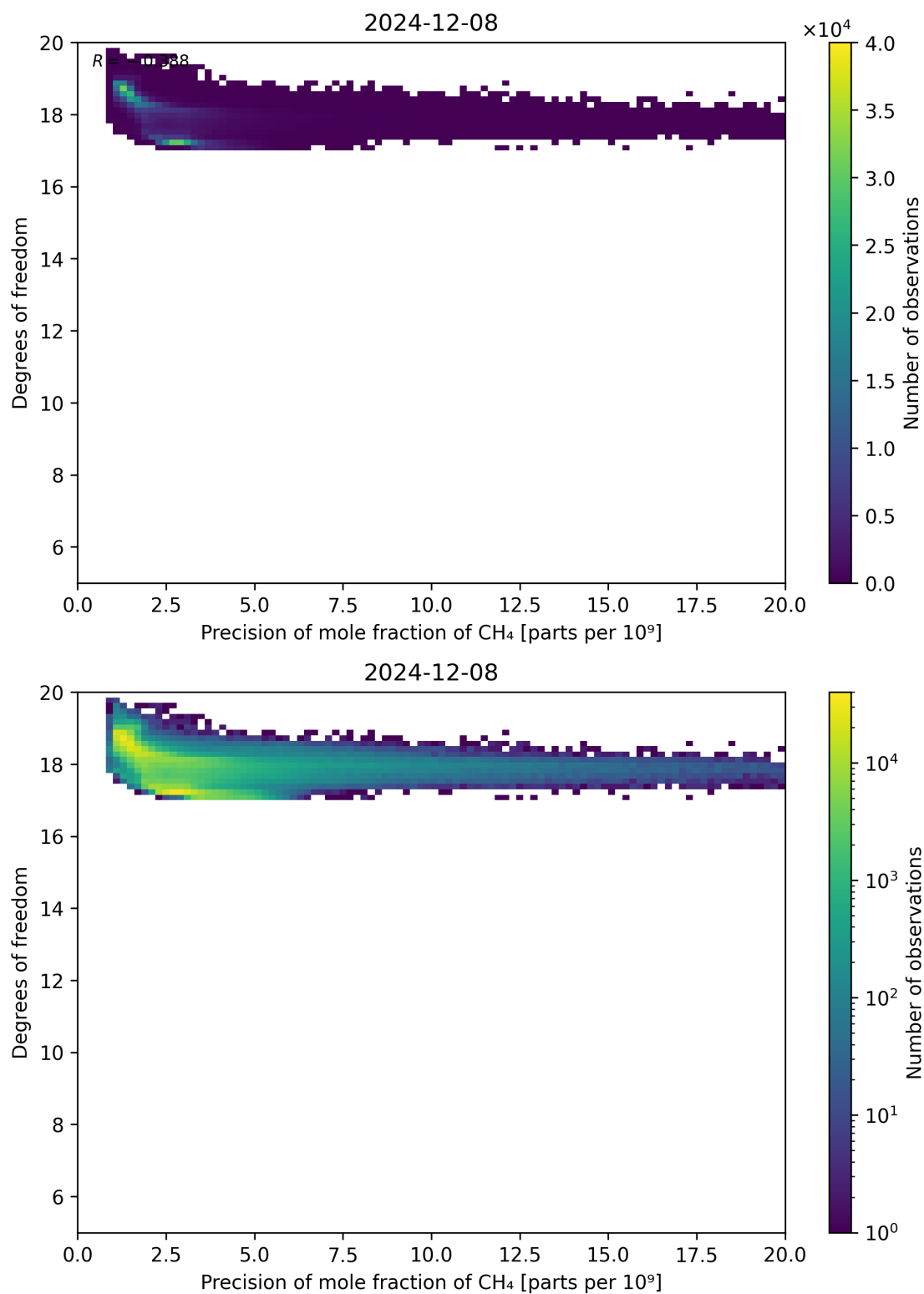
Figure 80: Scatter density plot of “Precision of mole fraction of CH 4 ” against “Degrees of freedom” for 2024-12-07 to 2024-12-09.
