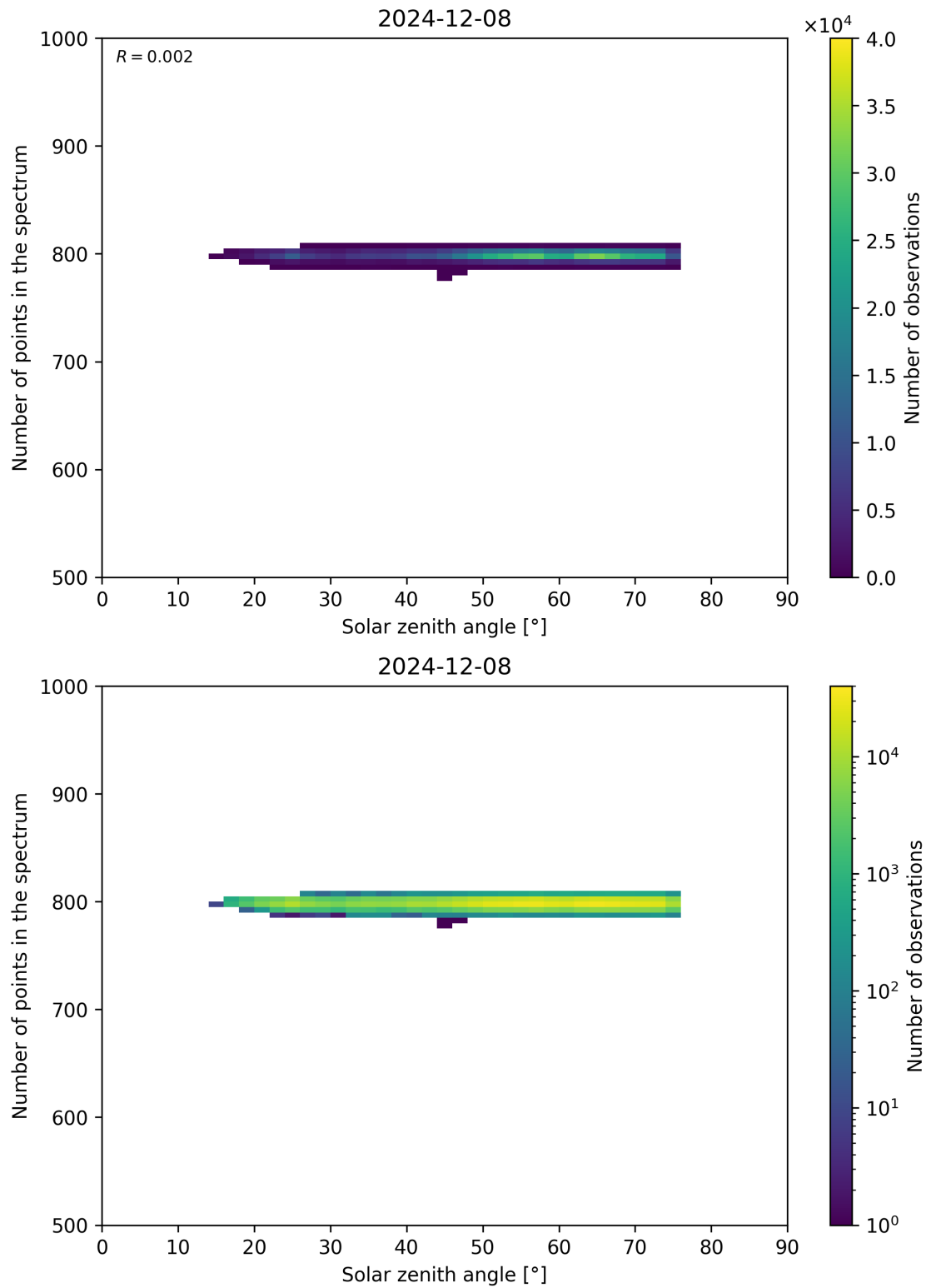
Figure 103: Scatter density plot of “Solar zenith angle” against “Number of points in the spectrum” for 2024-12-07 to 2024-12-09.
