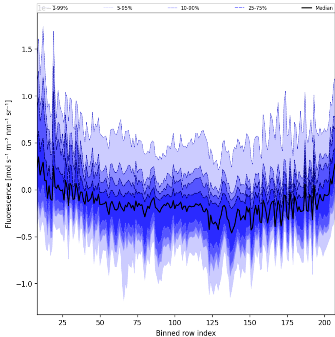
Figure 43: Along track statistics of “Fluorescence” for 2024-12-07 to 2024-12-09
