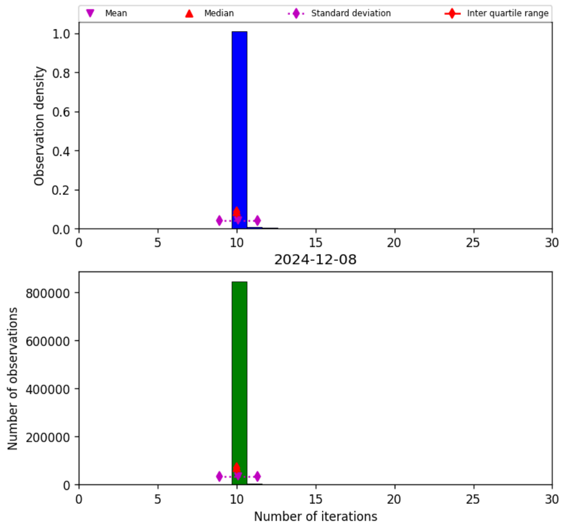
Figure 31: Histogram of “Number of iterations” for 2024-12-07 to 2024-12-09
