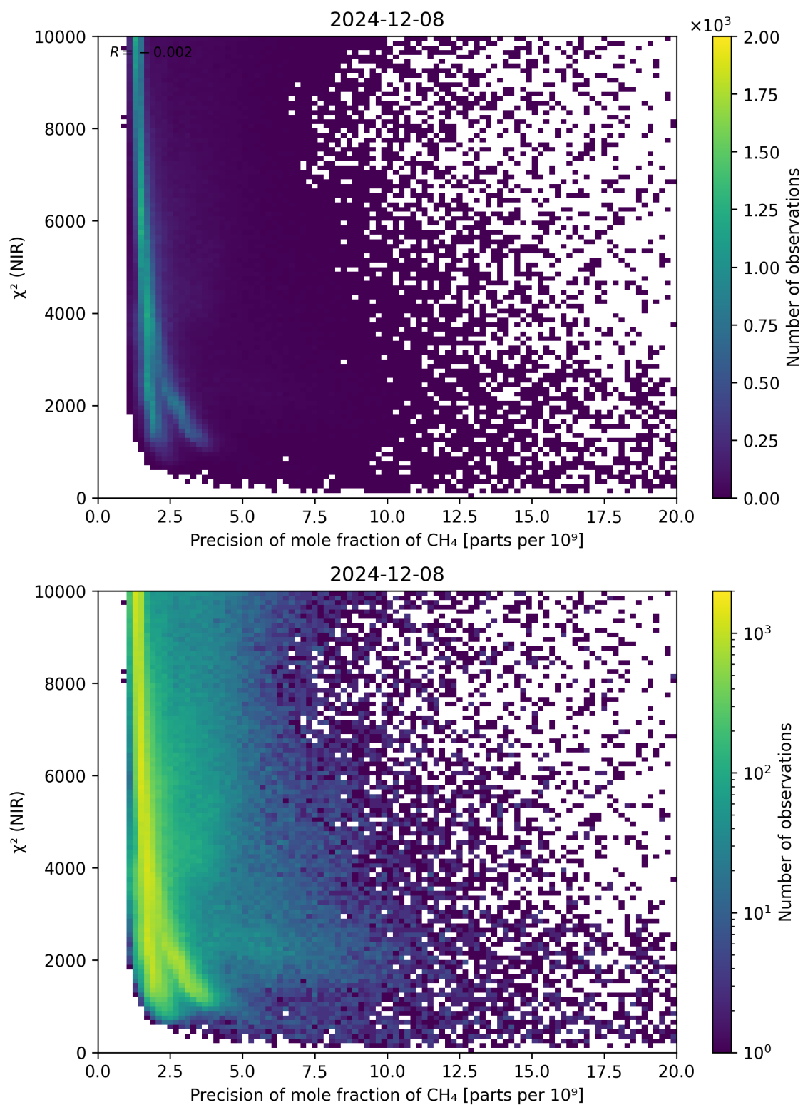
Figure 78: Scatter density plot of “Precision of mole fraction of CH 4 ” against “ \chi^2 (NIR)” for 2024-12-07 to 2024-12-09.
