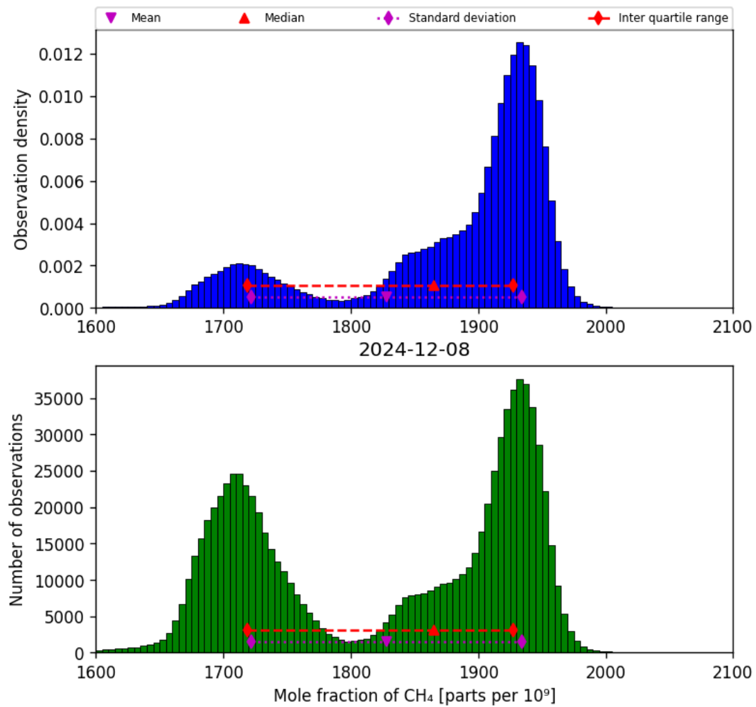
Figure 23: Histogram of “Mole fraction of CH 4 ” for 2024-12-07 to 2024-12-09
