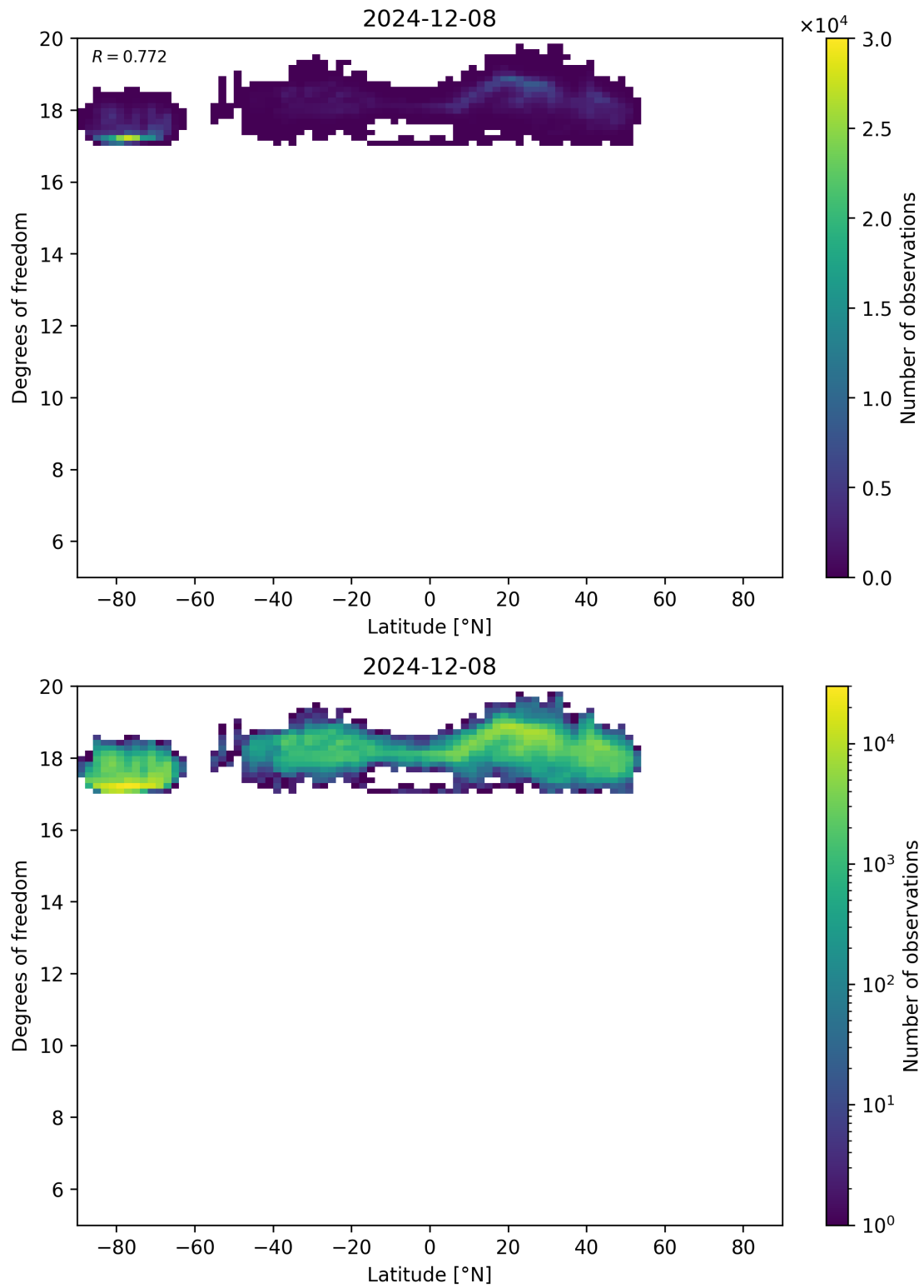
Figure 55: Scatter density plot of “Latitude” against “Degrees of freedom” for 2024-12-07 to 2024-12-09.
