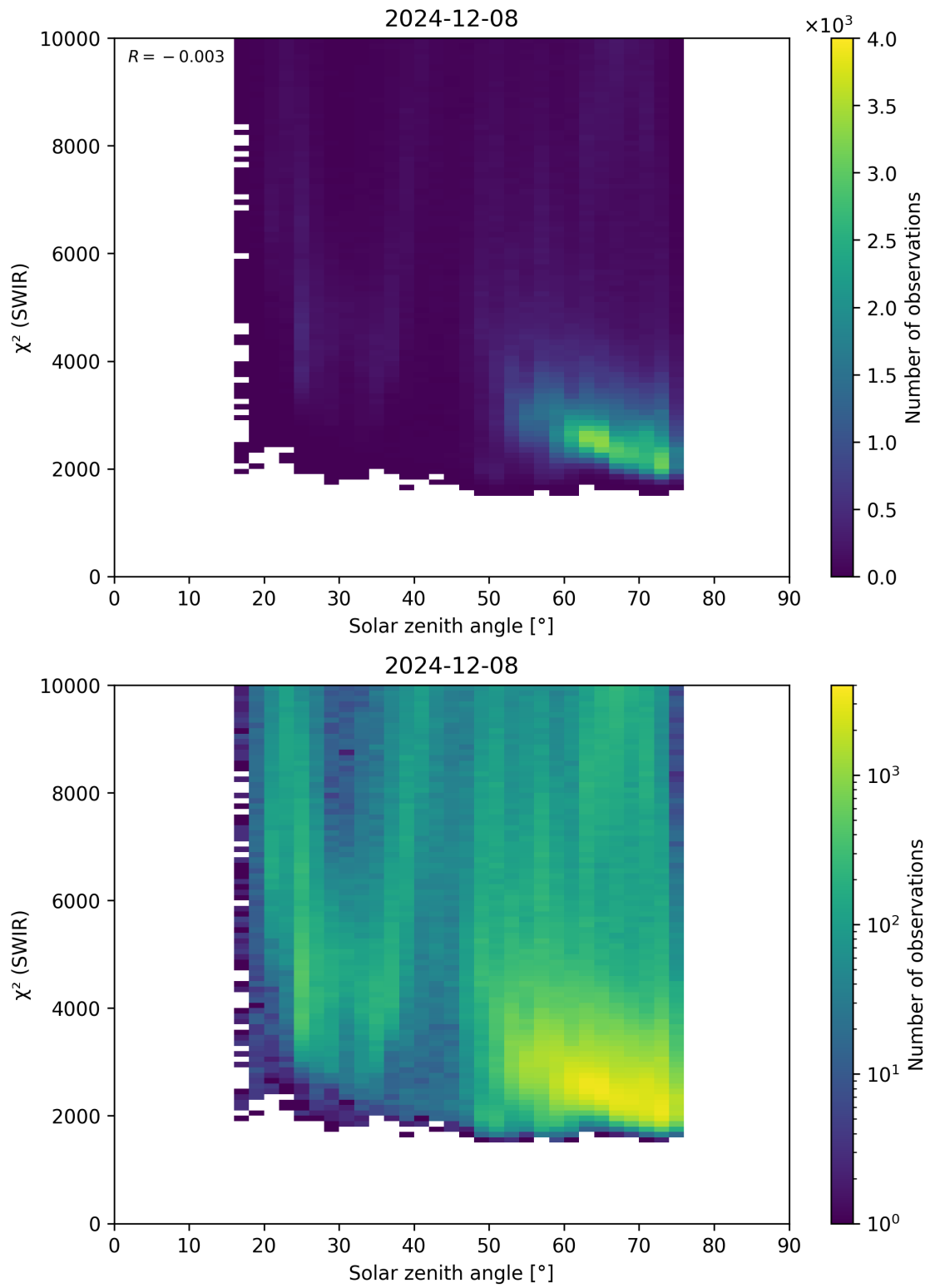
Figure 95: Scatter density plot of “Solar zenith angle” against “ \chi^2 (SWIR)” for 2024-12-07 to 2024-12-09.
