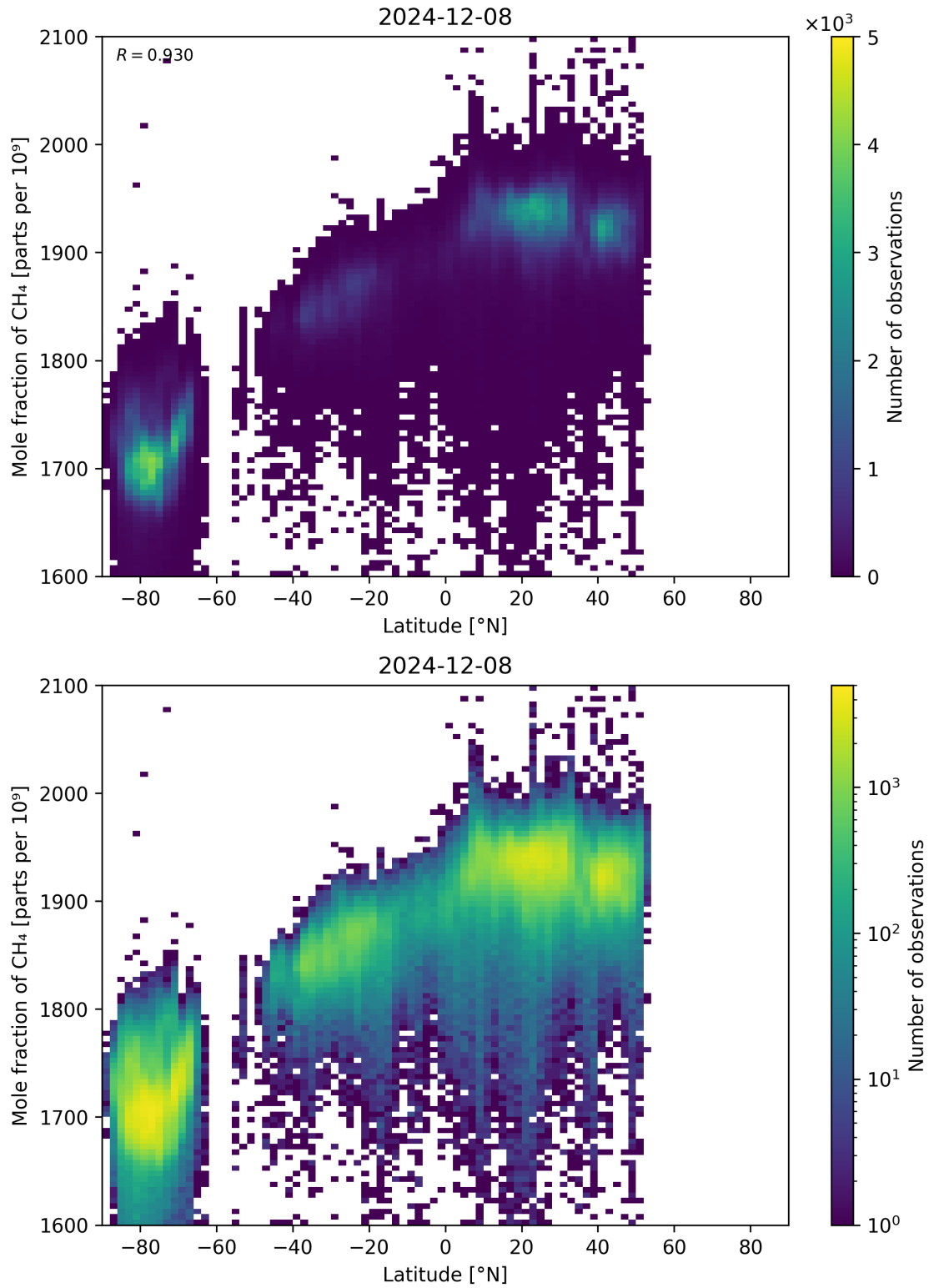
Figure 57: Scatter density plot of “Latitude” against “Mole fraction of CH 4 ” for 2024-12-07 to 2024-12-09.
