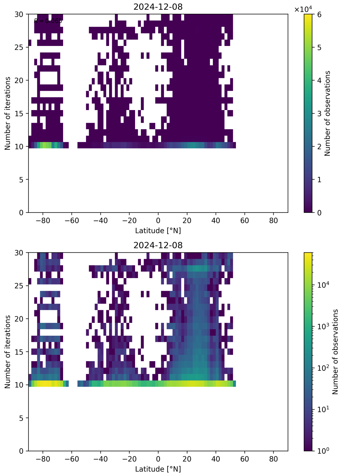
Figure 60: Scatter density plot of “Latitude” against “Number of iterations” for 2024-12-07 to 2024-12-09.
