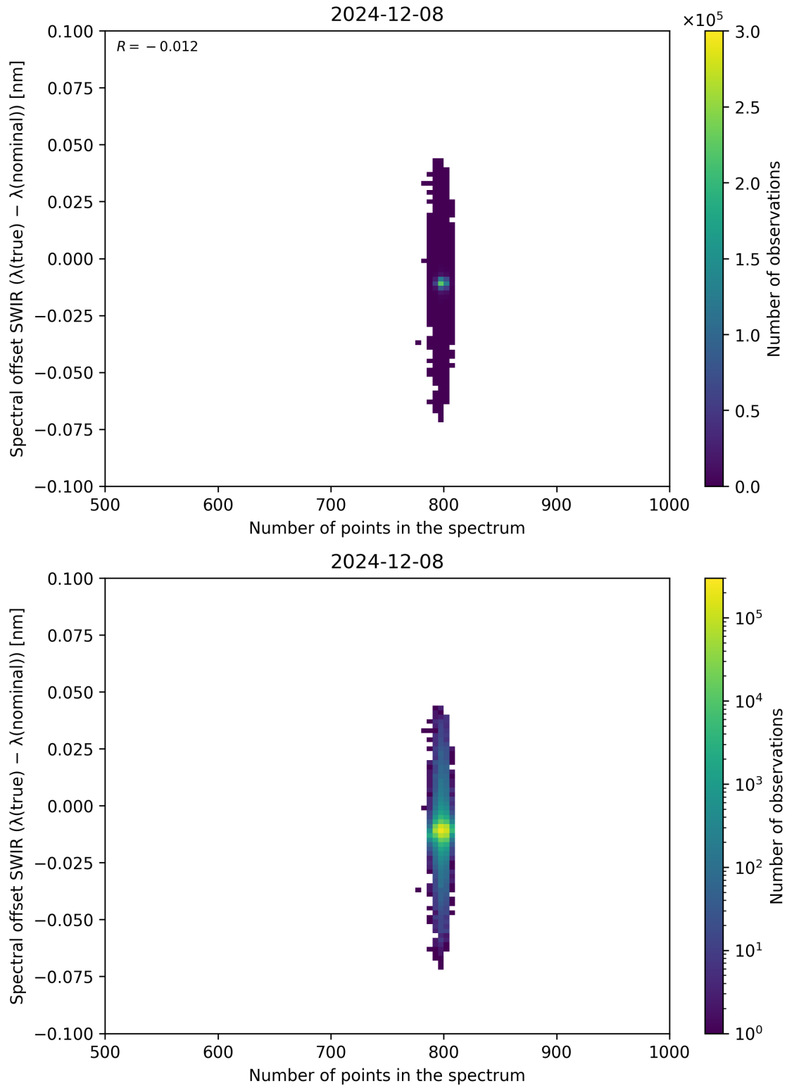
Figure 93: Scatter density plot of “Number of points in the spectrum” against “Spectral offset SWIR ( \lambda_{\text{true}} - \lambda_{\text{nominal}} )” for 2024-12-07 to 2024-12-09.
