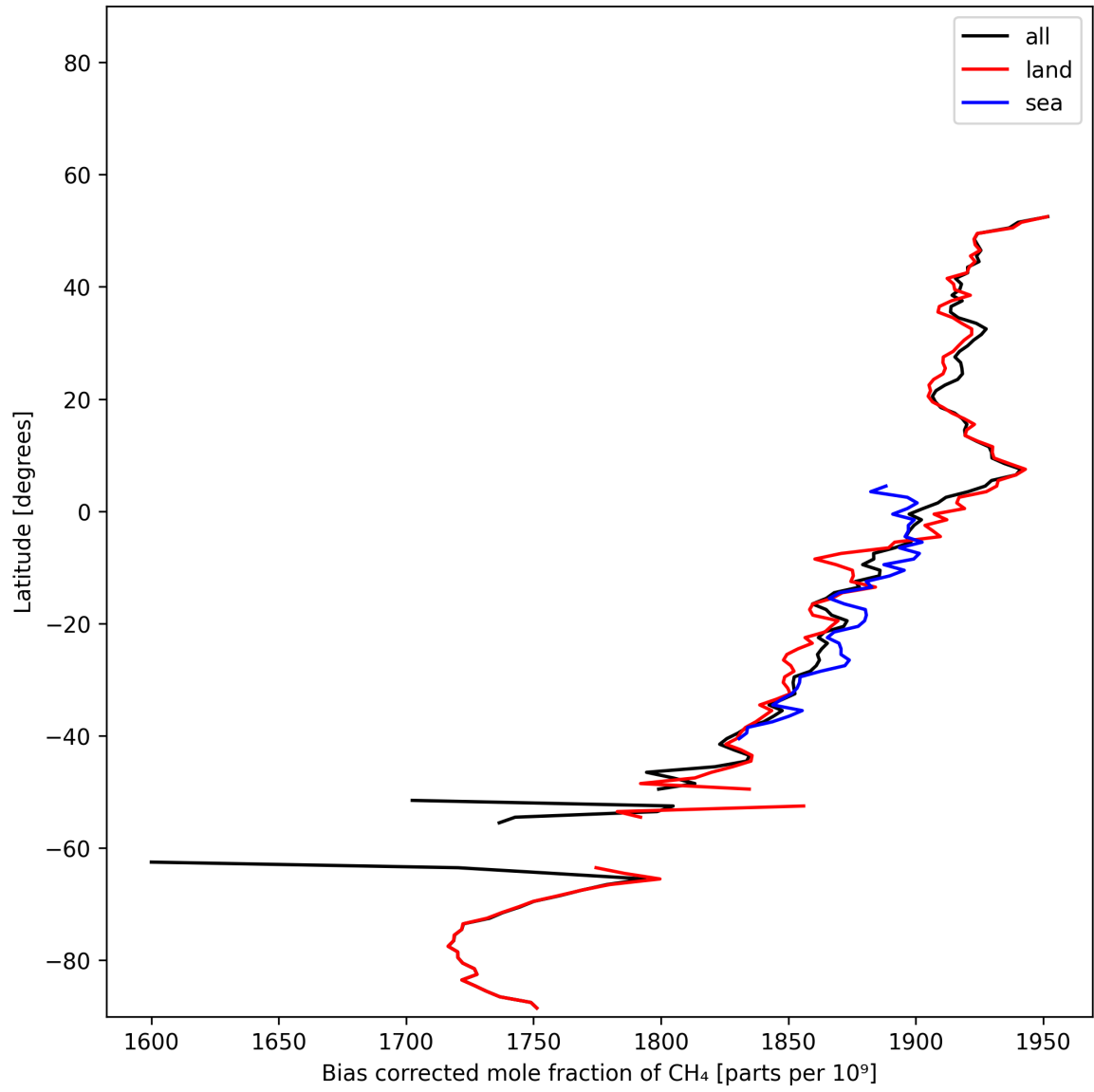
Figure 14: Zonal average of “Bias corrected mole fraction of CH 4 ” for 2024-12-07 to 2024-12-09.
