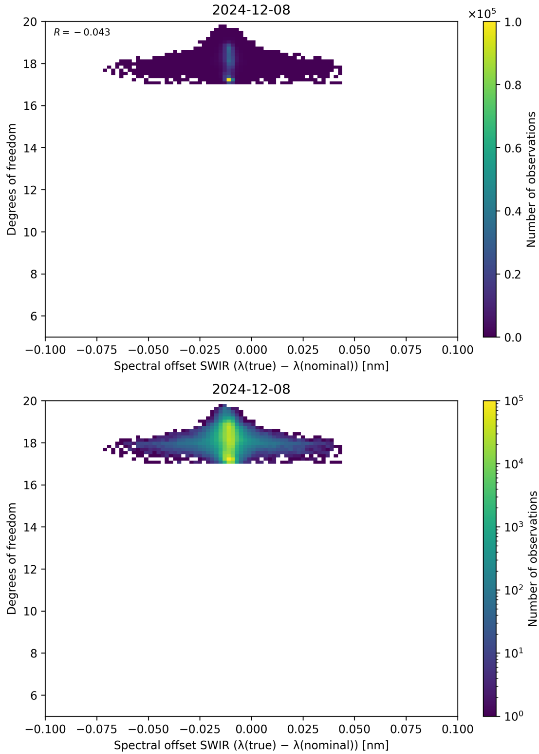
Figure 119: Scatter density plot of “Spectral offset SWIR ( \lambda_{\text{true}} - \lambda_{\text{nominal}} )” against “Degrees of freedom” for 2024-12-07 to 2024-12-09.
