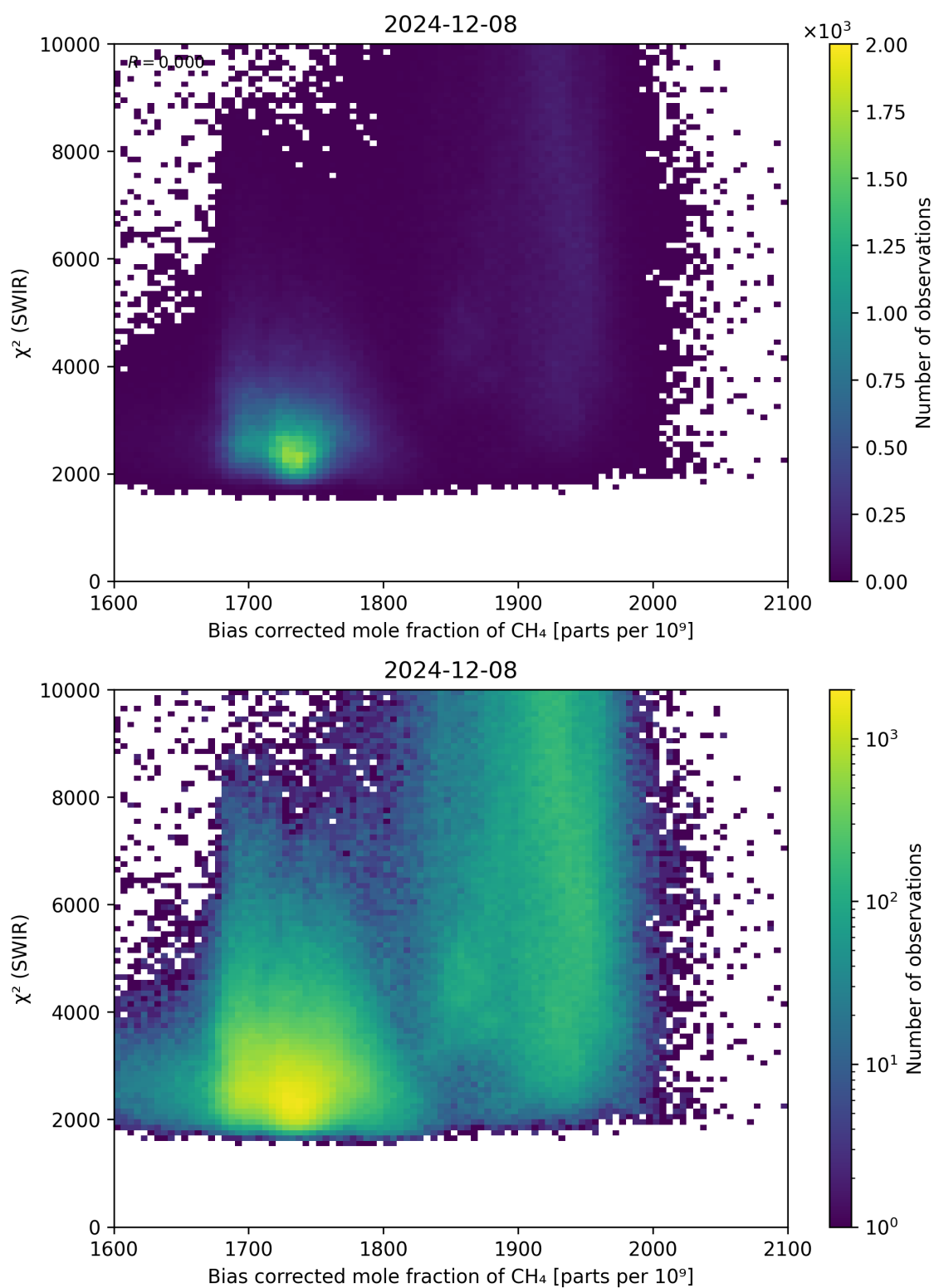
Figure 64: Scatter density plot of “Bias corrected mole fraction of \text{CH}_4 ” against “ \chi^2 (SWIR)” for 2024-12-07 to 2024-12-09.
