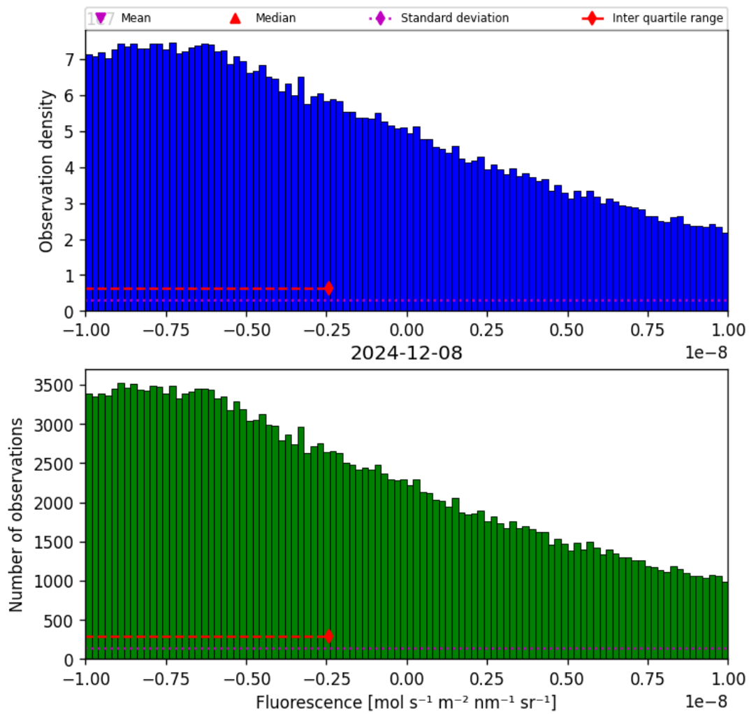
Figure 32: Histogram of “Fluorescence” for 2024-12-07 to 2024-12-09
