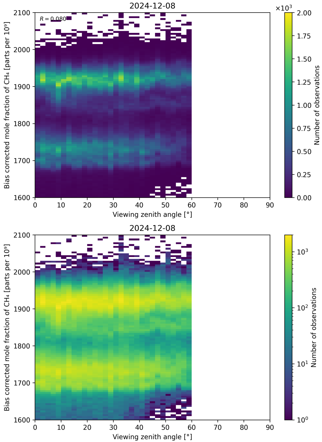
Figure 111: Scatter density plot of “Viewing zenith angle” against “Bias corrected mole fraction of CH 4 ” for 2024-12-07 to 2024-12-09.
