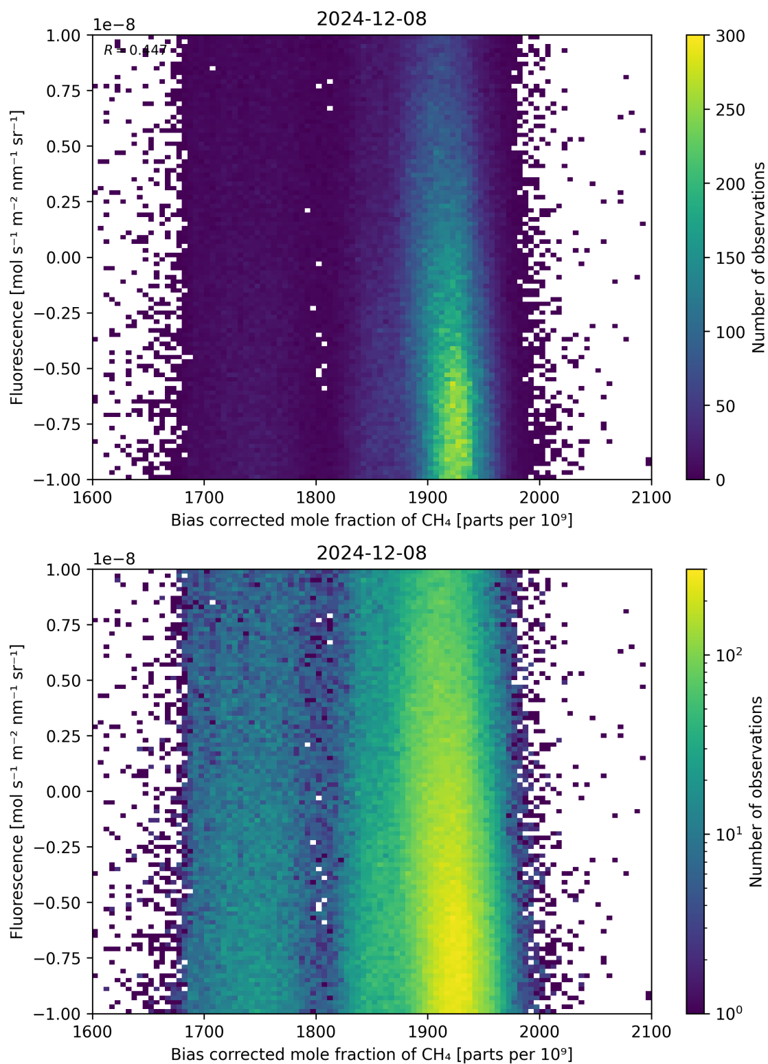
Figure 66: Scatter density plot of “Bias corrected mole fraction of \text{CH}_4 ” against “Fluorescence” for 2024-12-07 to 2024-12-09.
