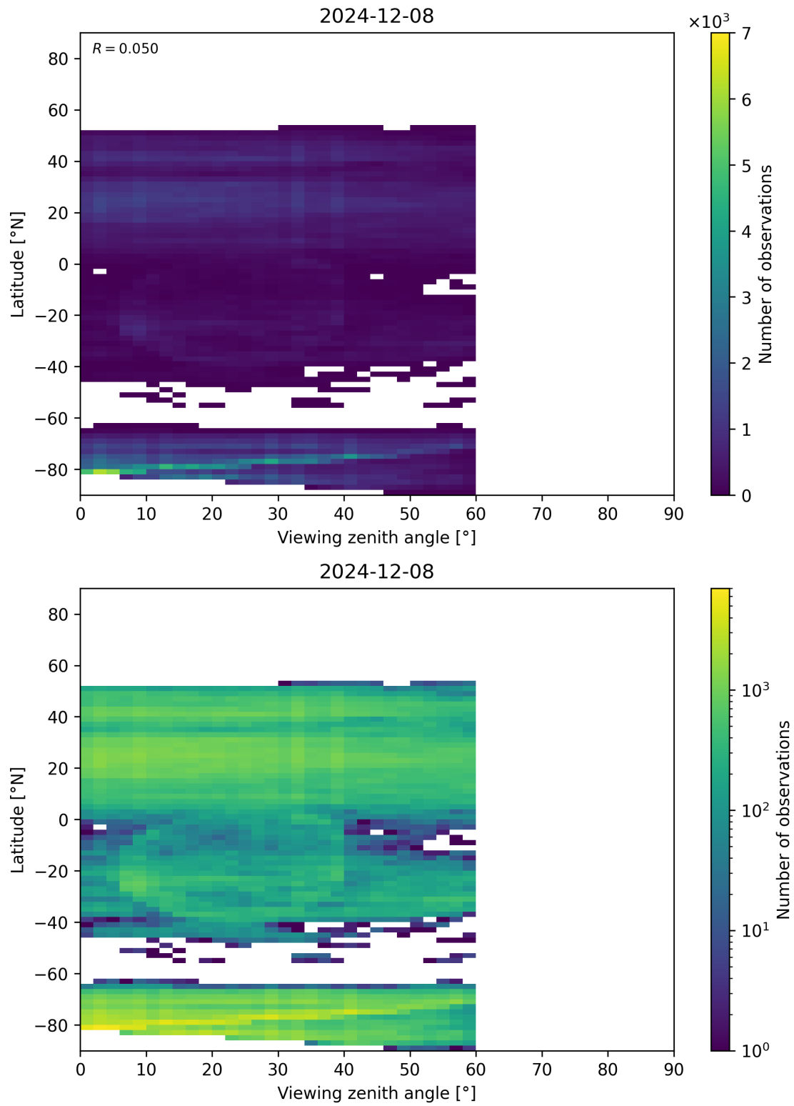
Figure 109: Scatter density plot of “Viewing zenith angle” against “Latitude” for 2024-12-07 to 2024-12-09.
