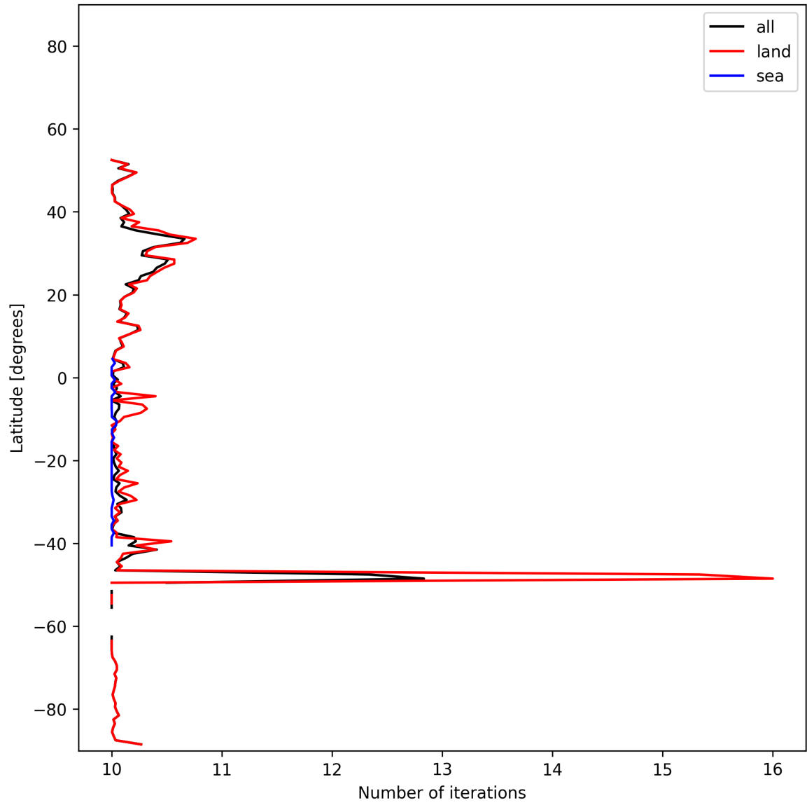
Figure 20: Zonal average of “Number of iterations” for 2024-12-07 to 2024-12-09.
