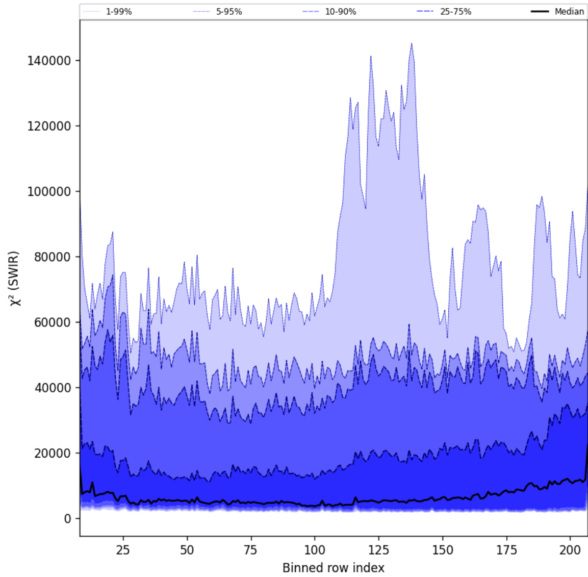
Figure 39: Along track statistics of “ \chi^2 (SWIR)” for 2024-12-07 to 2024-12-09
