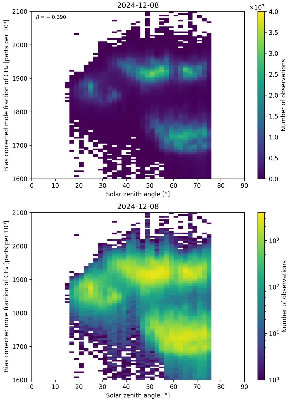
Figure 100: Scatter density plot of “Solar zenith angle” against “Bias corrected mole fraction of CH 4 ” for 2024-12-07 to 2024-12-09.
