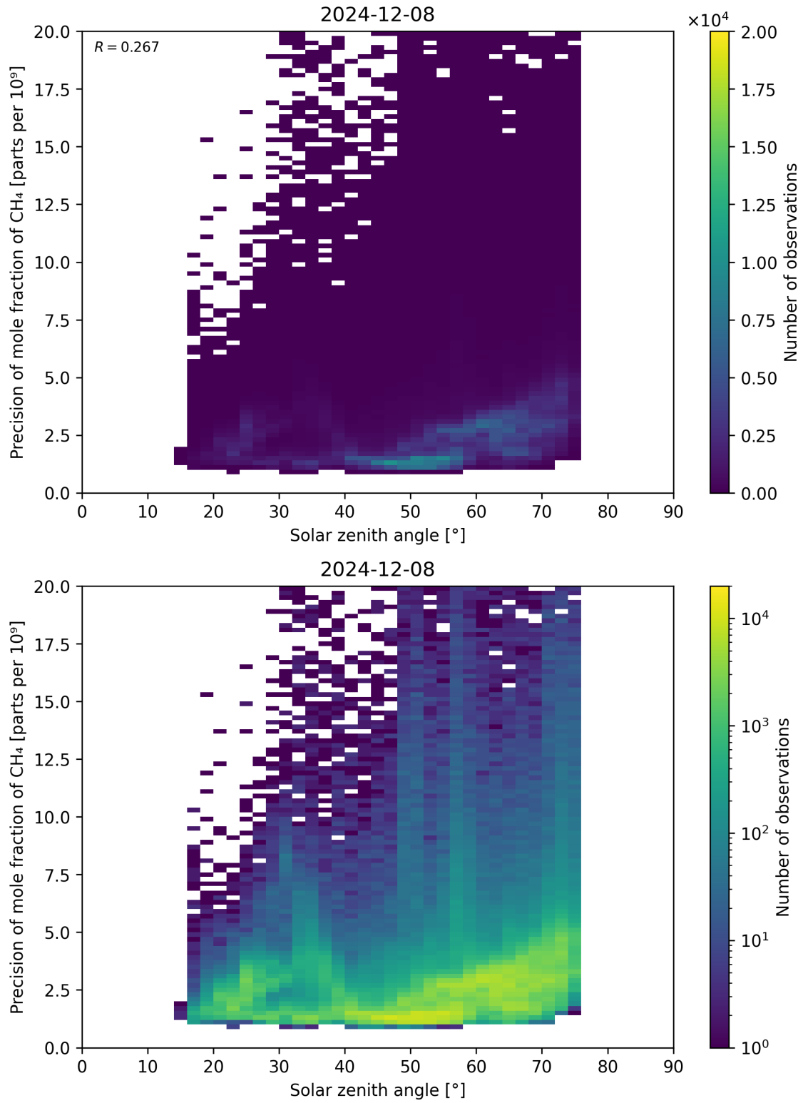
Figure 101: Scatter density plot of “Solar zenith angle” against “Precision of mole fraction of CH 4 ” for 2024-12-07 to 2024-12-09.
