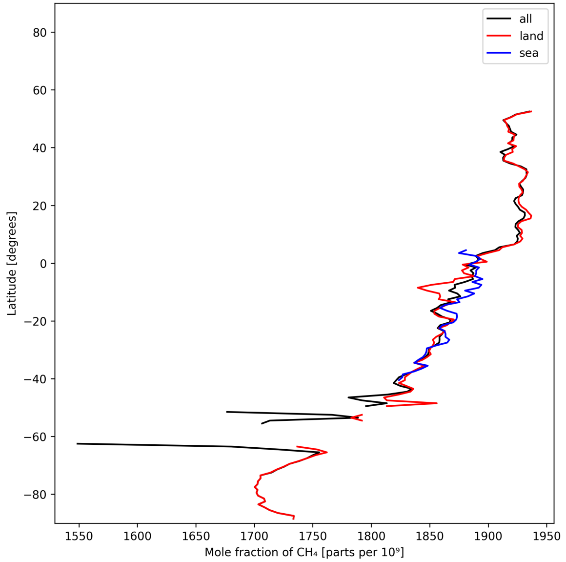
Figure 12: Zonal average of “Mole fraction of \text{CH}_4 ” for 2024-12-07 to 2024-12-09.
