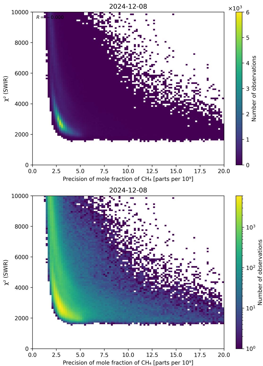
Figure 79: Scatter density plot of “Precision of mole fraction of \text{CH}_4 ” against “ \chi^2 (SWIR)” for 2024-12-07 to 2024-12-09.
