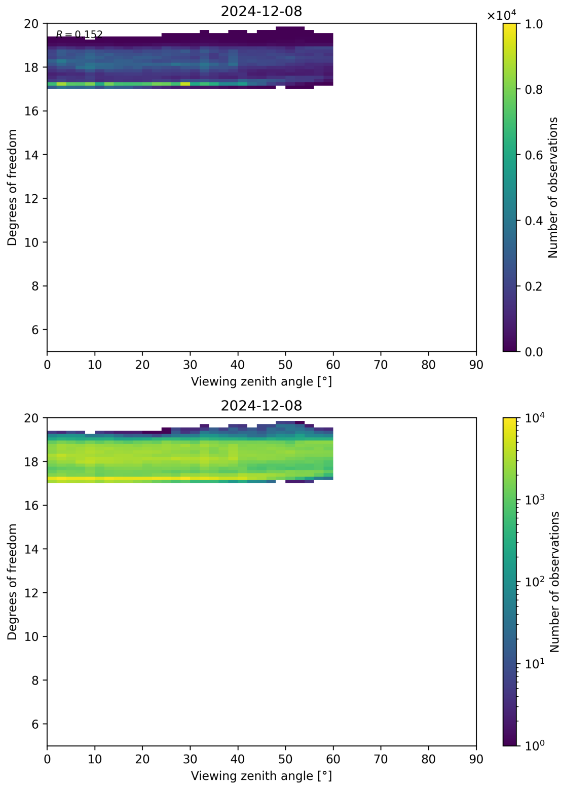
Figure 107: Scatter density plot of “Viewing zenith angle” against “Degrees of freedom” for 2024-12-07 to 2024-12-09.
