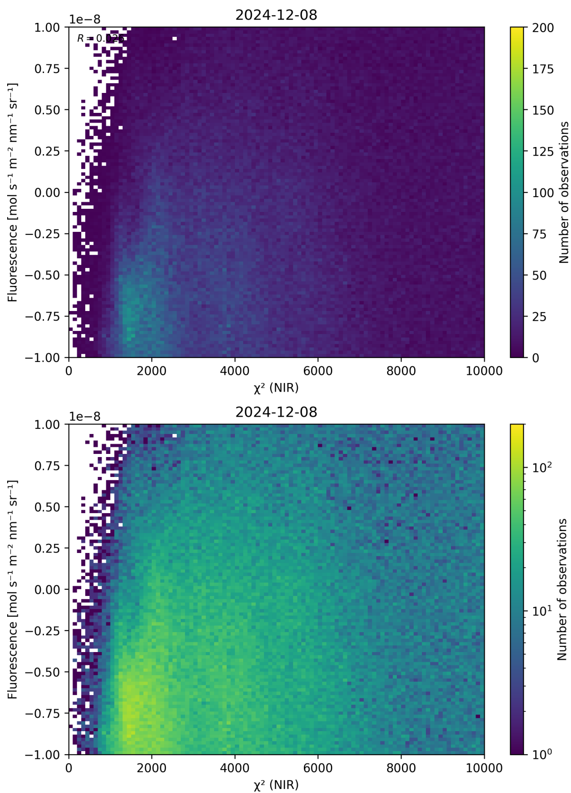
Figure 45: Scatter density plot of “ \chi^2 (NIR)” against “Fluorescence” for 2024-12-07 to 2024-12-09.
