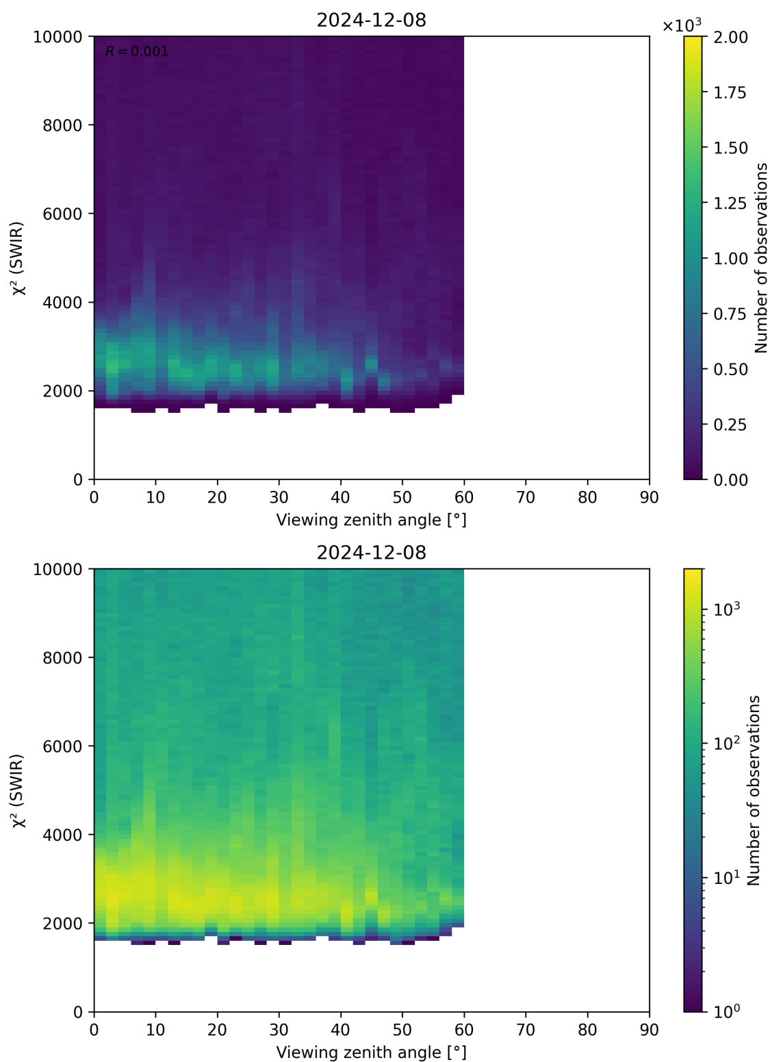
Figure 106: Scatter density plot of “Viewing zenith angle” against “ \chi^2 (SWIR)” for 2024-12-07 to 2024-12-09.
