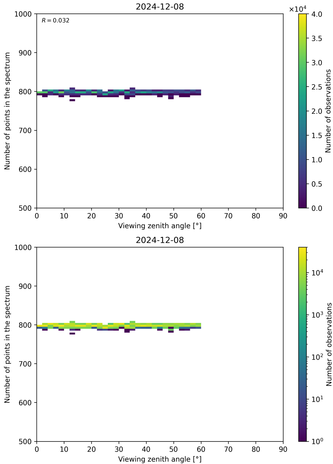
Figure 114: Scatter density plot of “Viewing zenith angle” against “Number of points in the spectrum” for 2024-12-07 to 2024-12-09.
