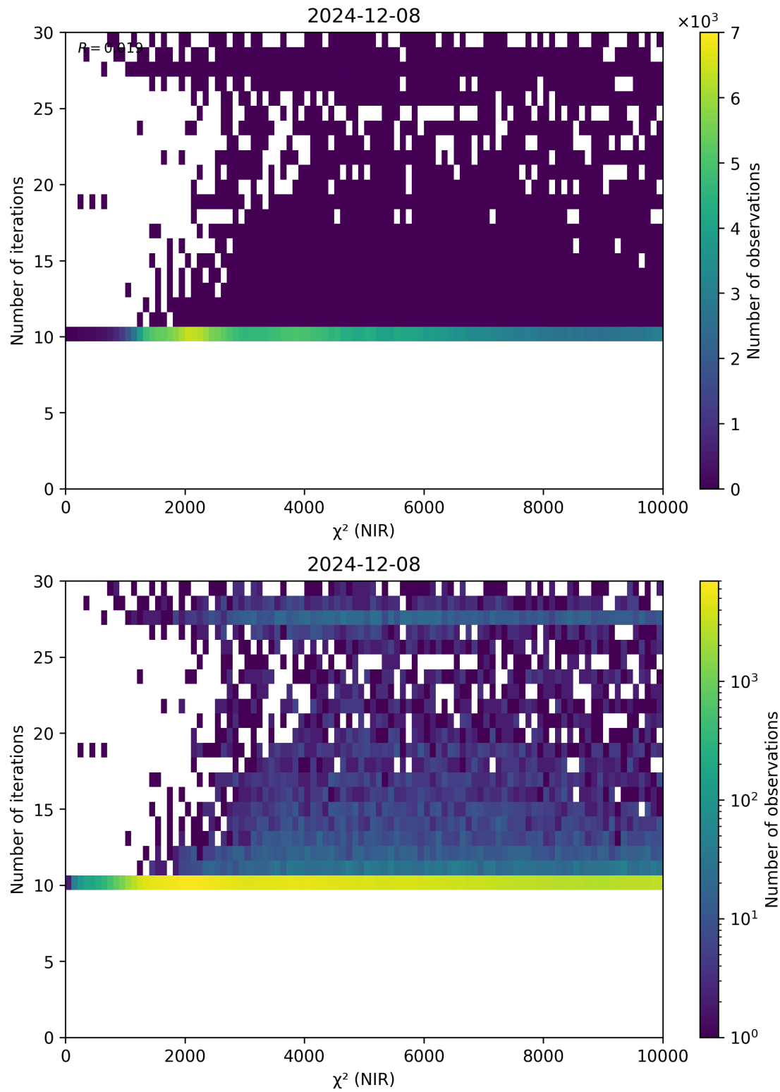
Figure 46: Scatter density plot of “ \chi^2 (NIR)” against “Number of iterations” for 2024-12-07 to 2024-12-09.
