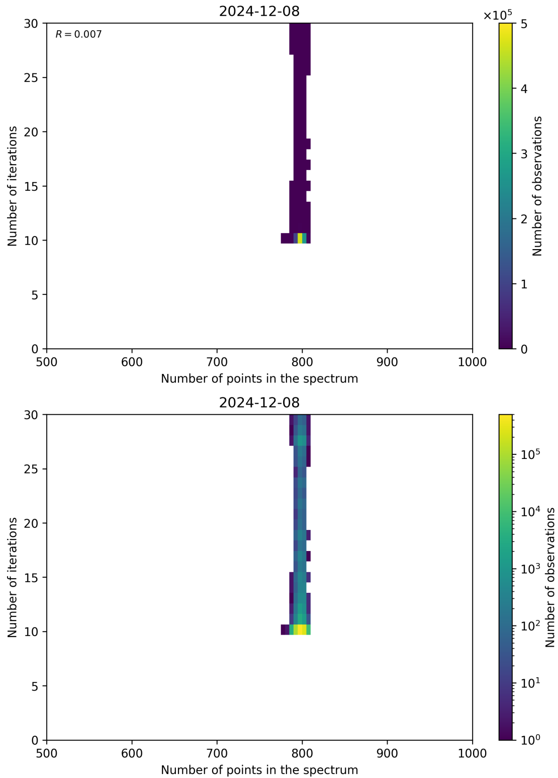
Figure 92: Scatter density plot of “Number of points in the spectrum” against “Number of iterations” for 2024-12-07 to 2024-12-09.
