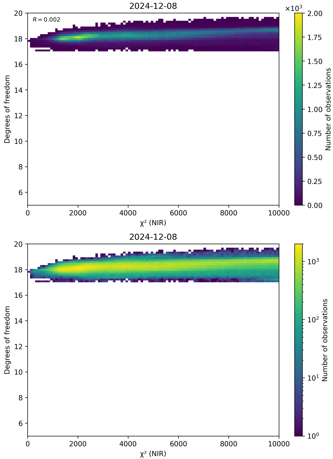
Figure 44: Scatter density plot of “ \chi^2 (NIR)” against “Degrees of freedom” for 2024-12-07 to 2024-12-09.
