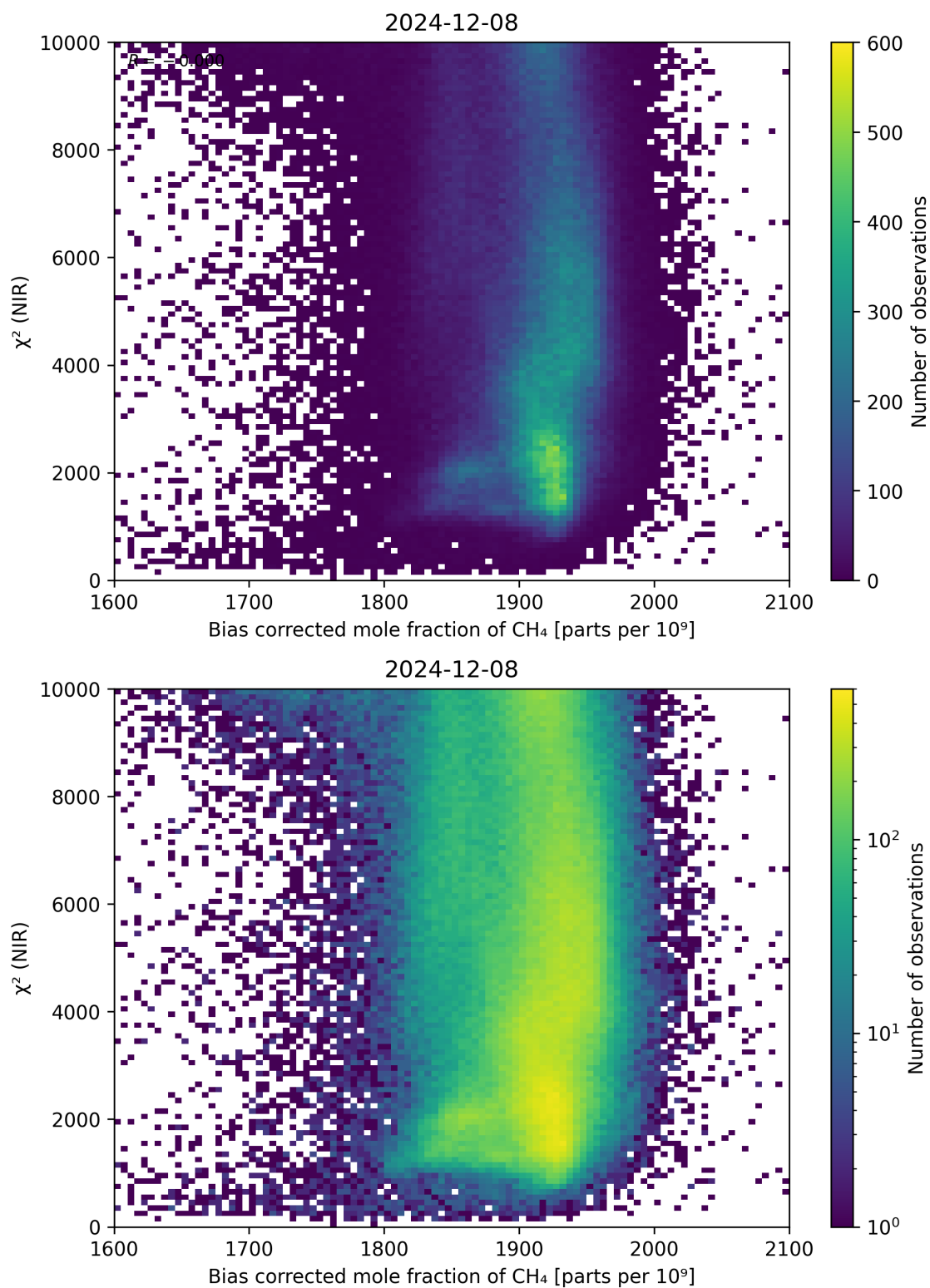
Figure 63: Scatter density plot of “Bias corrected mole fraction of \text{CH}_4 ” against “ \chi^2 (NIR)” for 2024-12-07 to 2024-12-09.
