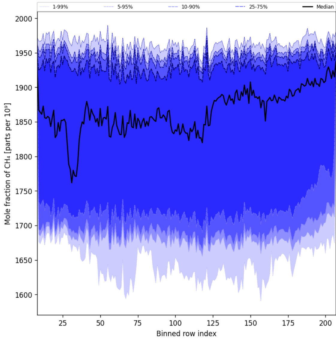
Figure 34: Along track statistics of “Mole fraction of CH 4 ” for 2024-12-07 to 2024-12-09
