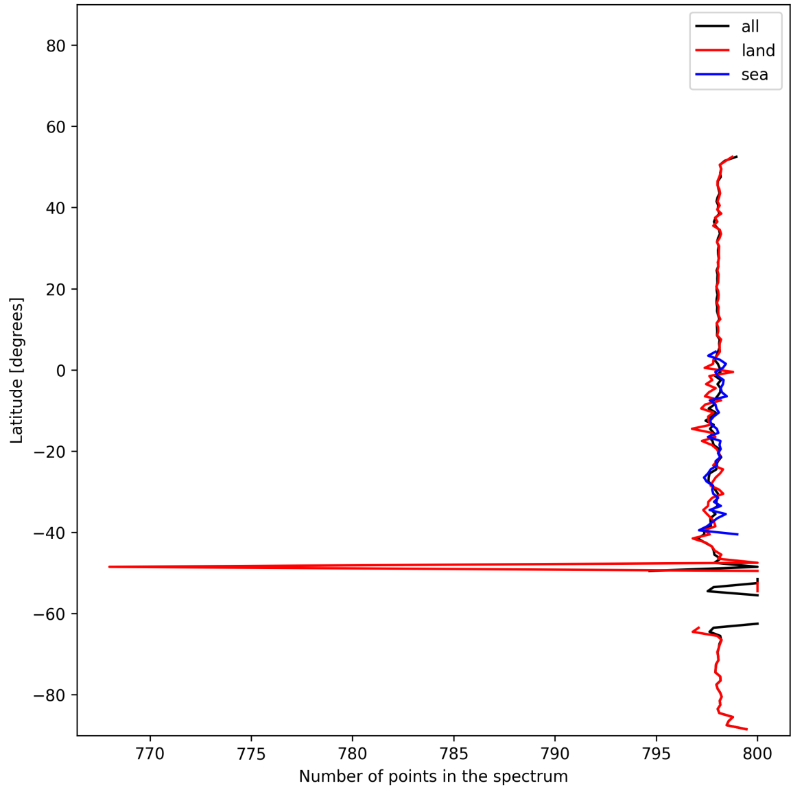
Figure 15: Zonal average of “Number of points in the spectrum” for 2024-12-07 to 2024-12-09.
