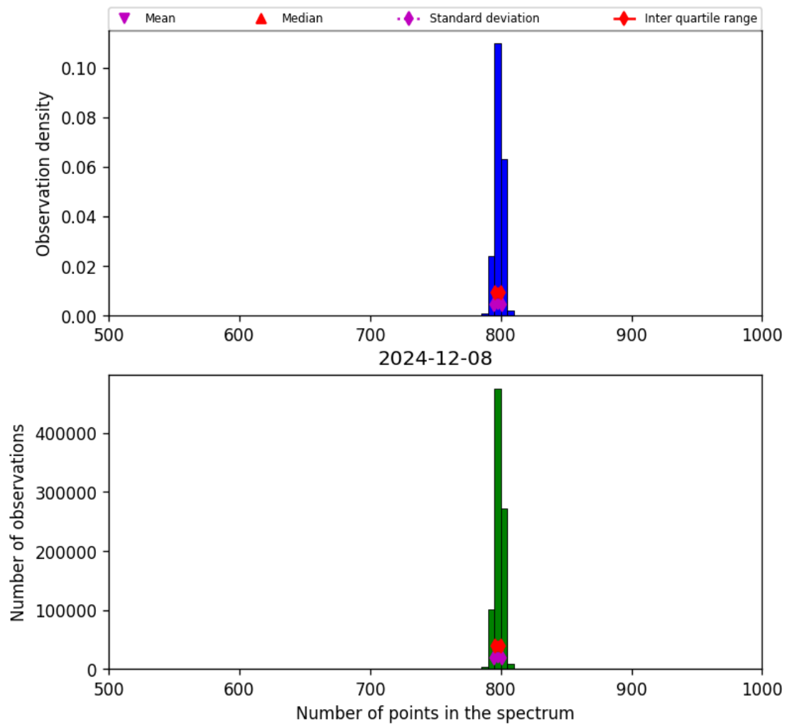
Figure 26: Histogram of “Number of points in the spectrum” for 2024-12-07 to 2024-12-09
