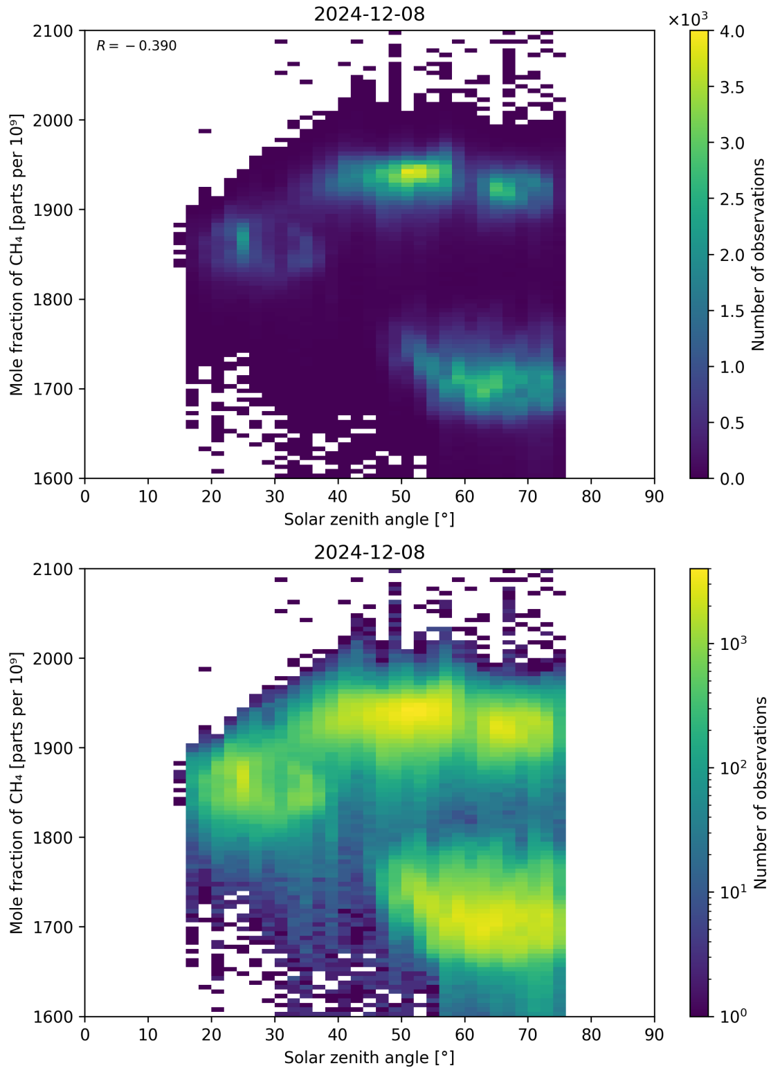
Figure 99: Scatter density plot of “Solar zenith angle” against “Mole fraction of CH 4 ” for 2024-12-07 to 2024-12-09.
