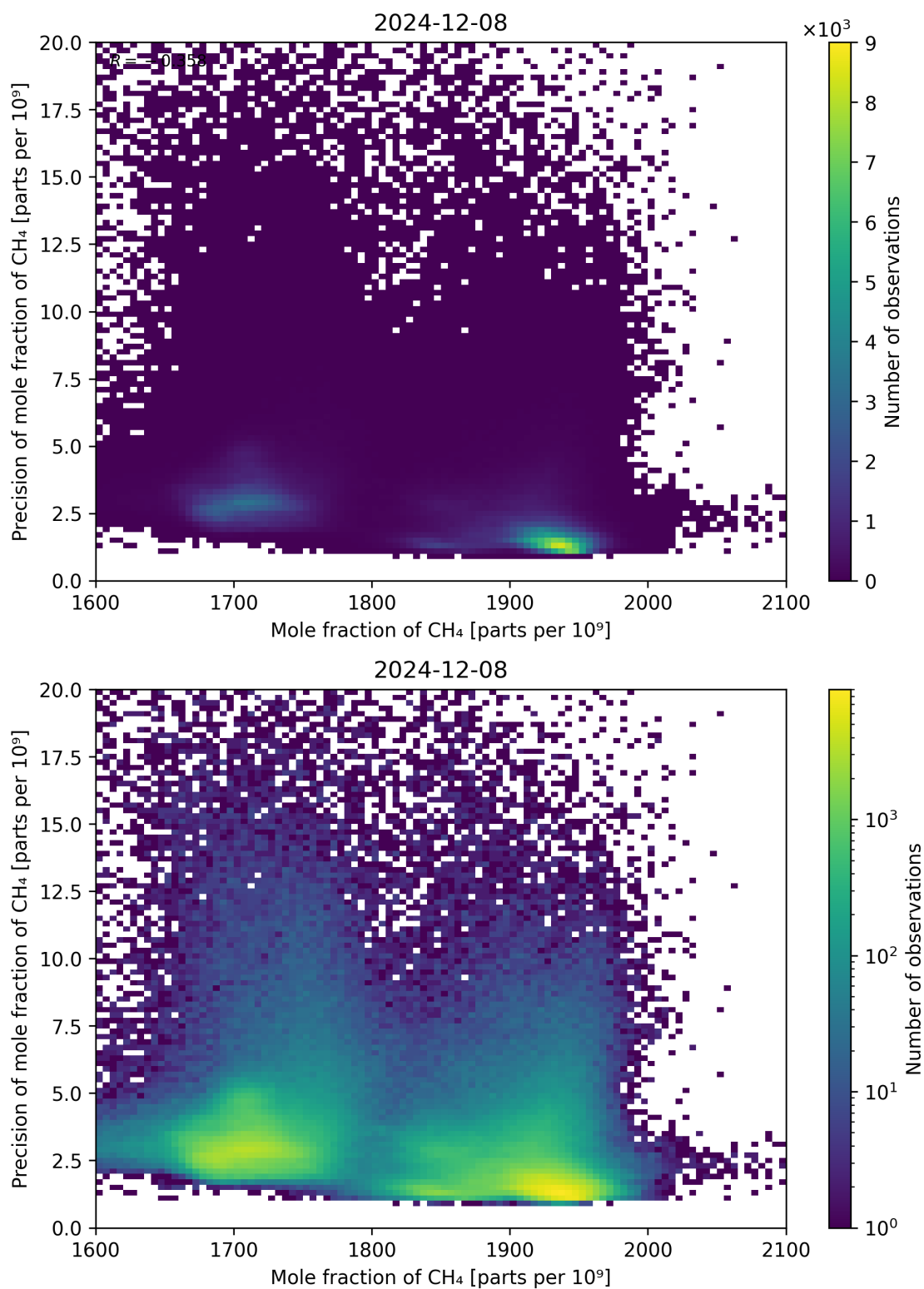
Figure 75: Scatter density plot of “Mole fraction of CH 4 ” against “Precision of mole fraction of CH 4 ” for 2024-12-07 to 2024-12-09.
