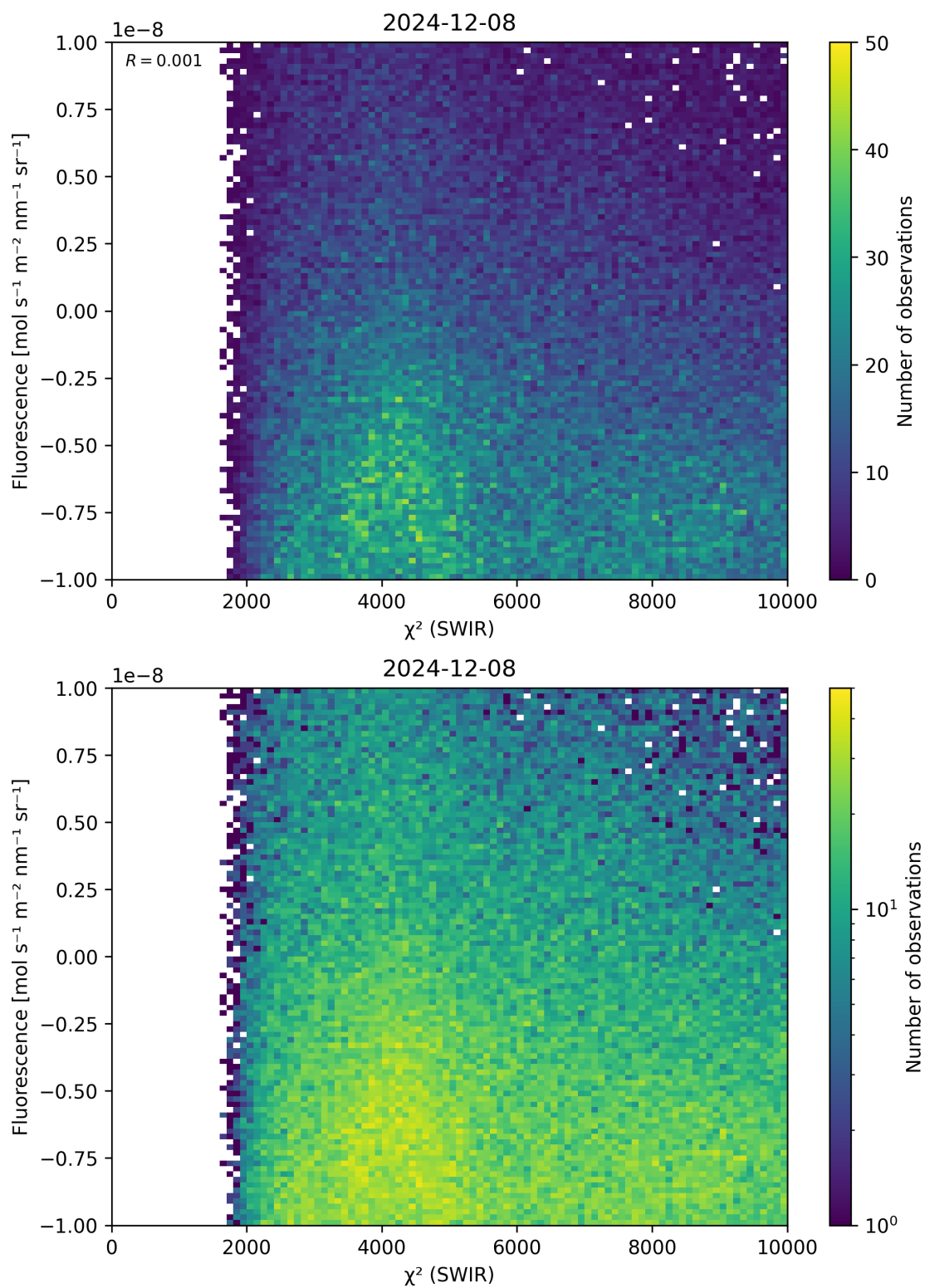
Figure 49: Scatter density plot of “ \chi^2 (SWIR)” against “Fluorescence” for 2024-12-07 to 2024-12-09.
