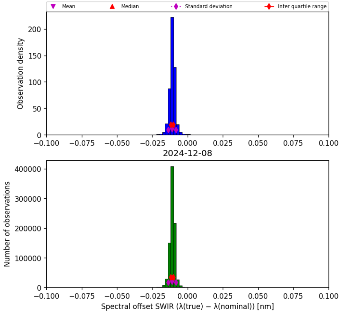
Figure 27: Histogram of “Spectral offset SWIR ( \lambda_{\text{true}} - \lambda_{\text{nominal}} )” for 2024-12-07 to 2024-12-09
