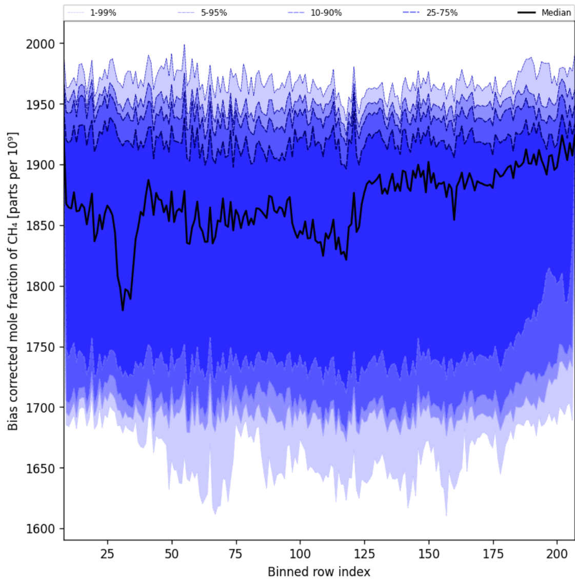
Figure 36: Along track statistics of “Bias corrected mole fraction of CH 4 ” for 2024-12-07 to 2024-12-09
