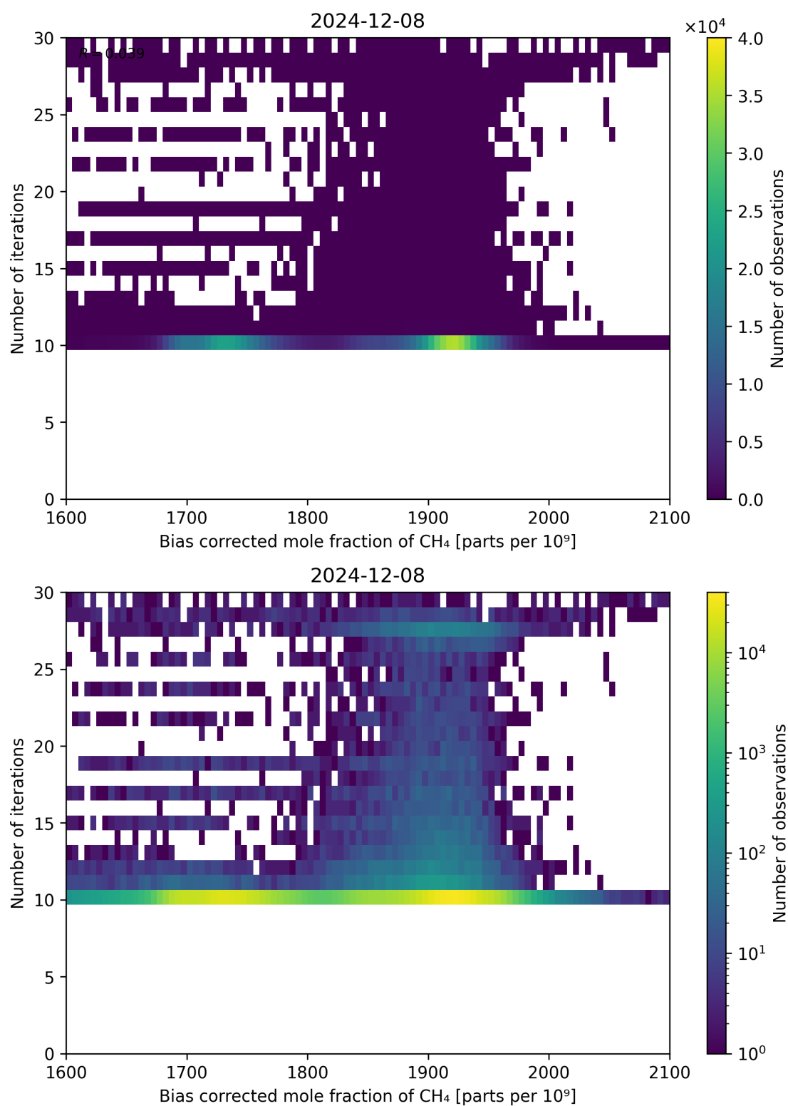
Figure 67: Scatter density plot of “Bias corrected mole fraction of \text{CH}_4 ” against “Number of iterations” for 2024-12-07 to 2024-12-09.
