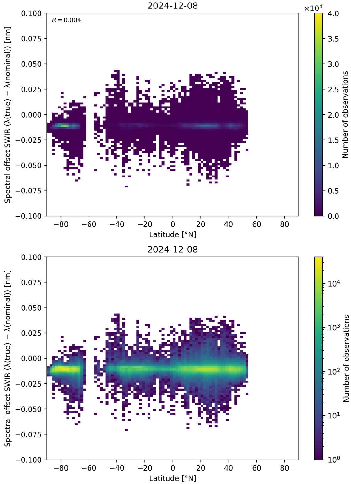
Figure 62: Scatter density plot of “Latitude” against “Spectral offset SWIR ( \lambda_{\text{true}} - \lambda_{\text{nominal}} )” for 2024-12-07 to 2024-12-09.
