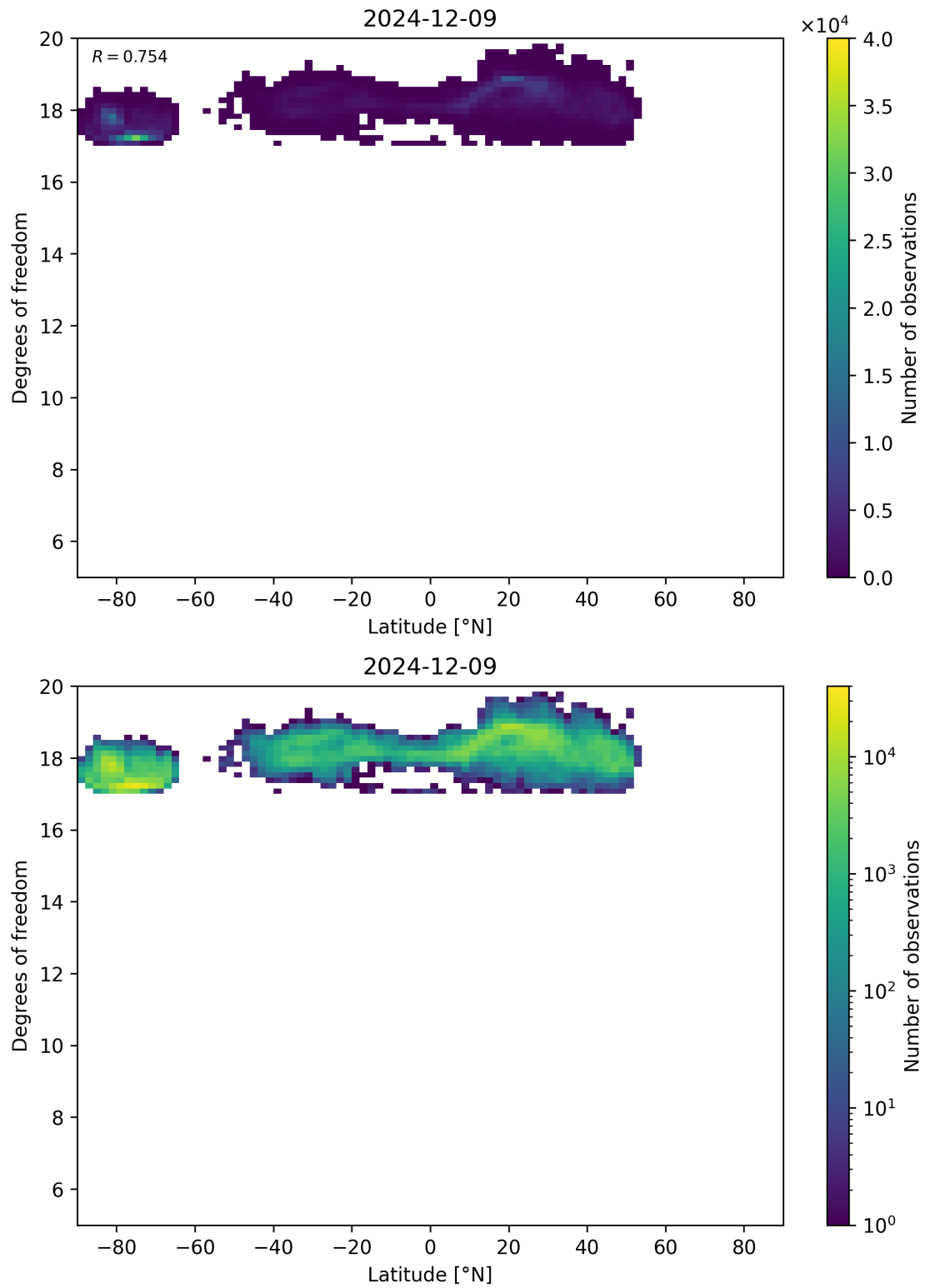
Figure 55: Scatter density plot of “Latitude” against “Degrees of freedom” for 2024-12-08 to 2024-12-10.
