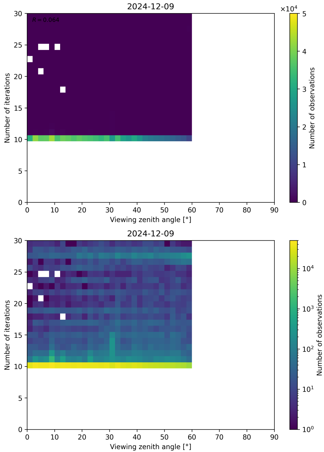
Figure 113: Scatter density plot of “Viewing zenith angle” against “Number of iterations” for 2024-12-08 to 2024-12-10.
