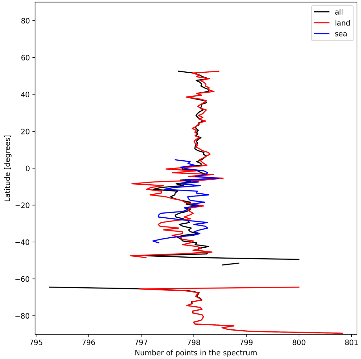
Figure 15: Zonal average of “Number of points in the spectrum” for 2024-12-08 to 2024-12-10.
