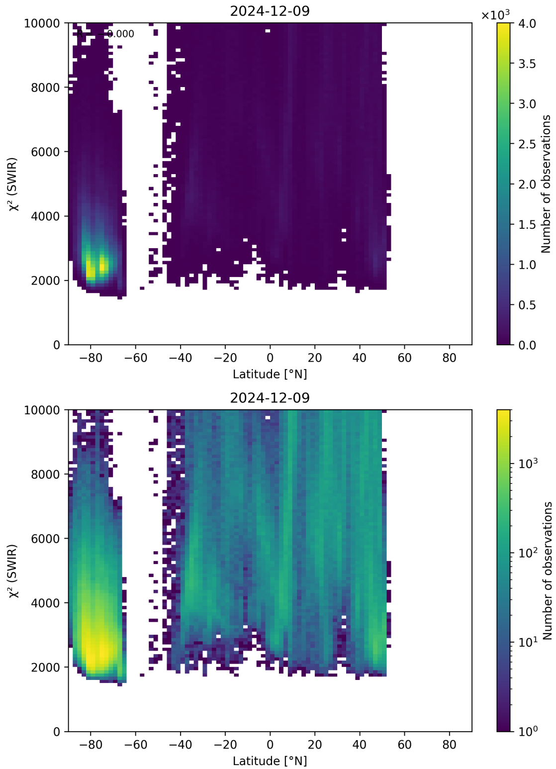
Figure 54: Scatter density plot of “Latitude” against “ \chi^2 (SWIR)” for 2024-12-08 to 2024-12-10.
