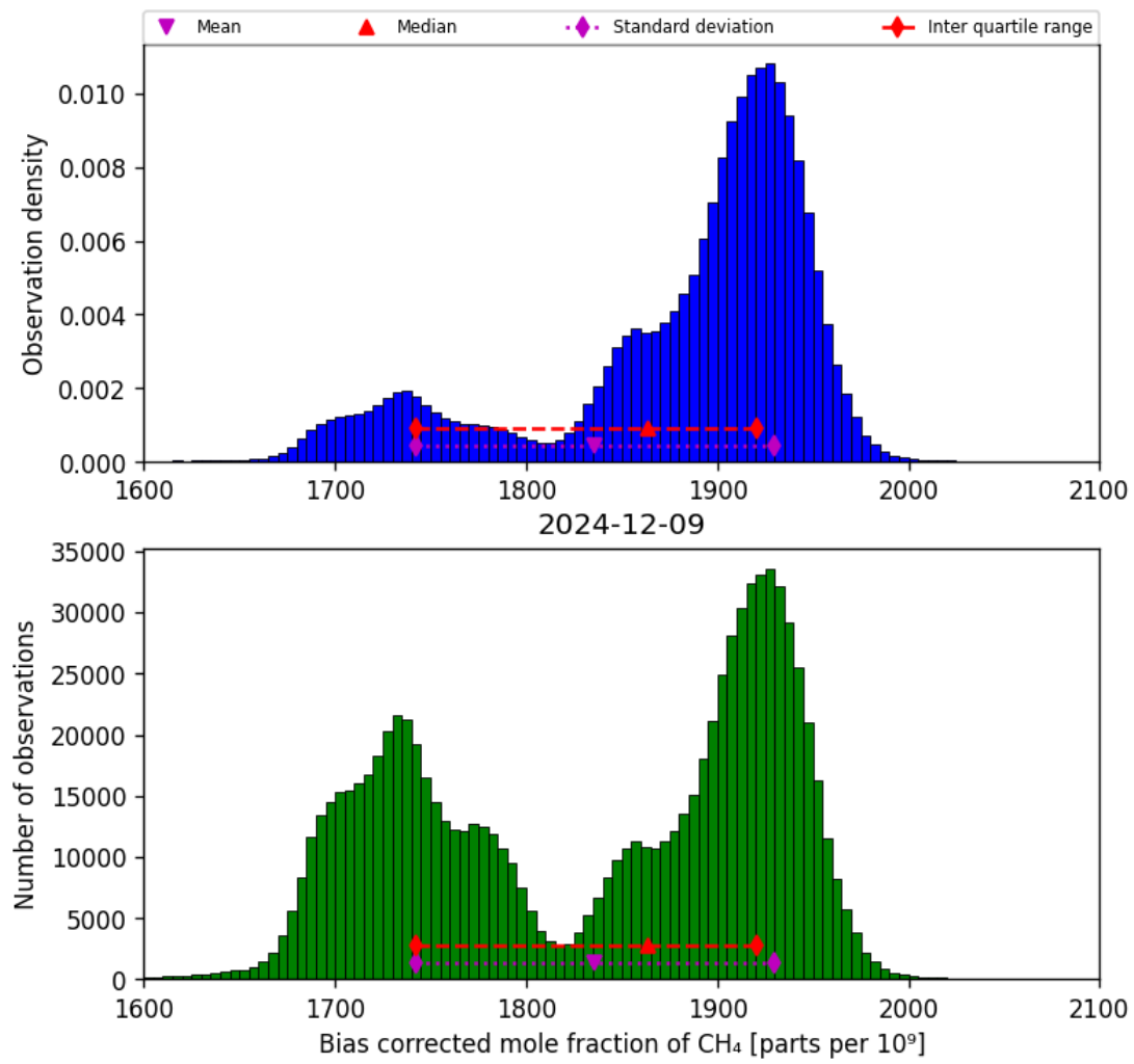
Figure 25: Histogram of “Bias corrected mole fraction of CH 4 ” for 2024-12-08 to 2024-12-10
