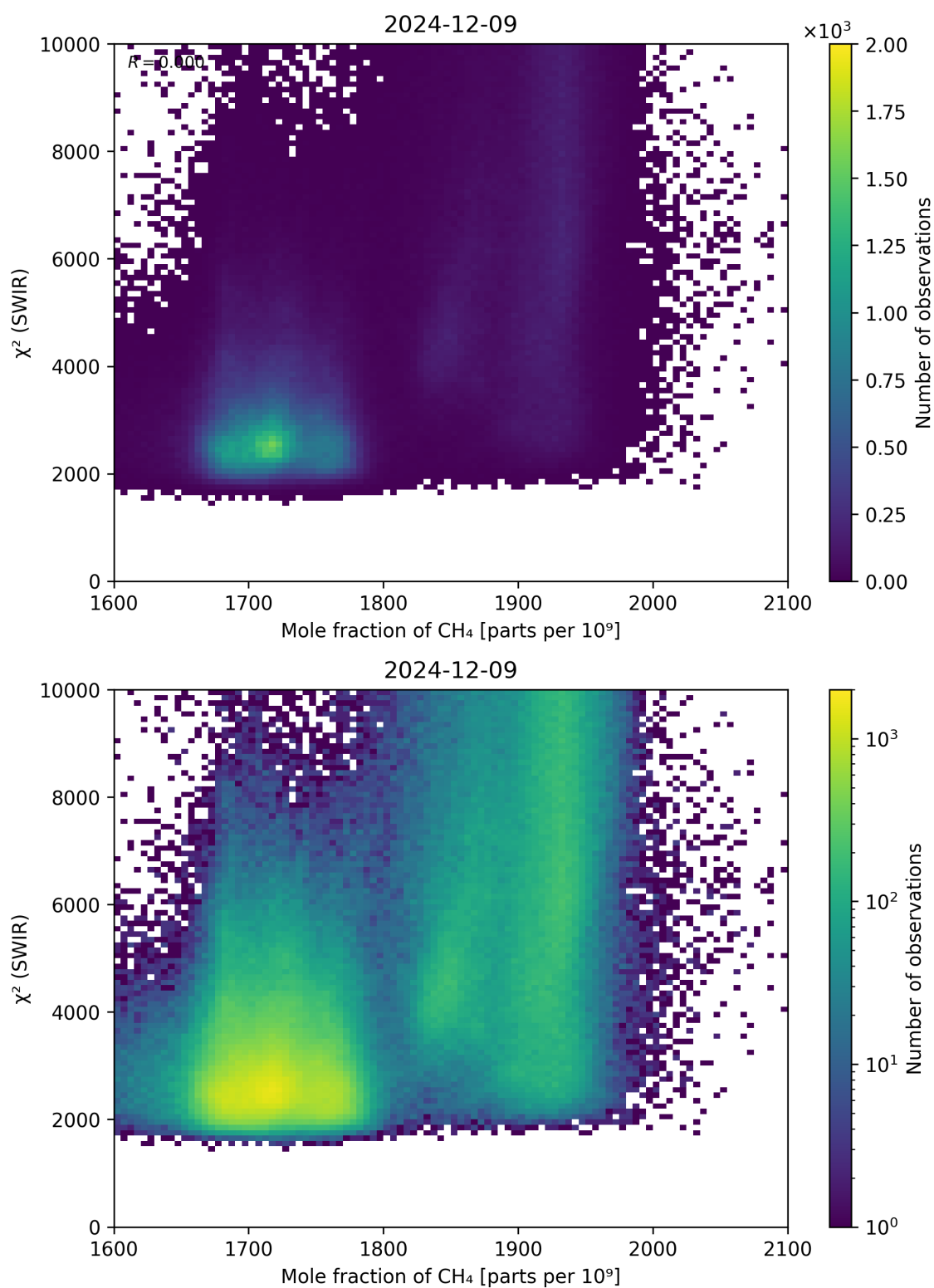
Figure 71: Scatter density plot of “Mole fraction of \text{CH}_4 ” against “ \chi^2 (SWIR)” for 2024-12-08 to 2024-12-10.
