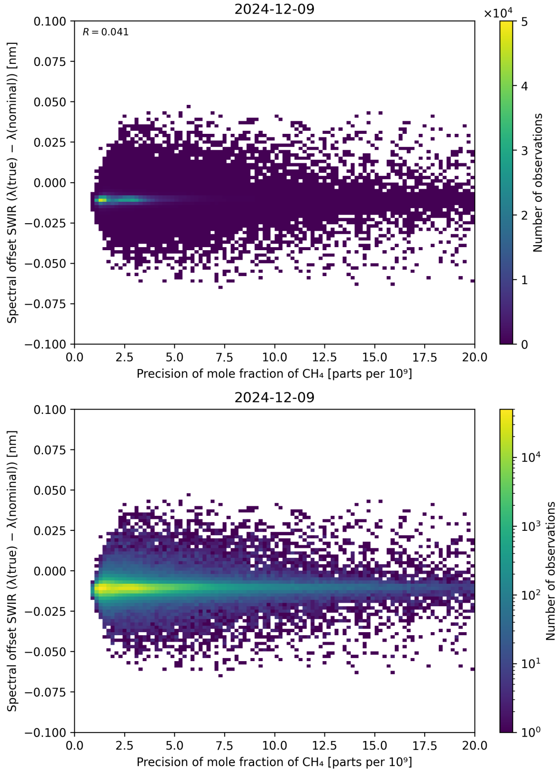
Figure 85: Scatter density plot of “Precision of mole fraction of \text{CH}_4 ” against “Spectral offset SWIR ( \lambda_{\text{true}} - \lambda_{\text{nominal}} )” for 2024-12-08 to 2024-12-10.
