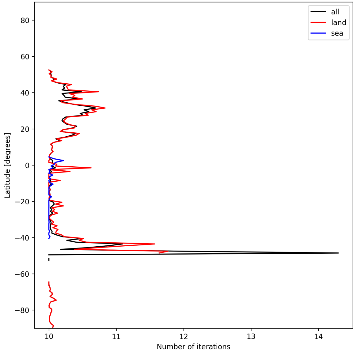
Figure 20: Zonal average of “Number of iterations” for 2024-12-08 to 2024-12-10.
