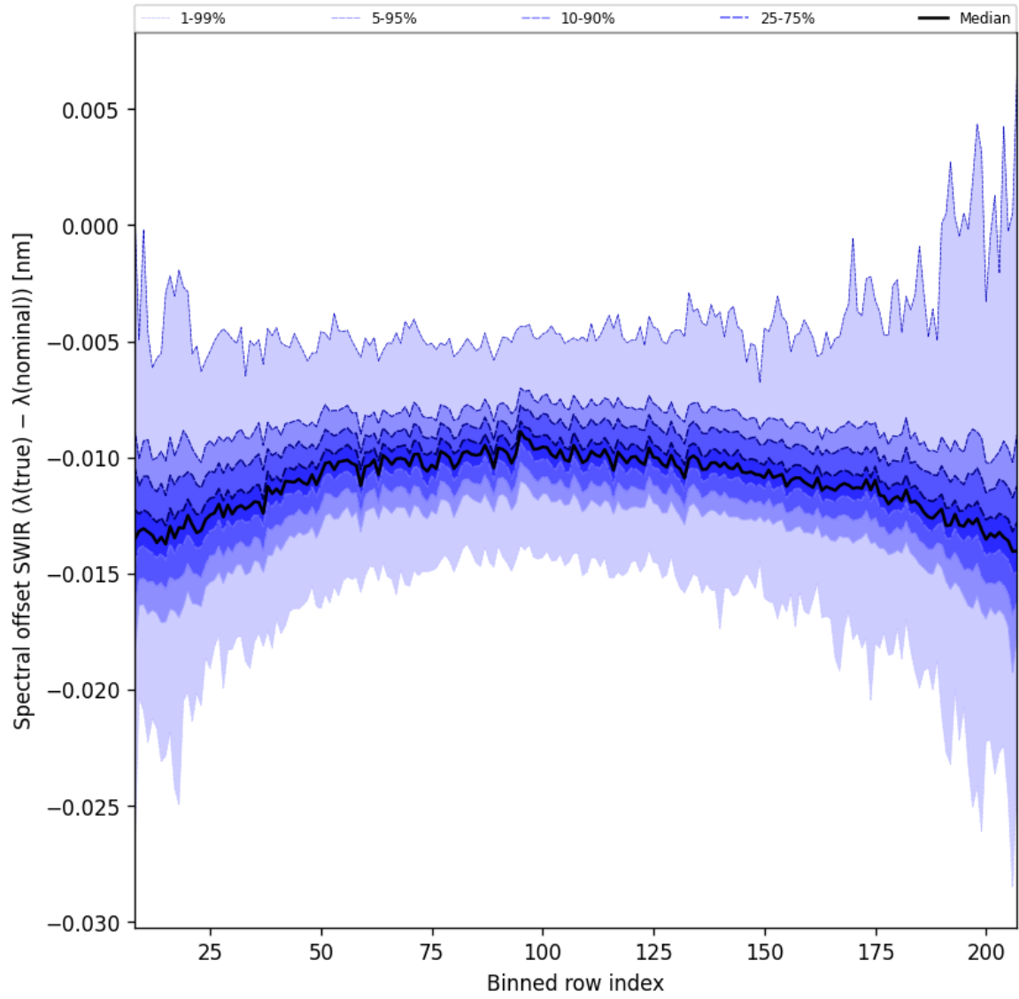
Figure 38: Along track statistics of “Spectral offset SWIR ( \lambda_{\text{true}} - \lambda_{\text{nominal}} )” for 2024-12-08 to 2024-12-10
