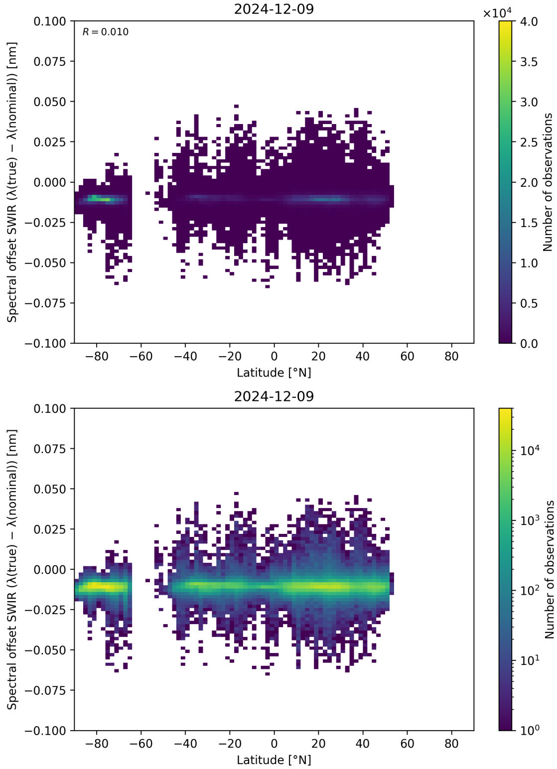
Figure 62: Scatter density plot of “Latitude” against “Spectral offset SWIR ( \lambda_{\text{true}} - \lambda_{\text{nominal}} )” for 2024-12-08 to 2024-12-10.
