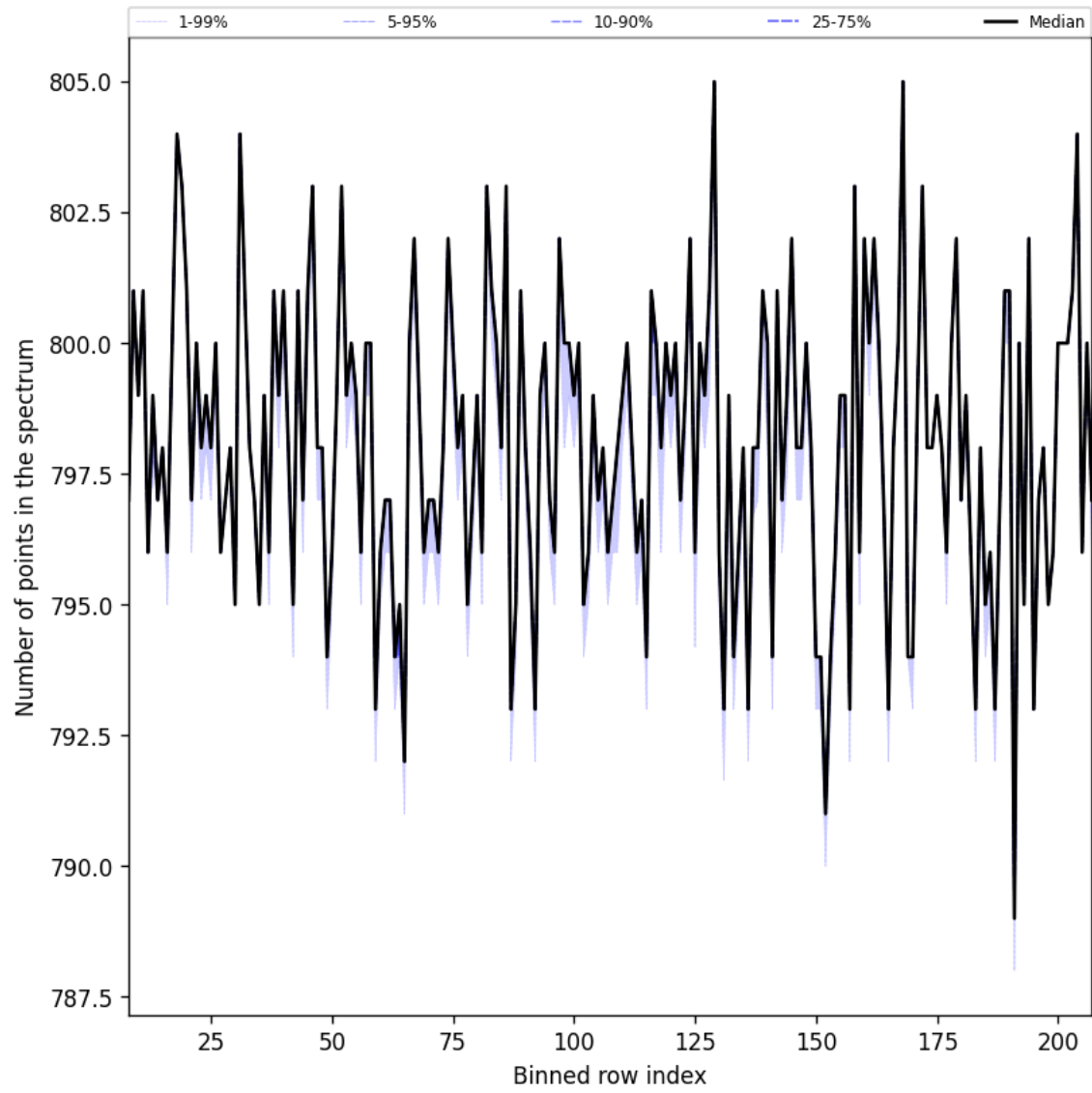
Figure 37: Along track statistics of “Number of points in the spectrum” for 2024-12-08 to 2024-12-10
