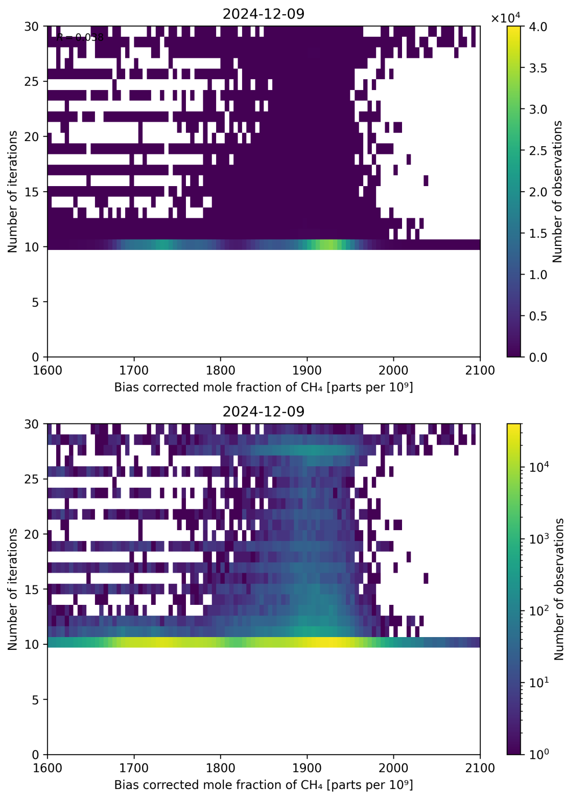
Figure 67: Scatter density plot of “Bias corrected mole fraction of CH 4 ” against “Number of iterations” for 2024-12-08 to 2024-12-10.
