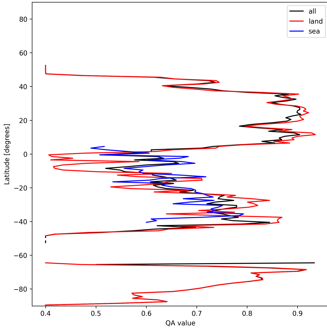
Figure 11: Zonal average of “QA value” for 2024-12-08 to 2024-12-10.
