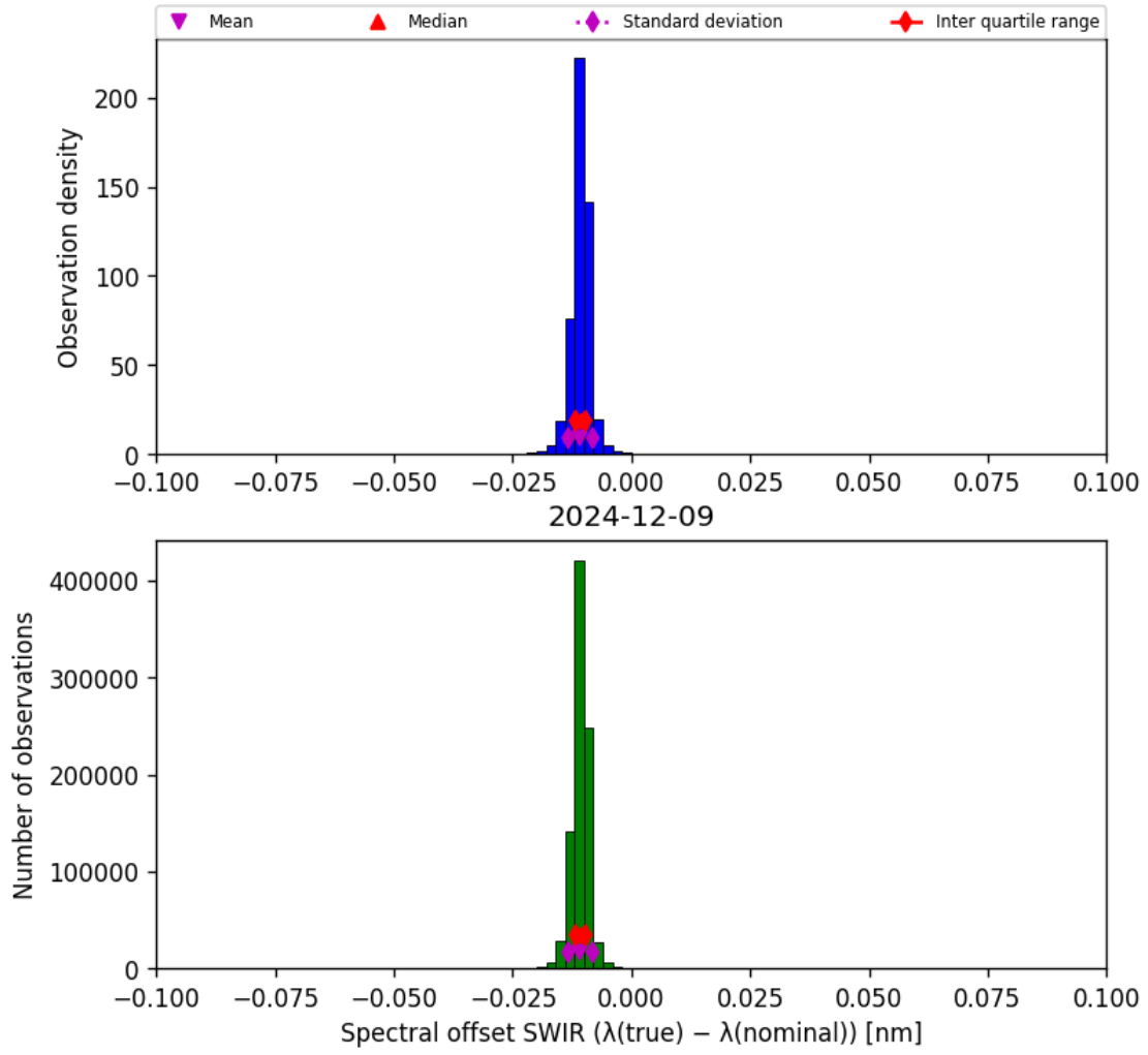
Figure 27: Histogram of “Spectral offset SWIR ( \lambda_{\text{true}} - \lambda_{\text{nominal}} )” for 2024-12-08 to 2024-12-10
