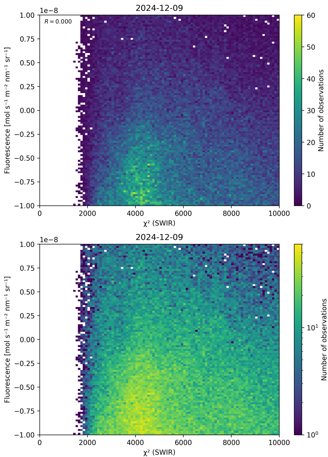
Figure 49: Scatter density plot of “ \chi^2 (SWIR)” against “Fluorescence” for 2024-12-08 to 2024-12-10.
