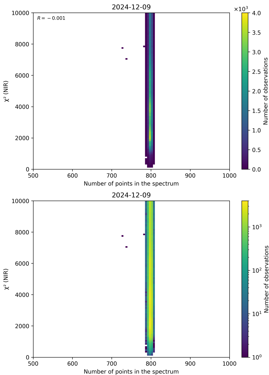
Figure 88: Scatter density plot of “Number of points in the spectrum” against “ \chi^2 (NIR)” for 2024-12-08 to 2024-12-10.
