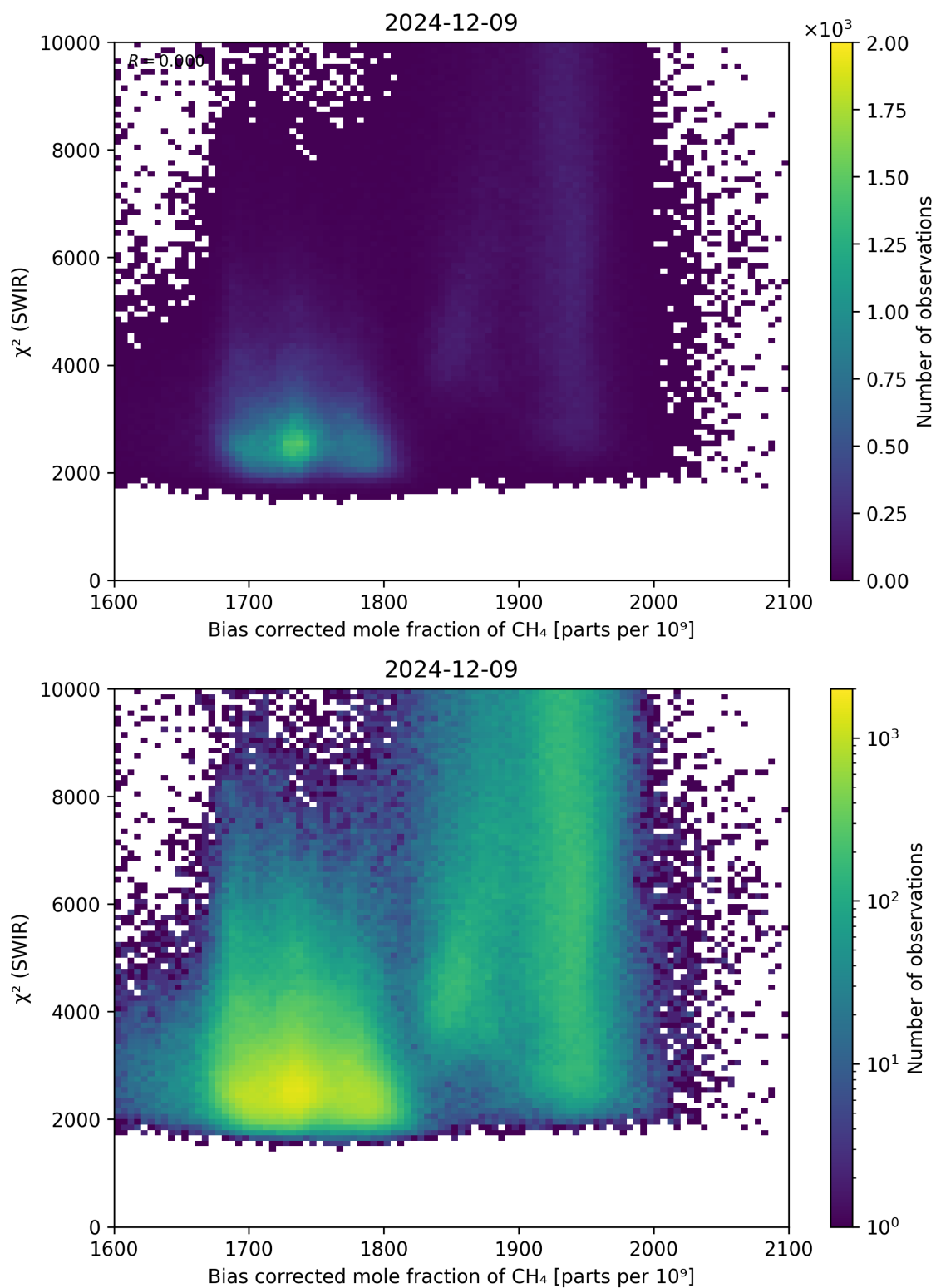
Figure 64: Scatter density plot of “Bias corrected mole fraction of \text{CH}_4 ” against “ \chi^2 (SWIR)” for 2024-12-08 to 2024-12-10.
