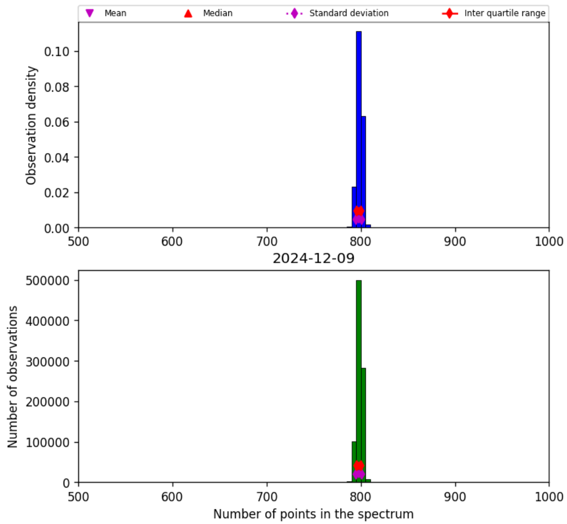
Figure 26: Histogram of “Number of points in the spectrum” for 2024-12-08 to 2024-12-10
