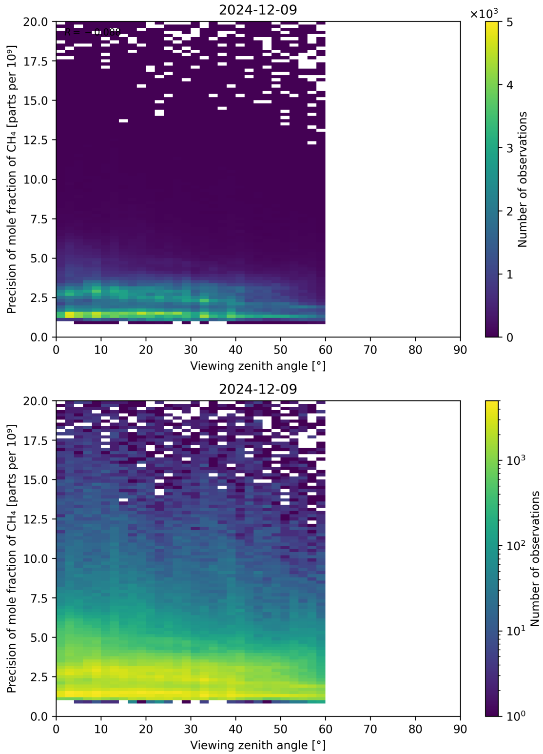
Figure 112: Scatter density plot of “Viewing zenith angle” against “Precision of mole fraction of CH 4 ” for 2024-12-08 to 2024-12-10.
