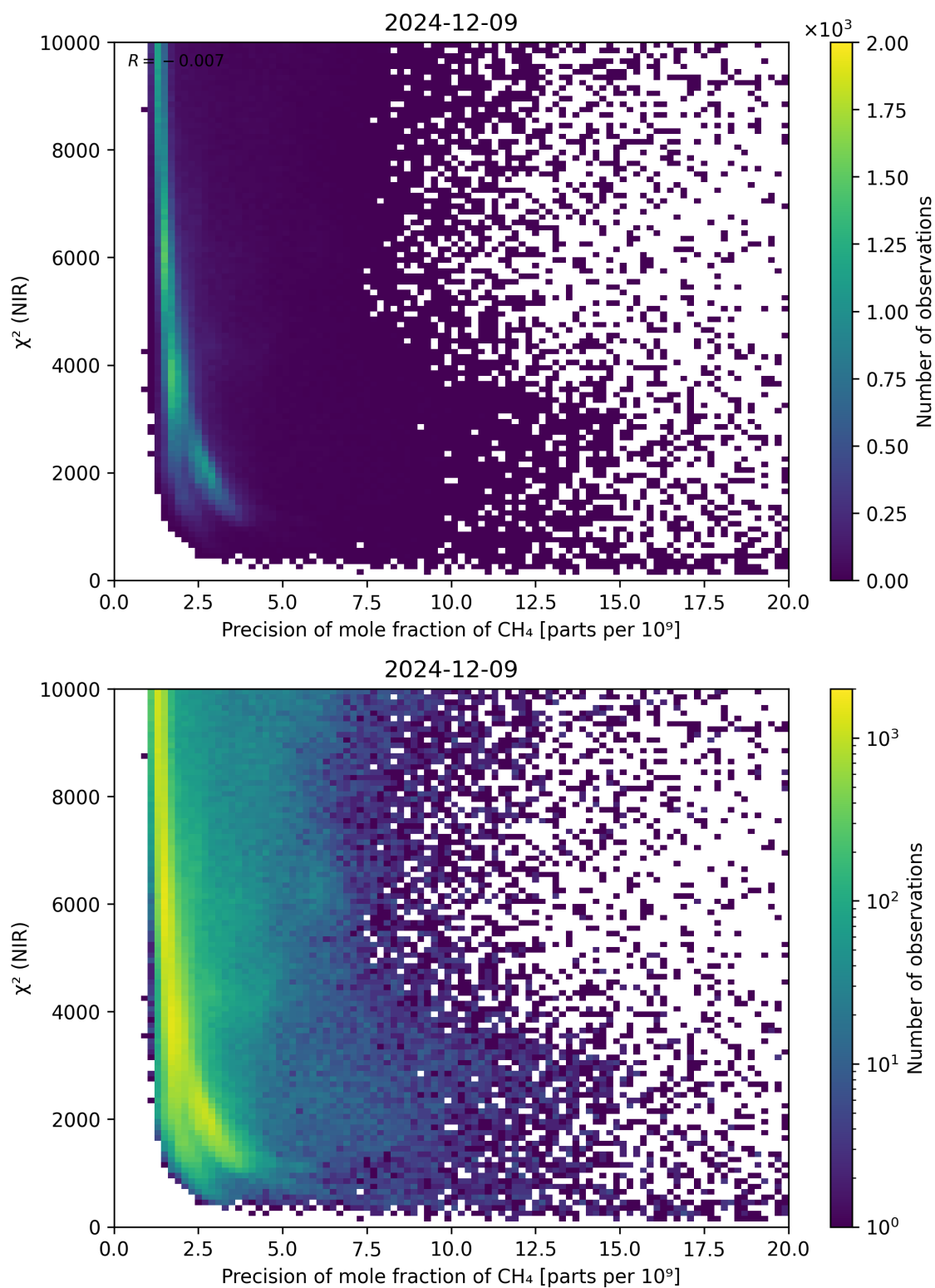
Figure 78: Scatter density plot of “Precision of mole fraction of \text{CH}_4 ” against “ \chi^2 (NIR)” for 2024-12-08 to 2024-12-10.
