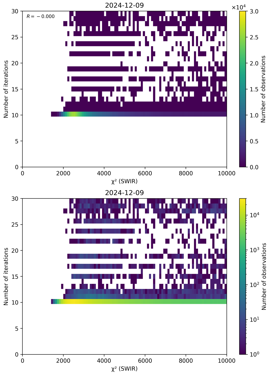
Figure 50: Scatter density plot of “ \chi^2 (SWIR)” against “Number of iterations” for 2024-12-08 to 2024-12-10.
