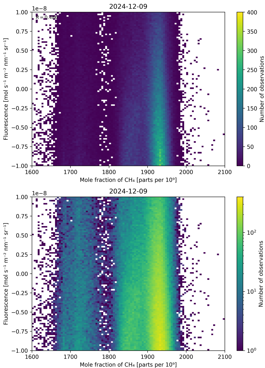
Figure 73: Scatter density plot of “Mole fraction of \text{CH}_4 ” against “Fluorescence” for 2024-12-08 to 2024-12-10.
