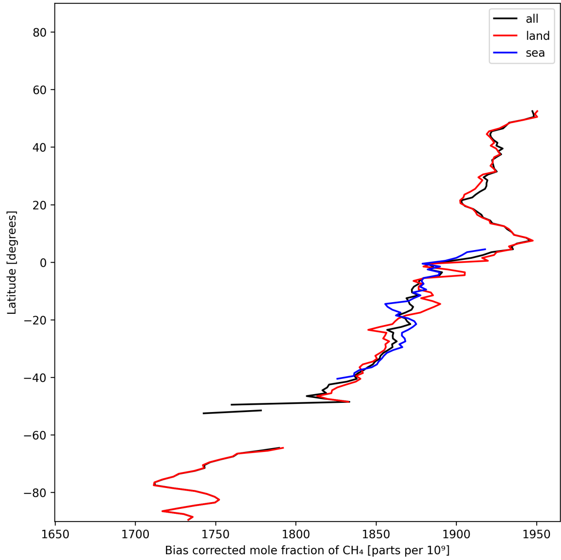
Figure 14: Zonal average of “Bias corrected mole fraction of CH 4 ” for 2024-12-08 to 2024-12-10.
