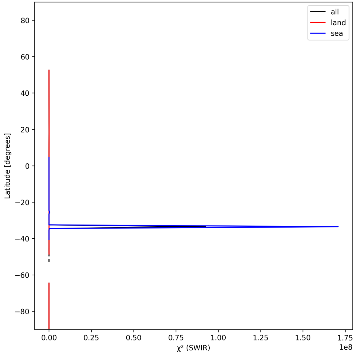
Figure 17: Zonal average of “ \chi^2 (SWIR)” for 2024-12-08 to 2024-12-10.
