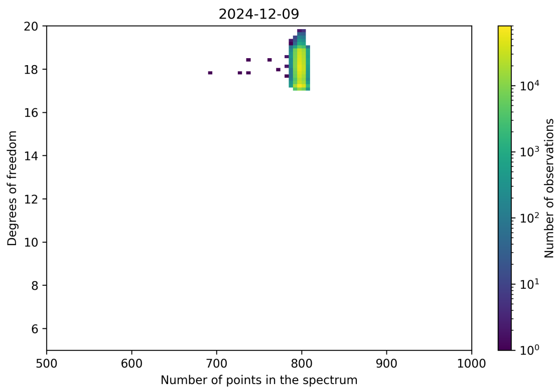
Figure 90: Scatter density plot of “Number of points in the spectrum” against “Degrees of freedom” for 2024-12-08 to 2024-12-10.
