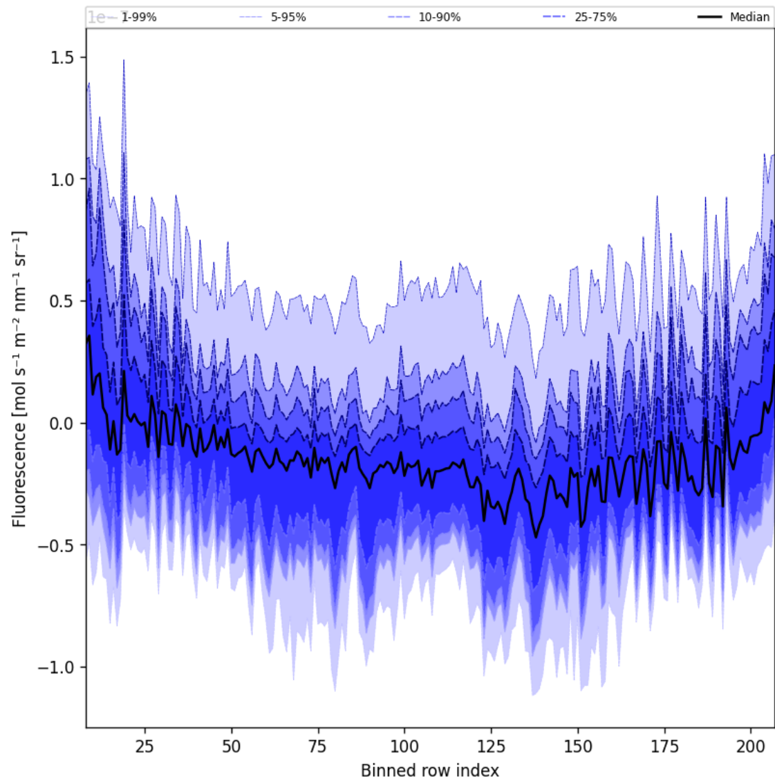
Figure 43: Along track statistics of “Fluorescence” for 2024-12-08 to 2024-12-10
