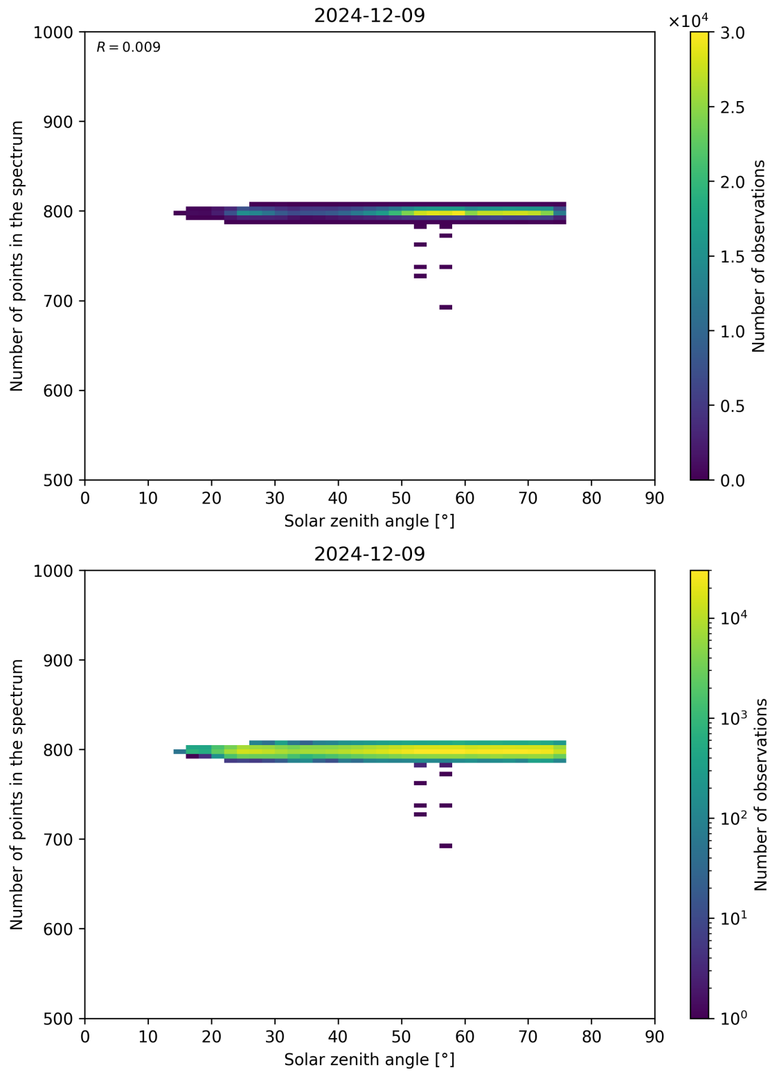
Figure 103: Scatter density plot of “Solar zenith angle” against “Number of points in the spectrum” for 2024-12-08 to 2024-12-10.
