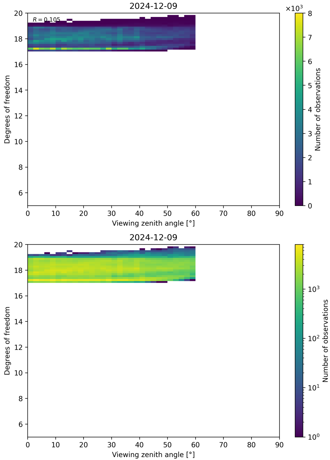
Figure 107: Scatter density plot of “Viewing zenith angle” against “Degrees of freedom” for 2024-12-08 to 2024-12-10.
