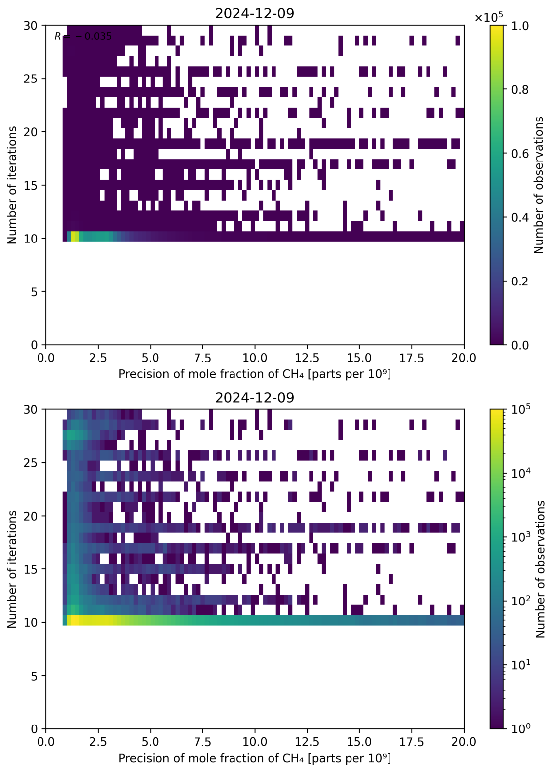
Figure 83: Scatter density plot of “Precision of mole fraction of CH 4 ” against “Number of iterations” for 2024-12-08 to 2024-12-10.
