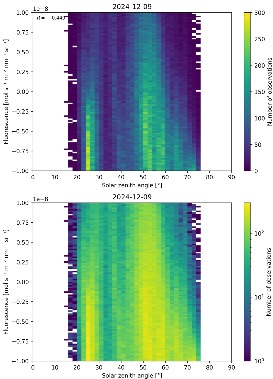
Figure 97: Scatter density plot of “Solar zenith angle” against “Fluorescence” for 2024-12-08 to 2024-12-10.
