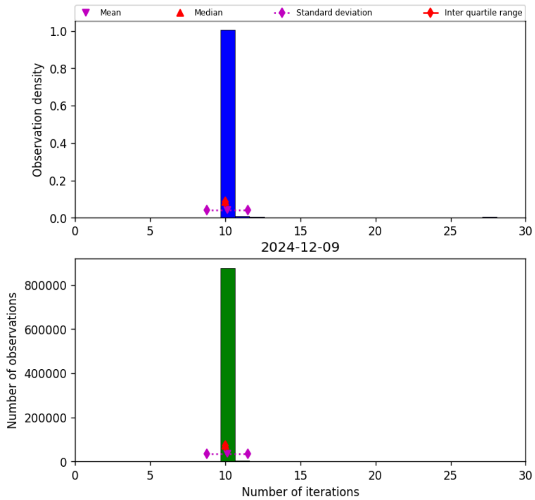
Figure 31: Histogram of “Number of iterations” for 2024-12-08 to 2024-12-10
