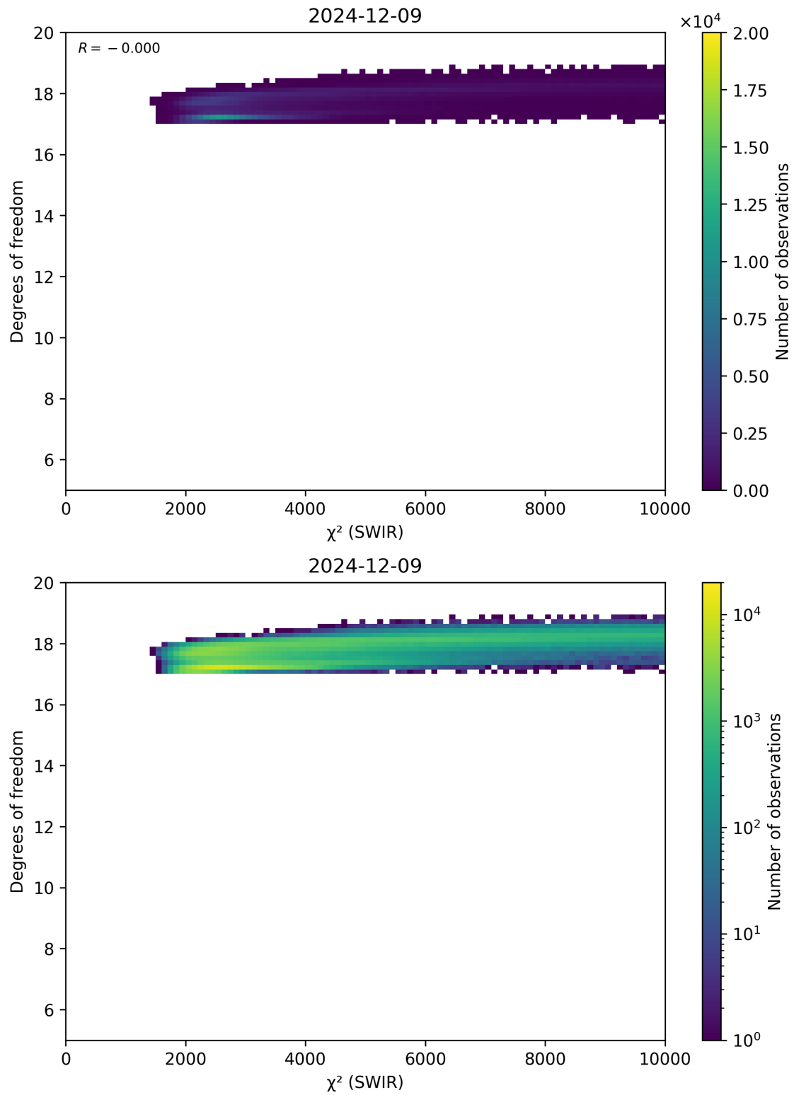
Figure 48: Scatter density plot of “ \chi^2 (SWIR)” against “Degrees of freedom” for 2024-12-08 to 2024-12-10.
