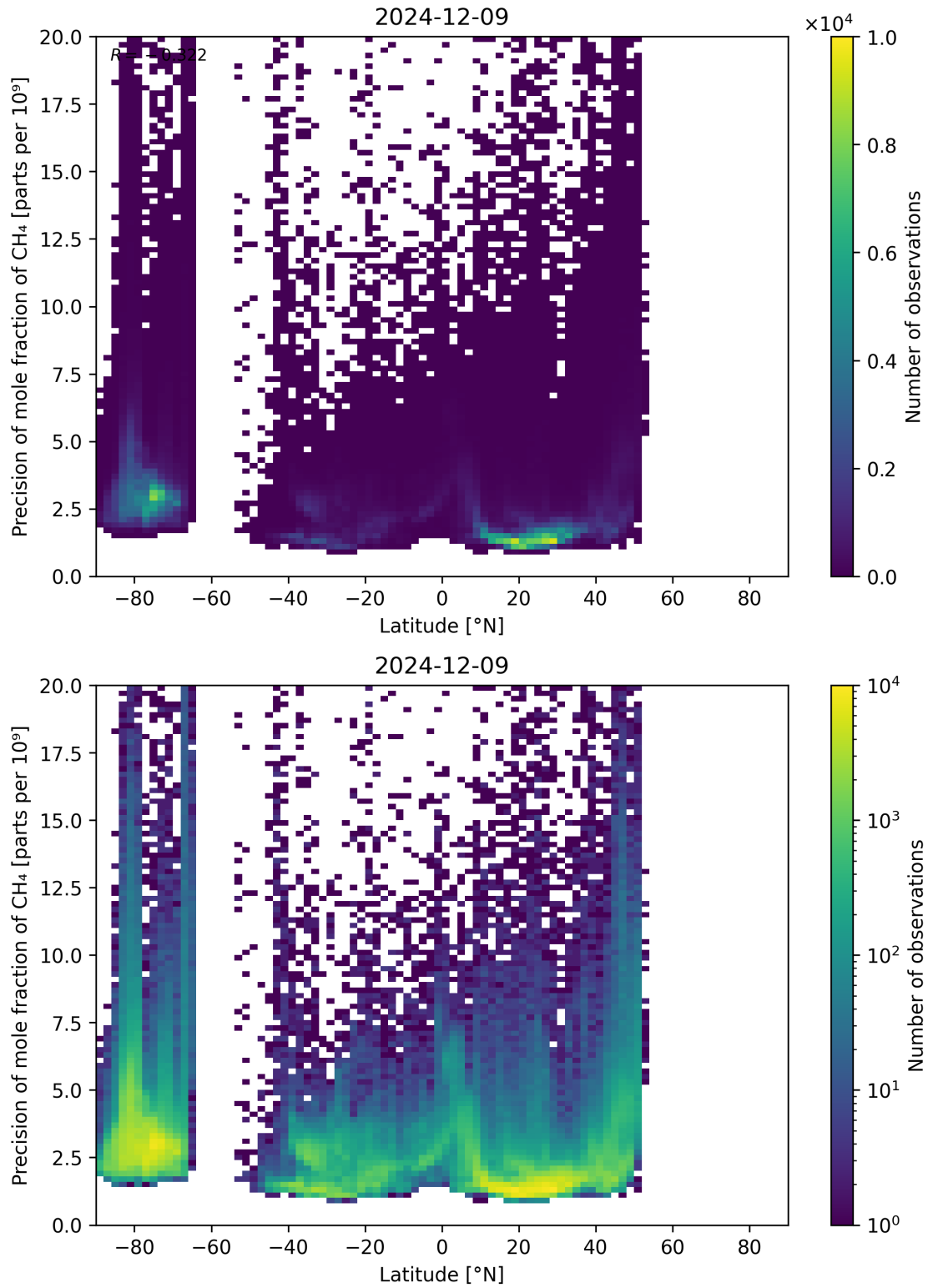
Figure 59: Scatter density plot of “Latitude” against “Precision of mole fraction of CH 4 ” for 2024-12-08 to 2024-12-10.
