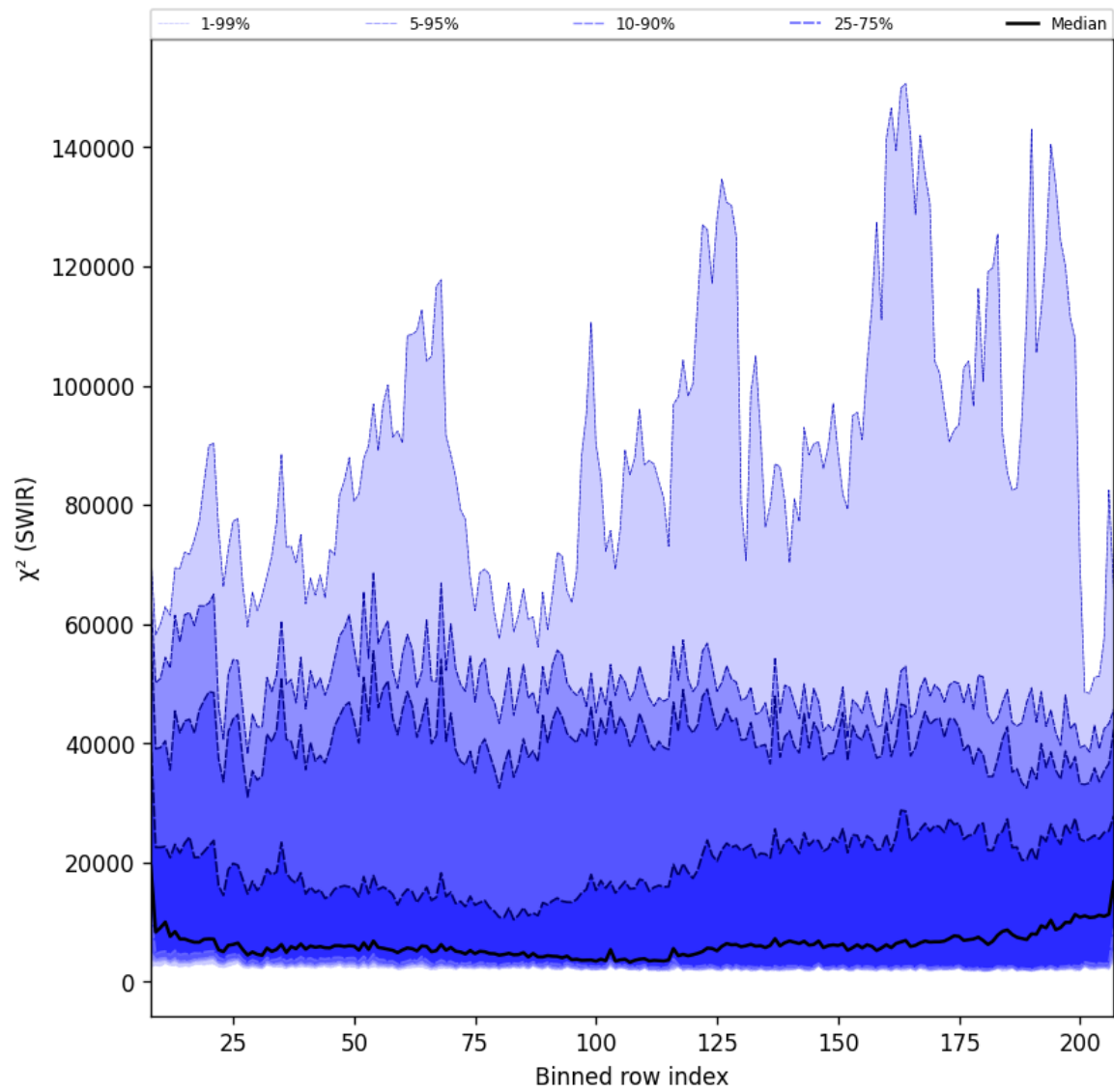
Figure 39: Along track statistics of “ \chi^2 (SWIR)” for 2024-12-08 to 2024-12-10
