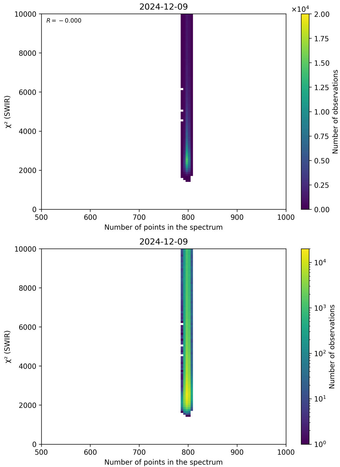
Figure 89: Scatter density plot of “Number of points in the spectrum” against “ \chi^2 (SWIR)” for 2024-12-08 to 2024-12-10.
