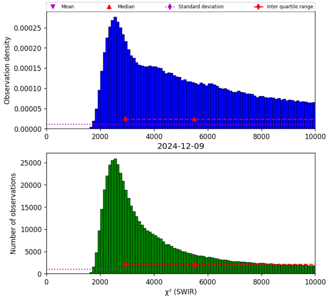
Figure 28: Histogram of “ \chi^2 (SWIR)” for 2024-12-08 to 2024-12-10
