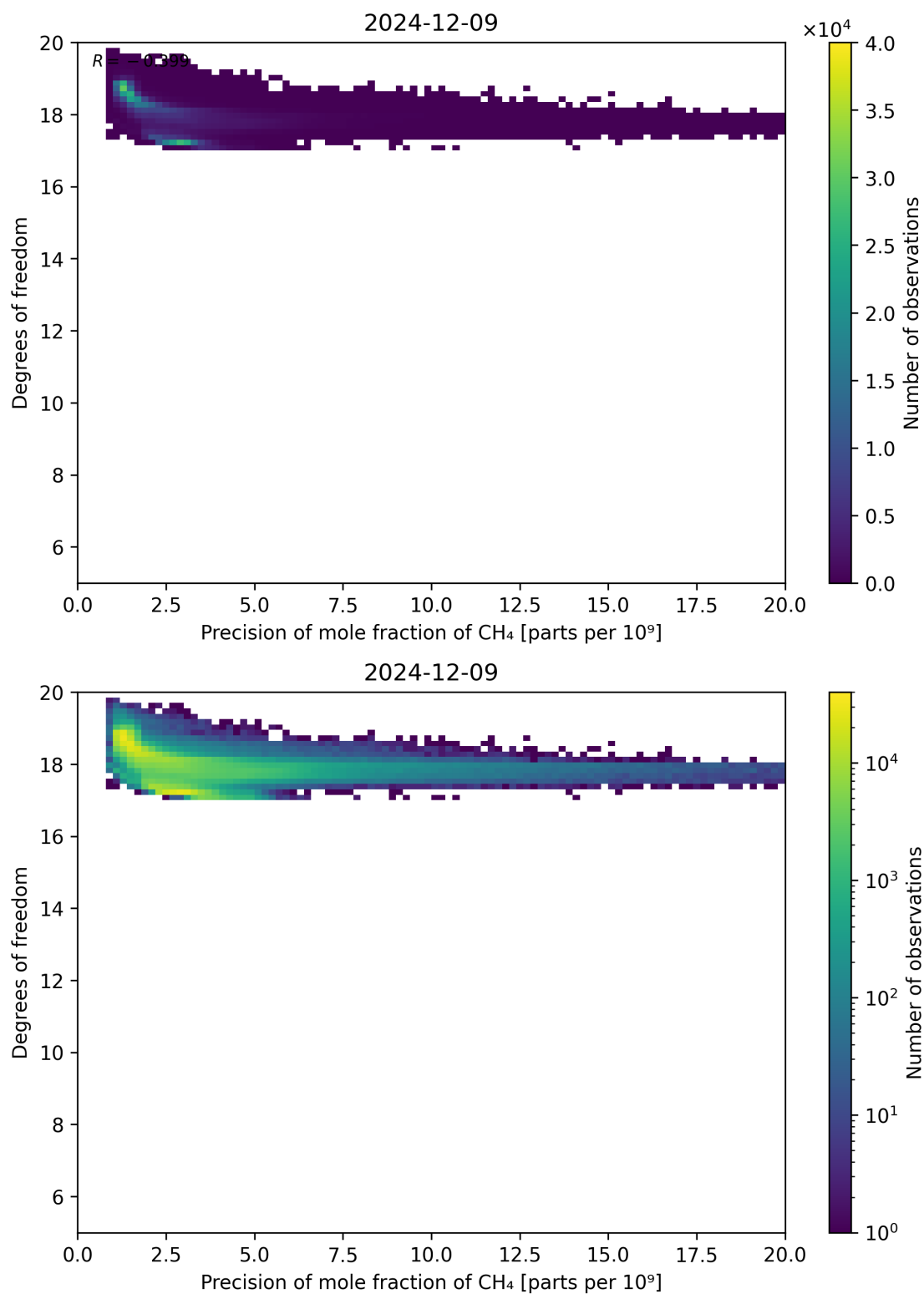
Figure 80: Scatter density plot of “Precision of mole fraction of CH 4 ” against “Degrees of freedom” for 2024-12-08 to 2024-12-10.
