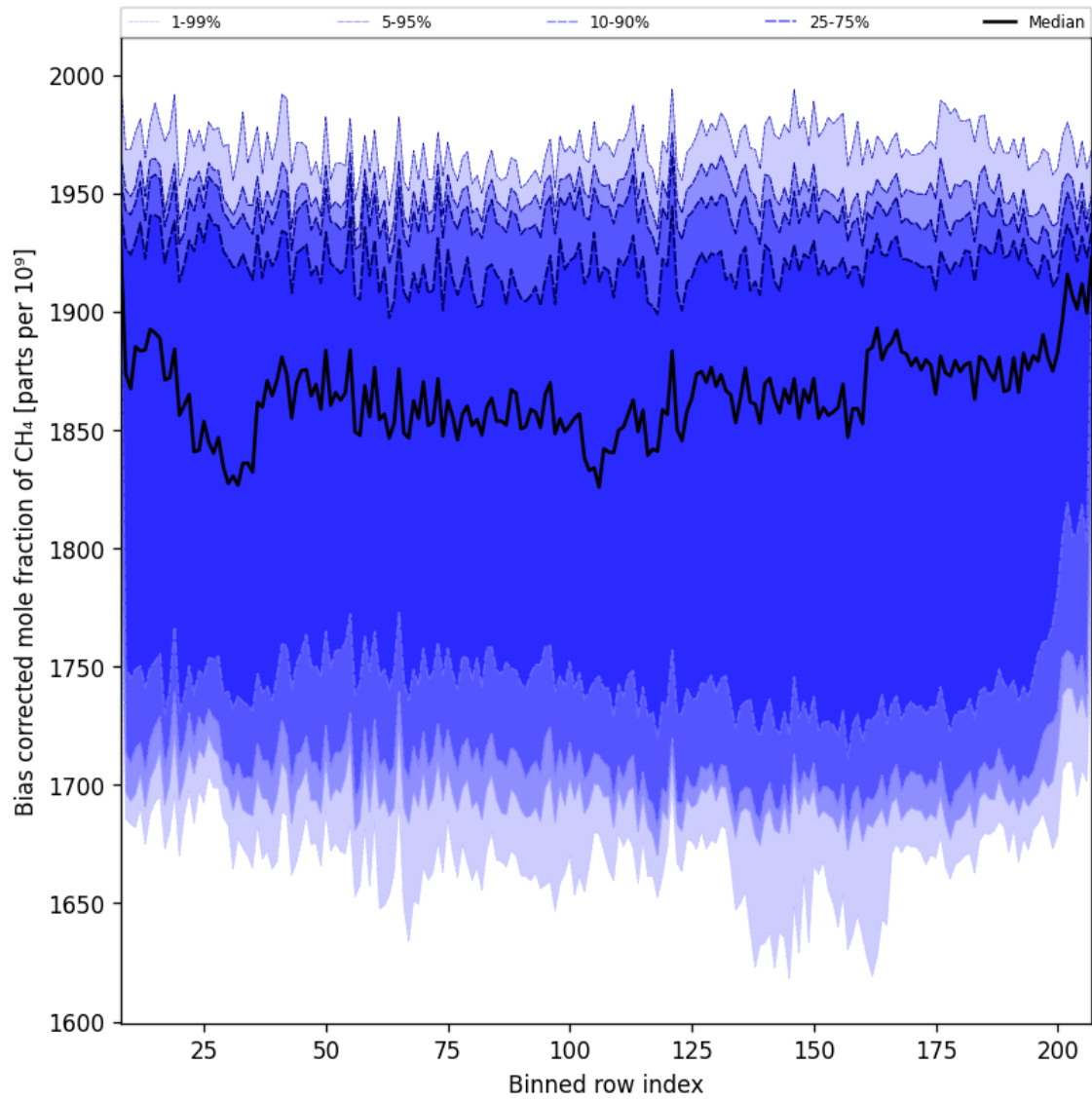
Figure 36: Along track statistics of “Bias corrected mole fraction of CH 4 ” for 2024-12-08 to 2024-12-10
