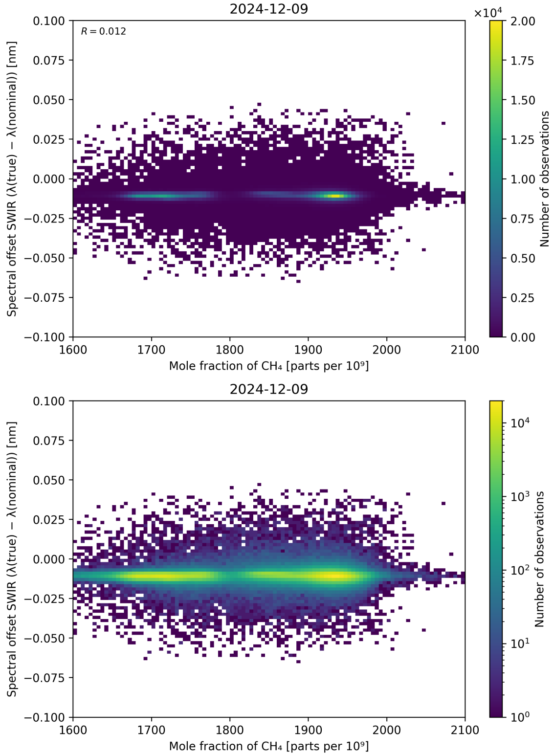
Figure 86: Scatter density plot of “Mole fraction of \text{CH}_4 ” against “Spectral offset SWIR ( \lambda_{\text{true}} - \lambda_{\text{nominal}} )” for 2024-12-08 to 2024-12-10.
