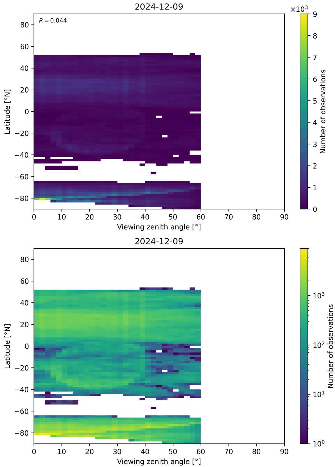
Figure 109: Scatter density plot of “Viewing zenith angle” against “Latitude” for 2024-12-08 to 2024-12-10.
