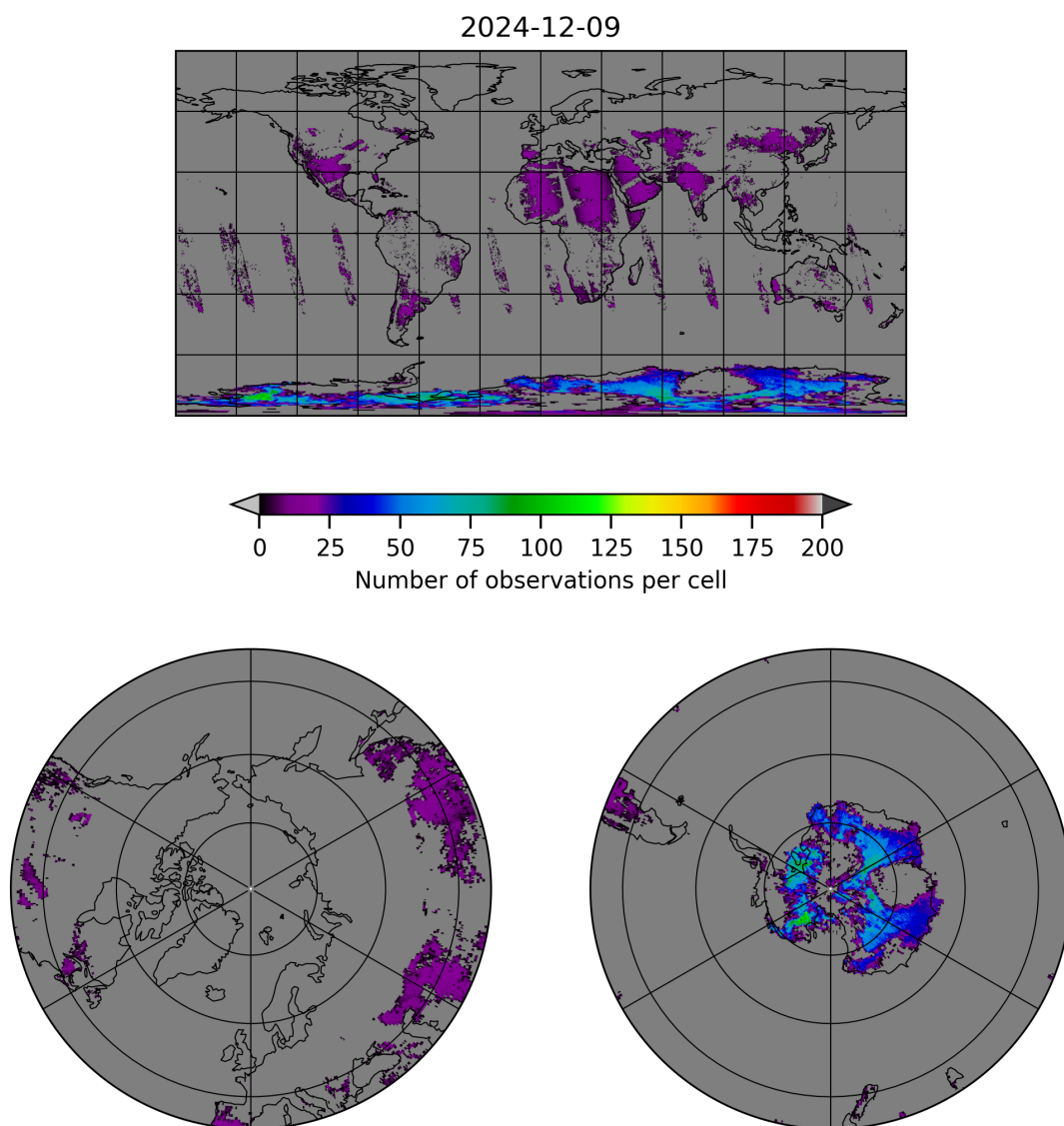
Figure 10: Map of the number of observations for 2024-12-08 to 2024-12-10
