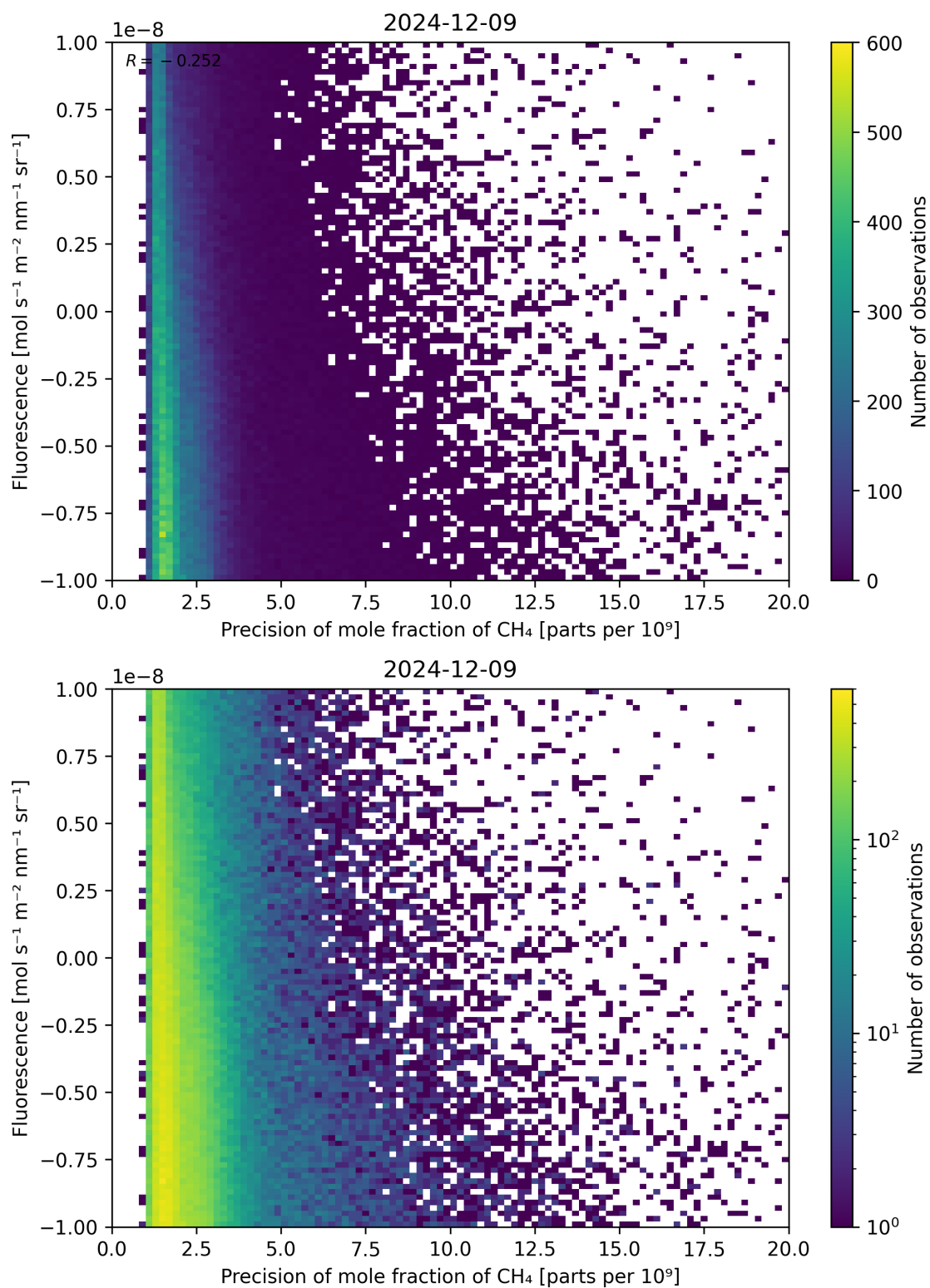
Figure 81: Scatter density plot of “Precision of mole fraction of \text{CH}_4 ” against “Fluorescence” for 2024-12-08 to 2024-12-10.
