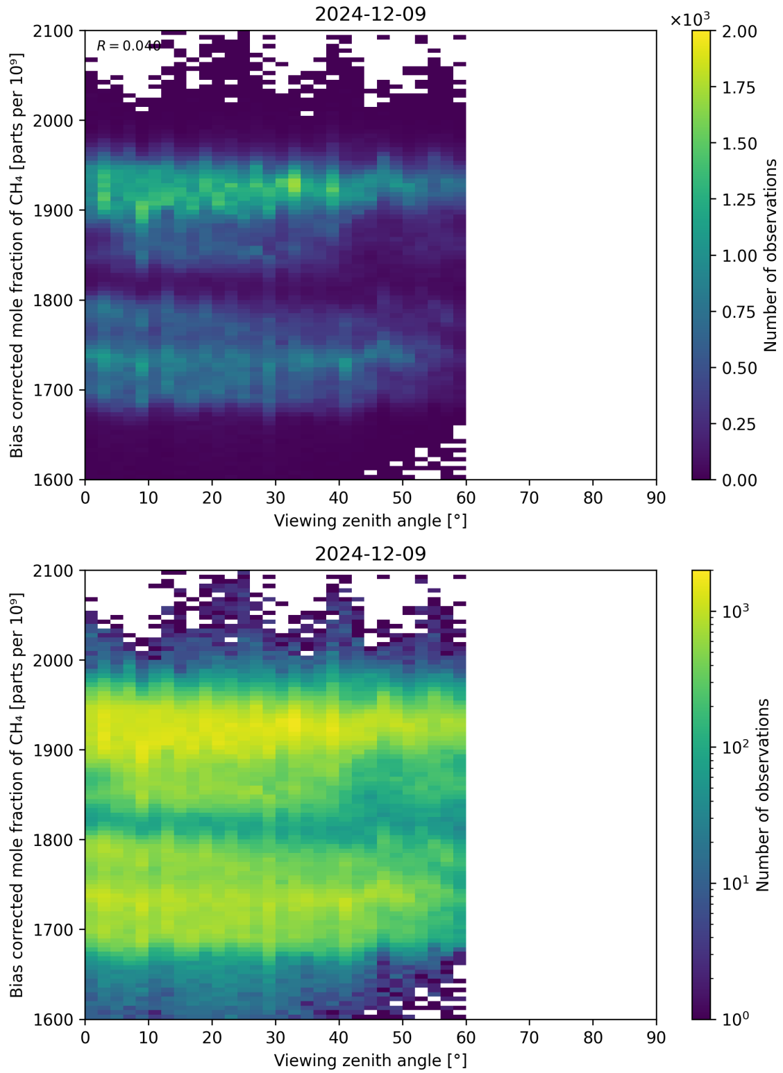
Figure 111: Scatter density plot of “Viewing zenith angle” against “Bias corrected mole fraction of CH 4 ” for 2024-12-08 to 2024-12-10.
