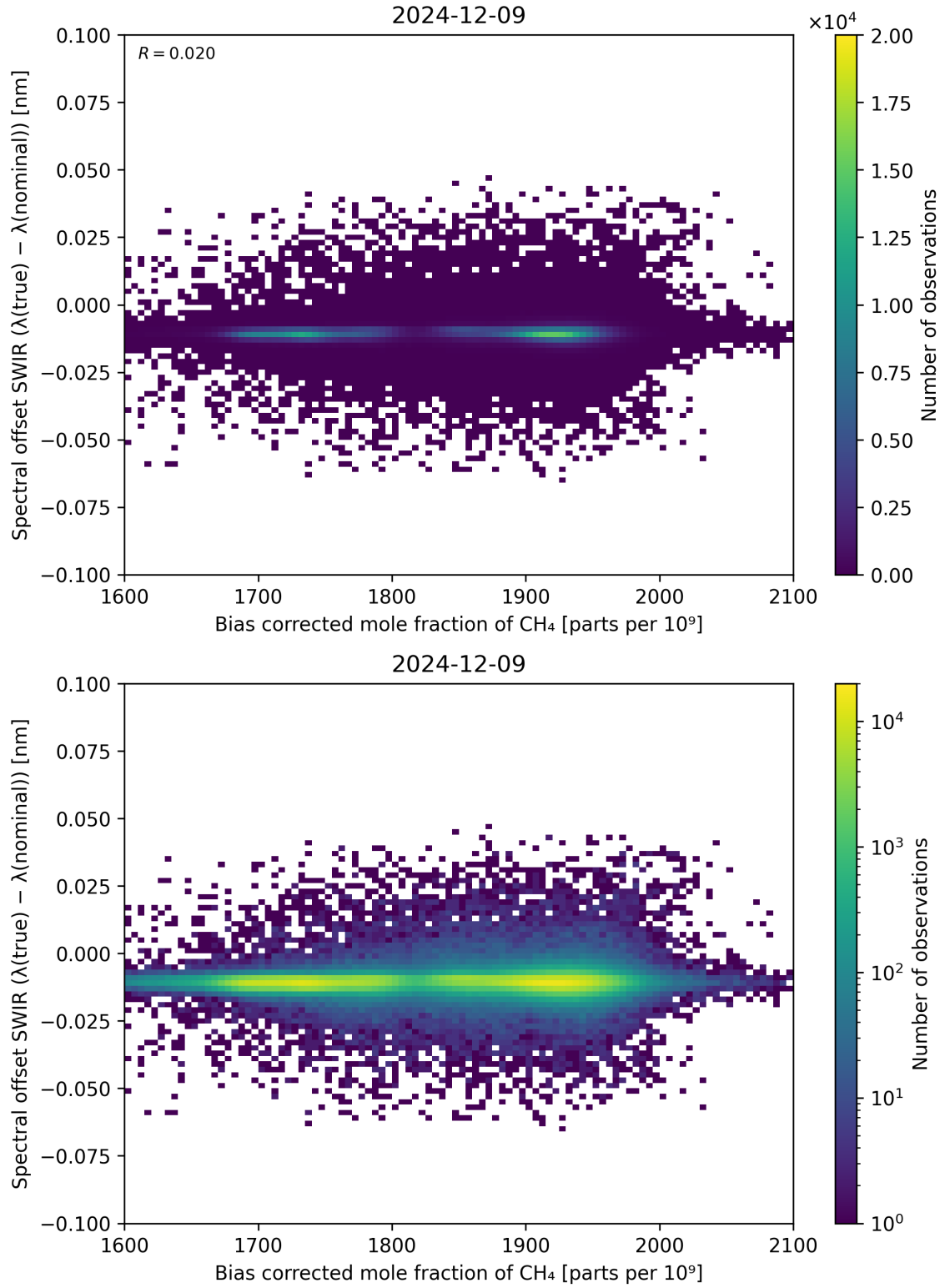
Figure 69: Scatter density plot of “Bias corrected mole fraction of \text{CH}_4 ” against “Spectral offset SWIR ( \lambda_{\text{true}} - \lambda_{\text{nominal}} )” for 2024-12-08 to 2024-12-10.
