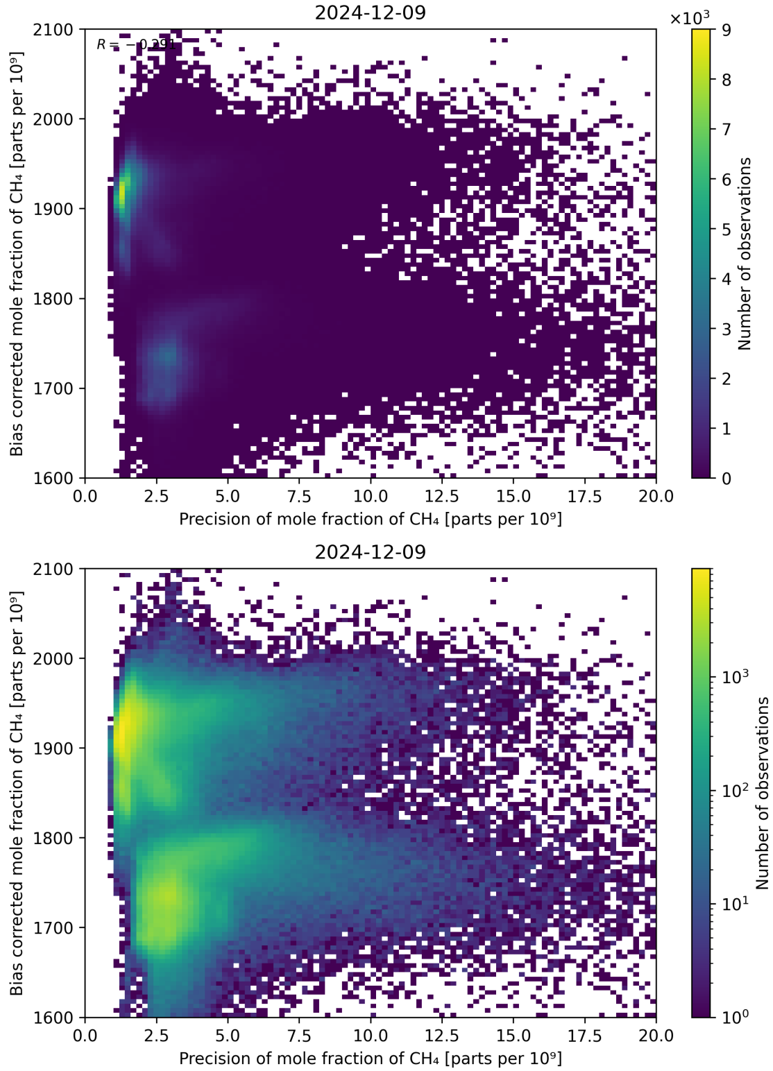
Figure 82: Scatter density plot of “Precision of mole fraction of CH 4 ” against “Bias corrected mole fraction of CH 4 ” for 2024-12-08 to 2024-12-10.
