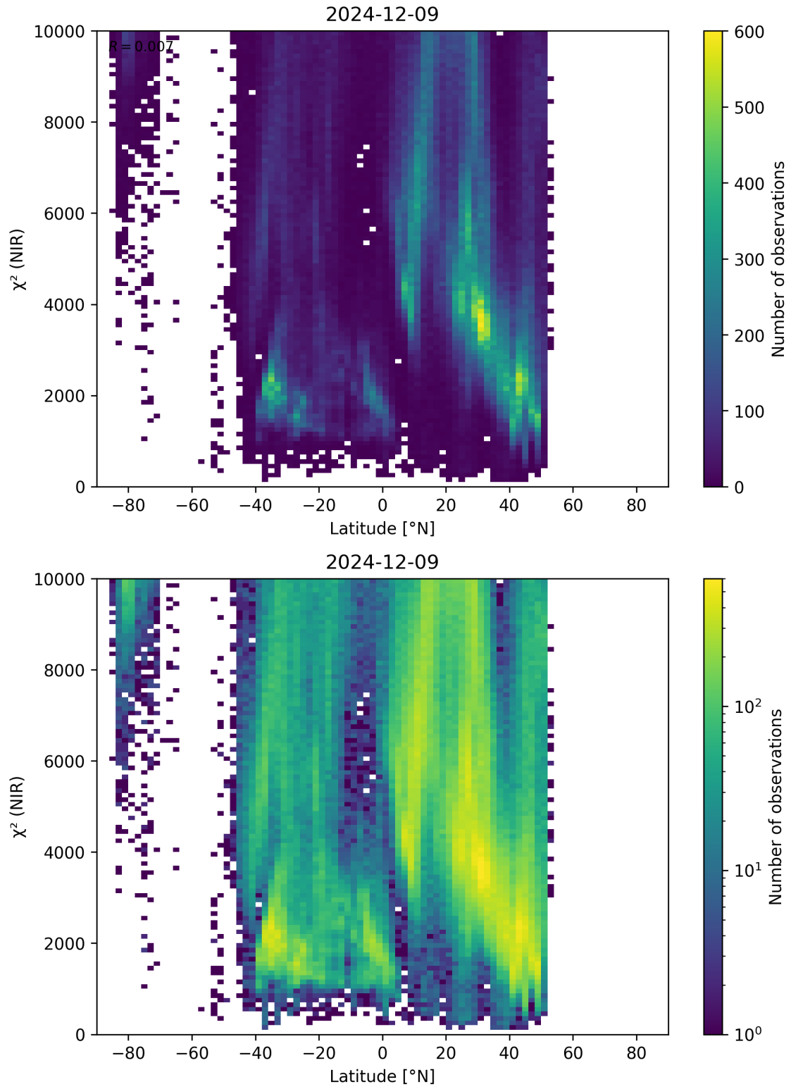
Figure 53: Scatter density plot of “Latitude” against “ \chi^2 (NIR)” for 2024-12-08 to 2024-12-10.
