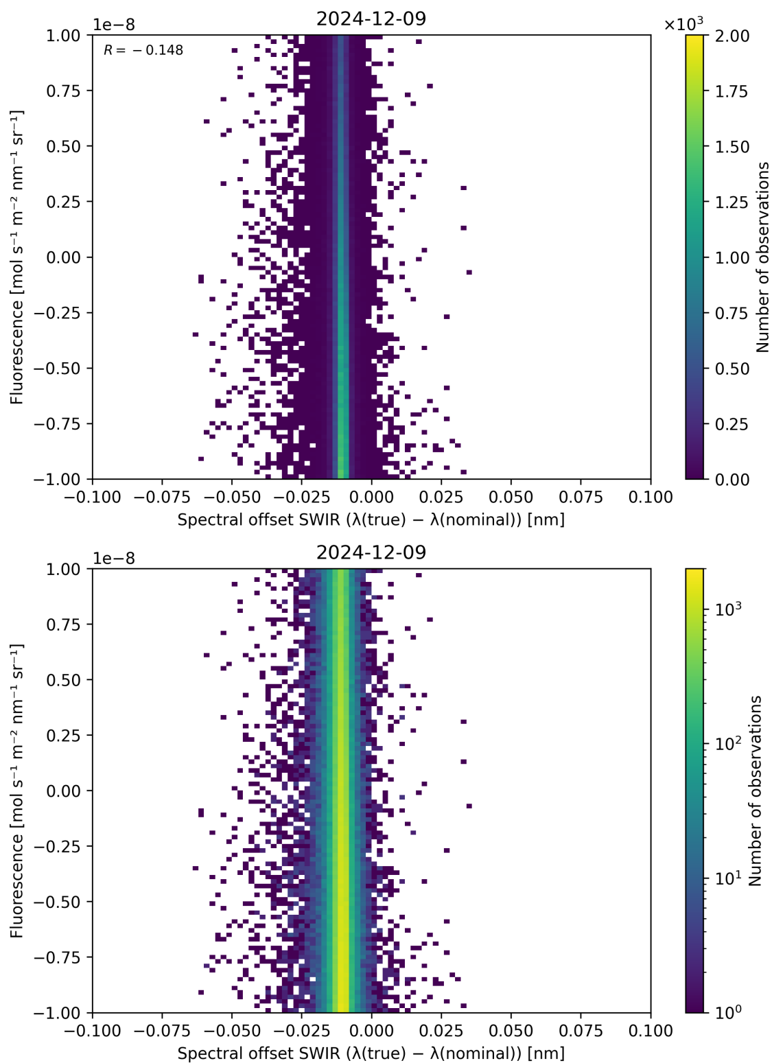
Figure 120: Scatter density plot of “Spectral offset SWIR ( \lambda_{\text{true}} - \lambda_{\text{nominal}} )” against “Fluorescence” for 2024-12-08 to 2024-12-10.
