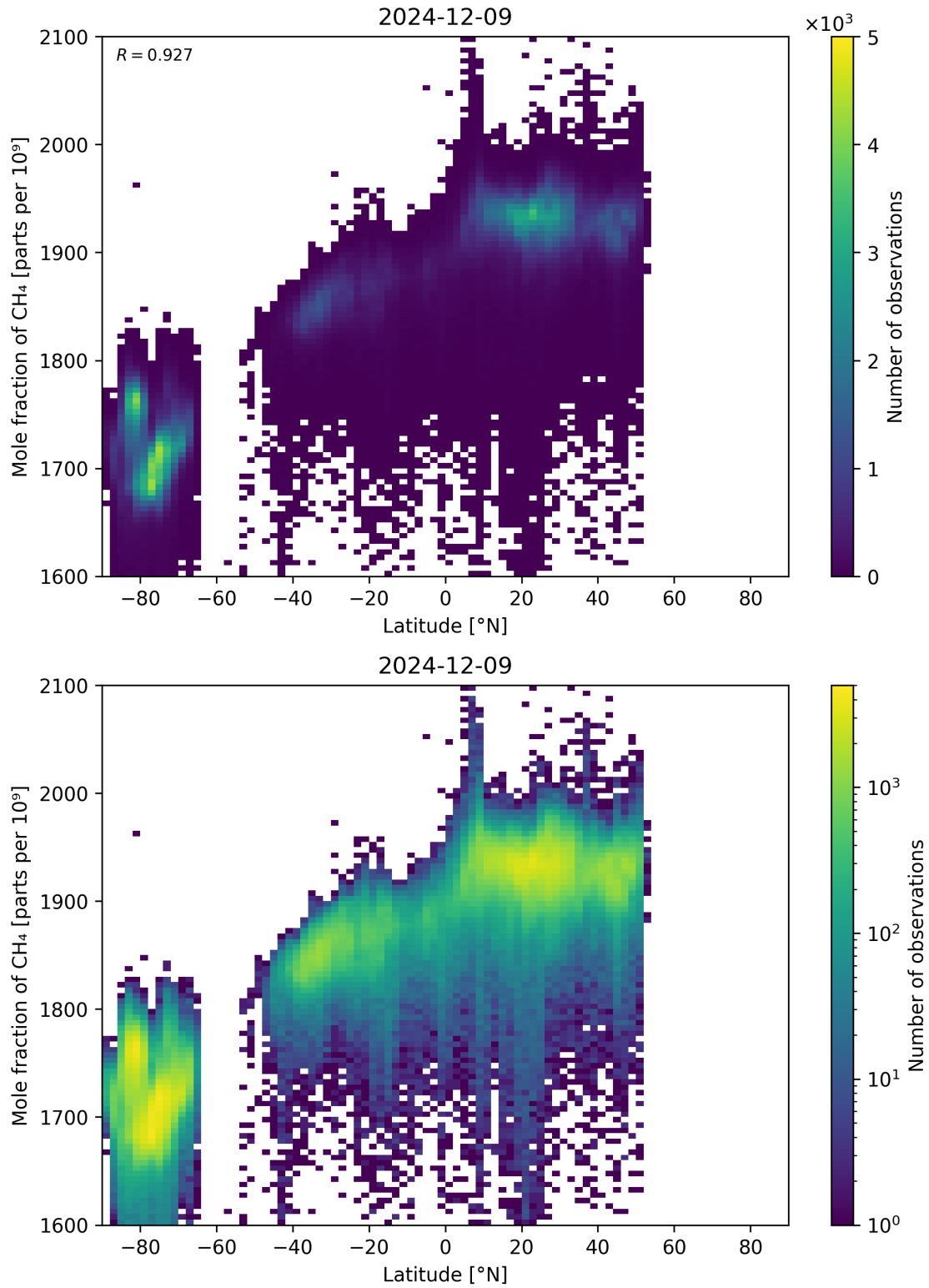
Figure 57: Scatter density plot of “Latitude” against “Mole fraction of CH 4 ” for 2024-12-08 to 2024-12-10.
