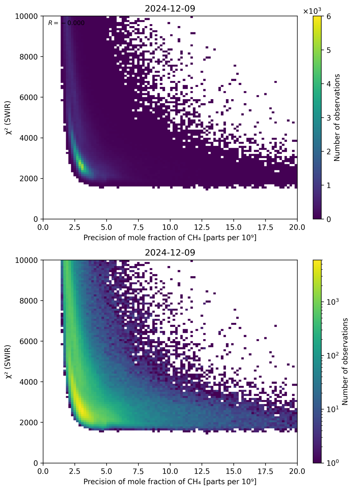
Figure 79: Scatter density plot of “Precision of mole fraction of CH 4 ” against “ \chi^2 (SWIR)” for 2024-12-08 to 2024-12-10.
