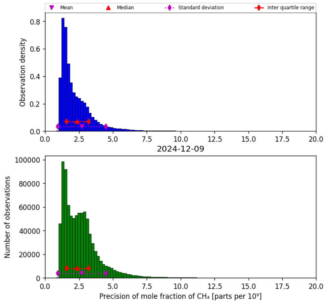
Figure 24: Histogram of “Precision of mole fraction of CH 4 ” for 2024-12-08 to 2024-12-10
