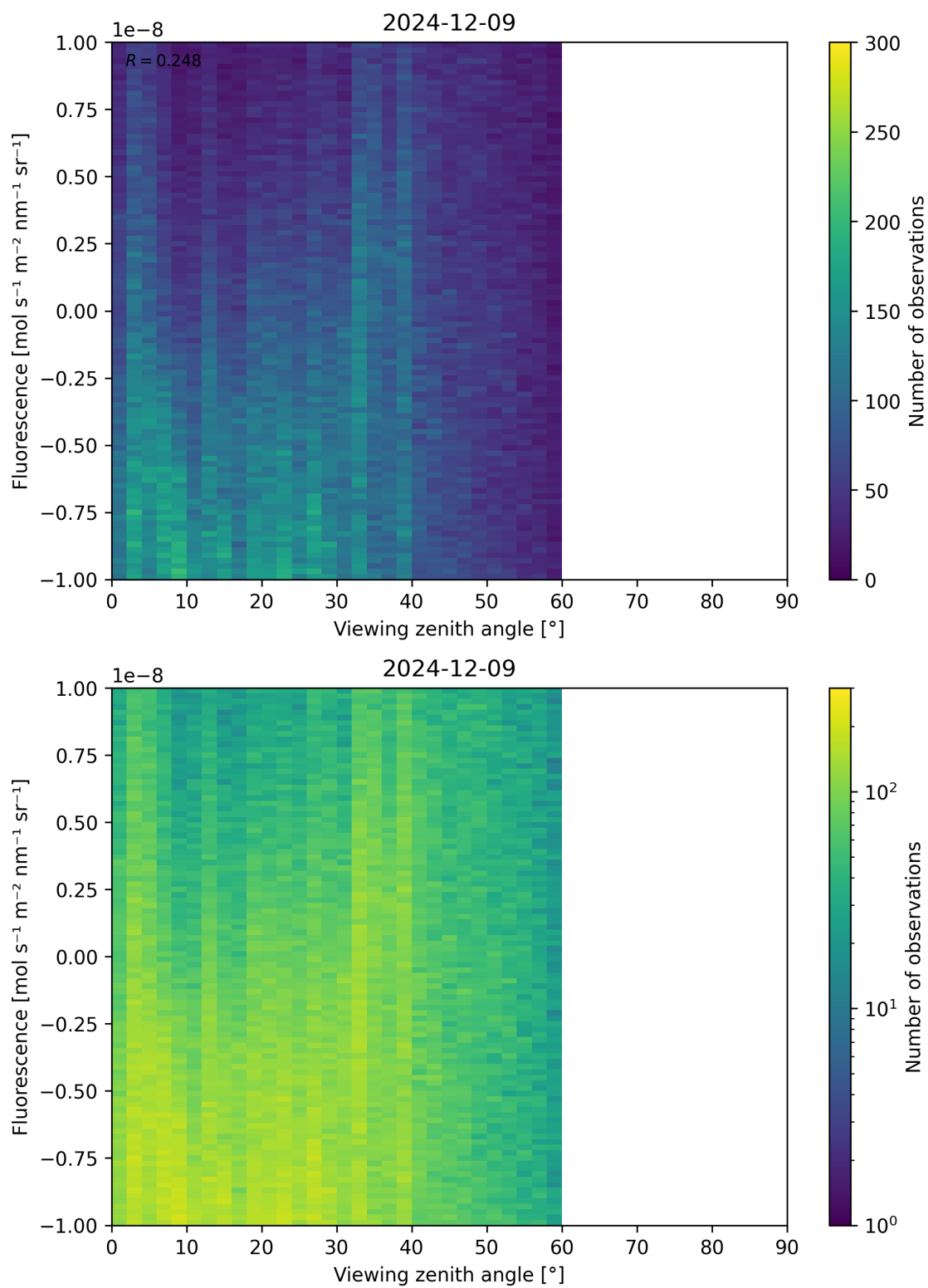
Figure 108: Scatter density plot of “Viewing zenith angle” against “Fluorescence” for 2024-12-08 to 2024-12-10.
