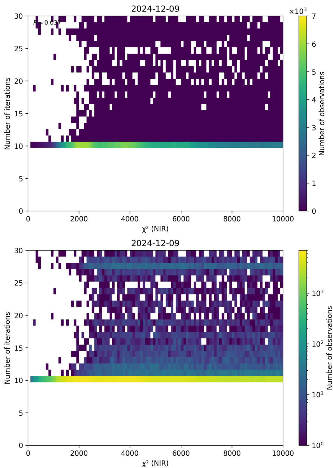
Figure 46: Scatter density plot of “ \chi^2 (NIR)” against “Number of iterations” for 2024-12-08 to 2024-12-10.
