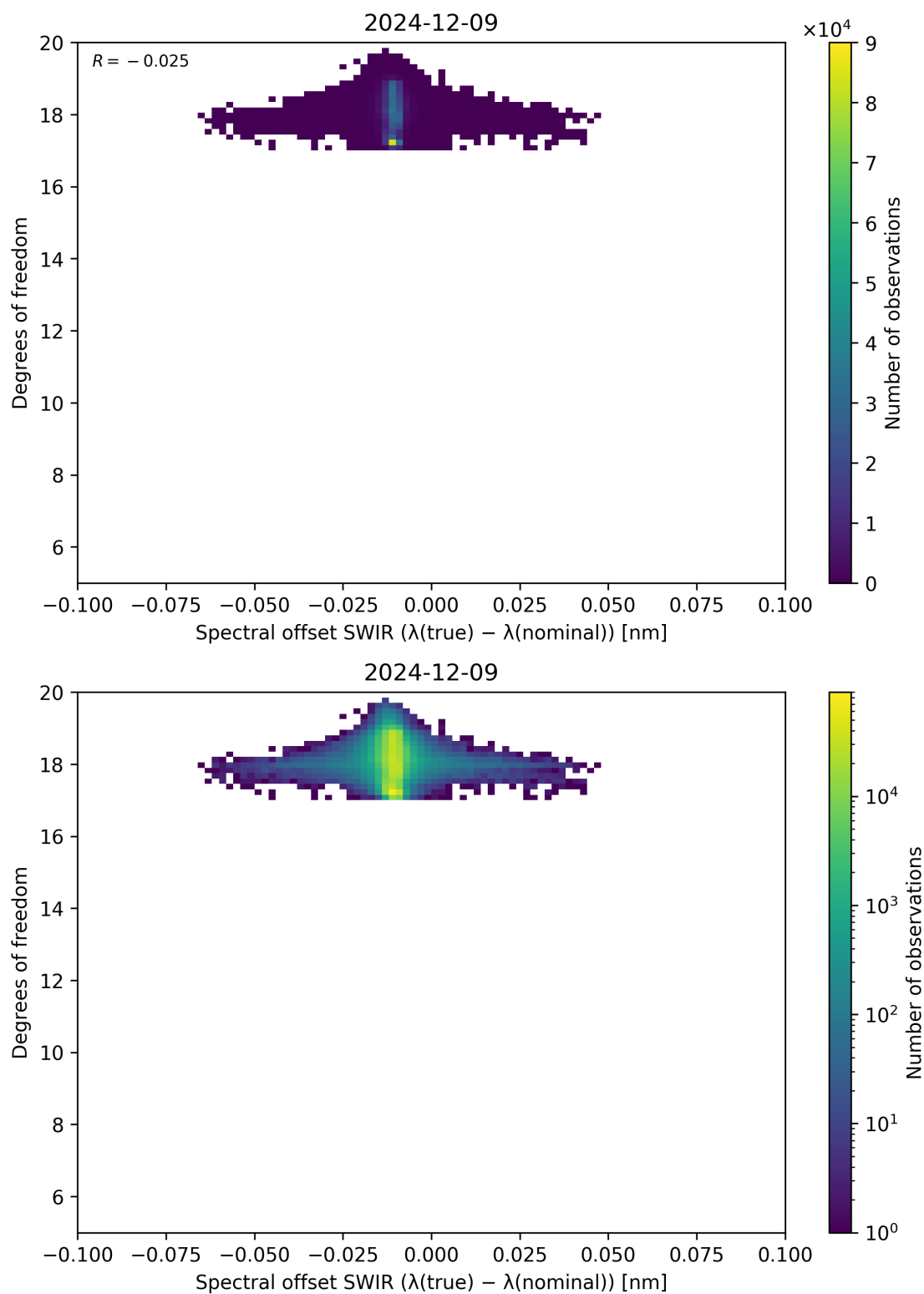
Figure 119: Scatter density plot of “Spectral offset SWIR ( \lambda_{\text{true}} - \lambda_{\text{nominal}} )” against “Degrees of freedom” for 2024-12-08 to 2024-12-10.
