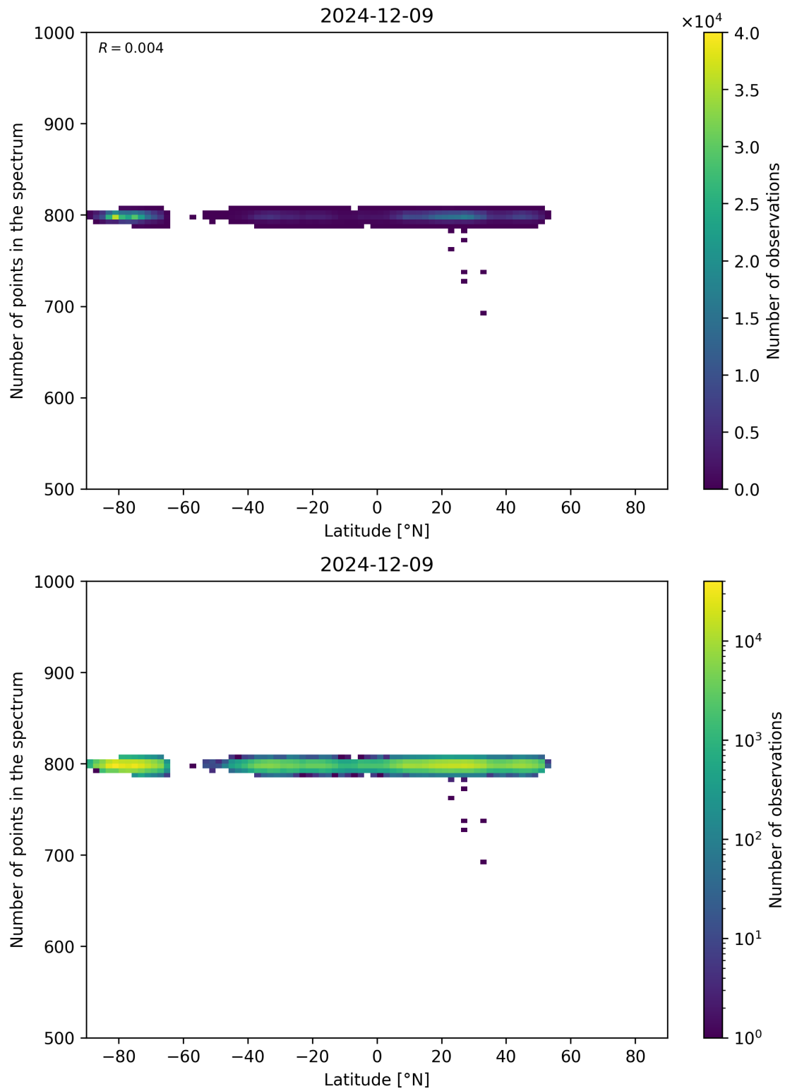
Figure 61: Scatter density plot of “Latitude” against “Number of points in the spectrum” for 2024-12-08 to 2024-12-10.
