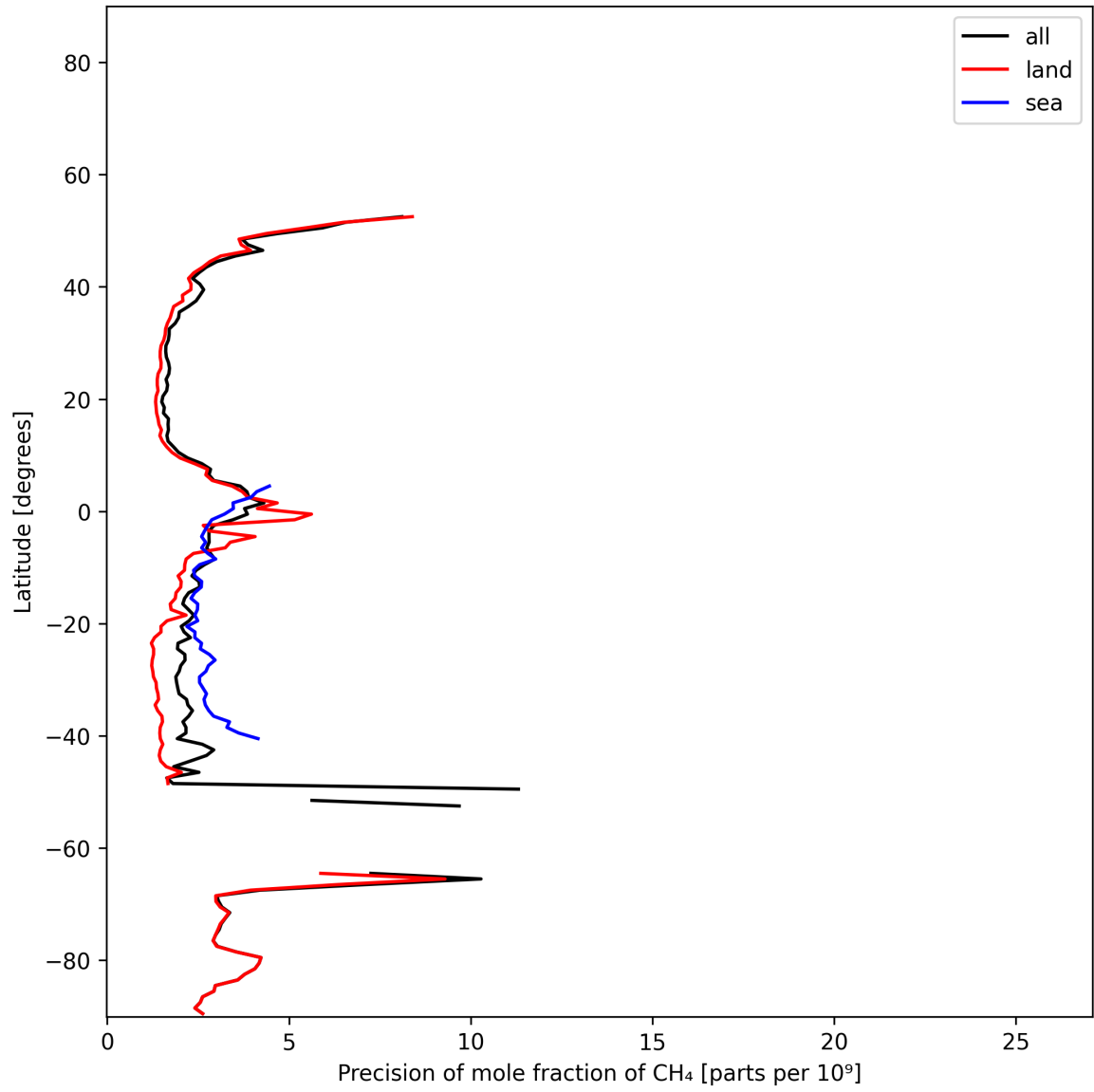
Figure 13: Zonal average of “Precision of mole fraction of CH 4 ” for 2024-12-08 to 2024-12-10.
