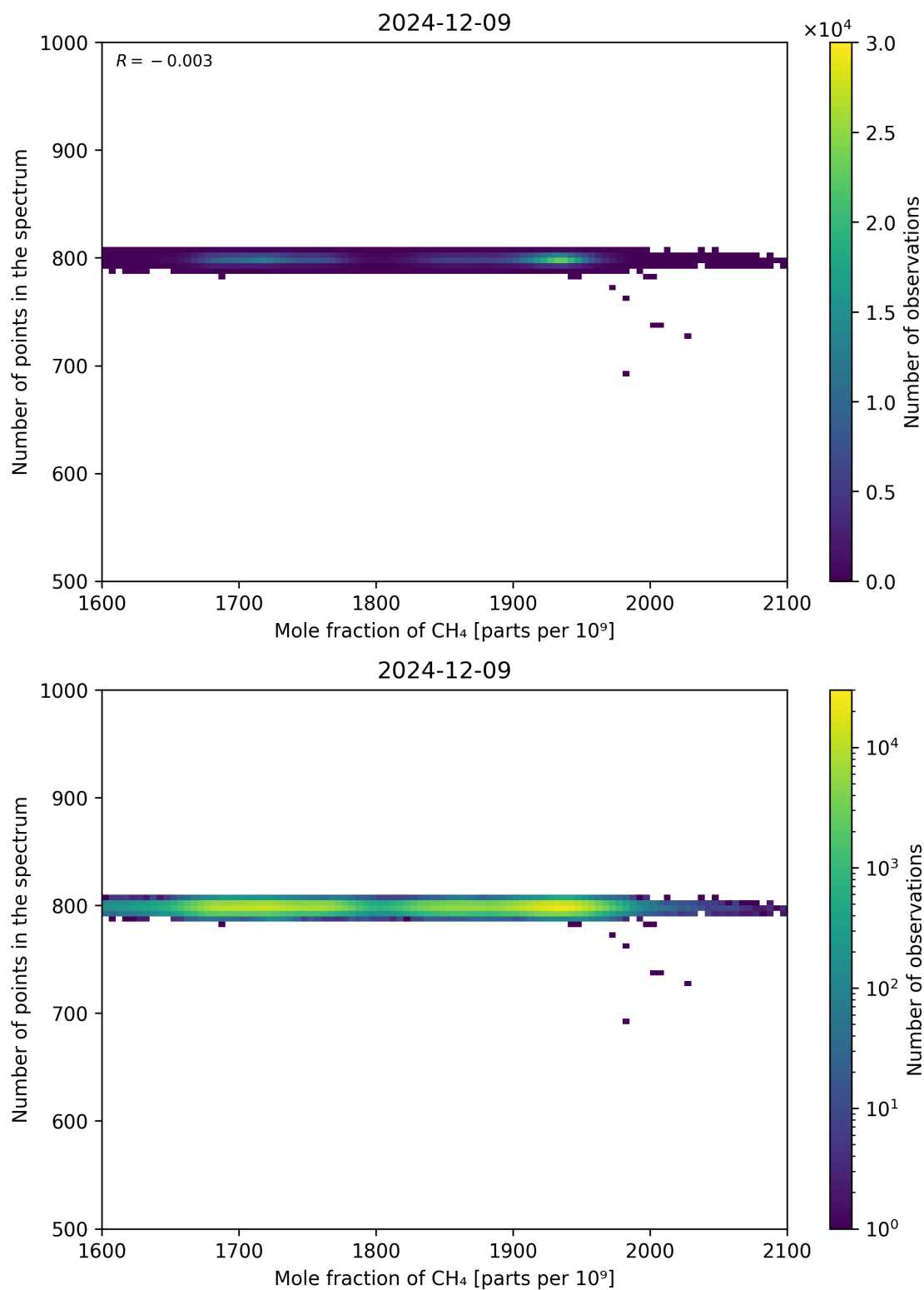
Figure 77: Scatter density plot of “Mole fraction of CH 4 ” against “Number of points in the spectrum” for 2024-12-08 to 2024-12-10.
