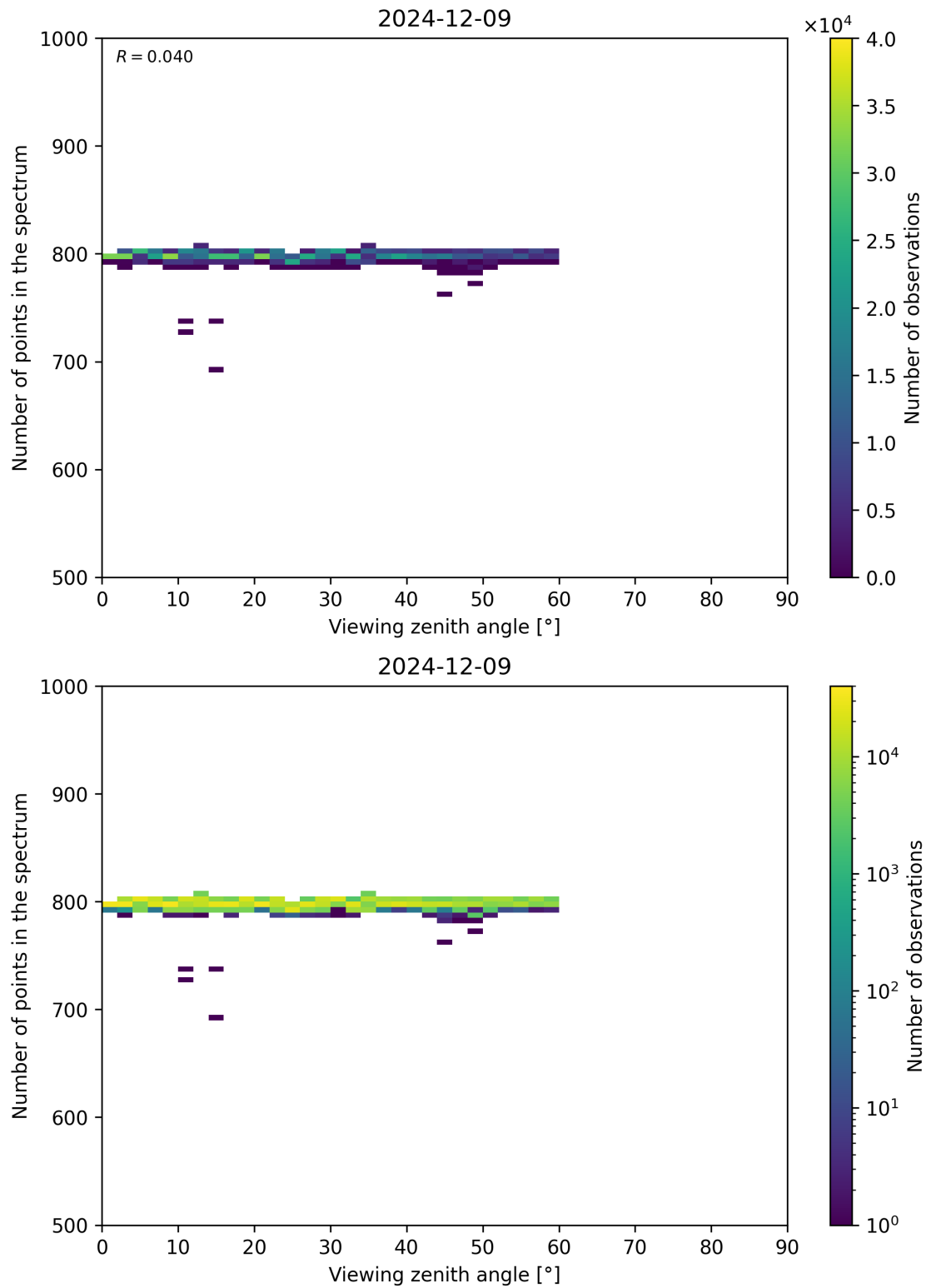
Figure 114: Scatter density plot of “Viewing zenith angle” against “Number of points in the spectrum” for 2024-12-08 to 2024-12-10.
