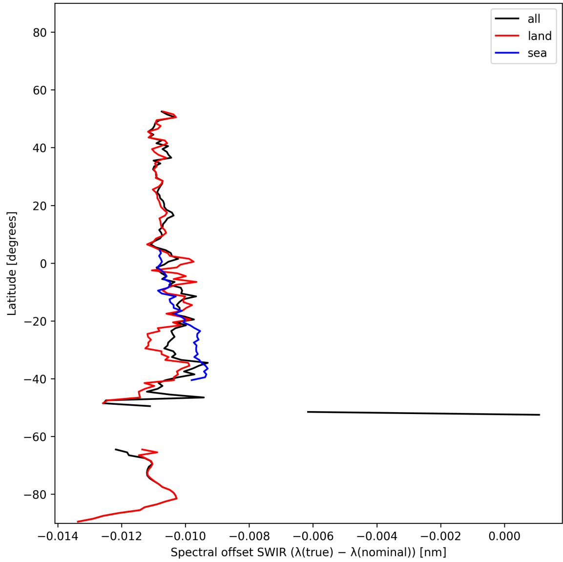
Figure 16: Zonal average of “Spectral offset SWIR ( \lambda_{\text{true}} - \lambda_{\text{nominal}} )” for 2024-12-08 to 2024-12-10.
