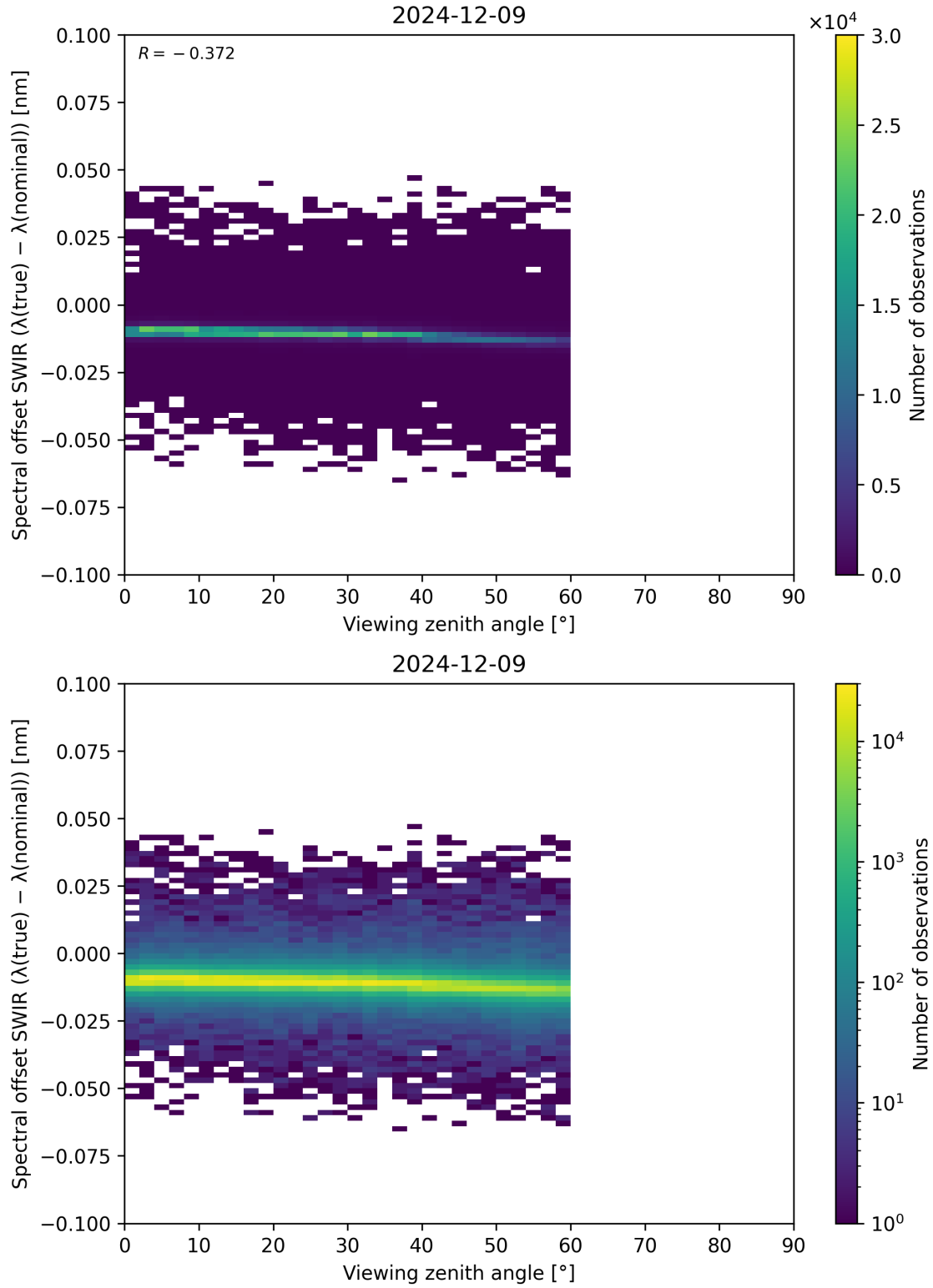
Figure 116: Scatter density plot of “Viewing zenith angle” against “Spectral offset SWIR ( \lambda_{\text{true}} - \lambda_{\text{nominal}} )” for 2024-12-08 to 2024-12-10.
