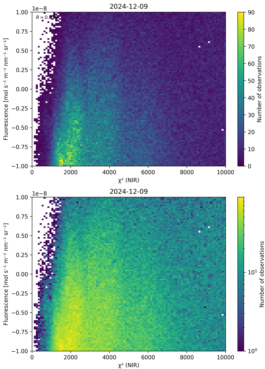
Figure 45: Scatter density plot of “ \chi^2 (NIR)” against “Fluorescence” for 2024-12-08 to 2024-12-10.
