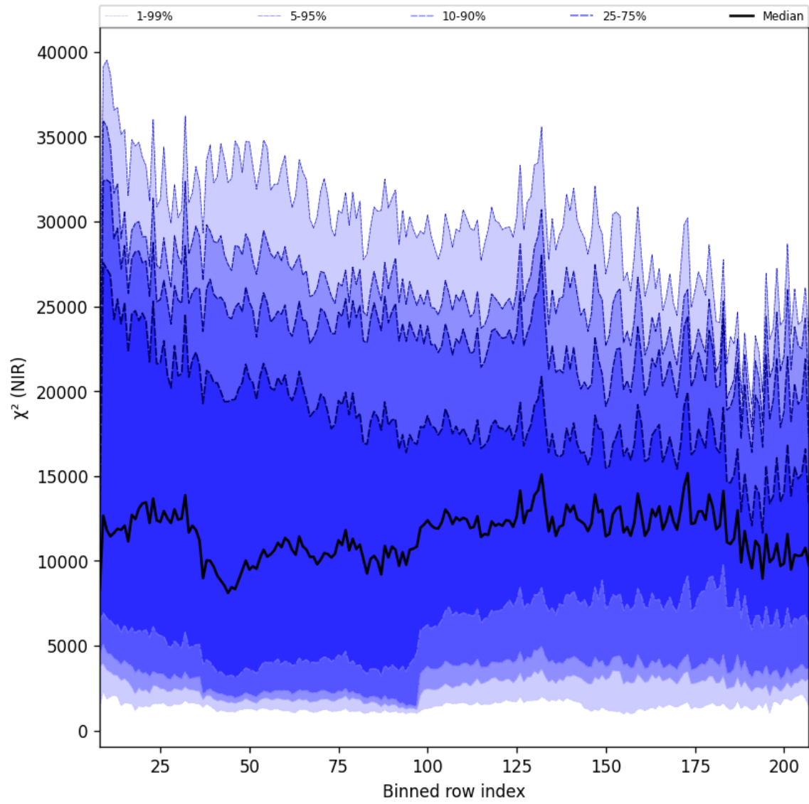
Figure 40: Along track statistics of “ \chi^2 (NIR)” for 2024-12-08 to 2024-12-10
