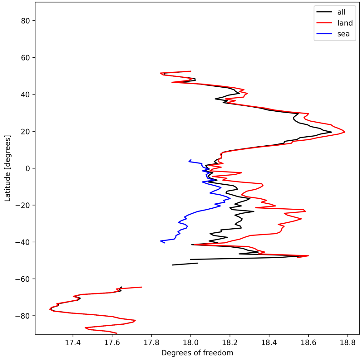
Figure 19: Zonal average of “Degrees of freedom” for 2024-12-08 to 2024-12-10.
