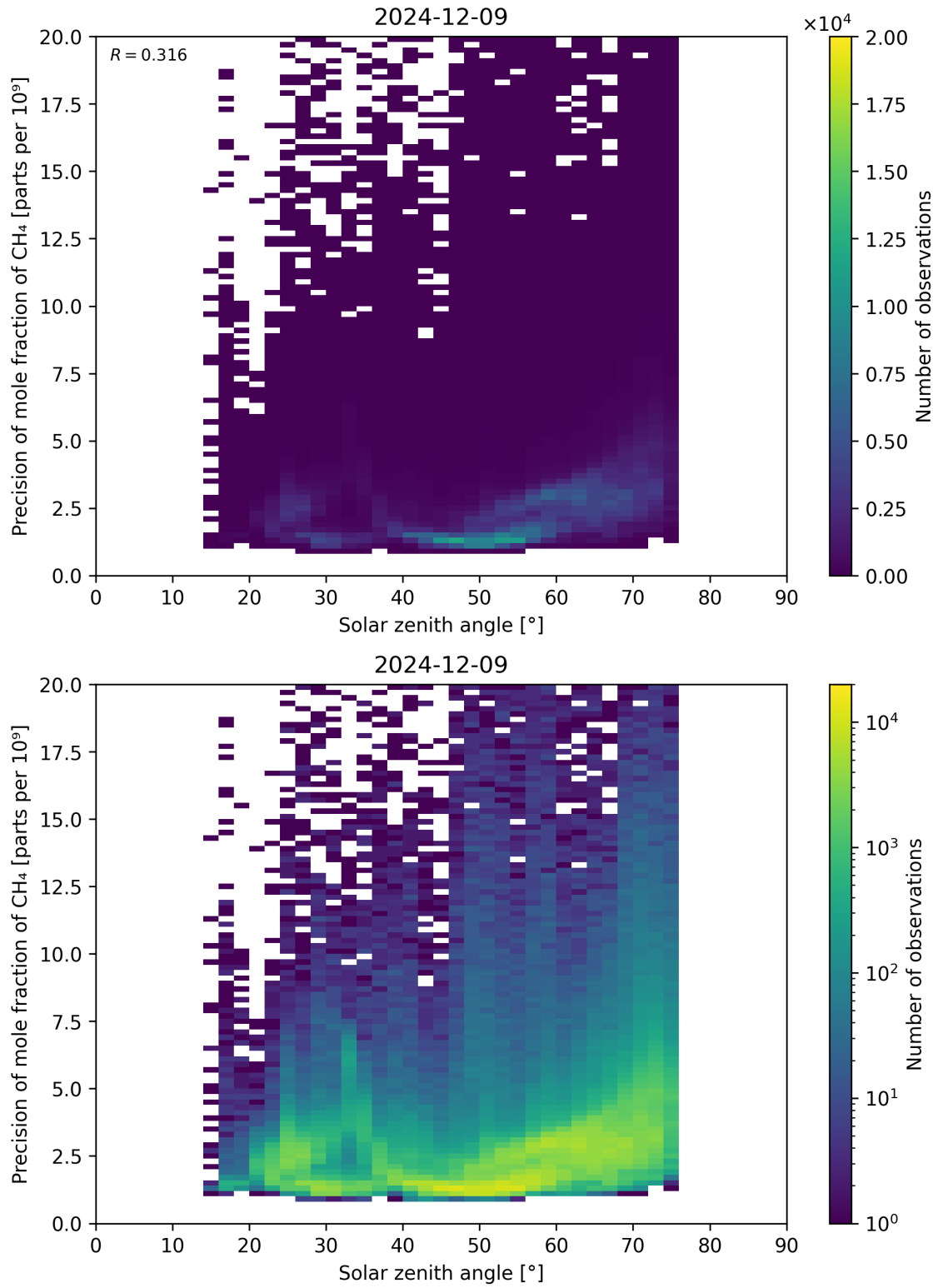
Figure 101: Scatter density plot of “Solar zenith angle” against “Precision of mole fraction of CH 4 ” for 2024-12-08 to 2024-12-10.
