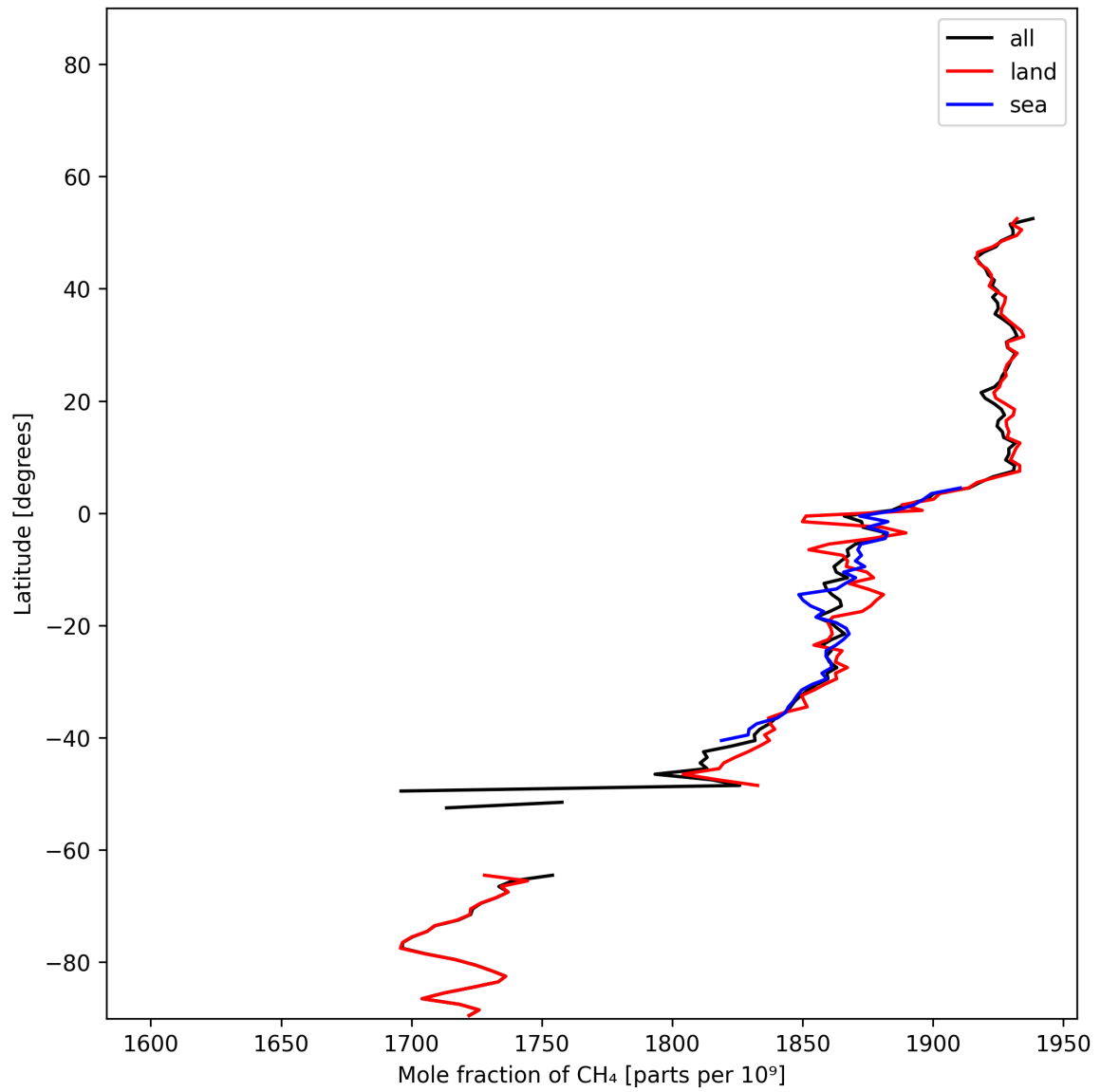
Figure 12: Zonal average of “Mole fraction of CH 4 ” for 2024-12-08 to 2024-12-10.
