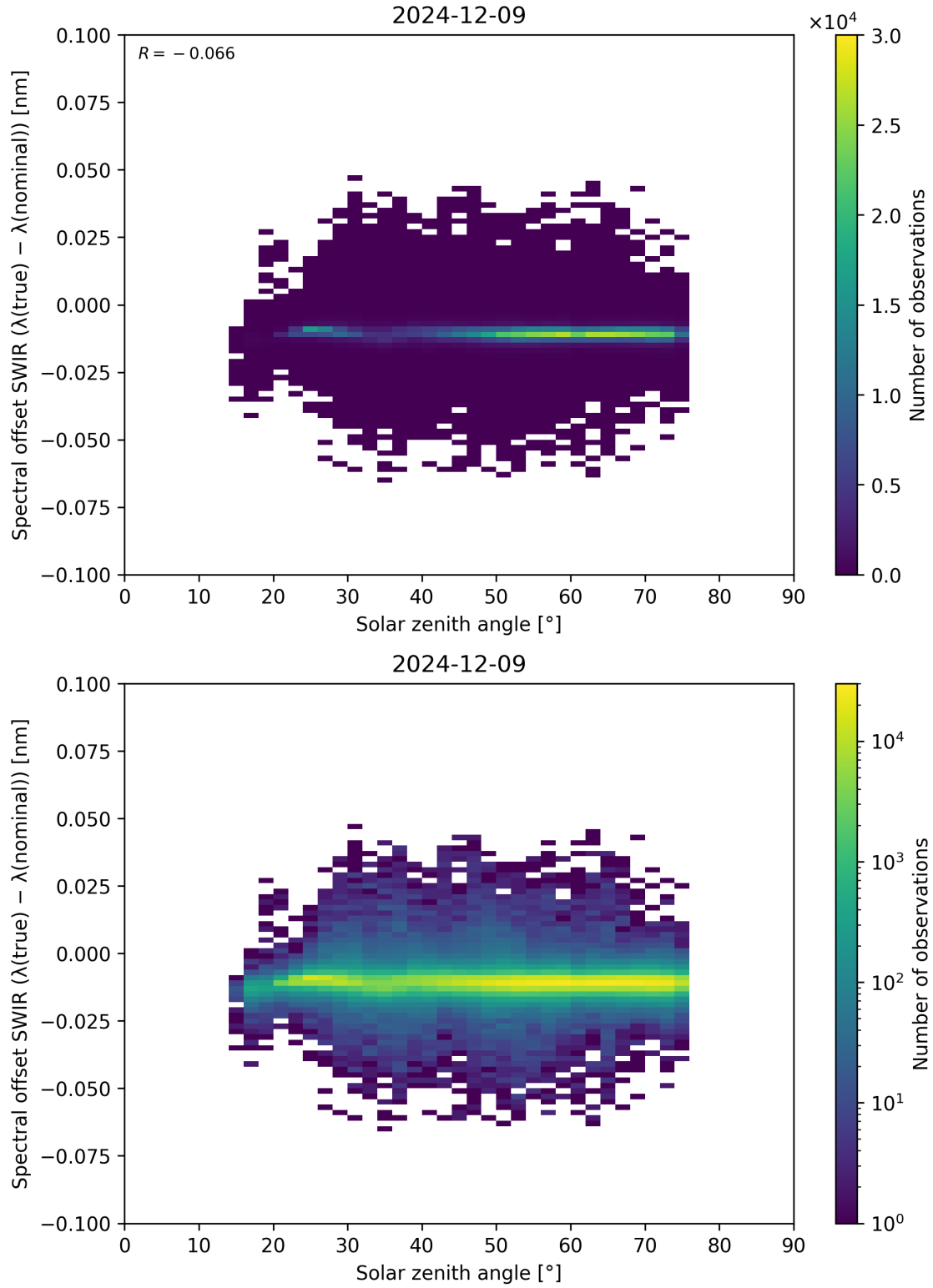
Figure 104: Scatter density plot of “Solar zenith angle” against “Spectral offset SWIR ( \lambda_{\text{true}} - \lambda_{\text{nominal}} )” for 2024-12-08 to 2024-12-10.
