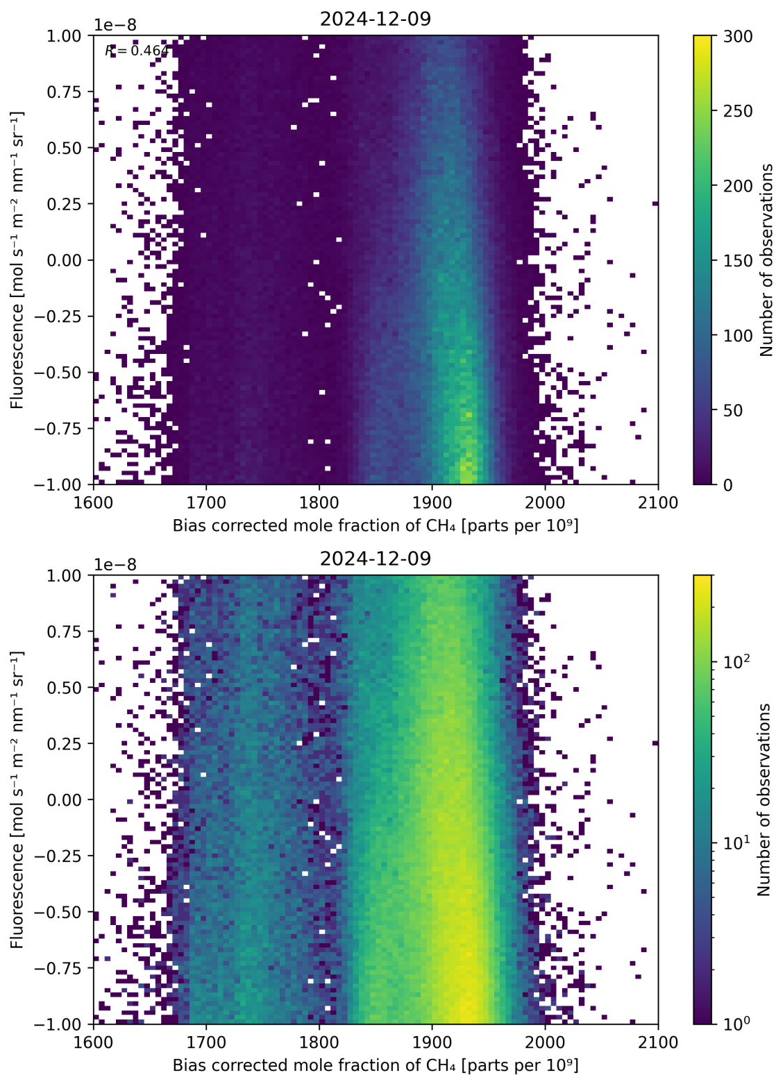
Figure 66: Scatter density plot of “Bias corrected mole fraction of \text{CH}_4 ” against “Fluorescence” for 2024-12-08 to 2024-12-10.
