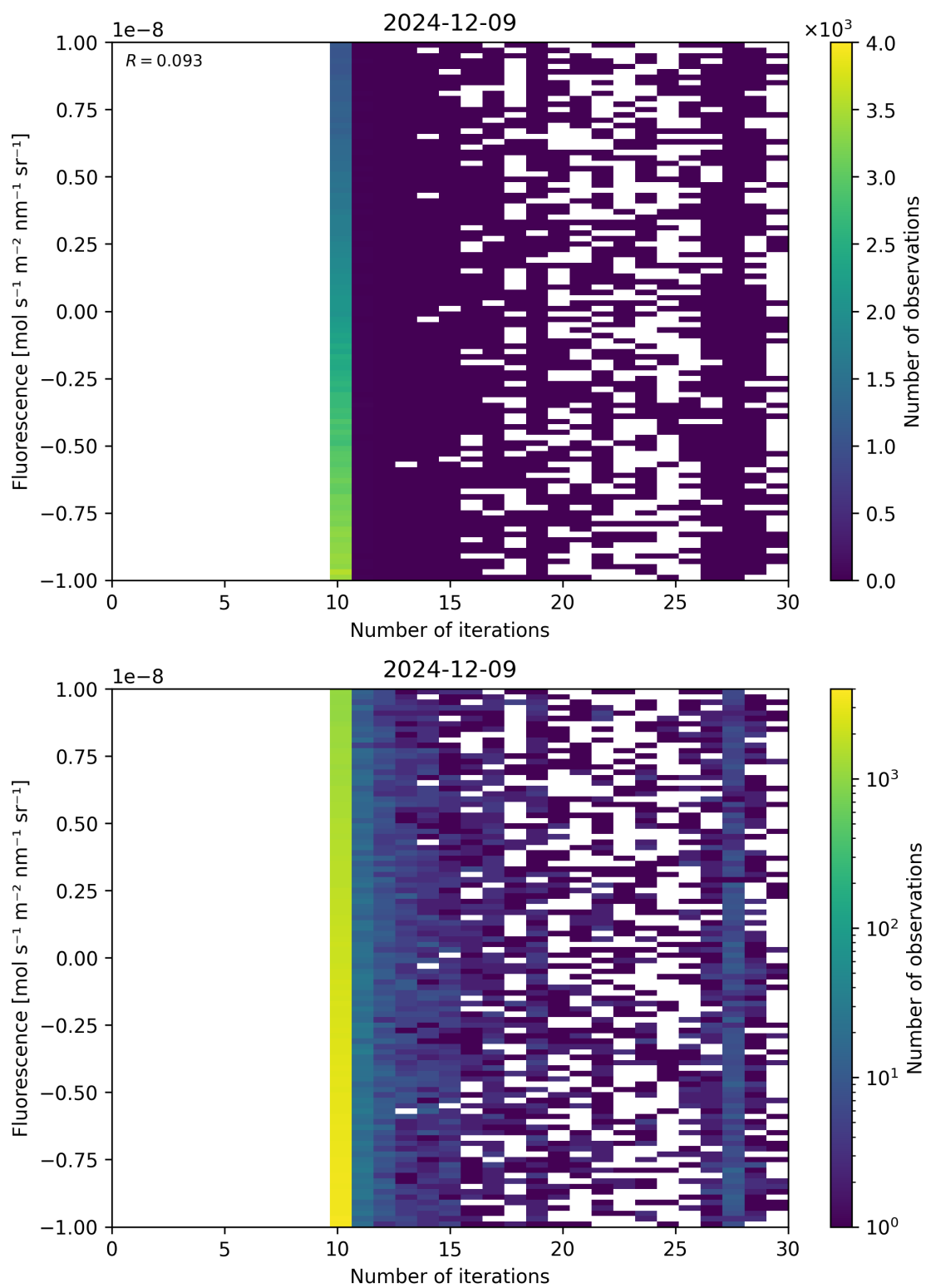
Figure 87: Scatter density plot of “Number of iterations” against “Fluorescence” for 2024-12-08 to 2024-12-10.
