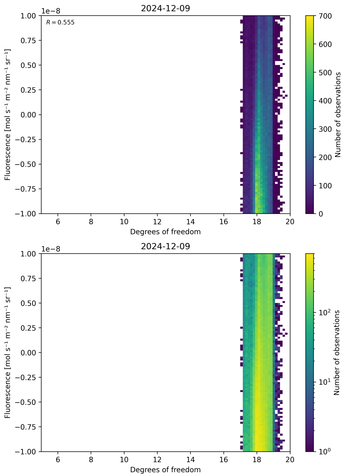
Figure 51: Scatter density plot of “Degrees of freedom” against “Fluorescence” for 2024-12-08 to 2024-12-10.
