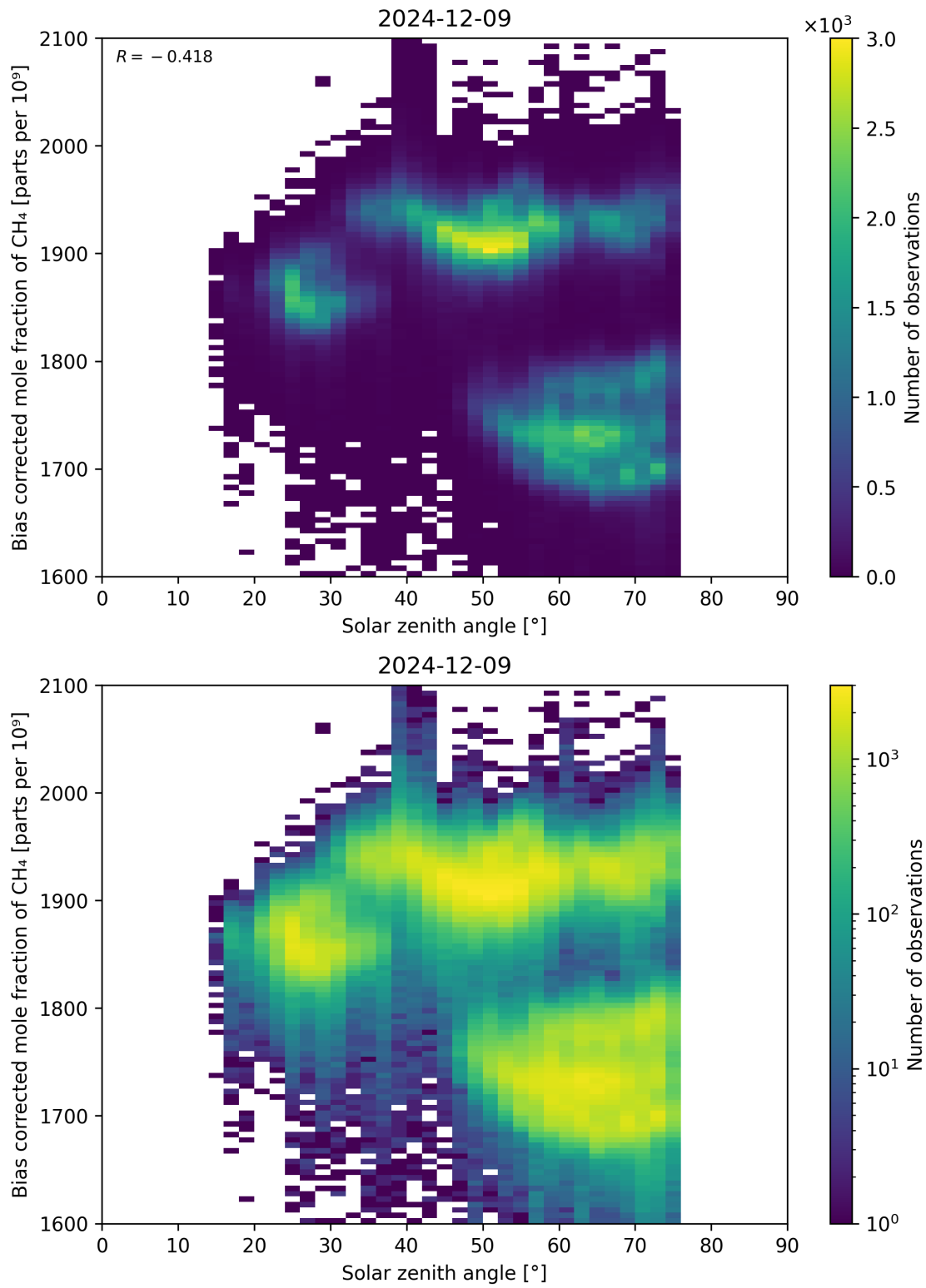
Figure 100: Scatter density plot of “Solar zenith angle” against “Bias corrected mole fraction of \text{CH}_4 ” for 2024-12-08 to 2024-12-10.
