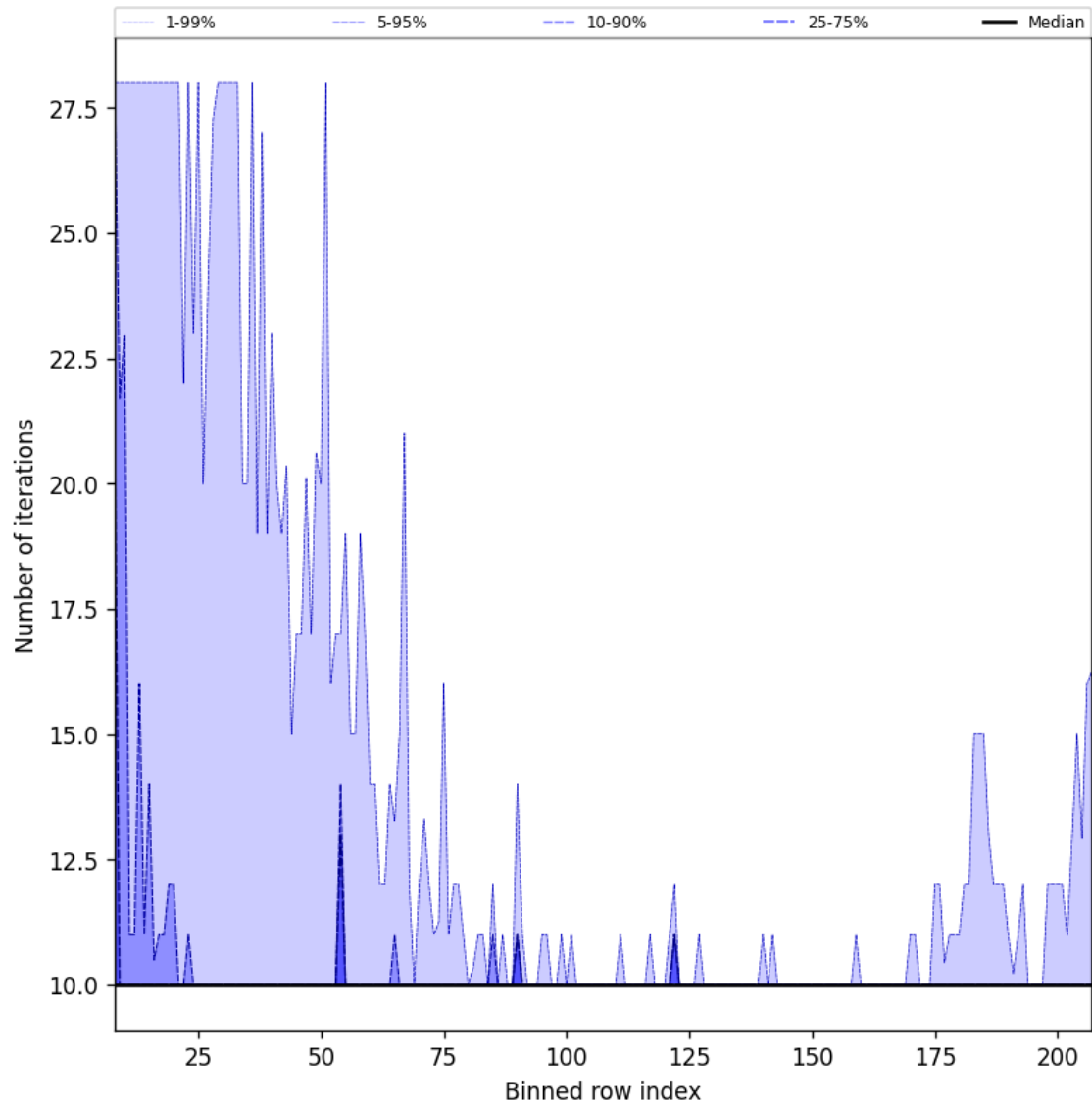
Figure 42: Along track statistics of “Number of iterations” for 2024-12-08 to 2024-12-10
