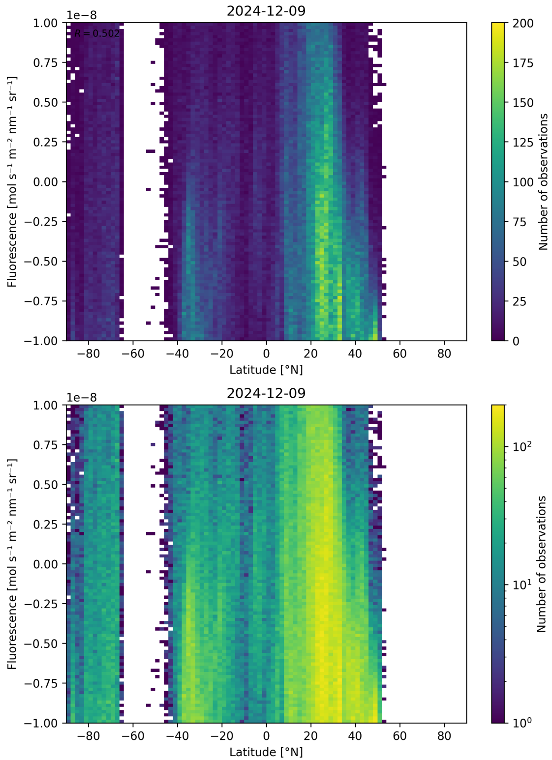
Figure 56: Scatter density plot of “Latitude” against “Fluorescence” for 2024-12-08 to 2024-12-10.
