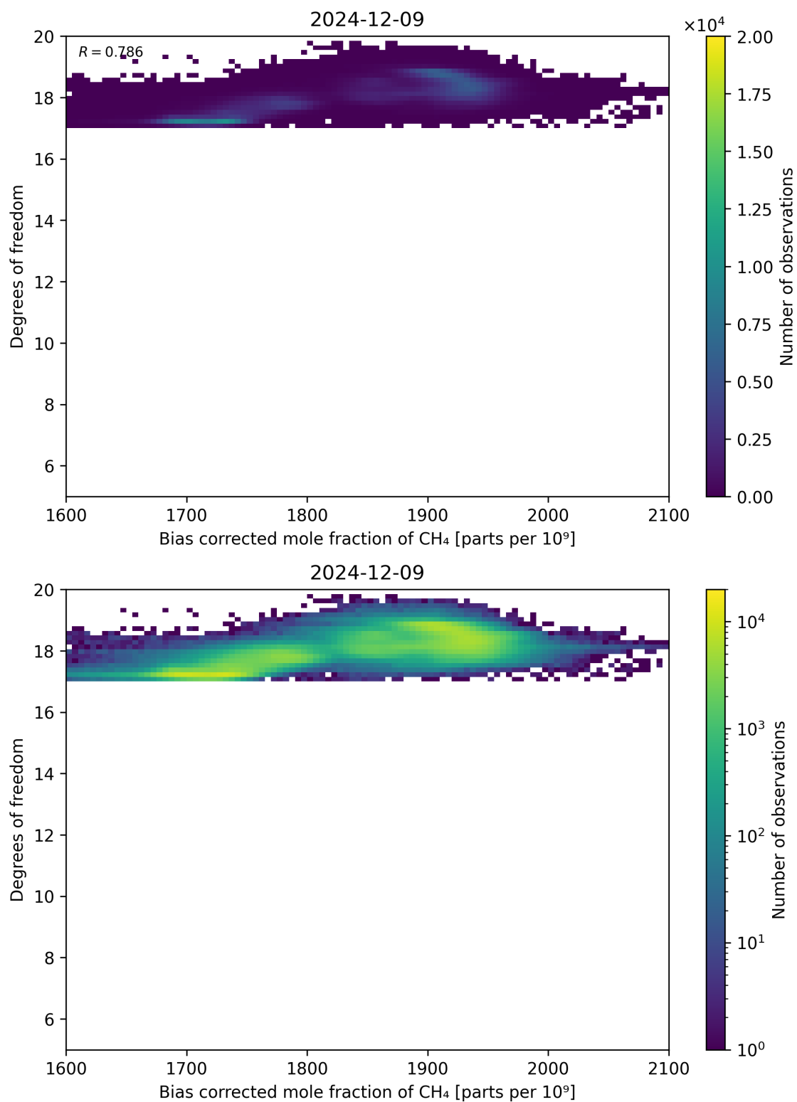
Figure 65: Scatter density plot of “Bias corrected mole fraction of CH 4 ” against “Degrees of freedom” for 2024-12-08 to 2024-12-10.
