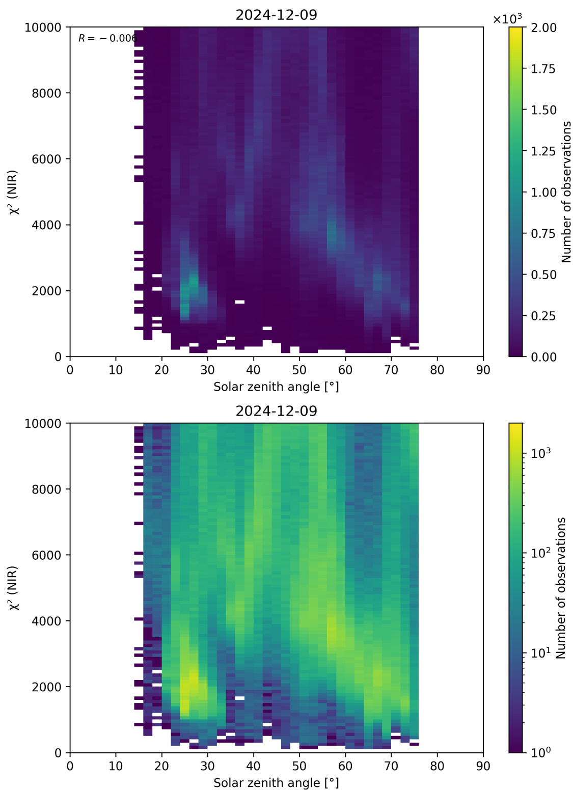
Figure 94: Scatter density plot of “Solar zenith angle” against “ \chi^2 (NIR)” for 2024-12-08 to 2024-12-10.
