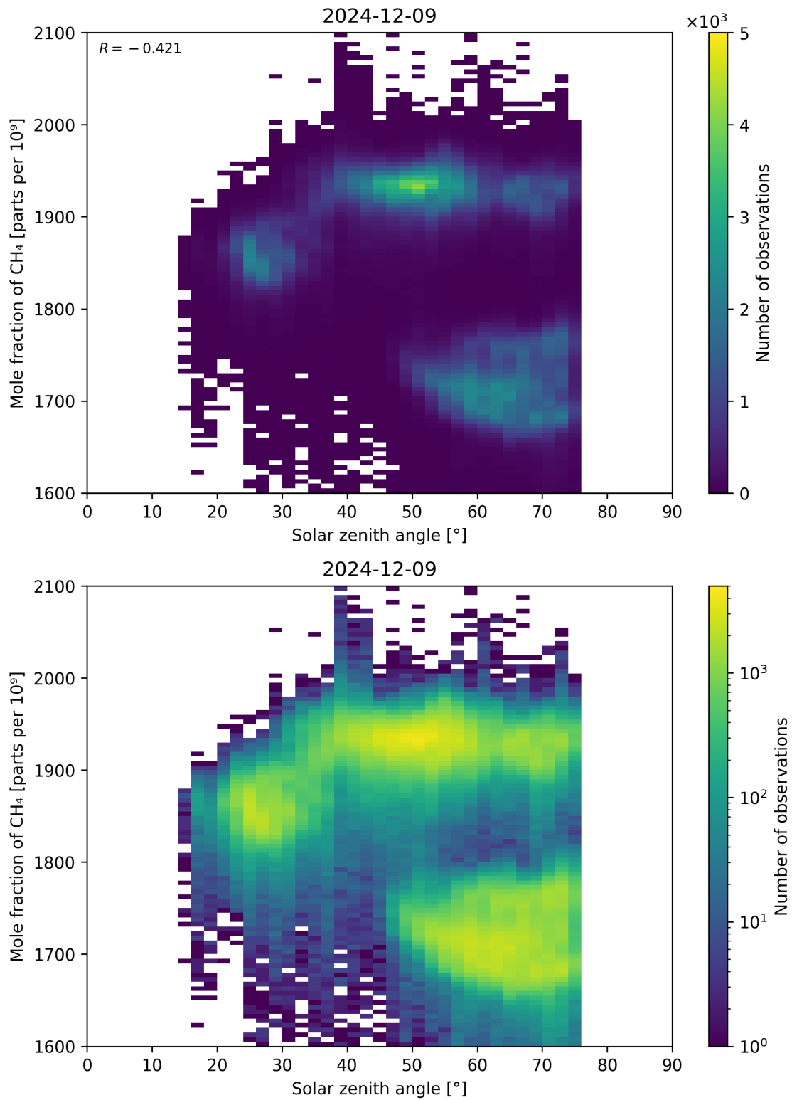
Figure 99: Scatter density plot of “Solar zenith angle” against “Mole fraction of CH 4 ” for 2024-12-08 to 2024-12-10.
