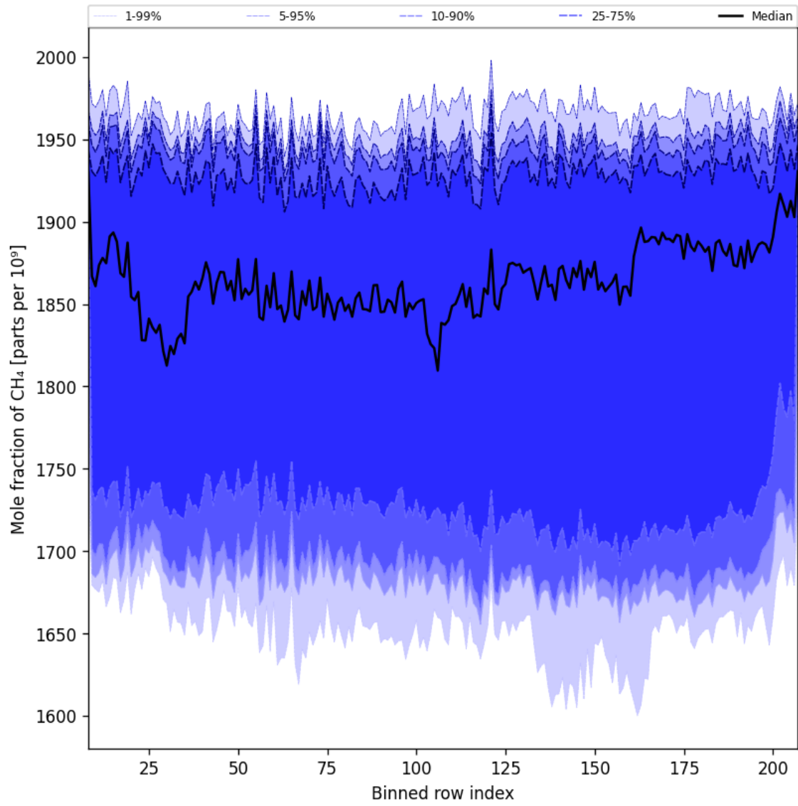
Figure 34: Along track statistics of “Mole fraction of CH 4 ” for 2024-12-08 to 2024-12-10
