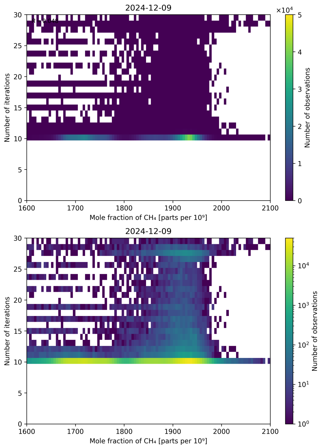
Figure 76: Scatter density plot of “Mole fraction of CH 4 ” against “Number of iterations” for 2024-12-08 to 2024-12-10.
