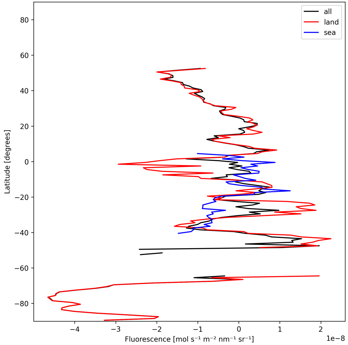
Figure 21: Zonal average of “Fluorescence” for 2024-12-08 to 2024-12-10.
