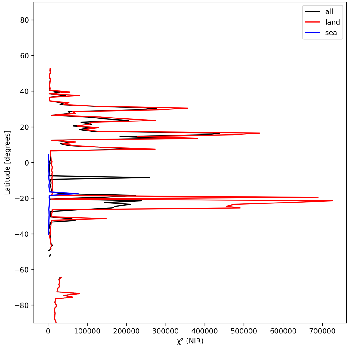
Figure 18: Zonal average of “ \chi^2 (NIR)” for 2024-12-08 to 2024-12-10.
