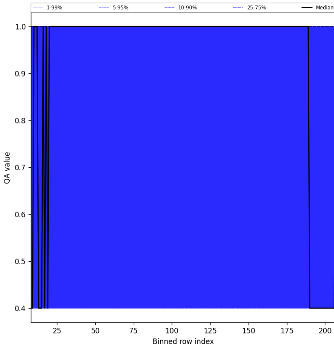
Figure 33: Along track statistics of “QA value” for 2024-12-08 to 2024-12-10
