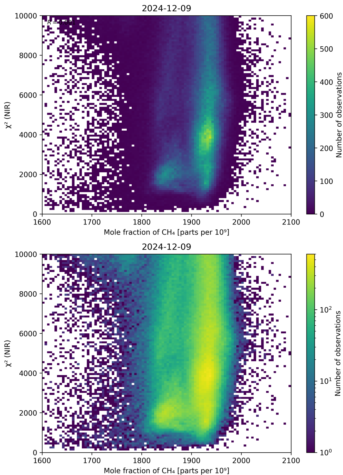
Figure 70: Scatter density plot of “Mole fraction of \text{CH}_4 ” against “ \chi^2 (NIR)” for 2024-12-08 to 2024-12-10.
