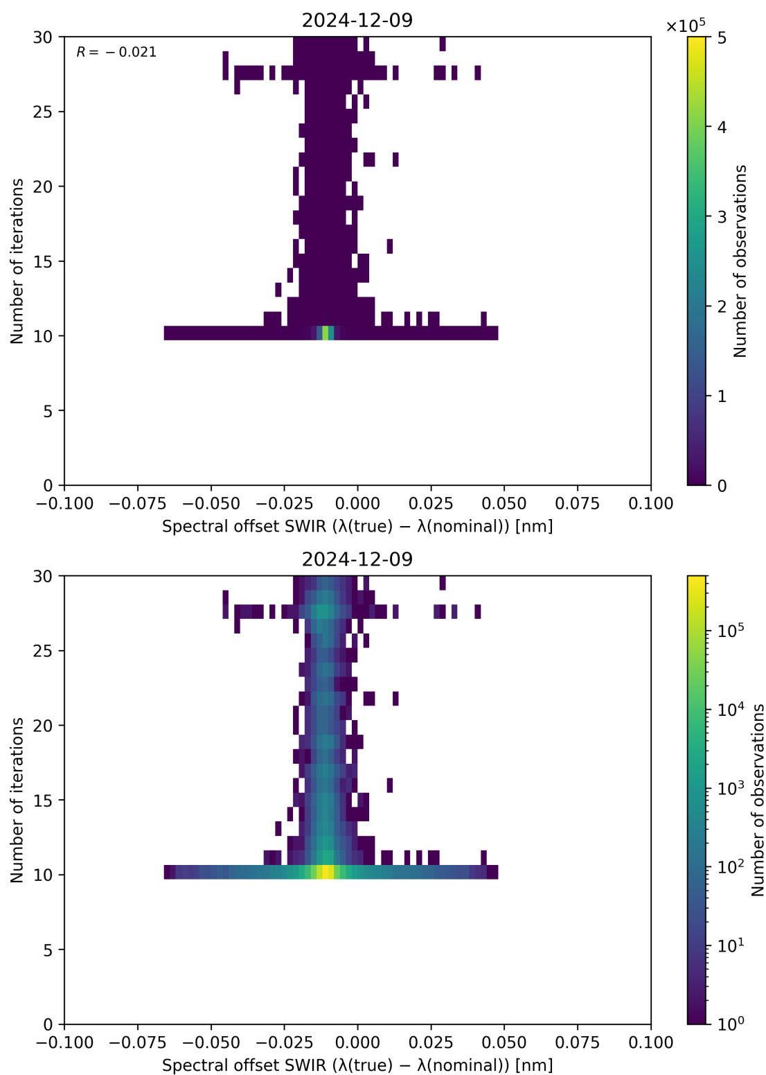
Figure 121: Scatter density plot of “Spectral offset SWIR ( \lambda_{\text{true}} - \lambda_{\text{nominal}} )” against “Number of iterations” for 2024-12-08 to 2024-12-10.
