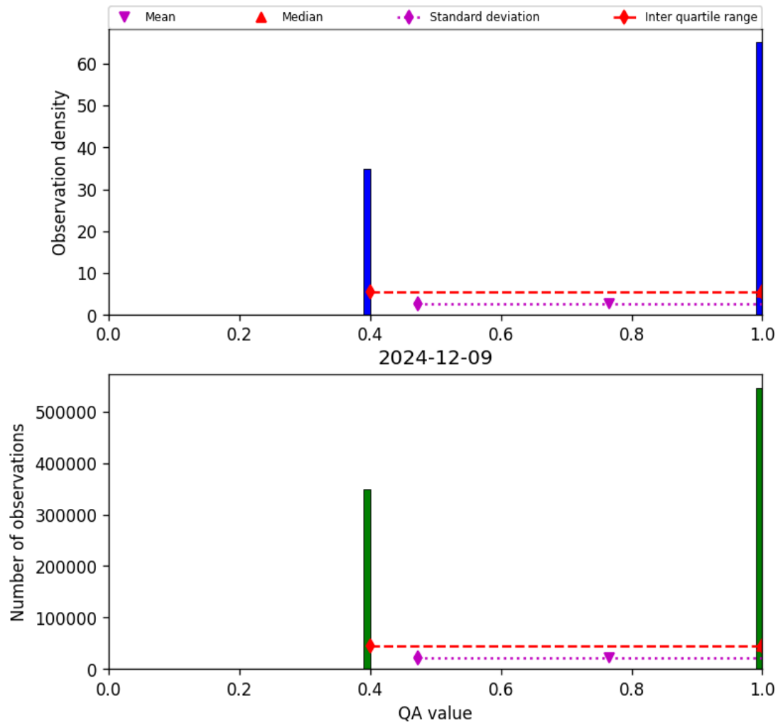
Figure 22: Histogram of “QA value” for 2024-12-08 to 2024-12-10
