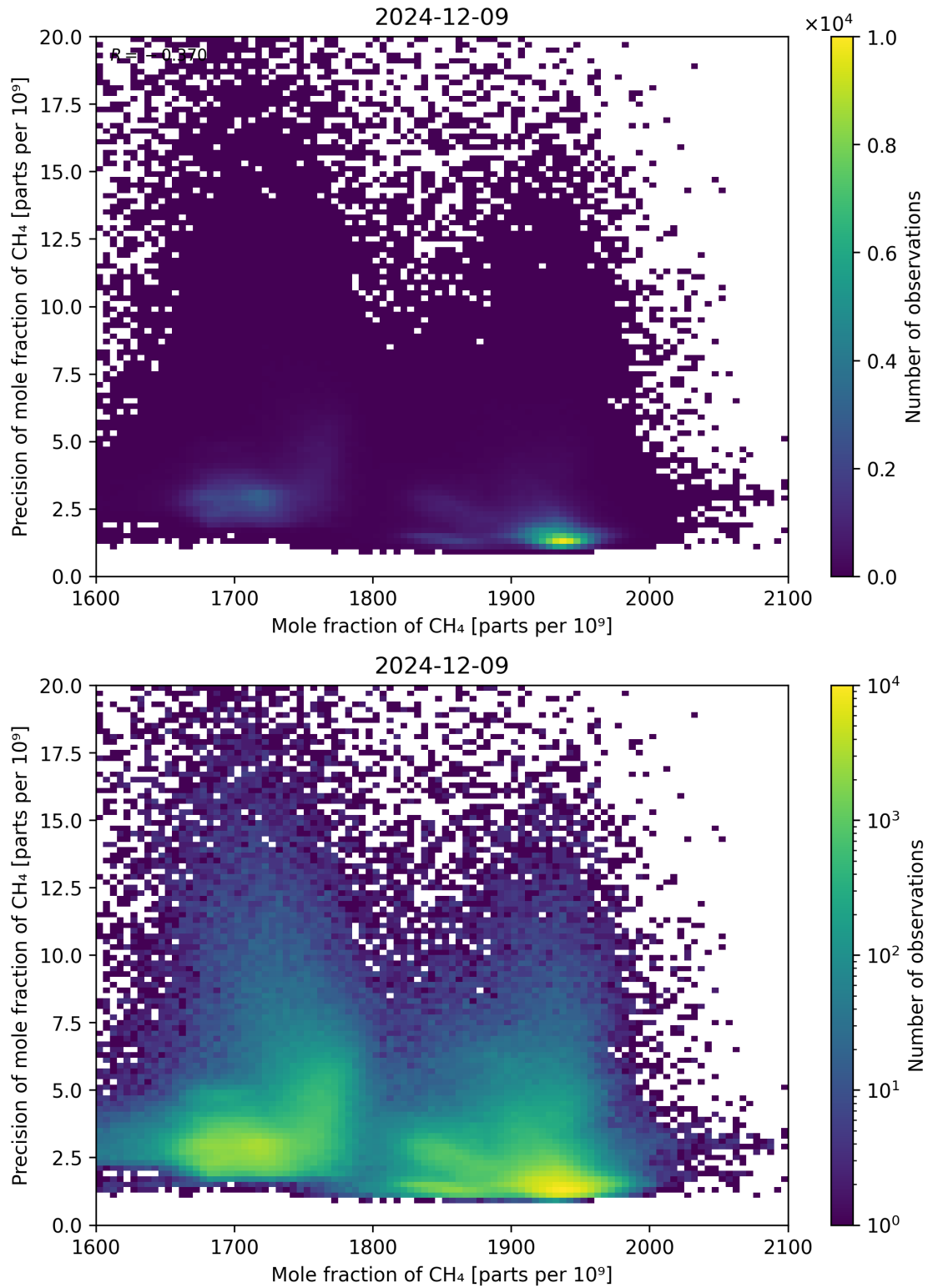
Figure 75: Scatter density plot of “Mole fraction of CH 4 ” against “Precision of mole fraction of CH 4 ” for 2024-12-08 to 2024-12-10.
