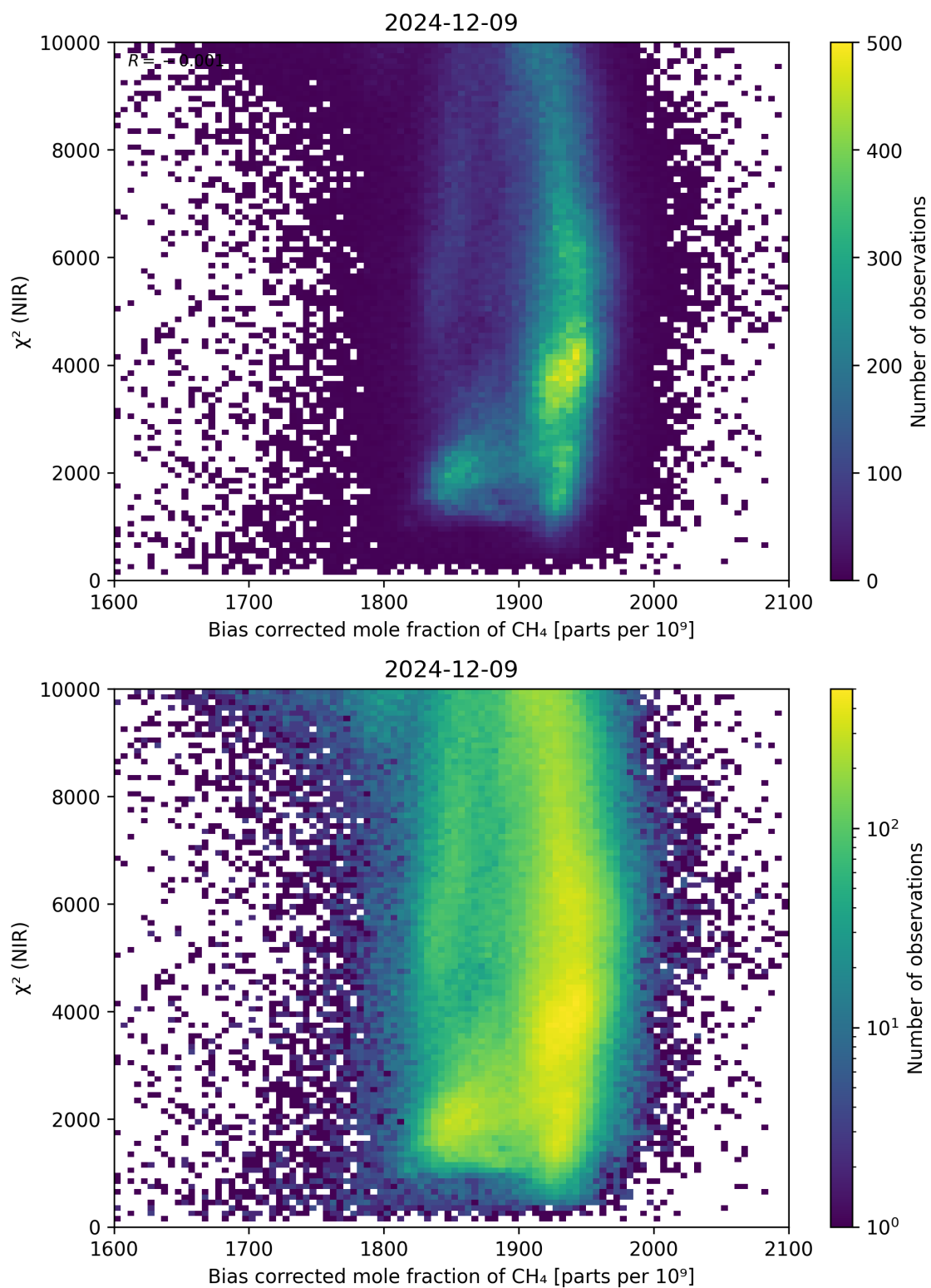
Figure 63: Scatter density plot of “Bias corrected mole fraction of \text{CH}_4 ” against “ \chi^2 (NIR)” for 2024-12-08 to 2024-12-10.
