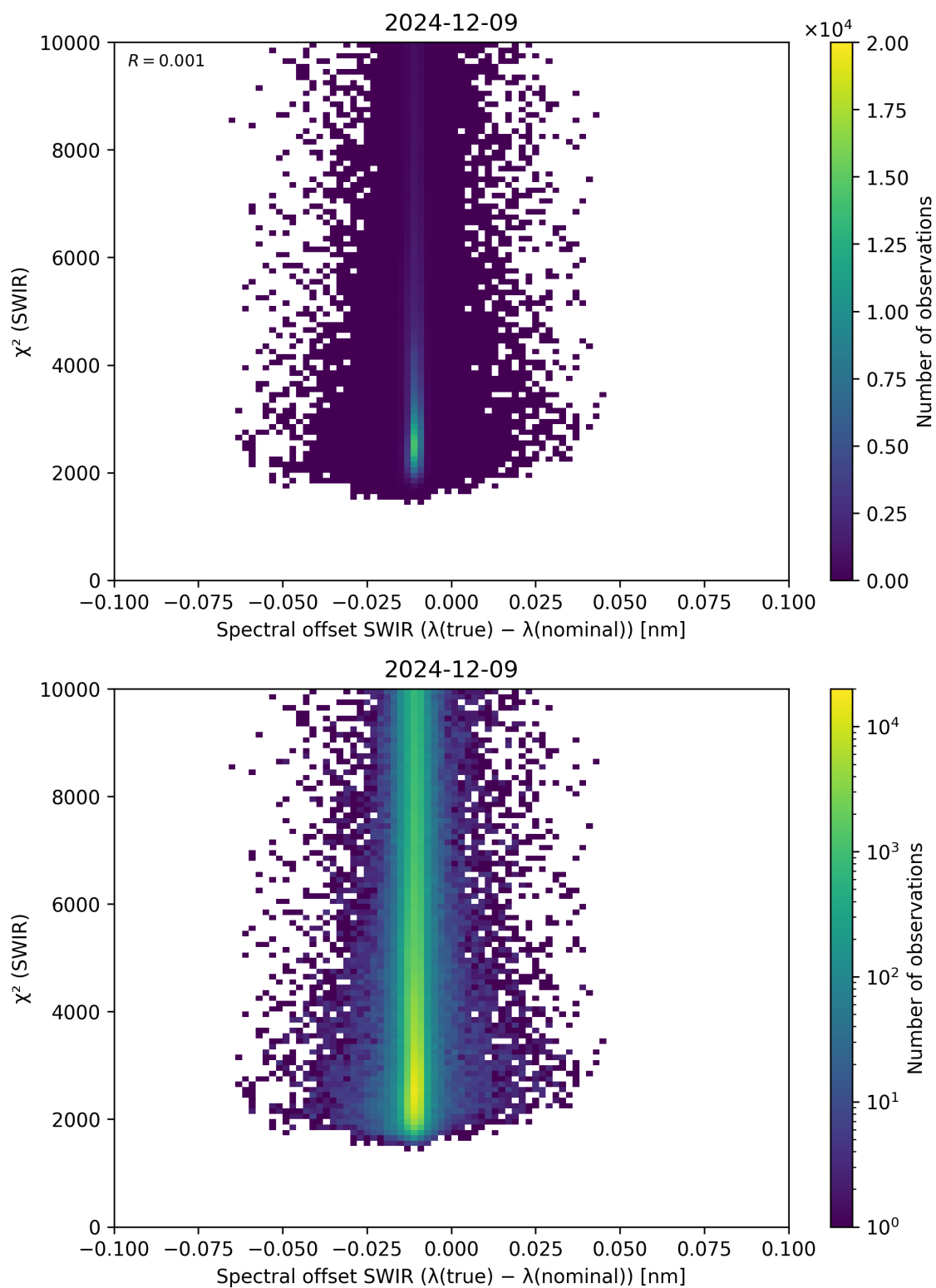
Figure 118: Scatter density plot of “Spectral offset SWIR ( \lambda_{\text{true}} - \lambda_{\text{nominal}} )” against “ \chi^2 (SWIR)” for 2024-12-08 to 2024-12-10.
