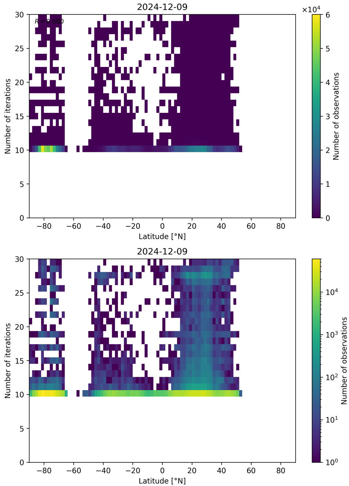
Figure 60: Scatter density plot of “Latitude” against “Number of iterations” for 2024-12-08 to 2024-12-10.
