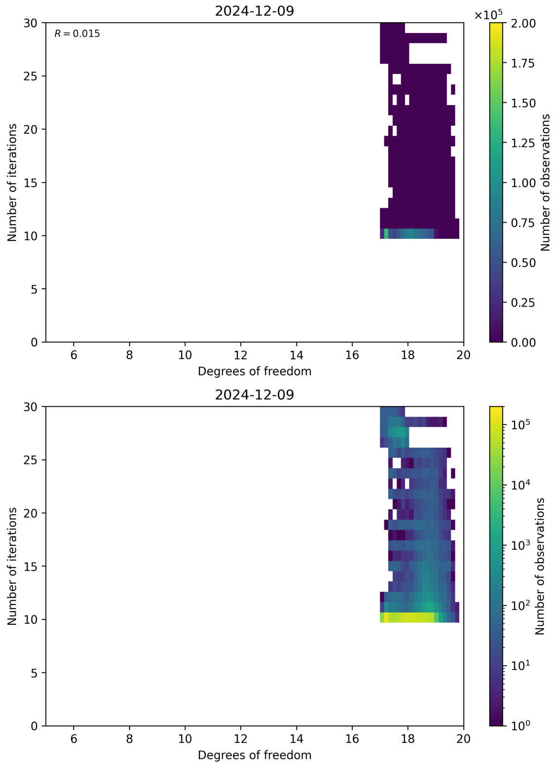
Figure 52: Scatter density plot of “Degrees of freedom” against “Number of iterations” for 2024-12-08 to 2024-12-10.
