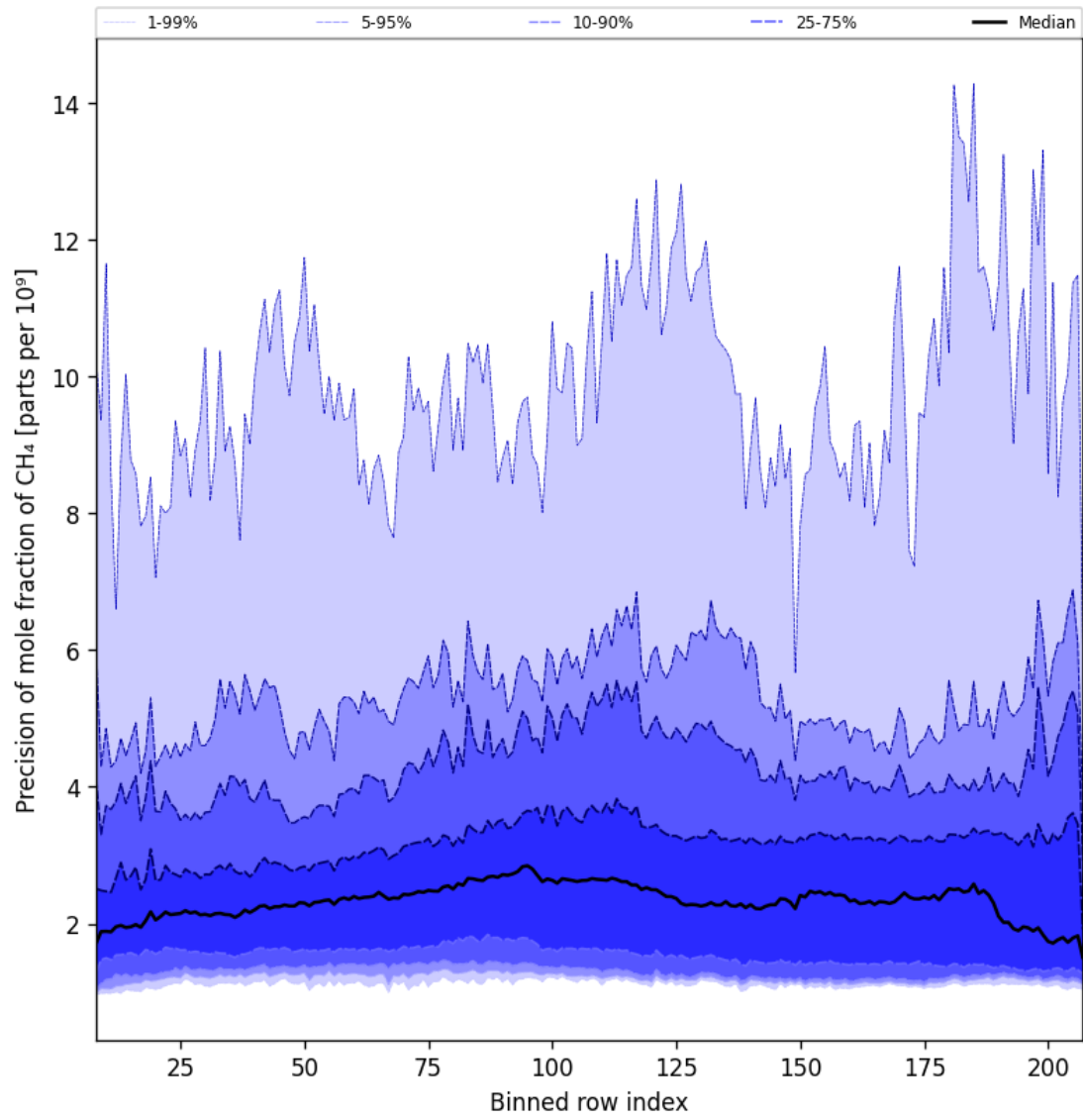
Figure 35: Along track statistics of “Precision of mole fraction of CH 4 ” for 2024-12-08 to 2024-12-10
