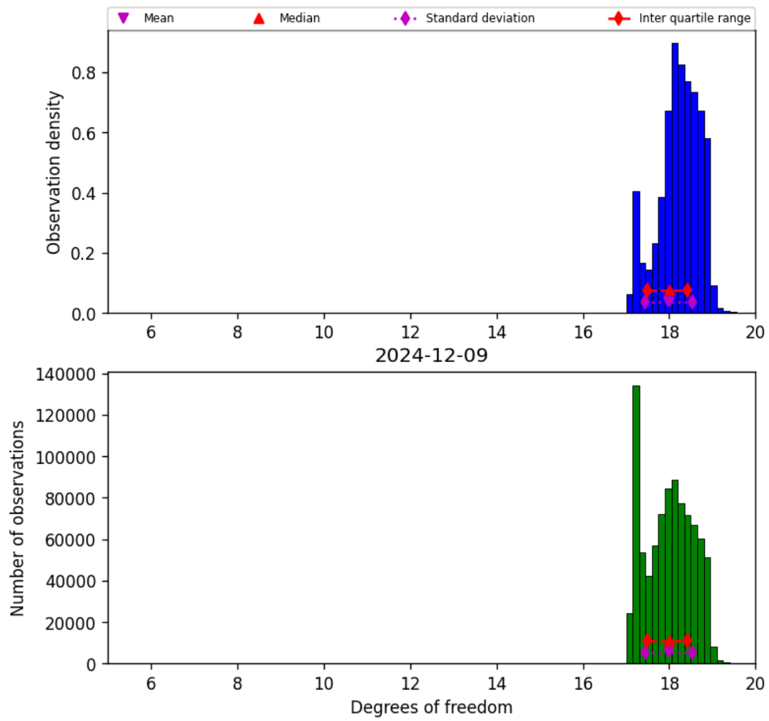
Figure 30: Histogram of “Degrees of freedom” for 2024-12-08 to 2024-12-10
