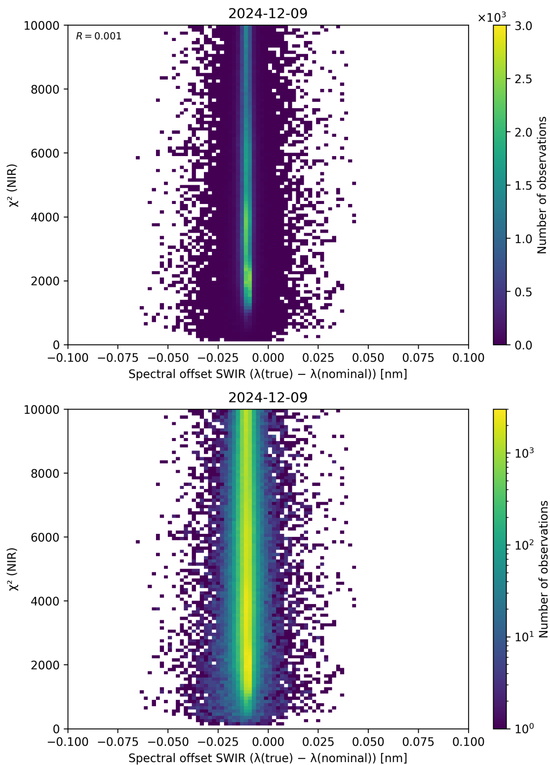
Figure 117: Scatter density plot of “Spectral offset SWIR ( \lambda_{\text{true}} - \lambda_{\text{nominal}} )” against “ \chi^2 (NIR)” for 2024-12-08 to 2024-12-10.
