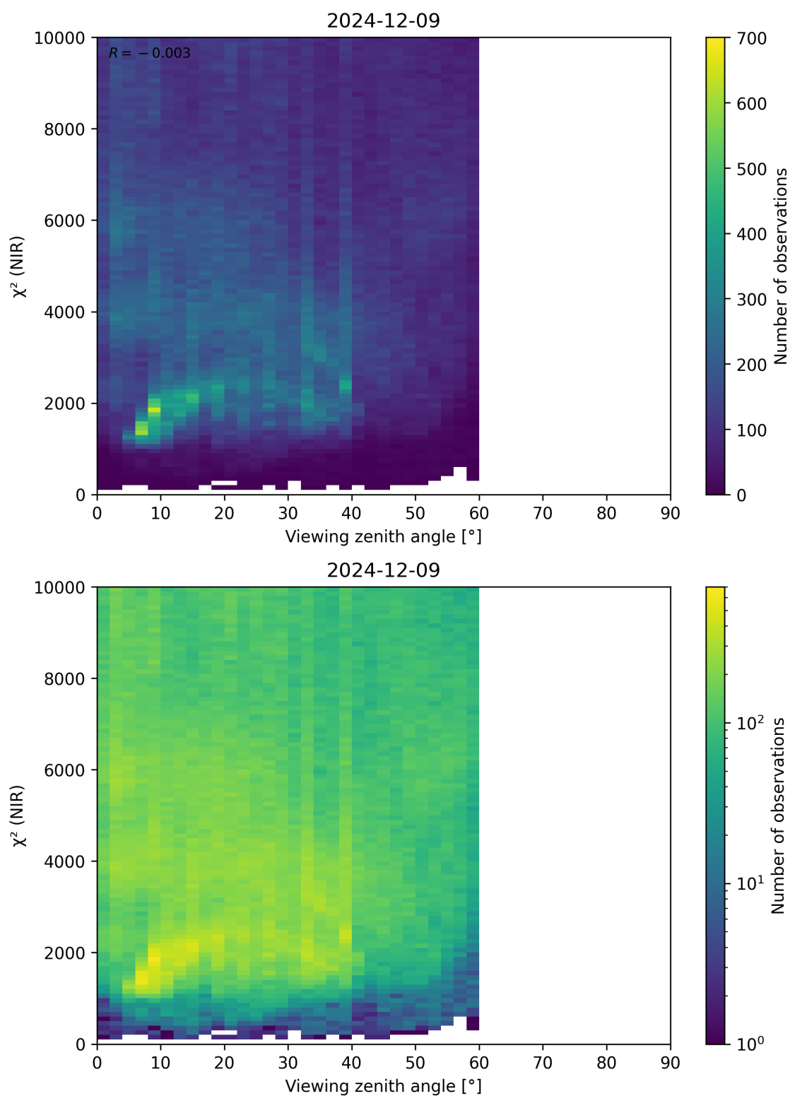
Figure 105: Scatter density plot of “Viewing zenith angle” against “ \chi^2 (NIR)” for 2024-12-08 to 2024-12-10.
