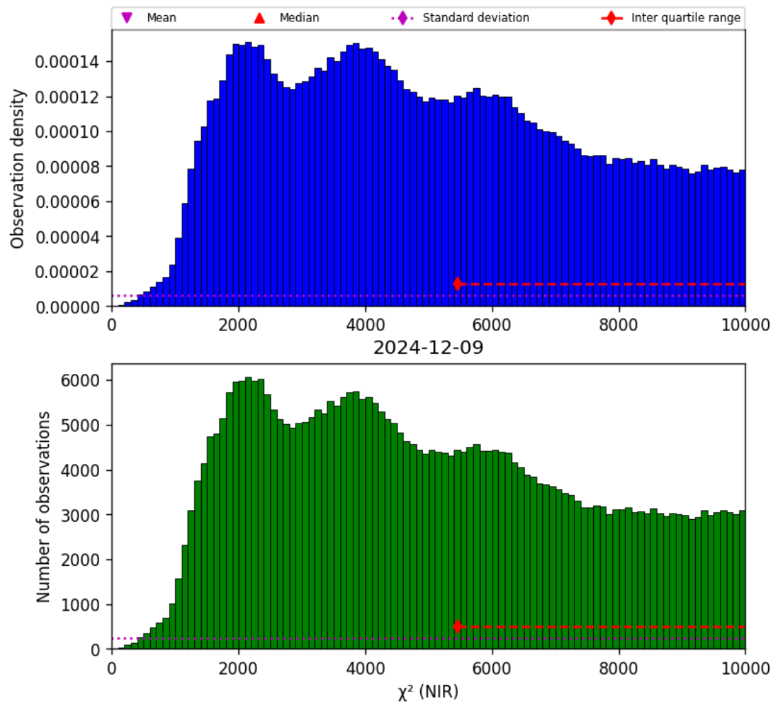
Figure 29: Histogram of " \chi^2 (NIR)" for 2024-12-08 to 2024-12-10
