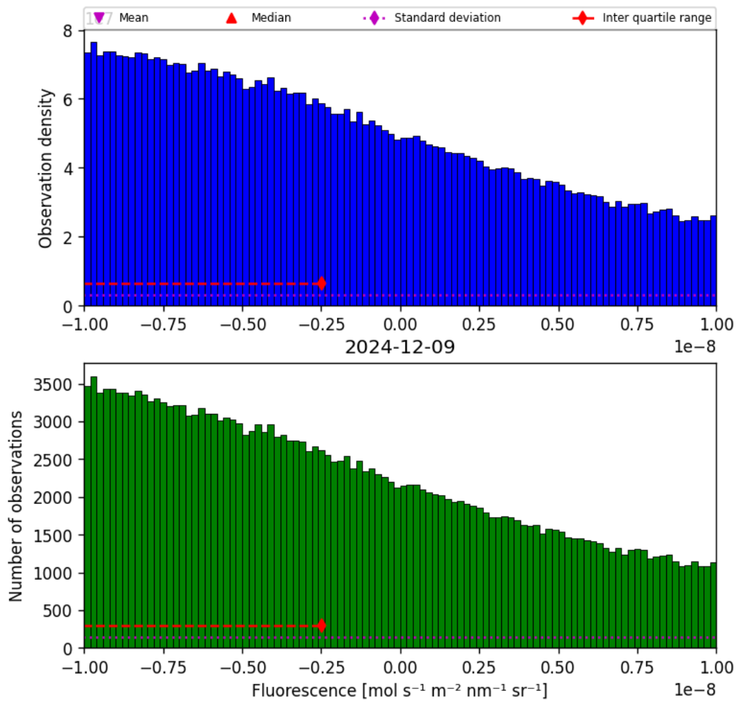
Figure 32: Histogram of “Fluorescence” for 2024-12-08 to 2024-12-10
