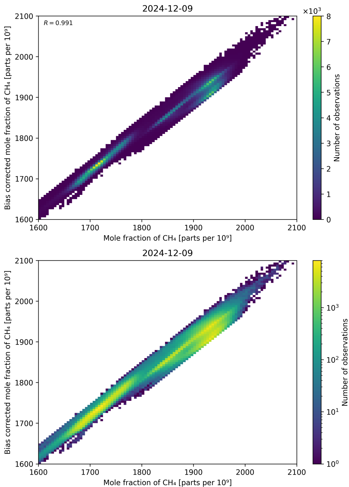
Figure 74: Scatter density plot of “Mole fraction of CH 4 ” against “Bias corrected mole fraction of CH 4 ” for 2024-12-08 to 2024-12-10.
