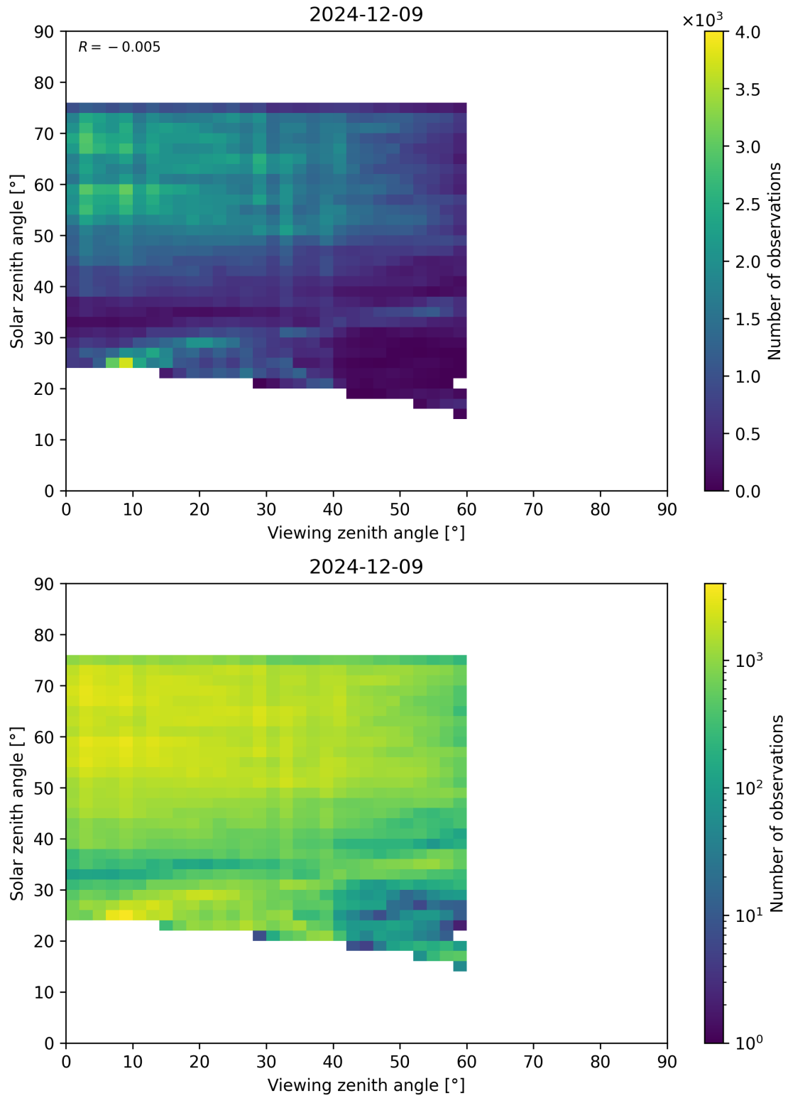
Figure 115: Scatter density plot of “Viewing zenith angle” against “Solar zenith angle” for 2024-12-08 to 2024-12-10.
