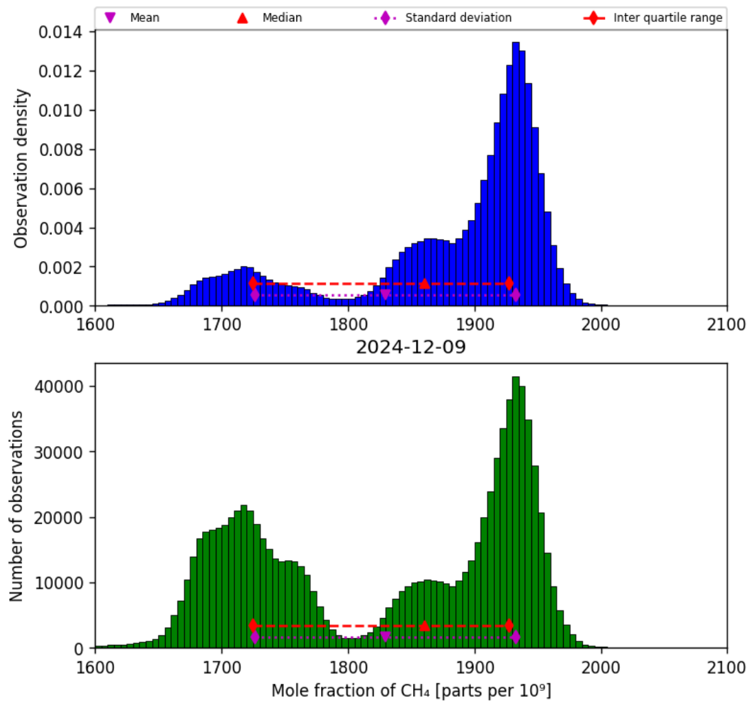
Figure 23: Histogram of “Mole fraction of CH 4 ” for 2024-12-08 to 2024-12-10
