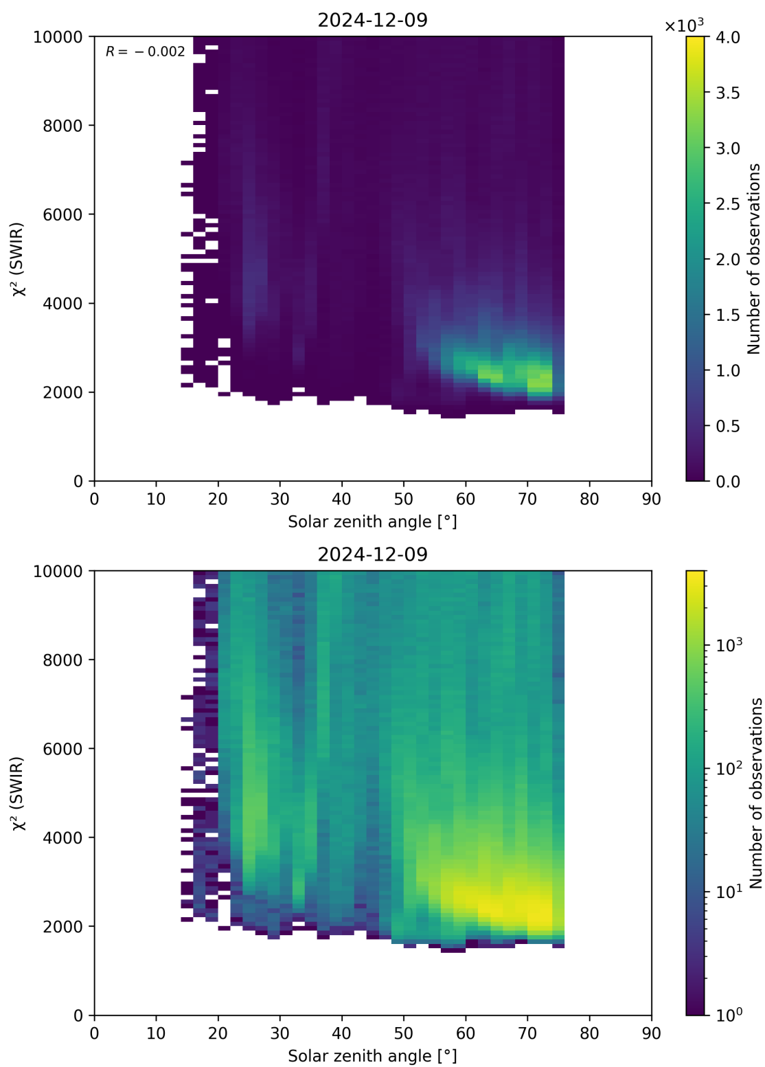
Figure 95: Scatter density plot of “Solar zenith angle” against “ \chi^2 (SWIR)” for 2024-12-08 to 2024-12-10.
