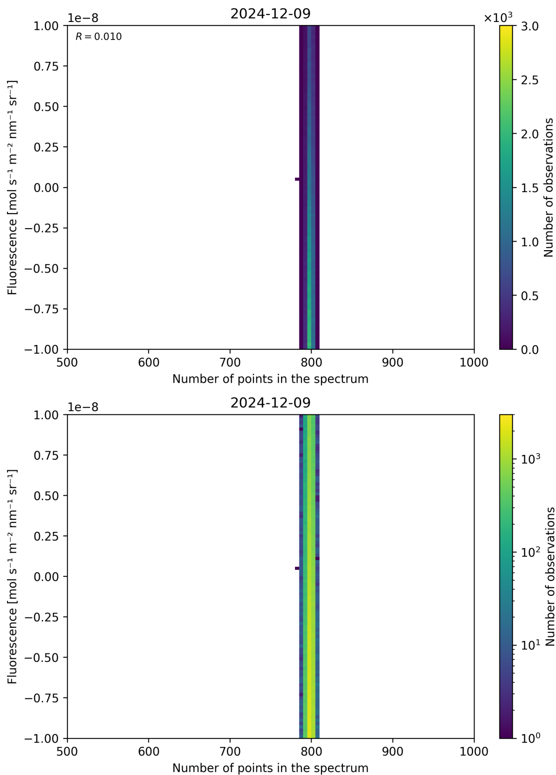
Figure 91: Scatter density plot of “Number of points in the spectrum” against “Fluorescence” for 2024-12-08 to 2024-12-10.
