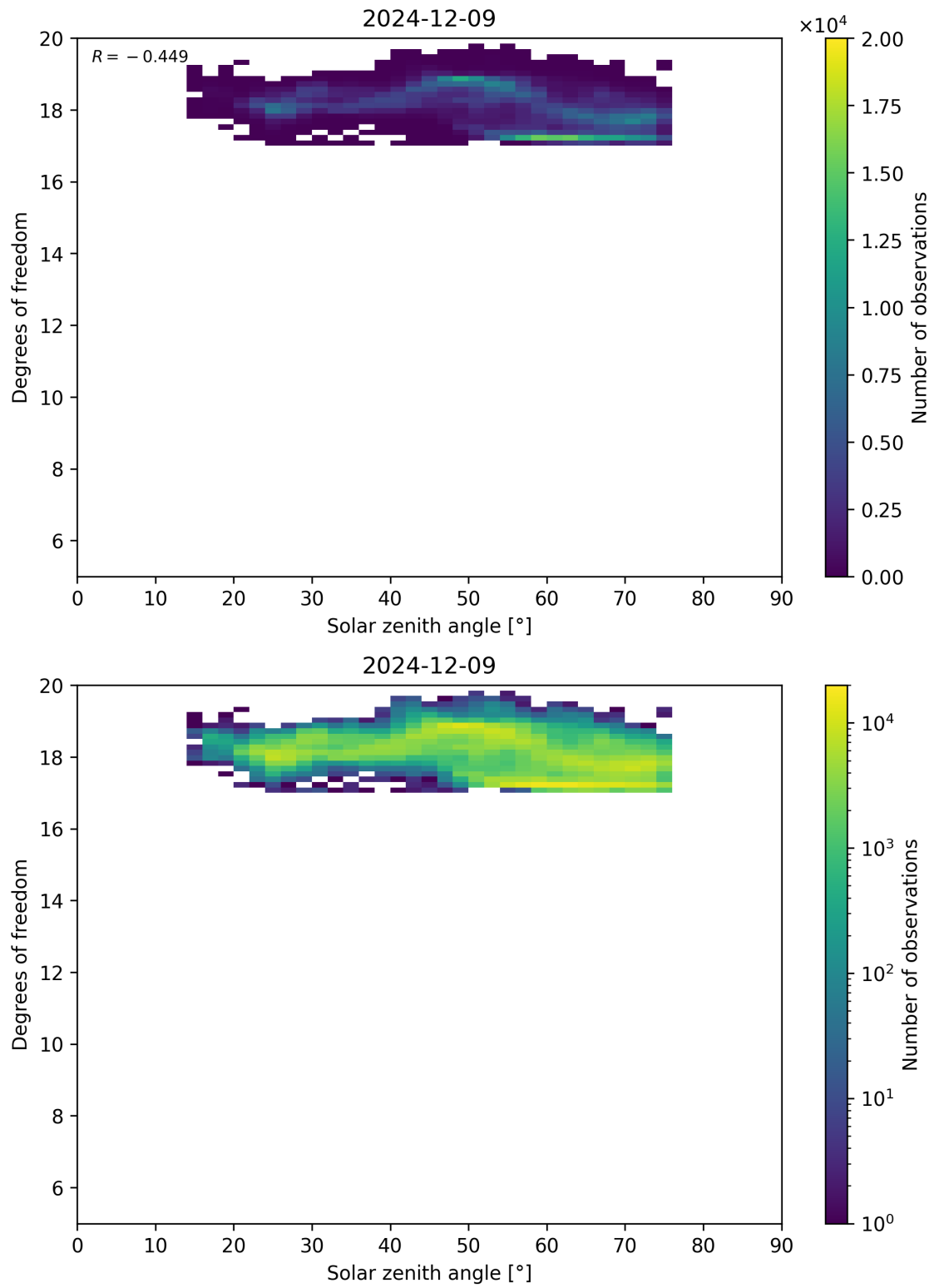
Figure 96: Scatter density plot of “Solar zenith angle” against “Degrees of freedom” for 2024-12-08 to 2024-12-10.
