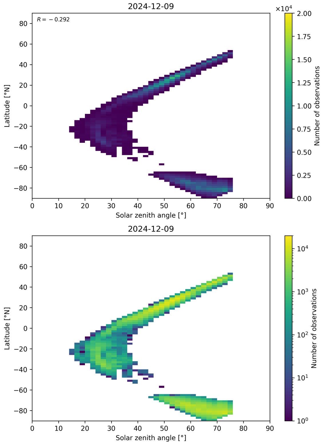
Figure 98: Scatter density plot of “Solar zenith angle” against “Latitude” for 2024-12-08 to 2024-12-10.
