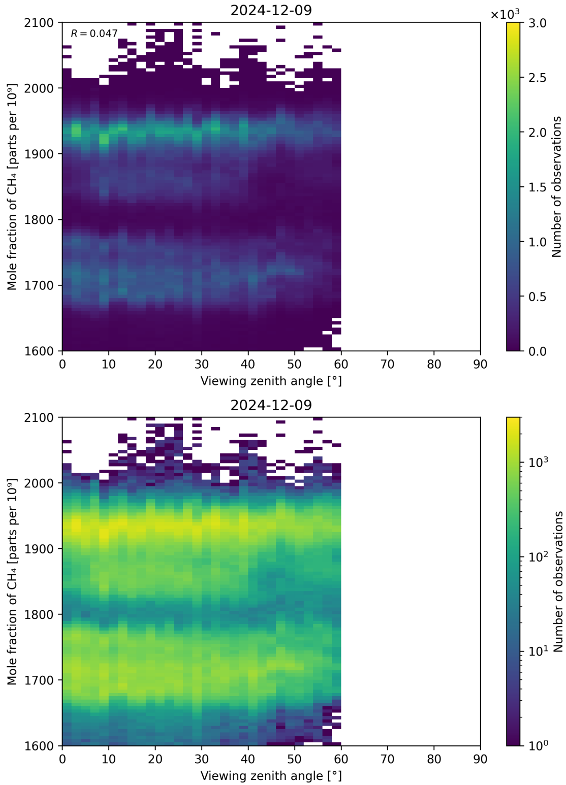
Figure 110: Scatter density plot of “Viewing zenith angle” against “Mole fraction of CH 4 ” for 2024-12-08 to 2024-12-10.
