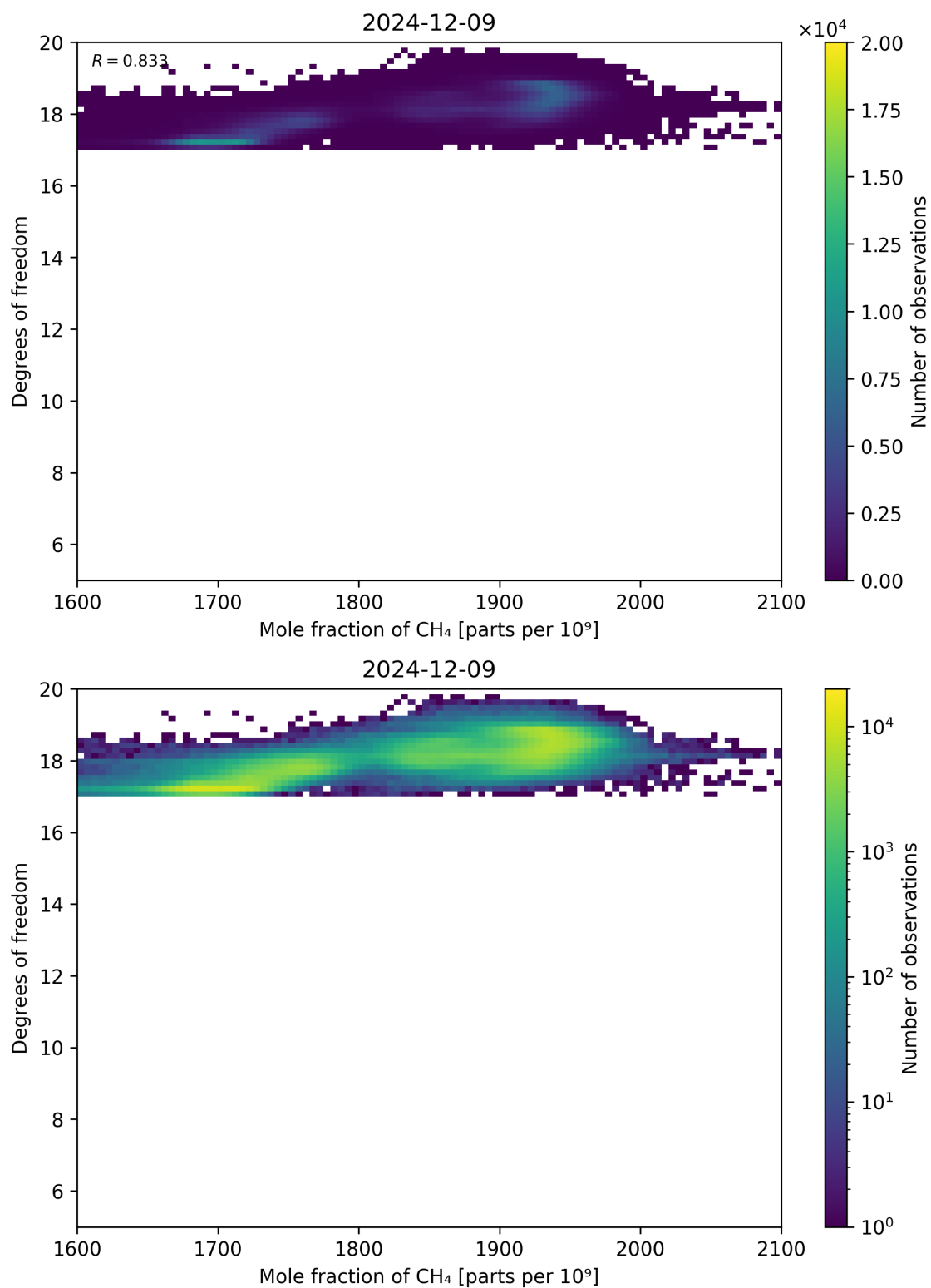
Figure 72: Scatter density plot of “Mole fraction of CH 4 ” against “Degrees of freedom” for 2024-12-08 to 2024-12-10.
