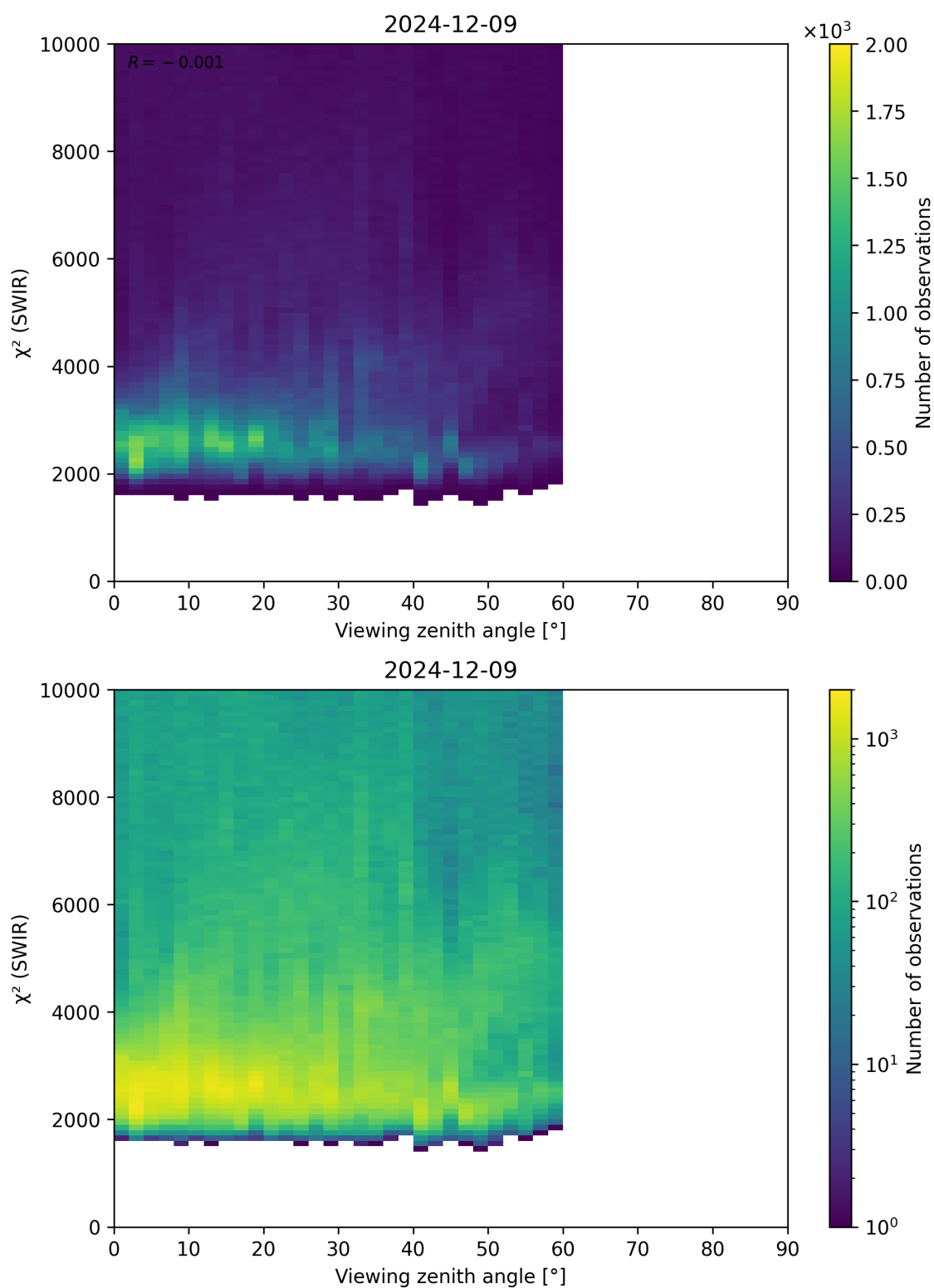
Figure 106: Scatter density plot of “Viewing zenith angle” against “ \chi^2 (SWIR)” for 2024-12-08 to 2024-12-10.
