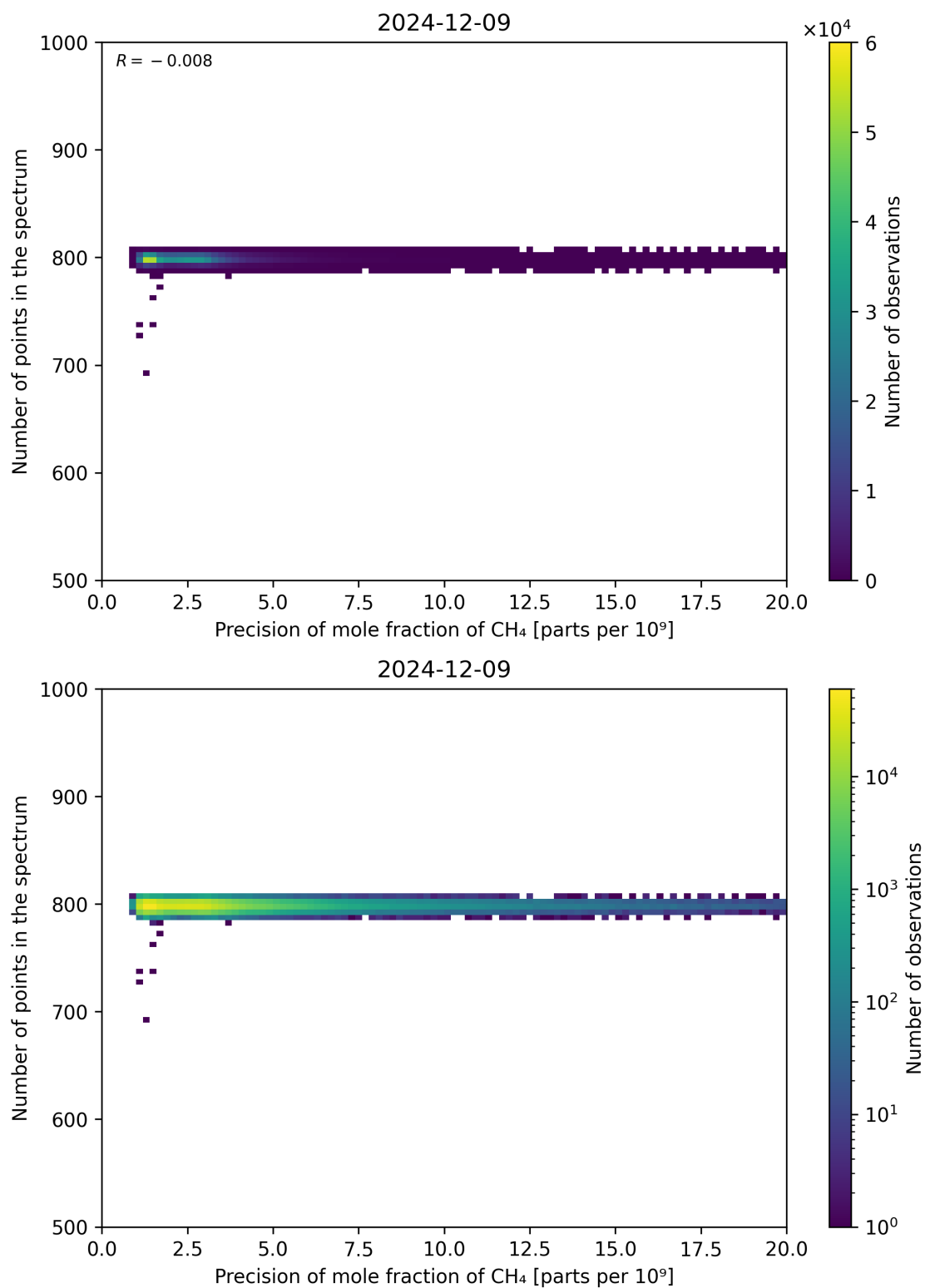
Figure 84: Scatter density plot of “Precision of mole fraction of CH 4 ” against “Number of points in the spectrum” for 2024-12-08 to 2024-12-10.
