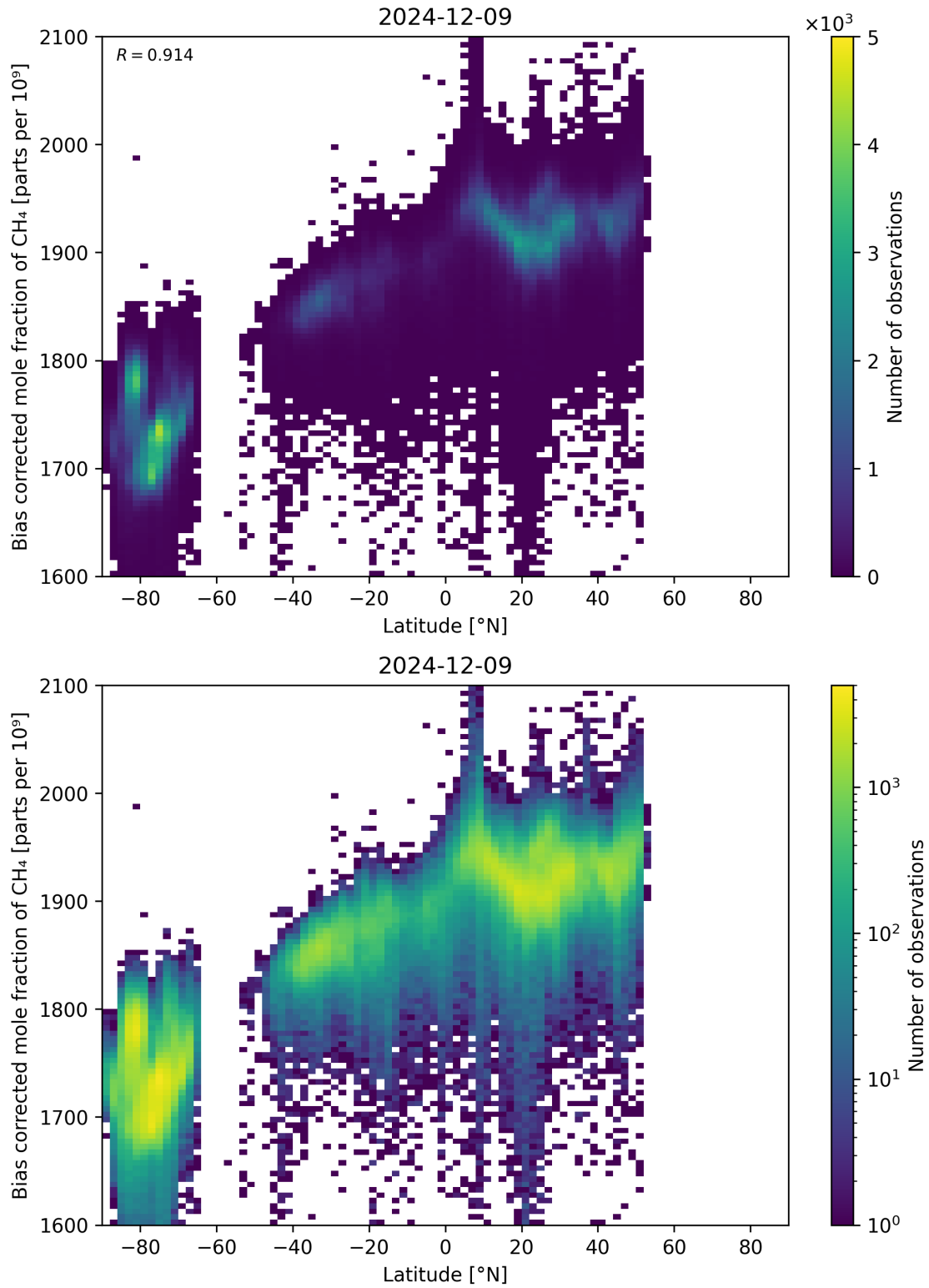
Figure 58: Scatter density plot of “Latitude” against “Bias corrected mole fraction of CH 4 ” for 2024-12-08 to 2024-12-10.
