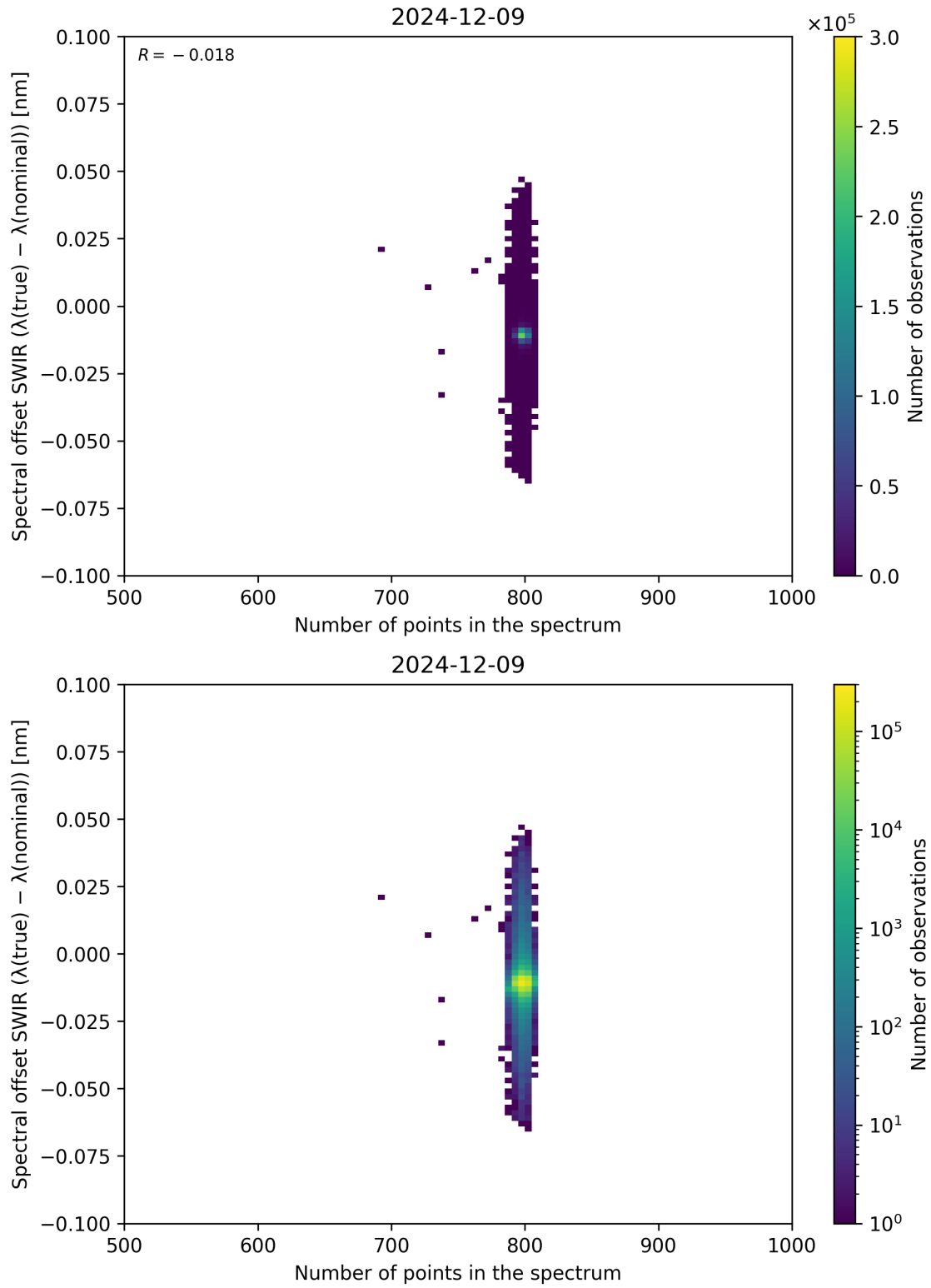
Figure 93: Scatter density plot of “Number of points in the spectrum” against “Spectral offset SWIR ( \lambda_{\text{true}} - \lambda_{\text{nominal}} )” for 2024-12-08 to 2024-12-10.
