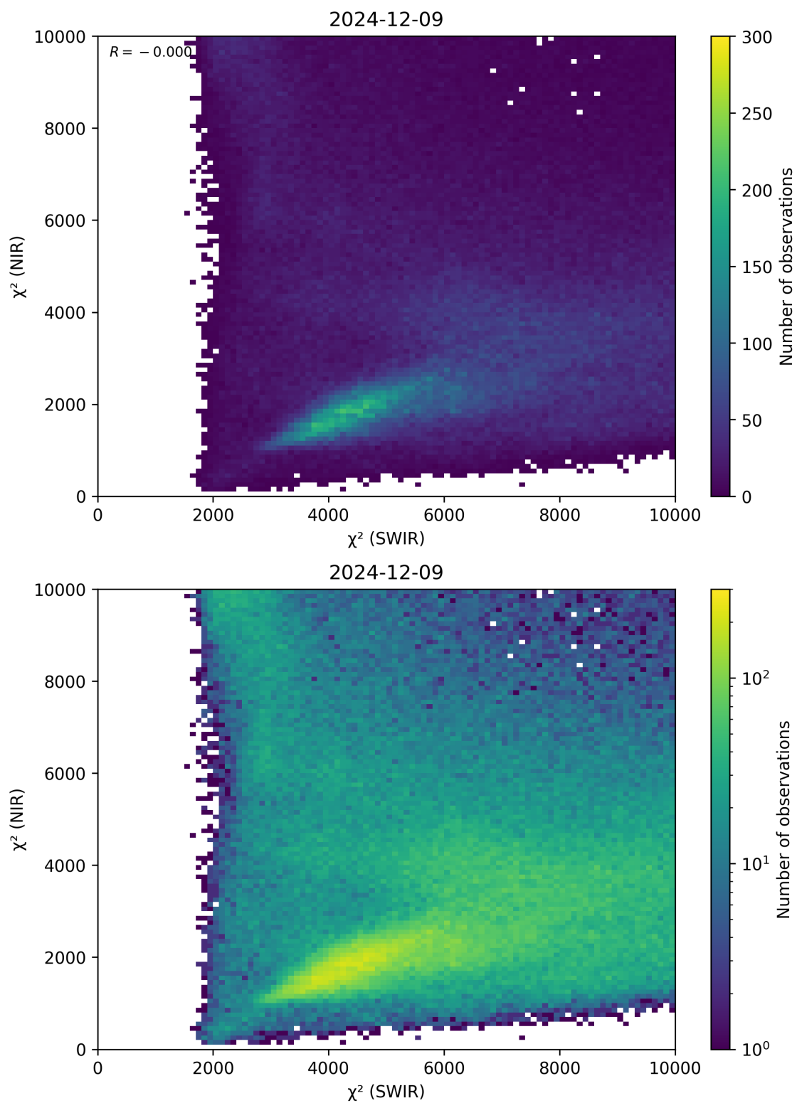
Figure 47: Scatter density plot of “ \chi^2 (SWIR)” against “ \chi^2 (NIR)” for 2024-12-08 to 2024-12-10.
