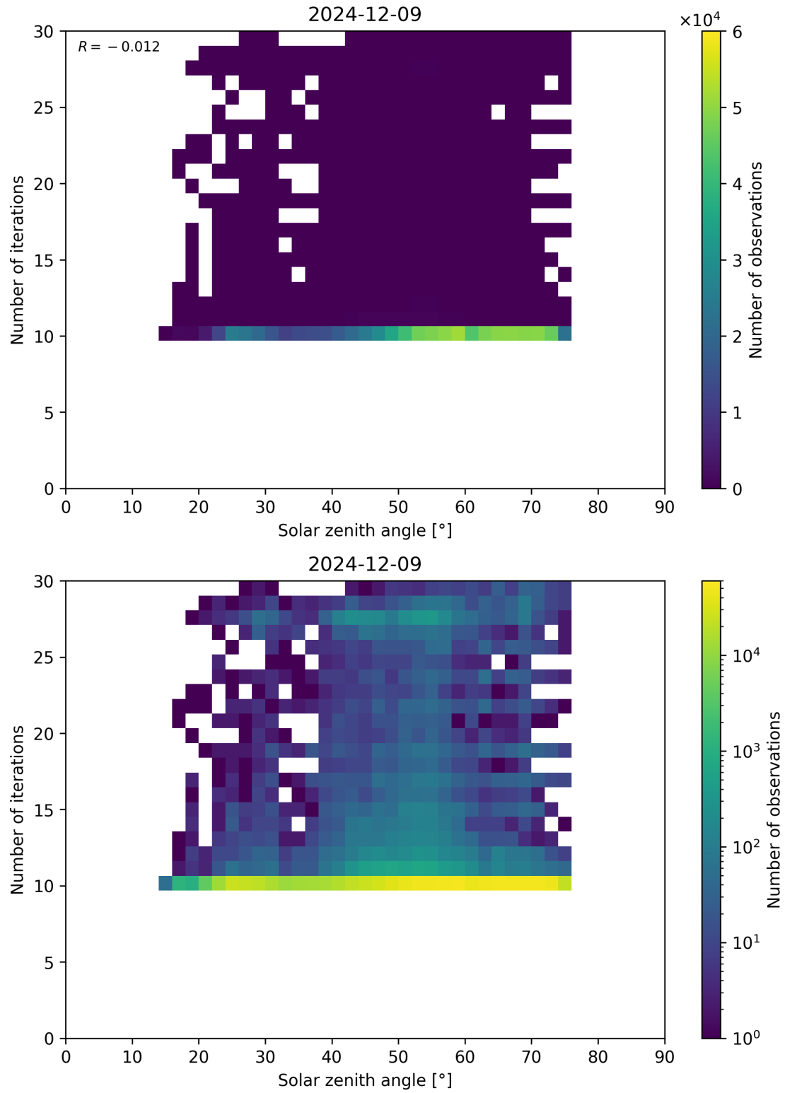
Figure 102: Scatter density plot of “Solar zenith angle” against “Number of iterations” for 2024-12-08 to 2024-12-10.
