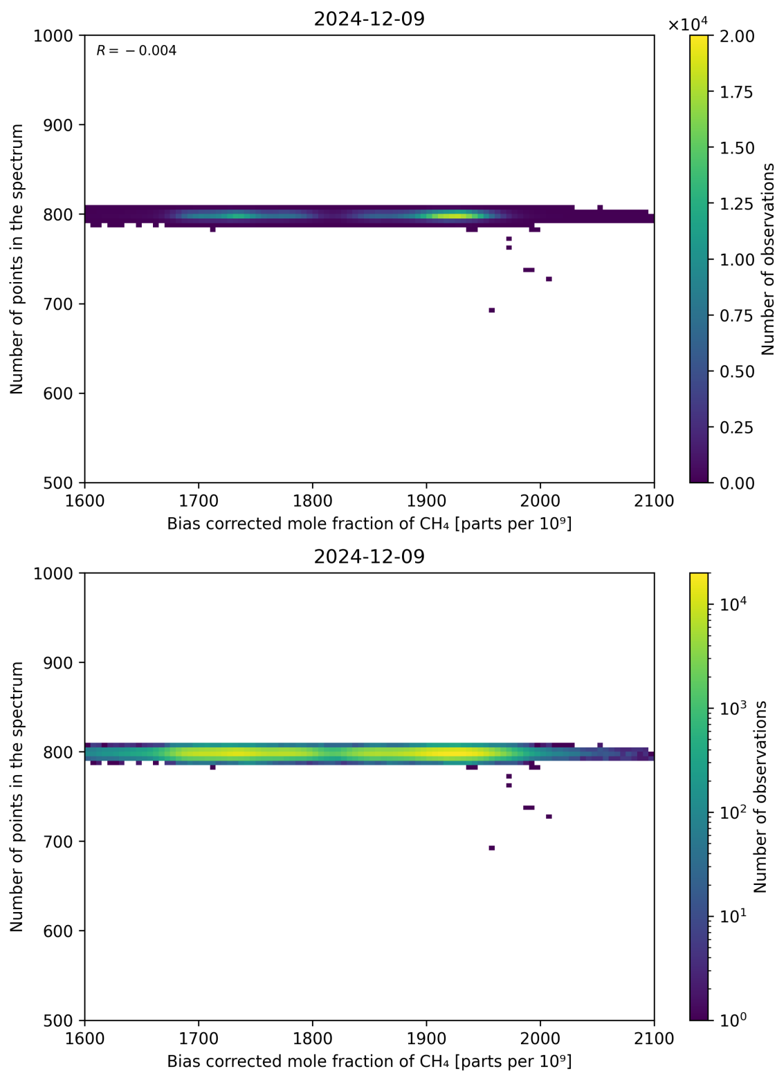
Figure 68: Scatter density plot of “Bias corrected mole fraction of CH 4 ” against “Number of points in the spectrum” for 2024-12-08 to 2024-12-10.
