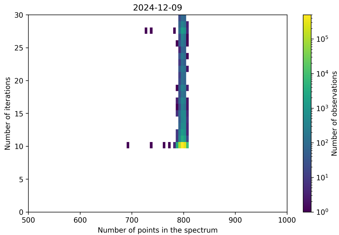
Figure 92: Scatter density plot of “Number of points in the spectrum” against “Number of iterations” for 2024-12-08 to 2024-12-10.
