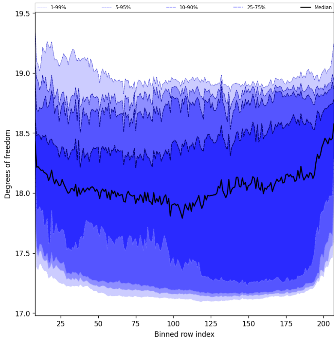
Figure 41: Along track statistics of “Degrees of freedom” for 2024-12-08 to 2024-12-10
