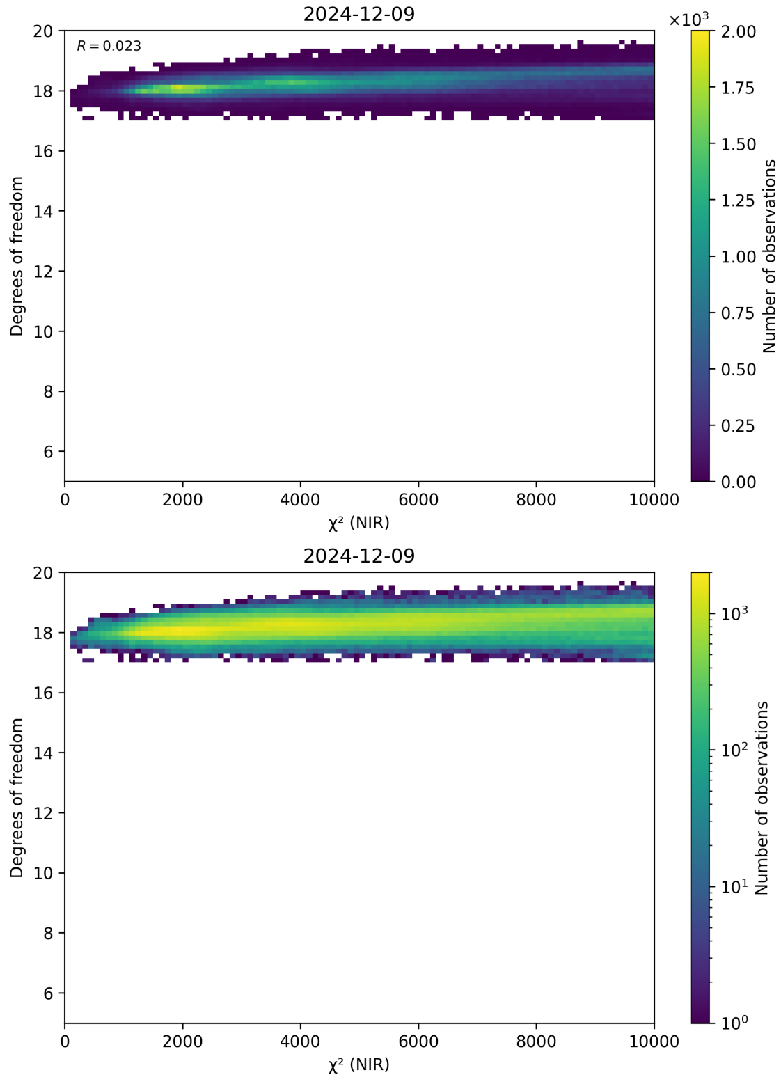
Figure 44: Scatter density plot of “ \chi^2 (NIR)” against “Degrees of freedom” for 2024-12-08 to 2024-12-10.
