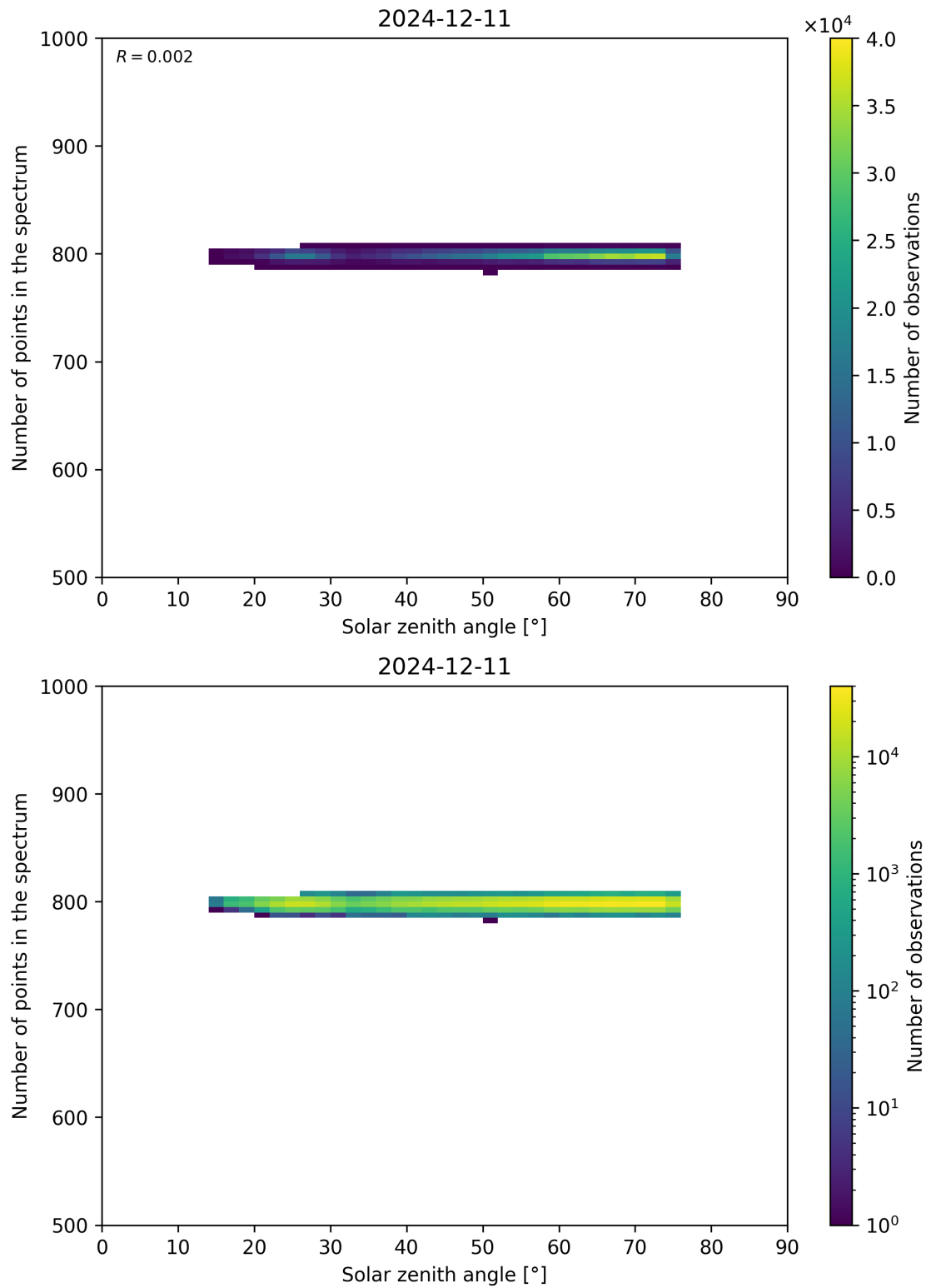
Figure 103: Scatter density plot of “Solar zenith angle” against “Number of points in the spectrum” for 2024-12-11 to 2024-12-12.
