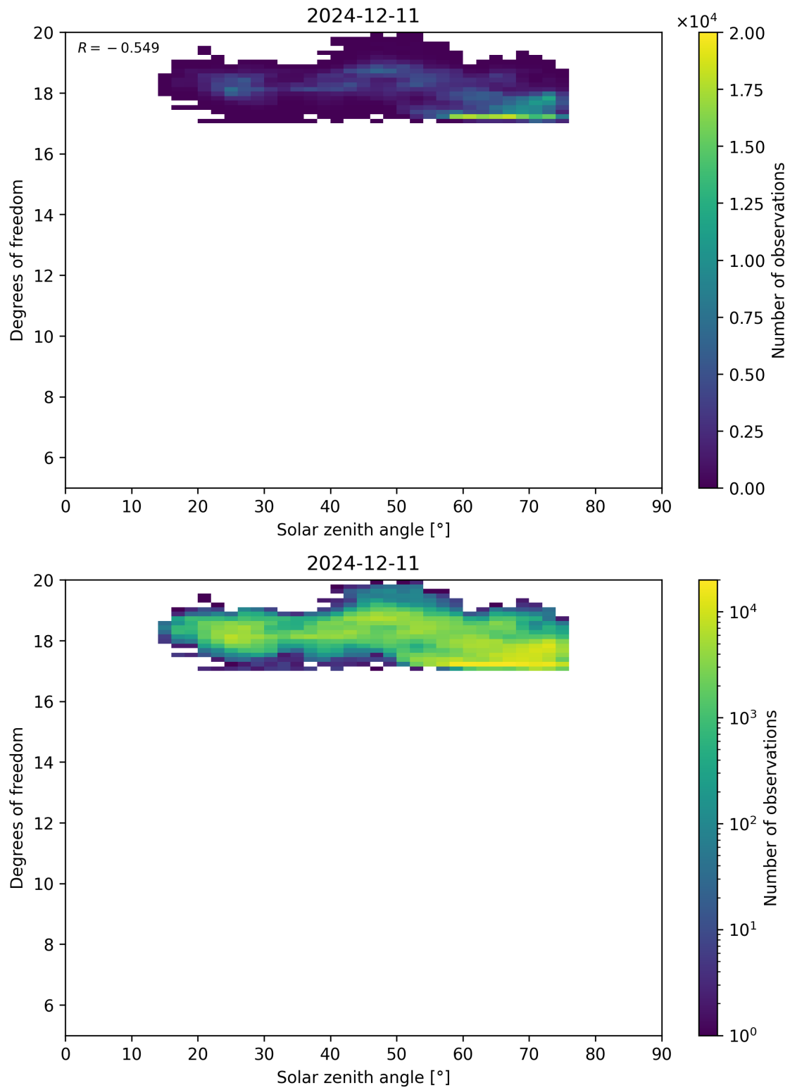
Figure 96: Scatter density plot of “Solar zenith angle” against “Degrees of freedom” for 2024-12-11 to 2024-12-12.
