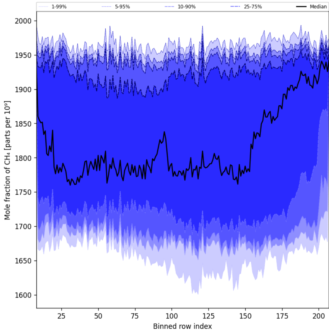
Figure 34: Along track statistics of “Mole fraction of CH 4 ” for 2024-12-11 to 2024-12-12
