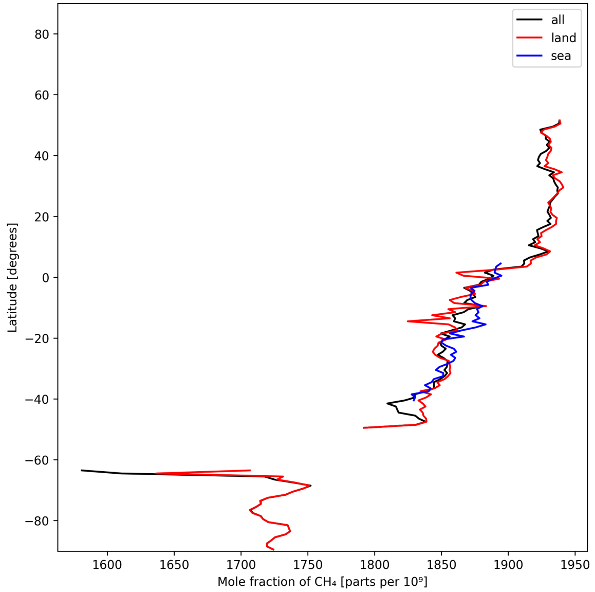
Figure 12: Zonal average of “Mole fraction of \text{CH}_4 ” for 2024-12-11 to 2024-12-12.
