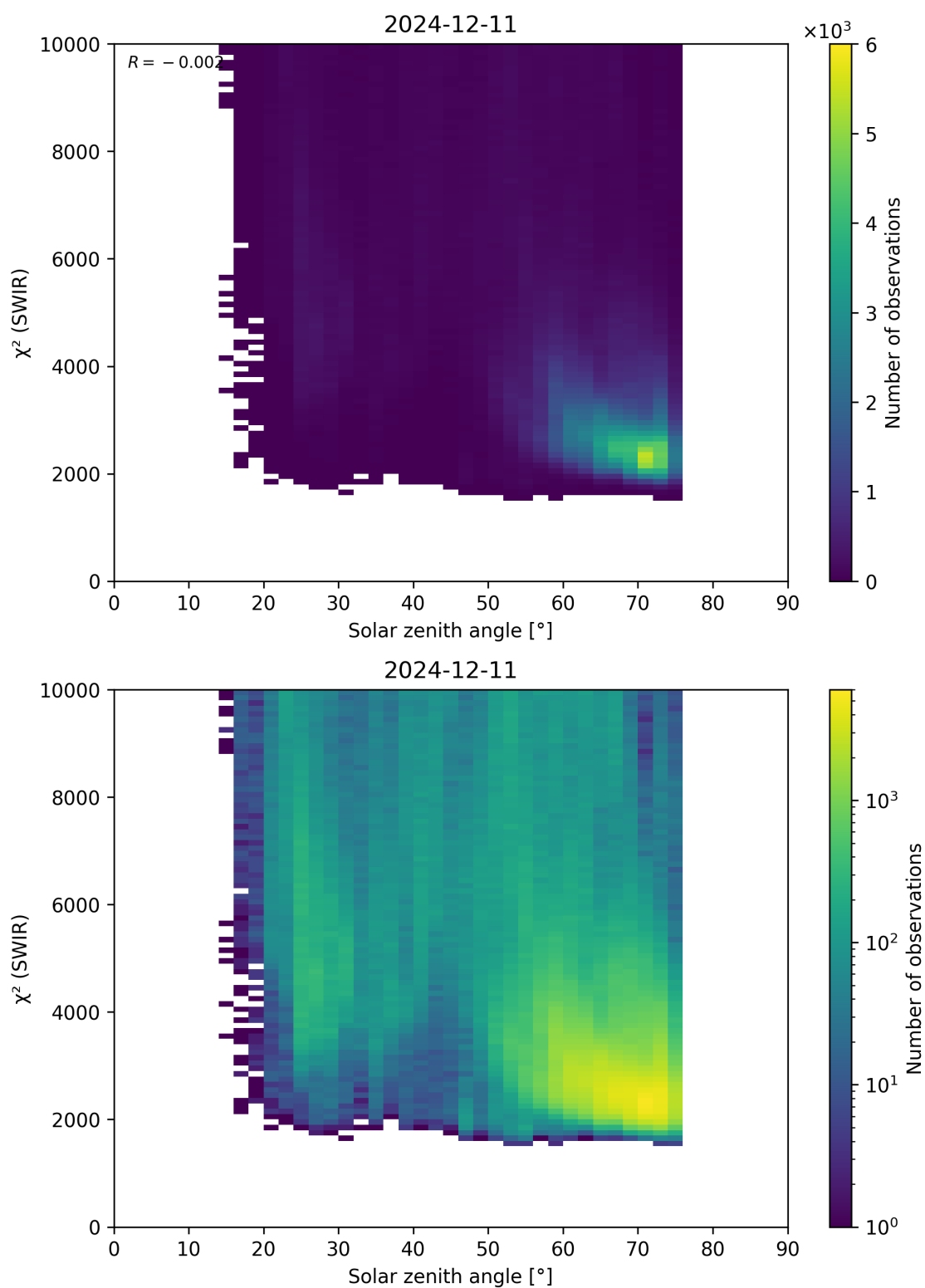
Figure 95: Scatter density plot of “Solar zenith angle” against “ \chi^2 (SWIR)” for 2024-12-11 to 2024-12-12.
