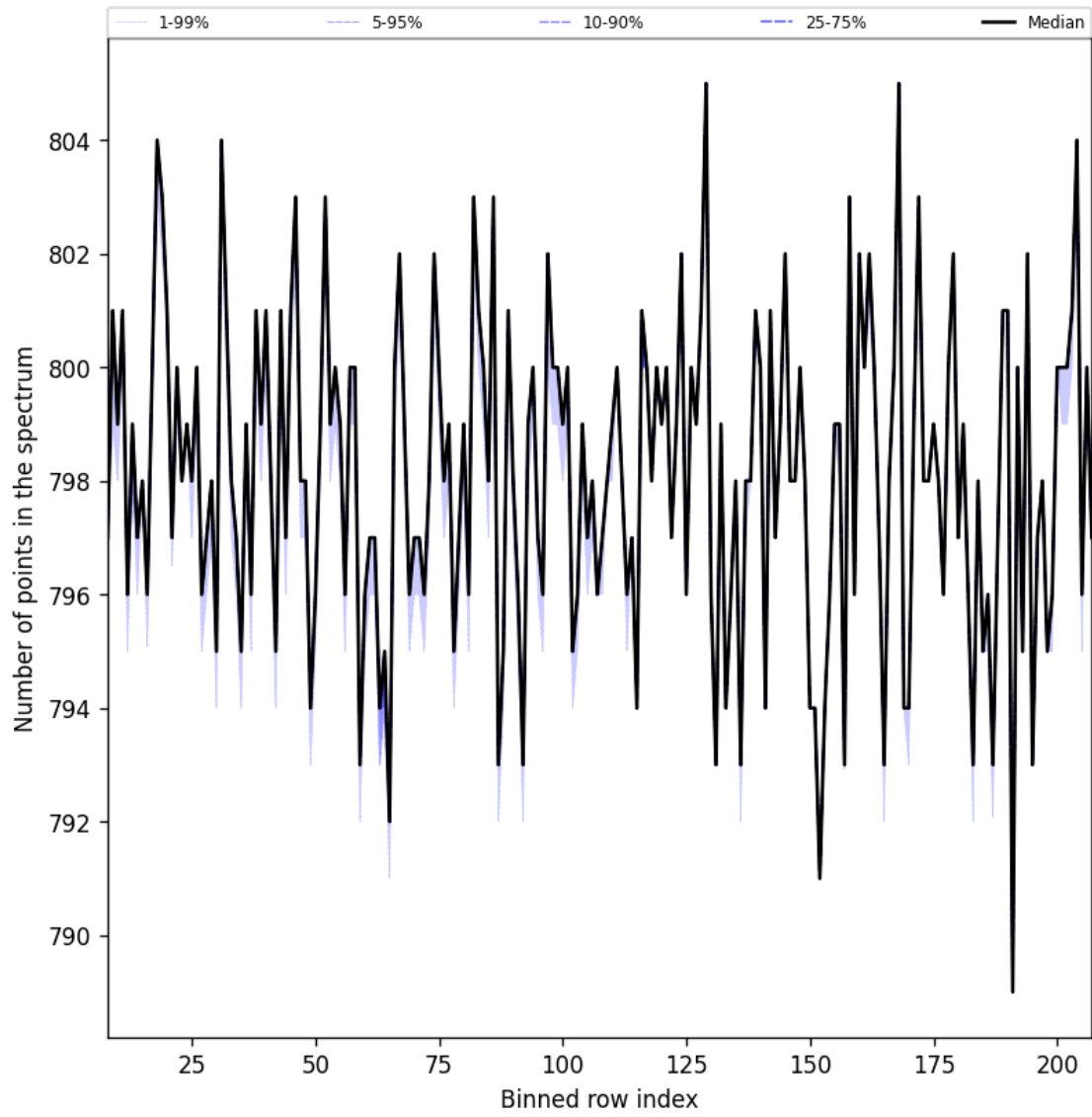
Figure 37: Along track statistics of “Number of points in the spectrum” for 2024-12-11 to 2024-12-12
