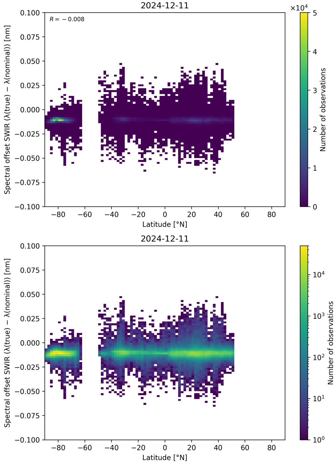
Figure 62: Scatter density plot of “Latitude” against “Spectral offset SWIR ( \lambda_{\text{true}} - \lambda_{\text{nominal}} )” for 2024-12-11 to 2024-12-12.
