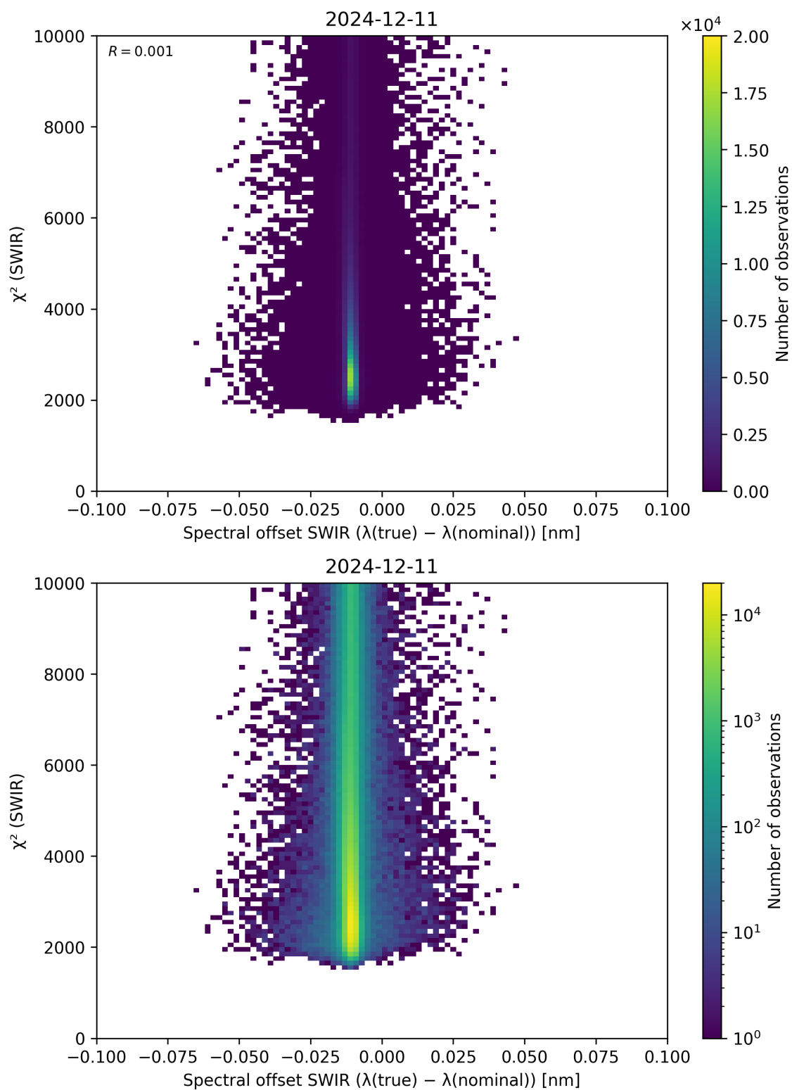
Figure 118: Scatter density plot of “Spectral offset SWIR ( \lambda_{\text{true}} - \lambda_{\text{nominal}} )” against “ \chi^2 (SWIR)” for 2024-12-11 to 2024-12-12.
