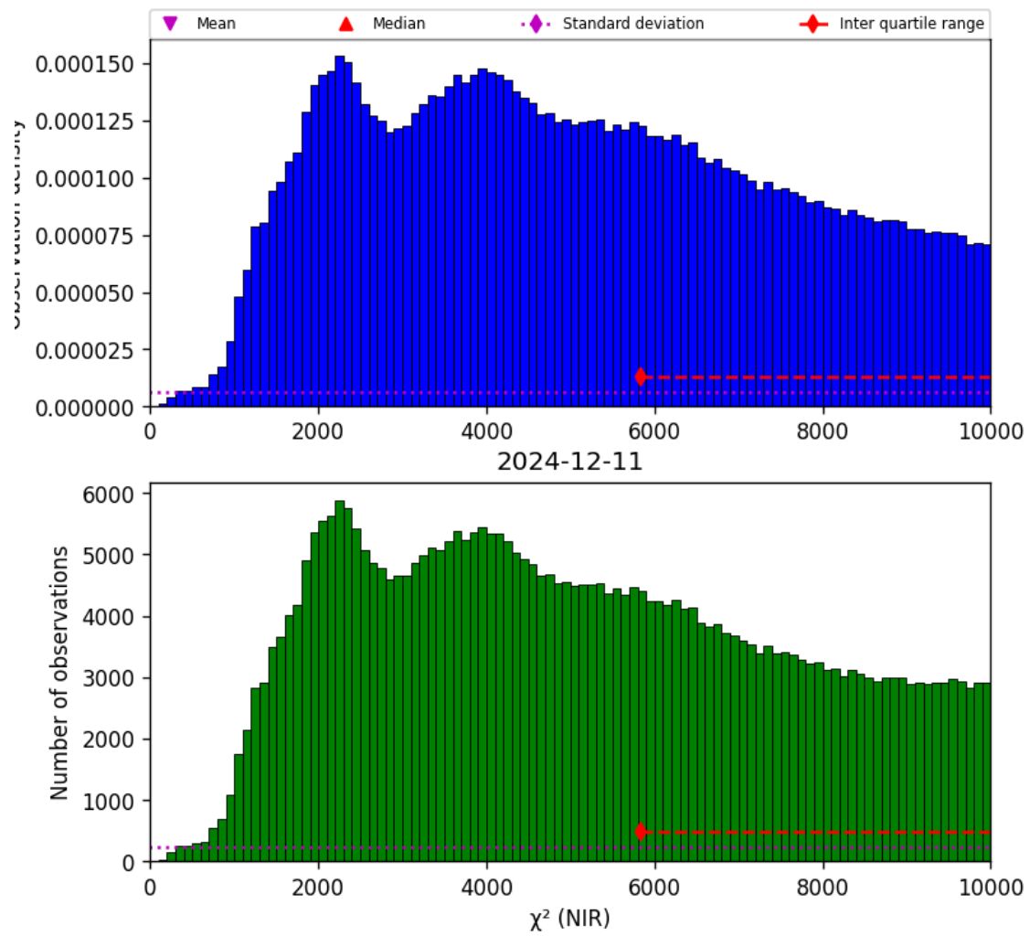
Figure 29: Histogram of “ \chi^2 (NIR)” for 2024-12-11 to 2024-12-12
