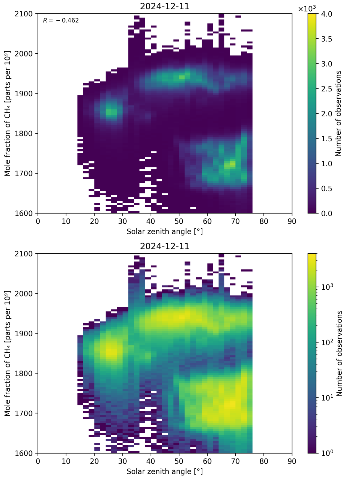
Figure 99: Scatter density plot of “Solar zenith angle” against “Mole fraction of CH 4 ” for 2024-12-11 to 2024-12-12.
