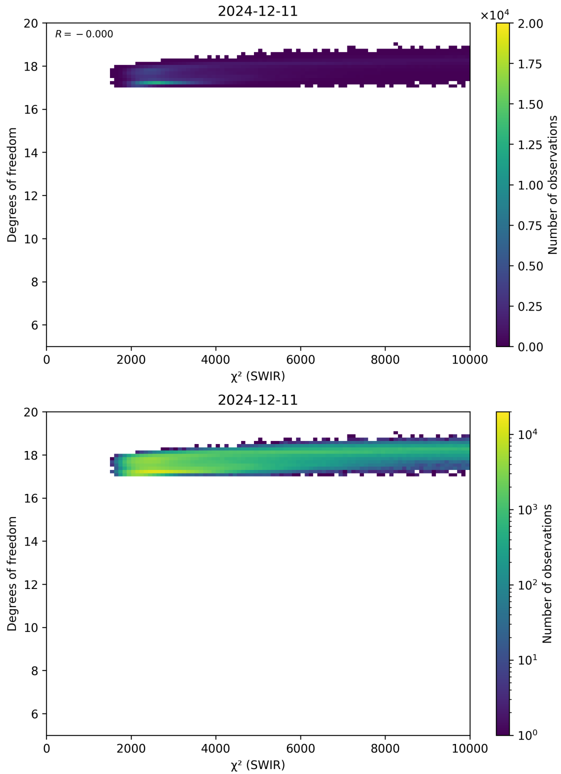
Figure 48: Scatter density plot of “ \chi^2 (SWIR)” against “Degrees of freedom” for 2024-12-11 to 2024-12-12.
