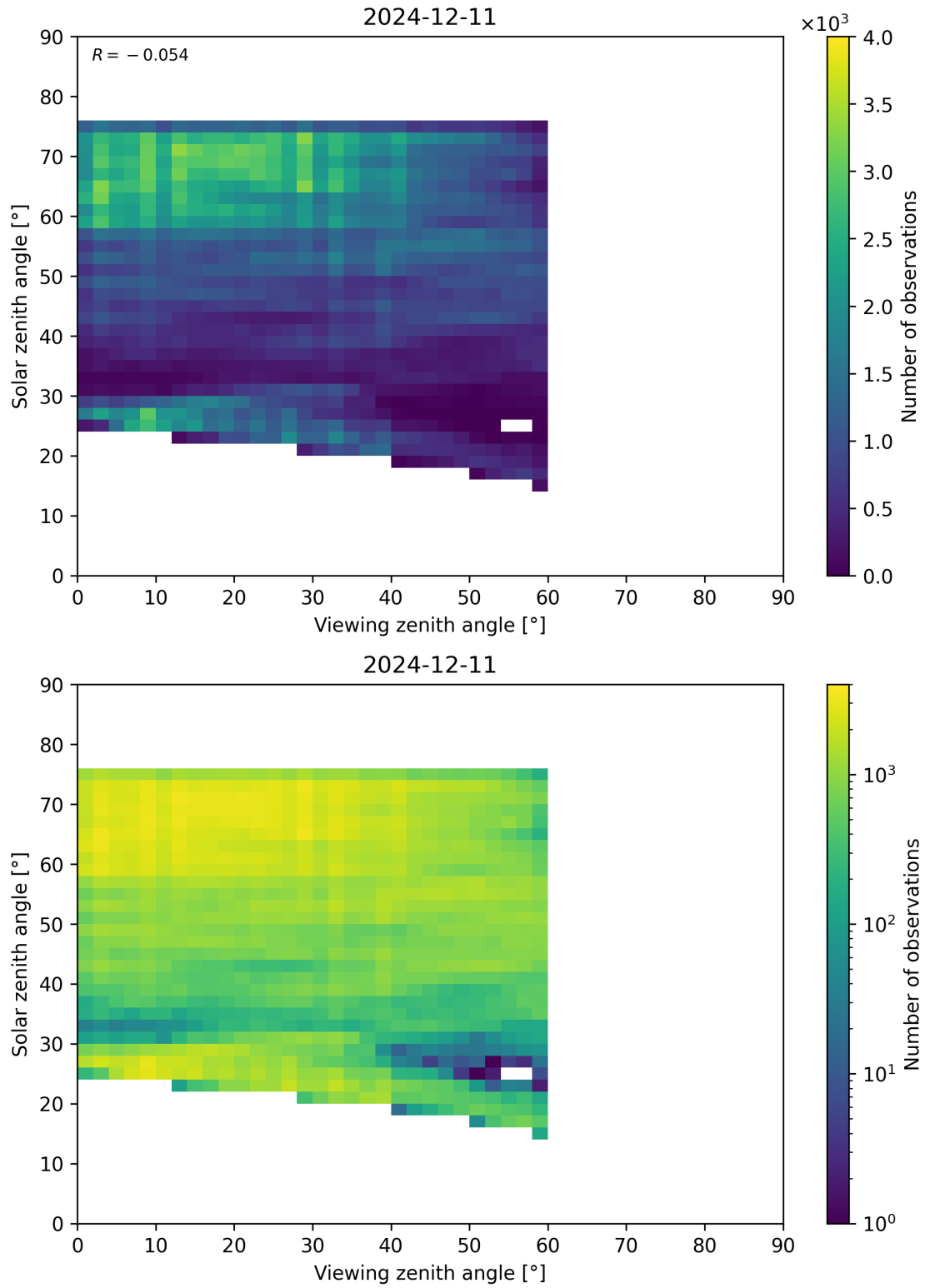
Figure 115: Scatter density plot of “Viewing zenith angle” against “Solar zenith angle” for 2024-12-11 to 2024-12-12.
