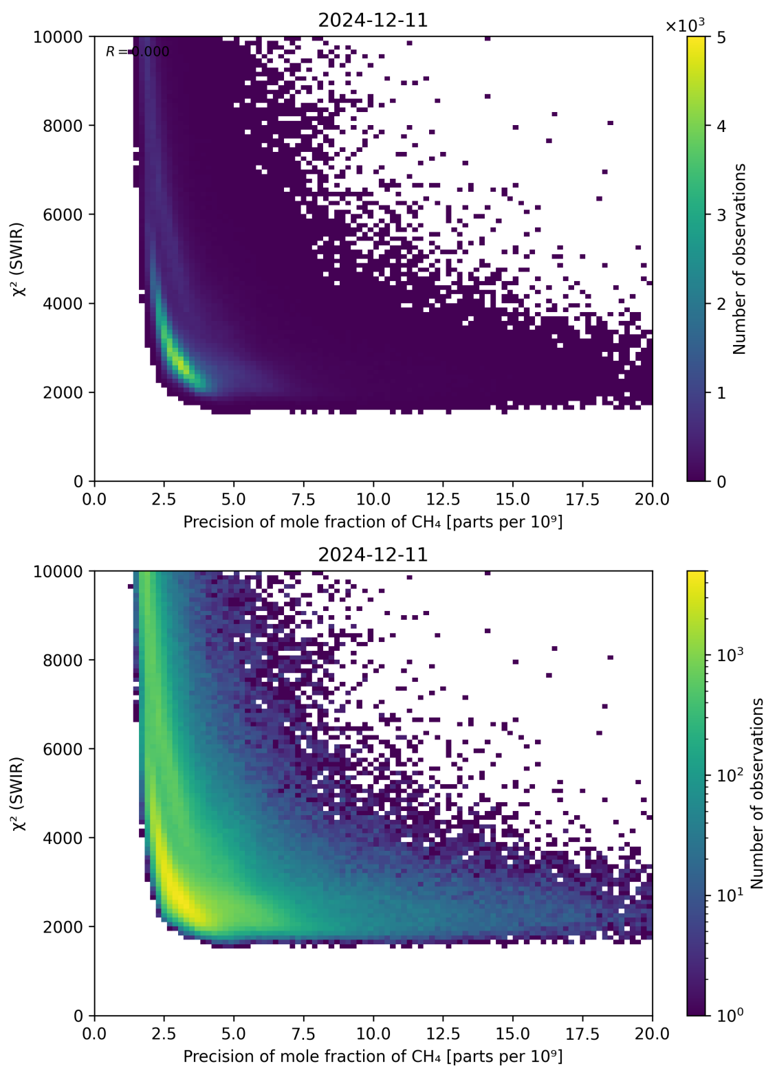
Figure 79: Scatter density plot of “Precision of mole fraction of \text{CH}_4 ” against “ \chi^2 (SWIR)” for 2024-12-11 to 2024-12-12.
