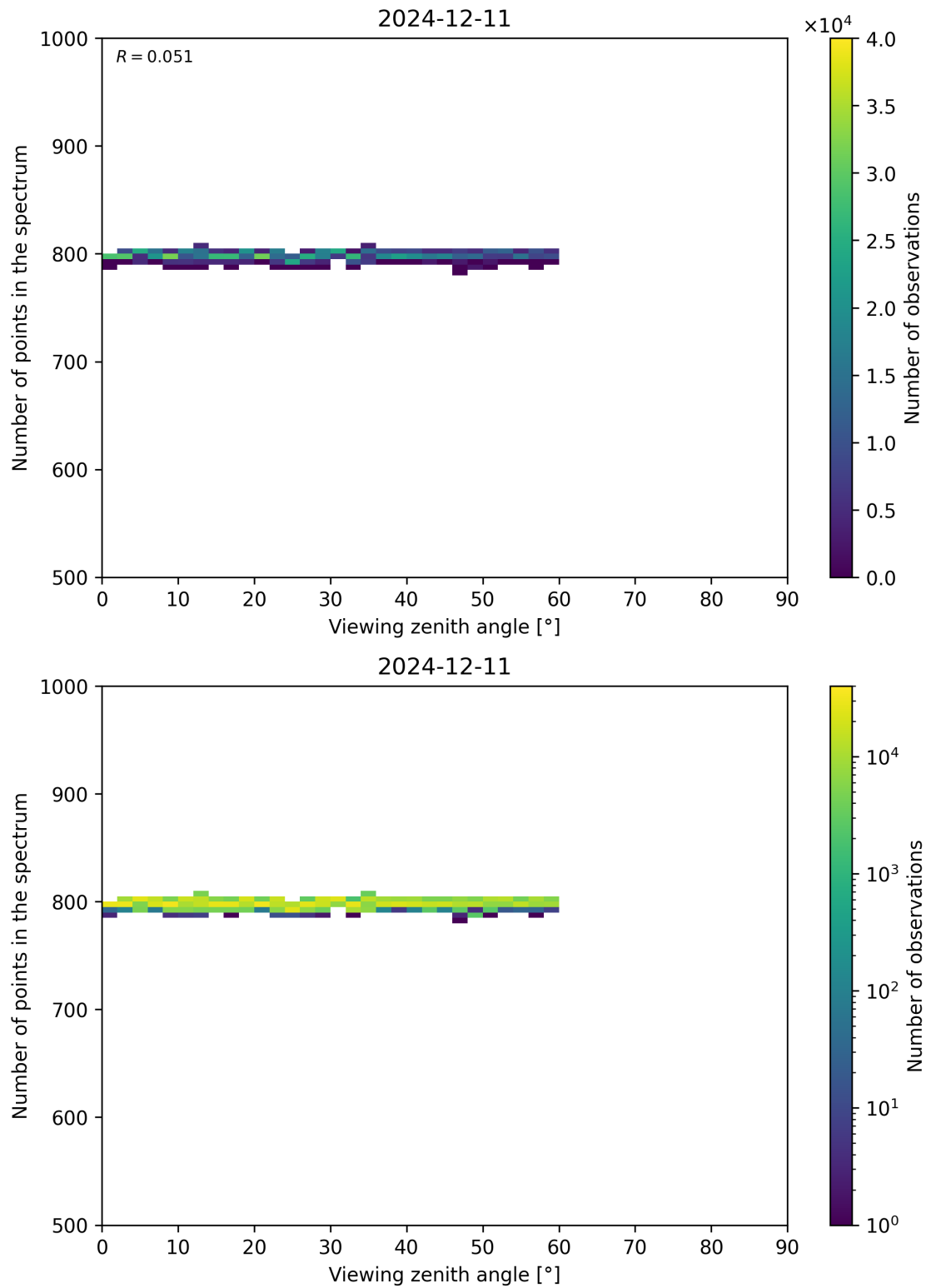
Figure 114: Scatter density plot of “Viewing zenith angle” against “Number of points in the spectrum” for 2024-12-11 to 2024-12-12.
