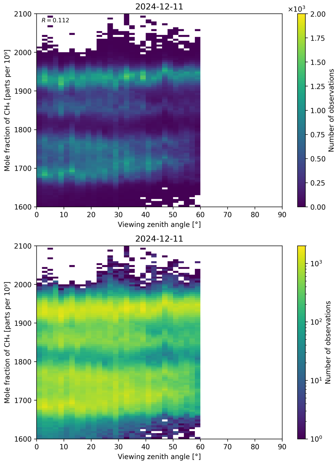
Figure 110: Scatter density plot of “Viewing zenith angle” against “Mole fraction of CH 4 ” for 2024-12-11 to 2024-12-12.
