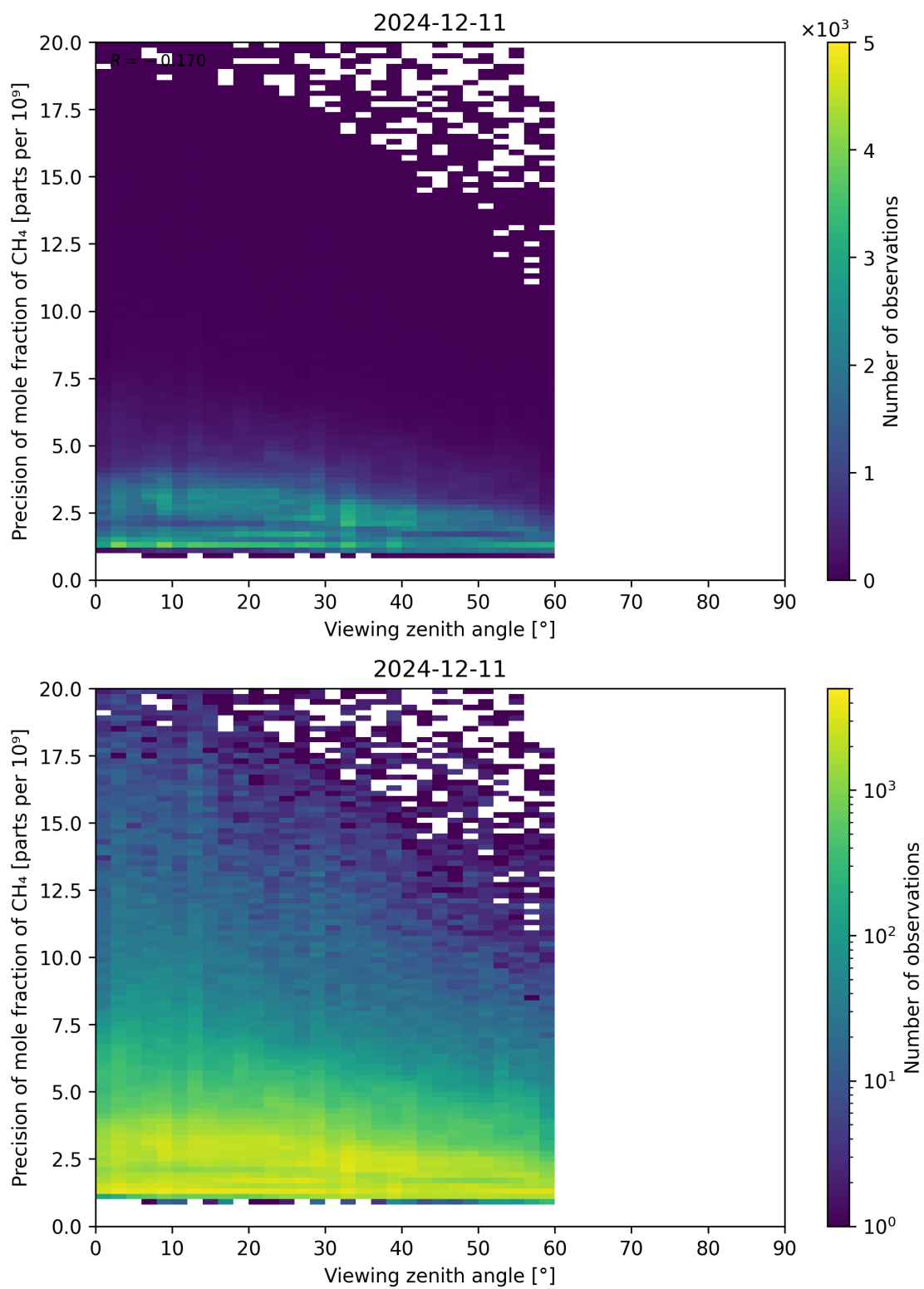
Figure 112: Scatter density plot of “Viewing zenith angle” against “Precision of mole fraction of \text{CH}_4 ” for 2024-12-11 to 2024-12-12.
