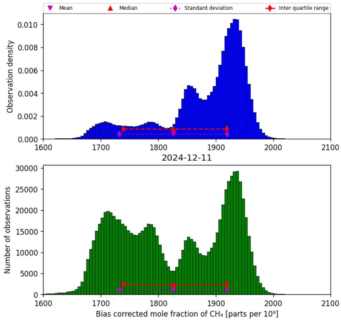
Figure 25: Histogram of “Bias corrected mole fraction of CH 4 ” for 2024-12-11 to 2024-12-12
