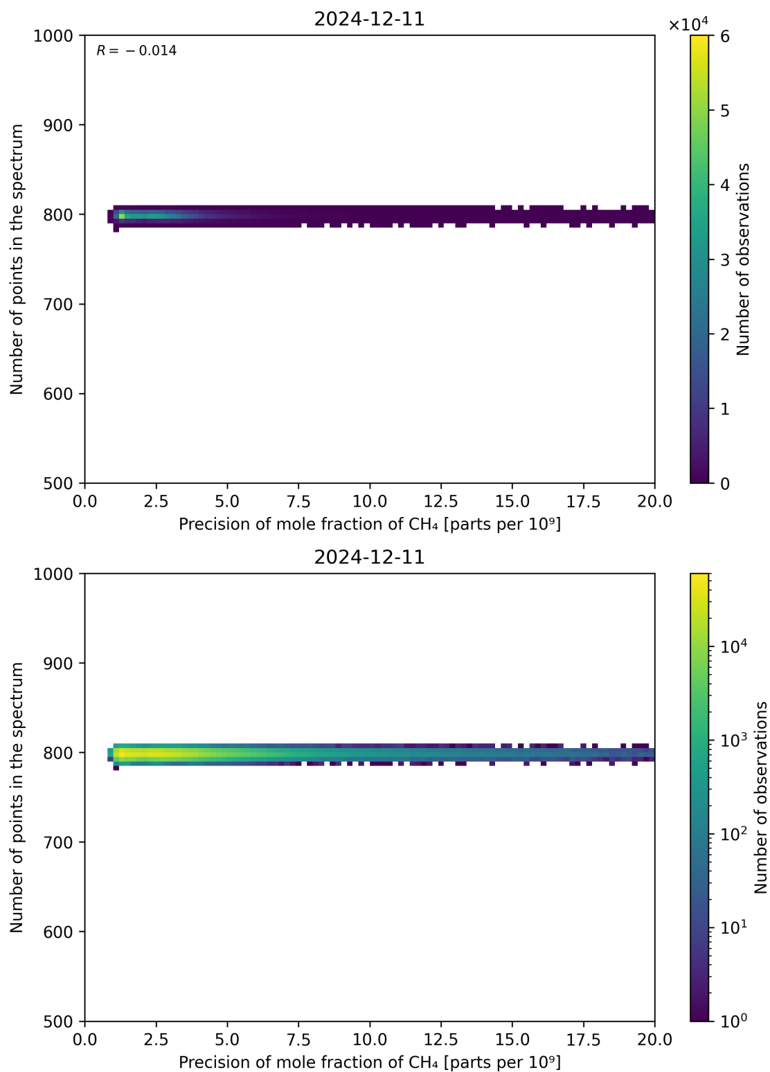
Figure 84: Scatter density plot of “Precision of mole fraction of CH 4 ” against “Number of points in the spectrum” for 2024-12-11 to 2024-12-12.
