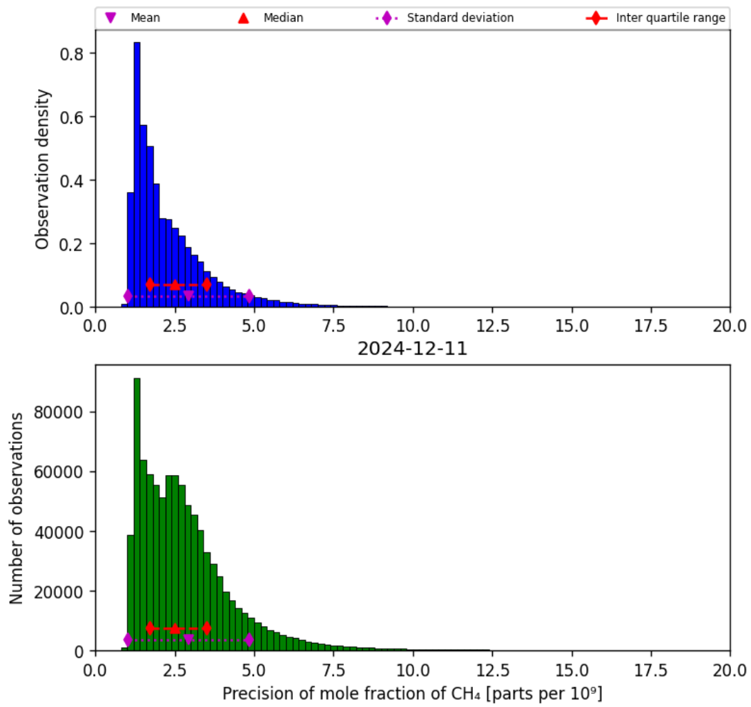
Figure 24: Histogram of “Precision of mole fraction of CH 4 ” for 2024-12-11 to 2024-12-12
