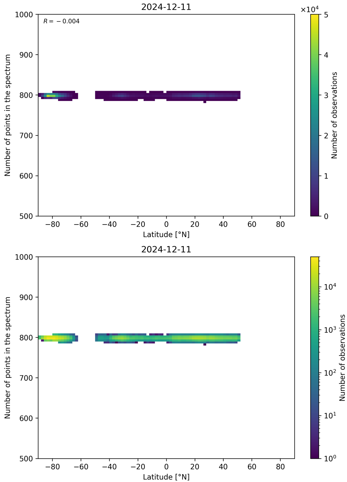
Figure 61: Scatter density plot of “Latitude” against “Number of points in the spectrum” for 2024-12-11 to 2024-12-12.
