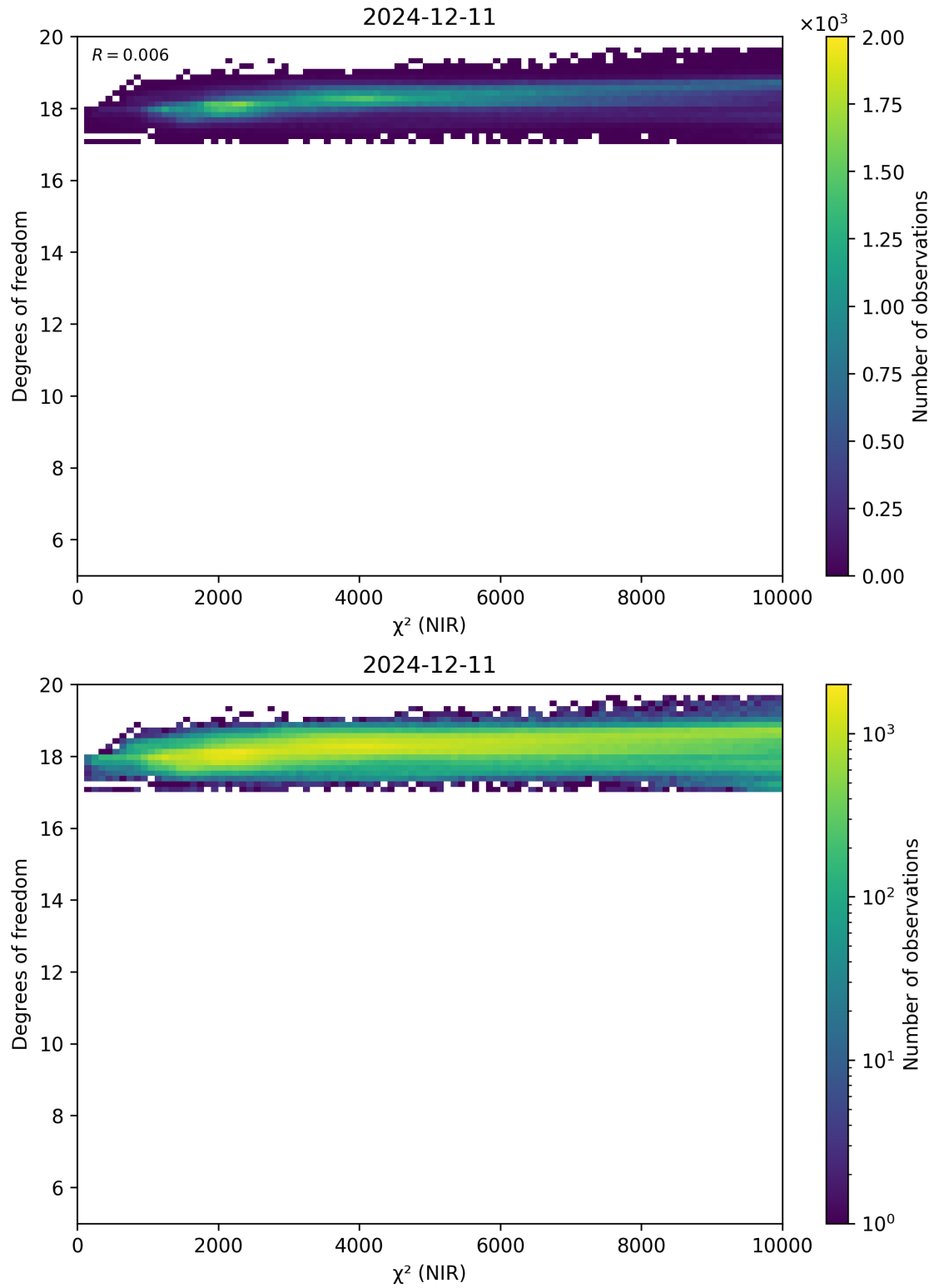
Figure 44: Scatter density plot of “ \chi^2 (NIR)” against “Degrees of freedom” for 2024-12-11 to 2024-12-12.
