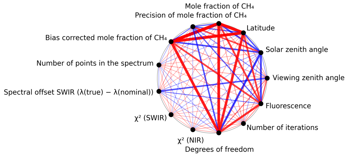
Figure 1: Map of correlation graph for 2024-12-12 to 2024-12-14.
