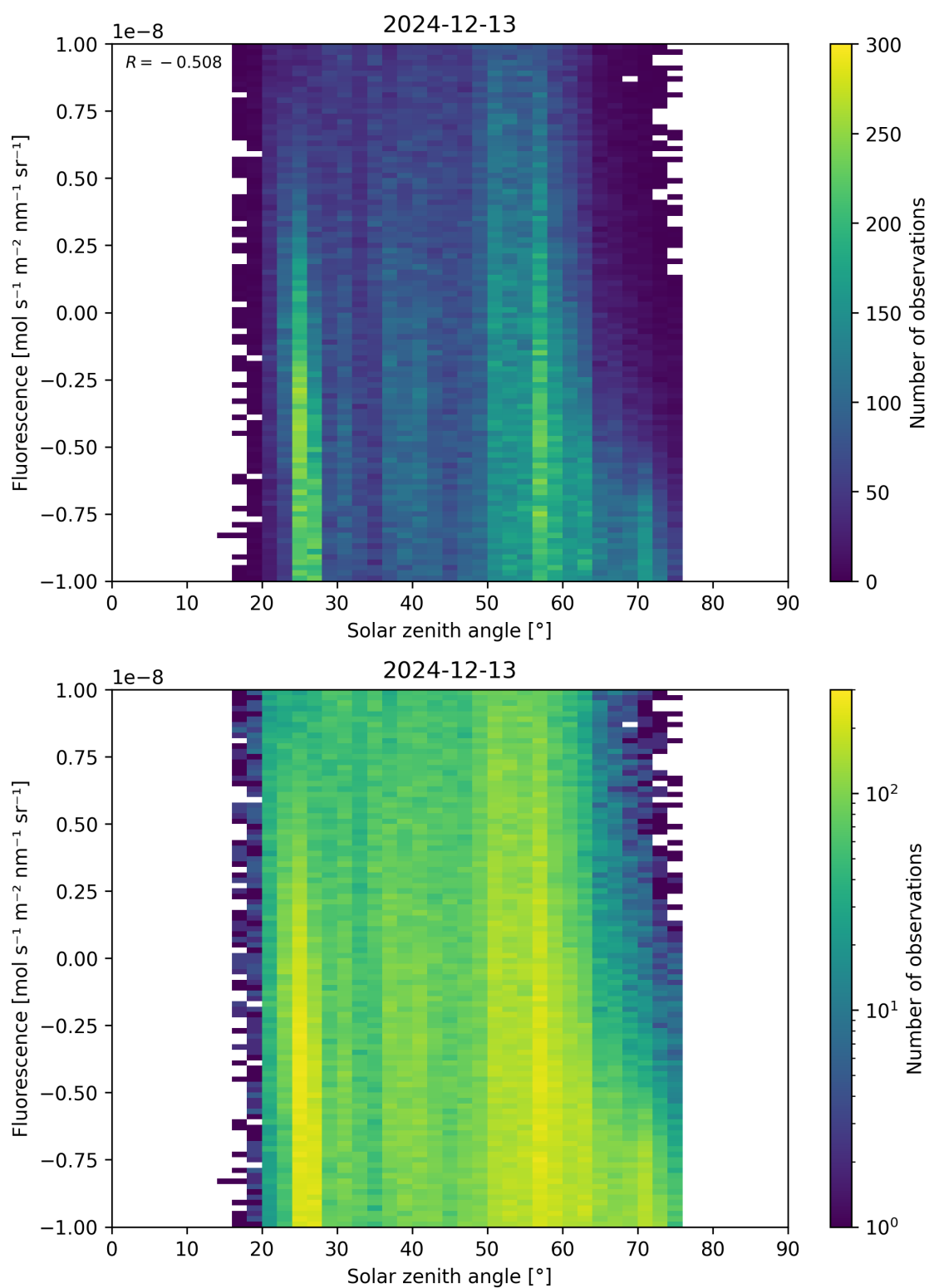
Figure 97: Scatter density plot of “Solar zenith angle” against “Fluorescence” for 2024-12-12 to 2024-12-14.
