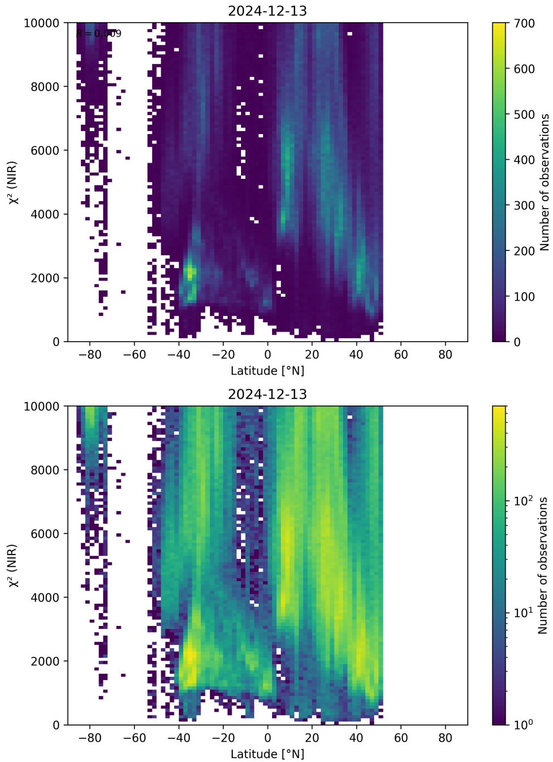
Figure 53: Scatter density plot of “Latitude” against “ \chi^2 (NIR)” for 2024-12-12 to 2024-12-14.
