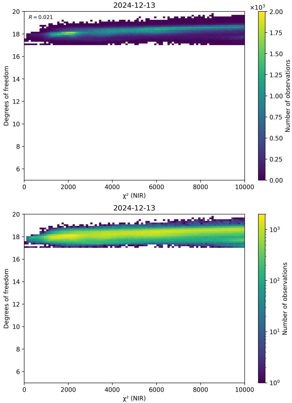
Figure 44: Scatter density plot of “ \chi^2 (NIR)” against “Degrees of freedom” for 2024-12-12 to 2024-12-14.
