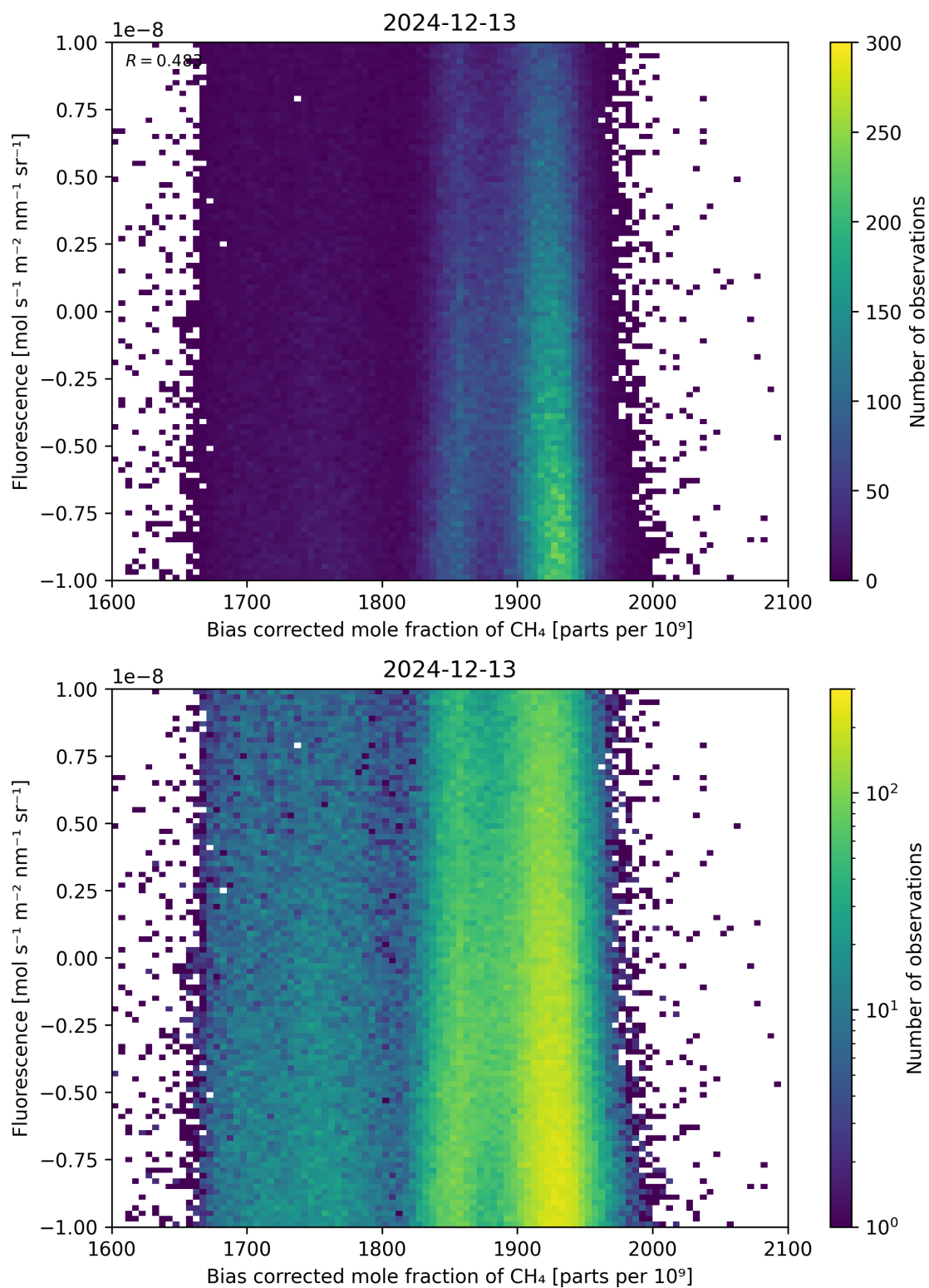
Figure 66: Scatter density plot of “Bias corrected mole fraction of \text{CH}_4 ” against “Fluorescence” for 2024-12-12 to 2024-12-14.
