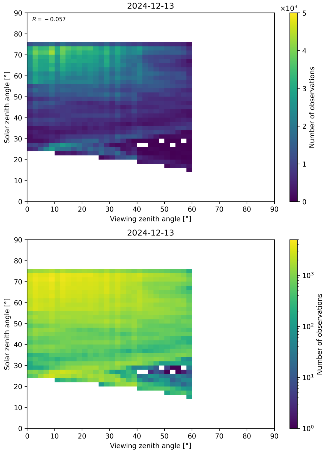
Figure 115: Scatter density plot of “Viewing zenith angle” against “Solar zenith angle” for 2024-12-12 to 2024-12-14.
