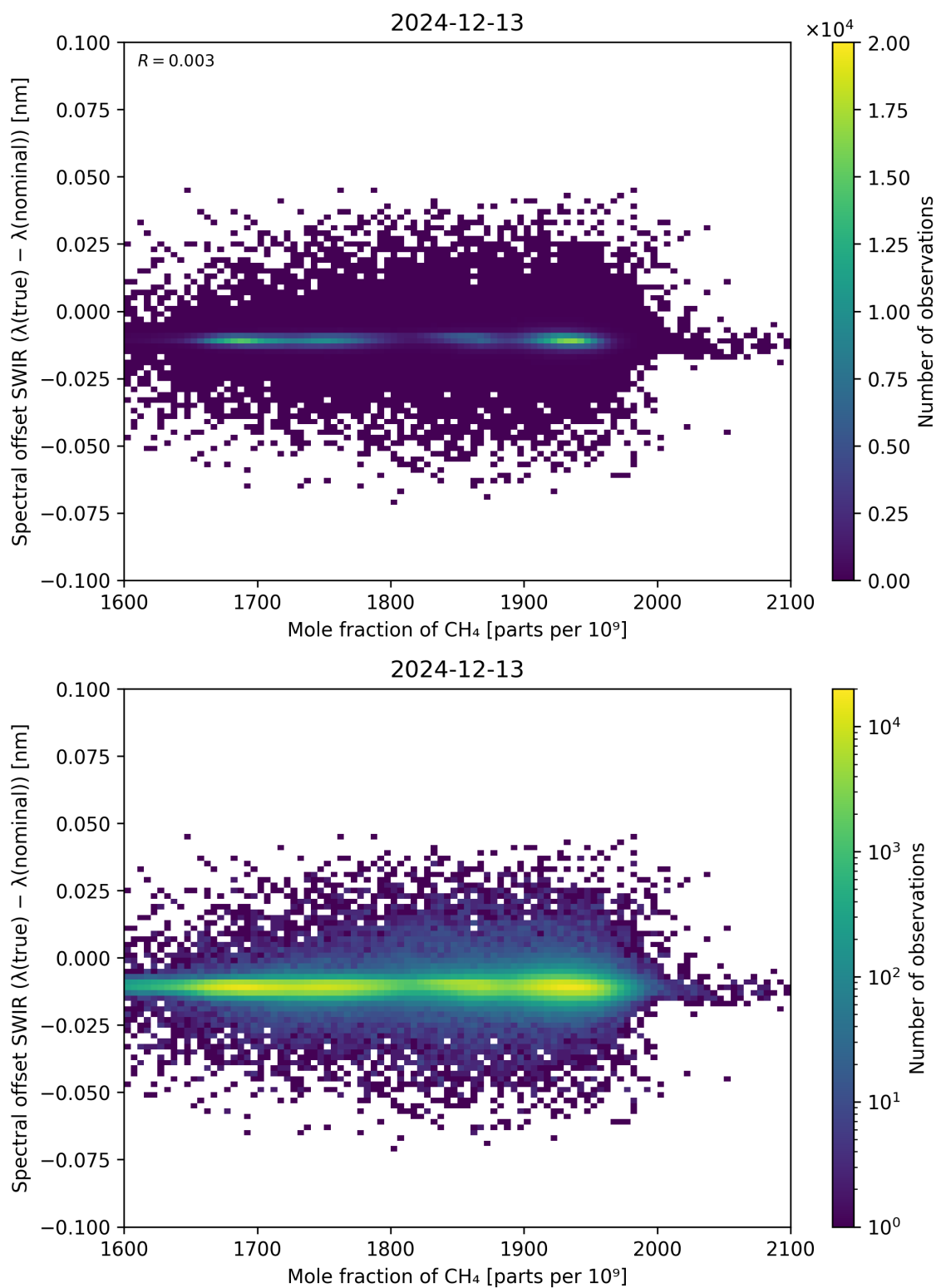
Figure 86: Scatter density plot of “Mole fraction of CH 4 ” against “Spectral offset SWIR ( \lambda_{\text{true}} - \lambda_{\text{nominal}} )” for 2024-12-12 to 2024-12-14.
