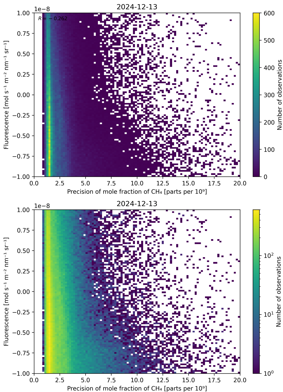
Figure 81: Scatter density plot of “Precision of mole fraction of \text{CH}_4 ” against “Fluorescence” for 2024-12-12 to 2024-12-14.
