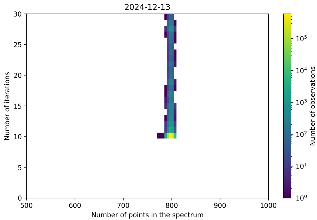
Figure 92: Scatter density plot of “Number of points in the spectrum” against “Number of iterations” for 2024-12-12 to 2024-12-14.
