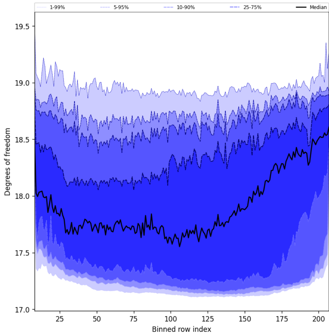
Figure 41: Along track statistics of “Degrees of freedom” for 2024-12-12 to 2024-12-14
