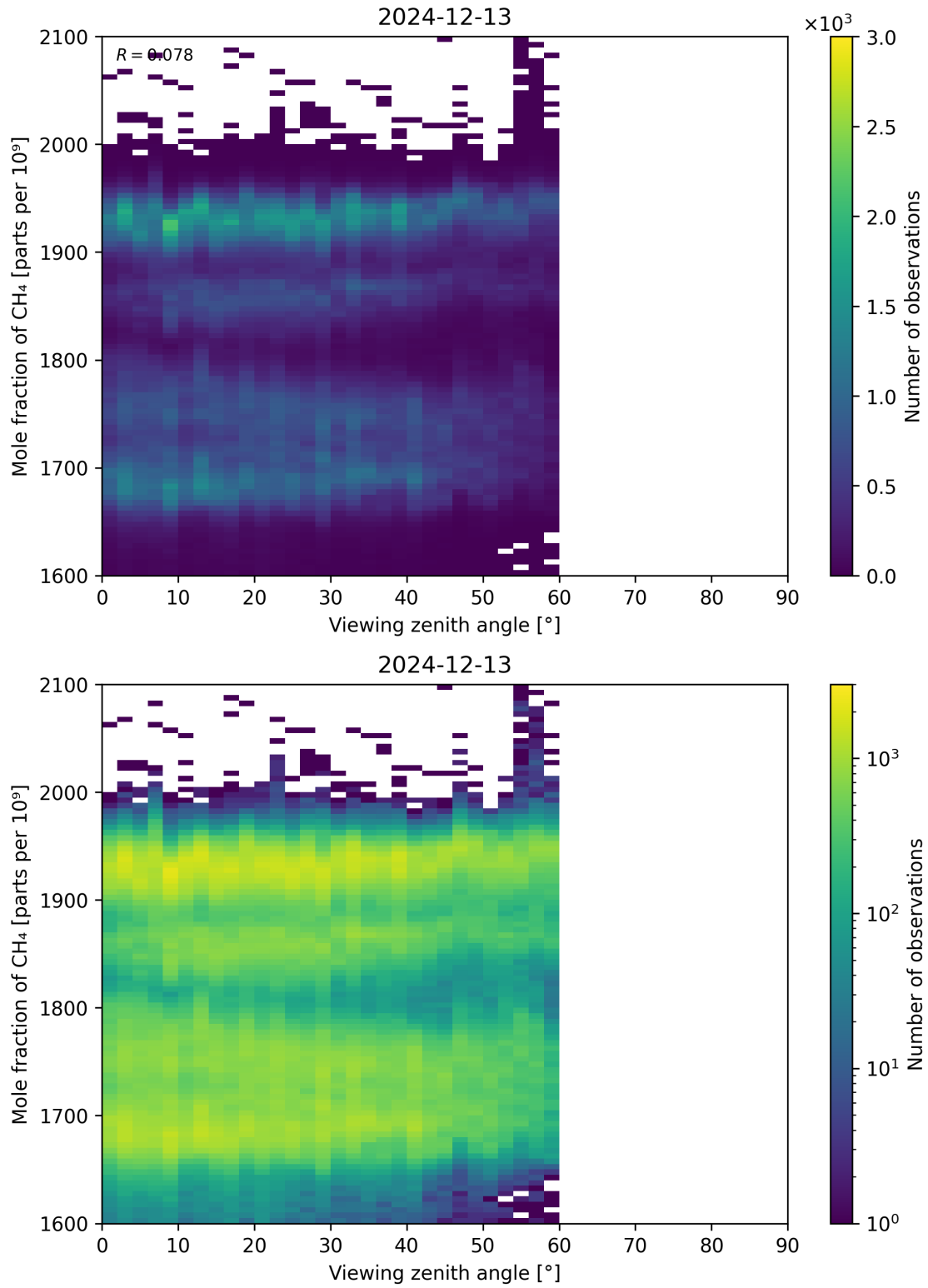
Figure 110: Scatter density plot of “Viewing zenith angle” against “Mole fraction of CH 4 ” for 2024-12-12 to 2024-12-14.
