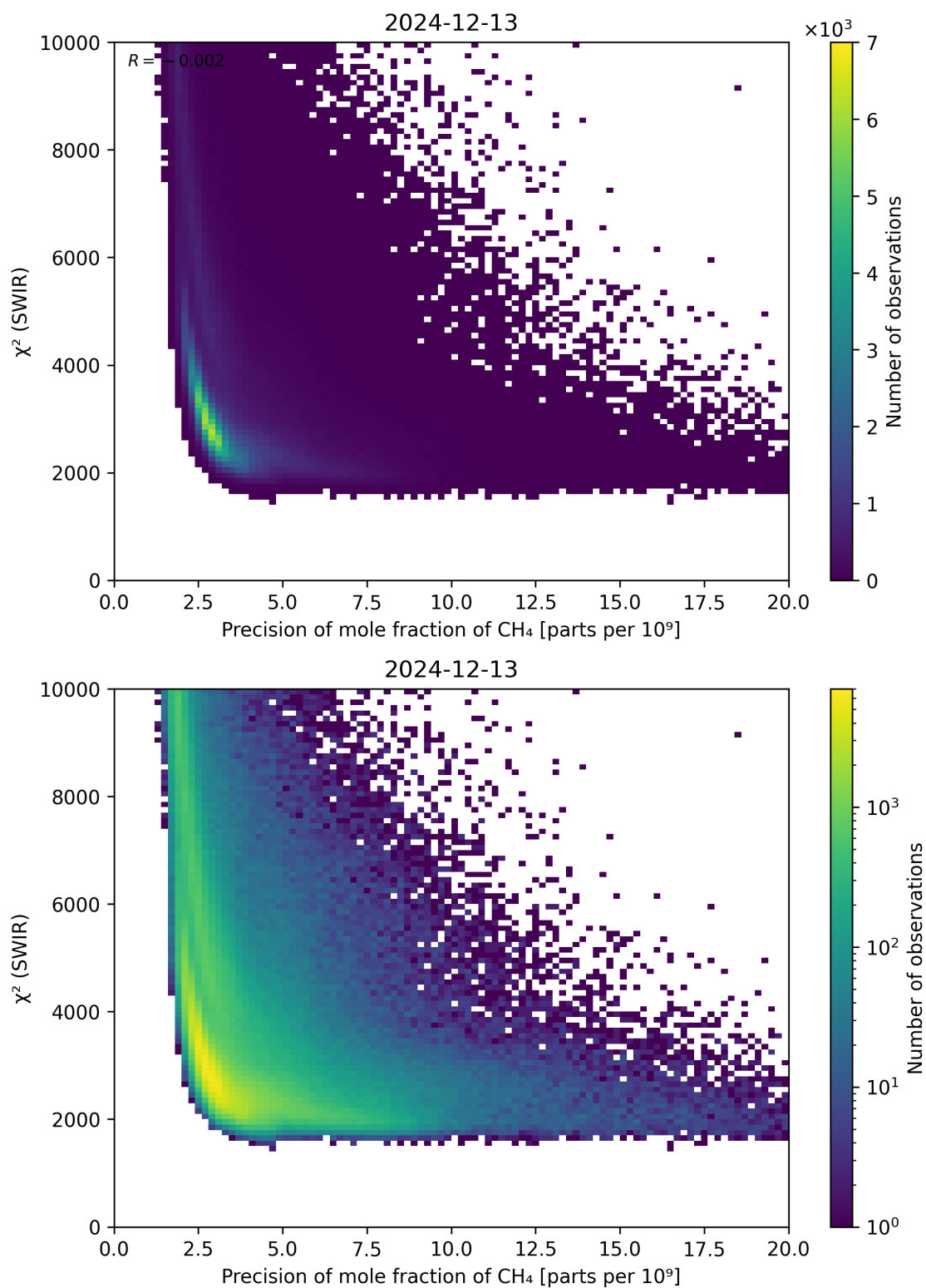
Figure 79: Scatter density plot of “Precision of mole fraction of \text{CH}_4 ” against “ \chi^2 (SWIR)” for 2024-12-12 to 2024-12-14.
