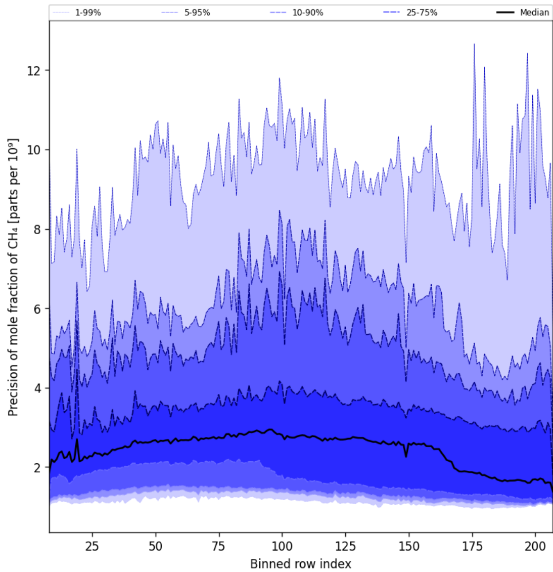
Figure 35: Along track statistics of “Precision of mole fraction of CH 4 ” for 2024-12-12 to 2024-12-14
