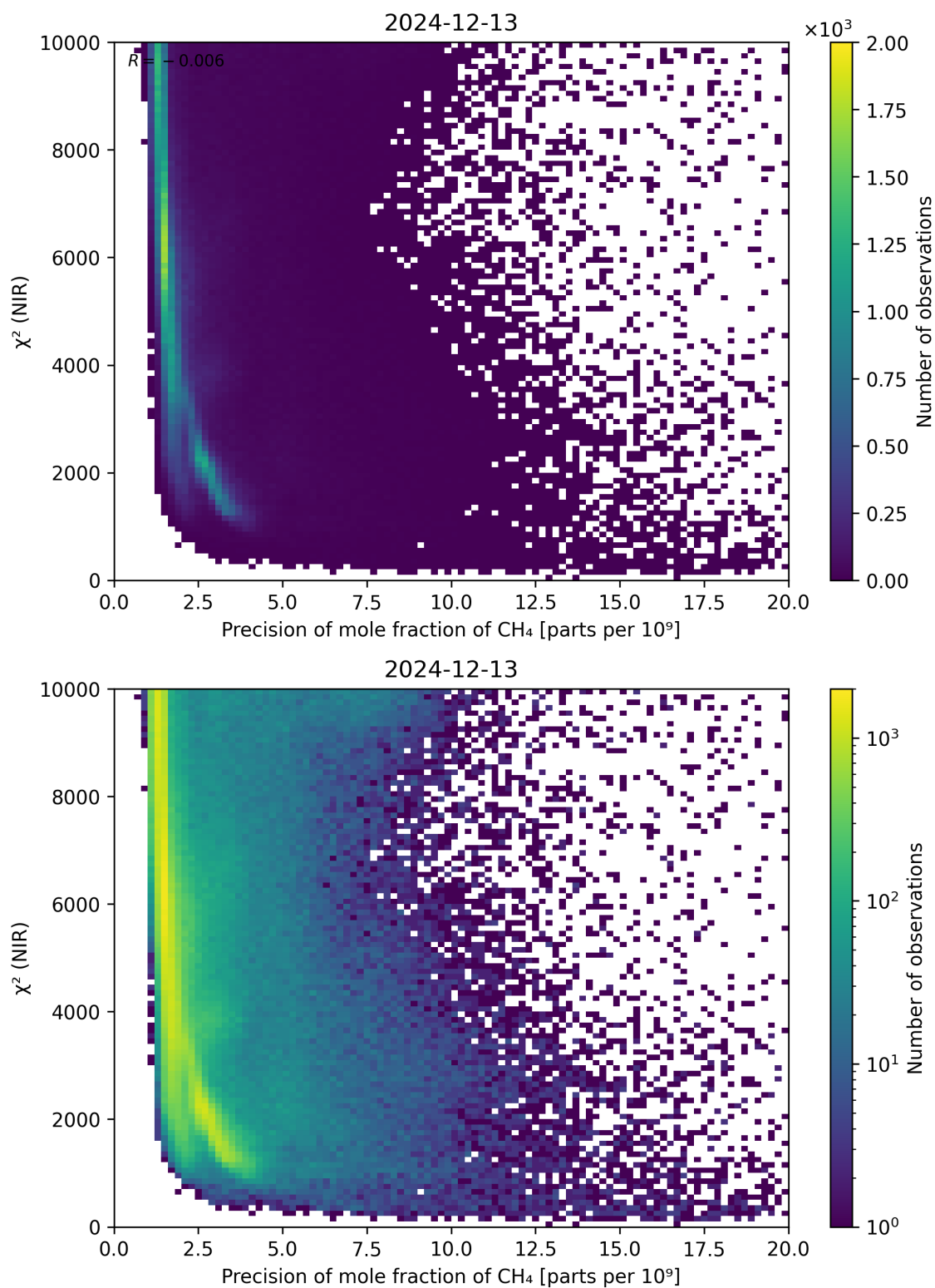
Figure 78: Scatter density plot of “Precision of mole fraction of CH 4 ” against “ \chi^2 (NIR)” for 2024-12-12 to 2024-12-14.
