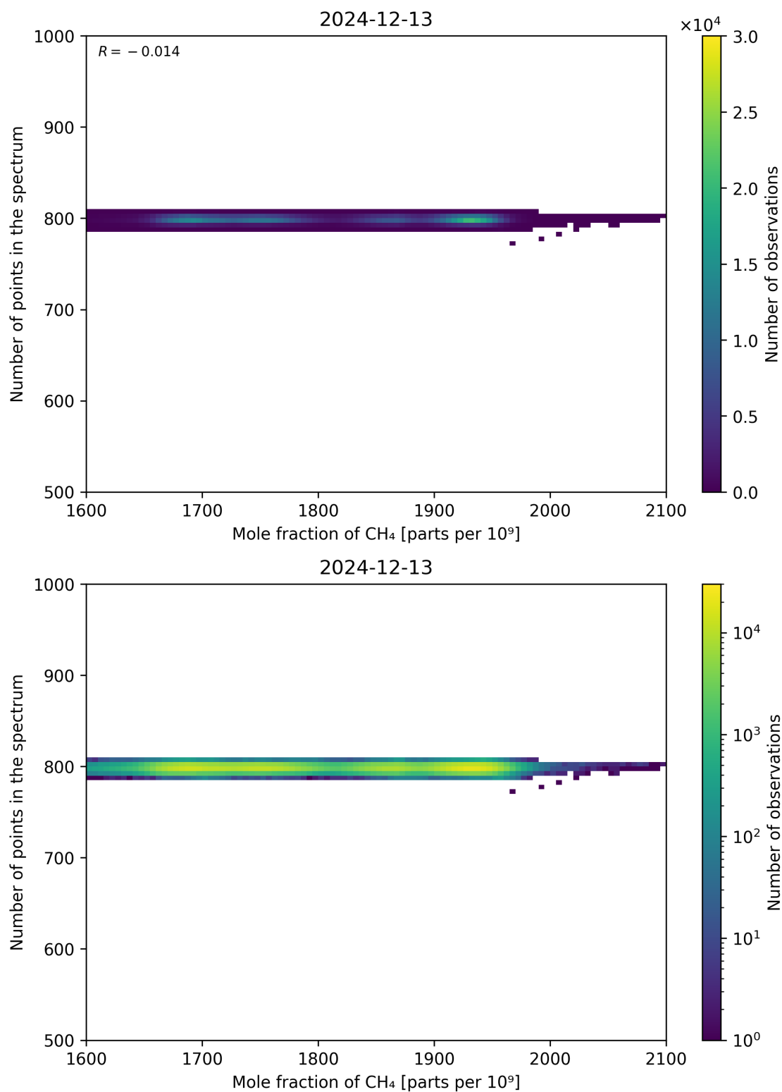
Figure 77: Scatter density plot of “Mole fraction of CH 4 ” against “Number of points in the spectrum” for 2024-12-12 to 2024-12-14.
