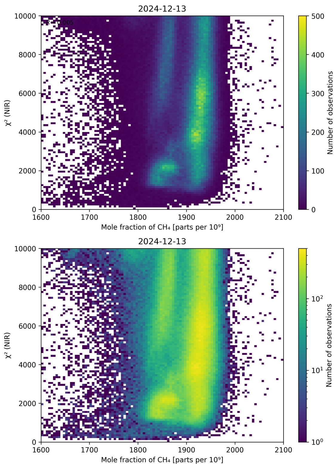
Figure 70: Scatter density plot of “Mole fraction of \text{CH}_4 ” against “ \chi^2 (NIR)” for 2024-12-12 to 2024-12-14.
