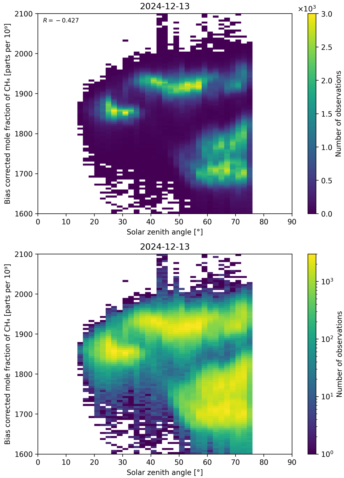
Figure 100: Scatter density plot of “Solar zenith angle” against “Bias corrected mole fraction of \text{CH}_4 ” for 2024-12-12 to 2024-12-14.
