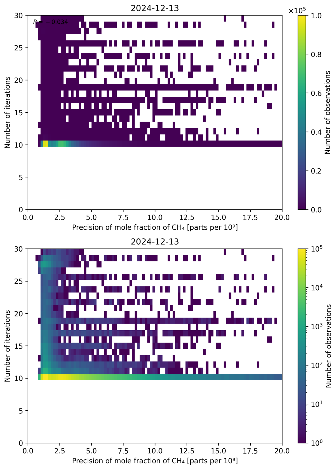
Figure 83: Scatter density plot of “Precision of mole fraction of CH 4 ” against “Number of iterations” for 2024-12-12 to 2024-12-14.
