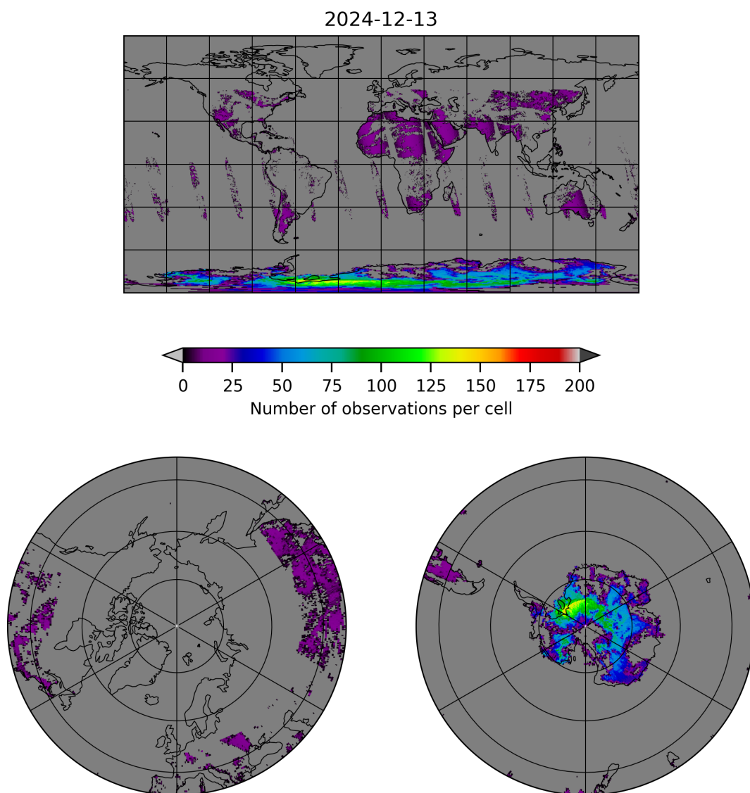
Figure 10: Map of the number of observations for 2024-12-12 to 2024-12-14
