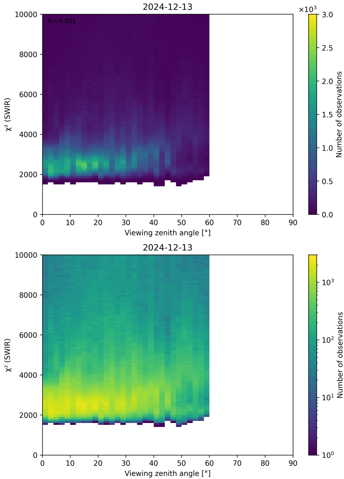
Figure 106: Scatter density plot of “Viewing zenith angle” against “ \chi^2 (SWIR)” for 2024-12-12 to 2024-12-14.
