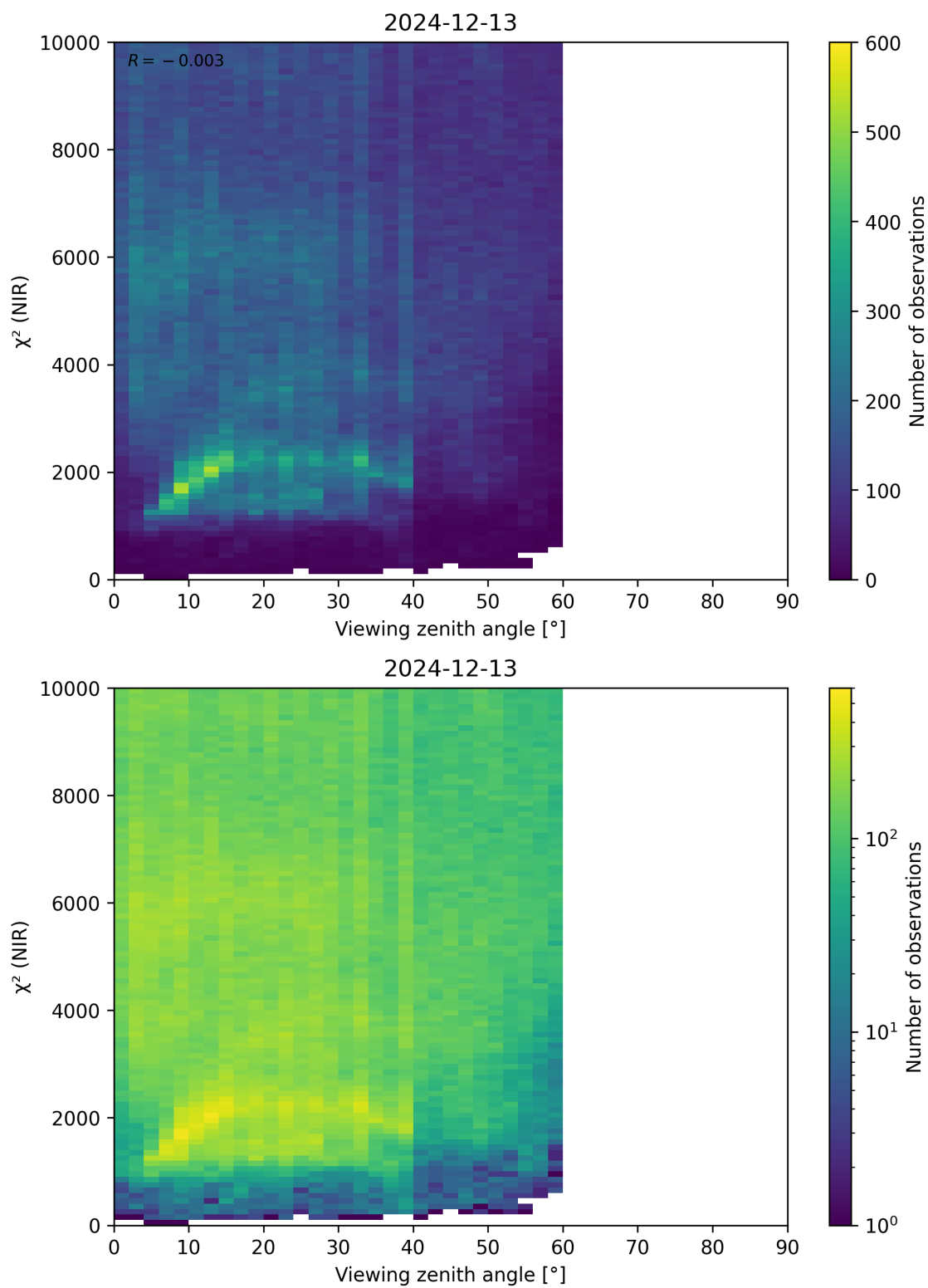
Figure 105: Scatter density plot of “Viewing zenith angle” against “ \chi^2 (NIR)” for 2024-12-12 to 2024-12-14.
