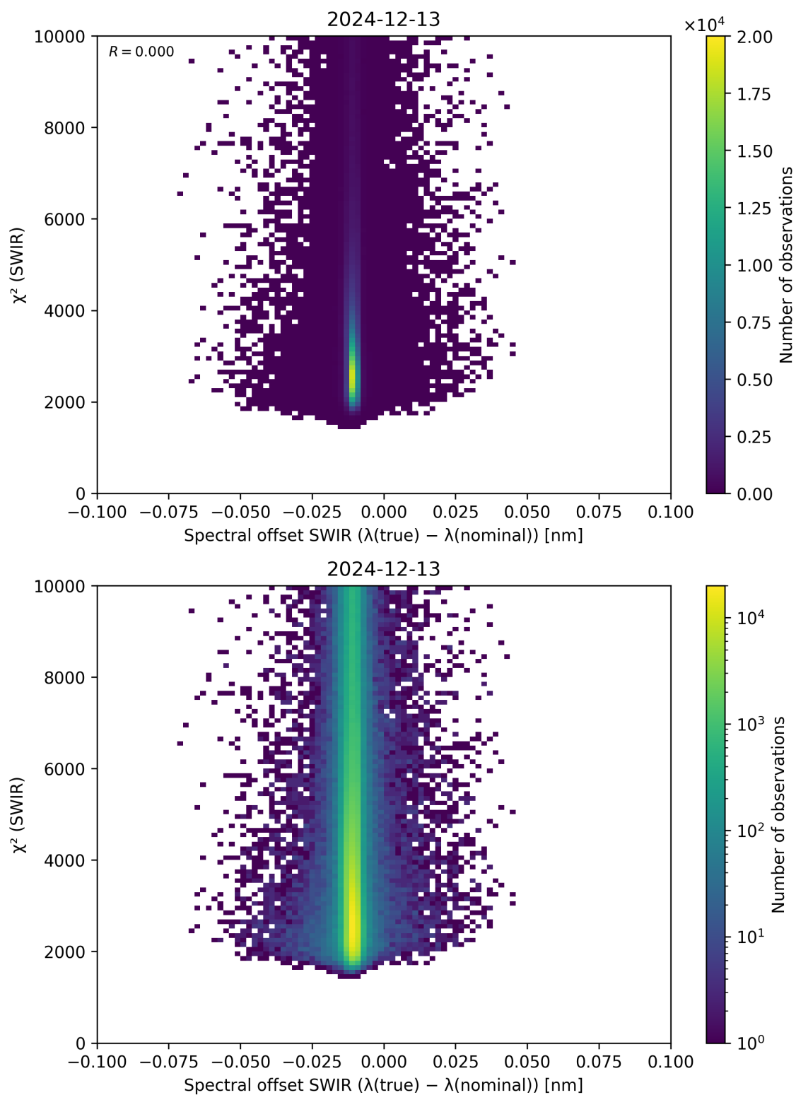
Figure 118: Scatter density plot of “Spectral offset SWIR ( \lambda_{\text{true}} - \lambda_{\text{nominal}} )” against “ \chi^2 (SWIR)” for 2024-12-12 to 2024-12-14.
