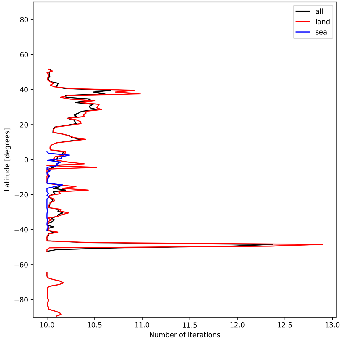
Figure 20: Zonal average of “Number of iterations” for 2024-12-12 to 2024-12-14.
