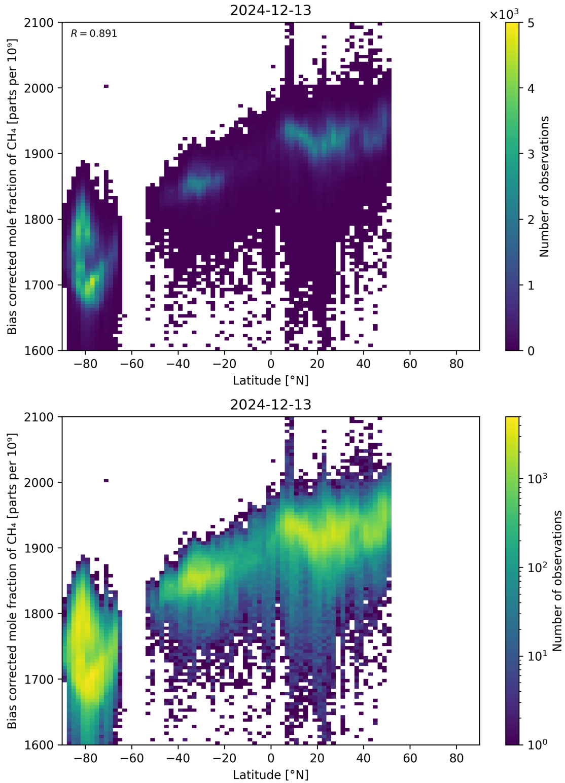
Figure 58: Scatter density plot of “Latitude” against “Bias corrected mole fraction of CH 4 ” for 2024-12-12 to 2024-12-14.
