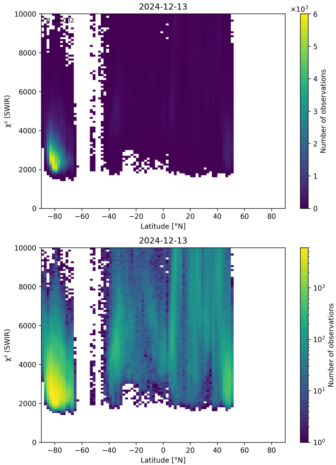
Figure 54: Scatter density plot of “Latitude” against “ \chi^2 (SWIR)” for 2024-12-12 to 2024-12-14.
