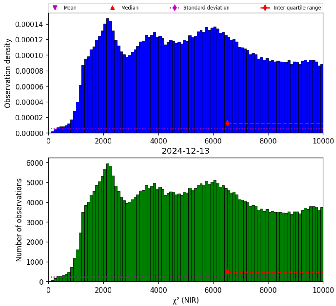
Figure 29: Histogram of “ \chi^2 (NIR)” for 2024-12-12 to 2024-12-14
