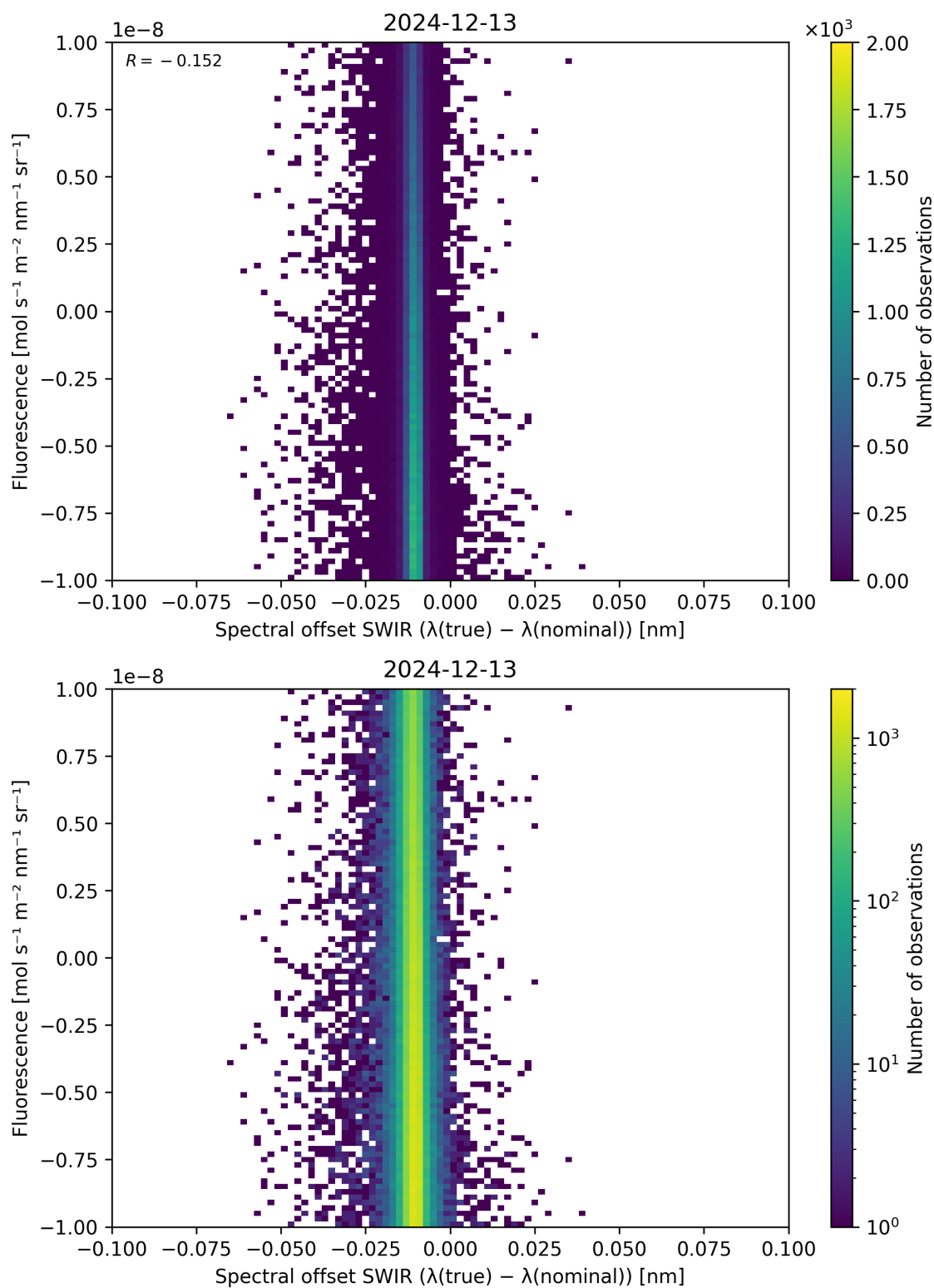
Figure 120: Scatter density plot of “Spectral offset SWIR ( \lambda_{\text{true}} - \lambda_{\text{nominal}} )” against “Fluorescence” for 2024-12-12 to 2024-12-14.
