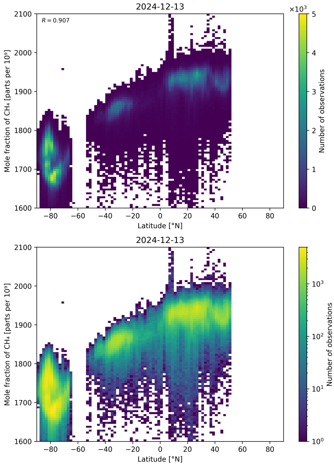
Figure 57: Scatter density plot of “Latitude” against “Mole fraction of CH 4 ” for 2024-12-12 to 2024-12-14.
