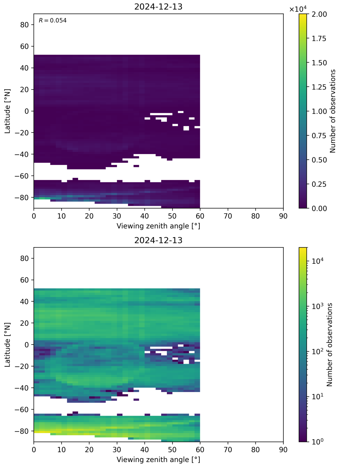
Figure 109: Scatter density plot of “Viewing zenith angle” against “Latitude” for 2024-12-12 to 2024-12-14.
