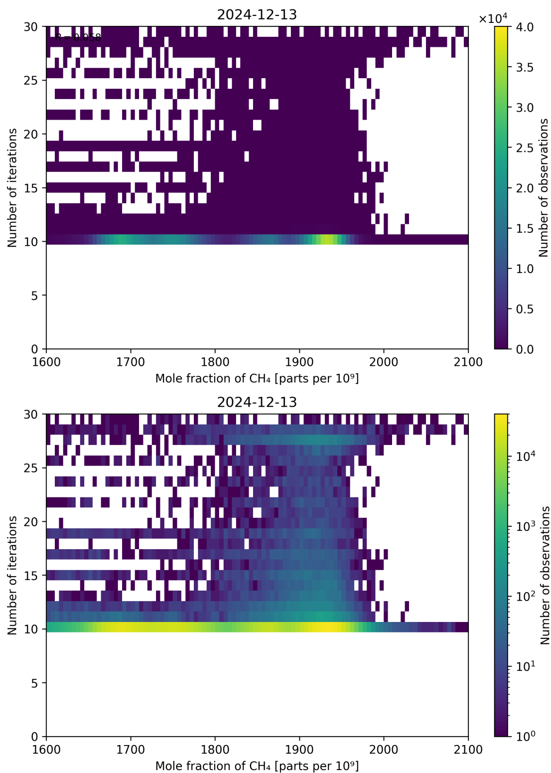
Figure 76: Scatter density plot of “Mole fraction of CH 4 ” against “Number of iterations” for 2024-12-12 to 2024-12-14.
