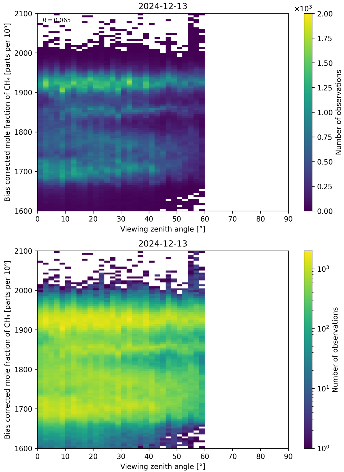
Figure 111: Scatter density plot of “Viewing zenith angle” against “Bias corrected mole fraction of CH 4 ” for 2024-12-12 to 2024-12-14.
