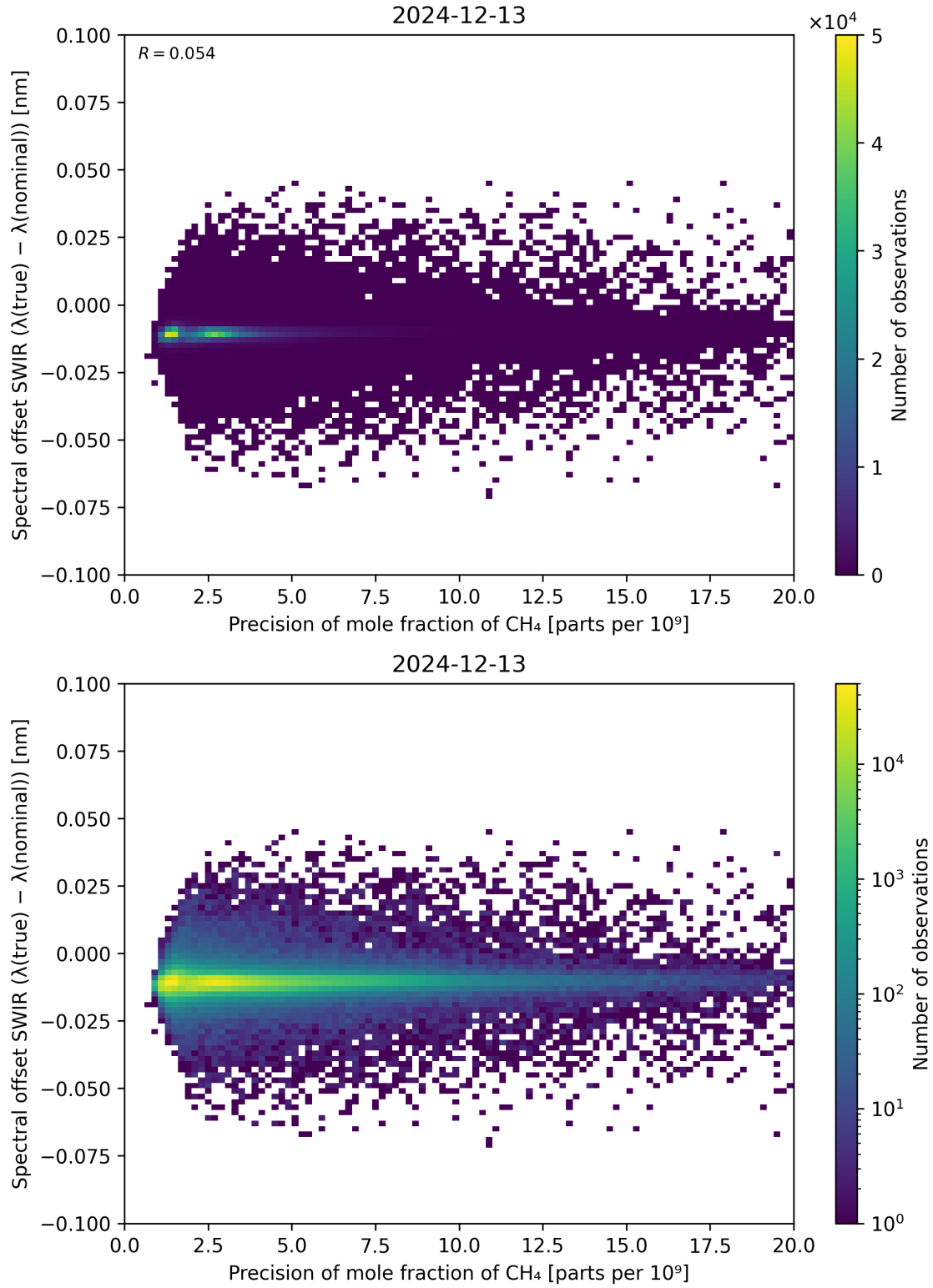
Figure 85: Scatter density plot of “Precision of mole fraction of \text{CH}_4 ” against “Spectral offset SWIR ( \lambda_{\text{true}} - \lambda_{\text{nominal}} )” for 2024-12-12 to 2024-12-14.
