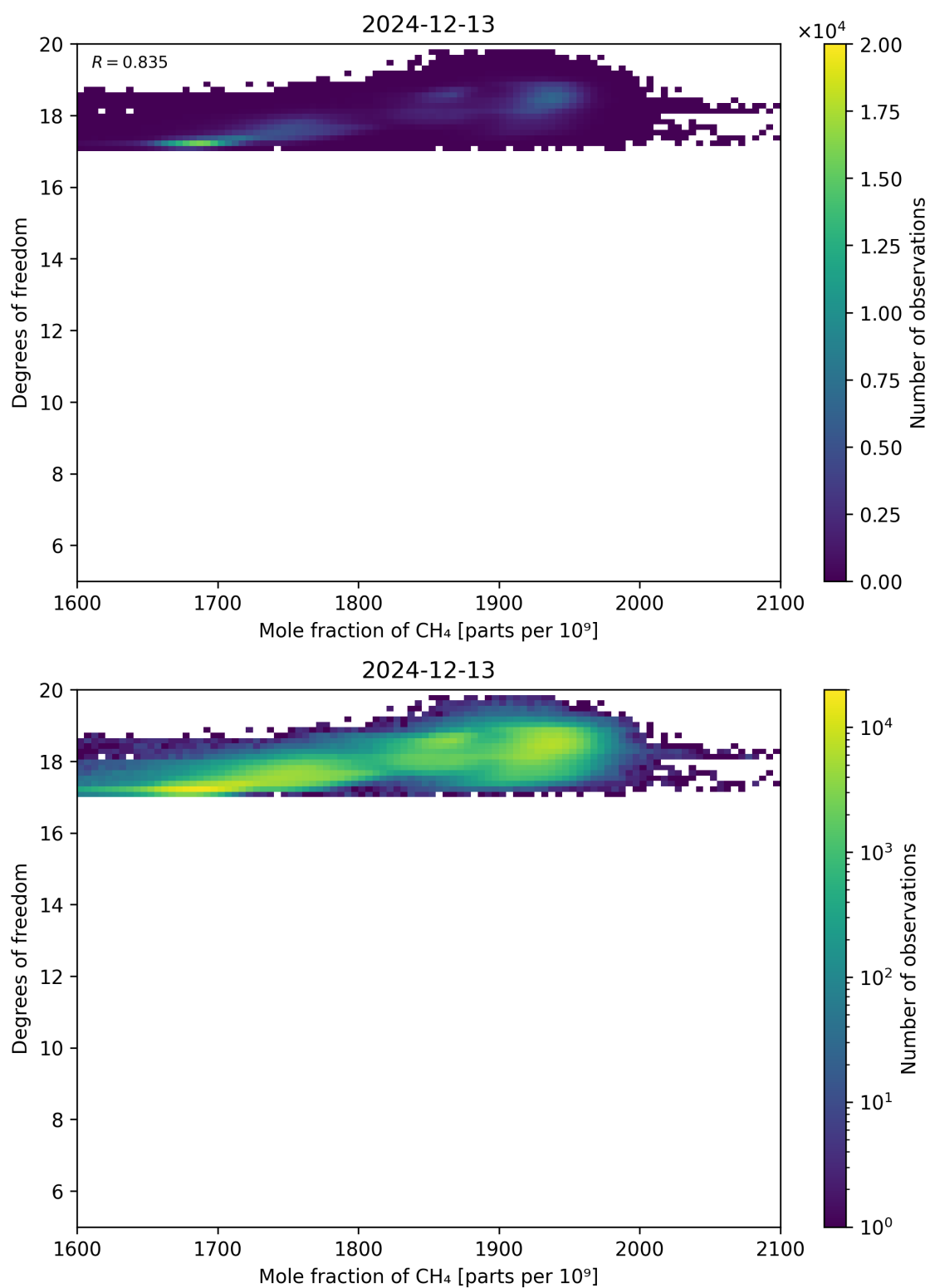
Figure 72: Scatter density plot of “Mole fraction of CH 4 ” against “Degrees of freedom” for 2024-12-12 to 2024-12-14.
