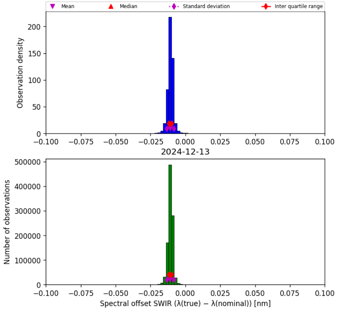
Figure 27: Histogram of “Spectral offset SWIR ( \lambda_{\text{true}} - \lambda_{\text{nominal}} )” for 2024-12-12 to 2024-12-14
