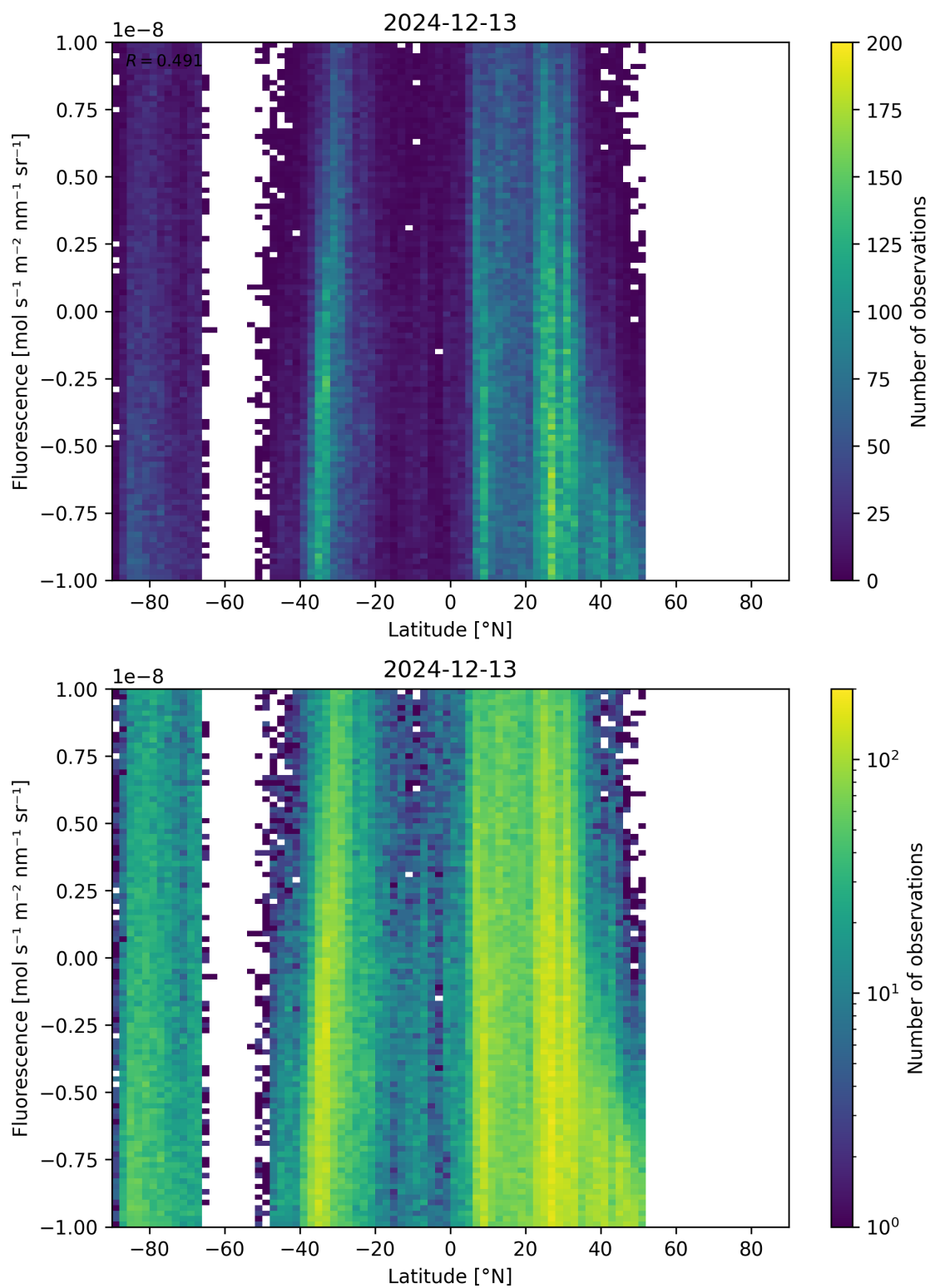
Figure 56: Scatter density plot of “Latitude” against “Fluorescence” for 2024-12-12 to 2024-12-14.
