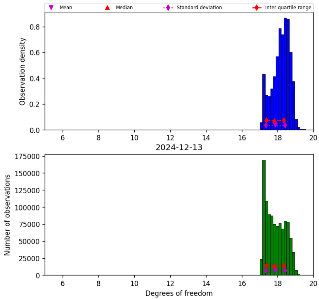
Figure 30: Histogram of “Degrees of freedom” for 2024-12-12 to 2024-12-14
