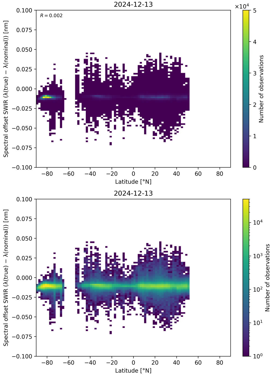
Figure 62: Scatter density plot of “Latitude” against “Spectral offset SWIR ( \lambda_{\text{true}} - \lambda_{\text{nominal}} )” for 2024-12-12 to 2024-12-14.
