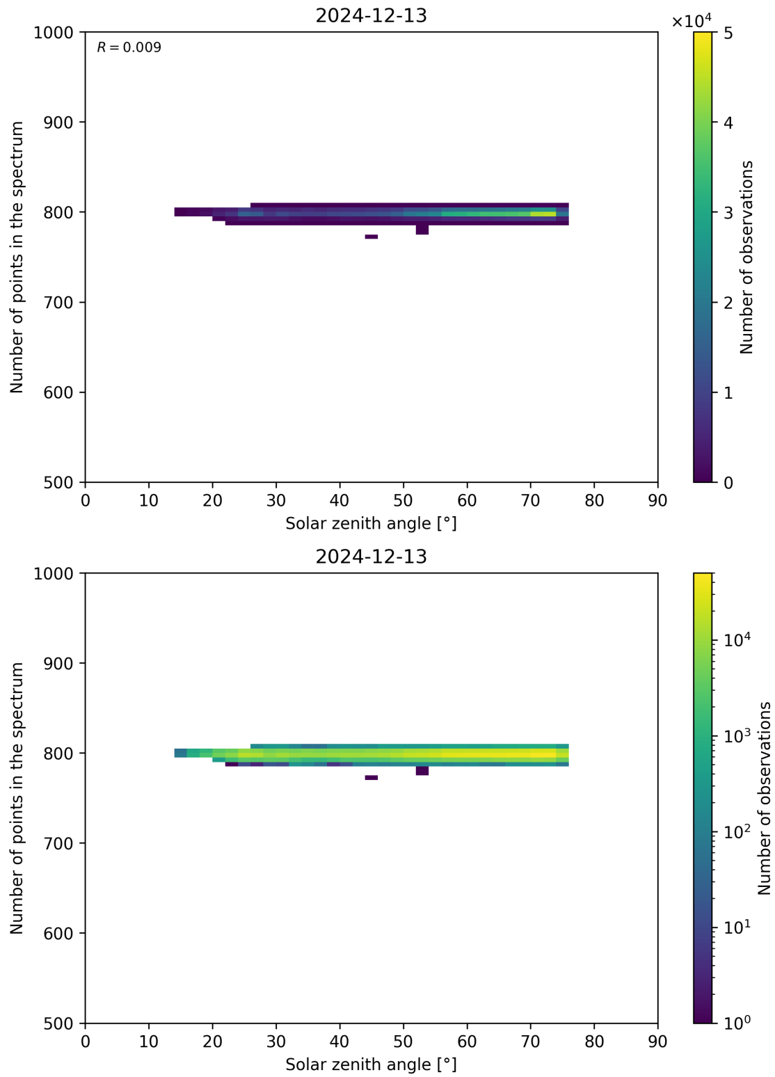
Figure 103: Scatter density plot of “Solar zenith angle” against “Number of points in the spectrum” for 2024-12-12 to 2024-12-14.
