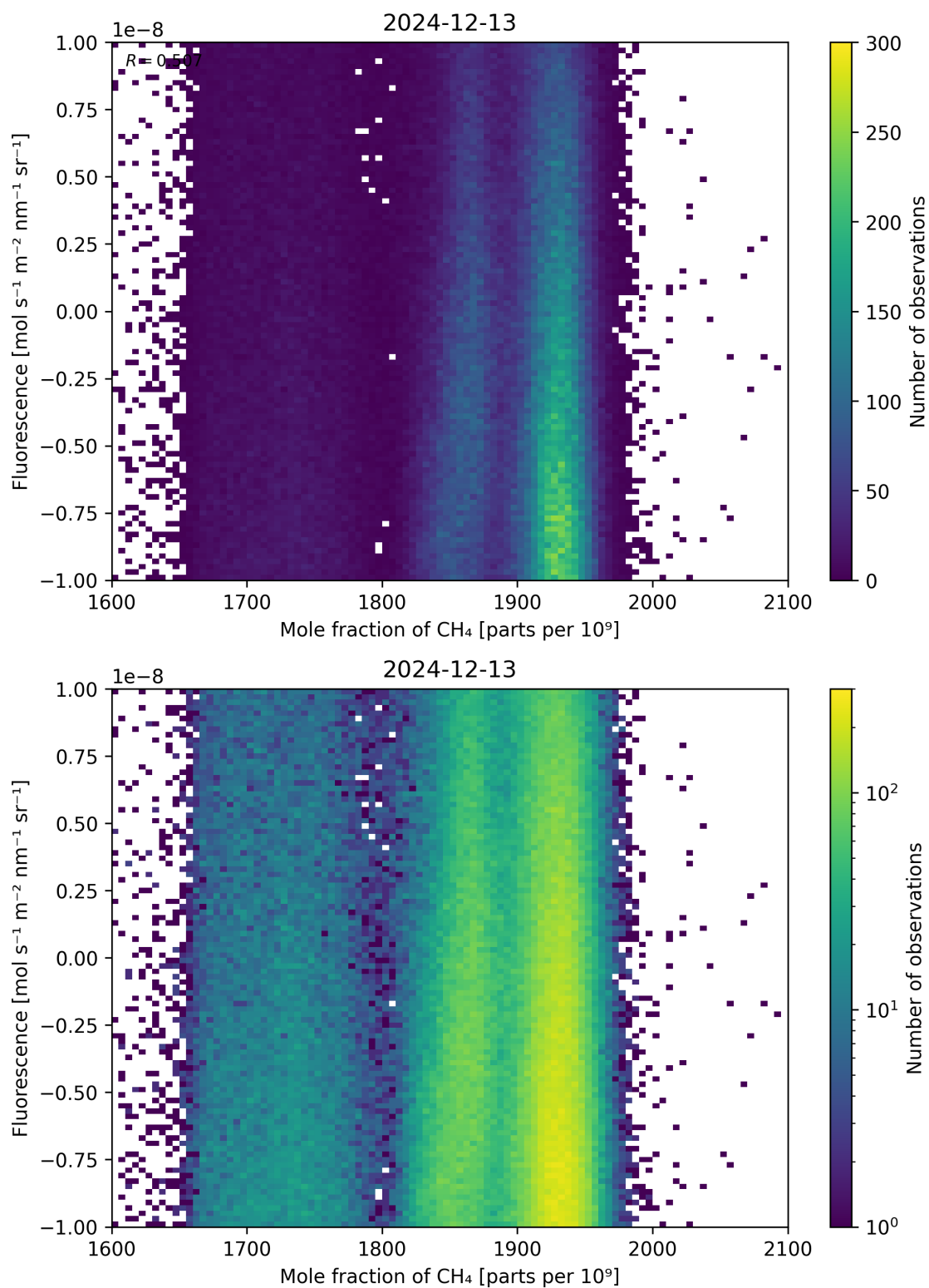
Figure 73: Scatter density plot of “Mole fraction of CH 4 ” against “Fluorescence” for 2024-12-12 to 2024-12-14.
