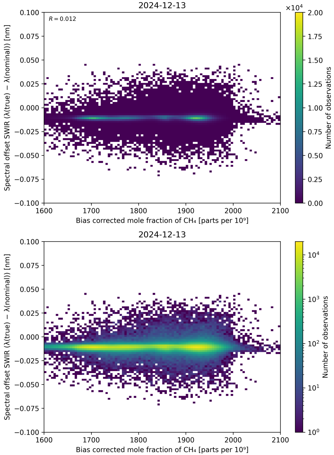
Figure 69: Scatter density plot of “Bias corrected mole fraction of \text{CH}_4 ” against “Spectral offset SWIR ( \lambda_{\text{true}} - \lambda_{\text{nominal}} )” for 2024-12-12 to 2024-12-14.
