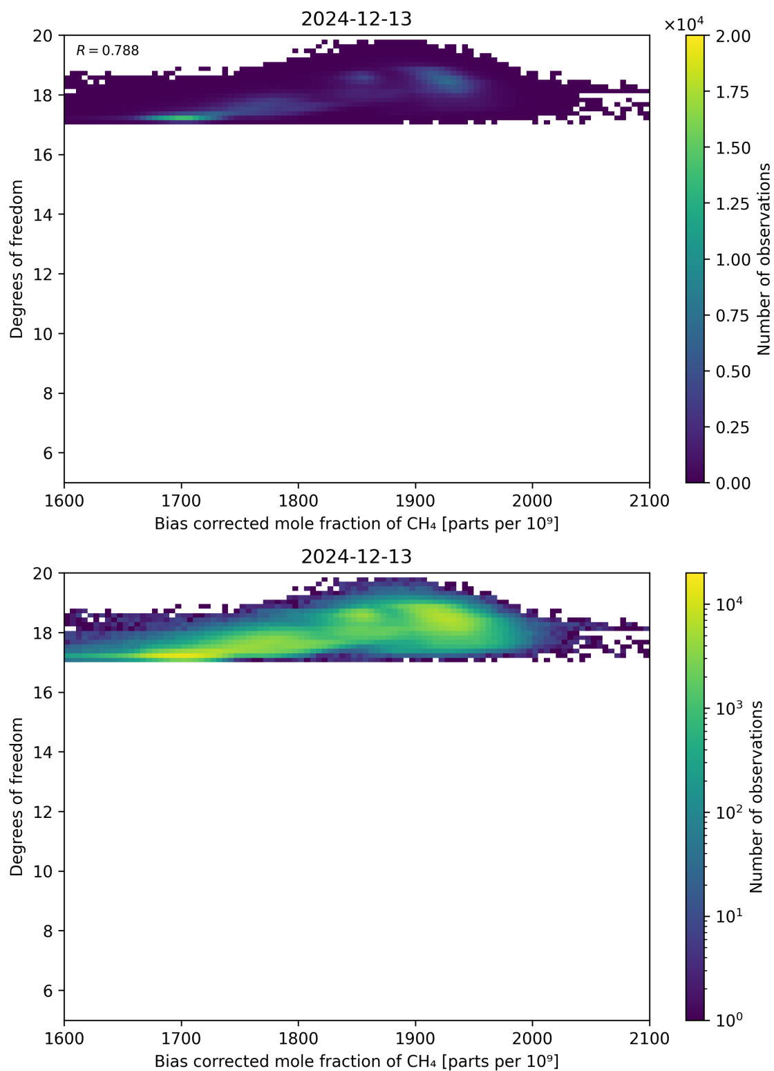
Figure 65: Scatter density plot of “Bias corrected mole fraction of CH 4 ” against “Degrees of freedom” for 2024-12-12 to 2024-12-14.
