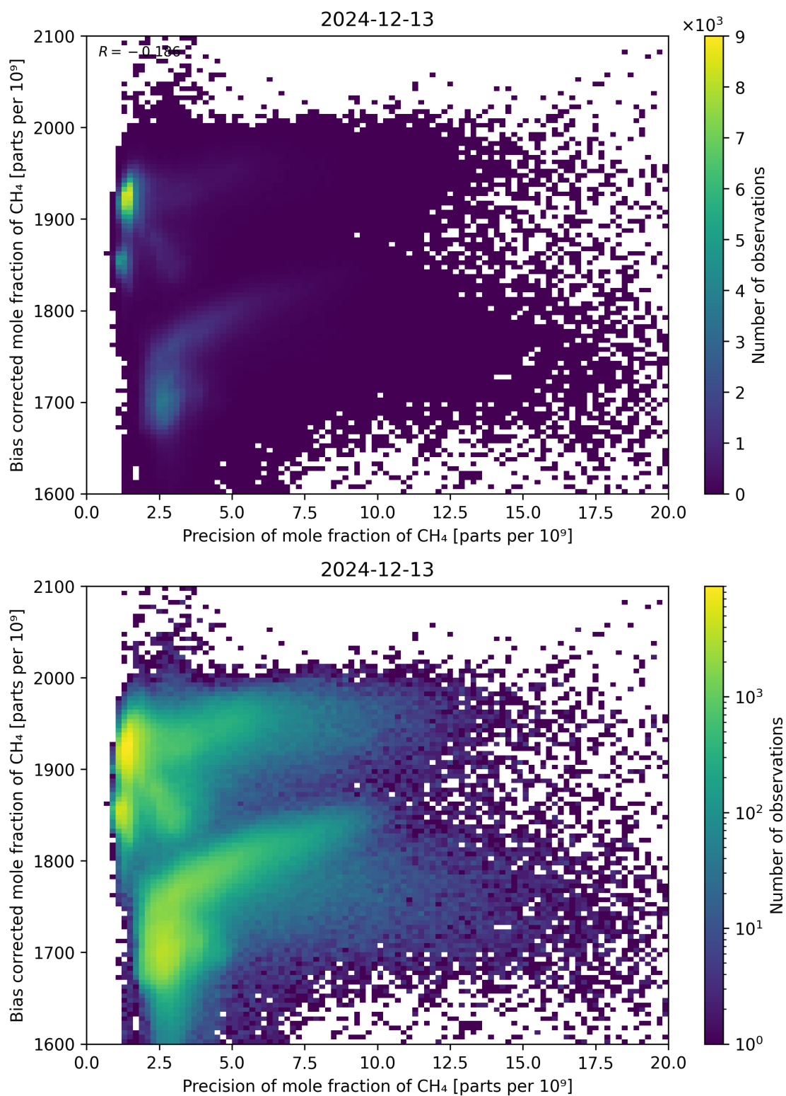
Figure 82: Scatter density plot of “Precision of mole fraction of CH 4 ” against “Bias corrected mole fraction of CH 4 ” for 2024-12-12 to 2024-12-14.
