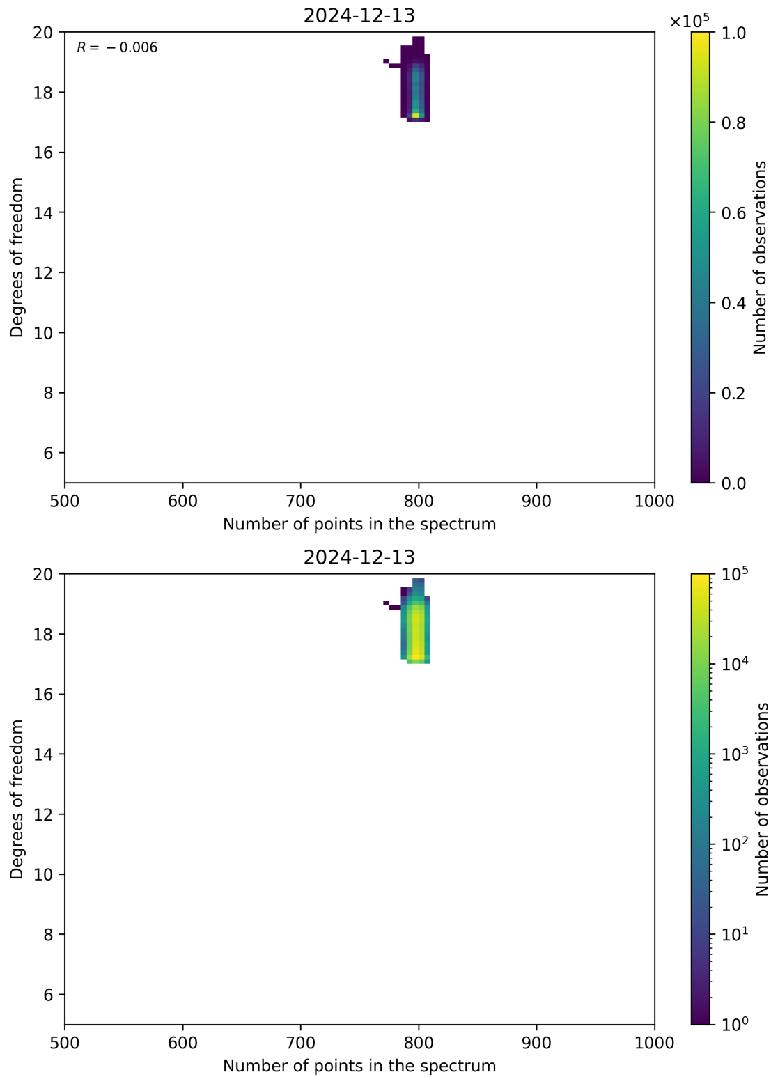
Figure 90: Scatter density plot of “Number of points in the spectrum” against “Degrees of freedom” for 2024-12-12 to 2024-12-14.
