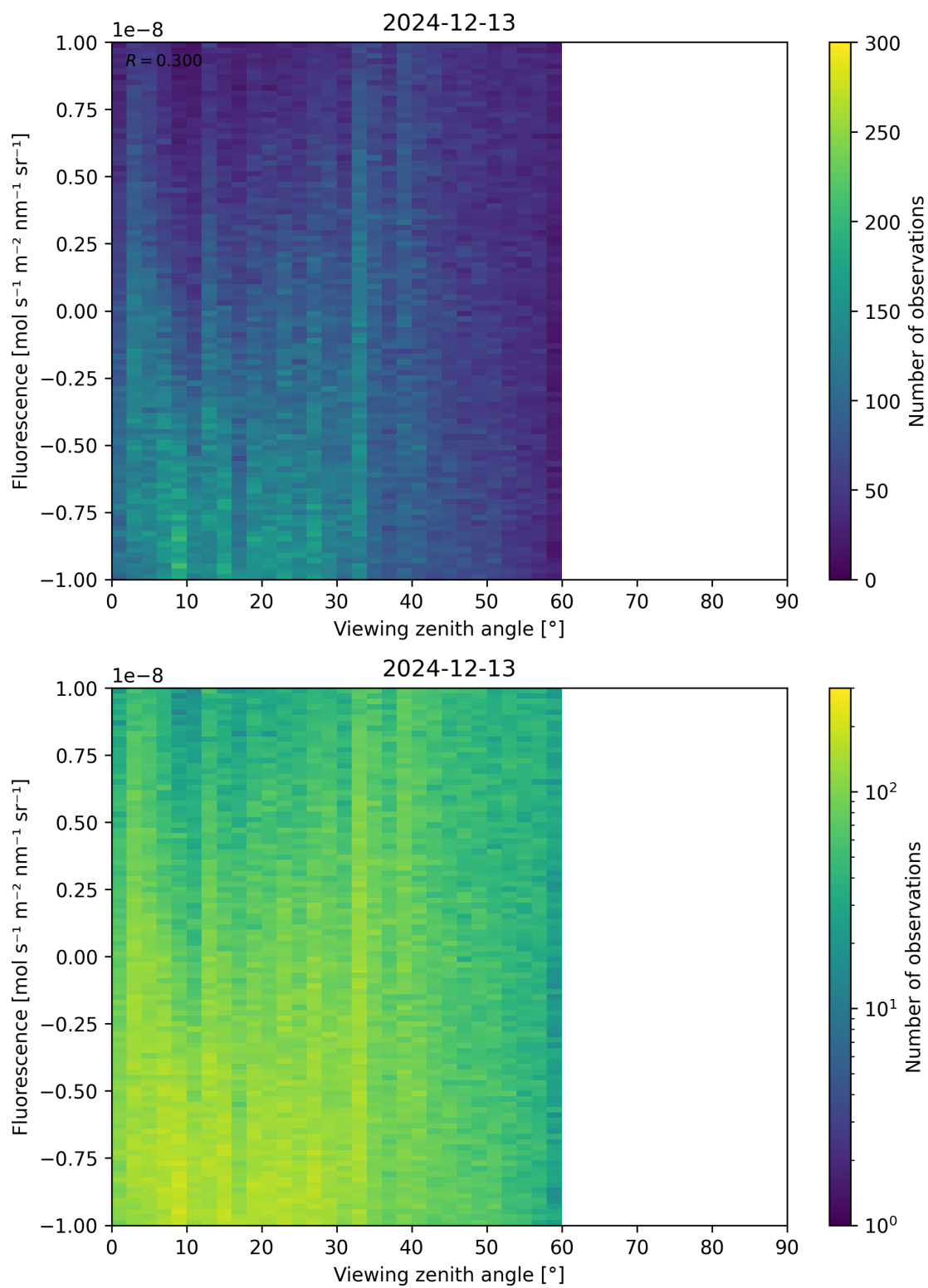
Figure 108: Scatter density plot of “Viewing zenith angle” against “Fluorescence” for 2024-12-12 to 2024-12-14.
