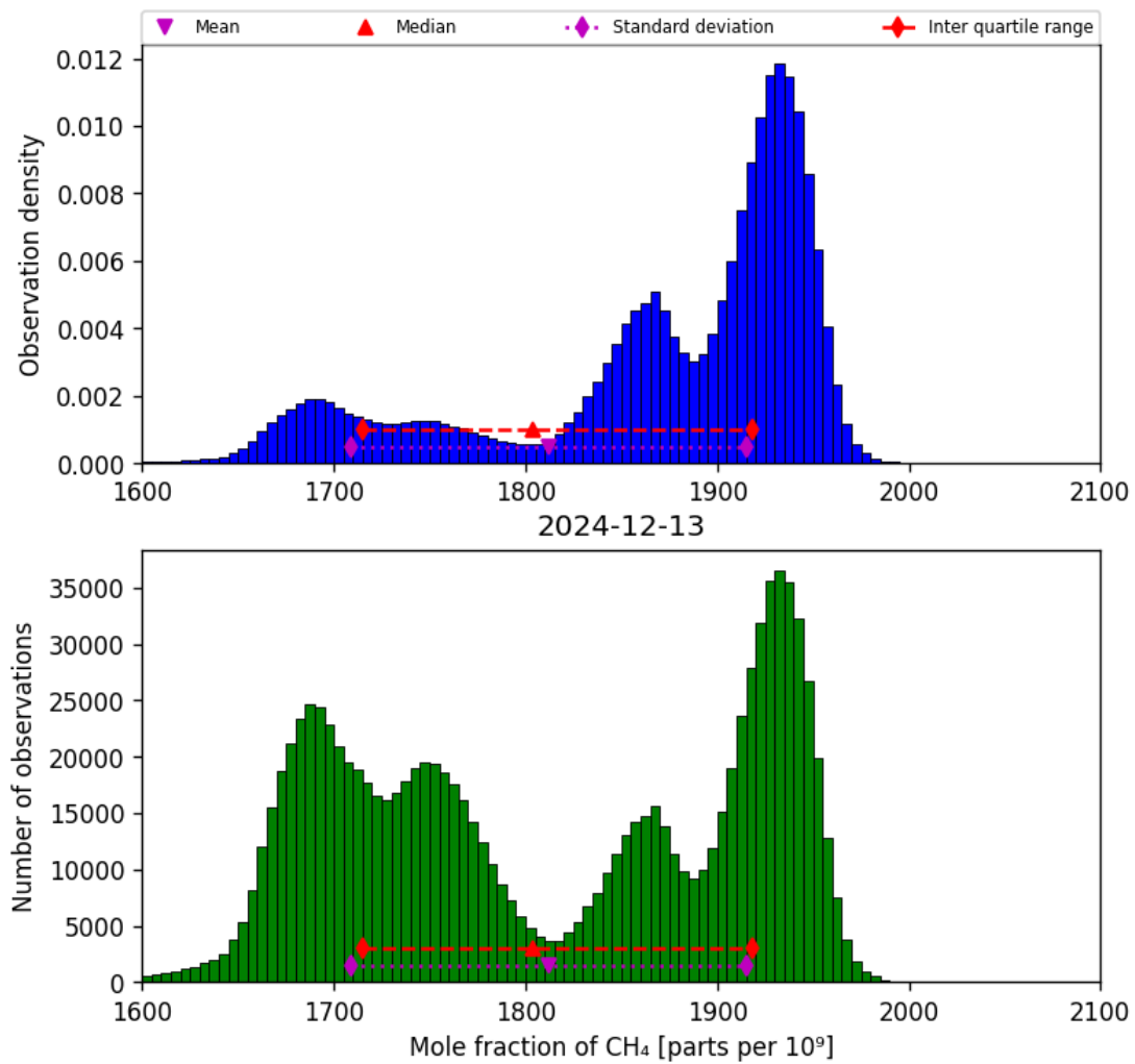
Figure 23: Histogram of “Mole fraction of CH 4 ” for 2024-12-12 to 2024-12-14
