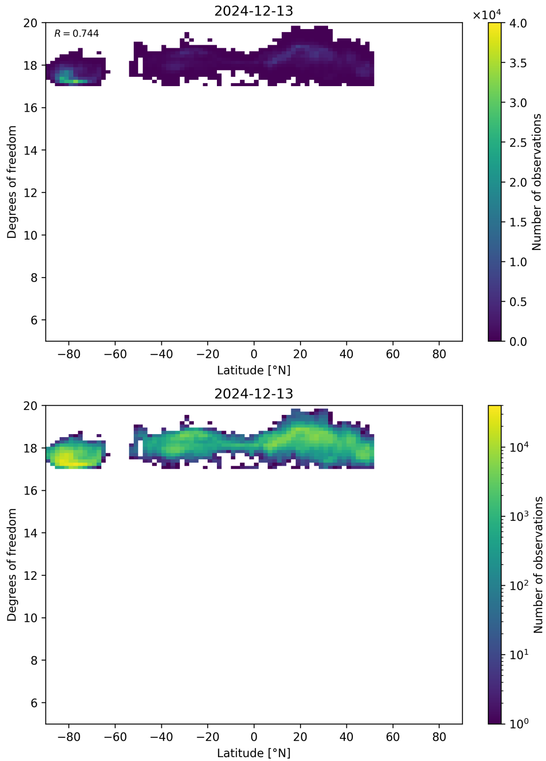
Figure 55: Scatter density plot of “Latitude” against “Degrees of freedom” for 2024-12-12 to 2024-12-14.
