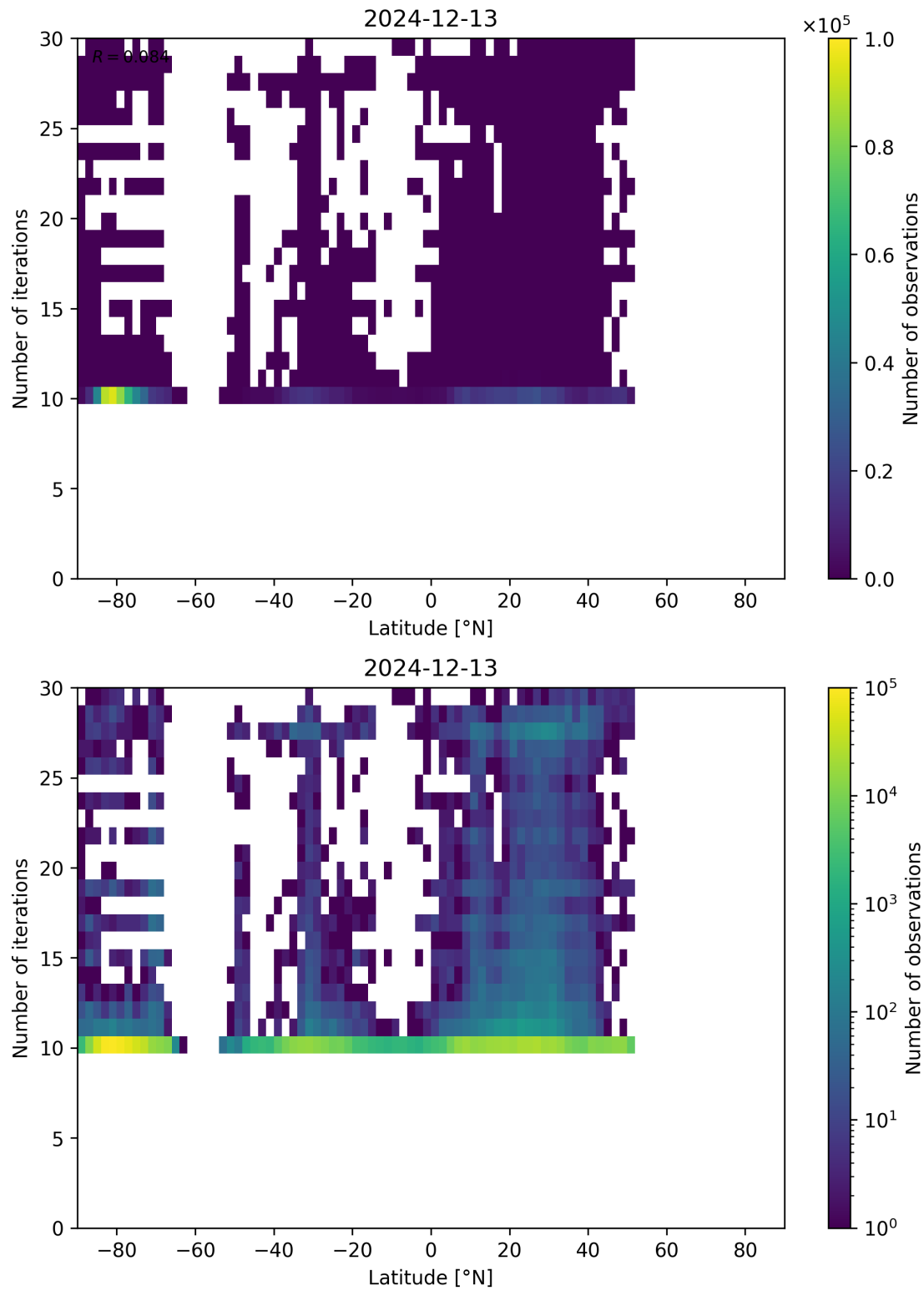
Figure 60: Scatter density plot of “Latitude” against “Number of iterations” for 2024-12-12 to 2024-12-14.
