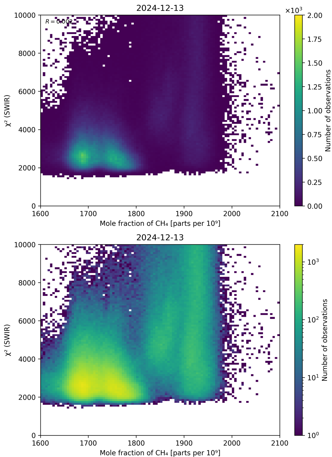
Figure 71: Scatter density plot of “Mole fraction of \text{CH}_4 ” against “ \chi^2 (SWIR)” for 2024-12-12 to 2024-12-14.
