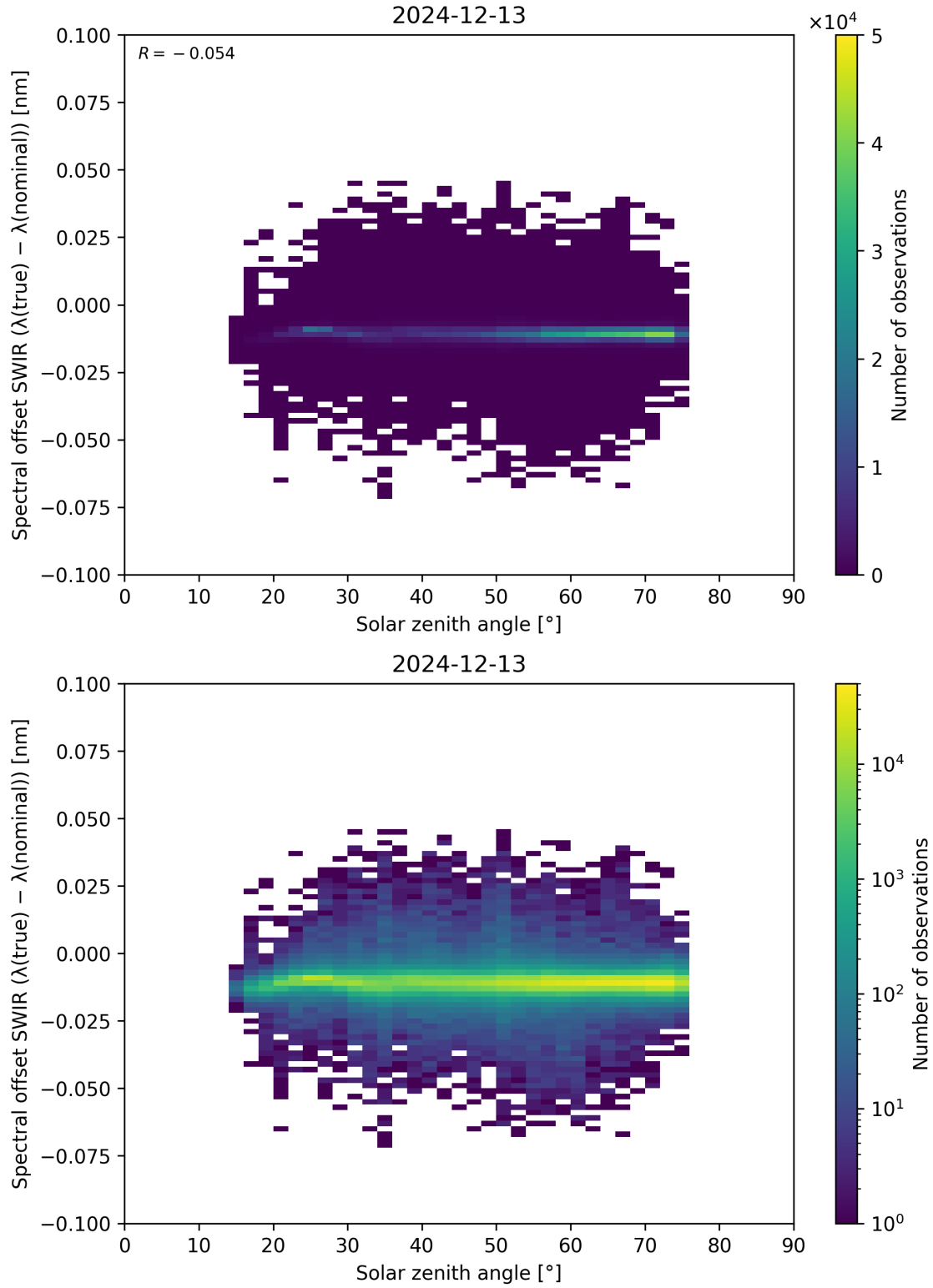
Figure 104: Scatter density plot of “Solar zenith angle” against “Spectral offset SWIR ( \lambda_{\text{true}} - \lambda_{\text{nominal}} )” for 2024-12-12 to 2024-12-14.
