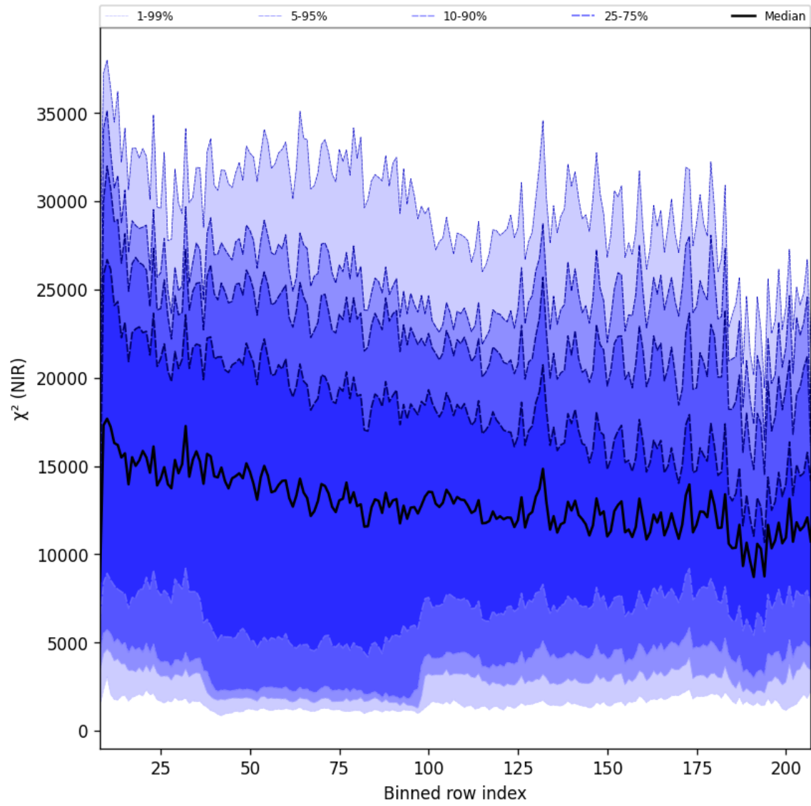
Figure 40: Along track statistics of “ \chi^2 (NIR)” for 2024-12-12 to 2024-12-14
