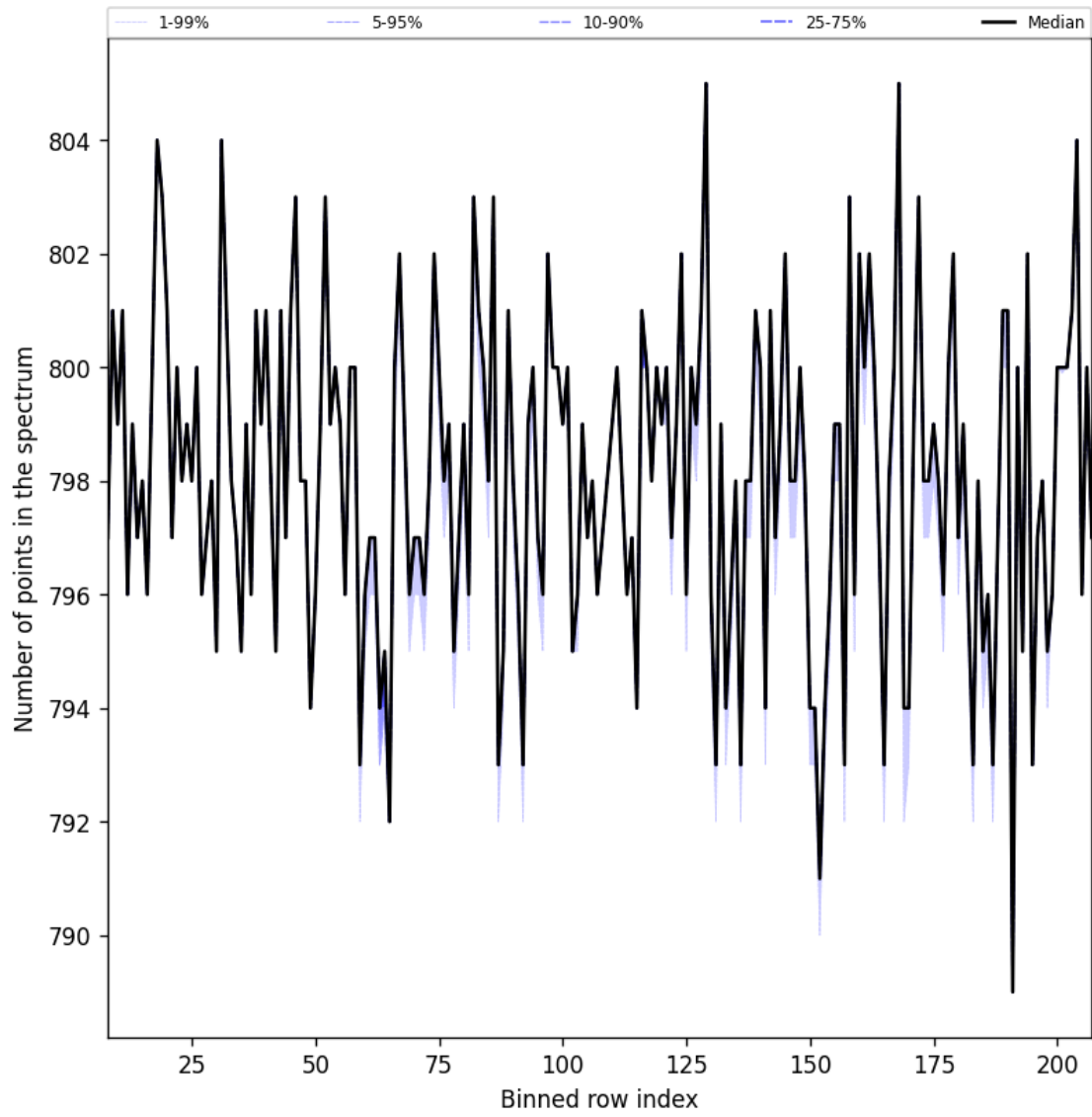
Figure 37: Along track statistics of “Number of points in the spectrum” for 2024-12-12 to 2024-12-14
