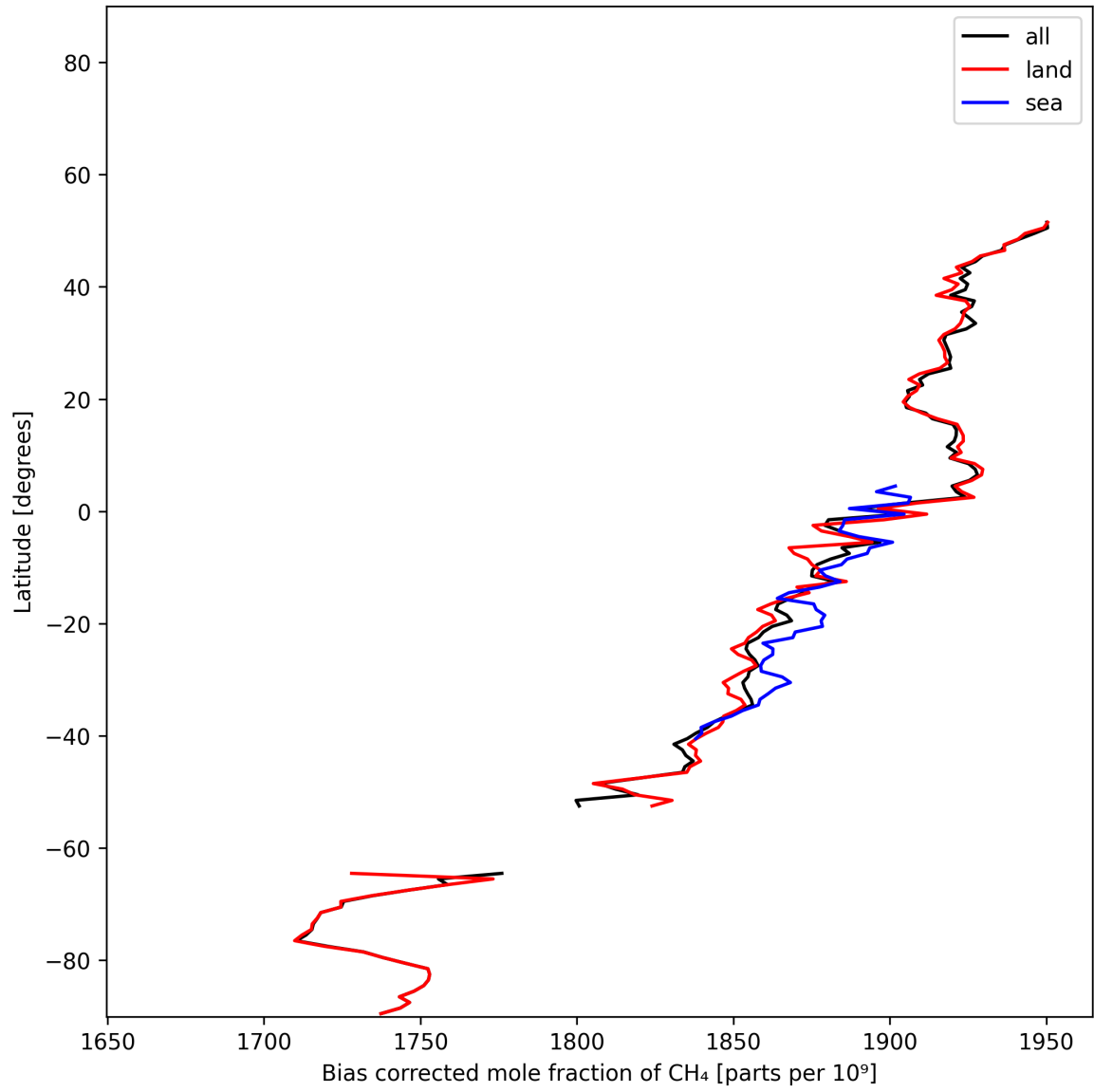
Figure 14: Zonal average of “Bias corrected mole fraction of CH 4 ” for 2024-12-12 to 2024-12-14.
