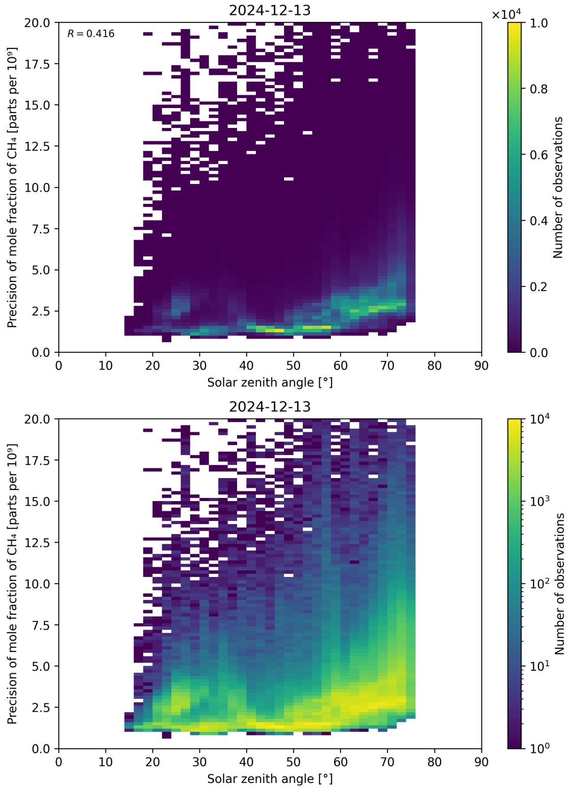
Figure 101: Scatter density plot of “Solar zenith angle” against “Precision of mole fraction of \text{CH}_4 ” for 2024-12-12 to 2024-12-14.
