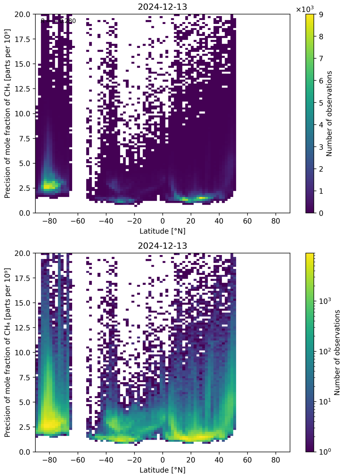
Figure 59: Scatter density plot of “Latitude” against “Precision of mole fraction of CH 4 ” for 2024-12-12 to 2024-12-14.
