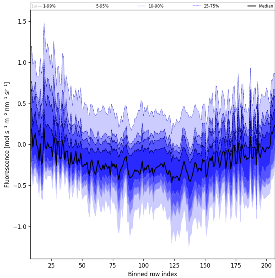
Figure 43: Along track statistics of “Fluorescence” for 2024-12-12 to 2024-12-14
