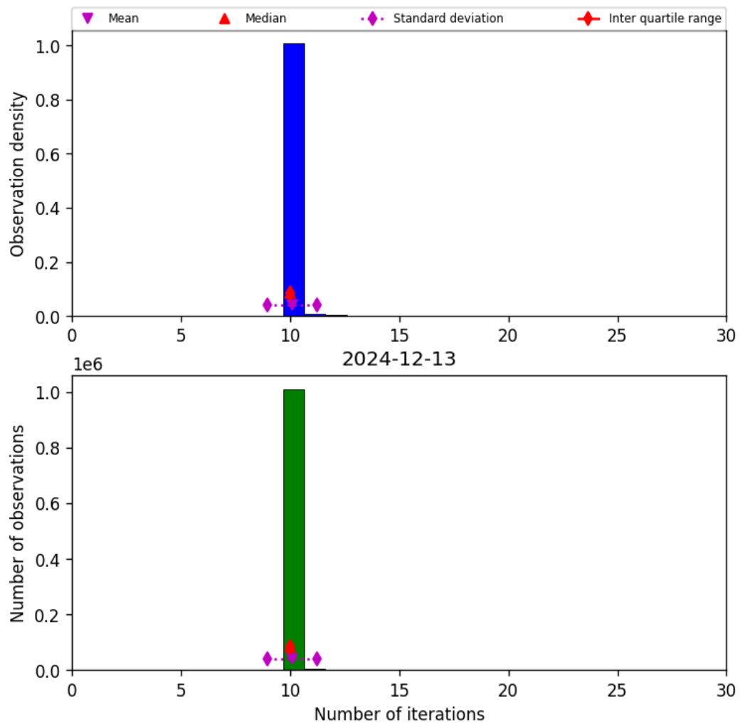
Figure 31: Histogram of “Number of iterations” for 2024-12-12 to 2024-12-14
