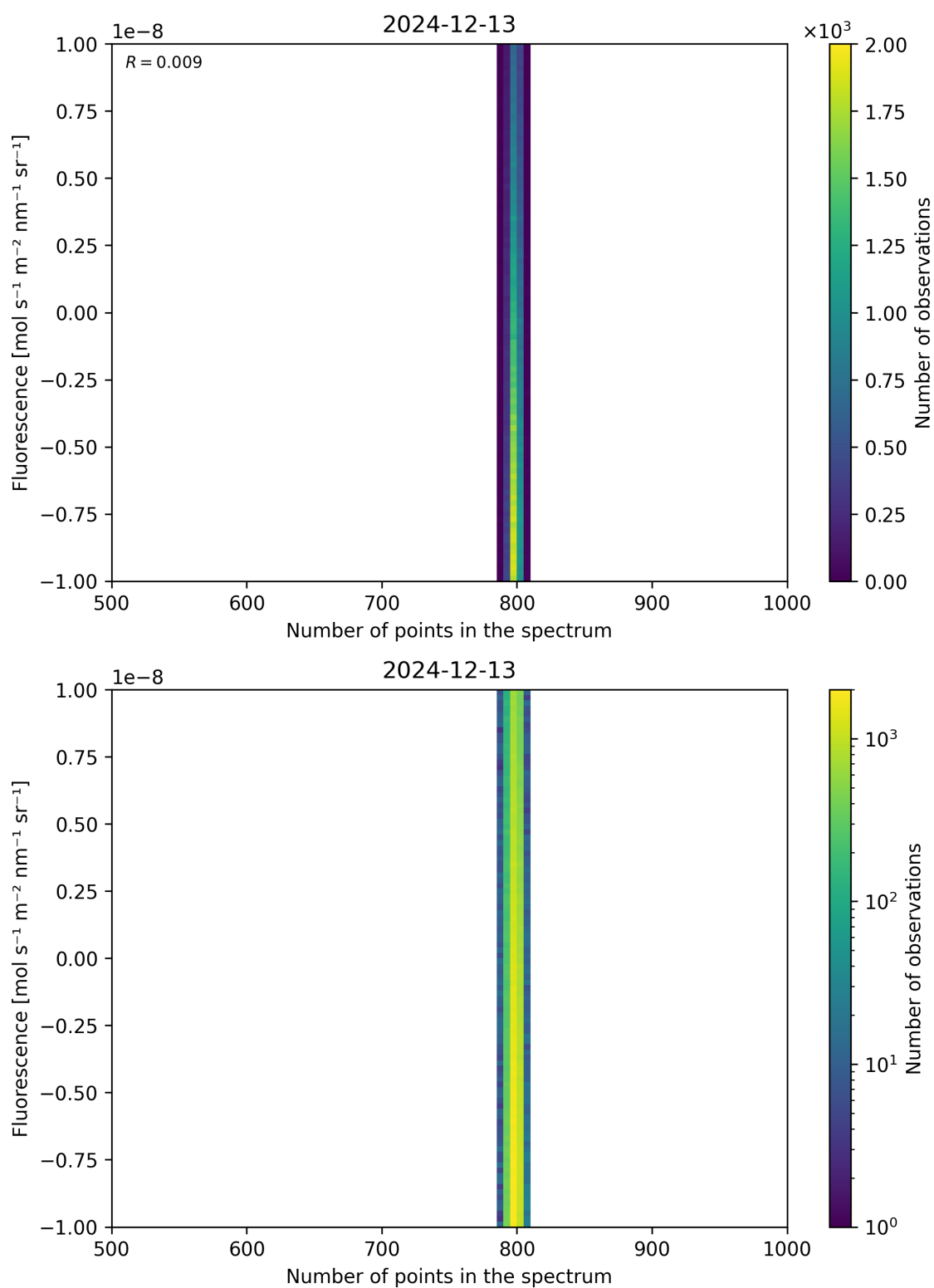
Figure 91: Scatter density plot of “Number of points in the spectrum” against “Fluorescence” for 2024-12-12 to 2024-12-14.
