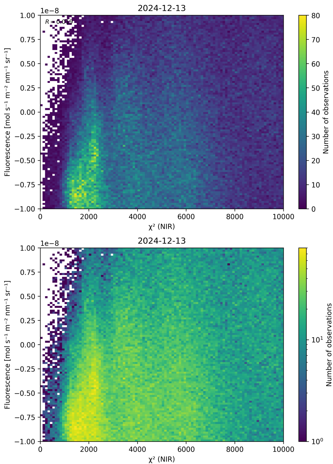
Figure 45: Scatter density plot of “ \chi^2 (NIR)” against “Fluorescence” for 2024-12-12 to 2024-12-14.
