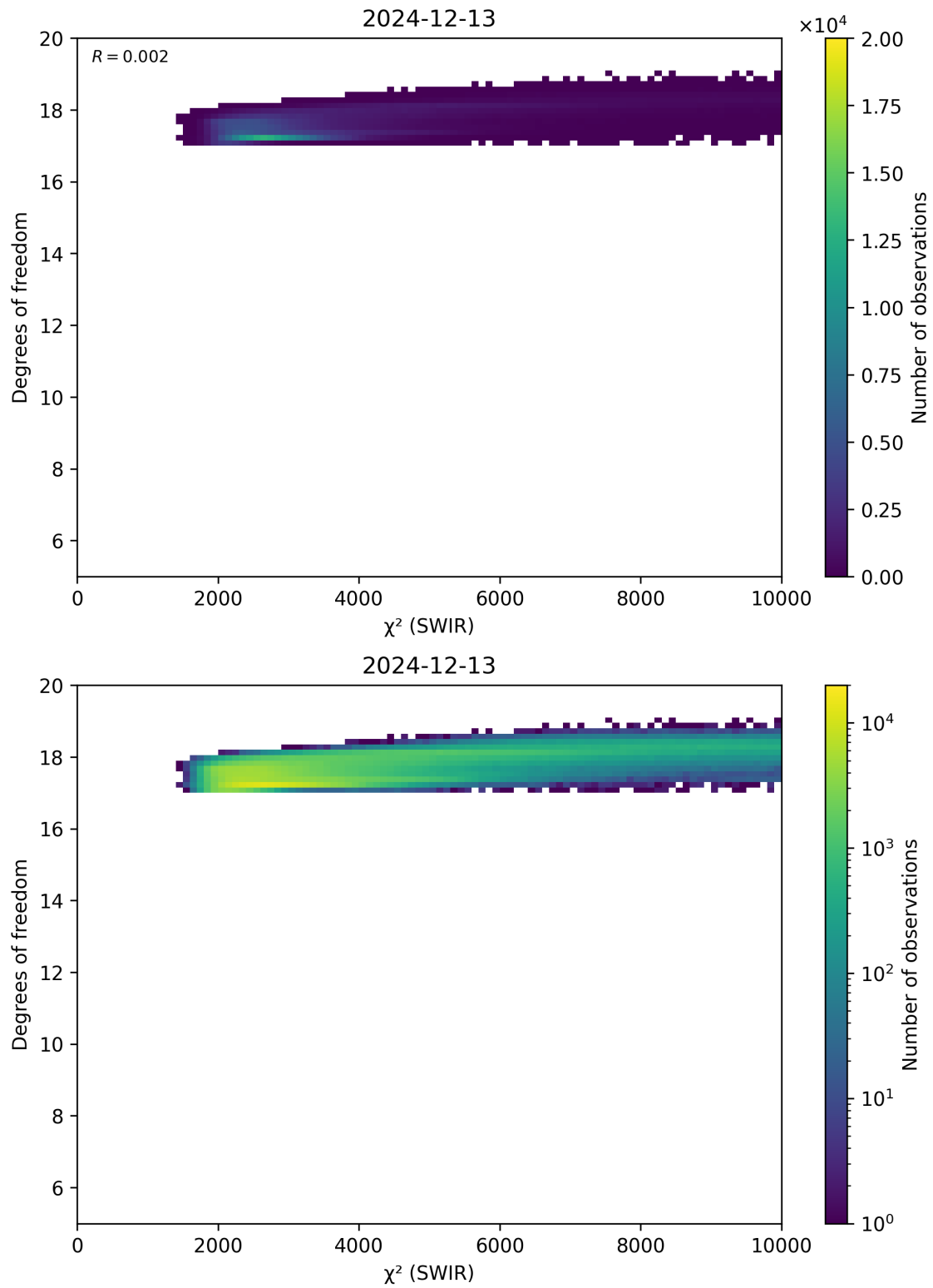
Figure 48: Scatter density plot of “ \chi^2 (SWIR)” against “Degrees of freedom” for 2024-12-12 to 2024-12-14.
