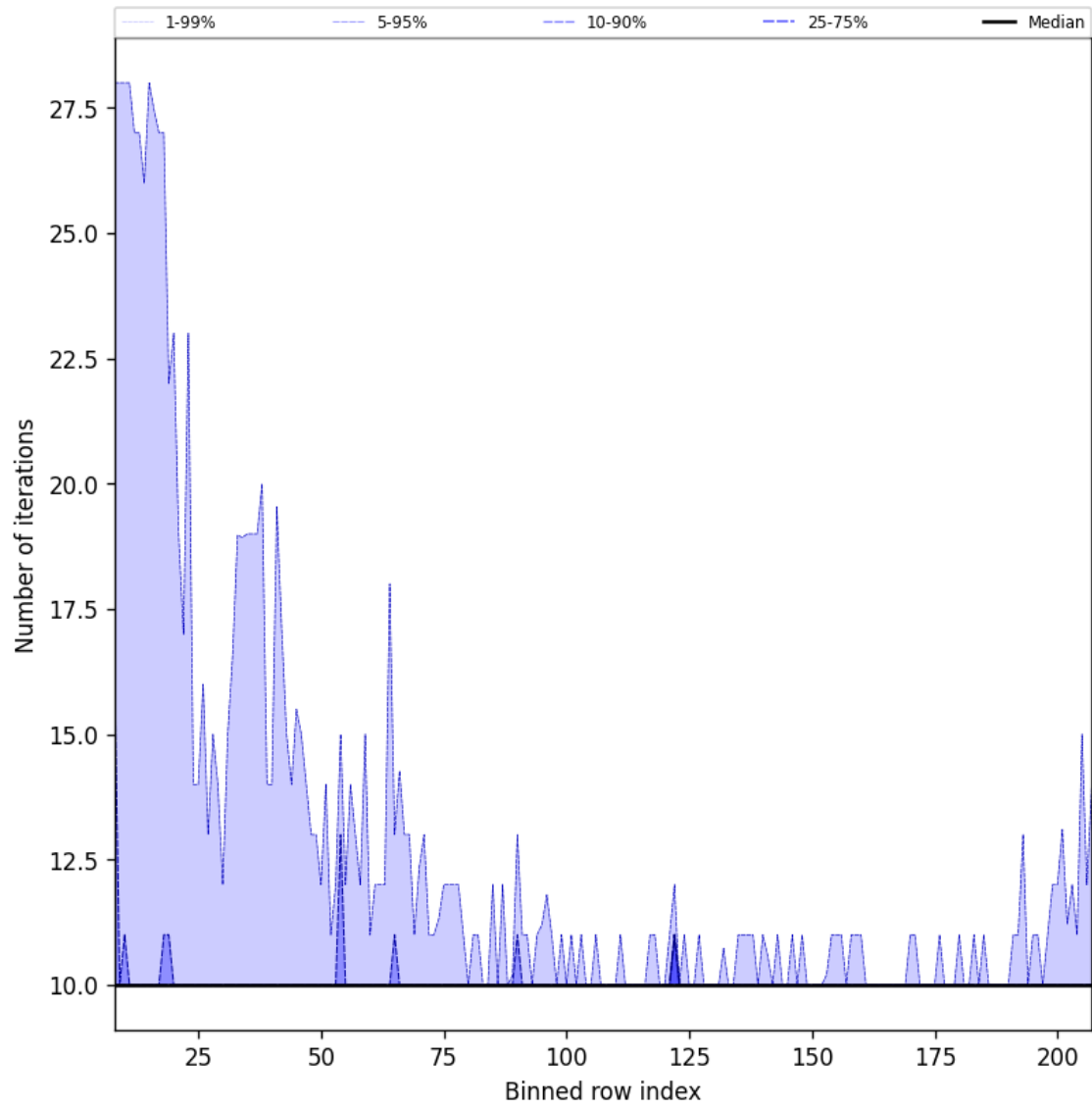
Figure 42: Along track statistics of “Number of iterations” for 2024-12-12 to 2024-12-14
