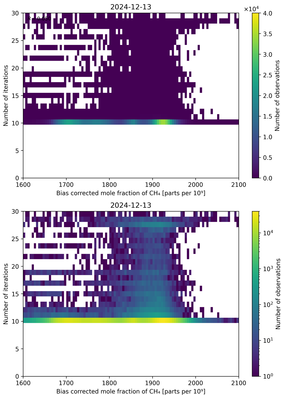
Figure 67: Scatter density plot of “Bias corrected mole fraction of \text{CH}_4 ” against “Number of iterations” for 2024-12-12 to 2024-12-14.
