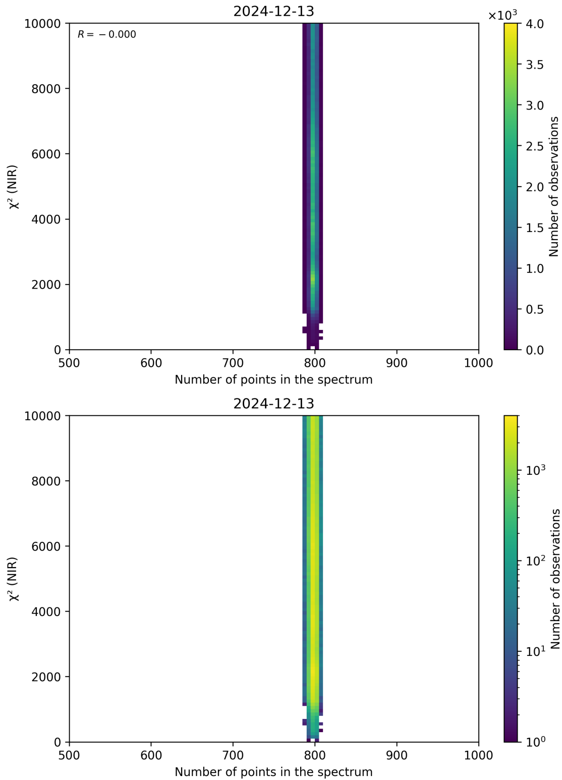
Figure 88: Scatter density plot of “Number of points in the spectrum” against “ \chi^2 (NIR)” for 2024-12-12 to 2024-12-14.
