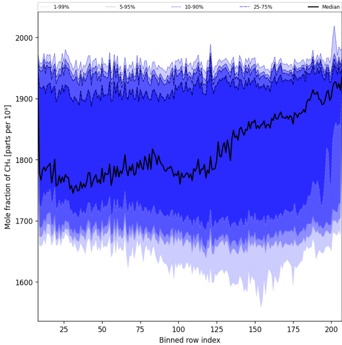
Figure 34: Along track statistics of “Mole fraction of CH 4 ” for 2024-12-12 to 2024-12-14
