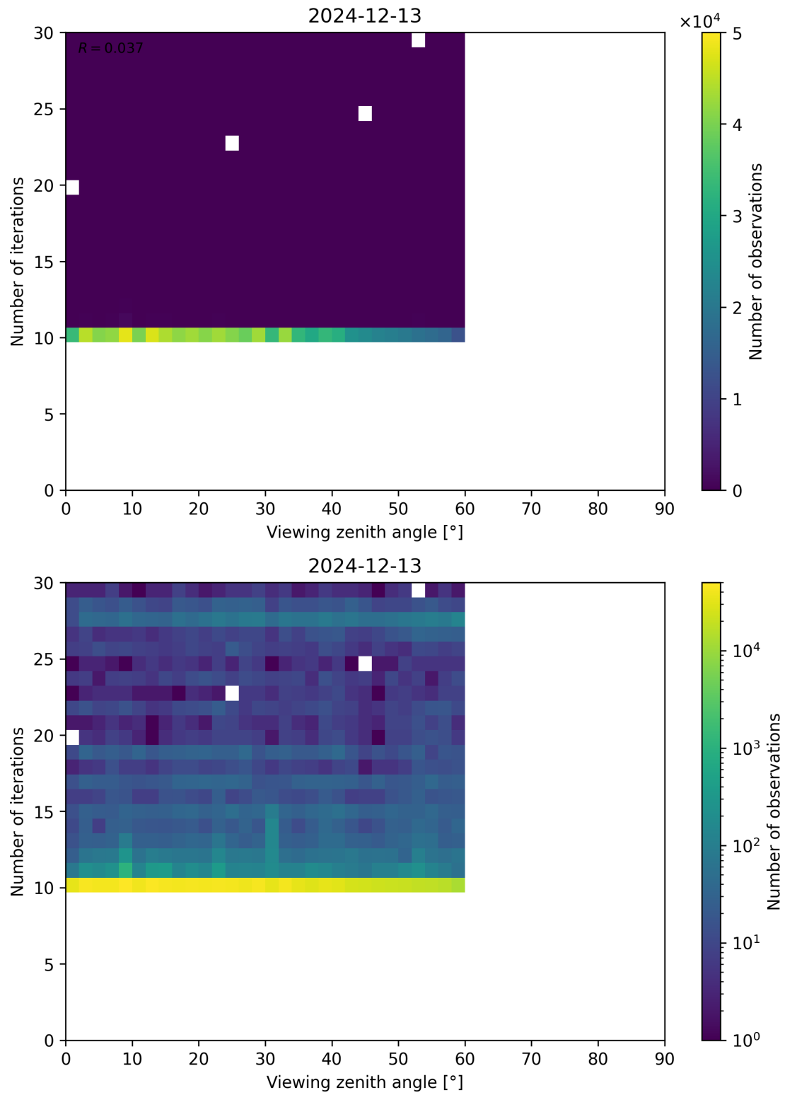
Figure 113: Scatter density plot of “Viewing zenith angle” against “Number of iterations” for 2024-12-12 to 2024-12-14.
