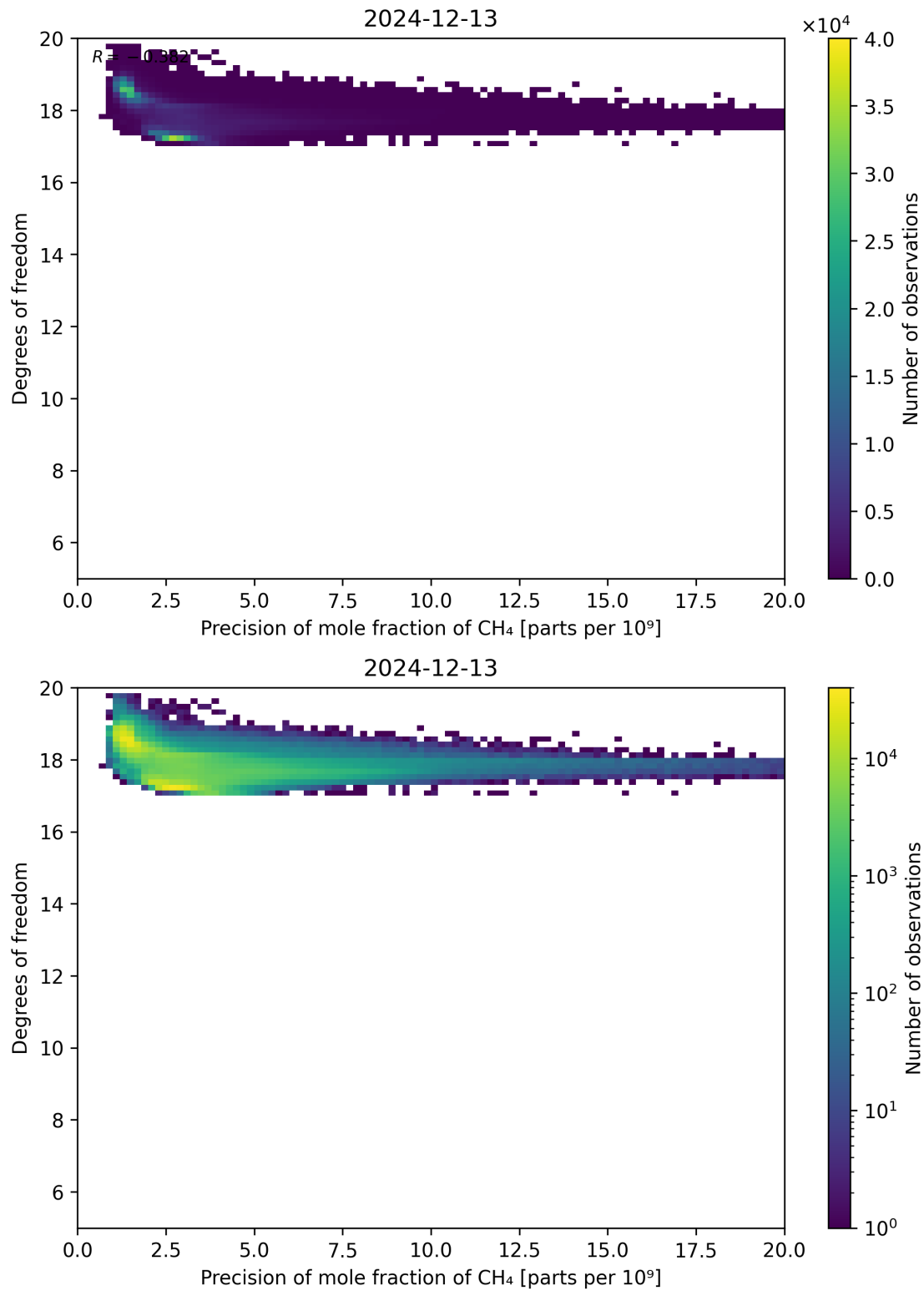
Figure 80: Scatter density plot of “Precision of mole fraction of CH 4 ” against “Degrees of freedom” for 2024-12-12 to 2024-12-14.
