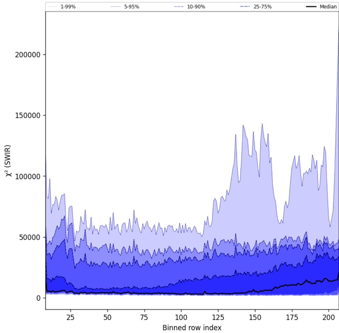
Figure 39: Along track statistics of “ \chi^2 (SWIR)” for 2024-12-12 to 2024-12-14
