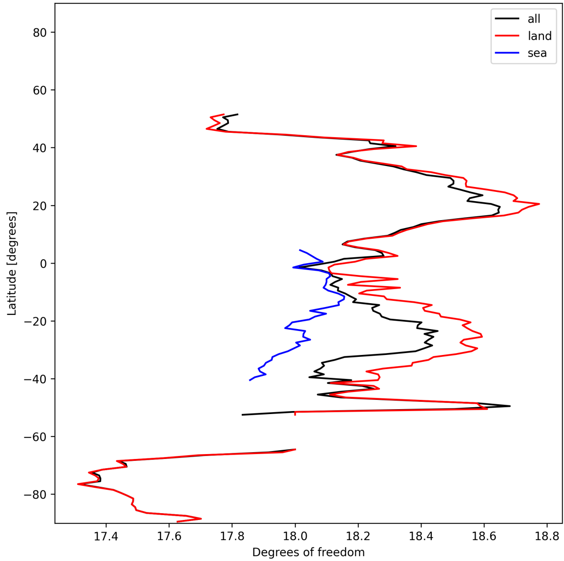
Figure 19: Zonal average of “Degrees of freedom” for 2024-12-12 to 2024-12-14.
