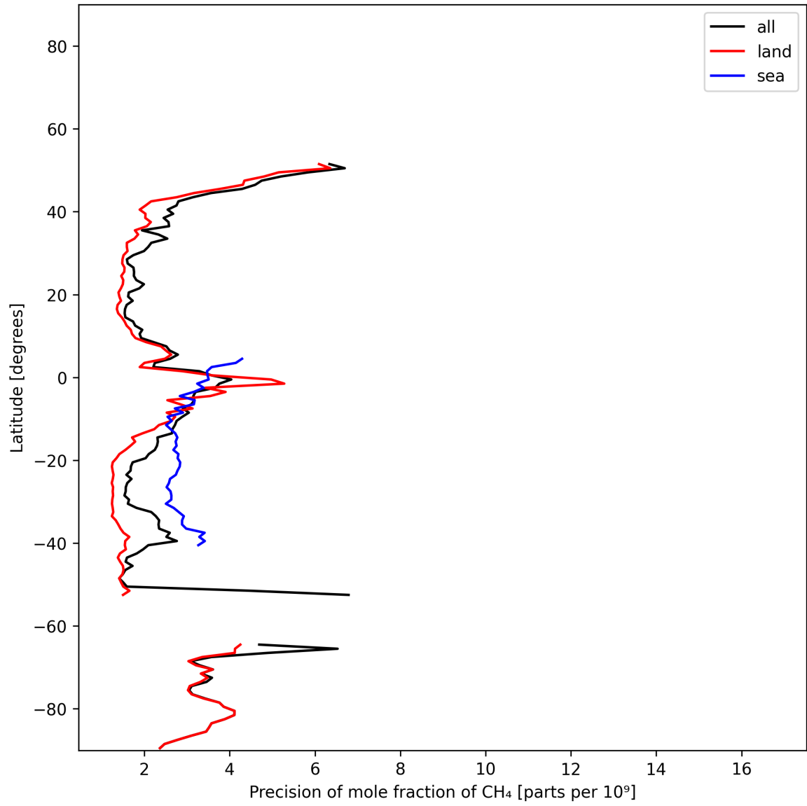
Figure 13: Zonal average of “Precision of mole fraction of CH 4 ” for 2024-12-12 to 2024-12-14.
