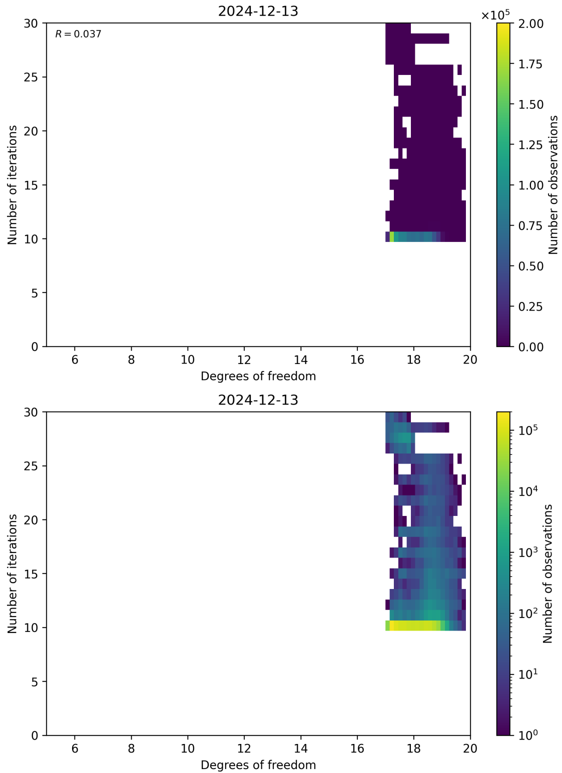
Figure 52: Scatter density plot of “Degrees of freedom” against “Number of iterations” for 2024-12-12 to 2024-12-14.
