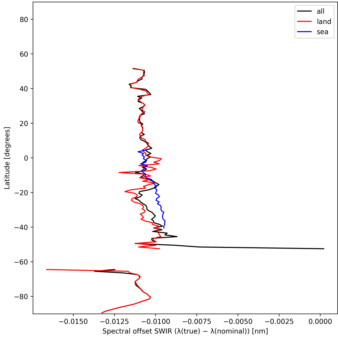
Figure 16: Zonal average of “Spectral offset SWIR ( \lambda_{\text{true}} - \lambda_{\text{nominal}} )” for 2024-12-12 to 2024-12-14.
