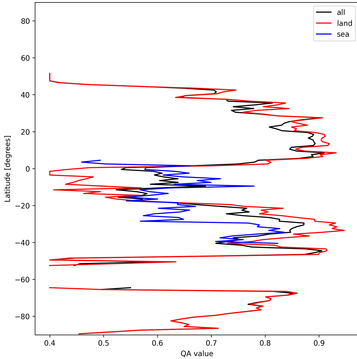
Figure 11: Zonal average of “QA value” for 2024-12-12 to 2024-12-14.
