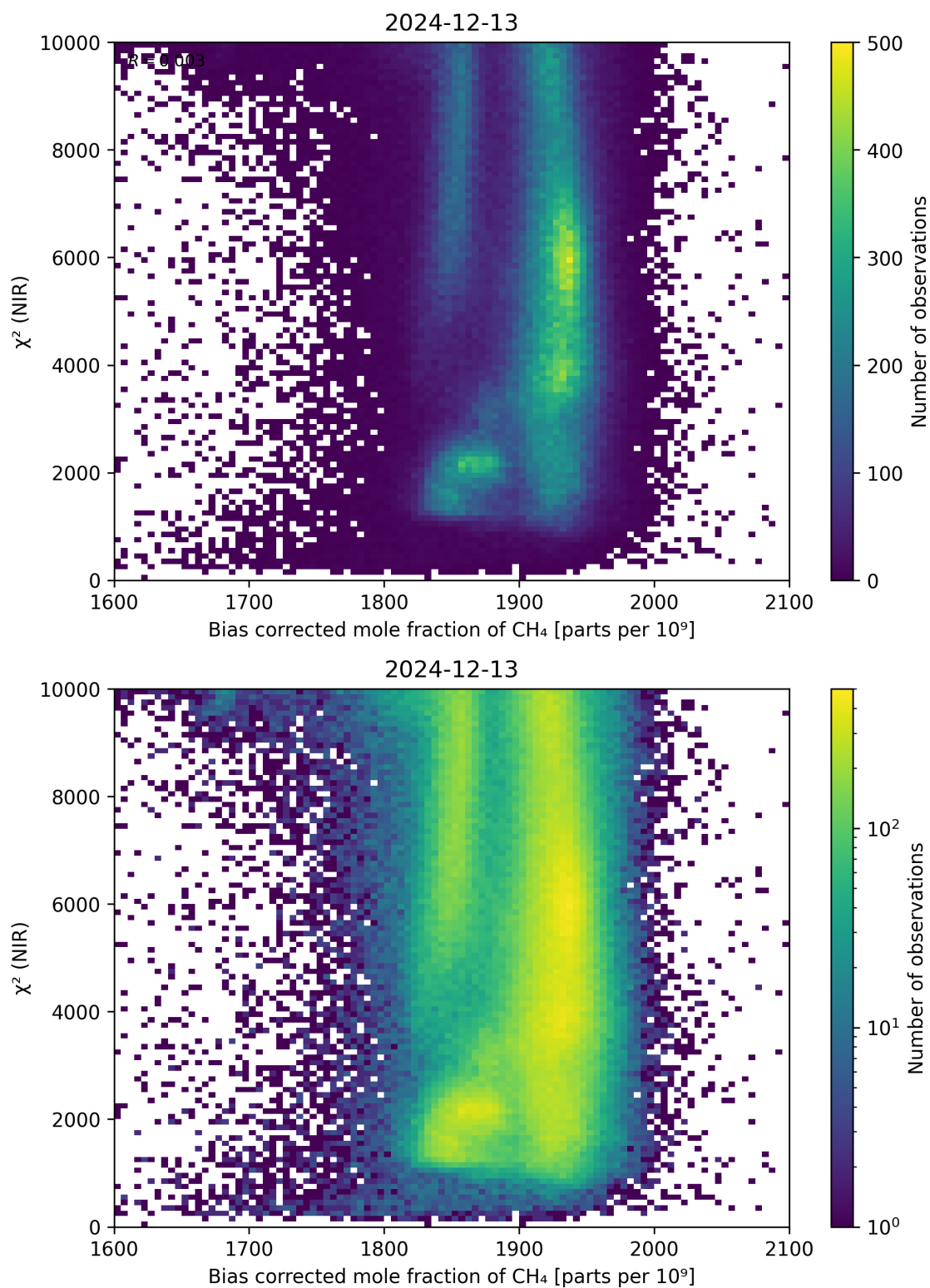
Figure 63: Scatter density plot of “Bias corrected mole fraction of \text{CH}_4 ” against “ \chi^2 (NIR)” for 2024-12-12 to 2024-12-14.
