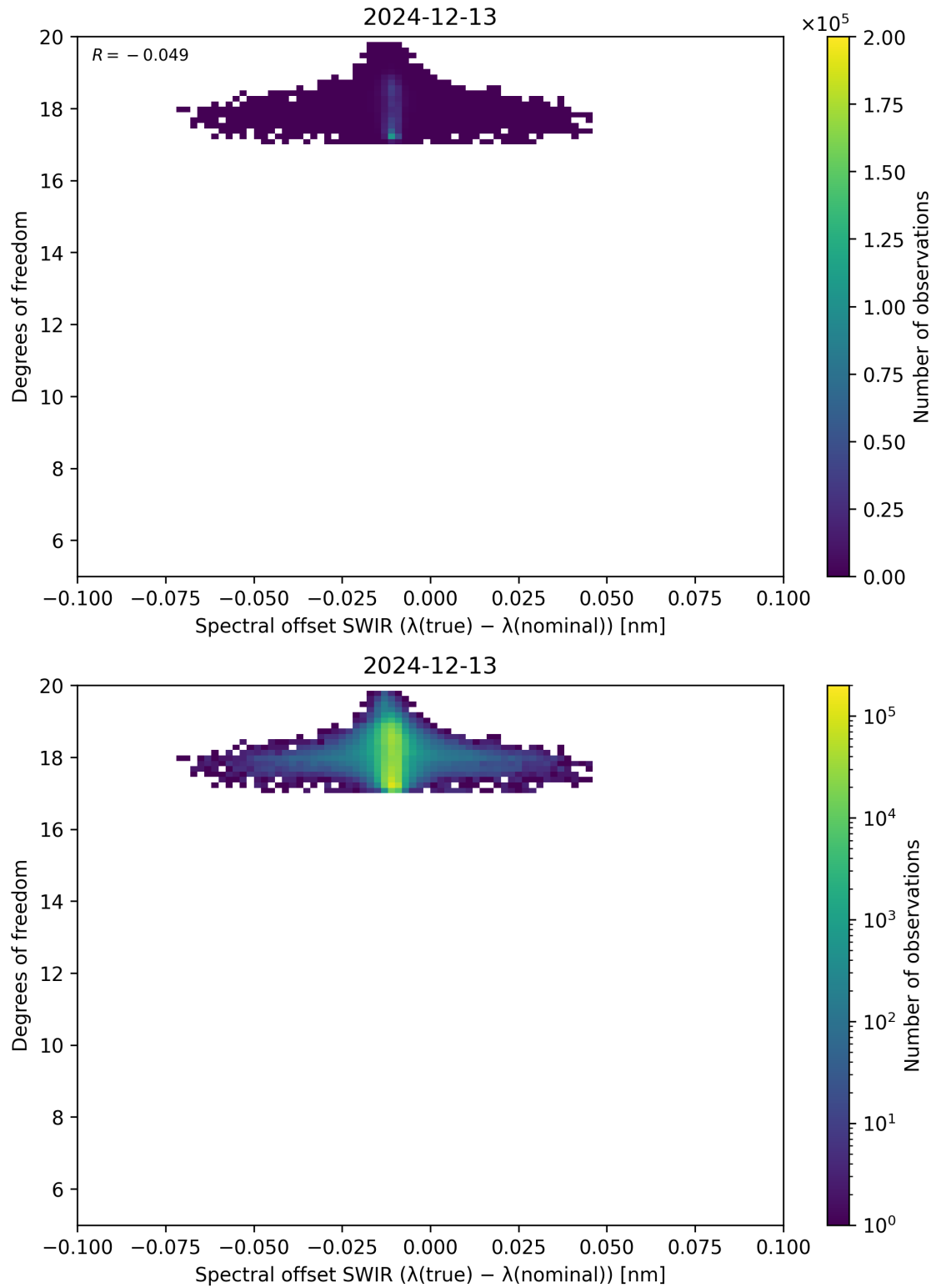
Figure 119: Scatter density plot of “Spectral offset SWIR ( \lambda_{\text{true}} - \lambda_{\text{nominal}} )” against “Degrees of freedom” for 2024-12-12 to 2024-12-14.
