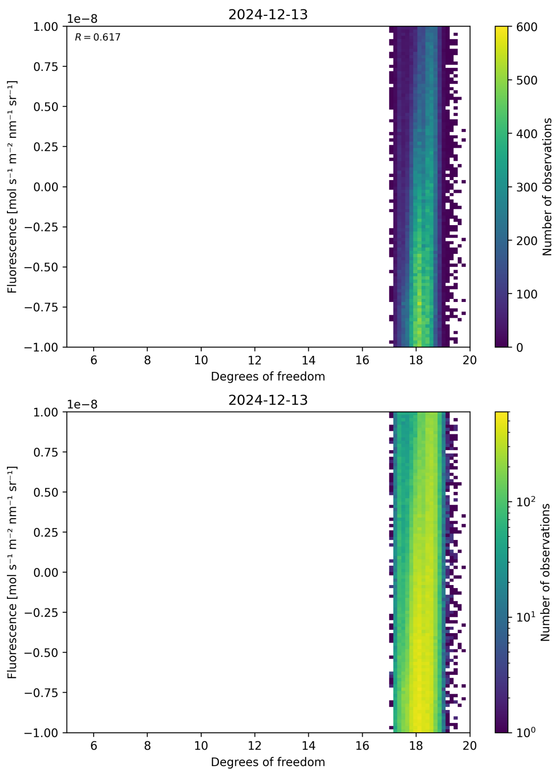
Figure 51: Scatter density plot of “Degrees of freedom” against “Fluorescence” for 2024-12-12 to 2024-12-14.
