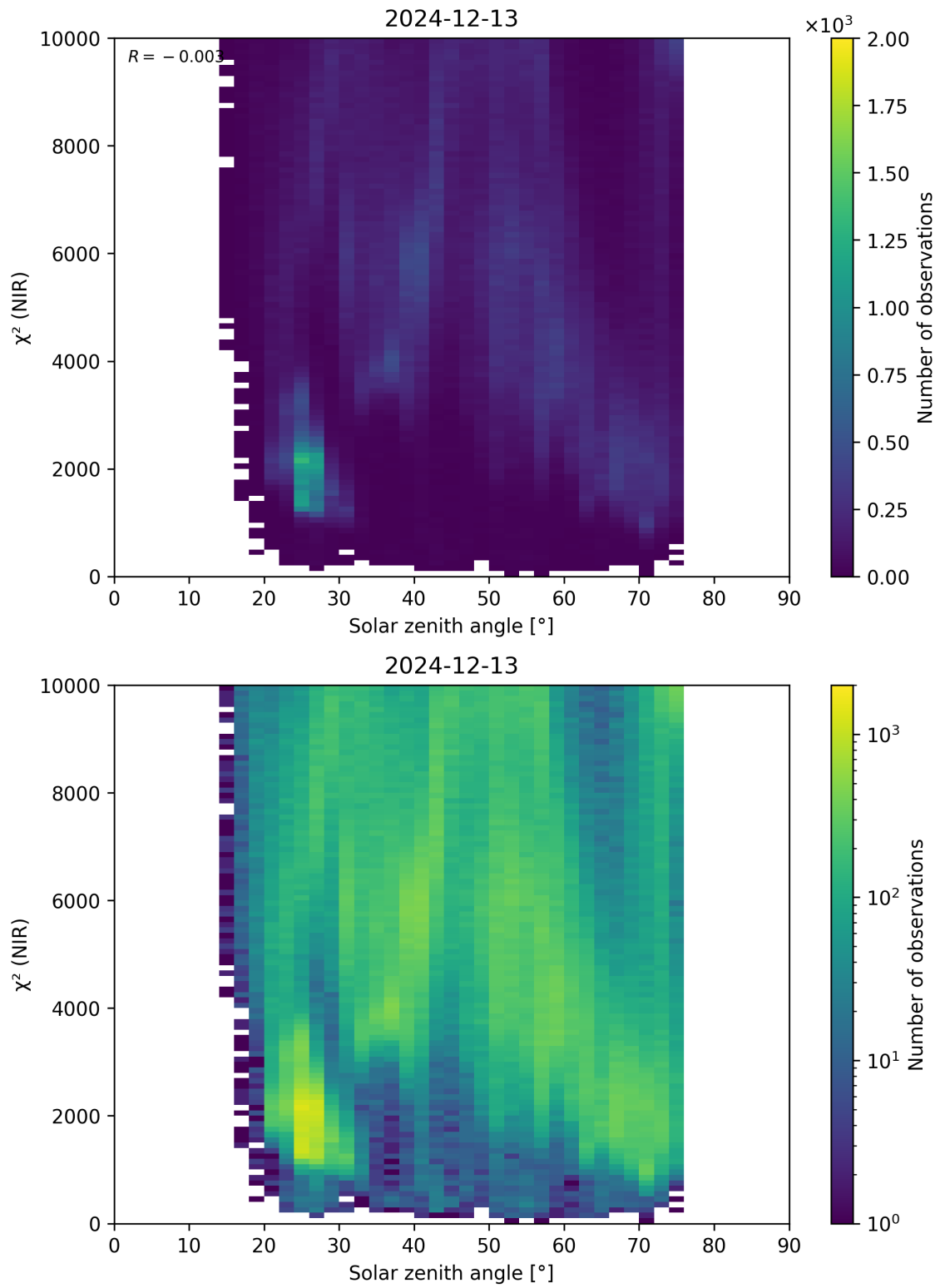
Figure 94: Scatter density plot of “Solar zenith angle” against “ \chi^2 (NIR)” for 2024-12-12 to 2024-12-14.
