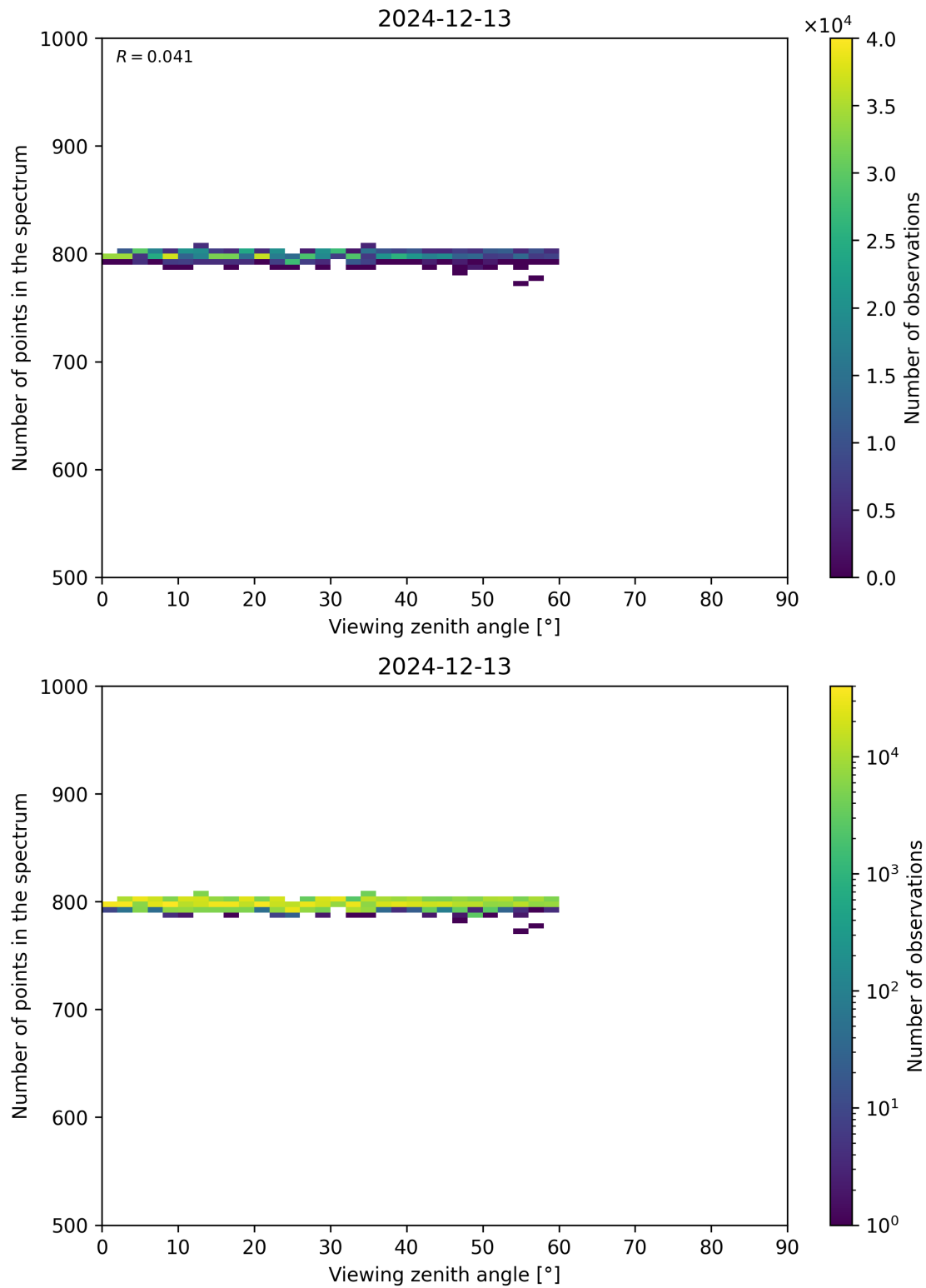
Figure 114: Scatter density plot of “Viewing zenith angle” against “Number of points in the spectrum” for 2024-12-12 to 2024-12-14.
