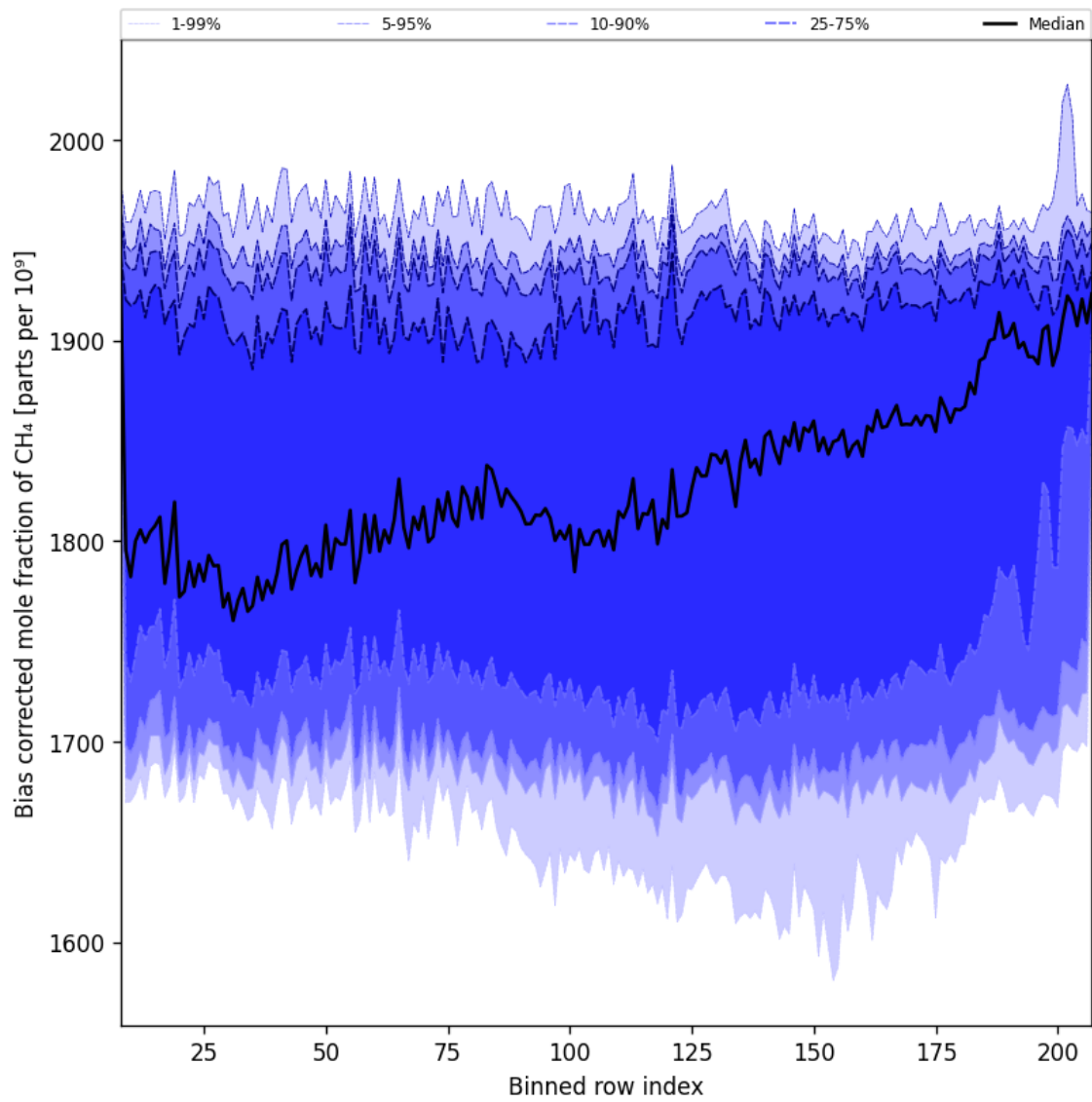
Figure 36: Along track statistics of “Bias corrected mole fraction of CH 4 ” for 2024-12-12 to 2024-12-14
