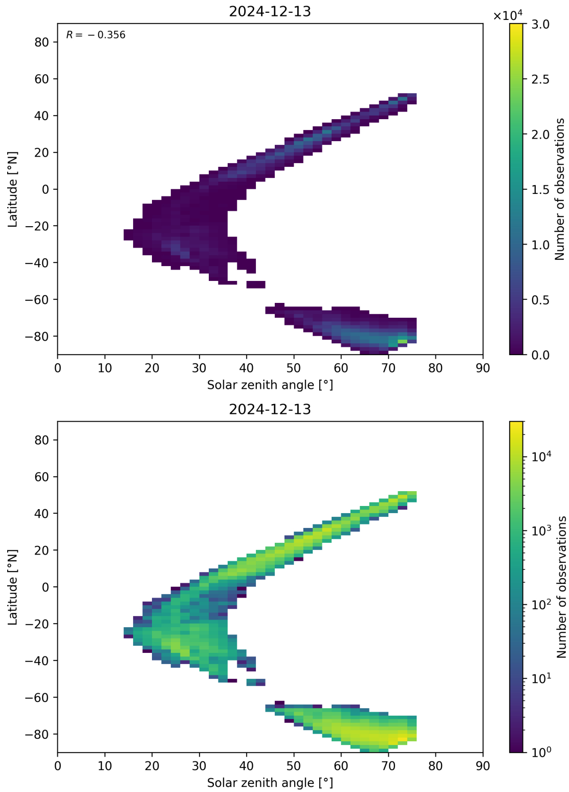
Figure 98: Scatter density plot of “Solar zenith angle” against “Latitude” for 2024-12-12 to 2024-12-14.
