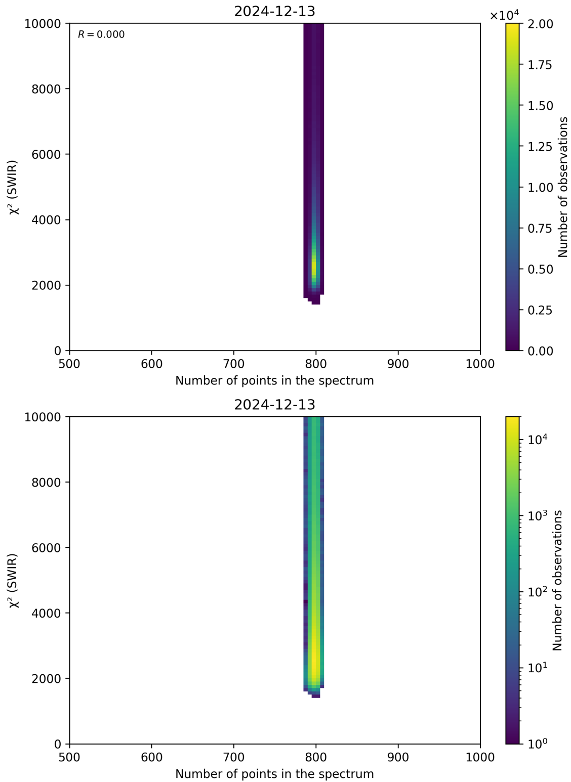
Figure 89: Scatter density plot of “Number of points in the spectrum” against “ \chi^2 (SWIR)” for 2024-12-12 to 2024-12-14.
