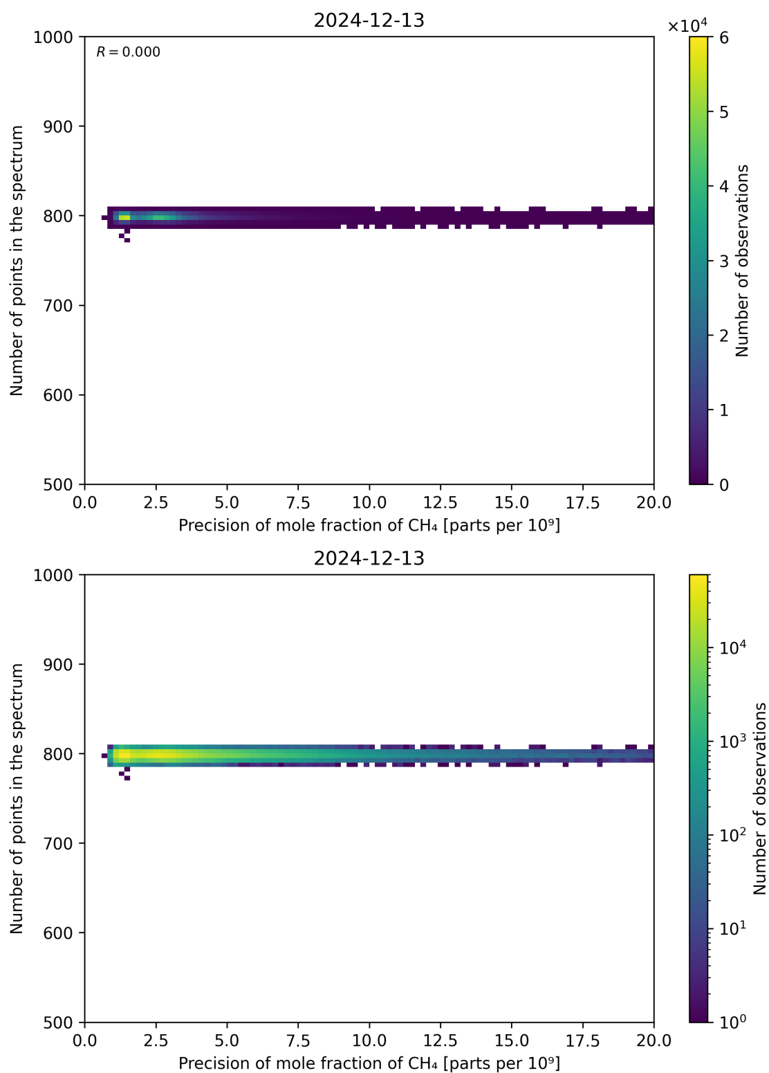
Figure 84: Scatter density plot of “Precision of mole fraction of CH 4 ” against “Number of points in the spectrum” for 2024-12-12 to 2024-12-14.
