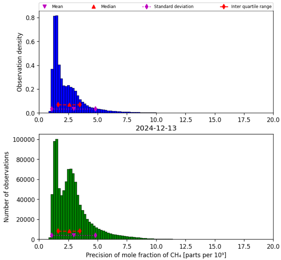
Figure 24: Histogram of “Precision of mole fraction of CH 4 ” for 2024-12-12 to 2024-12-14
