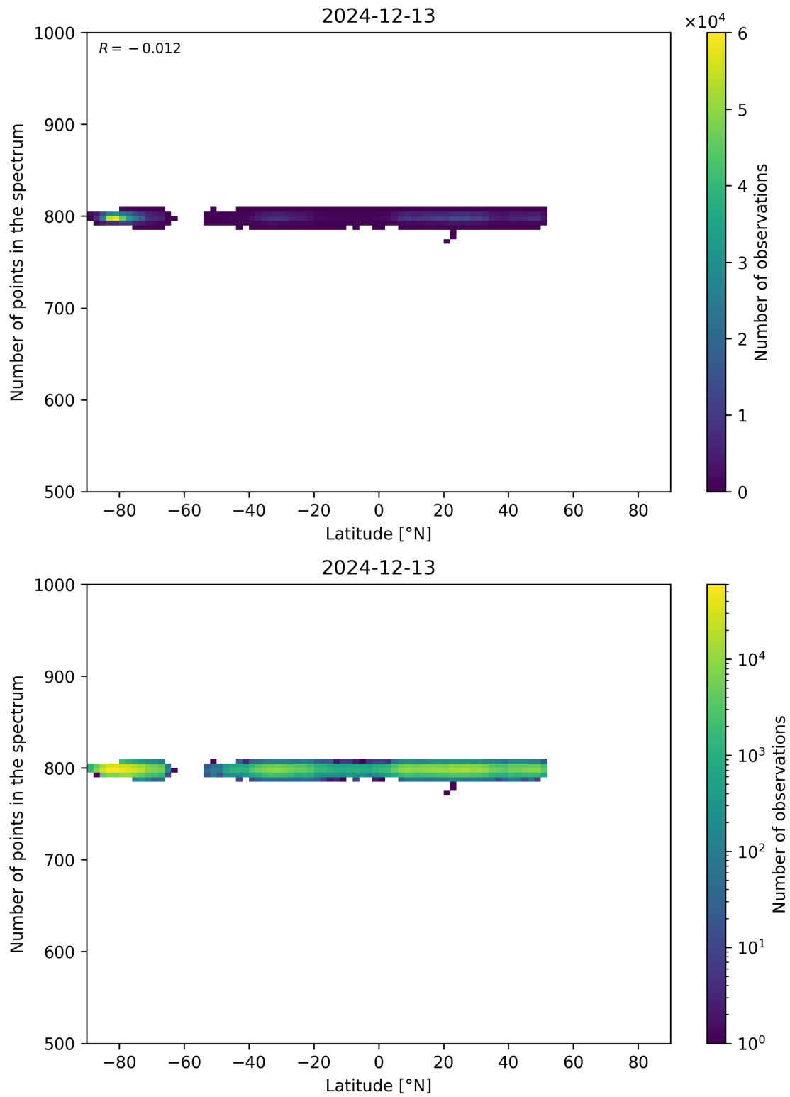
Figure 61: Scatter density plot of “Latitude” against “Number of points in the spectrum” for 2024-12-12 to 2024-12-14.
