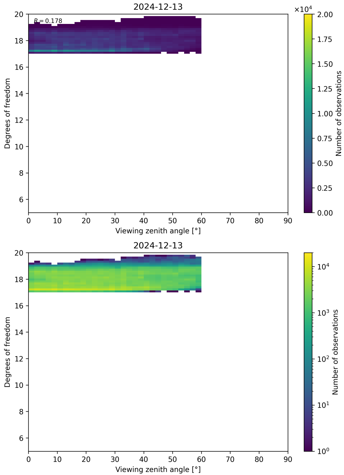
Figure 107: Scatter density plot of “Viewing zenith angle” against “Degrees of freedom” for 2024-12-12 to 2024-12-14.
