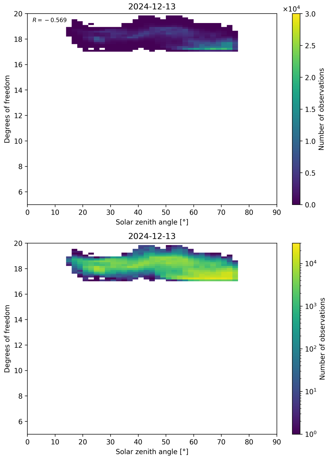
Figure 96: Scatter density plot of “Solar zenith angle” against “Degrees of freedom” for 2024-12-12 to 2024-12-14.
