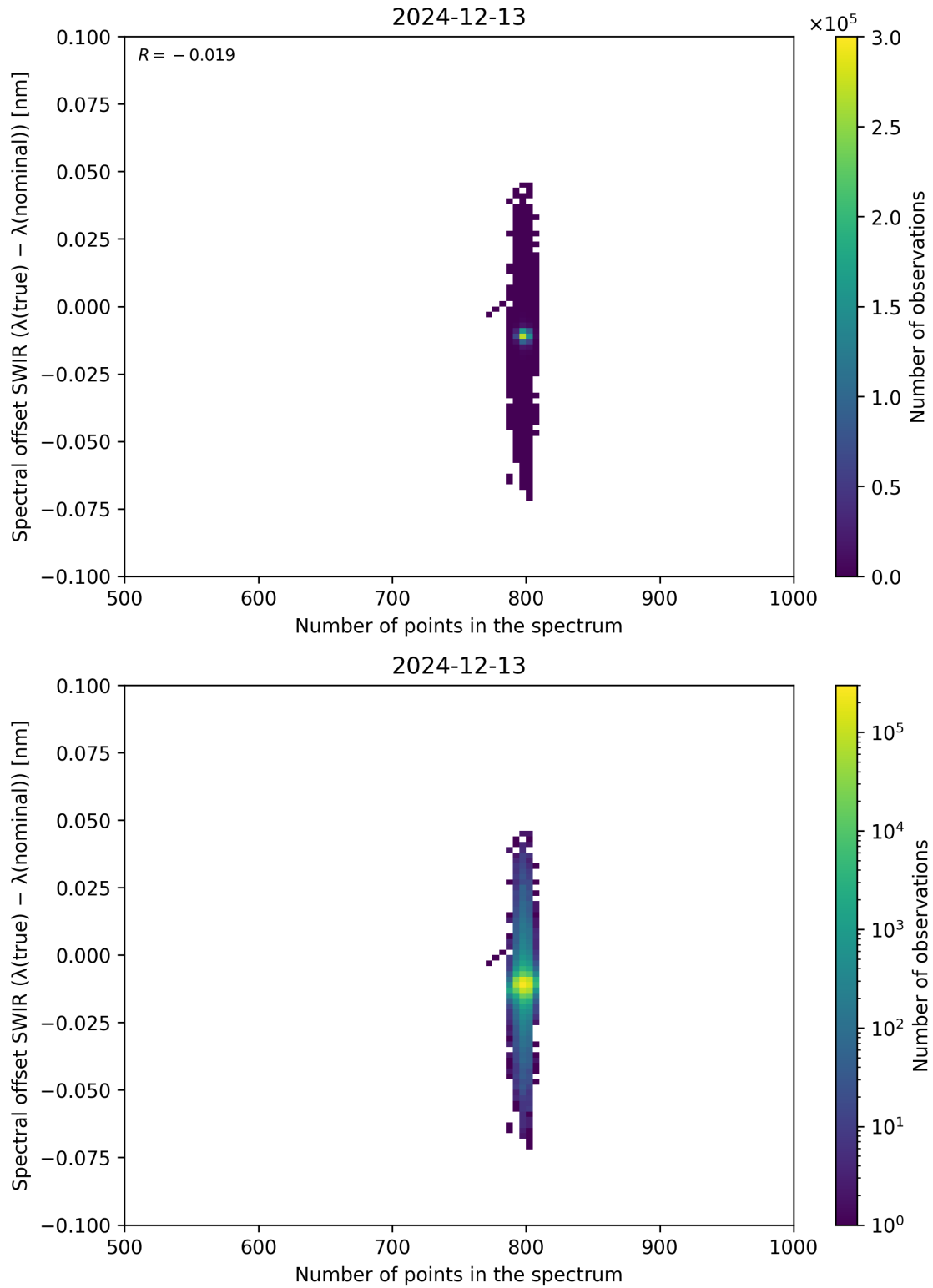
Figure 93: Scatter density plot of “Number of points in the spectrum” against “Spectral offset SWIR ( \lambda_{\text{true}} - \lambda_{\text{nominal}} )” for 2024-12-12 to 2024-12-14.
