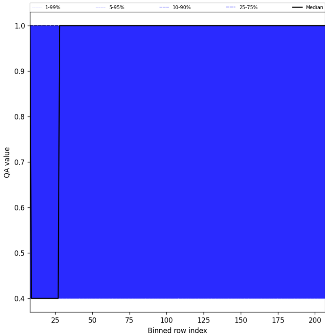
Figure 33: Along track statistics of “QA value” for 2024-12-12 to 2024-12-14
