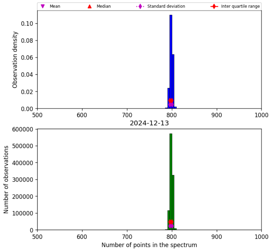
Figure 26: Histogram of “Number of points in the spectrum” for 2024-12-12 to 2024-12-14
