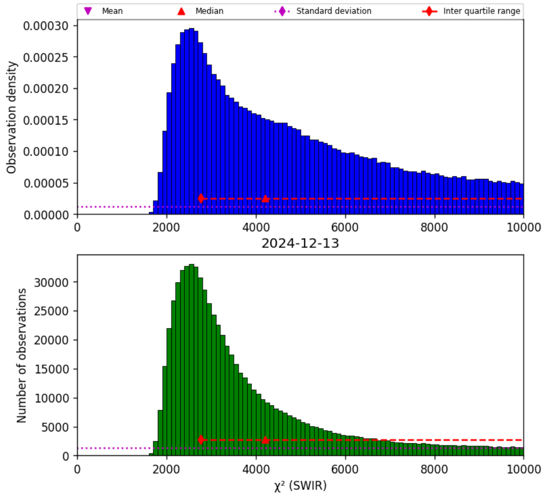
Figure 28: Histogram of “ \chi^2 (SWIR)” for 2024-12-12 to 2024-12-14
