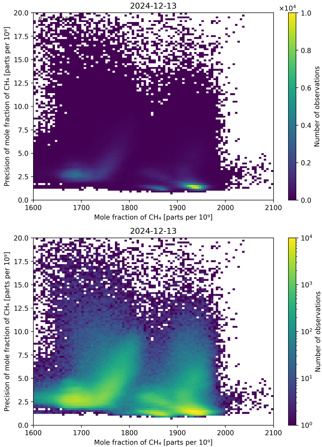
Figure 75: Scatter density plot of “Mole fraction of CH 4 ” against “Precision of mole fraction of CH 4 ” for 2024-12-12 to 2024-12-14.
