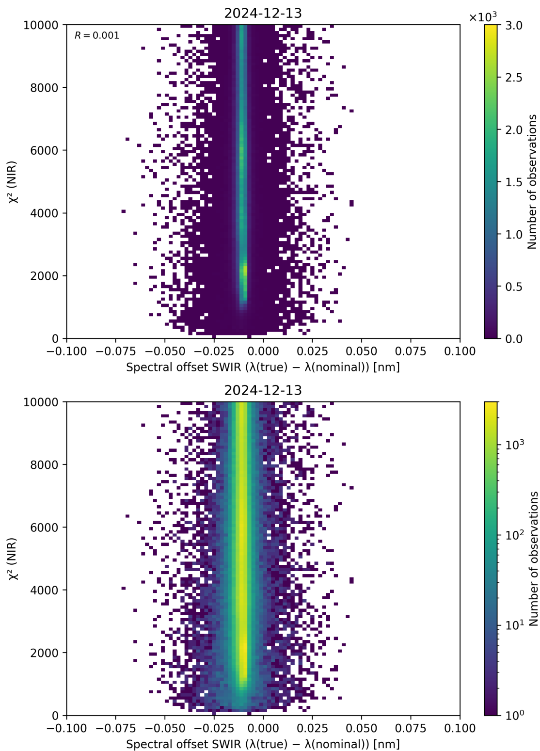
Figure 117: Scatter density plot of “Spectral offset SWIR ( \lambda_{\text{true}} - \lambda_{\text{nominal}} )” against “ \chi^2 (NIR)” for 2024-12-12 to 2024-12-14.
