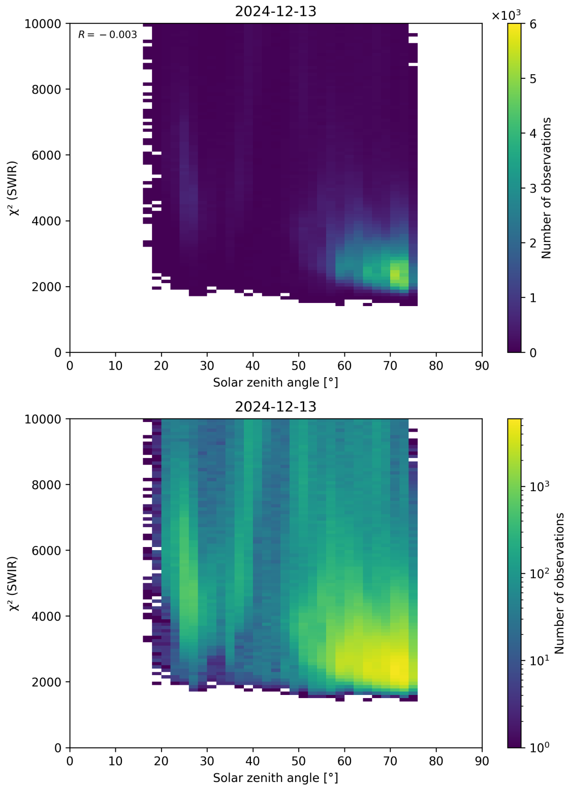
Figure 95: Scatter density plot of “Solar zenith angle” against “ \chi^2 (SWIR)” for 2024-12-12 to 2024-12-14.
