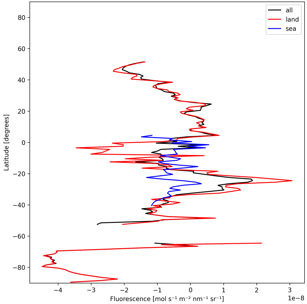
Figure 21: Zonal average of “Fluorescence” for 2024-12-12 to 2024-12-14.
