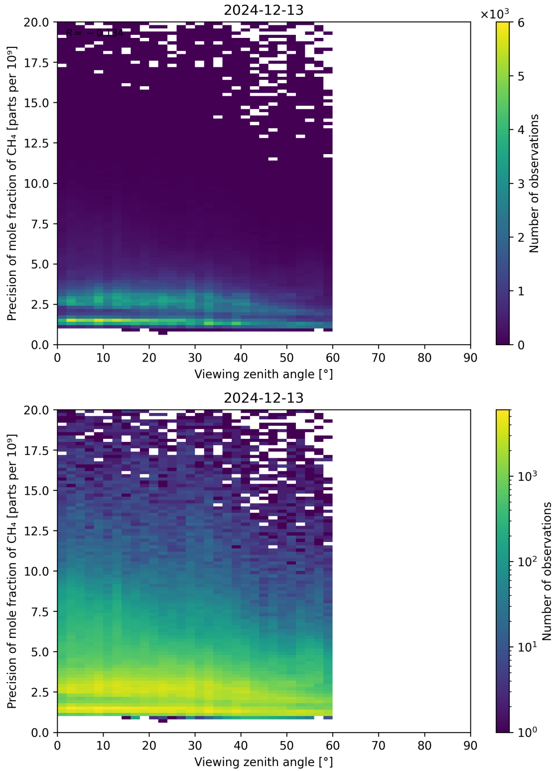
Figure 112: Scatter density plot of “Viewing zenith angle” against “Precision of mole fraction of \text{CH}_4 ” for 2024-12-12 to 2024-12-14.
