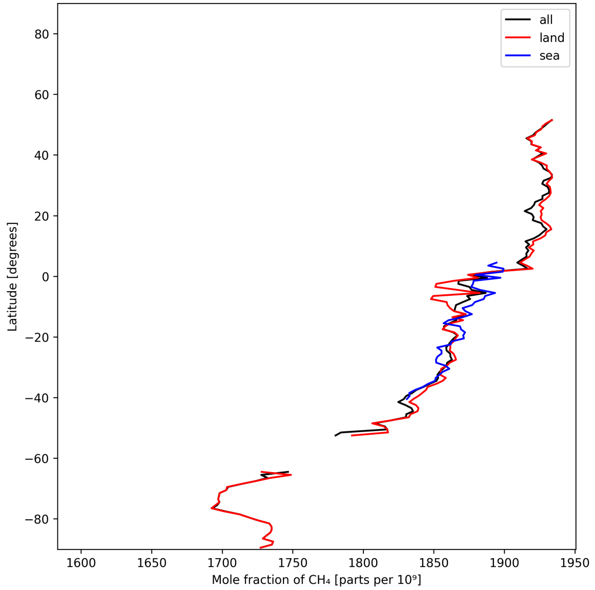
Figure 12: Zonal average of “Mole fraction of \text{CH}_4 ” for 2024-12-12 to 2024-12-14.
