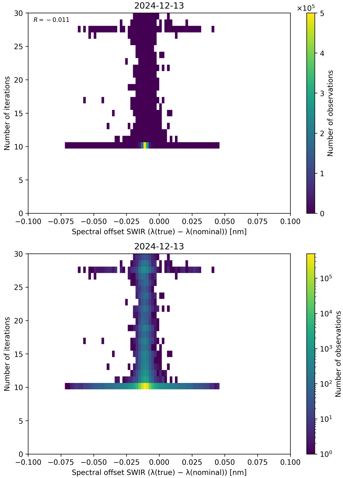
Figure 121: Scatter density plot of “Spectral offset SWIR ( \lambda_{\text{true}} - \lambda_{\text{nominal}} )” against “Number of iterations” for 2024-12-12 to 2024-12-14.
