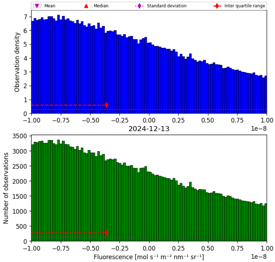
Figure 32: Histogram of “Fluorescence” for 2024-12-12 to 2024-12-14
