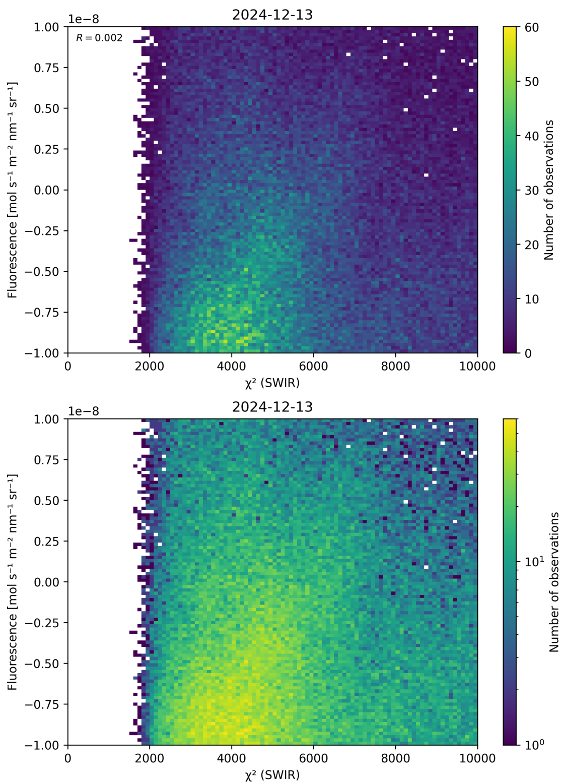
Figure 49: Scatter density plot of “ \chi^2 (SWIR)” against “Fluorescence” for 2024-12-12 to 2024-12-14.
