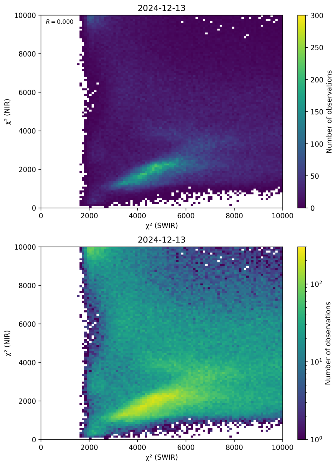
Figure 47: Scatter density plot of “ \chi^2 (SWIR)” against “ \chi^2 (NIR)” for 2024-12-12 to 2024-12-14.
