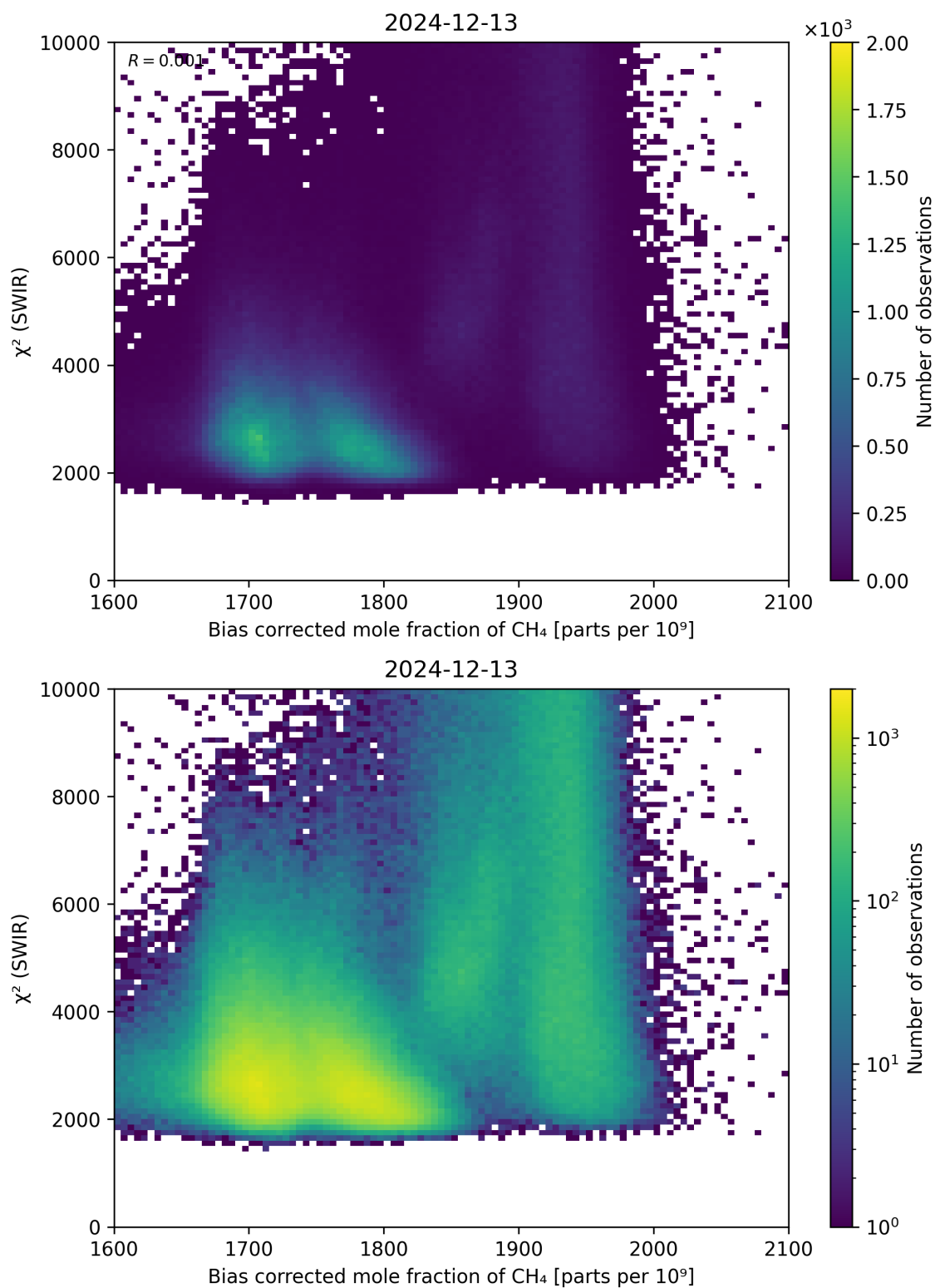
Figure 64: Scatter density plot of “Bias corrected mole fraction of \text{CH}_4 ” against “ \chi^2 (SWIR)” for 2024-12-12 to 2024-12-14.
