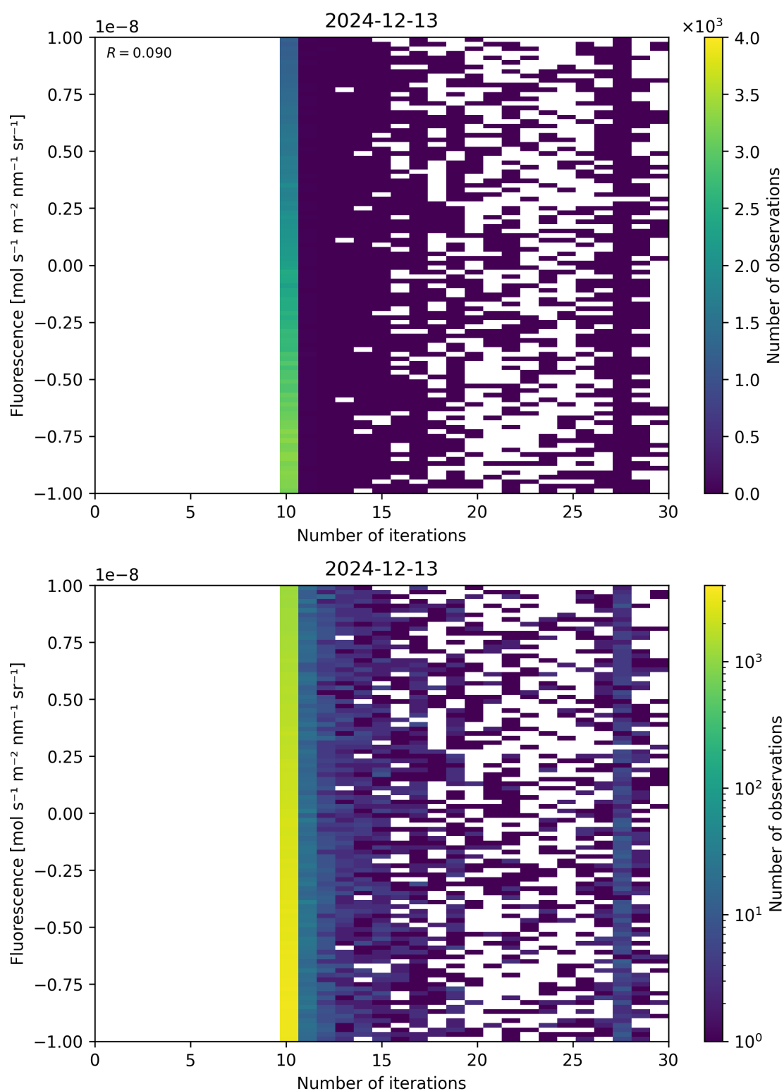
Figure 87: Scatter density plot of “Number of iterations” against “Fluorescence” for 2024-12-12 to 2024-12-14.
