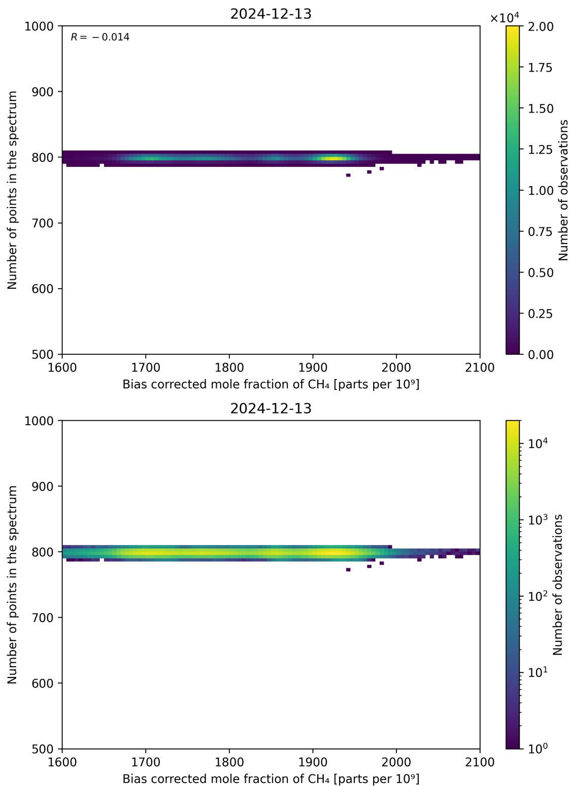
Figure 68: Scatter density plot of “Bias corrected mole fraction of CH 4 ” against “Number of points in the spectrum” for 2024-12-12 to 2024-12-14.
