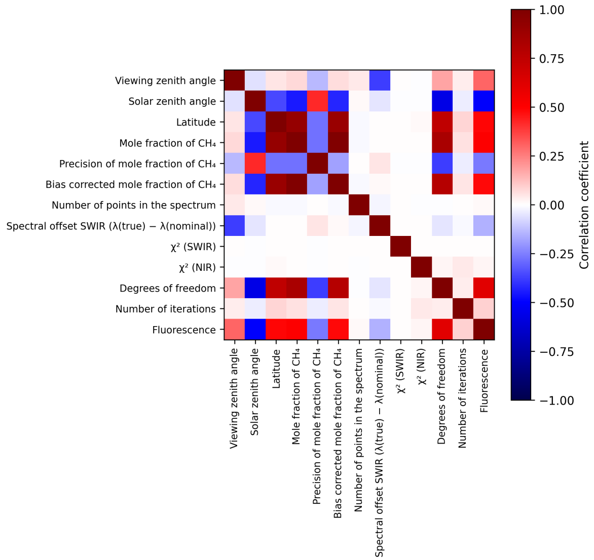
Figure 2: Map of correlation matrix for 2024-12-12 to 2024-12-14.
