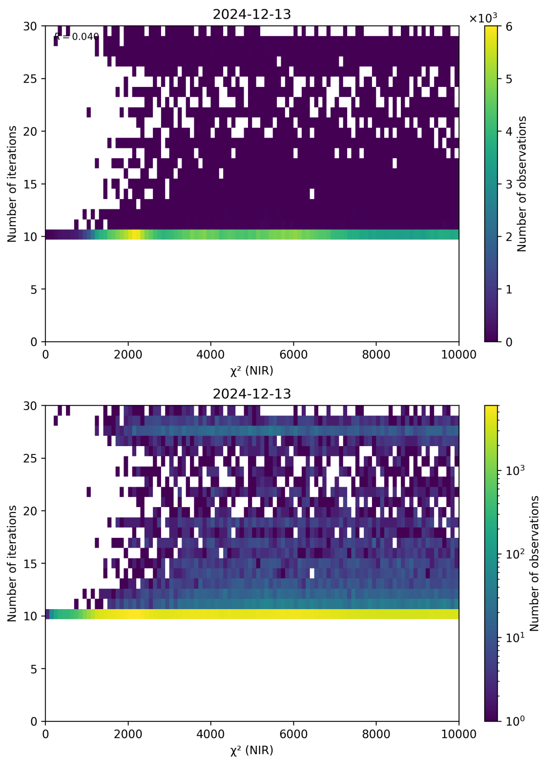
Figure 46: Scatter density plot of “ \chi^2 (NIR)” against “Number of iterations” for 2024-12-12 to 2024-12-14.
