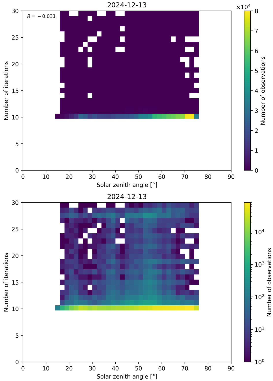
Figure 102: Scatter density plot of “Solar zenith angle” against “Number of iterations” for 2024-12-12 to 2024-12-14.
