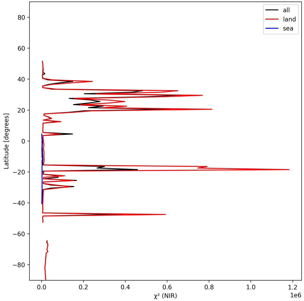
Figure 18: Zonal average of “ \chi^2 (NIR)” for 2024-12-12 to 2024-12-14.
