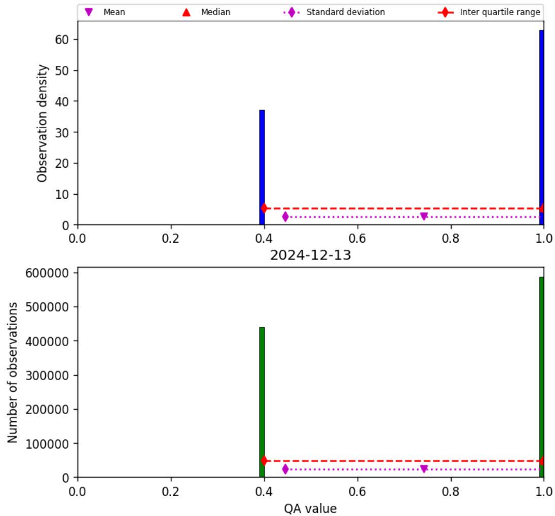
Figure 22: Histogram of “QA value” for 2024-12-12 to 2024-12-14
