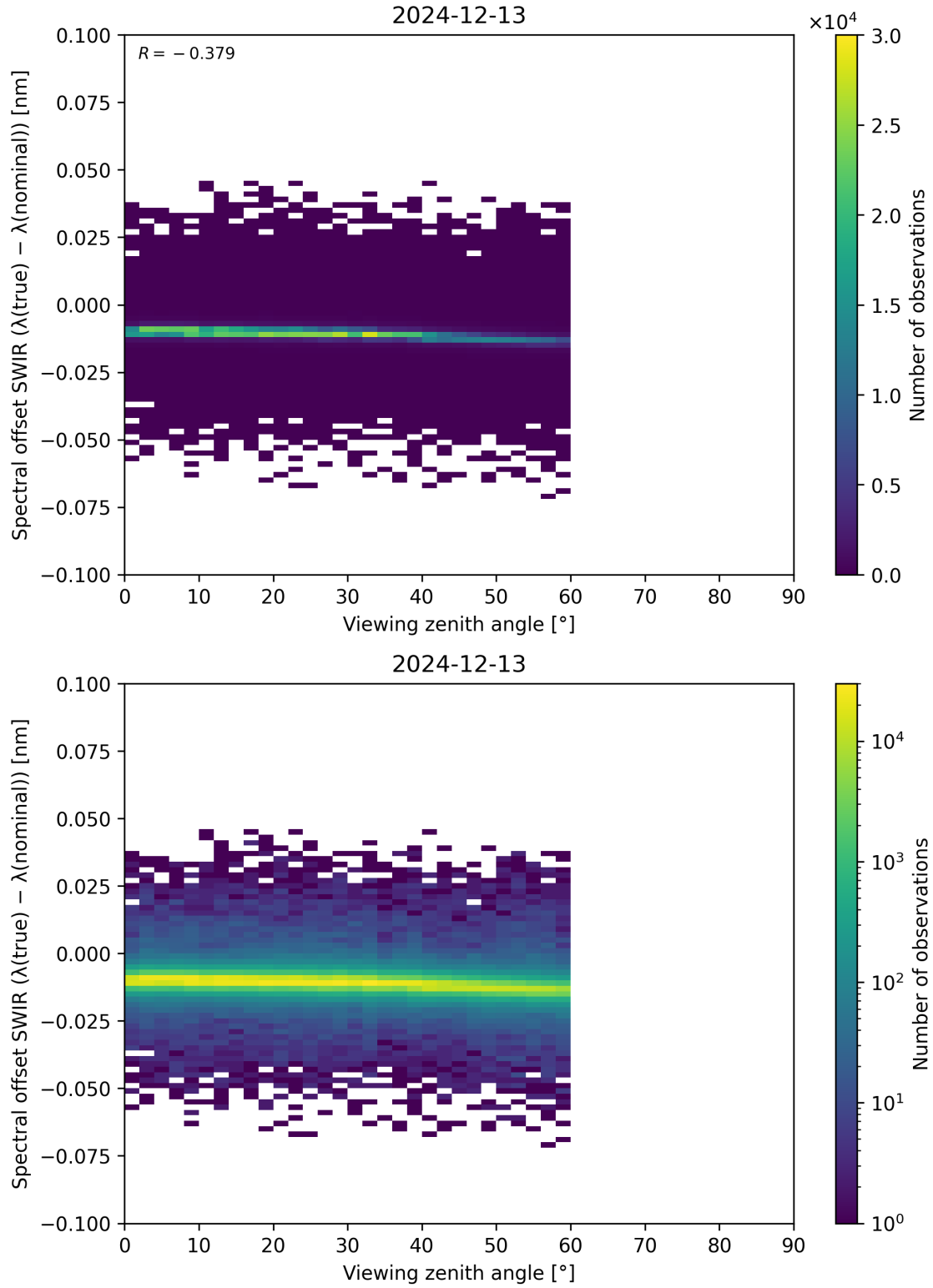
Figure 116: Scatter density plot of “Viewing zenith angle” against “Spectral offset SWIR ( \lambda_{\text{true}} - \lambda_{\text{nominal}} )” for 2024-12-12 to 2024-12-14.
