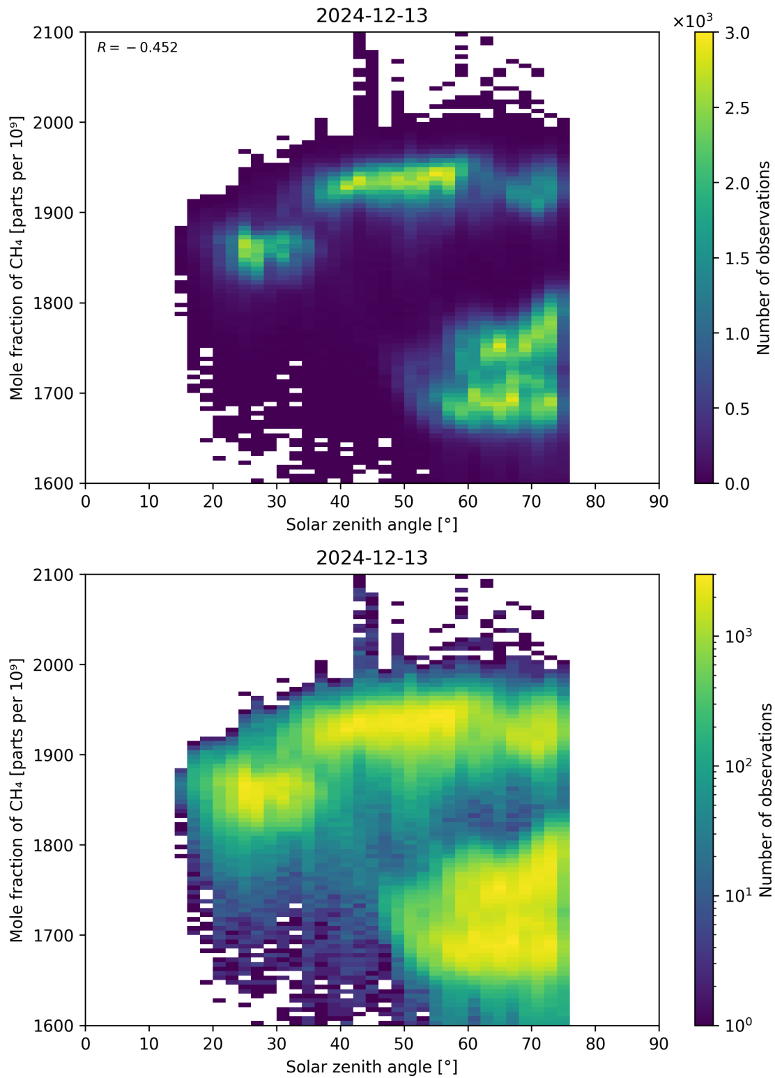
Figure 99: Scatter density plot of “Solar zenith angle” against “Mole fraction of CH 4 ” for 2024-12-12 to 2024-12-14.
