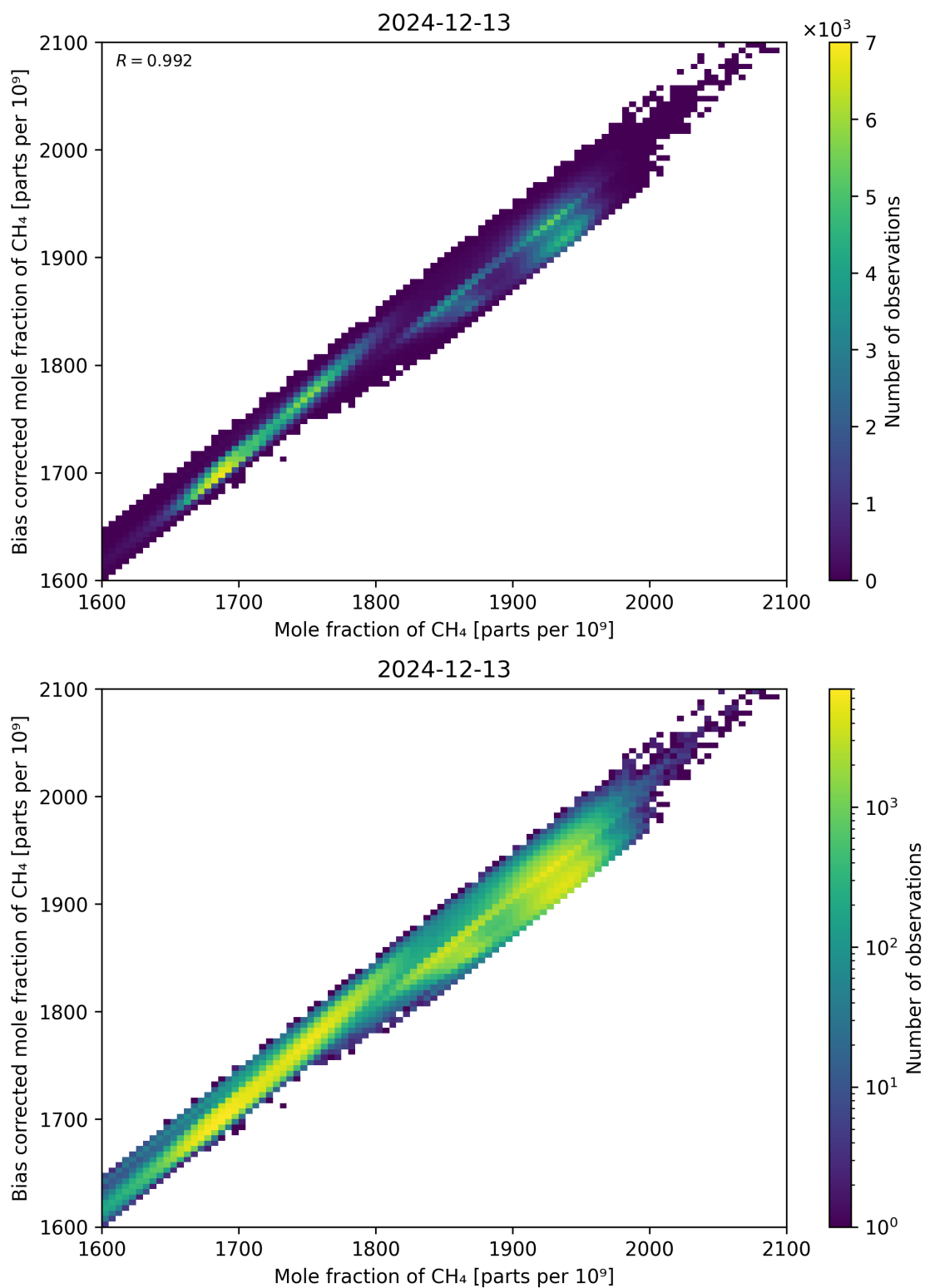
Figure 74: Scatter density plot of “Mole fraction of CH 4 ” against “Bias corrected mole fraction of CH 4 ” for 2024-12-12 to 2024-12-14.
