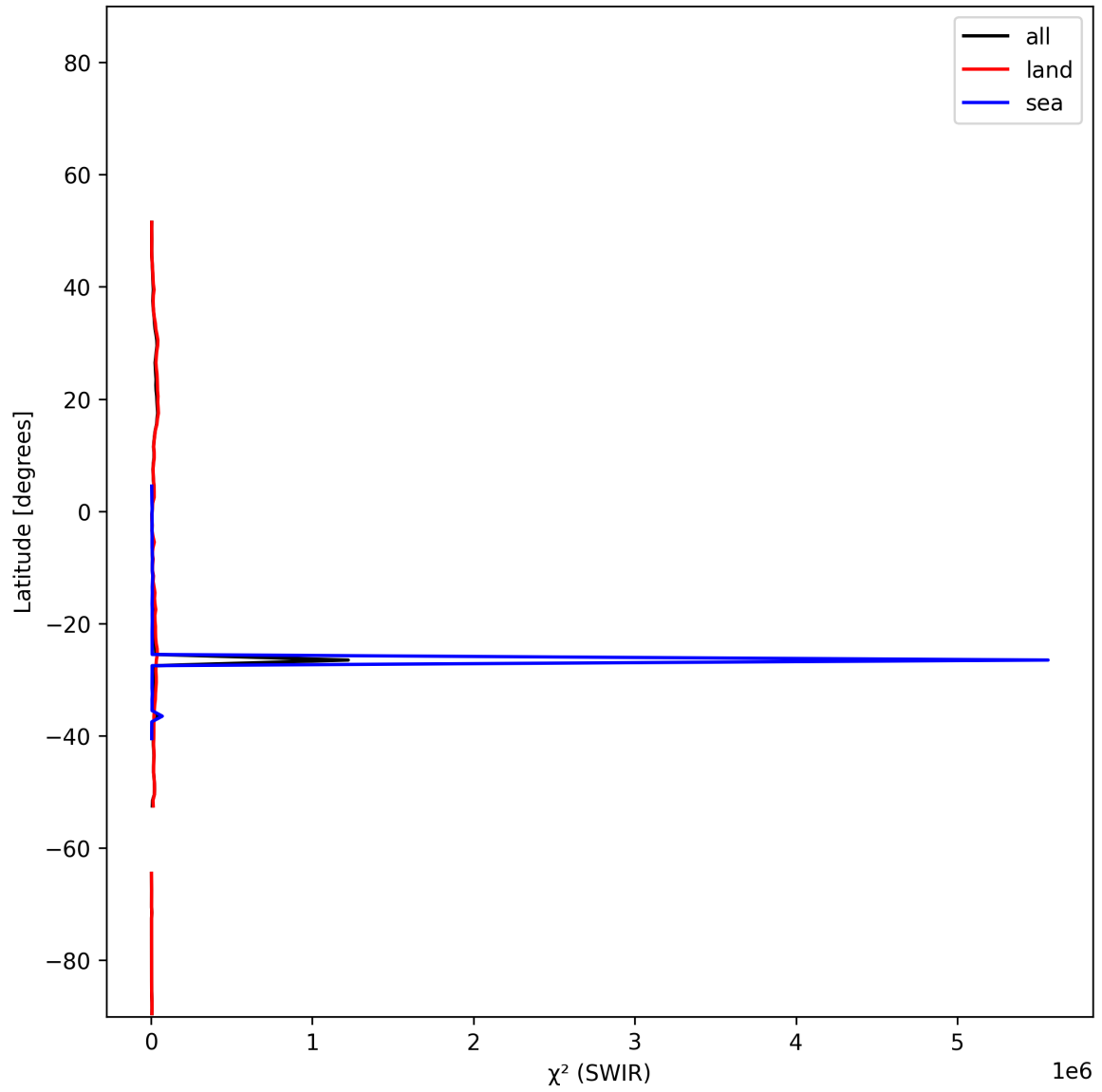
Figure 17: Zonal average of “ \chi^2 (SWIR)” for 2024-12-12 to 2024-12-14.
