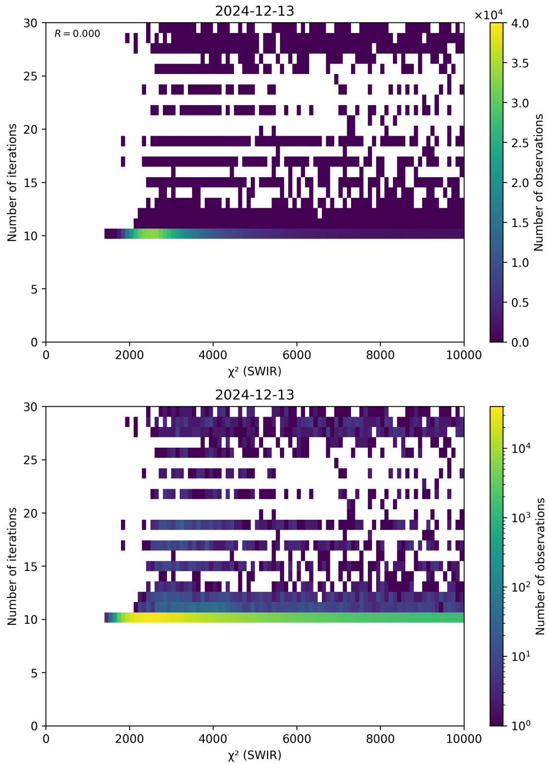
Figure 50: Scatter density plot of “ \chi^2 (SWIR)” against “Number of iterations” for 2024-12-12 to 2024-12-14.
