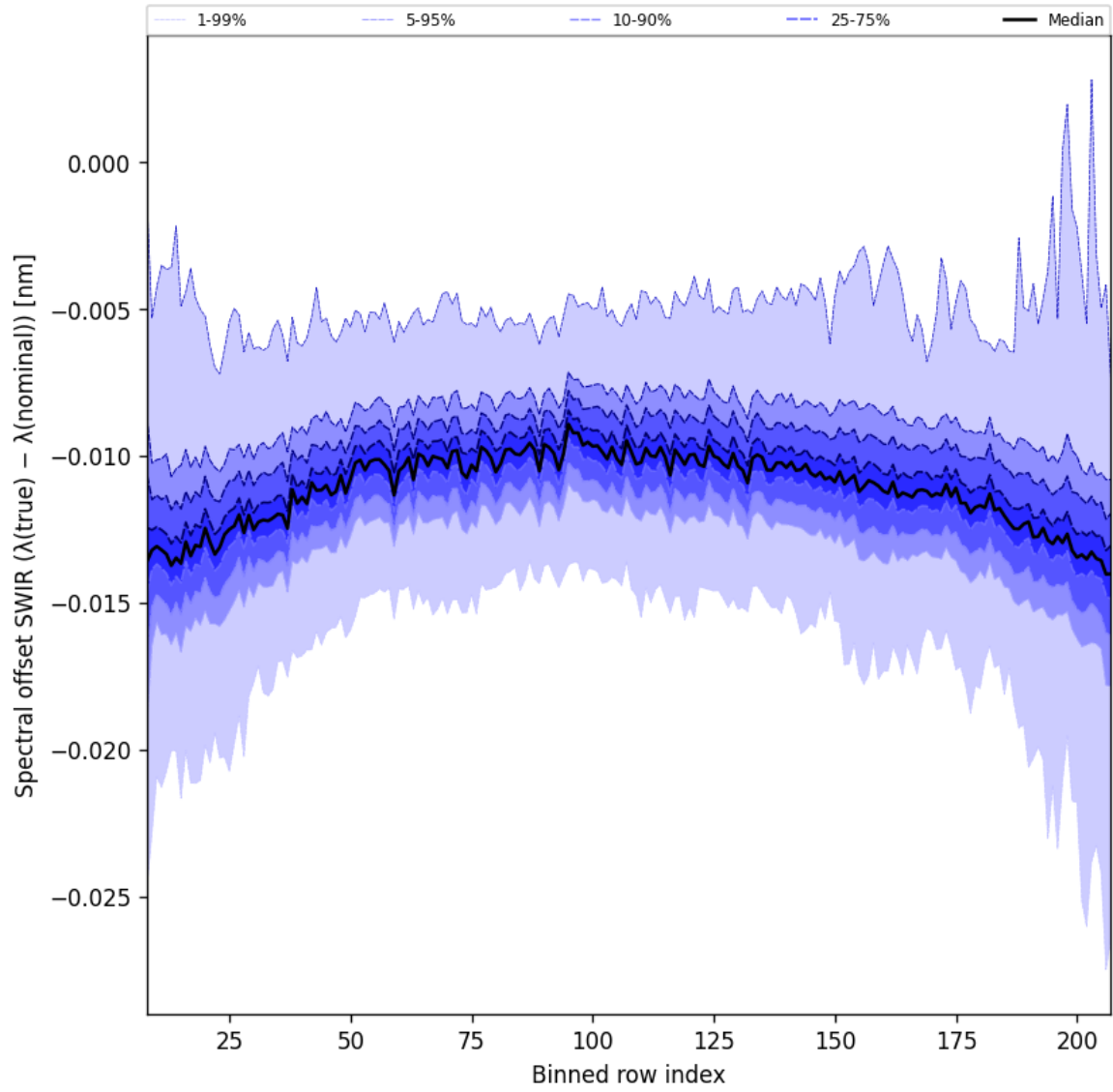
Figure 38: Along track statistics of “Spectral offset SWIR ( \lambda_{\text{true}} - \lambda_{\text{nominal}} )” for 2024-12-12 to 2024-12-14
