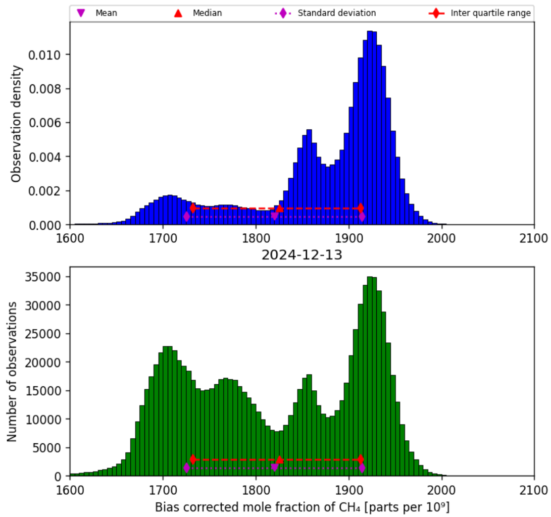
Figure 25: Histogram of “Bias corrected mole fraction of CH 4 ” for 2024-12-12 to 2024-12-14
