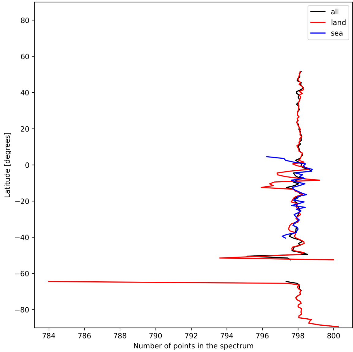
Figure 15: Zonal average of “Number of points in the spectrum” for 2024-12-12 to 2024-12-14.
