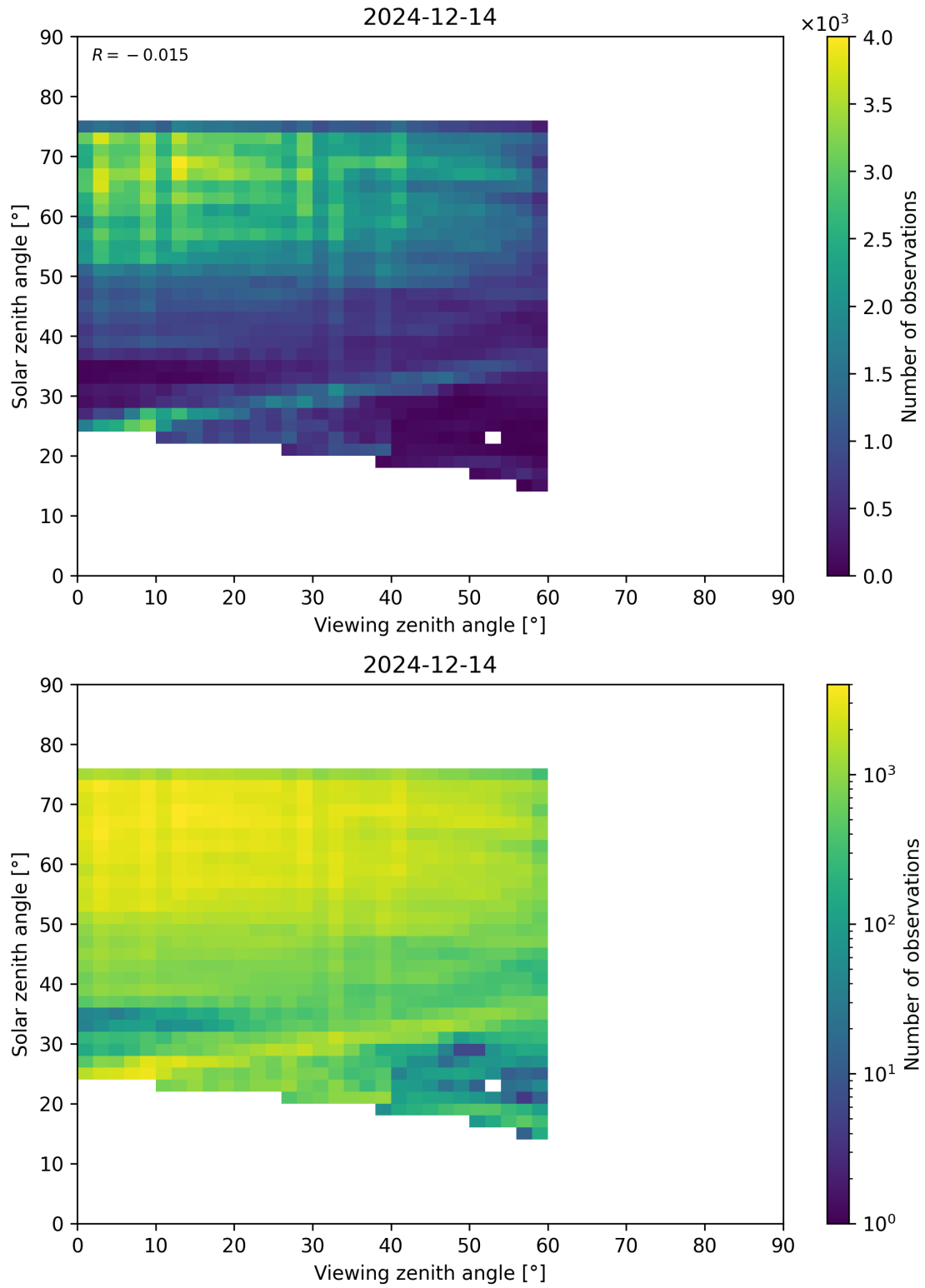
Figure 115: Scatter density plot of “Viewing zenith angle” against “Solar zenith angle” for 2024-12-13 to 2024-12-15.
