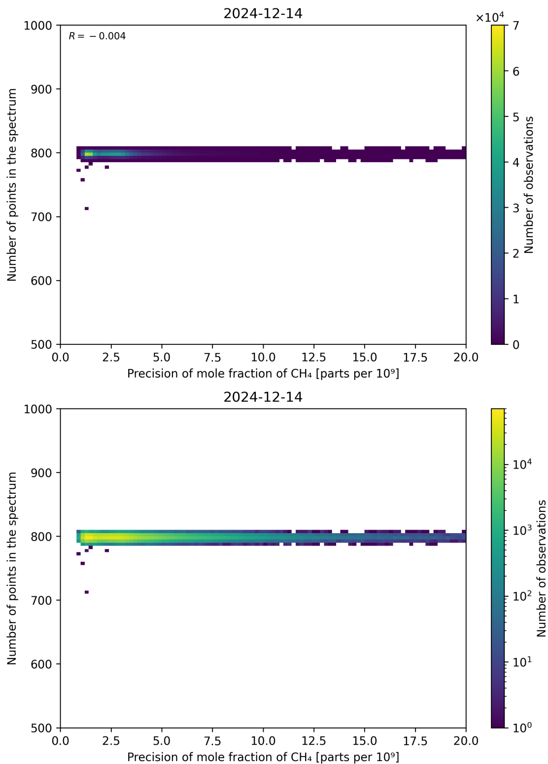
Figure 84: Scatter density plot of “Precision of mole fraction of CH 4 ” against “Number of points in the spectrum” for 2024-12-13 to 2024-12-15.
