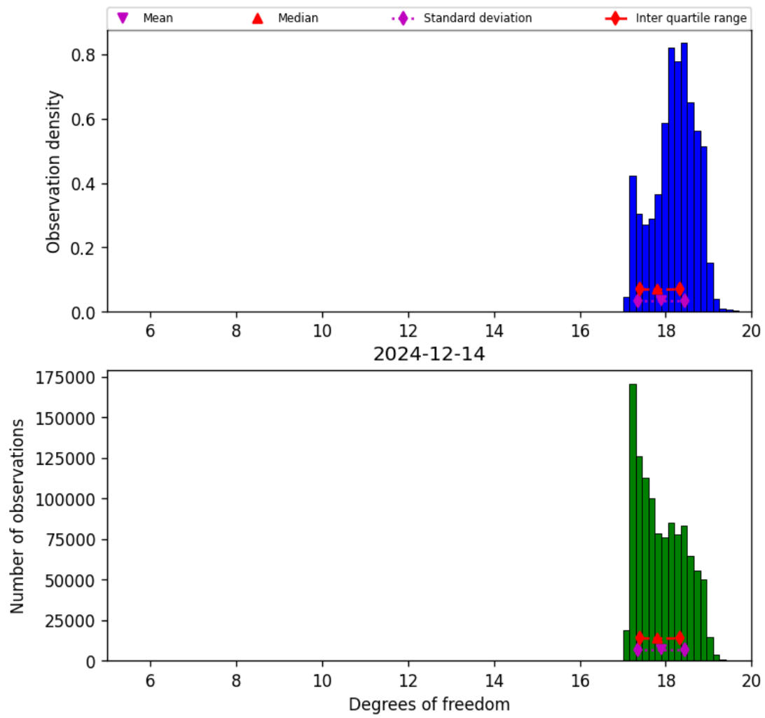
Figure 30: Histogram of “Degrees of freedom” for 2024-12-13 to 2024-12-15
