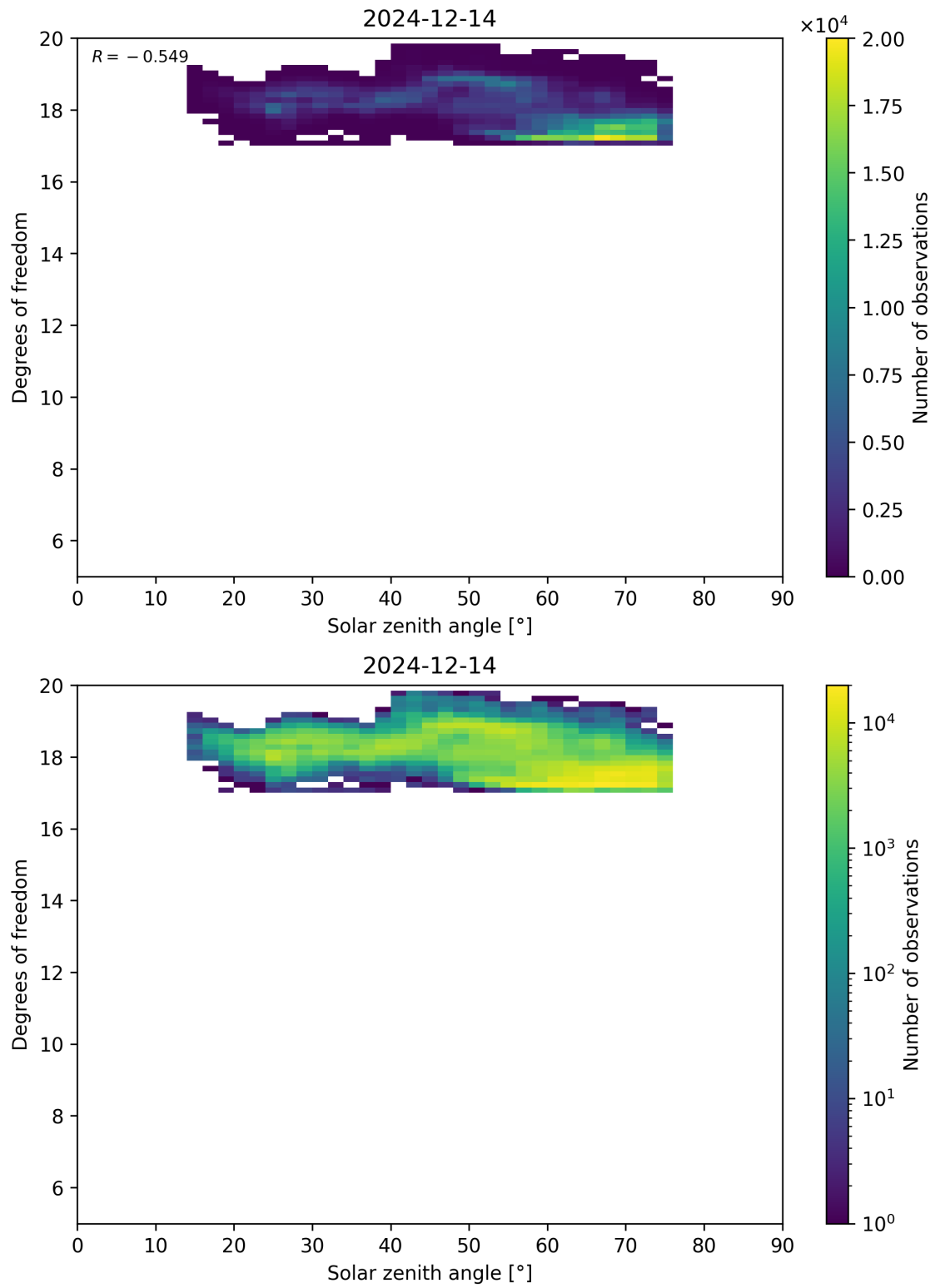
Figure 96: Scatter density plot of “Solar zenith angle” against “Degrees of freedom” for 2024-12-13 to 2024-12-15.
