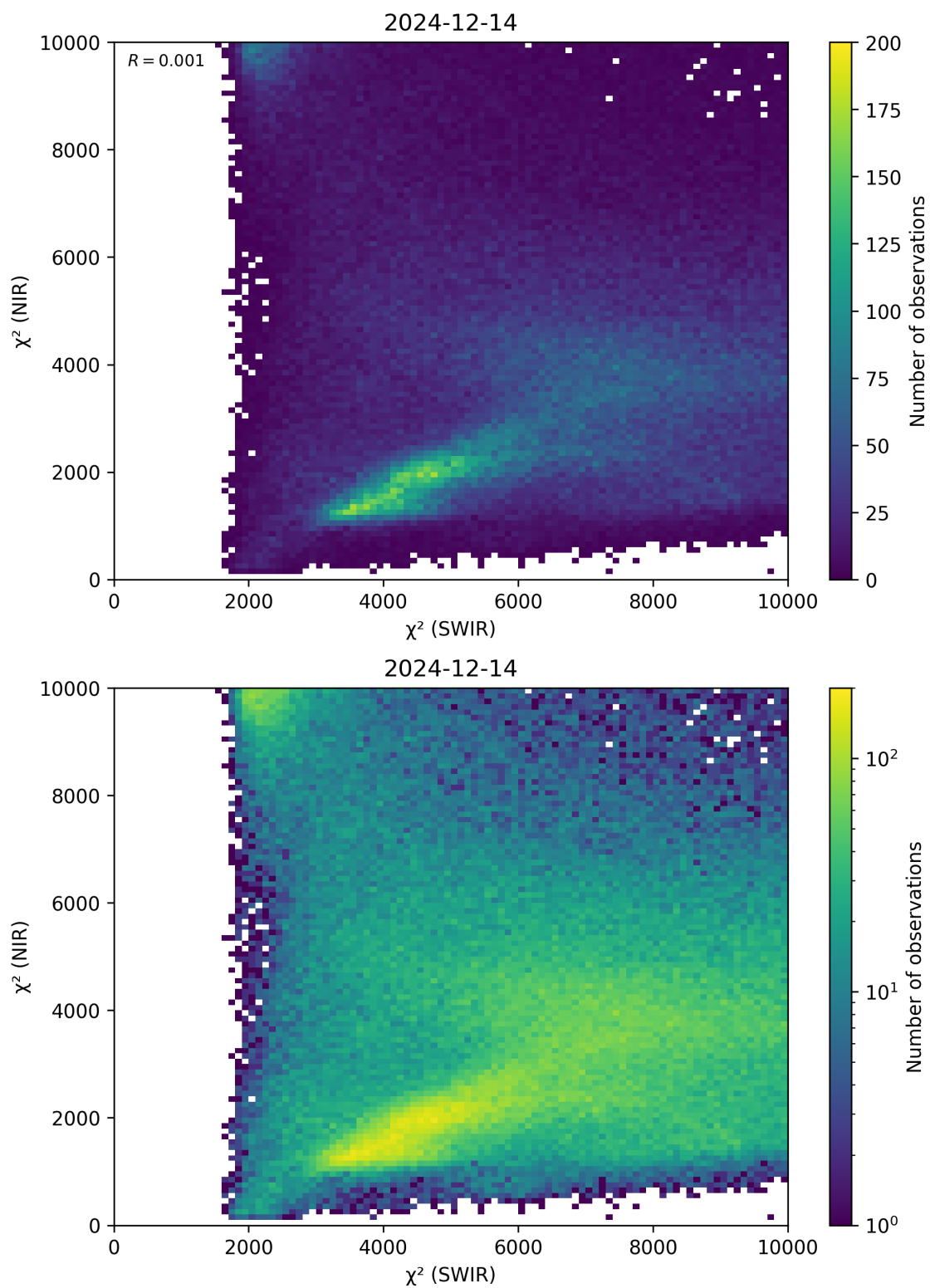
Figure 47: Scatter density plot of “ \chi^2 (SWIR)” against “ \chi^2 (NIR)” for 2024-12-13 to 2024-12-15.
