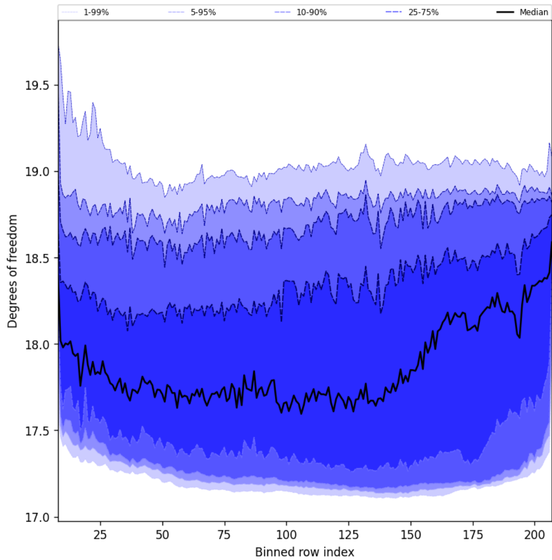
Figure 41: Along track statistics of “Degrees of freedom” for 2024-12-13 to 2024-12-15
