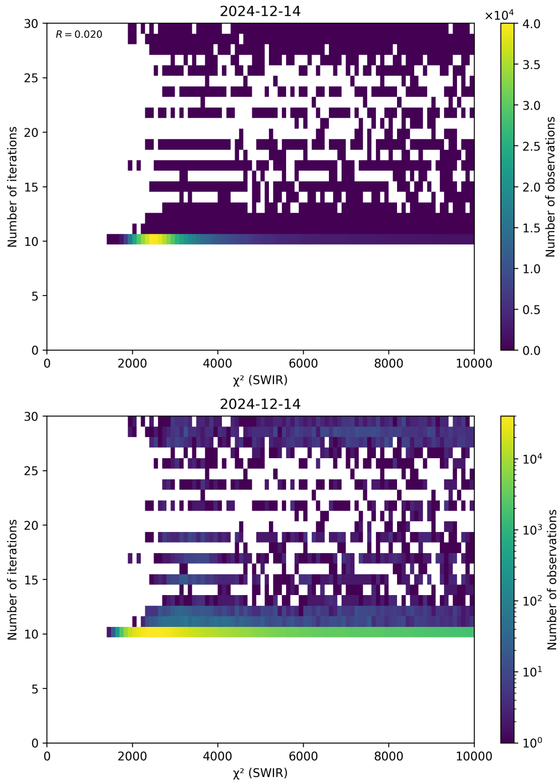
Figure 50: Scatter density plot of “ \chi^2 (SWIR)” against “Number of iterations” for 2024-12-13 to 2024-12-15.
