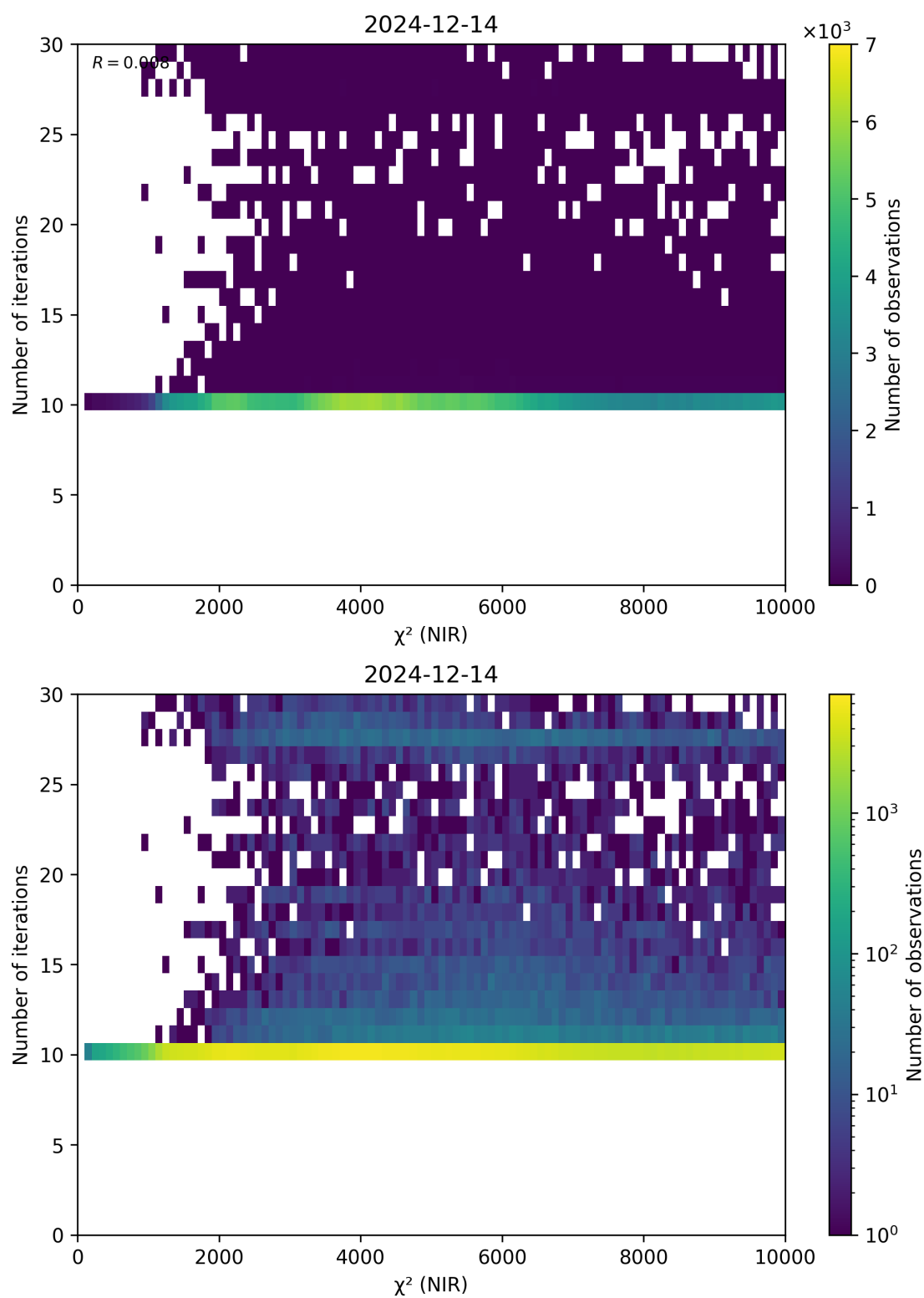
Figure 46: Scatter density plot of “ \chi^2 (NIR)” against “Number of iterations” for 2024-12-13 to 2024-12-15.
