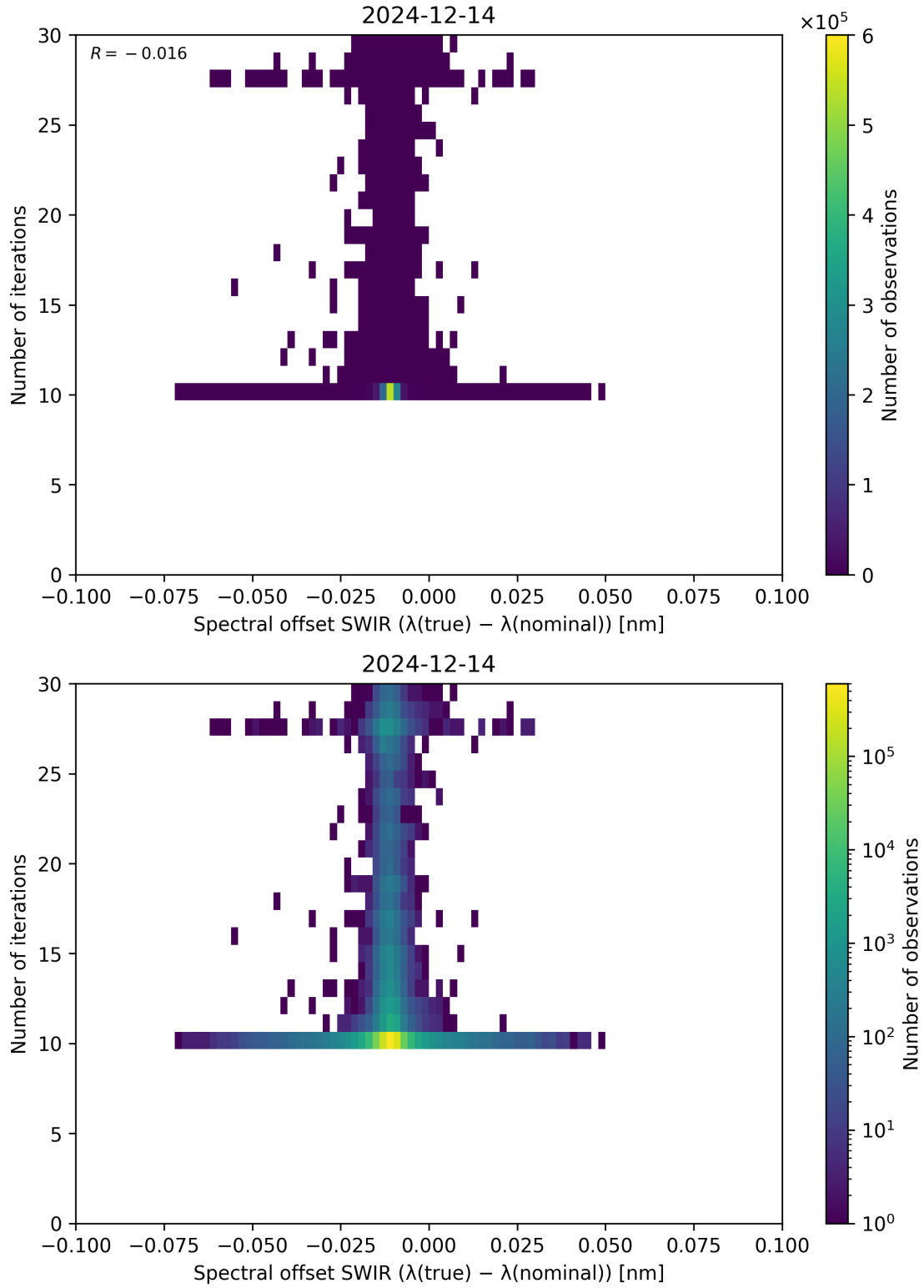
Figure 121: Scatter density plot of “Spectral offset SWIR ( \lambda_{\text{true}} - \lambda_{\text{nominal}} )” against “Number of iterations” for 2024-12-13 to 2024-12-15.
