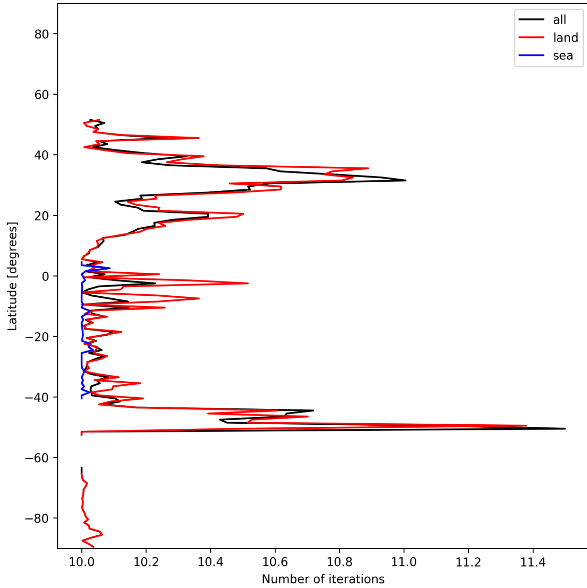
Figure 20: Zonal average of “Number of iterations” for 2024-12-13 to 2024-12-15.
