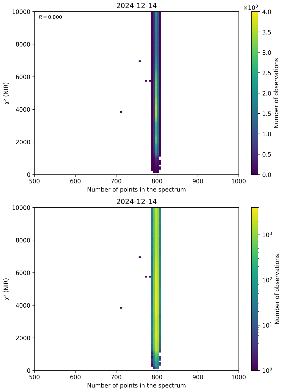
Figure 88: Scatter density plot of “Number of points in the spectrum” against “ \chi^2 (NIR)” for 2024-12-13 to 2024-12-15.
