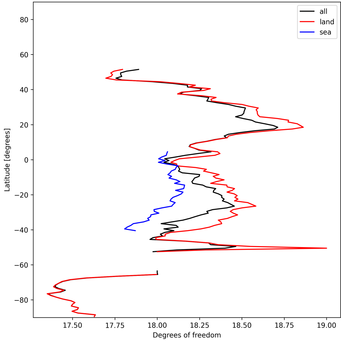
Figure 19: Zonal average of “Degrees of freedom” for 2024-12-13 to 2024-12-15.
