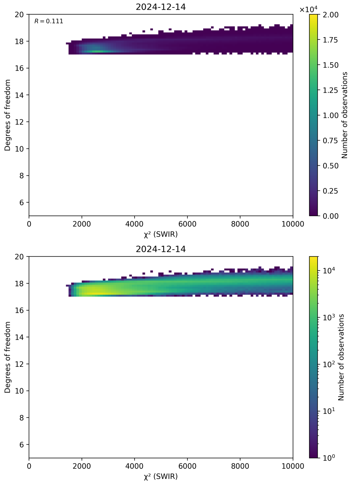
Figure 48: Scatter density plot of “ \chi^2 (SWIR)” against “Degrees of freedom” for 2024-12-13 to 2024-12-15.
