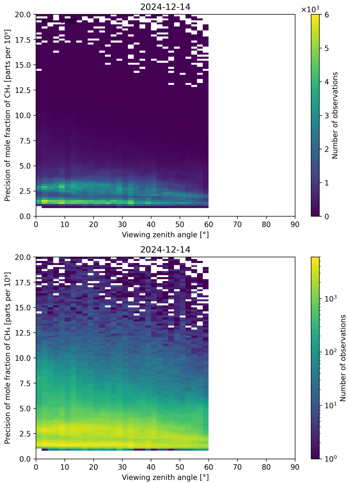
Figure 112: Scatter density plot of “Viewing zenith angle” against “Precision of mole fraction of CH 4 ” for 2024-12-13 to 2024-12-15.
