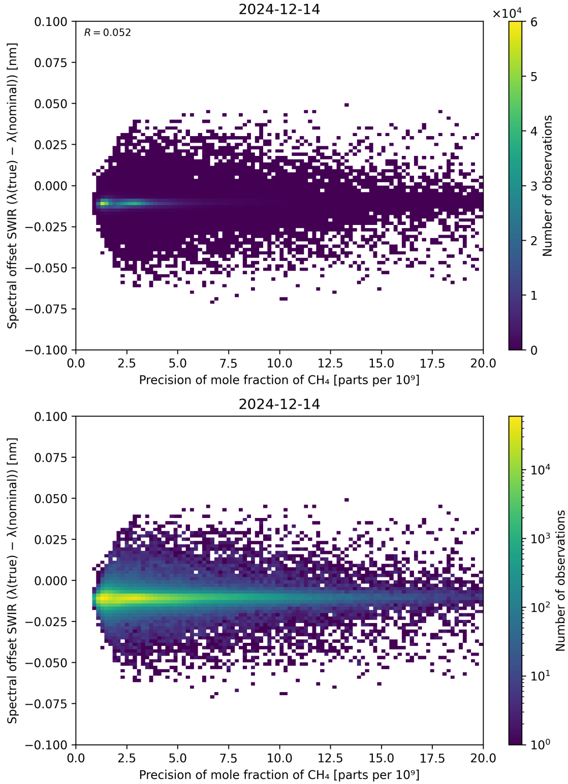
Figure 85: Scatter density plot of “Precision of mole fraction of CH 4 ” against “Spectral offset SWIR ( \lambda_{\text{true}} - \lambda_{\text{nominal}} )” for 2024-12-13 to 2024-12-15.
