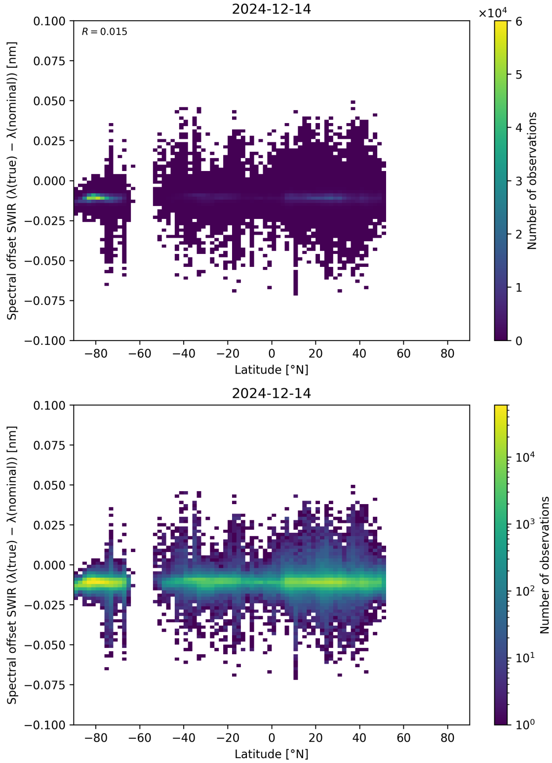
Figure 62: Scatter density plot of “Latitude” against “Spectral offset SWIR ( \lambda_{\text{true}} - \lambda_{\text{nominal}} )” for 2024-12-13 to 2024-12-15.
