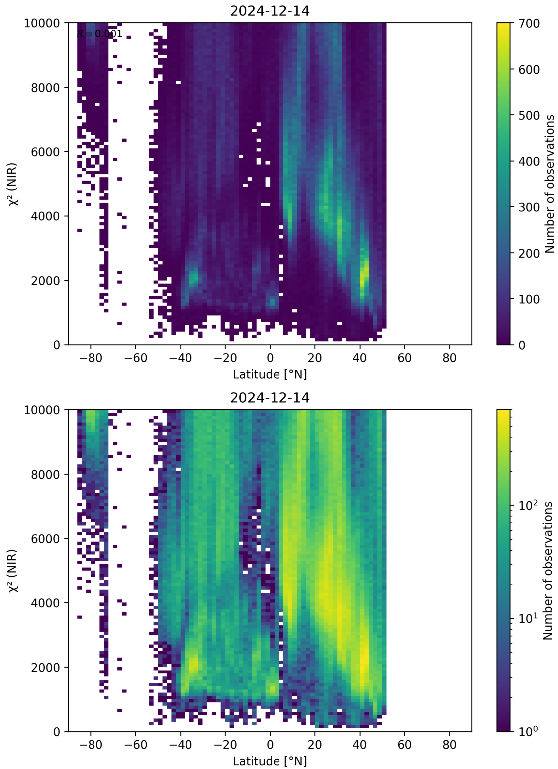
Figure 53: Scatter density plot of “Latitude” against “ \chi^2 (NIR)” for 2024-12-13 to 2024-12-15.
