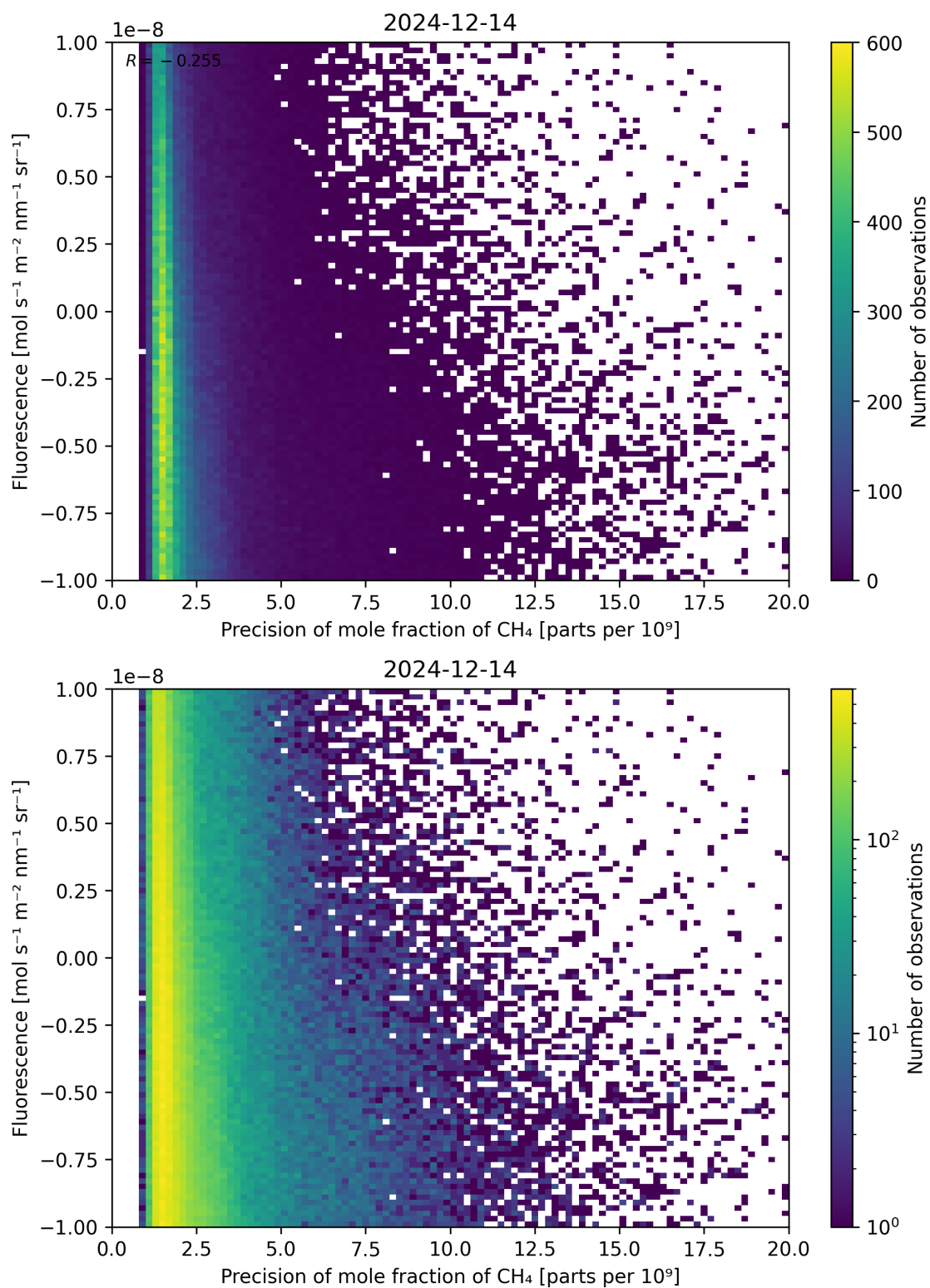
Figure 81: Scatter density plot of “Precision of mole fraction of \text{CH}_4 ” against “Fluorescence” for 2024-12-13 to 2024-12-15.
