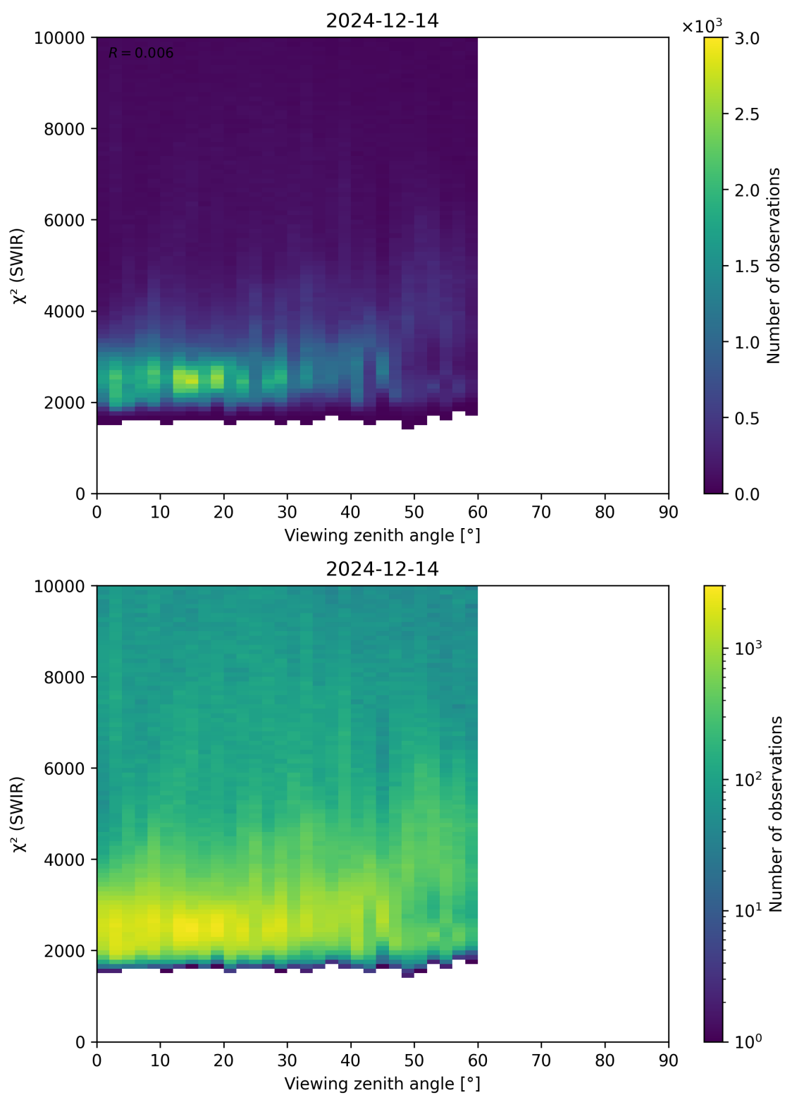
Figure 106: Scatter density plot of “Viewing zenith angle” against “ \chi^2 (SWIR)” for 2024-12-13 to 2024-12-15.
