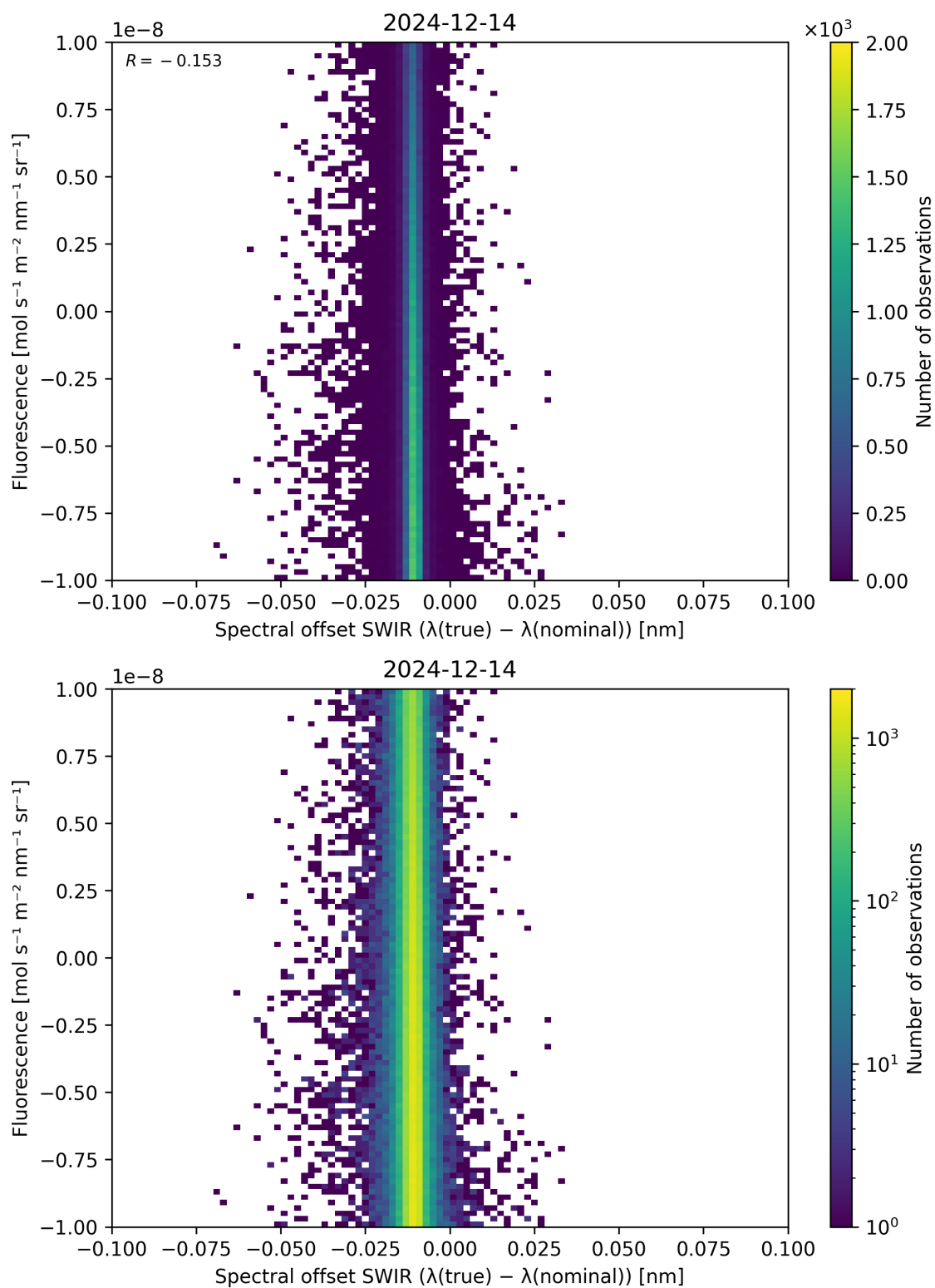
Figure 120: Scatter density plot of “Spectral offset SWIR ( \lambda_{\text{true}} - \lambda_{\text{nominal}} )” against “Fluorescence” for 2024-12-13 to 2024-12-15.
