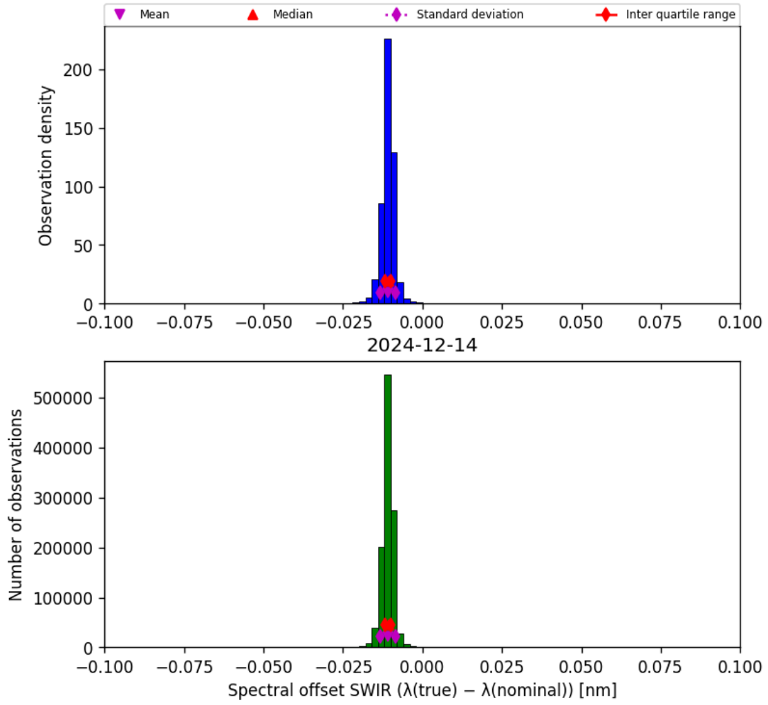
Figure 27: Histogram of “Spectral offset SWIR ( \lambda_{\text{true}} - \lambda_{\text{nominal}} )” for 2024-12-13 to 2024-12-15
