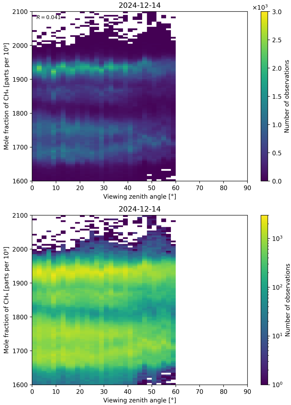
Figure 110: Scatter density plot of “Viewing zenith angle” against “Mole fraction of CH 4 ” for 2024-12-13 to 2024-12-15.
