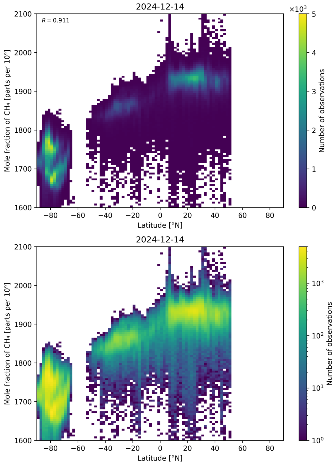
Figure 57: Scatter density plot of “Latitude” against “Mole fraction of \text{CH}_4 ” for 2024-12-13 to 2024-12-15.
