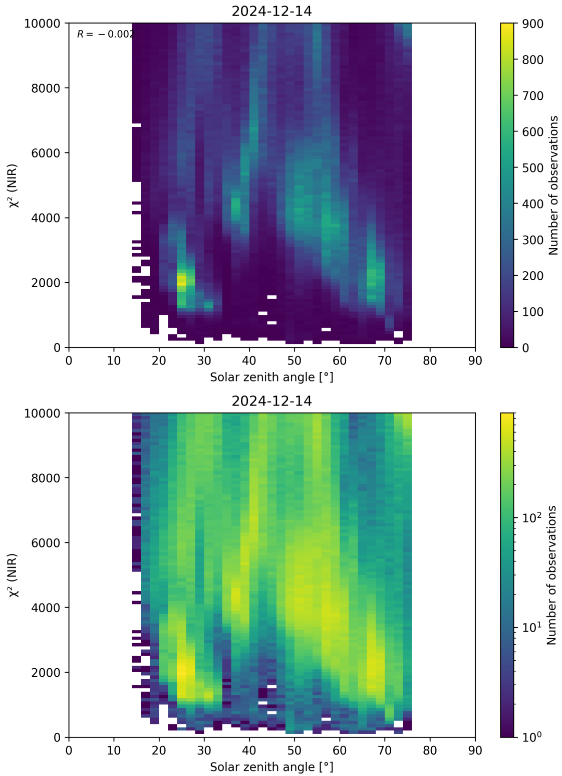
Figure 94: Scatter density plot of “Solar zenith angle” against “ \chi^2 (NIR)” for 2024-12-13 to 2024-12-15.
