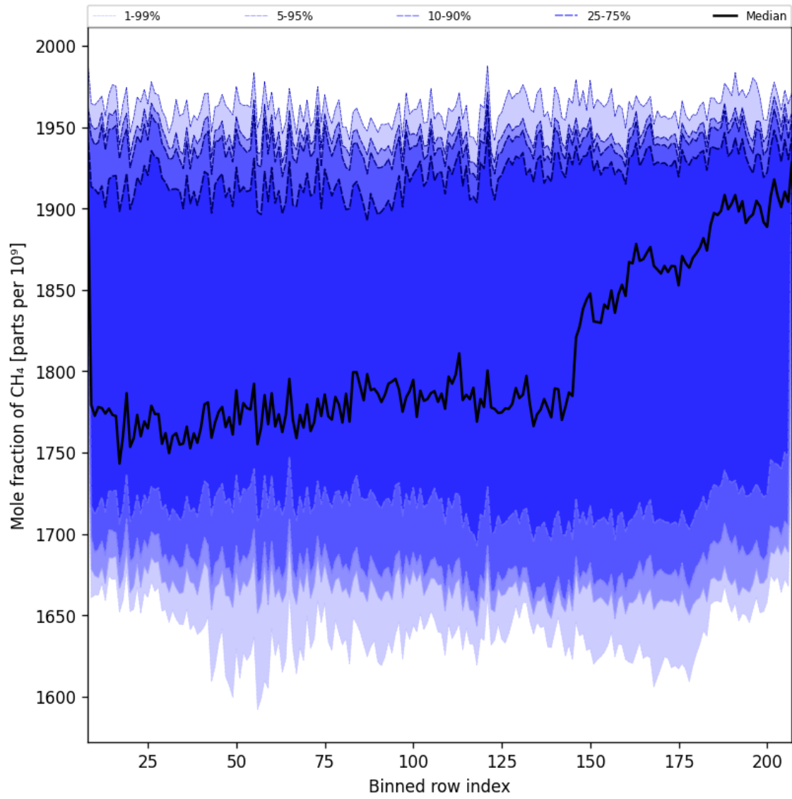
Figure 34: Along track statistics of “Mole fraction of CH 4 ” for 2024-12-13 to 2024-12-15
