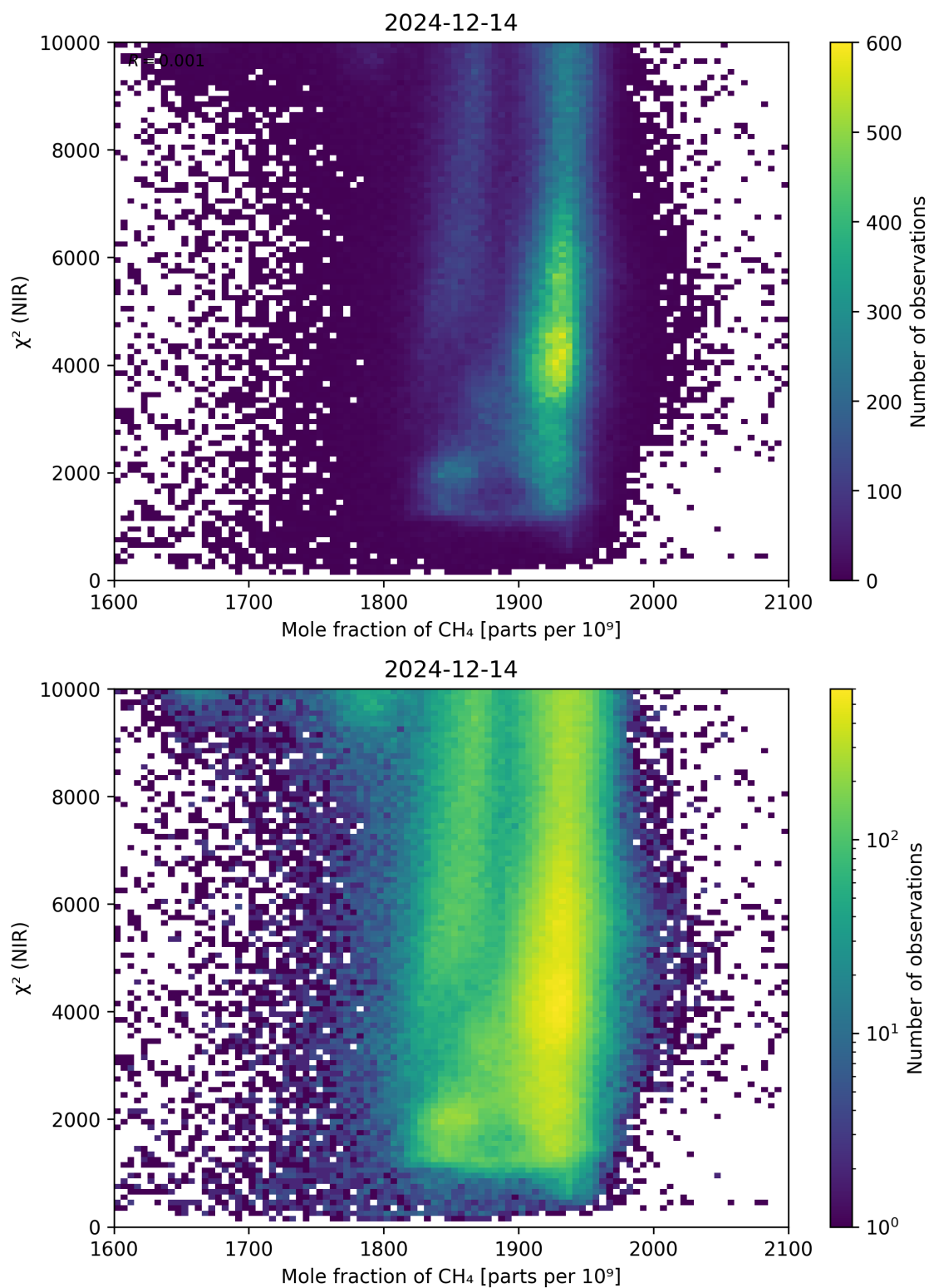
Figure 70: Scatter density plot of “Mole fraction of \text{CH}_4 ” against “ \chi^2 (NIR)” for 2024-12-13 to 2024-12-15.
