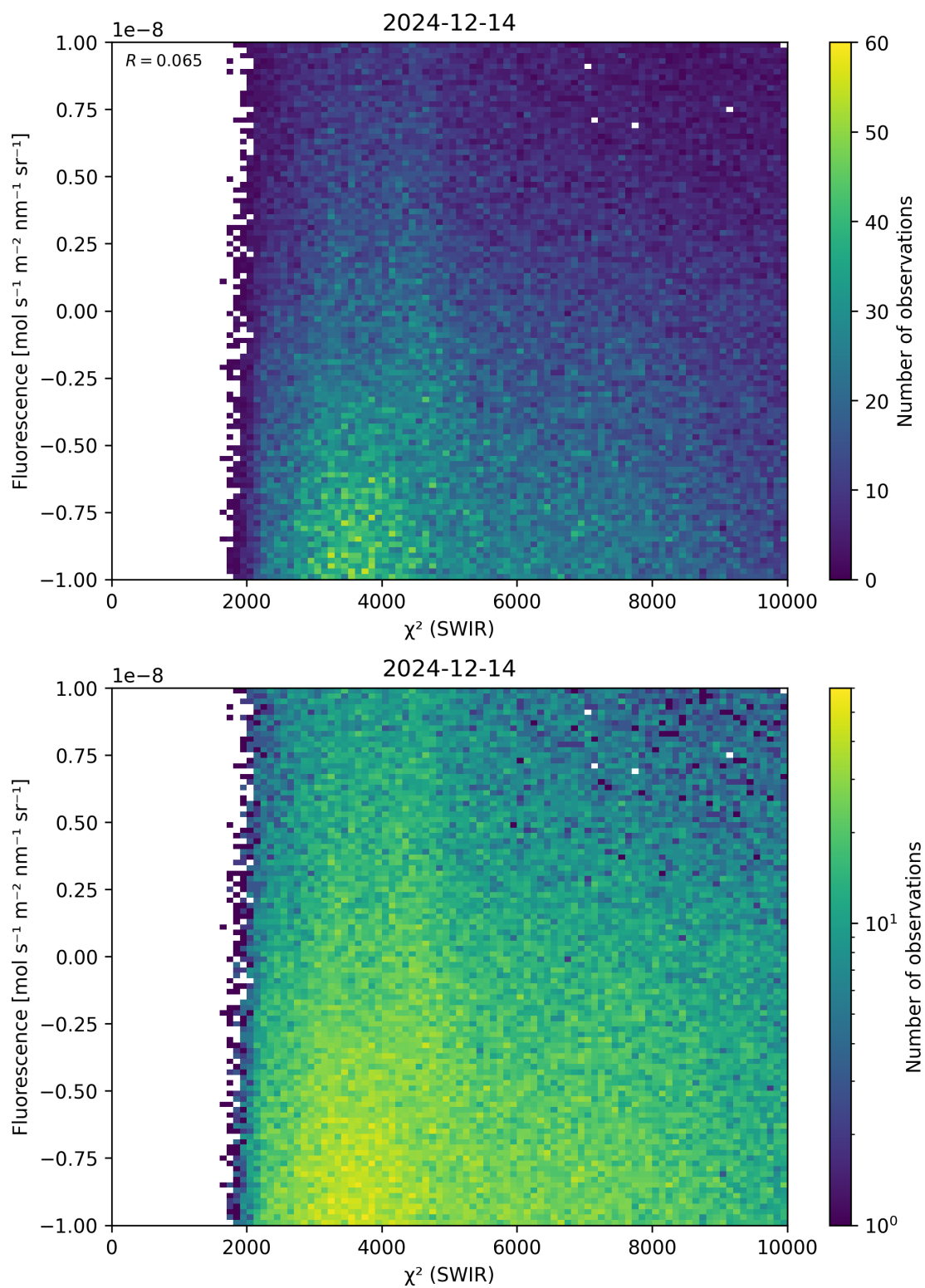
Figure 49: Scatter density plot of “ \chi^2 (SWIR)” against “Fluorescence” for 2024-12-13 to 2024-12-15.
