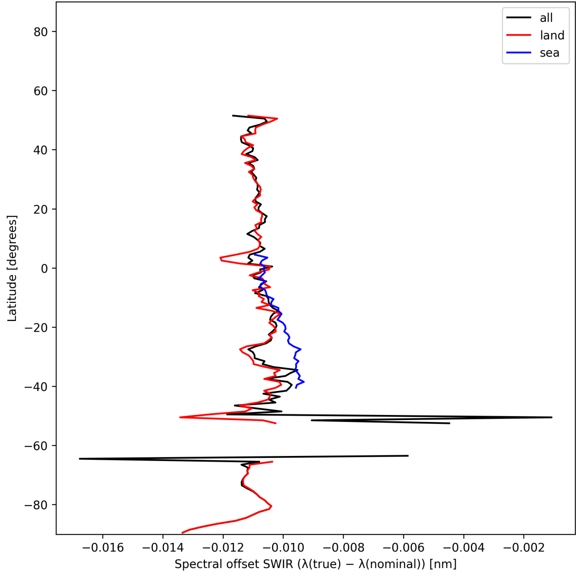
Figure 16: Zonal average of “Spectral offset SWIR ( \lambda_{\text{true}} - \lambda_{\text{nominal}} )” for 2024-12-13 to 2024-12-15.
