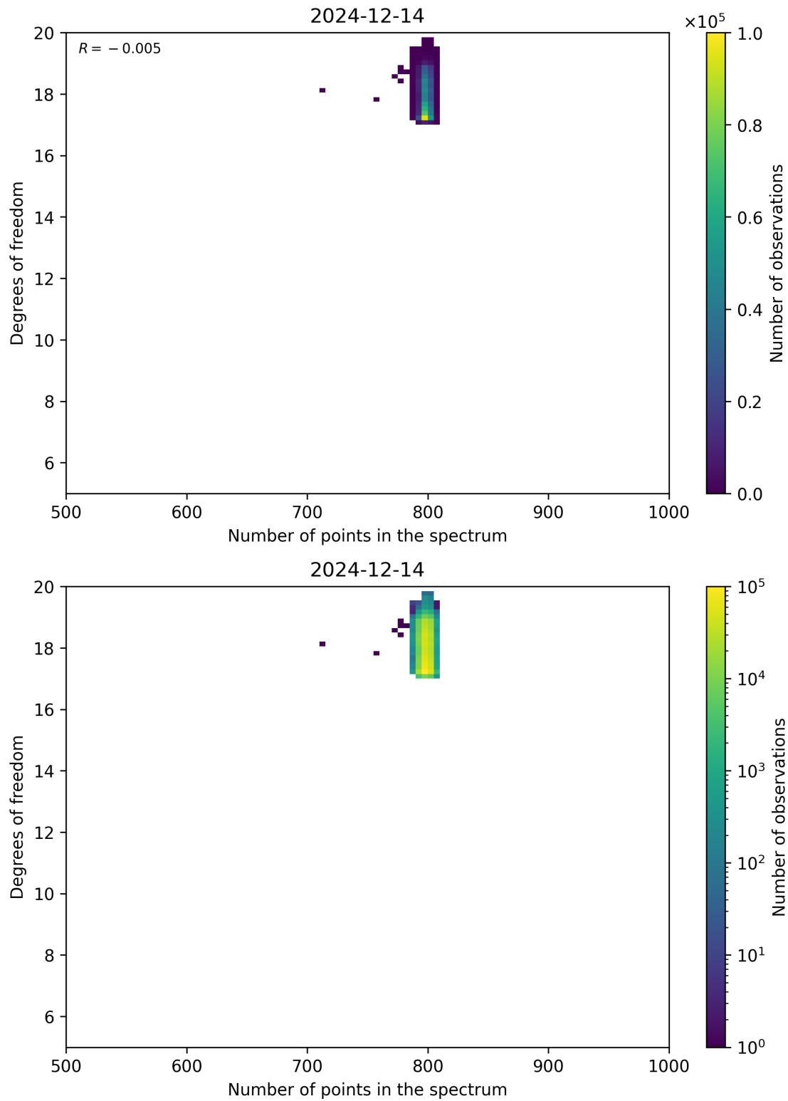
Figure 90: Scatter density plot of “Number of points in the spectrum” against “Degrees of freedom” for 2024-12-13 to 2024-12-15.
