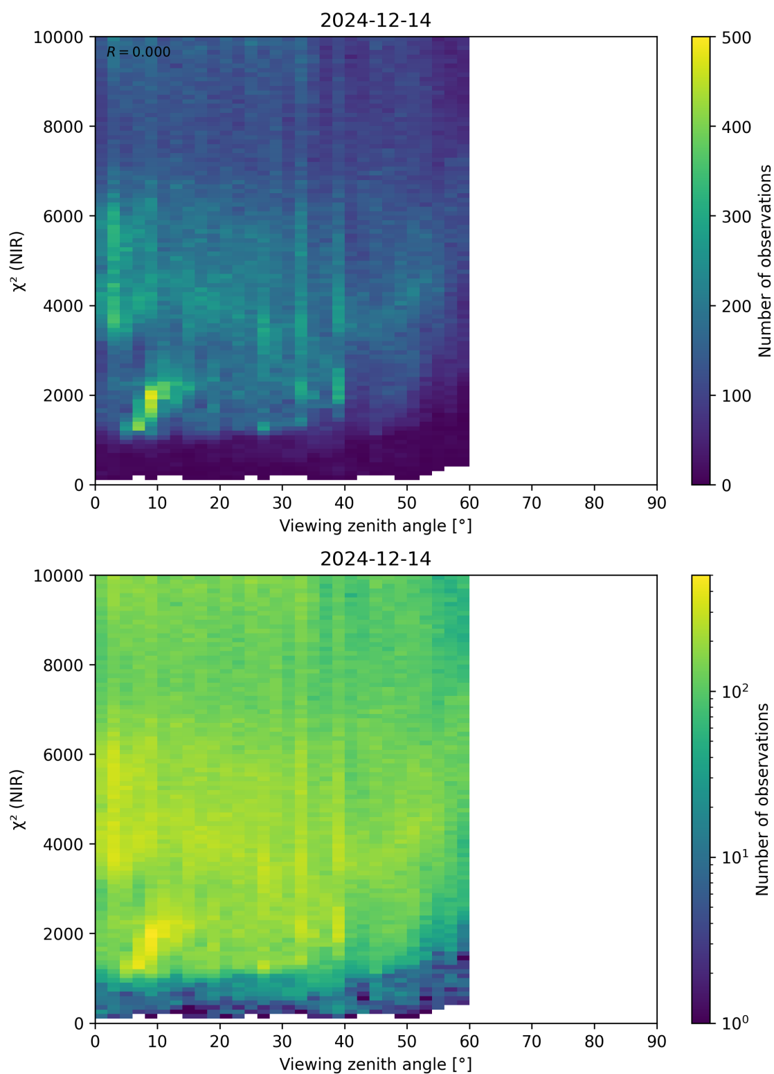
Figure 105: Scatter density plot of “Viewing zenith angle” against “ \chi^2 (NIR)” for 2024-12-13 to 2024-12-15.
