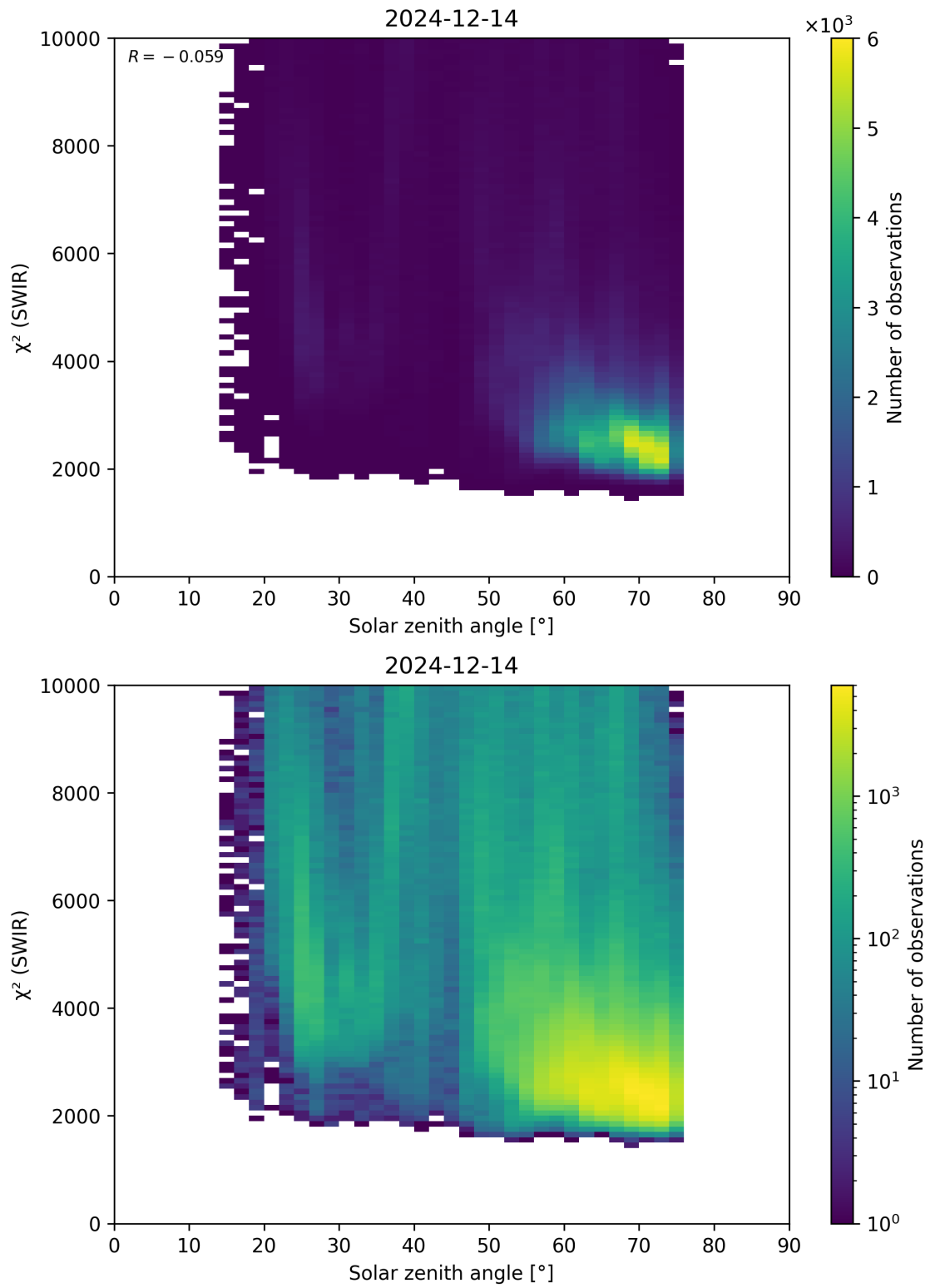
Figure 95: Scatter density plot of “Solar zenith angle” against “ \chi^2 (SWIR)” for 2024-12-13 to 2024-12-15.
