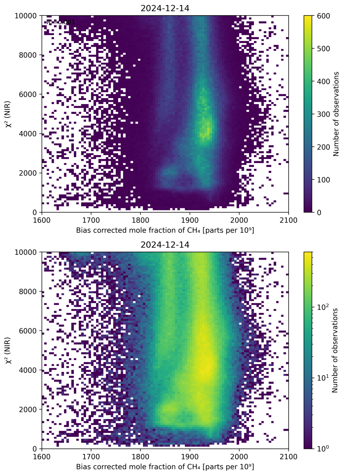
Figure 63: Scatter density plot of “Bias corrected mole fraction of \text{CH}_4 ” against “ \chi^2 (NIR)” for 2024-12-13 to 2024-12-15.
