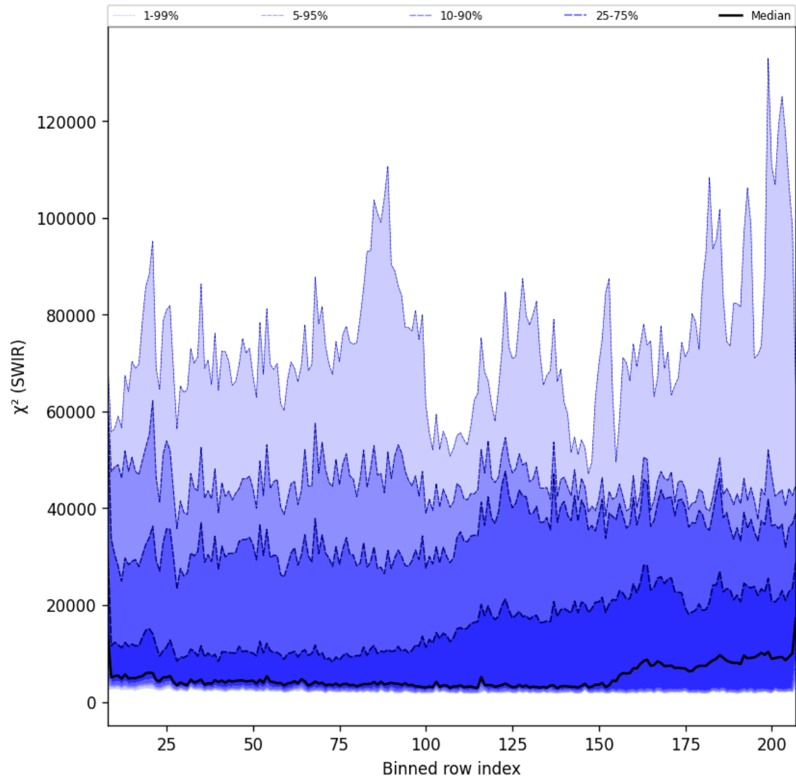
Figure 39: Along track statistics of “ \chi^2 (SWIR)” for 2024-12-13 to 2024-12-15
