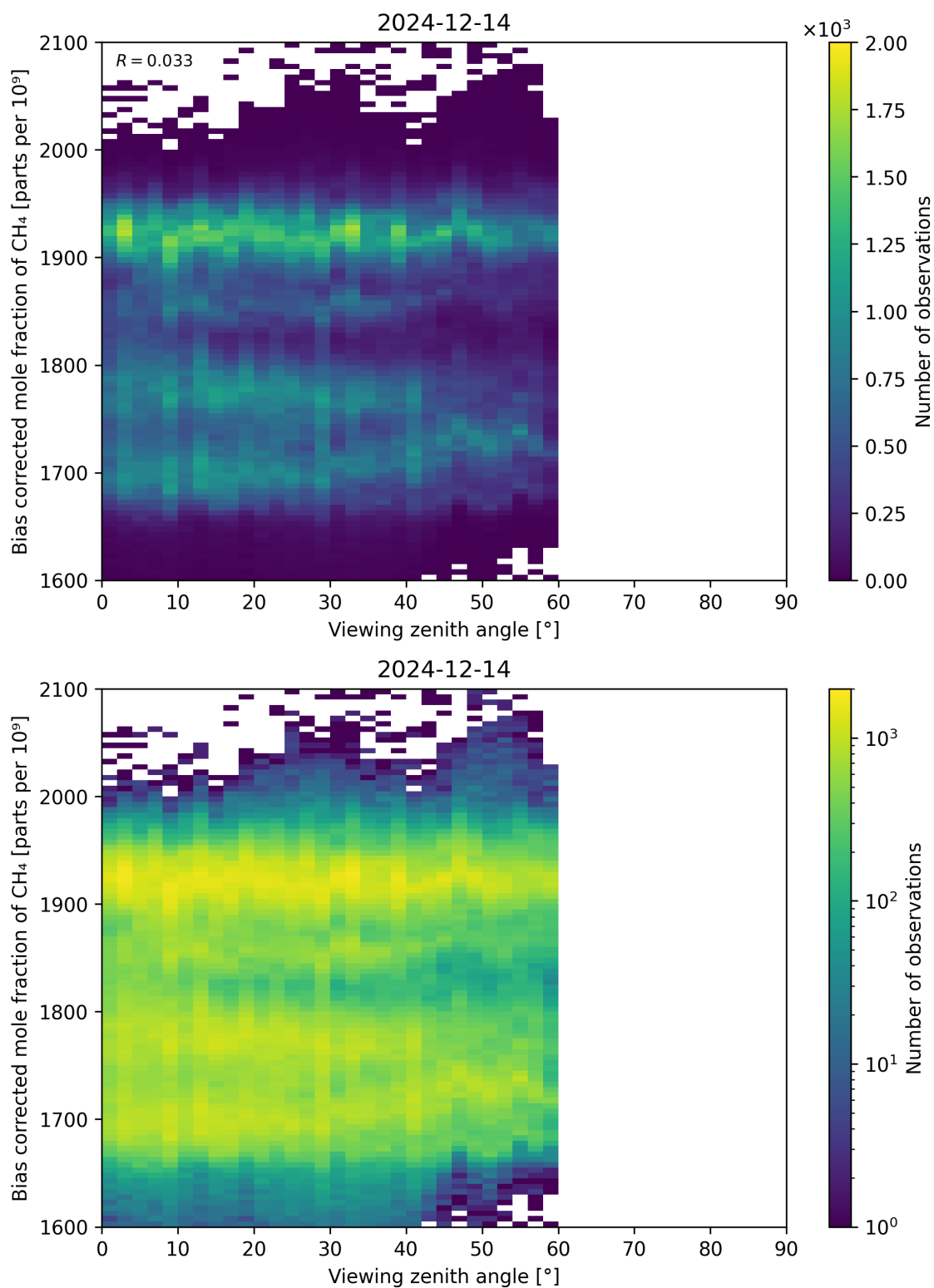
Figure 111: Scatter density plot of “Viewing zenith angle” against “Bias corrected mole fraction of CH 4 ” for 2024-12-13 to 2024-12-15.
