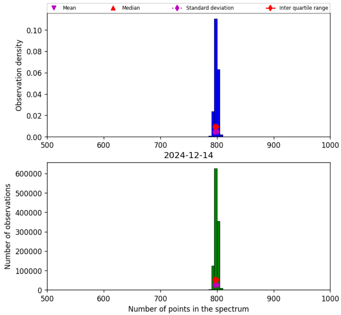
Figure 26: Histogram of “Number of points in the spectrum” for 2024-12-13 to 2024-12-15
