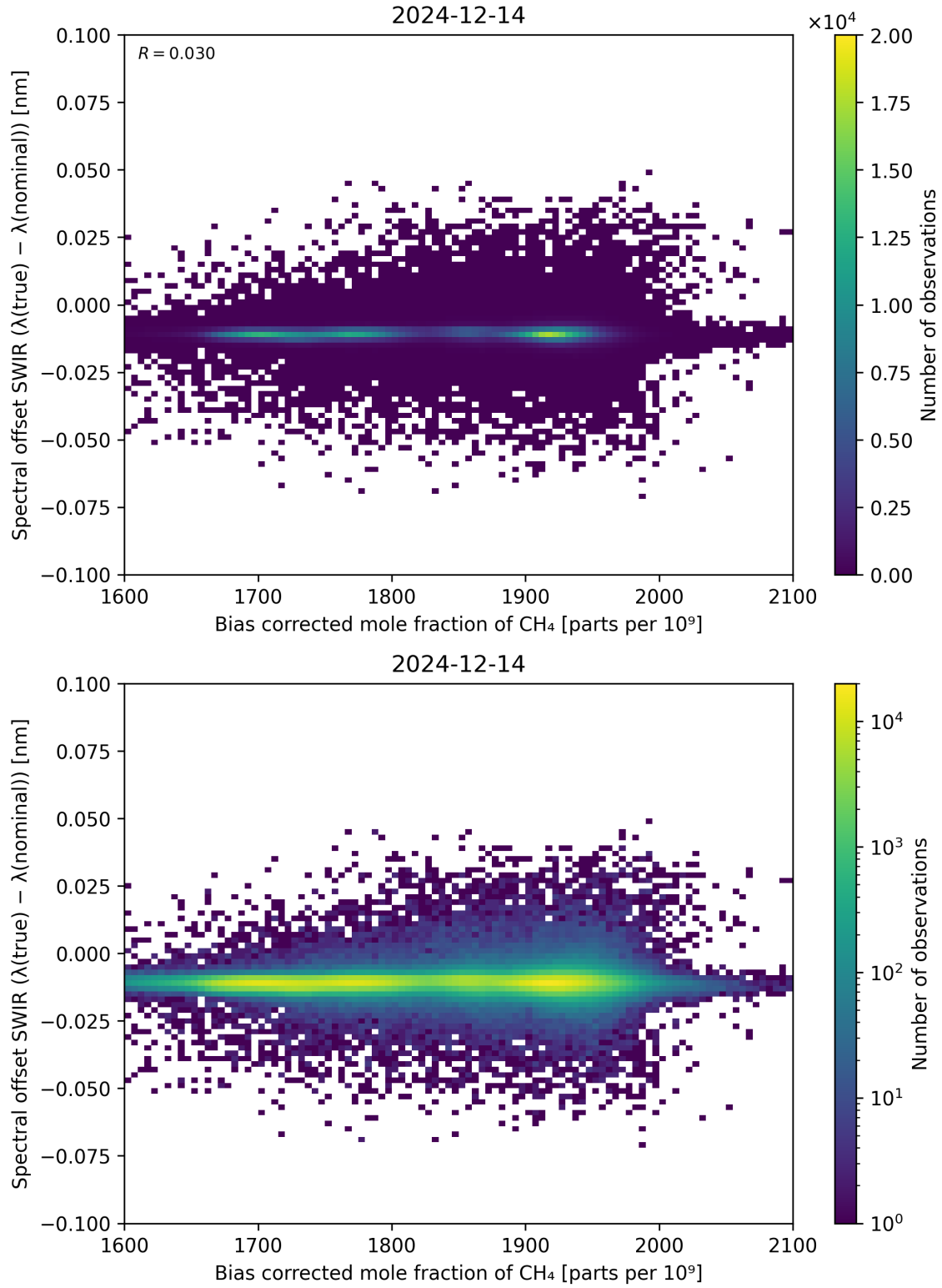
Figure 69: Scatter density plot of “Bias corrected mole fraction of \text{CH}_4 ” against “Spectral offset SWIR ( \lambda_{\text{true}} - \lambda_{\text{nominal}} )” for 2024-12-13 to 2024-12-15.
