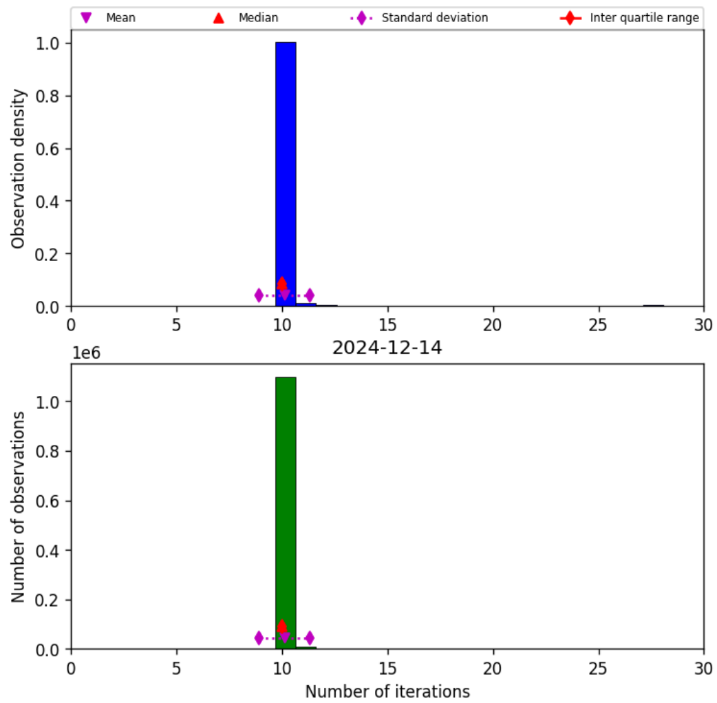
Figure 31: Histogram of “Number of iterations” for 2024-12-13 to 2024-12-15
