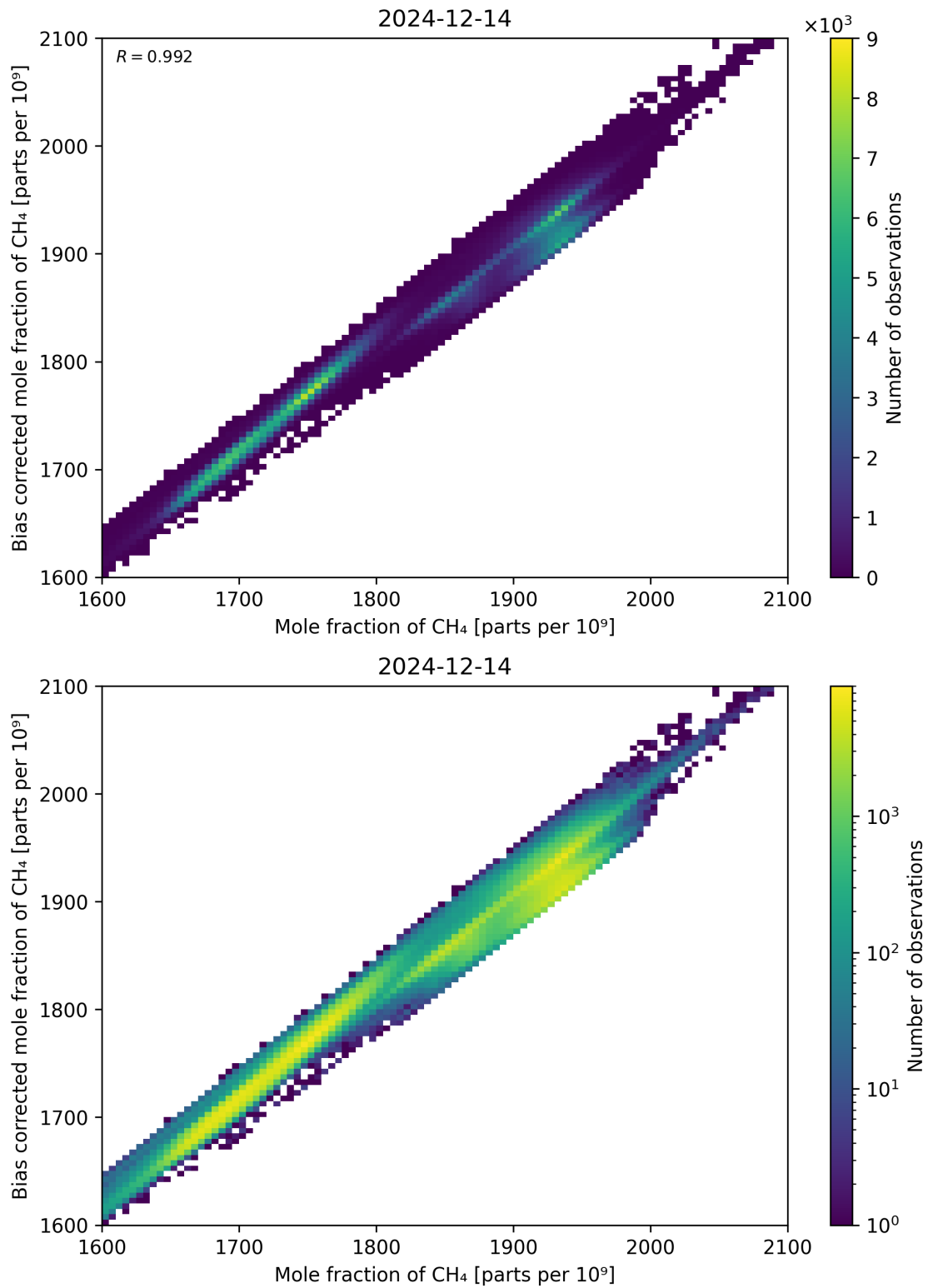
Figure 74: Scatter density plot of “Mole fraction of CH 4 ” against “Bias corrected mole fraction of CH 4 ” for 2024-12-13 to 2024-12-15.
