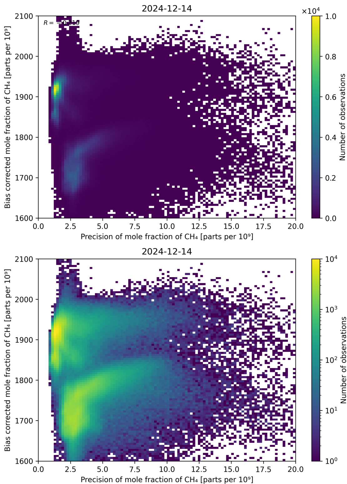
Figure 82: Scatter density plot of “Precision of mole fraction of CH 4 ” against “Bias corrected mole fraction of CH 4 ” for 2024-12-13 to 2024-12-15.
