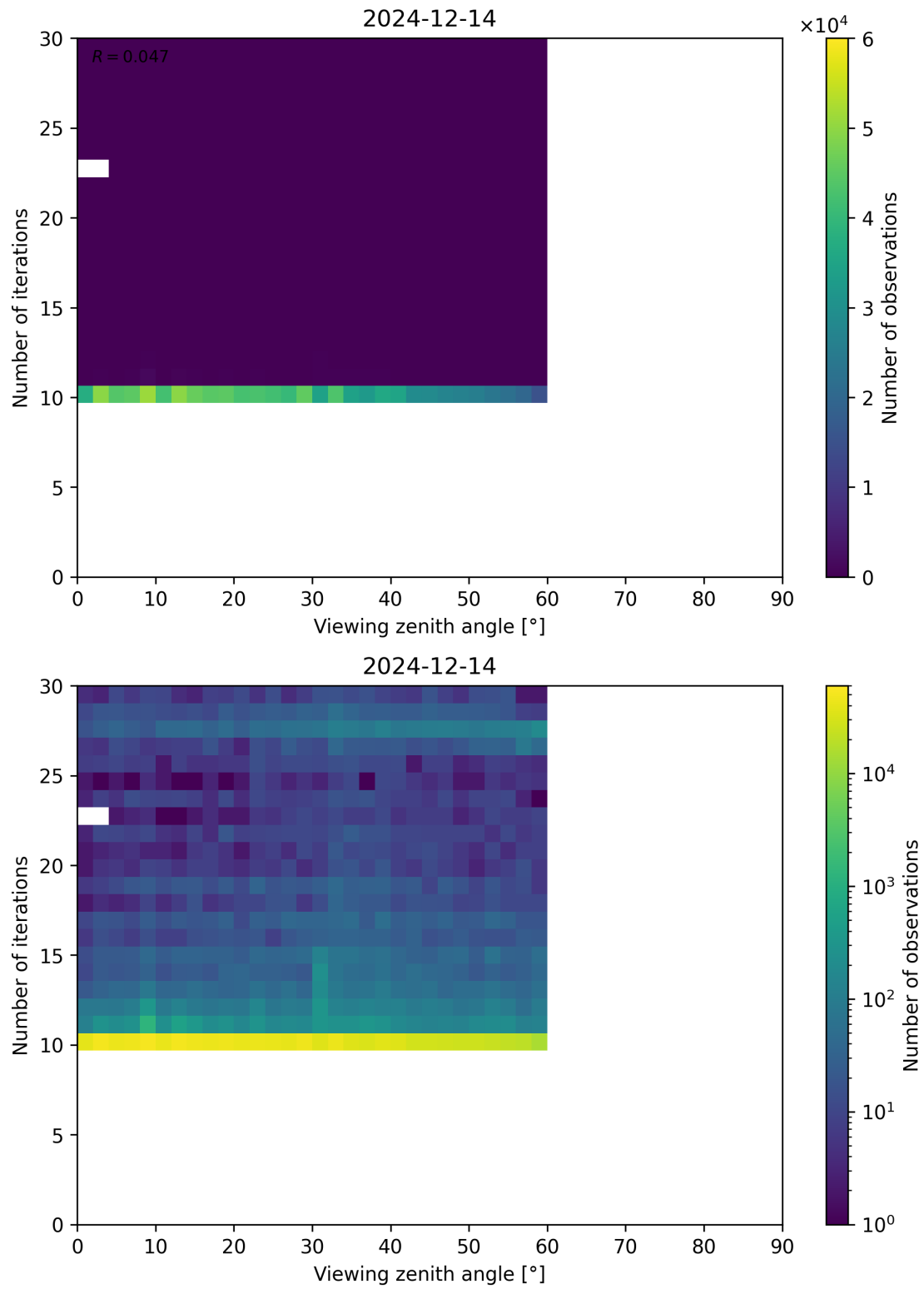
Figure 113: Scatter density plot of “Viewing zenith angle” against “Number of iterations” for 2024-12-13 to 2024-12-15.
