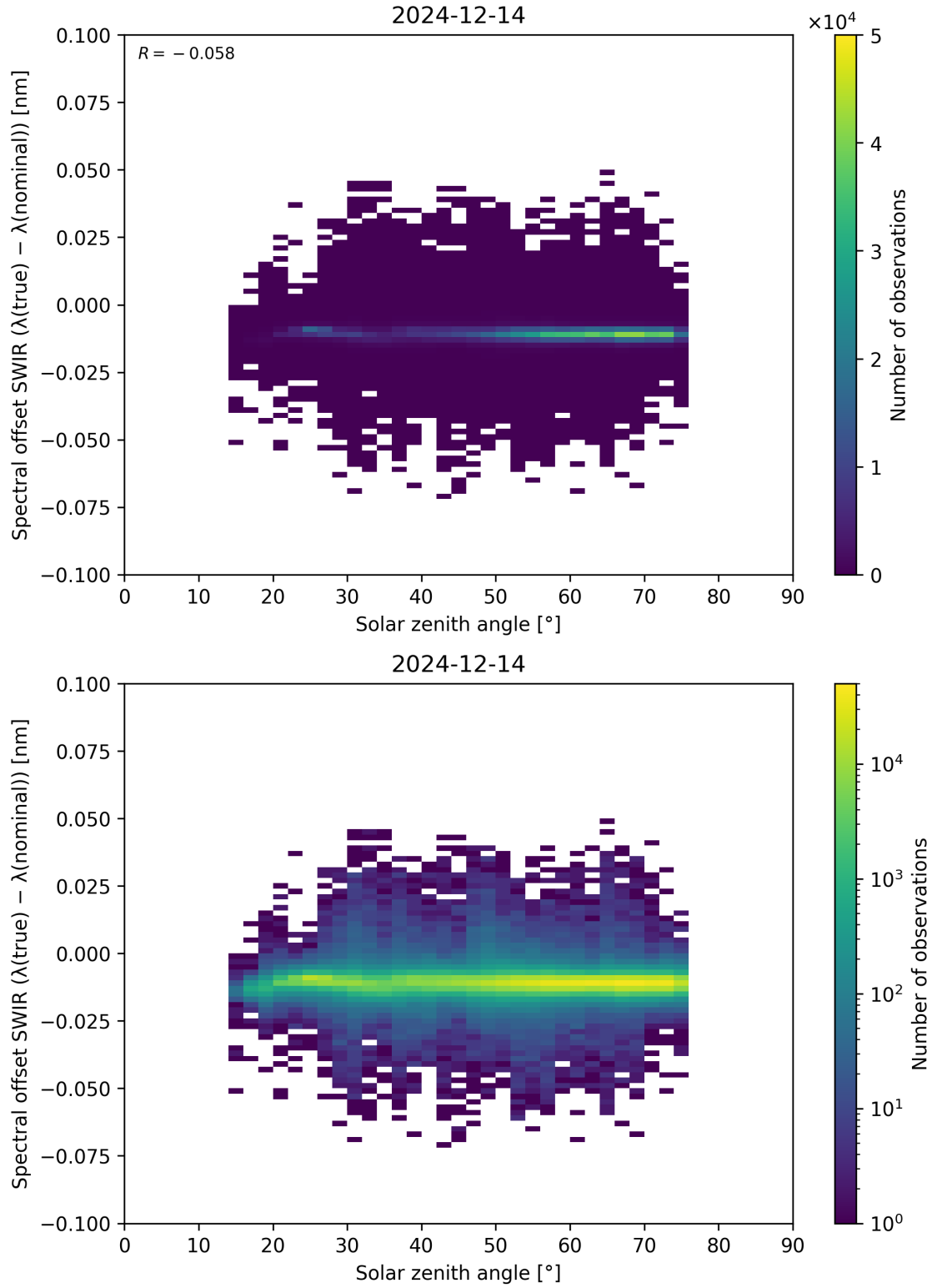
Figure 104: Scatter density plot of “Solar zenith angle” against “Spectral offset SWIR ( \lambda_{\text{true}} - \lambda_{\text{nominal}} )” for 2024-12-13 to 2024-12-15.
