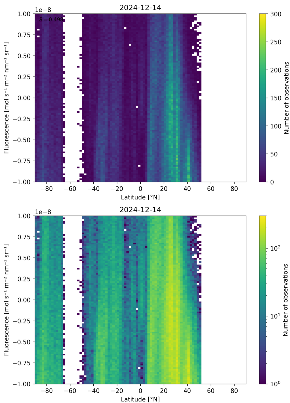
Figure 56: Scatter density plot of “Latitude” against “Fluorescence” for 2024-12-13 to 2024-12-15.
