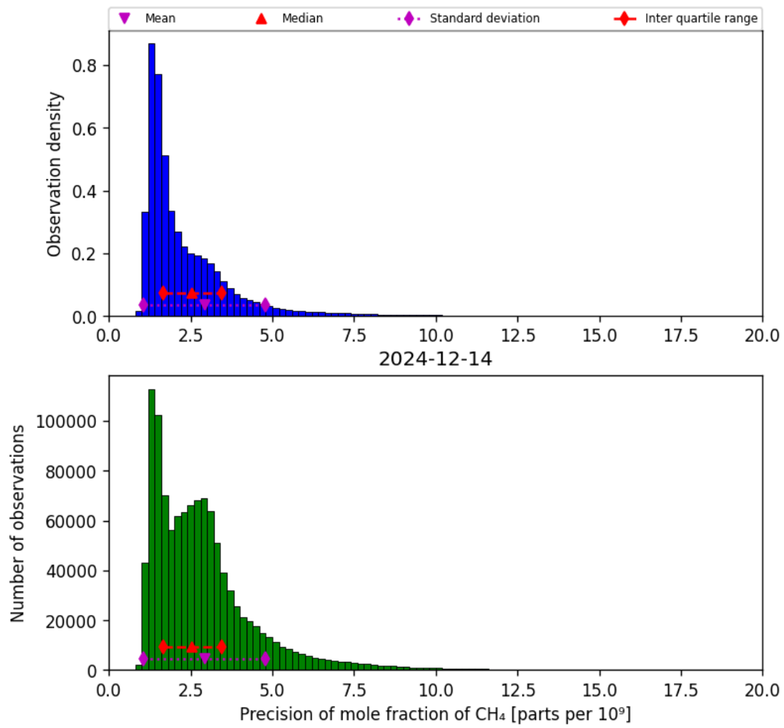
Figure 24: Histogram of “Precision of mole fraction of CH 4 ” for 2024-12-13 to 2024-12-15
