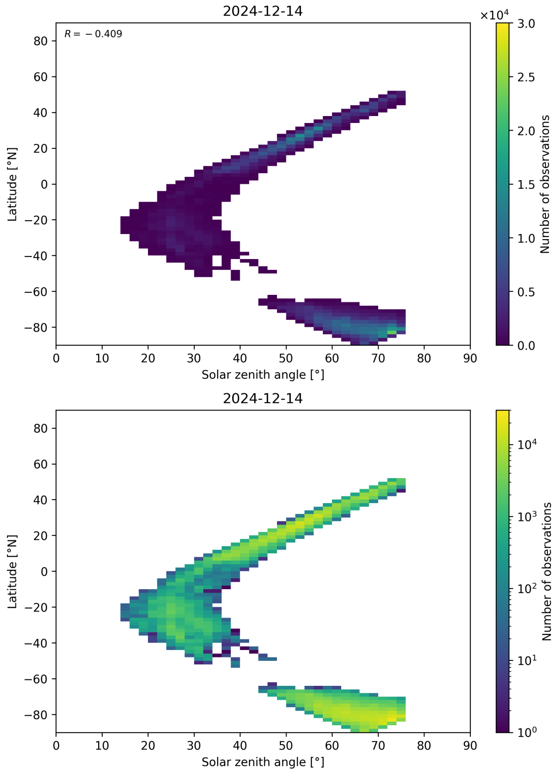
Figure 98: Scatter density plot of “Solar zenith angle” against “Latitude” for 2024-12-13 to 2024-12-15.
