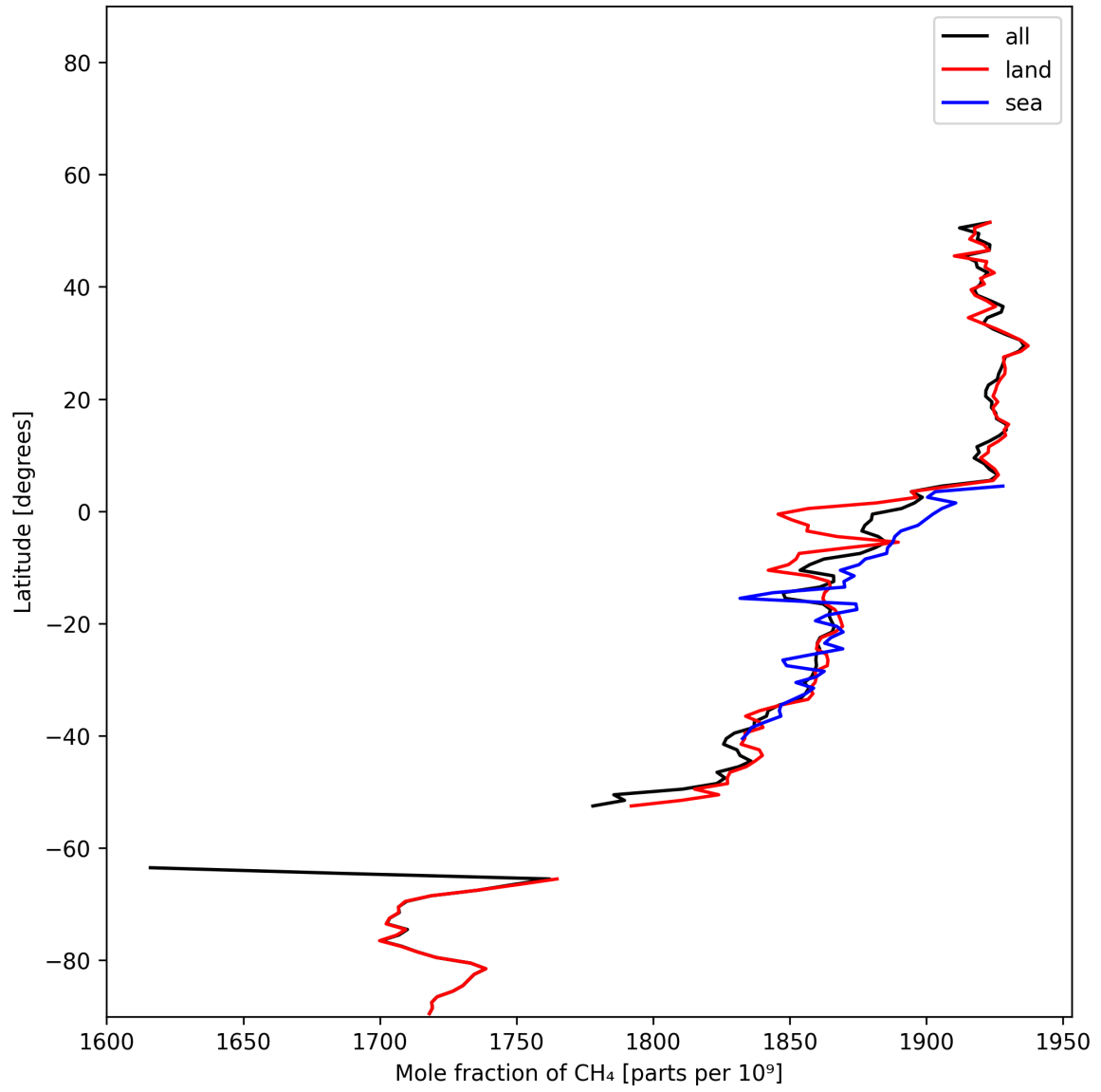
Figure 12: Zonal average of “Mole fraction of CH 4 ” for 2024-12-13 to 2024-12-15.
