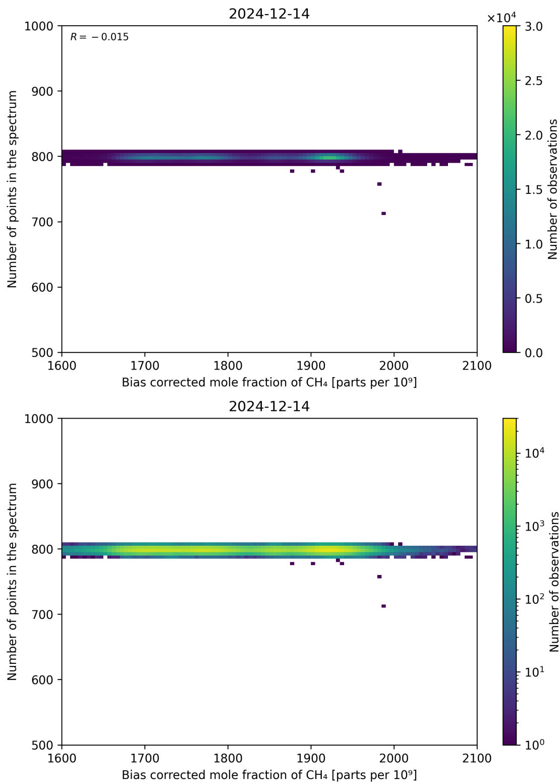
Figure 68: Scatter density plot of “Bias corrected mole fraction of CH 4 ” against “Number of points in the spectrum” for 2024-12-13 to 2024-12-15.
