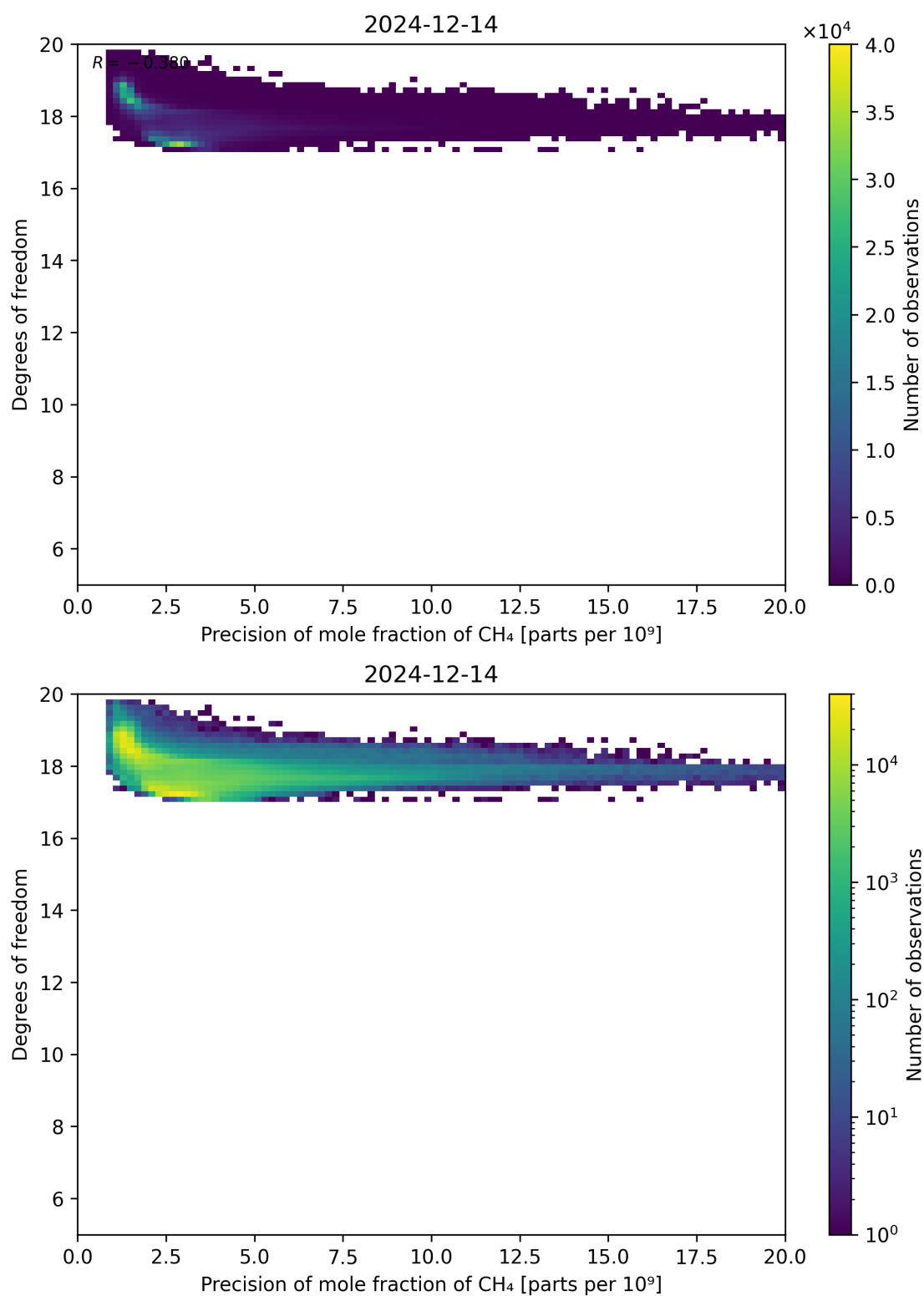
Figure 80: Scatter density plot of “Precision of mole fraction of CH 4 ” against “Degrees of freedom” for 2024-12-13 to 2024-12-15.
