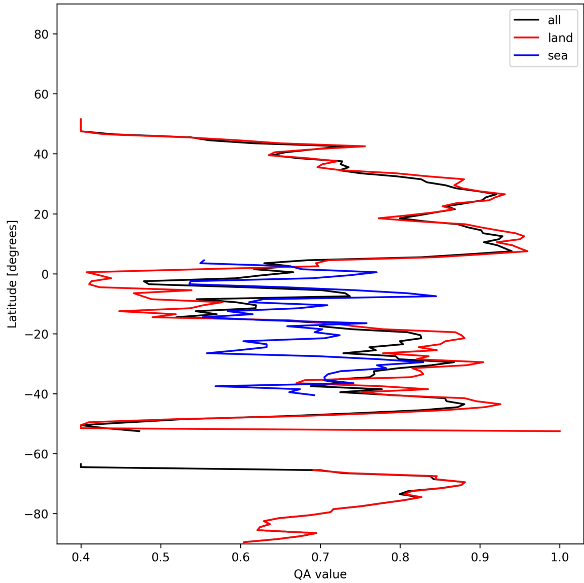
Figure 11: Zonal average of “QA value” for 2024-12-13 to 2024-12-15.
