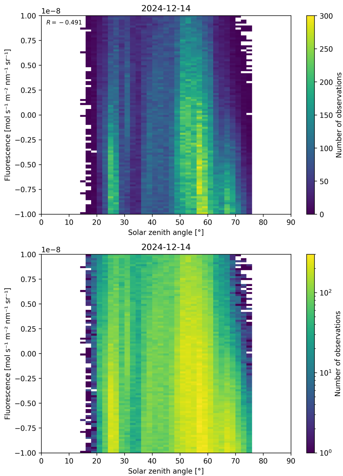
Figure 97: Scatter density plot of “Solar zenith angle” against “Fluorescence” for 2024-12-13 to 2024-12-15.
