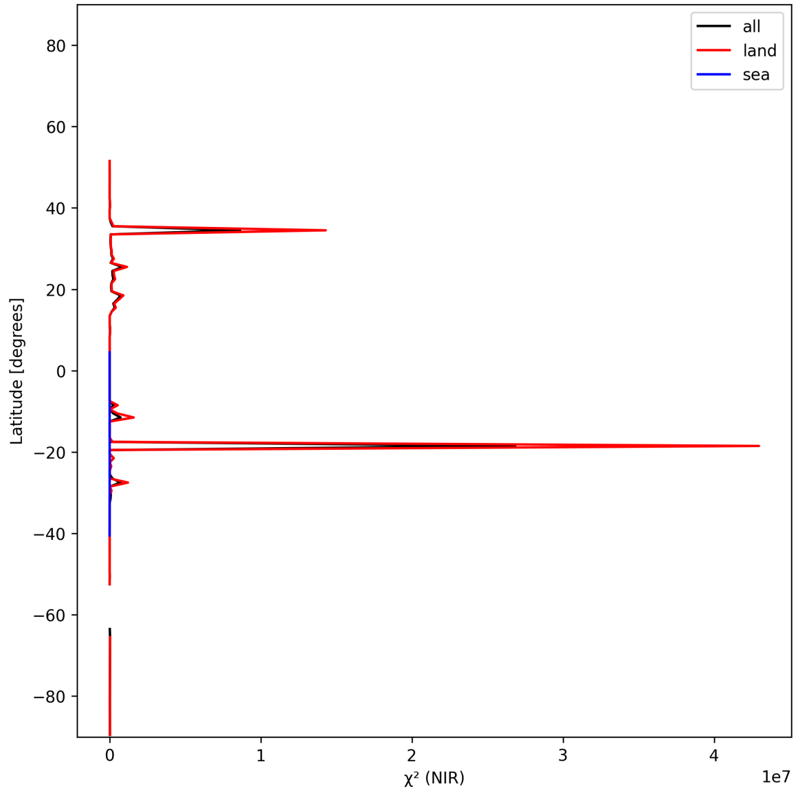
Figure 18: Zonal average of “ \chi^2 (NIR)” for 2024-12-13 to 2024-12-15.
