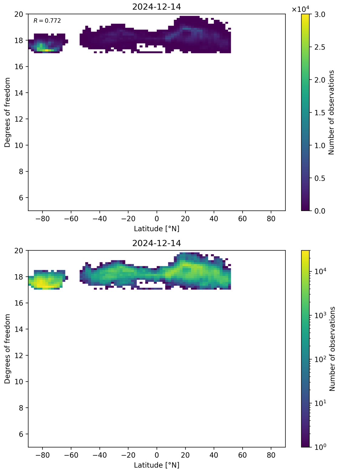
Figure 55: Scatter density plot of “Latitude” against “Degrees of freedom” for 2024-12-13 to 2024-12-15.
