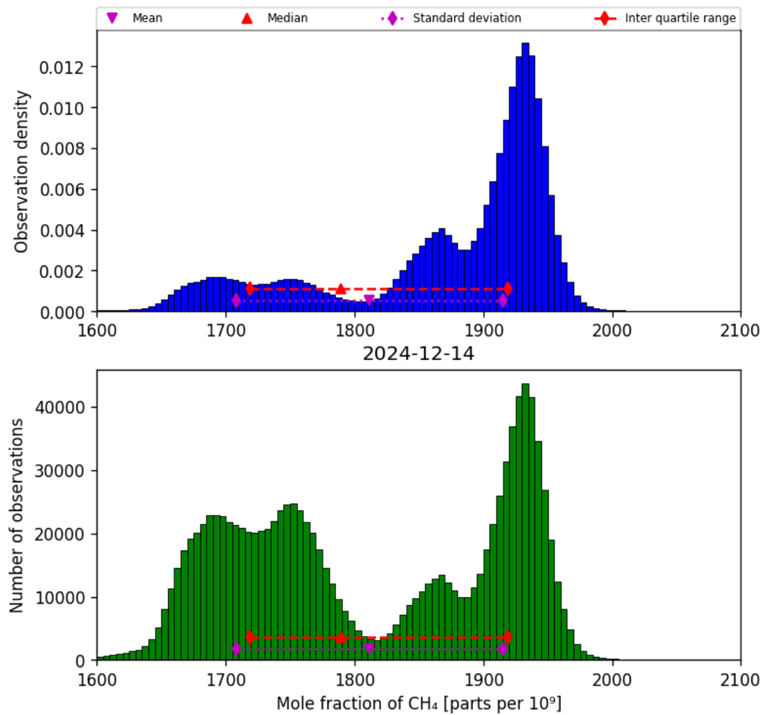
Figure 23: Histogram of “Mole fraction of CH 4 ” for 2024-12-13 to 2024-12-15
