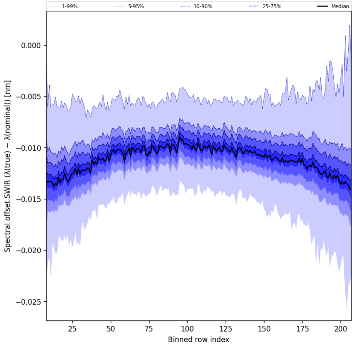
Figure 38: Along track statistics of “Spectral offset SWIR ( \lambda_{\text{true}} - \lambda_{\text{nominal}} )” for 2024-12-13 to 2024-12-15
