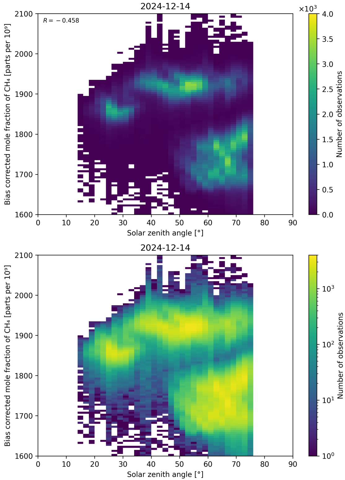
Figure 100: Scatter density plot of “Solar zenith angle” against “Bias corrected mole fraction of CH 4 ” for 2024-12-13 to 2024-12-15.
