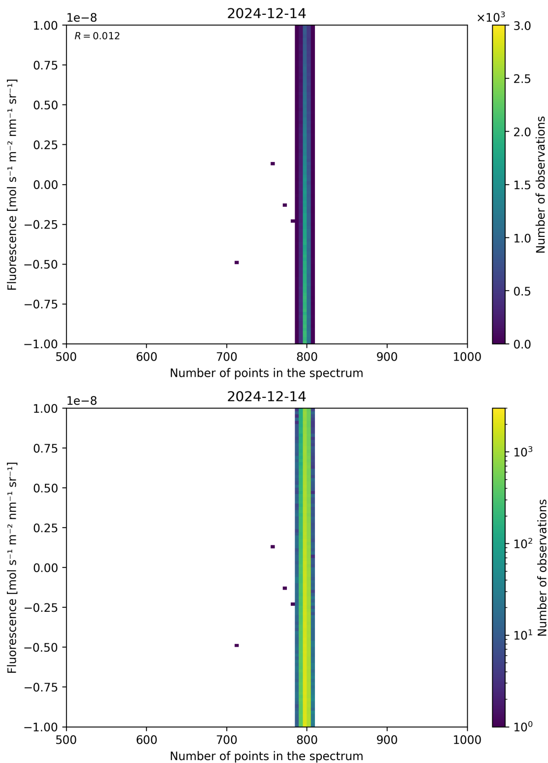
Figure 91: Scatter density plot of “Number of points in the spectrum” against “Fluorescence” for 2024-12-13 to 2024-12-15.
