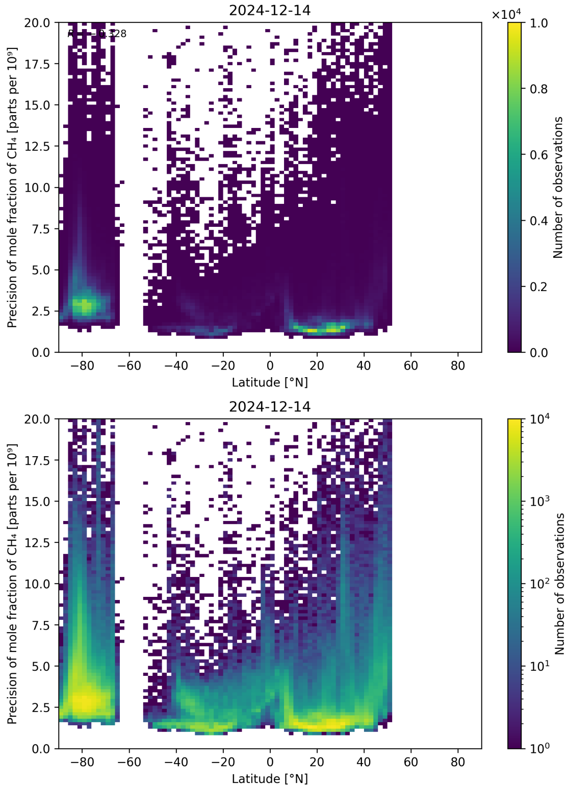
Figure 59: Scatter density plot of “Latitude” against “Precision of mole fraction of CH 4 ” for 2024-12-13 to 2024-12-15.
