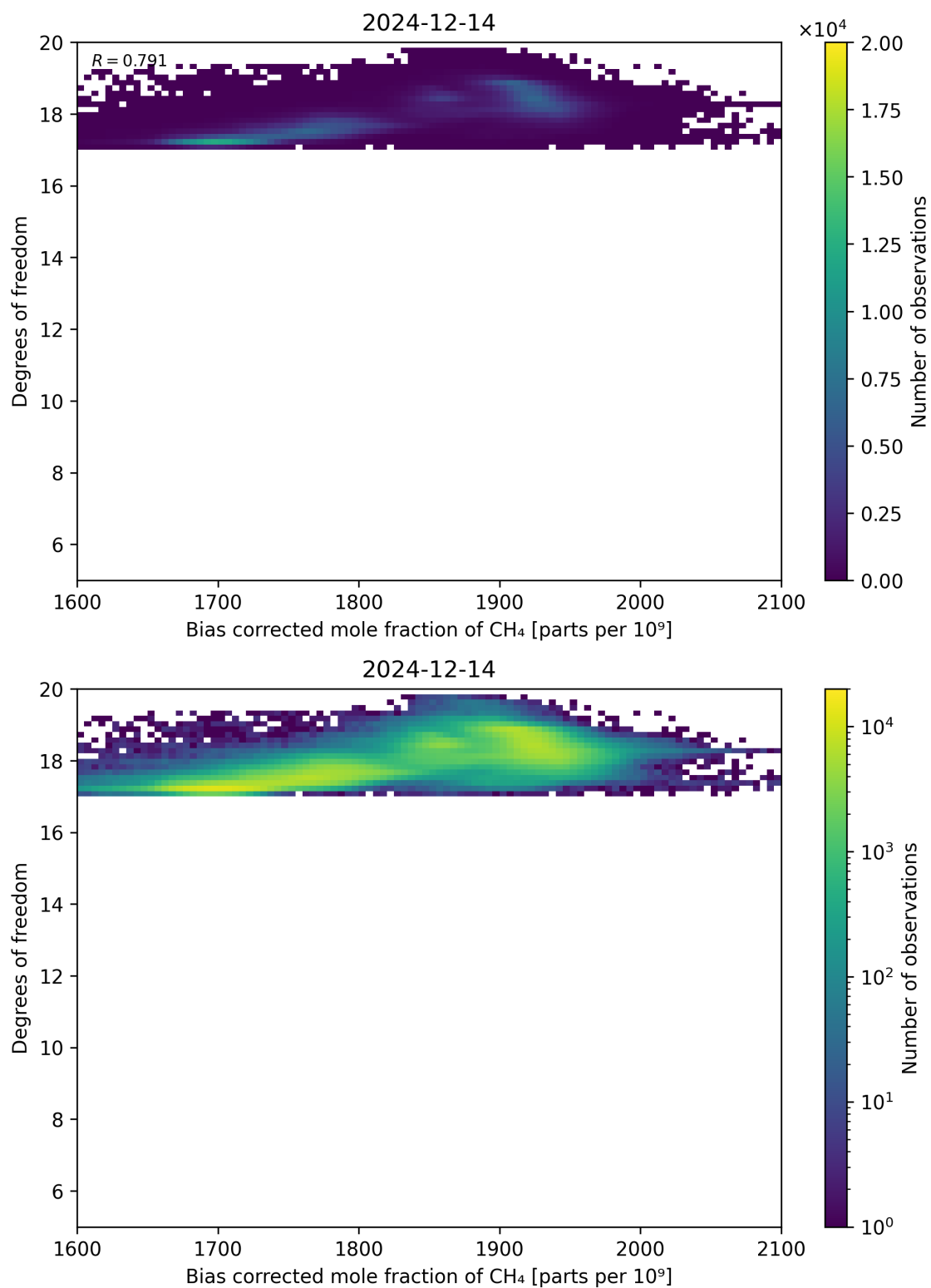
Figure 65: Scatter density plot of “Bias corrected mole fraction of CH 4 ” against “Degrees of freedom” for 2024-12-13 to 2024-12-15.
