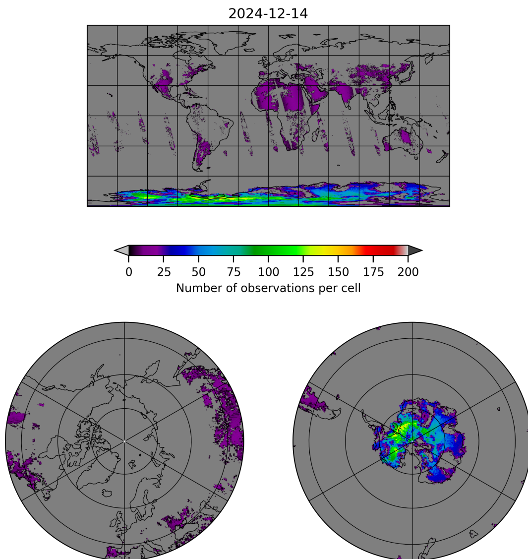
Figure 10: Map of the number of observations for 2024-12-13 to 2024-12-15
