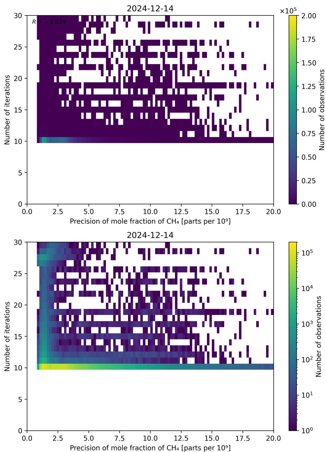
Figure 83: Scatter density plot of “Precision of mole fraction of CH 4 ” against “Number of iterations” for 2024-12-13 to 2024-12-15.
