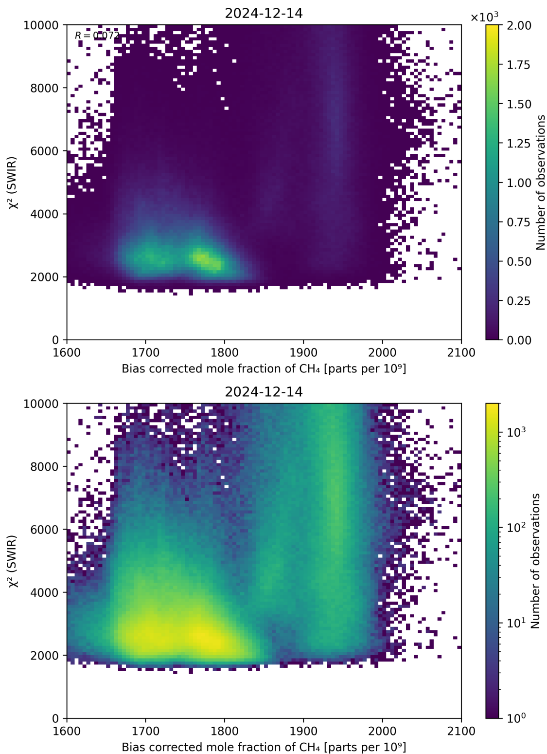
Figure 64: Scatter density plot of “Bias corrected mole fraction of \text{CH}_4 ” against “ \chi^2 (SWIR)” for 2024-12-13 to 2024-12-15.
