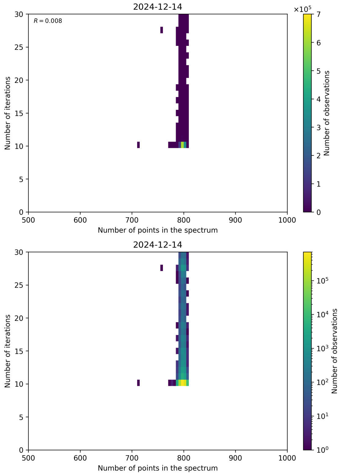
Figure 92: Scatter density plot of “Number of points in the spectrum” against “Number of iterations” for 2024-12-13 to 2024-12-15.
