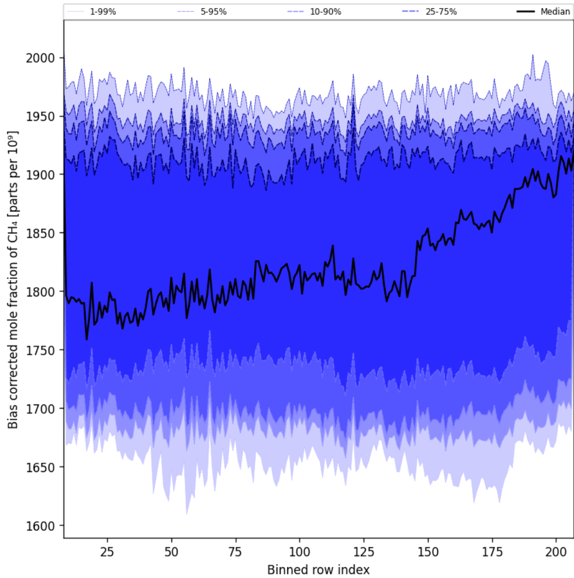
Figure 36: Along track statistics of “Bias corrected mole fraction of CH 4 ” for 2024-12-13 to 2024-12-15
