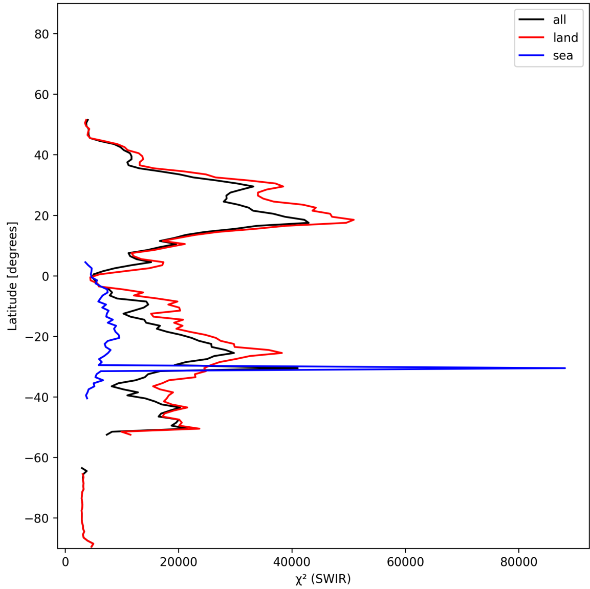
Figure 17: Zonal average of “ \chi^2 (SWIR)” for 2024-12-13 to 2024-12-15.
