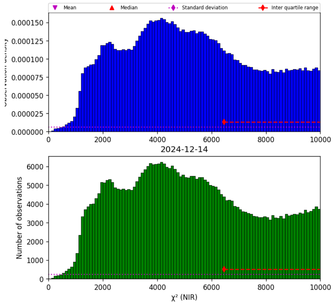
Figure 29: Histogram of “ \chi^2 (NIR)” for 2024-12-13 to 2024-12-15
