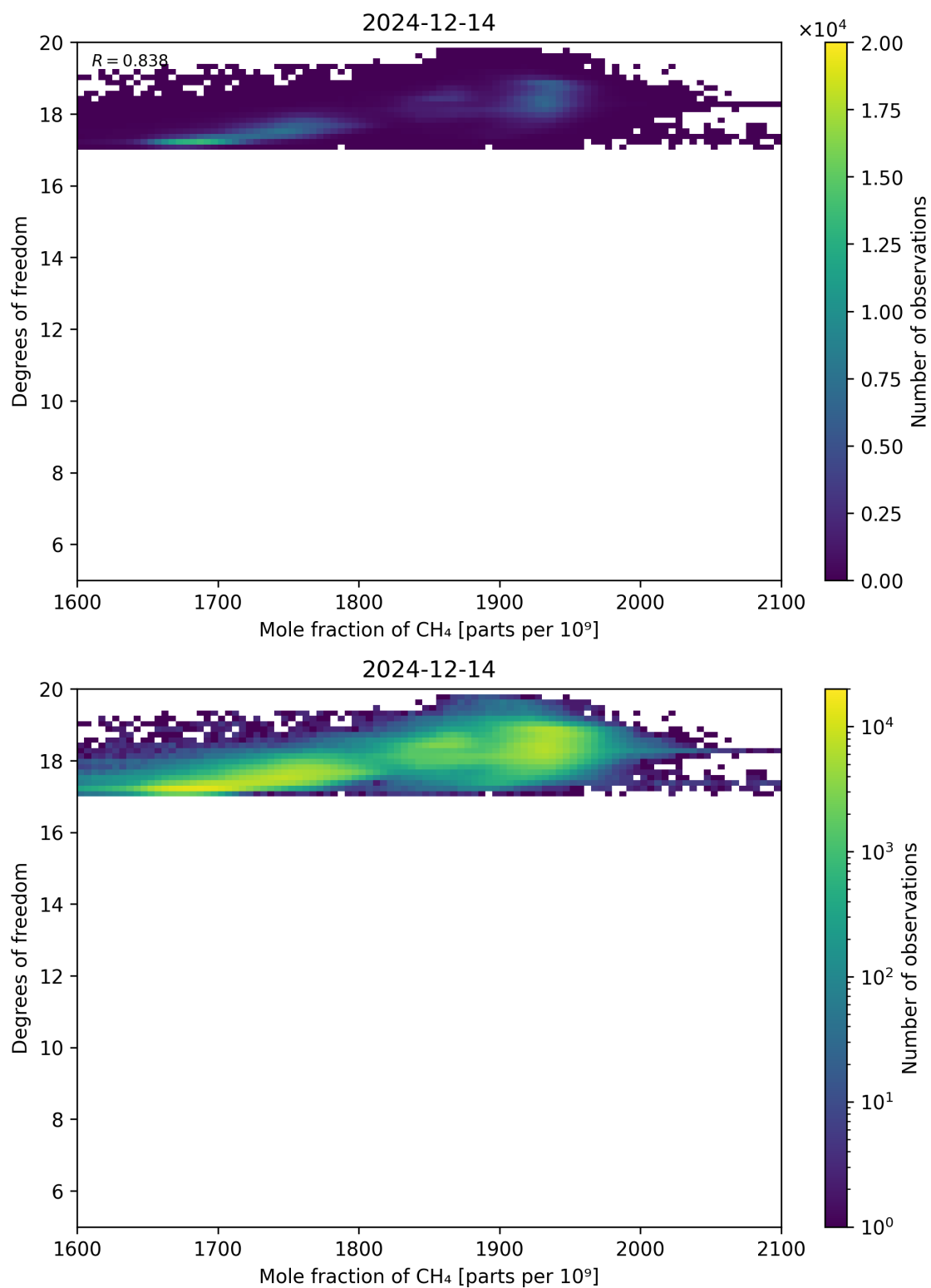
Figure 72: Scatter density plot of “Mole fraction of CH 4 ” against “Degrees of freedom” for 2024-12-13 to 2024-12-15.
