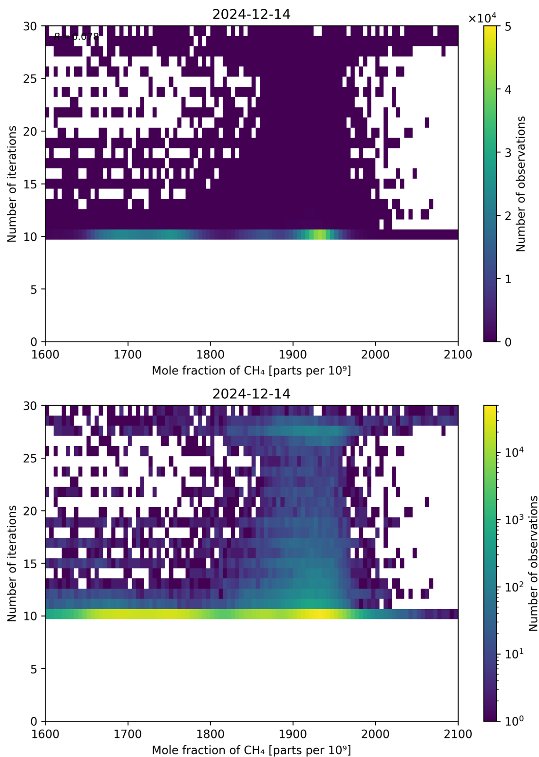
Figure 76: Scatter density plot of “Mole fraction of CH 4 ” against “Number of iterations” for 2024-12-13 to 2024-12-15.
