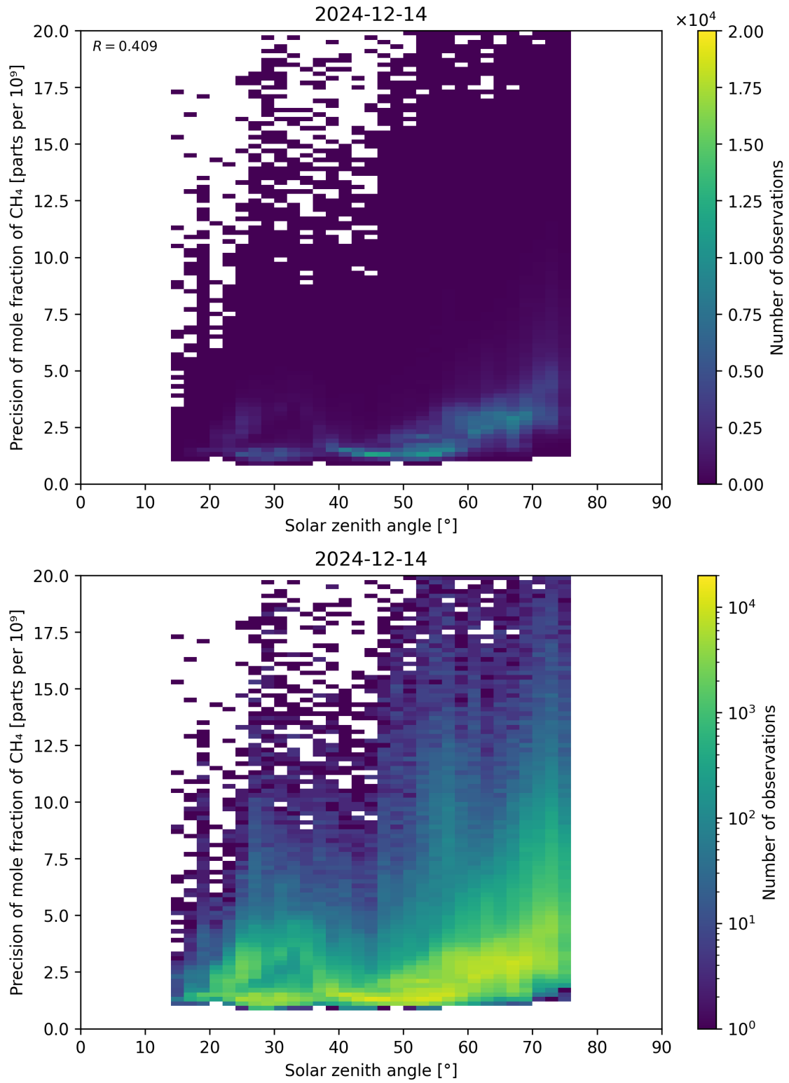
Figure 101: Scatter density plot of “Solar zenith angle” against “Precision of mole fraction of CH 4 ” for 2024-12-13 to 2024-12-15.
