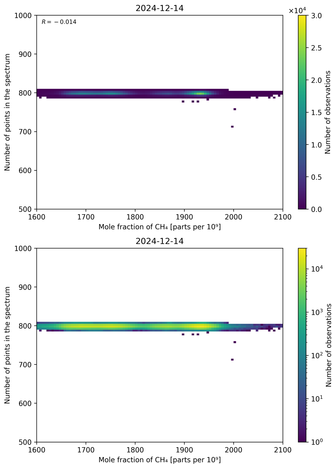
Figure 77: Scatter density plot of “Mole fraction of CH 4 ” against “Number of points in the spectrum” for 2024-12-13 to 2024-12-15.
