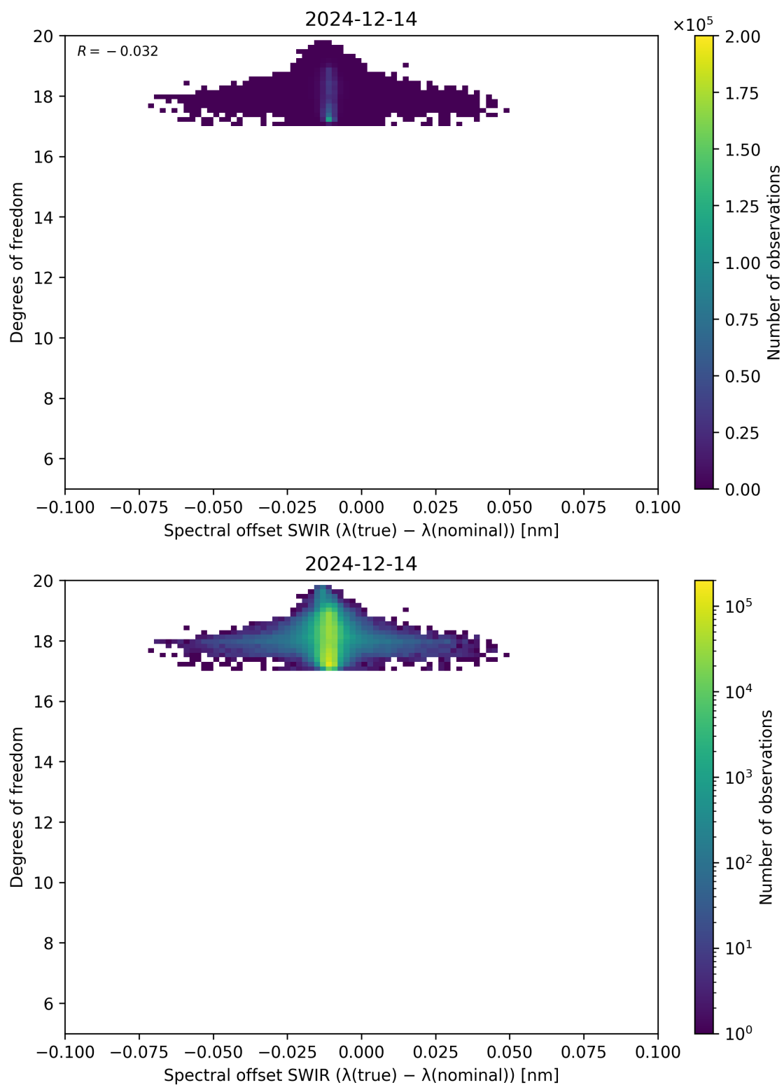
Figure 119: Scatter density plot of “Spectral offset SWIR ( \lambda_{\text{true}} - \lambda_{\text{nominal}} )” against “Degrees of freedom” for 2024-12-13 to 2024-12-15.
