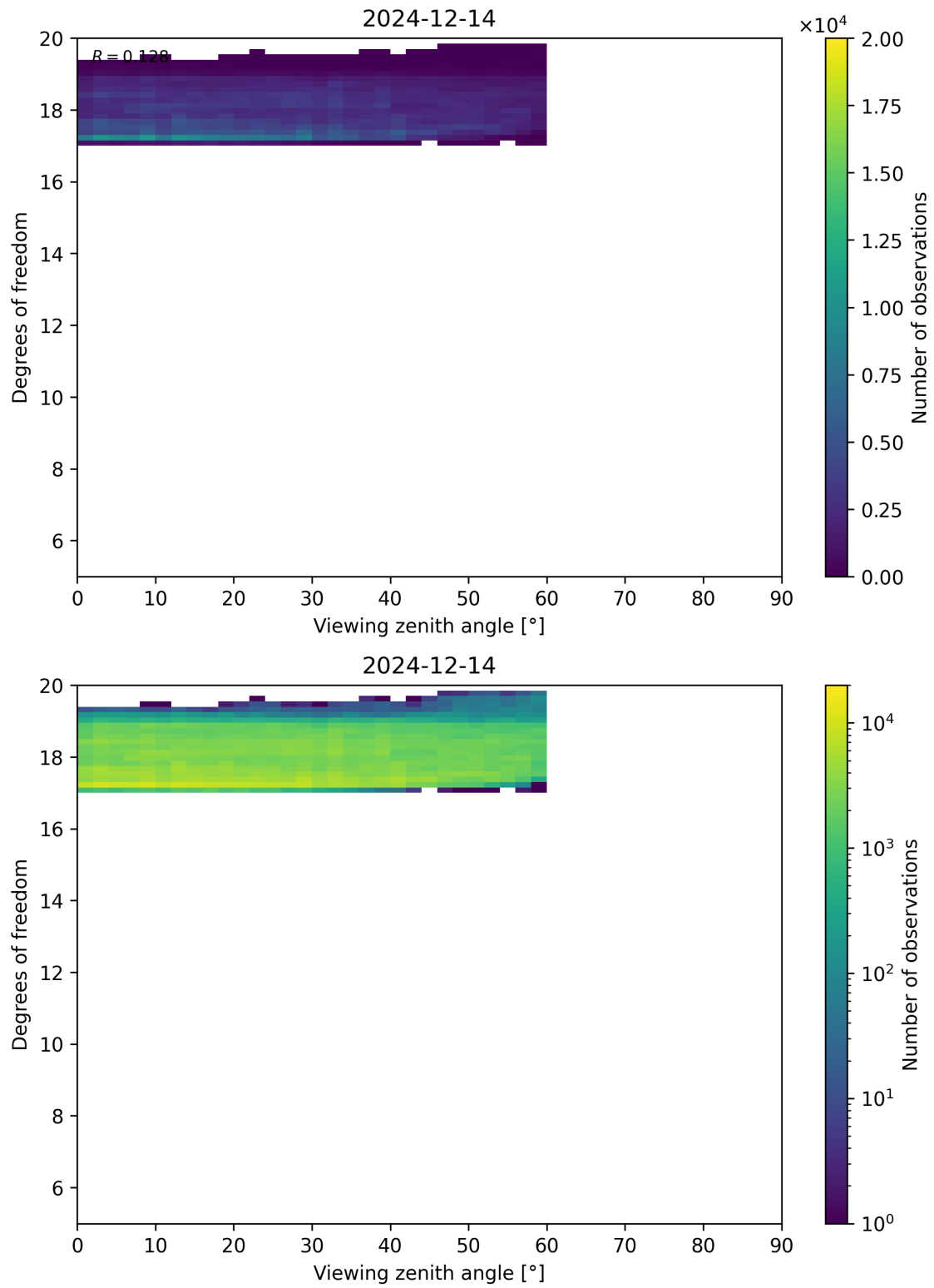
Figure 107: Scatter density plot of “Viewing zenith angle” against “Degrees of freedom” for 2024-12-13 to 2024-12-15.
