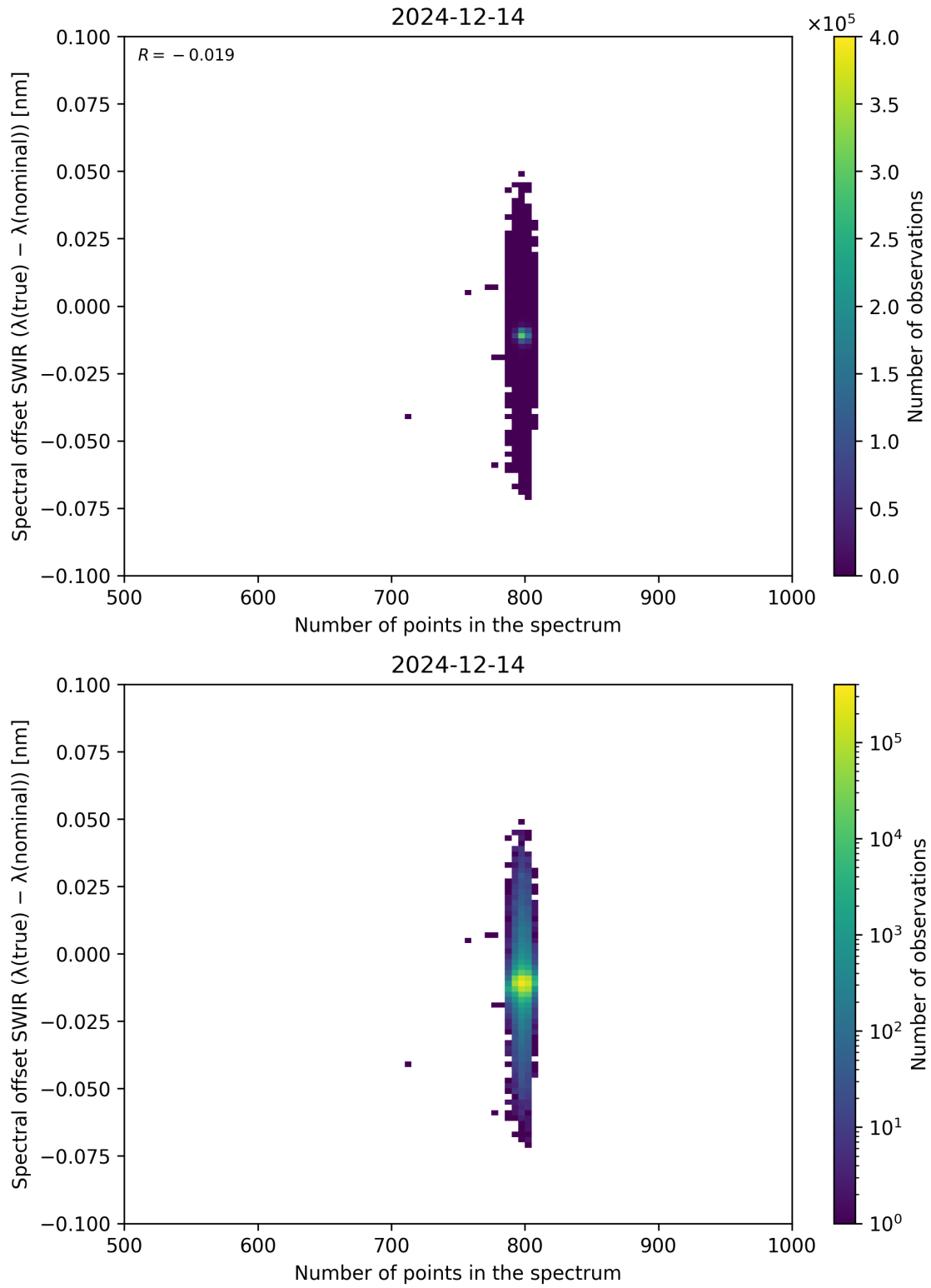
Figure 93: Scatter density plot of “Number of points in the spectrum” against “Spectral offset SWIR ( \lambda_{\text{true}} - \lambda_{\text{nominal}} )” for 2024-12-13 to 2024-12-15.
