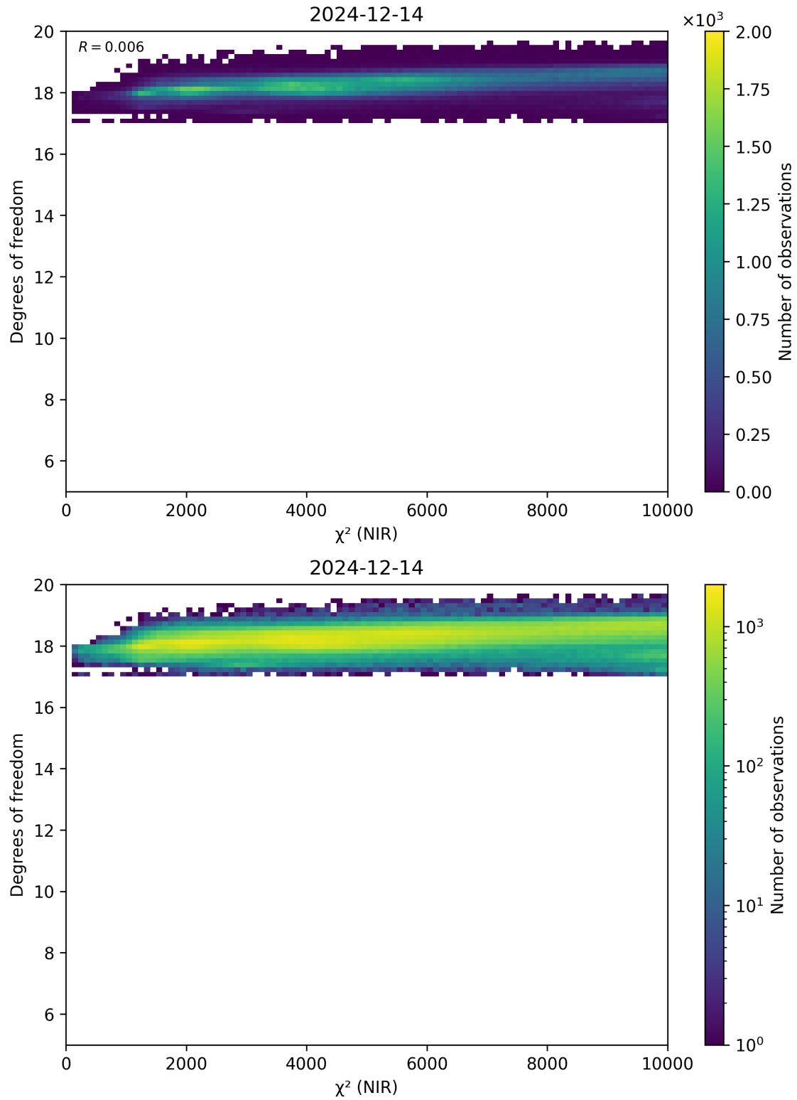
Figure 44: Scatter density plot of “ \chi^2 (NIR)” against “Degrees of freedom” for 2024-12-13 to 2024-12-15.
