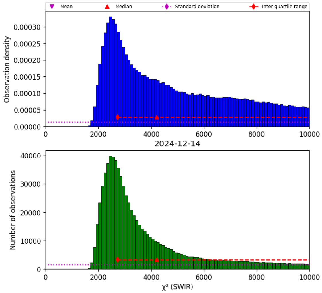
Figure 28: Histogram of “ \chi^2 (SWIR)” for 2024-12-13 to 2024-12-15
