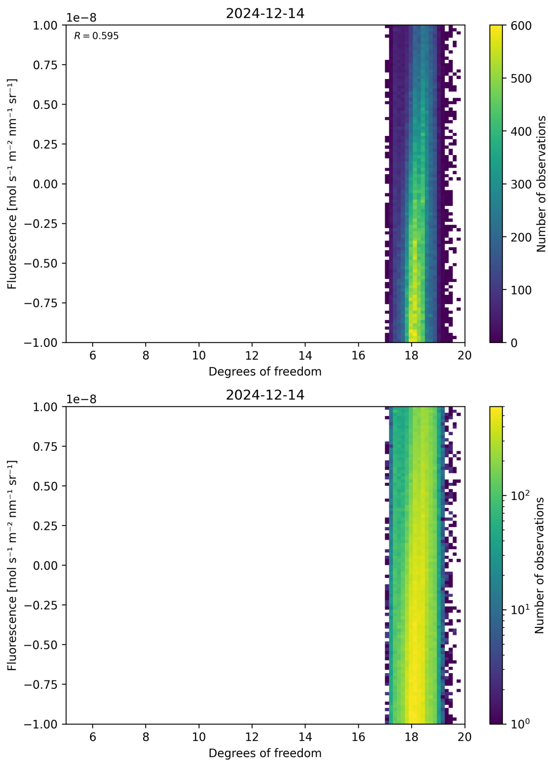
Figure 51: Scatter density plot of “Degrees of freedom” against “Fluorescence” for 2024-12-13 to 2024-12-15.
