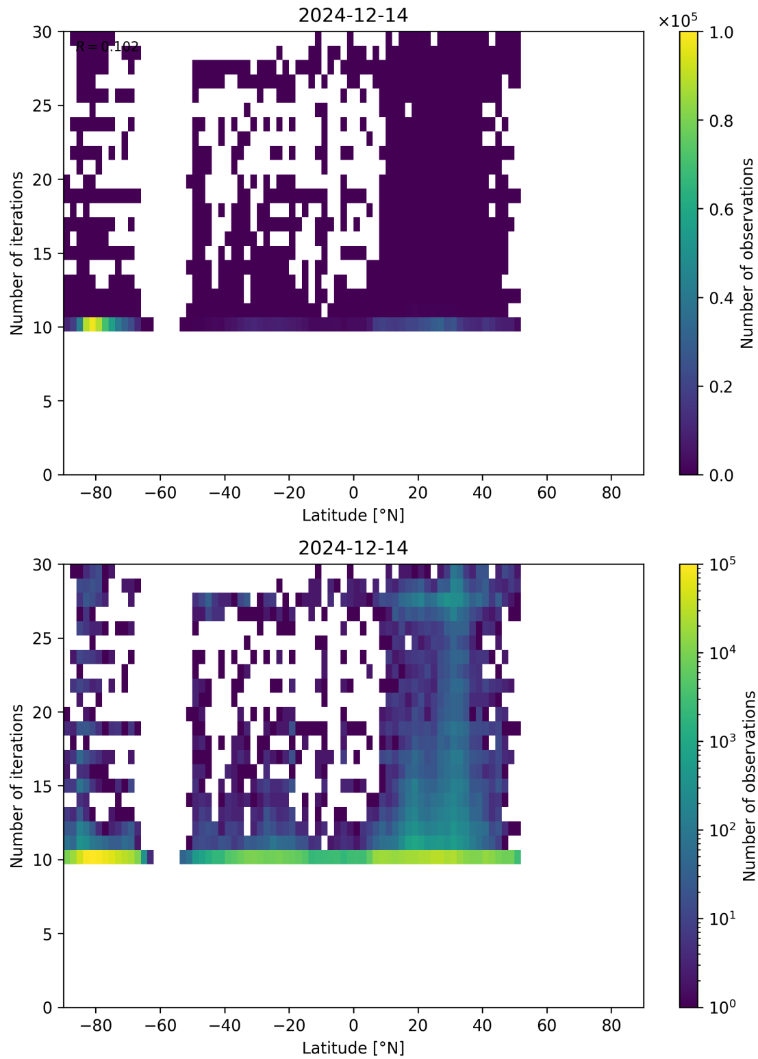
Figure 60: Scatter density plot of “Latitude” against “Number of iterations” for 2024-12-13 to 2024-12-15.
