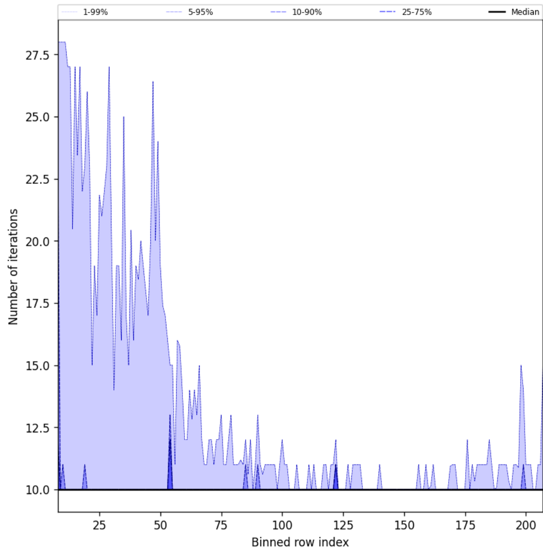
Figure 42: Along track statistics of “Number of iterations” for 2024-12-13 to 2024-12-15
