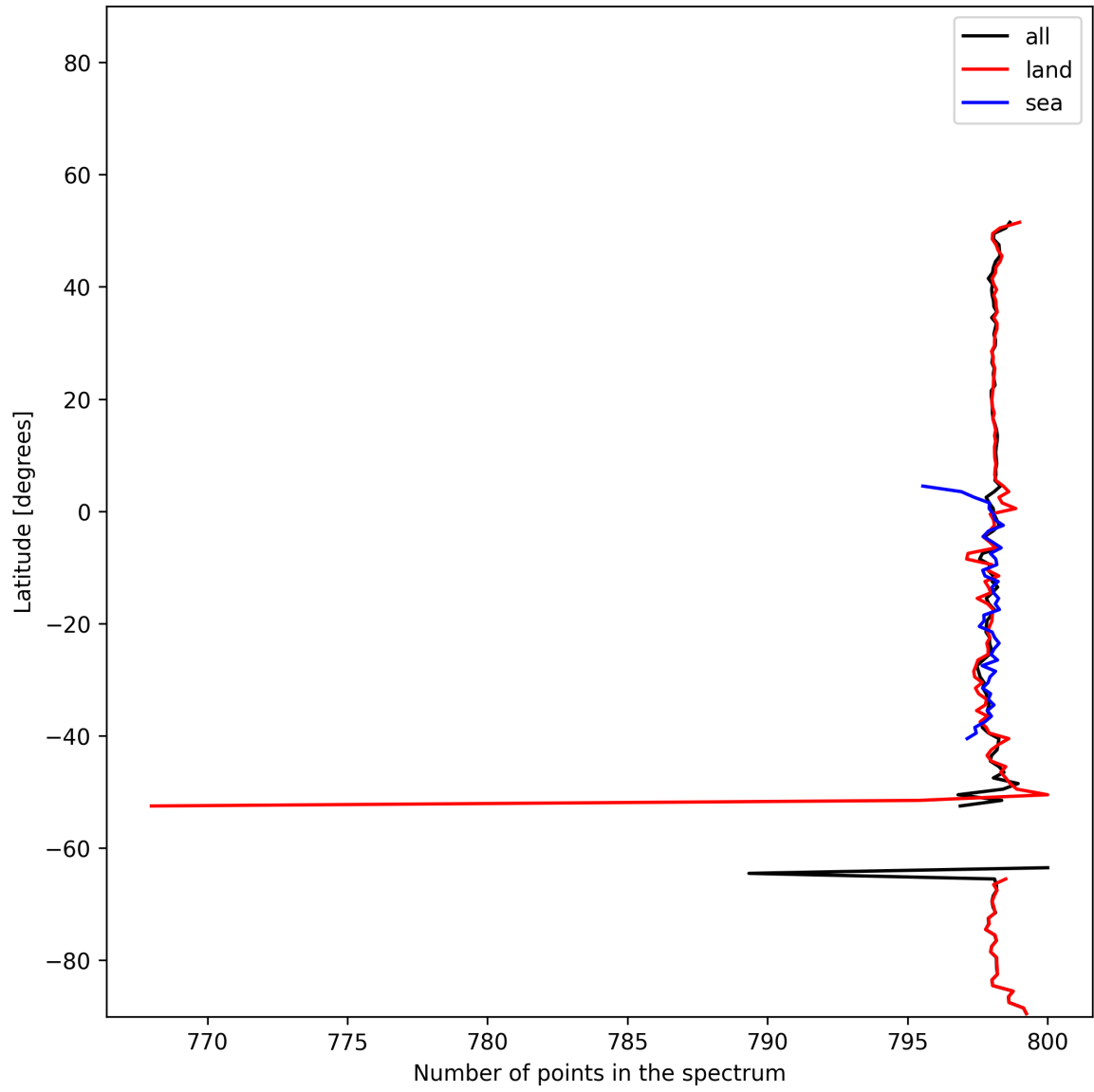
Figure 15: Zonal average of “Number of points in the spectrum” for 2024-12-13 to 2024-12-15.
