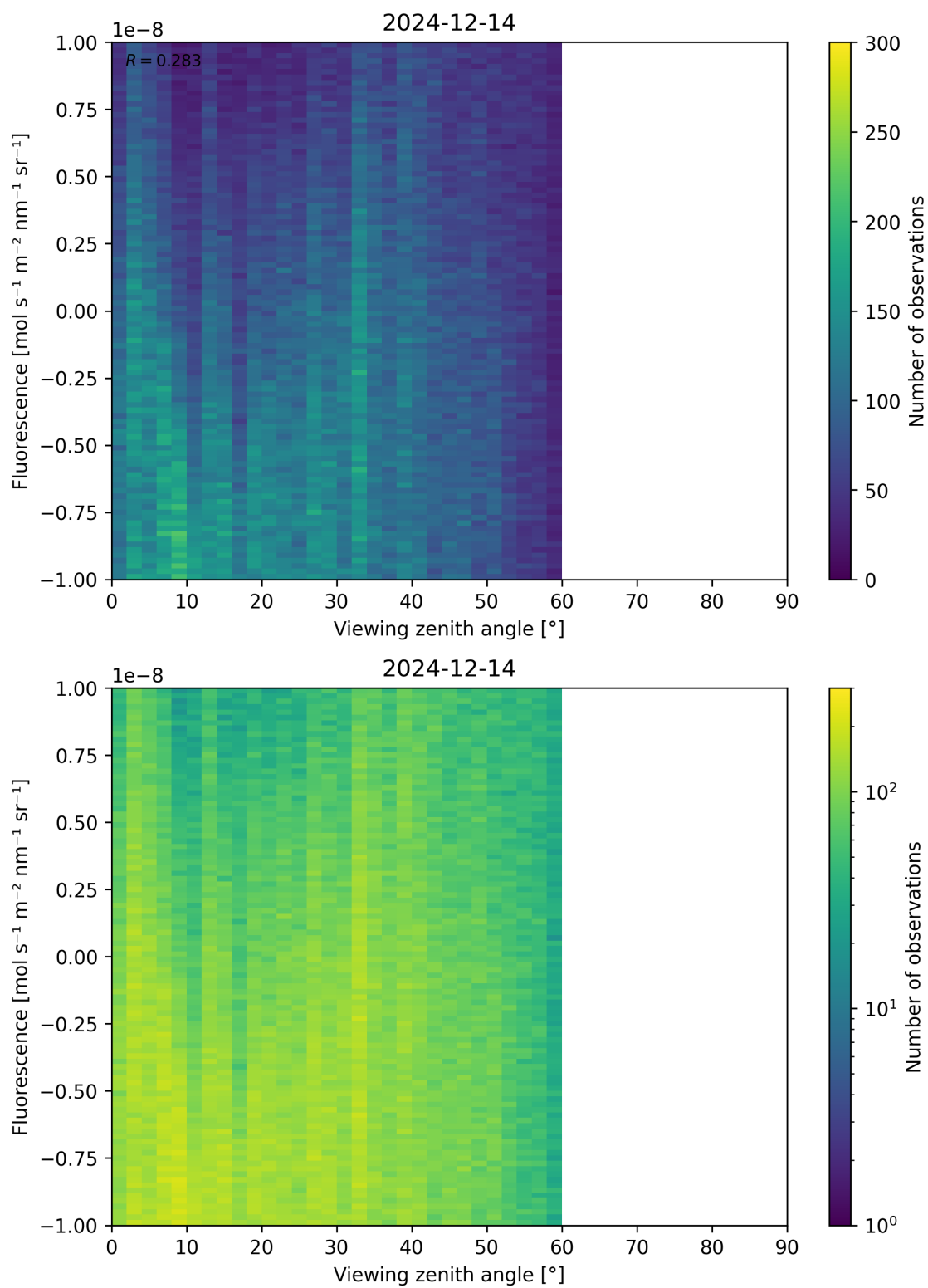
Figure 108: Scatter density plot of “Viewing zenith angle” against “Fluorescence” for 2024-12-13 to 2024-12-15.
