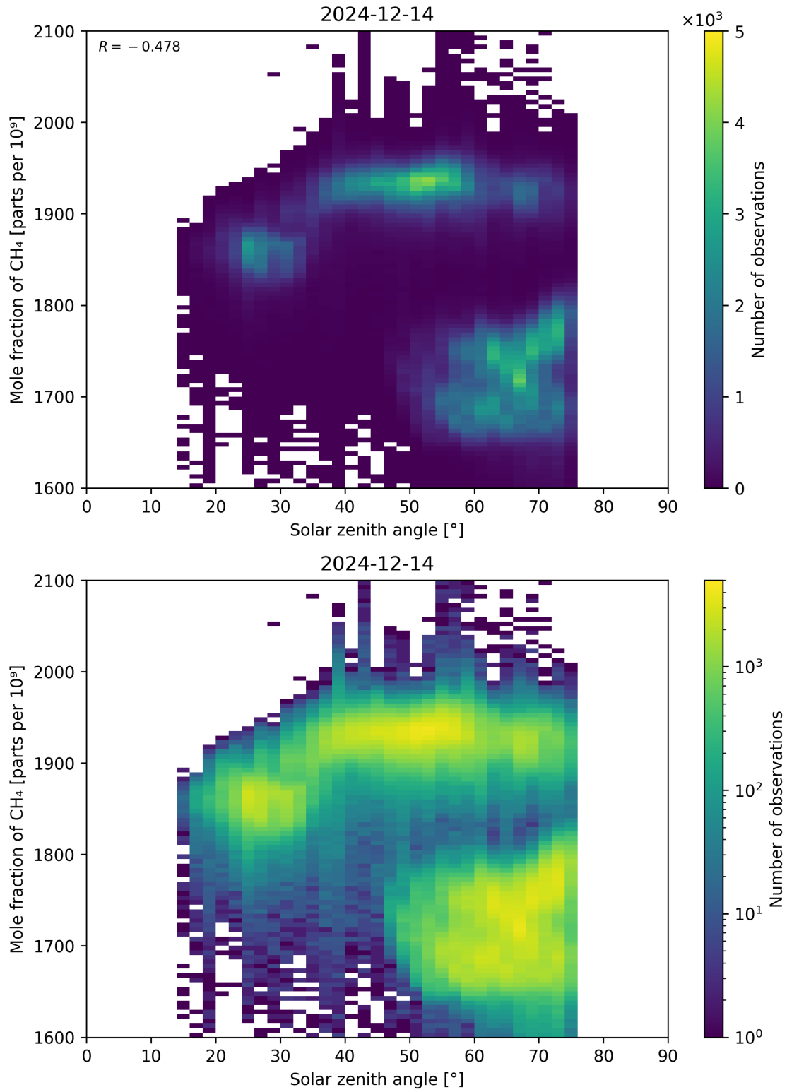
Figure 99: Scatter density plot of “Solar zenith angle” against “Mole fraction of \text{CH}_4 ” for 2024-12-13 to 2024-12-15.
