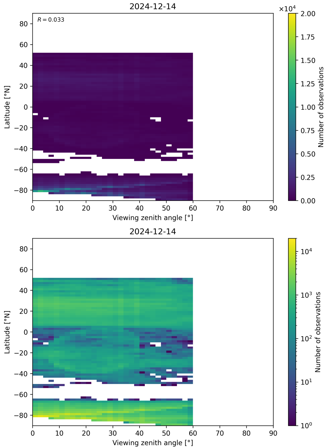
Figure 109: Scatter density plot of “Viewing zenith angle” against “Latitude” for 2024-12-13 to 2024-12-15.
