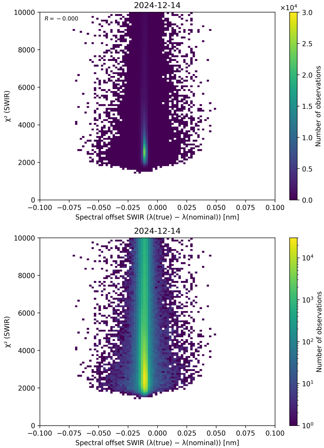
Figure 118: Scatter density plot of “Spectral offset SWIR ( \lambda_{\text{true}} - \lambda_{\text{nominal}} )” against “ \chi^2 (SWIR)” for 2024-12-13 to 2024-12-15.
