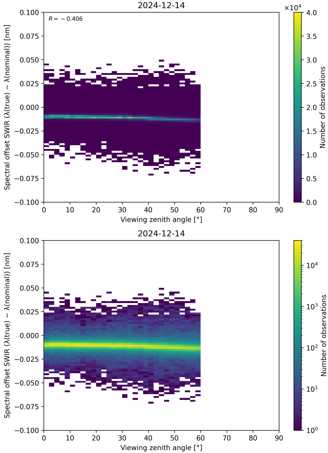
Figure 116: Scatter density plot of “Viewing zenith angle” against “Spectral offset SWIR ( \lambda_{\text{true}} - \lambda_{\text{nominal}} )” for 2024-12-13 to 2024-12-15.
