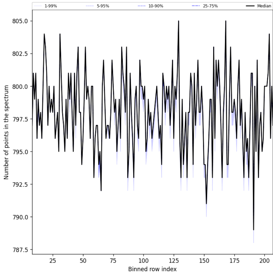
Figure 37: Along track statistics of “Number of points in the spectrum” for 2024-12-13 to 2024-12-15
