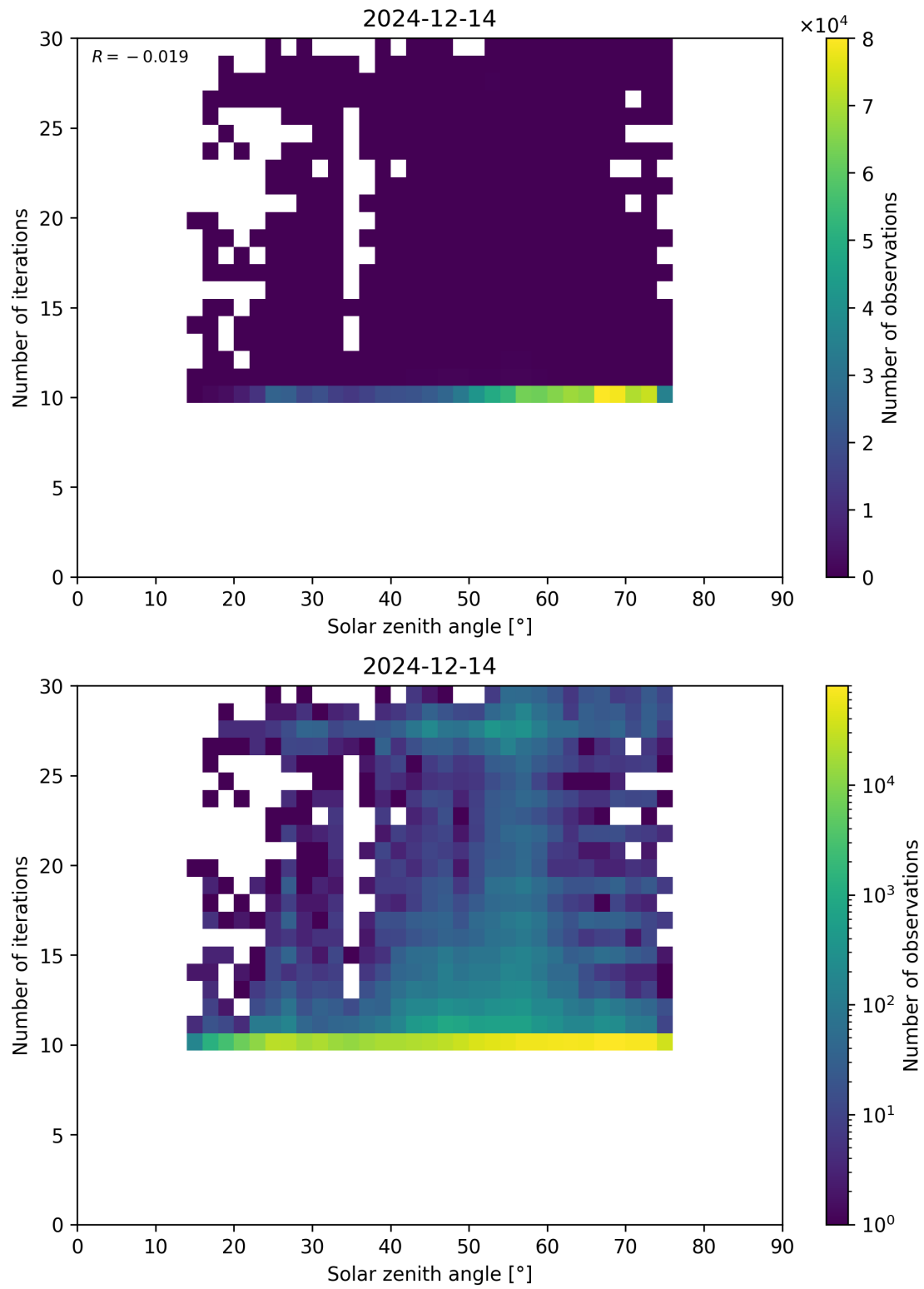
Figure 102: Scatter density plot of “Solar zenith angle” against “Number of iterations” for 2024-12-13 to 2024-12-15.
