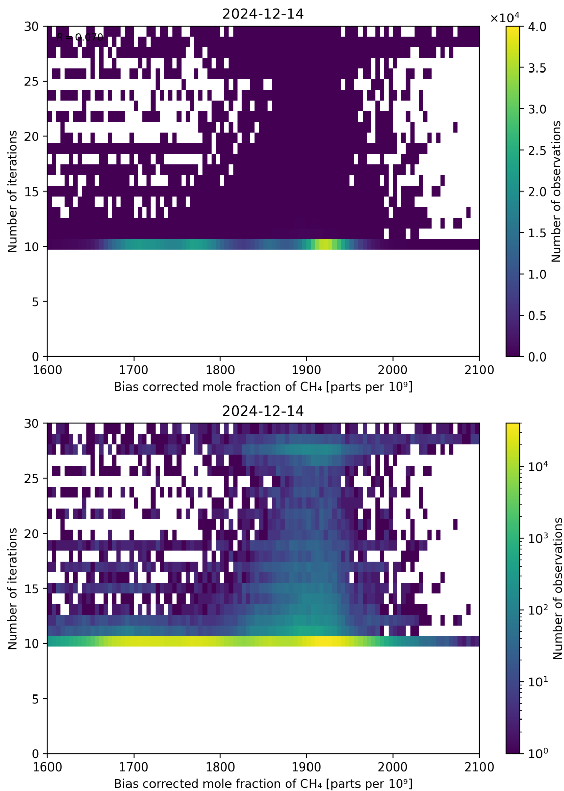
Figure 67: Scatter density plot of “Bias corrected mole fraction of \text{CH}_4 ” against “Number of iterations” for 2024-12-13 to 2024-12-15.
