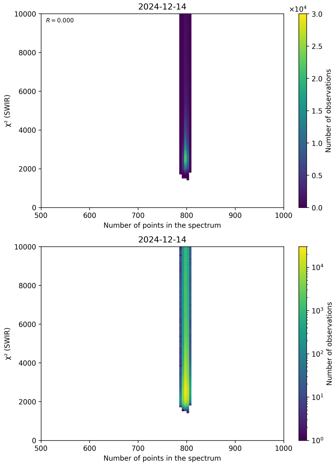
Figure 89: Scatter density plot of “Number of points in the spectrum” against “ \chi^2 (SWIR)” for 2024-12-13 to 2024-12-15.
