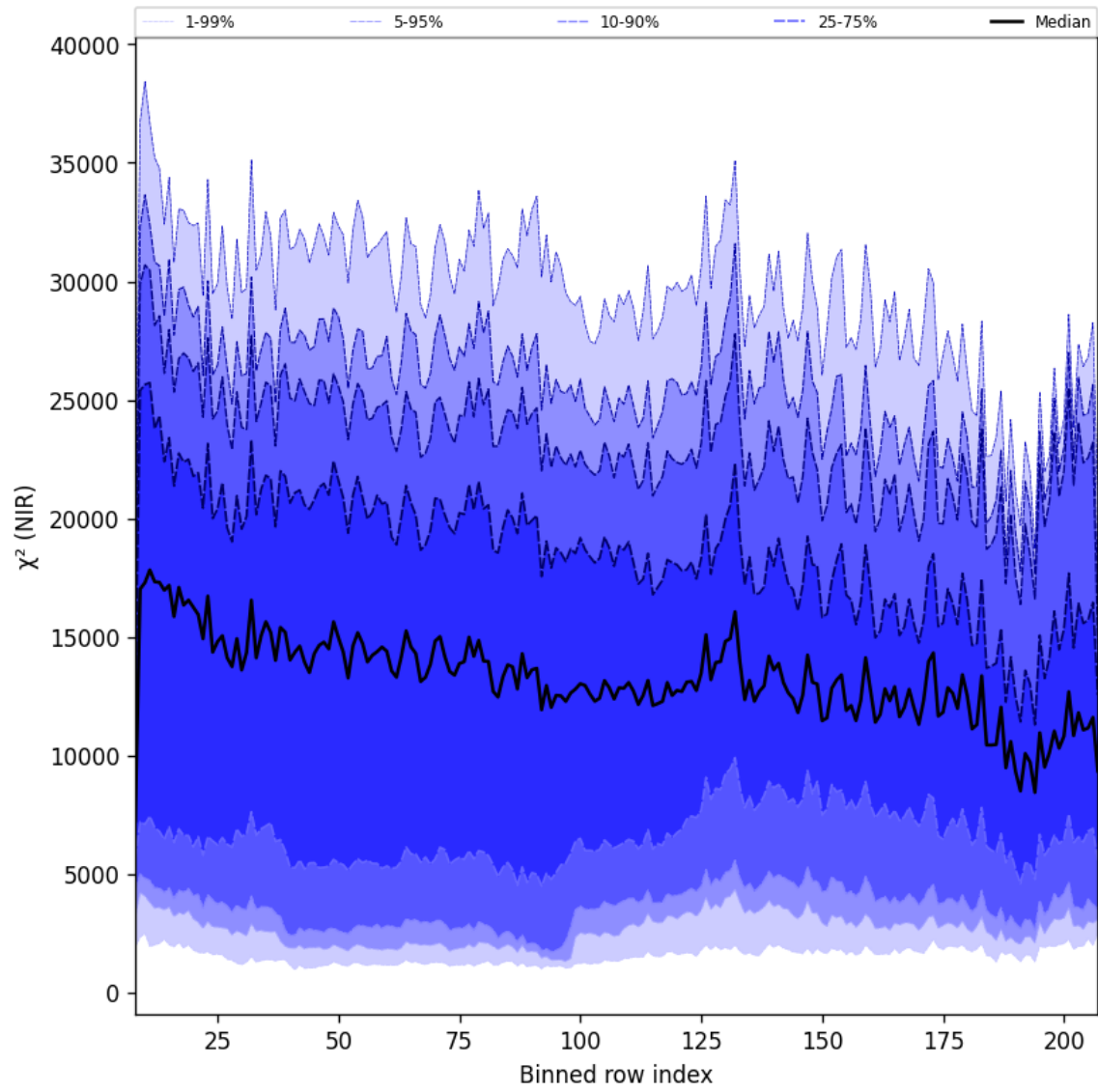
Figure 40: Along track statistics of “ \chi^2 (NIR)” for 2024-12-13 to 2024-12-15
