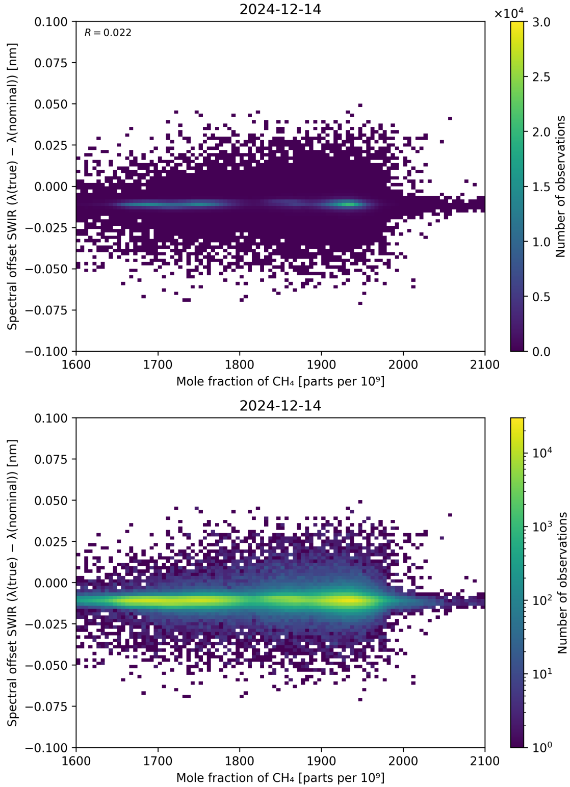
Figure 86: Scatter density plot of “Mole fraction of CH 4 ” against “Spectral offset SWIR ( \lambda_{\text{true}} - \lambda_{\text{nominal}} )” for 2024-12-13 to 2024-12-15.
