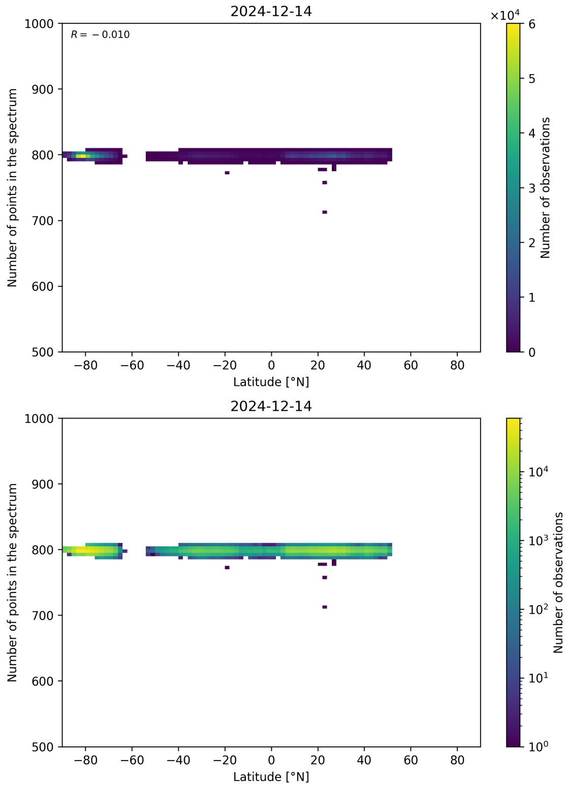
Figure 61: Scatter density plot of “Latitude” against “Number of points in the spectrum” for 2024-12-13 to 2024-12-15.
