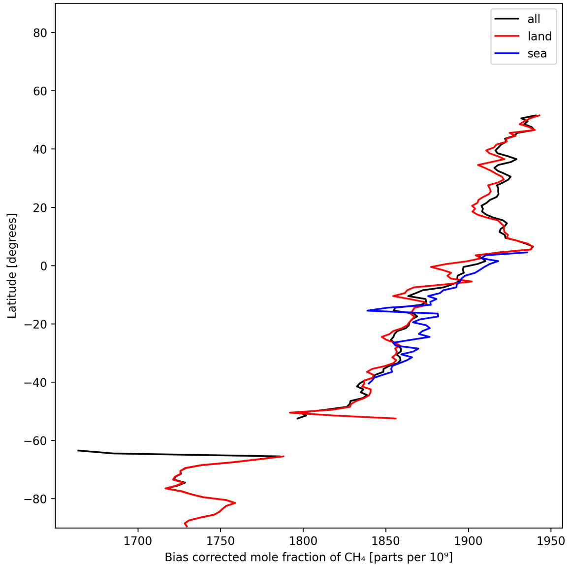
Figure 14: Zonal average of “Bias corrected mole fraction of CH 4 ” for 2024-12-13 to 2024-12-15.
