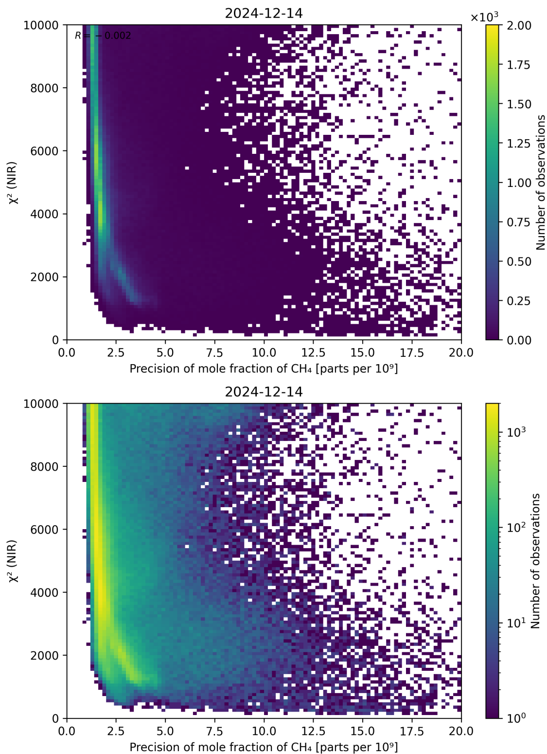
Figure 78: Scatter density plot of “Precision of mole fraction of \text{CH}_4 ” against “ \chi^2 (NIR)” for 2024-12-13 to 2024-12-15.
