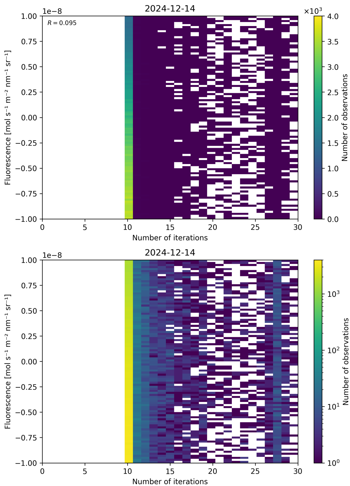
Figure 87: Scatter density plot of “Number of iterations” against “Fluorescence” for 2024-12-13 to 2024-12-15.
