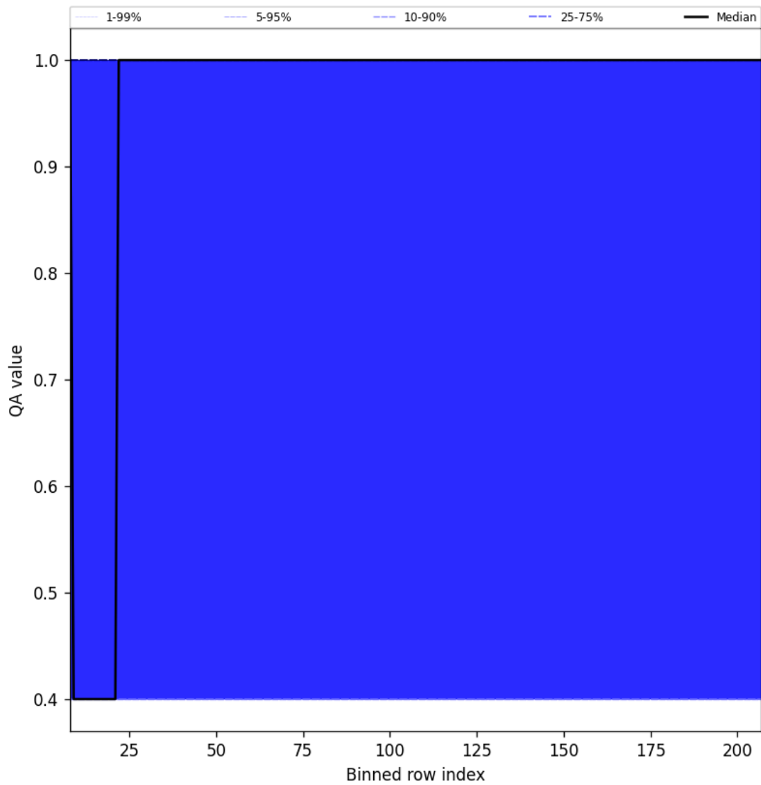
Figure 33: Along track statistics of “QA value” for 2024-12-13 to 2024-12-15
