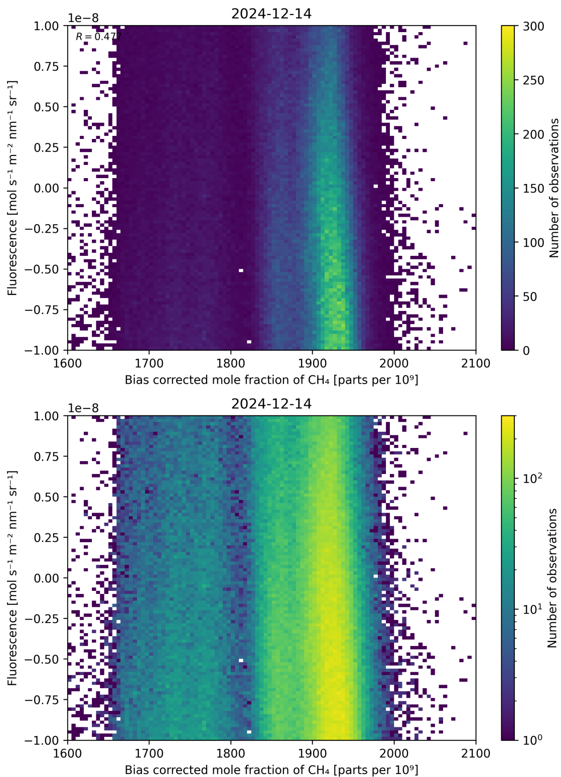
Figure 66: Scatter density plot of “Bias corrected mole fraction of \text{CH}_4 ” against “Fluorescence” for 2024-12-13 to 2024-12-15.
