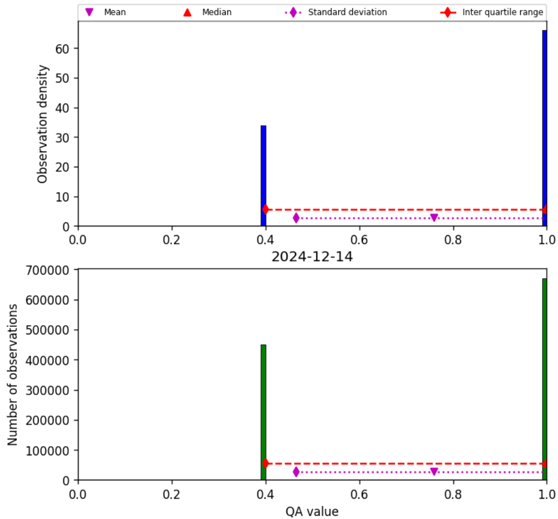
Figure 22: Histogram of “QA value” for 2024-12-13 to 2024-12-15
