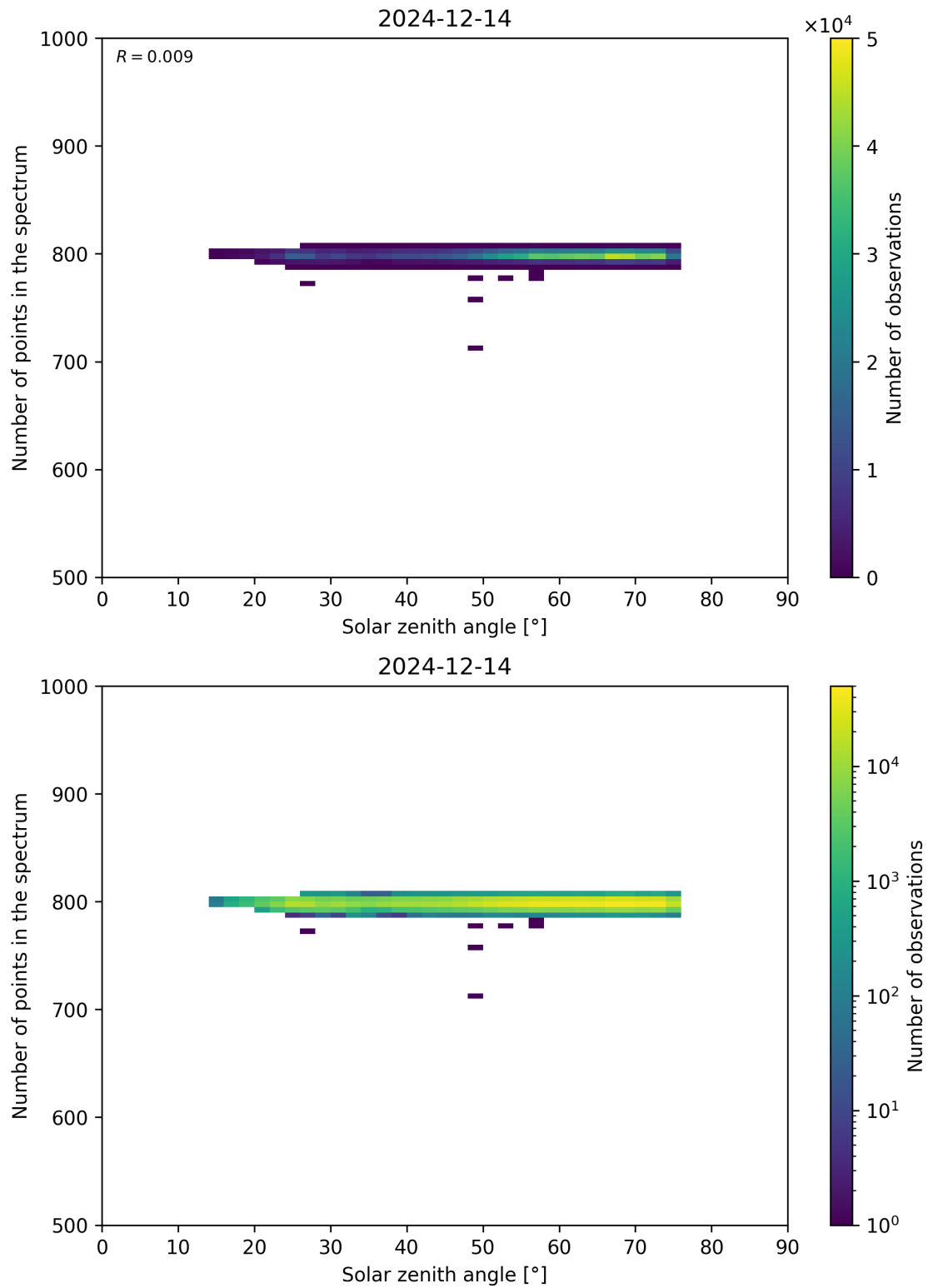
Figure 103: Scatter density plot of “Solar zenith angle” against “Number of points in the spectrum” for 2024-12-13 to 2024-12-15.
