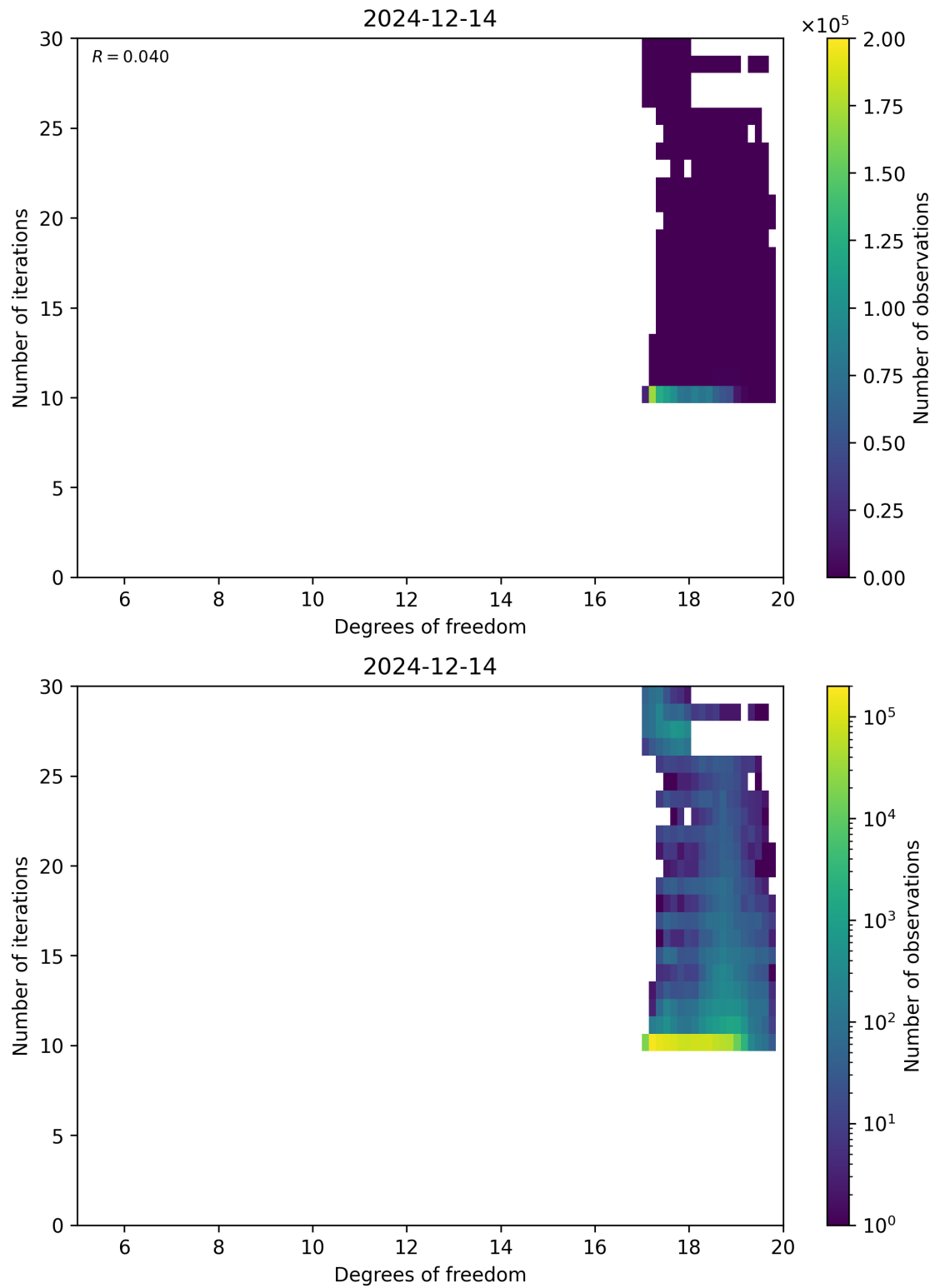
Figure 52: Scatter density plot of “Degrees of freedom” against “Number of iterations” for 2024-12-13 to 2024-12-15.
