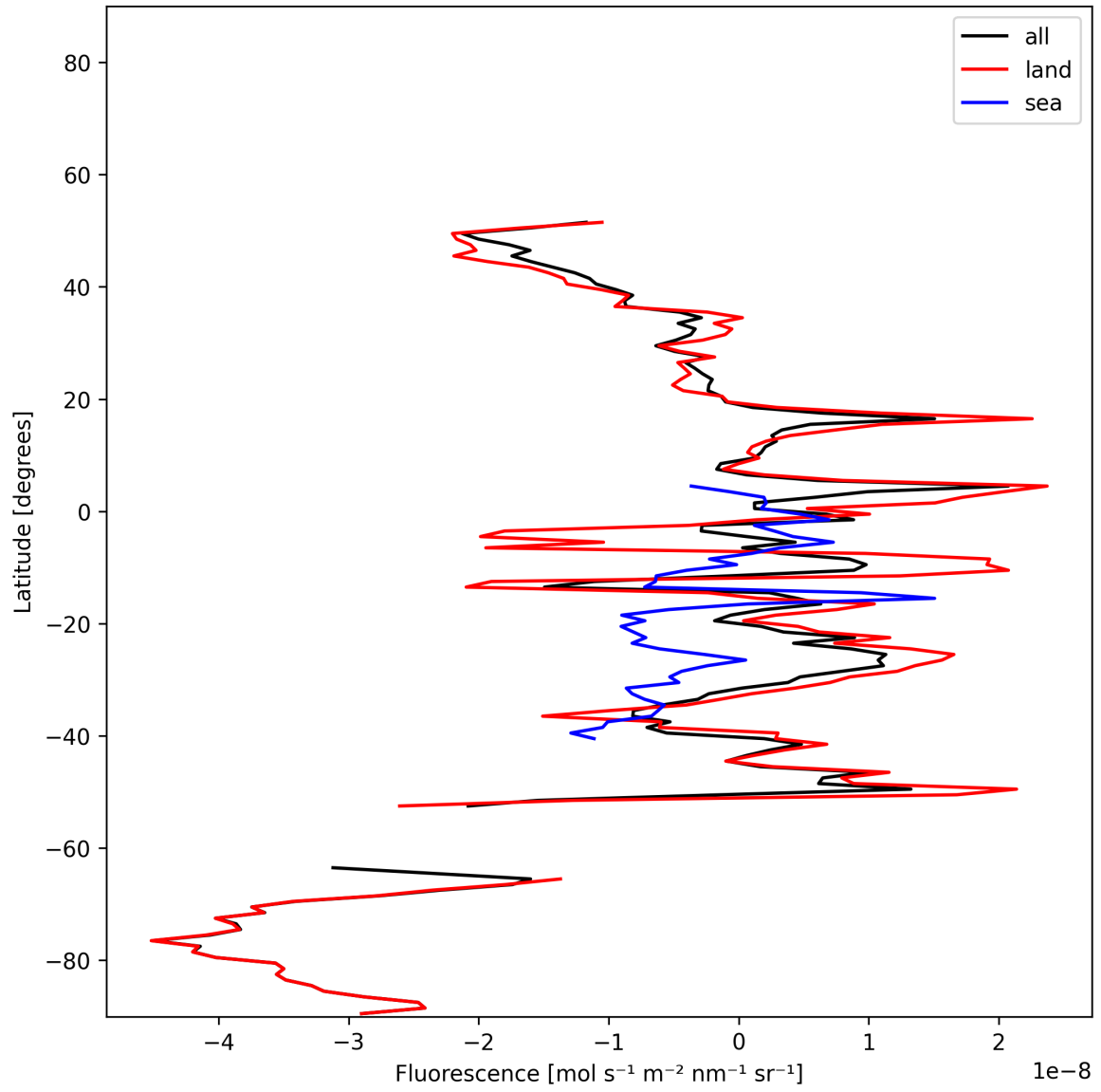
Figure 21: Zonal average of “Fluorescence” for 2024-12-13 to 2024-12-15.
