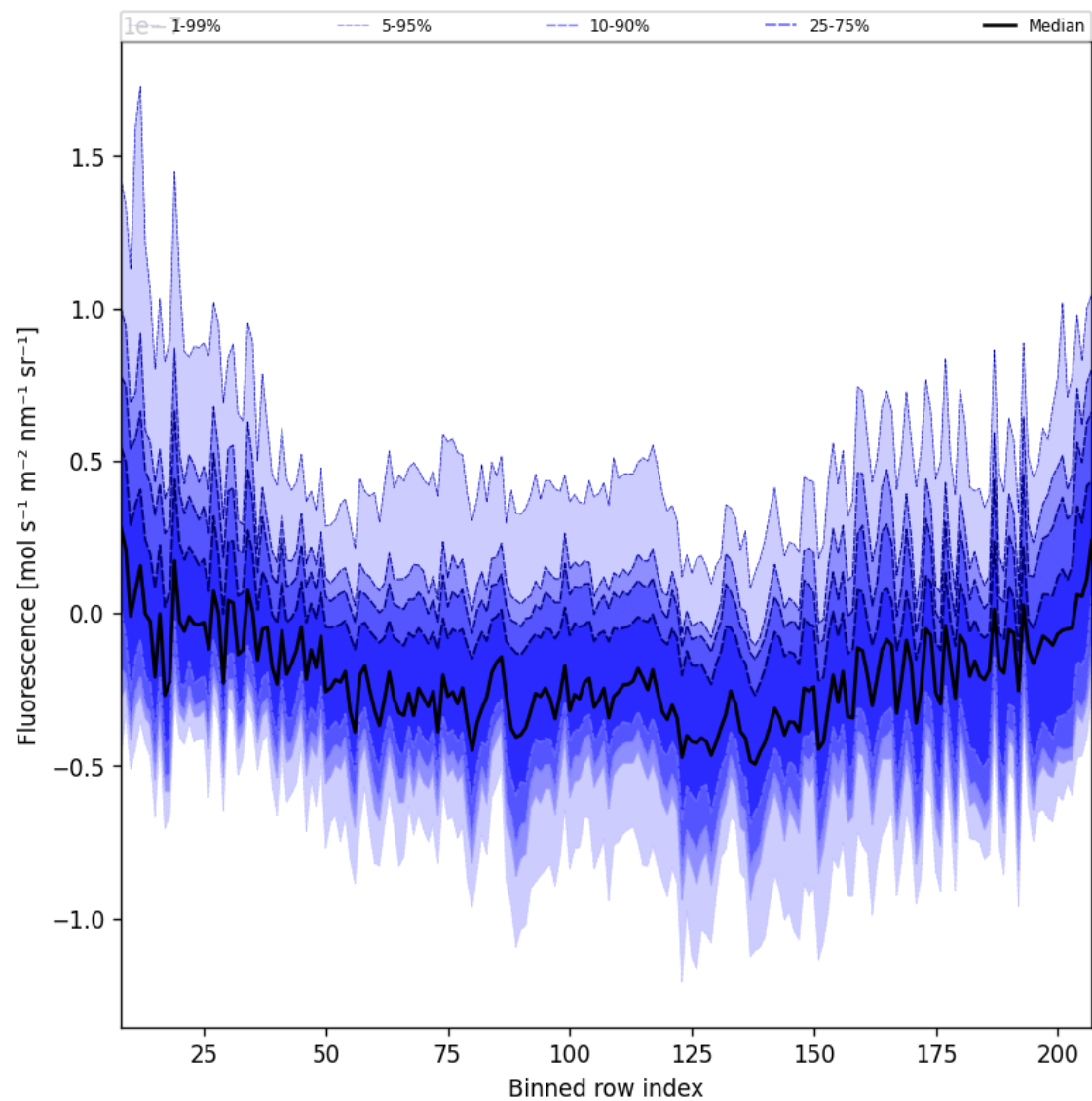
Figure 43: Along track statistics of “Fluorescence” for 2024-12-13 to 2024-12-15
