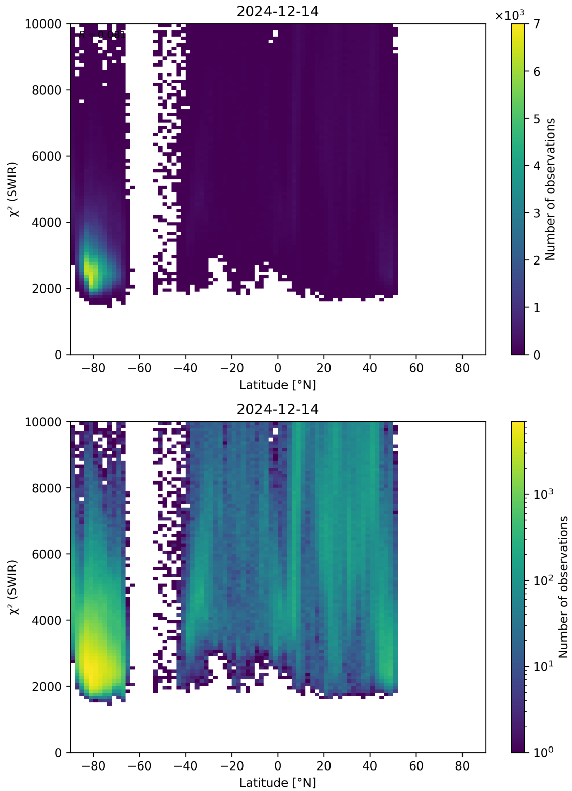
Figure 54: Scatter density plot of “Latitude” against “ \chi^2 (SWIR)” for 2024-12-13 to 2024-12-15.
