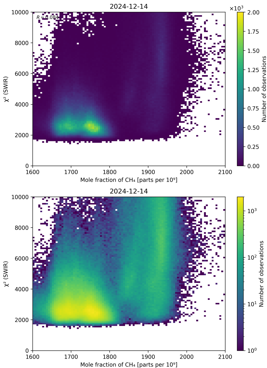
Figure 71: Scatter density plot of “Mole fraction of \text{CH}_4 ” against “ \chi^2 (SWIR)” for 2024-12-13 to 2024-12-15.
