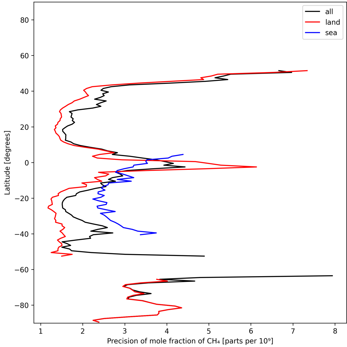
Figure 13: Zonal average of “Precision of mole fraction of CH 4 ” for 2024-12-13 to 2024-12-15.
