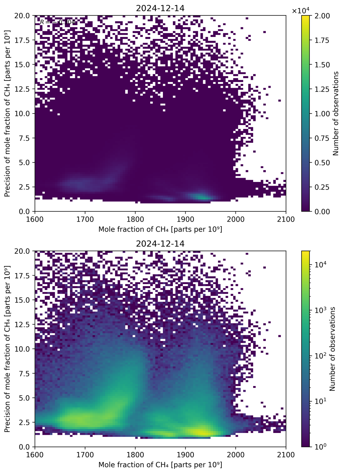
Figure 75: Scatter density plot of “Mole fraction of CH 4 ” against “Precision of mole fraction of CH 4 ” for 2024-12-13 to 2024-12-15.
