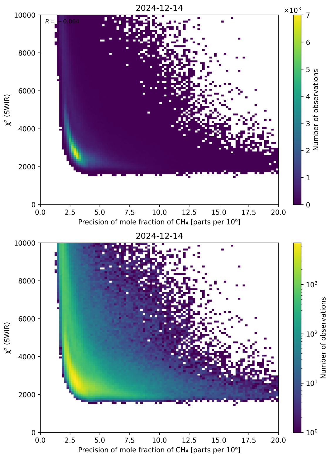
Figure 79: Scatter density plot of “Precision of mole fraction of CH 4 ” against “ \chi^2 (SWIR)” for 2024-12-13 to 2024-12-15.
