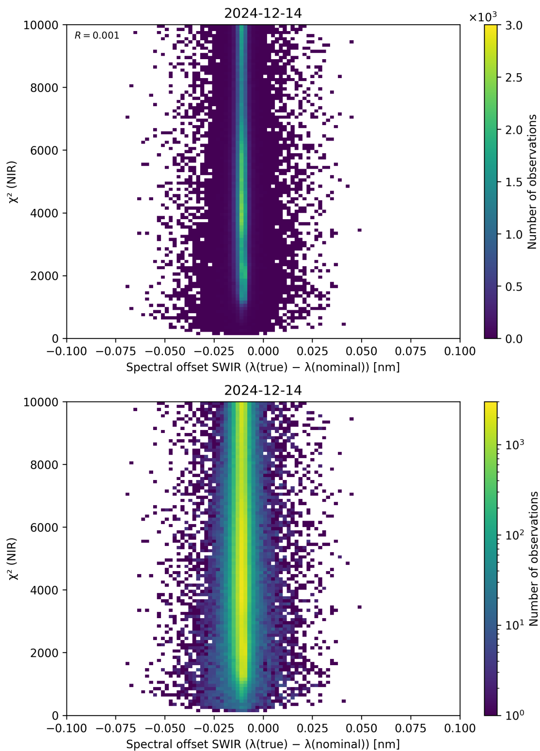
Figure 117: Scatter density plot of “Spectral offset SWIR ( \lambda_{\text{true}} - \lambda_{\text{nominal}} )” against “ \chi^2 (NIR)” for 2024-12-13 to 2024-12-15.
