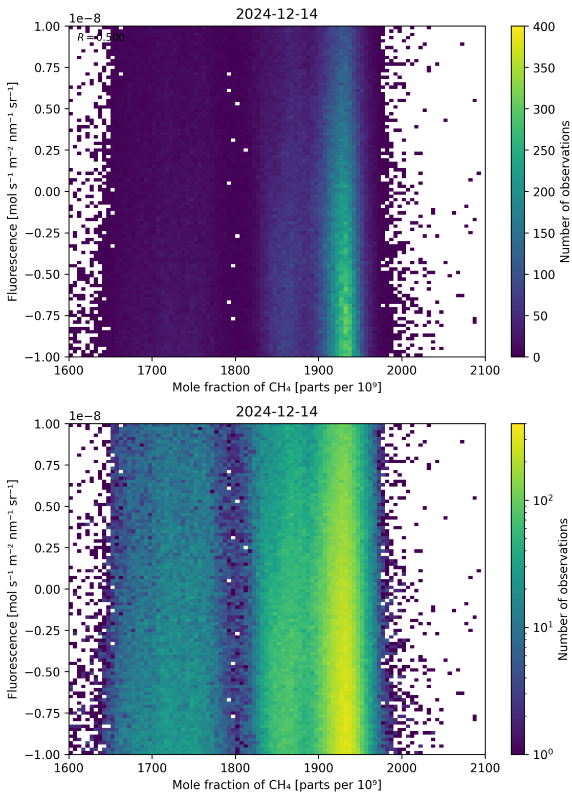
Figure 73: Scatter density plot of “Mole fraction of \text{CH}_4 ” against “Fluorescence” for 2024-12-13 to 2024-12-15.
