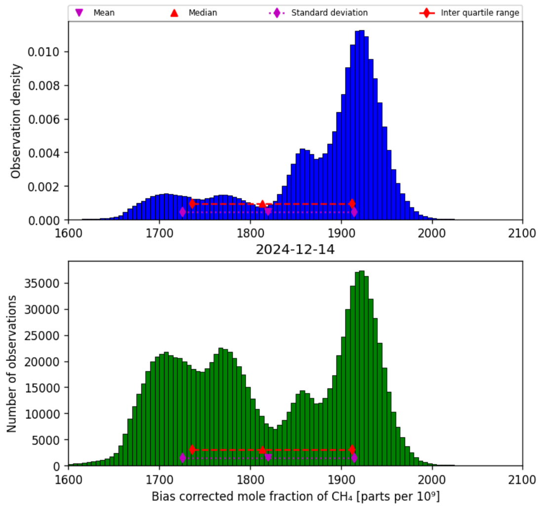
Figure 25: Histogram of “Bias corrected mole fraction of CH 4 ” for 2024-12-13 to 2024-12-15
