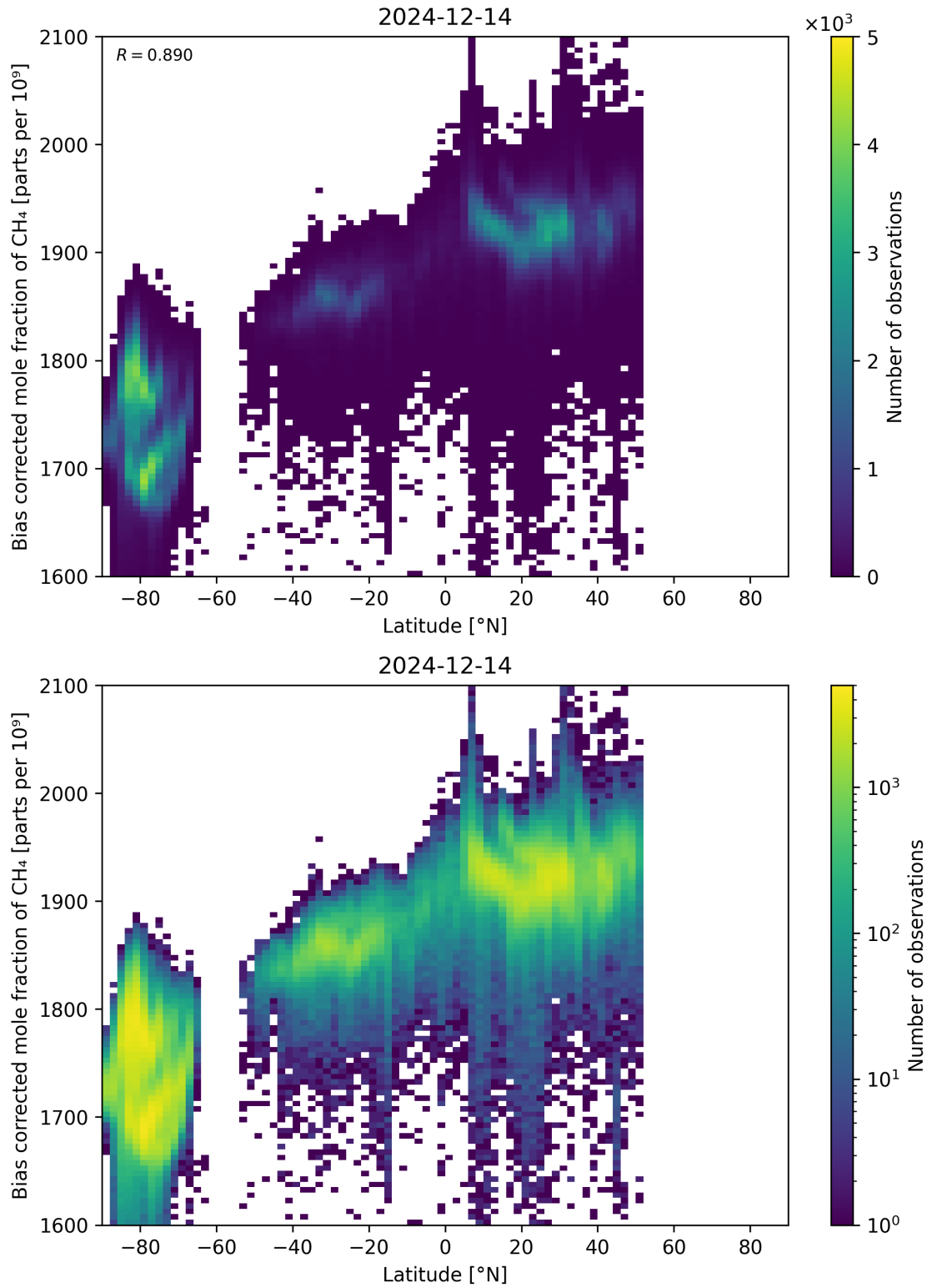
Figure 58: Scatter density plot of “Latitude” against “Bias corrected mole fraction of CH 4 ” for 2024-12-13 to 2024-12-15.
