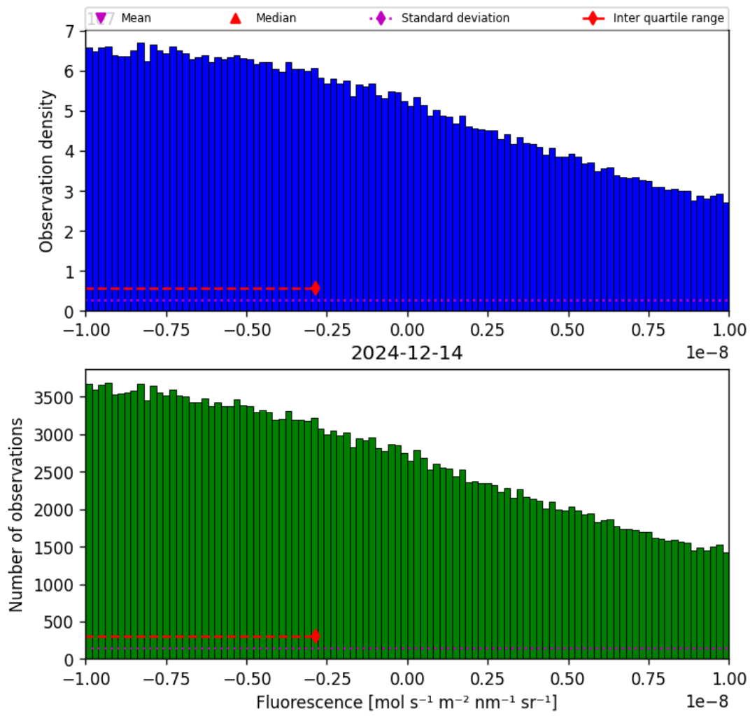
Figure 32: Histogram of “Fluorescence” for 2024-12-13 to 2024-12-15
