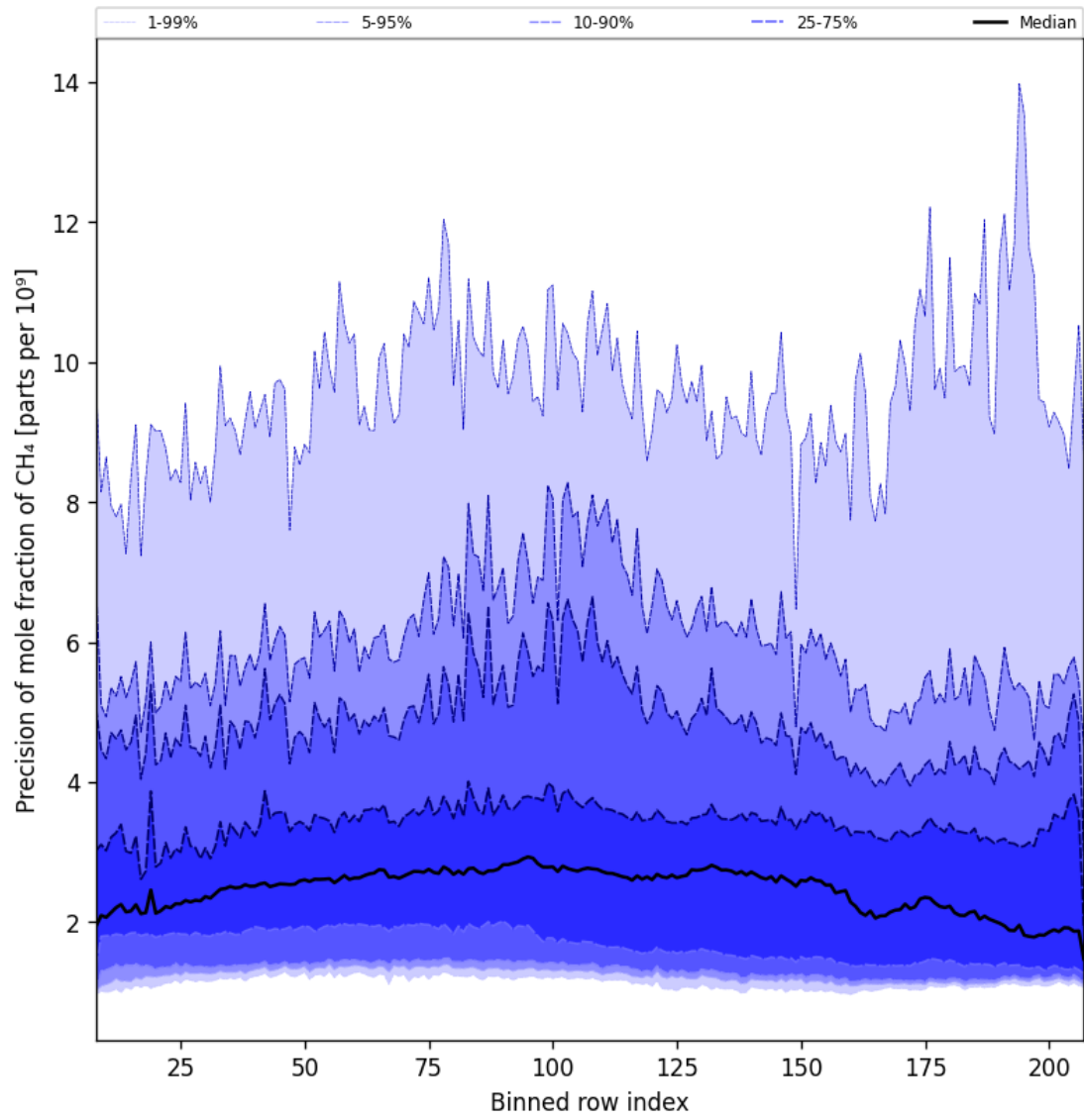
Figure 35: Along track statistics of “Precision of mole fraction of CH 4 ” for 2024-12-13 to 2024-12-15
