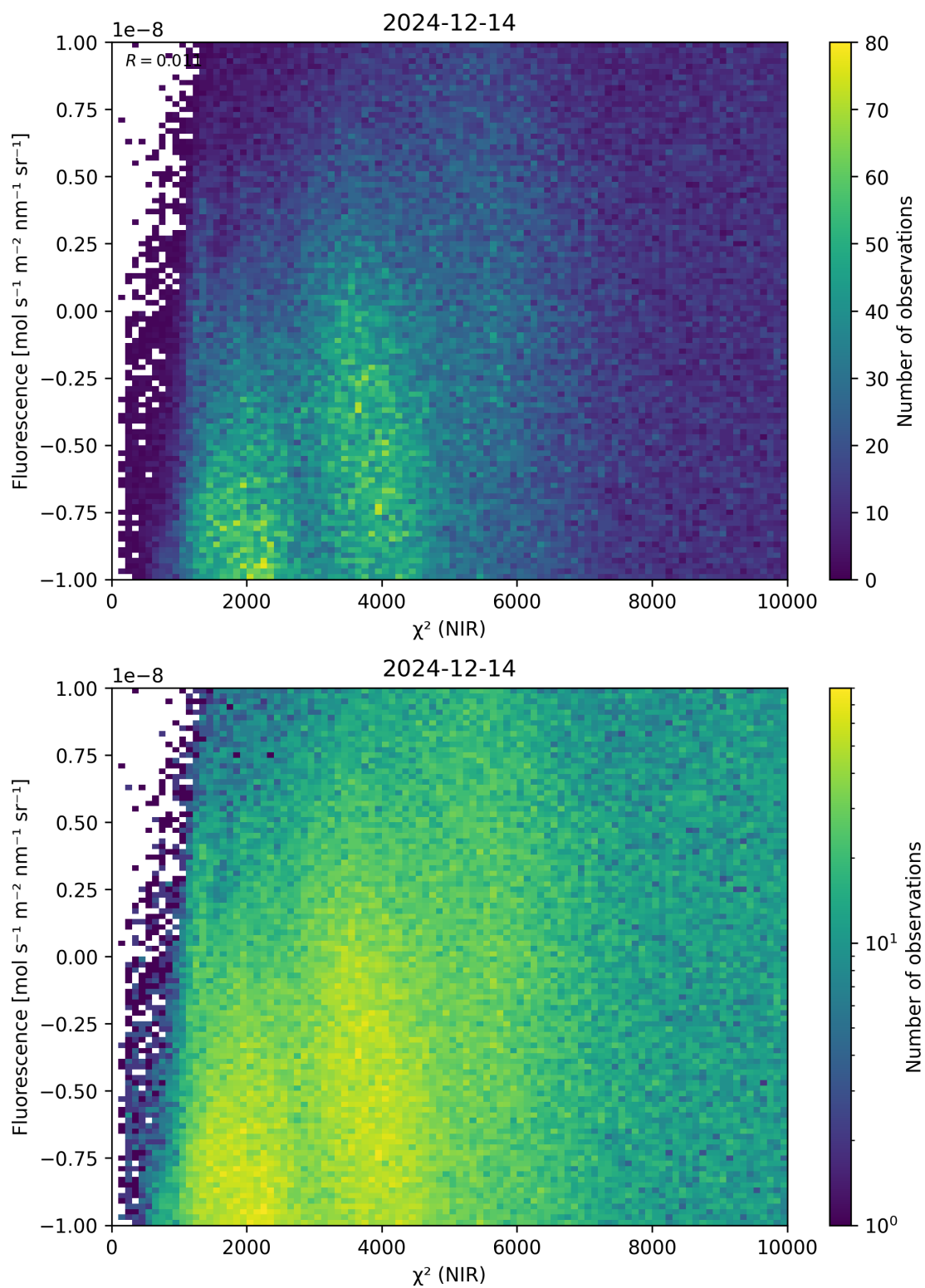
Figure 45: Scatter density plot of “ \chi^2 (NIR)” against “Fluorescence” for 2024-12-13 to 2024-12-15.
