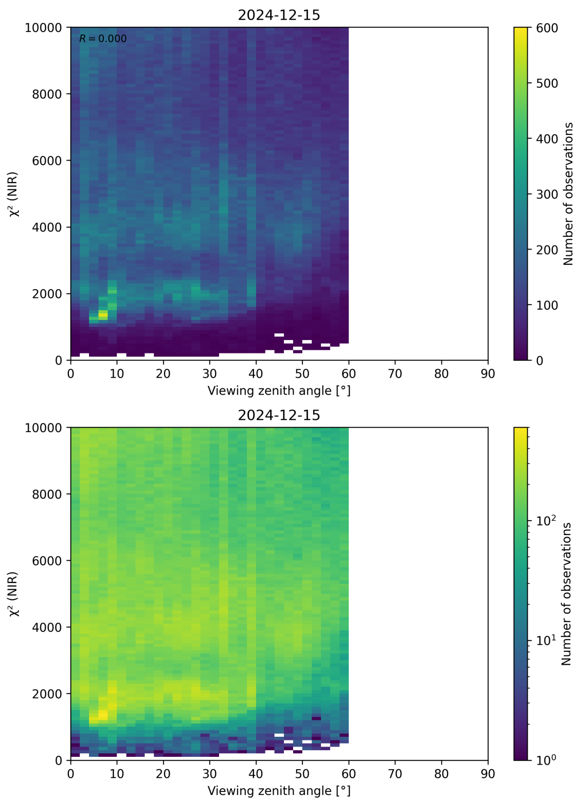
Figure 105: Scatter density plot of “Viewing zenith angle” against “ \chi^2 (NIR)” for 2024-12-14 to 2024-12-16.
