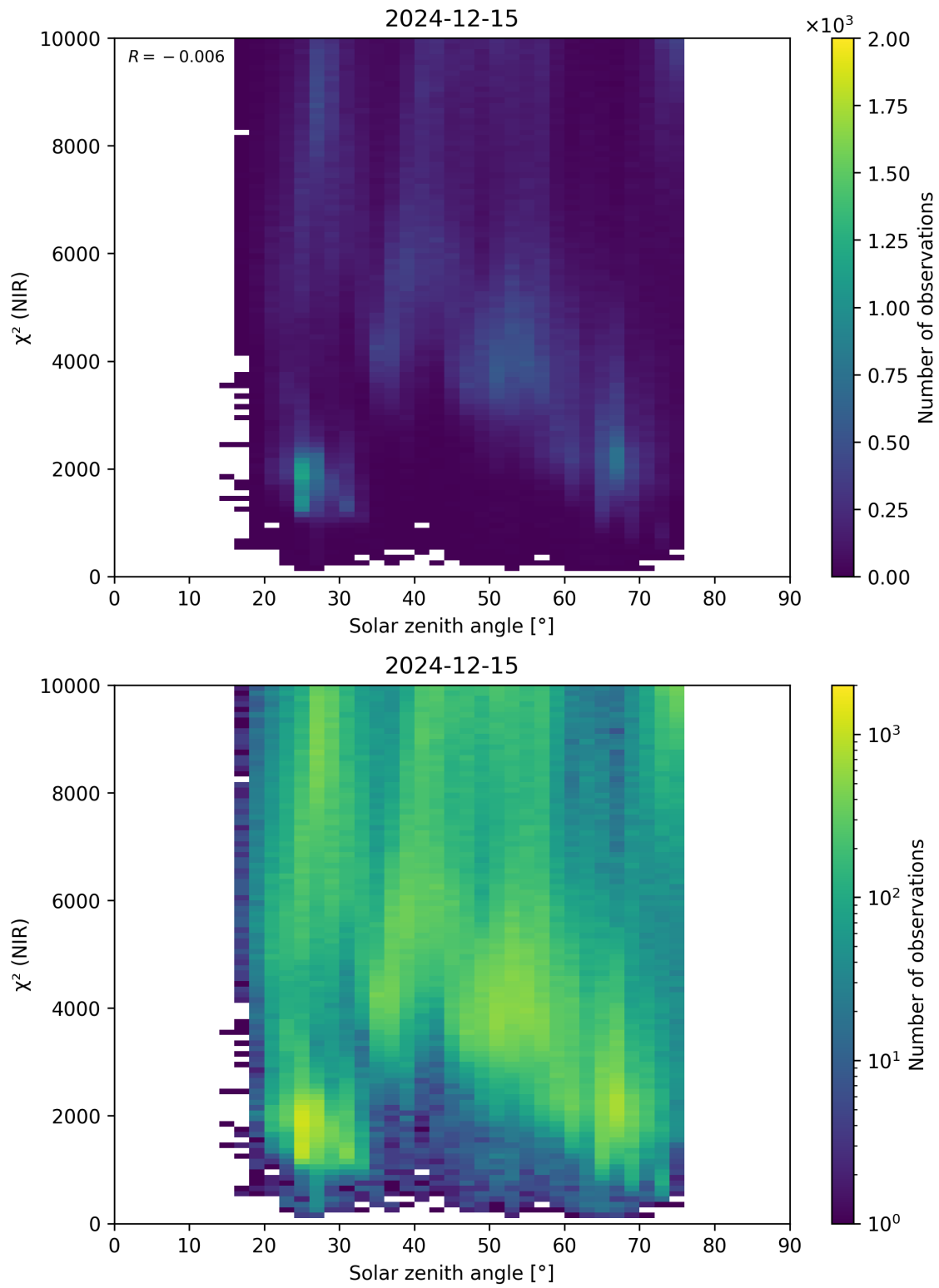
Figure 94: Scatter density plot of “Solar zenith angle” against “ \chi^2 (NIR)” for 2024-12-14 to 2024-12-16.
