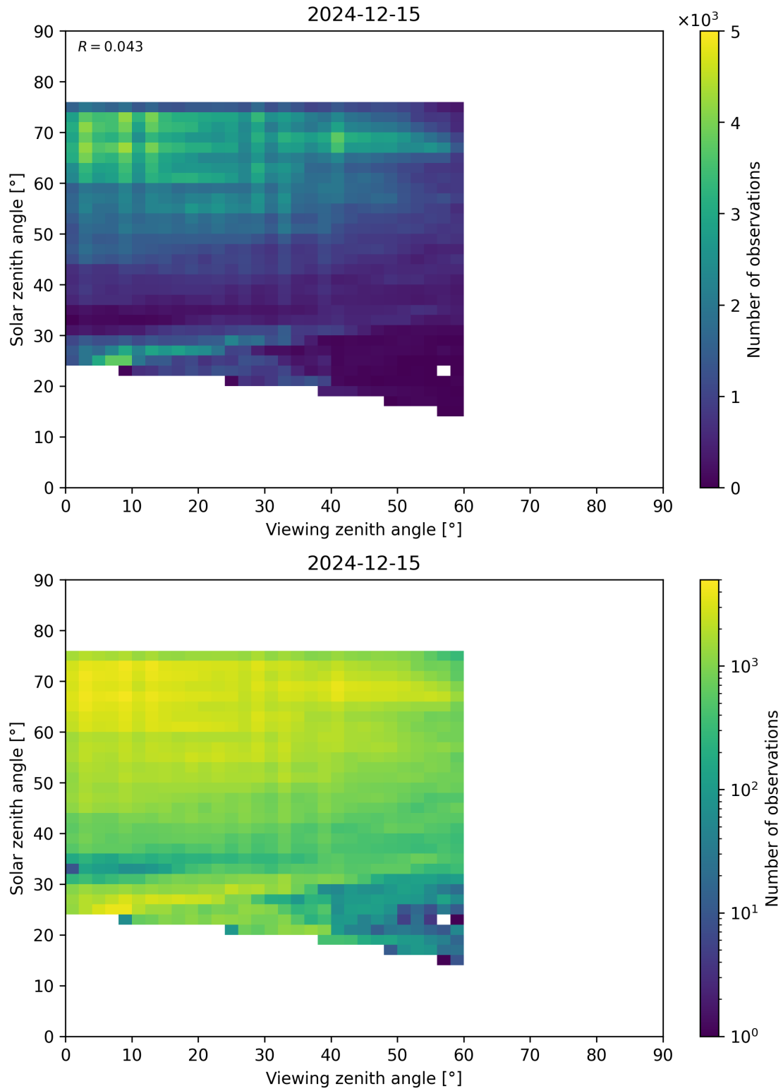
Figure 115: Scatter density plot of “Viewing zenith angle” against “Solar zenith angle” for 2024-12-14 to 2024-12-16.
