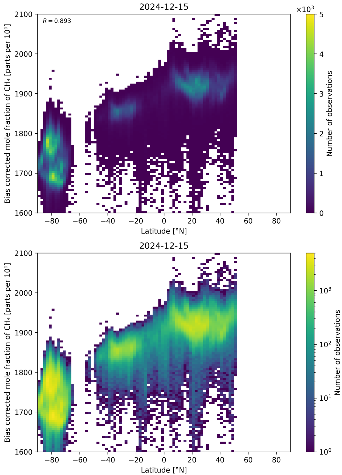
Figure 58: Scatter density plot of “Latitude” against “Bias corrected mole fraction of CH 4 ” for 2024-12-14 to 2024-12-16.
