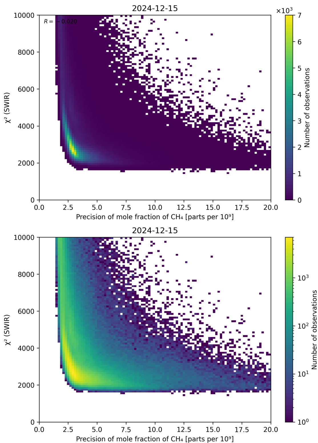
Figure 79: Scatter density plot of “Precision of mole fraction of CH 4 ” against “ \chi^2 (SWIR)” for 2024-12-14 to 2024-12-16.
