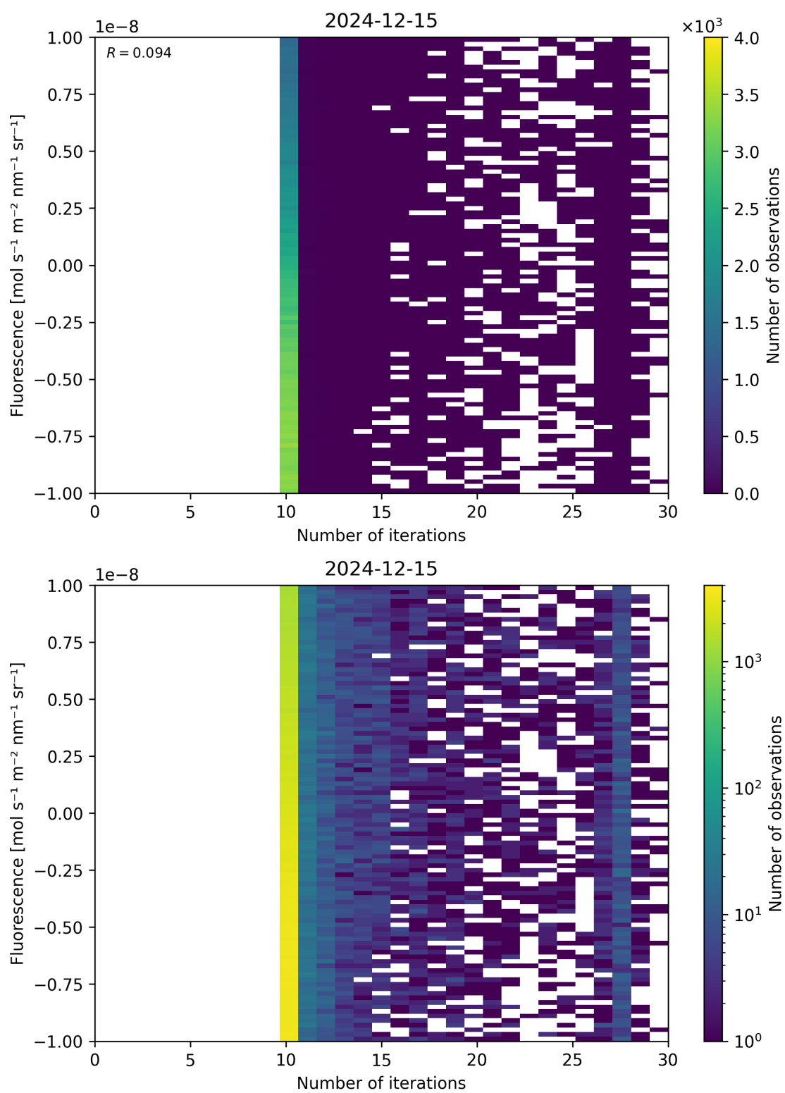
Figure 87: Scatter density plot of “Number of iterations” against “Fluorescence” for 2024-12-14 to 2024-12-16.
