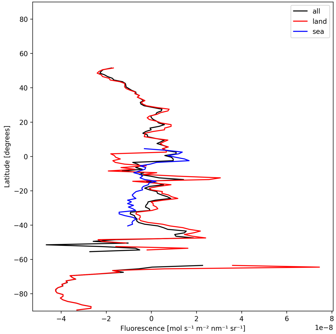
Figure 21: Zonal average of “Fluorescence” for 2024-12-14 to 2024-12-16.
