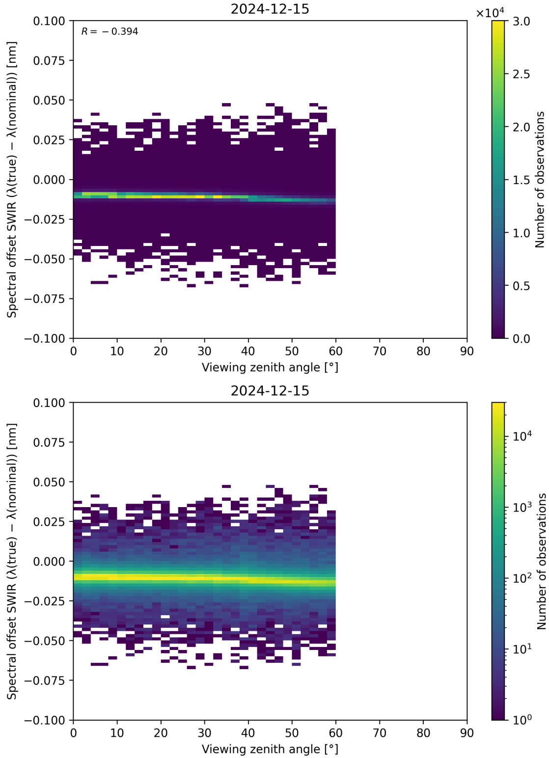
Figure 116: Scatter density plot of “Viewing zenith angle” against “Spectral offset SWIR ( \lambda_{\text{true}} - \lambda_{\text{nominal}} )” for 2024-12-14 to 2024-12-16.
