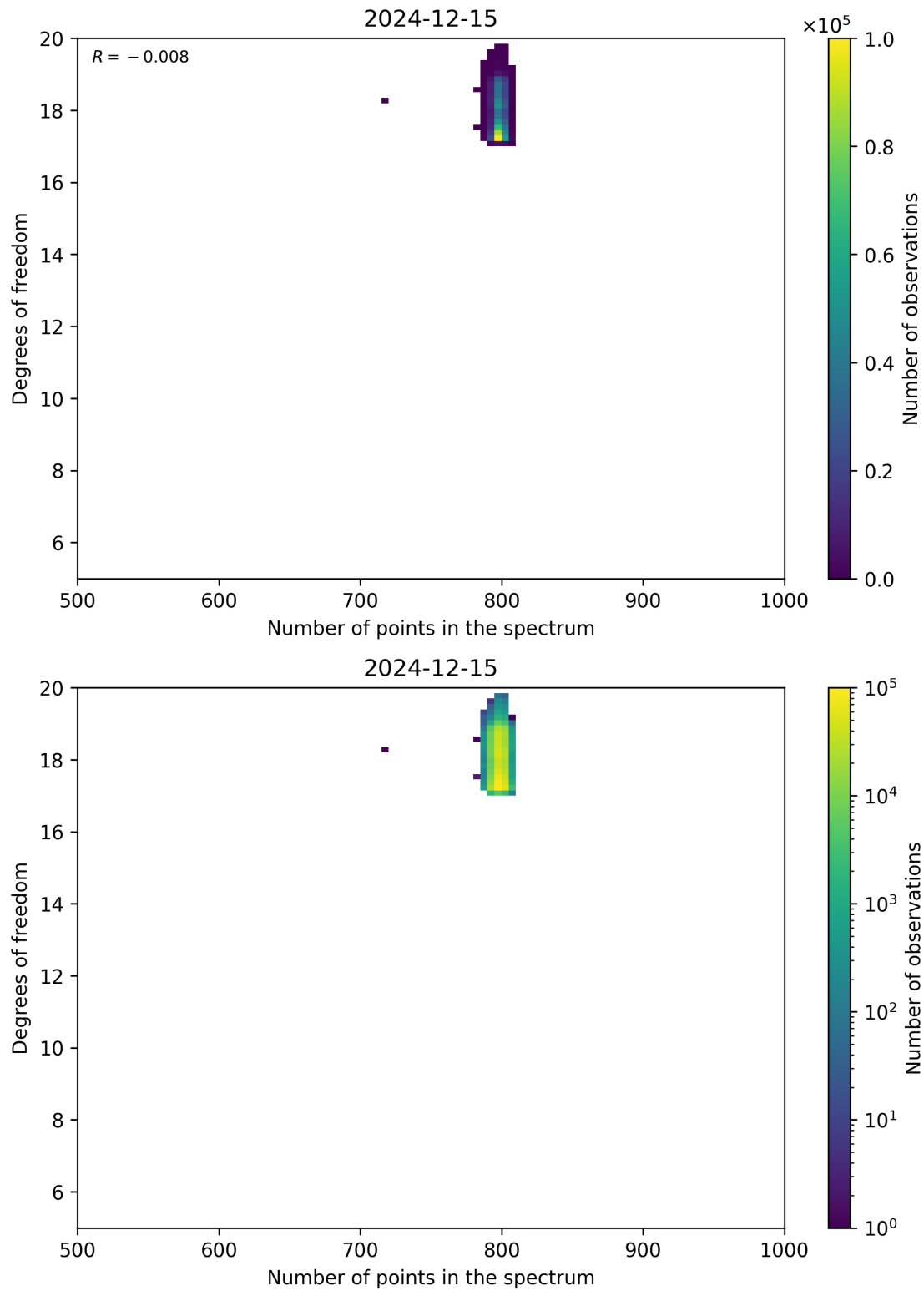
Figure 90: Scatter density plot of “Number of points in the spectrum” against “Degrees of freedom” for 2024-12-14 to 2024-12-16.
