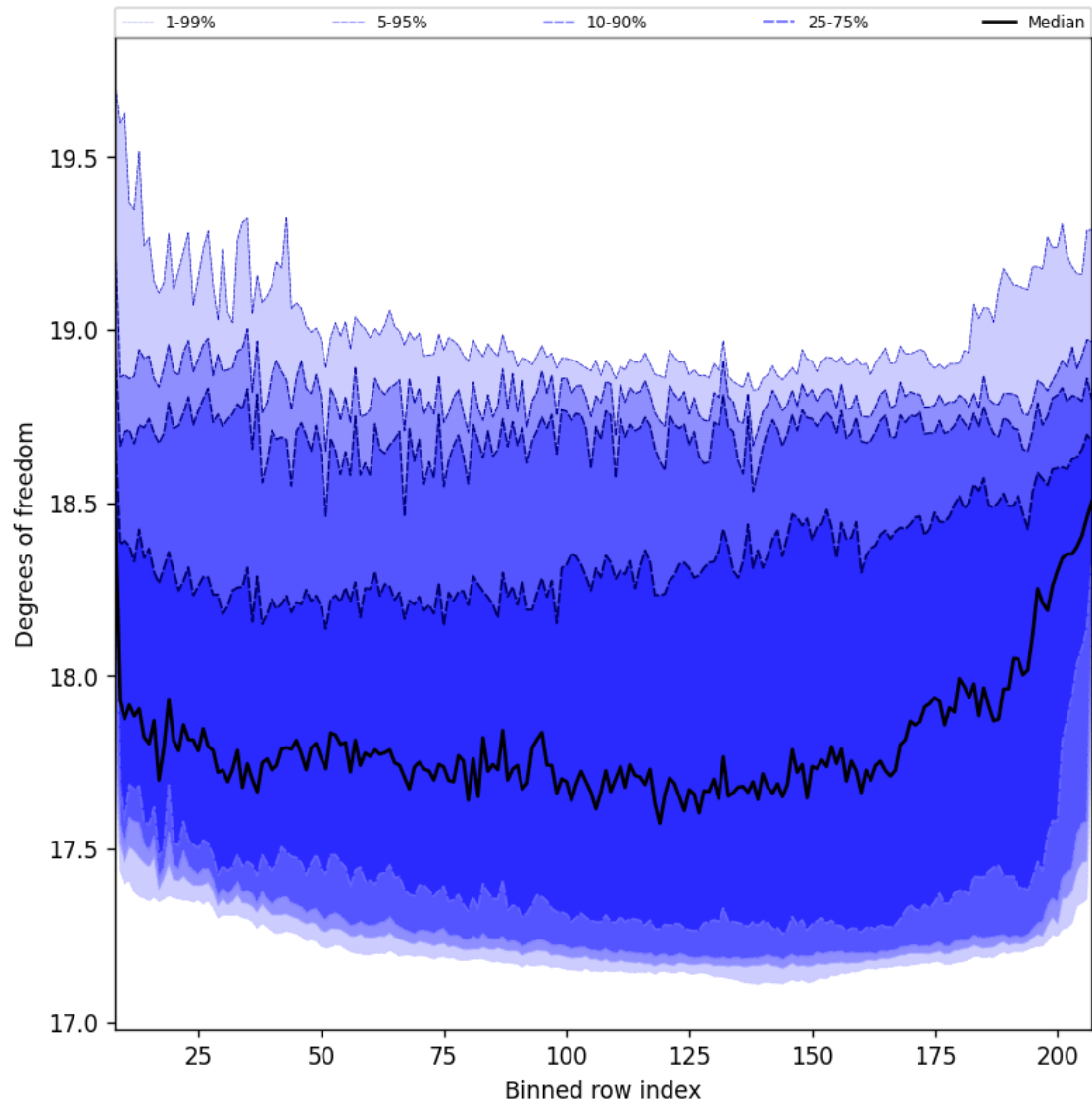
Figure 41: Along track statistics of “Degrees of freedom” for 2024-12-14 to 2024-12-16
