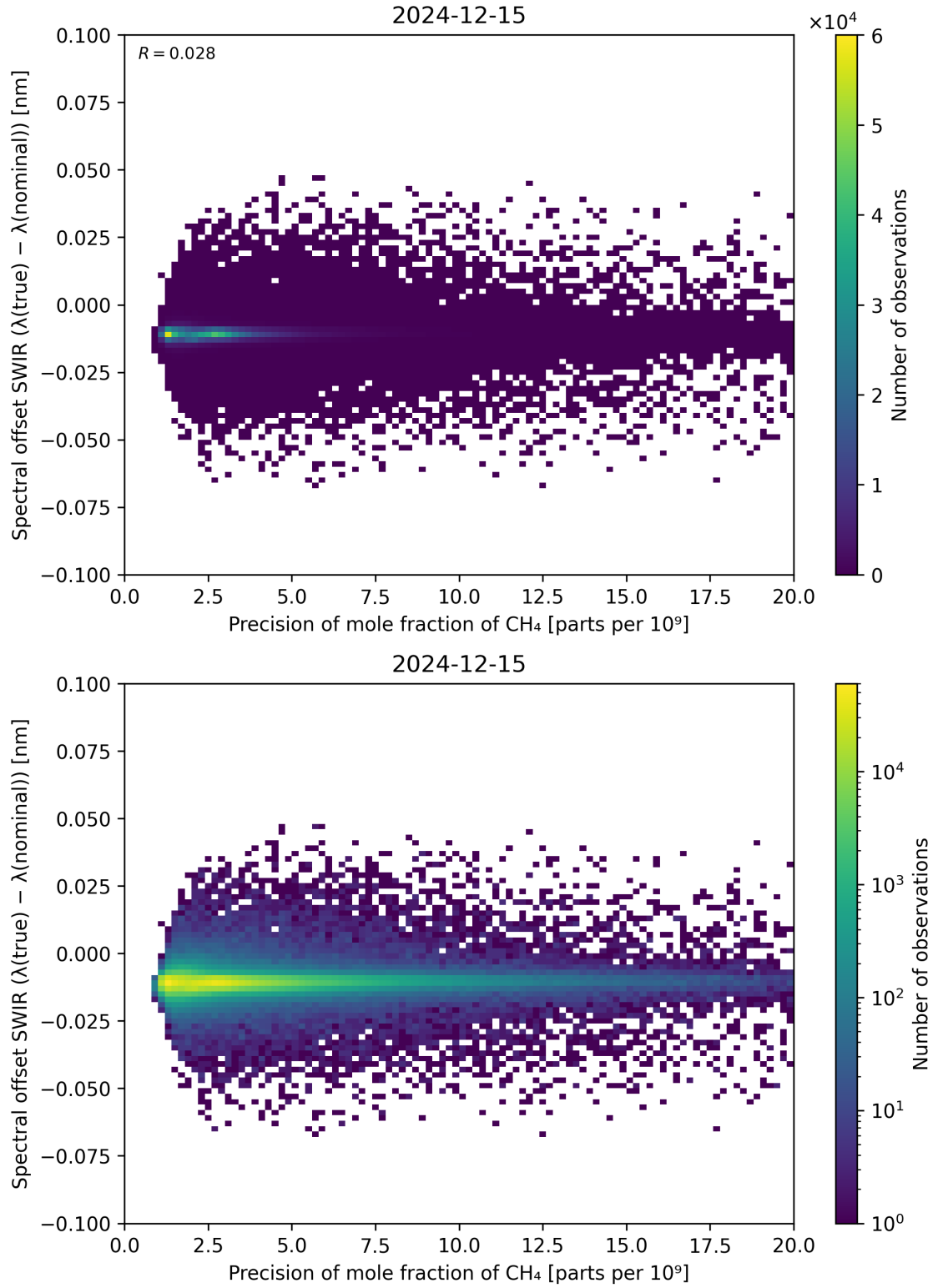
Figure 85: Scatter density plot of “Precision of mole fraction of CH 4 ” against “Spectral offset SWIR ( \lambda_{\text{true}} - \lambda_{\text{nominal}} )” for 2024-12-14 to 2024-12-16.
