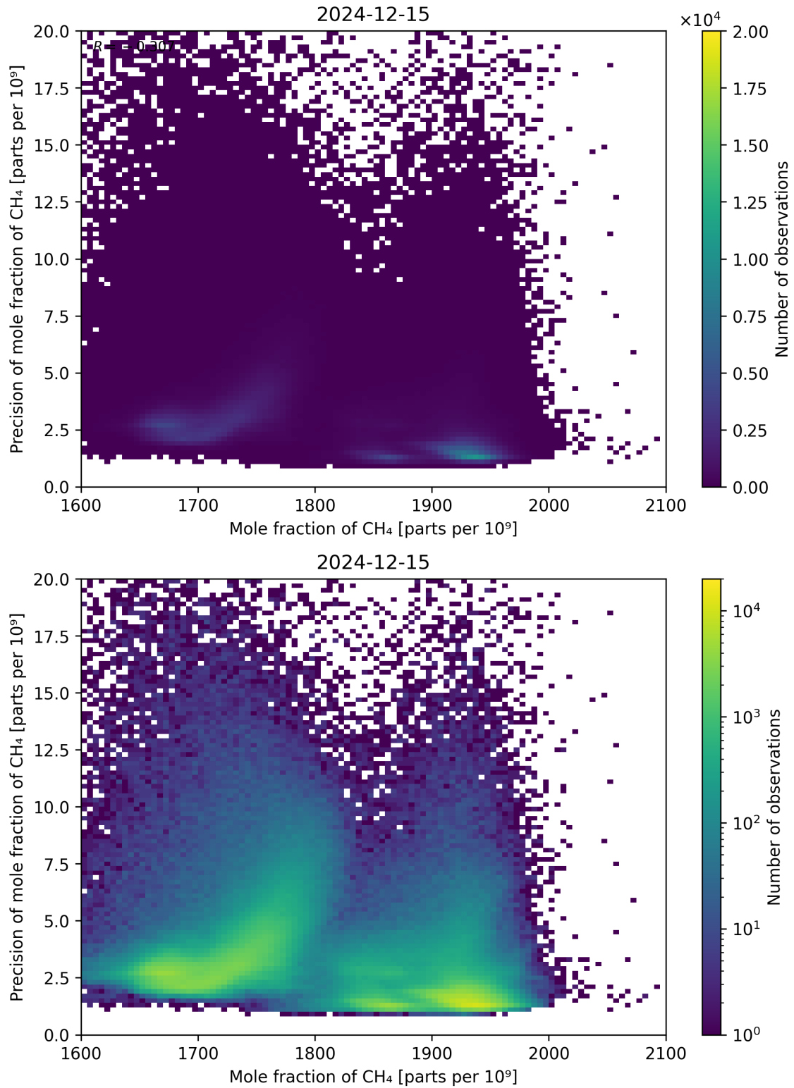
Figure 75: Scatter density plot of “Mole fraction of CH 4 ” against “Precision of mole fraction of CH 4 ” for 2024-12-14 to 2024-12-16.
