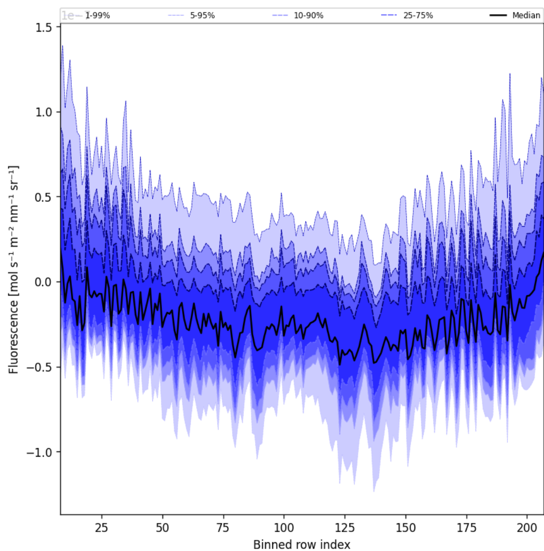
Figure 43: Along track statistics of “Fluorescence” for 2024-12-14 to 2024-12-16
