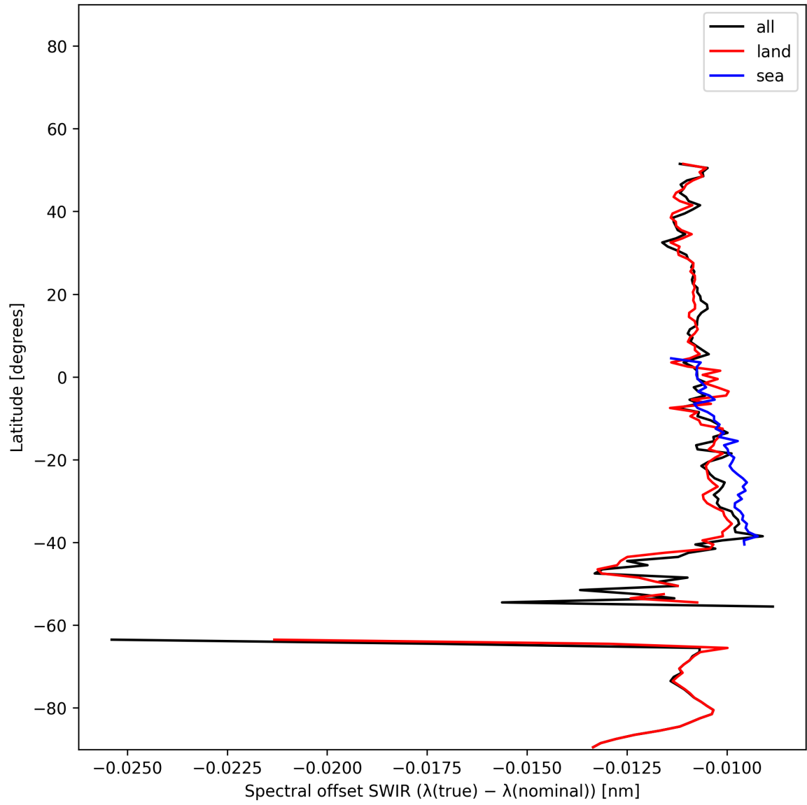
Figure 16: Zonal average of “Spectral offset SWIR ( \lambda_{\text{true}} - \lambda_{\text{nominal}} )” for 2024-12-14 to 2024-12-16.
