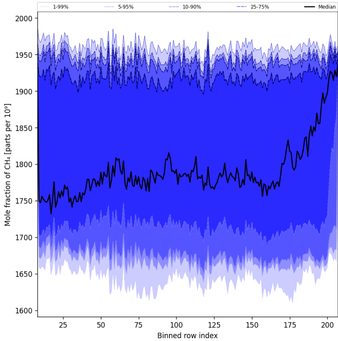
Figure 34: Along track statistics of “Mole fraction of CH 4 ” for 2024-12-14 to 2024-12-16
