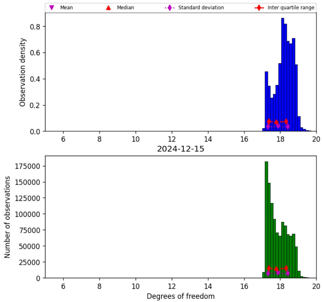
Figure 30: Histogram of “Degrees of freedom” for 2024-12-14 to 2024-12-16
