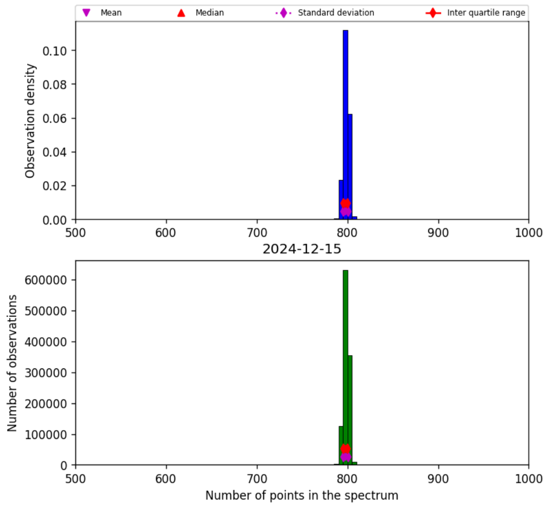
Figure 26: Histogram of “Number of points in the spectrum” for 2024-12-14 to 2024-12-16
