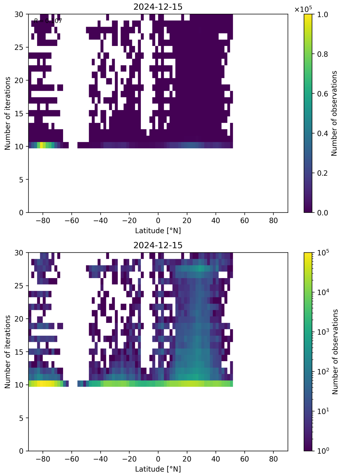
Figure 60: Scatter density plot of “Latitude” against “Number of iterations” for 2024-12-14 to 2024-12-16.
