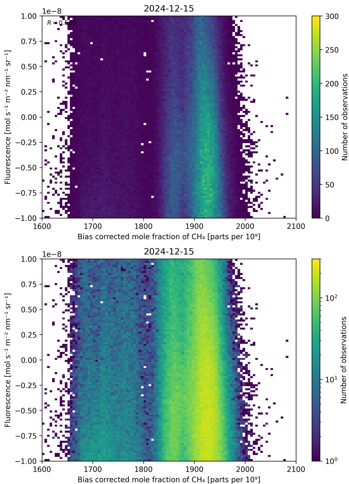
Figure 66: Scatter density plot of “Bias corrected mole fraction of \text{CH}_4 ” against “Fluorescence” for 2024-12-14 to 2024-12-16.
