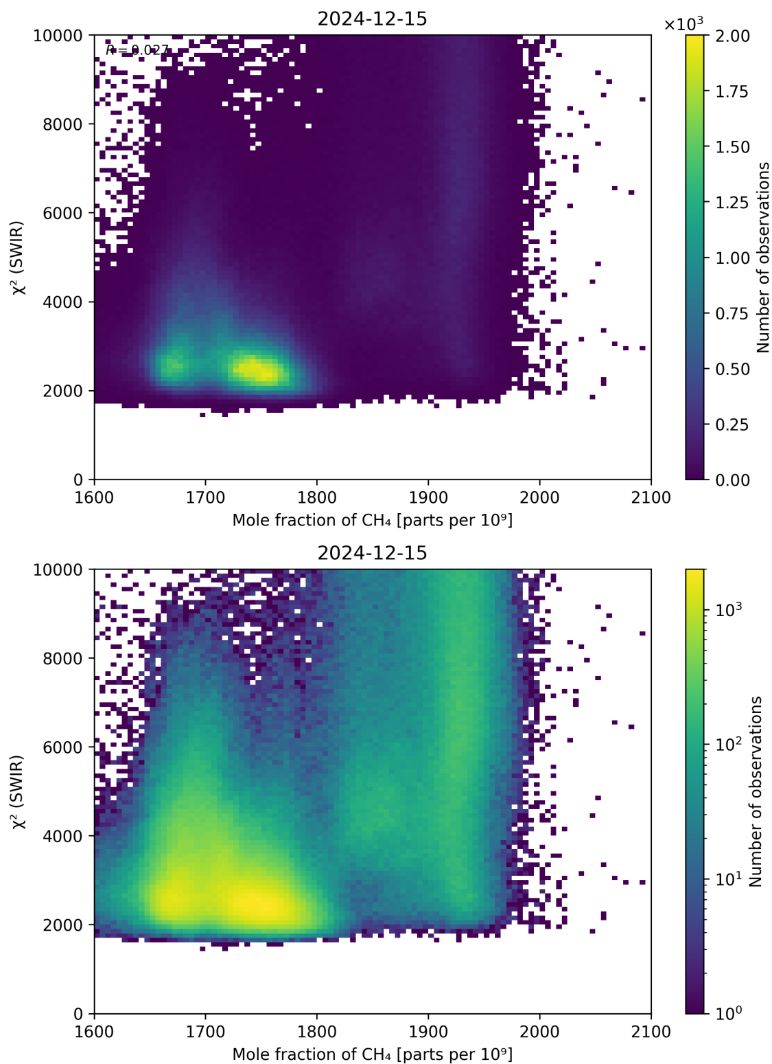
Figure 71: Scatter density plot of “Mole fraction of CH 4 ” against “ \chi^2 (SWIR)” for 2024-12-14 to 2024-12-16.
