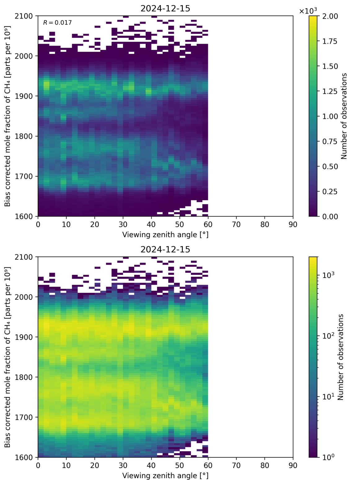
Figure 111: Scatter density plot of “Viewing zenith angle” against “Bias corrected mole fraction of CH 4 ” for 2024-12-14 to 2024-12-16.
