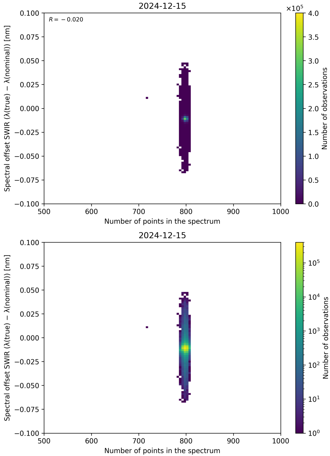
Figure 93: Scatter density plot of “Number of points in the spectrum” against “Spectral offset SWIR ( \lambda_{\text{true}} - \lambda_{\text{nominal}} )” for 2024-12-14 to 2024-12-16.
