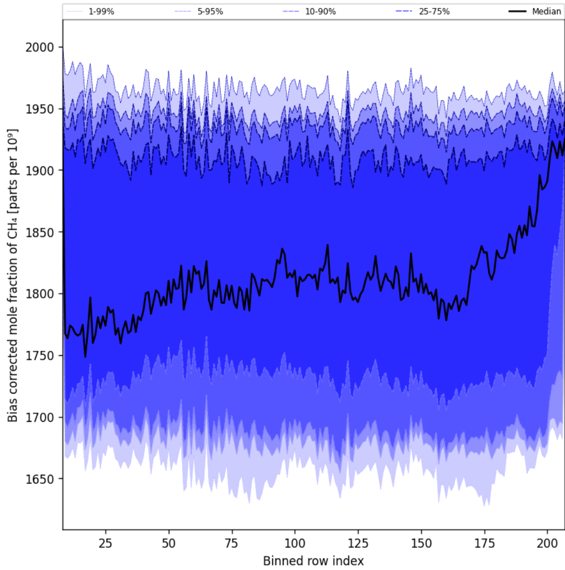
Figure 36: Along track statistics of “Bias corrected mole fraction of CH 4 ” for 2024-12-14 to 2024-12-16
