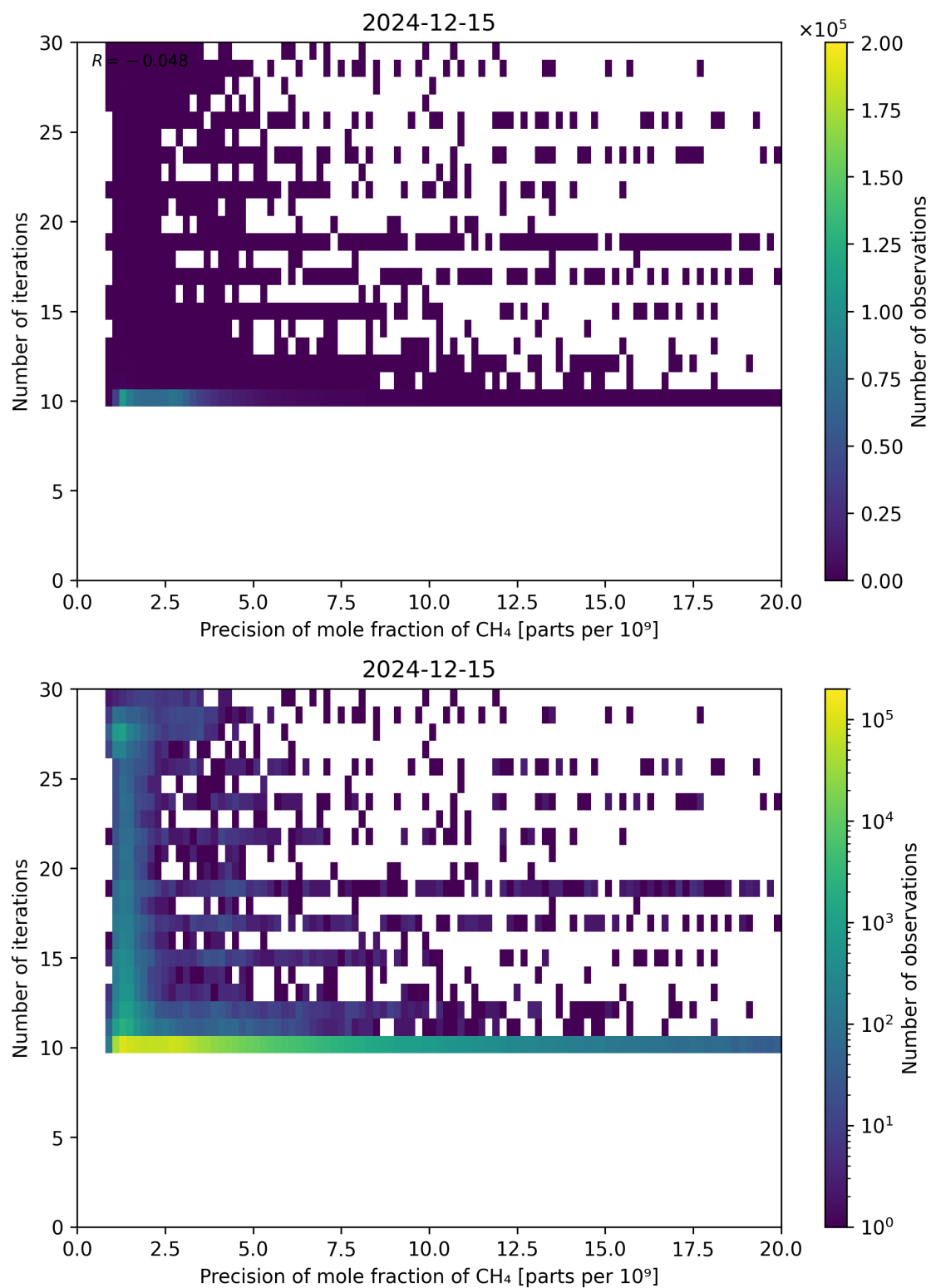
Figure 83: Scatter density plot of “Precision of mole fraction of CH 4 ” against “Number of iterations” for 2024-12-14 to 2024-12-16.
