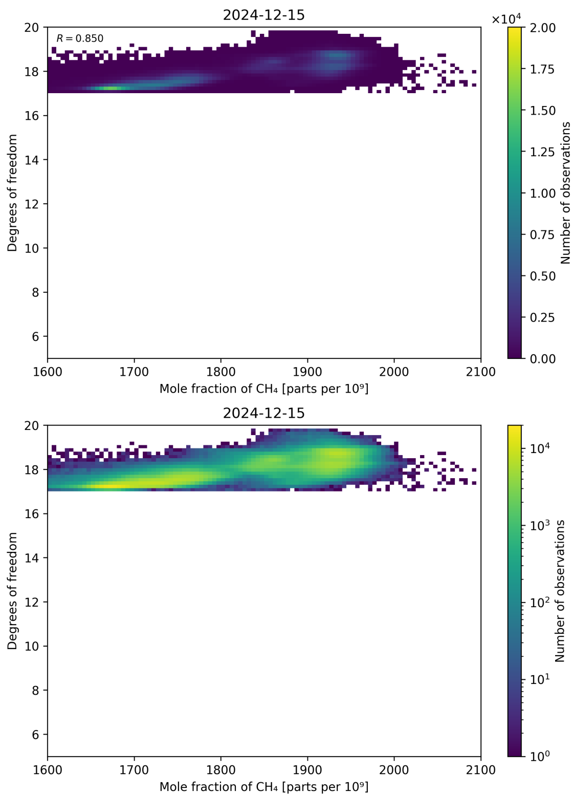
Figure 72: Scatter density plot of “Mole fraction of CH 4 ” against “Degrees of freedom” for 2024-12-14 to 2024-12-16.
