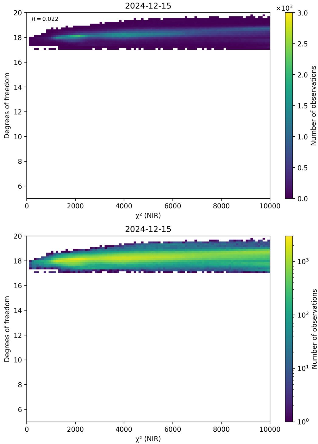
Figure 44: Scatter density plot of “ \chi^2 (NIR)” against “Degrees of freedom” for 2024-12-14 to 2024-12-16.
