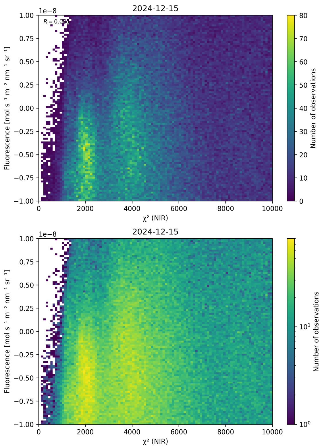
Figure 45: Scatter density plot of “ \chi^2 (NIR)” against “Fluorescence” for 2024-12-14 to 2024-12-16.
