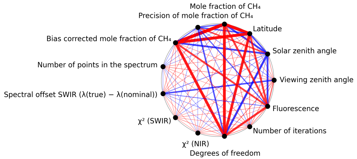
Figure 1: Map of correlation graph for 2024-12-14 to 2024-12-16.
