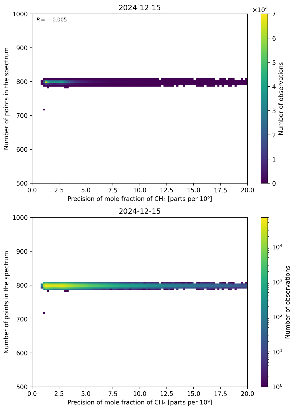
Figure 84: Scatter density plot of “Precision of mole fraction of CH 4 ” against “Number of points in the spectrum” for 2024-12-14 to 2024-12-16.
