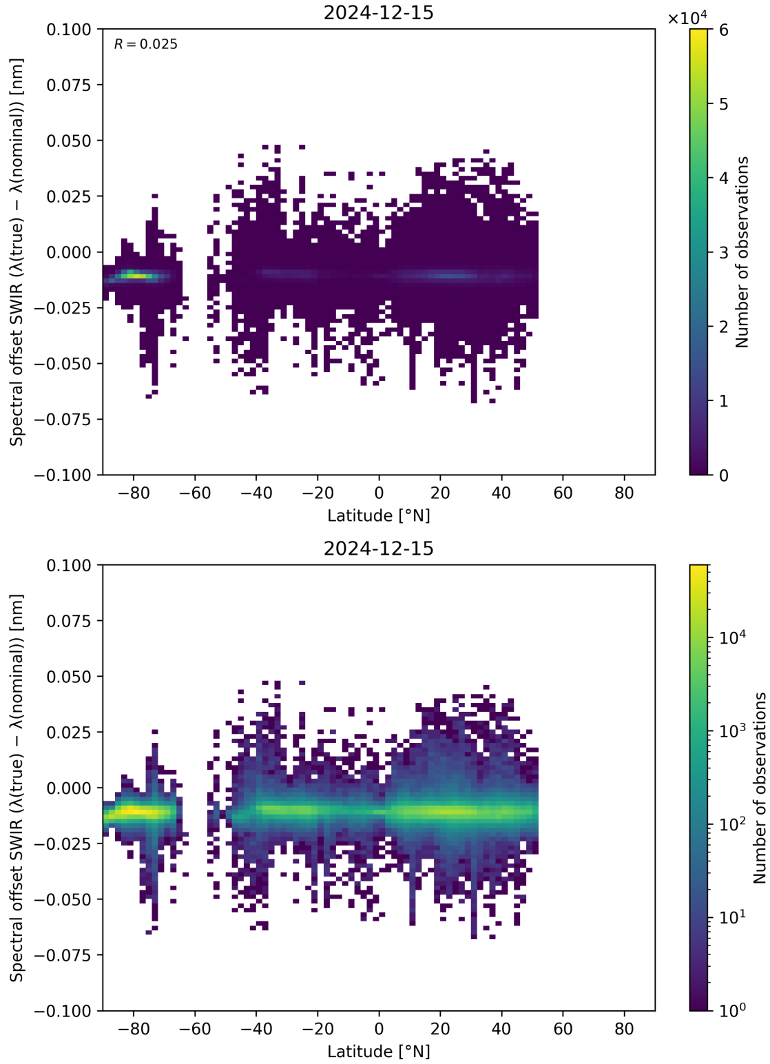
Figure 62: Scatter density plot of “Latitude” against “Spectral offset SWIR ( \lambda_{\text{true}} - \lambda_{\text{nominal}} )” for 2024-12-14 to 2024-12-16.
