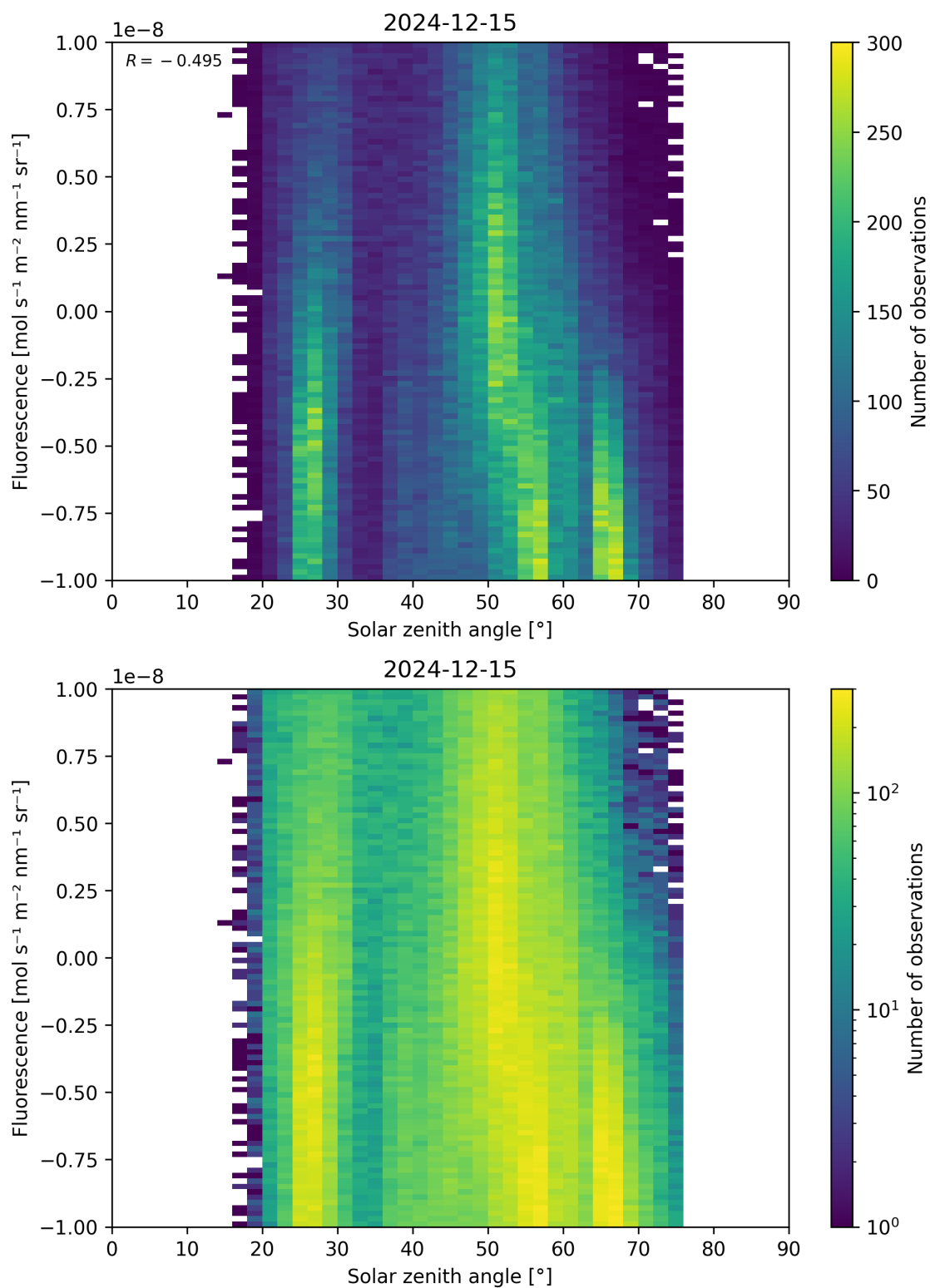
Figure 97: Scatter density plot of “Solar zenith angle” against “Fluorescence” for 2024-12-14 to 2024-12-16.
