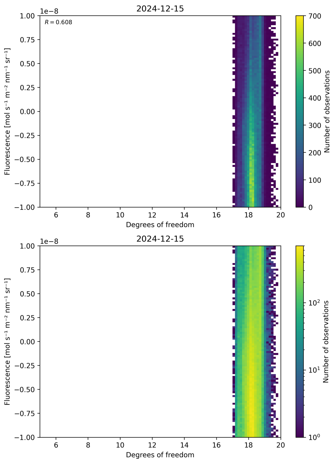
Figure 51: Scatter density plot of “Degrees of freedom” against “Fluorescence” for 2024-12-14 to 2024-12-16.
