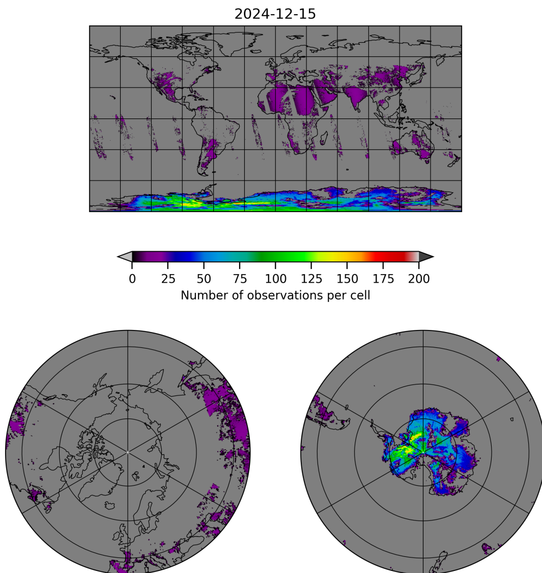
Figure 10: Map of the number of observations for 2024-12-14 to 2024-12-16
