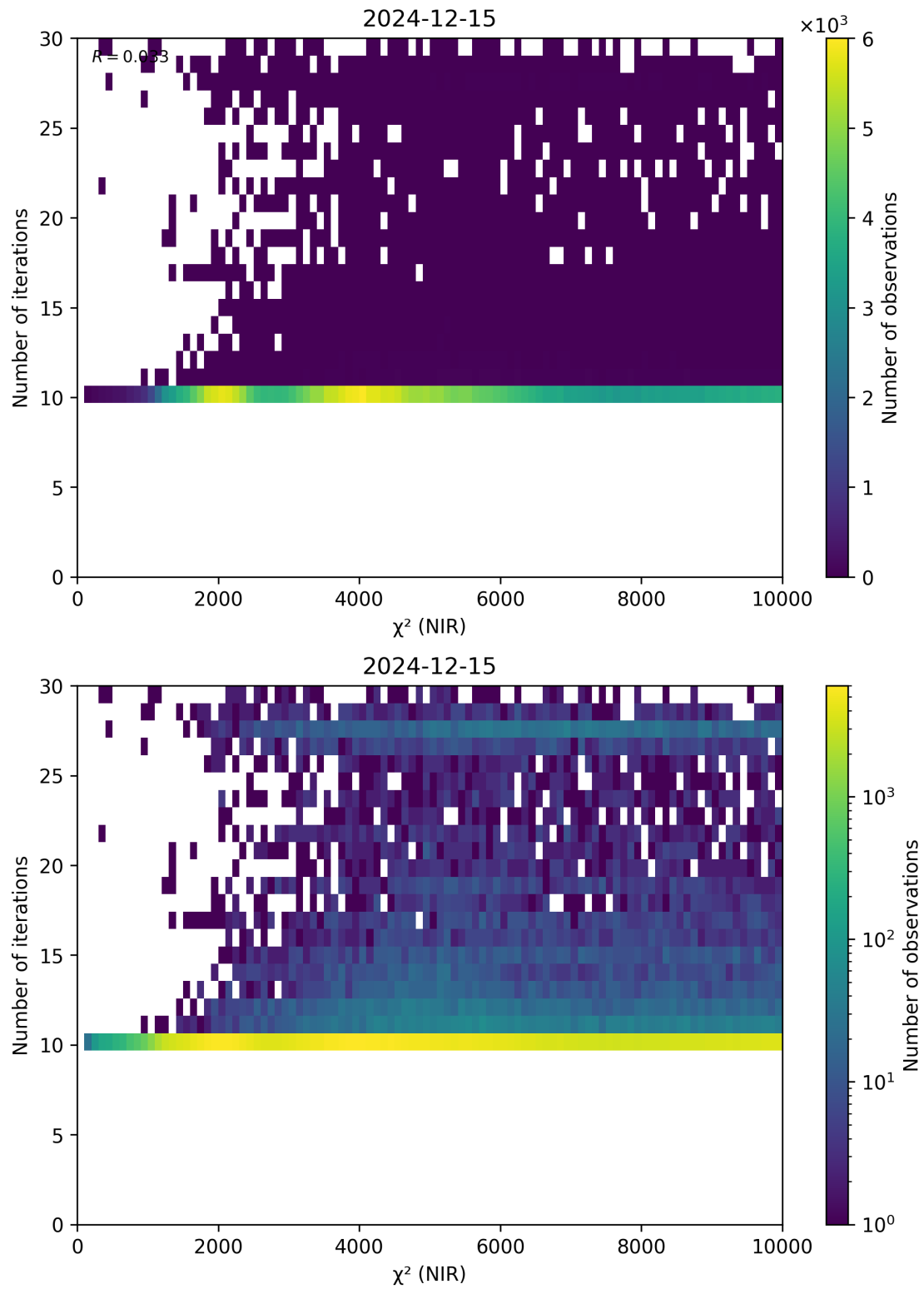
Figure 46: Scatter density plot of “ \chi^2 (NIR)” against “Number of iterations” for 2024-12-14 to 2024-12-16.
