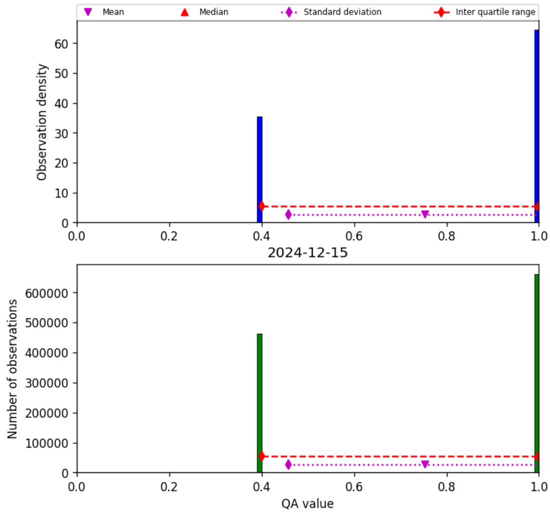
Figure 22: Histogram of “QA value” for 2024-12-14 to 2024-12-16
