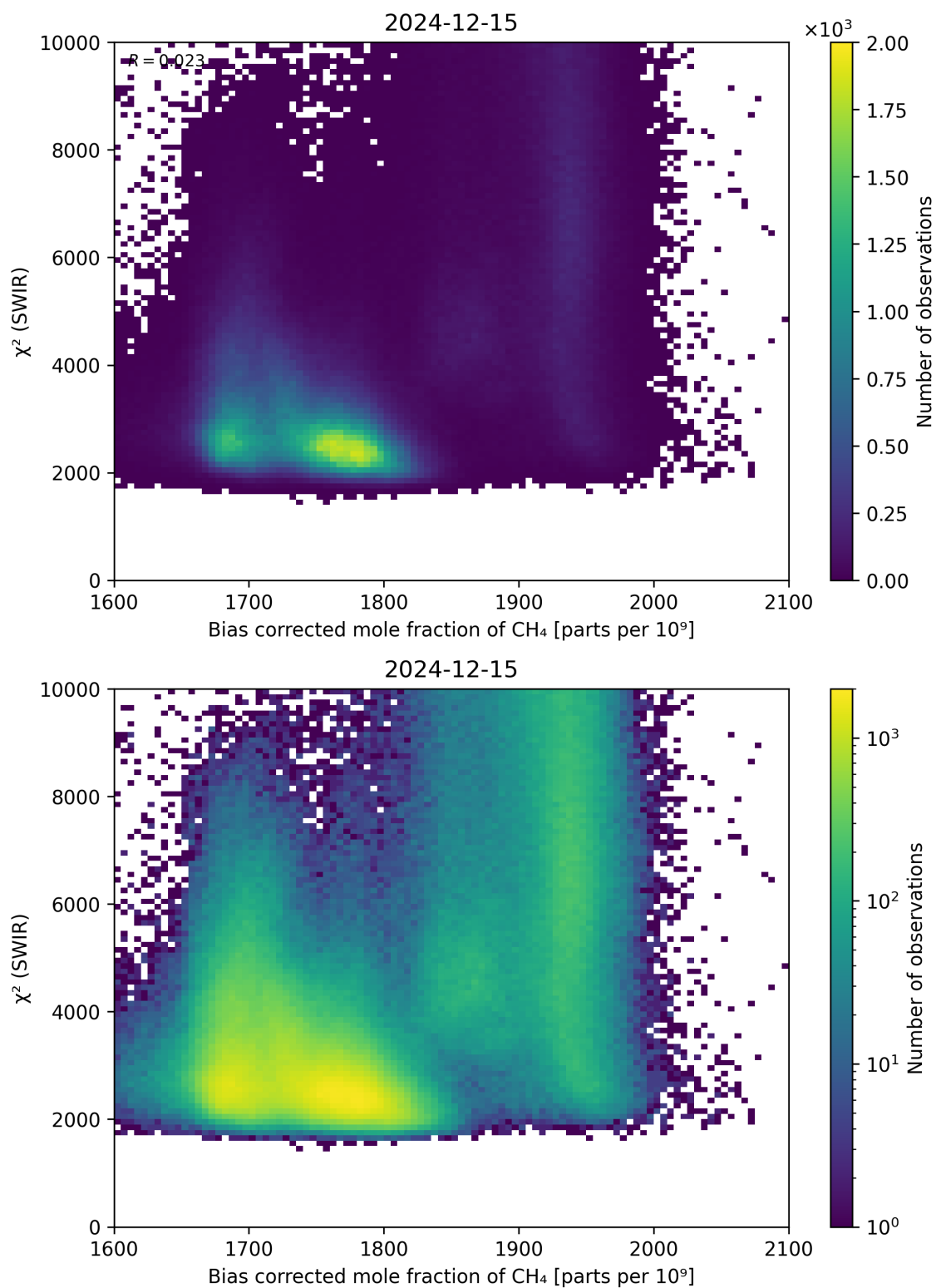
Figure 64: Scatter density plot of “Bias corrected mole fraction of \text{CH}_4 ” against “ \chi^2 (SWIR)” for 2024-12-14 to 2024-12-16.
