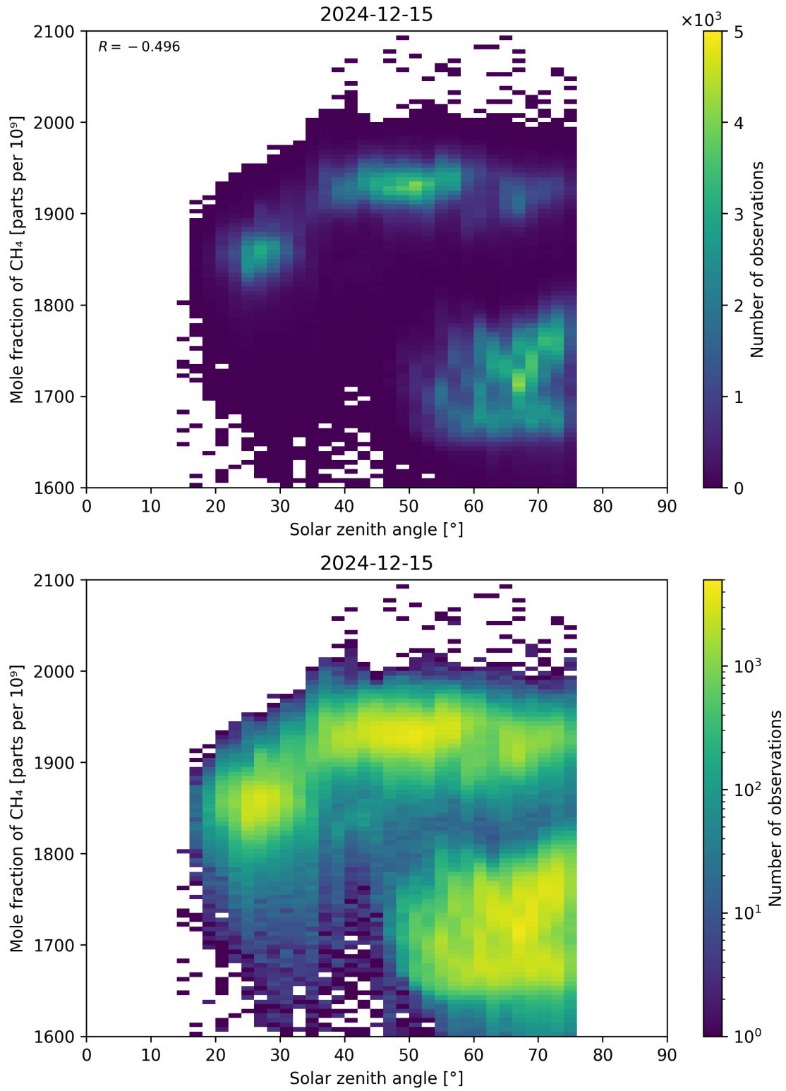
Figure 99: Scatter density plot of “Solar zenith angle” against “Mole fraction of CH 4 ” for 2024-12-14 to 2024-12-16.
