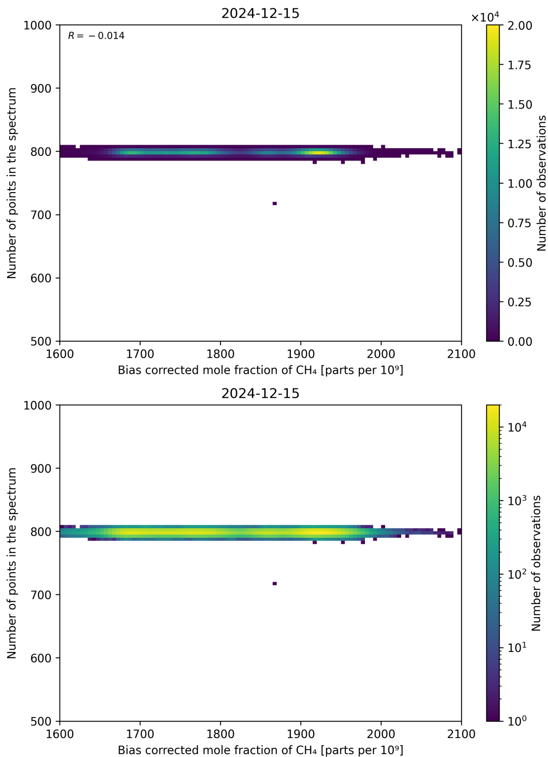
Figure 68: Scatter density plot of “Bias corrected mole fraction of CH 4 ” against “Number of points in the spectrum” for 2024-12-14 to 2024-12-16.
