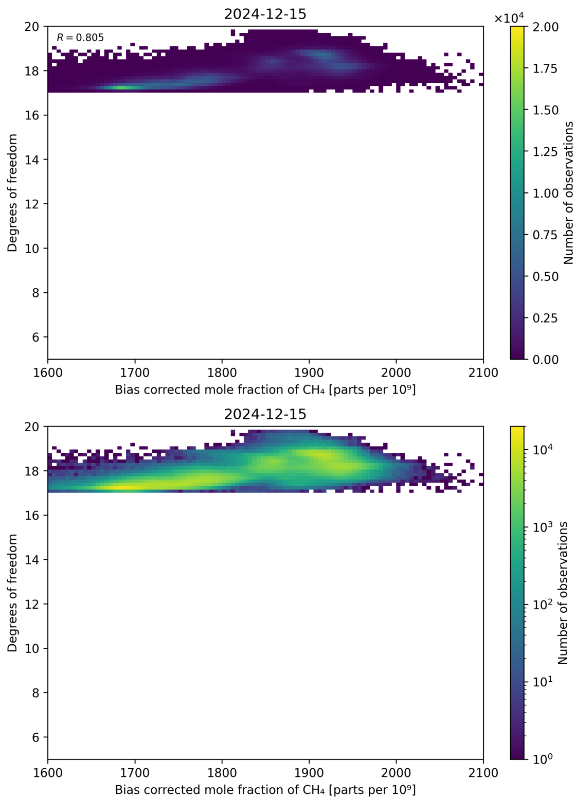
Figure 65: Scatter density plot of “Bias corrected mole fraction of CH 4 ” against “Degrees of freedom” for 2024-12-14 to 2024-12-16.
