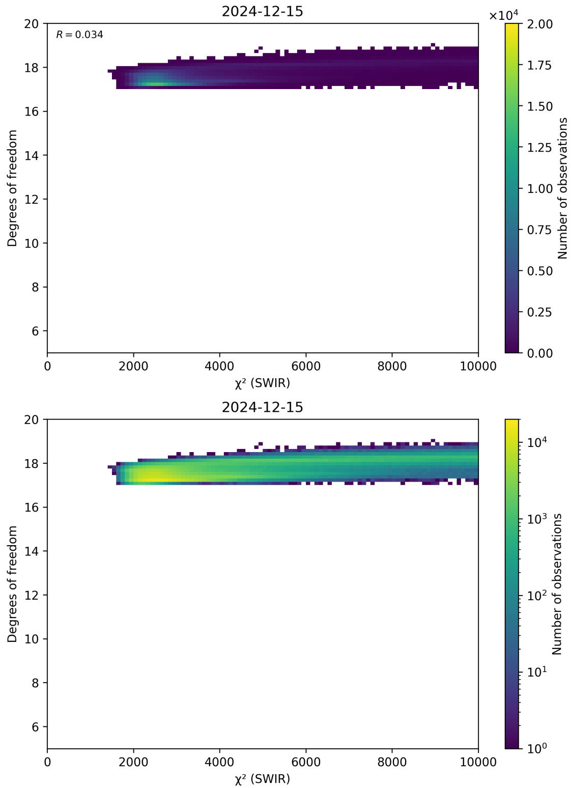
Figure 48: Scatter density plot of “ \chi^2 (SWIR)” against “Degrees of freedom” for 2024-12-14 to 2024-12-16.
