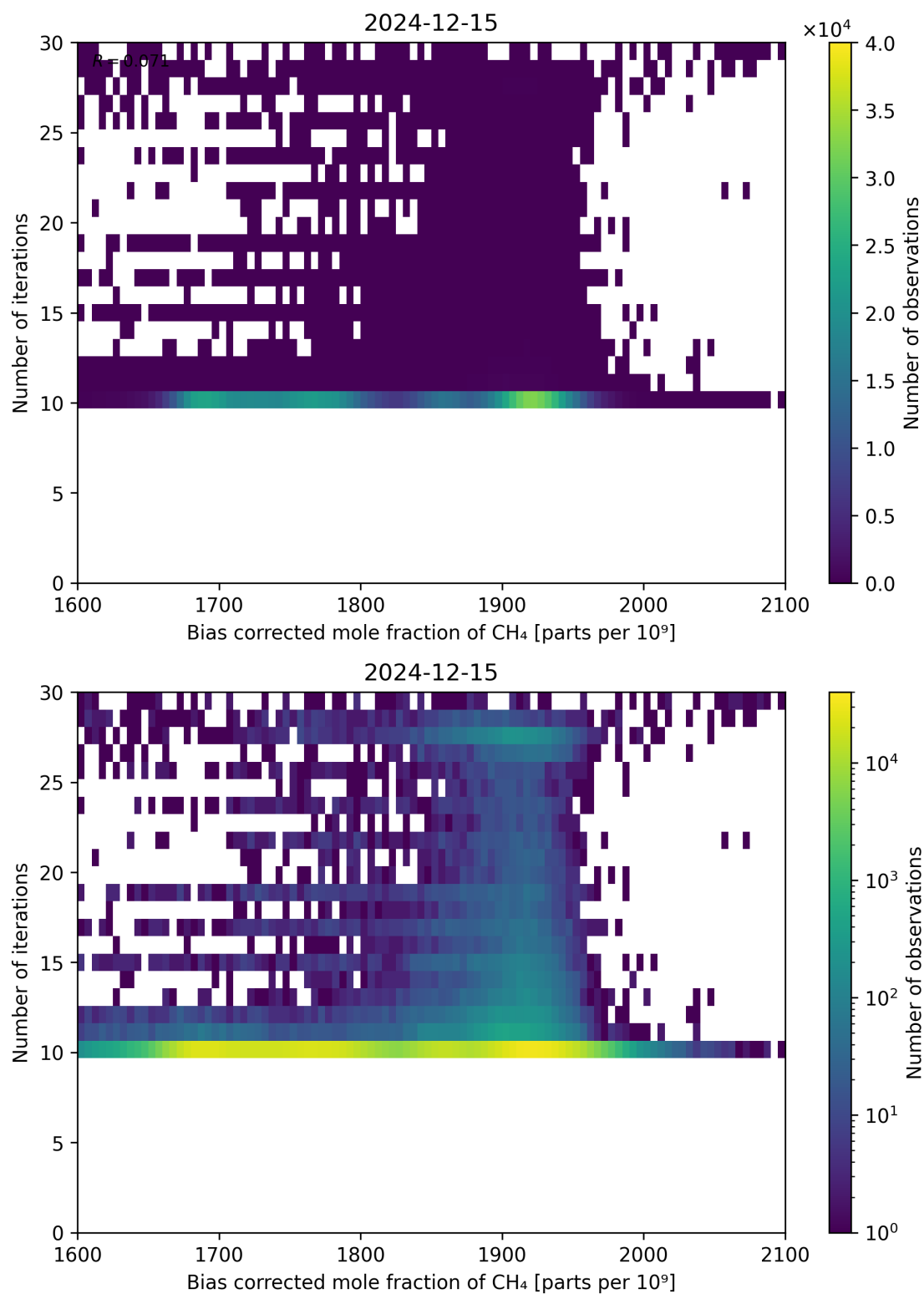
Figure 67: Scatter density plot of “Bias corrected mole fraction of CH 4 ” against “Number of iterations” for 2024-12-14 to 2024-12-16.
