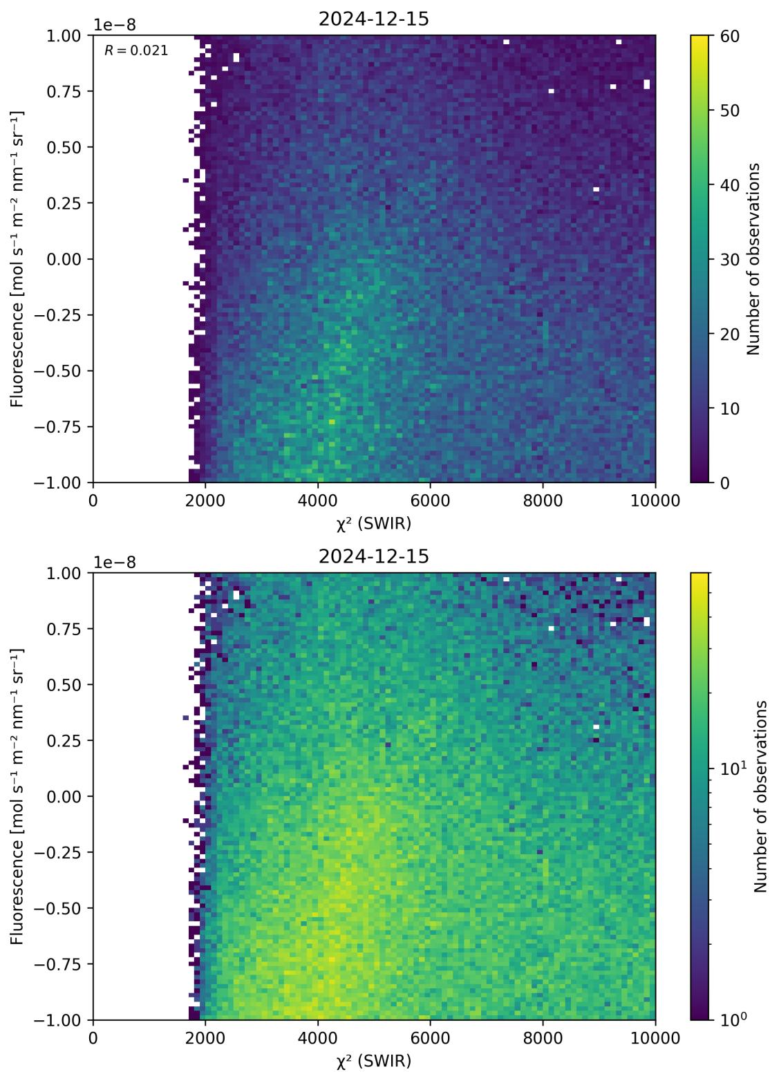
Figure 49: Scatter density plot of “ \chi^2 (SWIR)” against “Fluorescence” for 2024-12-14 to 2024-12-16.
