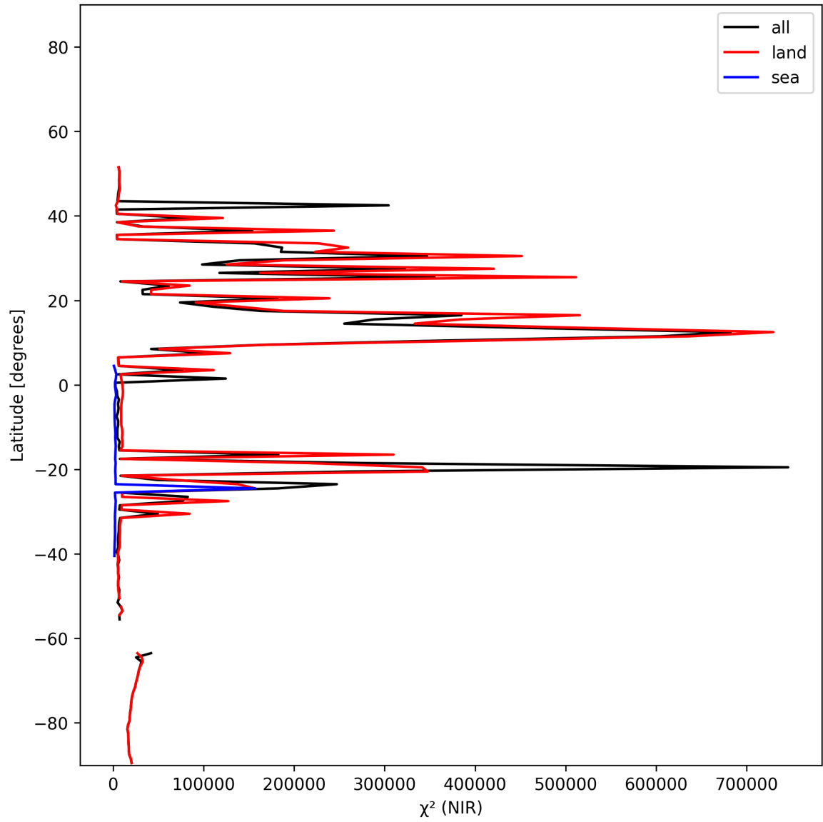
Figure 18: Zonal average of “ \chi^2 (NIR)” for 2024-12-14 to 2024-12-16.
