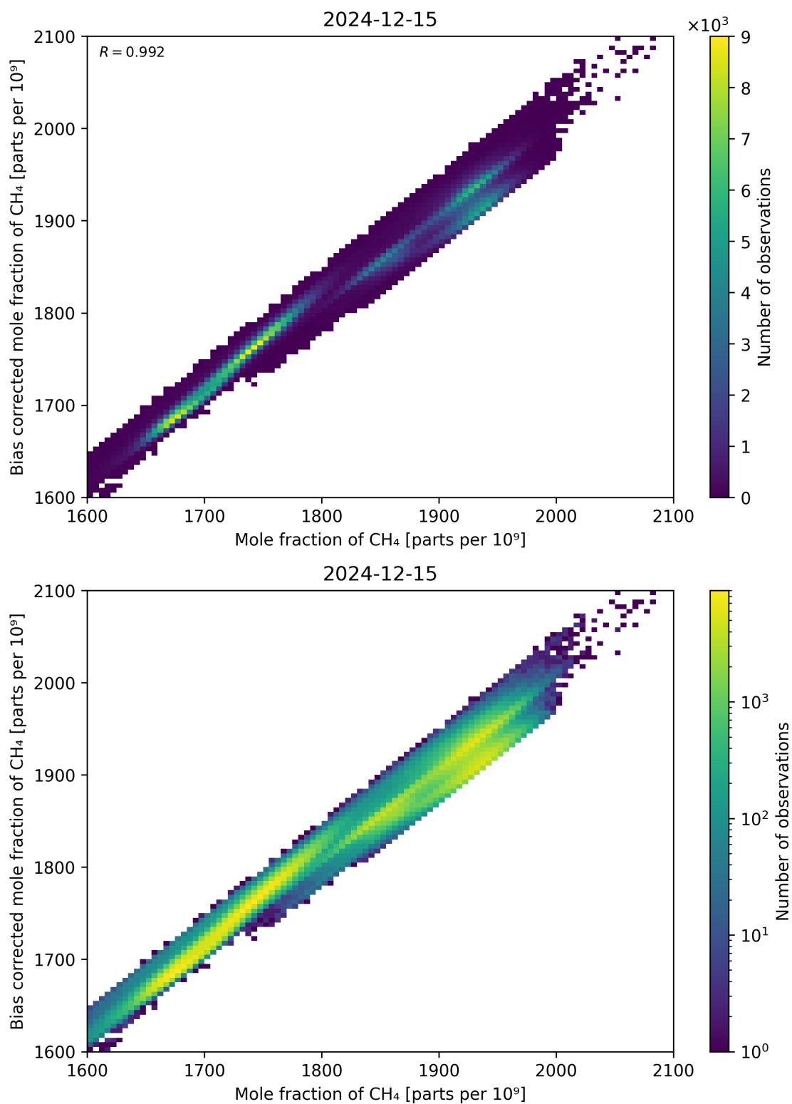
Figure 74: Scatter density plot of “Mole fraction of CH 4 ” against “Bias corrected mole fraction of CH 4 ” for 2024-12-14 to 2024-12-16.
