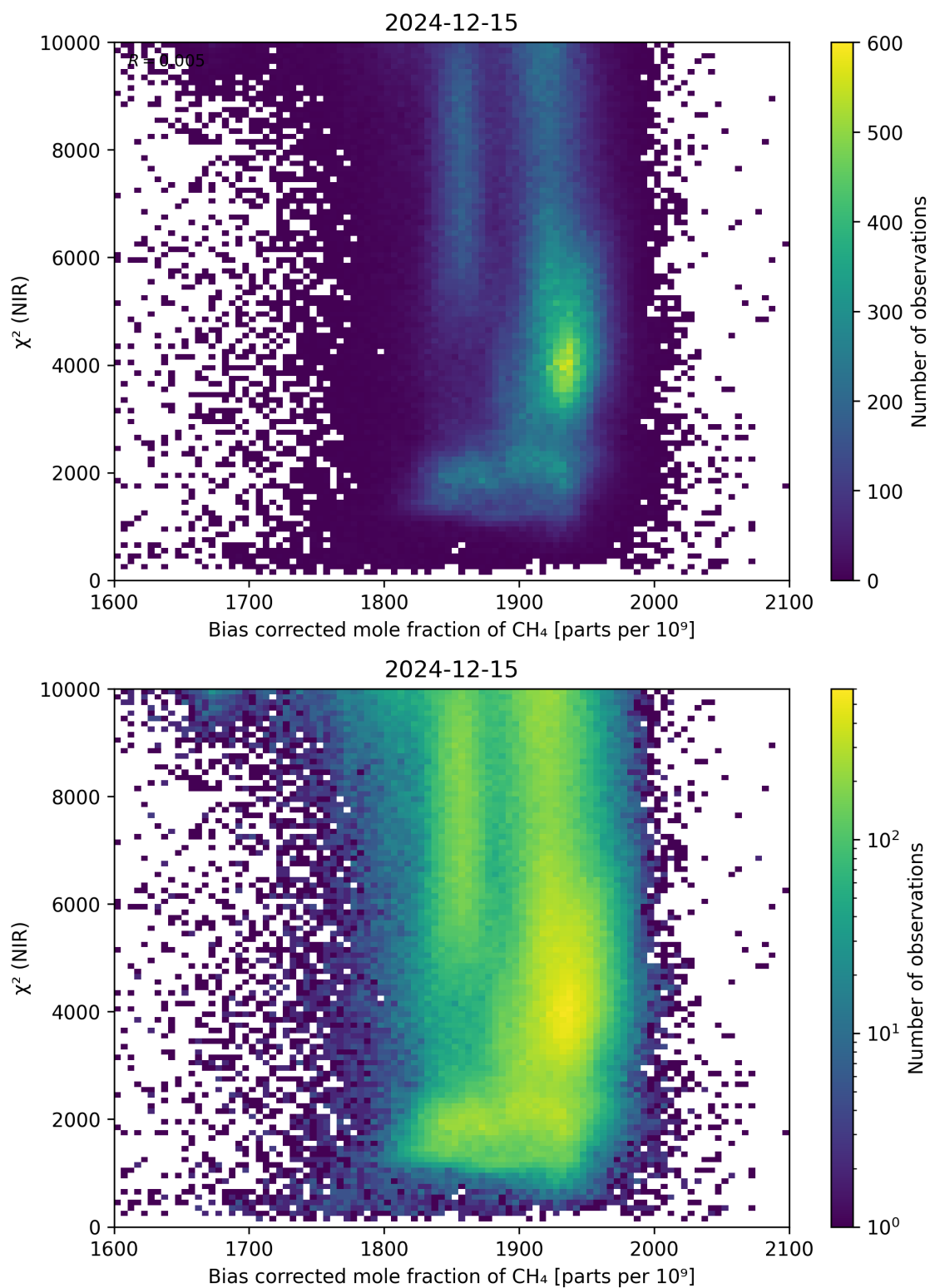
Figure 63: Scatter density plot of “Bias corrected mole fraction of \text{CH}_4 ” against “ \chi^2 (NIR)” for 2024-12-14 to 2024-12-16.
