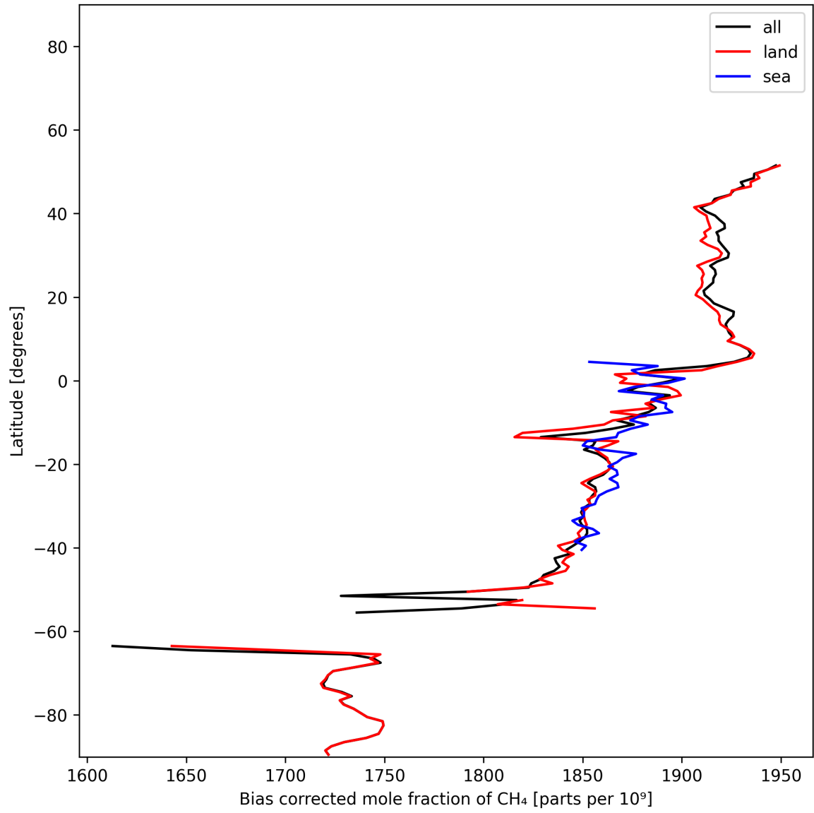
Figure 14: Zonal average of “Bias corrected mole fraction of \text{CH}_4 ” for 2024-12-14 to 2024-12-16.
