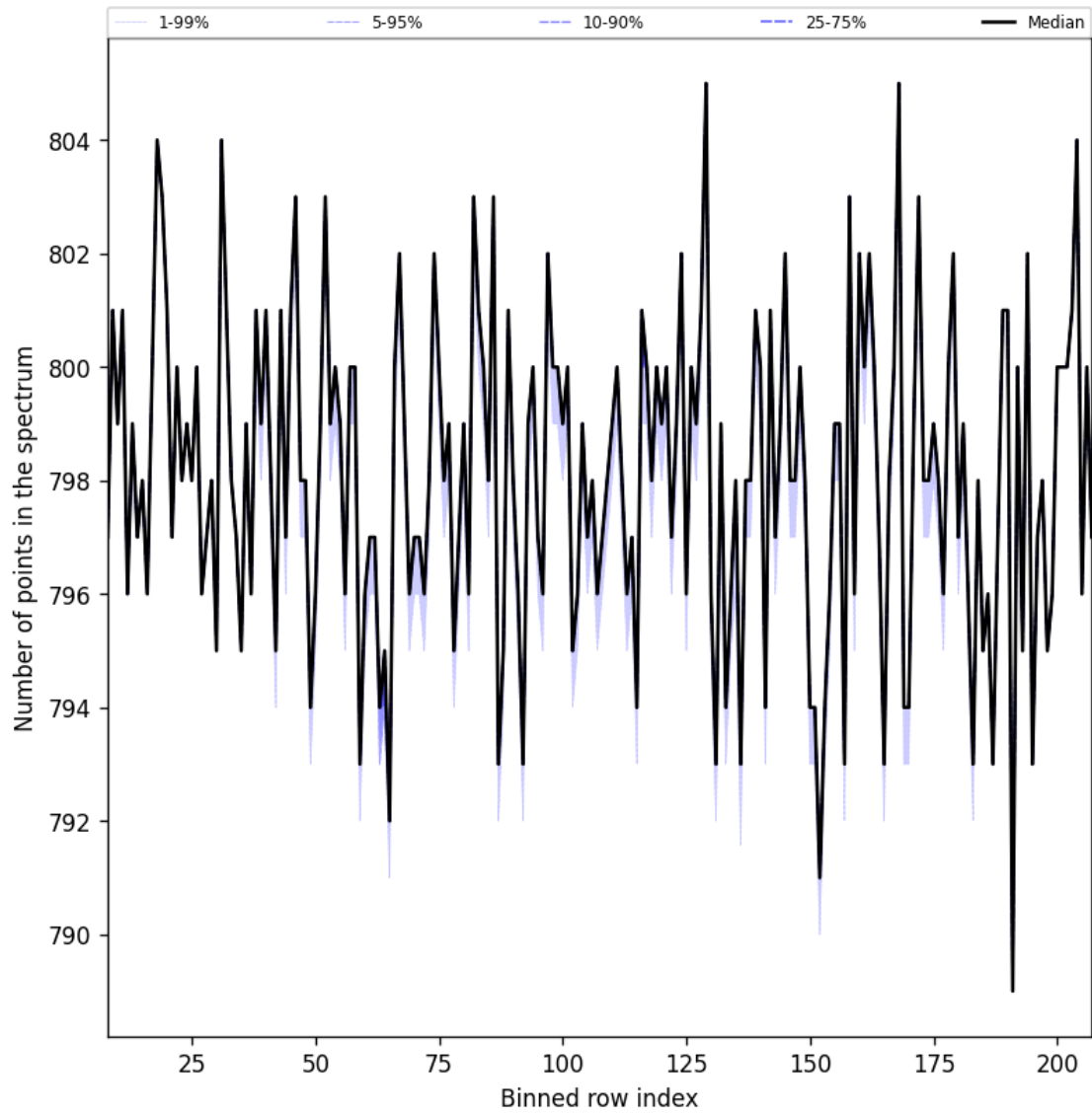
Figure 37: Along track statistics of “Number of points in the spectrum” for 2024-12-14 to 2024-12-16
