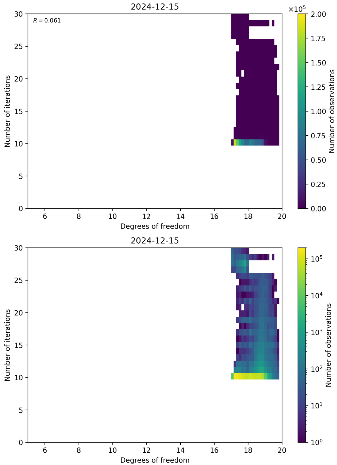
Figure 52: Scatter density plot of “Degrees of freedom” against “Number of iterations” for 2024-12-14 to 2024-12-16.
