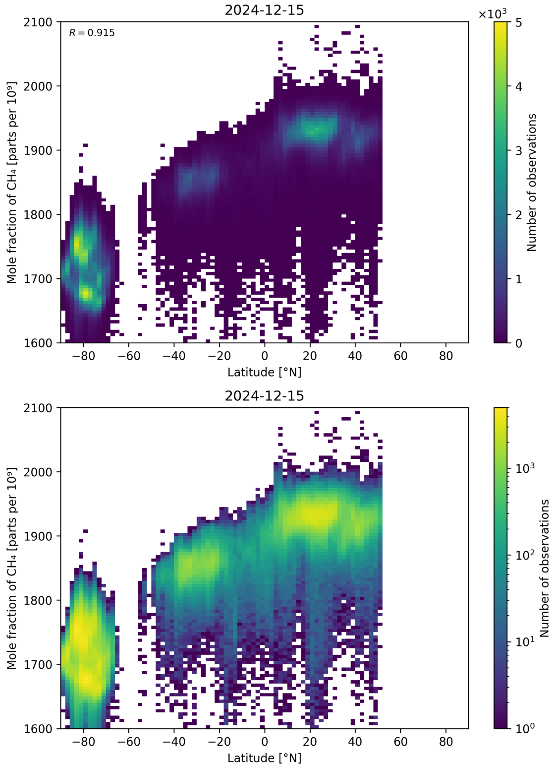
Figure 57: Scatter density plot of “Latitude” against “Mole fraction of CH 4 ” for 2024-12-14 to 2024-12-16.
