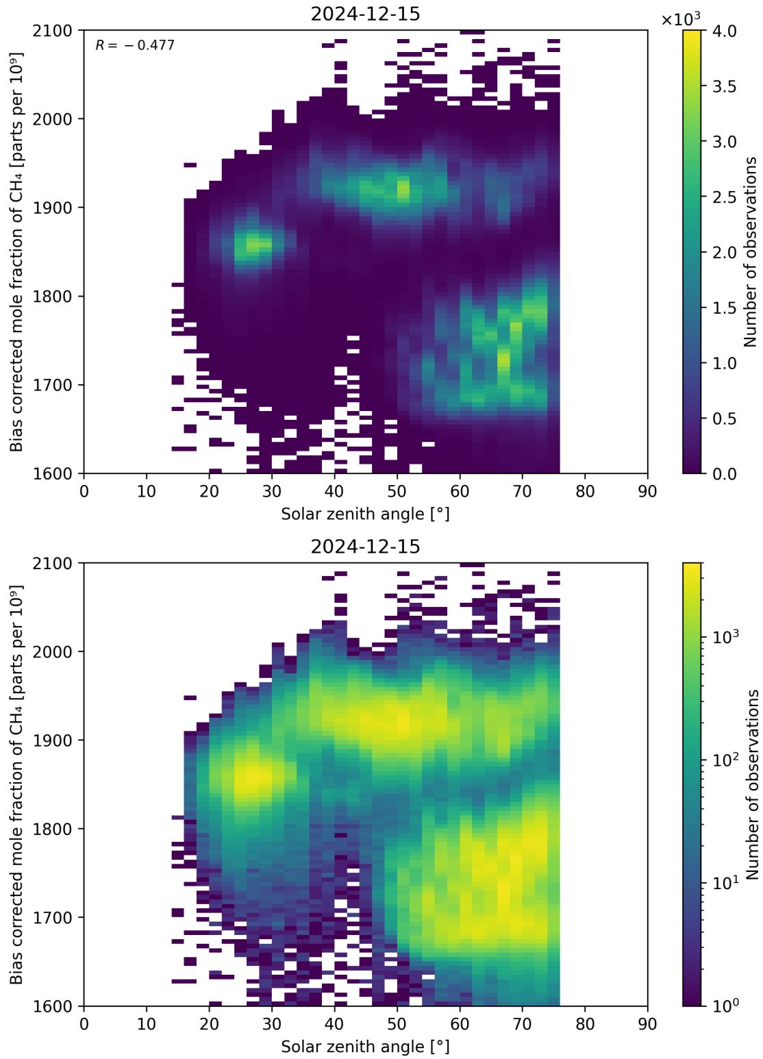
Figure 100: Scatter density plot of “Solar zenith angle” against “Bias corrected mole fraction of \text{CH}_4 ” for 2024-12-14 to 2024-12-16.
