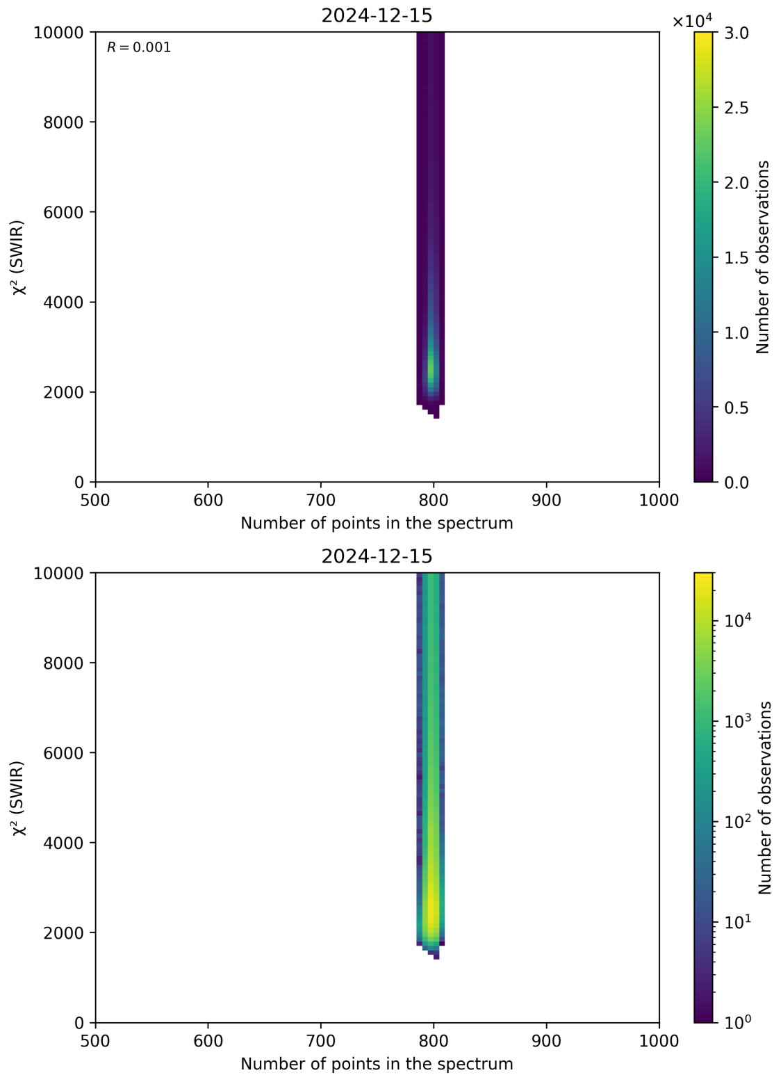
Figure 89: Scatter density plot of “Number of points in the spectrum” against “ \chi^2 (SWIR)” for 2024-12-14 to 2024-12-16.
