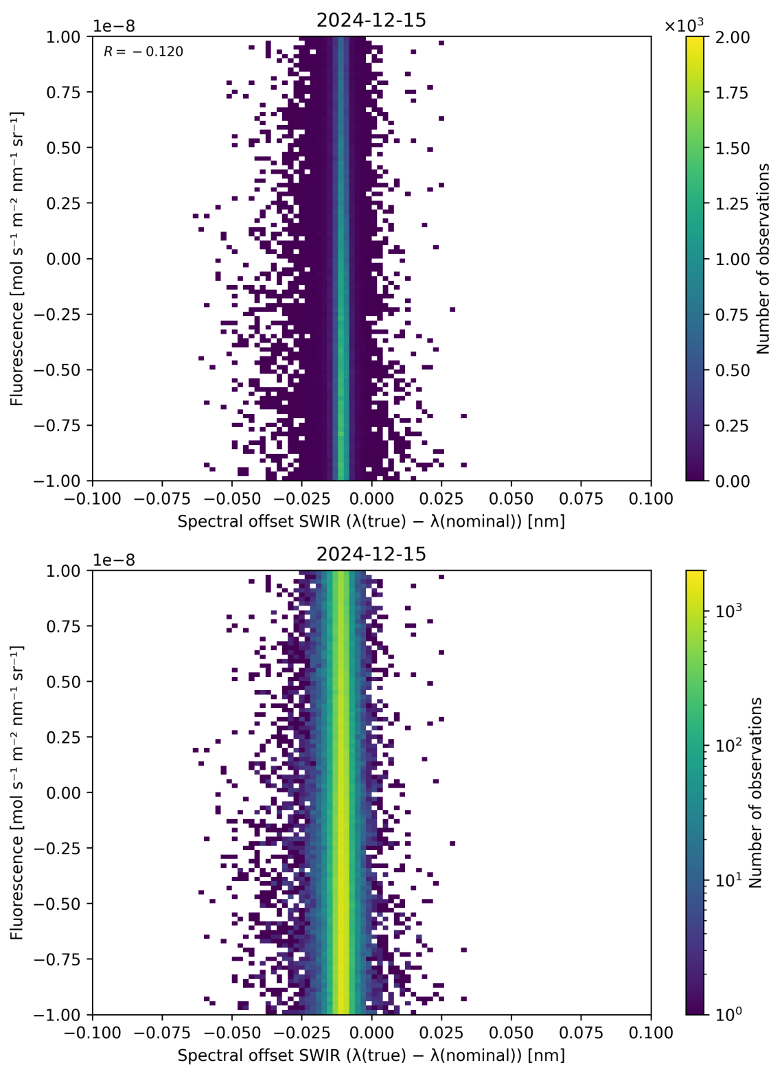
Figure 120: Scatter density plot of “Spectral offset SWIR ( \lambda_{\text{true}} - \lambda_{\text{nominal}} )” against “Fluorescence” for 2024-12-14 to 2024-12-16.
