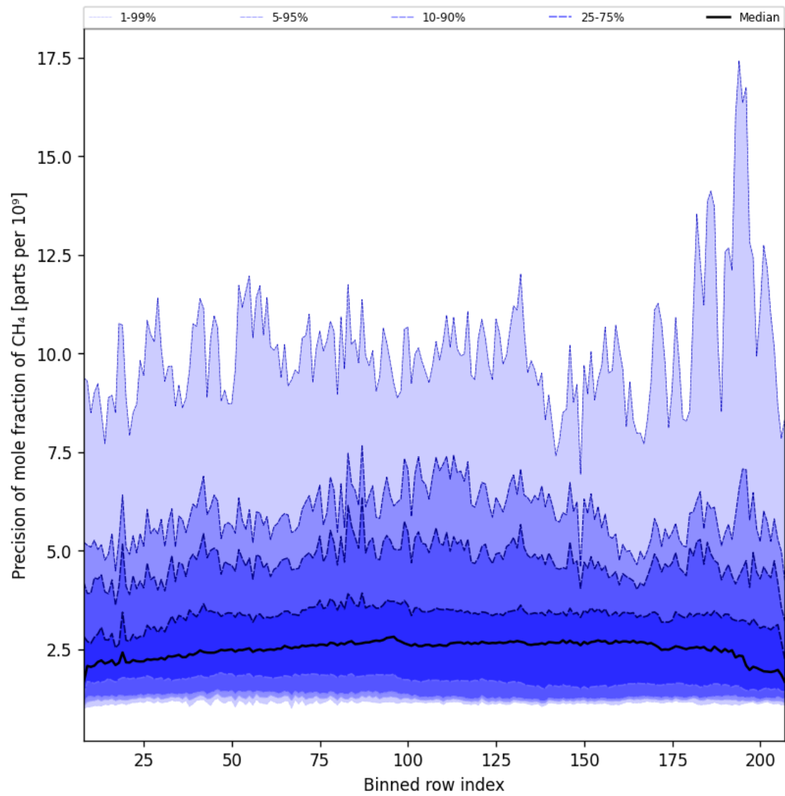
Figure 35: Along track statistics of “Precision of mole fraction of CH 4 ” for 2024-12-14 to 2024-12-16
