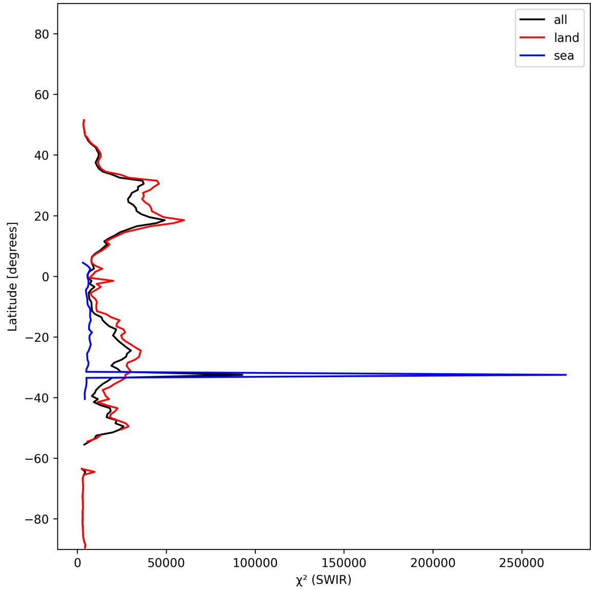
Figure 17: Zonal average of “ \chi^2 (SWIR)” for 2024-12-14 to 2024-12-16.
