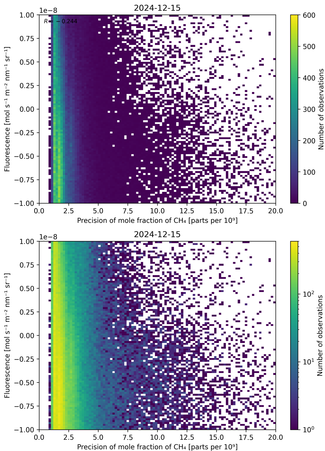
Figure 81: Scatter density plot of “Precision of mole fraction of \text{CH}_4 ” against “Fluorescence” for 2024-12-14 to 2024-12-16.
