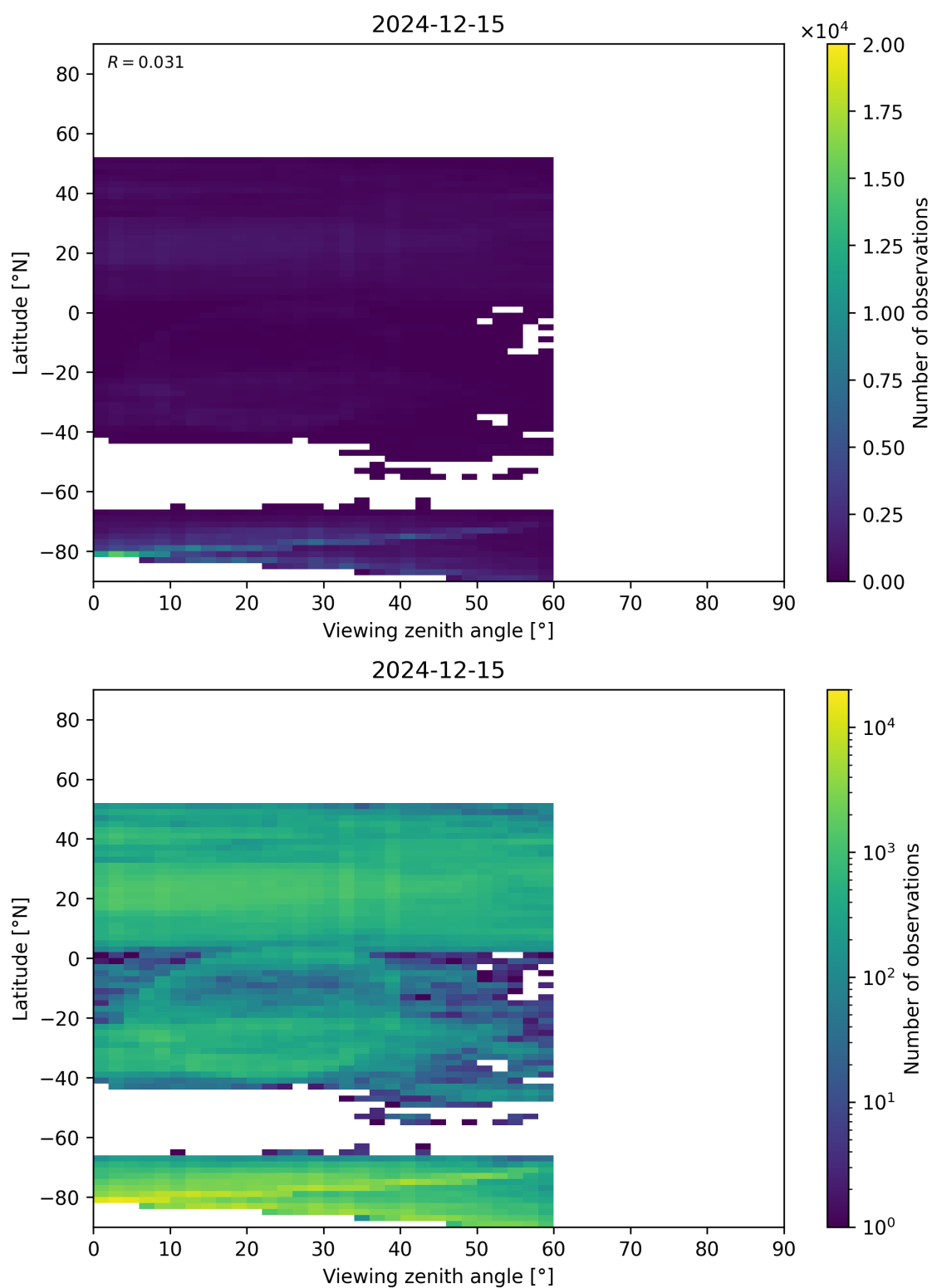
Figure 109: Scatter density plot of “Viewing zenith angle” against “Latitude” for 2024-12-14 to 2024-12-16.
