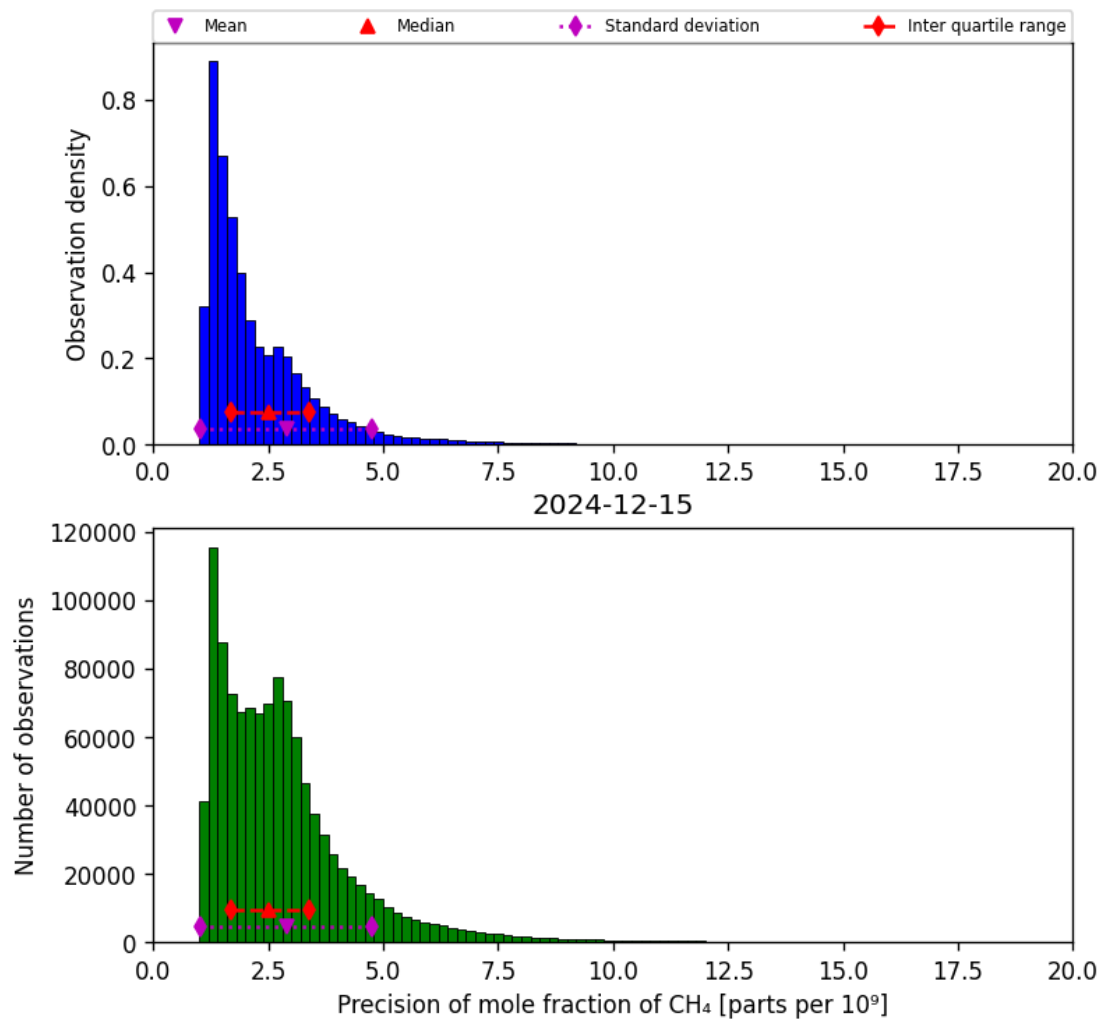
Figure 24: Histogram of “Precision of mole fraction of CH 4 ” for 2024-12-14 to 2024-12-16
