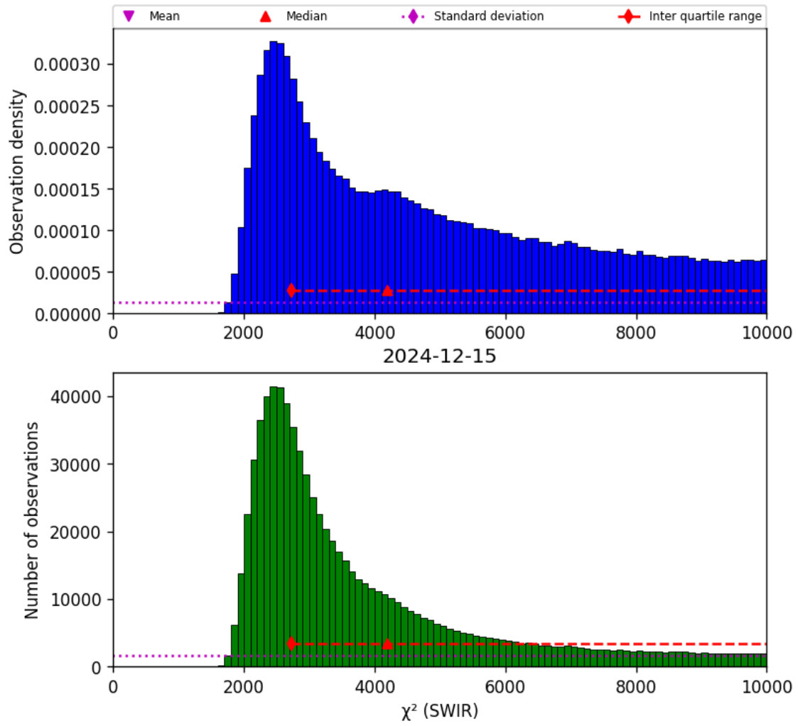
Figure 28: Histogram of “ \chi^2 (SWIR)” for 2024-12-14 to 2024-12-16
