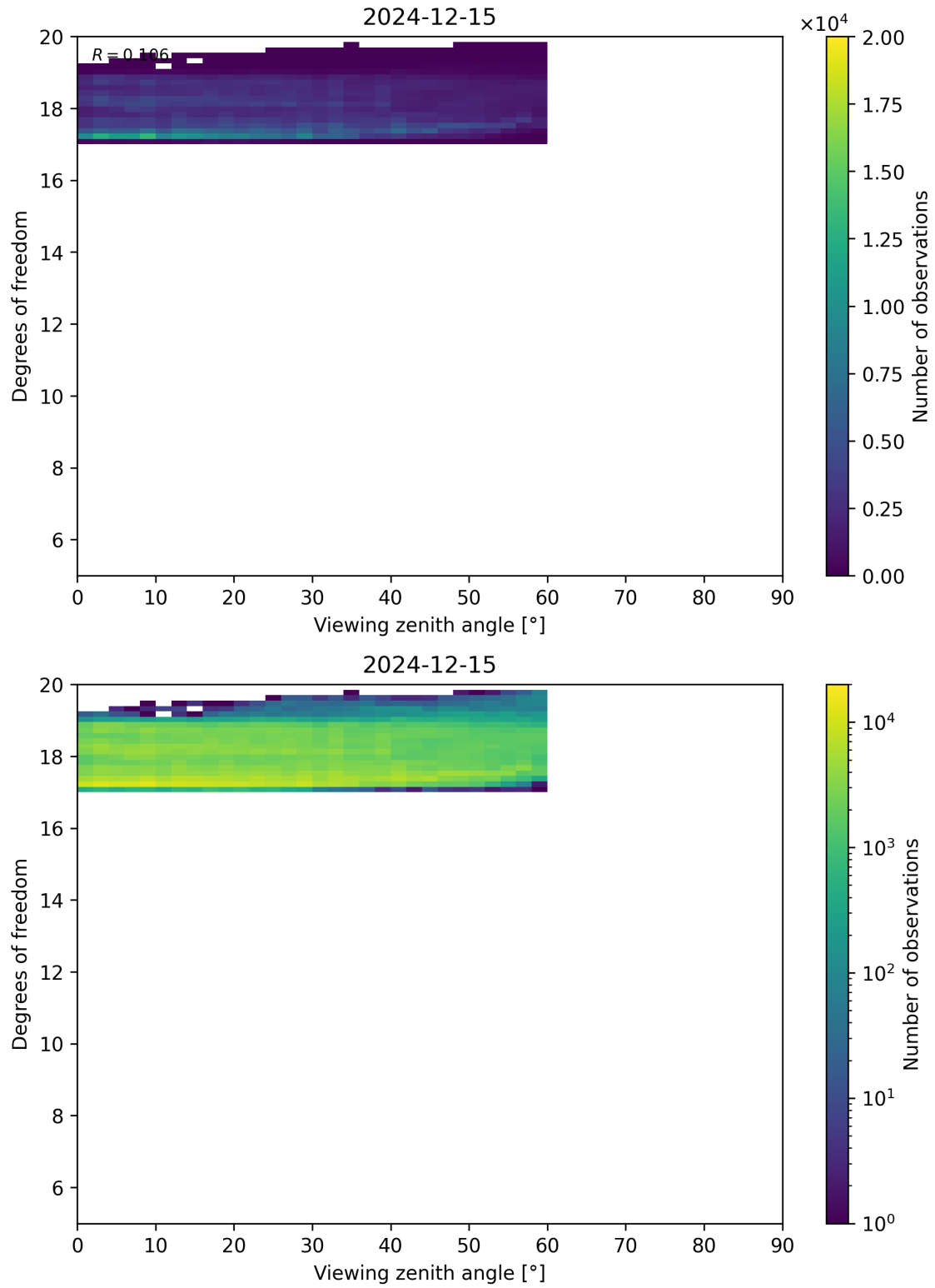
Figure 107: Scatter density plot of “Viewing zenith angle” against “Degrees of freedom” for 2024-12-14 to 2024-12-16.
