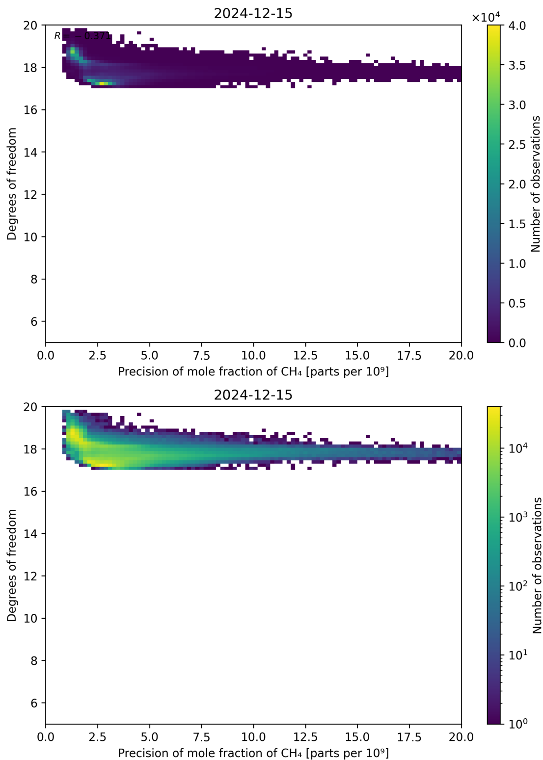
Figure 80: Scatter density plot of “Precision of mole fraction of CH 4 ” against “Degrees of freedom” for 2024-12-14 to 2024-12-16.
