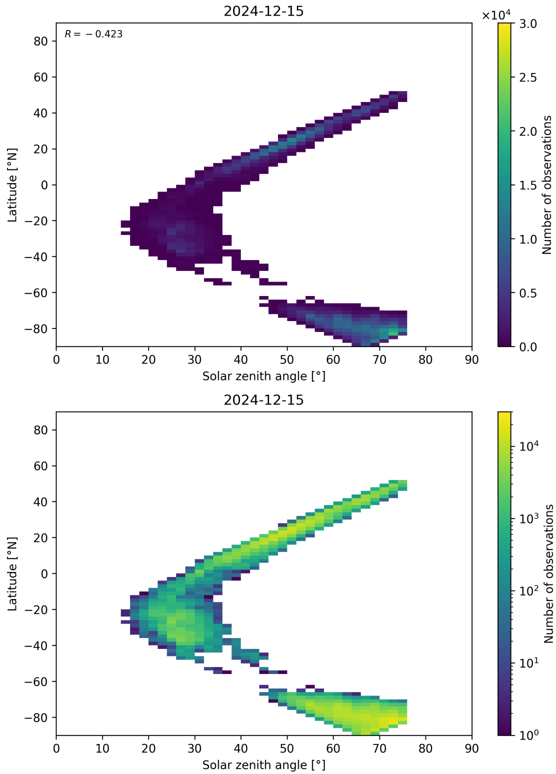
Figure 98: Scatter density plot of “Solar zenith angle” against “Latitude” for 2024-12-14 to 2024-12-16.
