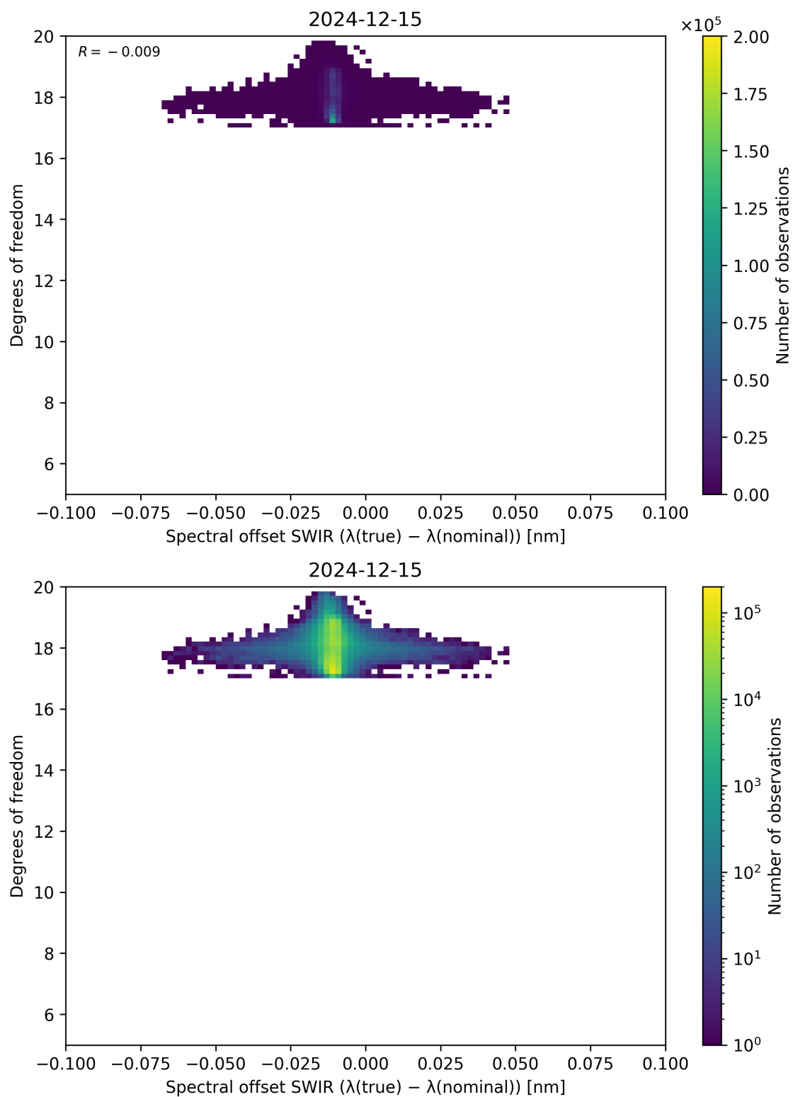
Figure 119: Scatter density plot of “Spectral offset SWIR ( \lambda_{\text{true}} - \lambda_{\text{nominal}} )” against “Degrees of freedom” for 2024-12-14 to 2024-12-16.
