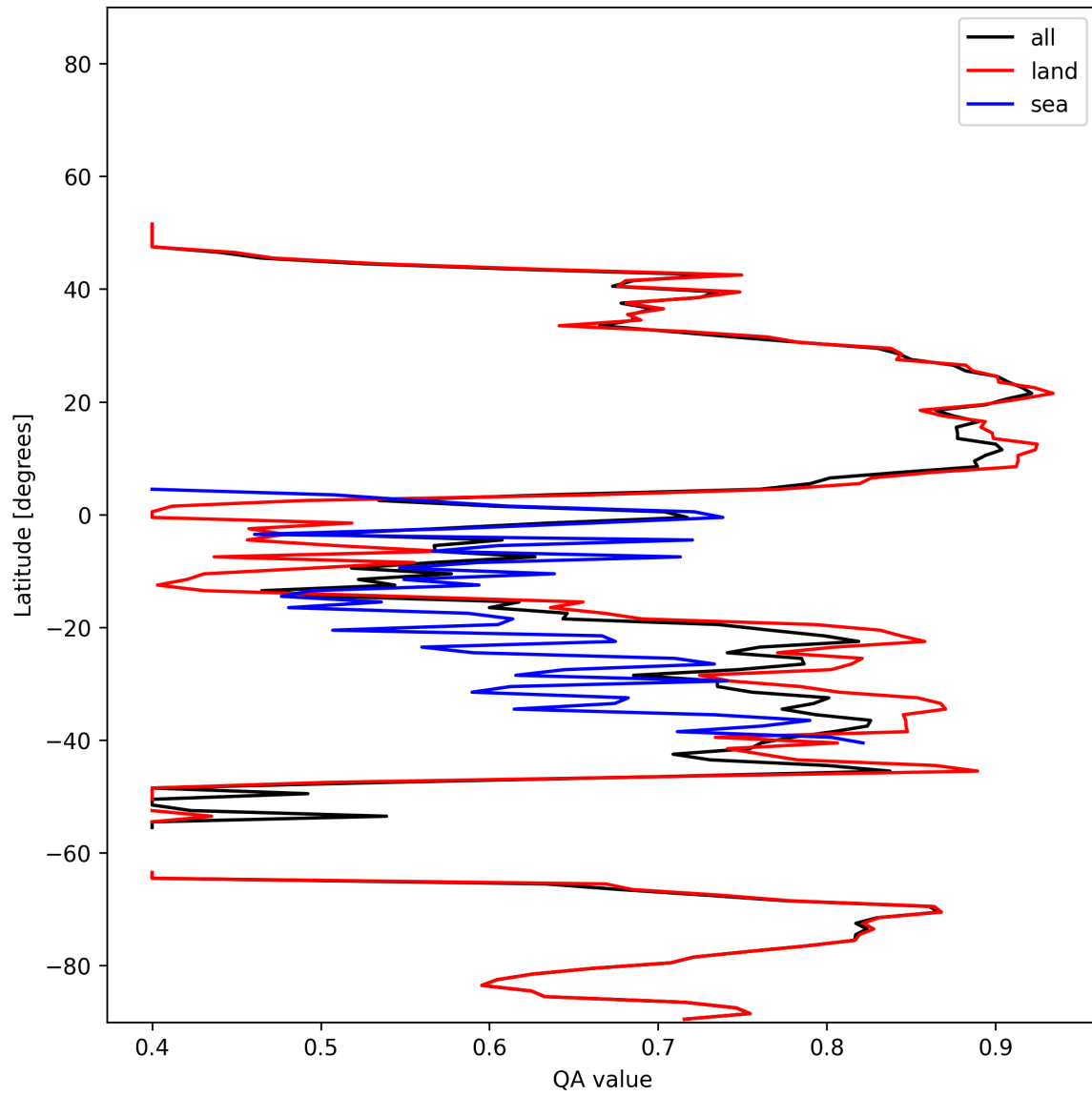
Figure 11: Zonal average of “QA value” for 2024-12-14 to 2024-12-16.
