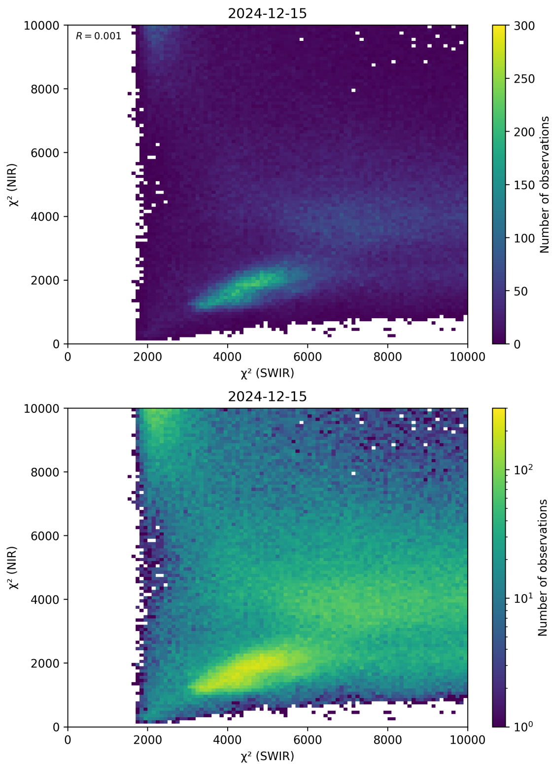
Figure 47: Scatter density plot of “ \chi^2 (SWIR)” against “ \chi^2 (NIR)” for 2024-12-14 to 2024-12-16.
