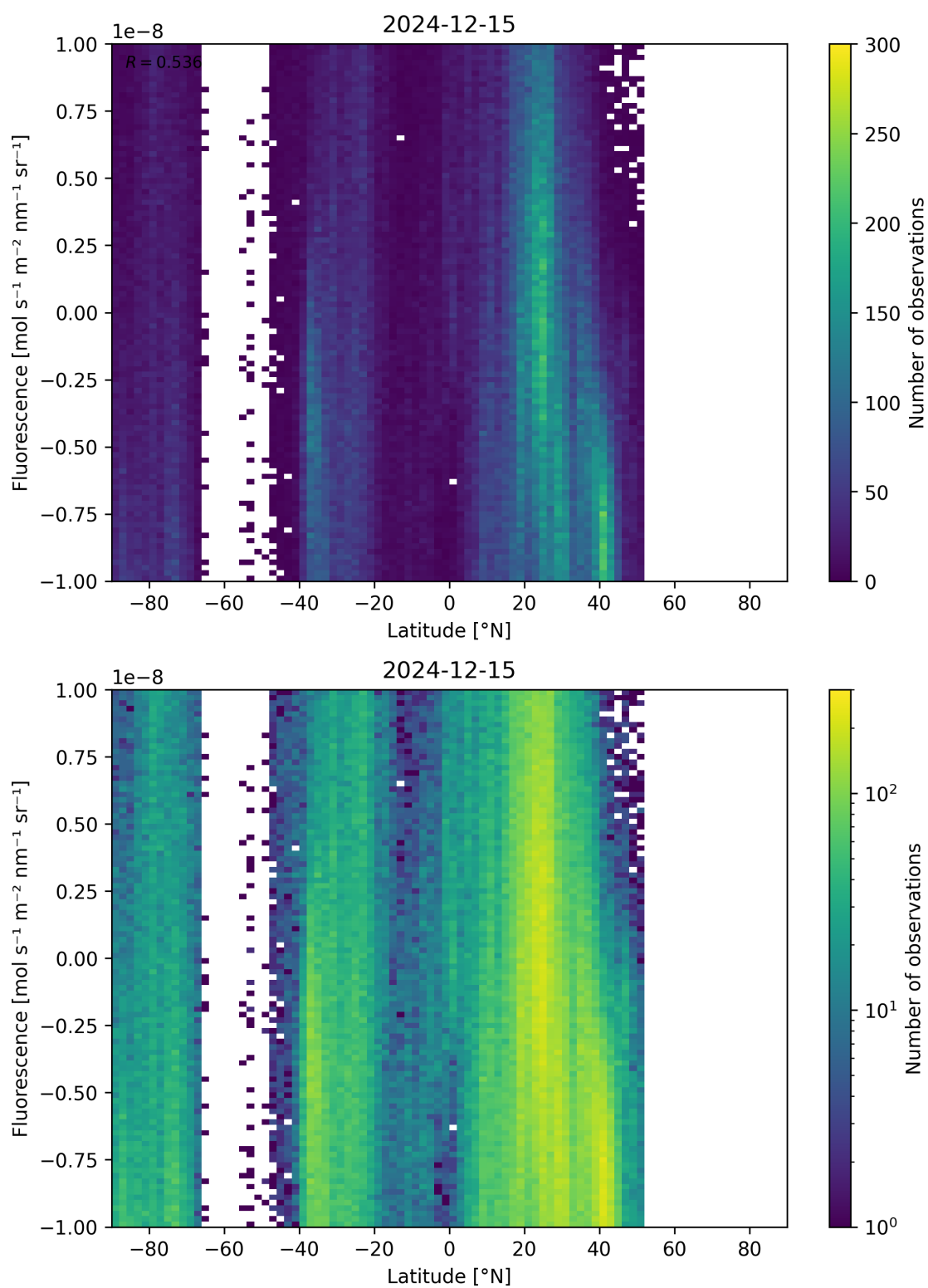
Figure 56: Scatter density plot of “Latitude” against “Fluorescence” for 2024-12-14 to 2024-12-16.
