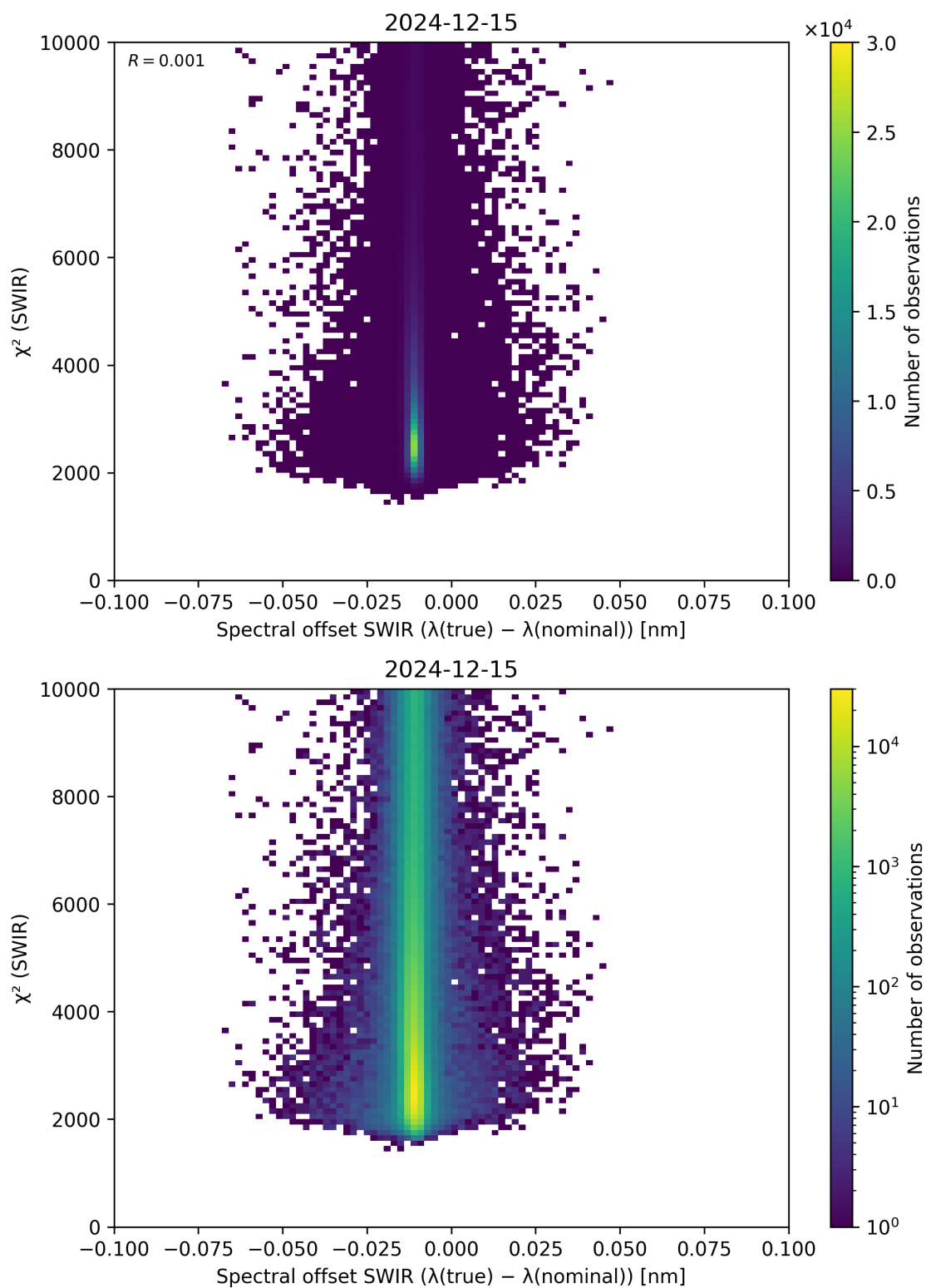
Figure 118: Scatter density plot of “Spectral offset SWIR ( \lambda_{\text{true}} - \lambda_{\text{nominal}} )” against “ \chi^2 (SWIR)” for 2024-12-14 to 2024-12-16.
