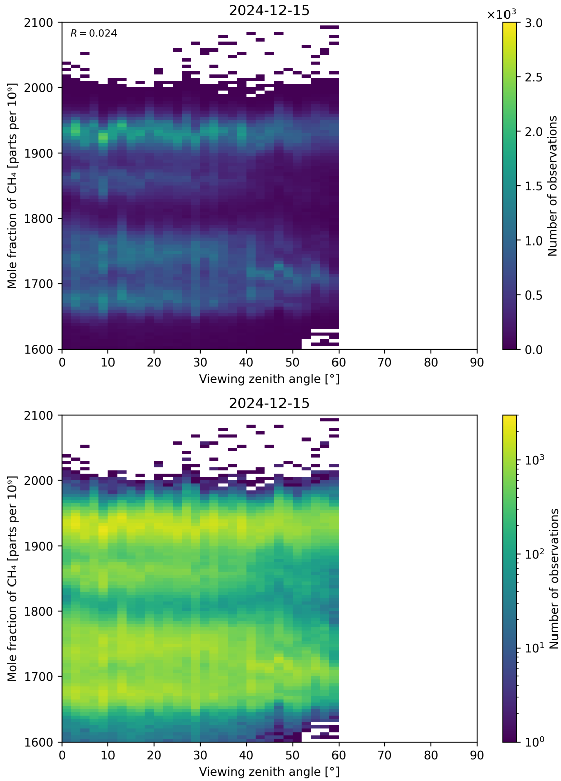
Figure 110: Scatter density plot of “Viewing zenith angle” against “Mole fraction of CH 4 ” for 2024-12-14 to 2024-12-16.
