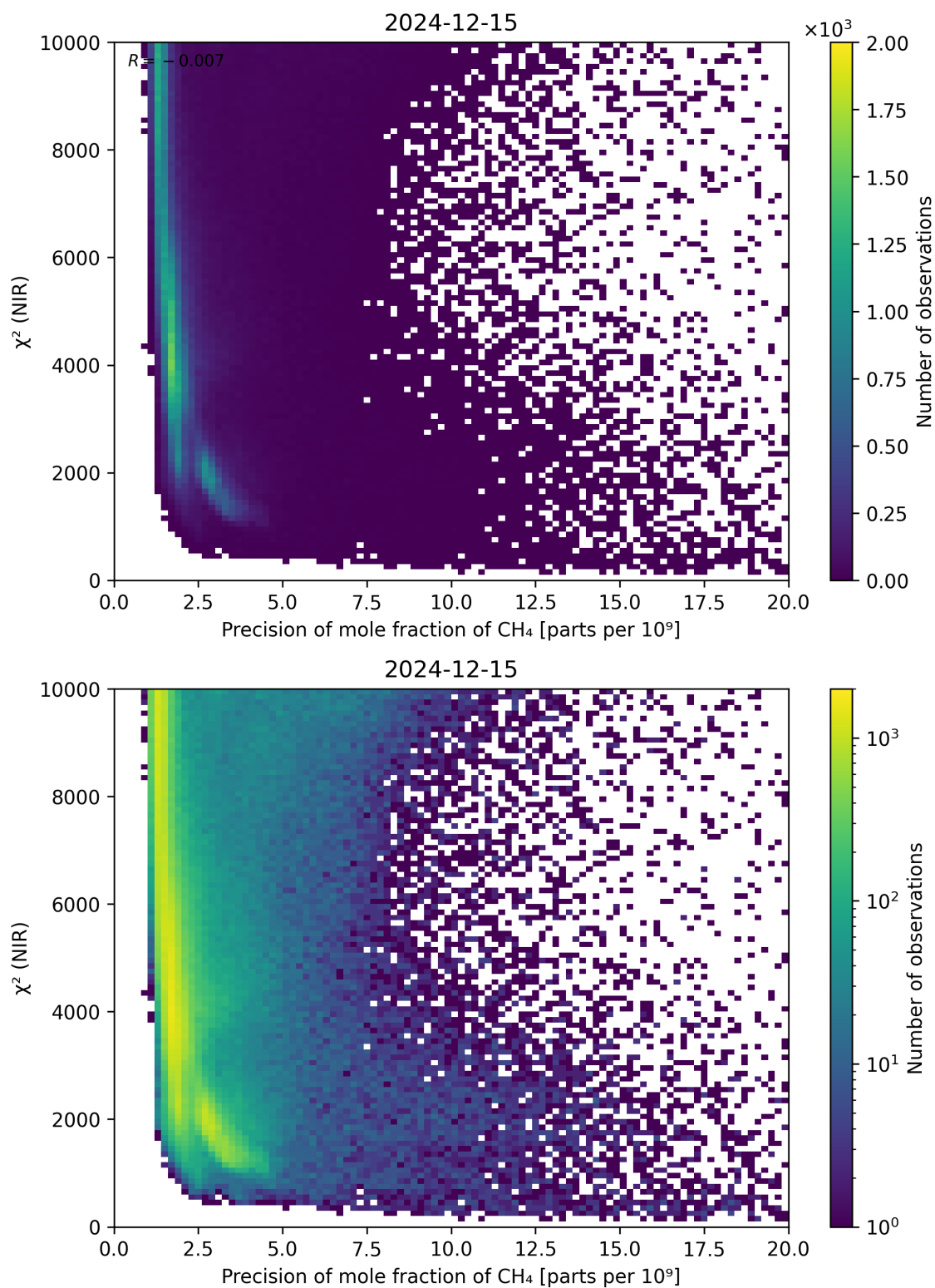
Figure 78: Scatter density plot of “Precision of mole fraction of CH 4 ” against “ \chi^2 (NIR)” for 2024-12-14 to 2024-12-16.
