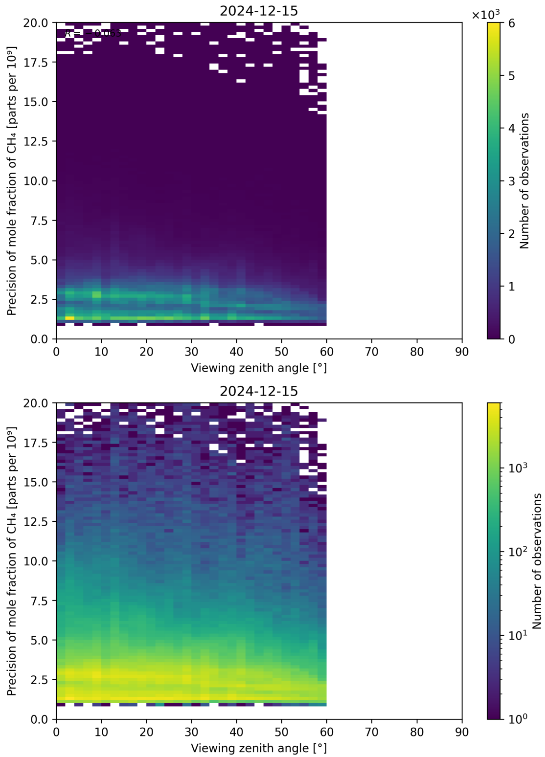
Figure 112: Scatter density plot of “Viewing zenith angle” against “Precision of mole fraction of CH 4 ” for 2024-12-14 to 2024-12-16.
