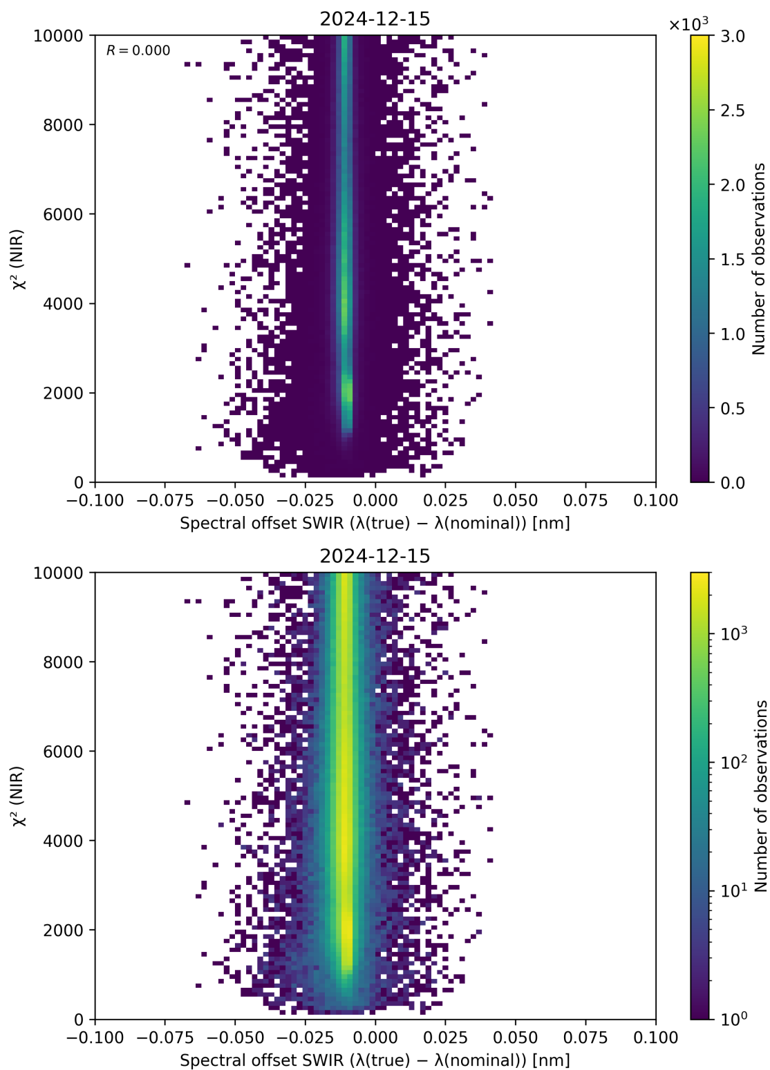
Figure 117: Scatter density plot of “Spectral offset SWIR ( \lambda_{\text{true}} - \lambda_{\text{nominal}} )” against “ \chi^2 (NIR)” for 2024-12-14 to 2024-12-16.
