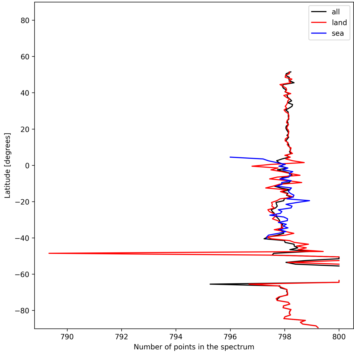
Figure 15: Zonal average of “Number of points in the spectrum” for 2024-12-14 to 2024-12-16.
