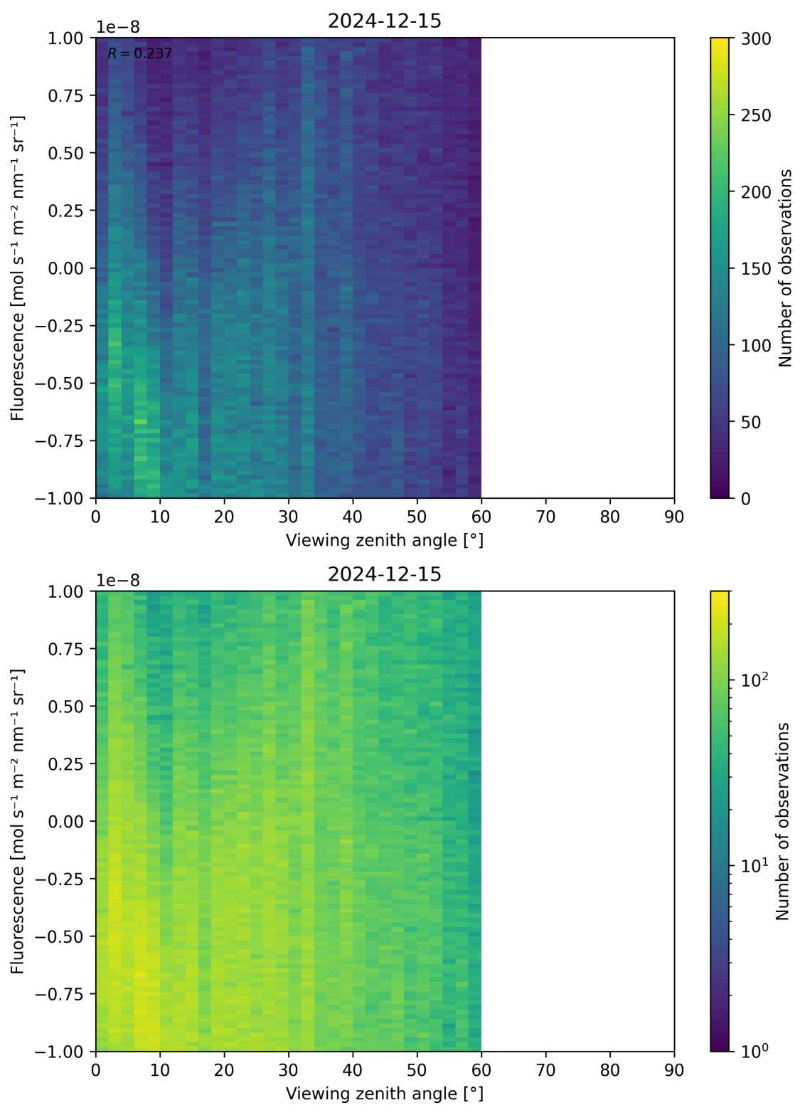
Figure 108: Scatter density plot of “Viewing zenith angle” against “Fluorescence” for 2024-12-14 to 2024-12-16.
