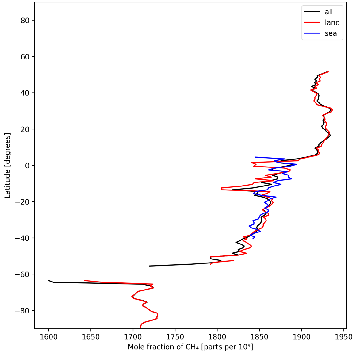
Figure 12: Zonal average of “Mole fraction of \text{CH}_4 ” for 2024-12-14 to 2024-12-16.
