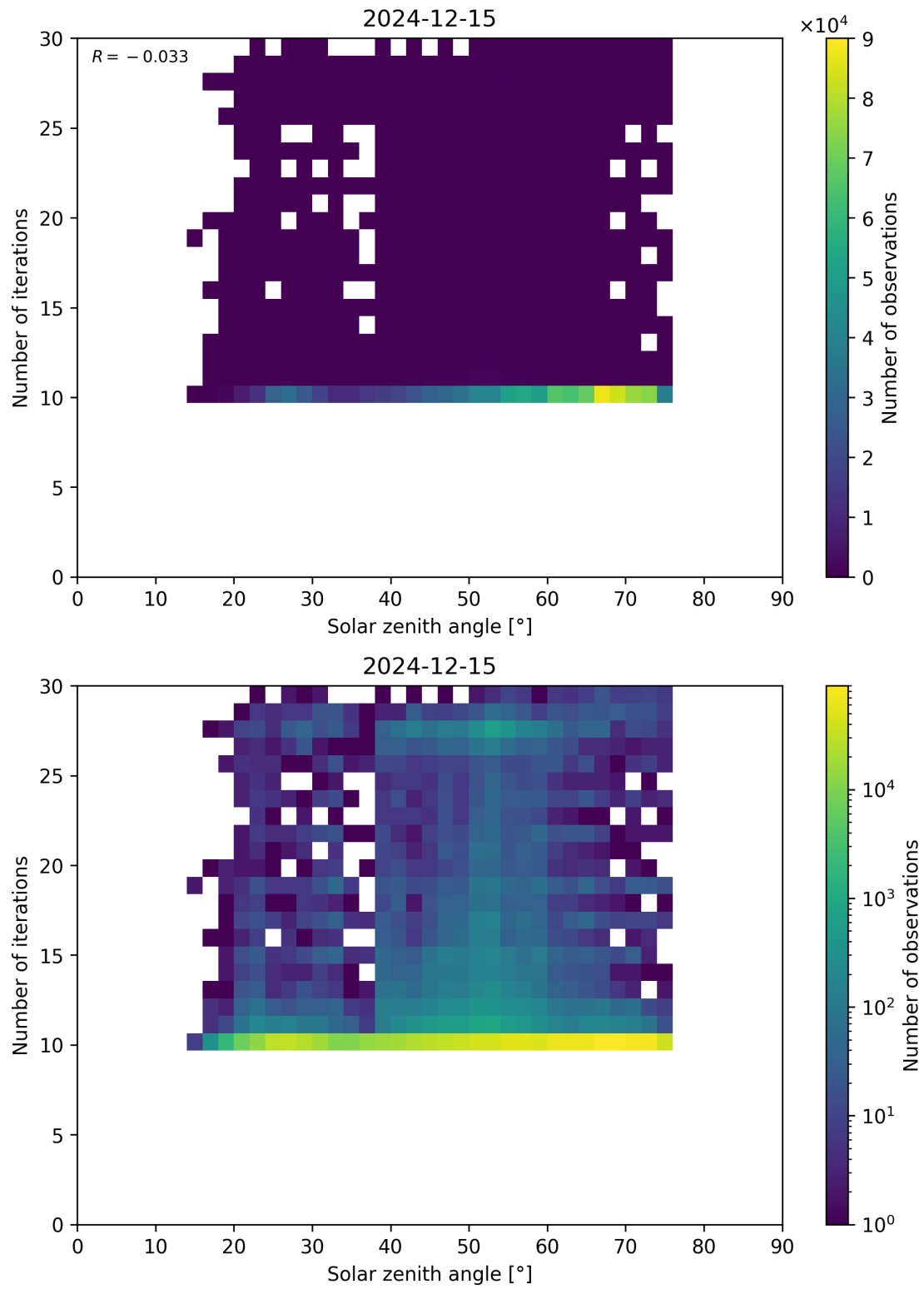
Figure 102: Scatter density plot of “Solar zenith angle” against “Number of iterations” for 2024-12-14 to 2024-12-16.
