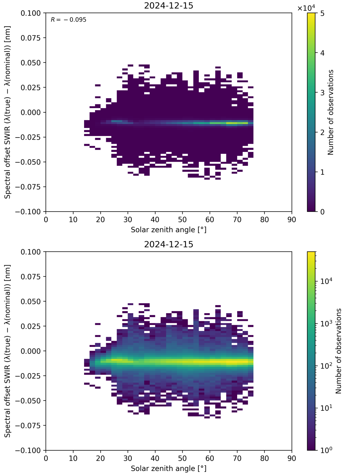
Figure 104: Scatter density plot of “Solar zenith angle” against “Spectral offset SWIR ( \lambda_{\text{true}} - \lambda_{\text{nominal}} )” for 2024-12-14 to 2024-12-16.
