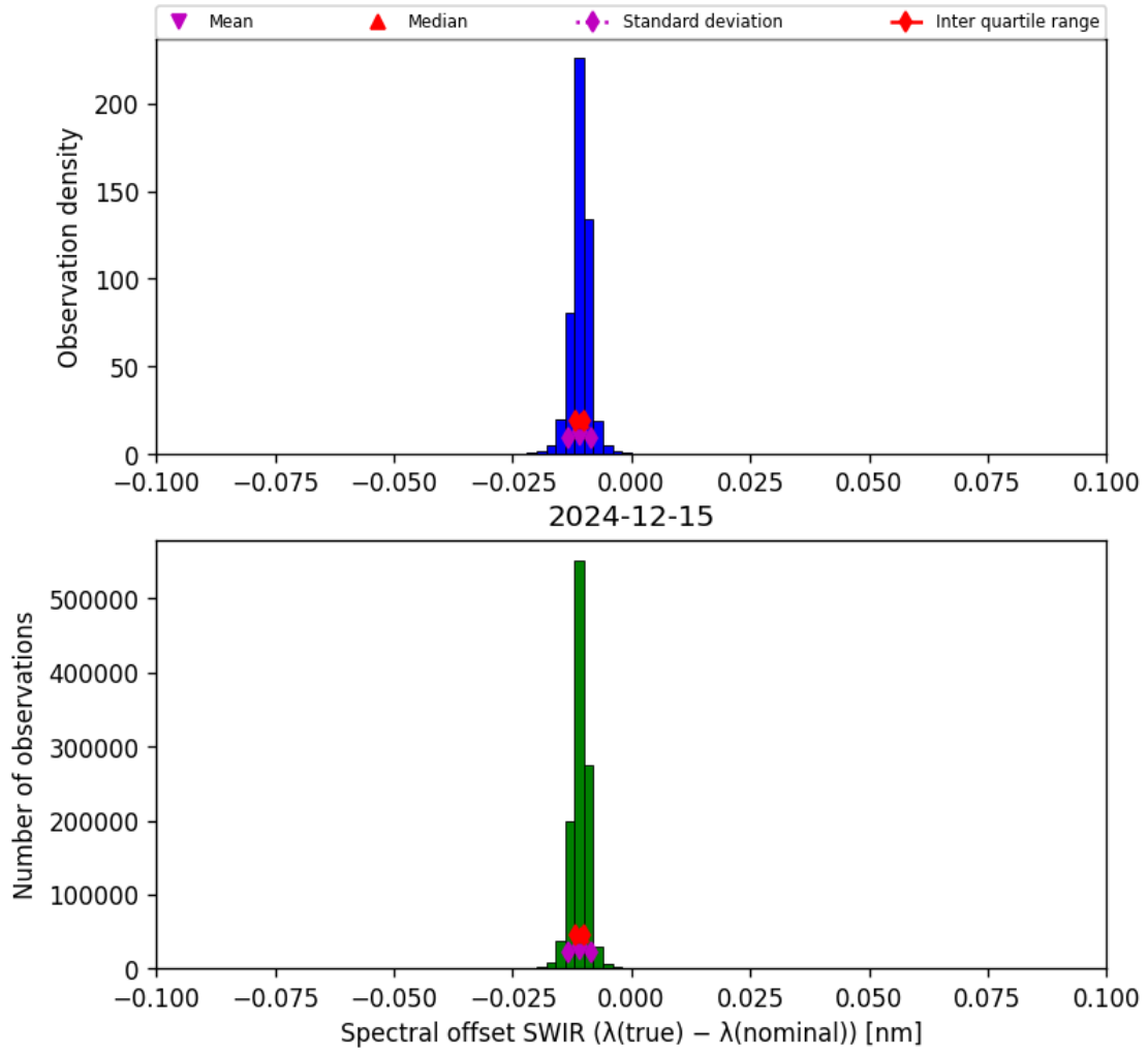
Figure 27: Histogram of “Spectral offset SWIR ( \lambda_{\text{true}} - \lambda_{\text{nominal}} )” for 2024-12-14 to 2024-12-16
