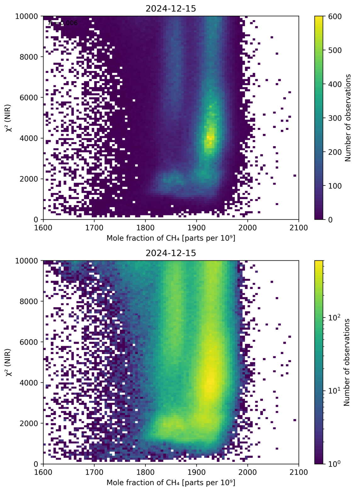
Figure 70: Scatter density plot of “Mole fraction of \text{CH}_4 ” against “ \chi^2 (NIR)” for 2024-12-14 to 2024-12-16.
