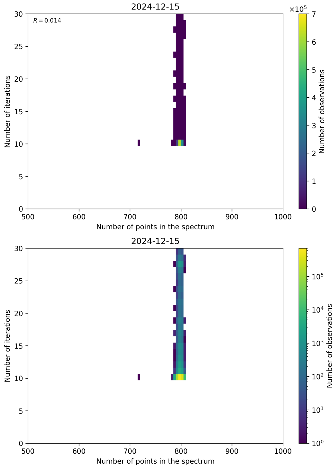
Figure 92: Scatter density plot of “Number of points in the spectrum” against “Number of iterations” for 2024-12-14 to 2024-12-16.
