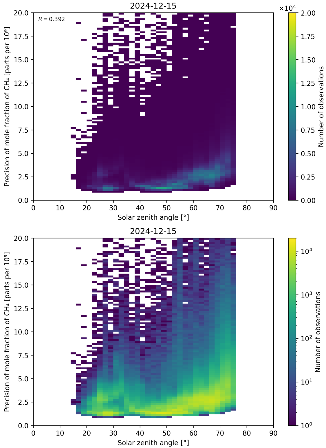
Figure 101: Scatter density plot of “Solar zenith angle” against “Precision of mole fraction of CH 4 ” for 2024-12-14 to 2024-12-16.
