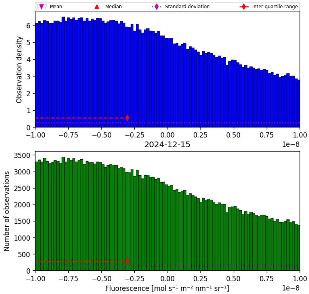
Figure 32: Histogram of “Fluorescence” for 2024-12-14 to 2024-12-16
