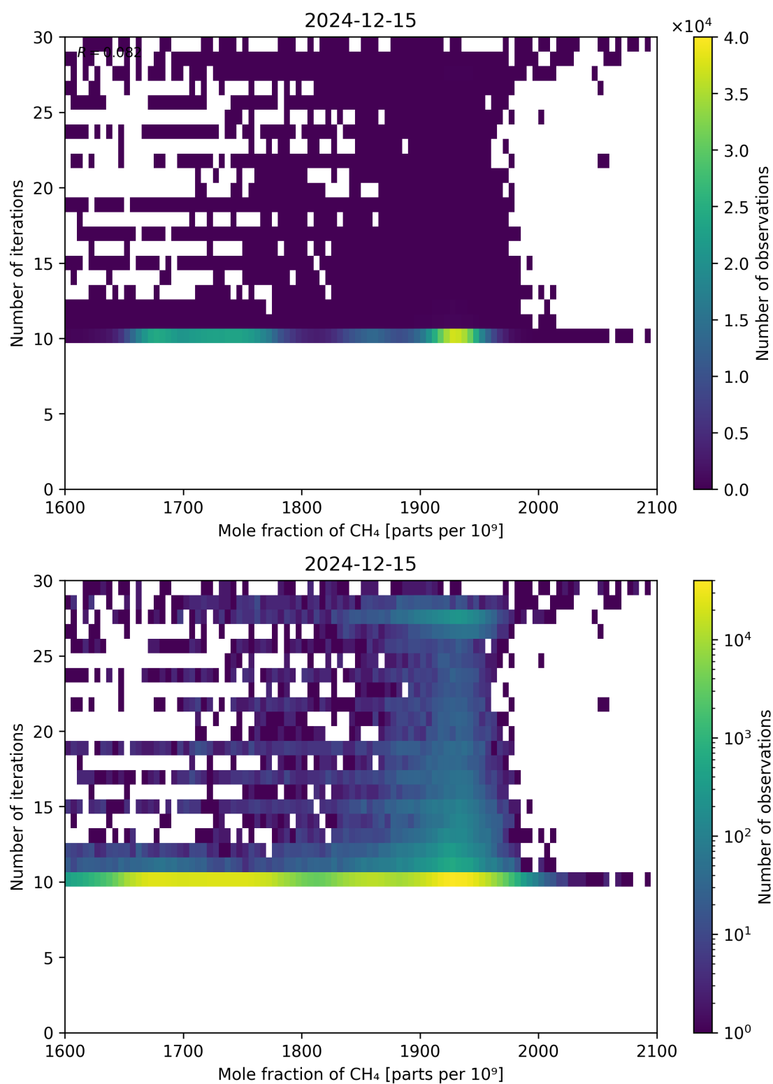
Figure 76: Scatter density plot of “Mole fraction of CH 4 ” against “Number of iterations” for 2024-12-14 to 2024-12-16.
