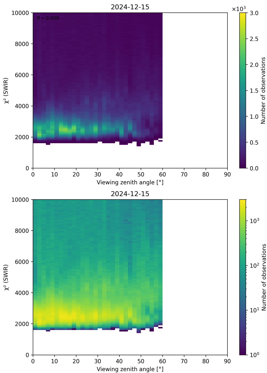
Figure 106: Scatter density plot of “Viewing zenith angle” against “ \chi^2 (SWIR)” for 2024-12-14 to 2024-12-16.
