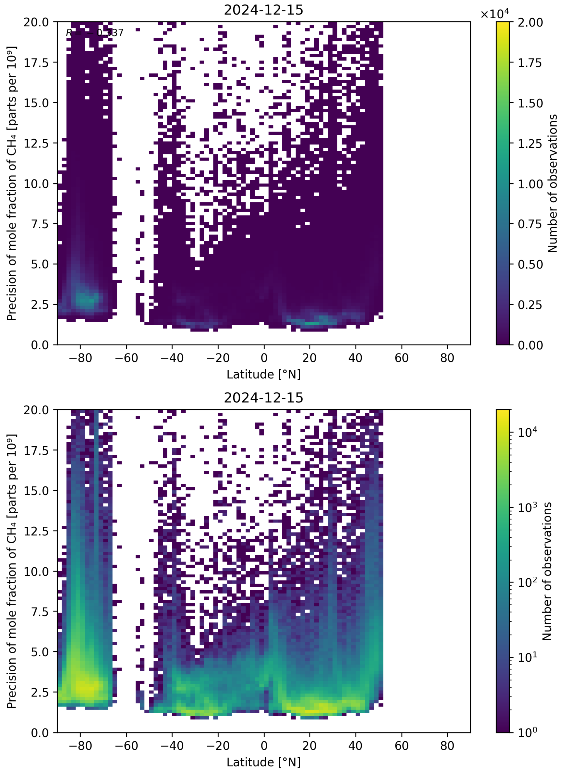
Figure 59: Scatter density plot of “Latitude” against “Precision of mole fraction of CH 4 ” for 2024-12-14 to 2024-12-16.
