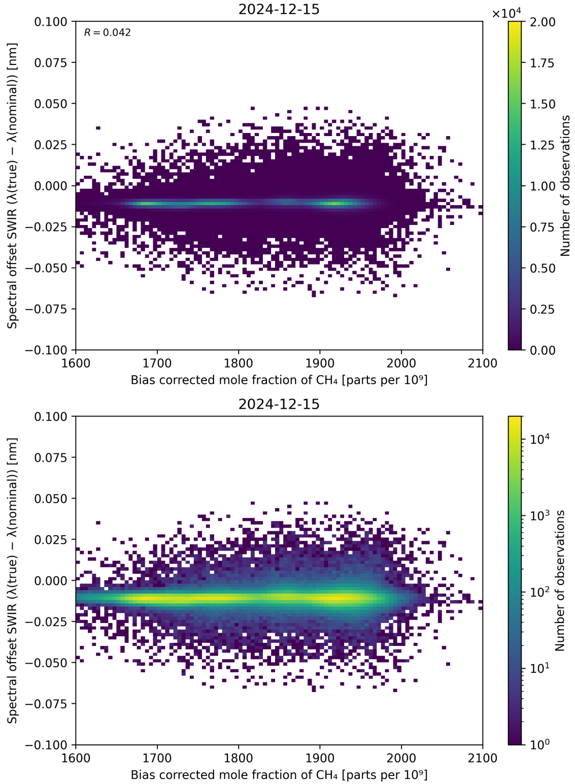
Figure 69: Scatter density plot of “Bias corrected mole fraction of \text{CH}_4 ” against “Spectral offset SWIR ( \lambda_{\text{true}} - \lambda_{\text{nominal}} )” for 2024-12-14 to 2024-12-16.
