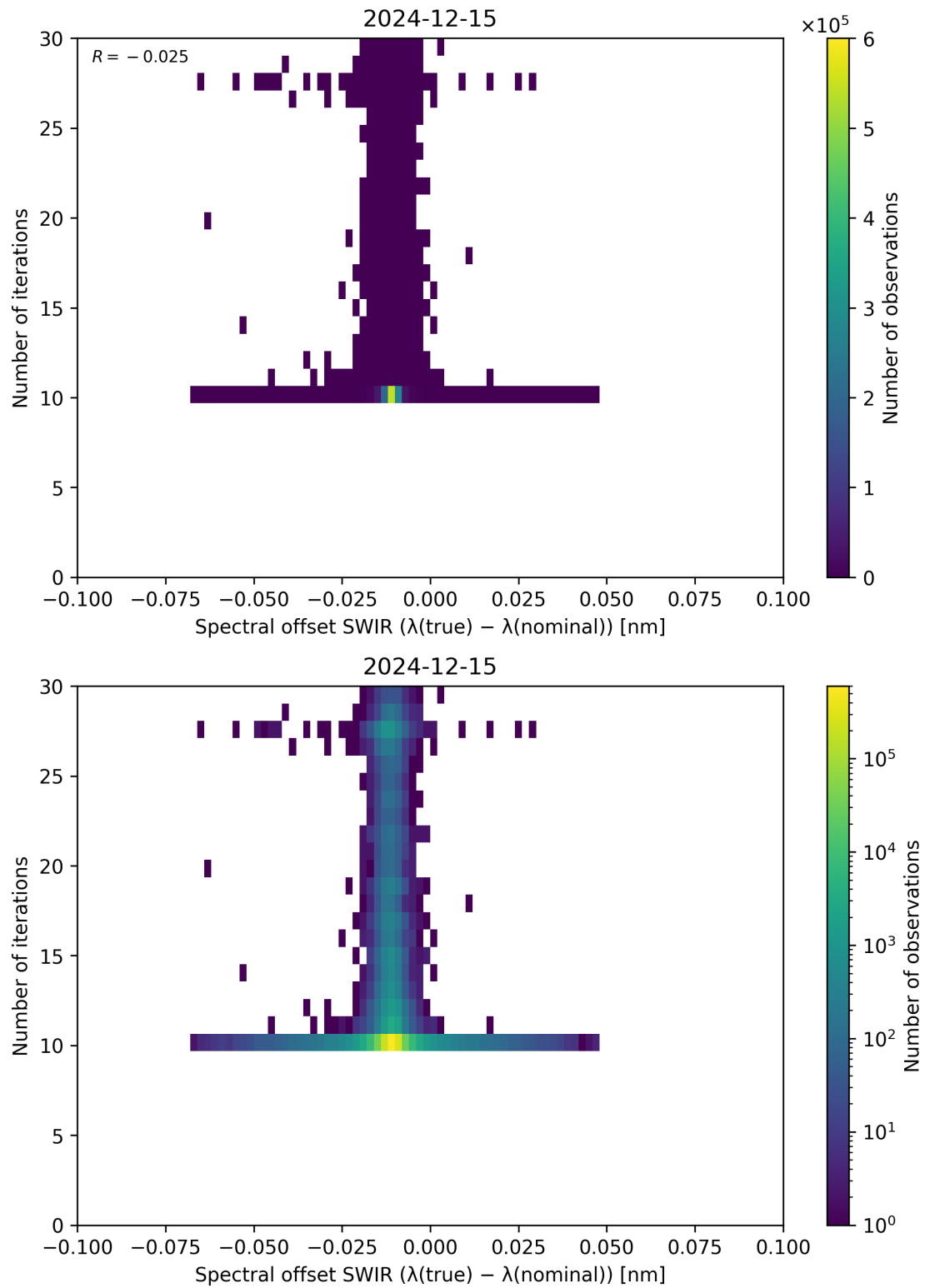
Figure 121: Scatter density plot of “Spectral offset SWIR ( \lambda_{\text{true}} - \lambda_{\text{nominal}} )” against “Number of iterations” for 2024-12-14 to 2024-12-16.
