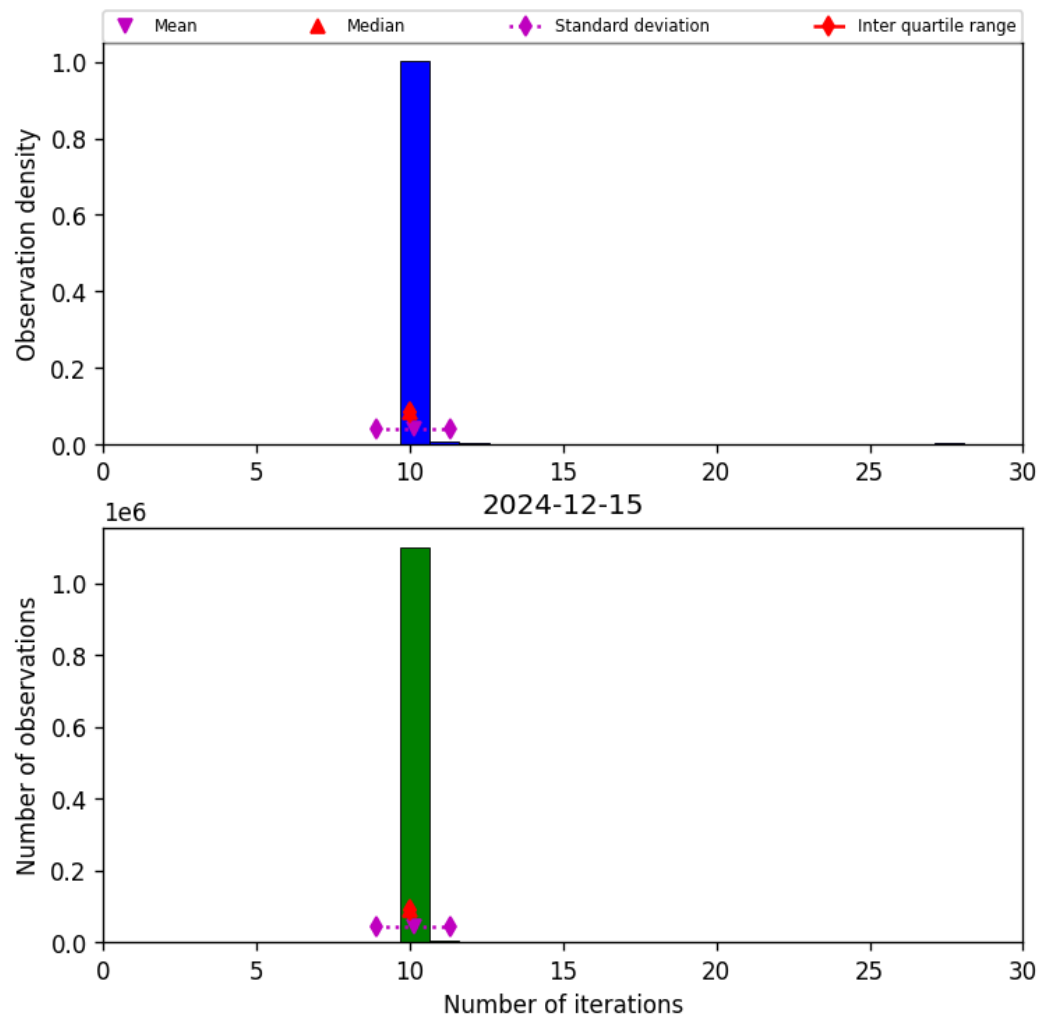
Figure 31: Histogram of “Number of iterations” for 2024-12-14 to 2024-12-16
