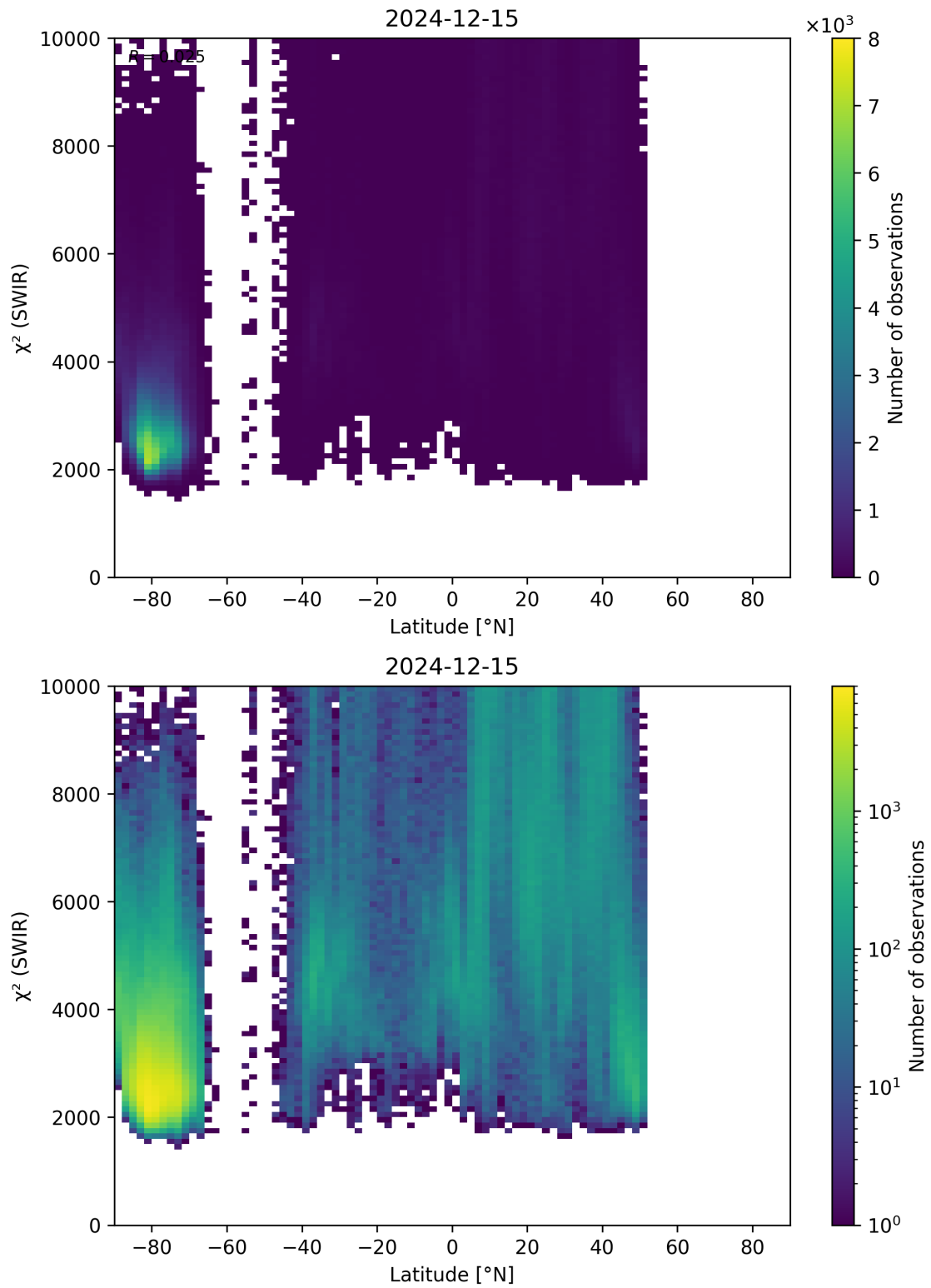
Figure 54: Scatter density plot of “Latitude” against “ \chi^2 (SWIR)” for 2024-12-14 to 2024-12-16.
