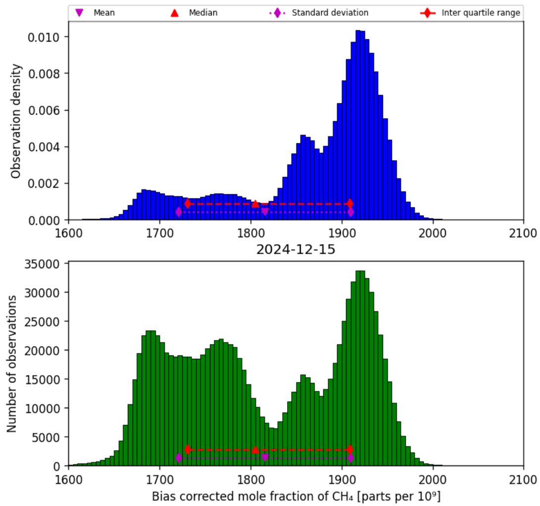
Figure 25: Histogram of “Bias corrected mole fraction of CH 4 ” for 2024-12-14 to 2024-12-16
