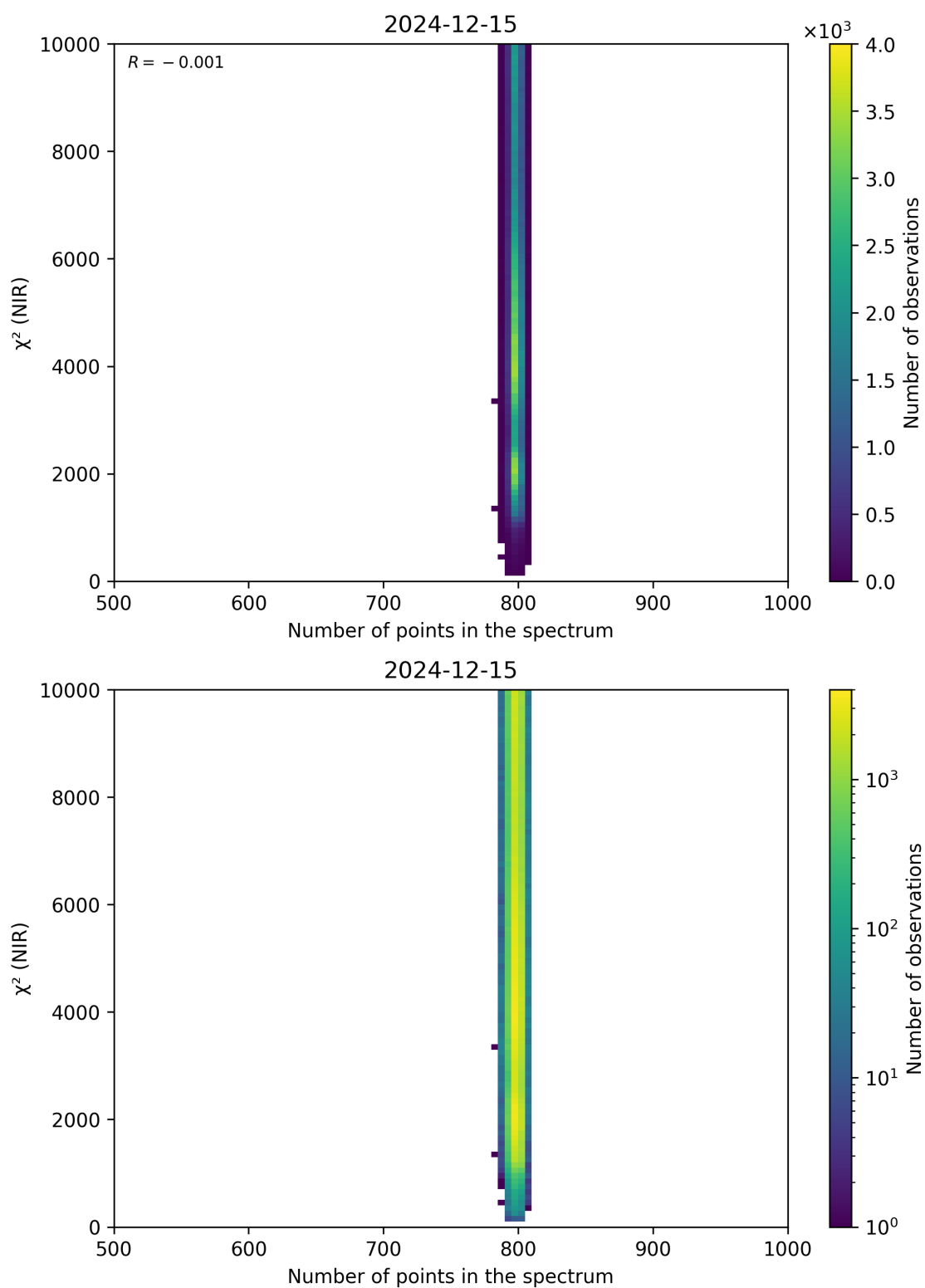
Figure 88: Scatter density plot of “Number of points in the spectrum” against “ \chi^2 (NIR)” for 2024-12-14 to 2024-12-16.
