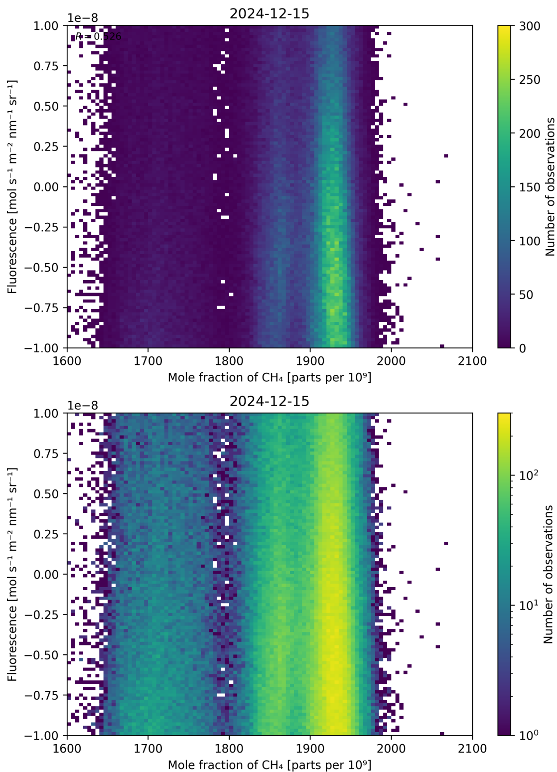
Figure 73: Scatter density plot of “Mole fraction of \text{CH}_4 ” against “Fluorescence” for 2024-12-14 to 2024-12-16.
