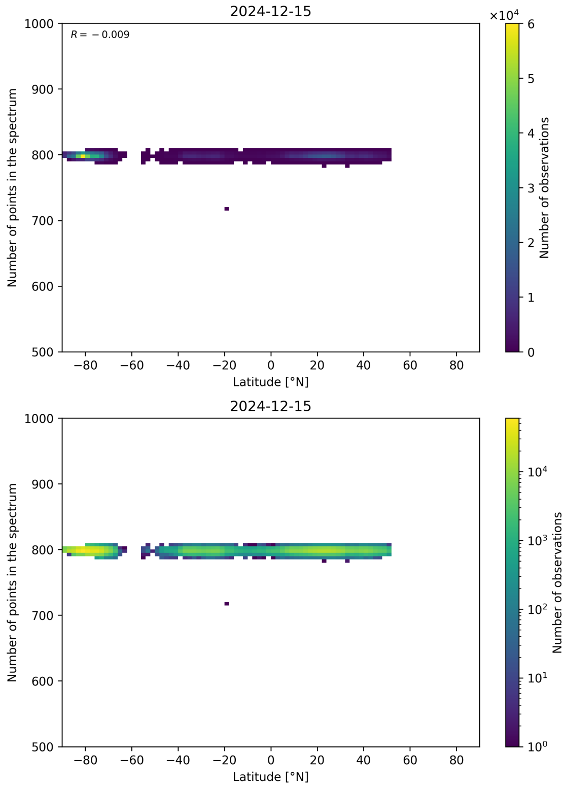
Figure 61: Scatter density plot of “Latitude” against “Number of points in the spectrum” for 2024-12-14 to 2024-12-16.
