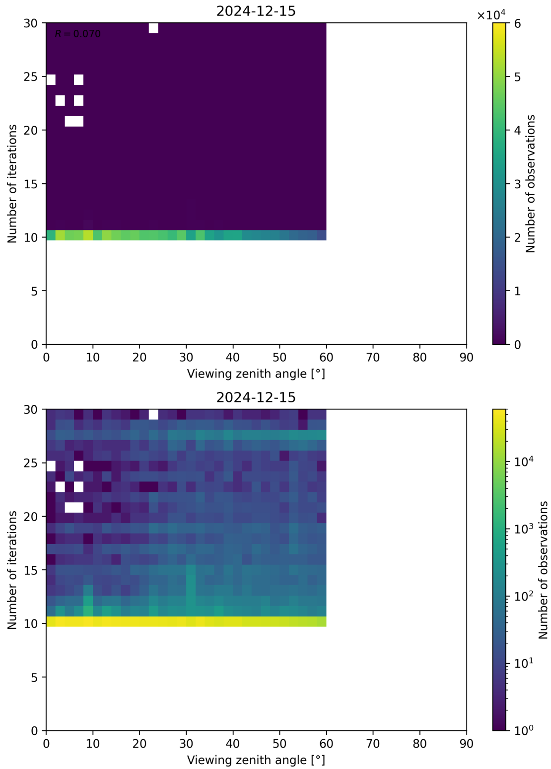
Figure 113: Scatter density plot of “Viewing zenith angle” against “Number of iterations” for 2024-12-14 to 2024-12-16.
