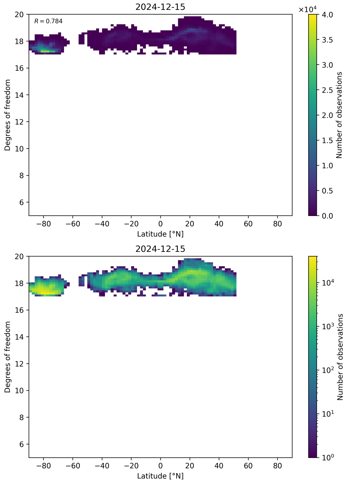
Figure 55: Scatter density plot of “Latitude” against “Degrees of freedom” for 2024-12-14 to 2024-12-16.
