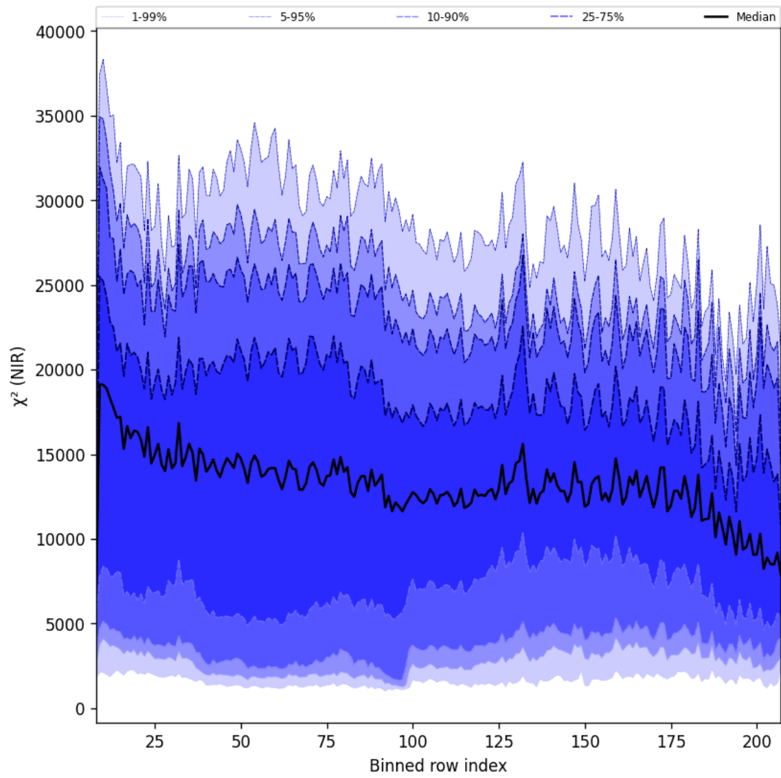
Figure 40: Along track statistics of “ \chi^2 (NIR)” for 2024-12-14 to 2024-12-16
