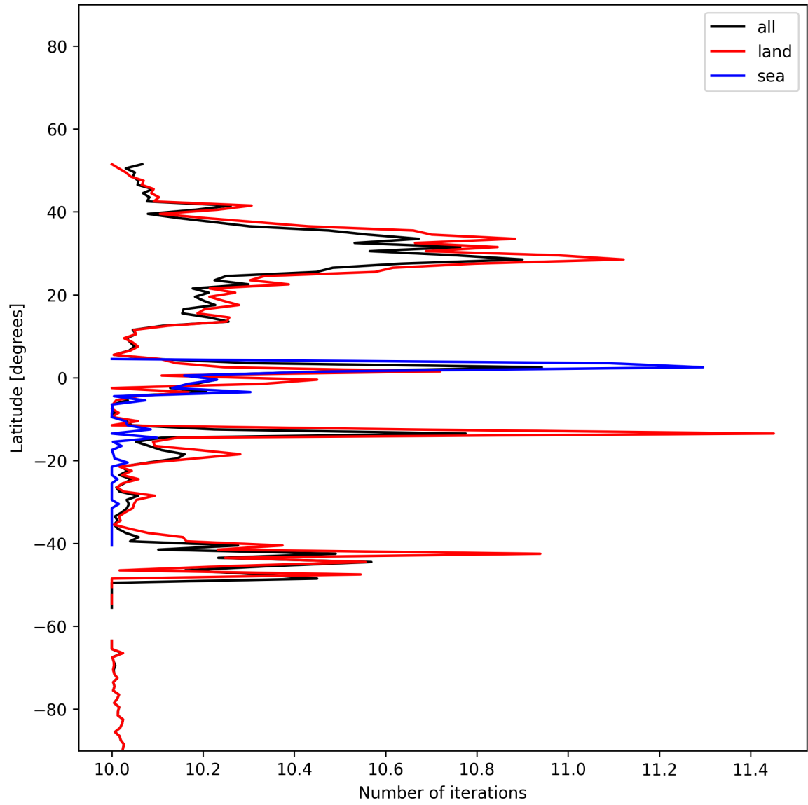
Figure 20: Zonal average of “Number of iterations” for 2024-12-14 to 2024-12-16.
