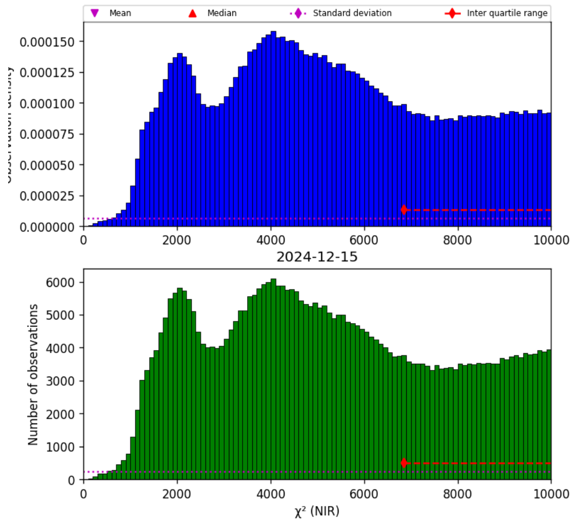
Figure 29: Histogram of “ \chi^2 (NIR)” for 2024-12-14 to 2024-12-16
