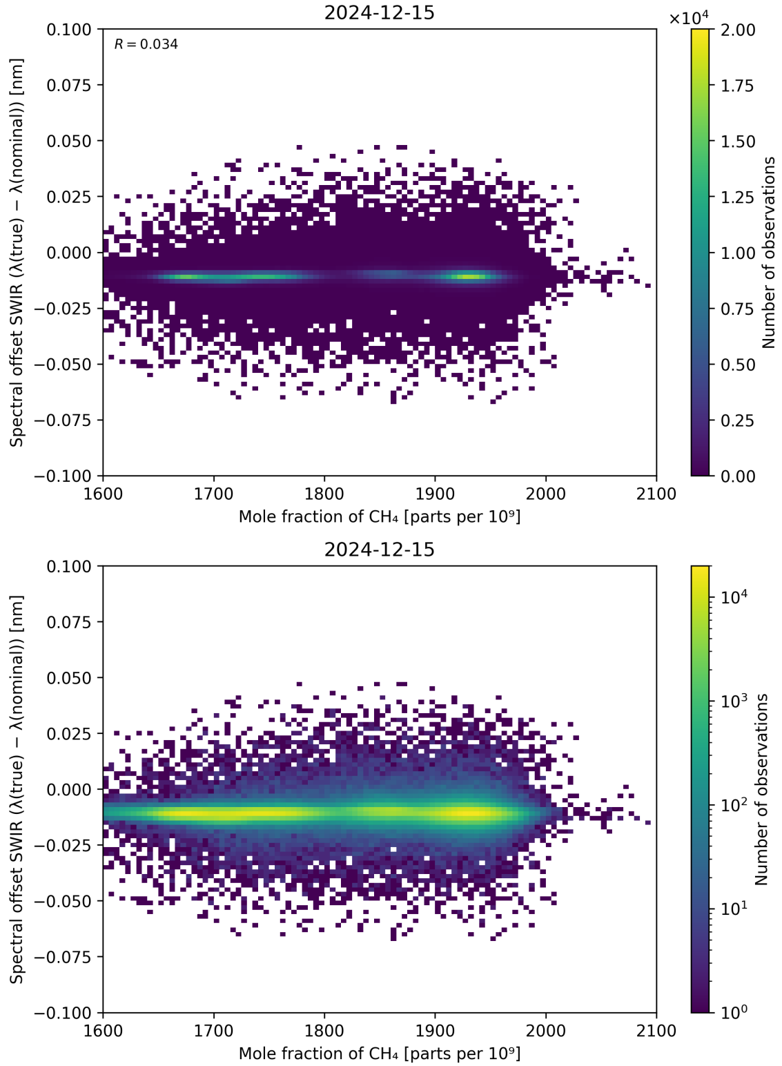
Figure 86: Scatter density plot of “Mole fraction of \text{CH}_4 ” against “Spectral offset SWIR ( \lambda_{\text{true}} - \lambda_{\text{nominal}} )” for 2024-12-14 to 2024-12-16.
