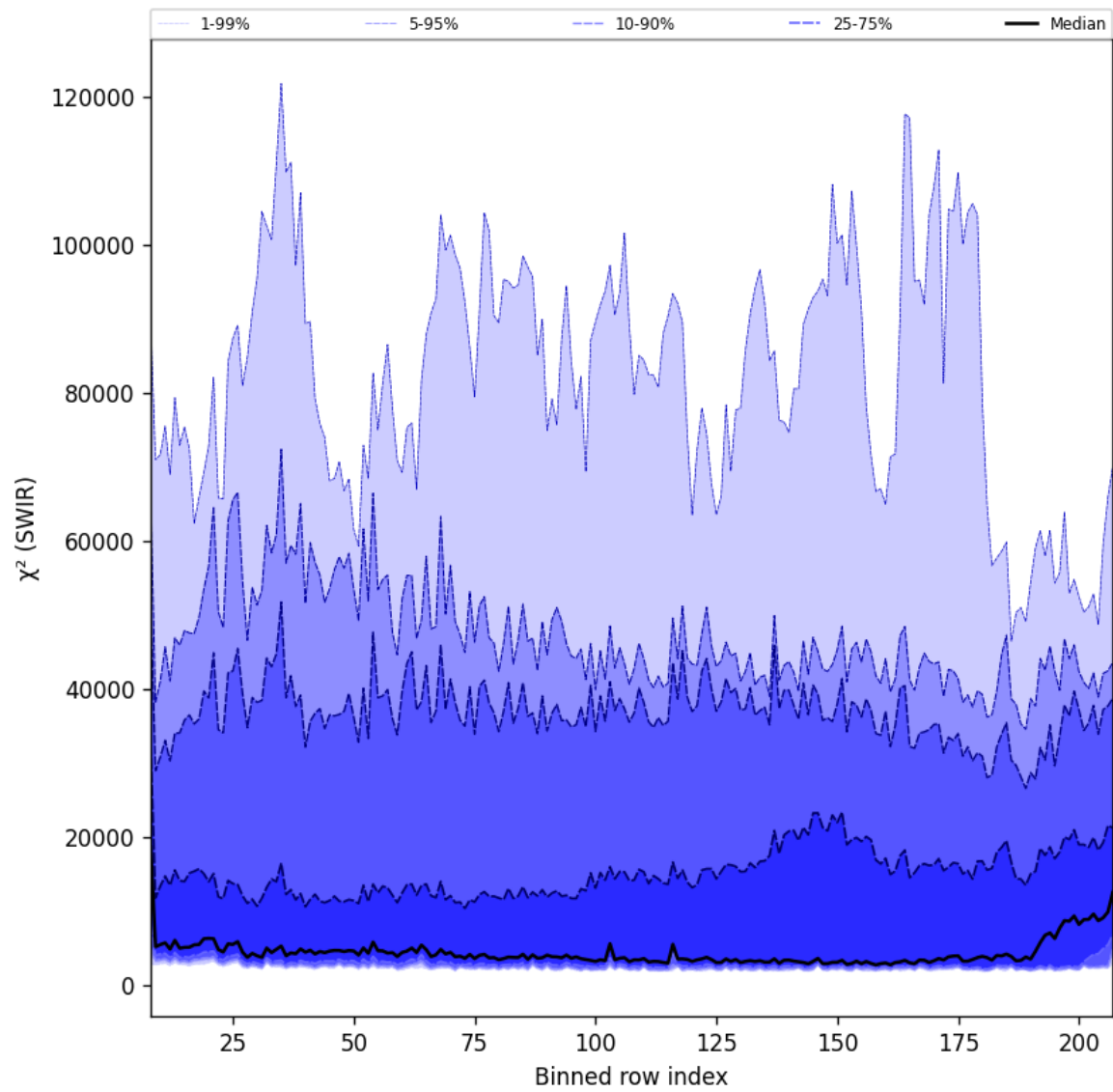
Figure 39: Along track statistics of “ \chi^2 (SWIR)” for 2024-12-14 to 2024-12-16
