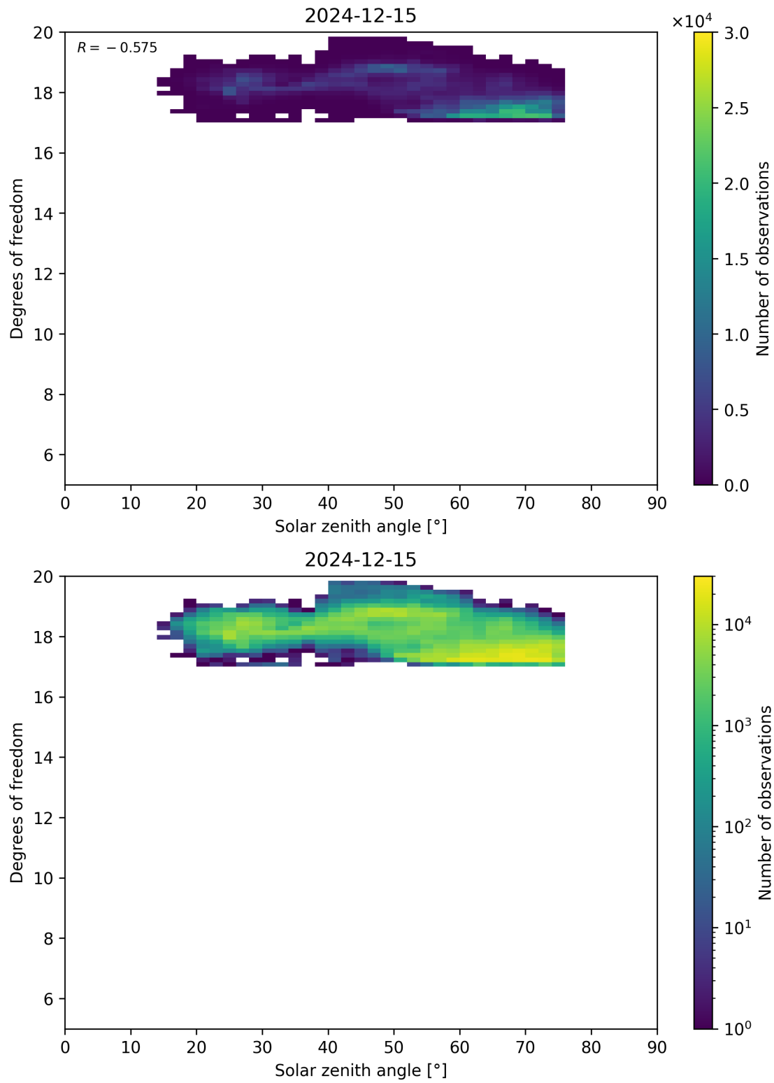
Figure 96: Scatter density plot of “Solar zenith angle” against “Degrees of freedom” for 2024-12-14 to 2024-12-16.
