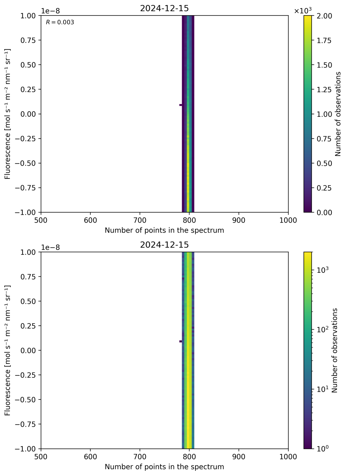
Figure 91: Scatter density plot of “Number of points in the spectrum” against “Fluorescence” for 2024-12-14 to 2024-12-16.
