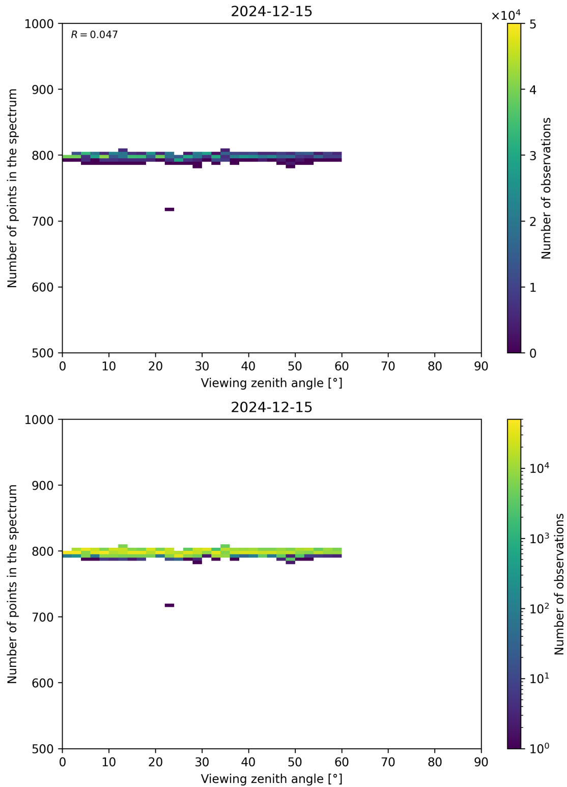
Figure 114: Scatter density plot of “Viewing zenith angle” against “Number of points in the spectrum” for 2024-12-14 to 2024-12-16.
