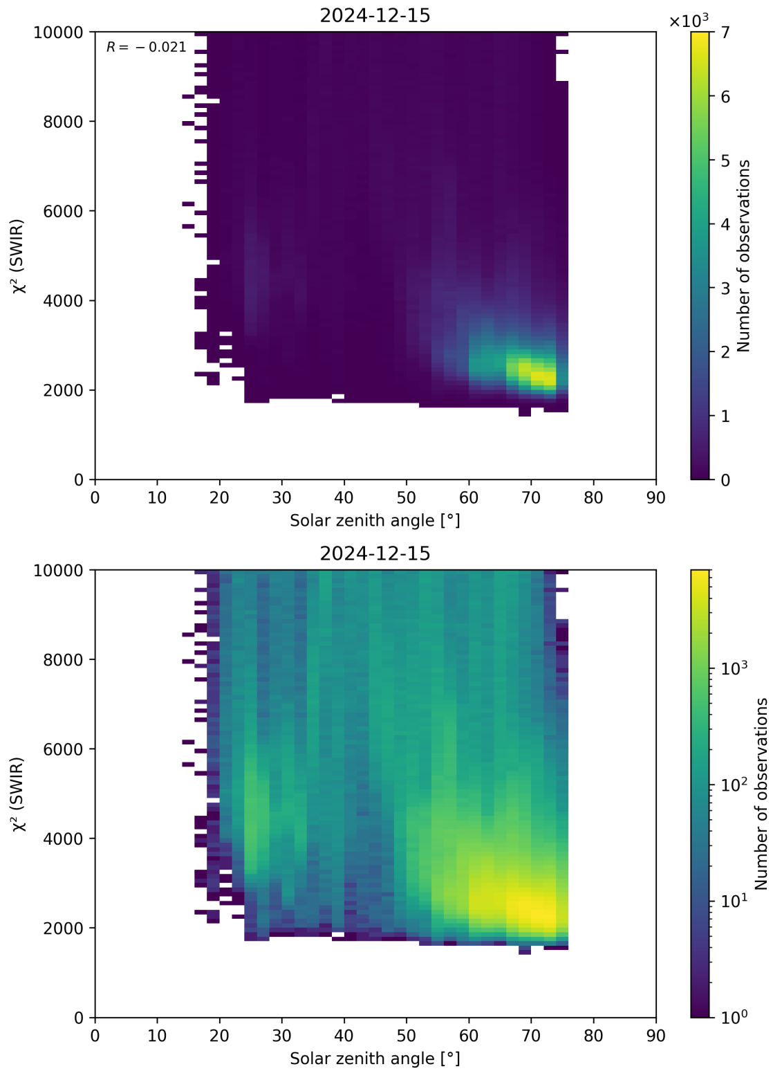
Figure 95: Scatter density plot of “Solar zenith angle” against “ \chi^2 (SWIR)” for 2024-12-14 to 2024-12-16.
