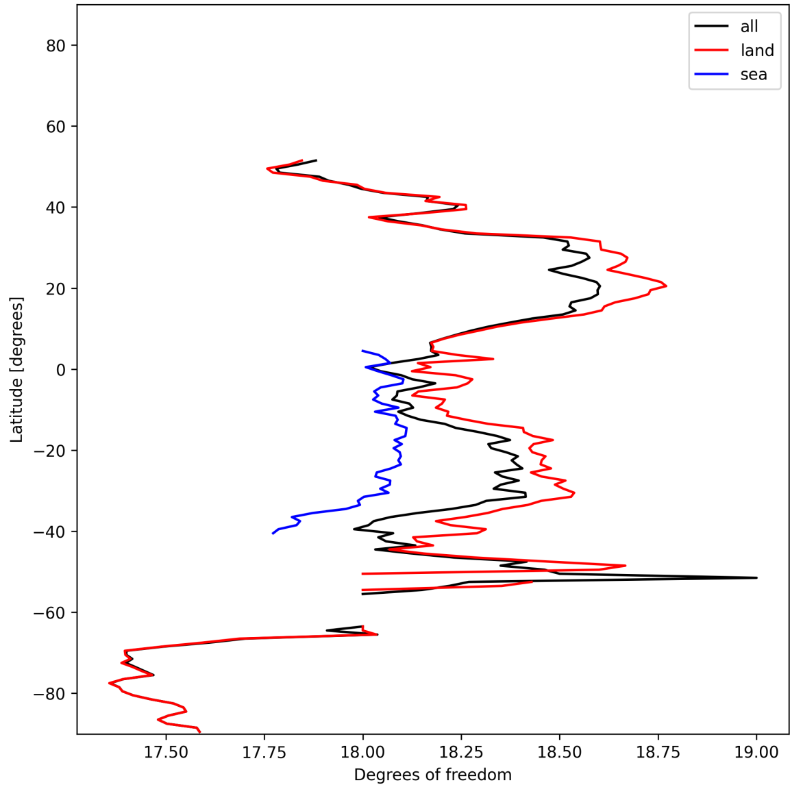
Figure 19: Zonal average of “Degrees of freedom” for 2024-12-14 to 2024-12-16.
