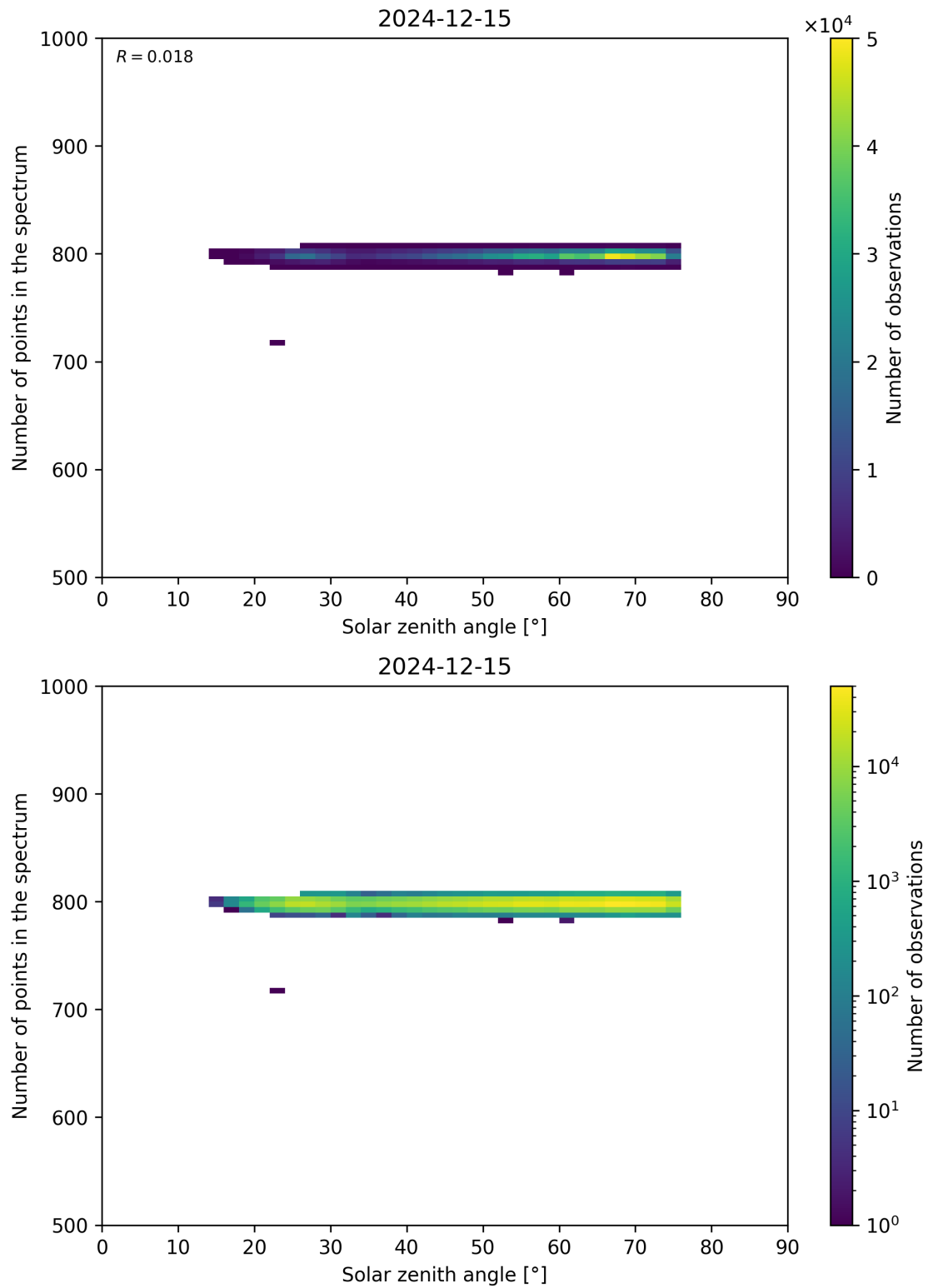
Figure 103: Scatter density plot of “Solar zenith angle” against “Number of points in the spectrum” for 2024-12-14 to 2024-12-16.
