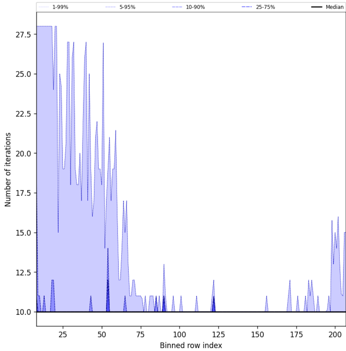
Figure 42: Along track statistics of “Number of iterations” for 2024-12-14 to 2024-12-16
