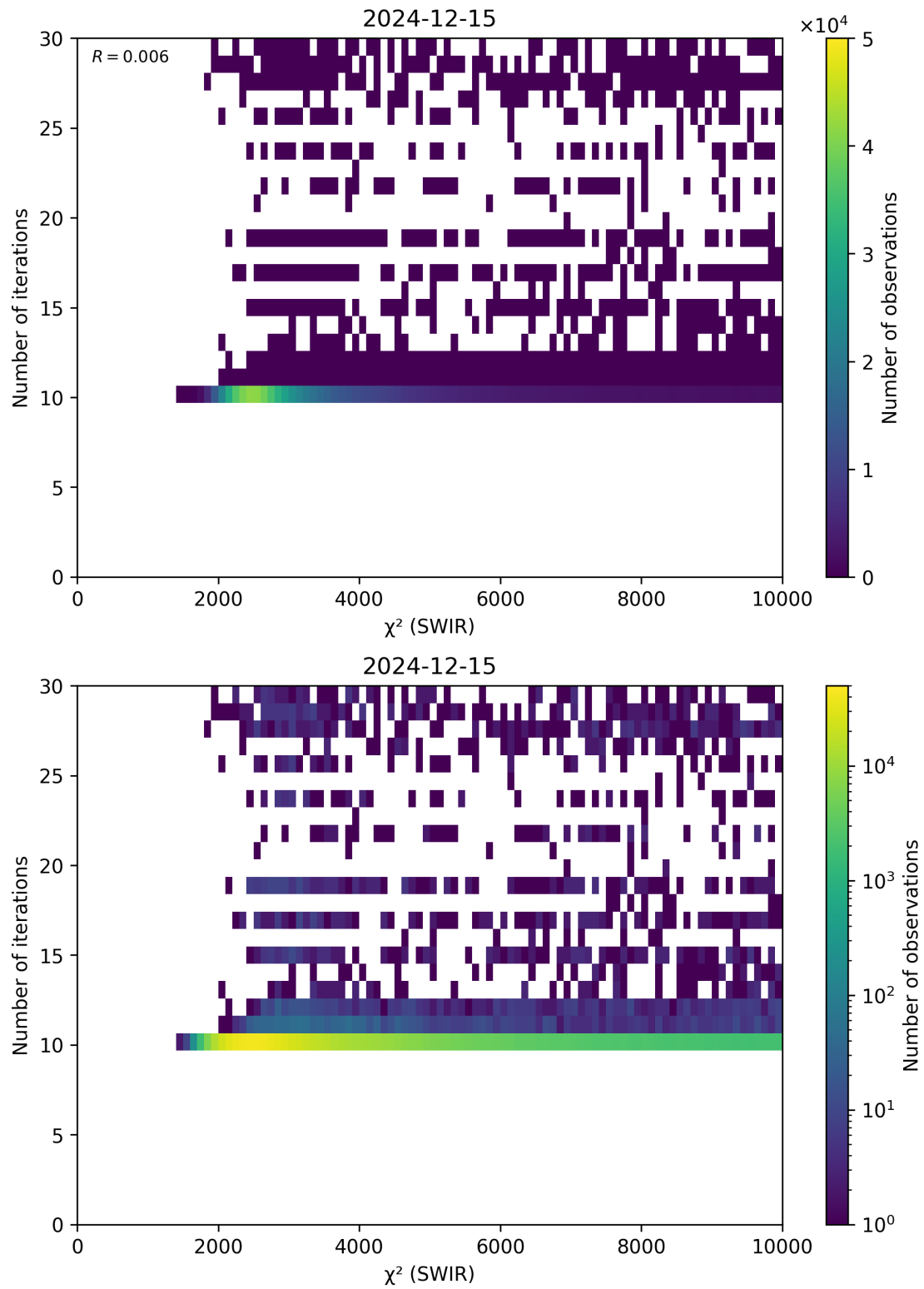
Figure 50: Scatter density plot of “ \chi^2 (SWIR)” against “Number of iterations” for 2024-12-14 to 2024-12-16.
