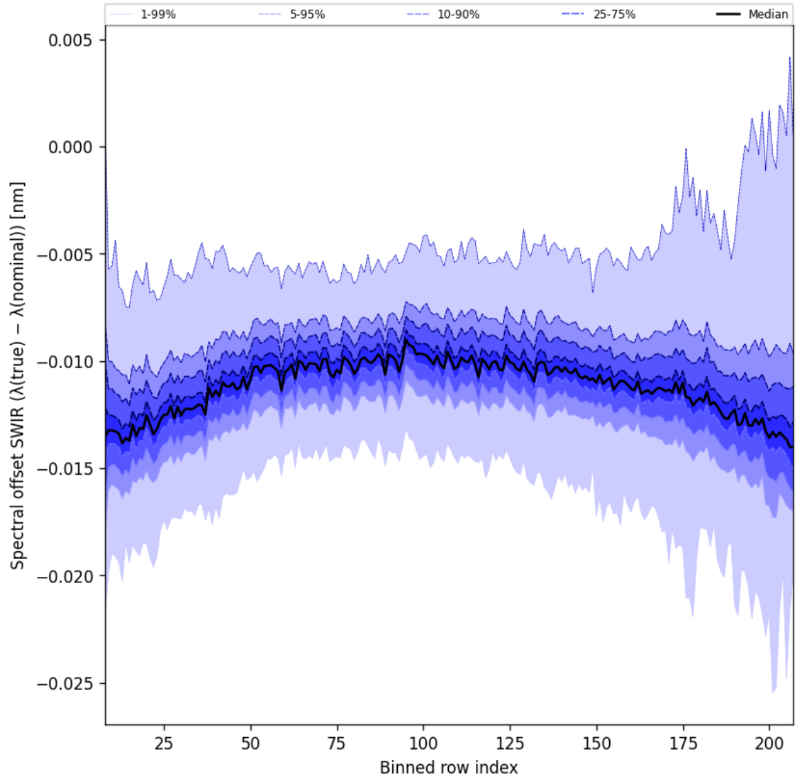
Figure 38: Along track statistics of “Spectral offset SWIR ( \lambda_{\text{true}} - \lambda_{\text{nominal}} )” for 2024-12-14 to 2024-12-16
