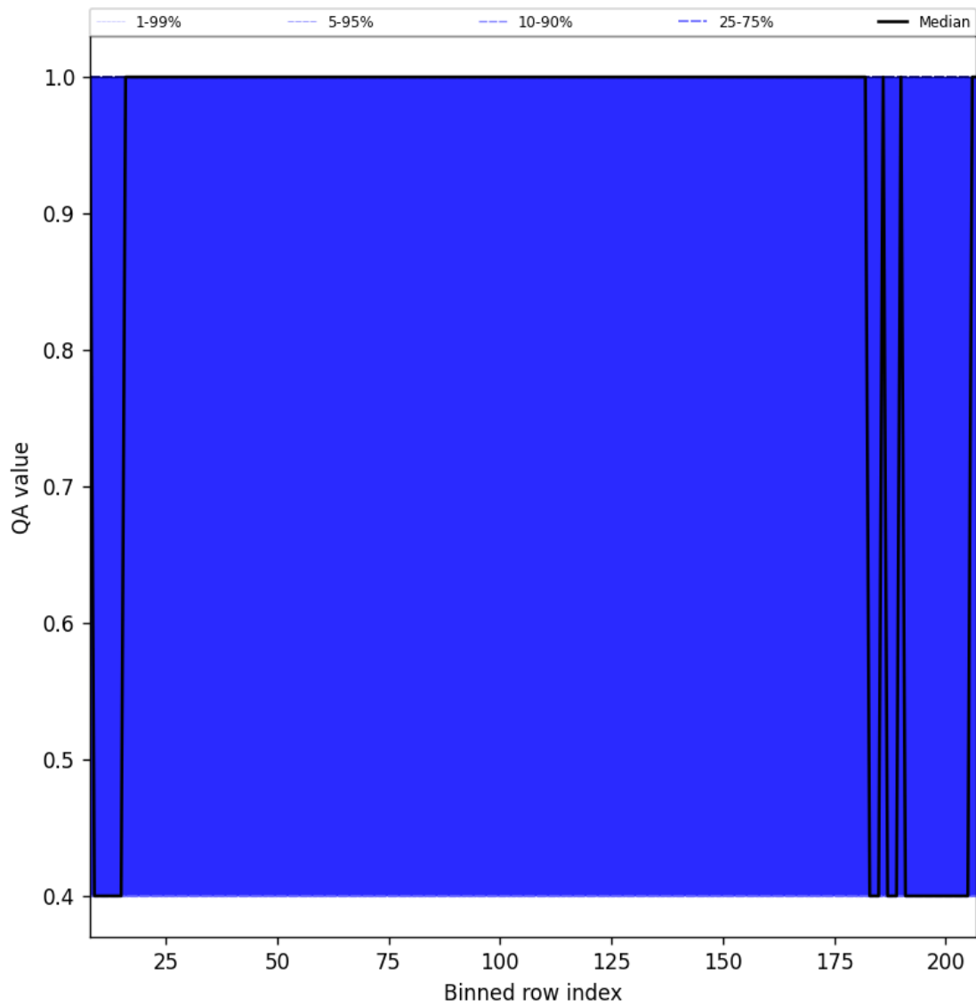
Figure 33: Along track statistics of “QA value” for 2024-12-14 to 2024-12-16
