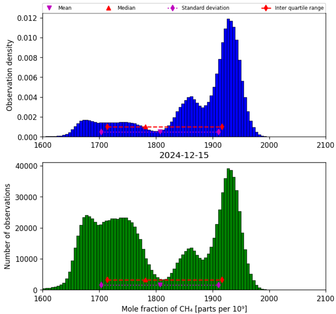
Figure 23: Histogram of “Mole fraction of CH 4 ” for 2024-12-14 to 2024-12-16
