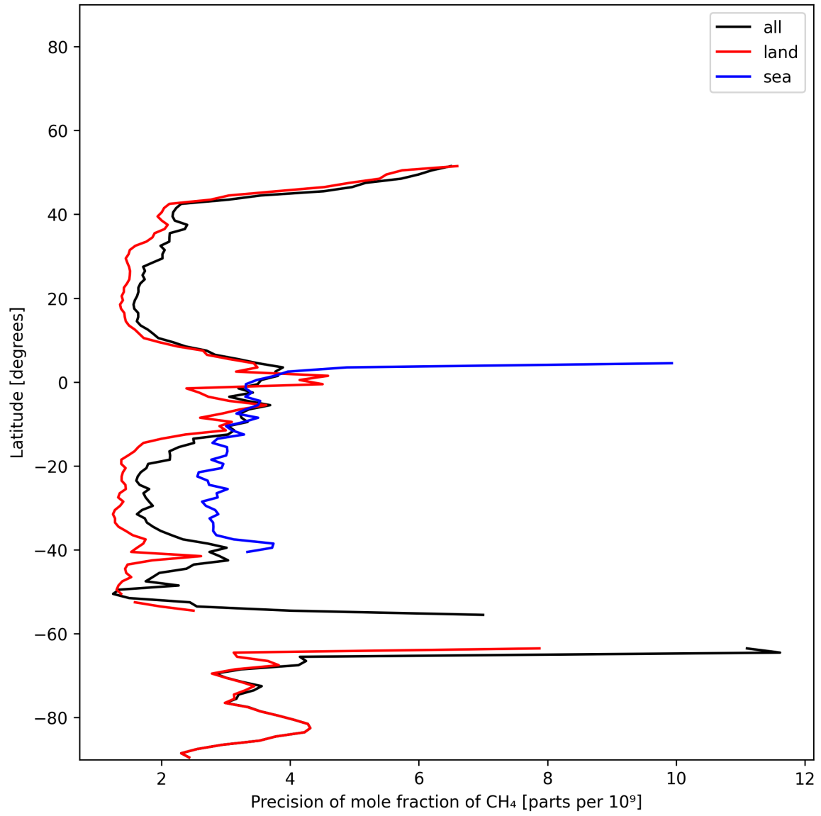
Figure 13: Zonal average of “Precision of mole fraction of CH 4 ” for 2024-12-14 to 2024-12-16.
