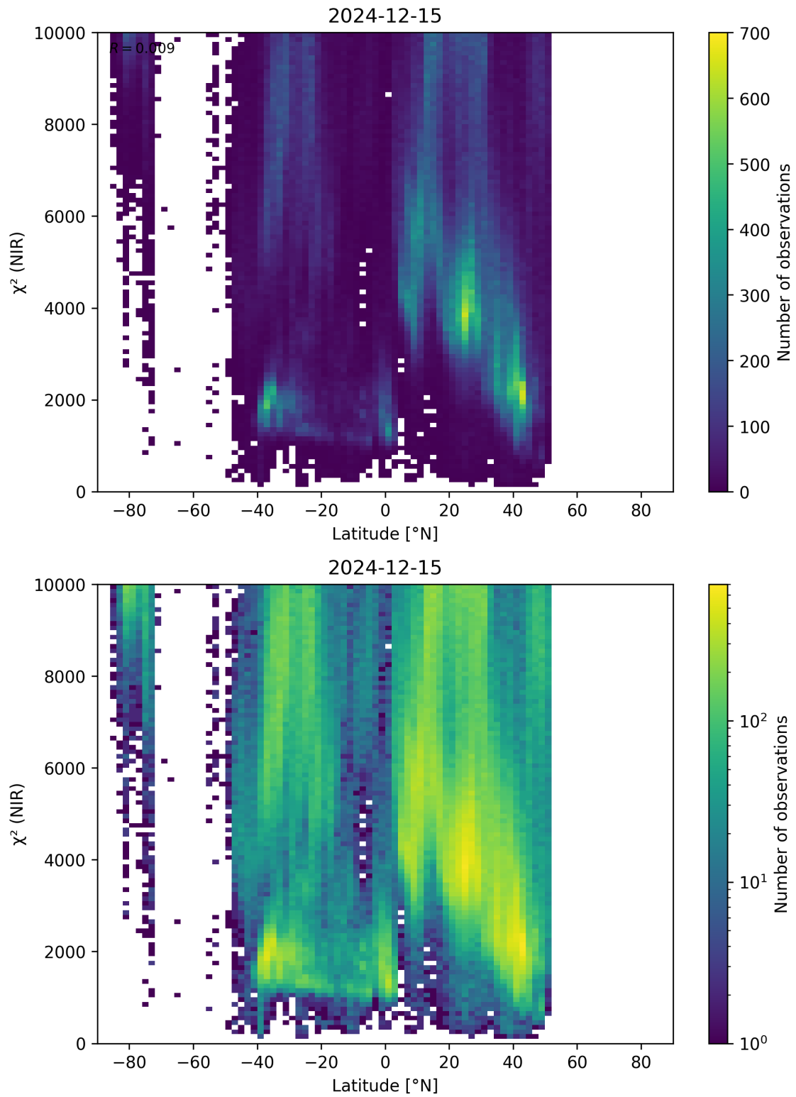
Figure 53: Scatter density plot of “Latitude” against “ \chi^2 (NIR)” for 2024-12-14 to 2024-12-16.
