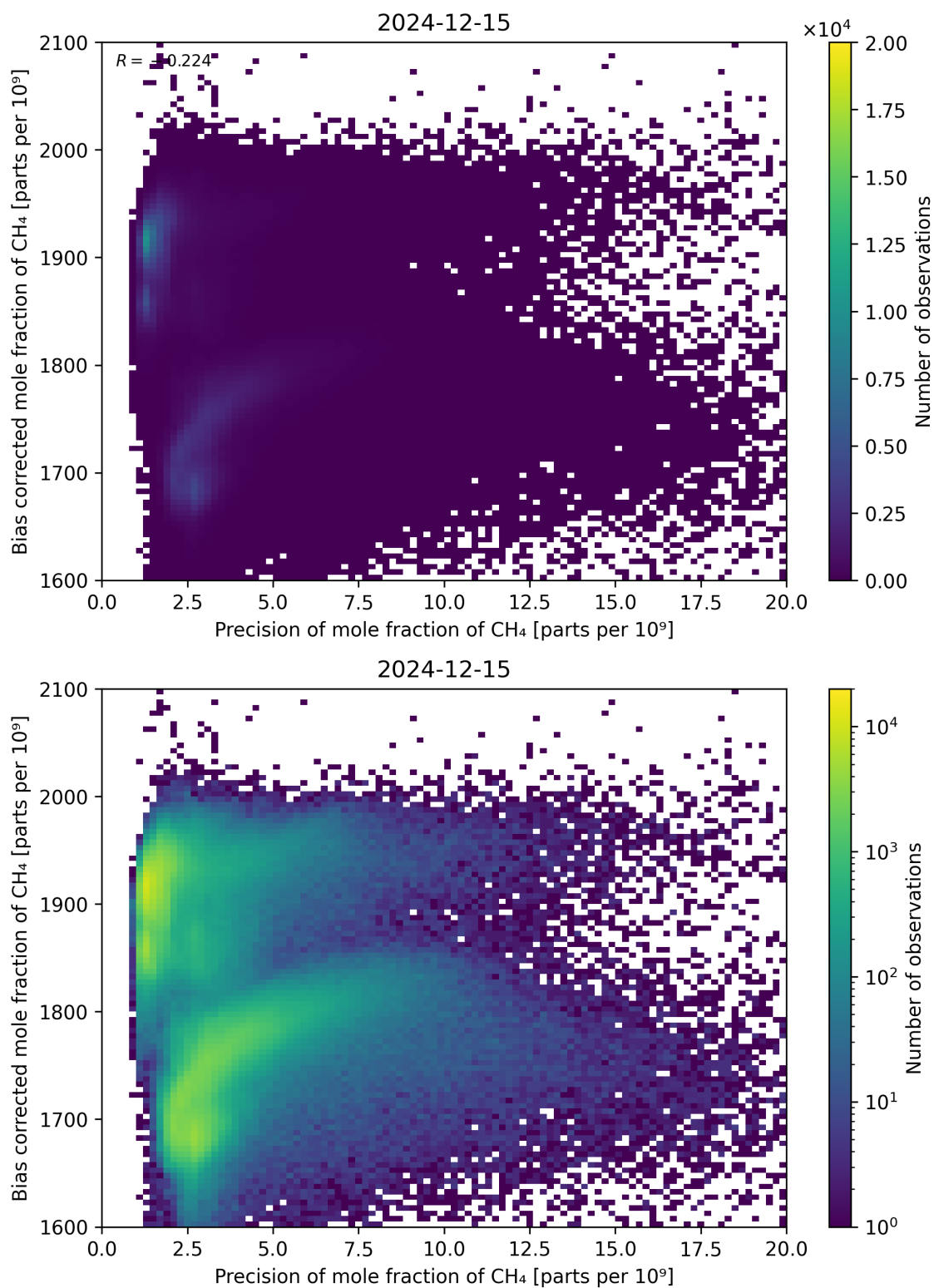
Figure 82: Scatter density plot of “Precision of mole fraction of \text{CH}_4 ” against “Bias corrected mole fraction of \text{CH}_4 ” for 2024-12-14 to 2024-12-16.
