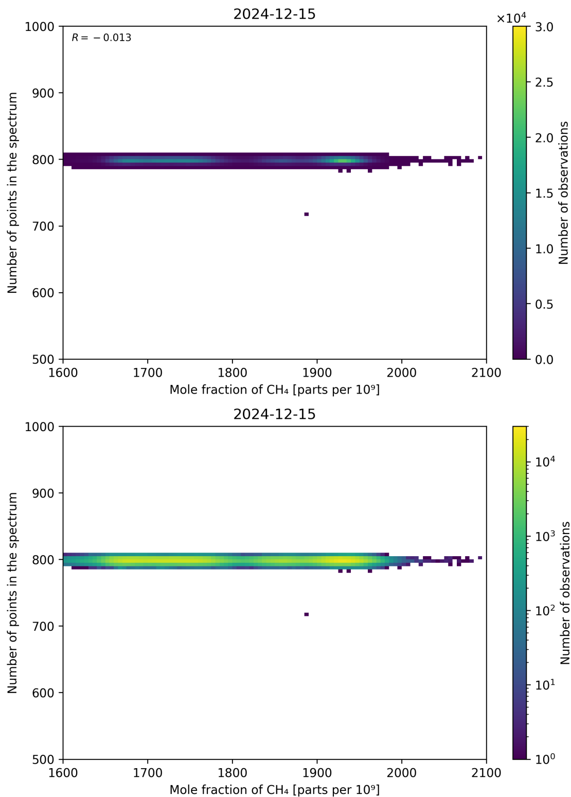
Figure 77: Scatter density plot of “Mole fraction of CH 4 ” against “Number of points in the spectrum” for 2024-12-14 to 2024-12-16.
