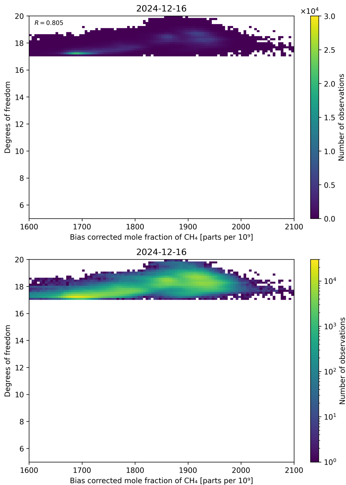
Figure 65: Scatter density plot of “Bias corrected mole fraction of CH 4 ” against “Degrees of freedom” for 2024-12-16 to 2024-12-17.
