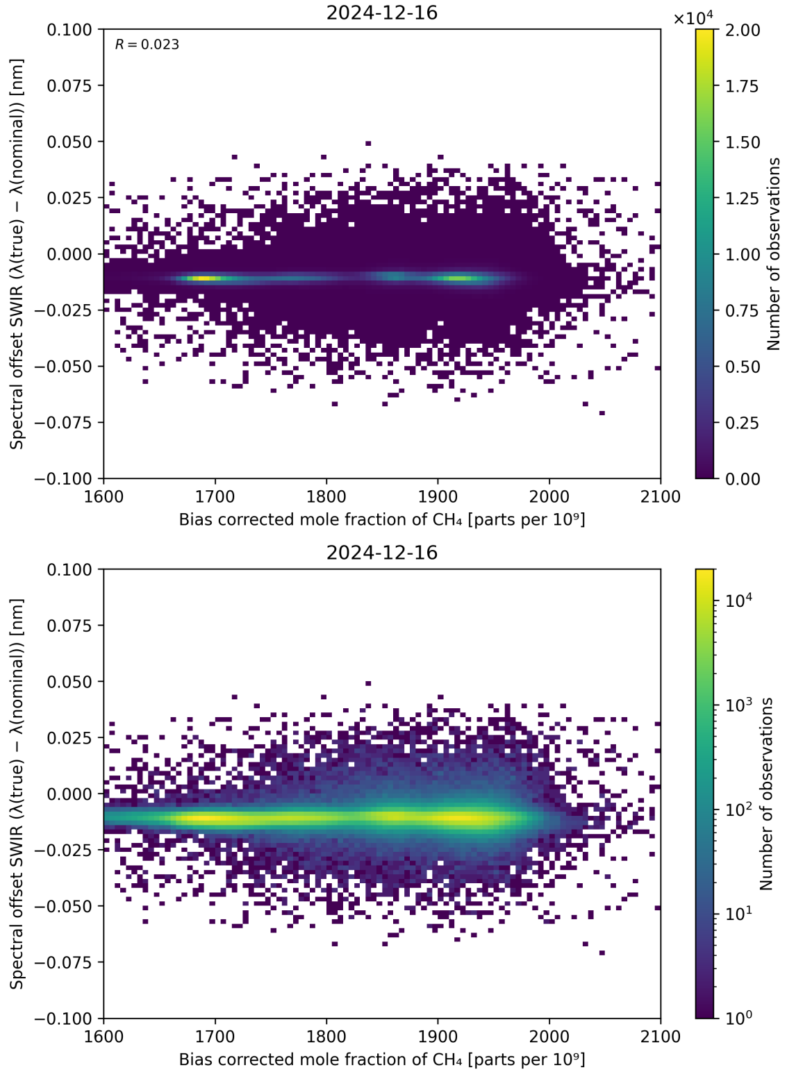
Figure 69: Scatter density plot of “Bias corrected mole fraction of \text{CH}_4 ” against “Spectral offset SWIR ( \lambda_{\text{true}} - \lambda_{\text{nominal}} )” for 2024-12-16 to 2024-12-17.
