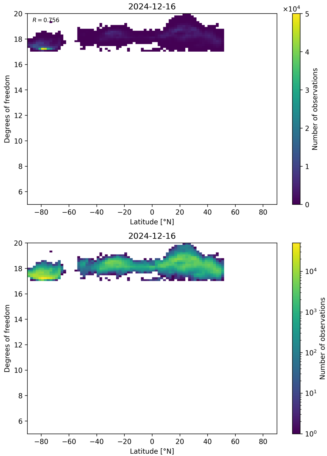
Figure 55: Scatter density plot of “Latitude” against “Degrees of freedom” for 2024-12-16 to 2024-12-17.
