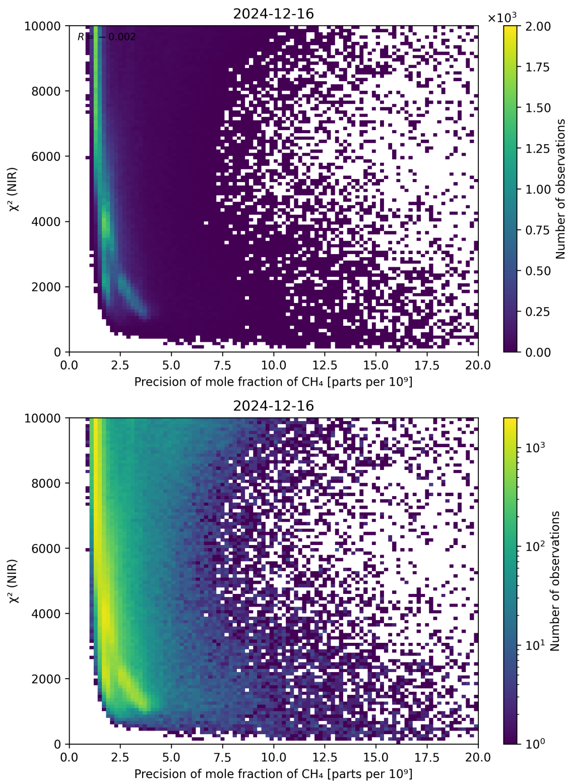
Figure 78: Scatter density plot of “Precision of mole fraction of \text{CH}_4 ” against “ \chi^2 (NIR)” for 2024-12-16 to 2024-12-17.
