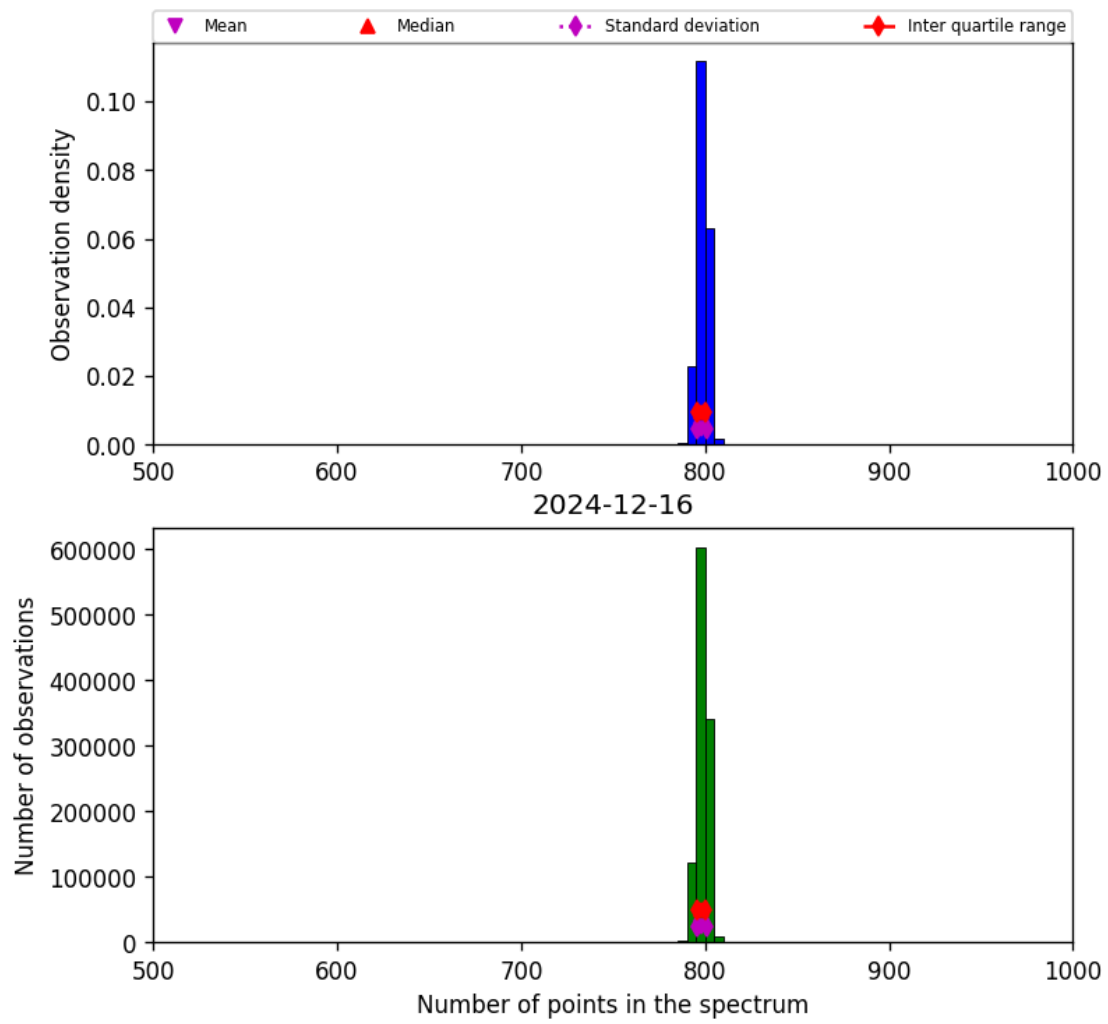
Figure 26: Histogram of “Number of points in the spectrum” for 2024-12-16 to 2024-12-17
