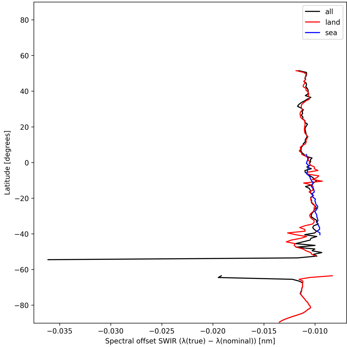
Figure 16: Zonal average of “Spectral offset SWIR ( \lambda_{\text{true}} - \lambda_{\text{nominal}} )” for 2024-12-16 to 2024-12-17.
