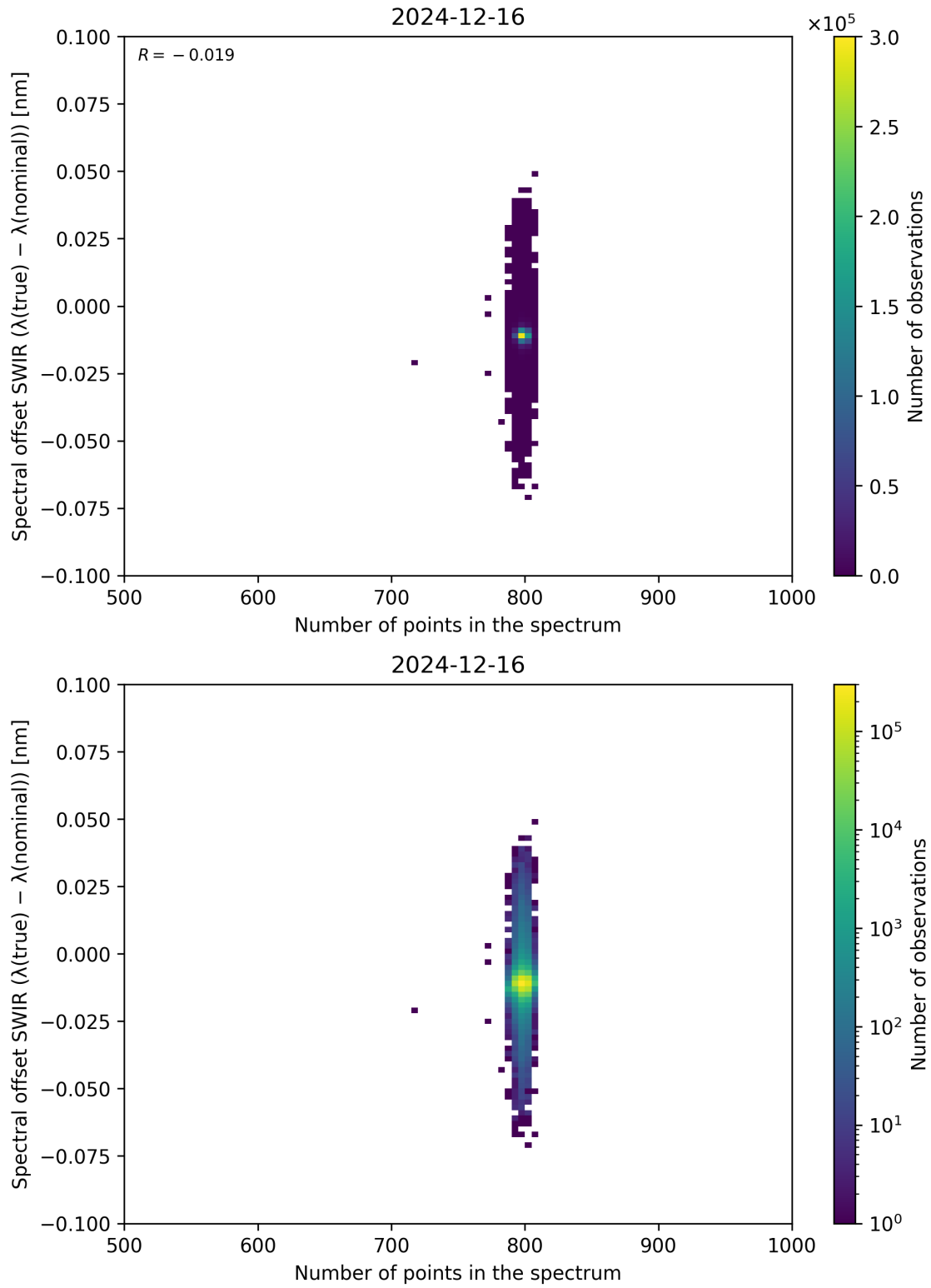
Figure 93: Scatter density plot of “Number of points in the spectrum” against “Spectral offset SWIR ( \lambda_{\text{true}} - \lambda_{\text{nominal}} )” for 2024-12-16 to 2024-12-17.
