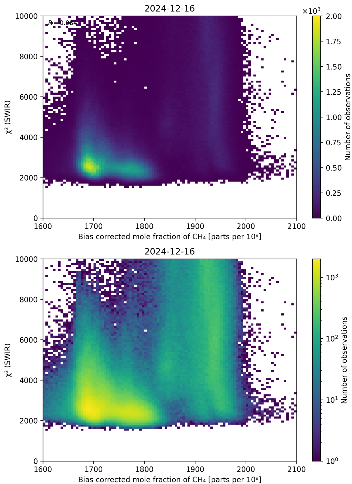
Figure 64: Scatter density plot of “Bias corrected mole fraction of \text{CH}_4 ” against “ \chi^2 (SWIR)” for 2024-12-16 to 2024-12-17.
