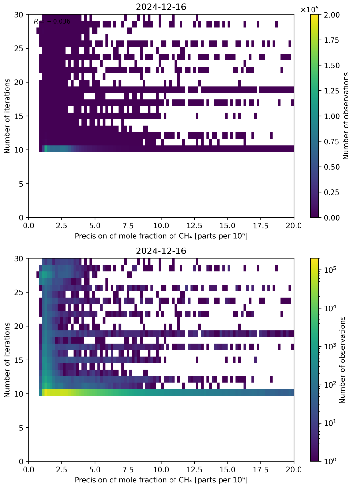
Figure 83: Scatter density plot of “Precision of mole fraction of CH 4 ” against “Number of iterations” for 2024-12-16 to 2024-12-17.
