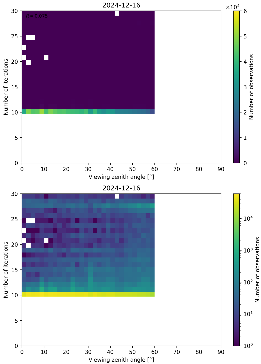
Figure 113: Scatter density plot of “Viewing zenith angle” against “Number of iterations” for 2024-12-16 to 2024-12-17.
