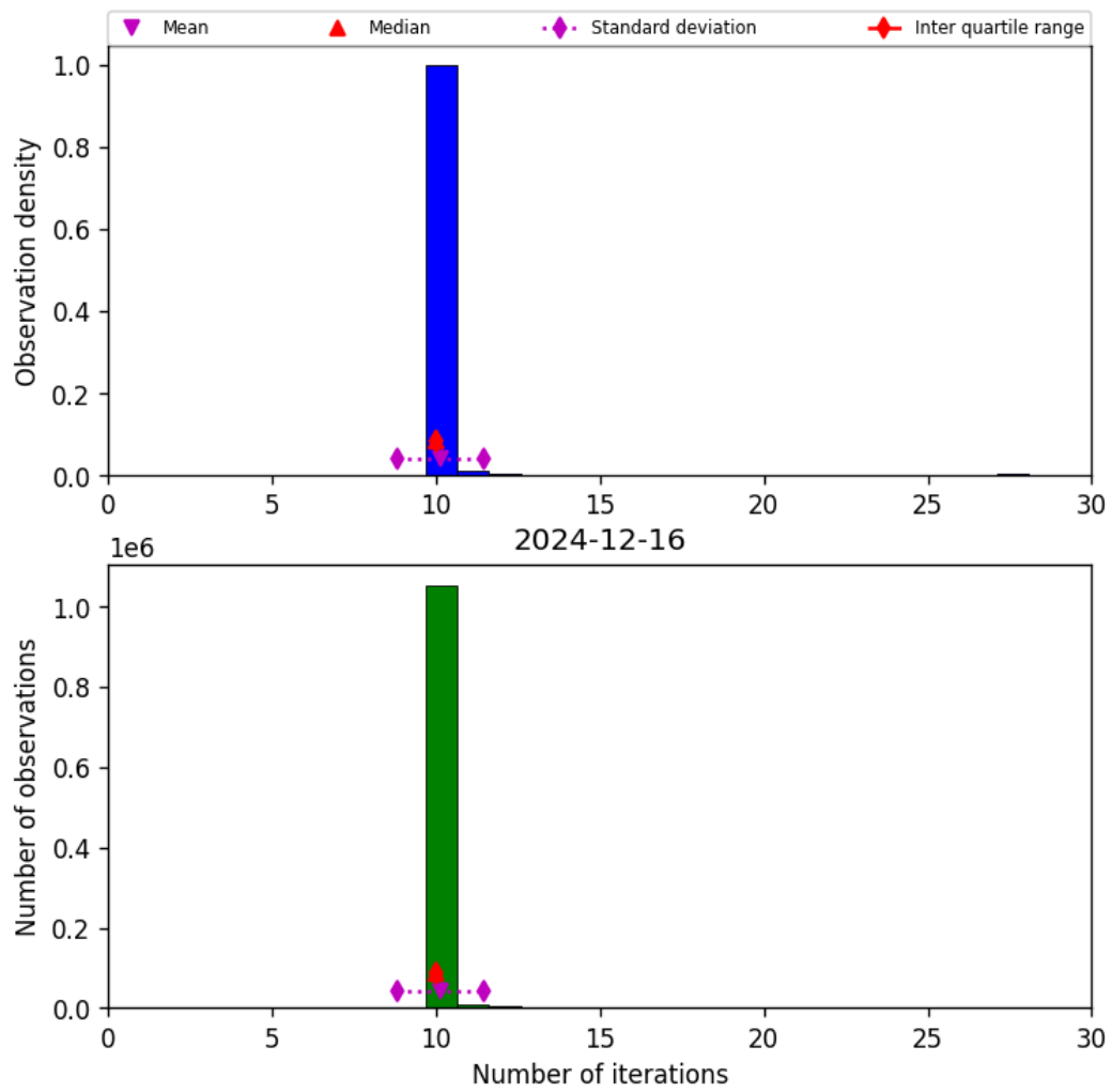
Figure 31: Histogram of “Number of iterations” for 2024-12-16 to 2024-12-17
