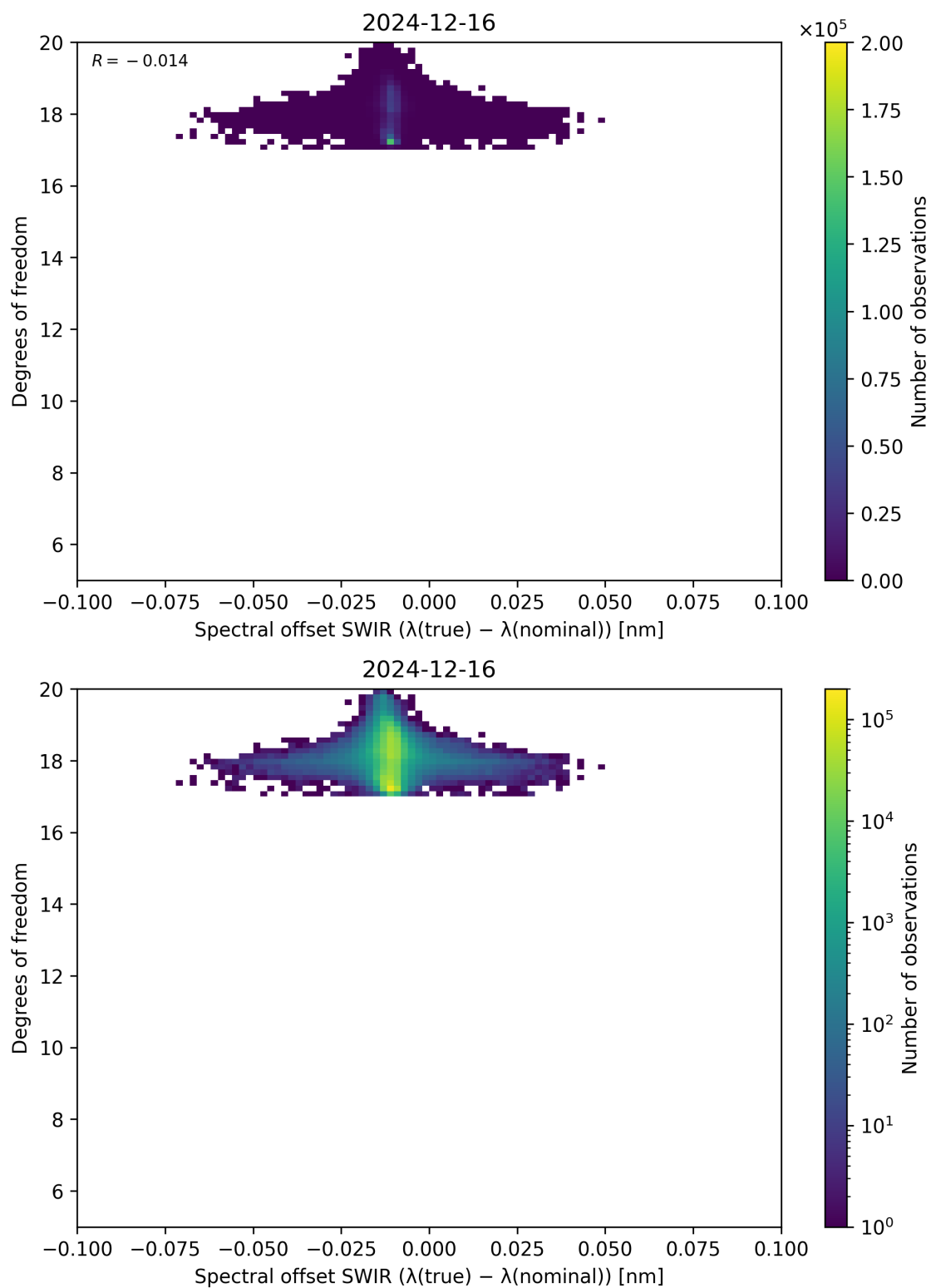
Figure 119: Scatter density plot of “Spectral offset SWIR ( \lambda_{\text{true}} - \lambda_{\text{nominal}} )” against “Degrees of freedom” for 2024-12-16 to 2024-12-17.
