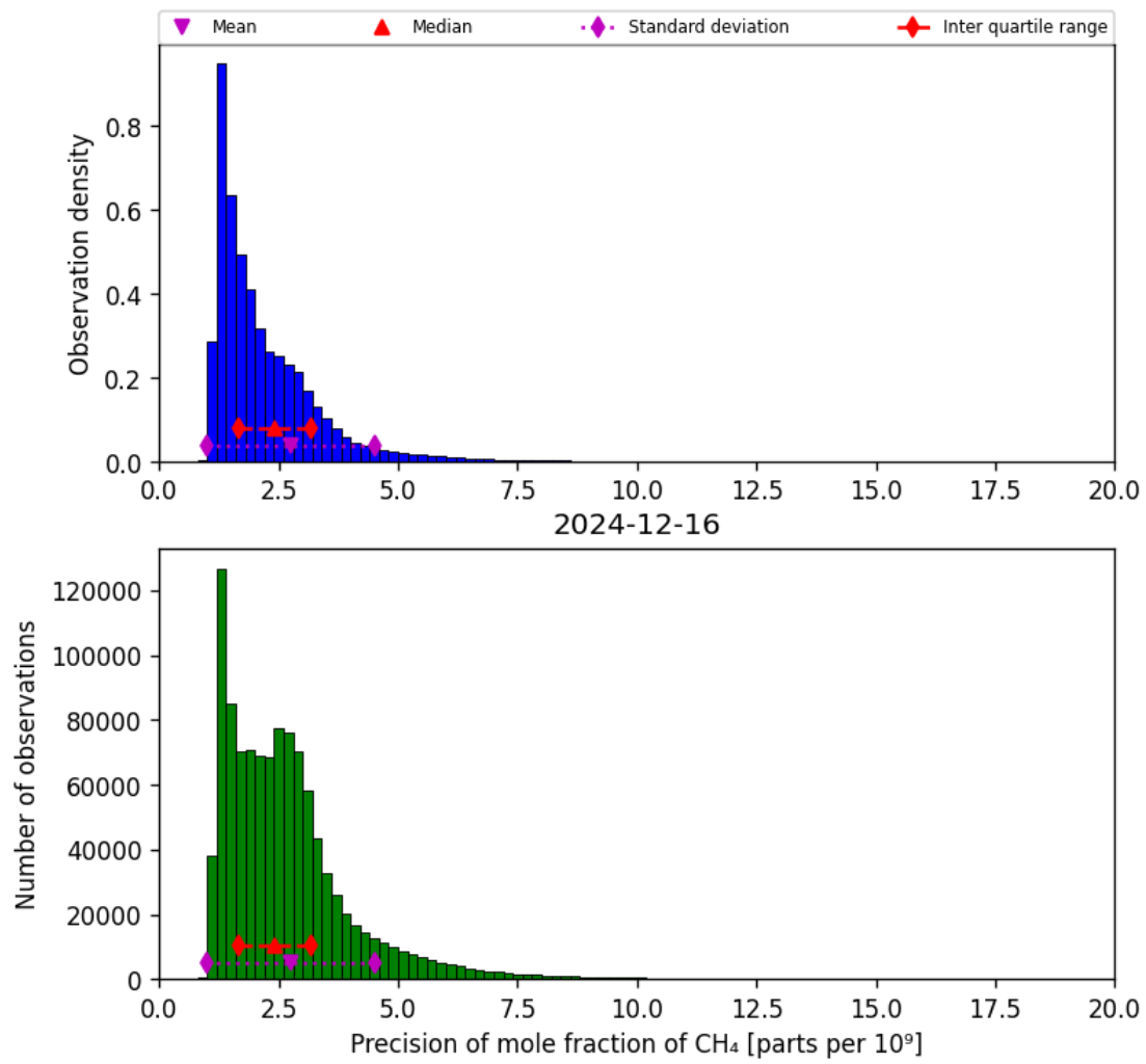
Figure 24: Histogram of “Precision of mole fraction of CH 4 ” for 2024-12-16 to 2024-12-17
