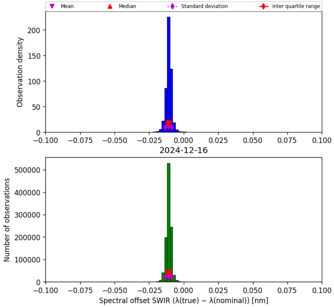
Figure 27: Histogram of “Spectral offset SWIR ( \lambda_{\text{true}} - \lambda_{\text{nominal}} )” for 2024-12-16 to 2024-12-17
