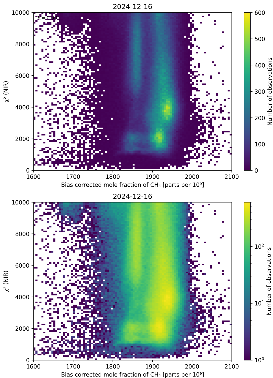
Figure 63: Scatter density plot of “Bias corrected mole fraction of \text{CH}_4 ” against “ \chi^2 (NIR)” for 2024-12-16 to 2024-12-17.
