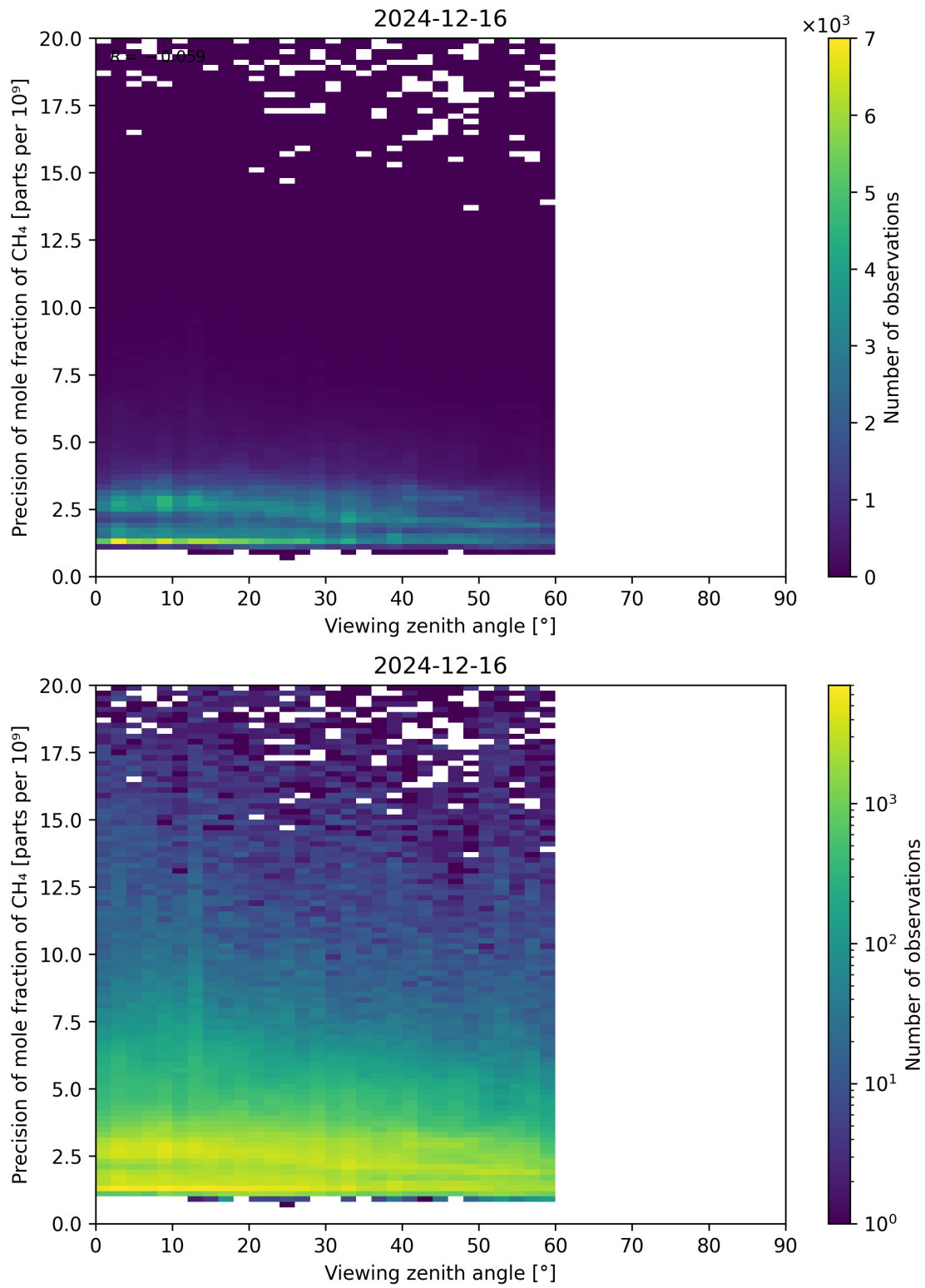
Figure 112: Scatter density plot of “Viewing zenith angle” against “Precision of mole fraction of CH 4 ” for 2024-12-16 to 2024-12-17.
