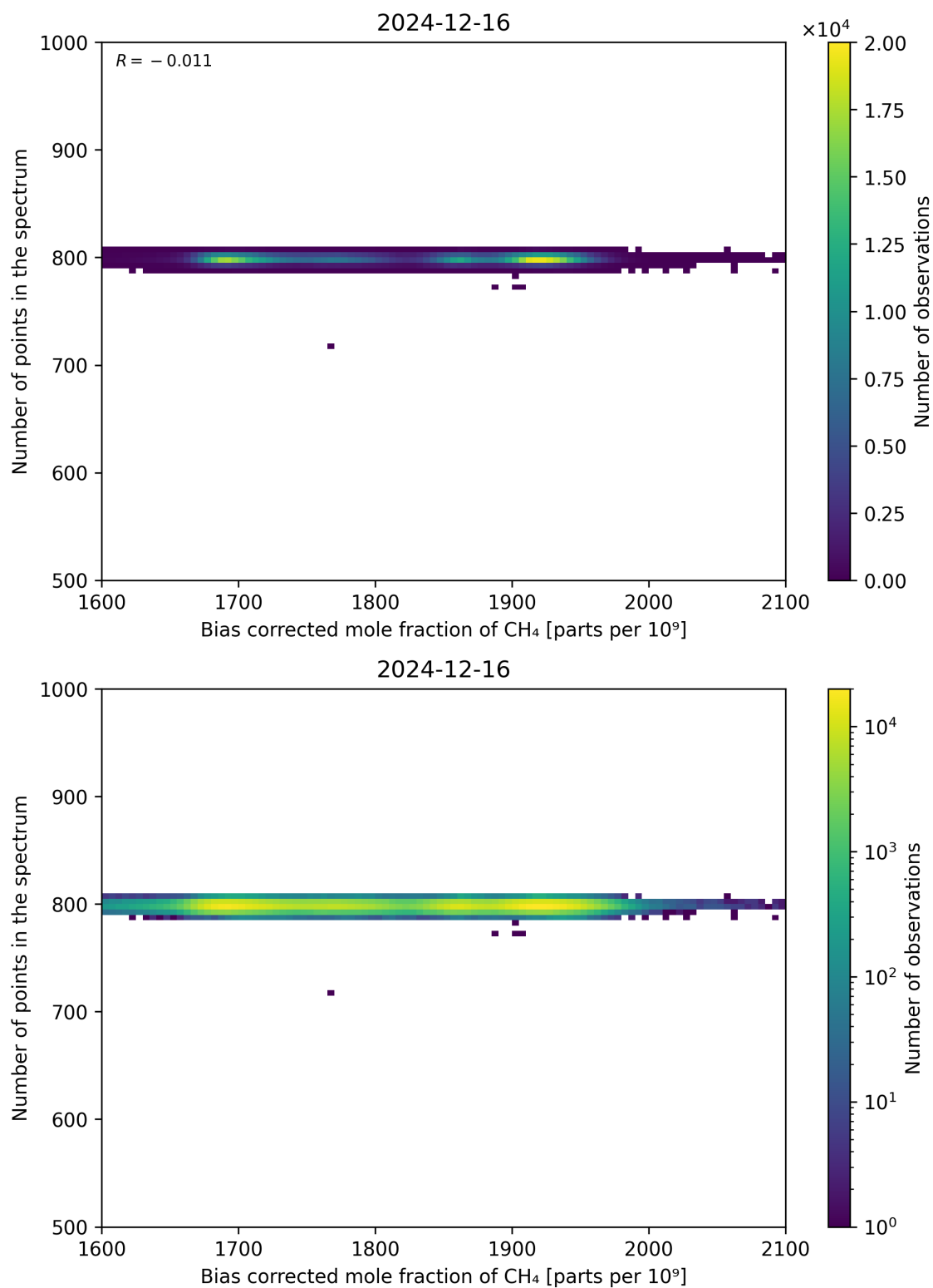
Figure 68: Scatter density plot of “Bias corrected mole fraction of CH 4 ” against “Number of points in the spectrum” for 2024-12-16 to 2024-12-17.
