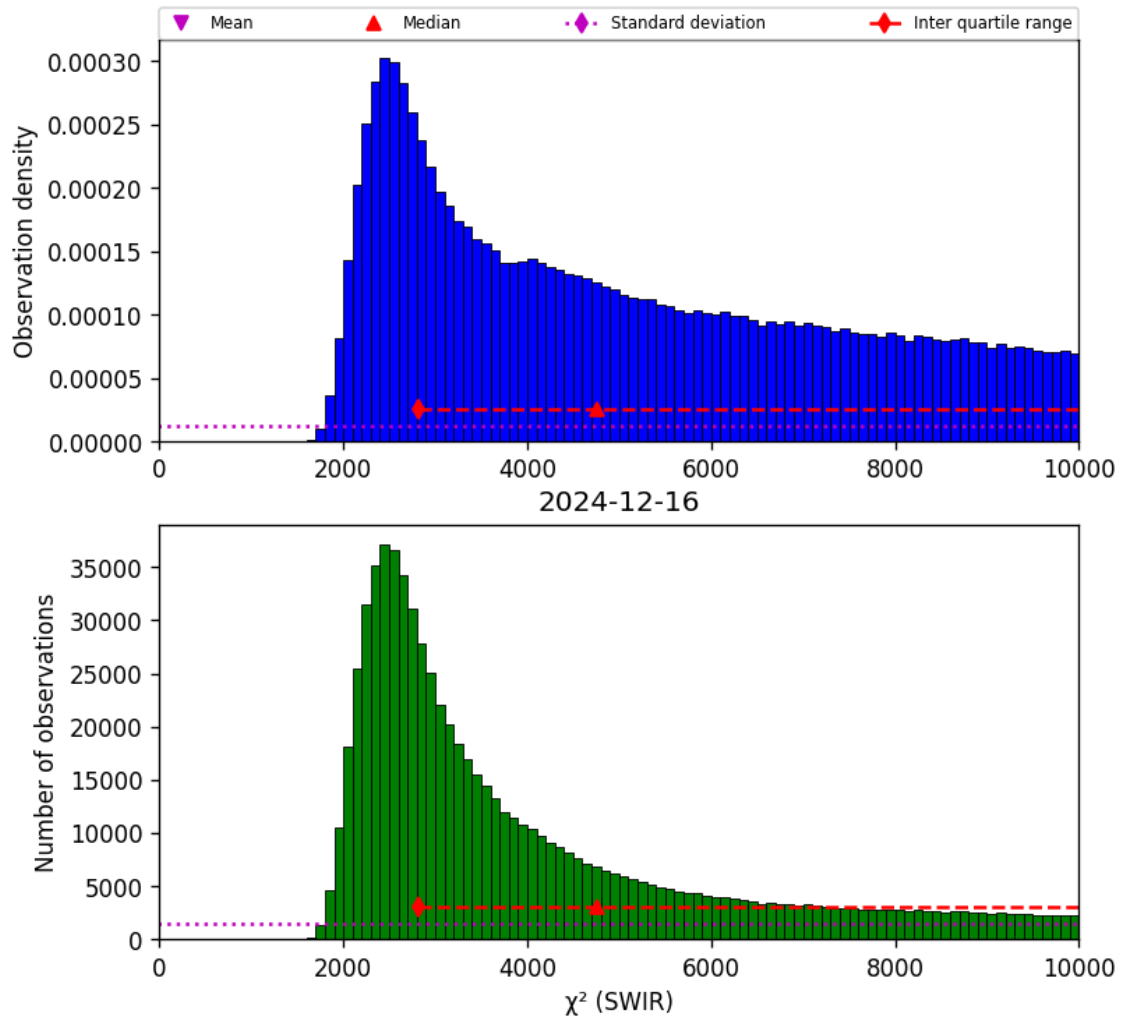
Figure 28: Histogram of “ \chi^2 (SWIR)” for 2024-12-16 to 2024-12-17
