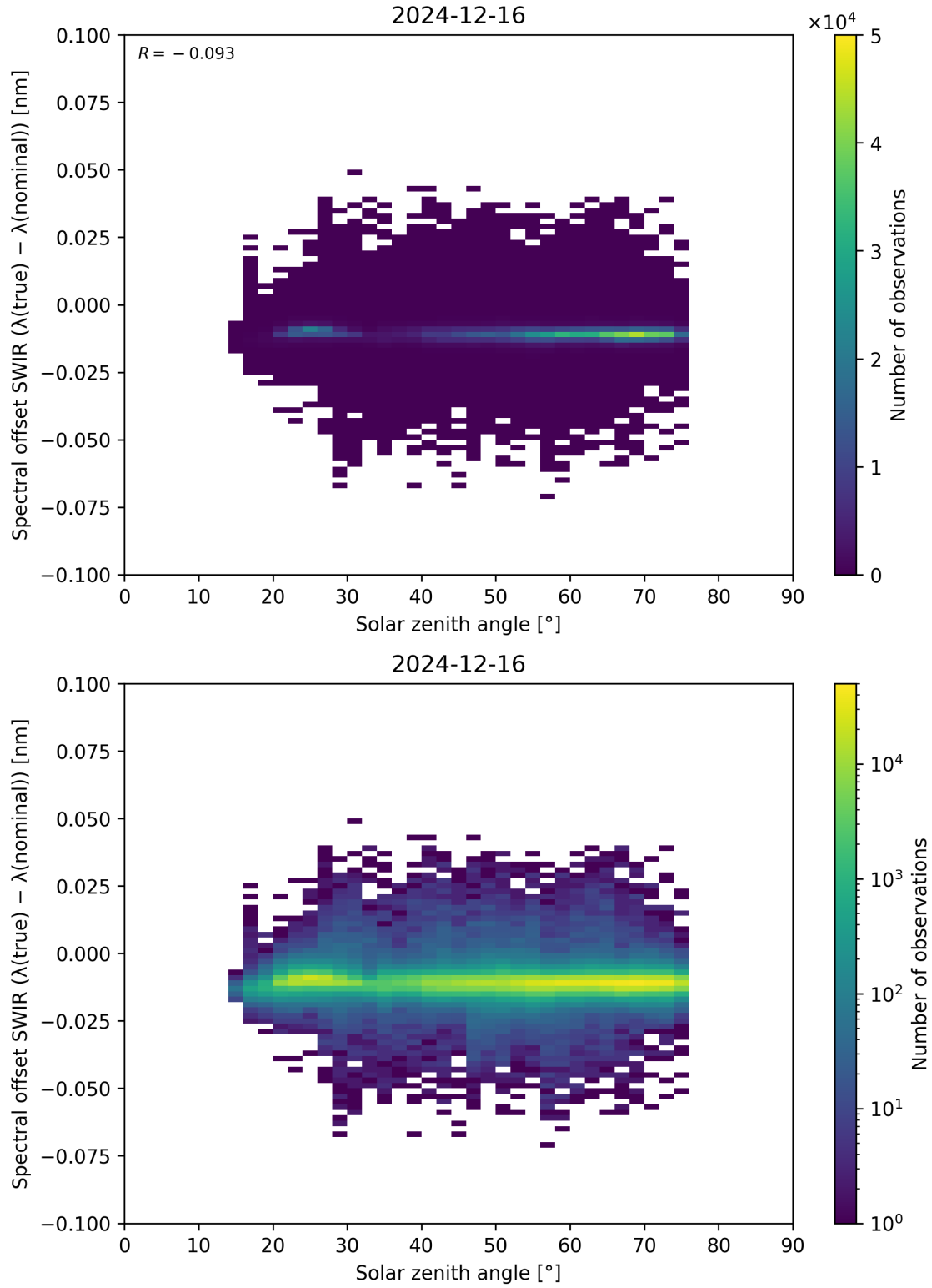
Figure 104: Scatter density plot of “Solar zenith angle” against “Spectral offset SWIR ( \lambda_{\text{true}} - \lambda_{\text{nominal}} )” for 2024-12-16 to 2024-12-17.
