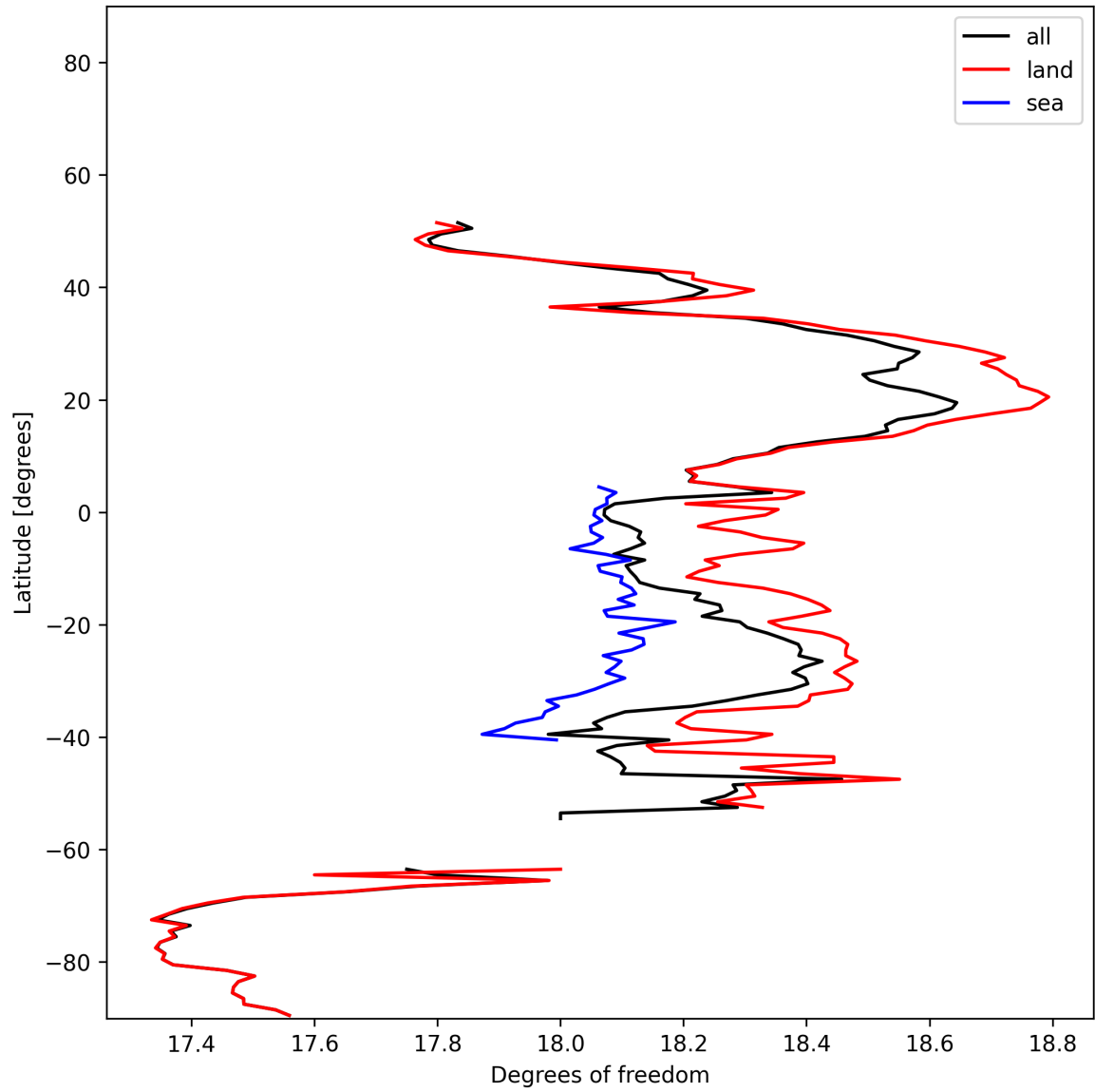
Figure 19: Zonal average of “Degrees of freedom” for 2024-12-16 to 2024-12-17.
