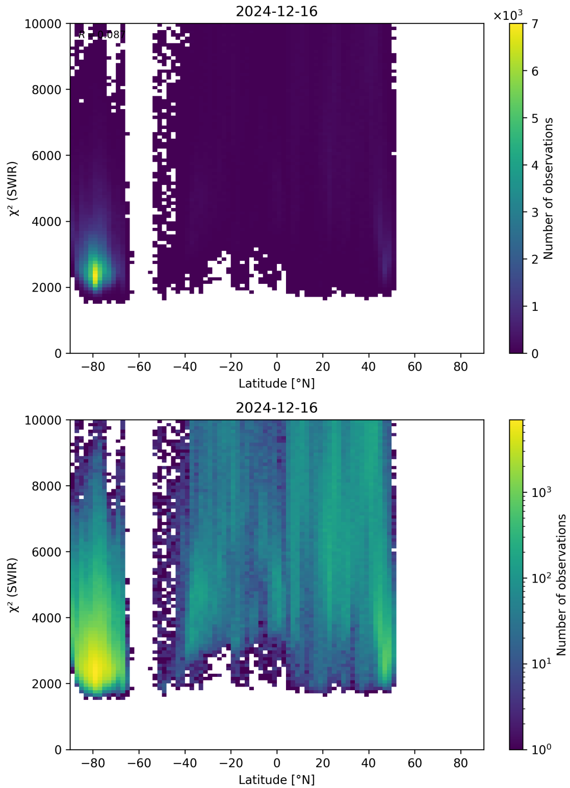
Figure 54: Scatter density plot of “Latitude” against “ \chi^2 (SWIR)” for 2024-12-16 to 2024-12-17.
