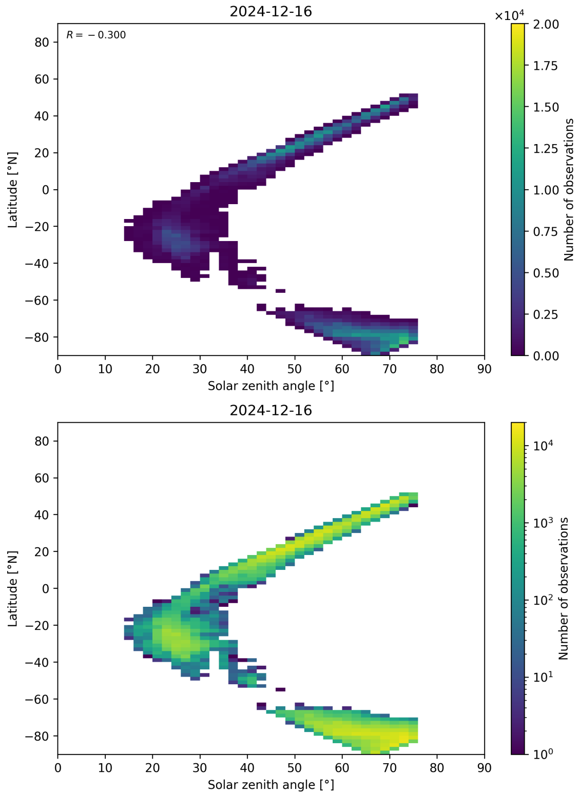
Figure 98: Scatter density plot of “Solar zenith angle” against “Latitude” for 2024-12-16 to 2024-12-17.
