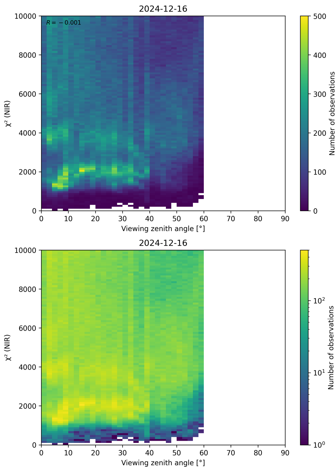
Figure 105: Scatter density plot of “Viewing zenith angle” against “ \chi^2 (NIR)” for 2024-12-16 to 2024-12-17.
