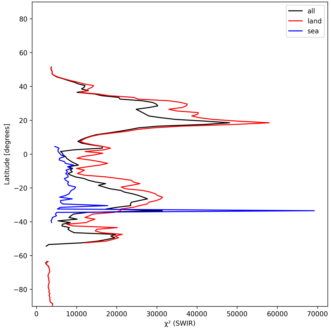
Figure 17: Zonal average of “ \chi^2 (SWIR)” for 2024-12-16 to 2024-12-17.
