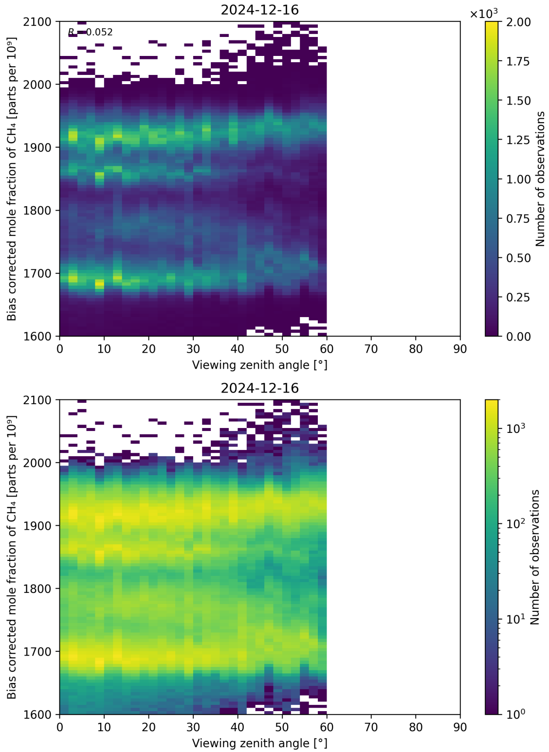
Figure 111: Scatter density plot of “Viewing zenith angle” against “Bias corrected mole fraction of CH 4 ” for 2024-12-16 to 2024-12-17.
