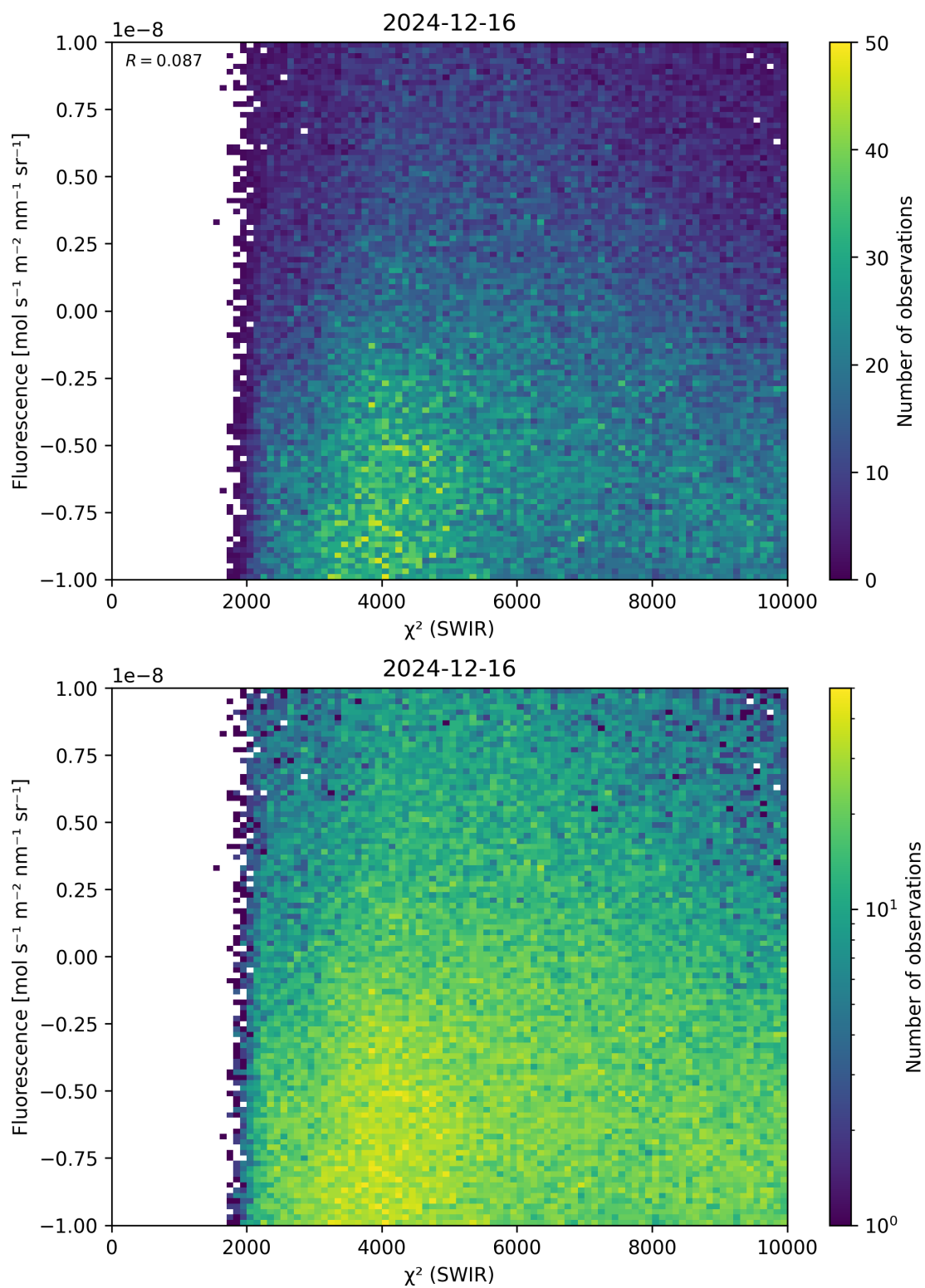
Figure 49: Scatter density plot of “ \chi^2 (SWIR)” against “Fluorescence” for 2024-12-16 to 2024-12-17.
