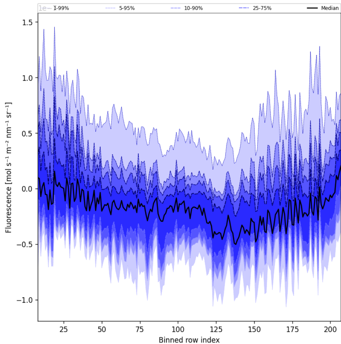
Figure 43: Along track statistics of “Fluorescence” for 2024-12-16 to 2024-12-17
