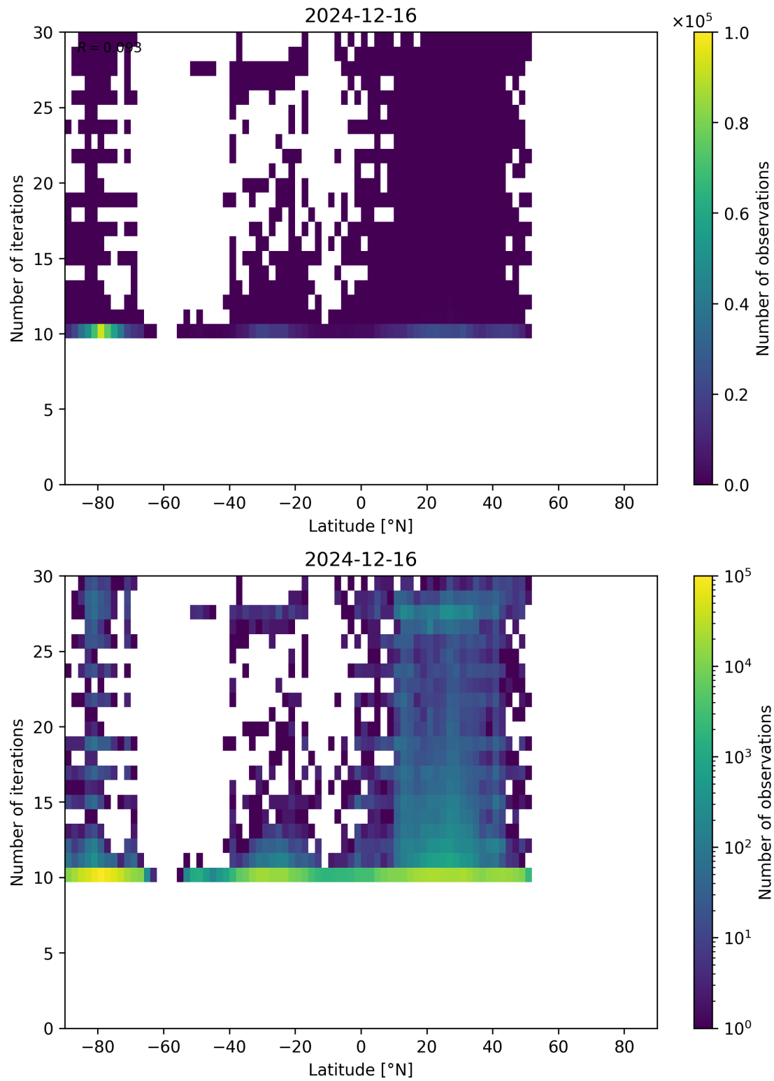
Figure 60: Scatter density plot of “Latitude” against “Number of iterations” for 2024-12-16 to 2024-12-17.
