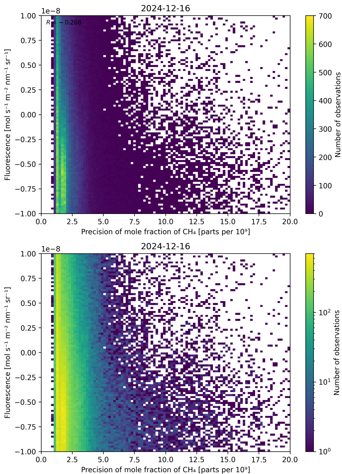
Figure 81: Scatter density plot of “Precision of mole fraction of \text{CH}_4 ” against “Fluorescence” for 2024-12-16 to 2024-12-17.
