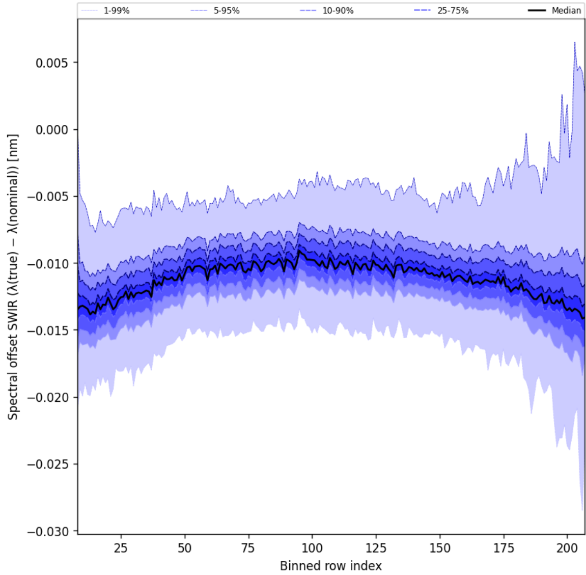
Figure 38: Along track statistics of “Spectral offset SWIR ( \lambda_{\text{true}} - \lambda_{\text{nominal}} )” for 2024-12-16 to 2024-12-17
