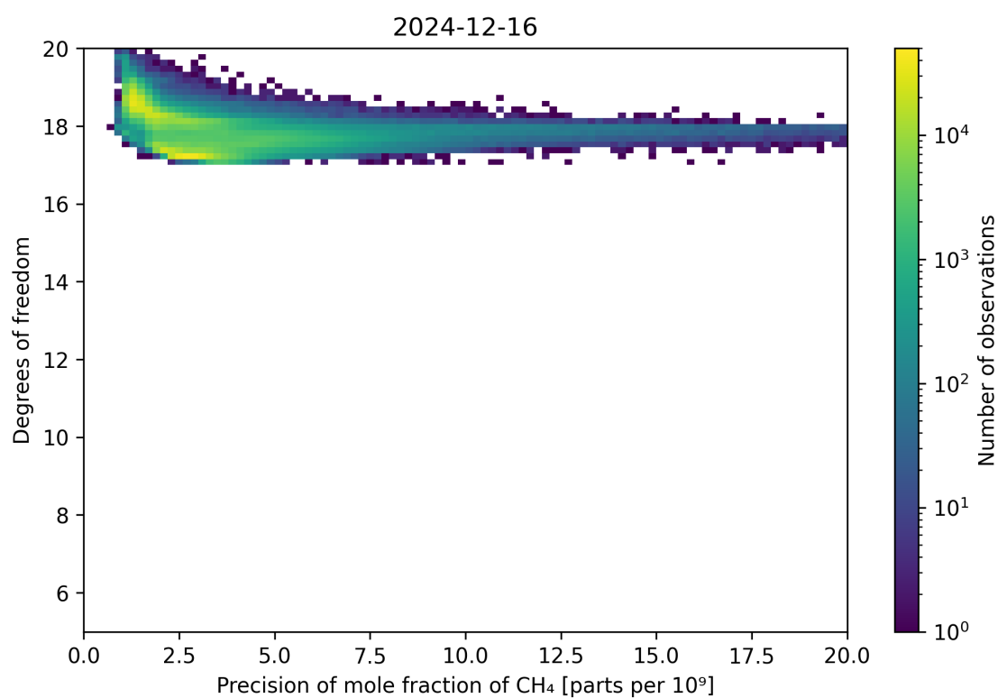
Figure 80: Scatter density plot of “Precision of mole fraction of CH 4 ” against “Degrees of freedom” for 2024-12-16 to 2024-12-17.
