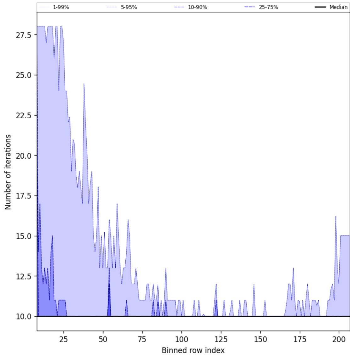
Figure 42: Along track statistics of “Number of iterations” for 2024-12-16 to 2024-12-17
