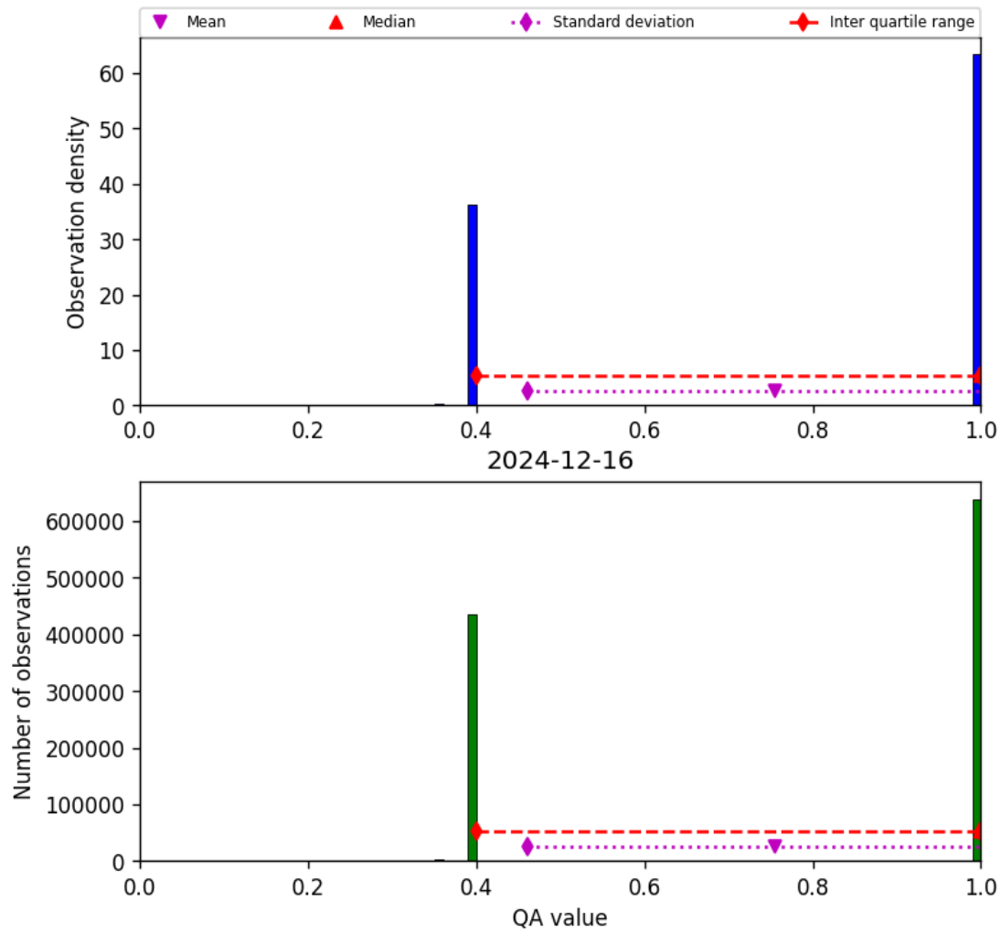
Figure 22: Histogram of “QA value” for 2024-12-16 to 2024-12-17
