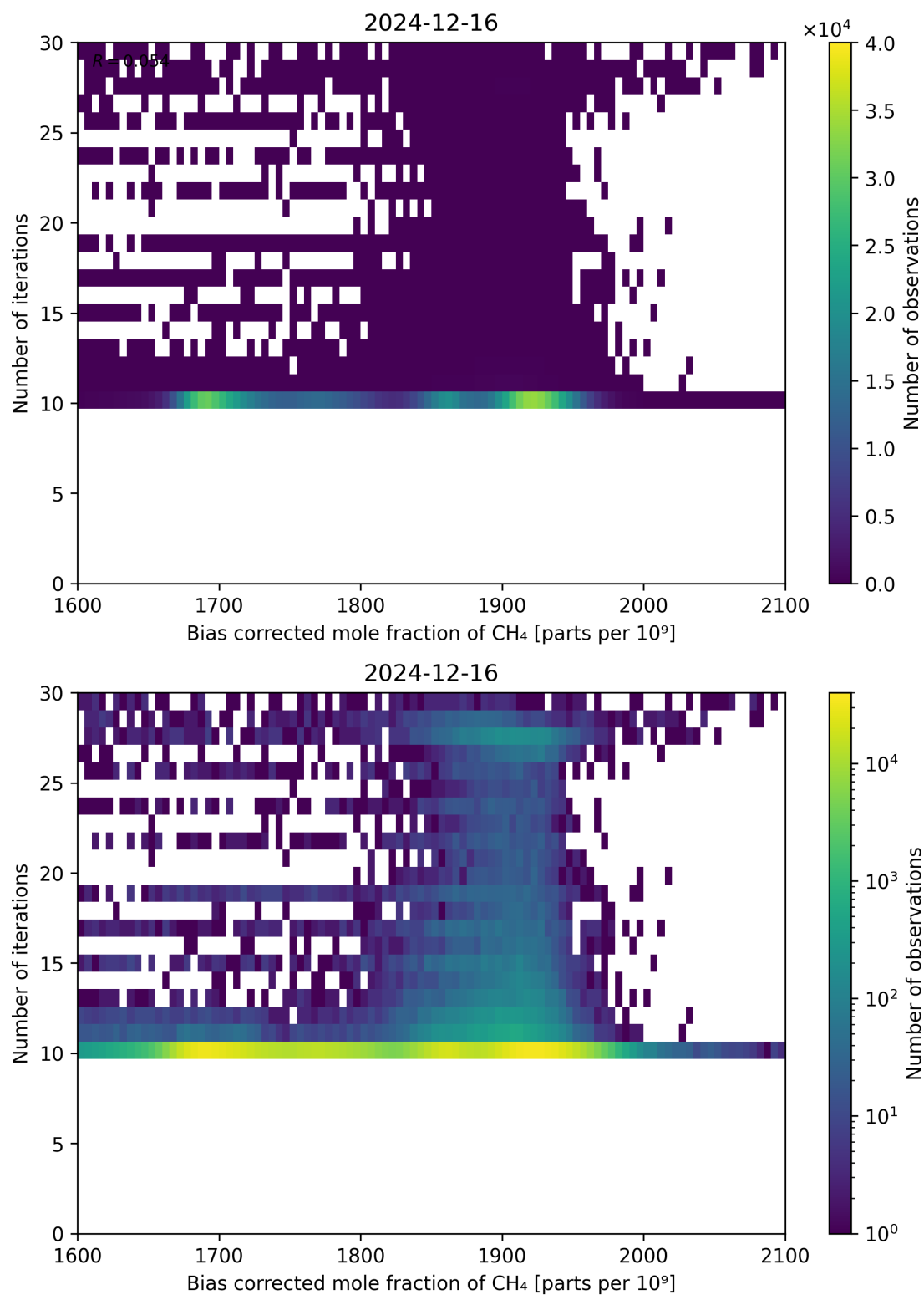
Figure 67: Scatter density plot of “Bias corrected mole fraction of \text{CH}_4 ” against “Number of iterations” for 2024-12-16 to 2024-12-17.
