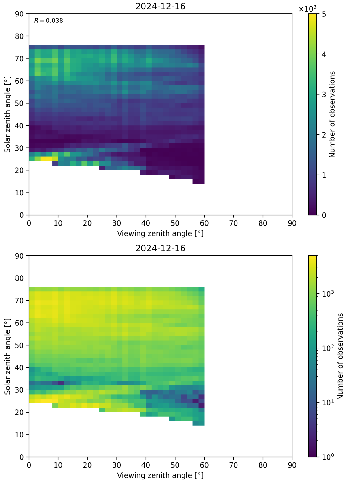
Figure 115: Scatter density plot of “Viewing zenith angle” against “Solar zenith angle” for 2024-12-16 to 2024-12-17.
