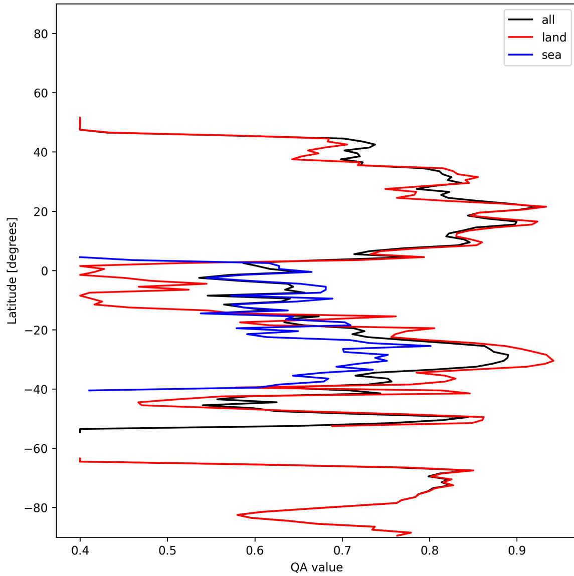
Figure 11: Zonal average of “QA value” for 2024-12-16 to 2024-12-17.
