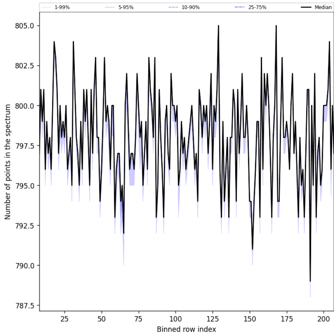
Figure 37: Along track statistics of “Number of points in the spectrum” for 2024-12-16 to 2024-12-17
