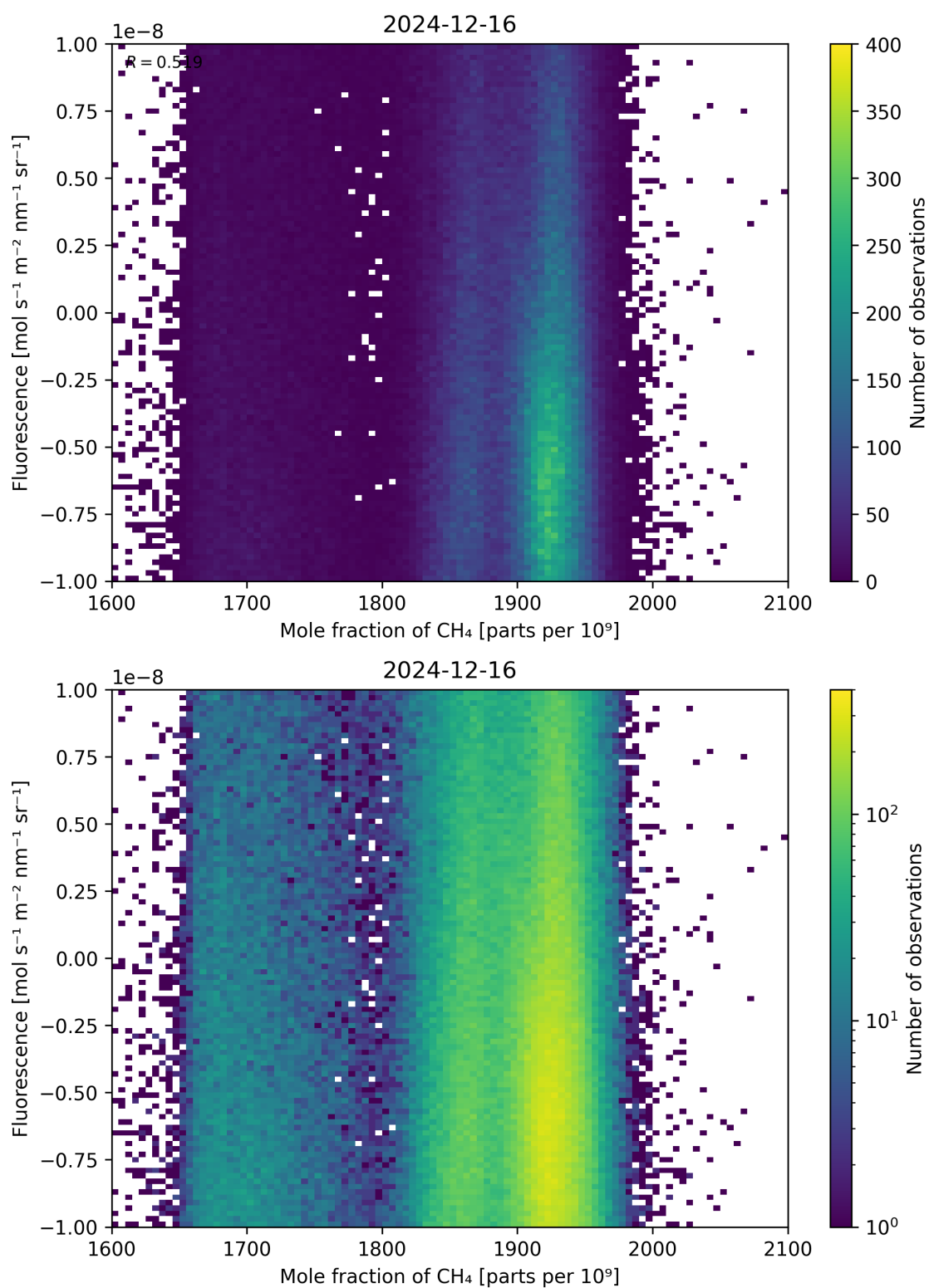
Figure 73: Scatter density plot of “Mole fraction of CH 4 ” against “Fluorescence” for 2024-12-16 to 2024-12-17.
