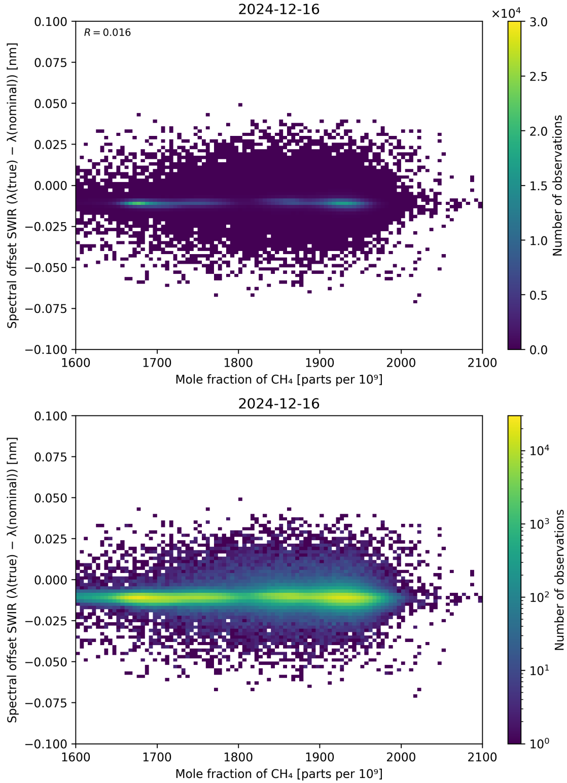
Figure 86: Scatter density plot of “Mole fraction of CH 4 ” against “Spectral offset SWIR ( \lambda_{\text{true}} - \lambda_{\text{nominal}} )” for 2024-12-16 to 2024-12-17.
