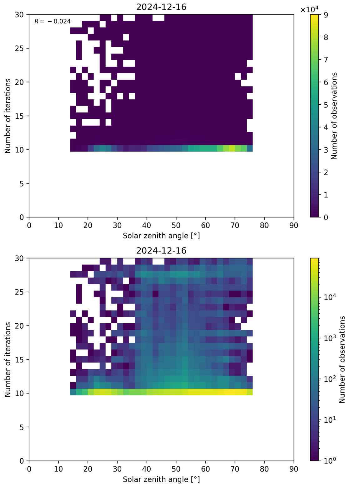
Figure 102: Scatter density plot of “Solar zenith angle” against “Number of iterations” for 2024-12-16 to 2024-12-17.
