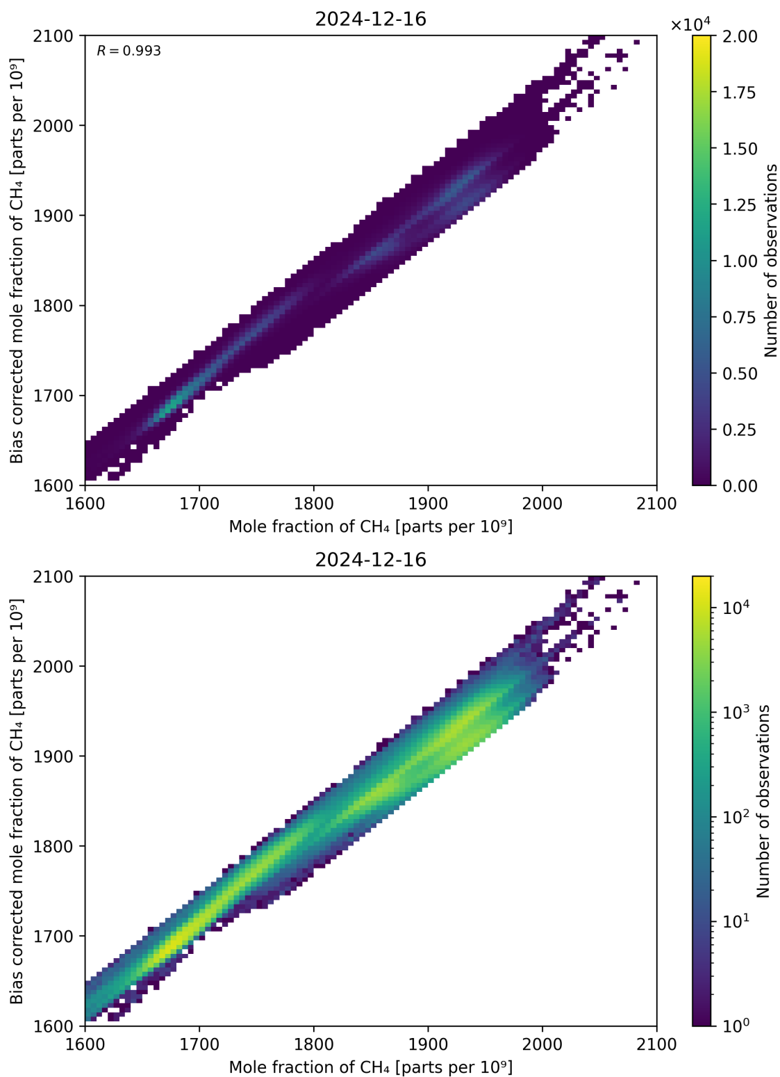
Figure 74: Scatter density plot of “Mole fraction of CH 4 ” against “Bias corrected mole fraction of CH 4 ” for 2024-12-16 to 2024-12-17.
