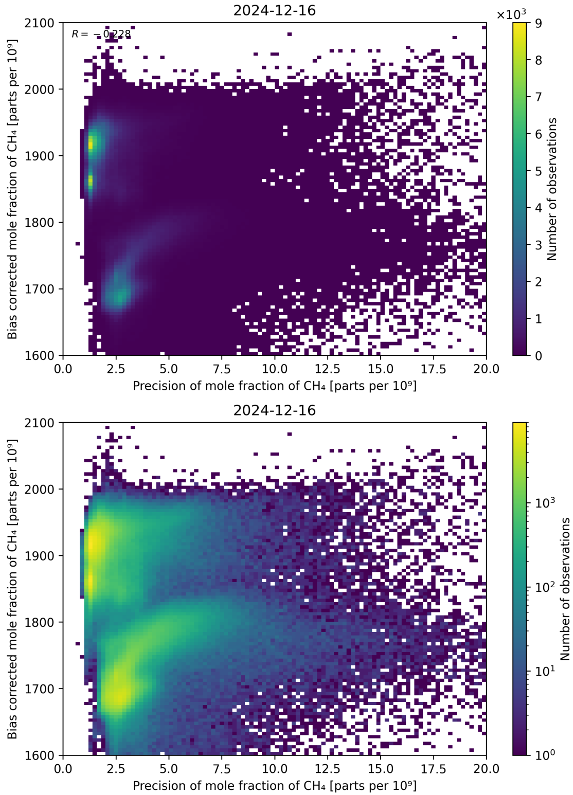
Figure 82: Scatter density plot of “Precision of mole fraction of CH 4 ” against “Bias corrected mole fraction of CH 4 ” for 2024-12-16 to 2024-12-17.
