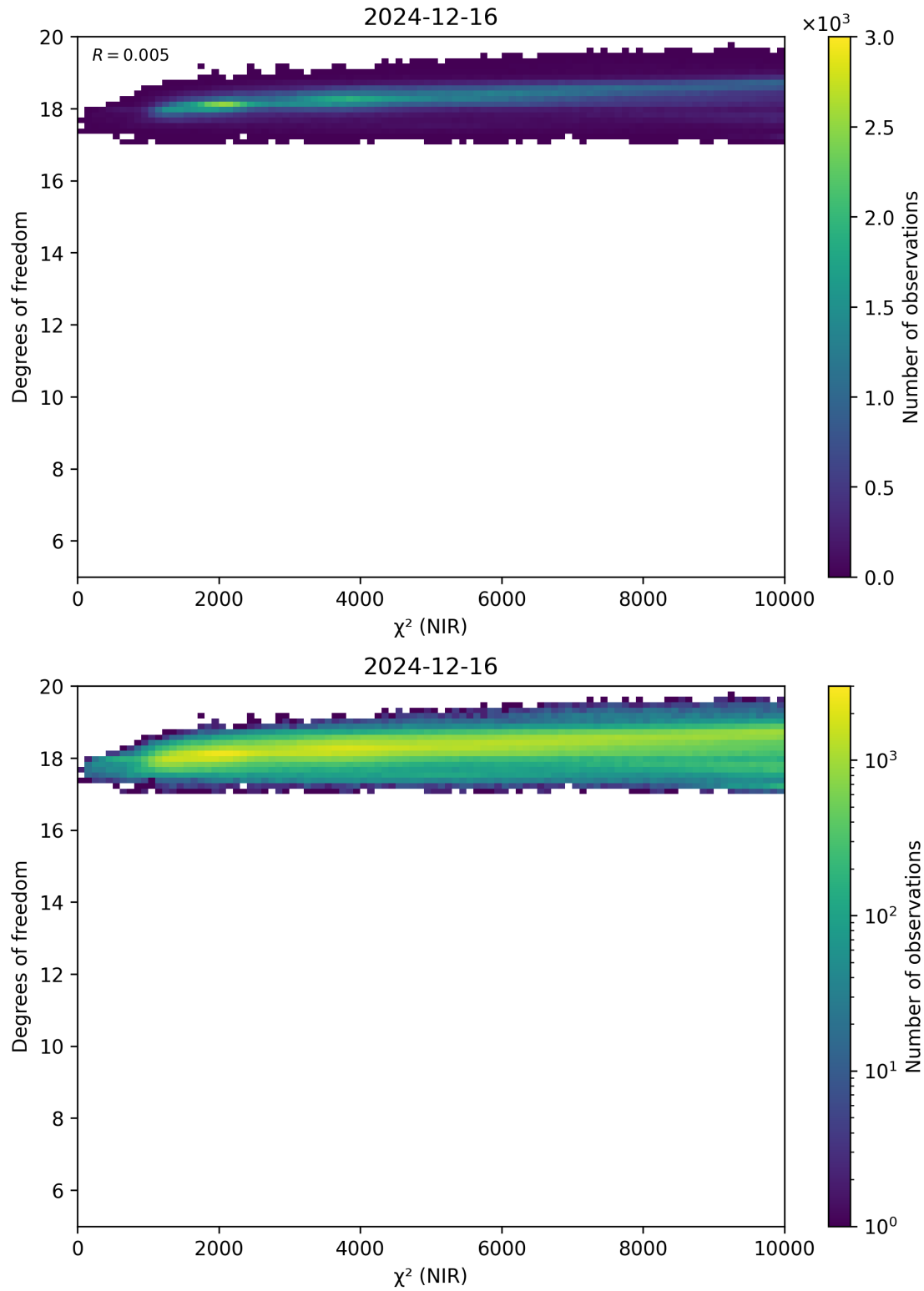
Figure 44: Scatter density plot of “ \chi^2 (NIR)” against “Degrees of freedom” for 2024-12-16 to 2024-12-17.
