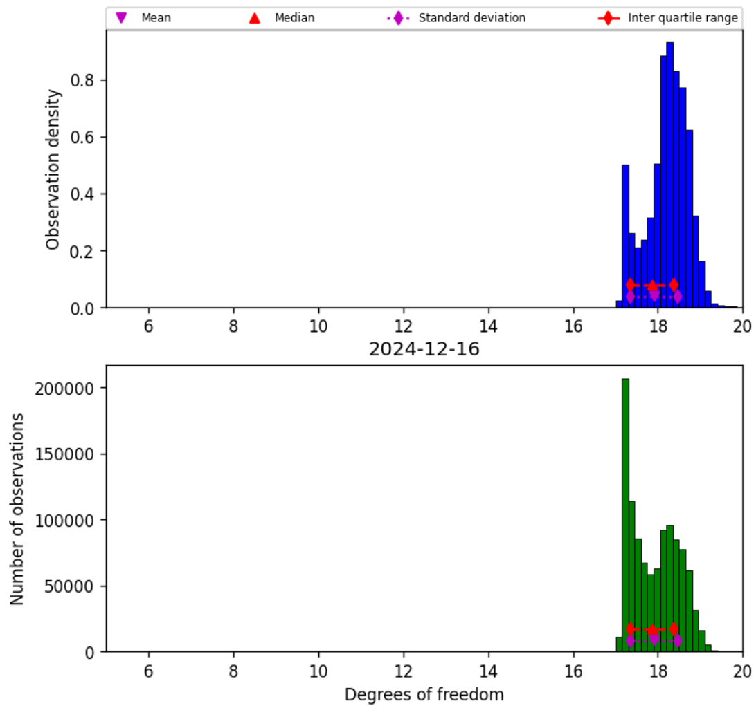
Figure 30: Histogram of “Degrees of freedom” for 2024-12-16 to 2024-12-17
