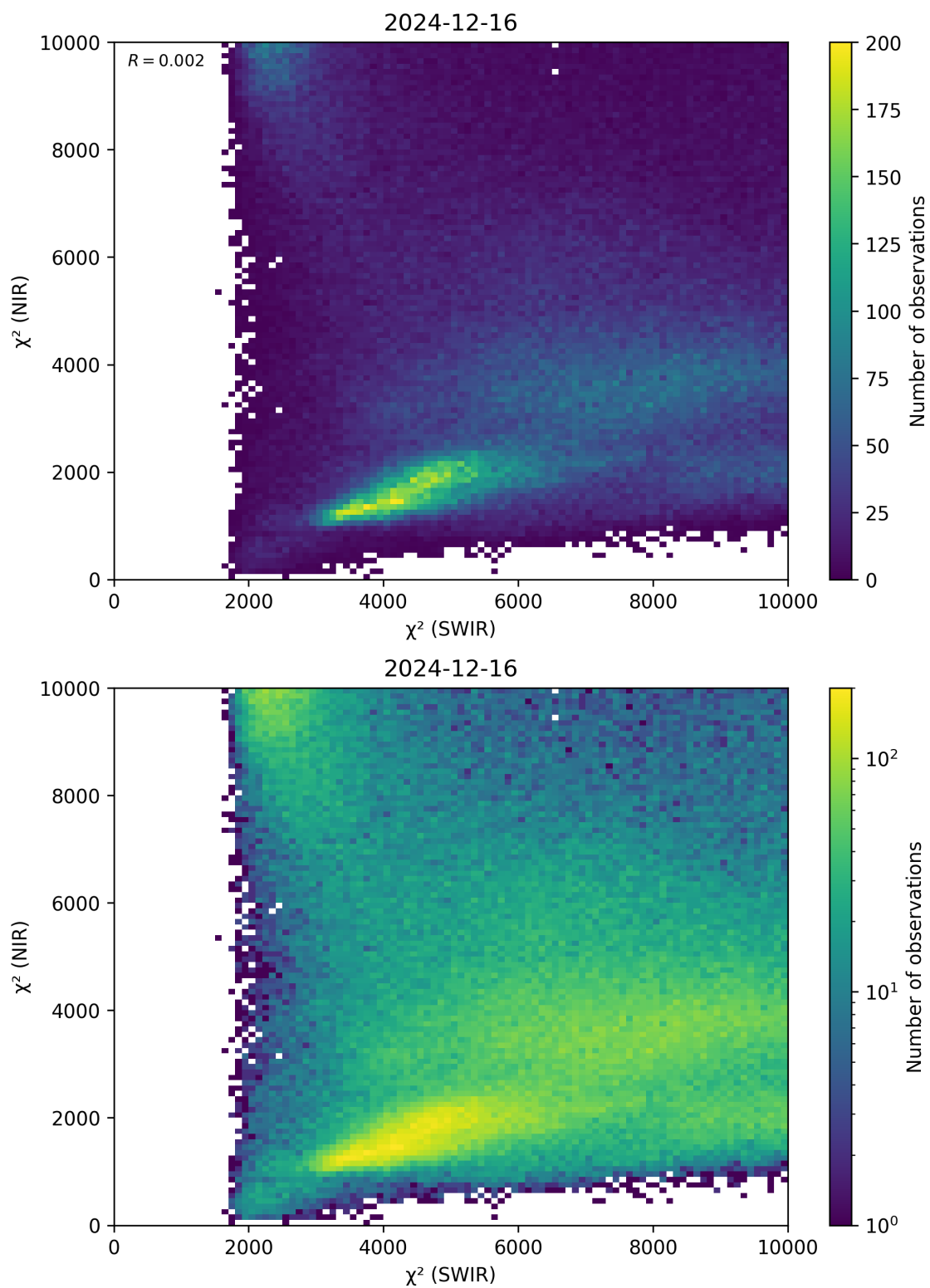
Figure 47: Scatter density plot of “ \chi^2 (SWIR)” against “ \chi^2 (NIR)” for 2024-12-16 to 2024-12-17.
