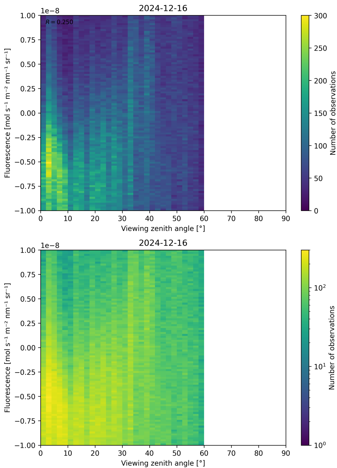
Figure 108: Scatter density plot of “Viewing zenith angle” against “Fluorescence” for 2024-12-16 to 2024-12-17.
