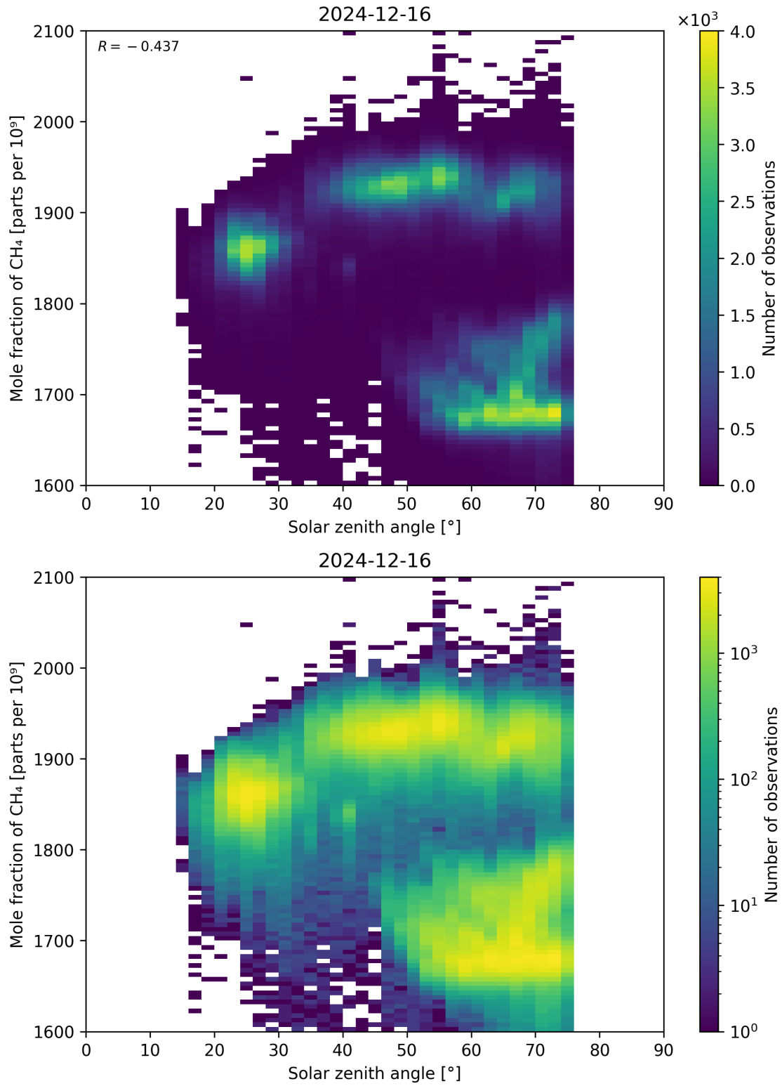
Figure 99: Scatter density plot of “Solar zenith angle” against “Mole fraction of CH 4 ” for 2024-12-16 to 2024-12-17.
