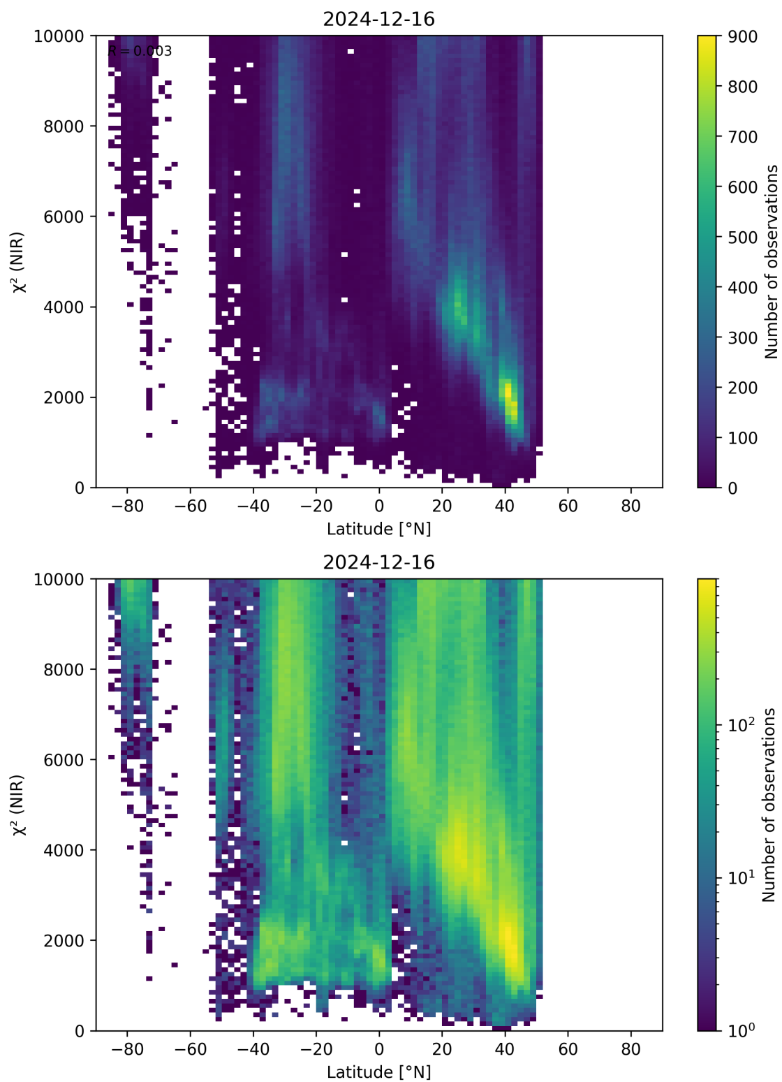
Figure 53: Scatter density plot of “Latitude” against “ \chi^2 (NIR)” for 2024-12-16 to 2024-12-17.
