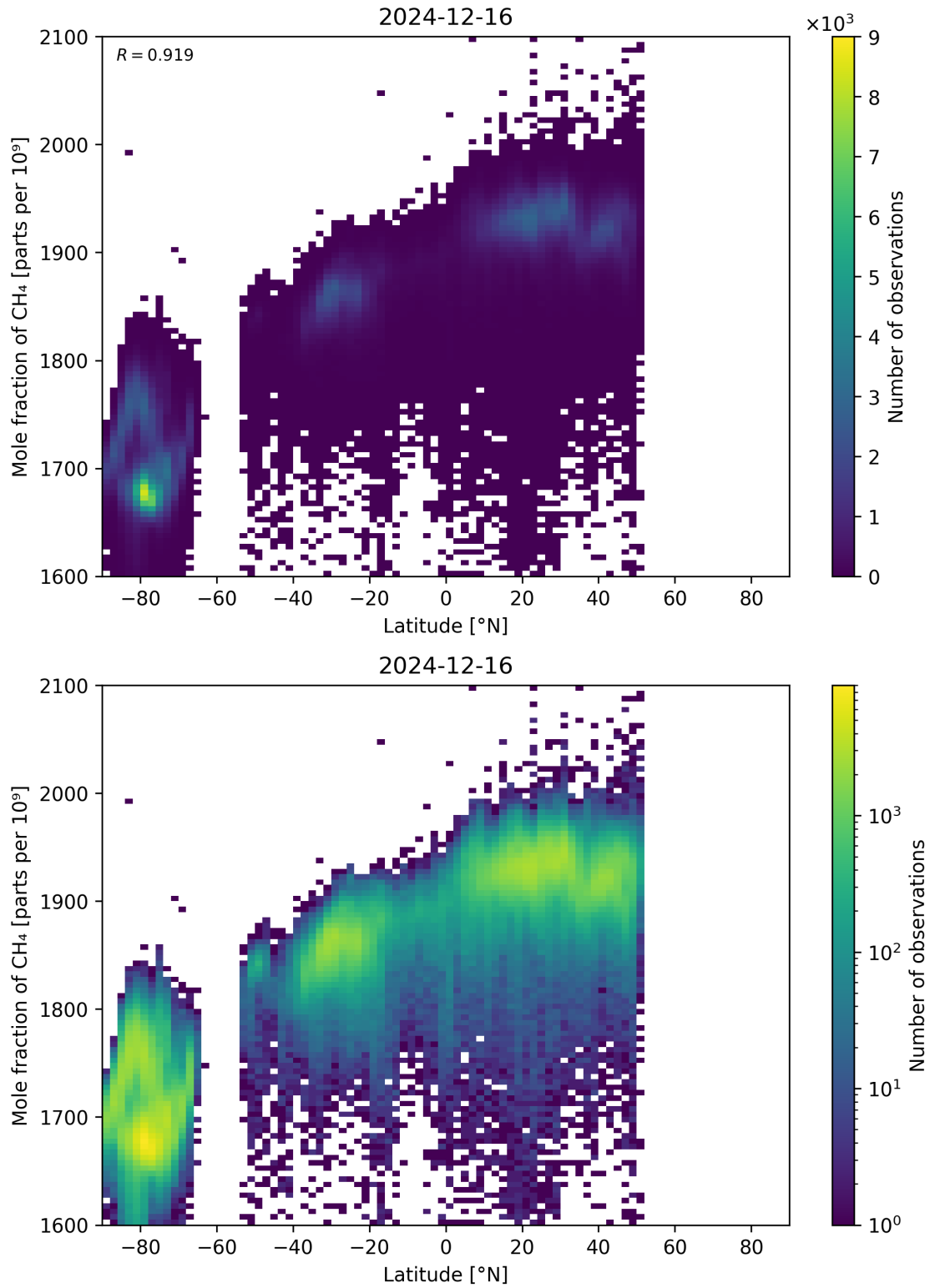
Figure 57: Scatter density plot of “Latitude” against “Mole fraction of CH 4 ” for 2024-12-16 to 2024-12-17.
