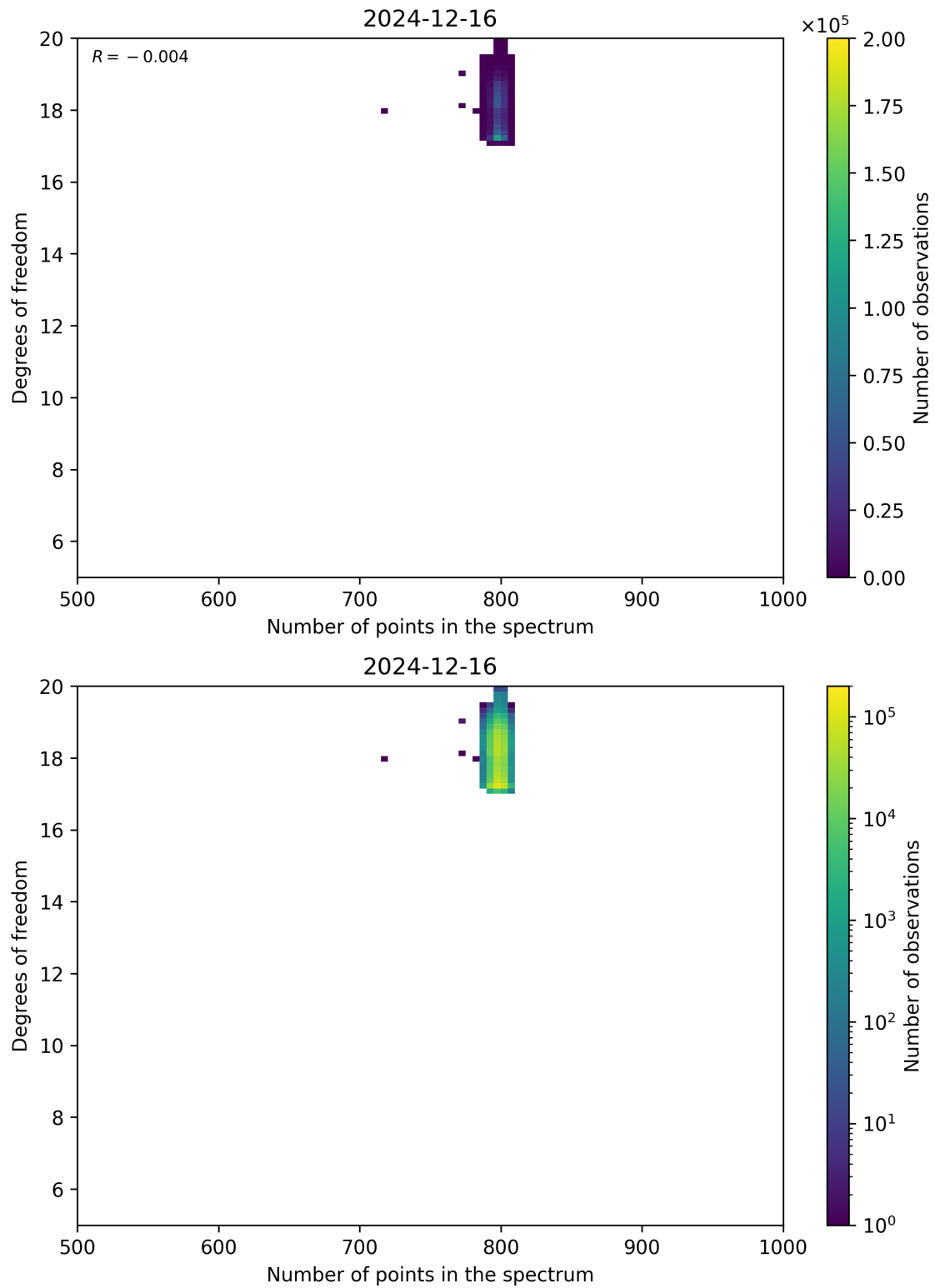
Figure 90: Scatter density plot of “Number of points in the spectrum” against “Degrees of freedom” for 2024-12-16 to 2024-12-17.
