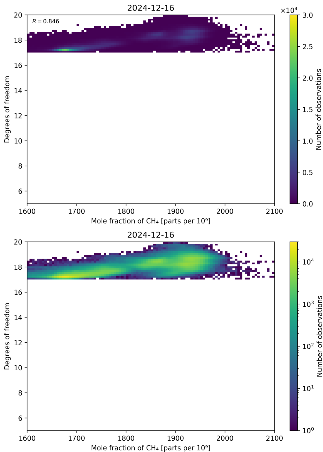
Figure 72: Scatter density plot of “Mole fraction of CH 4 ” against “Degrees of freedom” for 2024-12-16 to 2024-12-17.
