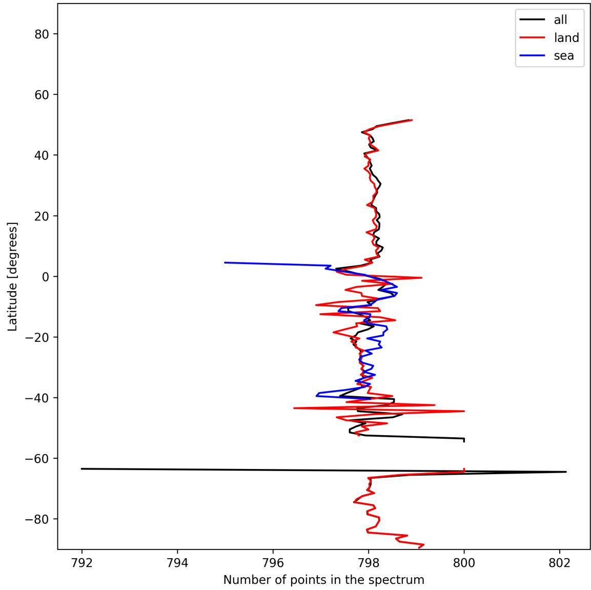
Figure 15: Zonal average of “Number of points in the spectrum” for 2024-12-16 to 2024-12-17.
