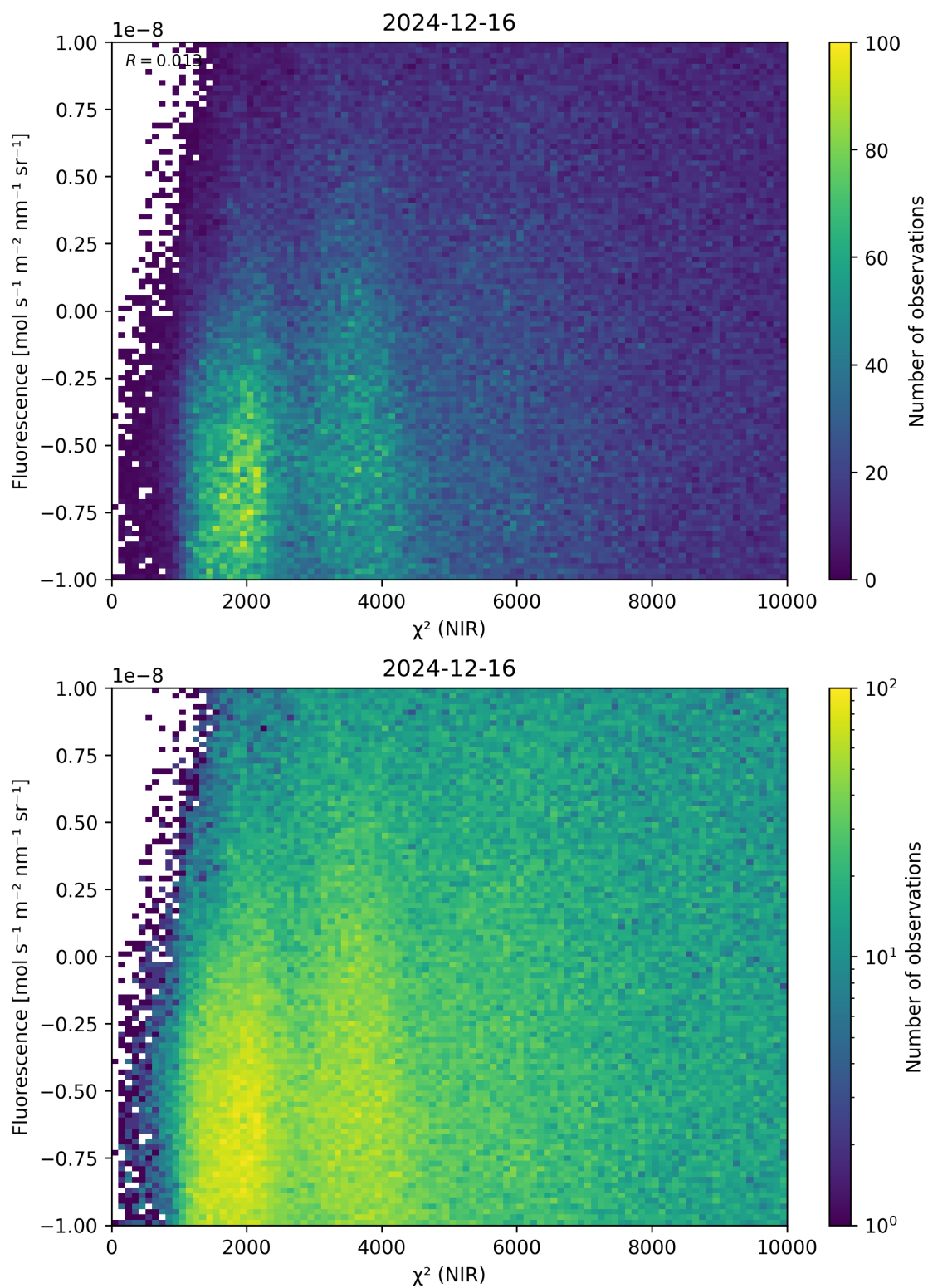
Figure 45: Scatter density plot of “ \chi^2 (NIR)” against “Fluorescence” for 2024-12-16 to 2024-12-17.
