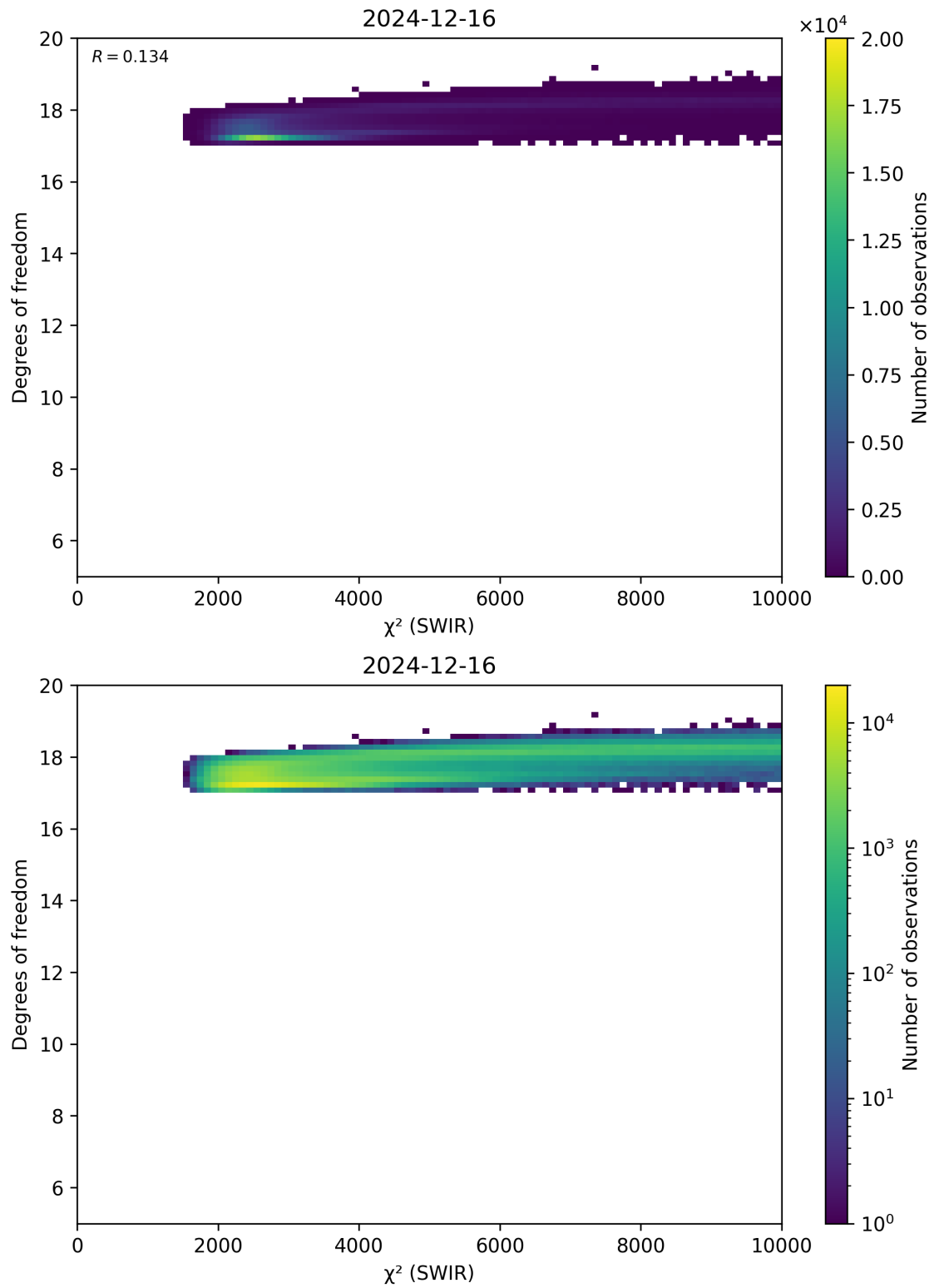
Figure 48: Scatter density plot of “ \chi^2 (SWIR)” against “Degrees of freedom” for 2024-12-16 to 2024-12-17.
