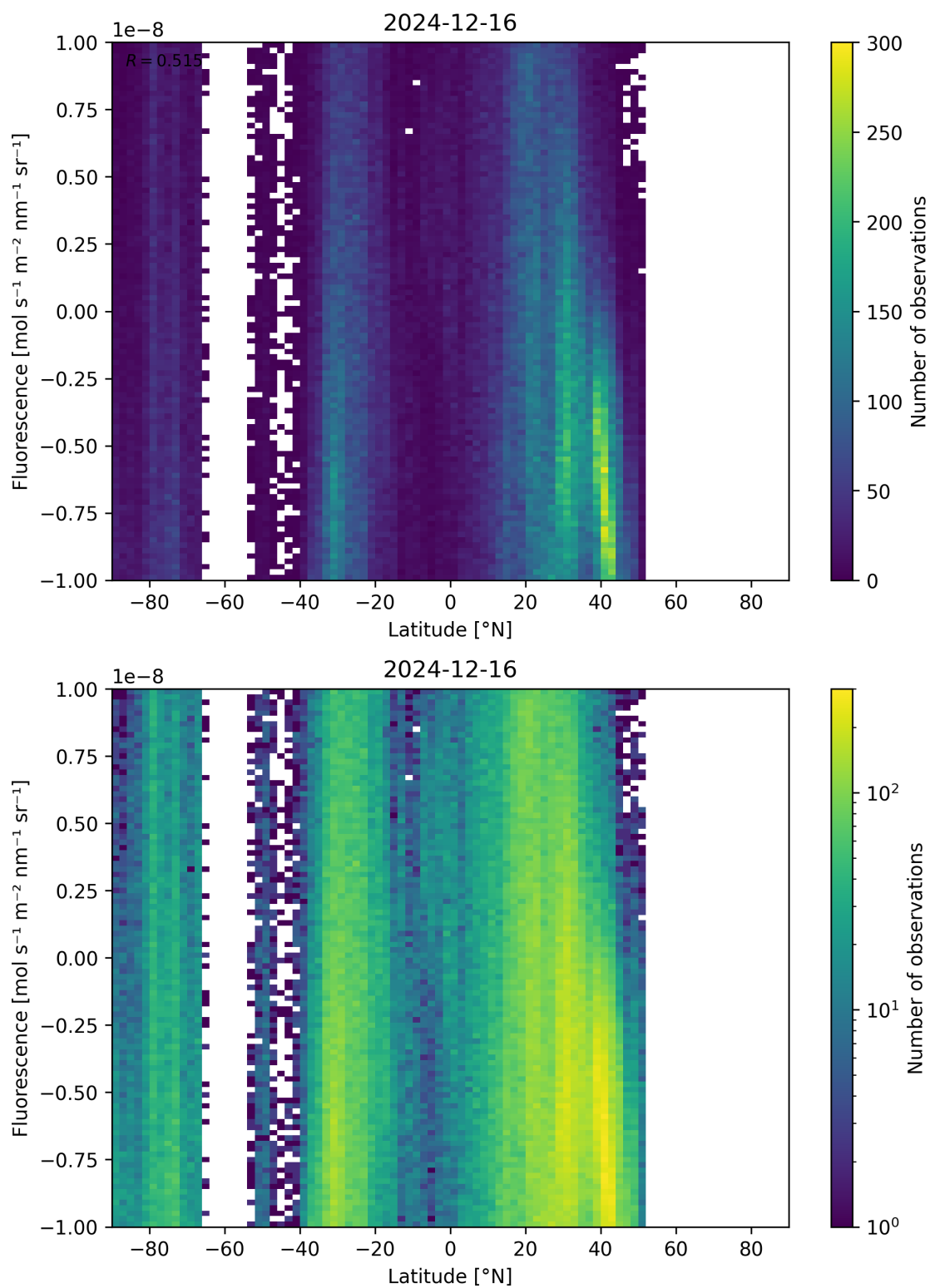
Figure 56: Scatter density plot of “Latitude” against “Fluorescence” for 2024-12-16 to 2024-12-17.
