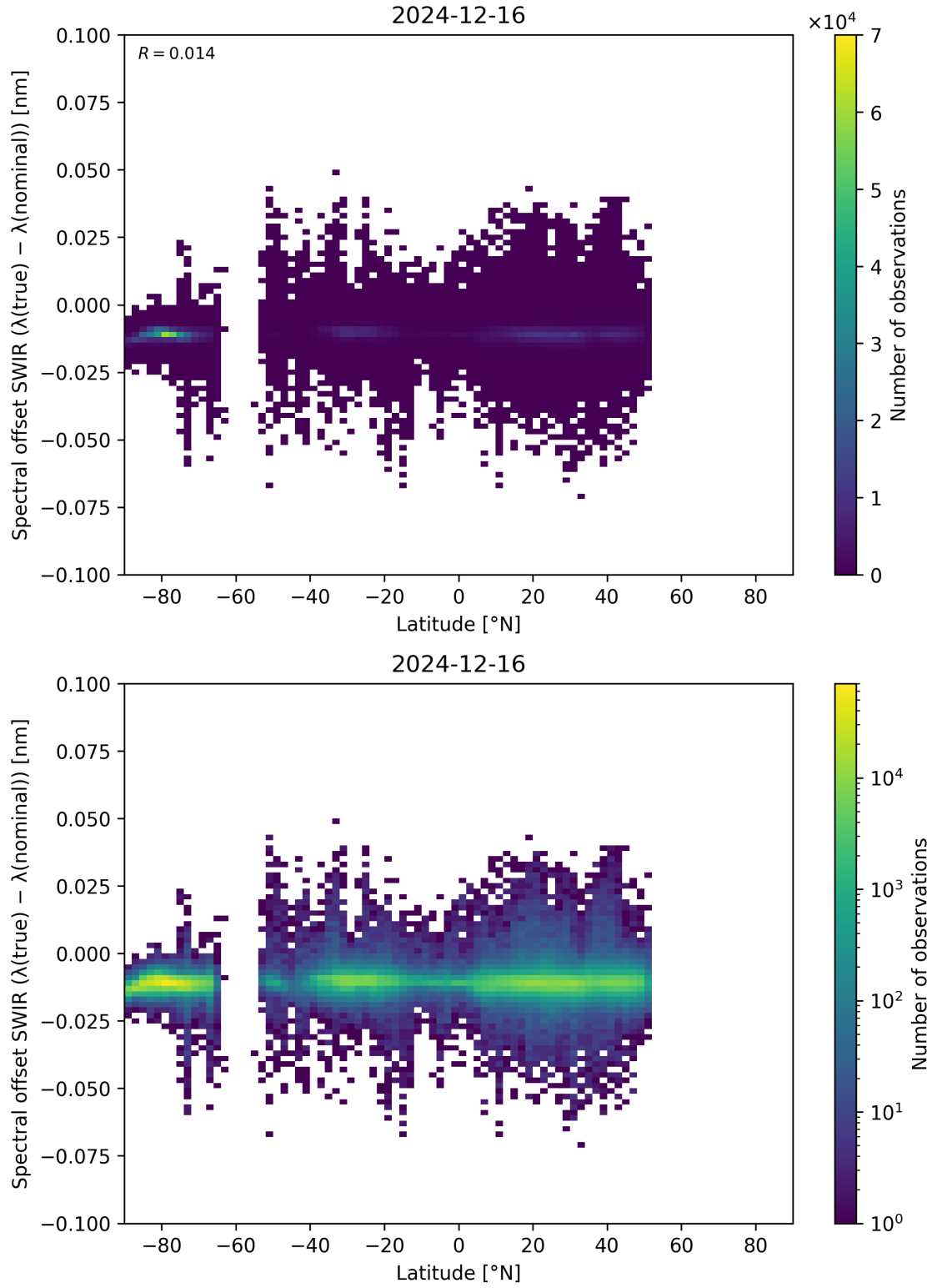
Figure 62: Scatter density plot of “Latitude” against “Spectral offset SWIR ( \lambda_{\text{true}} - \lambda_{\text{nominal}} )” for 2024-12-16 to 2024-12-17.
