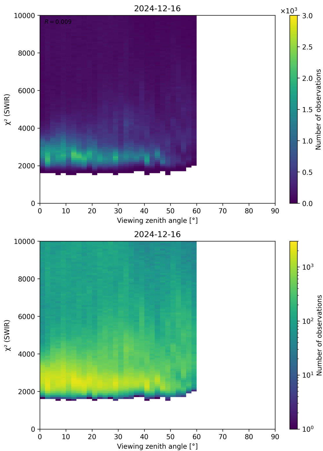
Figure 106: Scatter density plot of “Viewing zenith angle” against “ \chi^2 (SWIR)” for 2024-12-16 to 2024-12-17.
