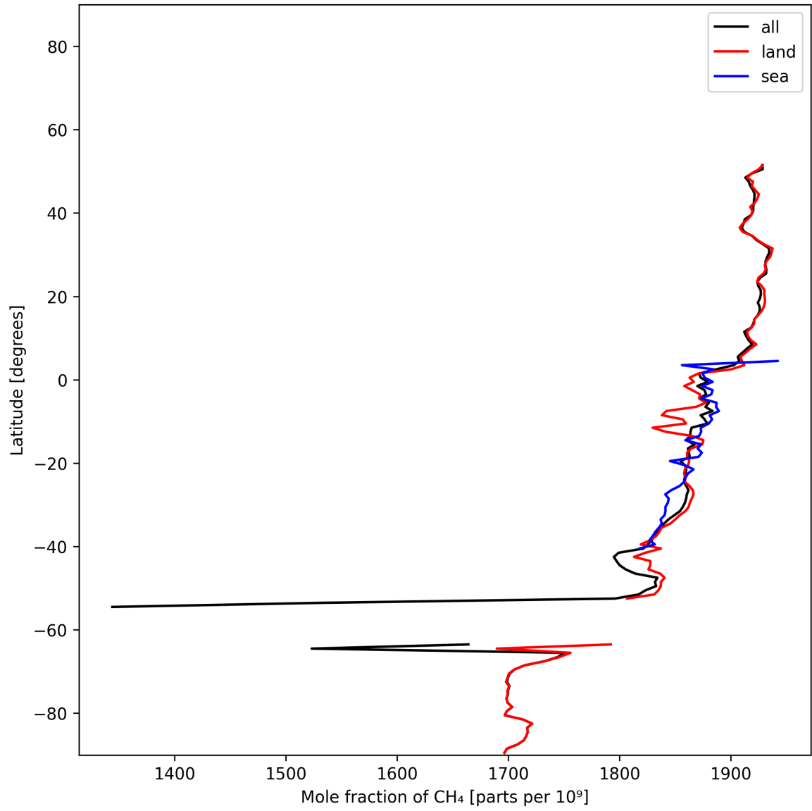
Figure 12: Zonal average of “Mole fraction of \text{CH}_4 ” for 2024-12-16 to 2024-12-17.
