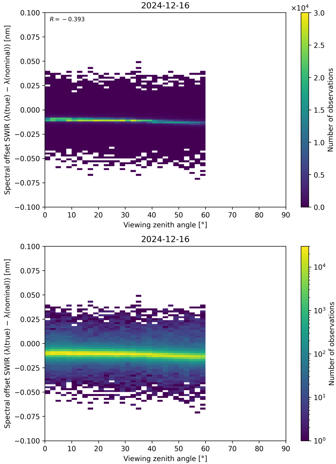
Figure 116: Scatter density plot of “Viewing zenith angle” against “Spectral offset SWIR ( \lambda_{\text{true}} - \lambda_{\text{nominal}} )” for 2024-12-16 to 2024-12-17.
