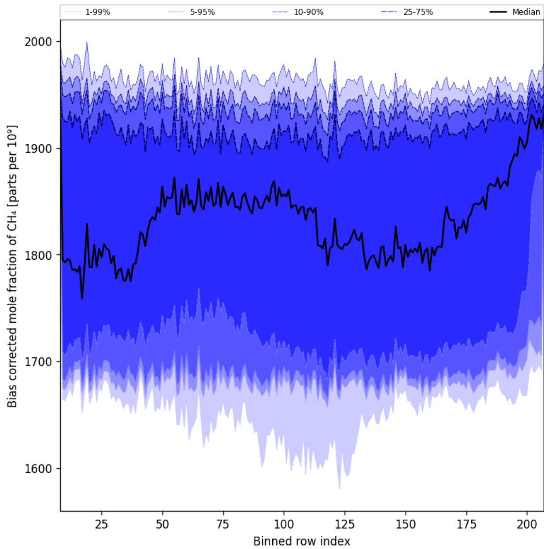
Figure 36: Along track statistics of “Bias corrected mole fraction of CH 4 ” for 2024-12-16 to 2024-12-17
