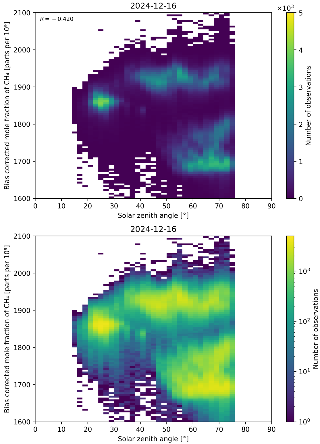
Figure 100: Scatter density plot of “Solar zenith angle” against “Bias corrected mole fraction of CH 4 ” for 2024-12-16 to 2024-12-17.
