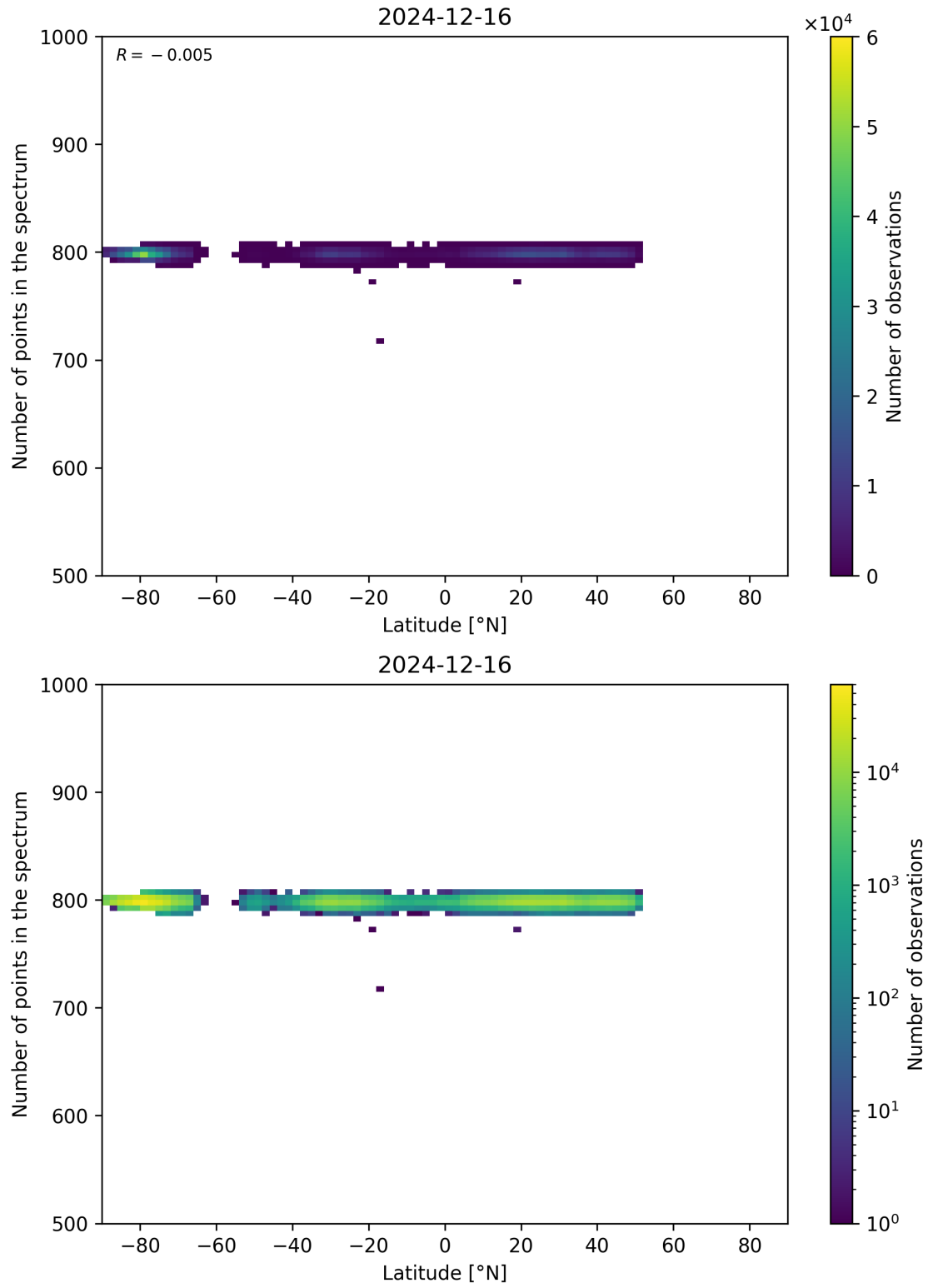
Figure 61: Scatter density plot of “Latitude” against “Number of points in the spectrum” for 2024-12-16 to 2024-12-17.
