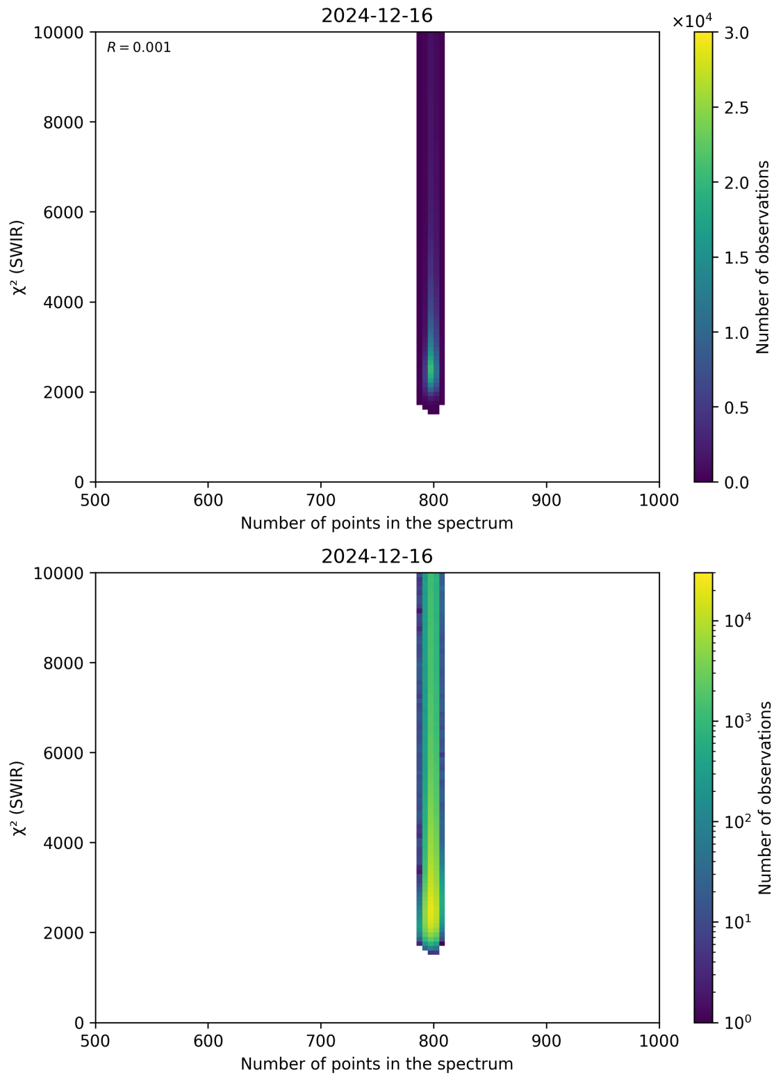
Figure 89: Scatter density plot of “Number of points in the spectrum” against “ \chi^2 (SWIR)” for 2024-12-16 to 2024-12-17.
