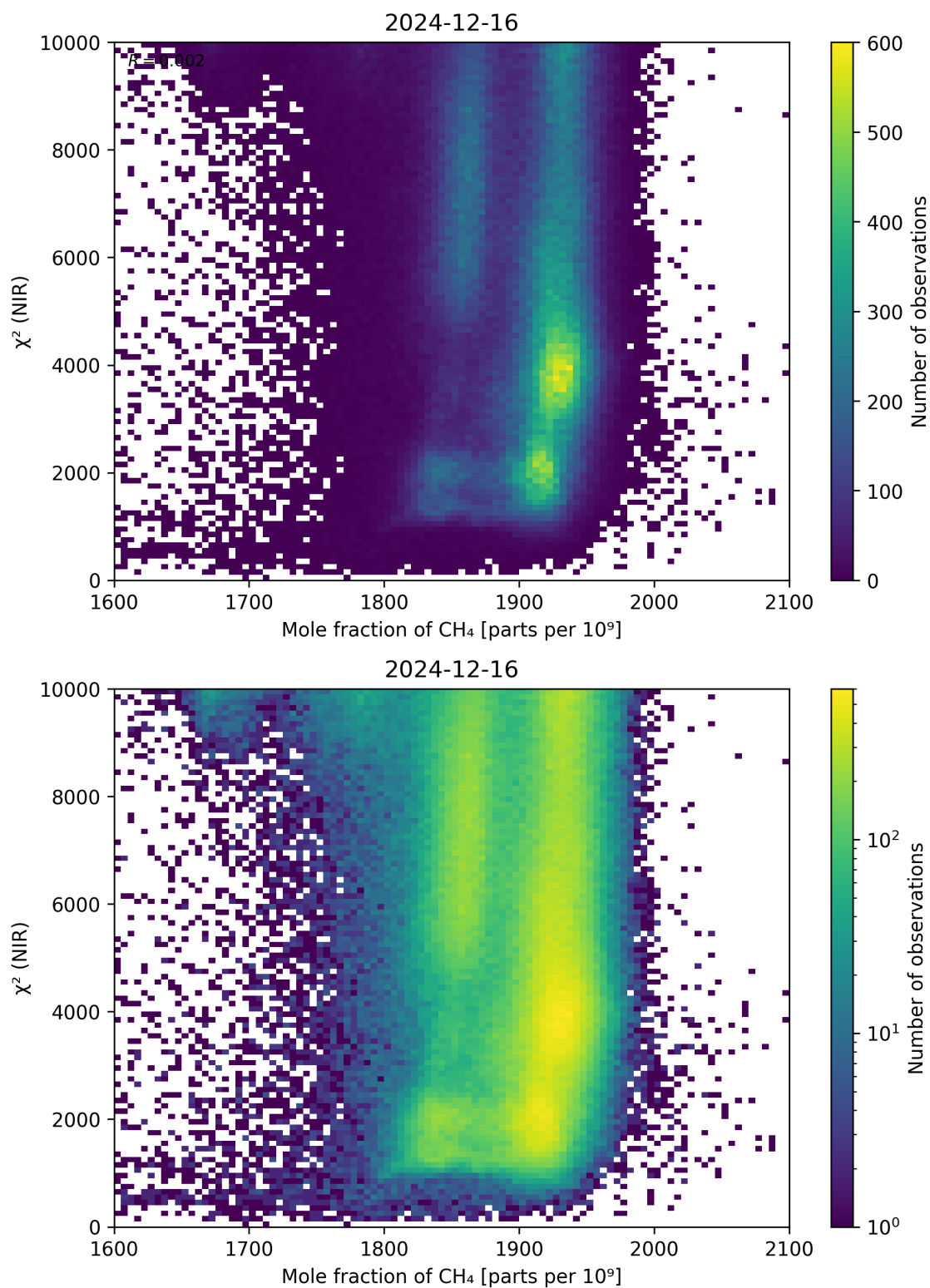
Figure 70: Scatter density plot of “Mole fraction of \text{CH}_4 ” against “ \chi^2 (NIR)” for 2024-12-16 to 2024-12-17.
