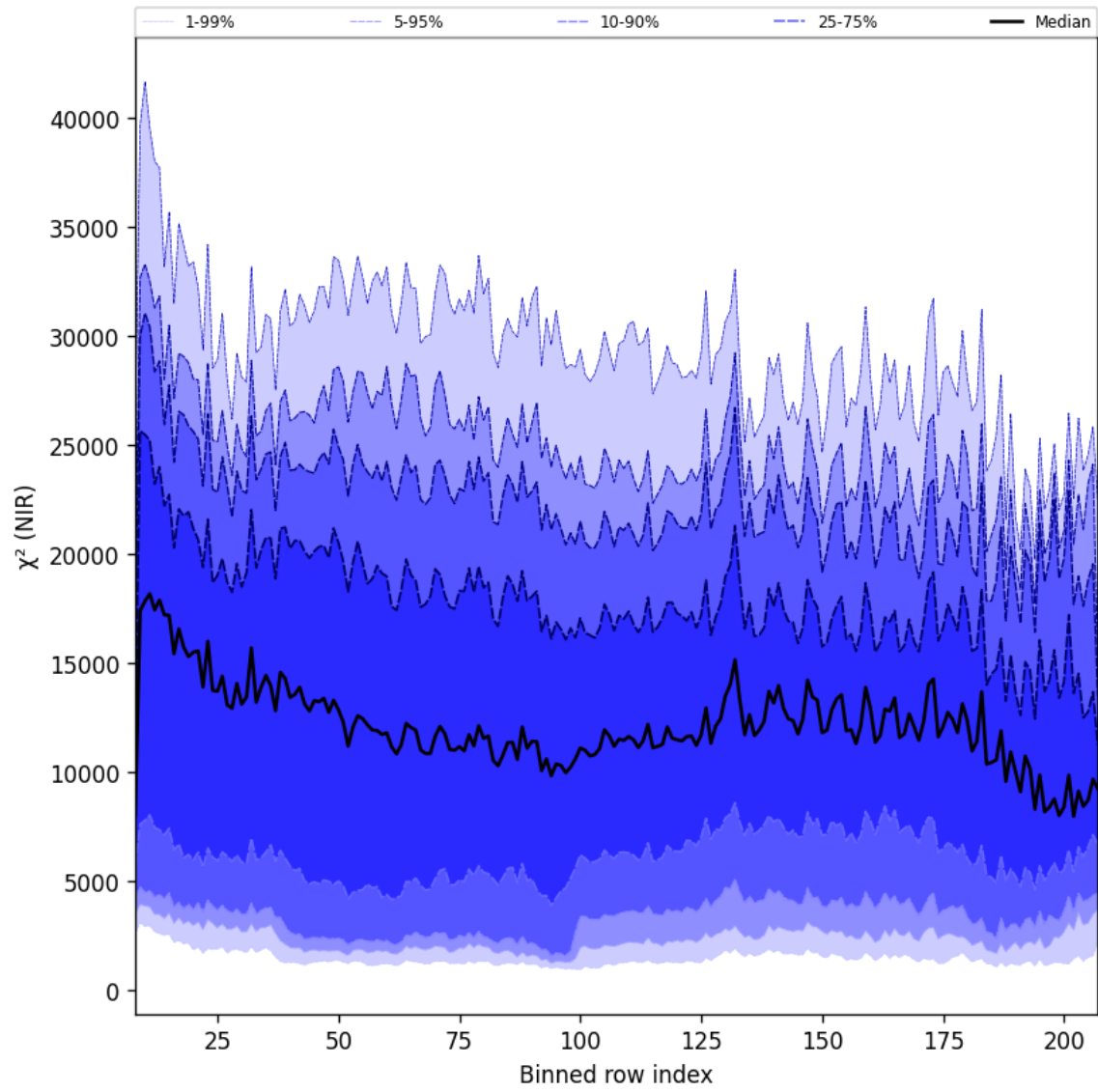
Figure 40: Along track statistics of “ \chi^2 (NIR)” for 2024-12-16 to 2024-12-17
