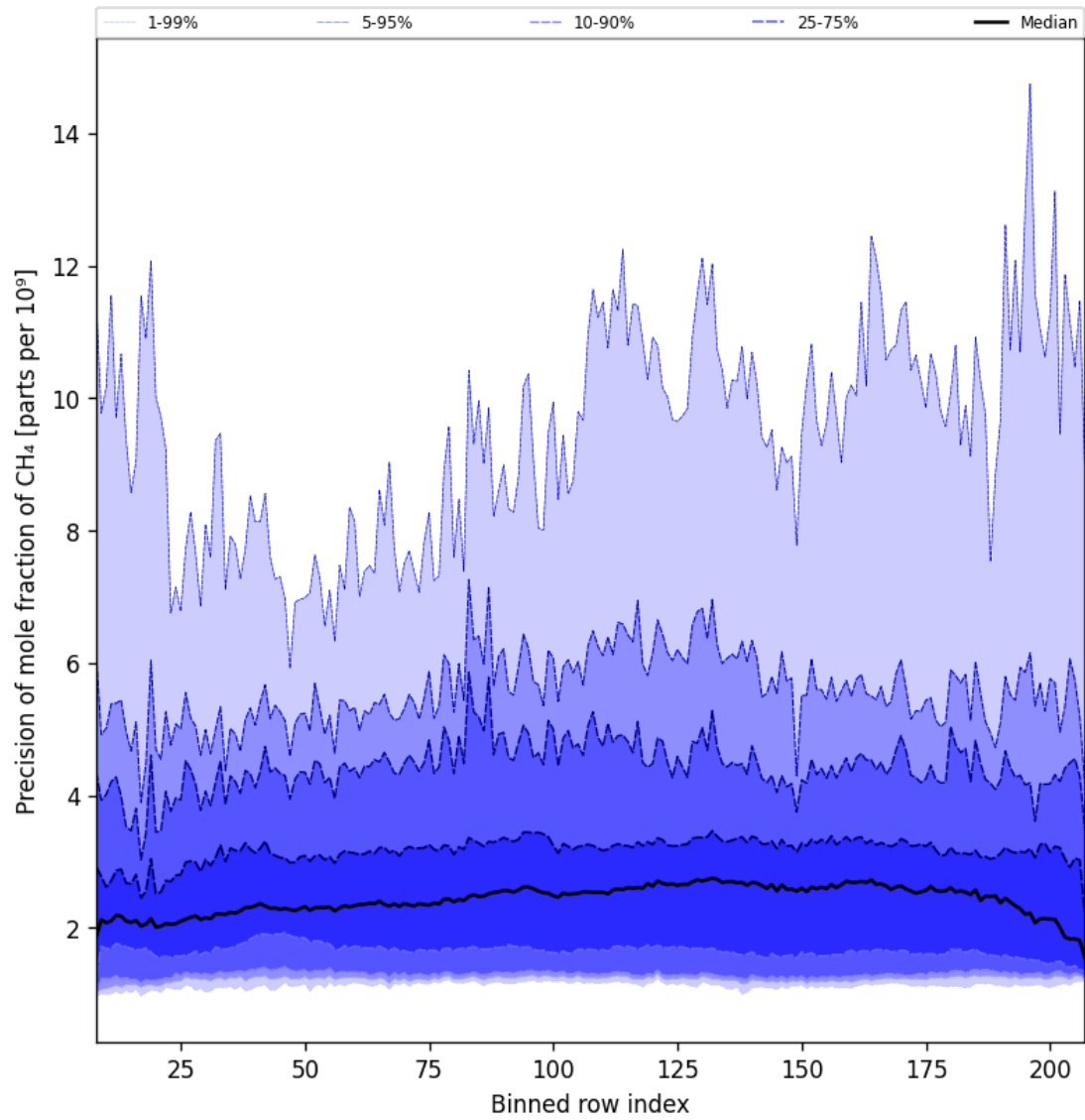
Figure 35: Along track statistics of “Precision of mole fraction of CH 4 ” for 2024-12-16 to 2024-12-17
