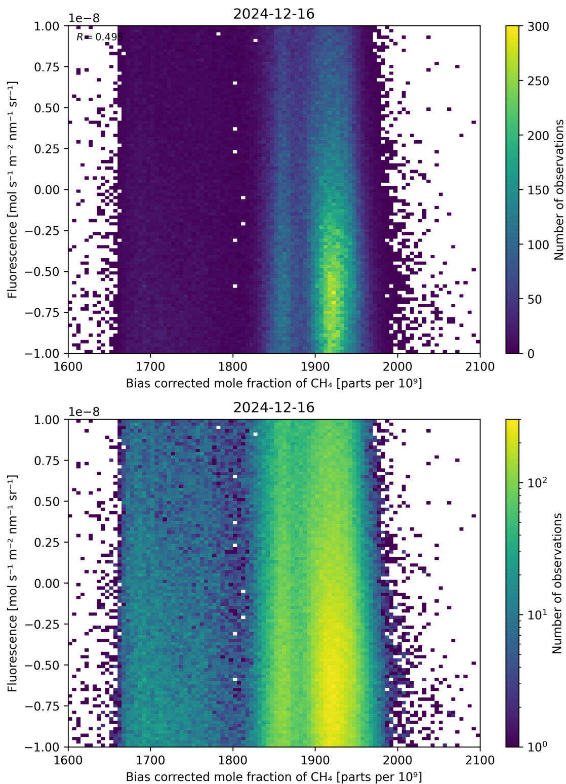
Figure 66: Scatter density plot of “Bias corrected mole fraction of \text{CH}_4 ” against “Fluorescence” for 2024-12-16 to 2024-12-17.
