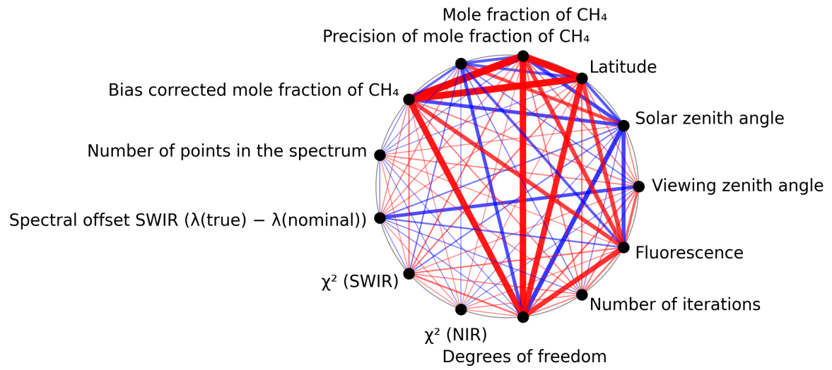
Figure 1: Map of correlation graph for 2024-12-16 to 2024-12-17.
