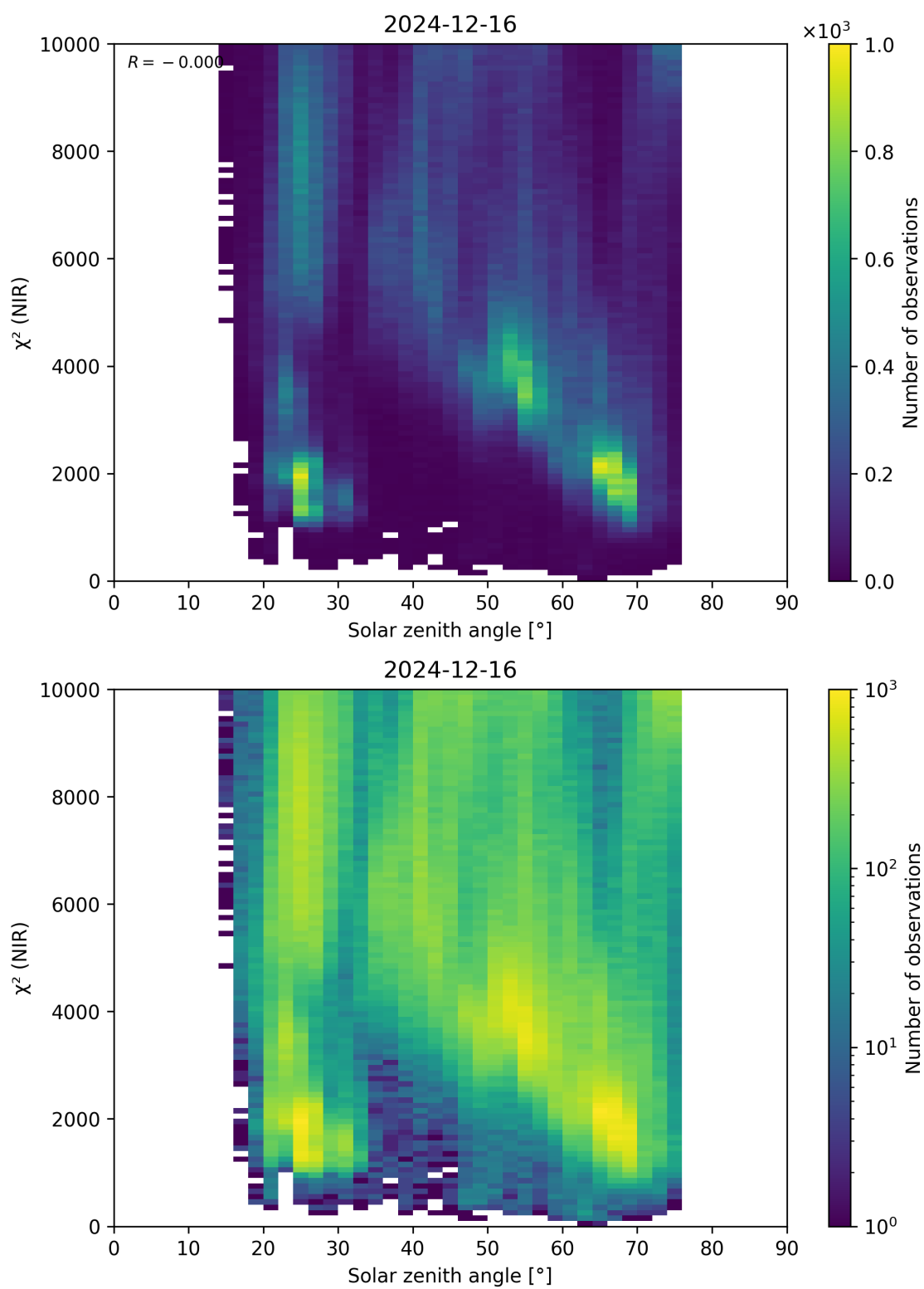
Figure 94: Scatter density plot of “Solar zenith angle” against “ \chi^2 (NIR)” for 2024-12-16 to 2024-12-17.
