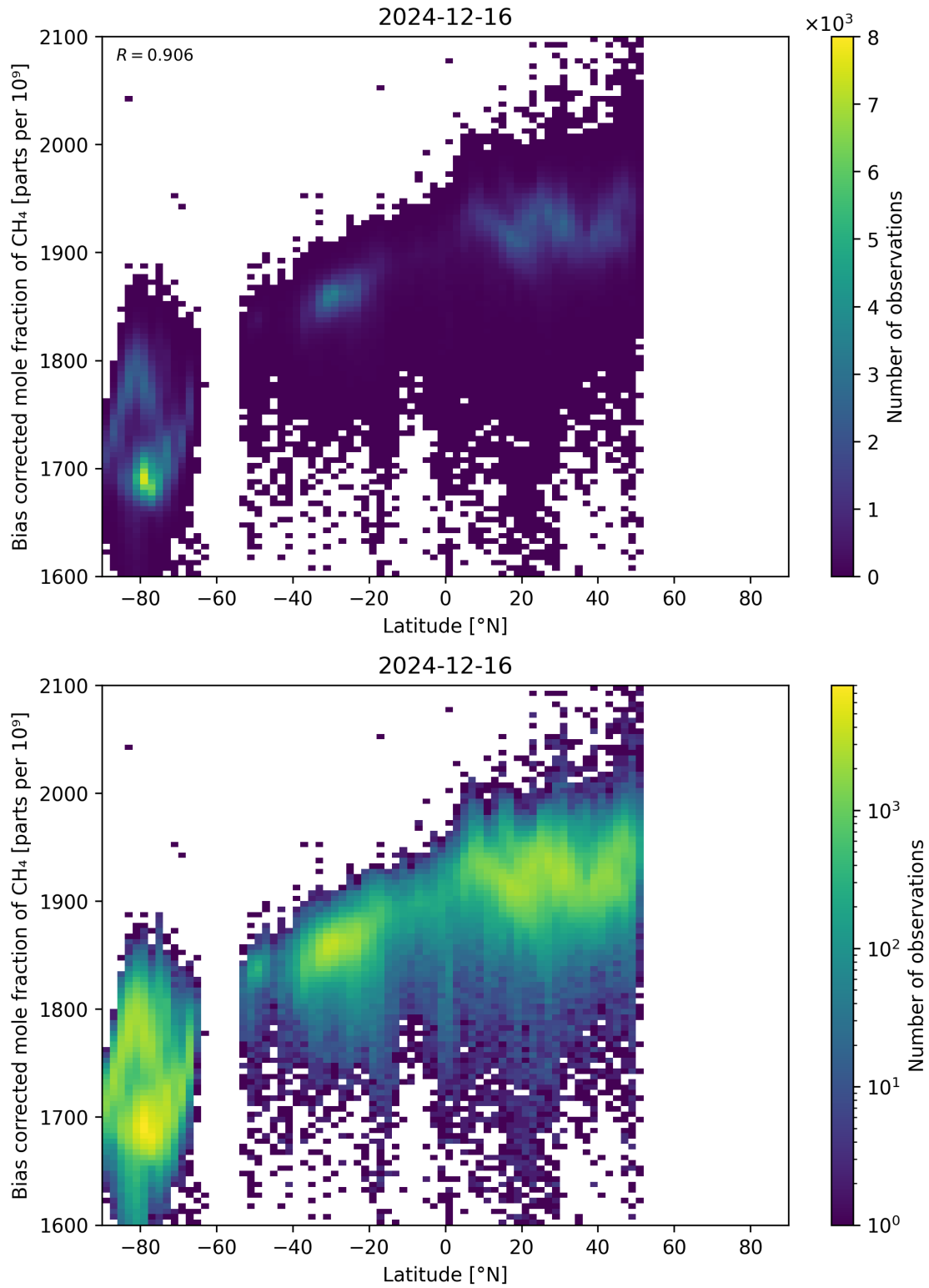
Figure 58: Scatter density plot of “Latitude” against “Bias corrected mole fraction of CH 4 ” for 2024-12-16 to 2024-12-17.
