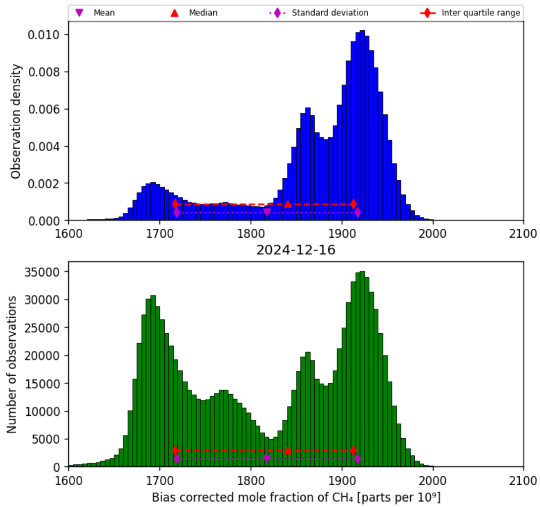
Figure 25: Histogram of “Bias corrected mole fraction of CH 4 ” for 2024-12-16 to 2024-12-17
