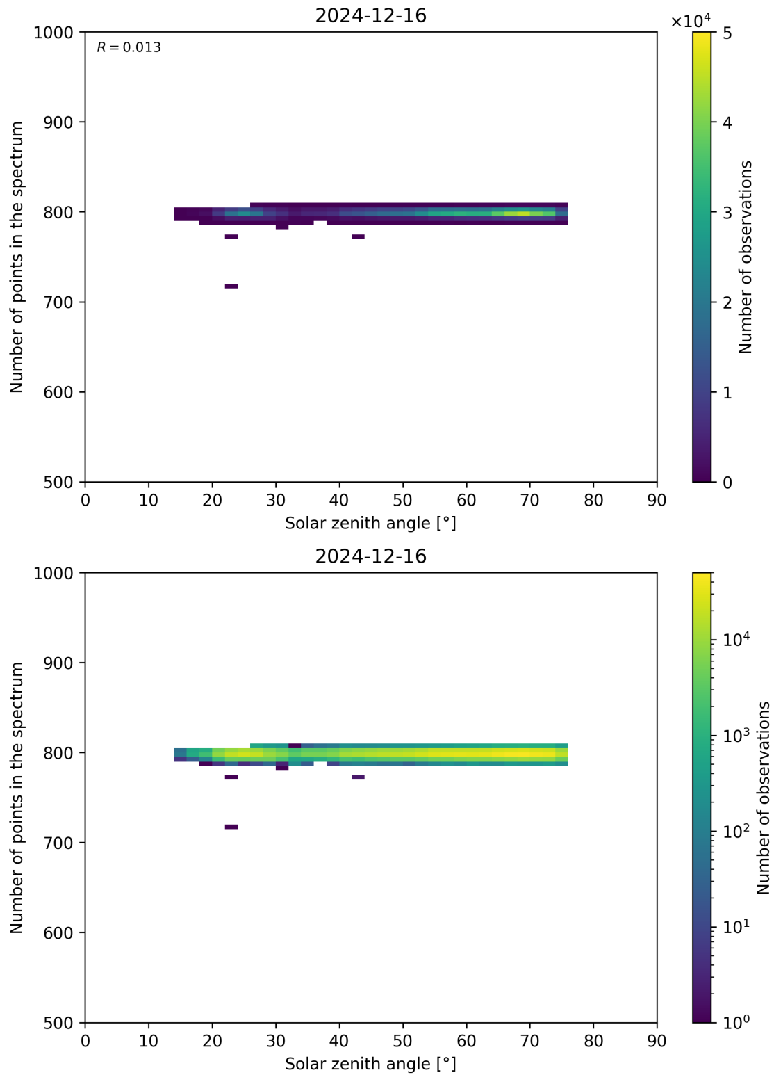
Figure 103: Scatter density plot of “Solar zenith angle” against “Number of points in the spectrum” for 2024-12-16 to 2024-12-17.
