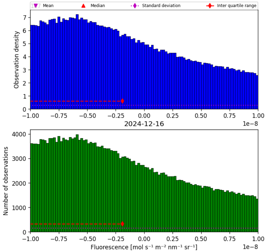
Figure 32: Histogram of “Fluorescence” for 2024-12-16 to 2024-12-17
