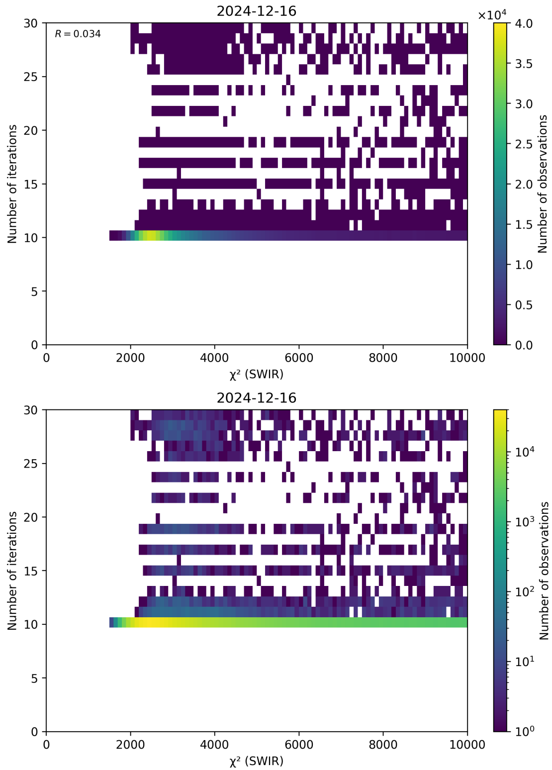
Figure 50: Scatter density plot of “ \chi^2 (SWIR)” against “Number of iterations” for 2024-12-16 to 2024-12-17.
