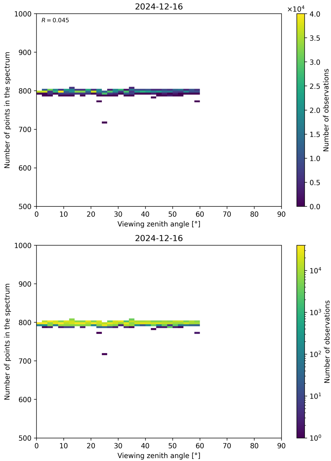
Figure 114: Scatter density plot of “Viewing zenith angle” against “Number of points in the spectrum” for 2024-12-16 to 2024-12-17.
