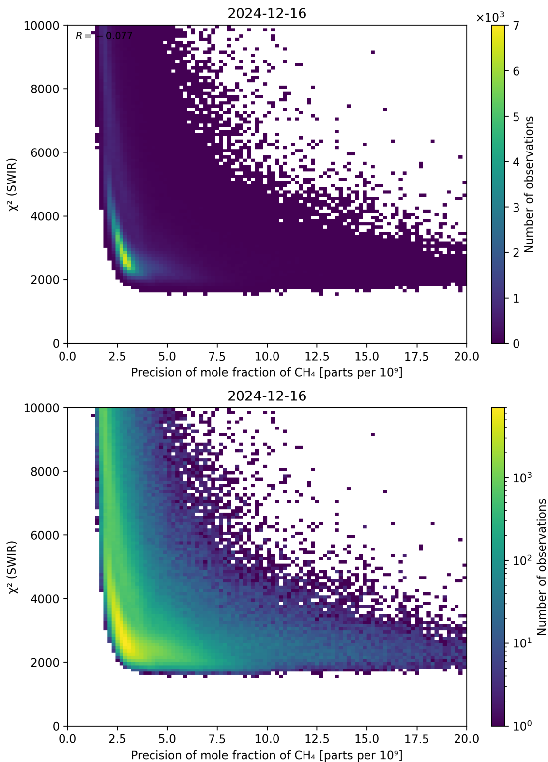
Figure 79: Scatter density plot of “Precision of mole fraction of CH 4 ” against “ \chi^2 (SWIR)” for 2024-12-16 to 2024-12-17.
