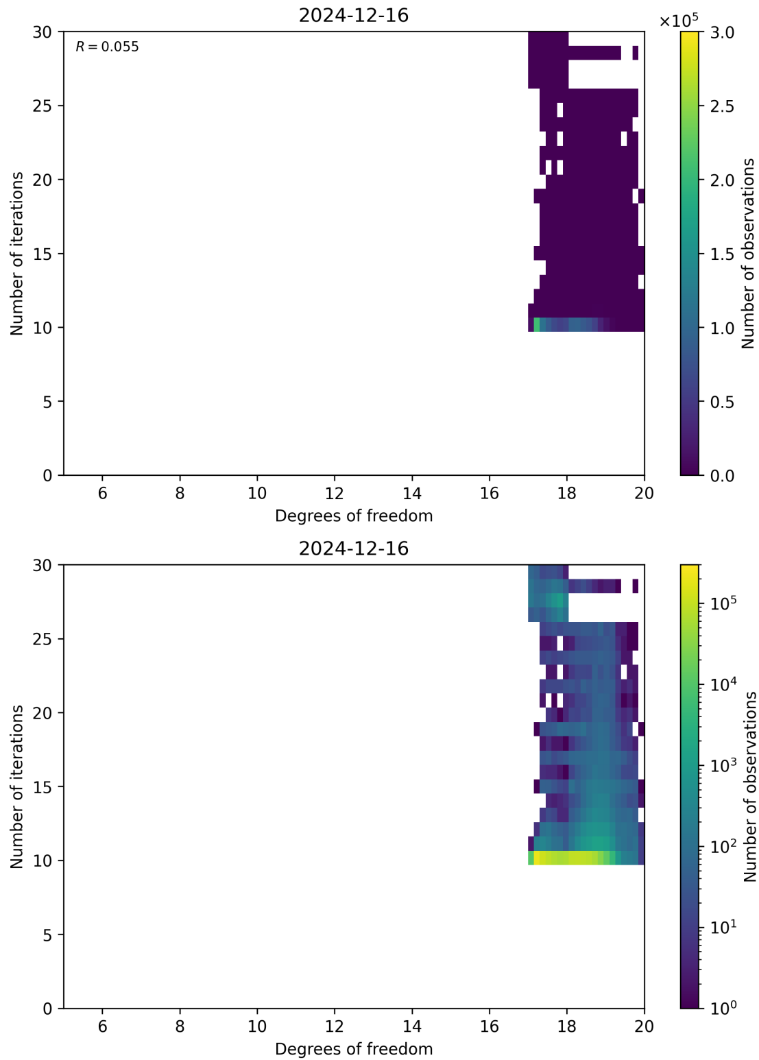
Figure 52: Scatter density plot of “Degrees of freedom” against “Number of iterations” for 2024-12-16 to 2024-12-17.
