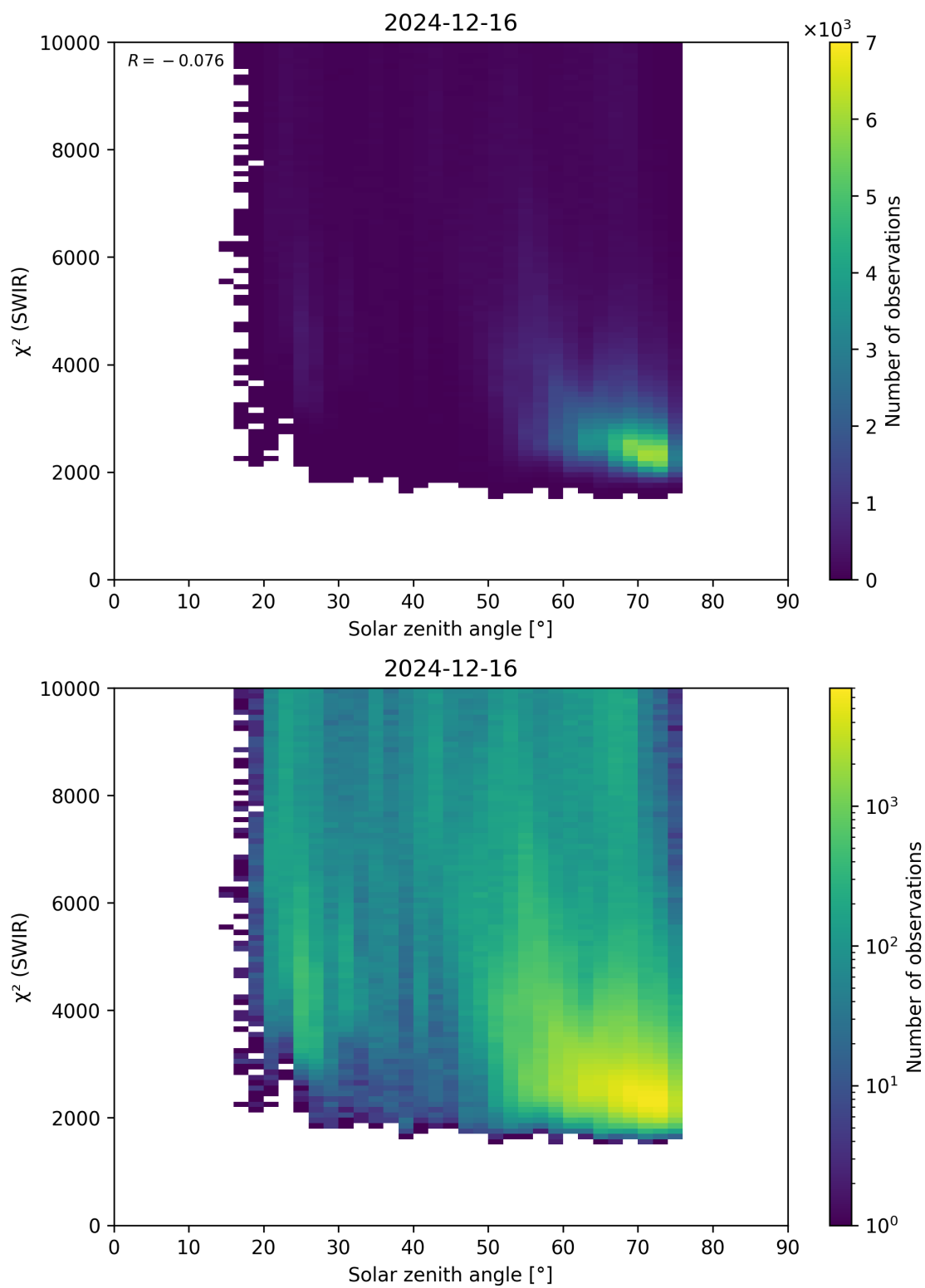
Figure 95: Scatter density plot of “Solar zenith angle” against “ \chi^2 (SWIR)” for 2024-12-16 to 2024-12-17.
