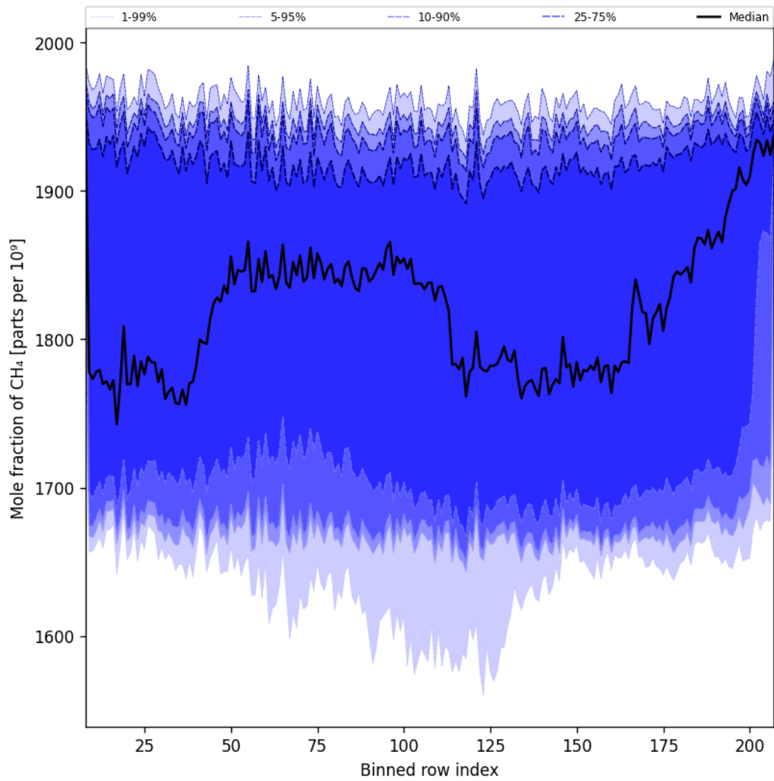
Figure 34: Along track statistics of “Mole fraction of CH 4 ” for 2024-12-16 to 2024-12-17
