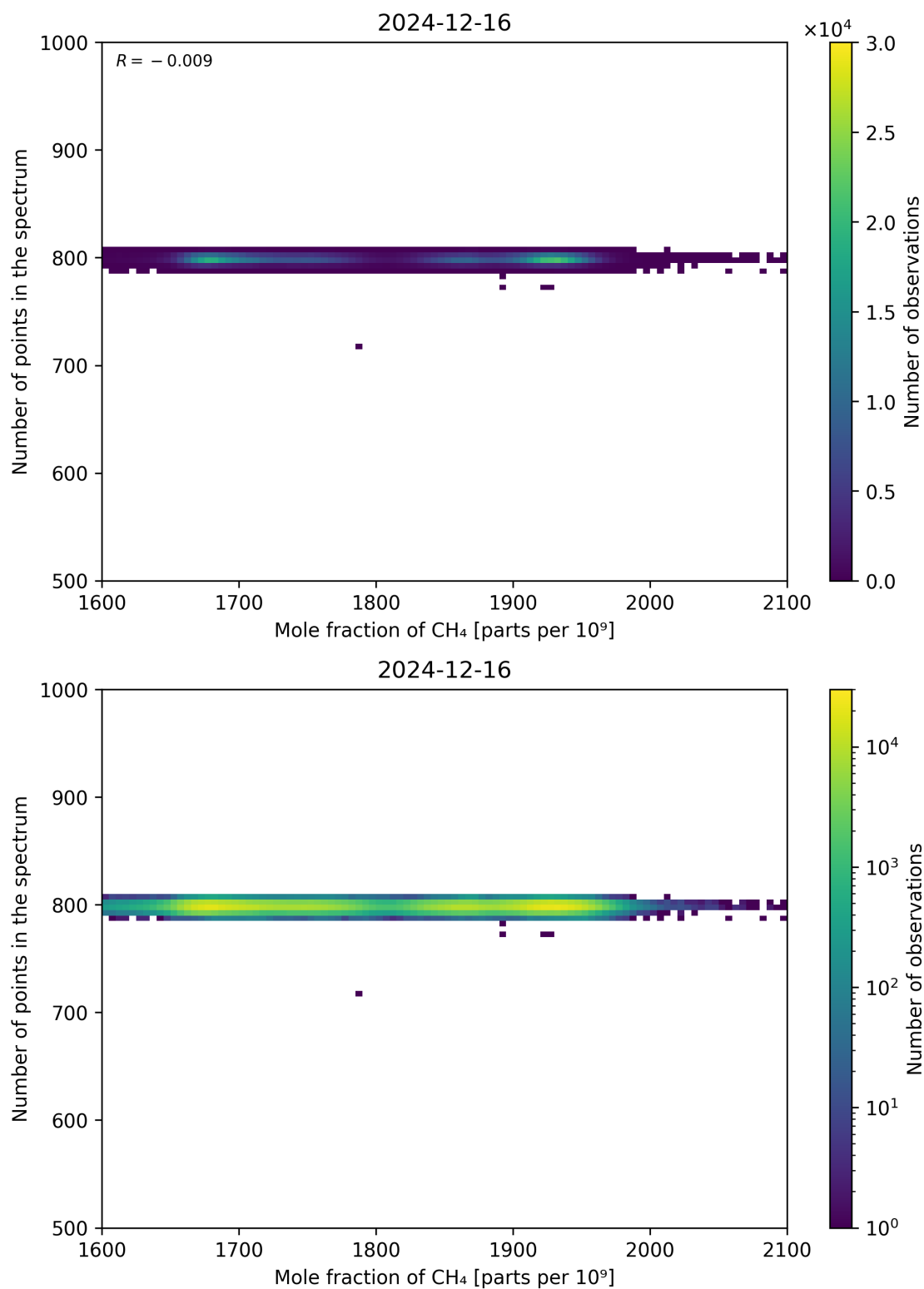
Figure 77: Scatter density plot of “Mole fraction of CH 4 ” against “Number of points in the spectrum” for 2024-12-16 to 2024-12-17.
