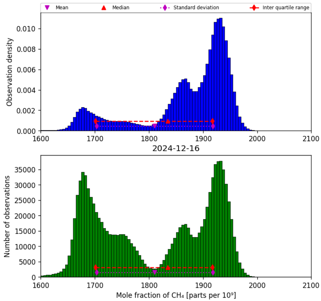
Figure 23: Histogram of “Mole fraction of CH 4 ” for 2024-12-16 to 2024-12-17
