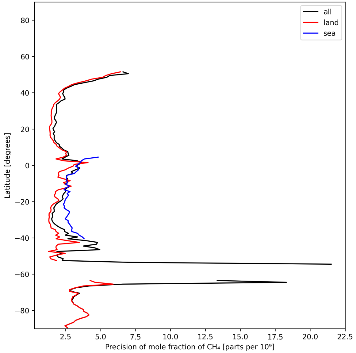
Figure 13: Zonal average of “Precision of mole fraction of CH 4 ” for 2024-12-16 to 2024-12-17.
