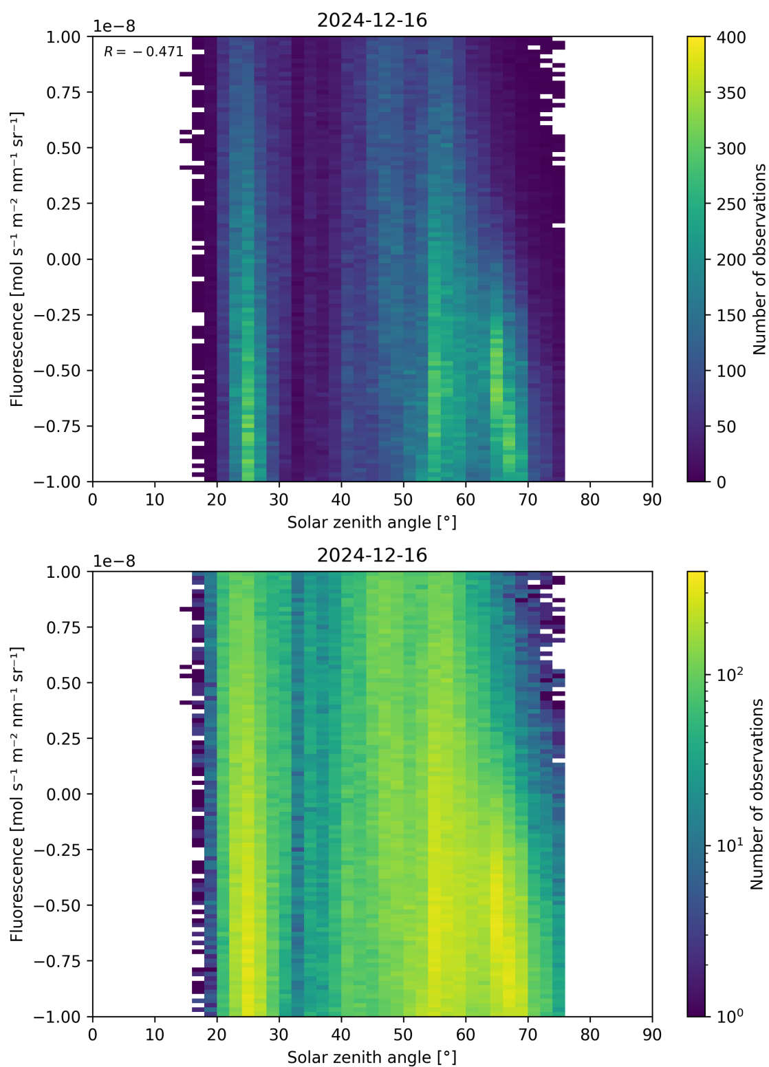
Figure 97: Scatter density plot of “Solar zenith angle” against “Fluorescence” for 2024-12-16 to 2024-12-17.
