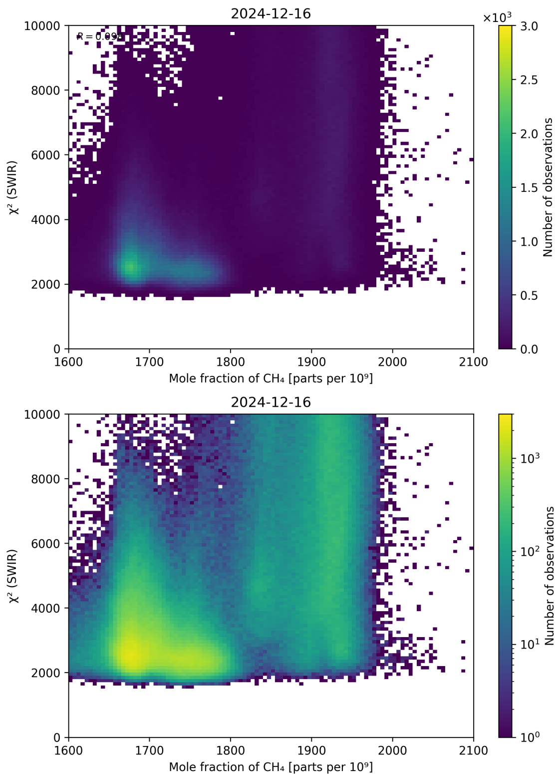
Figure 71: Scatter density plot of “Mole fraction of \text{CH}_4 ” against “ \chi^2 (SWIR)” for 2024-12-16 to 2024-12-17.
