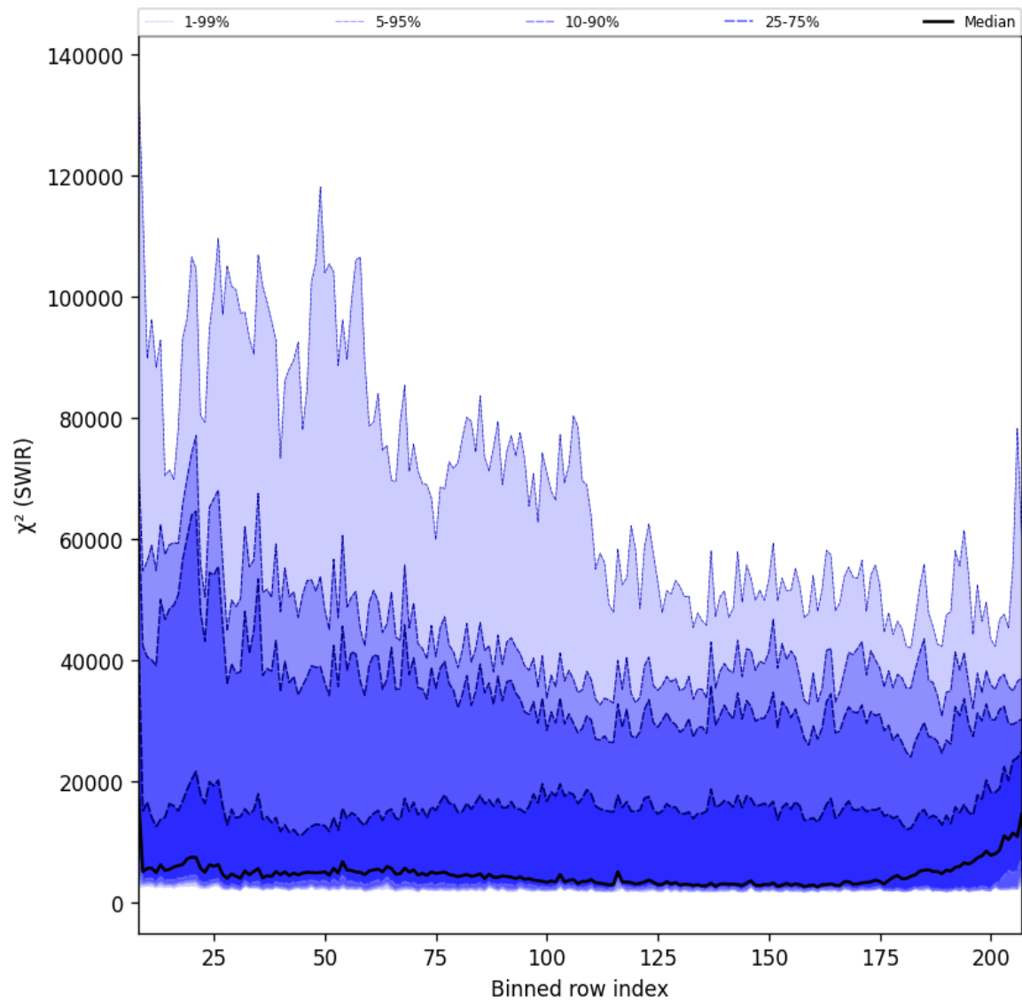
Figure 39: Along track statistics of " \chi^2 (SWIR)" for 2024-12-16 to 2024-12-17
