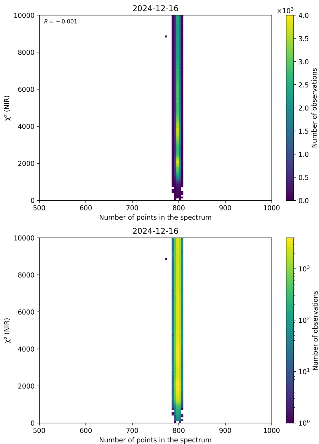
Figure 88: Scatter density plot of “Number of points in the spectrum” against “ \chi^2 (NIR)” for 2024-12-16 to 2024-12-17.
