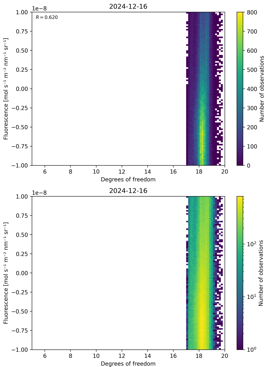
Figure 51: Scatter density plot of “Degrees of freedom” against “Fluorescence” for 2024-12-16 to 2024-12-17.
