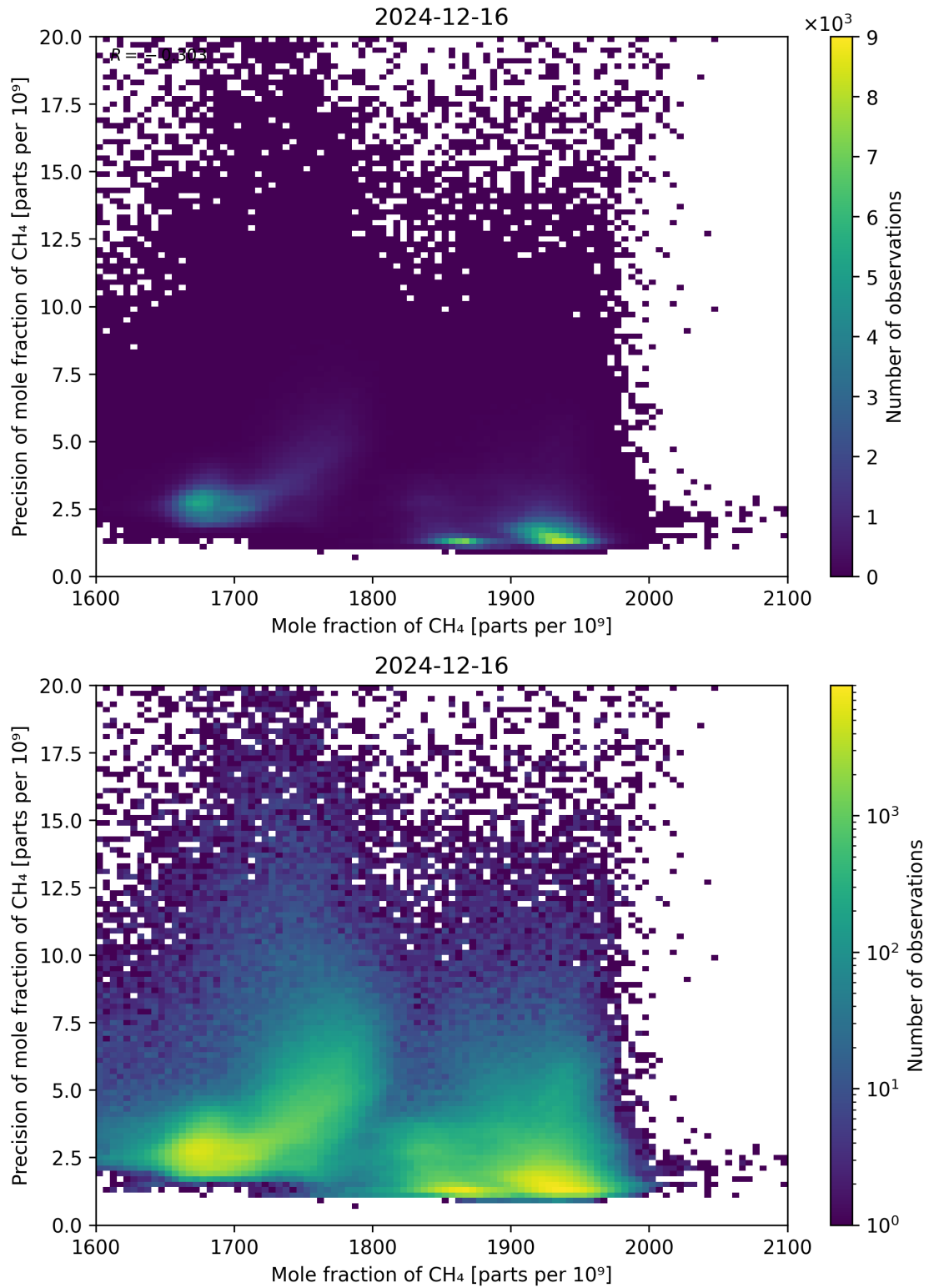
Figure 75: Scatter density plot of “Mole fraction of CH 4 ” against “Precision of mole fraction of CH 4 ” for 2024-12-16 to 2024-12-17.
