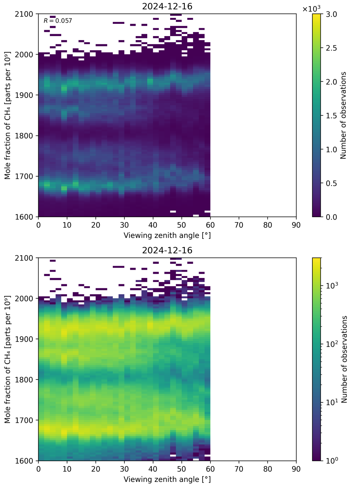
Figure 110: Scatter density plot of “Viewing zenith angle” against “Mole fraction of CH 4 ” for 2024-12-16 to 2024-12-17.
