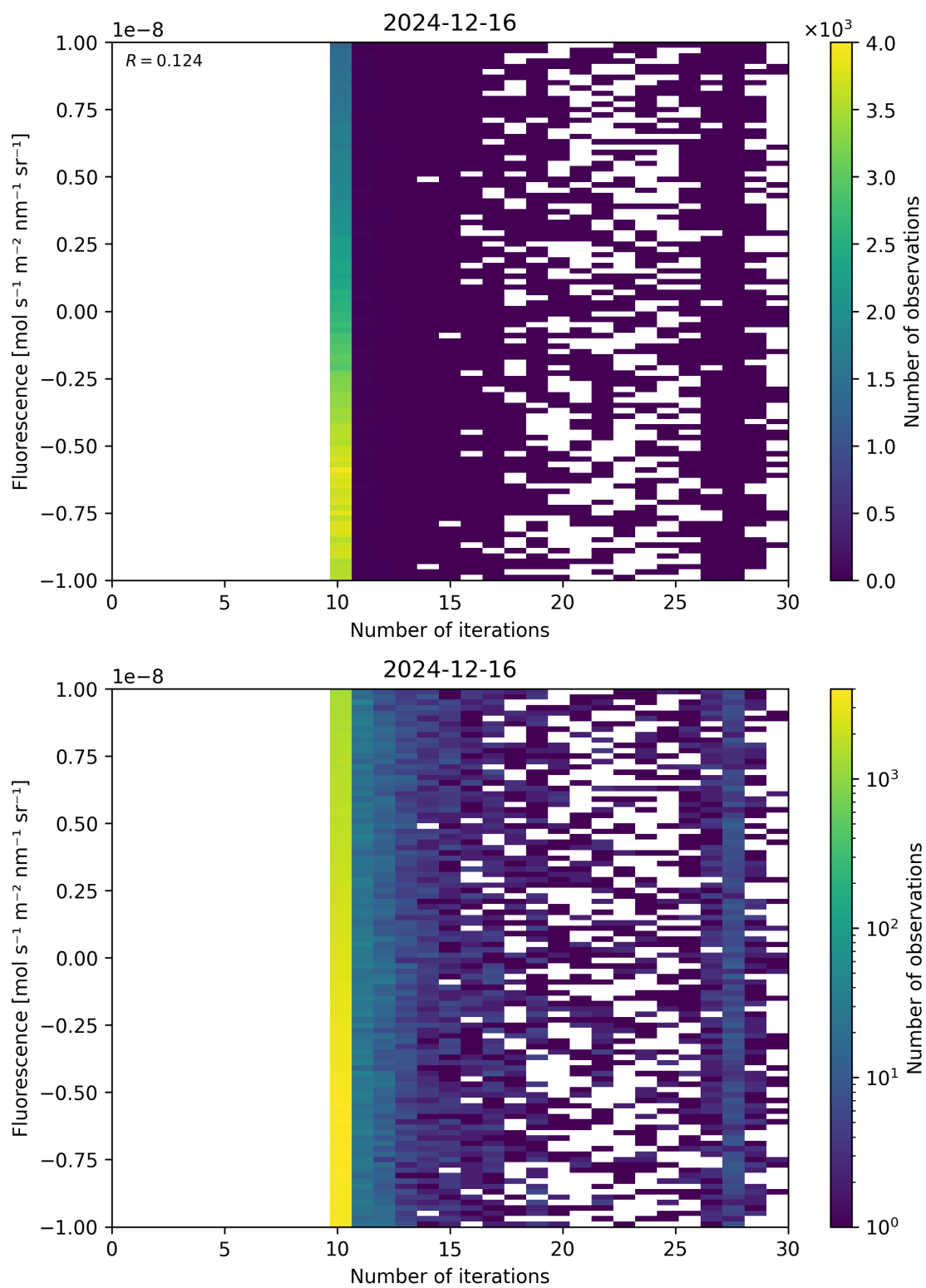
Figure 87: Scatter density plot of “Number of iterations” against “Fluorescence” for 2024-12-16 to 2024-12-17.
