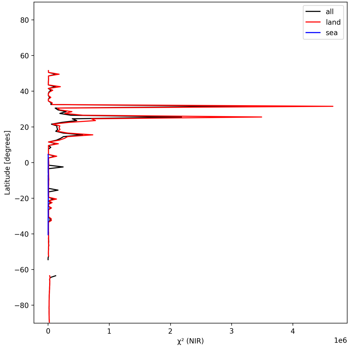
Figure 18: Zonal average of “ \chi^2 (NIR)” for 2024-12-16 to 2024-12-17.
