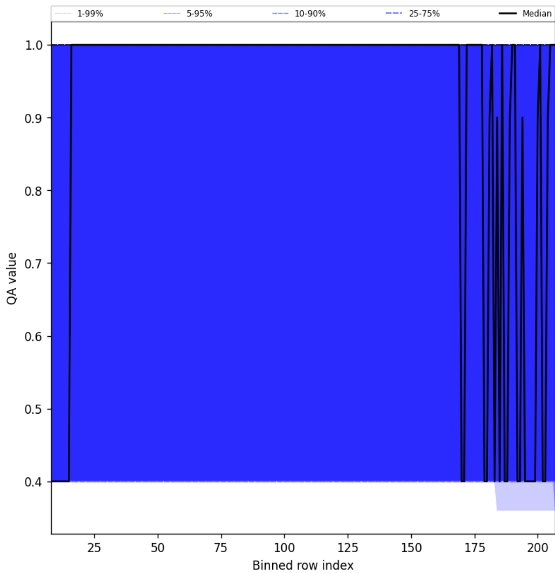
Figure 33: Along track statistics of “QA value” for 2024-12-16 to 2024-12-17
