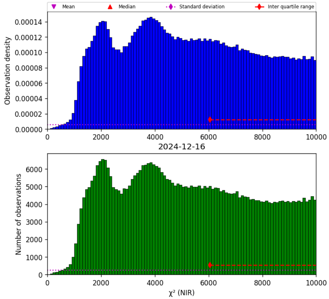
Figure 29: Histogram of “ \chi^2 (NIR)” for 2024-12-16 to 2024-12-17
