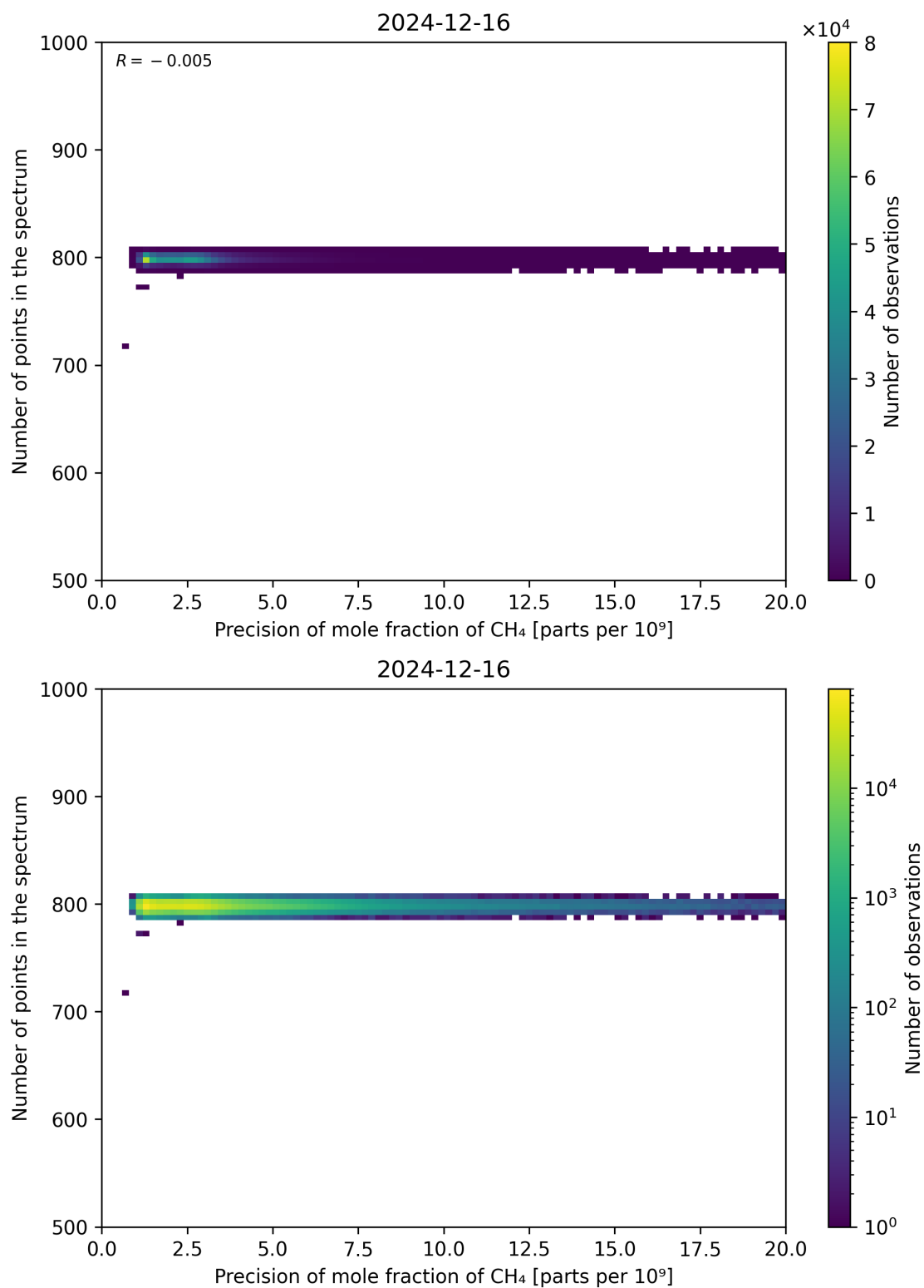
Figure 84: Scatter density plot of “Precision of mole fraction of CH 4 ” against “Number of points in the spectrum” for 2024-12-16 to 2024-12-17.
