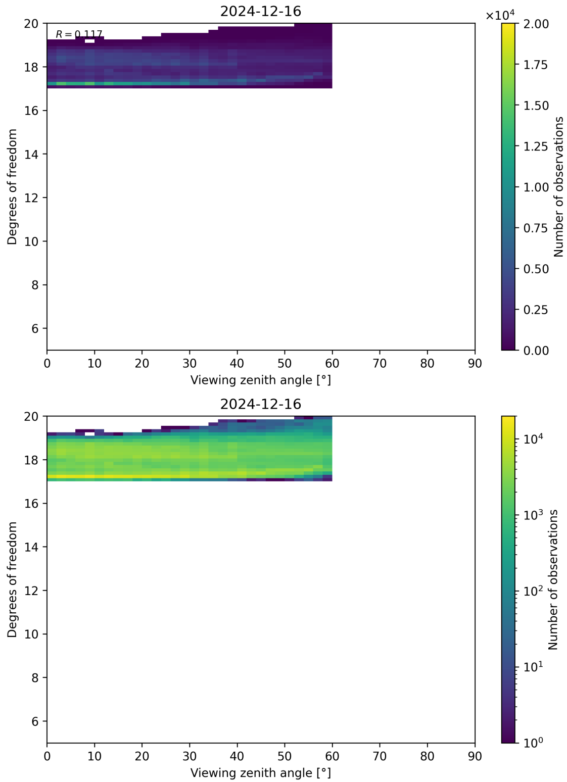
Figure 107: Scatter density plot of “Viewing zenith angle” against “Degrees of freedom” for 2024-12-16 to 2024-12-17.
