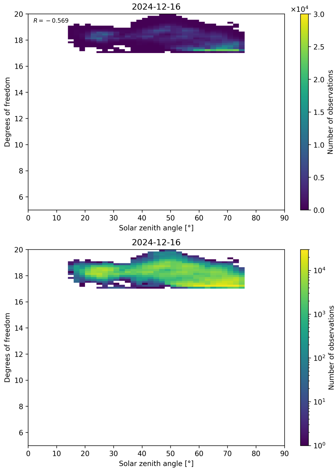
Figure 96: Scatter density plot of “Solar zenith angle” against “Degrees of freedom” for 2024-12-16 to 2024-12-17.
