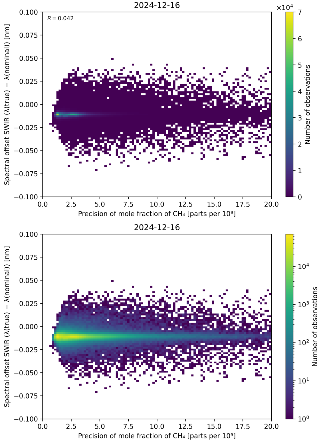
Figure 85: Scatter density plot of “Precision of mole fraction of CH 4 ” against “Spectral offset SWIR ( \lambda_{\text{true}} - \lambda_{\text{nominal}} )” for 2024-12-16 to 2024-12-17.
