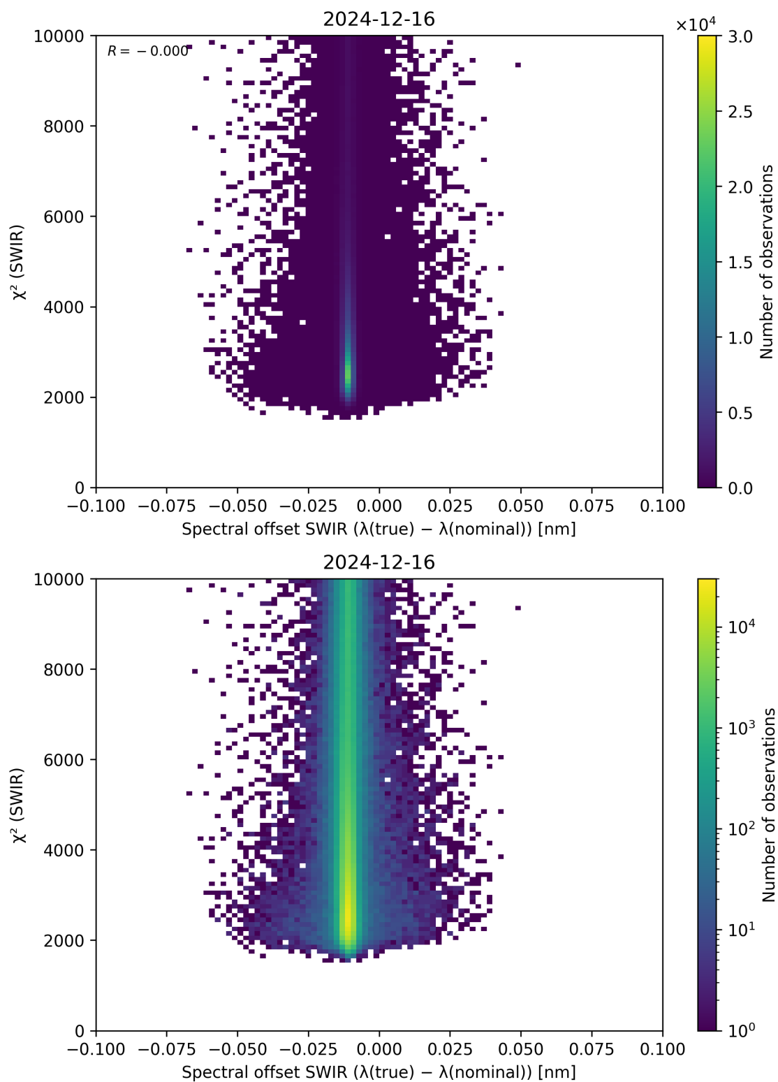
Figure 118: Scatter density plot of “Spectral offset SWIR ( \lambda_{\text{true}} - \lambda_{\text{nominal}} )” against “ \chi^2 (SWIR)” for 2024-12-16 to 2024-12-17.
