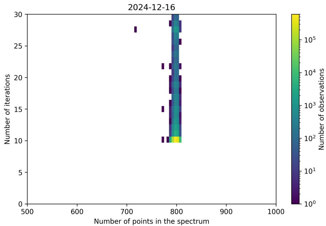
Figure 92: Scatter density plot of “Number of points in the spectrum” against “Number of iterations” for 2024-12-16 to 2024-12-17.
