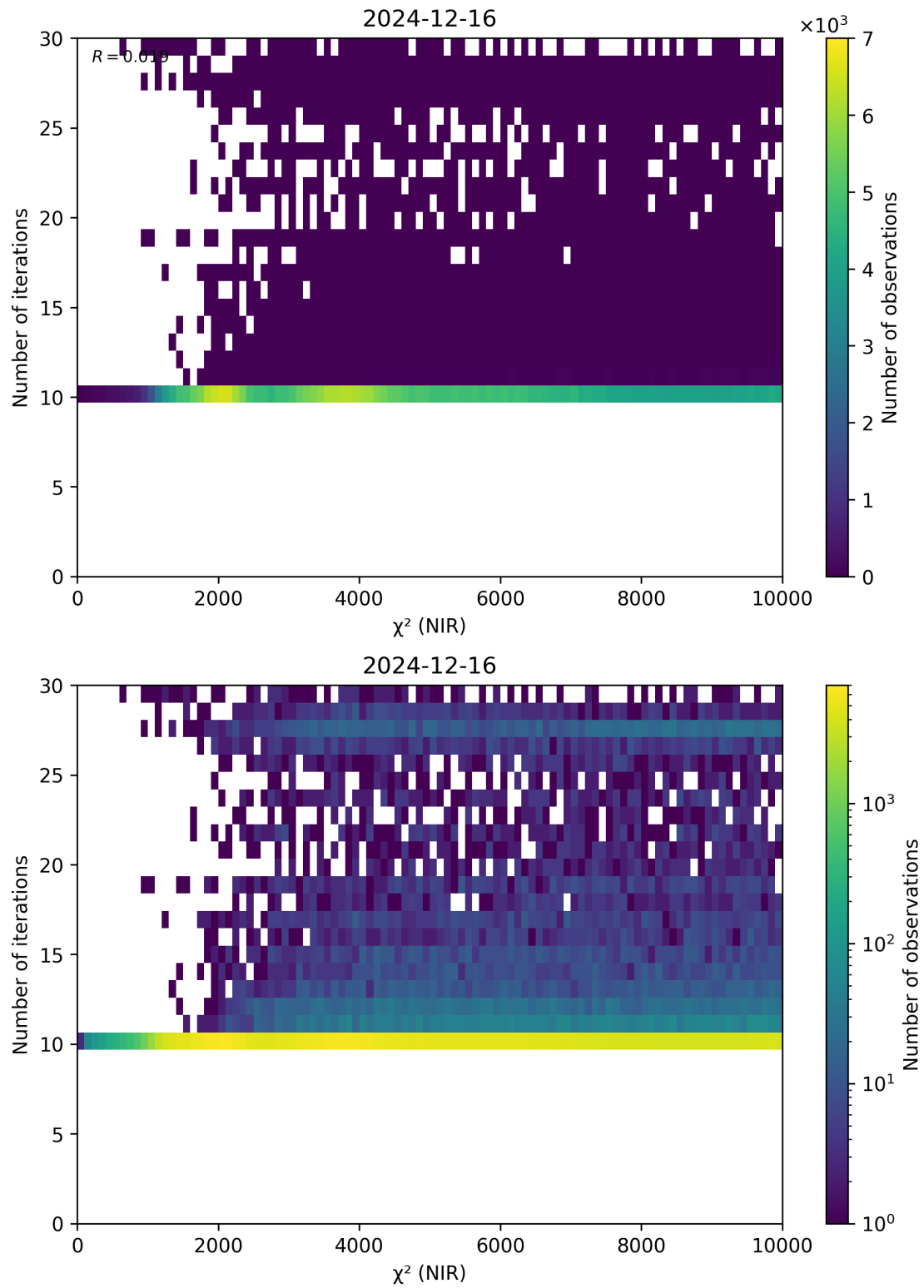
Figure 46: Scatter density plot of “ \chi^2 (NIR)” against “Number of iterations” for 2024-12-16 to 2024-12-17.
