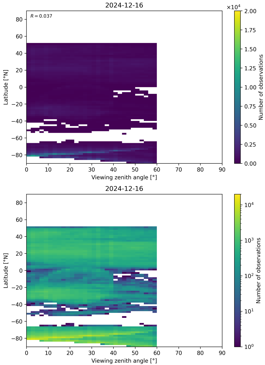
Figure 109: Scatter density plot of “Viewing zenith angle” against “Latitude” for 2024-12-16 to 2024-12-17.
