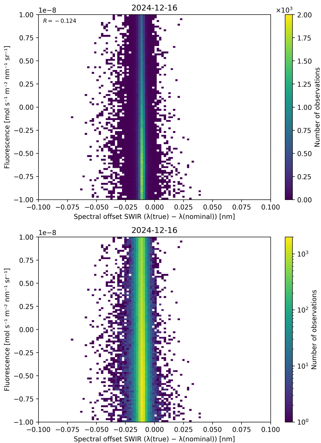
Figure 120: Scatter density plot of “Spectral offset SWIR ( \lambda_{\text{true}} - \lambda_{\text{nominal}} )” against “Fluorescence” for 2024-12-16 to 2024-12-17.
