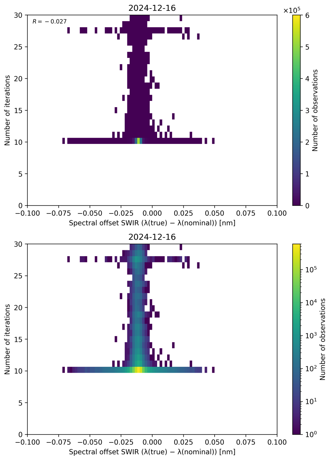
Figure 121: Scatter density plot of “Spectral offset SWIR ( \lambda_{\text{true}} - \lambda_{\text{nominal}} )” against “Number of iterations” for 2024-12-16 to 2024-12-17.
