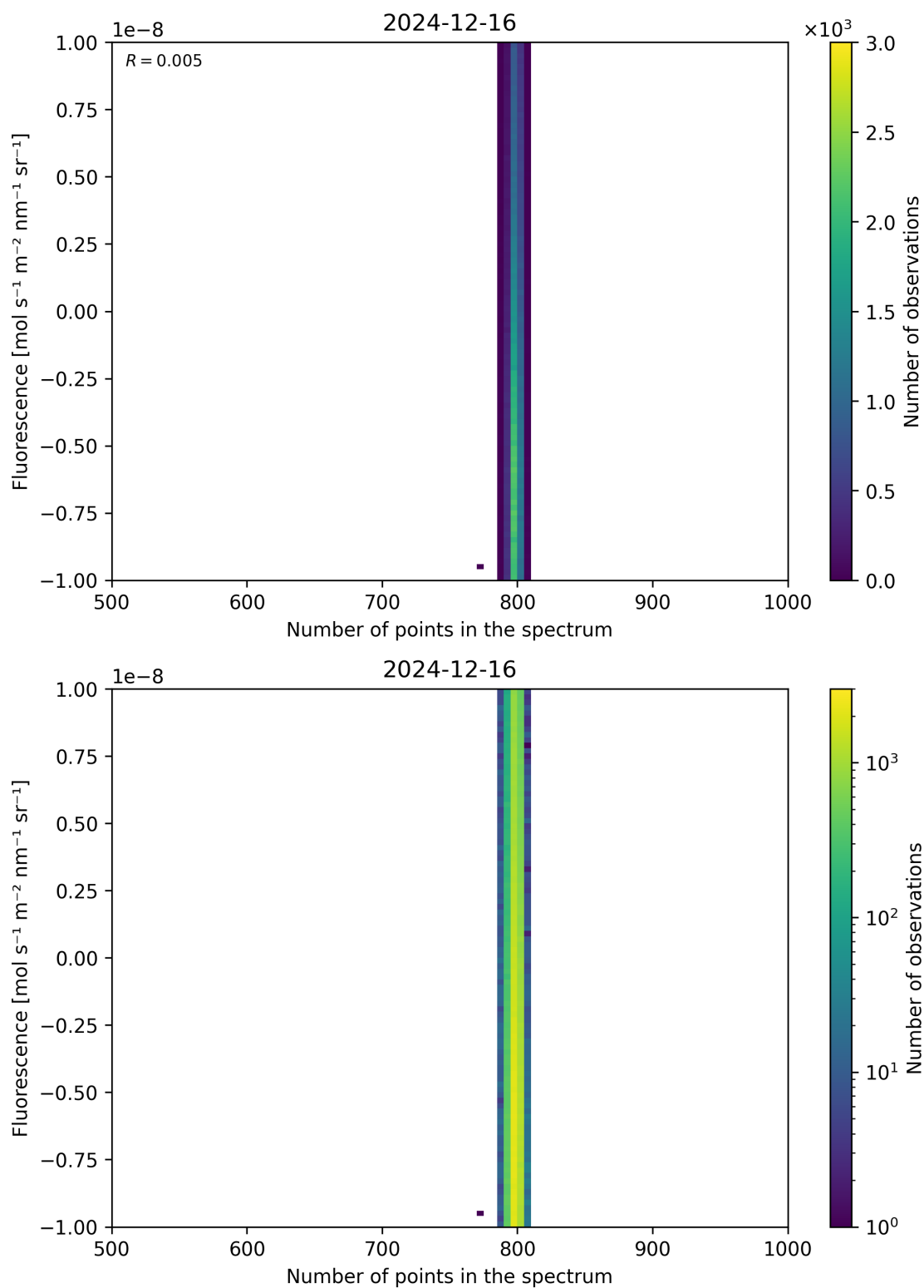
Figure 91: Scatter density plot of “Number of points in the spectrum” against “Fluorescence” for 2024-12-16 to 2024-12-17.
