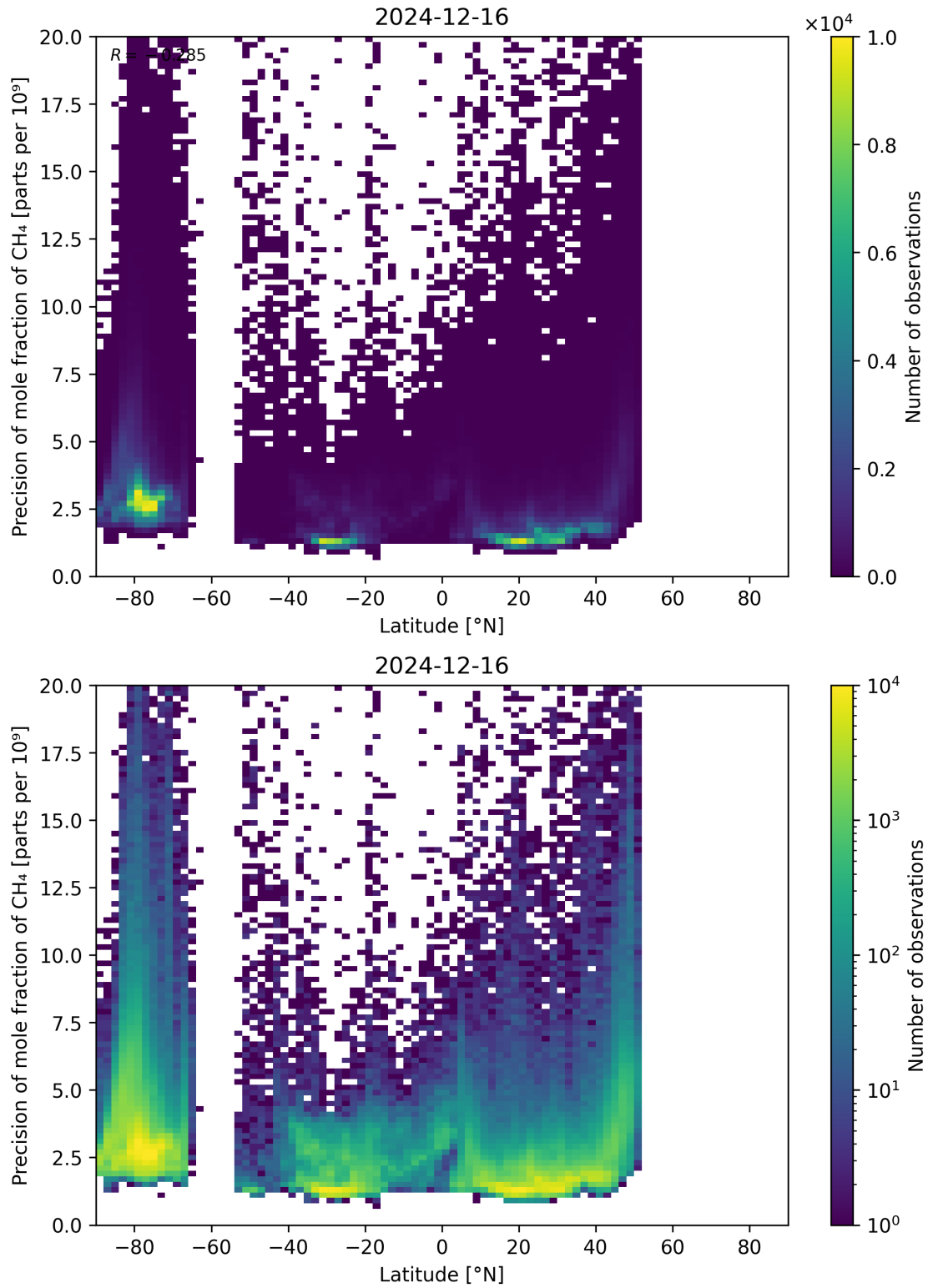
Figure 59: Scatter density plot of “Latitude” against “Precision of mole fraction of \text{CH}_4 ” for 2024-12-16 to 2024-12-17.
