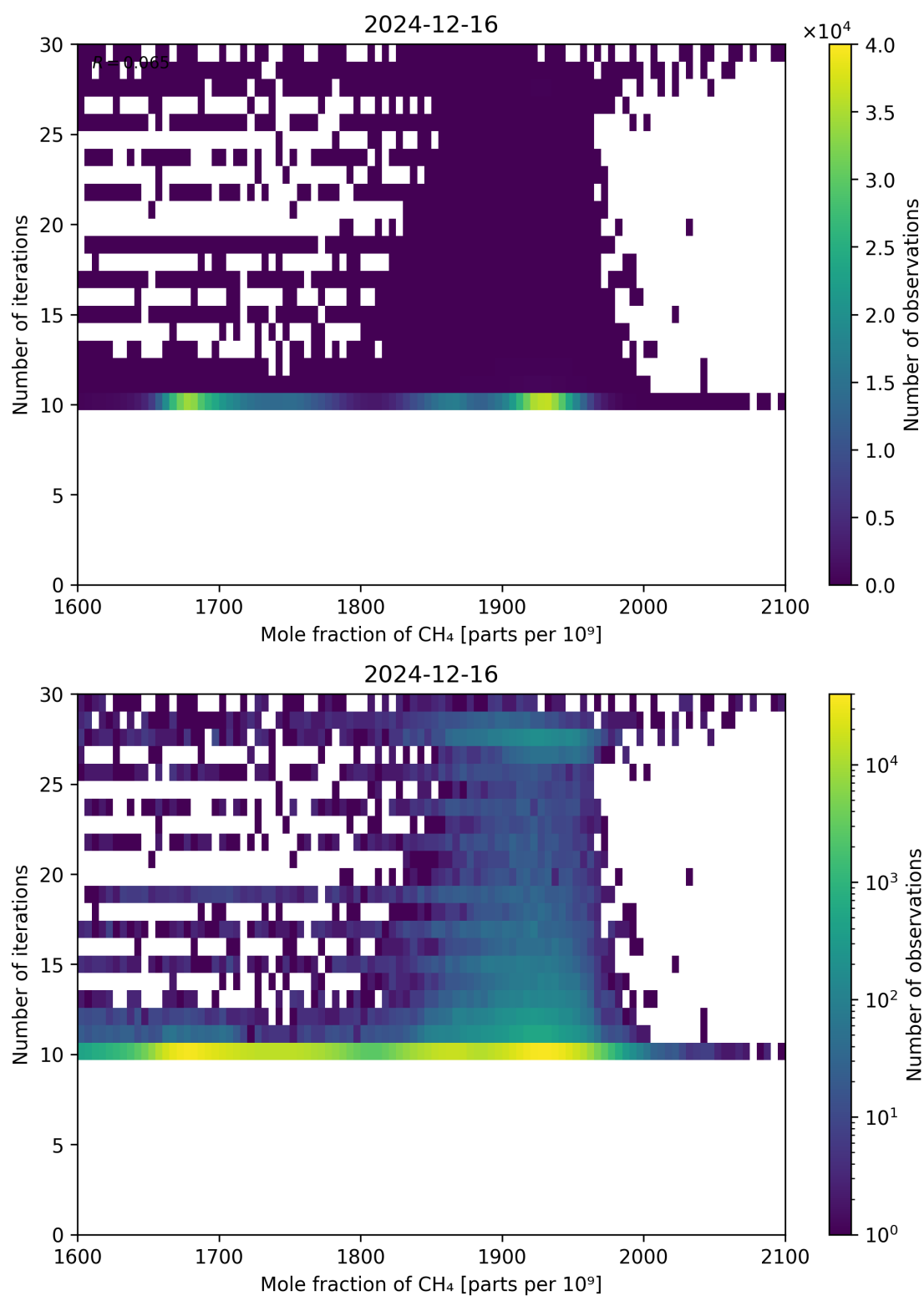
Figure 76: Scatter density plot of “Mole fraction of CH 4 ” against “Number of iterations” for 2024-12-16 to 2024-12-17.
