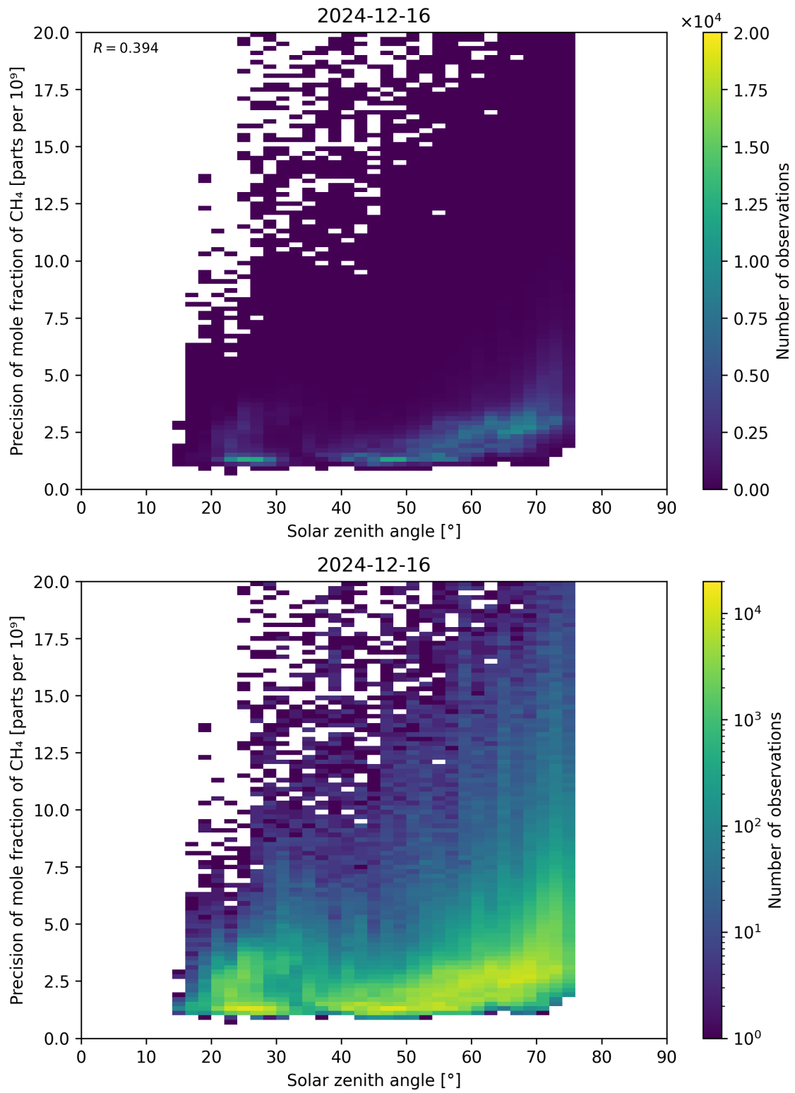
Figure 101: Scatter density plot of “Solar zenith angle” against “Precision of mole fraction of \text{CH}_4 ” for 2024-12-16 to 2024-12-17.
