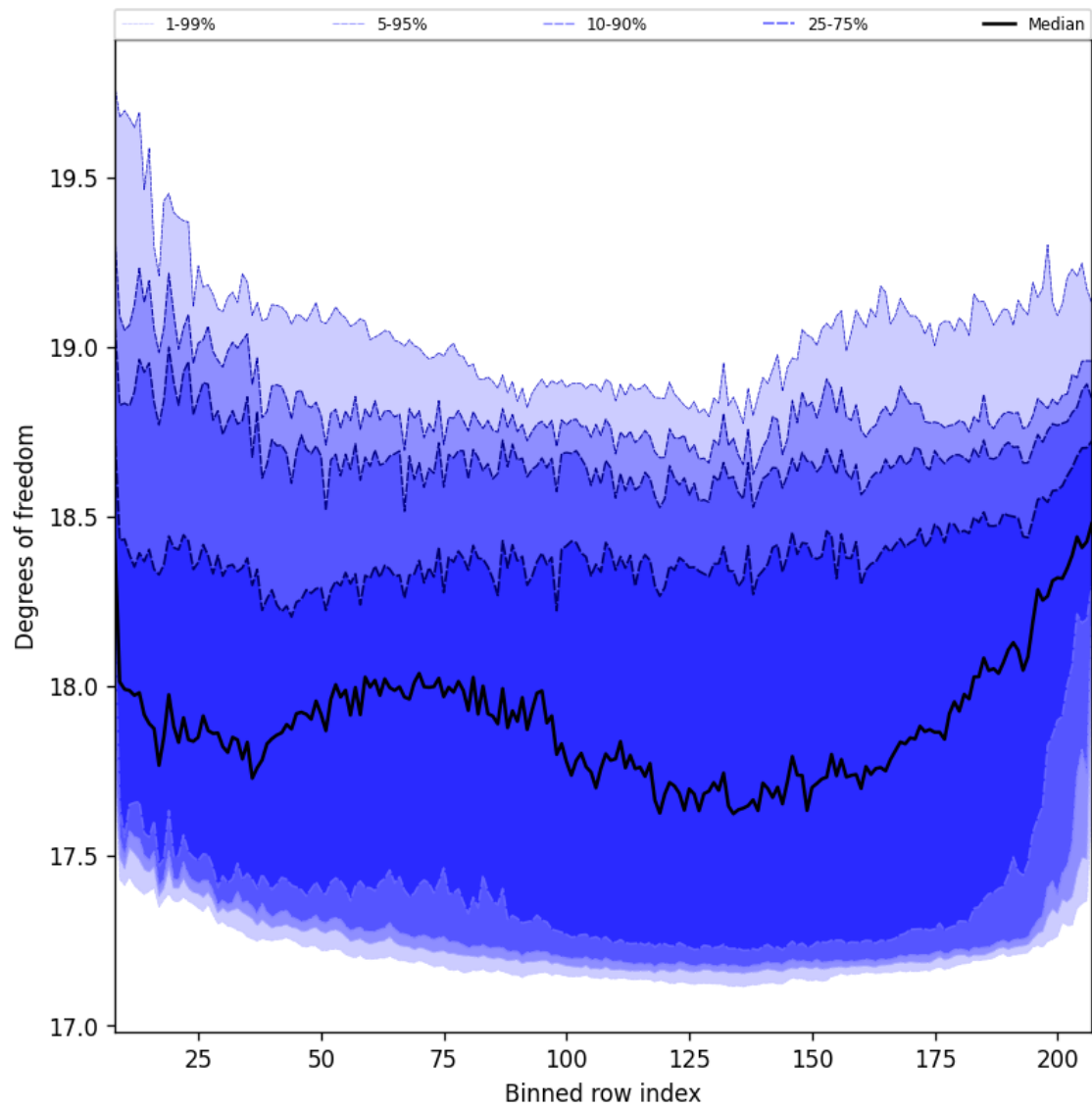
Figure 41: Along track statistics of “Degrees of freedom” for 2024-12-16 to 2024-12-17
