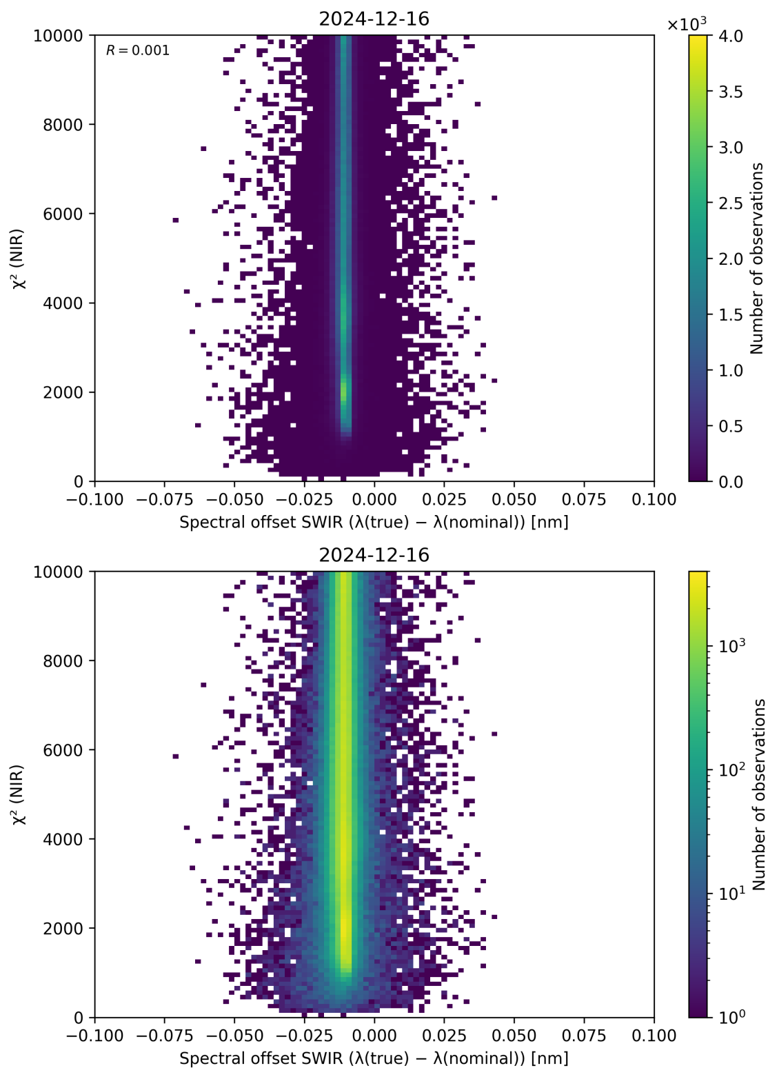
Figure 117: Scatter density plot of “Spectral offset SWIR ( \lambda_{\text{true}} - \lambda_{\text{nominal}} )” against “ \chi^2 (NIR)” for 2024-12-16 to 2024-12-17.
