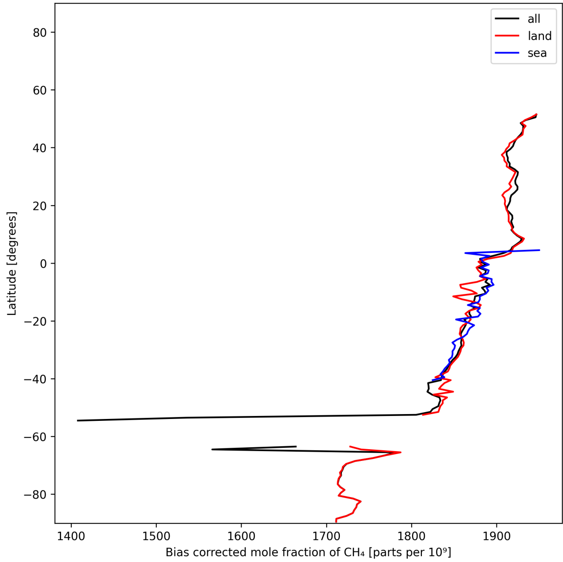
Figure 14: Zonal average of “Bias corrected mole fraction of CH 4 ” for 2024-12-16 to 2024-12-17.
