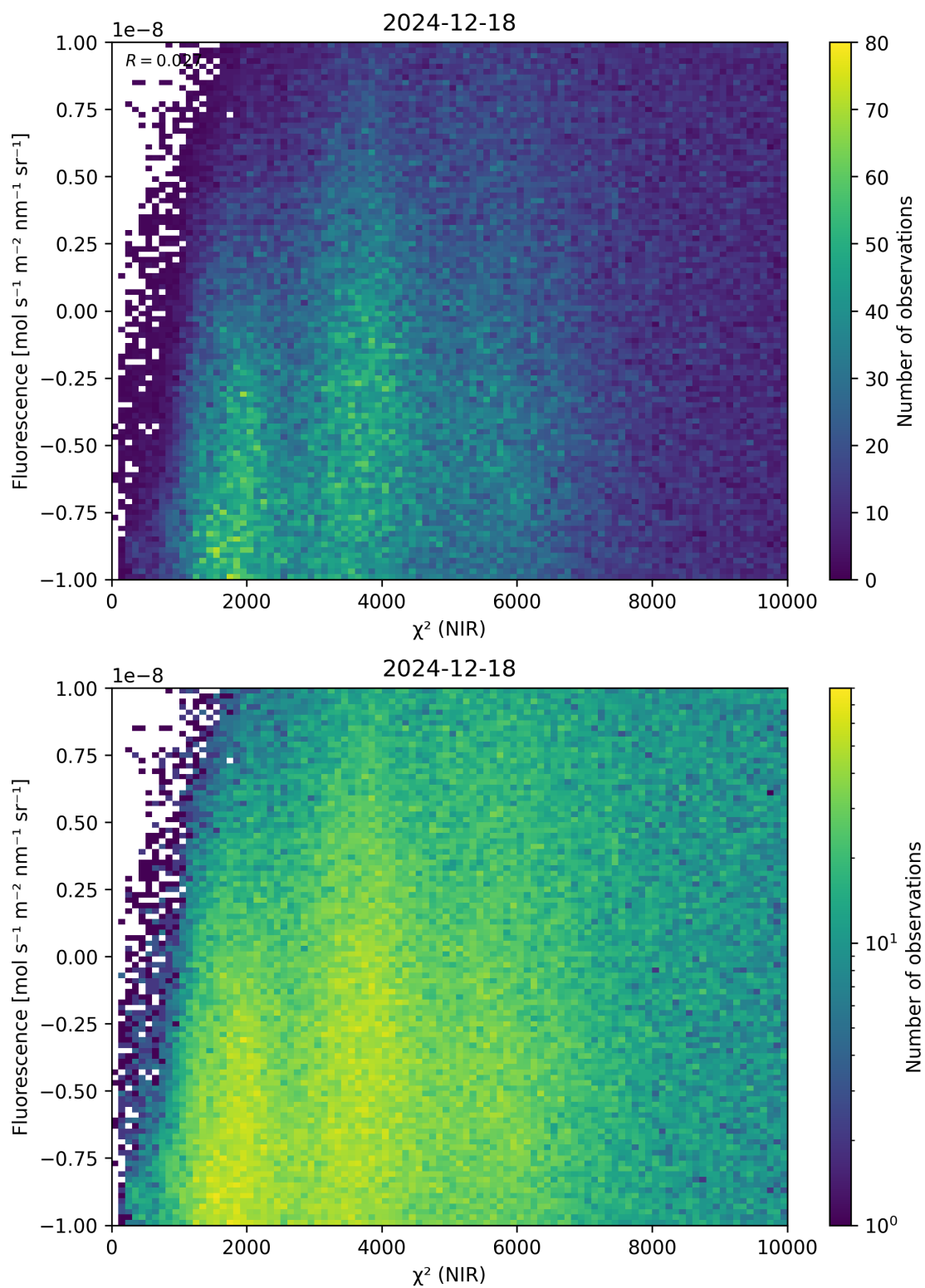
Figure 45: Scatter density plot of “ \chi^2 (NIR)” against “Fluorescence” for 2024-12-17 to 2024-12-19.
