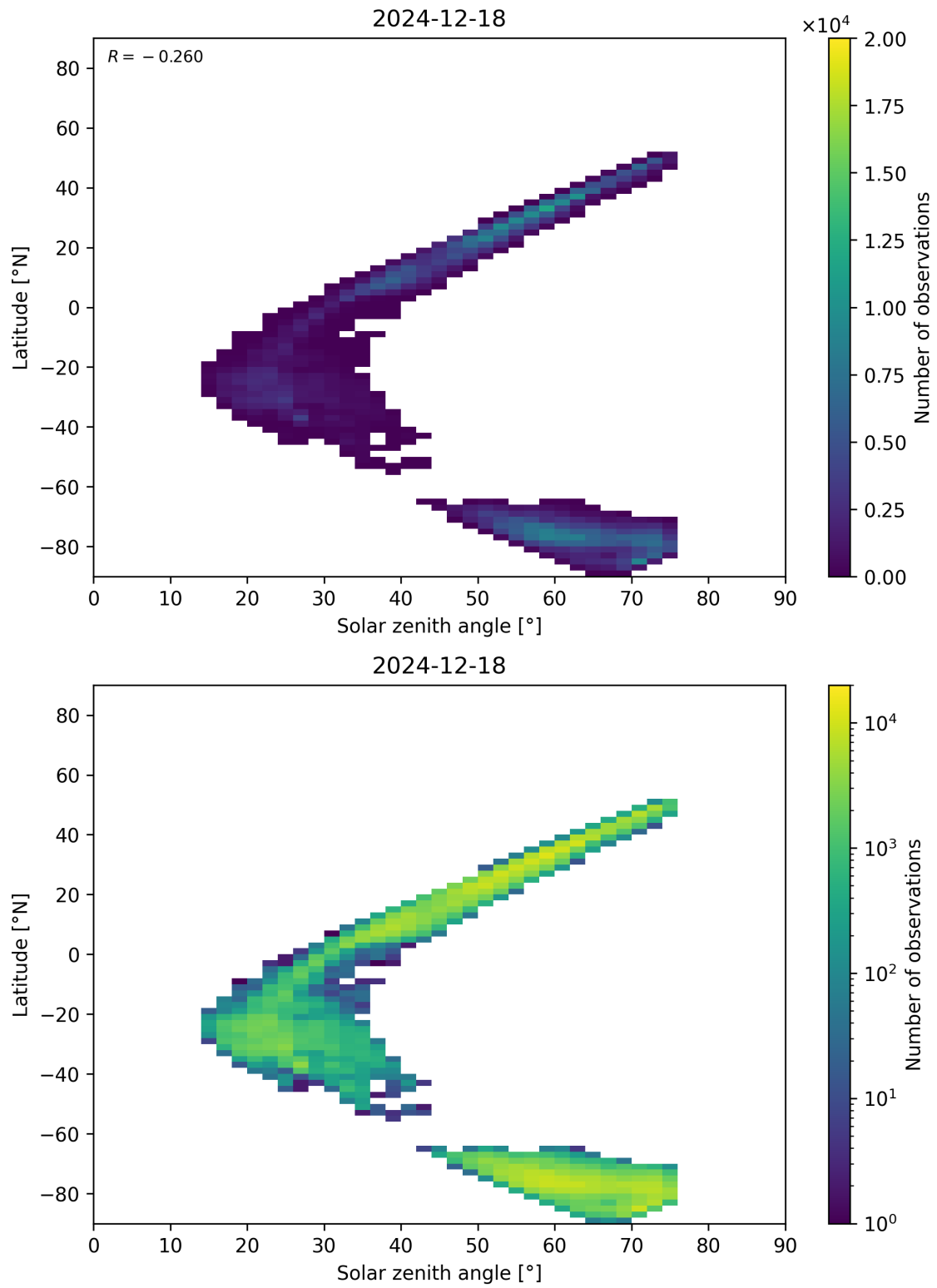
Figure 98: Scatter density plot of “Solar zenith angle” against “Latitude” for 2024-12-17 to 2024-12-19.
