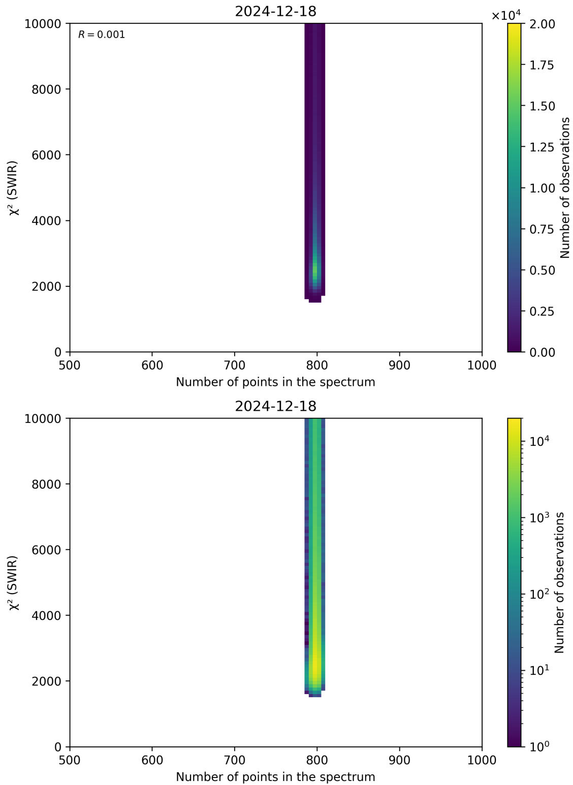
Figure 89: Scatter density plot of “Number of points in the spectrum” against “ \chi^2 (SWIR)” for 2024-12-17 to 2024-12-19.
