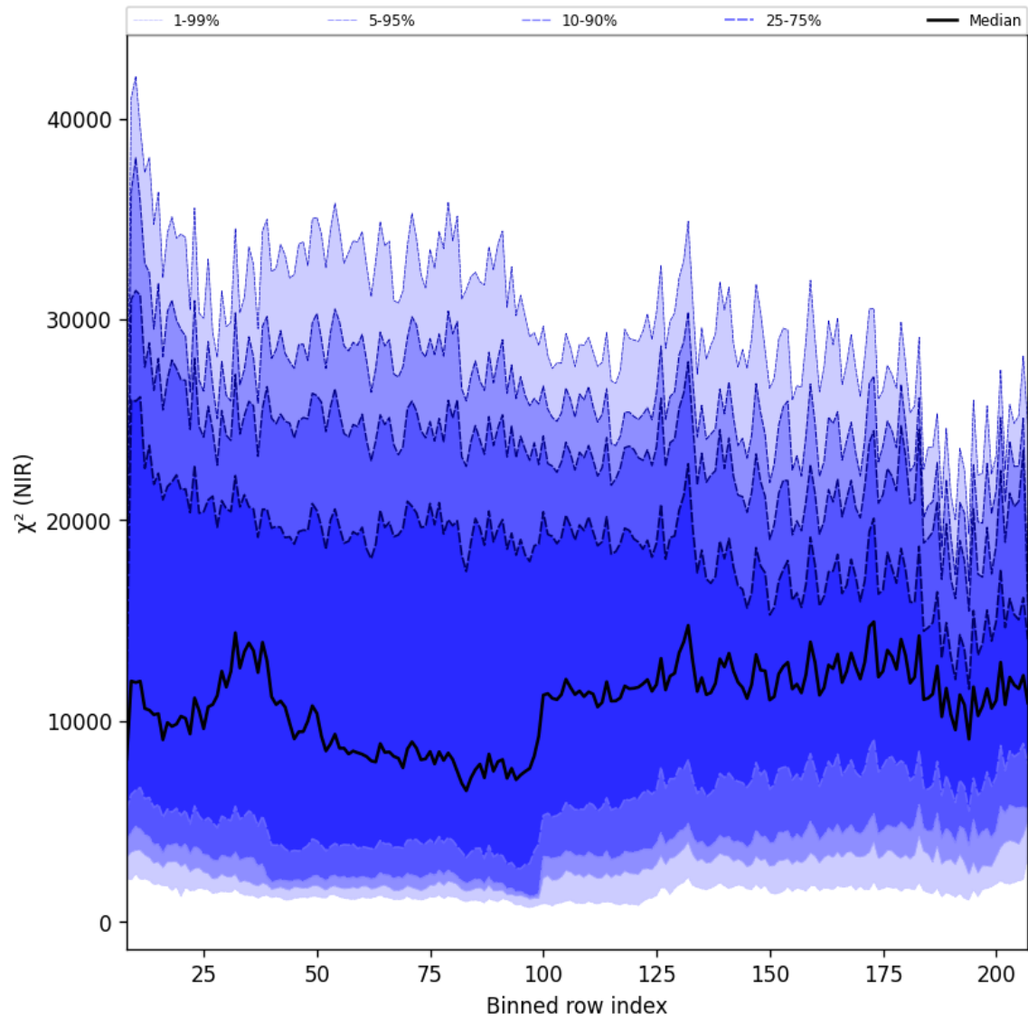
Figure 40: Along track statistics of “ \chi^2 (NIR)” for 2024-12-17 to 2024-12-19
