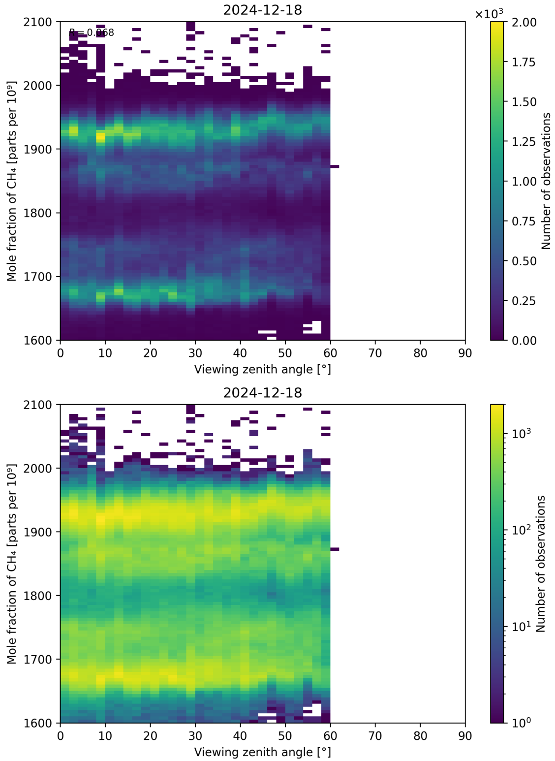
Figure 110: Scatter density plot of “Viewing zenith angle” against “Mole fraction of CH 4 ” for 2024-12-17 to 2024-12-19.
