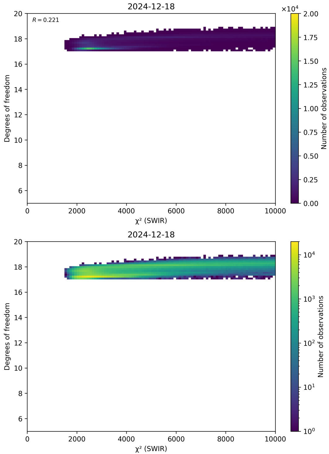
Figure 48: Scatter density plot of “ \chi^2 (SWIR)” against “Degrees of freedom” for 2024-12-17 to 2024-12-19.
