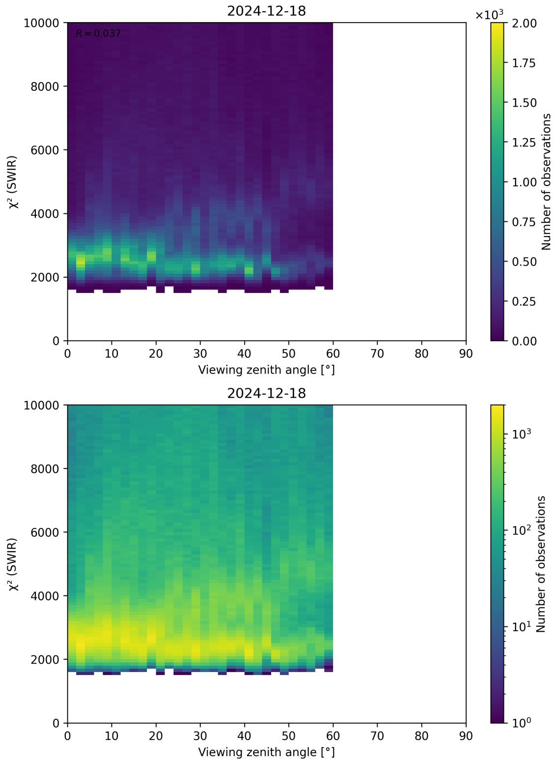
Figure 106: Scatter density plot of “Viewing zenith angle” against “ \chi^2 (SWIR)” for 2024-12-17 to 2024-12-19.
