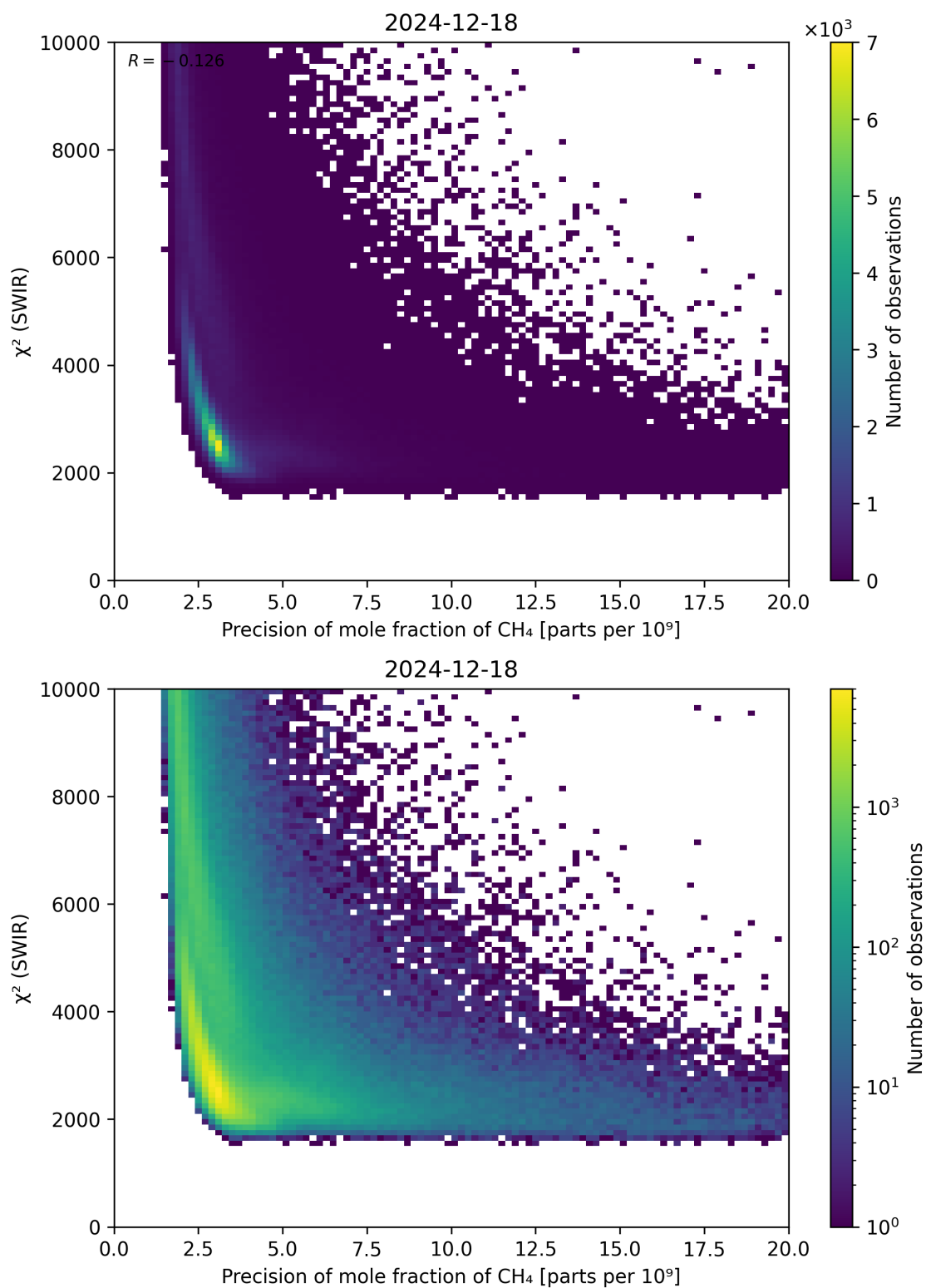
Figure 79: Scatter density plot of “Precision of mole fraction of \text{CH}_4 ” against “ \chi^2 (SWIR)” for 2024-12-17 to 2024-12-19.
