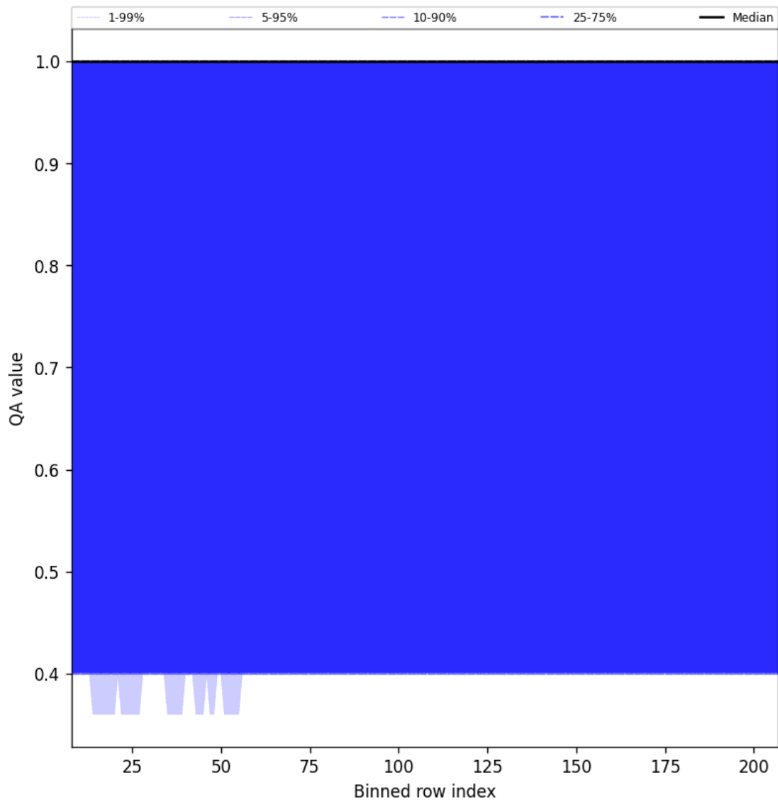
Figure 33: Along track statistics of “QA value” for 2024-12-17 to 2024-12-19
