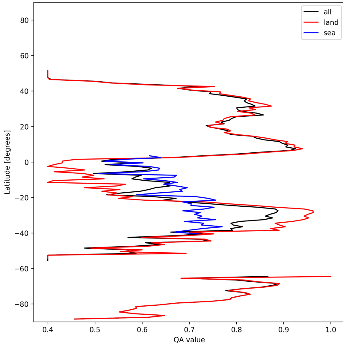
Figure 11: Zonal average of “QA value” for 2024-12-17 to 2024-12-19.
