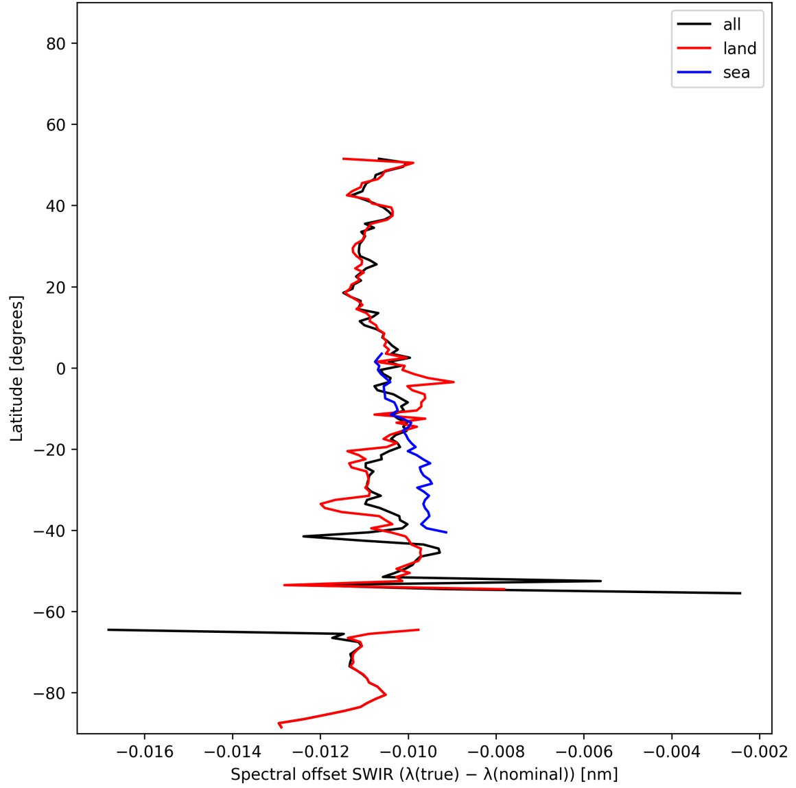
Figure 16: Zonal average of “Spectral offset SWIR ( \lambda_{\text{true}} - \lambda_{\text{nominal}} )” for 2024-12-17 to 2024-12-19.
