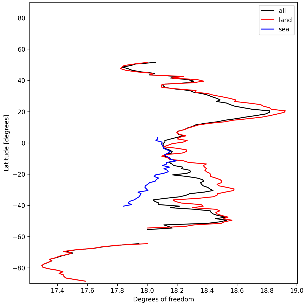
Figure 19: Zonal average of “Degrees of freedom” for 2024-12-17 to 2024-12-19.
