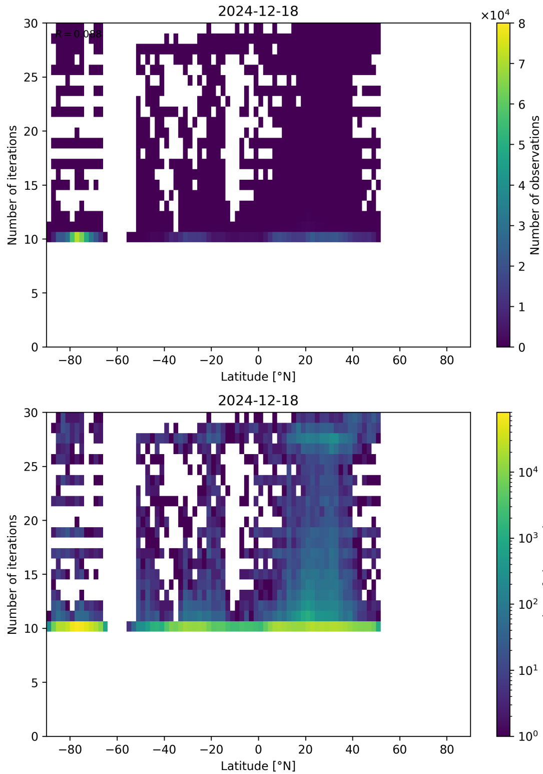
Figure 60: Scatter density plot of “Latitude” against “Number of iterations” for 2024-12-17 to 2024-12-19.
