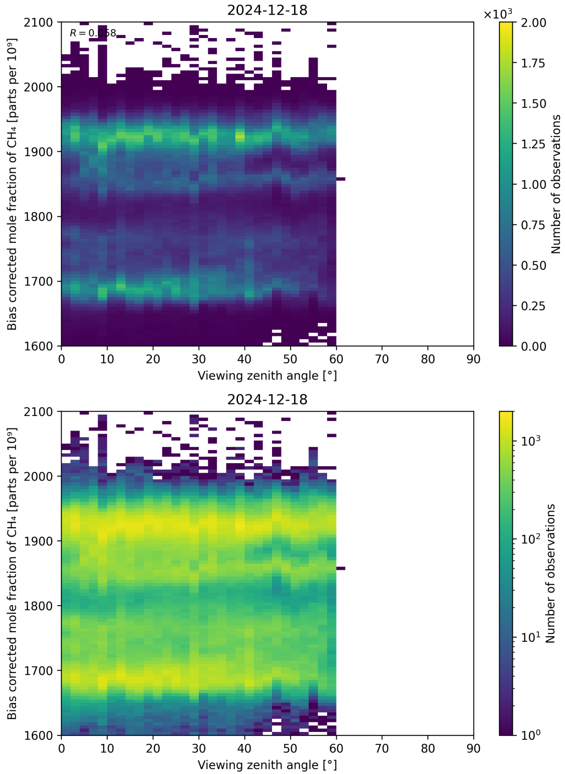
Figure 111: Scatter density plot of “Viewing zenith angle” against “Bias corrected mole fraction of CH 4 ” for 2024-12-17 to 2024-12-19.
