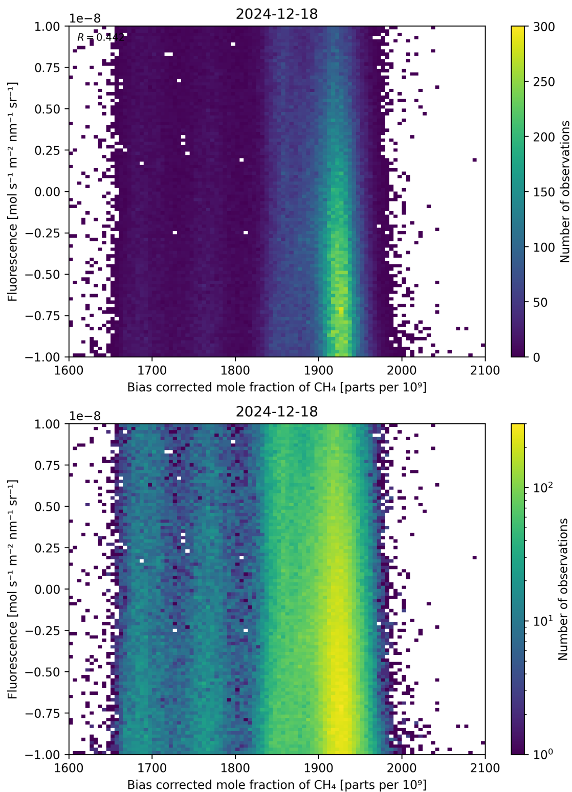
Figure 66: Scatter density plot of “Bias corrected mole fraction of \text{CH}_4 ” against “Fluorescence” for 2024-12-17 to 2024-12-19.
