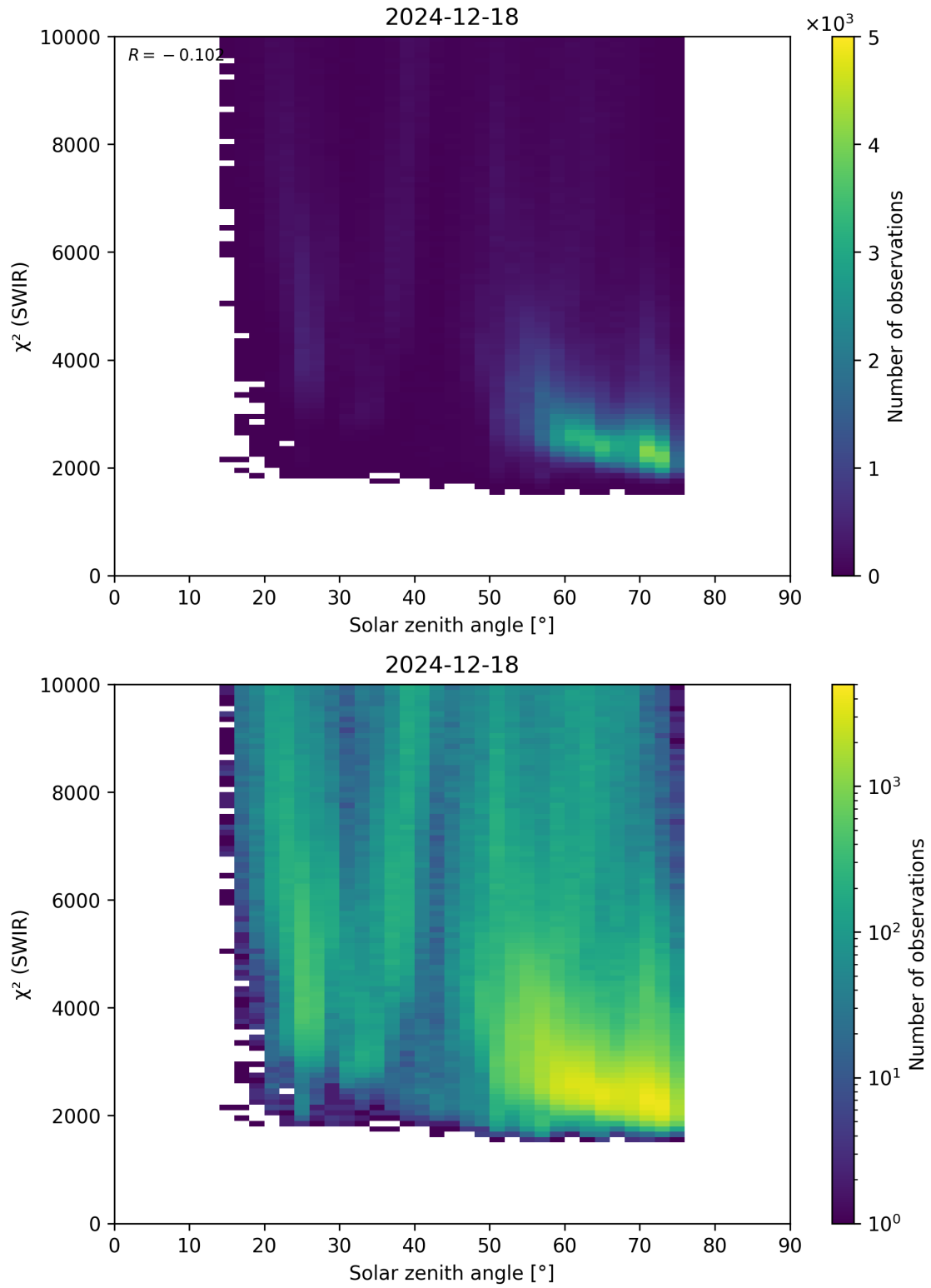
Figure 95: Scatter density plot of “Solar zenith angle” against “ \chi^2 (SWIR)” for 2024-12-17 to 2024-12-19.
