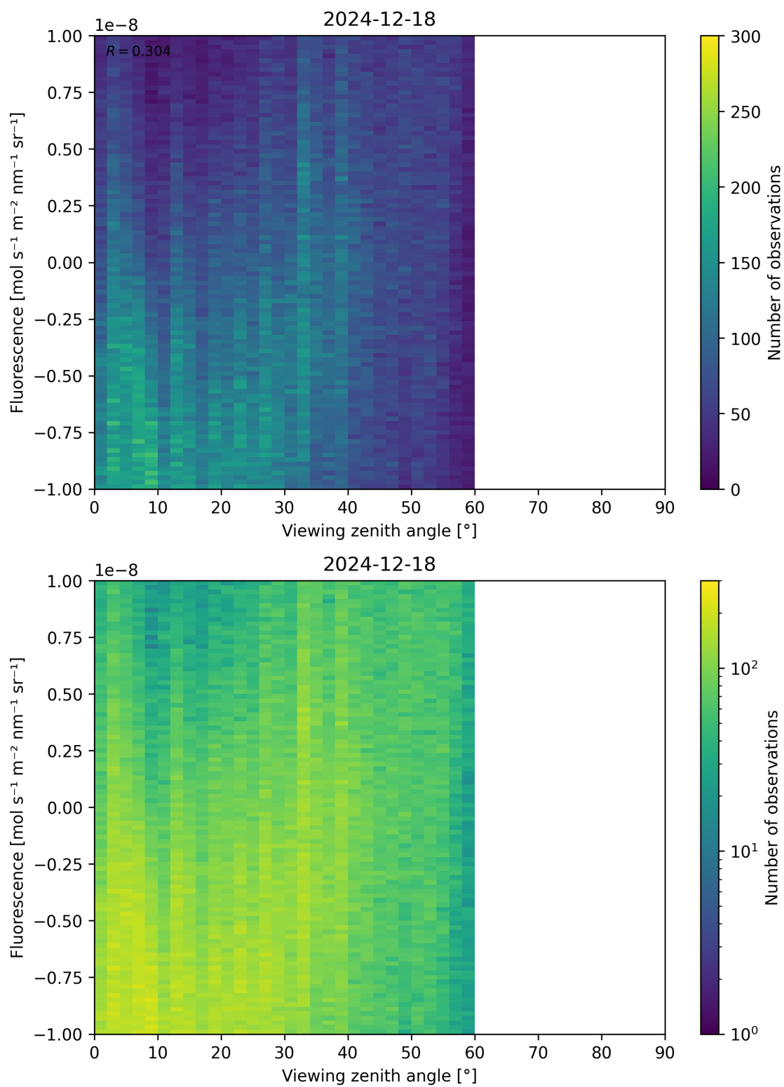
Figure 108: Scatter density plot of “Viewing zenith angle” against “Fluorescence” for 2024-12-17 to 2024-12-19.
