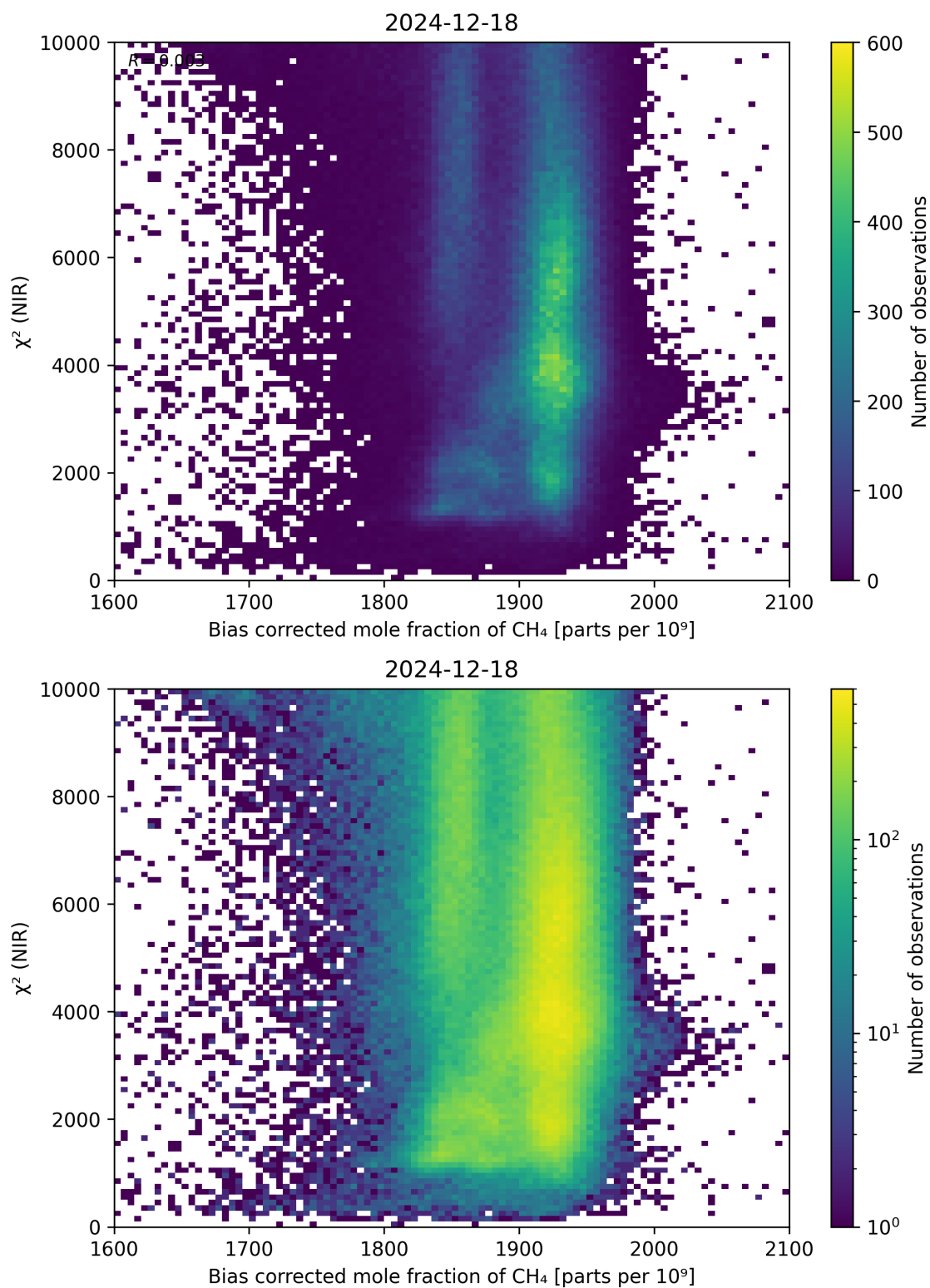
Figure 63: Scatter density plot of “Bias corrected mole fraction of \text{CH}_4 ” against “ \chi^2 (NIR)” for 2024-12-17 to 2024-12-19.
