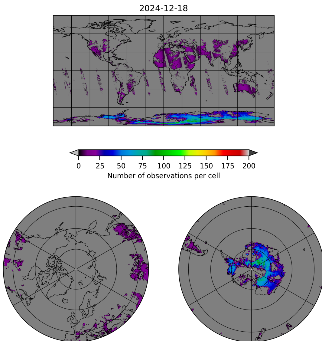
Figure 10: Map of the number of observations for 2024-12-17 to 2024-12-19
