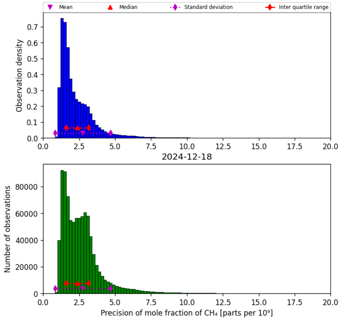
Figure 24: Histogram of “Precision of mole fraction of CH 4 ” for 2024-12-17 to 2024-12-19
