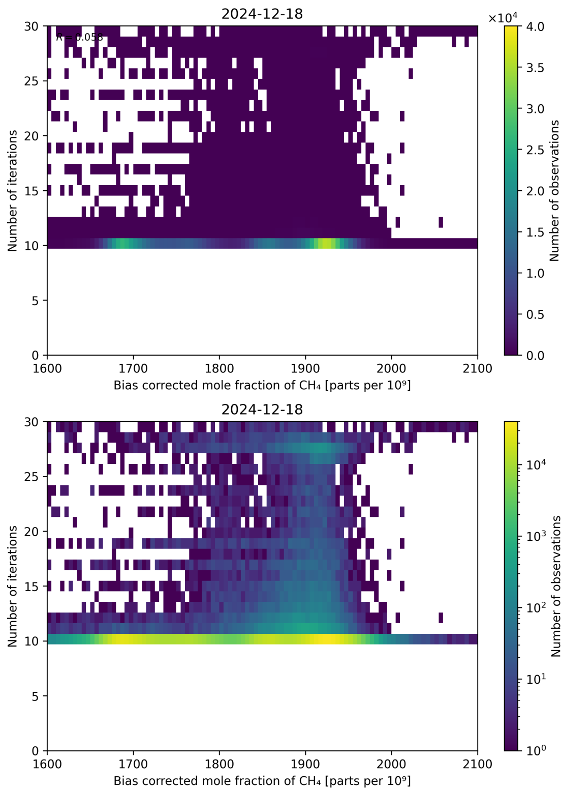
Figure 67: Scatter density plot of “Bias corrected mole fraction of CH 4 ” against “Number of iterations” for 2024-12-17 to 2024-12-19.
