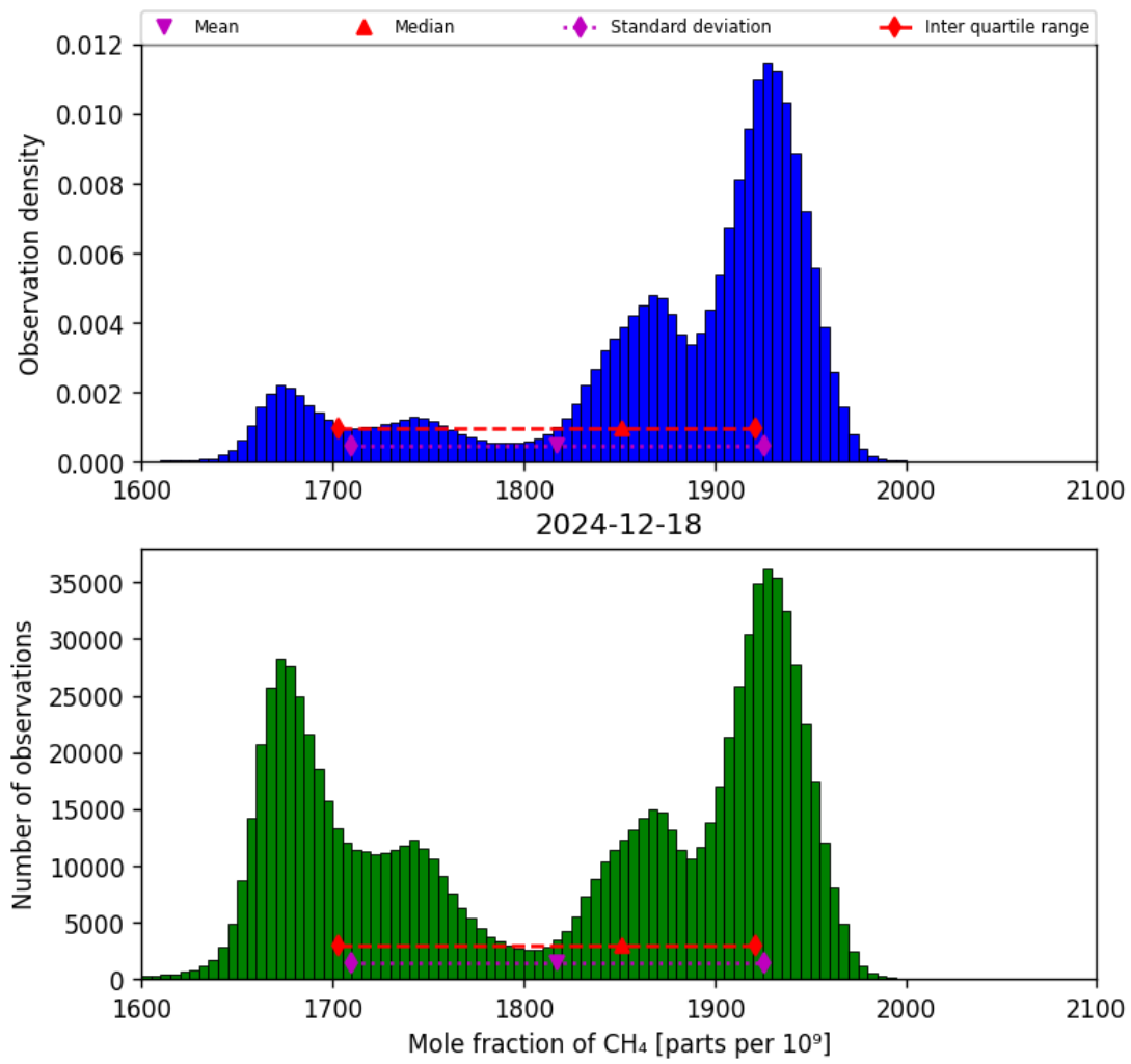
Figure 23: Histogram of “Mole fraction of CH 4 ” for 2024-12-17 to 2024-12-19
