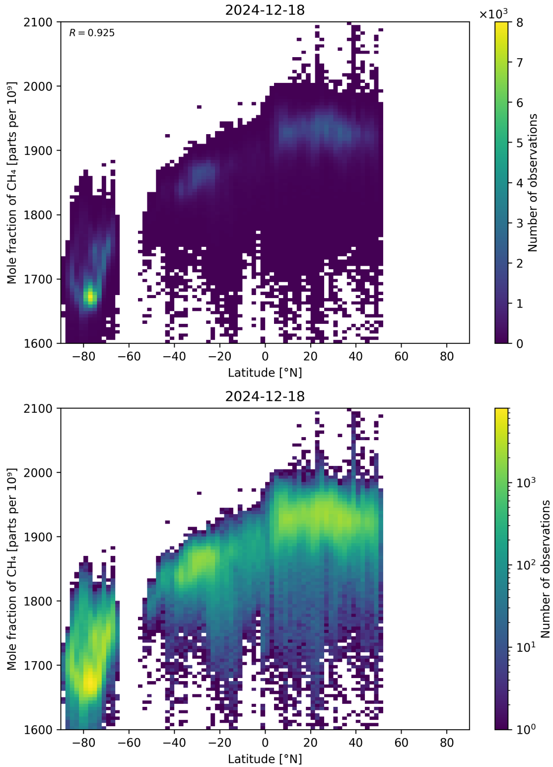
Figure 57: Scatter density plot of “Latitude” against “Mole fraction of CH 4 ” for 2024-12-17 to 2024-12-19.
