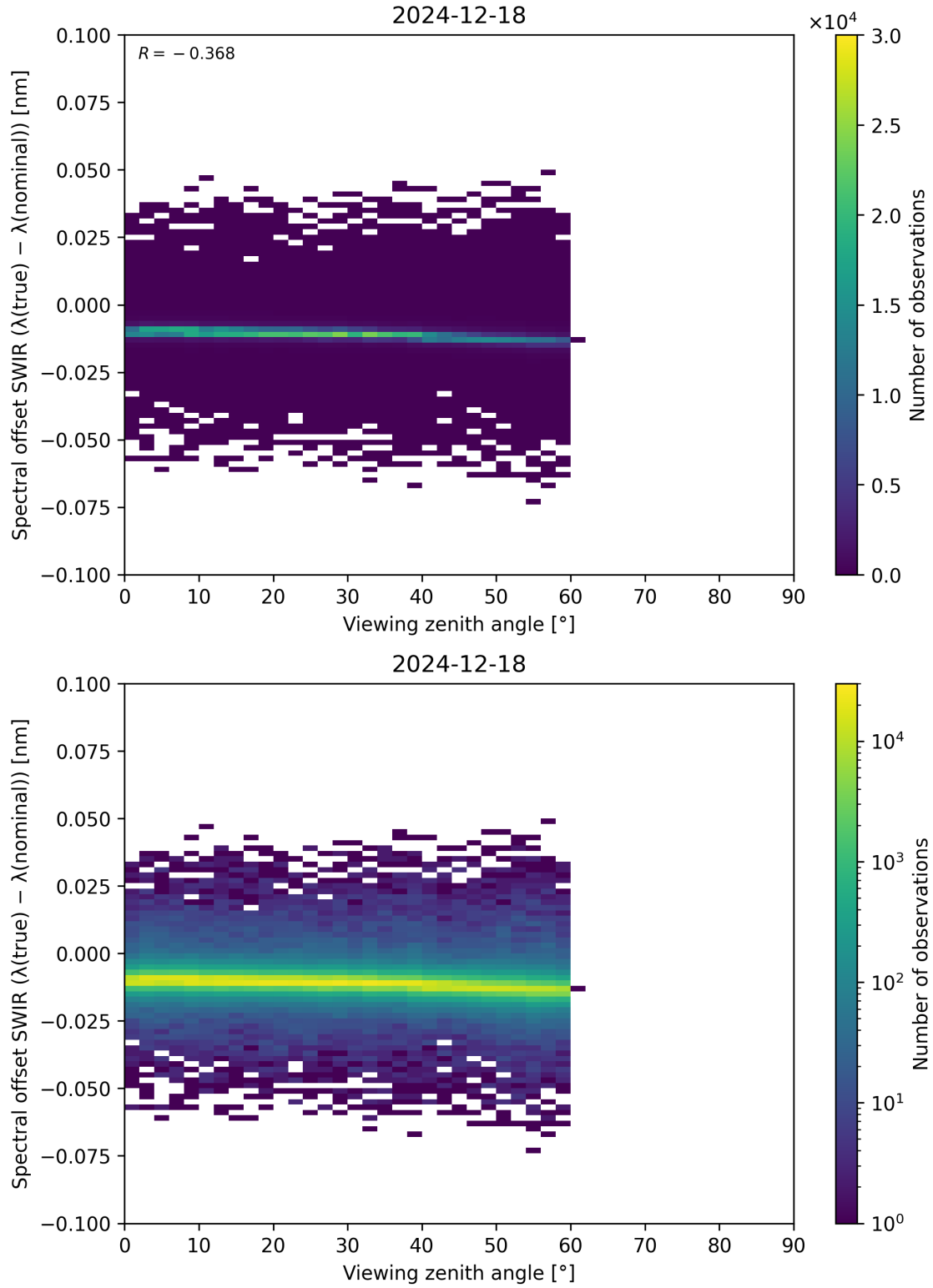
Figure 116: Scatter density plot of “Viewing zenith angle” against “Spectral offset SWIR ( \lambda_{\text{true}} - \lambda_{\text{nominal}} )” for 2024-12-17 to 2024-12-19.
