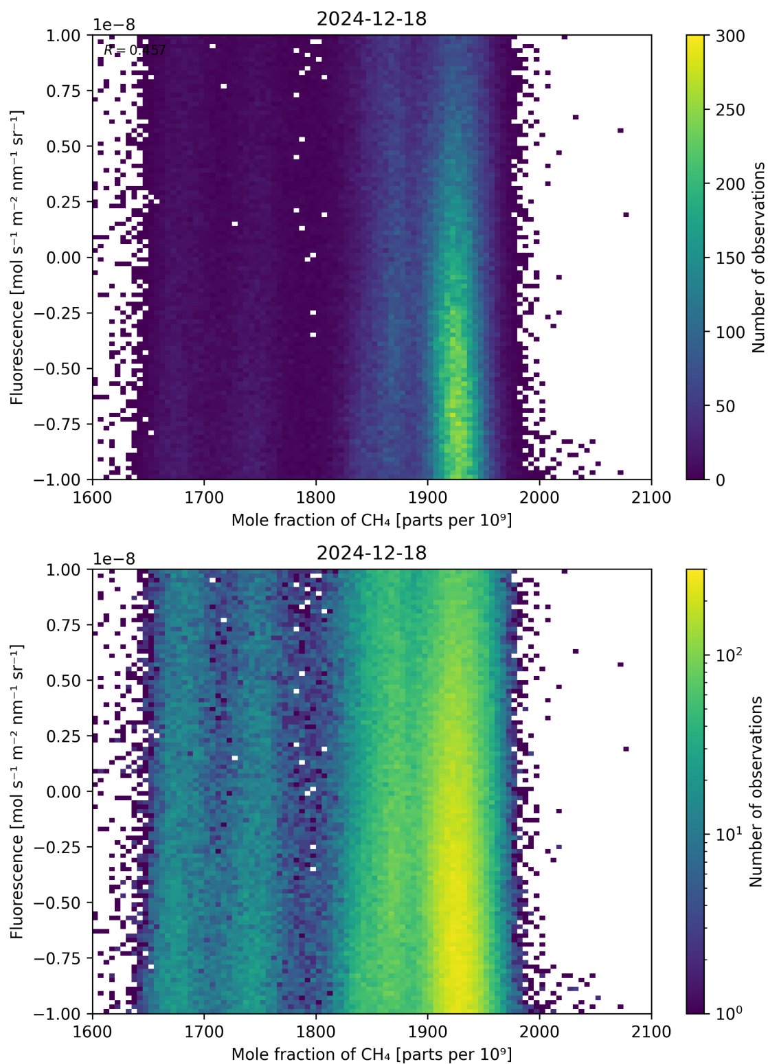
Figure 73: Scatter density plot of “Mole fraction of \text{CH}_4 ” against “Fluorescence” for 2024-12-17 to 2024-12-19.
