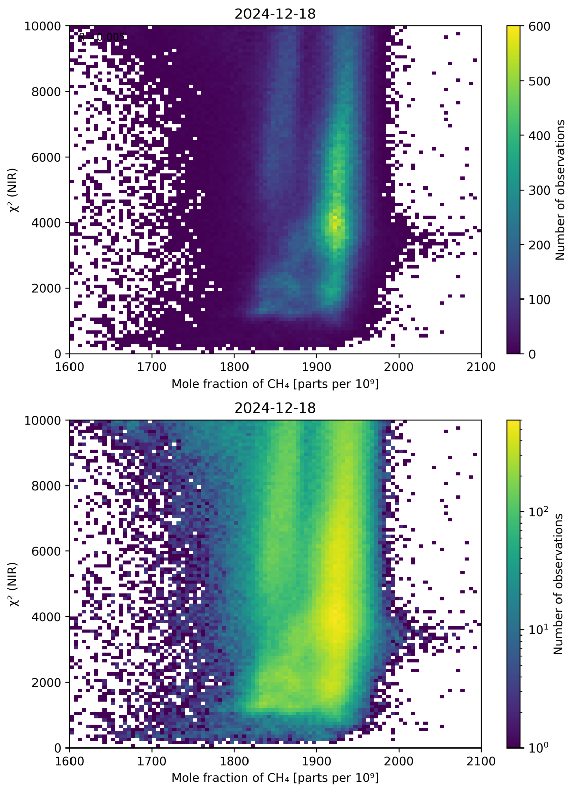
Figure 70: Scatter density plot of “Mole fraction of CH 4 ” against “ \chi^2 (NIR)” for 2024-12-17 to 2024-12-19.
