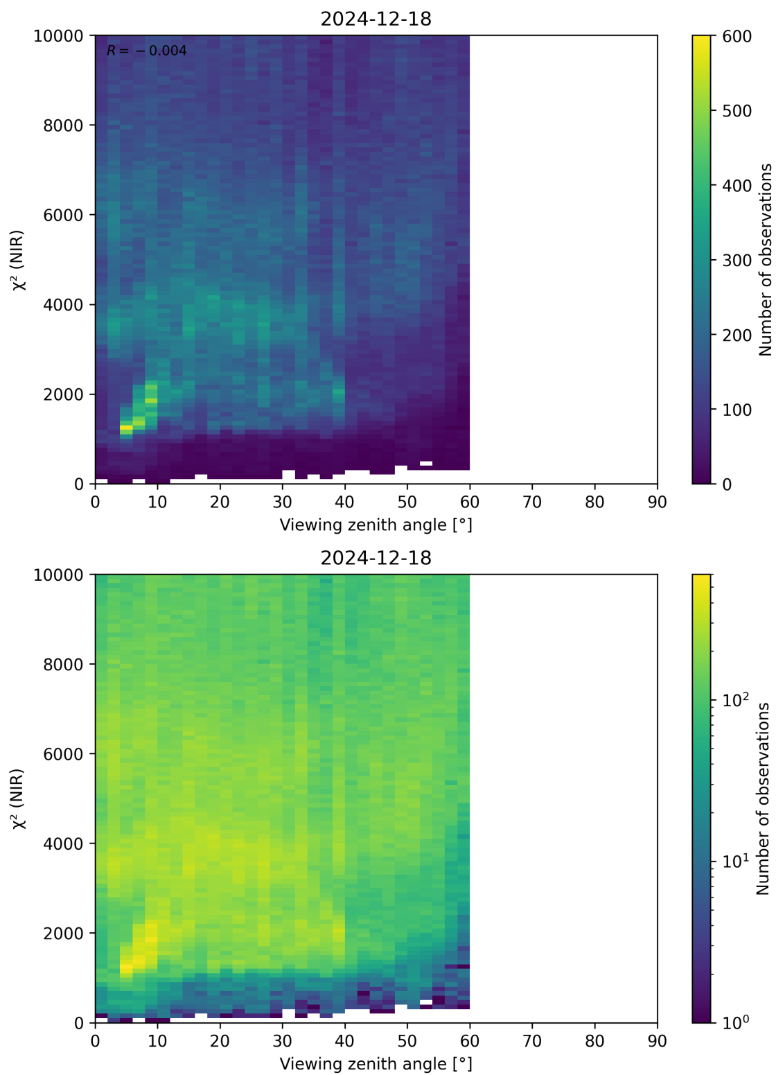
Figure 105: Scatter density plot of “Viewing zenith angle” against “ \chi^2 (NIR)” for 2024-12-17 to 2024-12-19.
