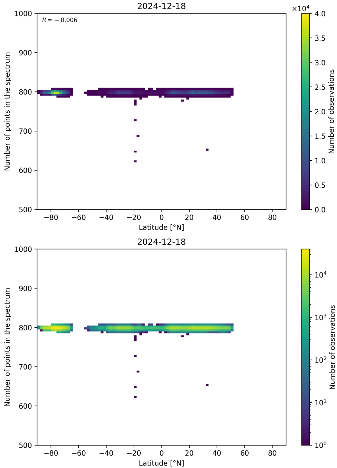
Figure 61: Scatter density plot of “Latitude” against “Number of points in the spectrum” for 2024-12-17 to 2024-12-19.
