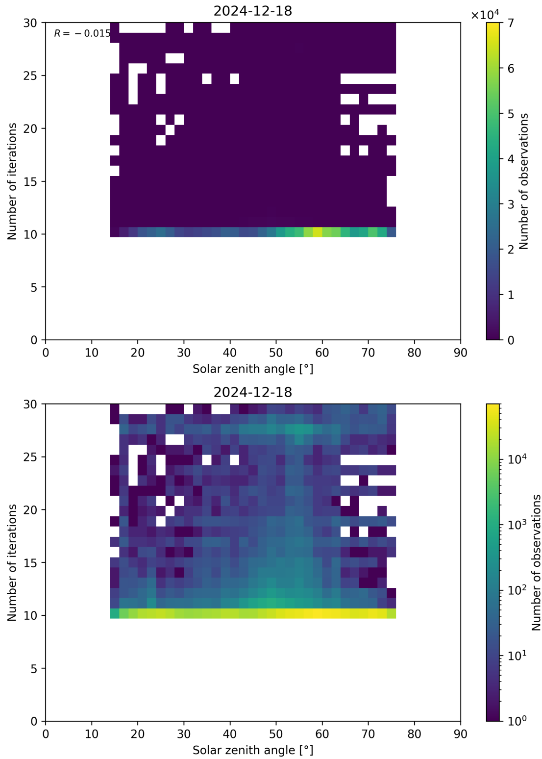
Figure 102: Scatter density plot of “Solar zenith angle” against “Number of iterations” for 2024-12-17 to 2024-12-19.
