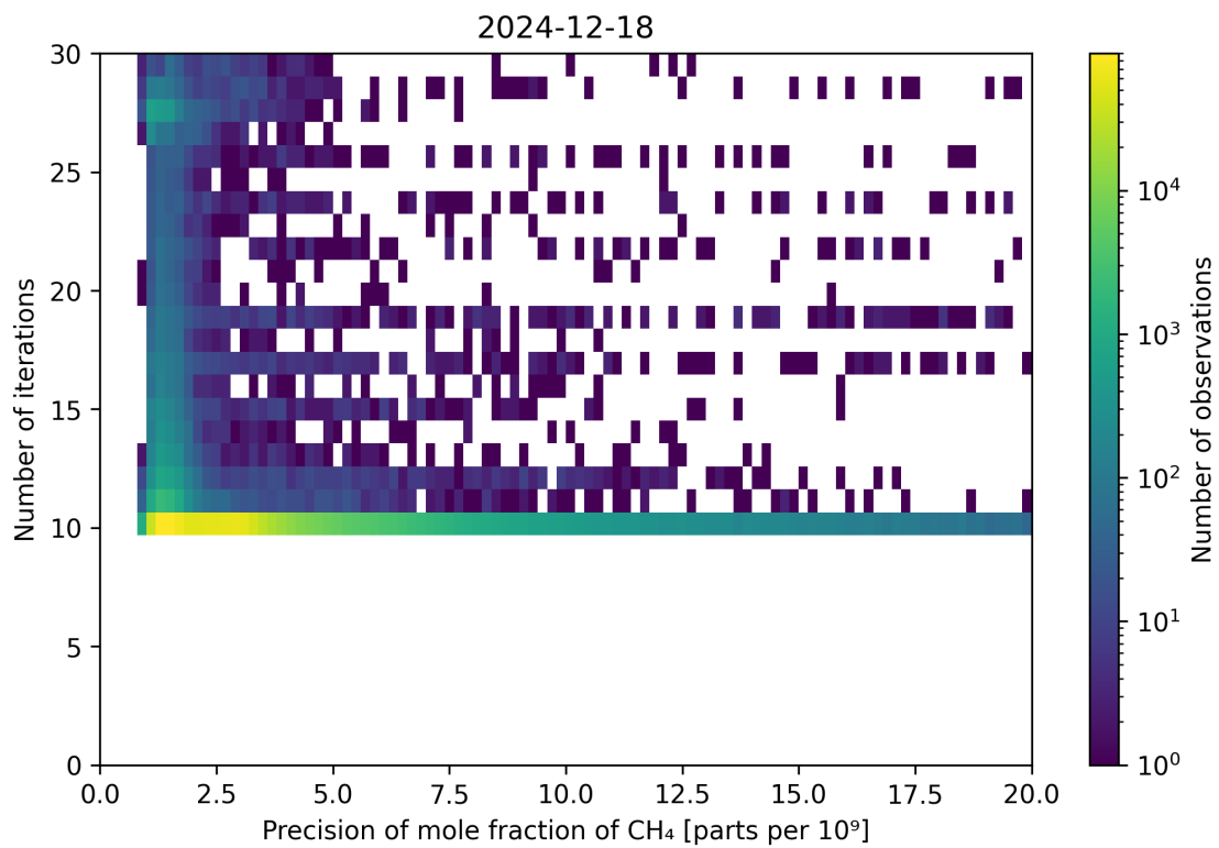
Figure 83: Scatter density plot of “Precision of mole fraction of \text{CH}_4 ” against “Number of iterations” for 2024-12-17 to 2024-12-19.
