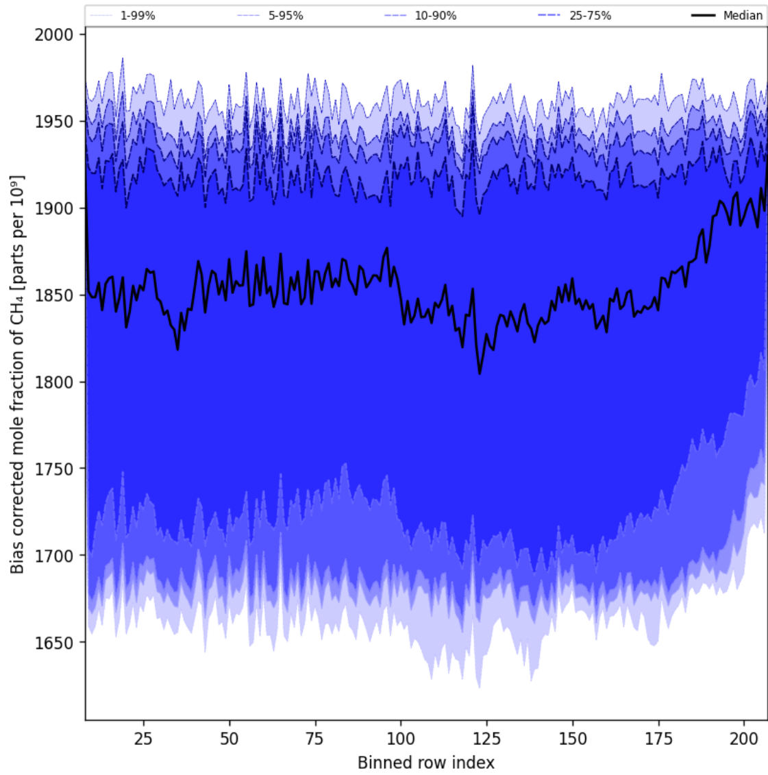
Figure 36: Along track statistics of “Bias corrected mole fraction of CH 4 ” for 2024-12-17 to 2024-12-19
