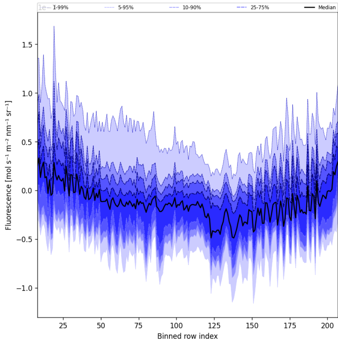
Figure 43: Along track statistics of “Fluorescence” for 2024-12-17 to 2024-12-19
