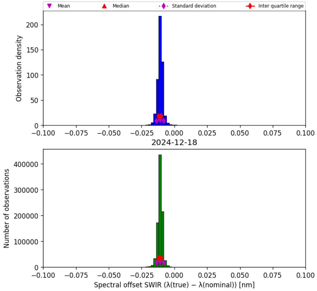
Figure 27: Histogram of “Spectral offset SWIR ( \lambda_{\text{true}} - \lambda_{\text{nominal}} )” for 2024-12-17 to 2024-12-19
