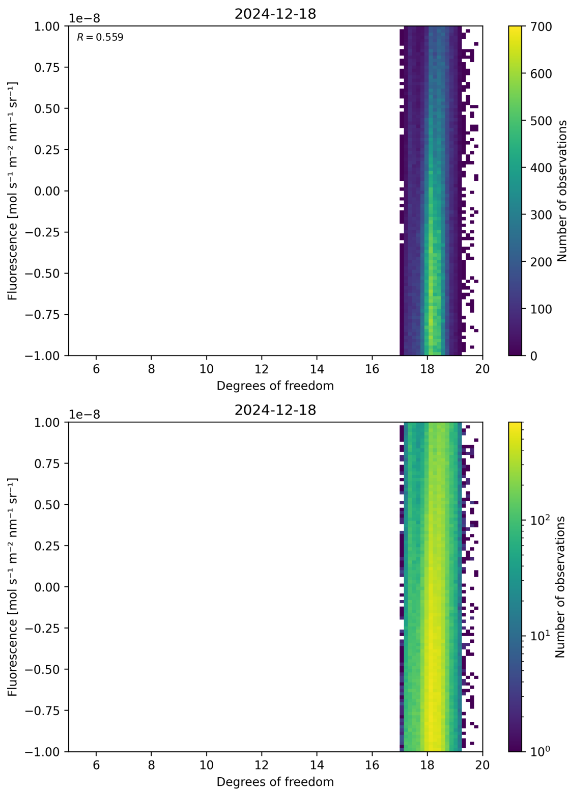
Figure 51: Scatter density plot of “Degrees of freedom” against “Fluorescence” for 2024-12-17 to 2024-12-19.
