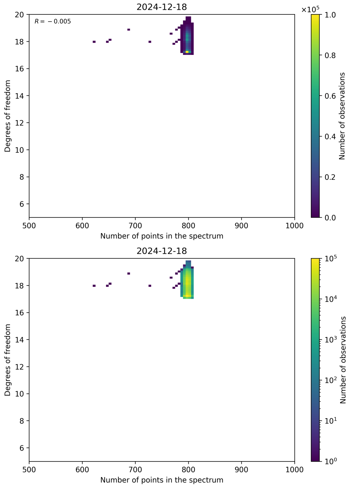
Figure 90: Scatter density plot of “Number of points in the spectrum” against “Degrees of freedom” for 2024-12-17 to 2024-12-19.
