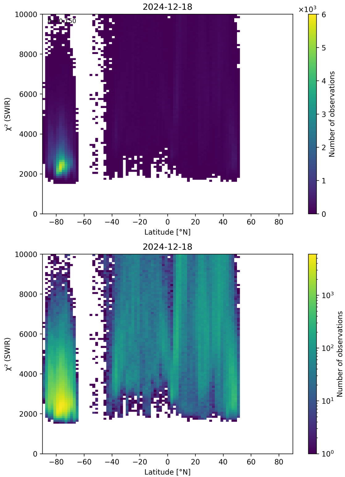
Figure 54: Scatter density plot of “Latitude” against “ \chi^2 (SWIR)” for 2024-12-17 to 2024-12-19.
