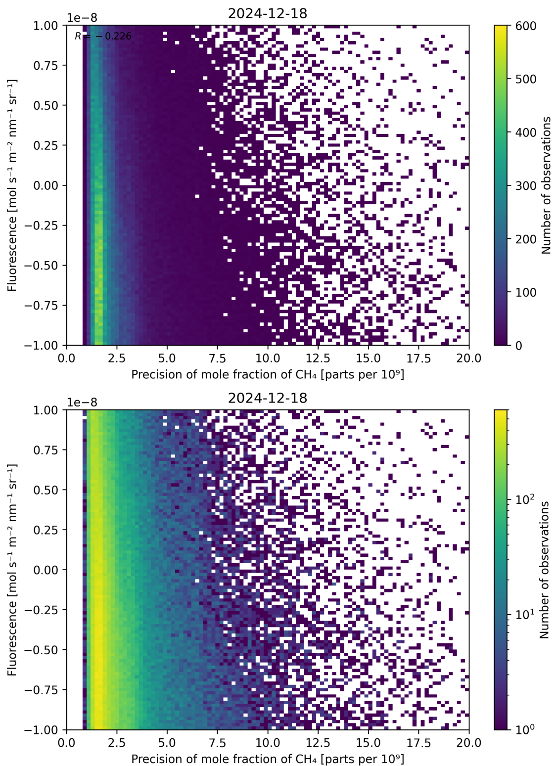
Figure 81: Scatter density plot of “Precision of mole fraction of \text{CH}_4 ” against “Fluorescence” for 2024-12-17 to 2024-12-19.
