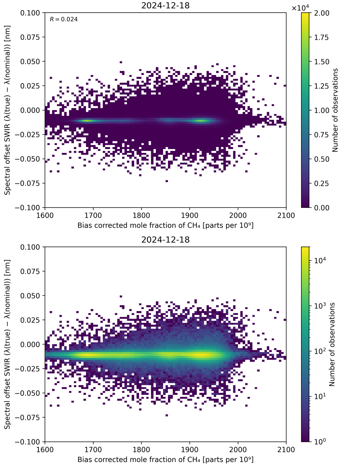
Figure 69: Scatter density plot of “Bias corrected mole fraction of \text{CH}_4 ” against “Spectral offset SWIR ( \lambda_{\text{true}} - \lambda_{\text{nominal}} )” for 2024-12-17 to 2024-12-19.
