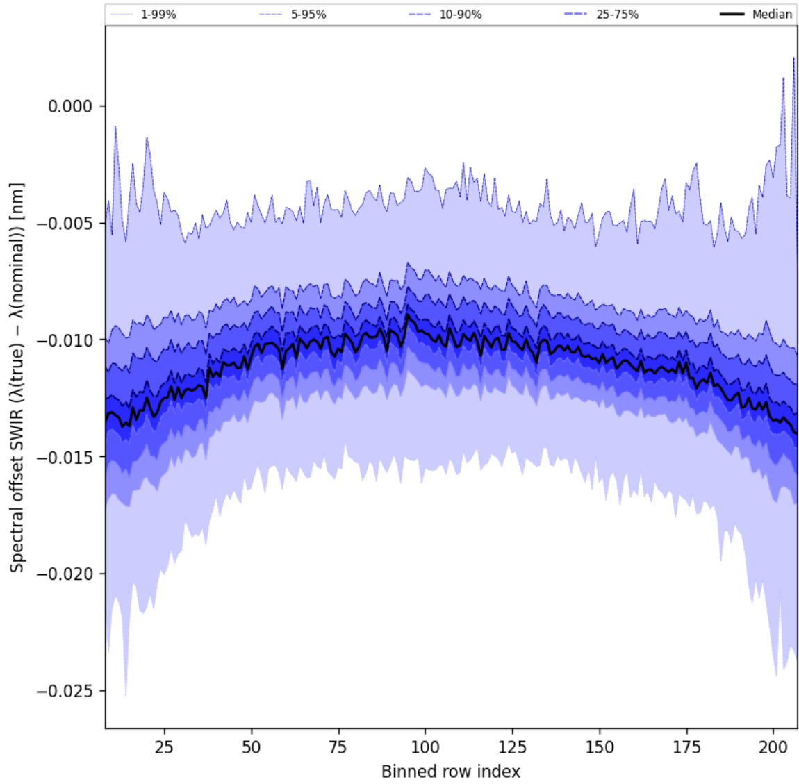
Figure 38: Along track statistics of “Spectral offset SWIR ( \lambda_{\text{true}} - \lambda_{\text{nominal}} )” for 2024-12-17 to 2024-12-19
