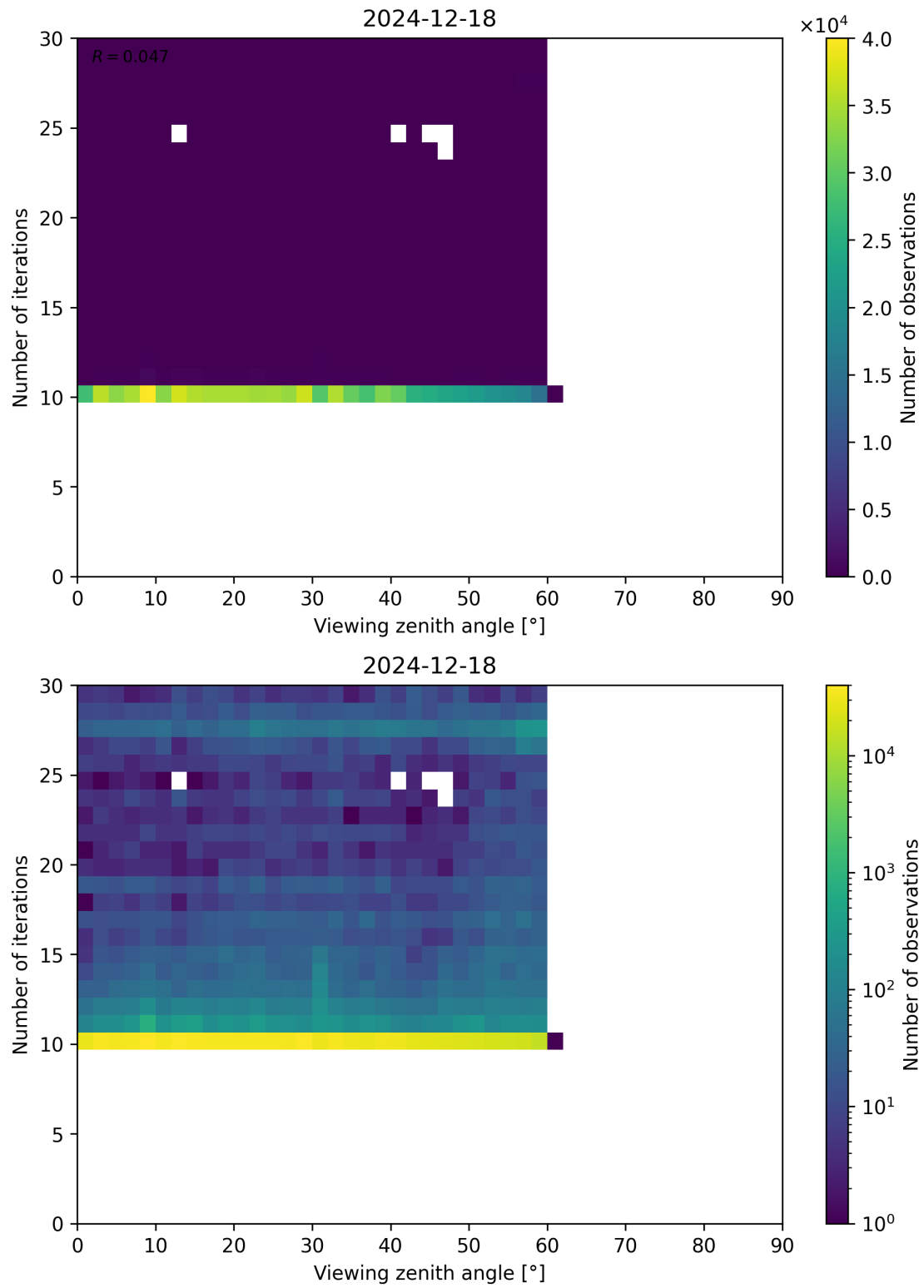
Figure 113: Scatter density plot of “Viewing zenith angle” against “Number of iterations” for 2024-12-17 to 2024-12-19.
