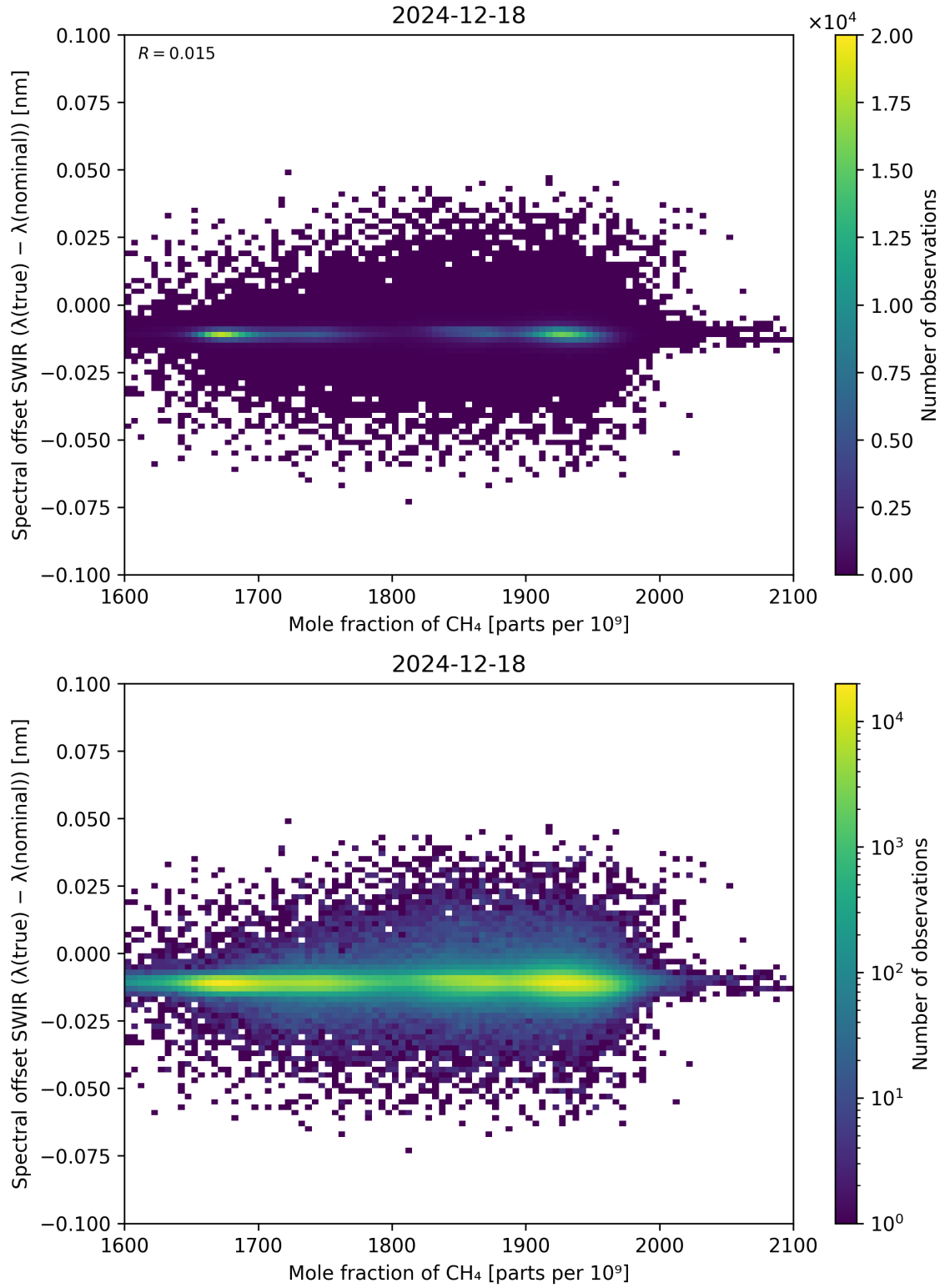
Figure 86: Scatter density plot of “Mole fraction of CH 4 ” against “Spectral offset SWIR ( \lambda_{\text{true}} - \lambda_{\text{nominal}} )” for 2024-12-17 to 2024-12-19.
