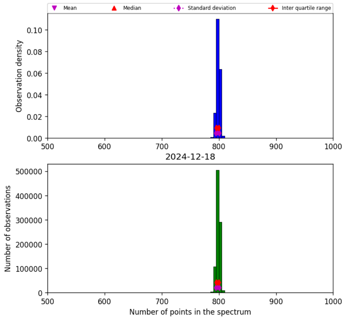
Figure 26: Histogram of “Number of points in the spectrum” for 2024-12-17 to 2024-12-19
