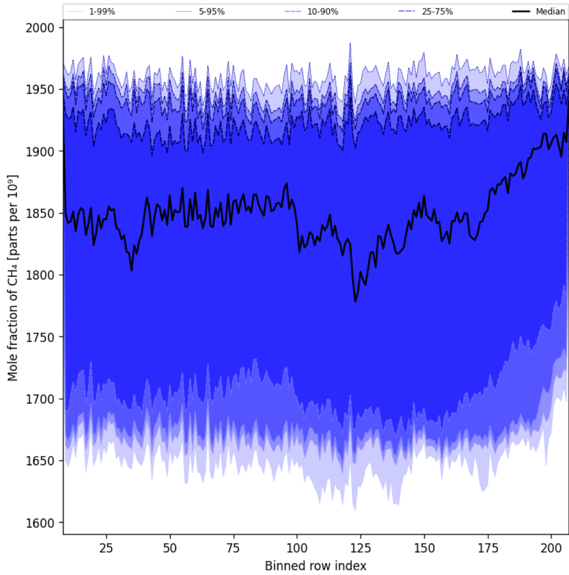
Figure 34: Along track statistics of “Mole fraction of CH 4 ” for 2024-12-17 to 2024-12-19
