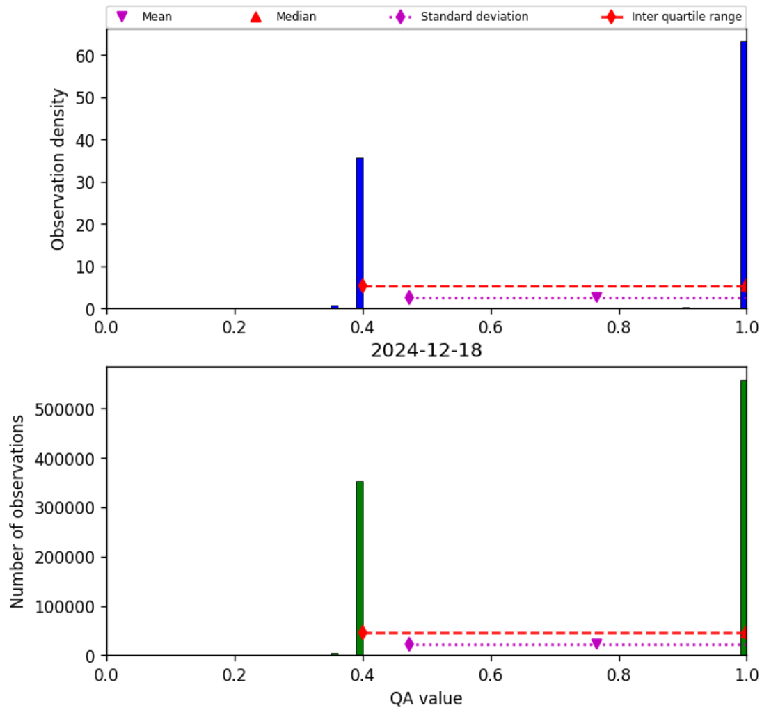
Figure 22: Histogram of “QA value” for 2024-12-17 to 2024-12-19
