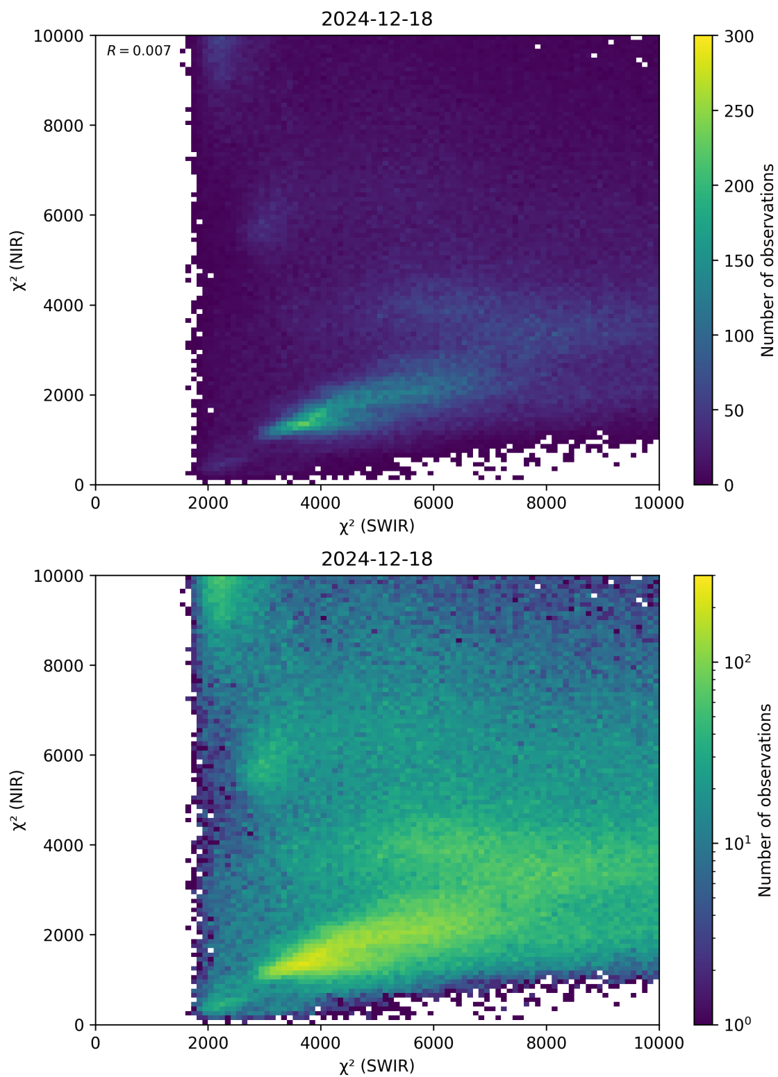
Figure 47: Scatter density plot of “ \chi^2 (SWIR)” against “ \chi^2 (NIR)” for 2024-12-17 to 2024-12-19.
