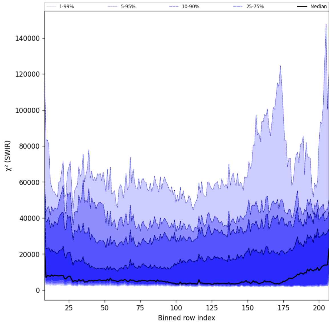
Figure 39: Along track statistics of “ \chi^2 (SWIR)” for 2024-12-17 to 2024-12-19
