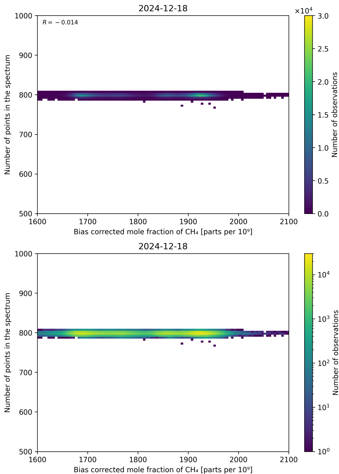
Figure 68: Scatter density plot of “Bias corrected mole fraction of CH 4 ” against “Number of points in the spectrum” for 2024-12-17 to 2024-12-19.
