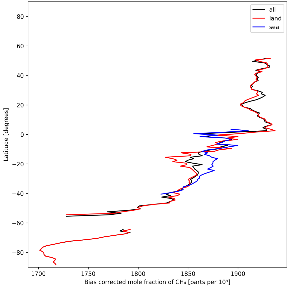
Figure 14: Zonal average of “Bias corrected mole fraction of CH 4 ” for 2024-12-17 to 2024-12-19.
