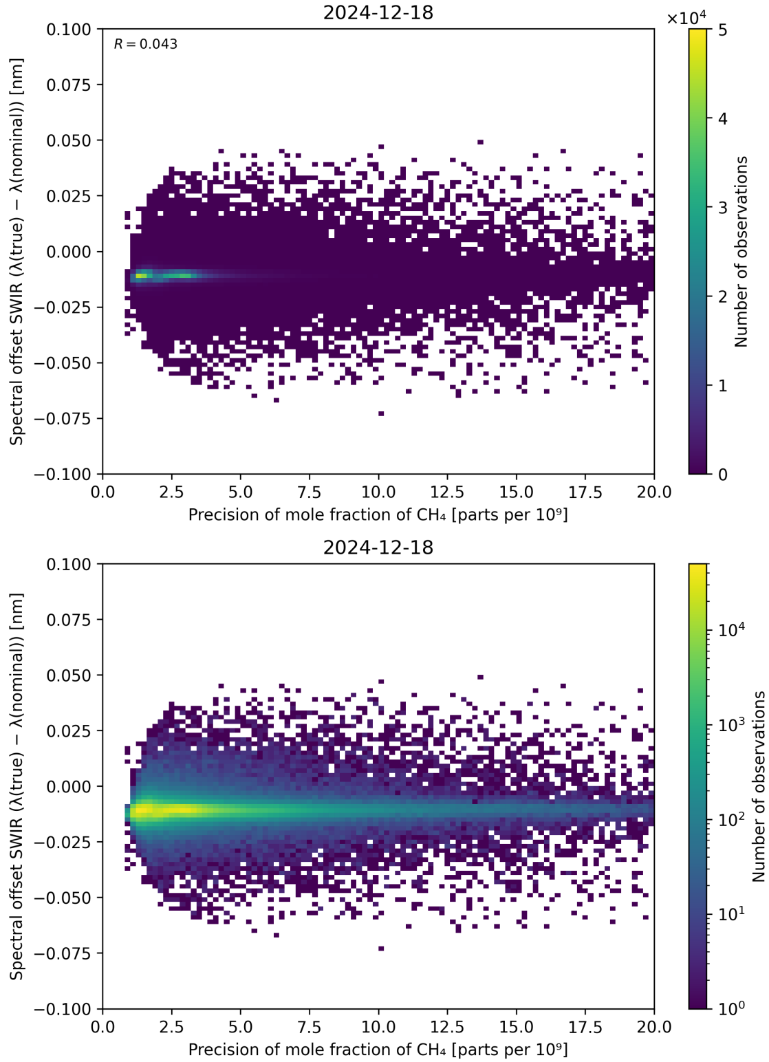
Figure 85: Scatter density plot of “Precision of mole fraction of CH 4 ” against “Spectral offset SWIR ( \lambda_{\text{true}} - \lambda_{\text{nominal}} )” for 2024-12-17 to 2024-12-19.
