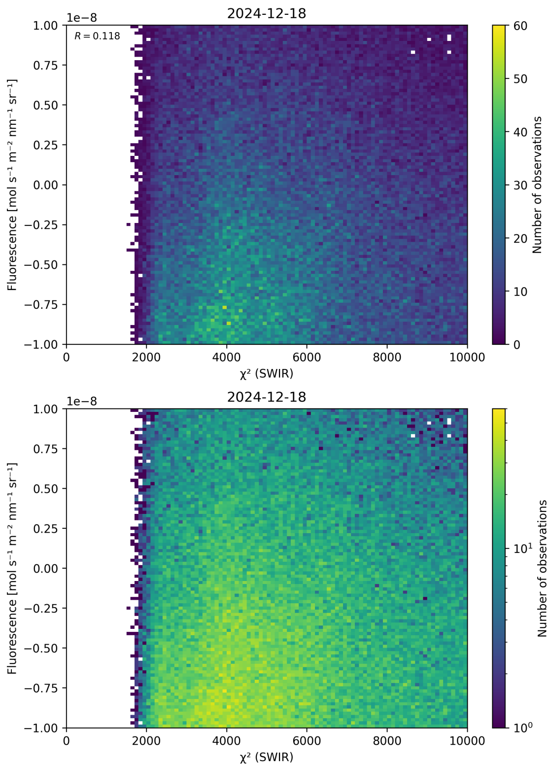
Figure 49: Scatter density plot of “ \chi^2 (SWIR)” against “Fluorescence” for 2024-12-17 to 2024-12-19.
