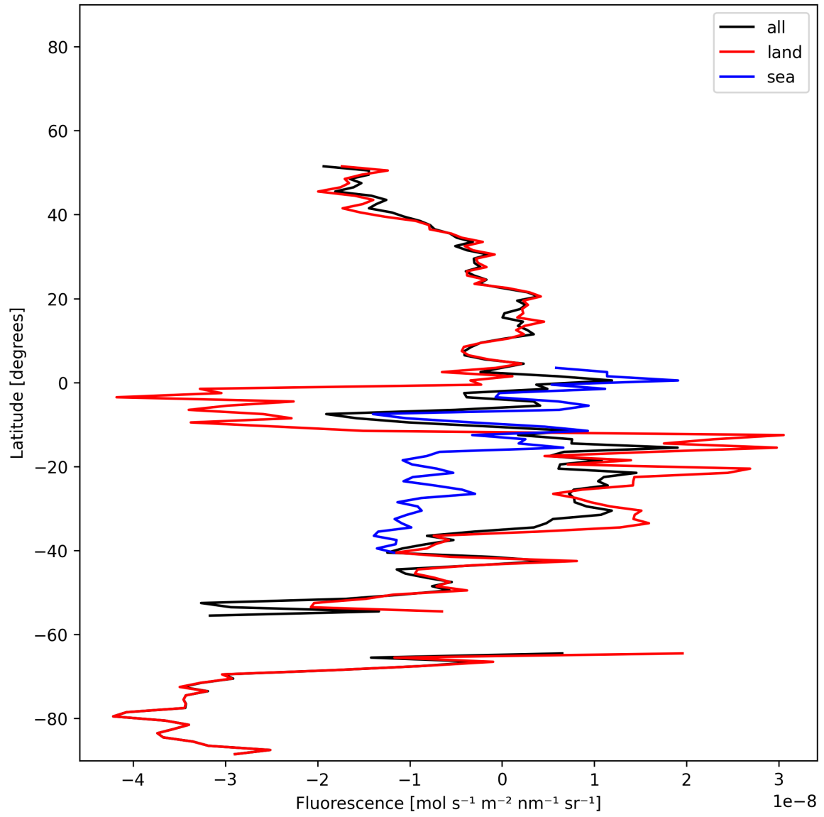
Figure 21: Zonal average of “Fluorescence” for 2024-12-17 to 2024-12-19.
