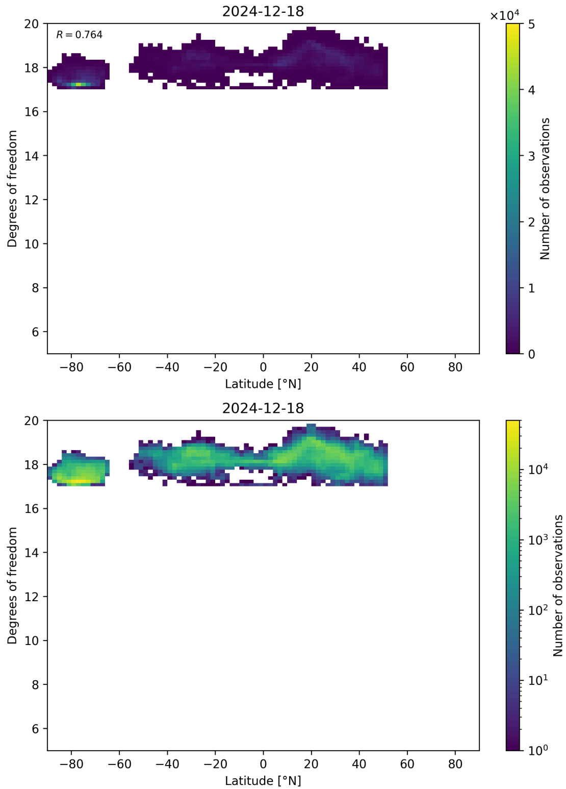
Figure 55: Scatter density plot of “Latitude” against “Degrees of freedom” for 2024-12-17 to 2024-12-19.
