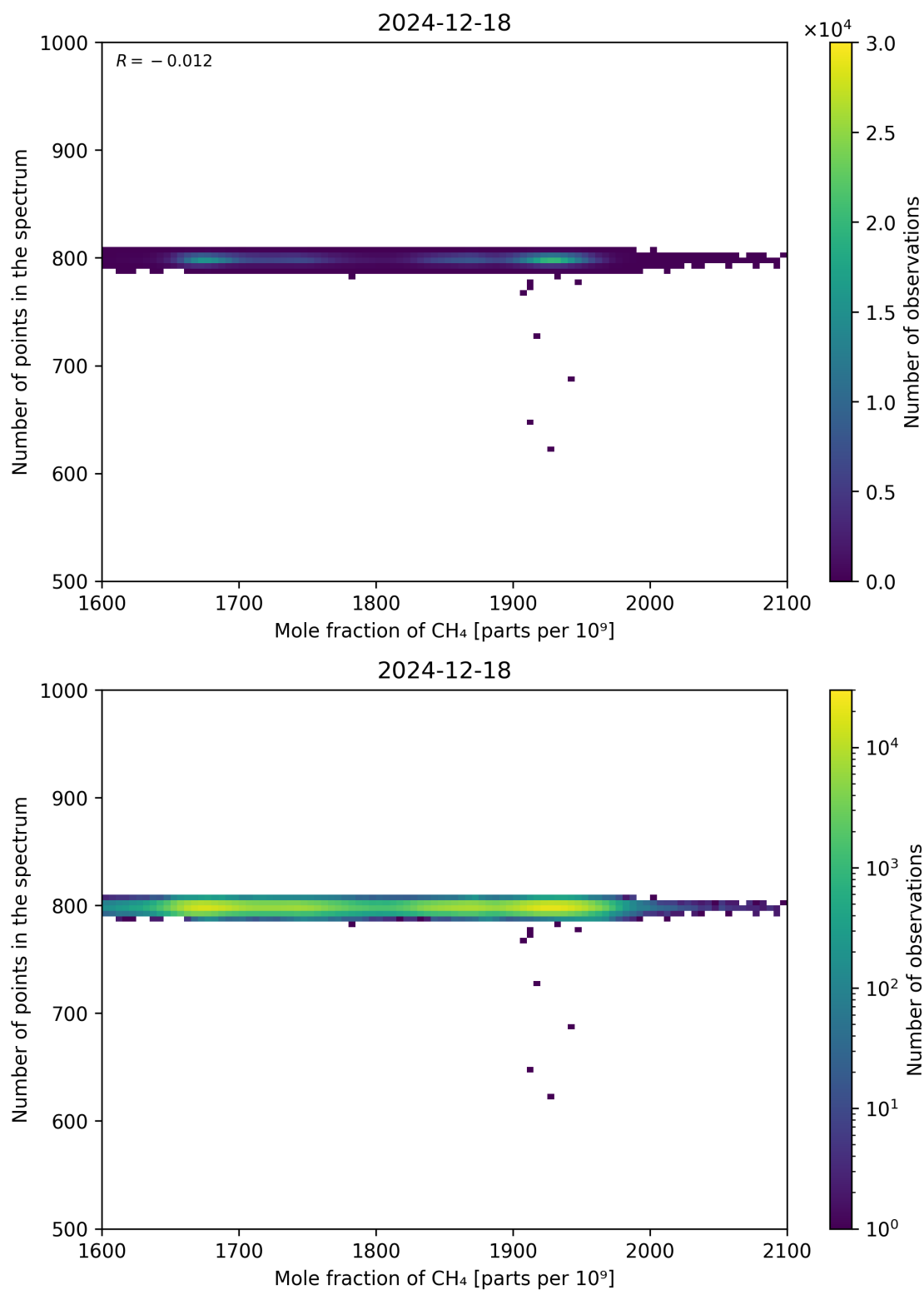
Figure 77: Scatter density plot of “Mole fraction of CH 4 ” against “Number of points in the spectrum” for 2024-12-17 to 2024-12-19.
