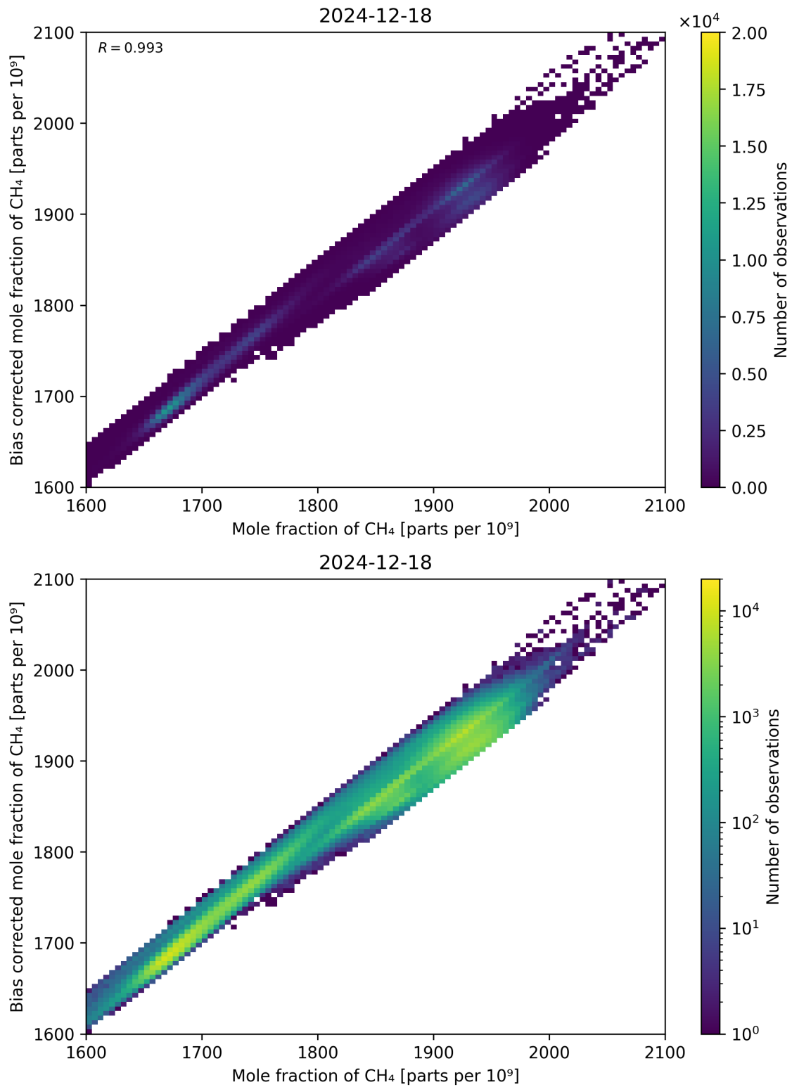
Figure 74: Scatter density plot of “Mole fraction of CH 4 ” against “Bias corrected mole fraction of CH 4 ” for 2024-12-17 to 2024-12-19.
