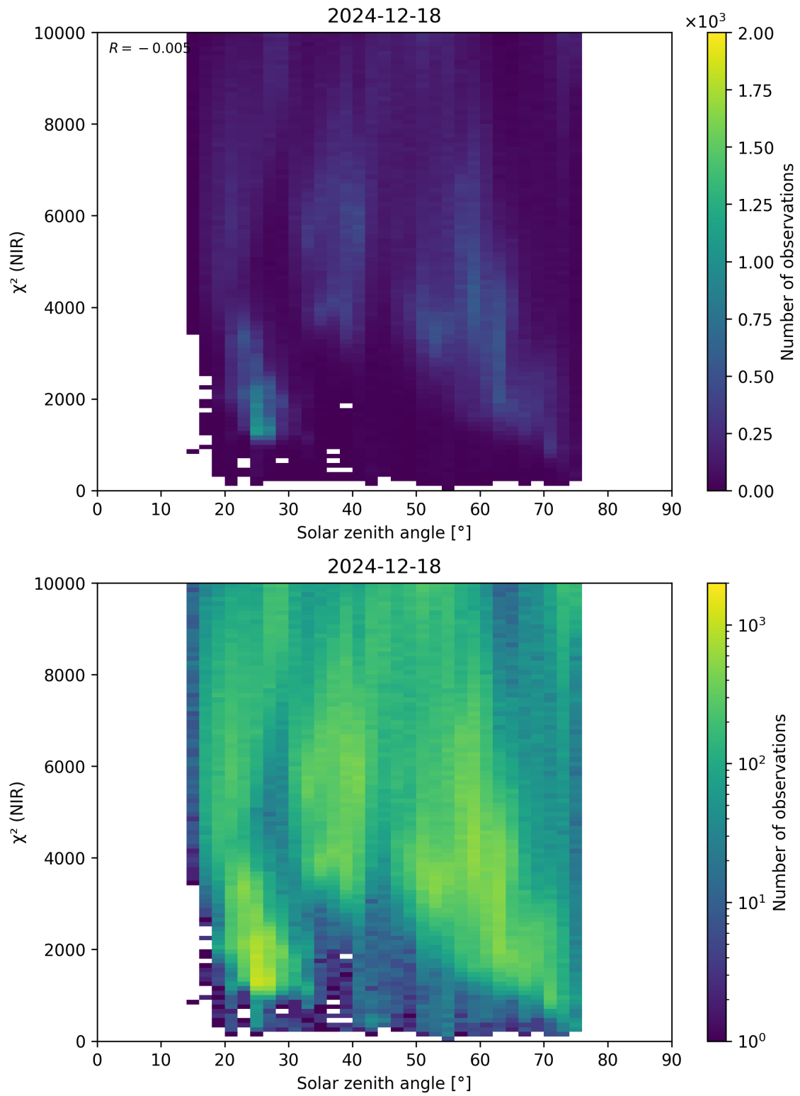
Figure 94: Scatter density plot of “Solar zenith angle” against “ \chi^2 (NIR)” for 2024-12-17 to 2024-12-19.
