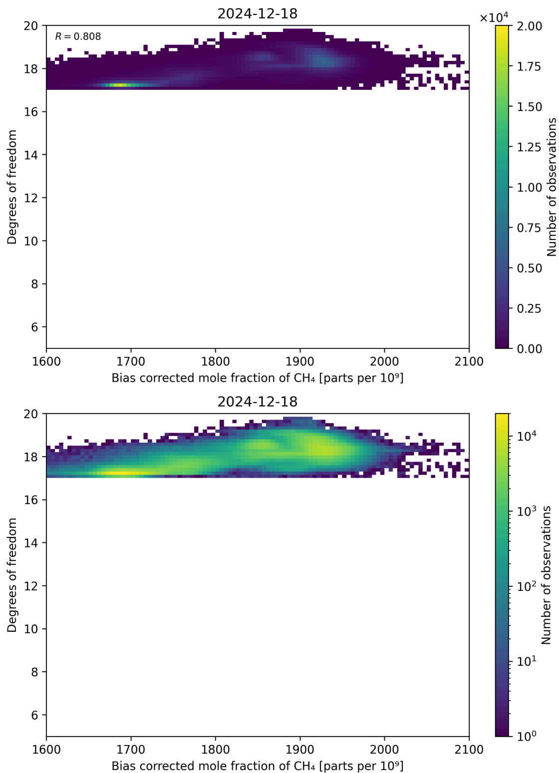
Figure 65: Scatter density plot of “Bias corrected mole fraction of CH 4 ” against “Degrees of freedom” for 2024-12-17 to 2024-12-19.
