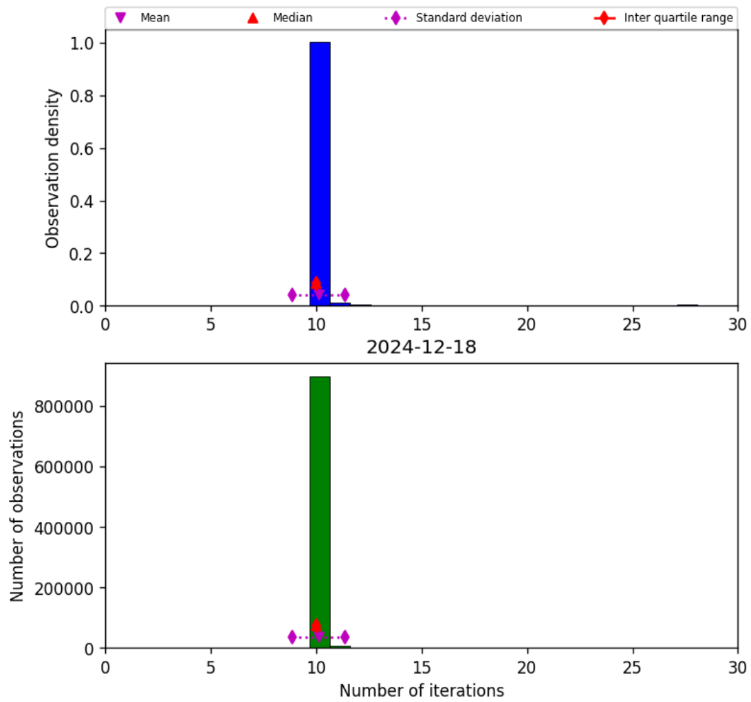
Figure 31: Histogram of “Number of iterations” for 2024-12-17 to 2024-12-19
