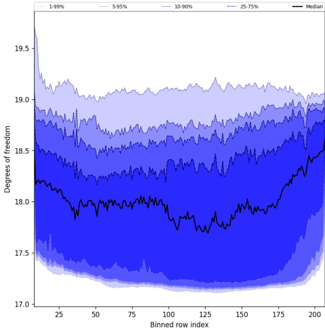
Figure 41: Along track statistics of “Degrees of freedom” for 2024-12-17 to 2024-12-19
