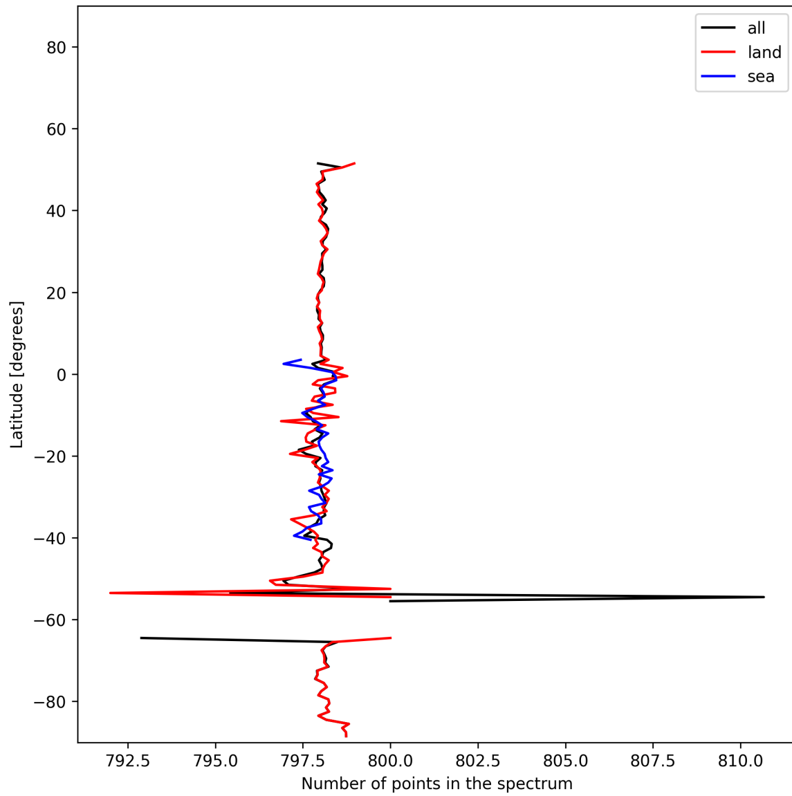
Figure 15: Zonal average of “Number of points in the spectrum” for 2024-12-17 to 2024-12-19.
