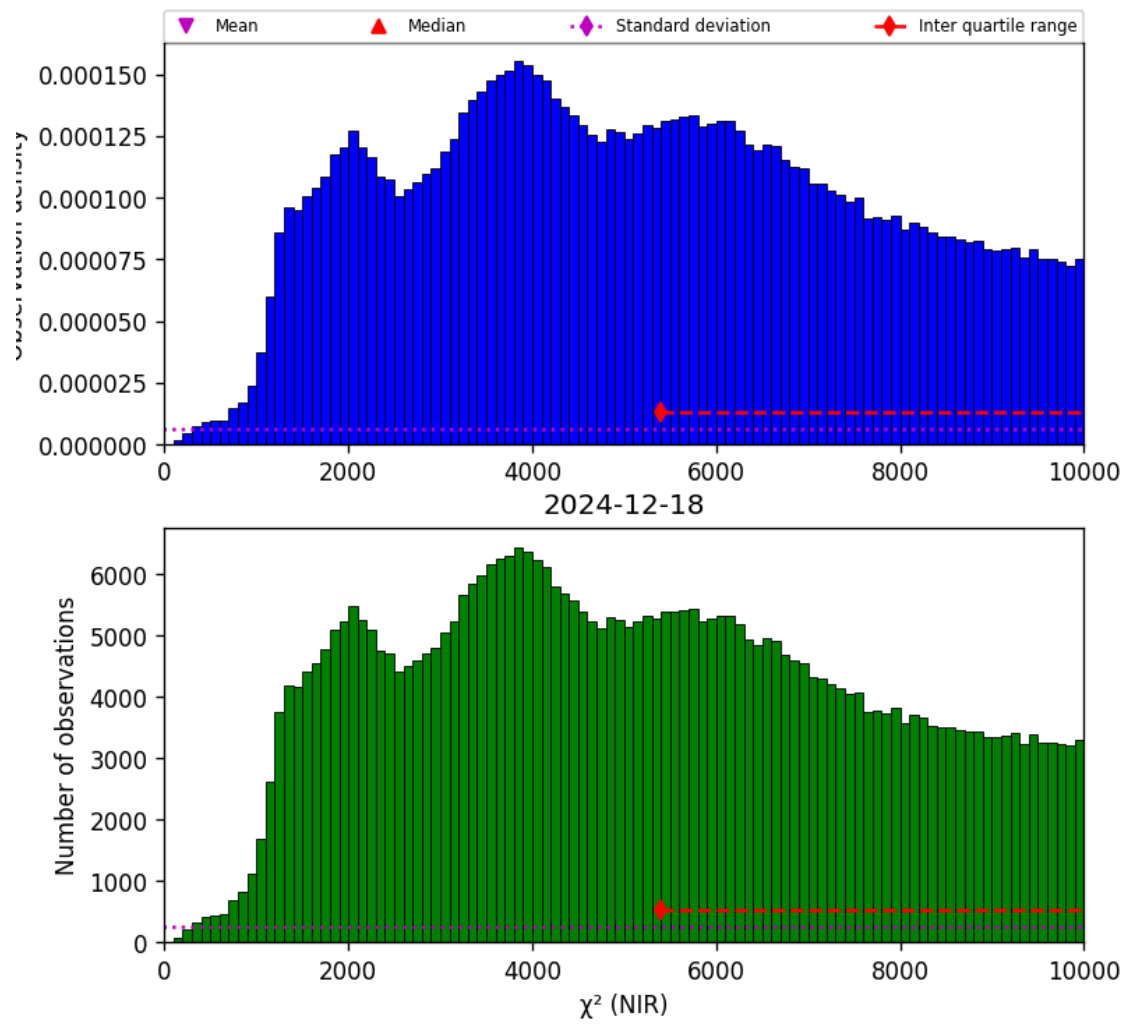
Figure 29: Histogram of “ \chi^2 (NIR)” for 2024-12-17 to 2024-12-19
