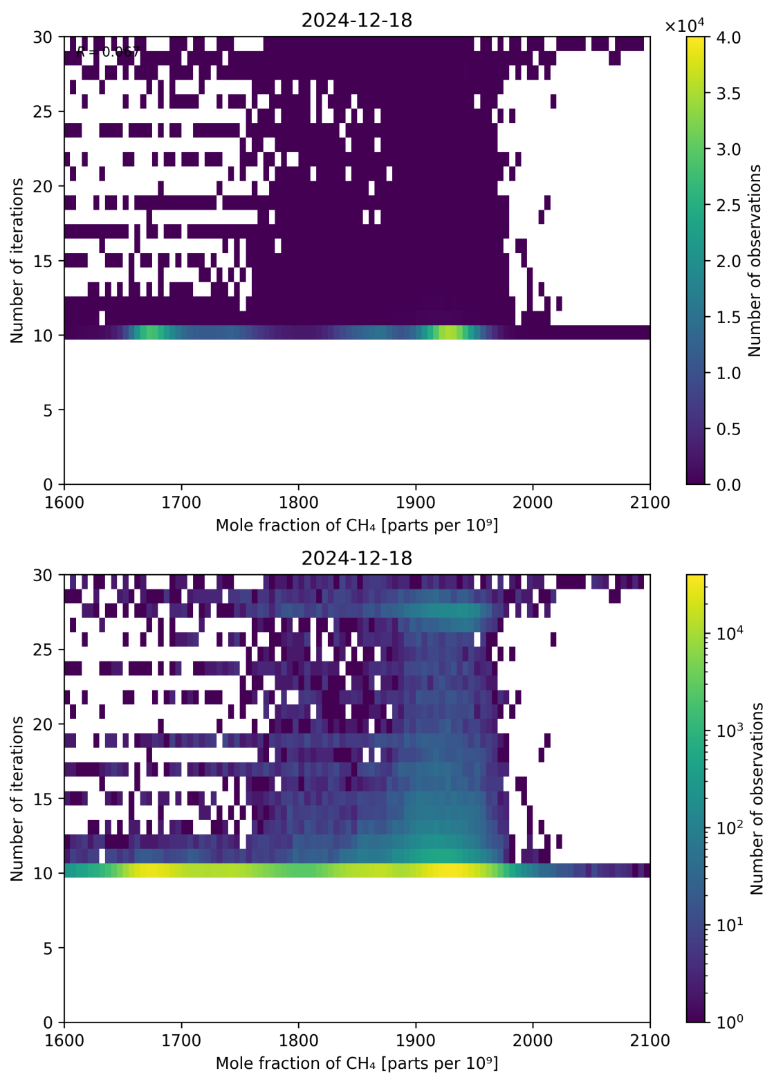
Figure 76: Scatter density plot of “Mole fraction of CH 4 ” against “Number of iterations” for 2024-12-17 to 2024-12-19.
