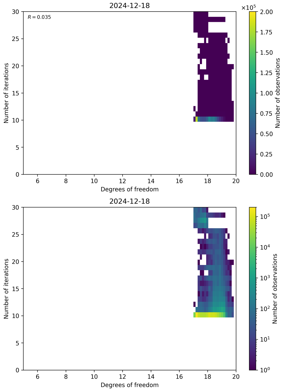
Figure 52: Scatter density plot of “Degrees of freedom” against “Number of iterations” for 2024-12-17 to 2024-12-19.
