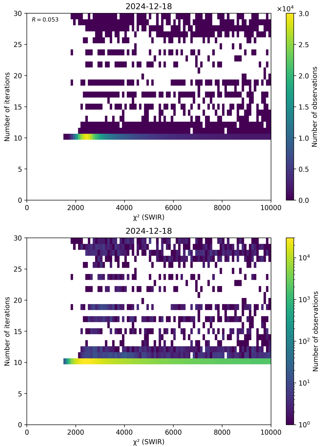
Figure 50: Scatter density plot of “ \chi^2 (SWIR)” against “Number of iterations” for 2024-12-17 to 2024-12-19.
