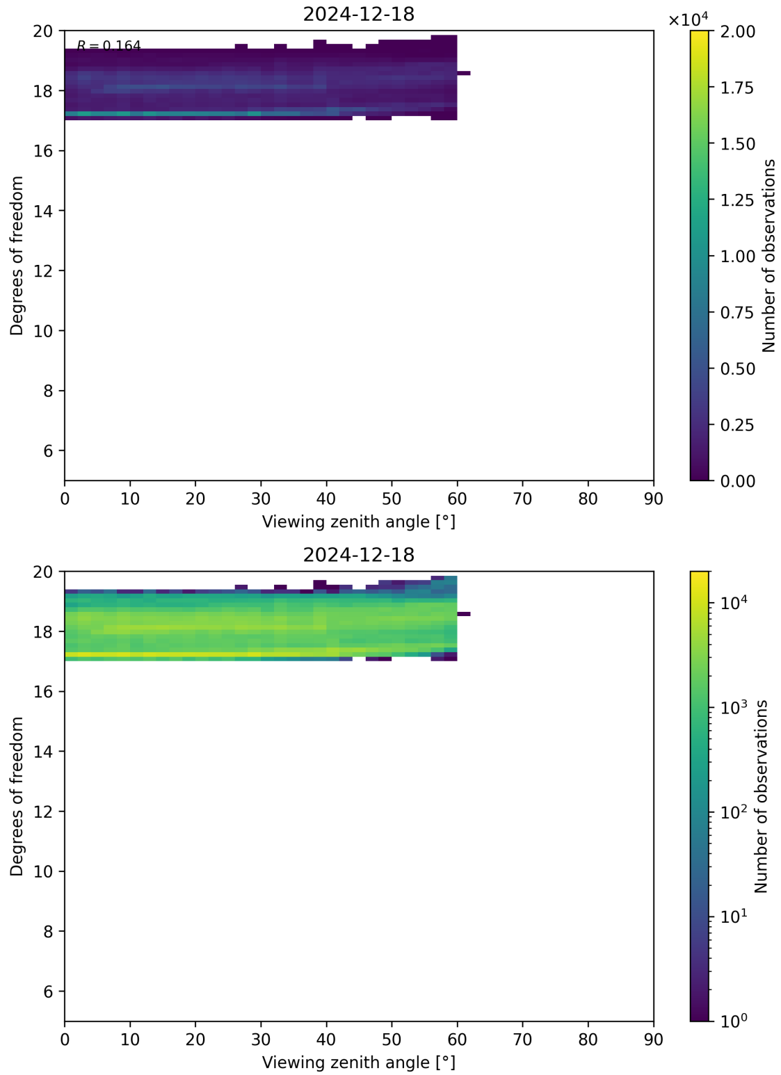
Figure 107: Scatter density plot of “Viewing zenith angle” against “Degrees of freedom” for 2024-12-17 to 2024-12-19.
