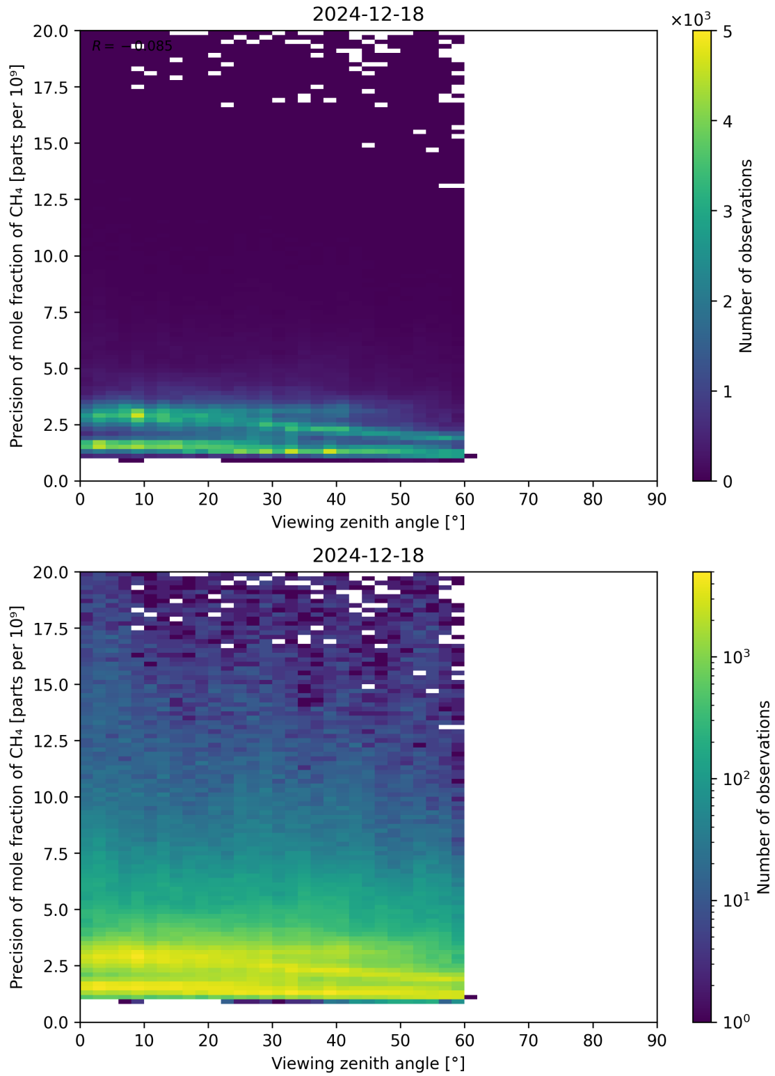
Figure 112: Scatter density plot of “Viewing zenith angle” against “Precision of mole fraction of CH 4 ” for 2024-12-17 to 2024-12-19.
