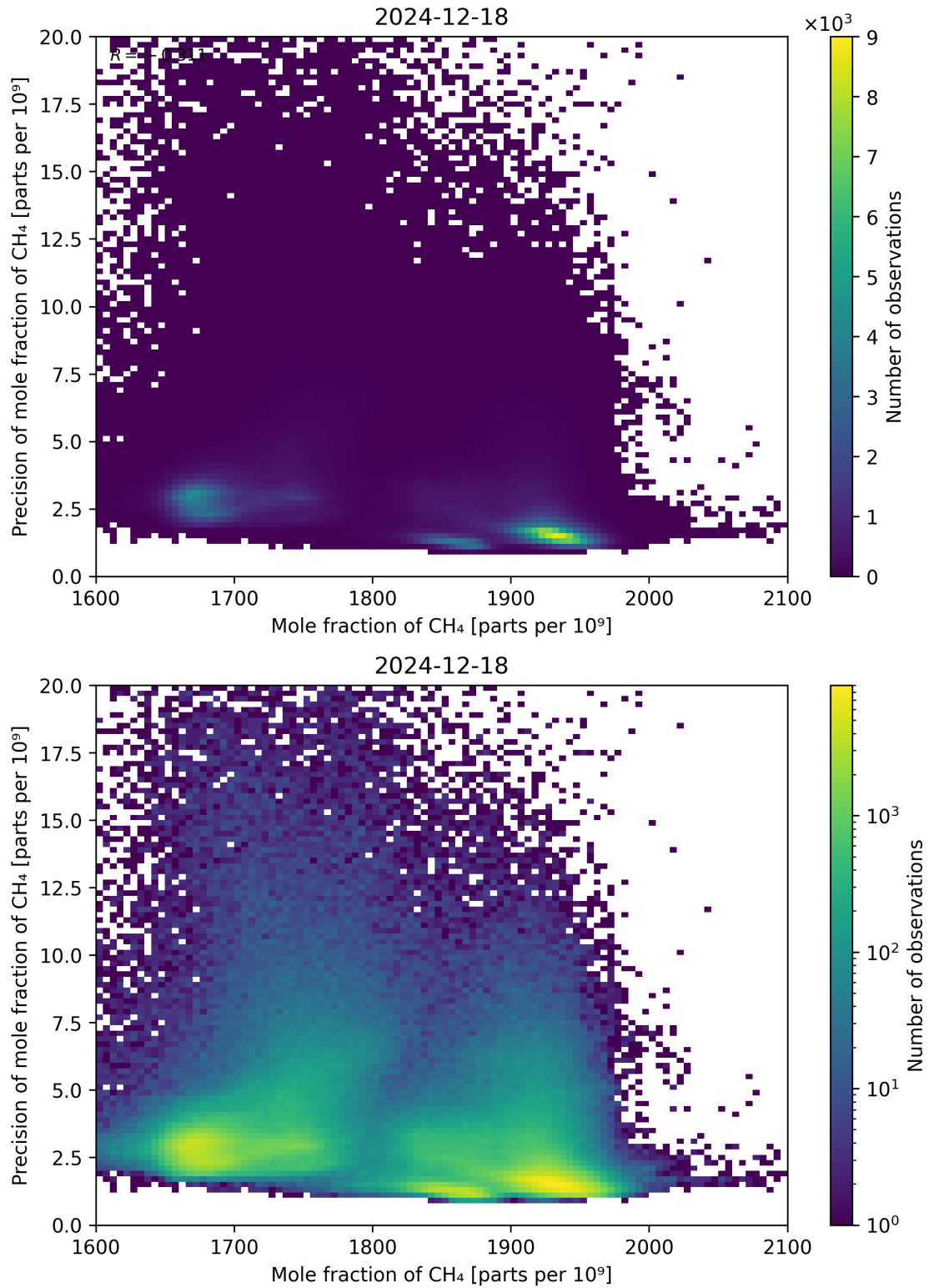
Figure 75: Scatter density plot of “Mole fraction of CH 4 ” against “Precision of mole fraction of CH 4 ” for 2024-12-17 to 2024-12-19.
