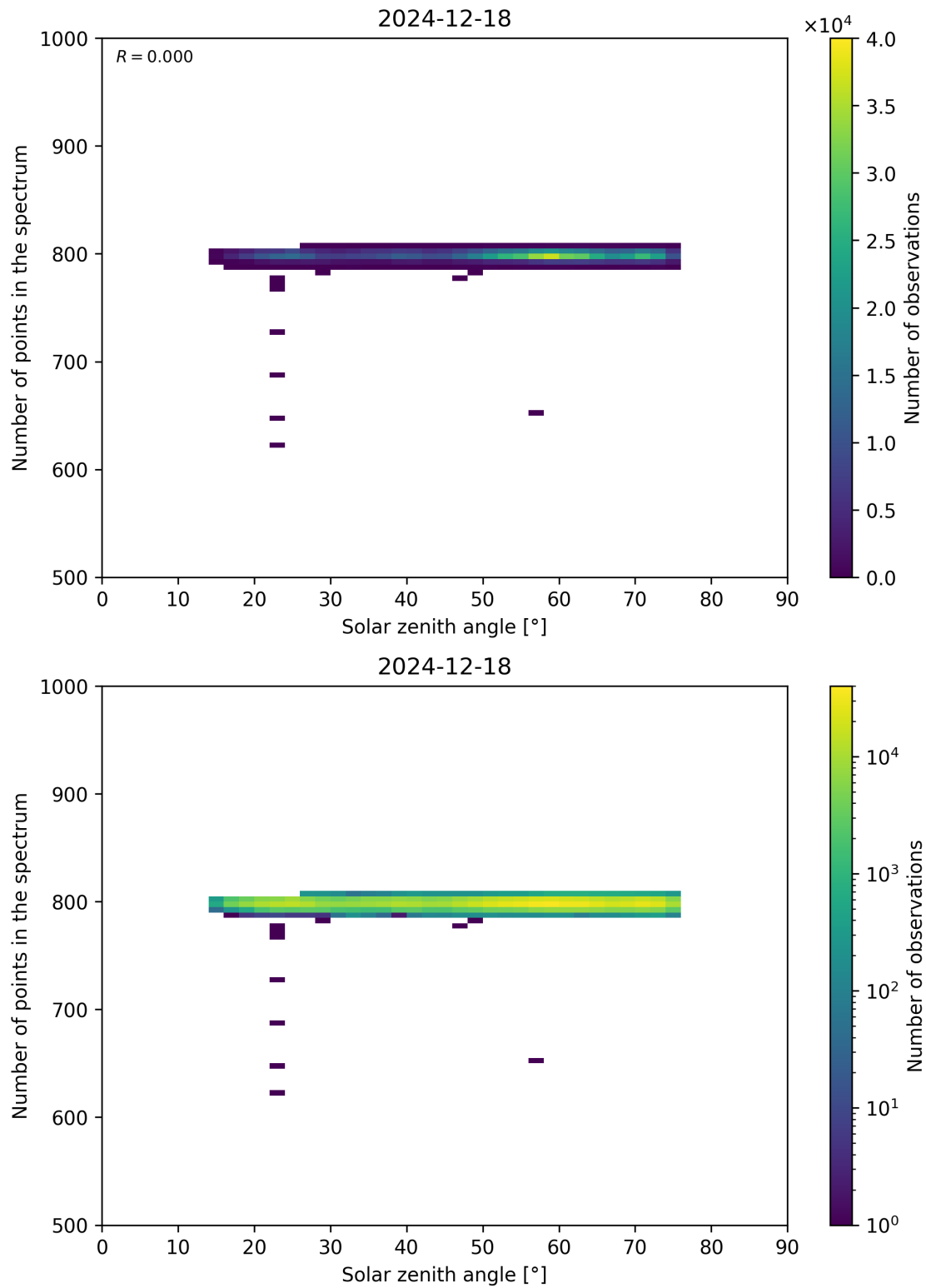
Figure 103: Scatter density plot of “Solar zenith angle” against “Number of points in the spectrum” for 2024-12-17 to 2024-12-19.
