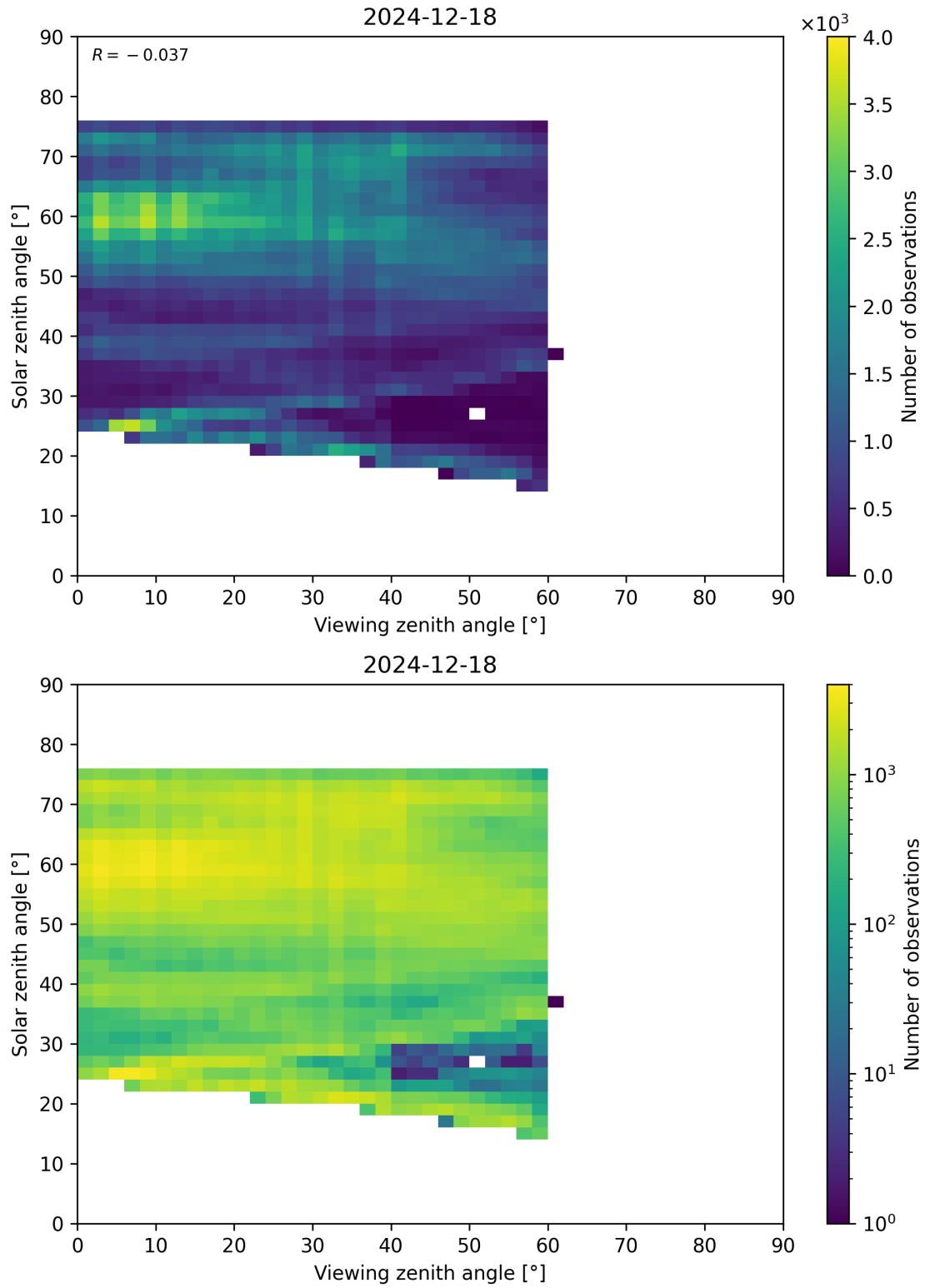
Figure 115: Scatter density plot of “Viewing zenith angle” against “Solar zenith angle” for 2024-12-17 to 2024-12-19.
