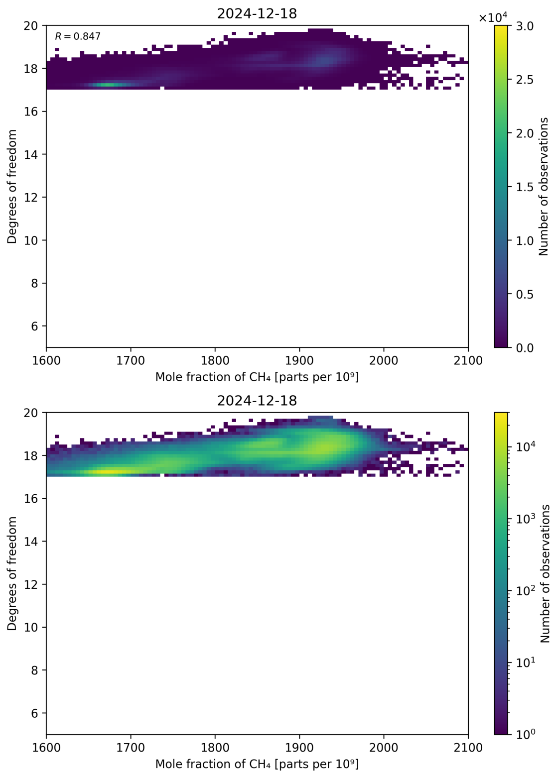
Figure 72: Scatter density plot of “Mole fraction of CH 4 ” against “Degrees of freedom” for 2024-12-17 to 2024-12-19.
