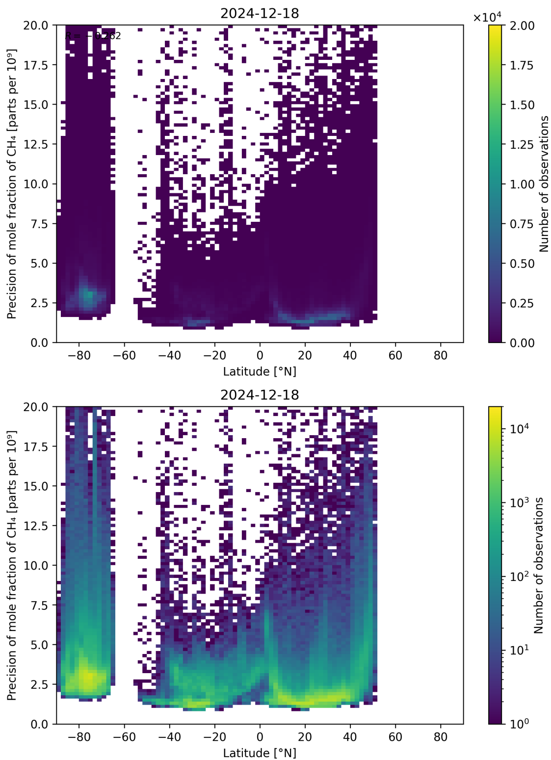
Figure 59: Scatter density plot of “Latitude” against “Precision of mole fraction of CH 4 ” for 2024-12-17 to 2024-12-19.
