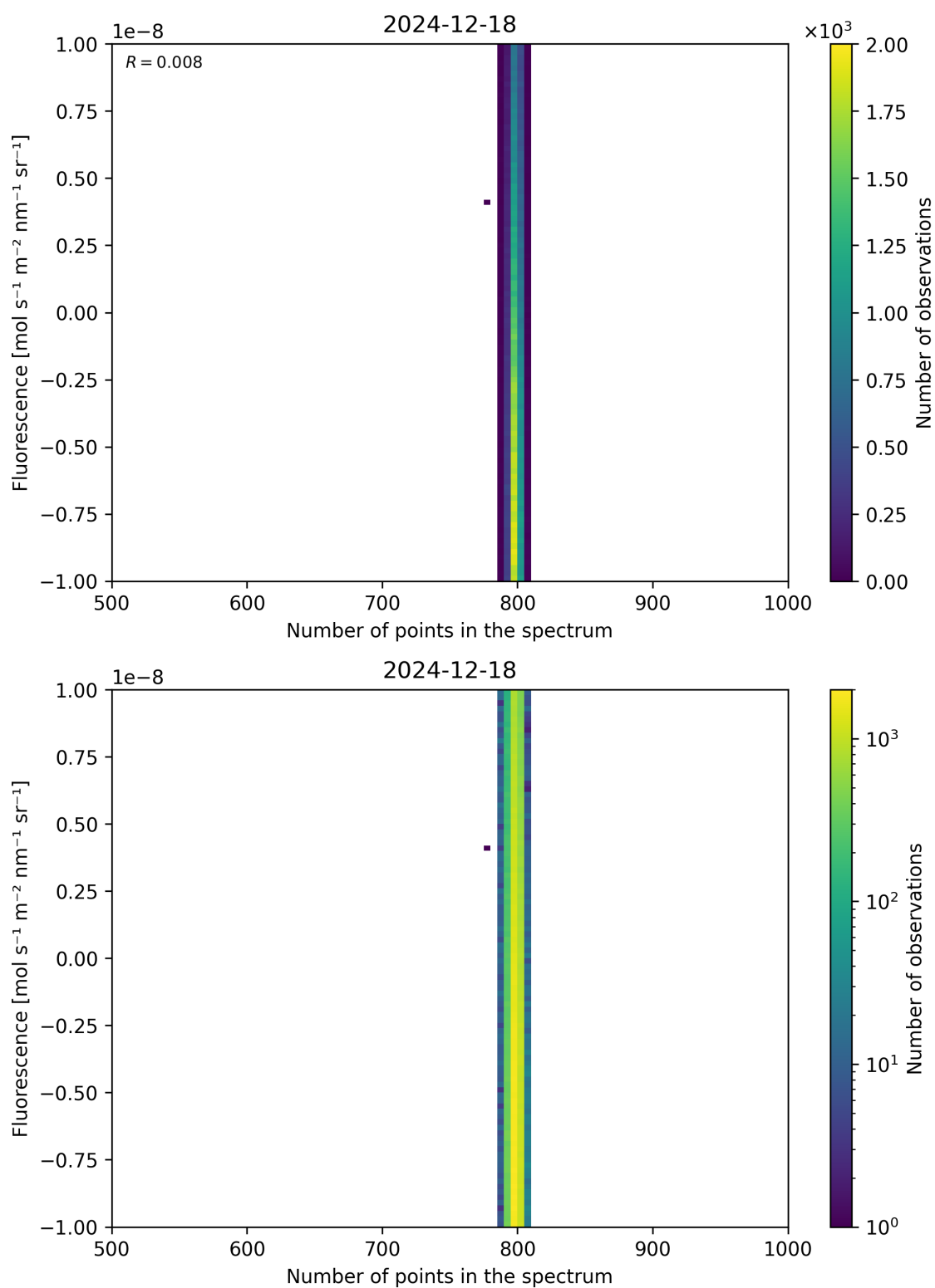
Figure 91: Scatter density plot of “Number of points in the spectrum” against “Fluorescence” for 2024-12-17 to 2024-12-19.
