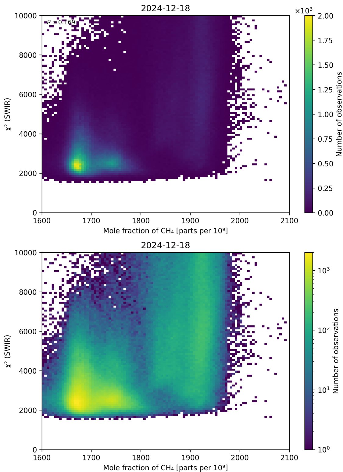
Figure 71: Scatter density plot of “Mole fraction of \text{CH}_4 ” against “ \chi^2 (SWIR)” for 2024-12-17 to 2024-12-19.
