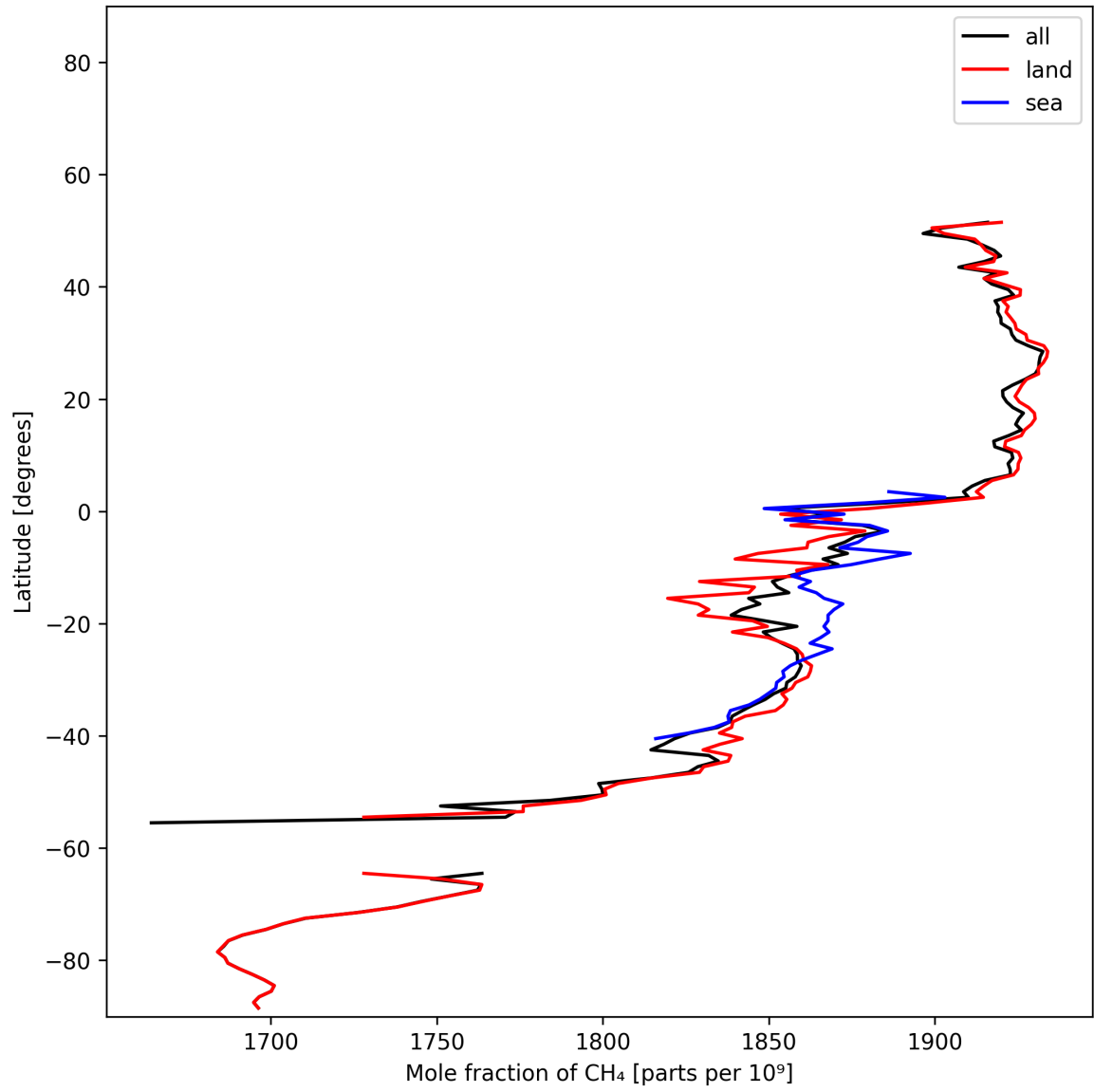
Figure 12: Zonal average of “Mole fraction of CH 4 ” for 2024-12-17 to 2024-12-19.
