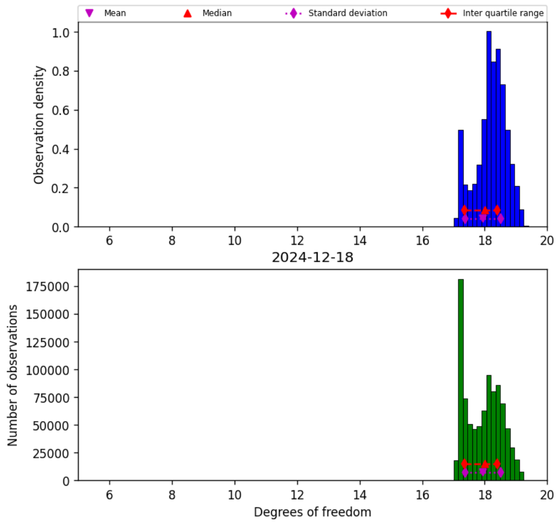
Figure 30: Histogram of “Degrees of freedom” for 2024-12-17 to 2024-12-19
