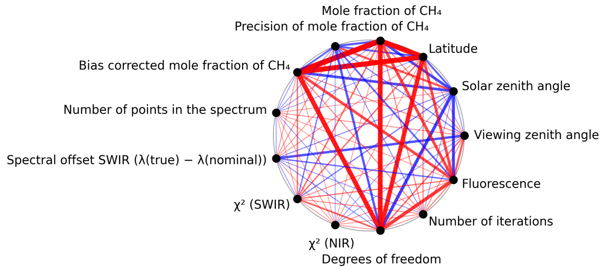
Figure 1: Map of correlation graph for 2024-12-17 to 2024-12-19.
