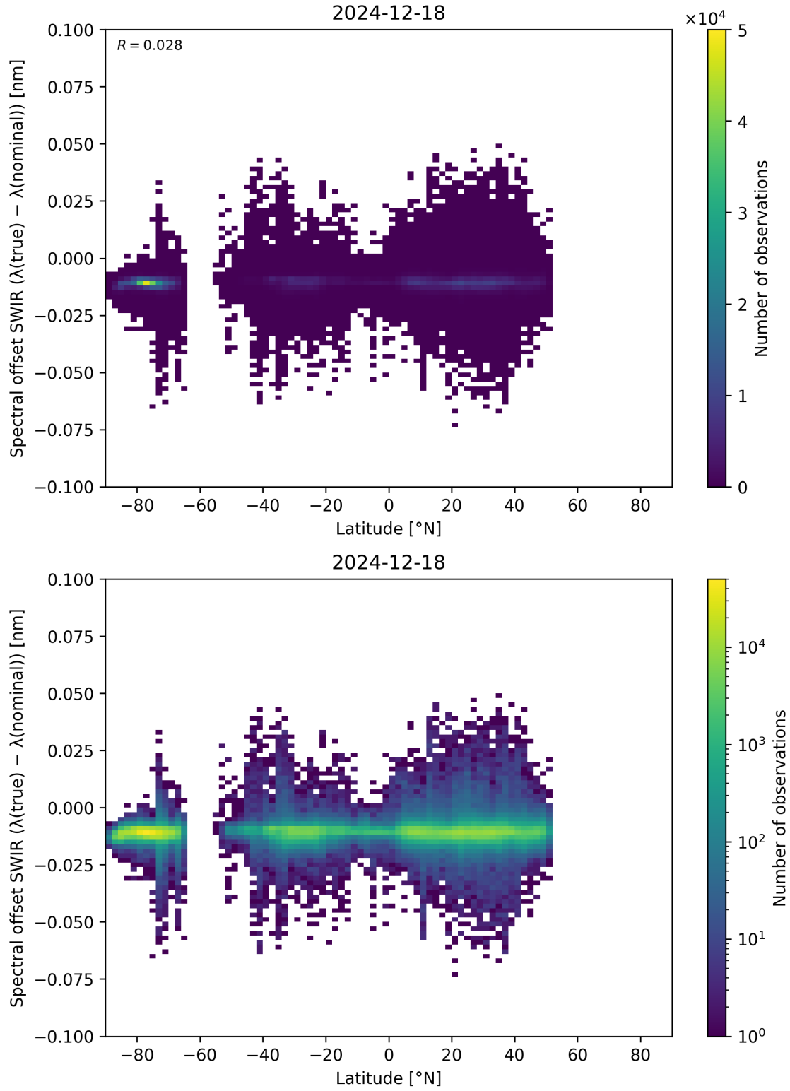
Figure 62: Scatter density plot of “Latitude” against “Spectral offset SWIR ( \lambda_{\text{true}} - \lambda_{\text{nominal}} )” for 2024-12-17 to 2024-12-19.
