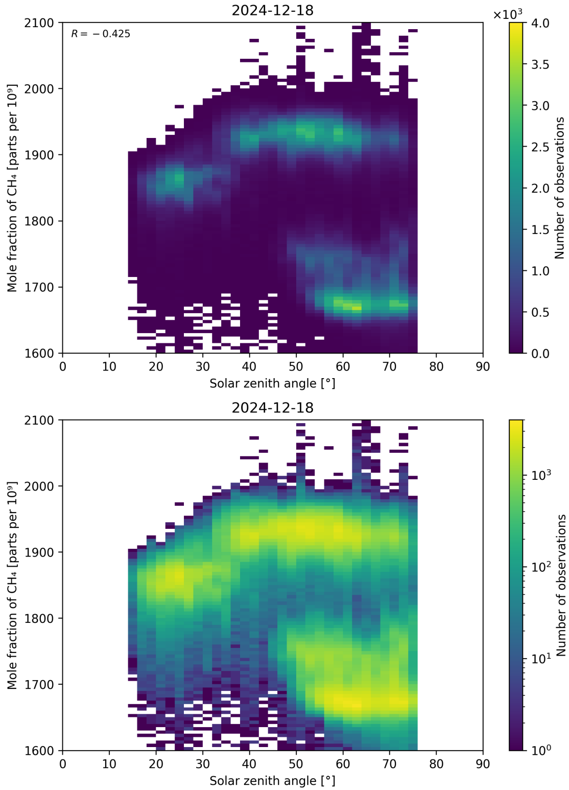
Figure 99: Scatter density plot of “Solar zenith angle” against “Mole fraction of CH 4 ” for 2024-12-17 to 2024-12-19.
