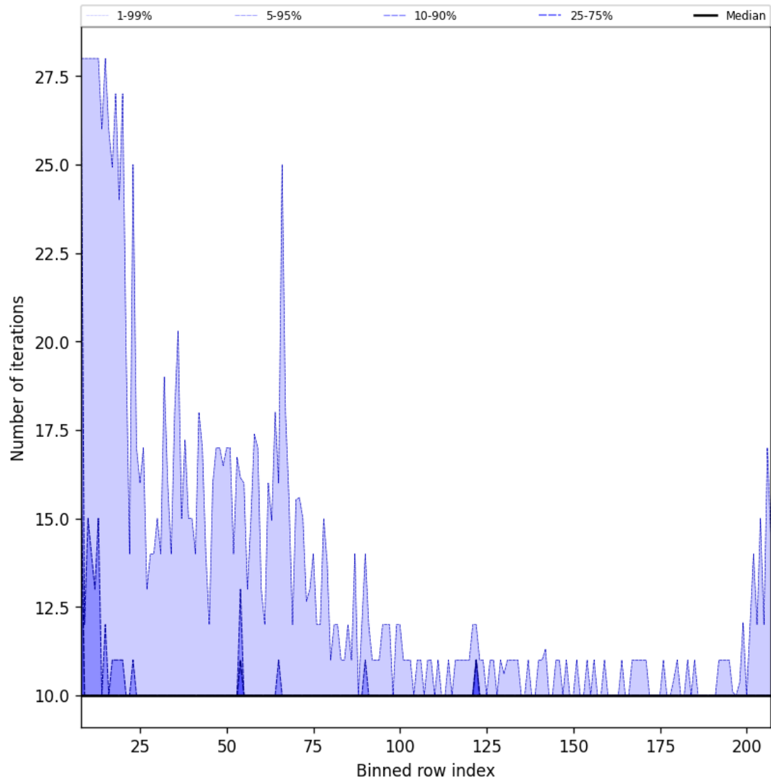
Figure 42: Along track statistics of “Number of iterations” for 2024-12-17 to 2024-12-19
