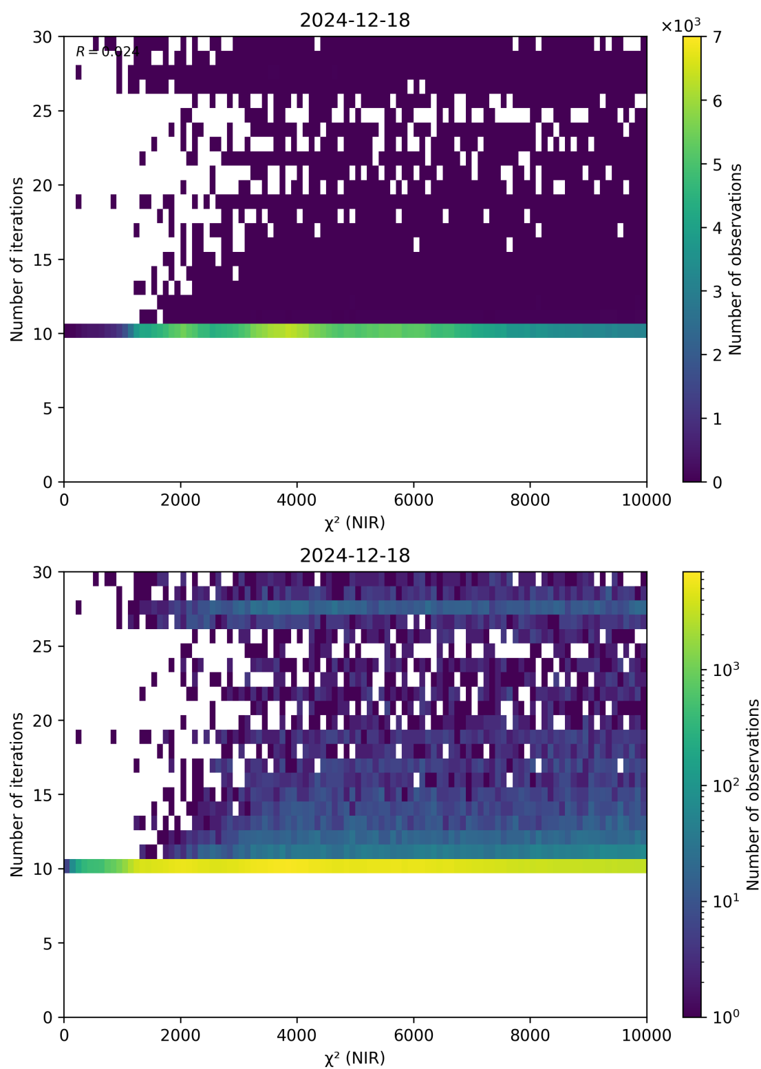
Figure 46: Scatter density plot of “ \chi^2 (NIR)” against “Number of iterations” for 2024-12-17 to 2024-12-19.
