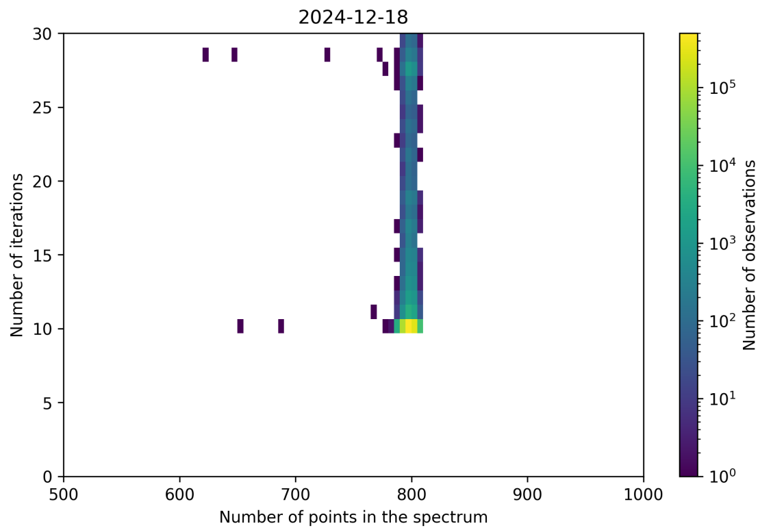
Figure 92: Scatter density plot of “Number of points in the spectrum” against “Number of iterations” for 2024-12-17 to 2024-12-19.
