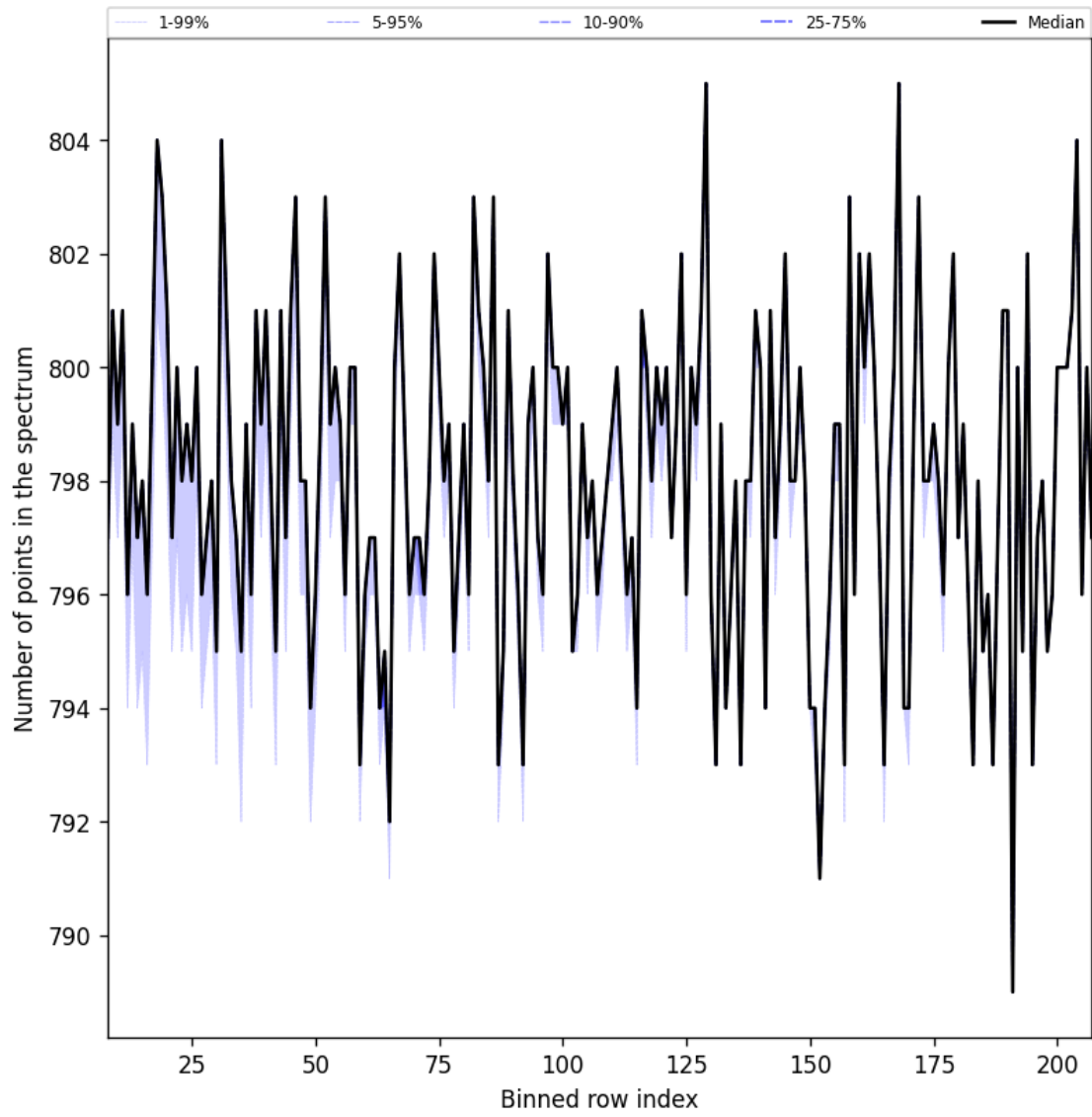
Figure 37: Along track statistics of “Number of points in the spectrum” for 2024-12-17 to 2024-12-19
