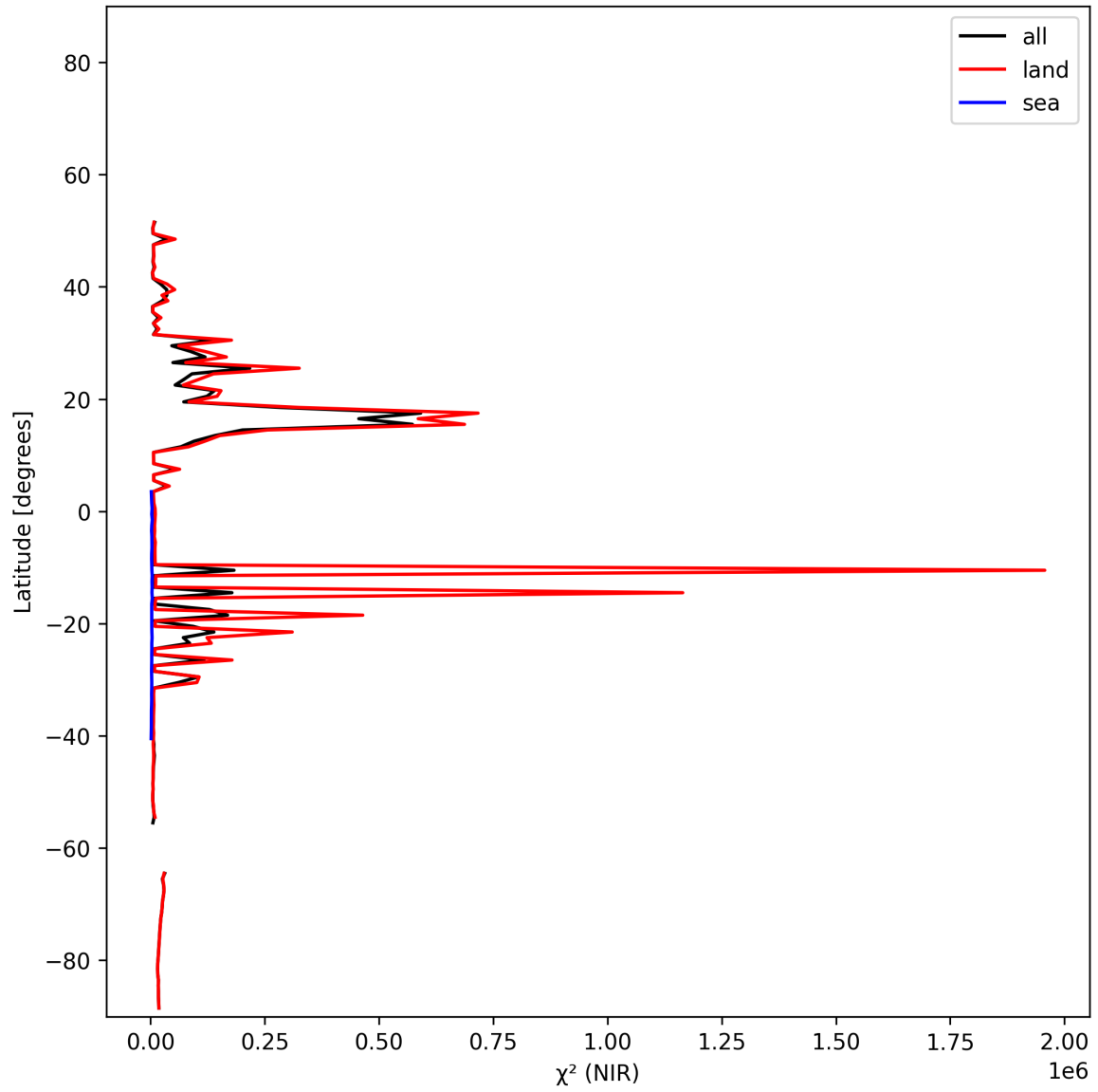
Figure 18: Zonal average of “ \chi^2 (NIR)” for 2024-12-17 to 2024-12-19.
