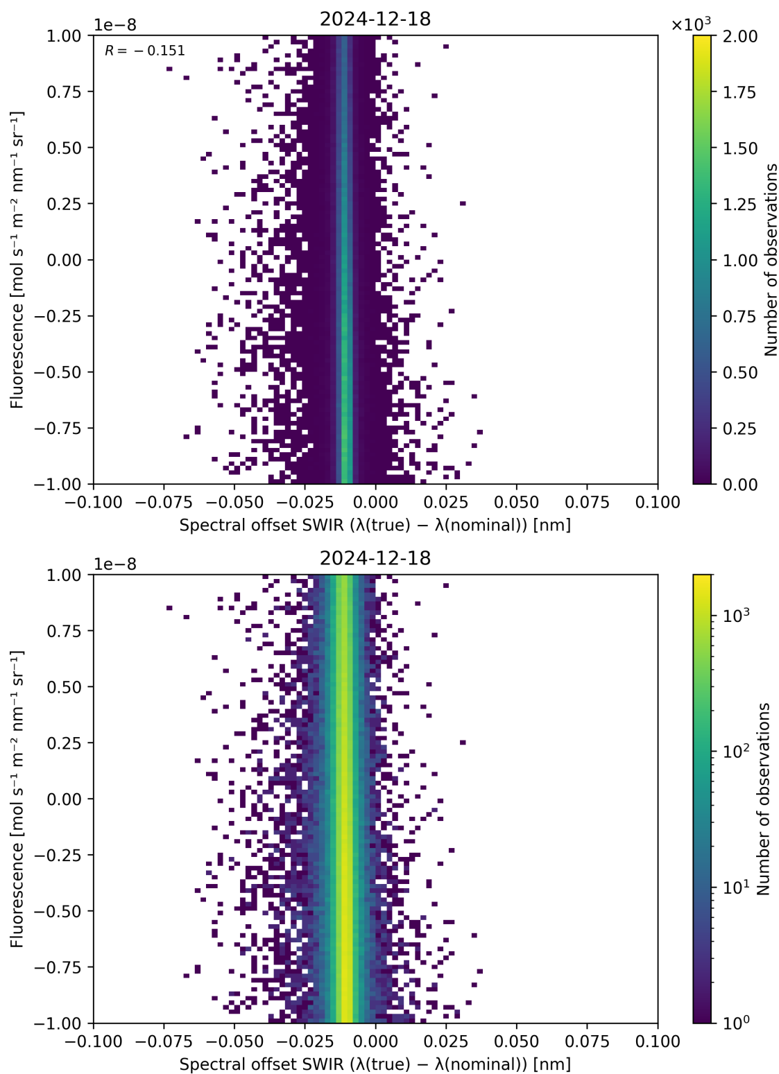
Figure 120: Scatter density plot of “Spectral offset SWIR ( \lambda_{\text{true}} - \lambda_{\text{nominal}} )” against “Fluorescence” for 2024-12-17 to 2024-12-19.
