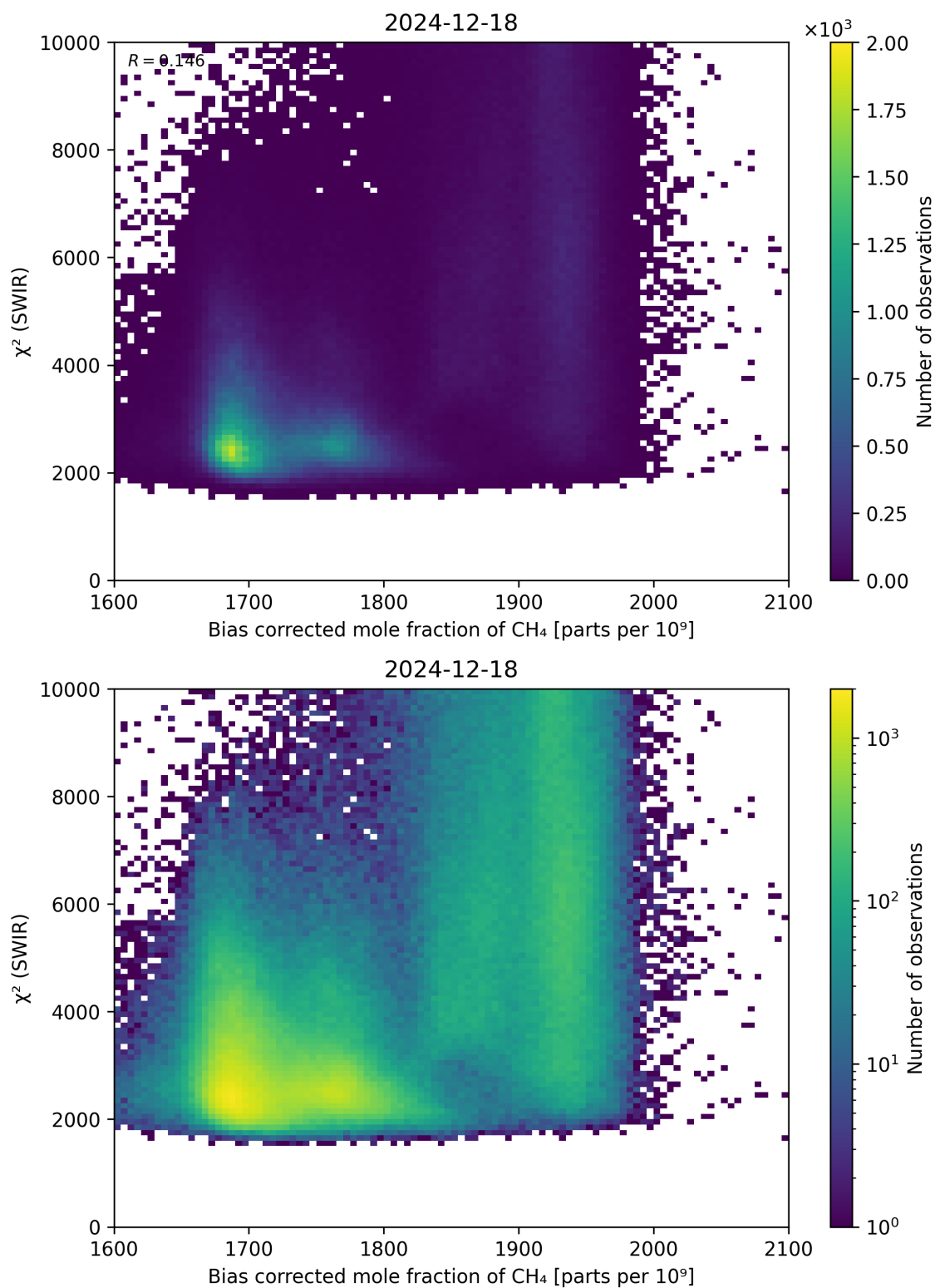
Figure 64: Scatter density plot of “Bias corrected mole fraction of \text{CH}_4 ” against “ \chi^2 (SWIR)” for 2024-12-17 to 2024-12-19.
