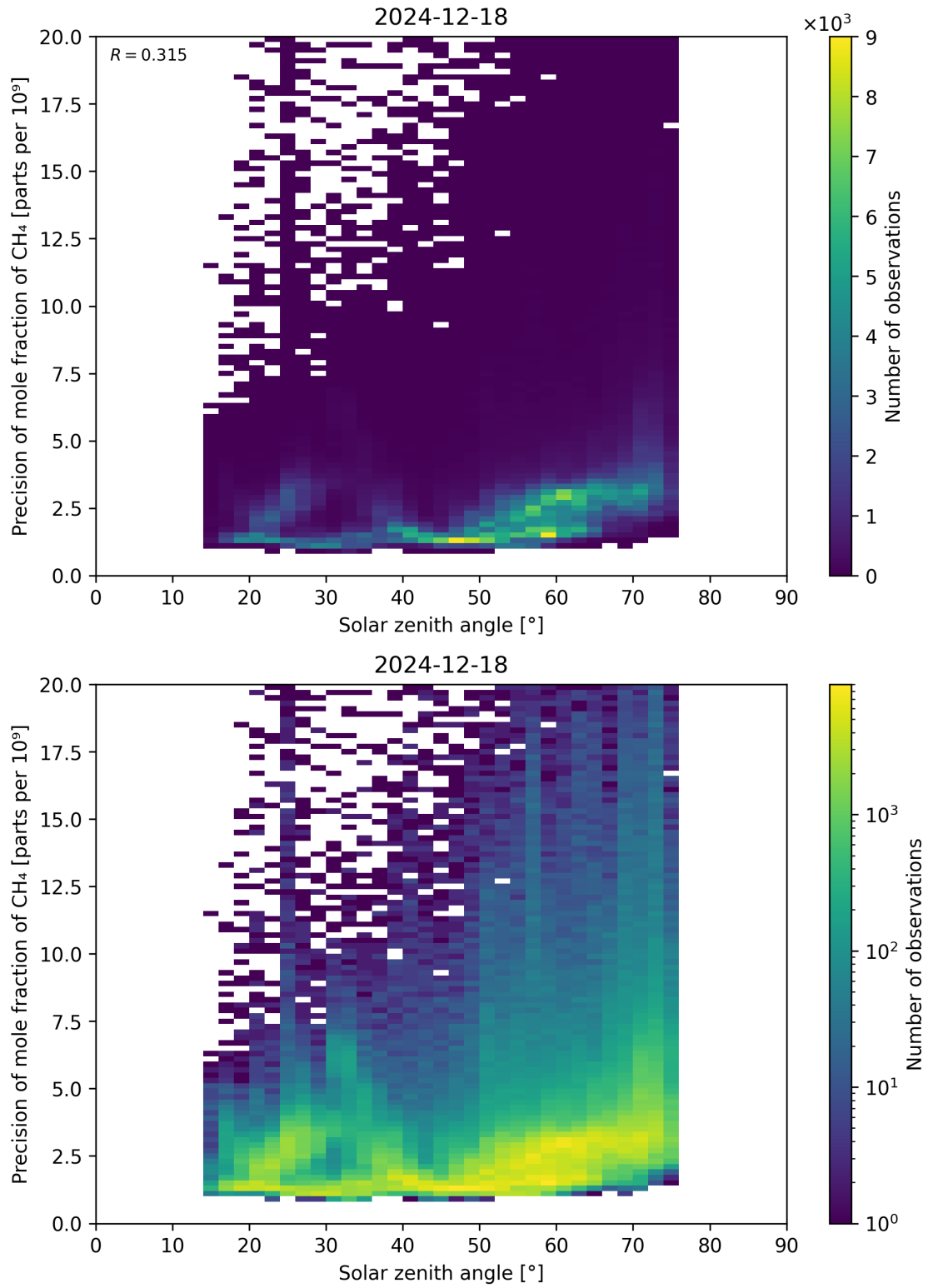
Figure 101: Scatter density plot of “Solar zenith angle” against “Precision of mole fraction of \text{CH}_4 ” for 2024-12-17 to 2024-12-19.
