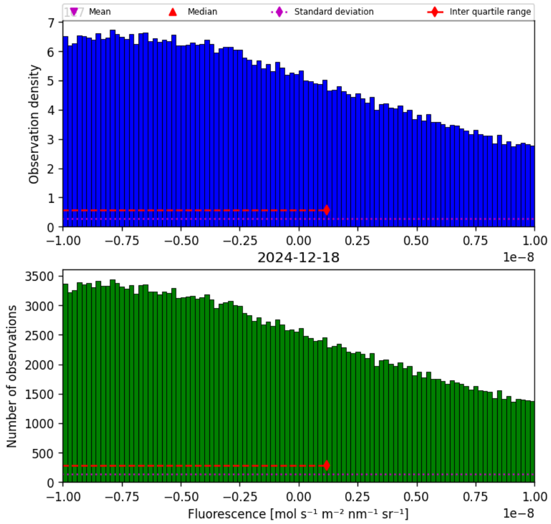
Figure 32: Histogram of “Fluorescence” for 2024-12-17 to 2024-12-19
