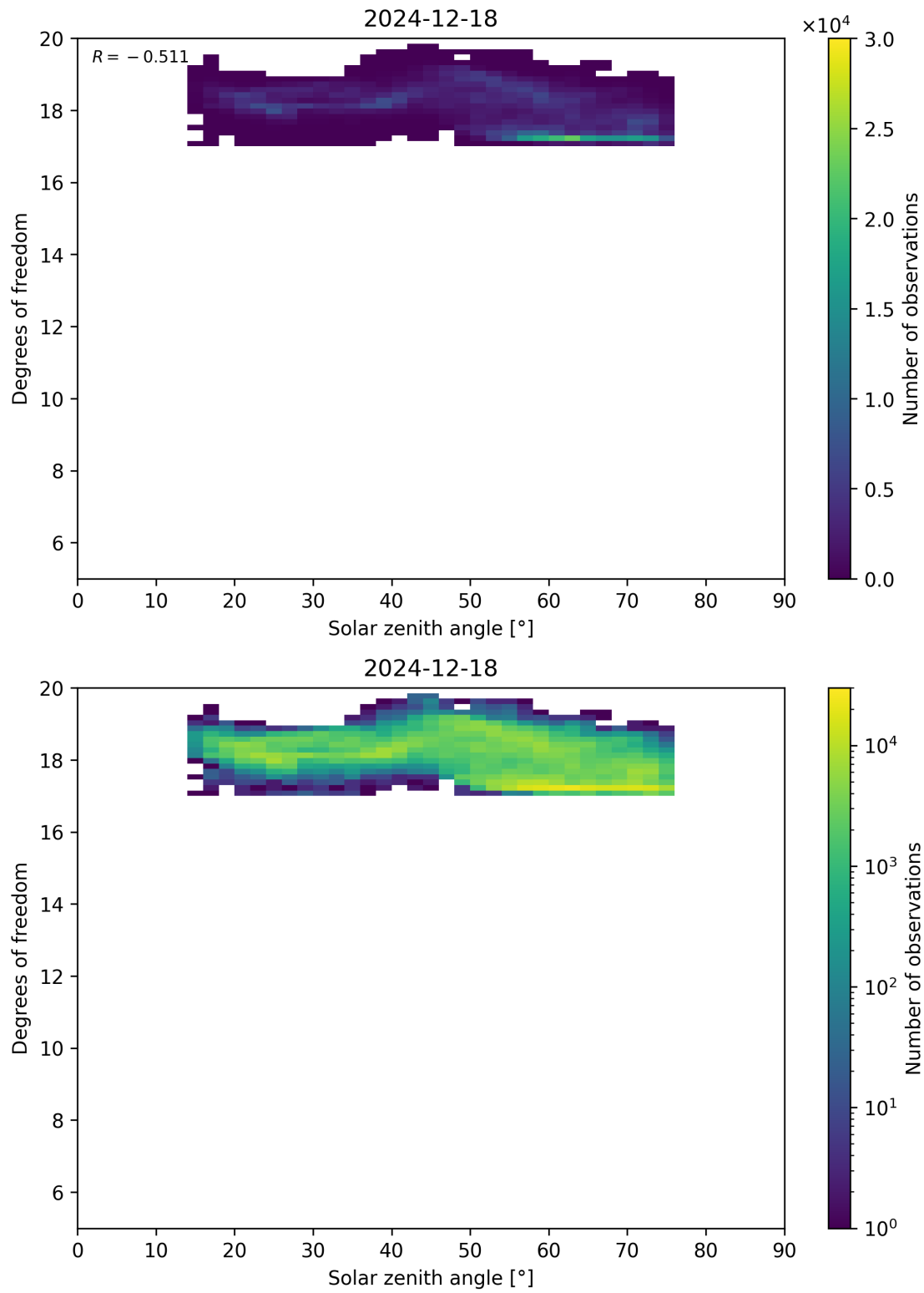
Figure 96: Scatter density plot of “Solar zenith angle” against “Degrees of freedom” for 2024-12-17 to 2024-12-19.
