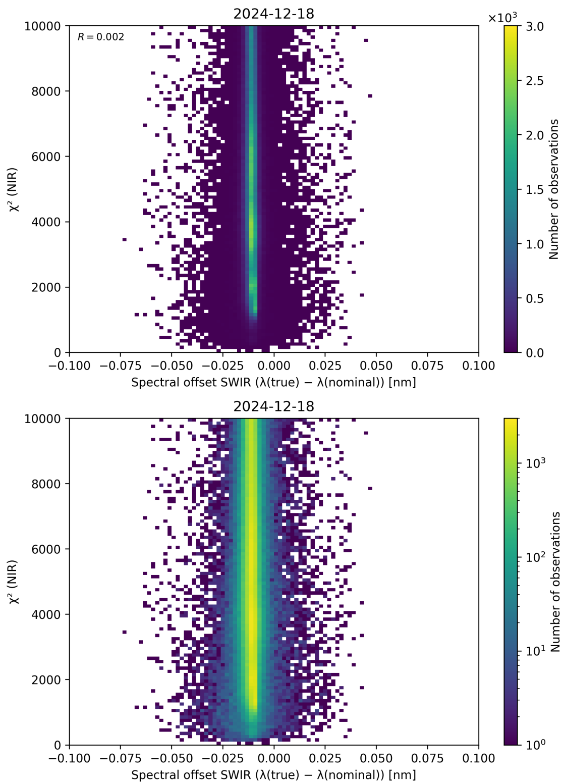
Figure 117: Scatter density plot of “Spectral offset SWIR ( \lambda_{\text{true}} - \lambda_{\text{nominal}} )” against “ \chi^2 (NIR)” for 2024-12-17 to 2024-12-19.
