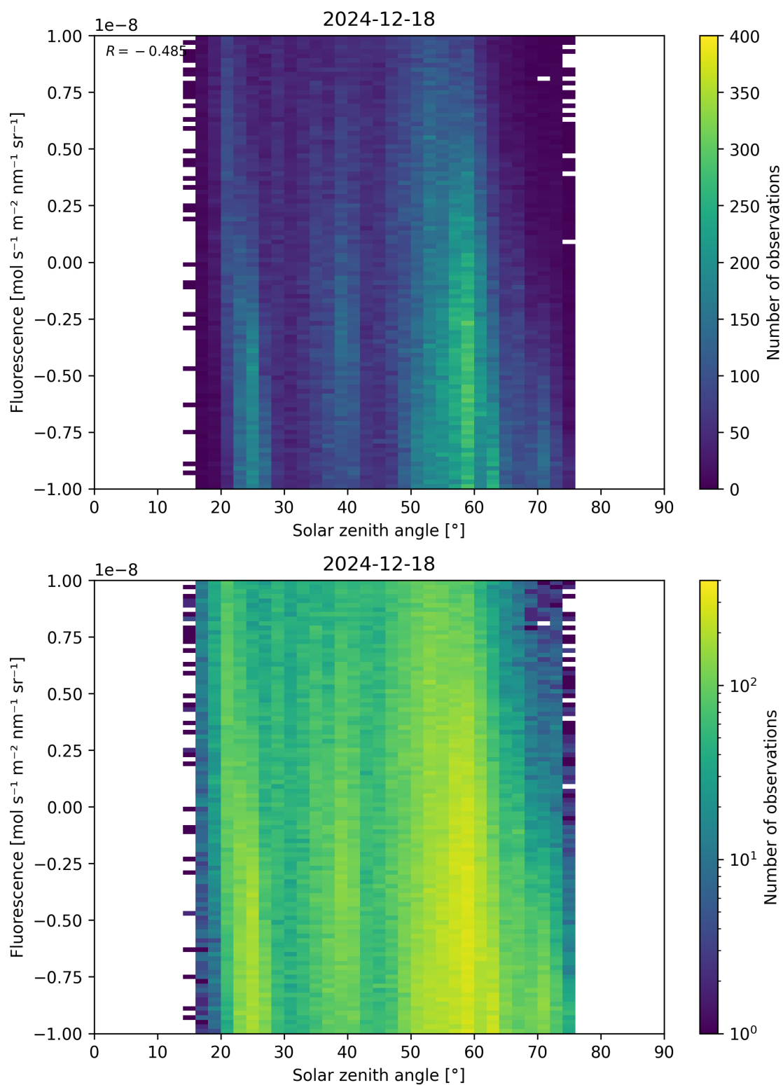
Figure 97: Scatter density plot of “Solar zenith angle” against “Fluorescence” for 2024-12-17 to 2024-12-19.
