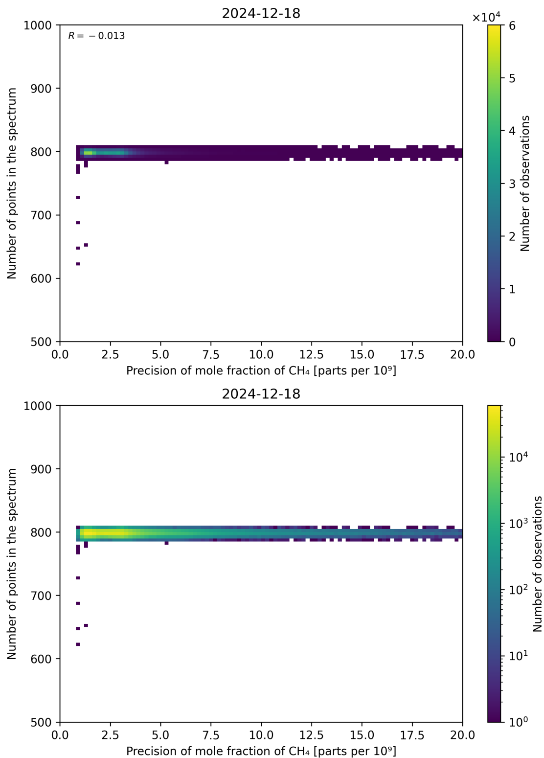
Figure 84: Scatter density plot of “Precision of mole fraction of CH 4 ” against “Number of points in the spectrum” for 2024-12-17 to 2024-12-19.
