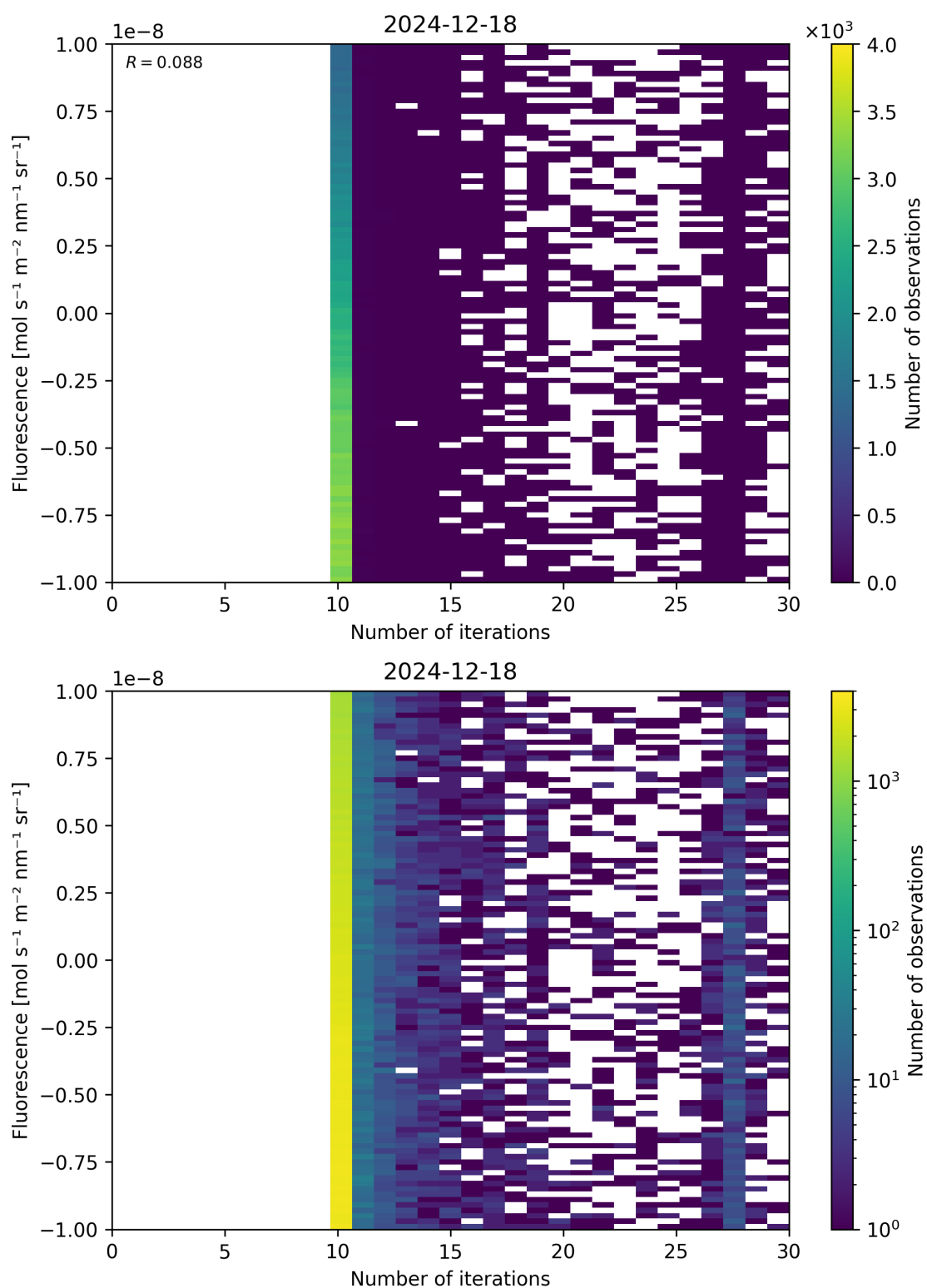
Figure 87: Scatter density plot of “Number of iterations” against “Fluorescence” for 2024-12-17 to 2024-12-19.
