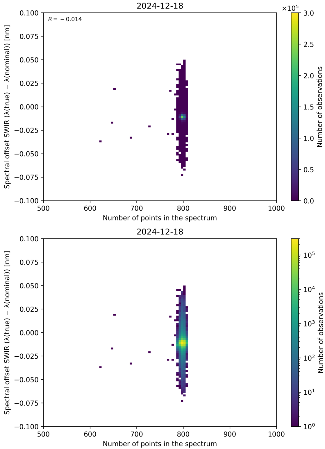
Figure 93: Scatter density plot of “Number of points in the spectrum” against “Spectral offset SWIR ( \lambda_{\text{true}} - \lambda_{\text{nominal}} )” for 2024-12-17 to 2024-12-19.
