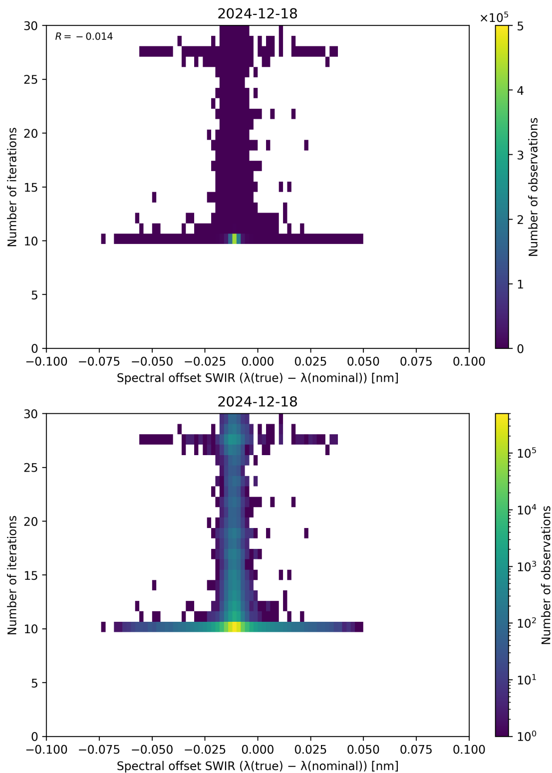
Figure 121: Scatter density plot of “Spectral offset SWIR ( \lambda_{\text{true}} - \lambda_{\text{nominal}} )” against “Number of iterations” for 2024-12-17 to 2024-12-19.
