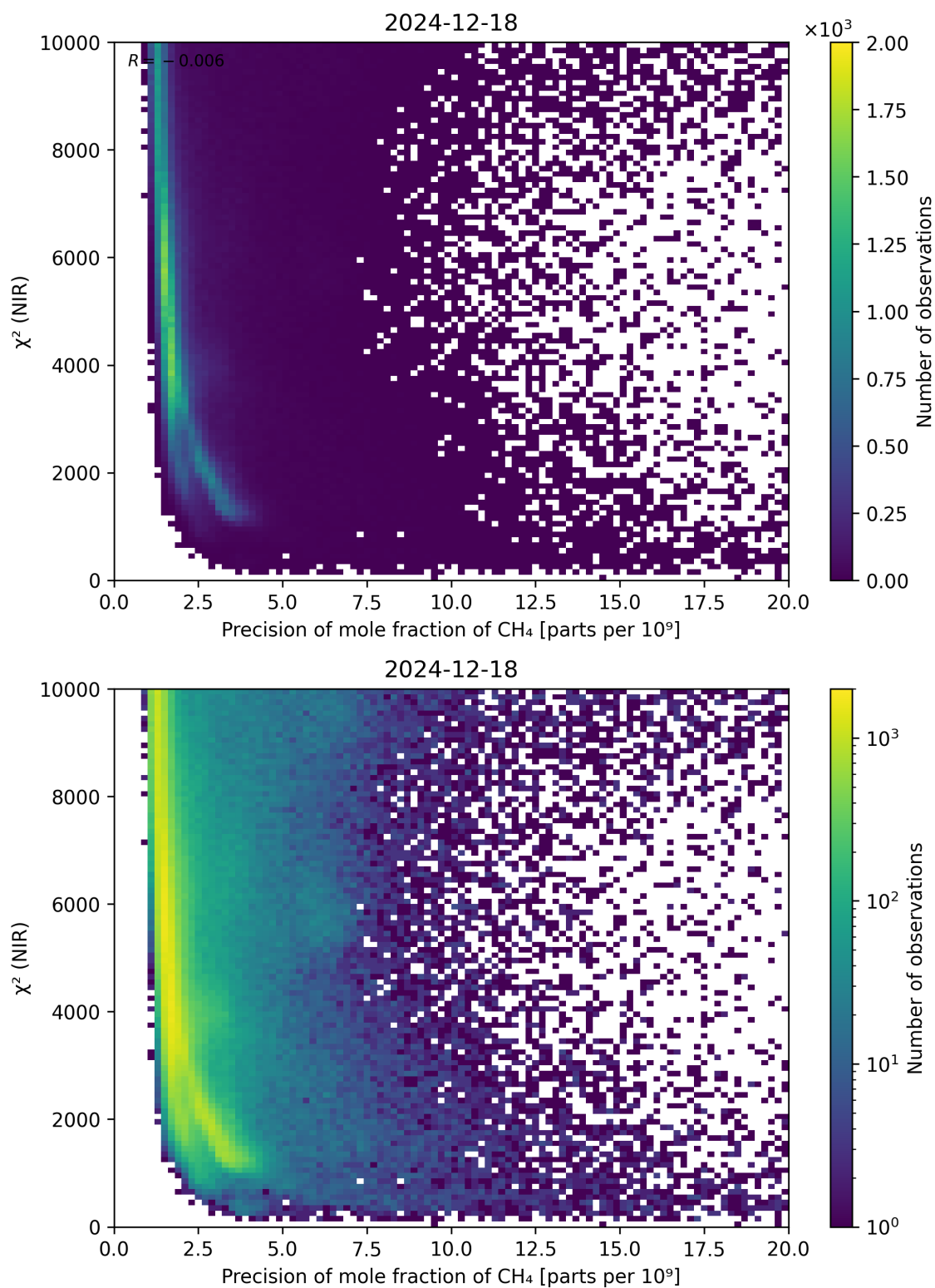
Figure 78: Scatter density plot of “Precision of mole fraction of \text{CH}_4 ” against “ \chi^2 (NIR)” for 2024-12-17 to 2024-12-19.
