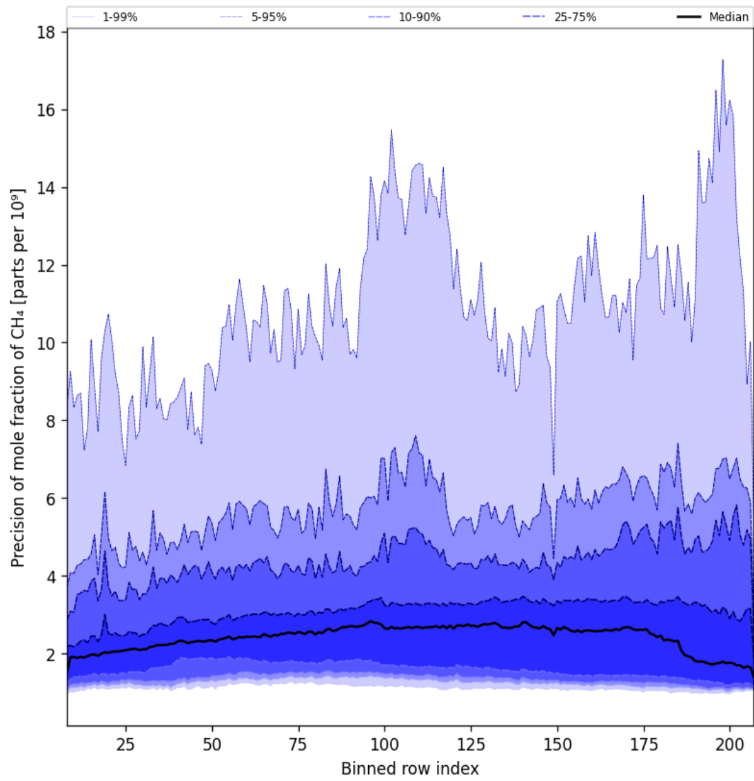
Figure 35: Along track statistics of “Precision of mole fraction of CH 4 ” for 2024-12-17 to 2024-12-19
