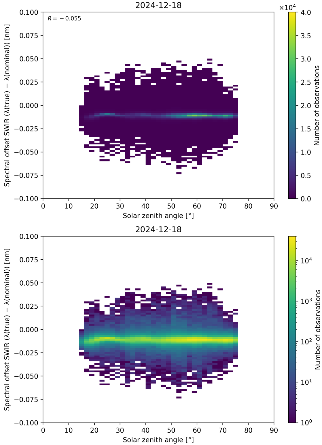
Figure 104: Scatter density plot of “Solar zenith angle” against “Spectral offset SWIR ( \lambda_{\text{true}} - \lambda_{\text{nominal}} )” for 2024-12-17 to 2024-12-19.
