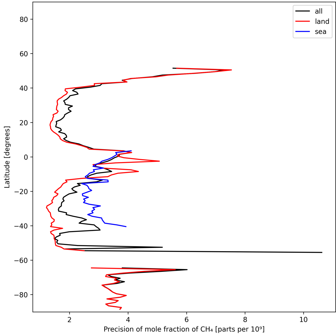
Figure 13: Zonal average of “Precision of mole fraction of CH 4 ” for 2024-12-17 to 2024-12-19.
