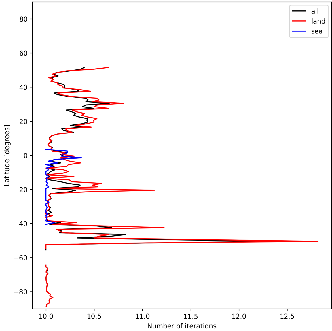
Figure 20: Zonal average of “Number of iterations” for 2024-12-17 to 2024-12-19.
