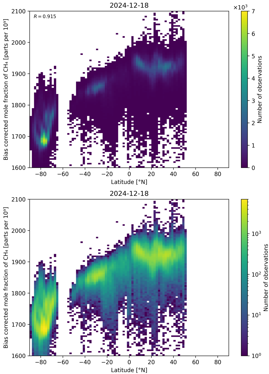
Figure 58: Scatter density plot of “Latitude” against “Bias corrected mole fraction of CH 4 ” for 2024-12-17 to 2024-12-19.
