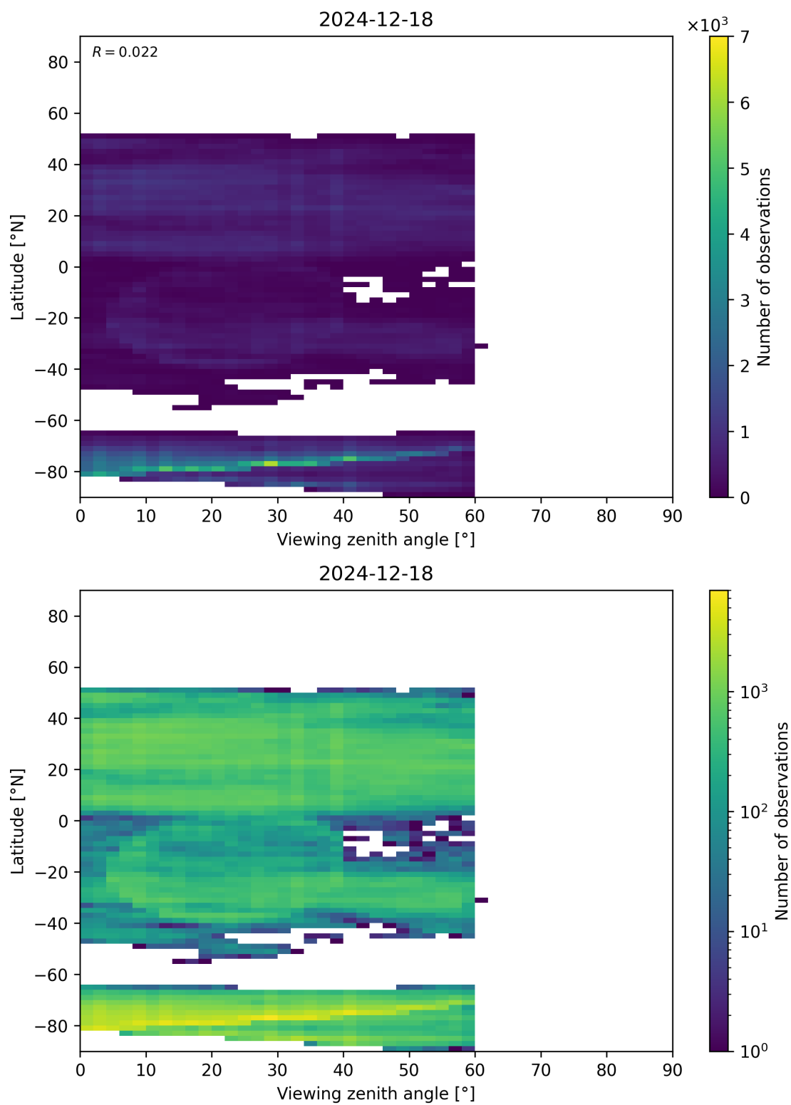
Figure 109: Scatter density plot of “Viewing zenith angle” against “Latitude” for 2024-12-17 to 2024-12-19.
