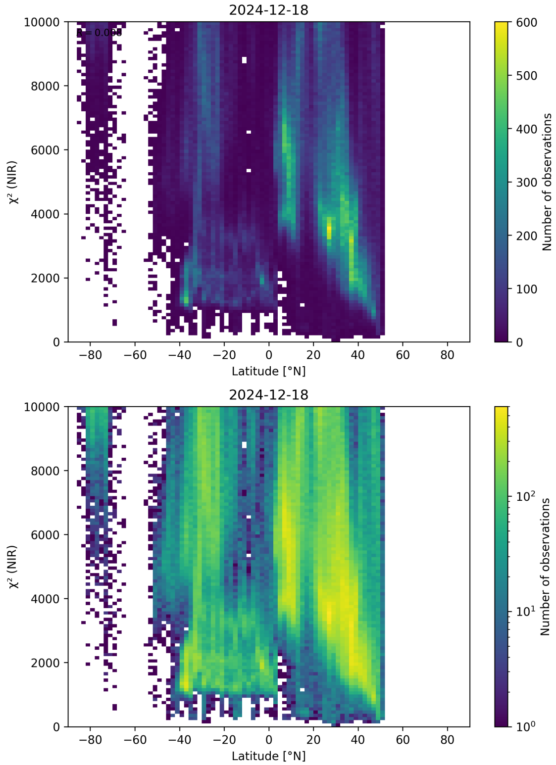
Figure 53: Scatter density plot of “Latitude” against “ \chi^2 (NIR)” for 2024-12-17 to 2024-12-19.
