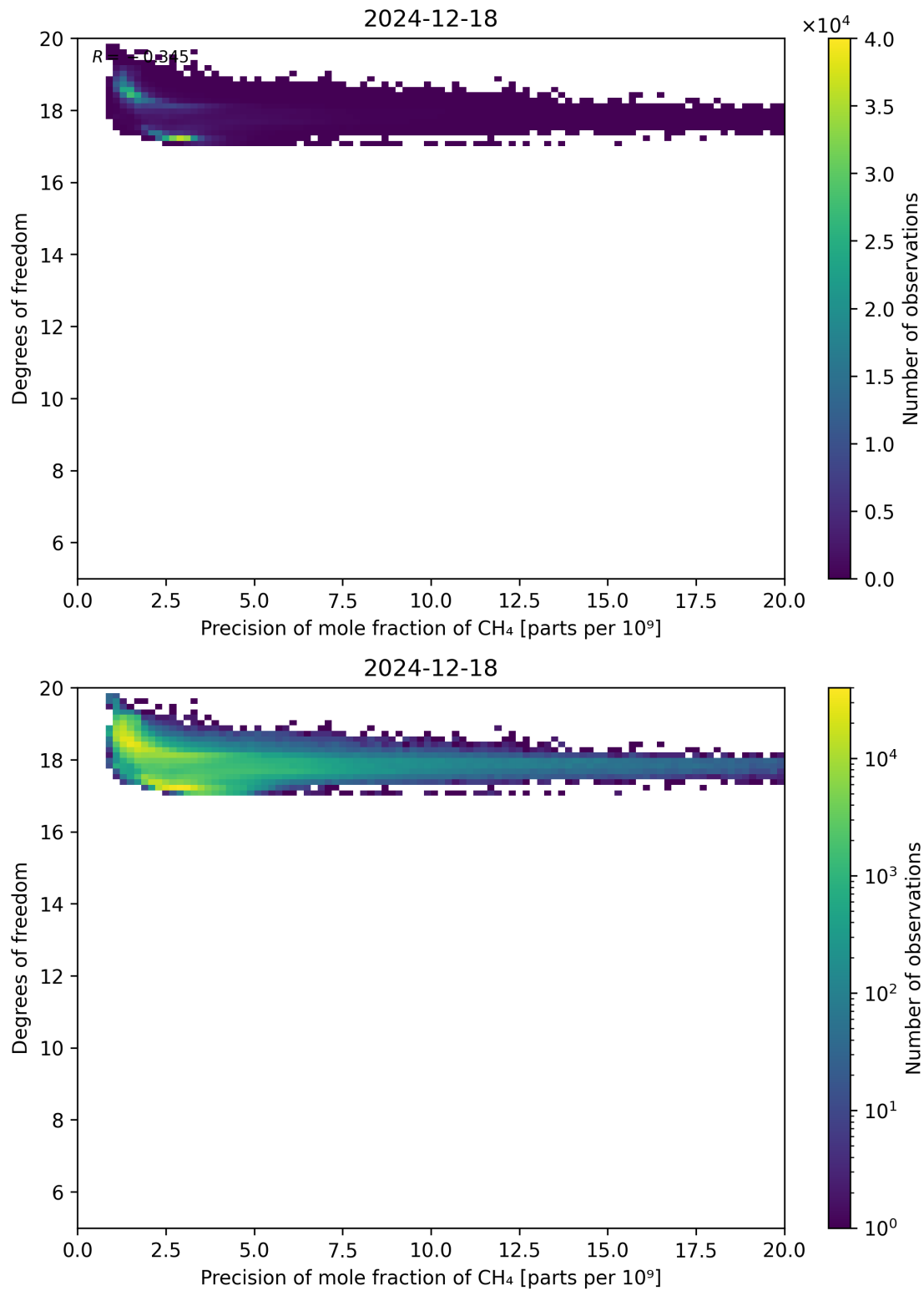
Figure 80: Scatter density plot of “Precision of mole fraction of CH 4 ” against “Degrees of freedom” for 2024-12-17 to 2024-12-19.
