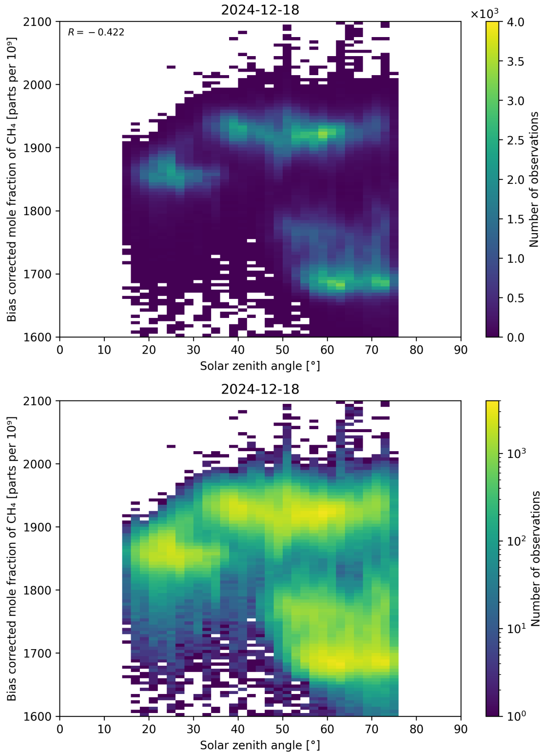
Figure 100: Scatter density plot of “Solar zenith angle” against “Bias corrected mole fraction of CH 4 ” for 2024-12-17 to 2024-12-19.
