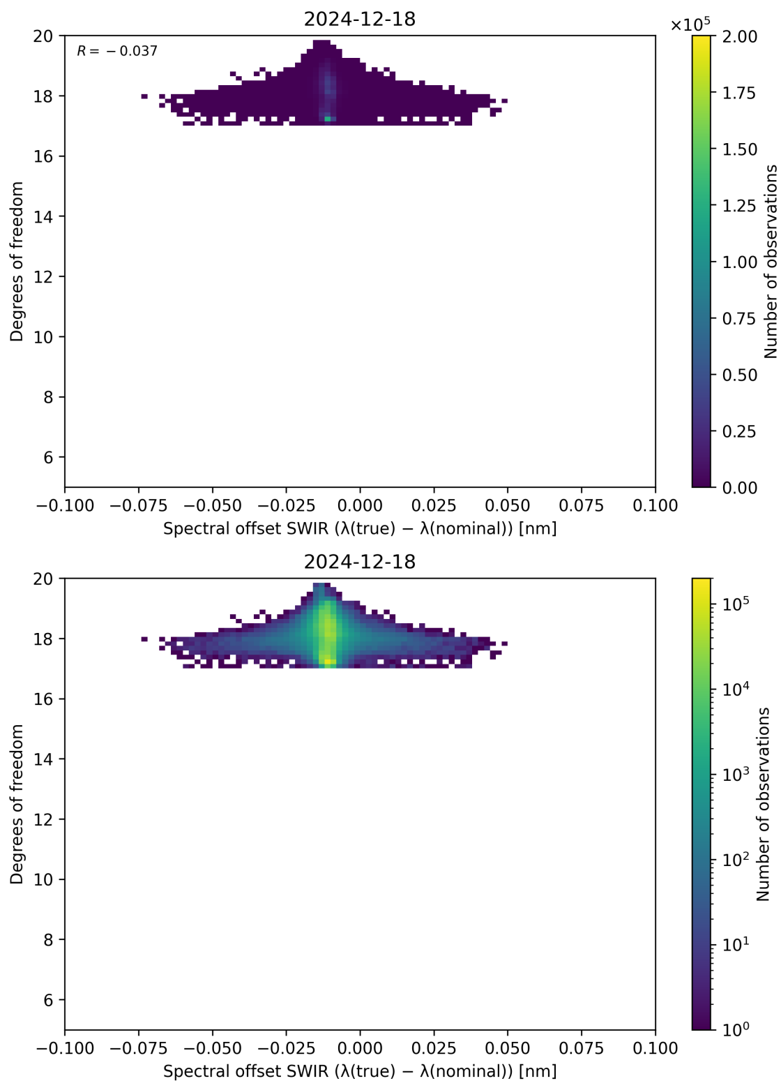
Figure 119: Scatter density plot of “Spectral offset SWIR ( \lambda_{\text{true}} - \lambda_{\text{nominal}} )” against “Degrees of freedom” for 2024-12-17 to 2024-12-19.
