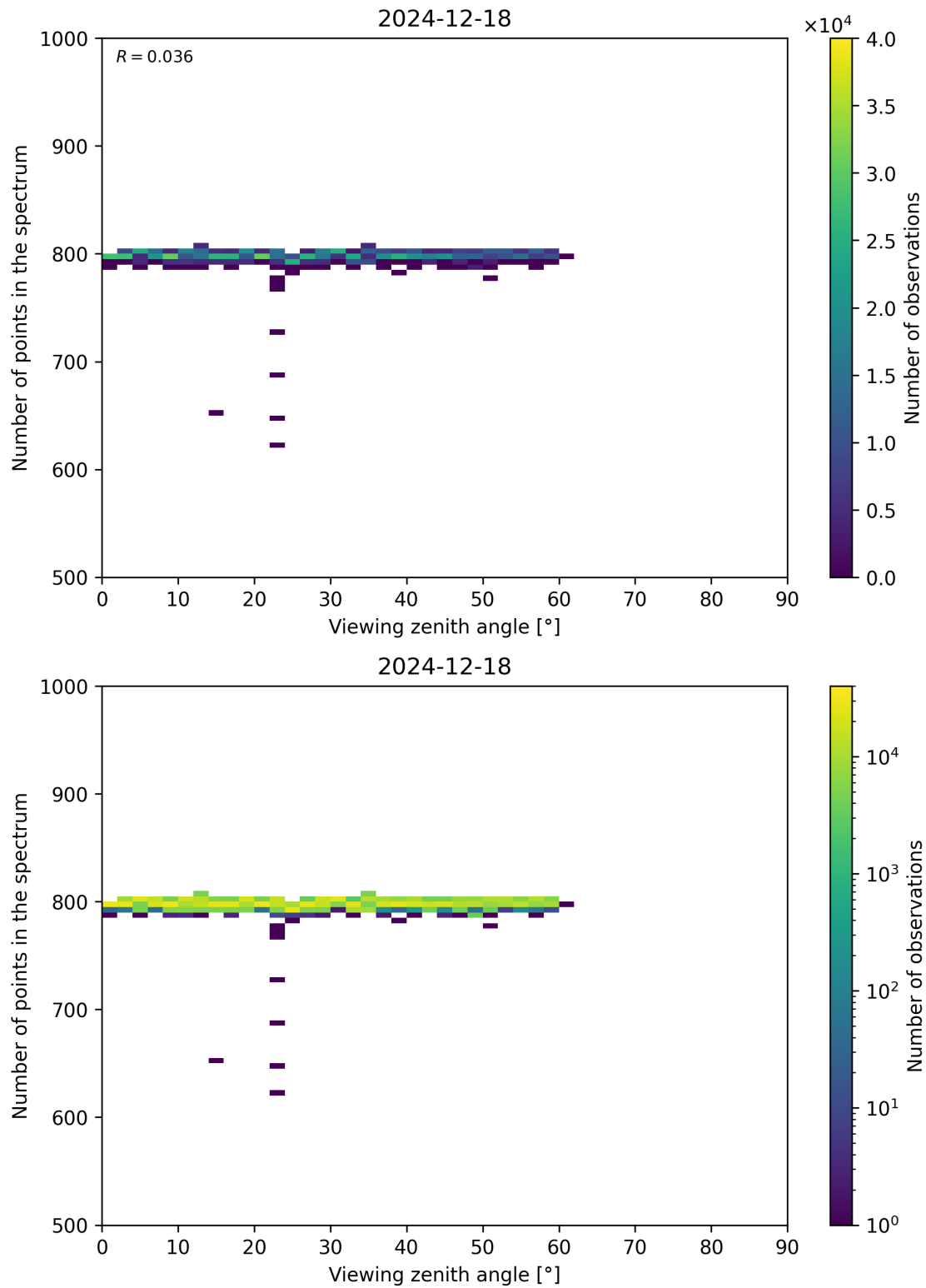
Figure 114: Scatter density plot of “Viewing zenith angle” against “Number of points in the spectrum” for 2024-12-17 to 2024-12-19.
