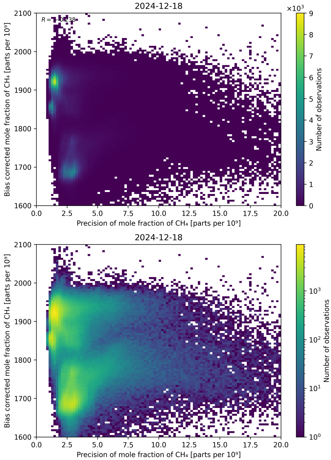
Figure 82: Scatter density plot of “Precision of mole fraction of \text{CH}_4 ” against “Bias corrected mole fraction of \text{CH}_4 ” for 2024-12-17 to 2024-12-19.
