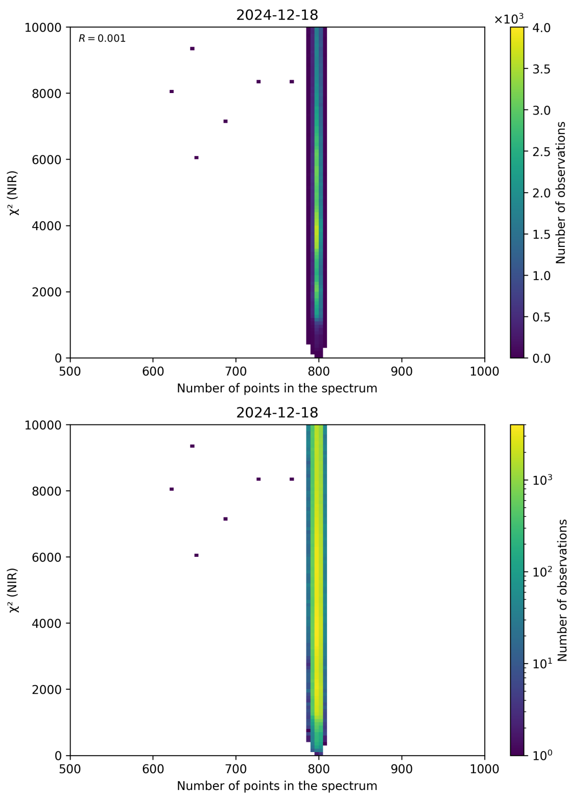
Figure 88: Scatter density plot of “Number of points in the spectrum” against “ \chi^2 (NIR)” for 2024-12-17 to 2024-12-19.
