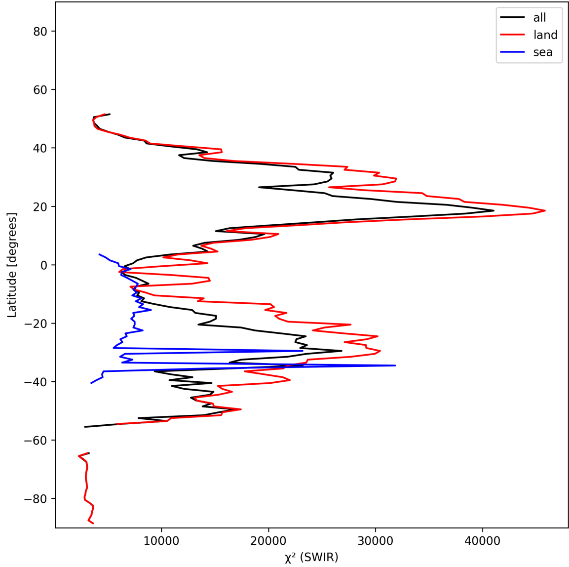
Figure 17: Zonal average of “ \chi^2 (SWIR)” for 2024-12-17 to 2024-12-19.
