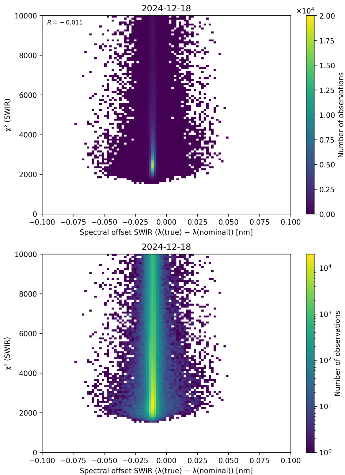
Figure 118: Scatter density plot of “Spectral offset SWIR ( \lambda_{\text{true}} - \lambda_{\text{nominal}} )” against “ \chi^2 (SWIR)” for 2024-12-17 to 2024-12-19.
