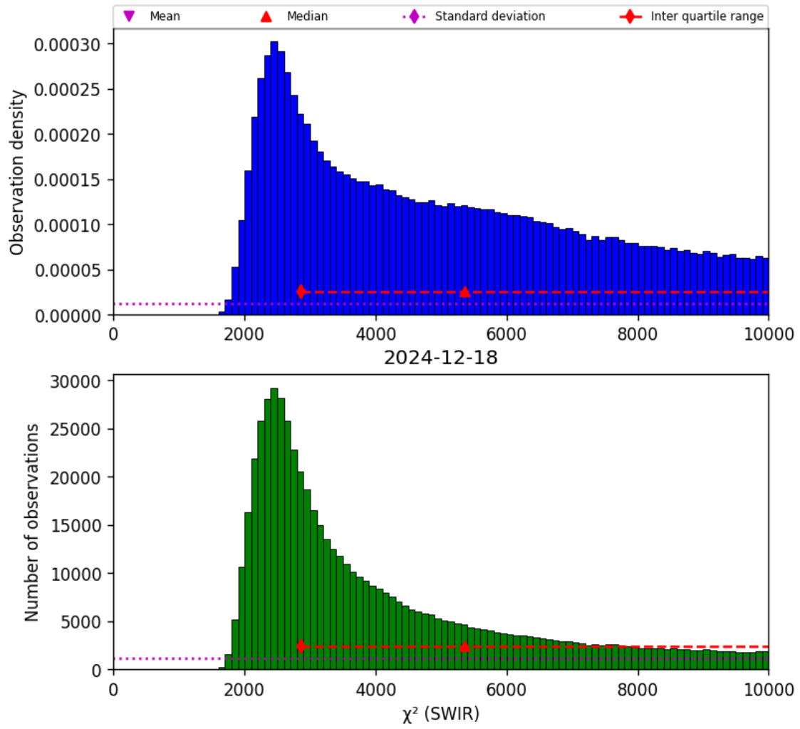
Figure 28: Histogram of “ \chi^2 (SWIR)” for 2024-12-17 to 2024-12-19
