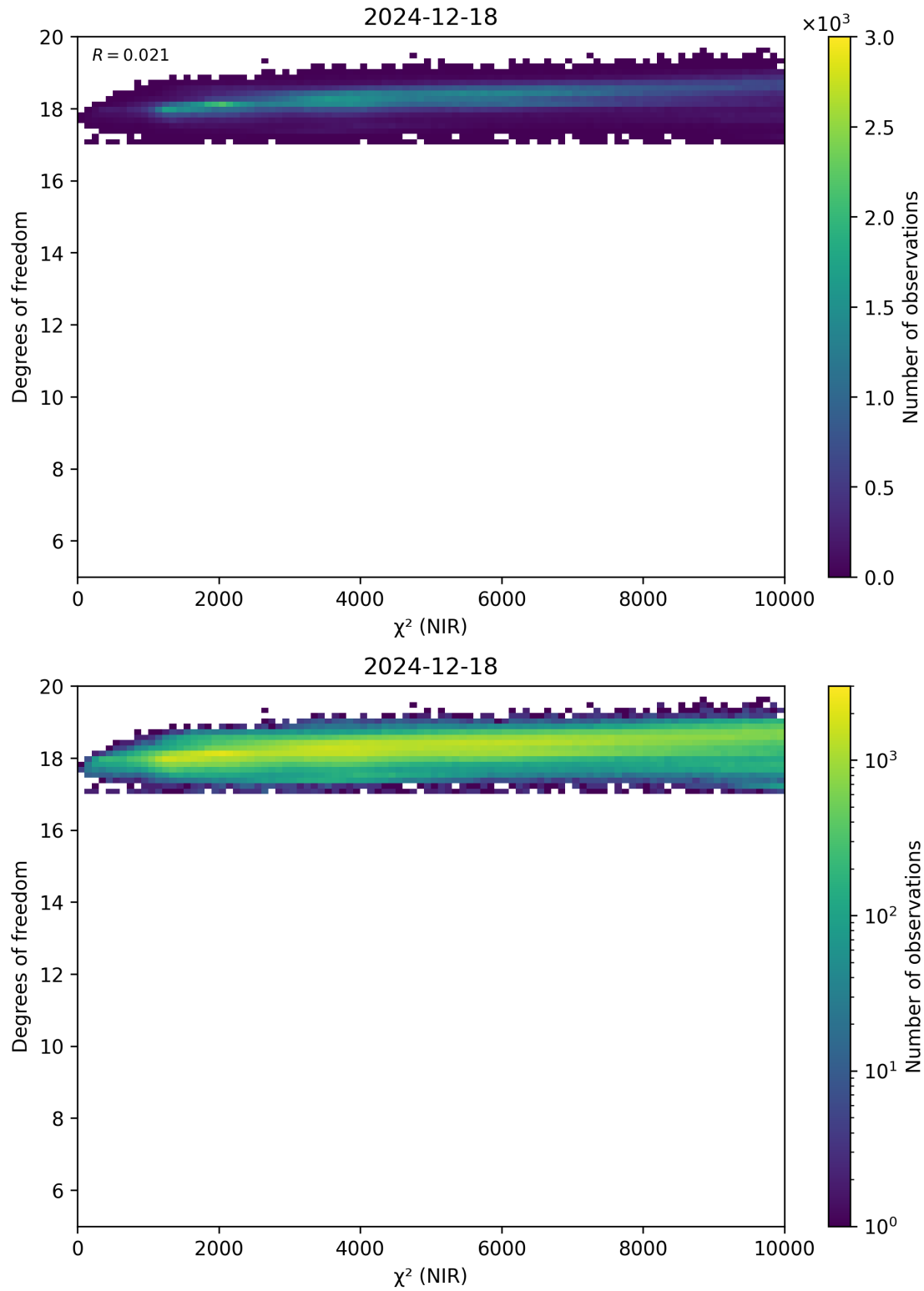
Figure 44: Scatter density plot of “ \chi^2 (NIR)” against “Degrees of freedom” for 2024-12-17 to 2024-12-19.
