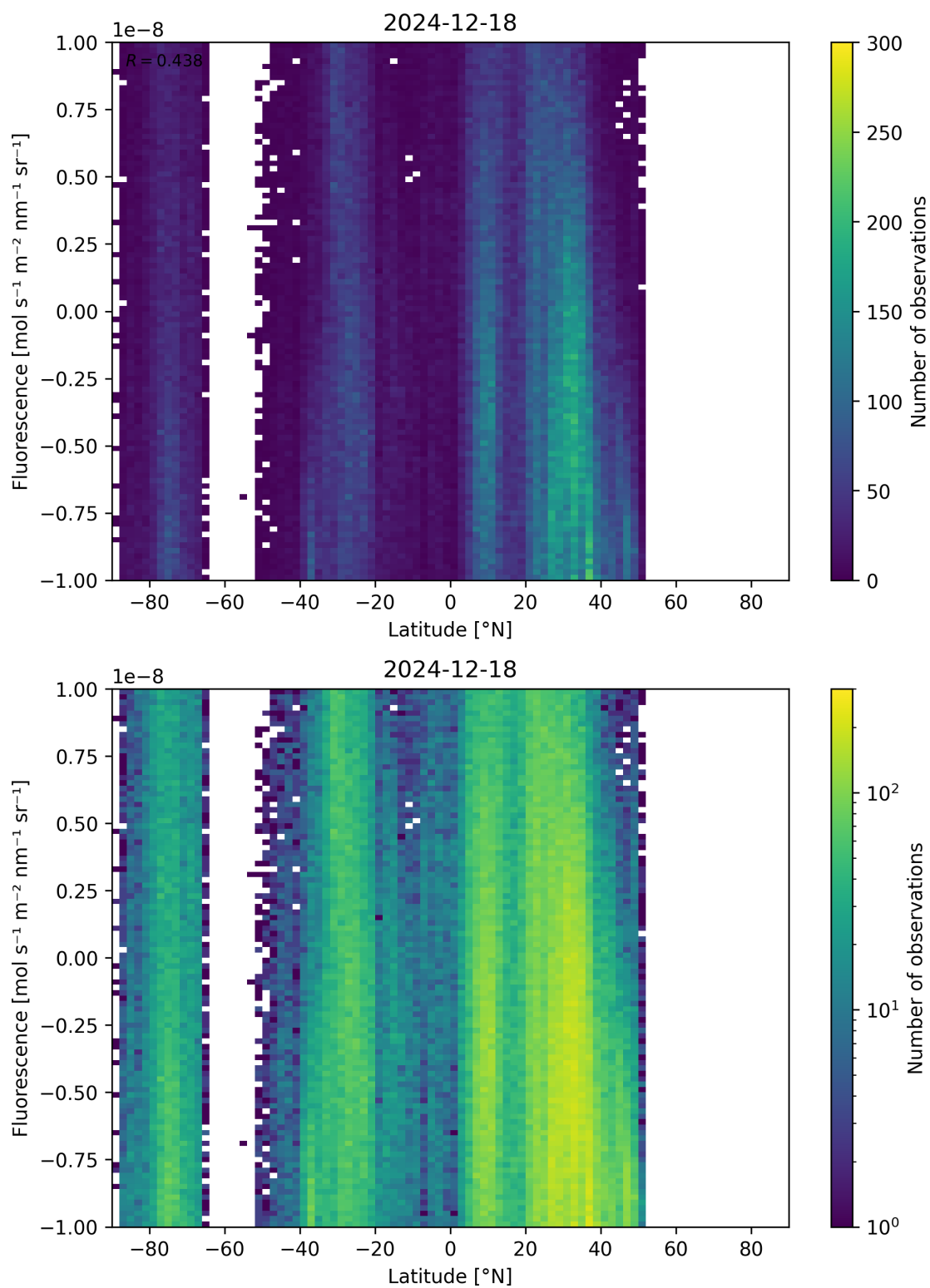
Figure 56: Scatter density plot of “Latitude” against “Fluorescence” for 2024-12-17 to 2024-12-19.
