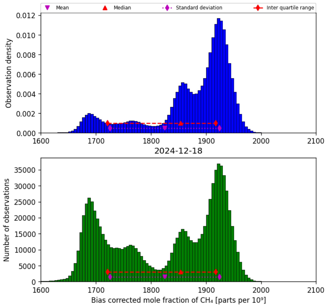
Figure 25: Histogram of “Bias corrected mole fraction of CH 4 ” for 2024-12-17 to 2024-12-19
