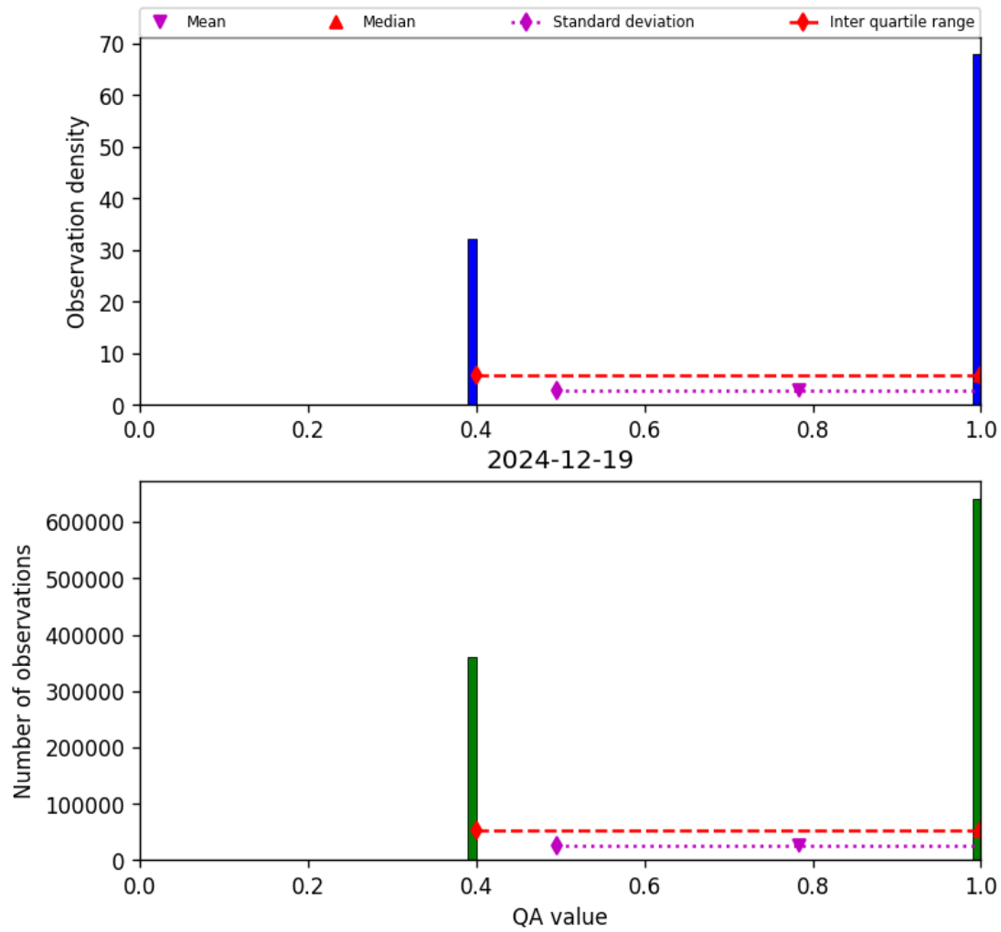
Figure 22: Histogram of “QA value” for 2024-12-18 to 2024-12-20
