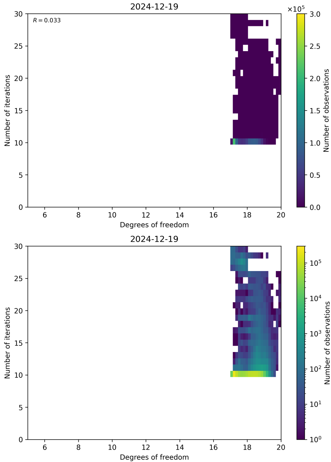
Figure 52: Scatter density plot of “Degrees of freedom” against “Number of iterations” for 2024-12-18 to 2024-12-20.
