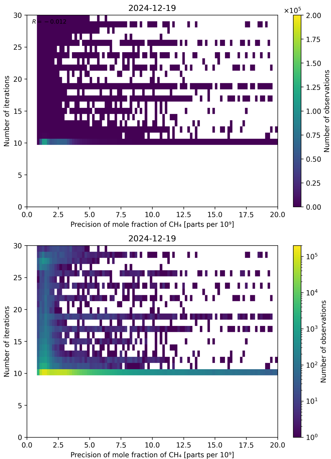
Figure 83: Scatter density plot of “Precision of mole fraction of CH 4 ” against “Number of iterations” for 2024-12-18 to 2024-12-20.
