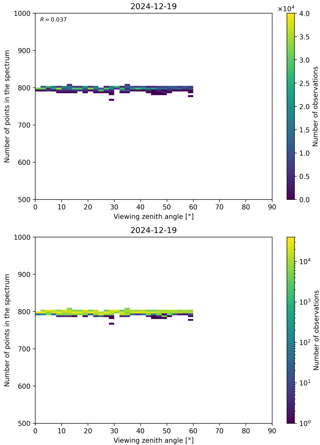
Figure 114: Scatter density plot of “Viewing zenith angle” against “Number of points in the spectrum” for 2024-12-18 to 2024-12-20.
