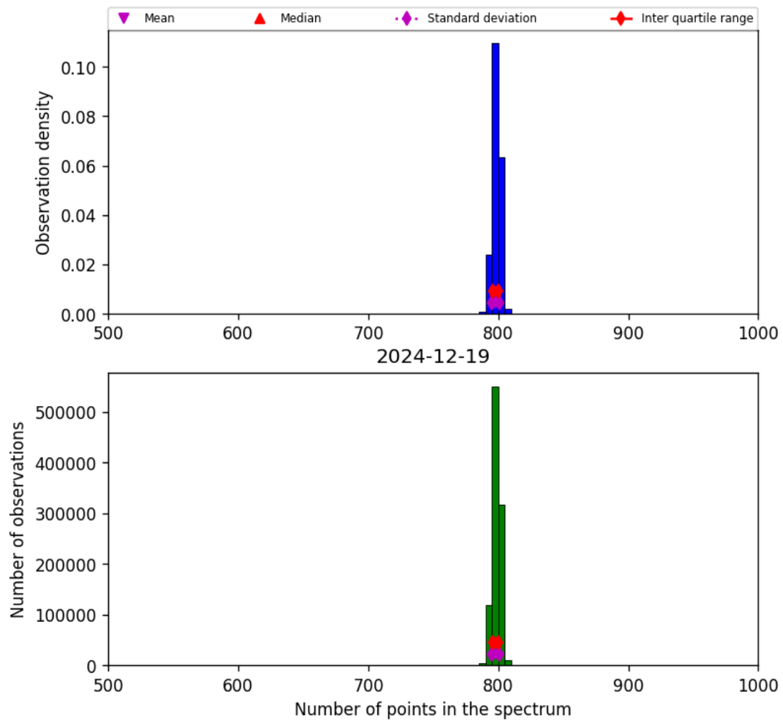
Figure 26: Histogram of “Number of points in the spectrum” for 2024-12-18 to 2024-12-20
