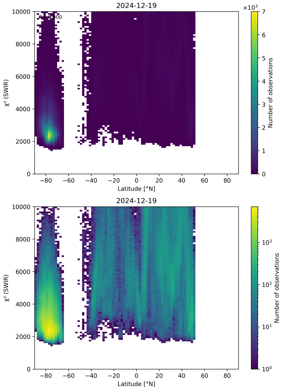
Figure 54: Scatter density plot of “Latitude” against “ \chi^2 (SWIR)” for 2024-12-18 to 2024-12-20.
