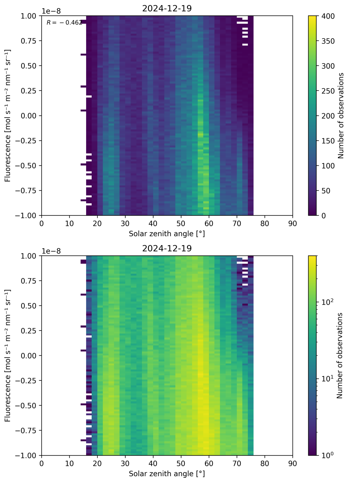
Figure 97: Scatter density plot of “Solar zenith angle” against “Fluorescence” for 2024-12-18 to 2024-12-20.
