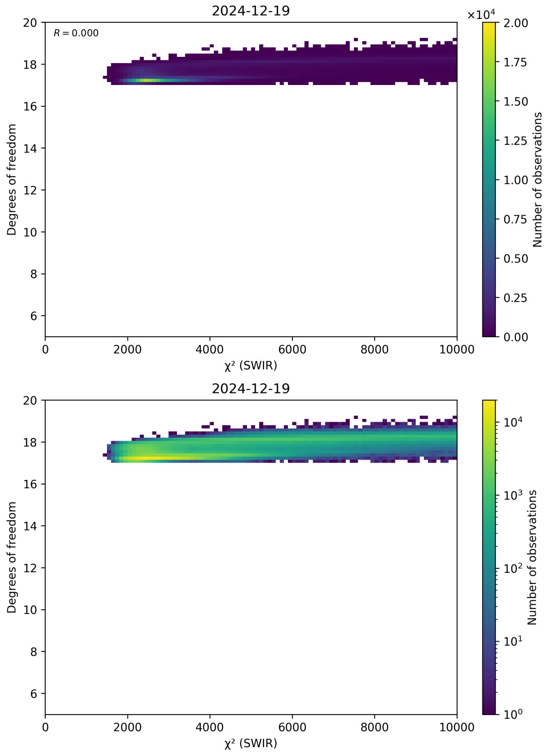
Figure 48: Scatter density plot of “ \chi^2 (SWIR)” against “Degrees of freedom” for 2024-12-18 to 2024-12-20.
