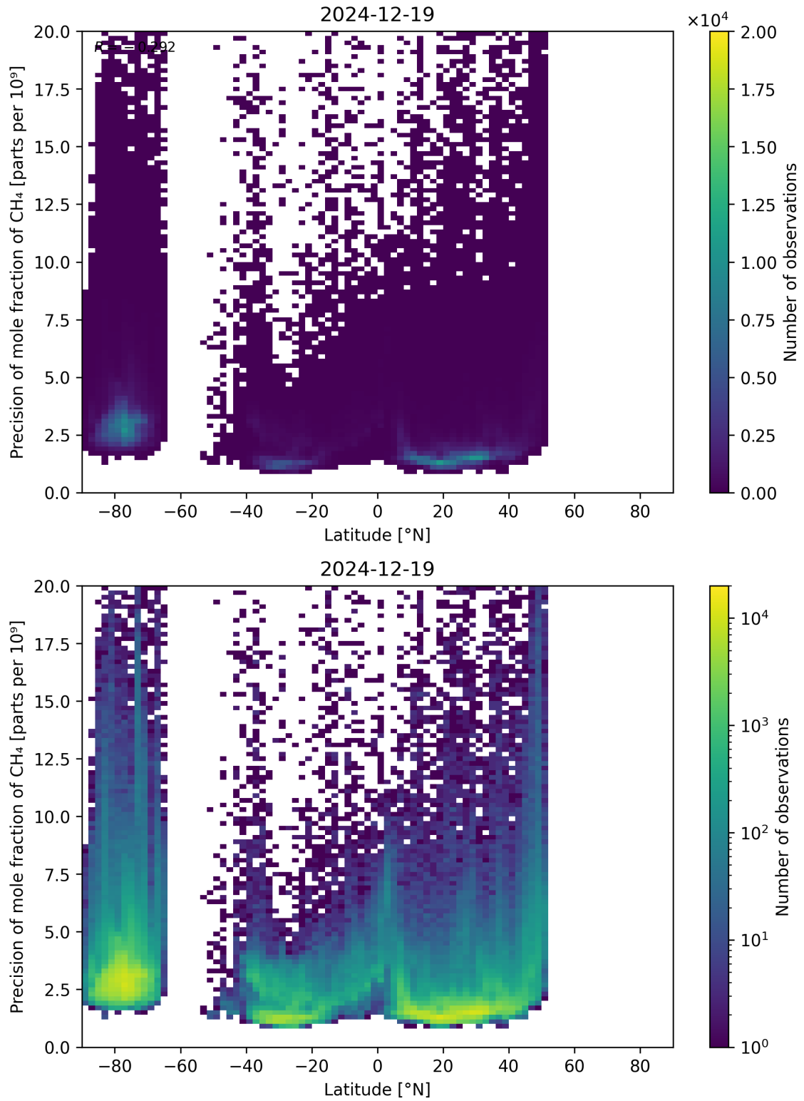
Figure 59: Scatter density plot of “Latitude” against “Precision of mole fraction of CH 4 ” for 2024-12-18 to 2024-12-20.
