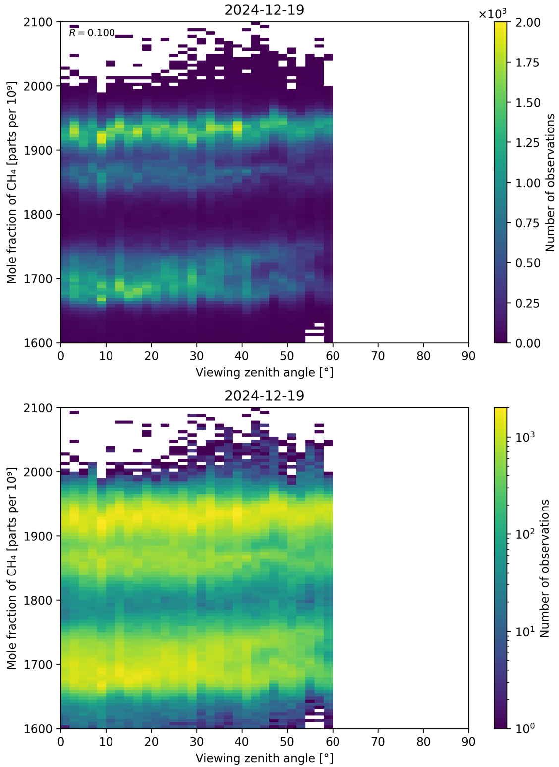
Figure 110: Scatter density plot of “Viewing zenith angle” against “Mole fraction of \text{CH}_4 ” for 2024-12-18 to 2024-12-20.
