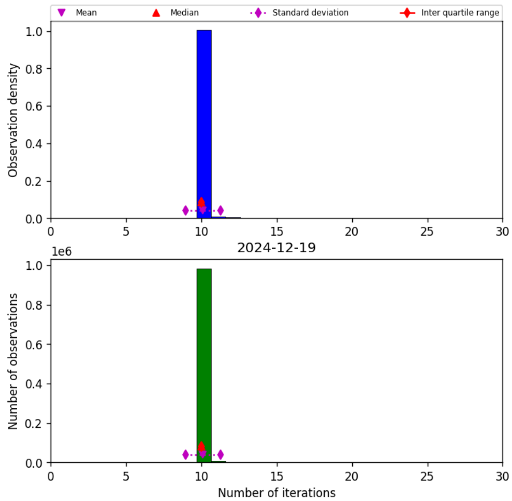
Figure 31: Histogram of “Number of iterations” for 2024-12-18 to 2024-12-20
