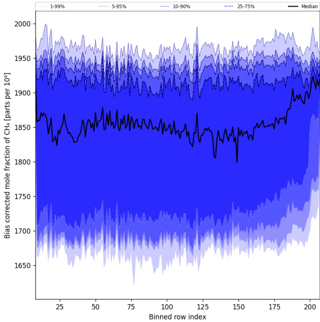
Figure 36: Along track statistics of “Bias corrected mole fraction of CH 4 ” for 2024-12-18 to 2024-12-20
