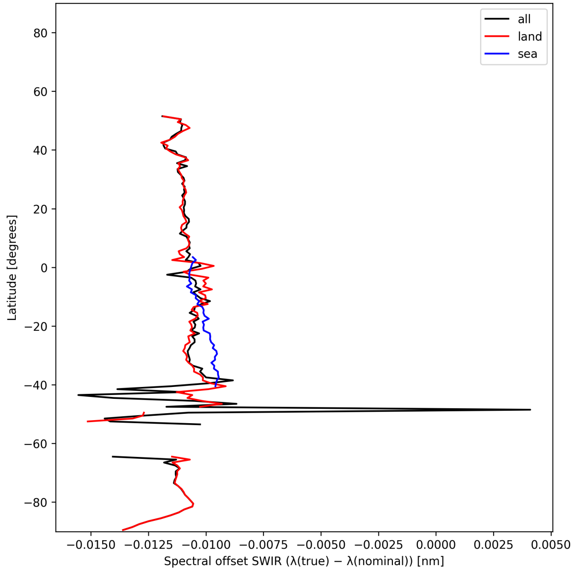
Figure 16: Zonal average of “Spectral offset SWIR ( \lambda_{\text{true}} - \lambda_{\text{nominal}} )” for 2024-12-18 to 2024-12-20.
