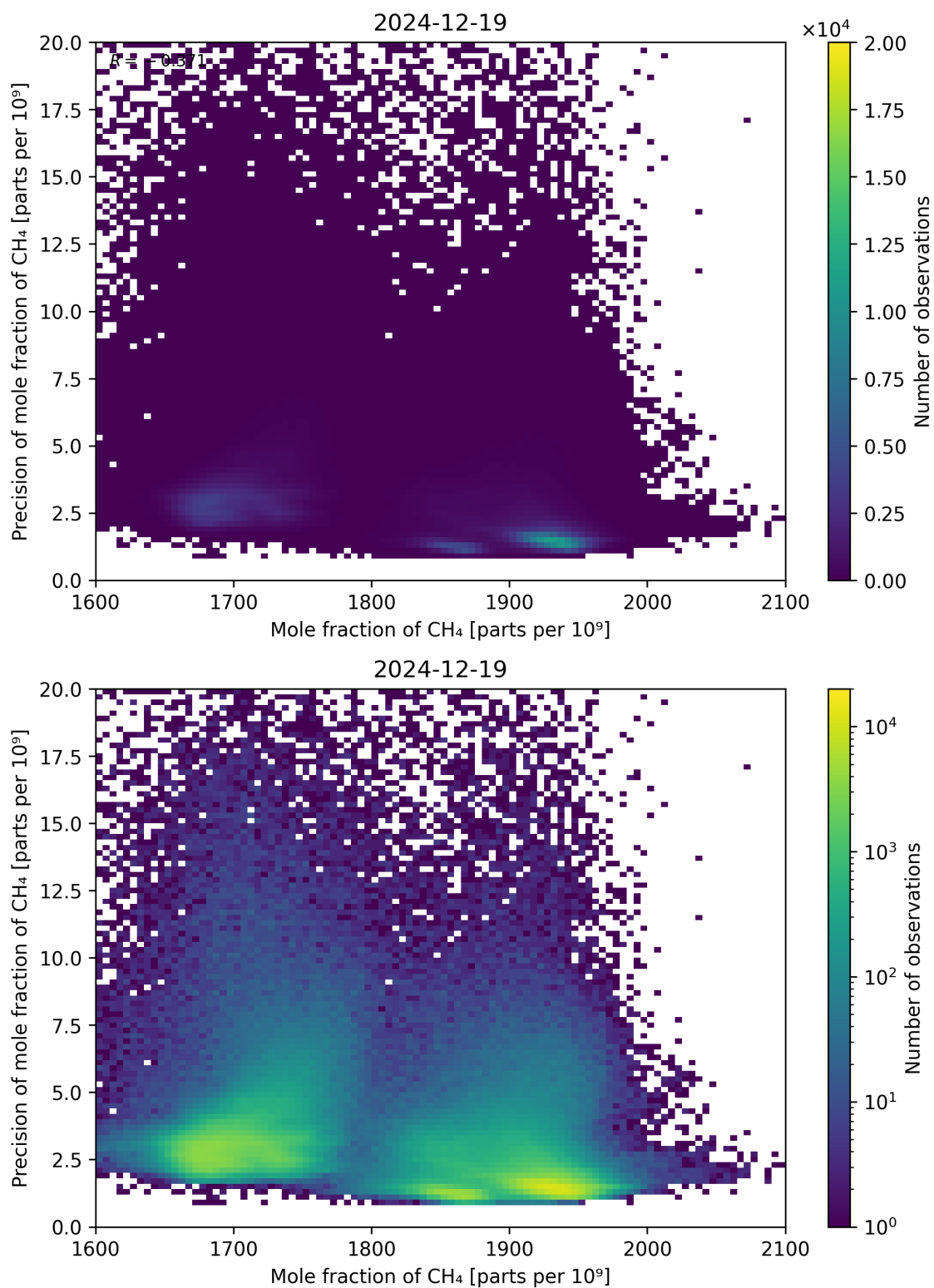
Figure 75: Scatter density plot of “Mole fraction of CH 4 ” against “Precision of mole fraction of CH 4 ” for 2024-12-18 to 2024-12-20.
