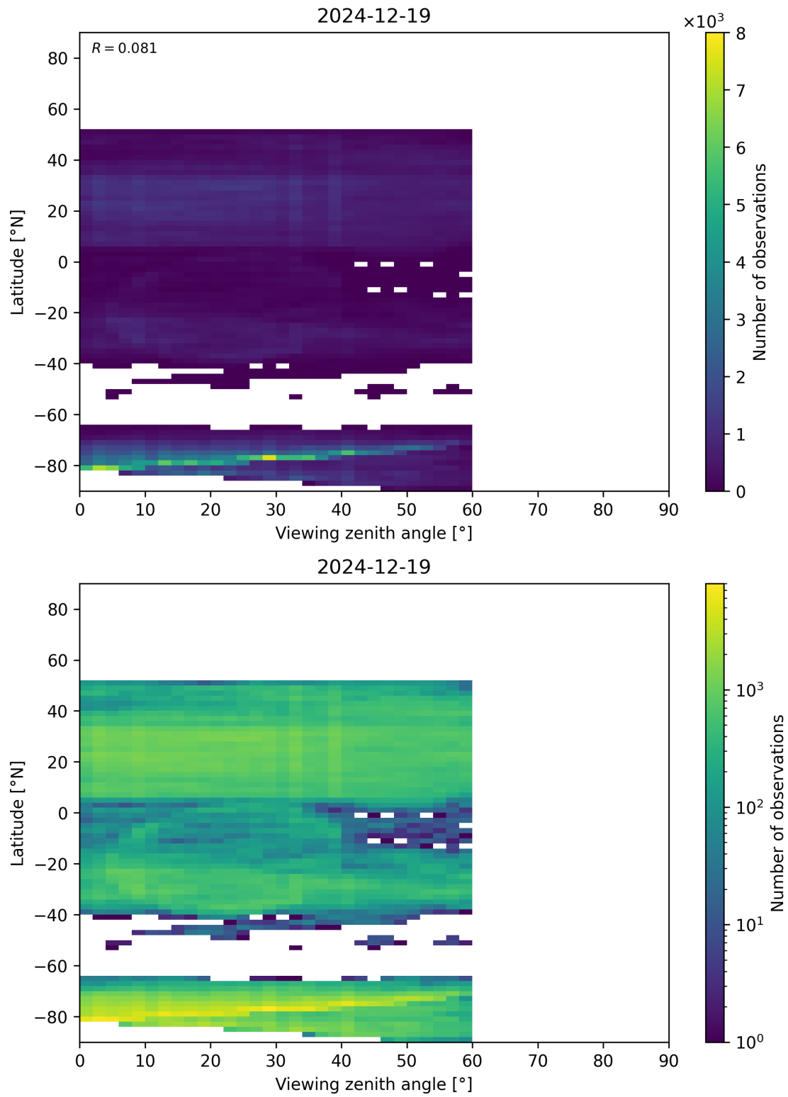
Figure 109: Scatter density plot of “Viewing zenith angle” against “Latitude” for 2024-12-18 to 2024-12-20.
