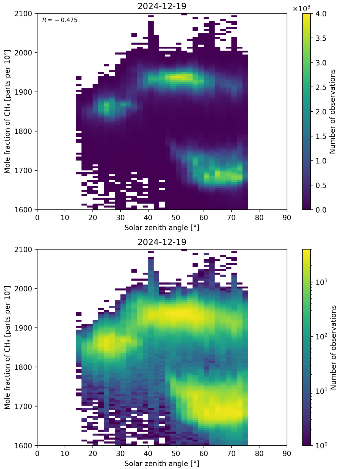
Figure 99: Scatter density plot of “Solar zenith angle” against “Mole fraction of CH 4 ” for 2024-12-18 to 2024-12-20.
