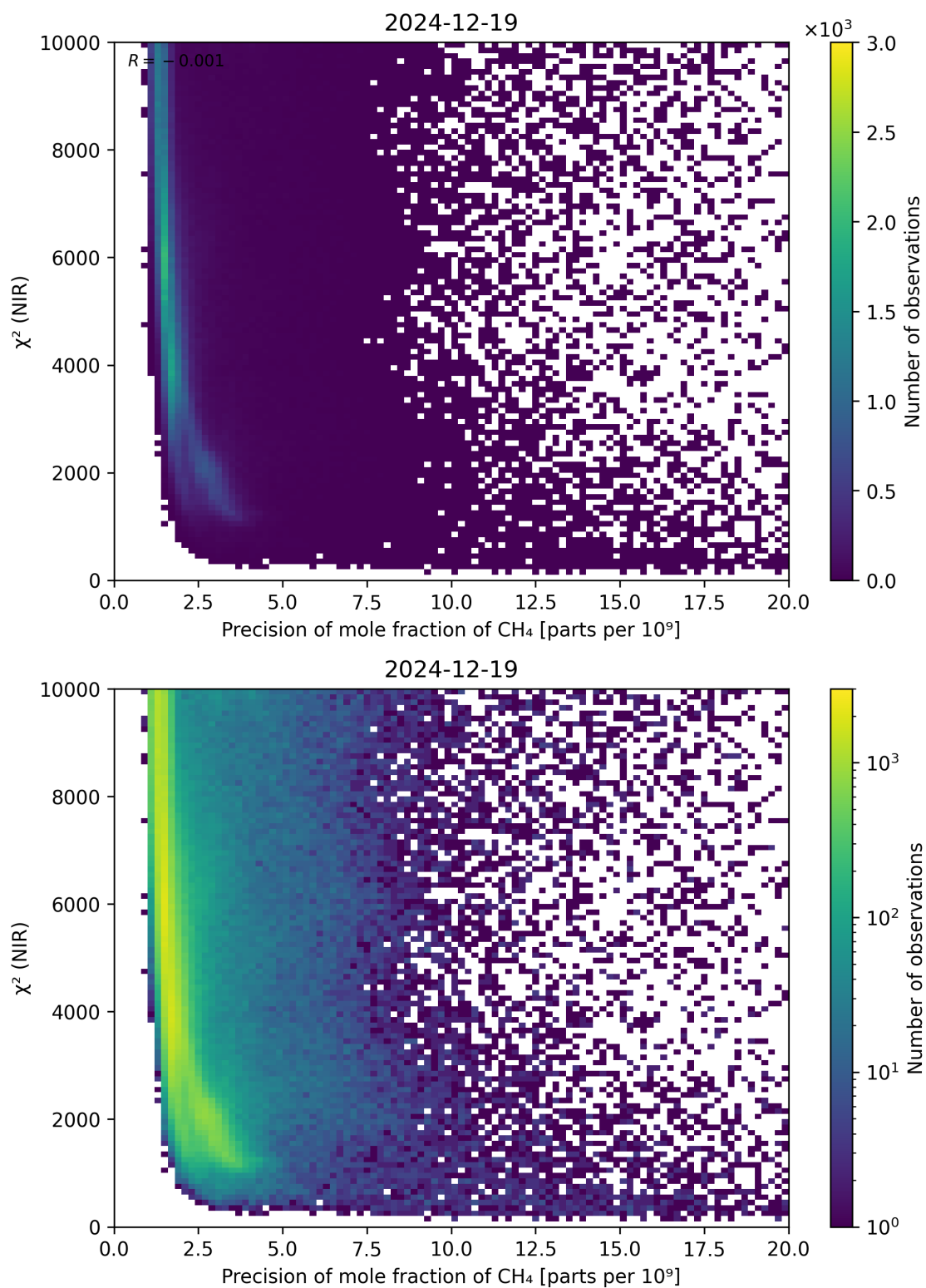
Figure 78: Scatter density plot of “Precision of mole fraction of CH 4 ” against “ \chi^2 (NIR)” for 2024-12-18 to 2024-12-20.
