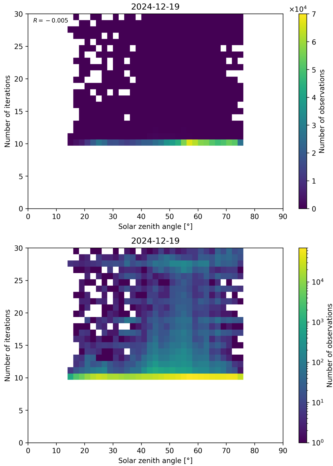
Figure 102: Scatter density plot of “Solar zenith angle” against “Number of iterations” for 2024-12-18 to 2024-12-20.
