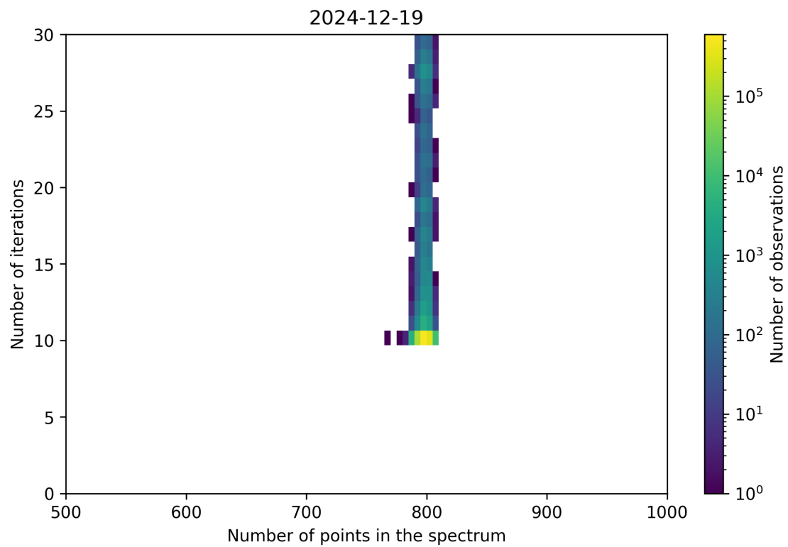
Figure 92: Scatter density plot of “Number of points in the spectrum” against “Number of iterations” for 2024-12-18 to 2024-12-20.
