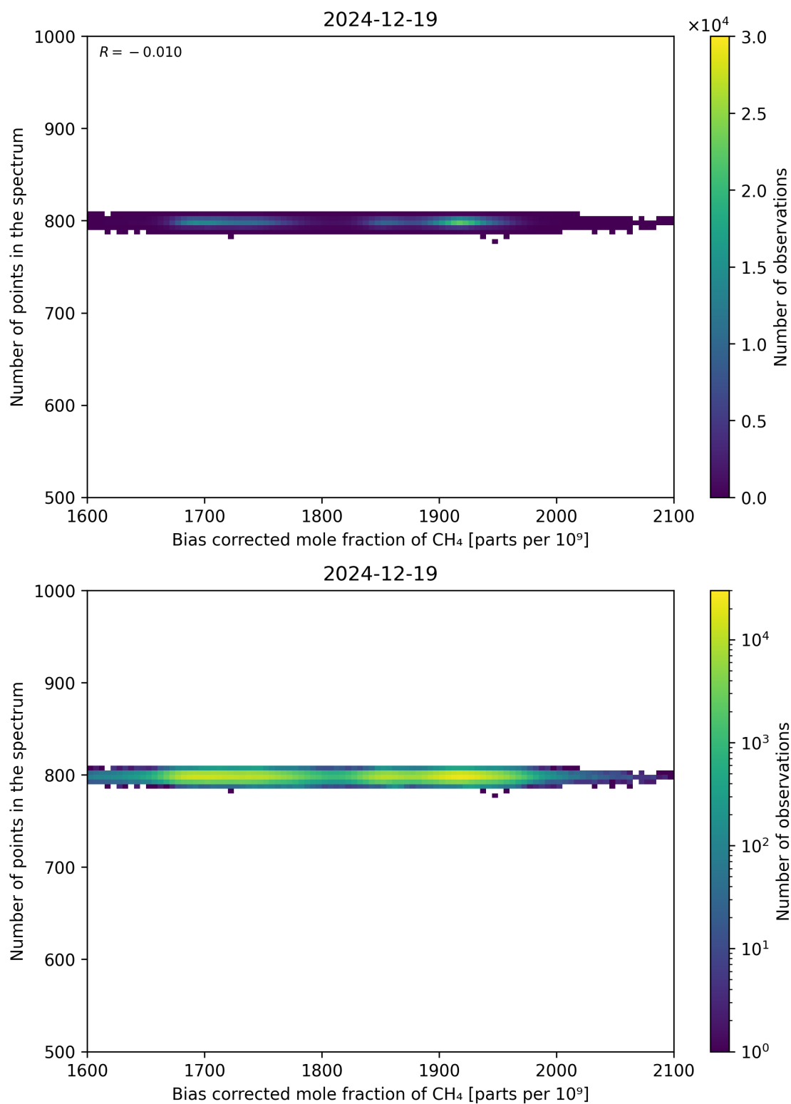
Figure 68: Scatter density plot of “Bias corrected mole fraction of CH 4 ” against “Number of points in the spectrum” for 2024-12-18 to 2024-12-20.
