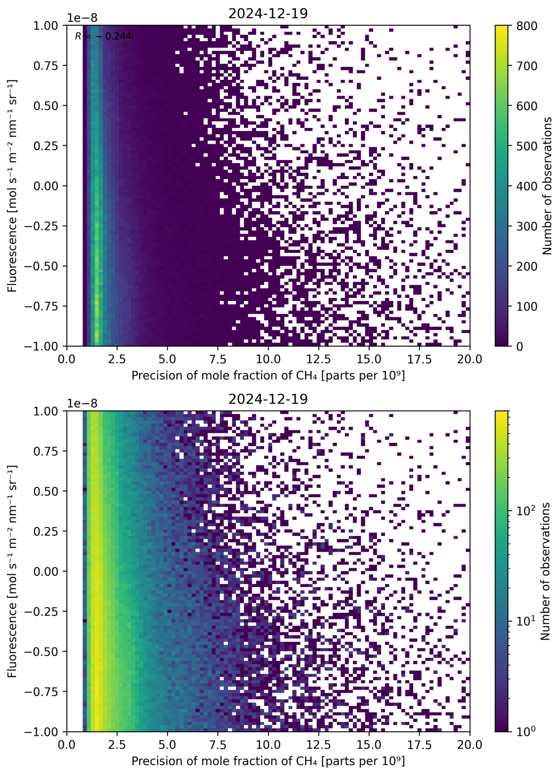
Figure 81: Scatter density plot of “Precision of mole fraction of CH 4 ” against “Fluorescence” for 2024-12-18 to 2024-12-20.
