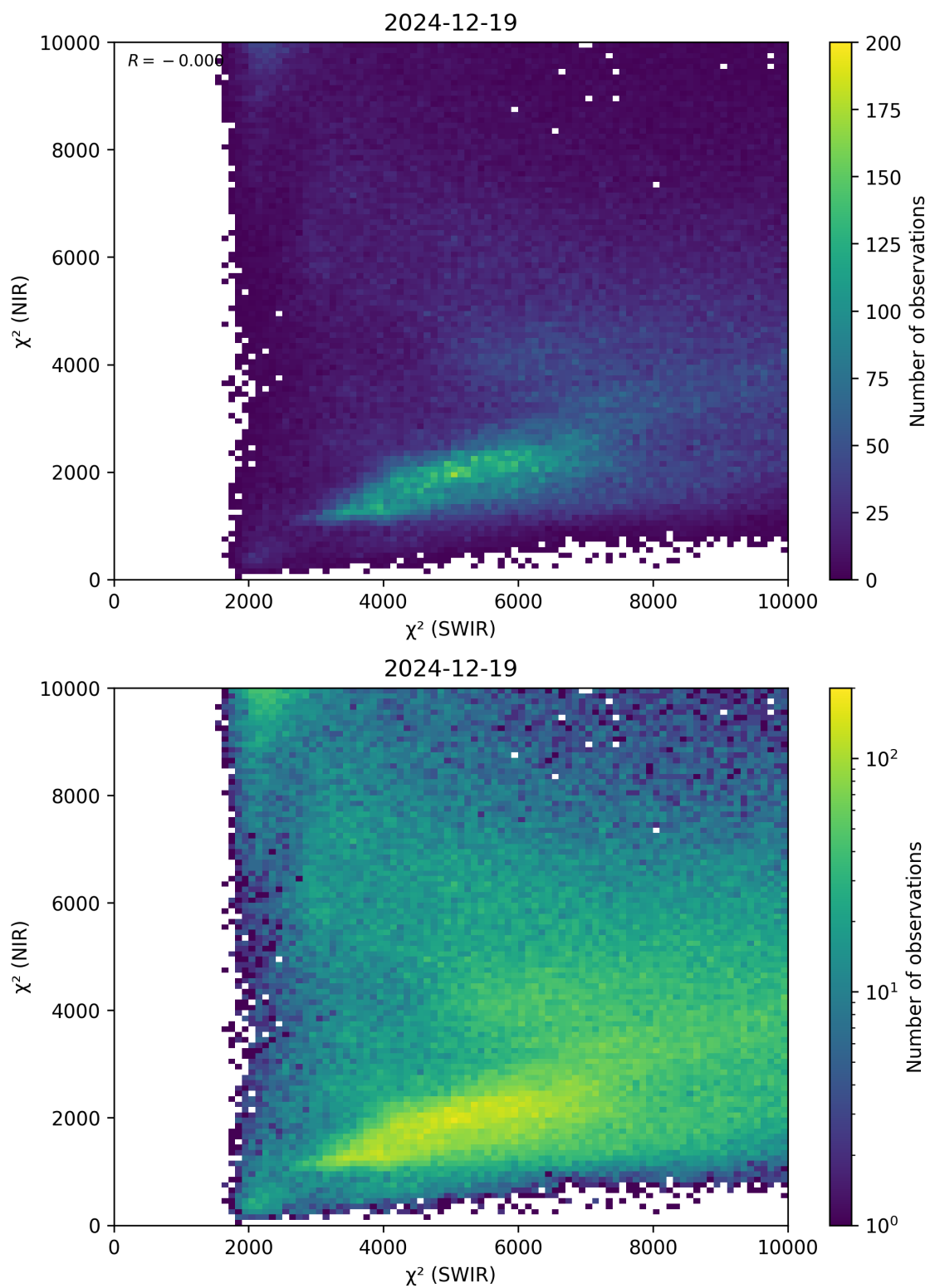
Figure 47: Scatter density plot of “ \chi^2 (SWIR)” against “ \chi^2 (NIR)” for 2024-12-18 to 2024-12-20.
