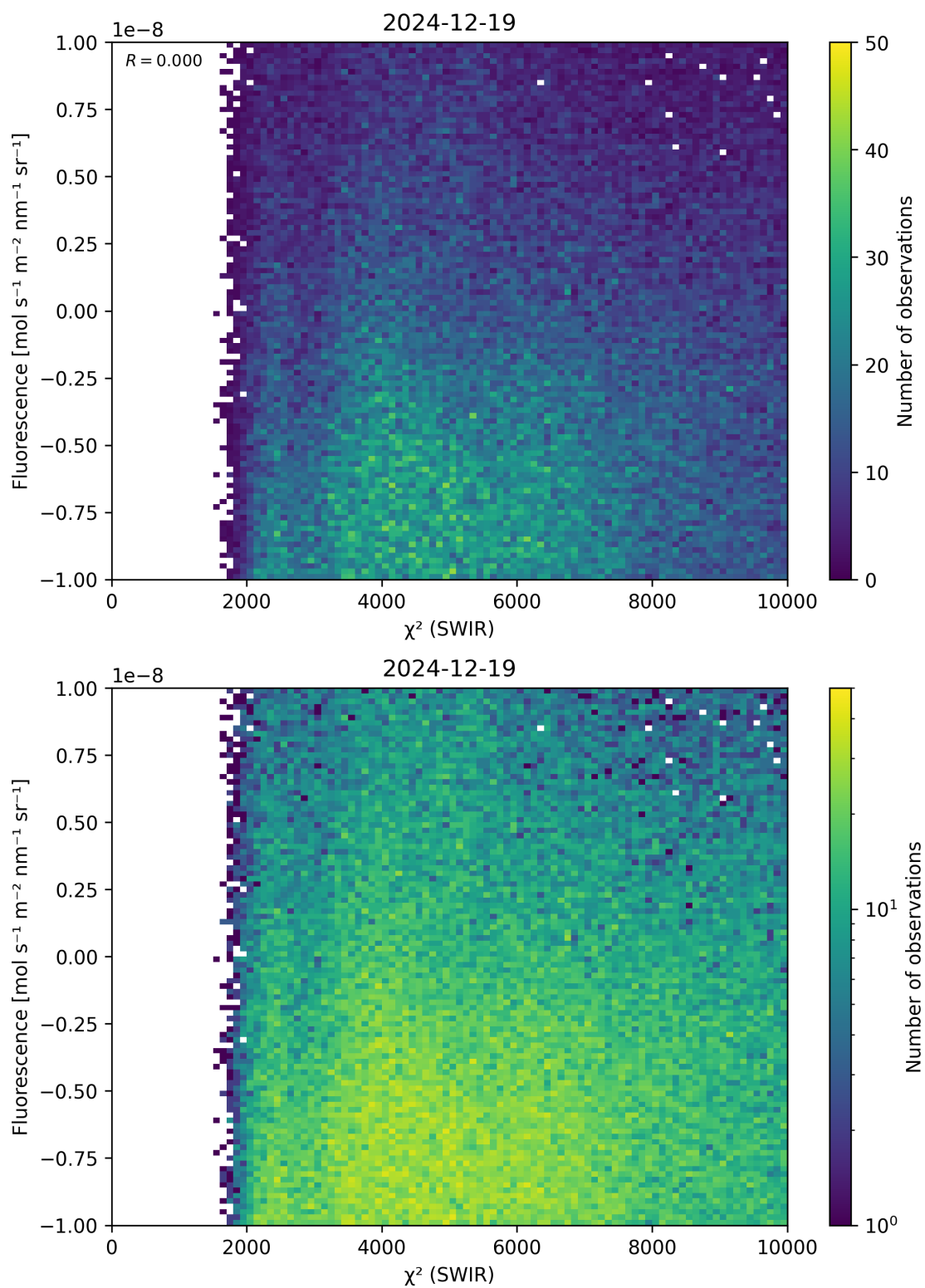
Figure 49: Scatter density plot of “ \chi^2 (SWIR)” against “Fluorescence” for 2024-12-18 to 2024-12-20.
