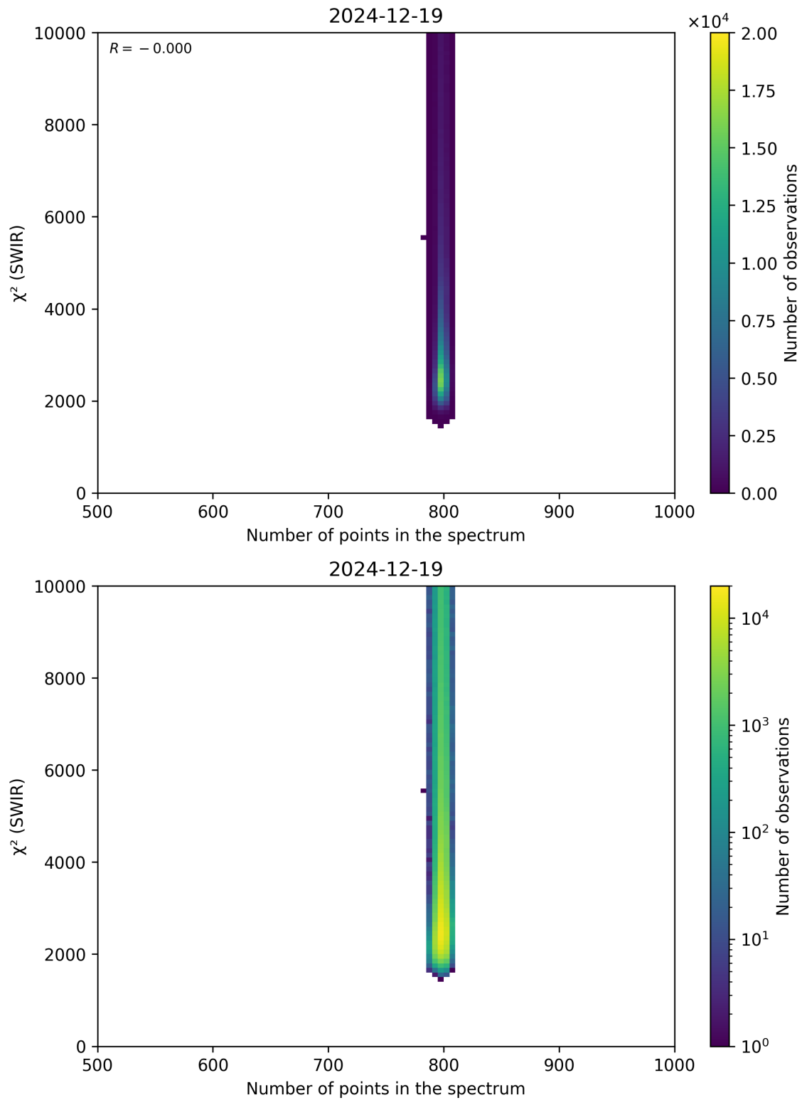
Figure 89: Scatter density plot of “Number of points in the spectrum” against “ \chi^2 (SWIR)” for 2024-12-18 to 2024-12-20.
