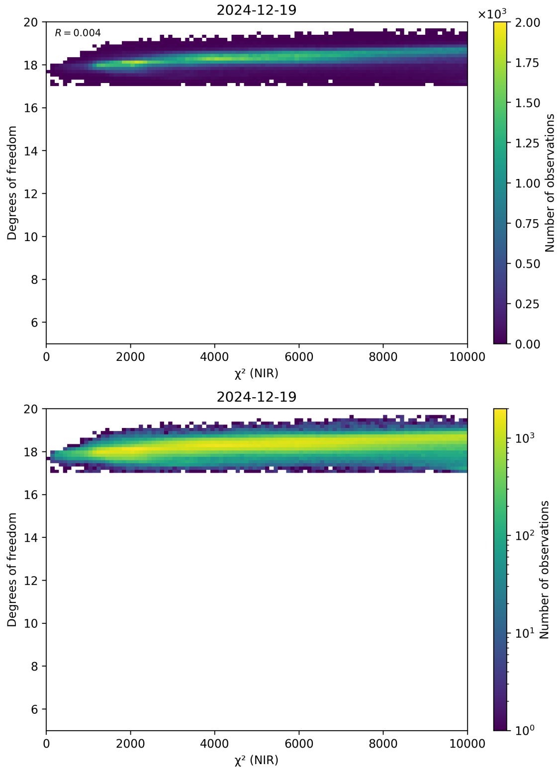
Figure 44: Scatter density plot of “ \chi^2 (NIR)” against “Degrees of freedom” for 2024-12-18 to 2024-12-20.
