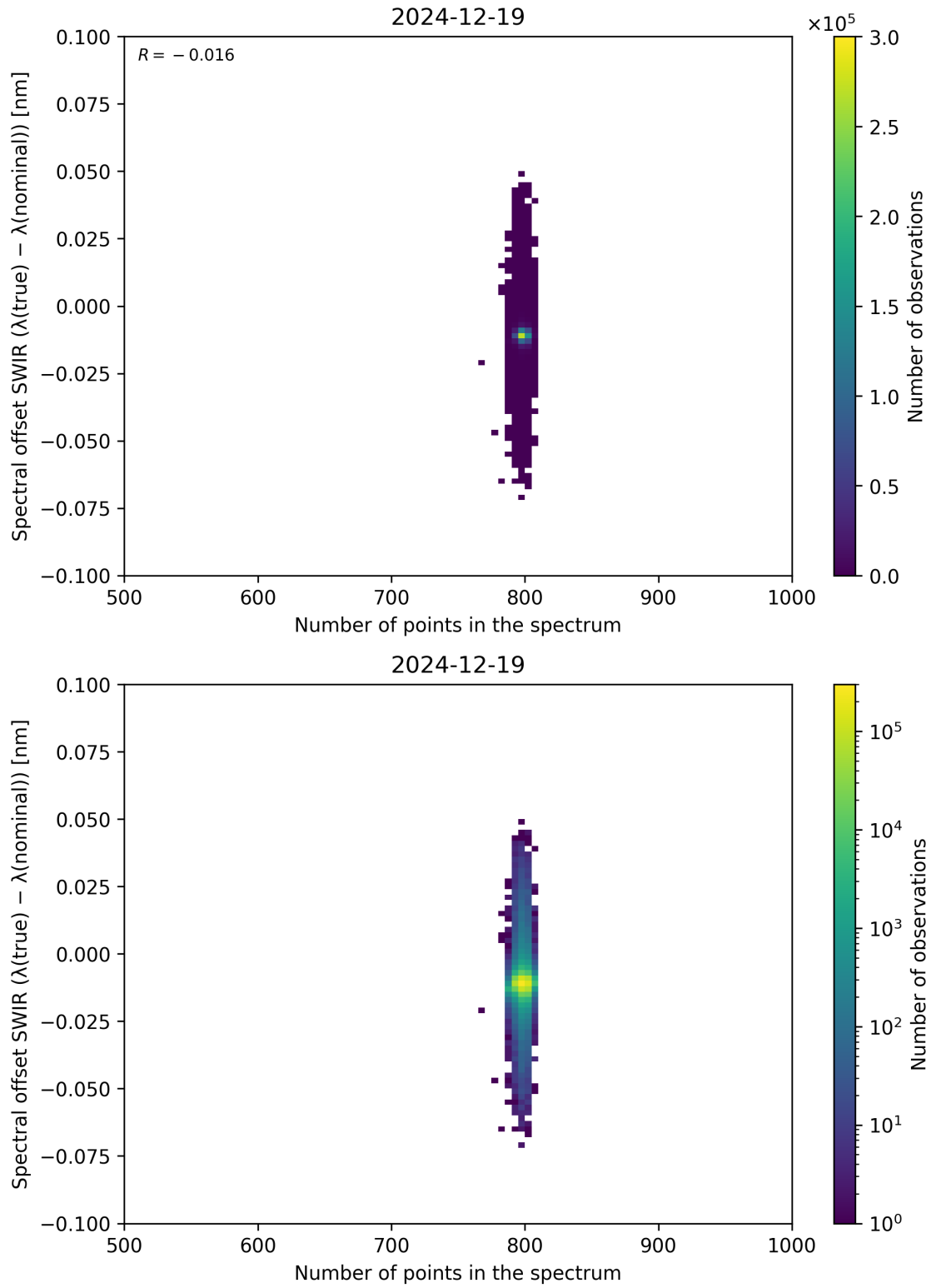
Figure 93: Scatter density plot of “Number of points in the spectrum” against “Spectral offset SWIR ( \lambda_{\text{true}} - \lambda_{\text{nominal}} )” for 2024-12-18 to 2024-12-20.
