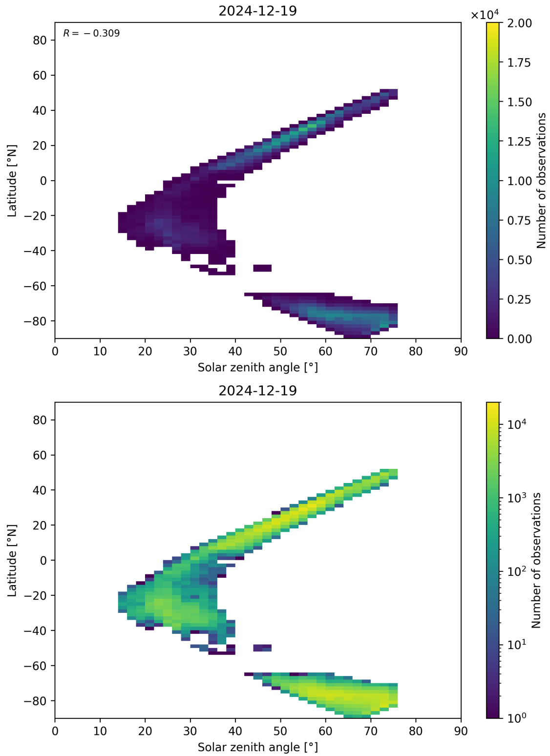
Figure 98: Scatter density plot of “Solar zenith angle” against “Latitude” for 2024-12-18 to 2024-12-20.
