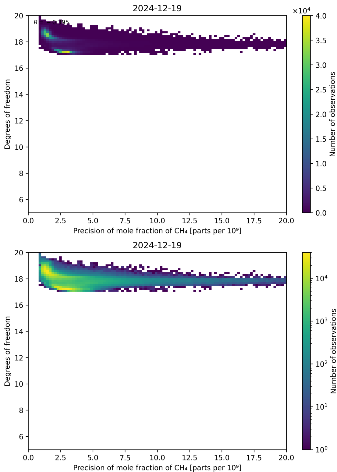
Figure 80: Scatter density plot of “Precision of mole fraction of CH 4 ” against “Degrees of freedom” for 2024-12-18 to 2024-12-20.
