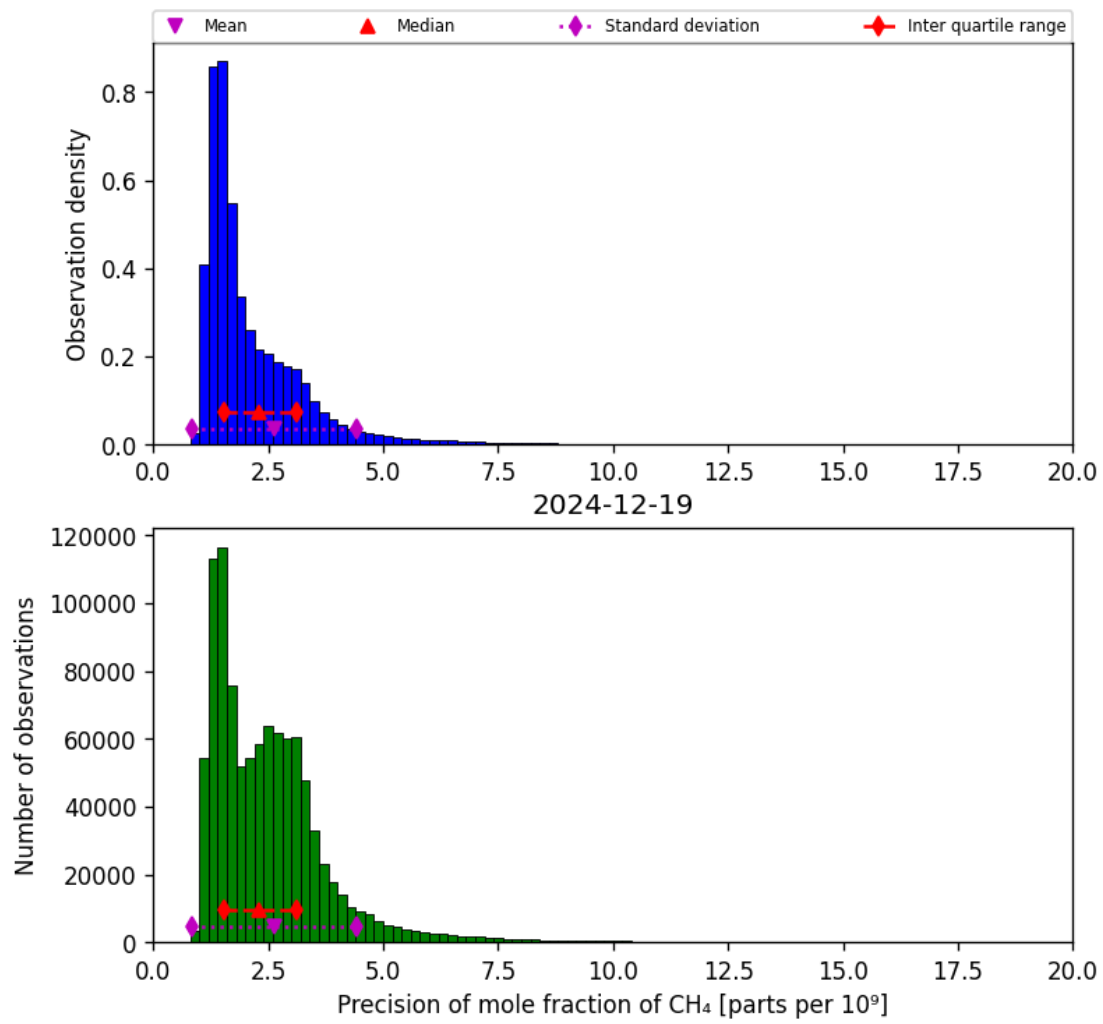
Figure 24: Histogram of “Precision of mole fraction of CH 4 ” for 2024-12-18 to 2024-12-20
