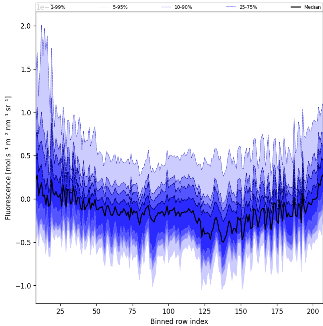
Figure 43: Along track statistics of “Fluorescence” for 2024-12-18 to 2024-12-20
