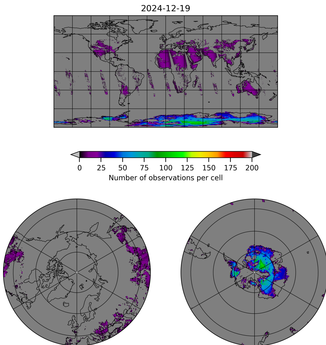
Figure 10: Map of the number of observations for 2024-12-18 to 2024-12-20
