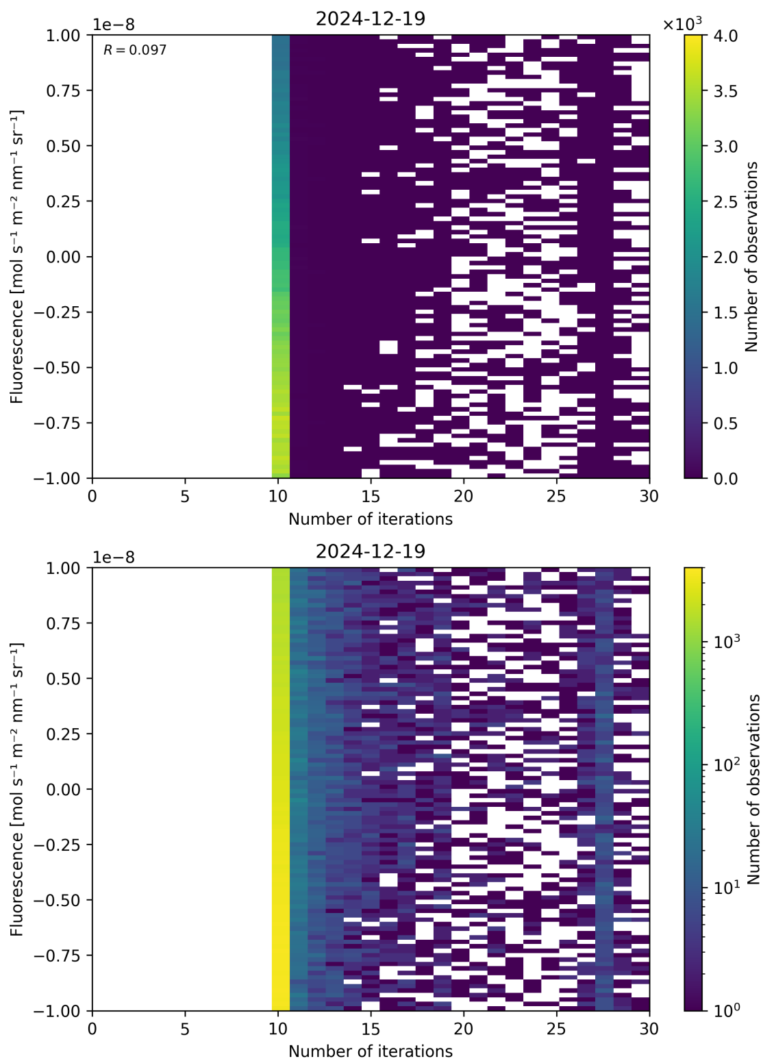
Figure 87: Scatter density plot of “Number of iterations” against “Fluorescence” for 2024-12-18 to 2024-12-20.
