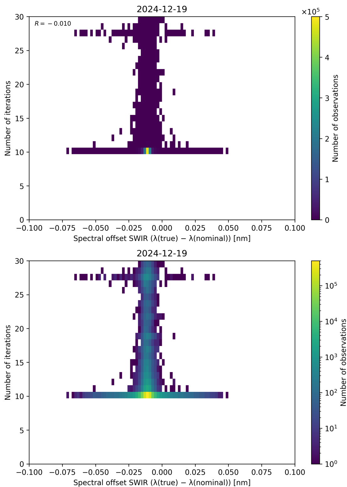
Figure 121: Scatter density plot of “Spectral offset SWIR ( \lambda_{\text{true}} - \lambda_{\text{nominal}} )” against “Number of iterations” for 2024-12-18 to 2024-12-20.
