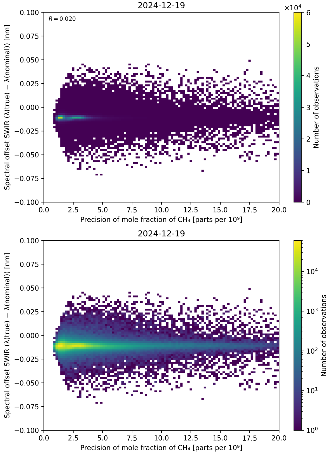
Figure 85: Scatter density plot of “Precision of mole fraction of CH 4 ” against “Spectral offset SWIR ( \lambda_{\text{true}} - \lambda_{\text{nominal}} )” for 2024-12-18 to 2024-12-20.
