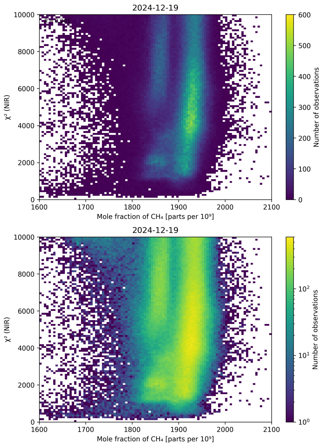
Figure 70: Scatter density plot of “Mole fraction of \text{CH}_4 ” against “ \chi^2 (NIR)” for 2024-12-18 to 2024-12-20.
