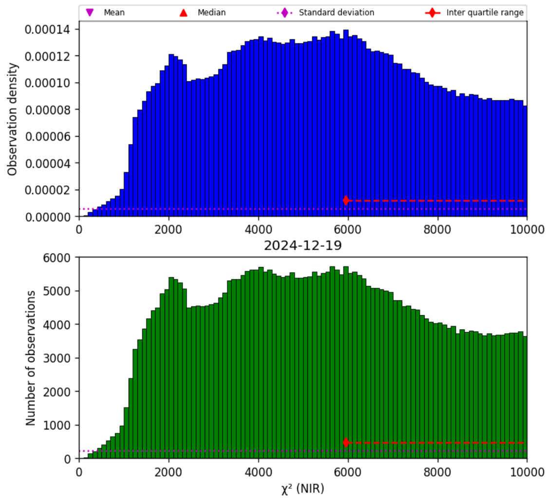
Figure 29: Histogram of " \chi^2 (NIR)" for 2024-12-18 to 2024-12-20
