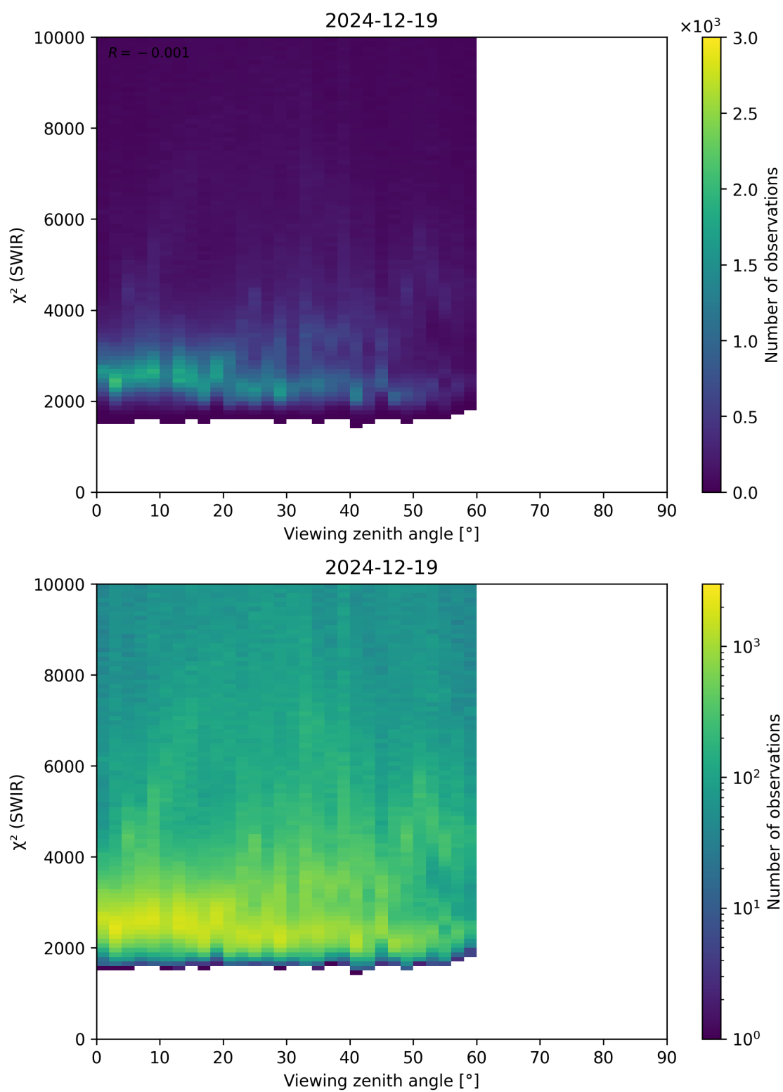
Figure 106: Scatter density plot of “Viewing zenith angle” against “ \chi^2 (SWIR)” for 2024-12-18 to 2024-12-20.
