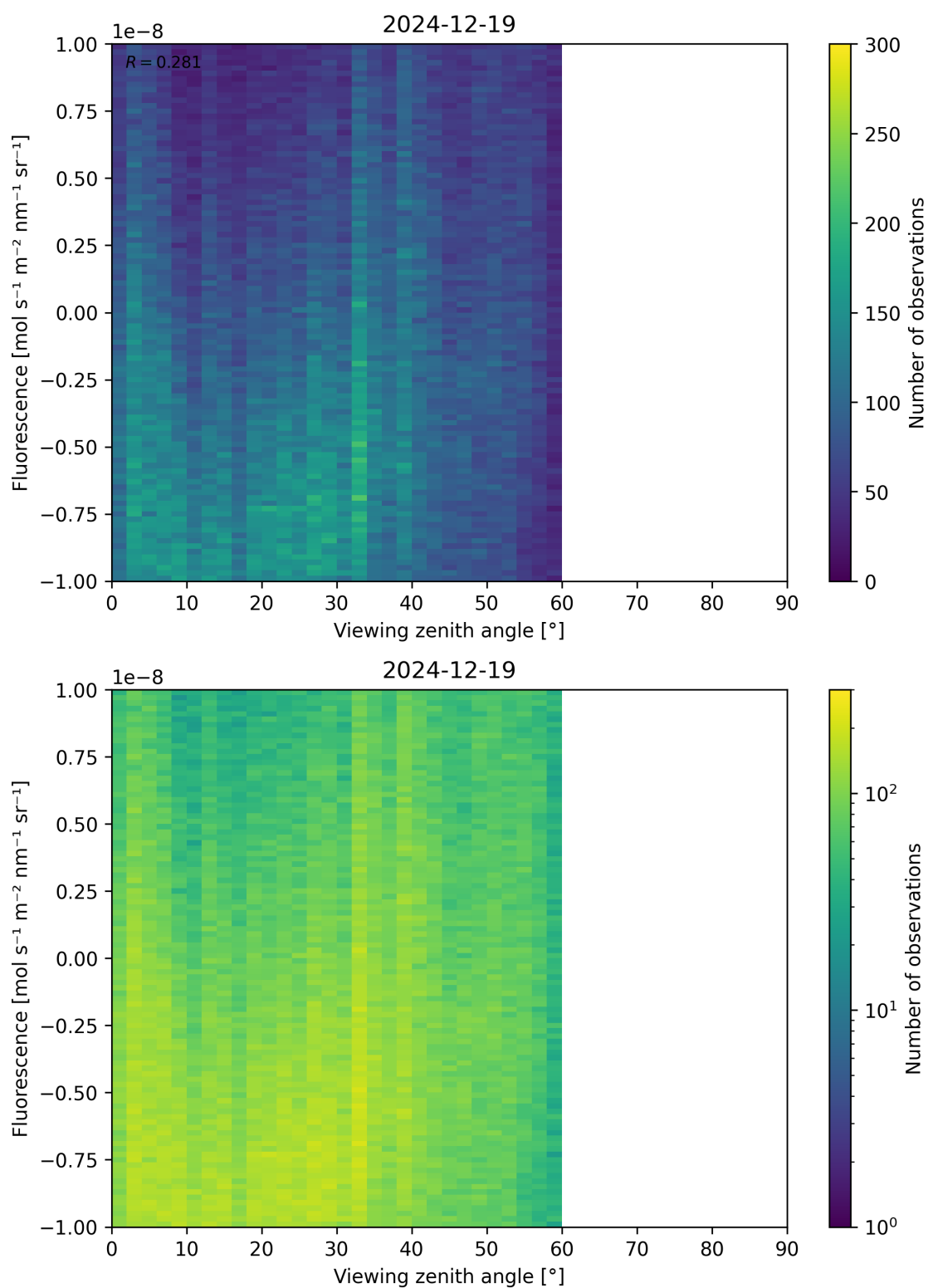
Figure 108: Scatter density plot of “Viewing zenith angle” against “Fluorescence” for 2024-12-18 to 2024-12-20.
