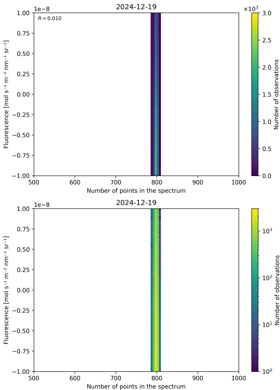
Figure 91: Scatter density plot of “Number of points in the spectrum” against “Fluorescence” for 2024-12-18 to 2024-12-20.
