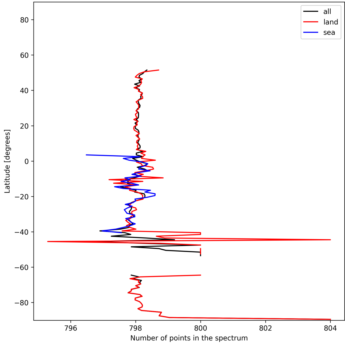
Figure 15: Zonal average of “Number of points in the spectrum” for 2024-12-18 to 2024-12-20.
