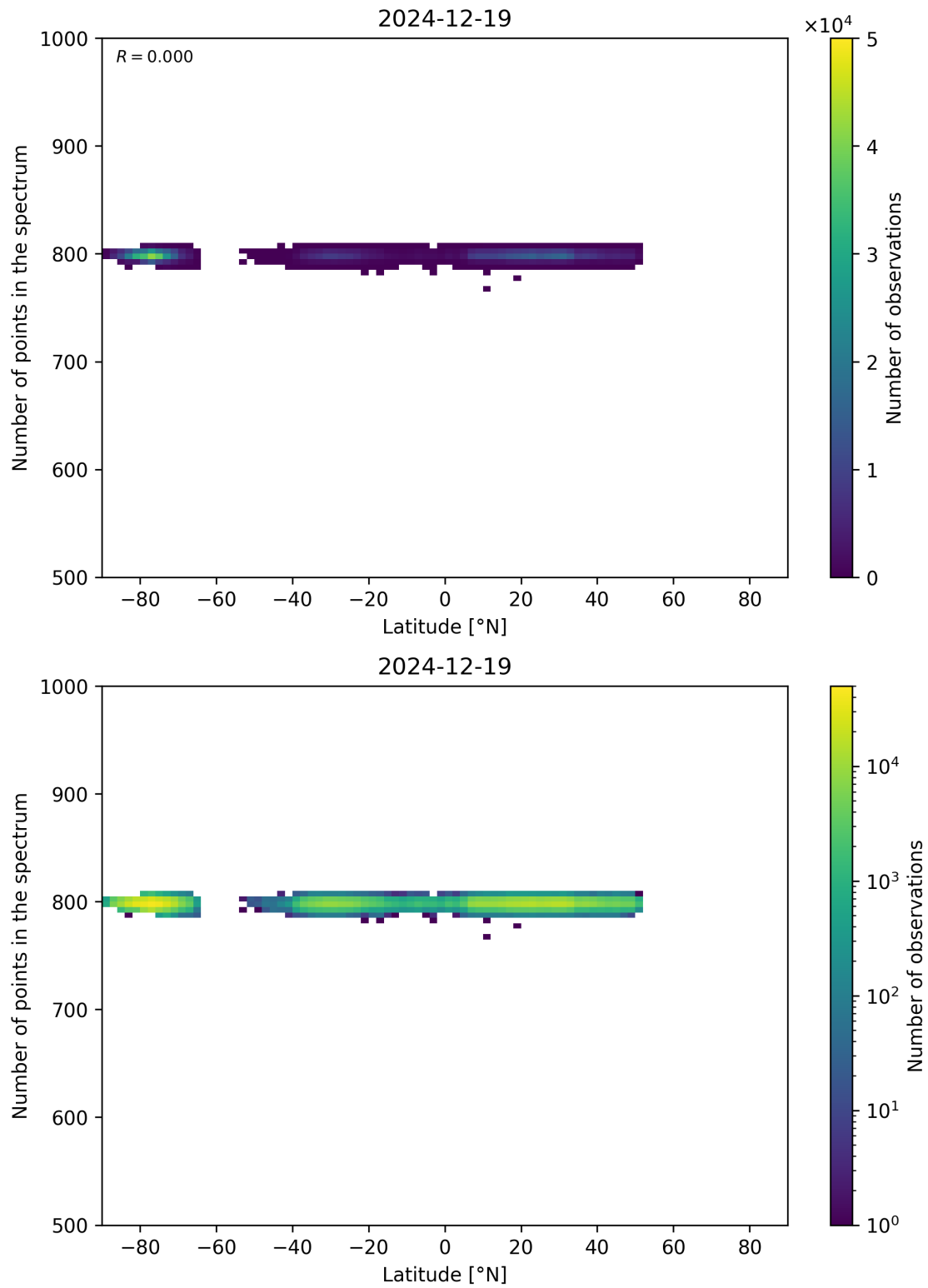
Figure 61: Scatter density plot of “Latitude” against “Number of points in the spectrum” for 2024-12-18 to 2024-12-20.
