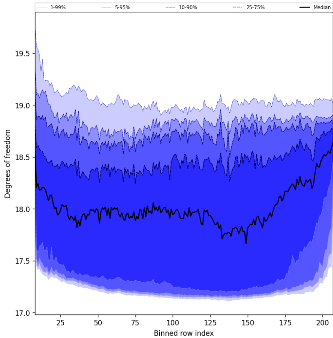
Figure 41: Along track statistics of “Degrees of freedom” for 2024-12-18 to 2024-12-20
