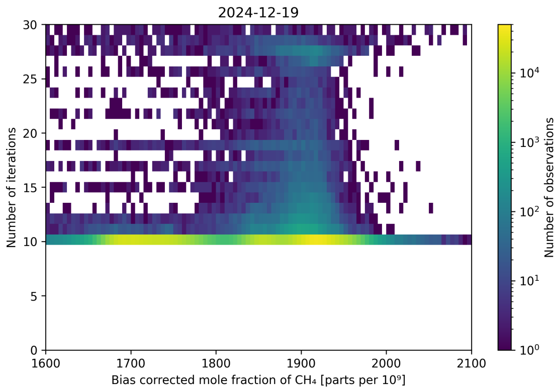
Figure 67: Scatter density plot of “Bias corrected mole fraction of CH 4 ” against “Number of iterations” for 2024-12-18 to 2024-12-20.
