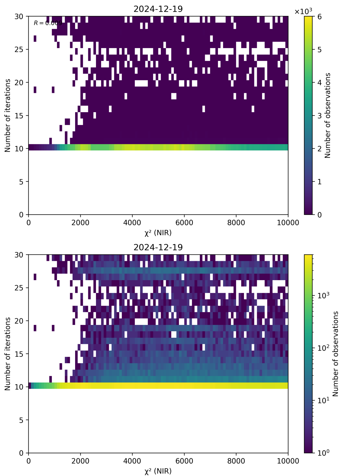
Figure 46: Scatter density plot of “ \chi^2 (NIR)” against “Number of iterations” for 2024-12-18 to 2024-12-20.
