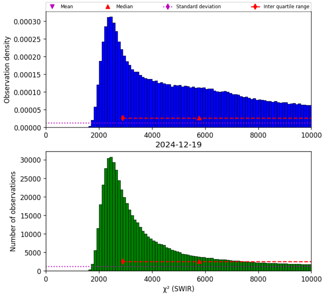
Figure 28: Histogram of “ \chi^2 (SWIR)” for 2024-12-18 to 2024-12-20
