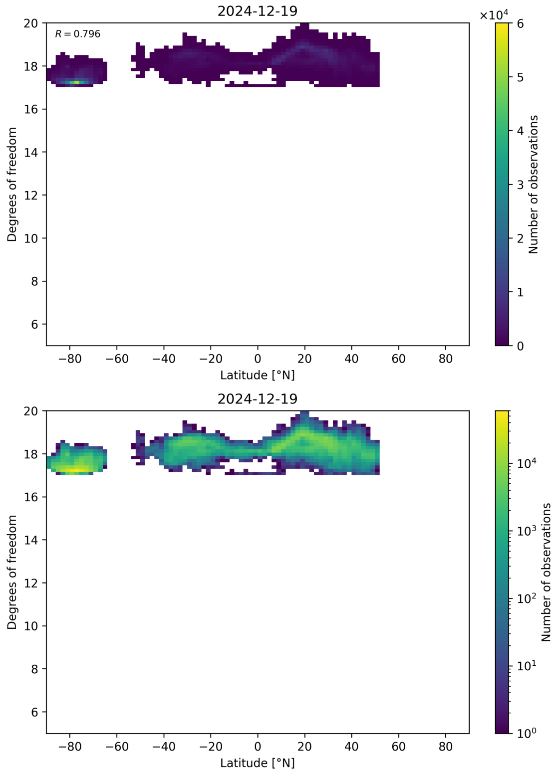
Figure 55: Scatter density plot of “Latitude” against “Degrees of freedom” for 2024-12-18 to 2024-12-20.
