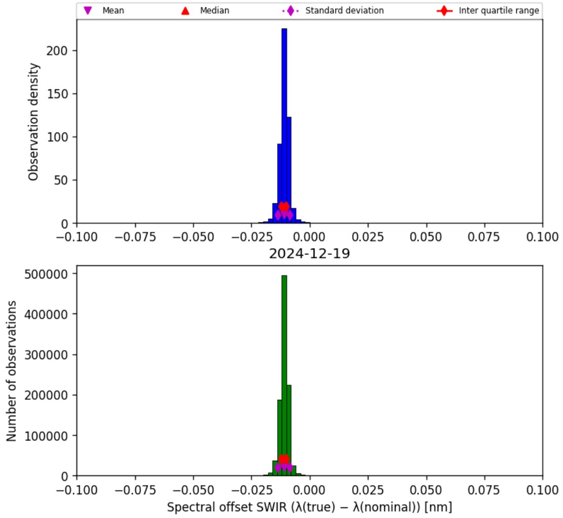
Figure 27: Histogram of “Spectral offset SWIR ( \lambda_{\text{true}} - \lambda_{\text{nominal}} )” for 2024-12-18 to 2024-12-20
