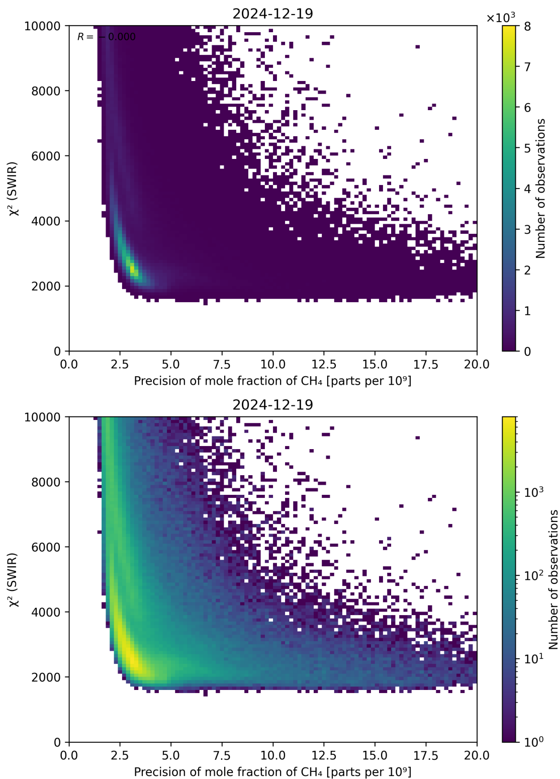
Figure 79: Scatter density plot of “Precision of mole fraction of CH 4 ” against “ \chi^2 (SWIR)” for 2024-12-18 to 2024-12-20.
