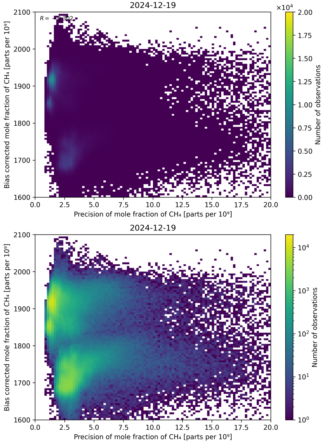
Figure 82: Scatter density plot of “Precision of mole fraction of CH 4 ” against “Bias corrected mole fraction of CH 4 ” for 2024-12-18 to 2024-12-20.
