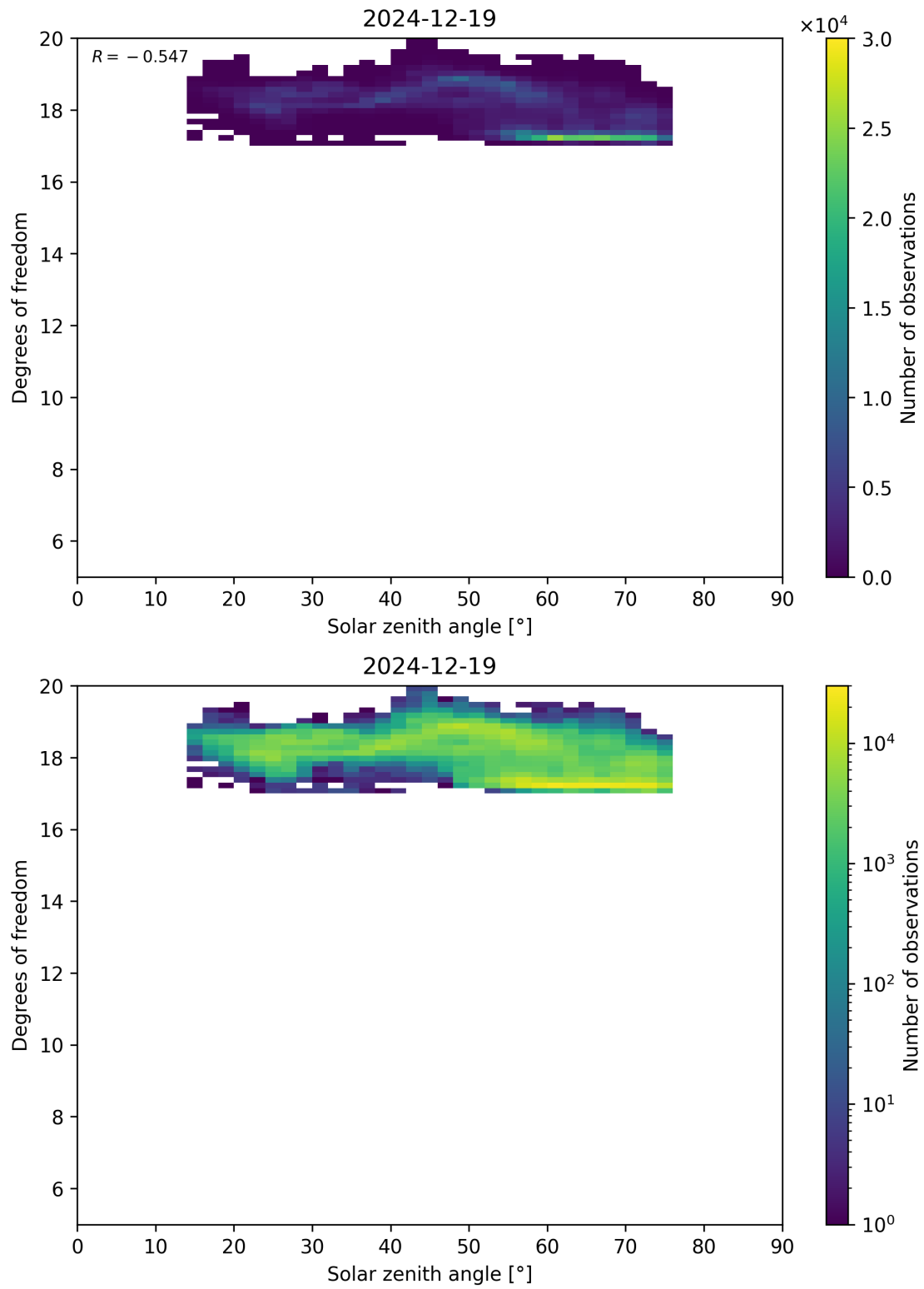
Figure 96: Scatter density plot of “Solar zenith angle” against “Degrees of freedom” for 2024-12-18 to 2024-12-20.
