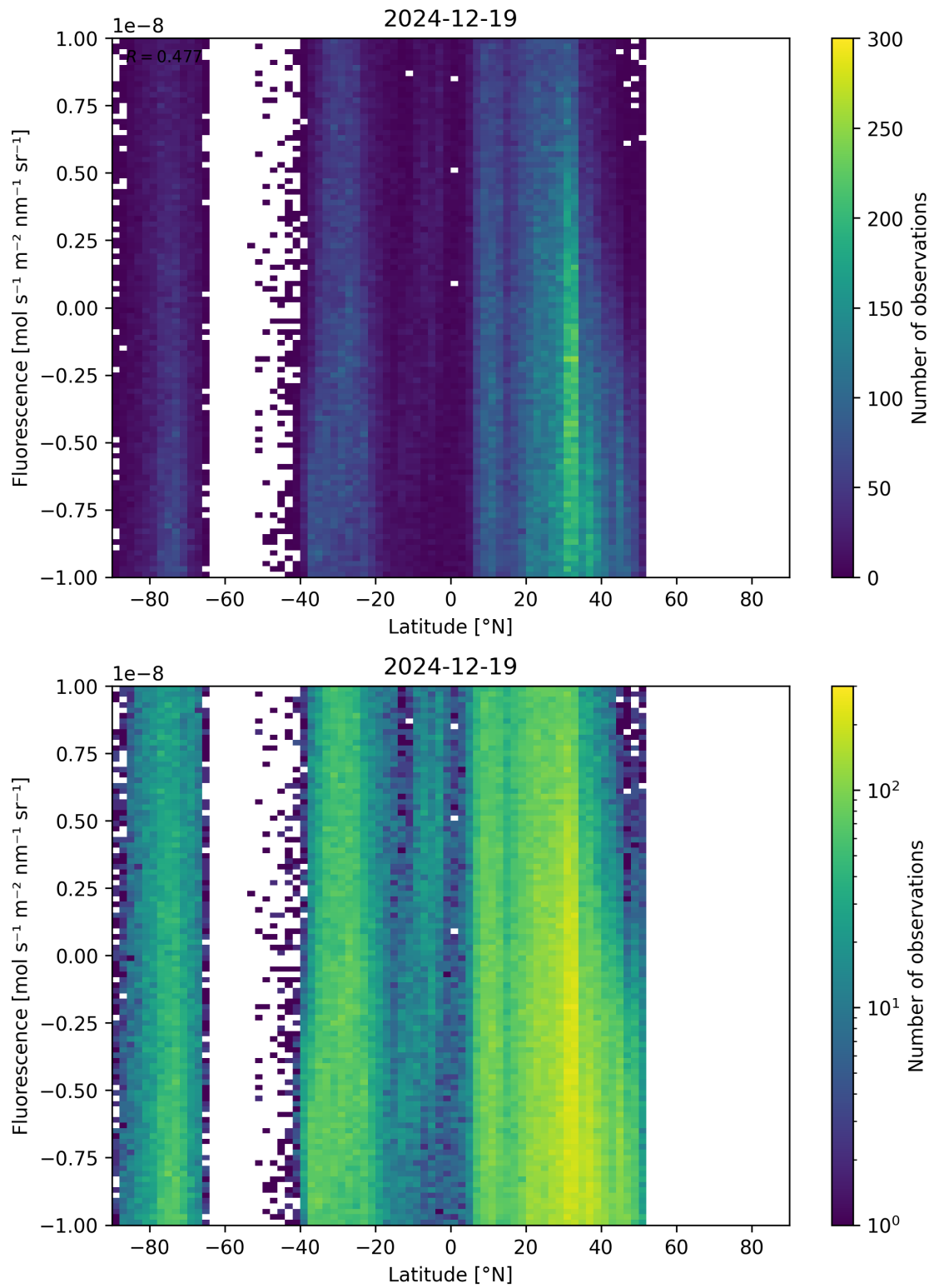
Figure 56: Scatter density plot of “Latitude” against “Fluorescence” for 2024-12-18 to 2024-12-20.
