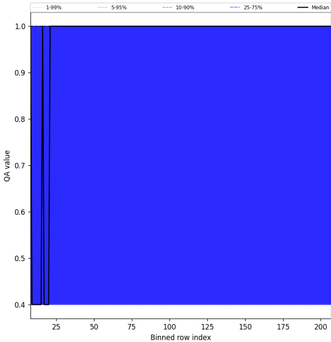
Figure 33: Along track statistics of “QA value” for 2024-12-18 to 2024-12-20
