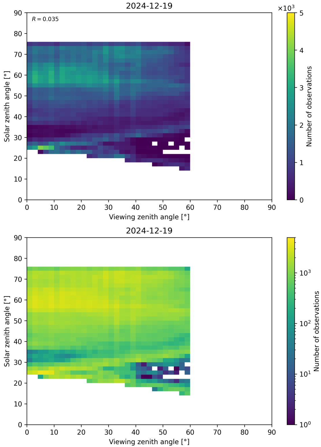
Figure 115: Scatter density plot of “Viewing zenith angle” against “Solar zenith angle” for 2024-12-18 to 2024-12-20.
