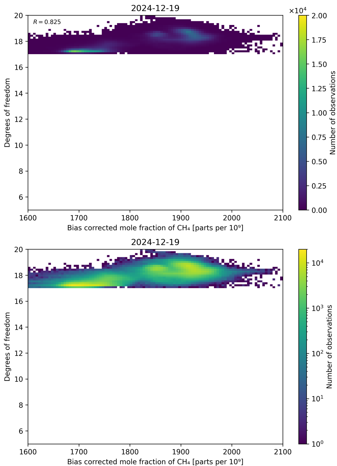
Figure 65: Scatter density plot of “Bias corrected mole fraction of CH 4 ” against “Degrees of freedom” for 2024-12-18 to 2024-12-20.
