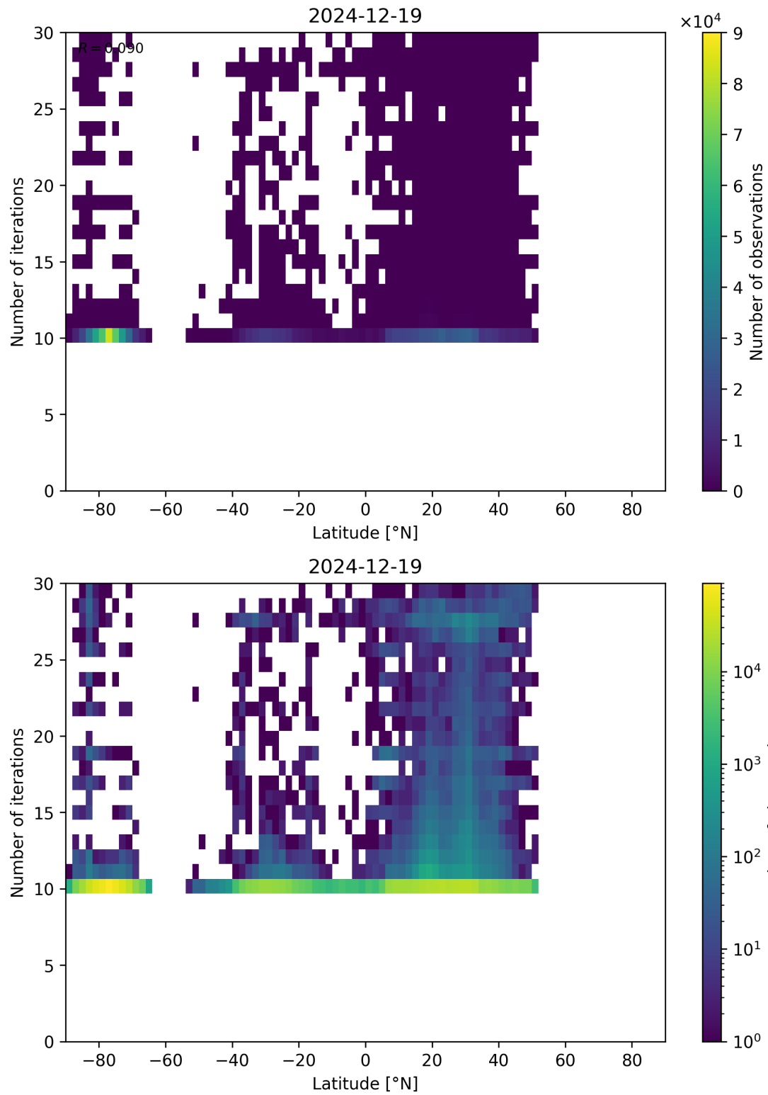
Figure 60: Scatter density plot of “Latitude” against “Number of iterations” for 2024-12-18 to 2024-12-20.
