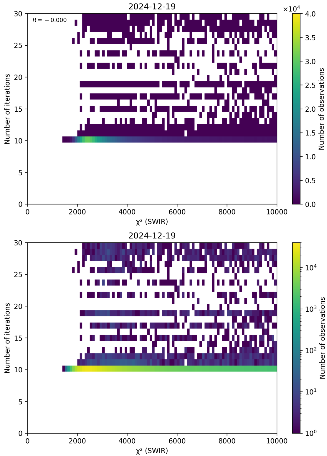
Figure 50: Scatter density plot of “ \chi^2 (SWIR)” against “Number of iterations” for 2024-12-18 to 2024-12-20.
