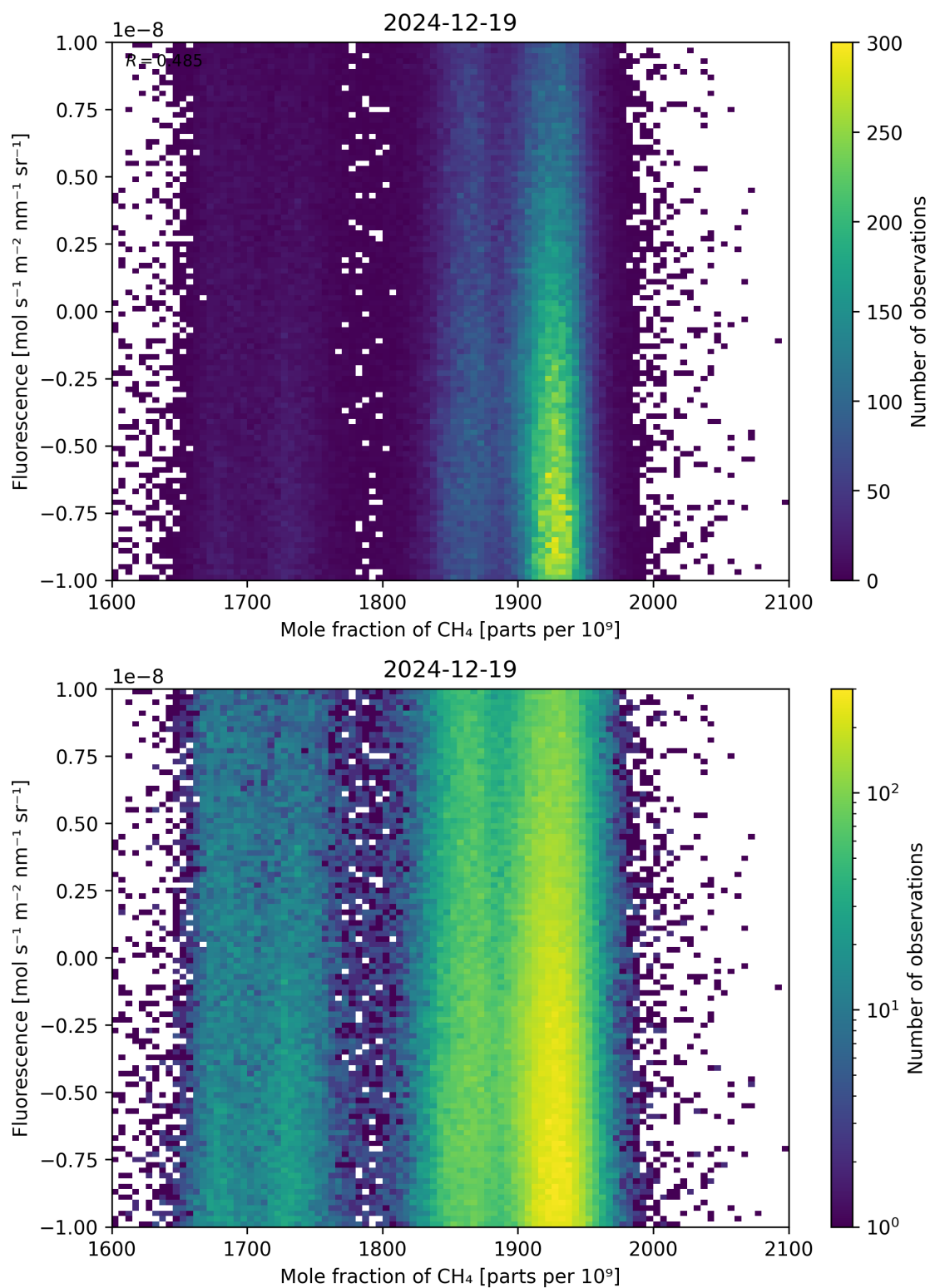
Figure 73: Scatter density plot of “Mole fraction of \text{CH}_4 ” against “Fluorescence” for 2024-12-18 to 2024-12-20.
