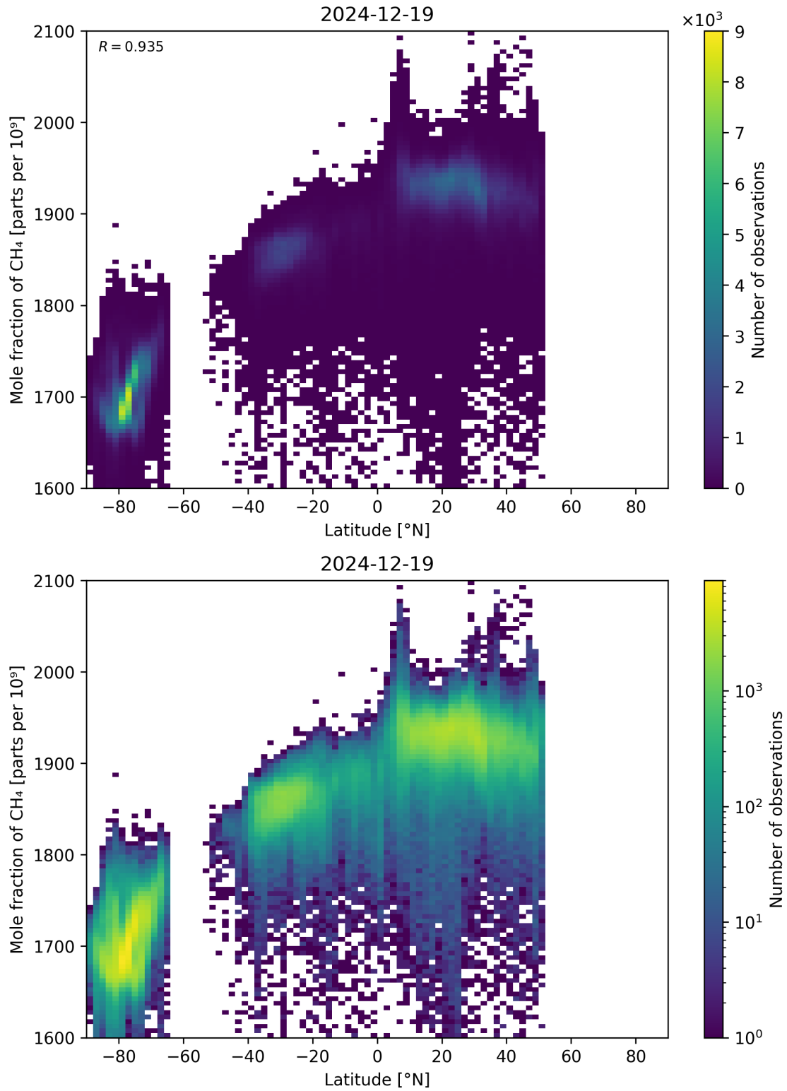
Figure 57: Scatter density plot of “Latitude” against “Mole fraction of \text{CH}_4 ” for 2024-12-18 to 2024-12-20.
