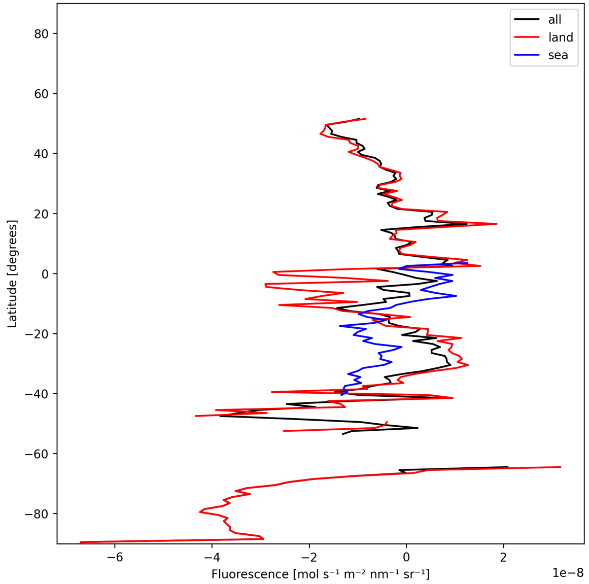
Figure 21: Zonal average of “Fluorescence” for 2024-12-18 to 2024-12-20.
