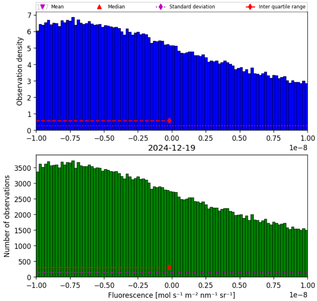
Figure 32: Histogram of “Fluorescence” for 2024-12-18 to 2024-12-20
