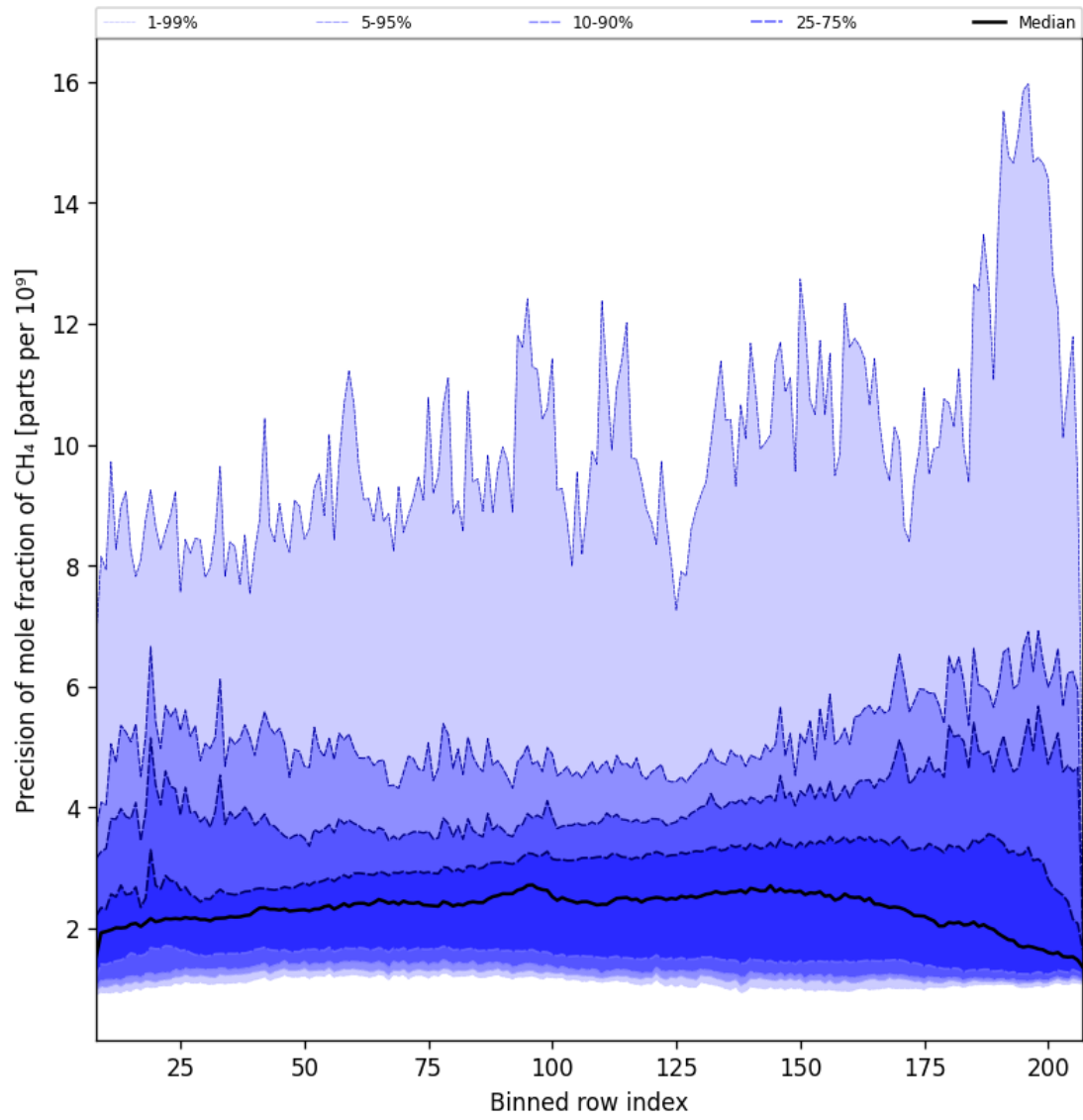
Figure 35: Along track statistics of “Precision of mole fraction of CH 4 ” for 2024-12-18 to 2024-12-20
