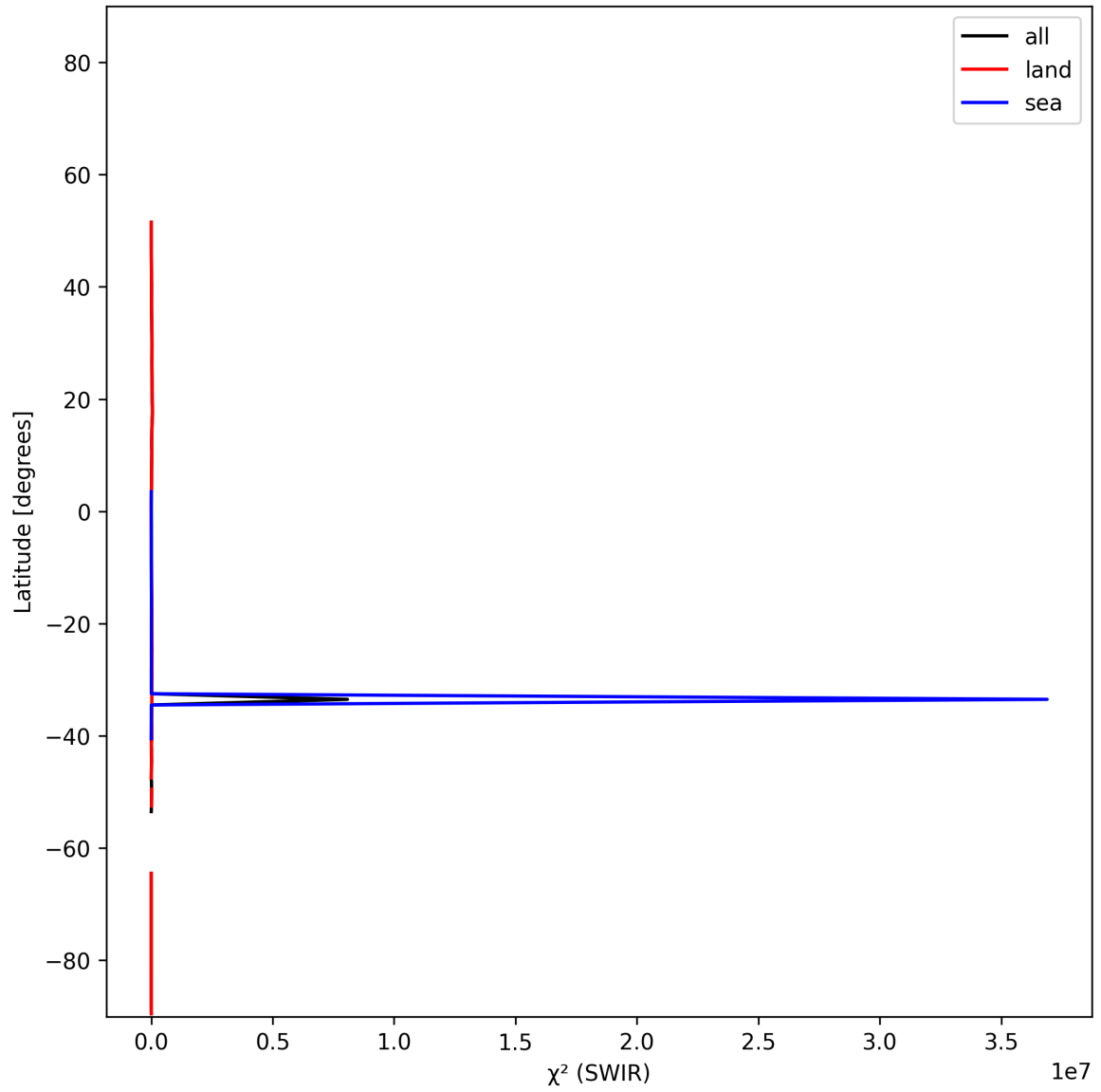
Figure 17: Zonal average of “ \chi^2 (SWIR)” for 2024-12-18 to 2024-12-20.
