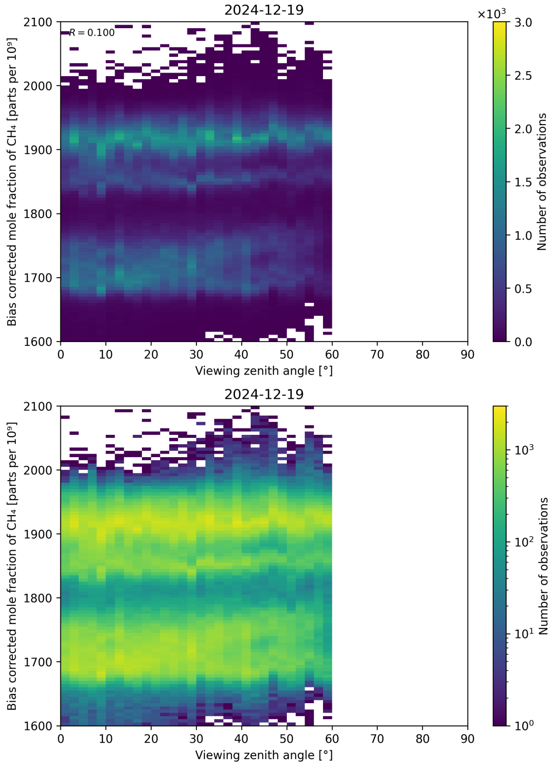
Figure 111: Scatter density plot of “Viewing zenith angle” against “Bias corrected mole fraction of CH 4 ” for 2024-12-18 to 2024-12-20.
