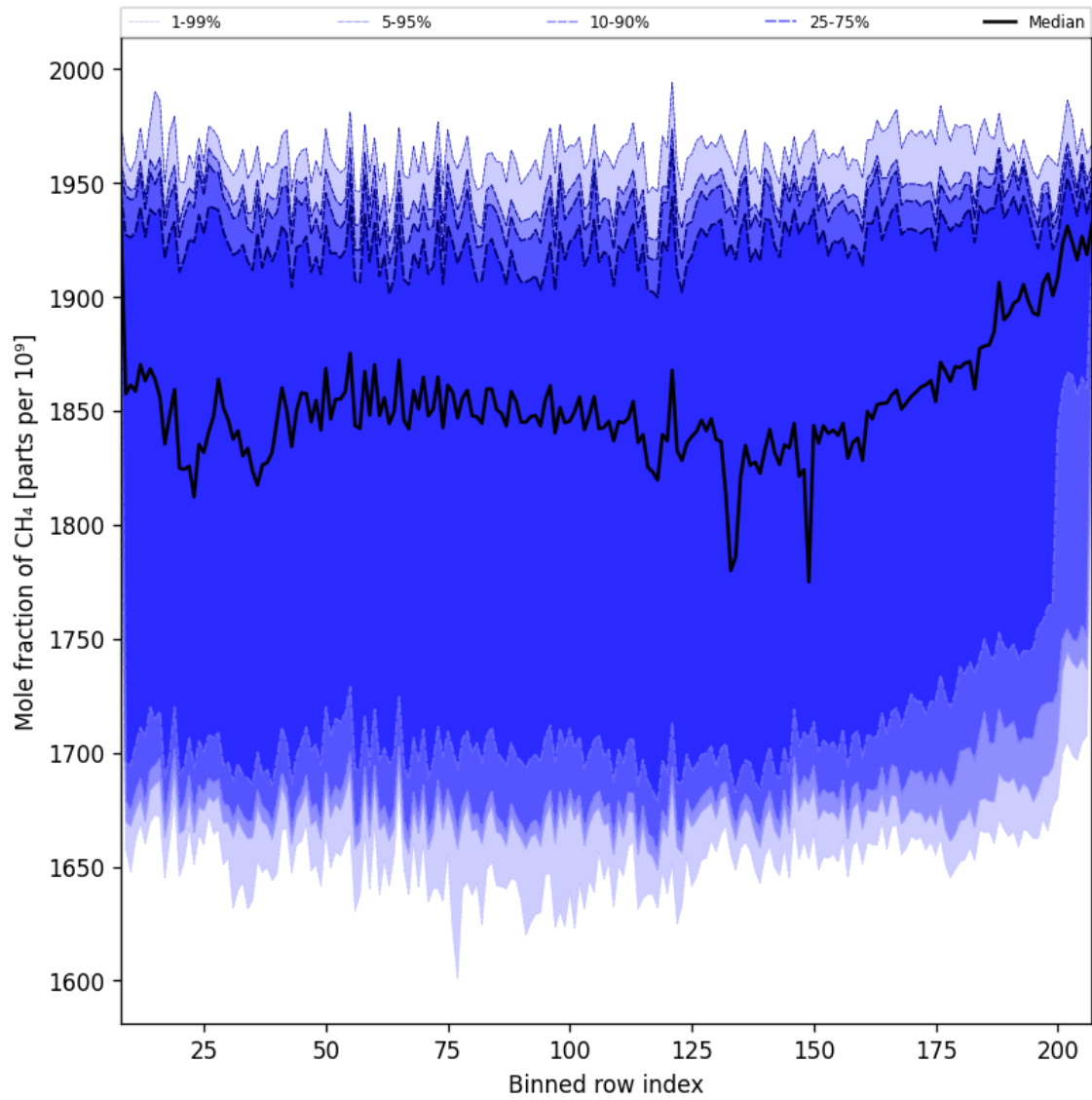
Figure 34: Along track statistics of “Mole fraction of CH 4 ” for 2024-12-18 to 2024-12-20
