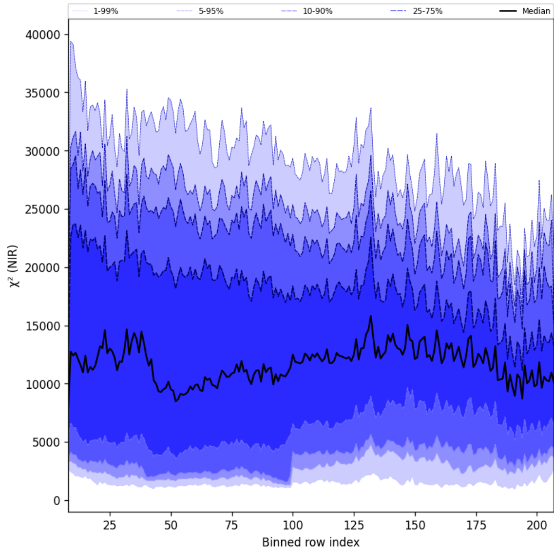
Figure 40: Along track statistics of “ \chi^2 (NIR)” for 2024-12-18 to 2024-12-20
