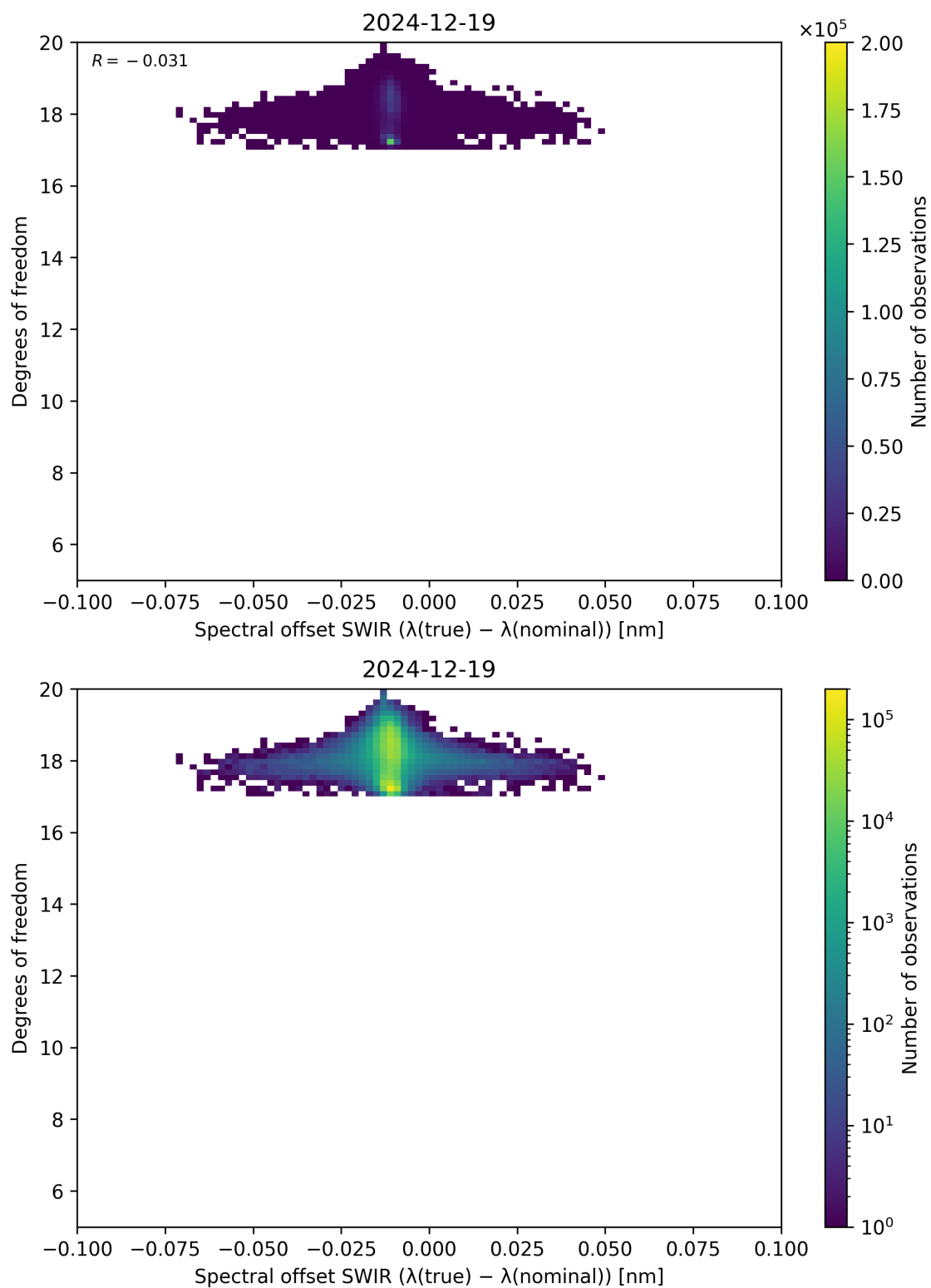
Figure 119: Scatter density plot of “Spectral offset SWIR ( \lambda_{\text{true}} - \lambda_{\text{nominal}} )” against “Degrees of freedom” for 2024-12-18 to 2024-12-20.
