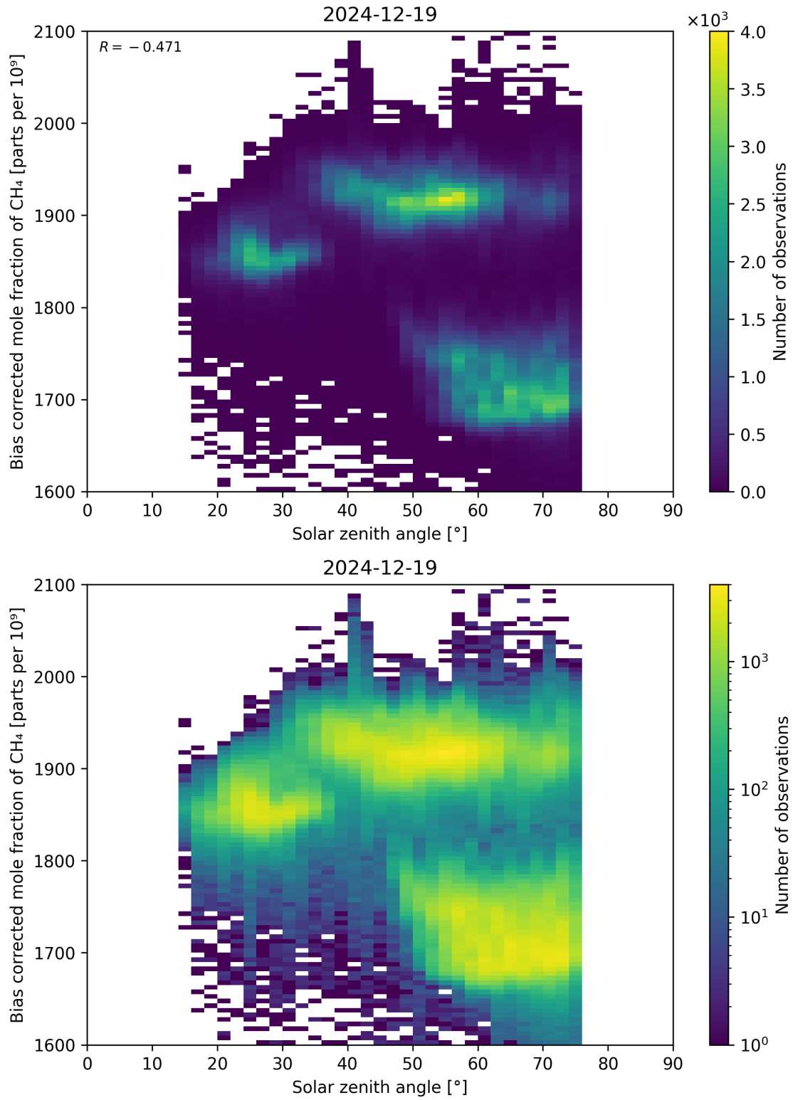
Figure 100: Scatter density plot of “Solar zenith angle” against “Bias corrected mole fraction of CH 4 ” for 2024-12-18 to 2024-12-20.
