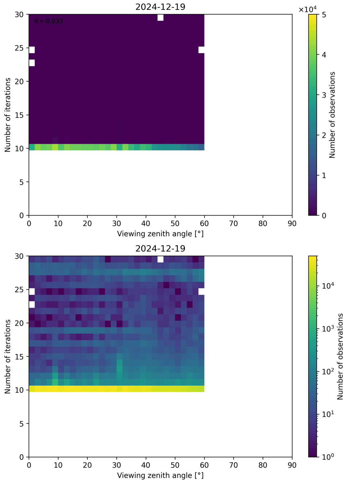
Figure 113: Scatter density plot of “Viewing zenith angle” against “Number of iterations” for 2024-12-18 to 2024-12-20.
