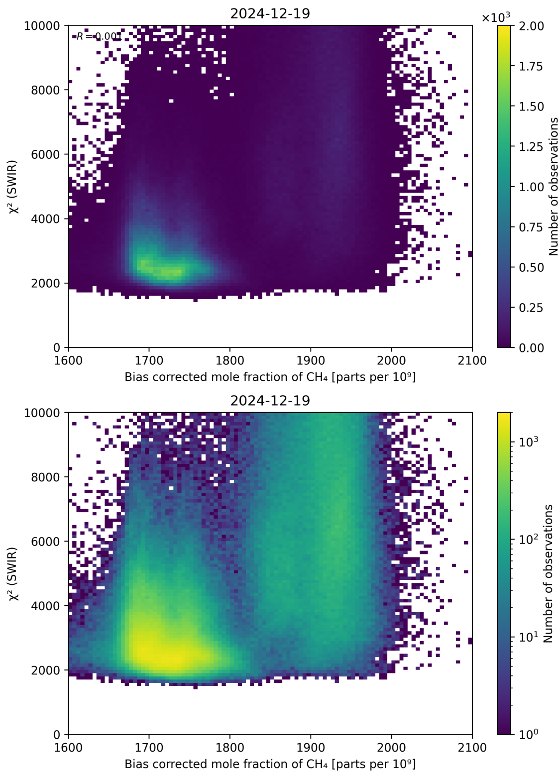
Figure 64: Scatter density plot of “Bias corrected mole fraction of \text{CH}_4 ” against “ \chi^2 (SWIR)” for 2024-12-18 to 2024-12-20.
