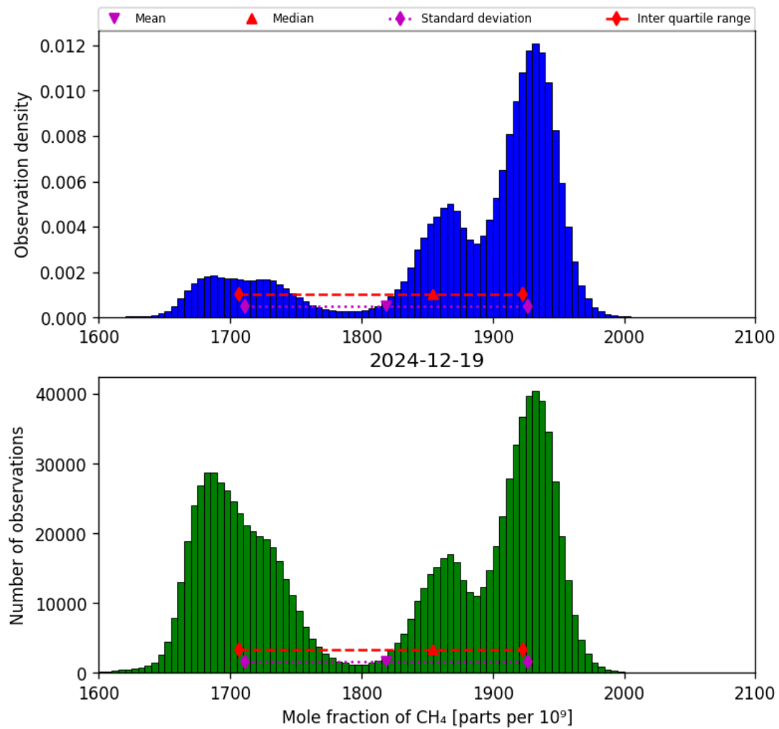
Figure 23: Histogram of “Mole fraction of CH 4 ” for 2024-12-18 to 2024-12-20
