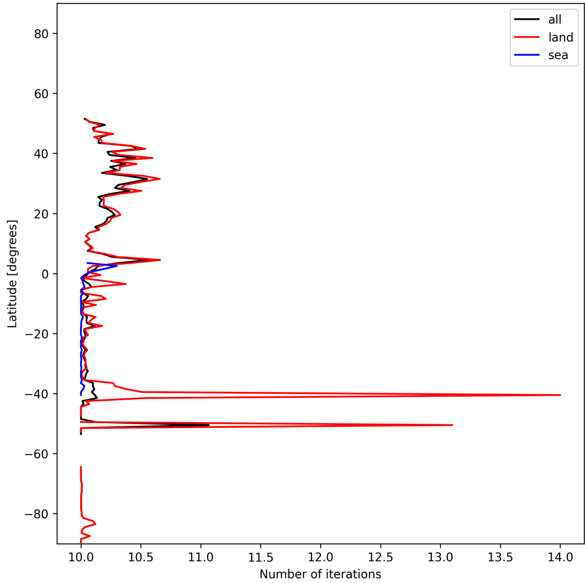
Figure 20: Zonal average of “Number of iterations” for 2024-12-18 to 2024-12-20.
