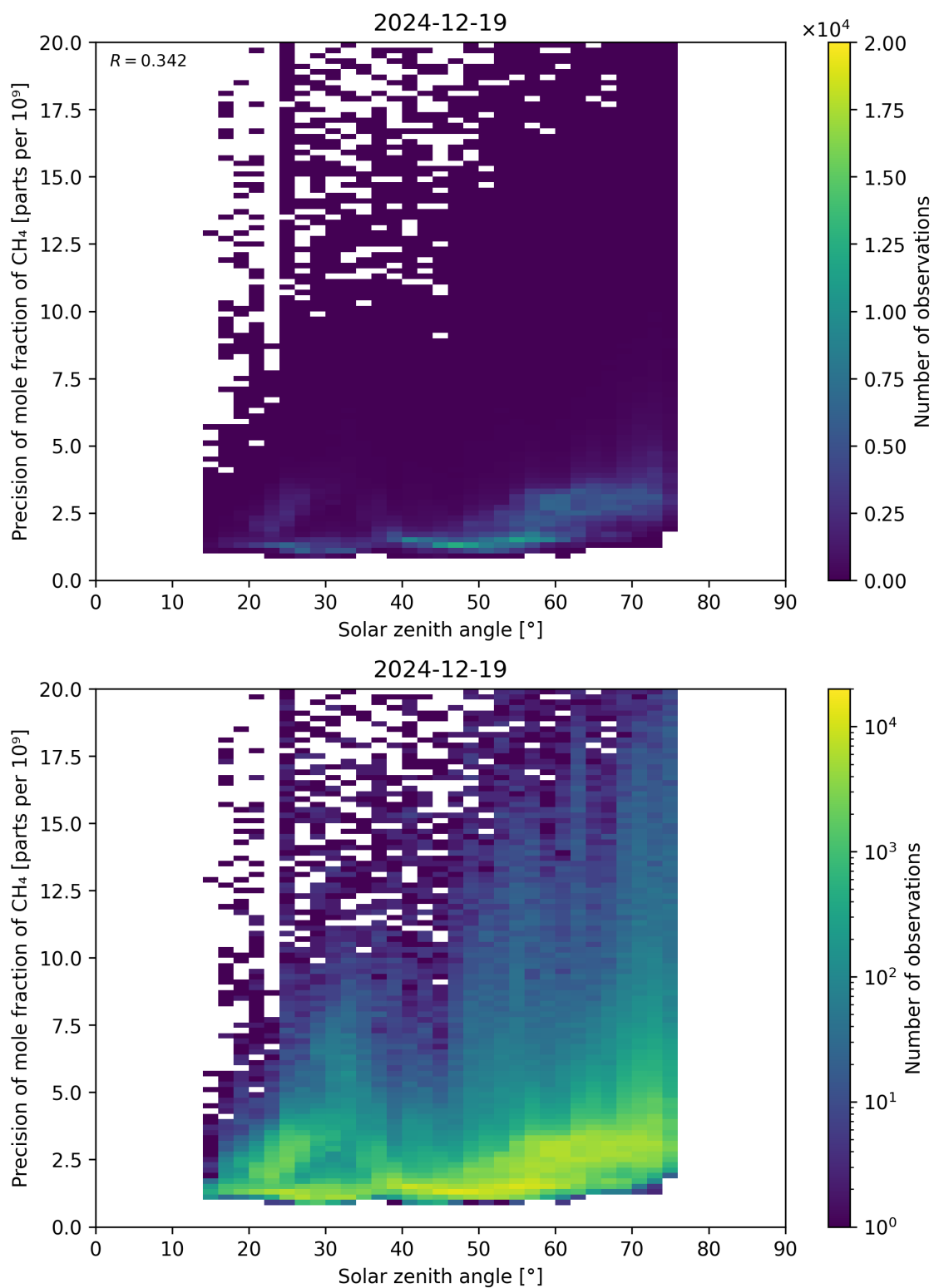
Figure 101: Scatter density plot of “Solar zenith angle” against “Precision of mole fraction of \text{CH}_4 ” for 2024-12-18 to 2024-12-20.
