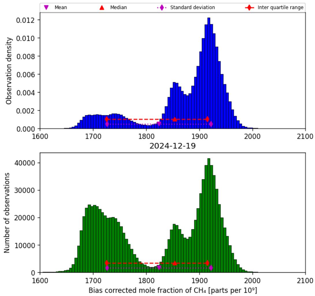
Figure 25: Histogram of “Bias corrected mole fraction of CH 4 ” for 2024-12-18 to 2024-12-20
