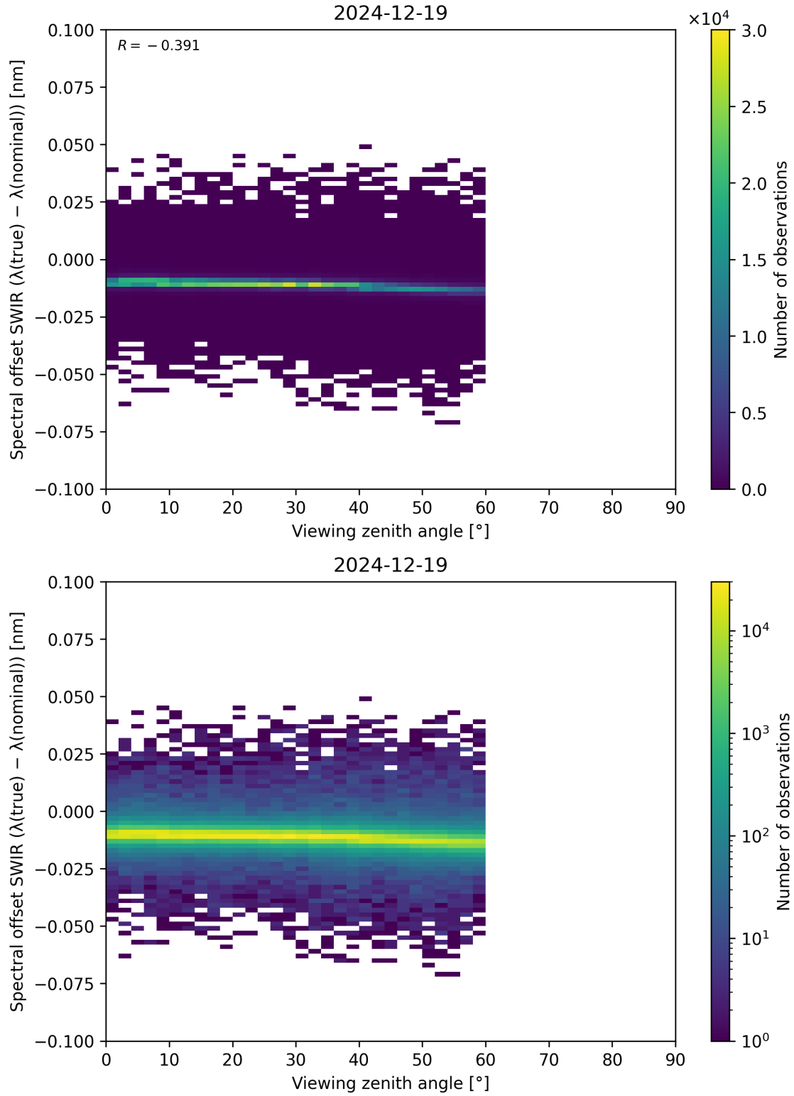
Figure 116: Scatter density plot of “Viewing zenith angle” against “Spectral offset SWIR ( \lambda_{\text{true}} - \lambda_{\text{nominal}} )” for 2024-12-18 to 2024-12-20.
