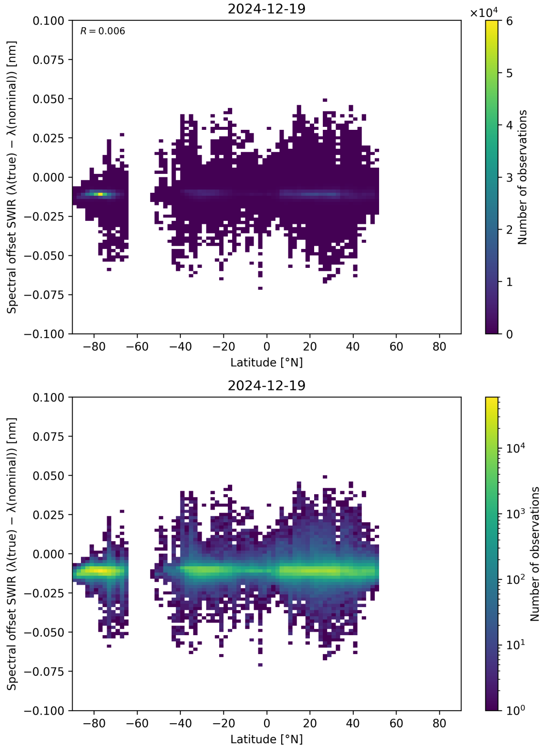
Figure 62: Scatter density plot of “Latitude” against “Spectral offset SWIR ( \lambda_{\text{true}} - \lambda_{\text{nominal}} )” for 2024-12-18 to 2024-12-20.
