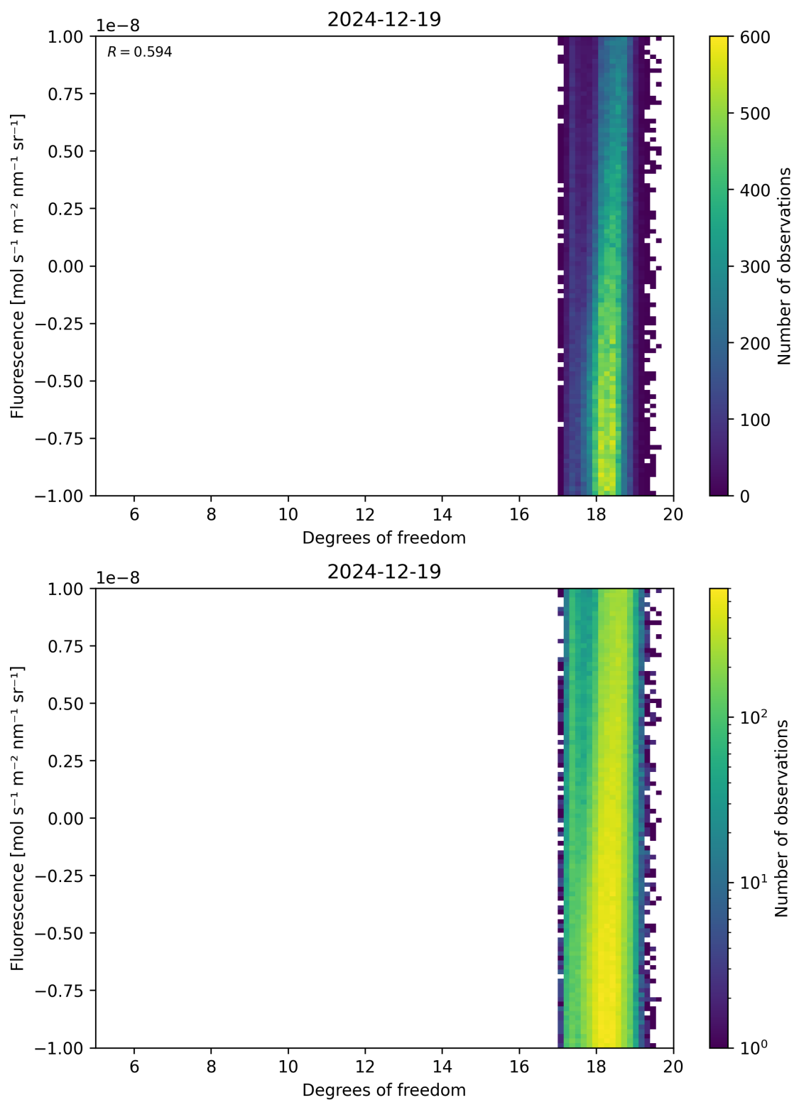
Figure 51: Scatter density plot of “Degrees of freedom” against “Fluorescence” for 2024-12-18 to 2024-12-20.
