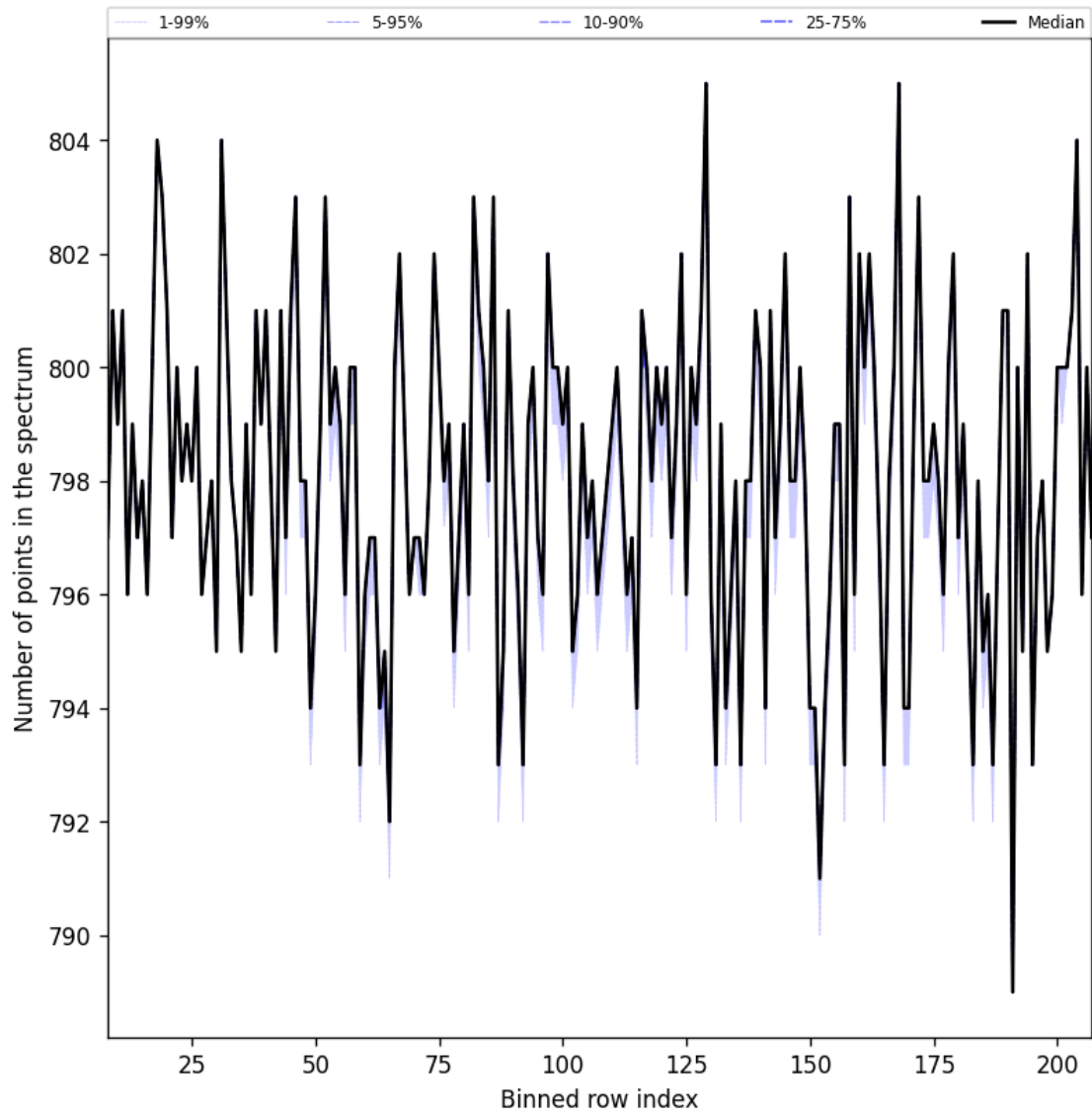
Figure 37: Along track statistics of “Number of points in the spectrum” for 2024-12-18 to 2024-12-20
