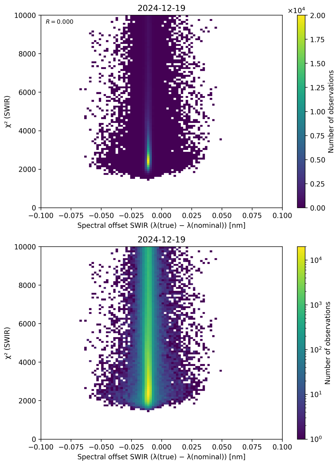
Figure 118: Scatter density plot of “Spectral offset SWIR ( \lambda_{\text{true}} - \lambda_{\text{nominal}} )” against “ \chi^2 (SWIR)” for 2024-12-18 to 2024-12-20.
