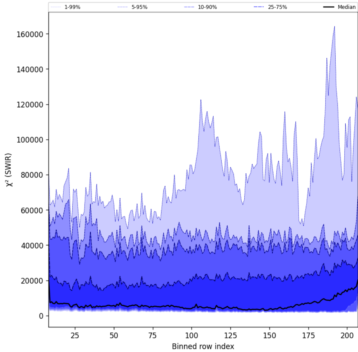
Figure 39: Along track statistics of “ \chi^2 (SWIR)” for 2024-12-18 to 2024-12-20
