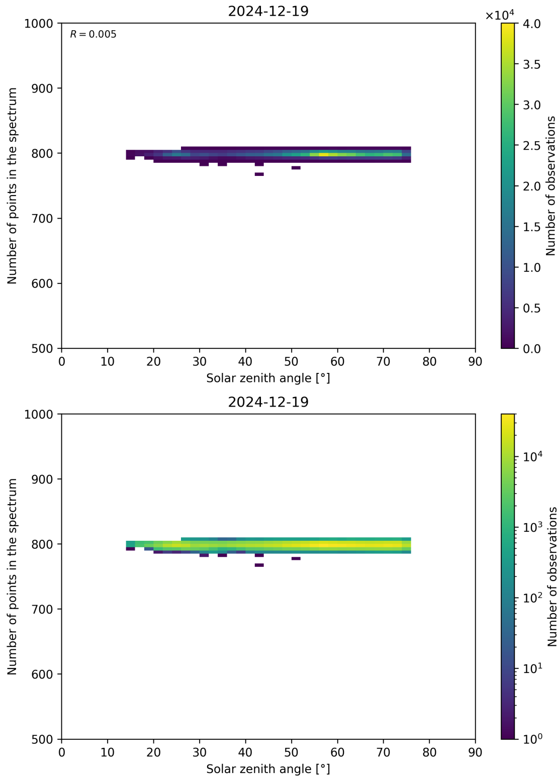
Figure 103: Scatter density plot of “Solar zenith angle” against “Number of points in the spectrum” for 2024-12-18 to 2024-12-20.
