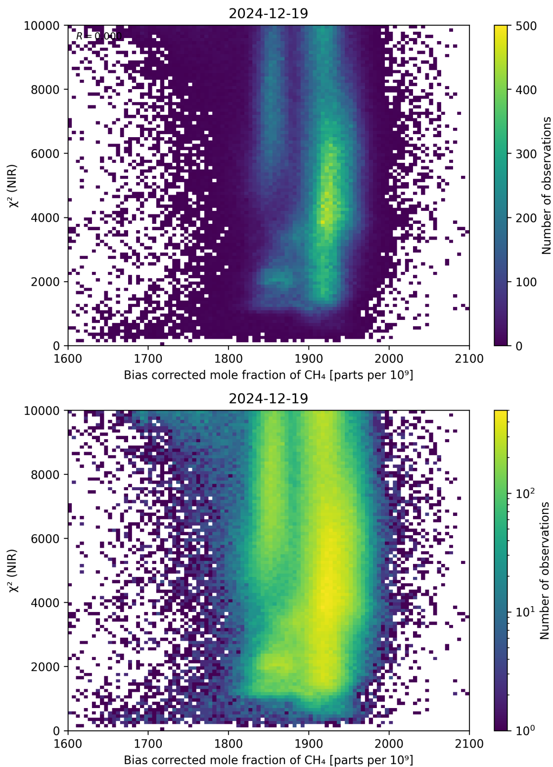
Figure 63: Scatter density plot of “Bias corrected mole fraction of CH 4 ” against “ \chi^2 (NIR)” for 2024-12-18 to 2024-12-20.
