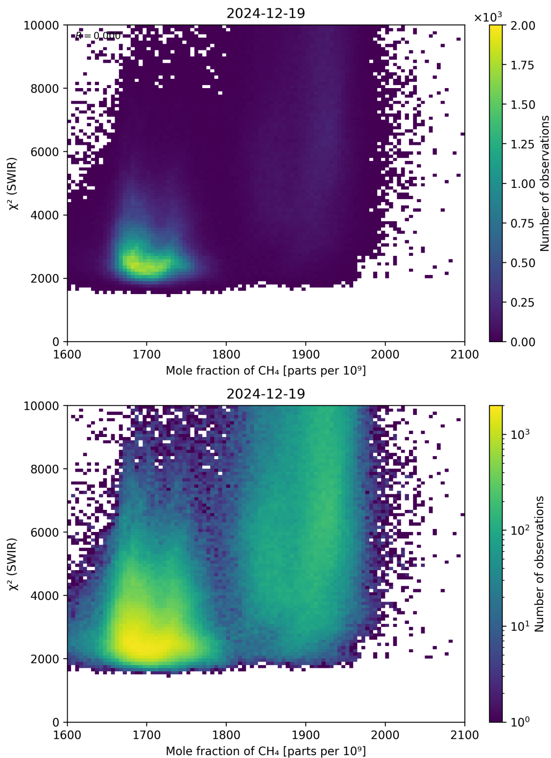
Figure 71: Scatter density plot of “Mole fraction of CH 4 ” against “ \chi^2 (SWIR)” for 2024-12-18 to 2024-12-20.
