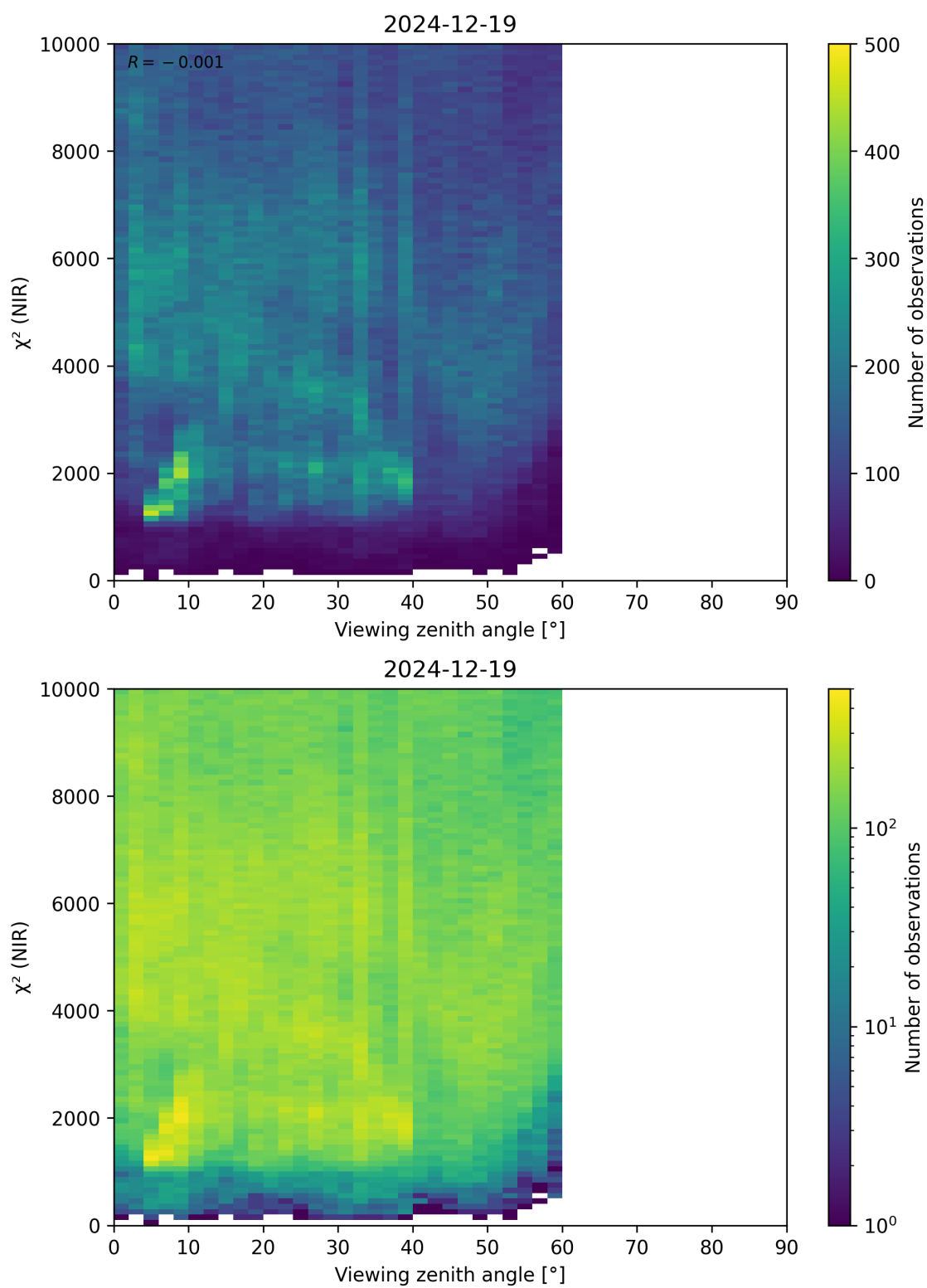
Figure 105: Scatter density plot of “Viewing zenith angle” against “ \chi^2 (NIR)” for 2024-12-18 to 2024-12-20.
