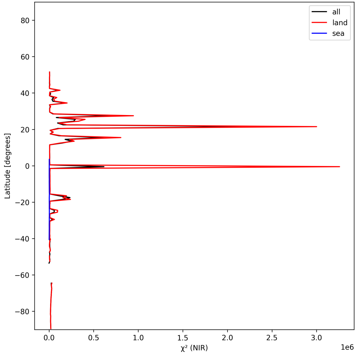
Figure 18: Zonal average of “ \chi^2 (NIR)” for 2024-12-18 to 2024-12-20.
