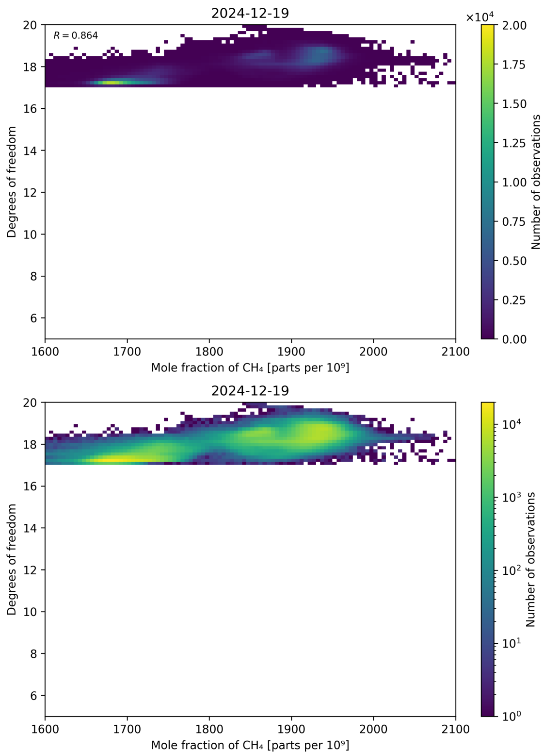
Figure 72: Scatter density plot of “Mole fraction of CH 4 ” against “Degrees of freedom” for 2024-12-18 to 2024-12-20.
