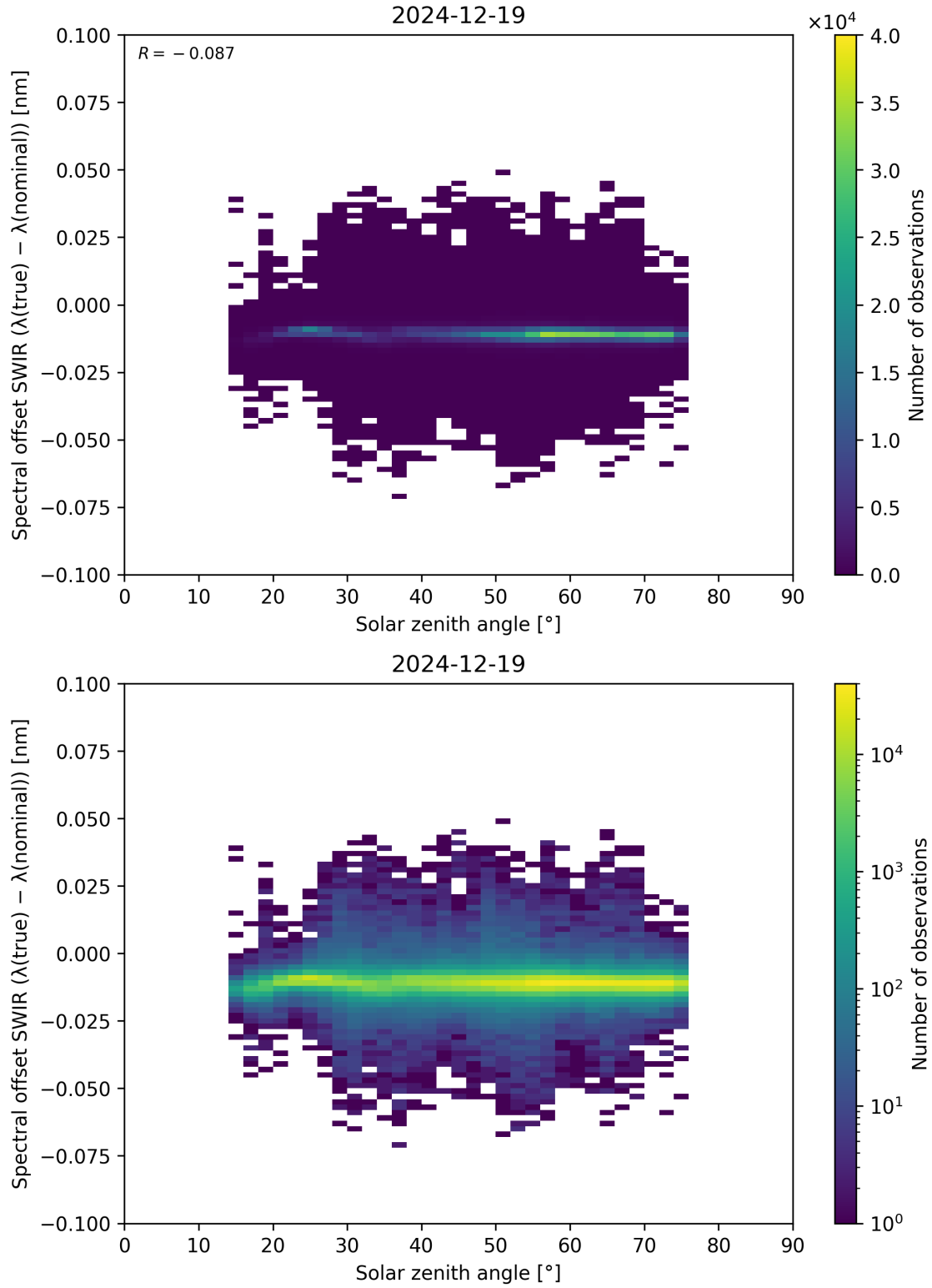
Figure 104: Scatter density plot of “Solar zenith angle” against “Spectral offset SWIR ( \lambda_{\text{true}} - \lambda_{\text{nominal}} )” for 2024-12-18 to 2024-12-20.
