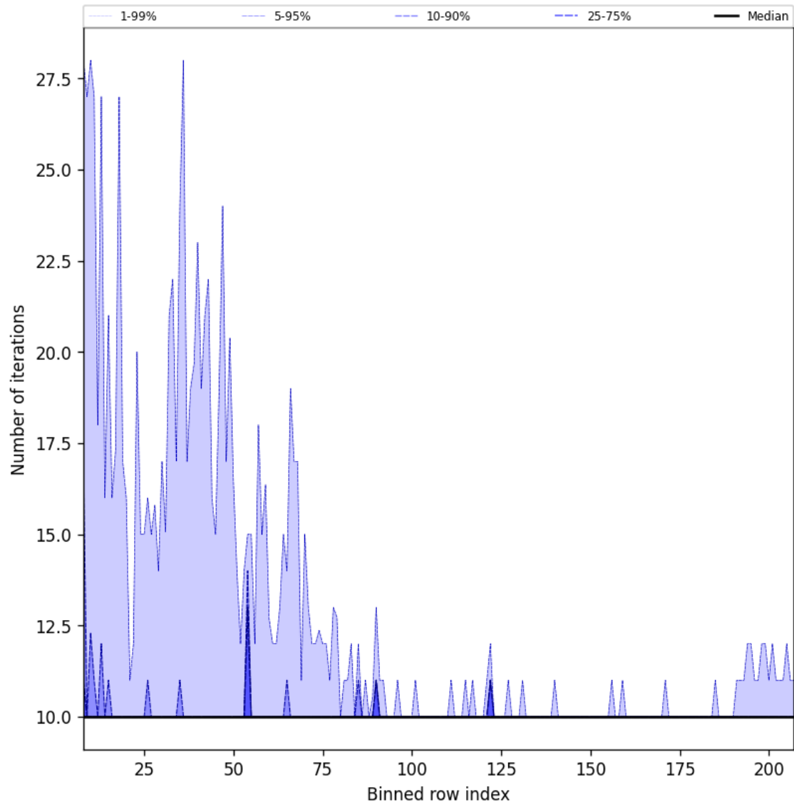
Figure 42: Along track statistics of “Number of iterations” for 2024-12-18 to 2024-12-20
