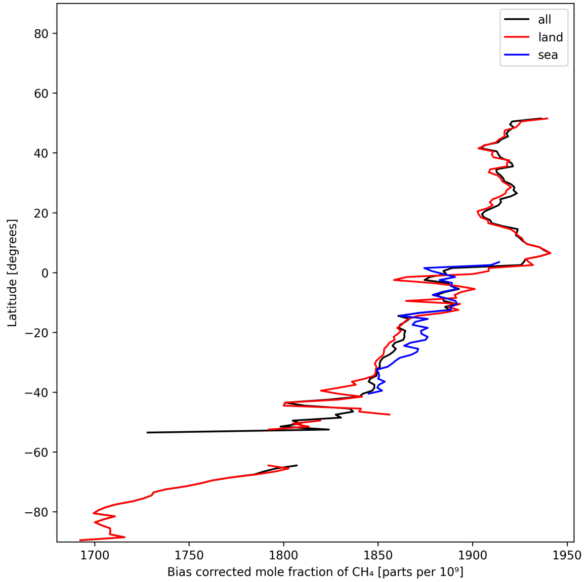
Figure 14: Zonal average of “Bias corrected mole fraction of CH 4 ” for 2024-12-18 to 2024-12-20.
