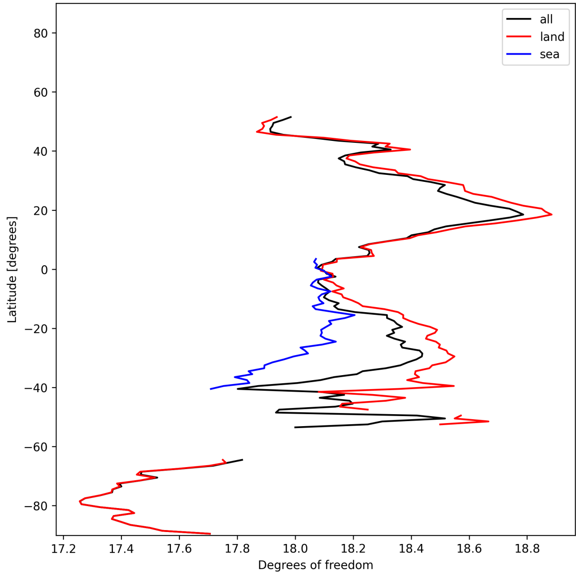
Figure 19: Zonal average of “Degrees of freedom” for 2024-12-18 to 2024-12-20.
