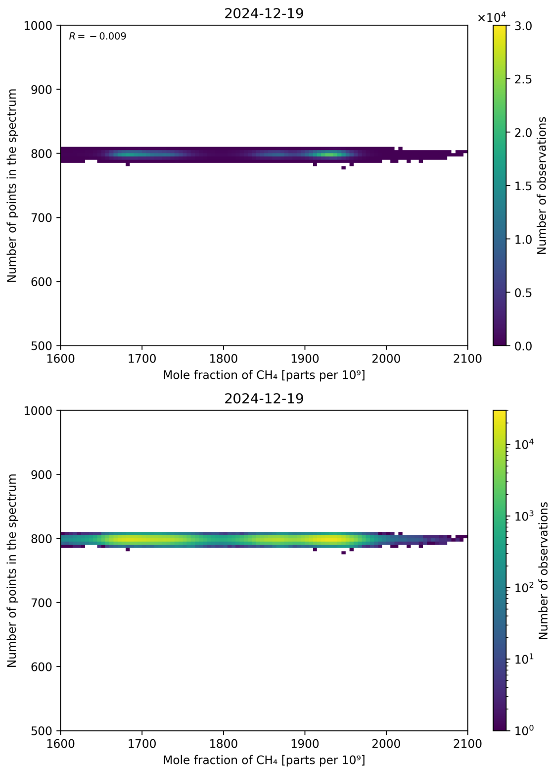
Figure 77: Scatter density plot of “Mole fraction of CH 4 ” against “Number of points in the spectrum” for 2024-12-18 to 2024-12-20.
