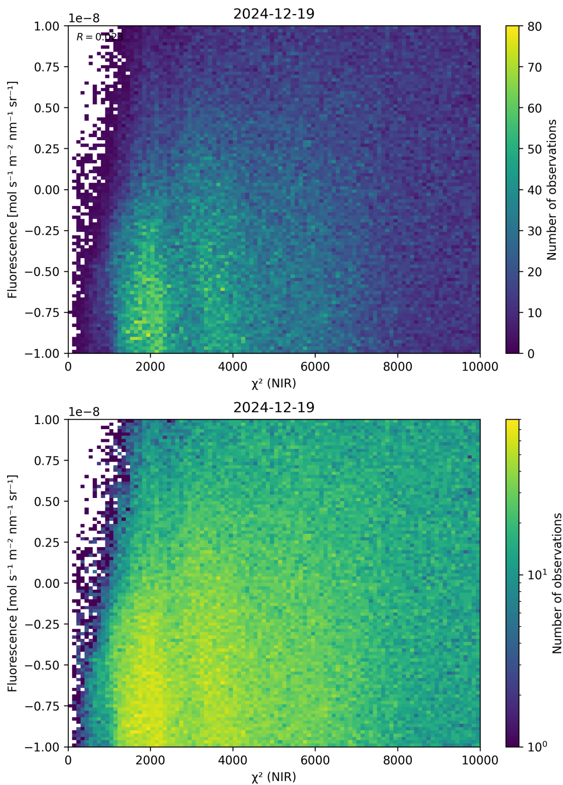
Figure 45: Scatter density plot of “ \chi^2 (NIR)” against “Fluorescence” for 2024-12-18 to 2024-12-20.
