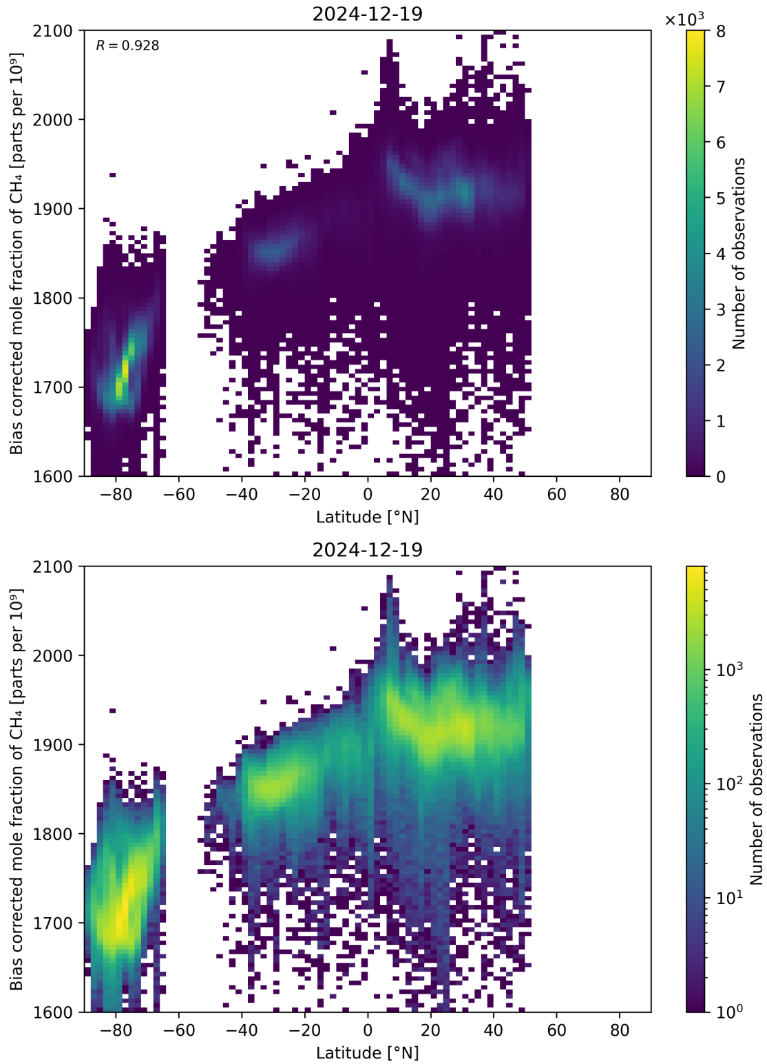
Figure 58: Scatter density plot of “Latitude” against “Bias corrected mole fraction of \text{CH}_4 ” for 2024-12-18 to 2024-12-20.
