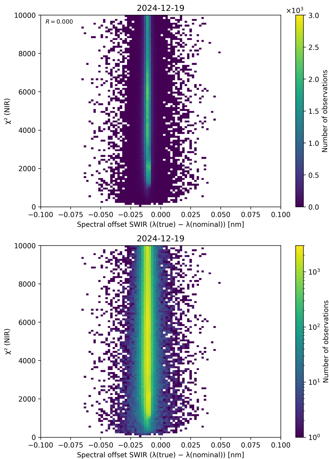
Figure 117: Scatter density plot of “Spectral offset SWIR ( \lambda_{\text{true}} - \lambda_{\text{nominal}} )” against “ \chi^2 (NIR)” for 2024-12-18 to 2024-12-20.
