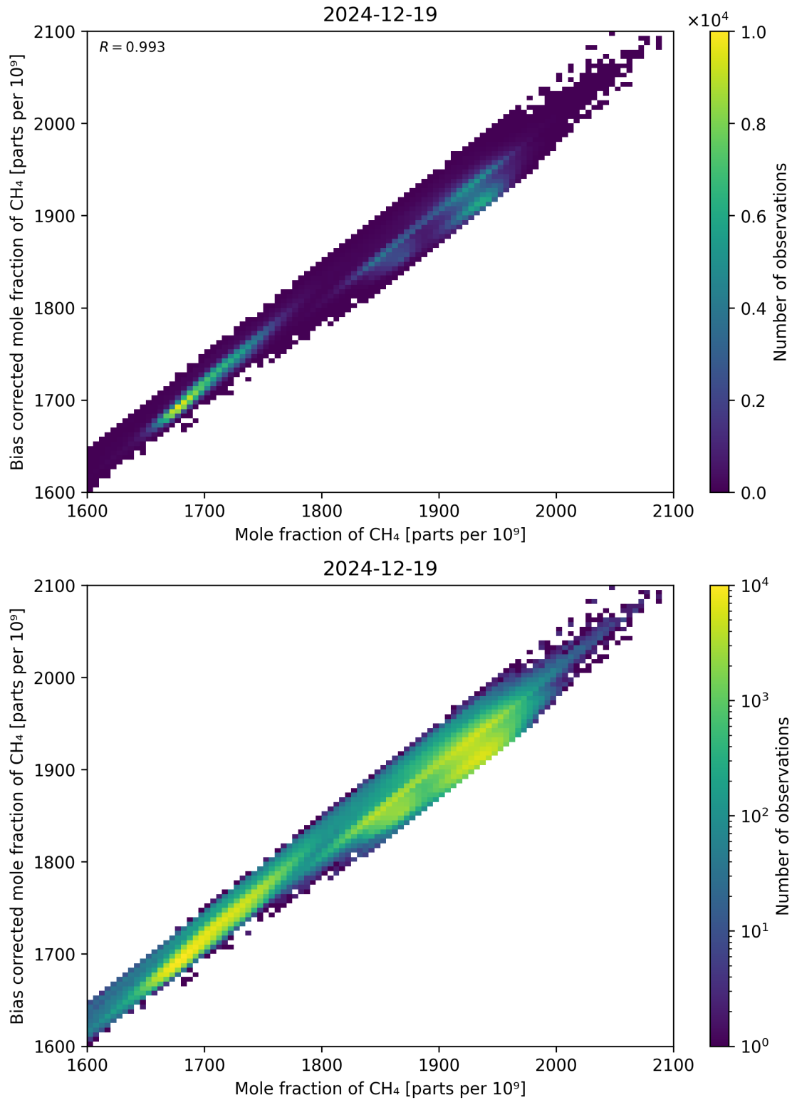
Figure 74: Scatter density plot of “Mole fraction of \text{CH}_4 ” against “Bias corrected mole fraction of \text{CH}_4 ” for 2024-12-18 to 2024-12-20.
