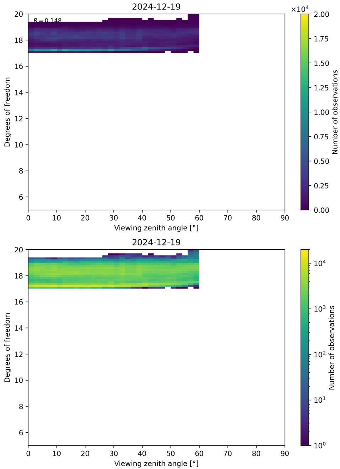
Figure 107: Scatter density plot of “Viewing zenith angle” against “Degrees of freedom” for 2024-12-18 to 2024-12-20.
