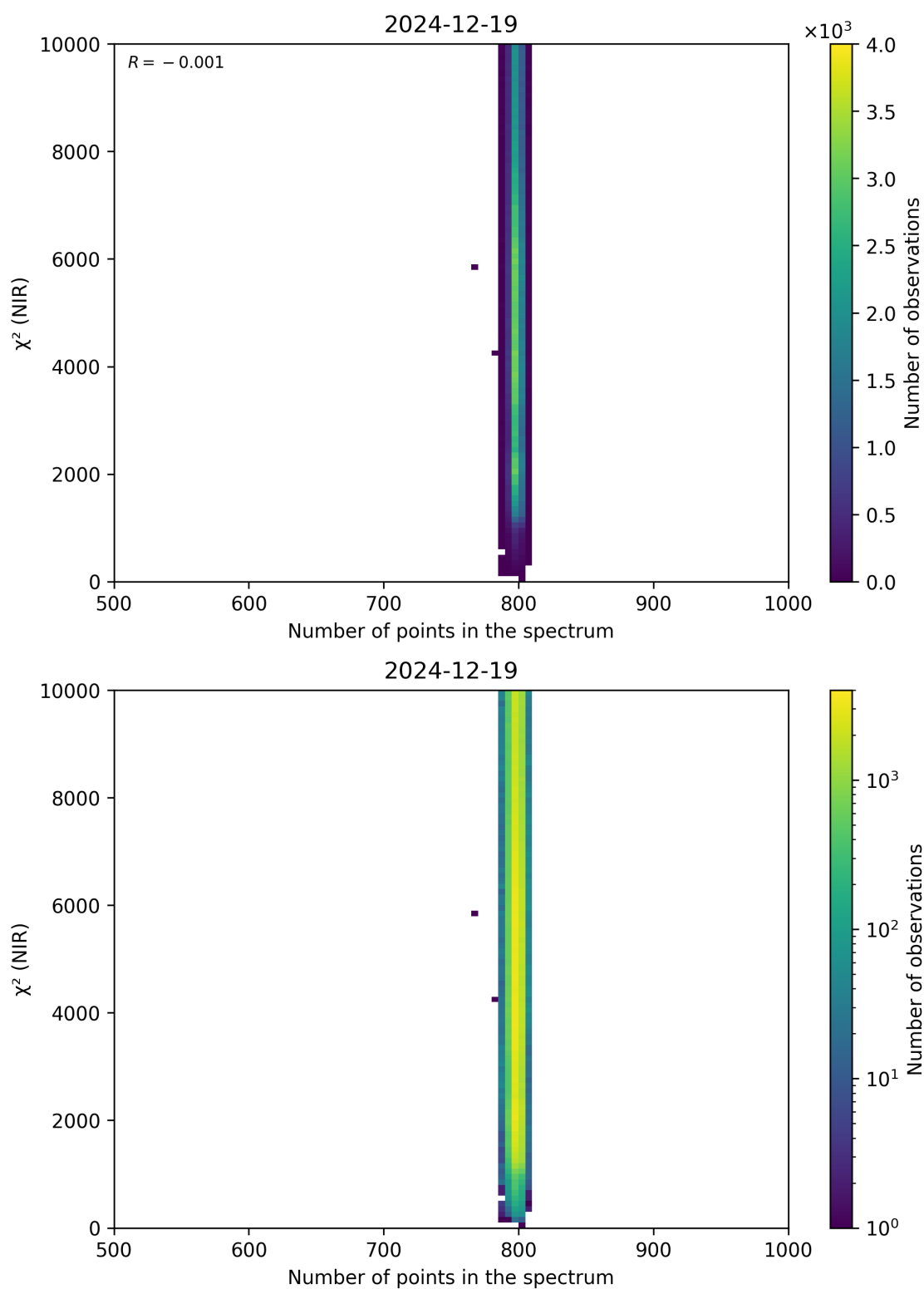
Figure 88: Scatter density plot of “Number of points in the spectrum” against “ \chi^2 (NIR)” for 2024-12-18 to 2024-12-20.
