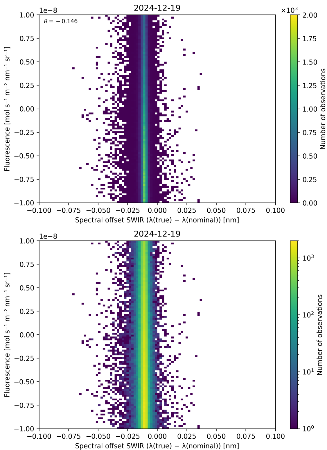
Figure 120: Scatter density plot of “Spectral offset SWIR ( \lambda_{\text{true}} - \lambda_{\text{nominal}} )” against “Fluorescence” for 2024-12-18 to 2024-12-20.
