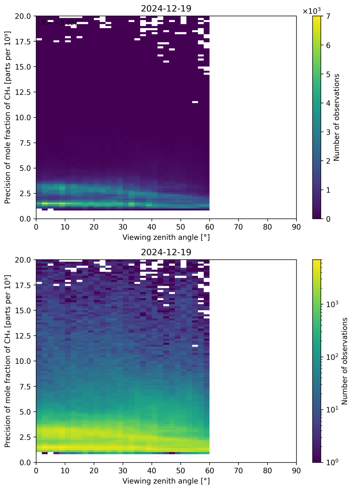
Figure 112: Scatter density plot of “Viewing zenith angle” against “Precision of mole fraction of CH 4 ” for 2024-12-18 to 2024-12-20.
