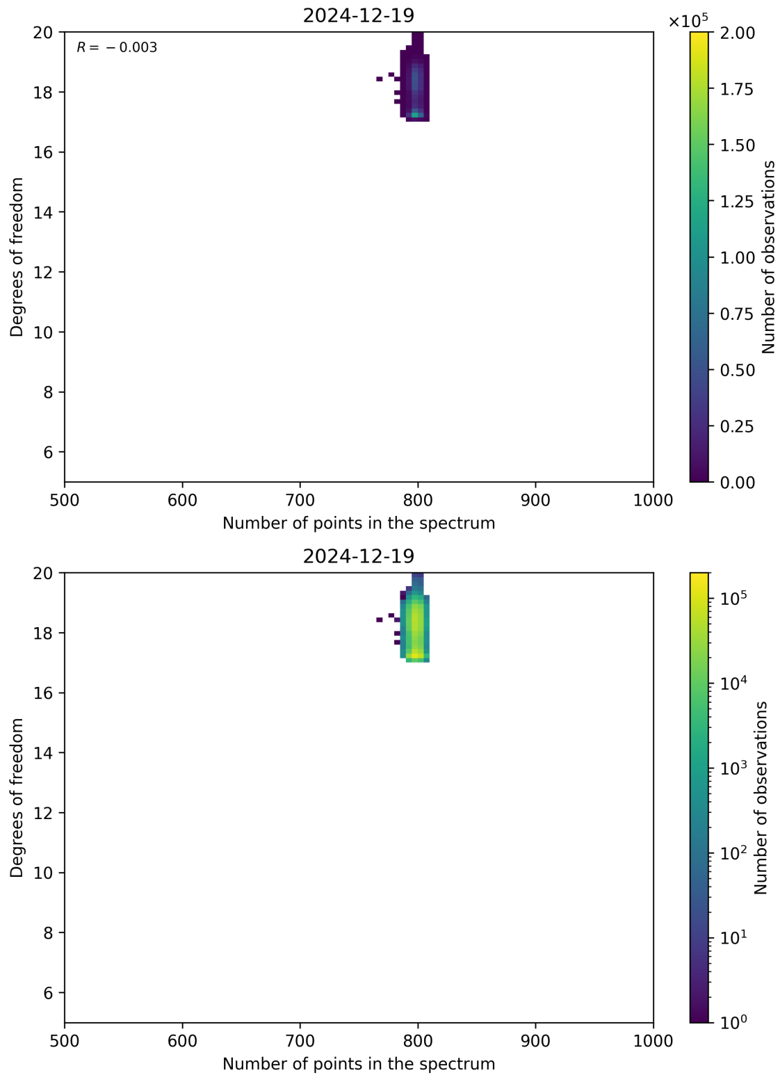
Figure 90: Scatter density plot of “Number of points in the spectrum” against “Degrees of freedom” for 2024-12-18 to 2024-12-20.
