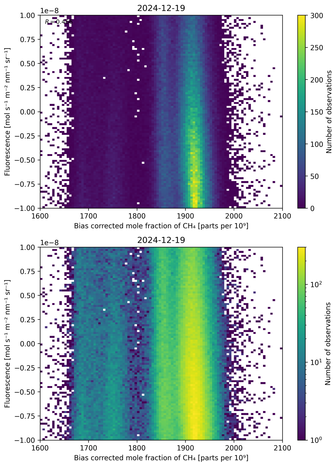
Figure 66: Scatter density plot of “Bias corrected mole fraction of \text{CH}_4 ” against “Fluorescence” for 2024-12-18 to 2024-12-20.
