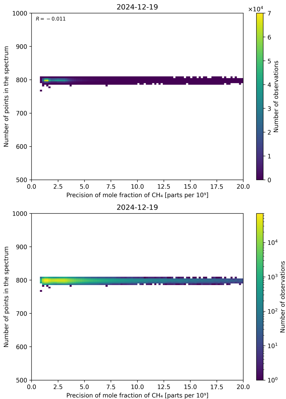
Figure 84: Scatter density plot of “Precision of mole fraction of CH 4 ” against “Number of points in the spectrum” for 2024-12-18 to 2024-12-20.
