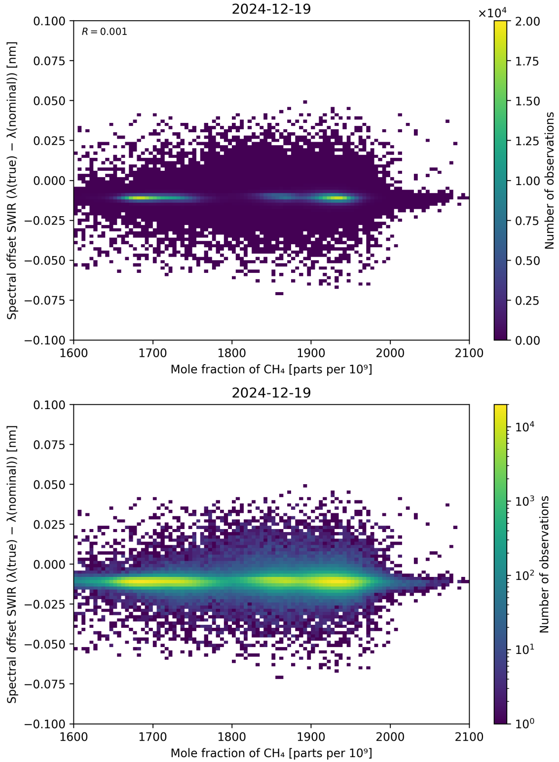
Figure 86: Scatter density plot of “Mole fraction of \text{CH}_4 ” against “Spectral offset SWIR ( \lambda_{\text{true}} - \lambda_{\text{nominal}} )” for 2024-12-18 to 2024-12-20.
