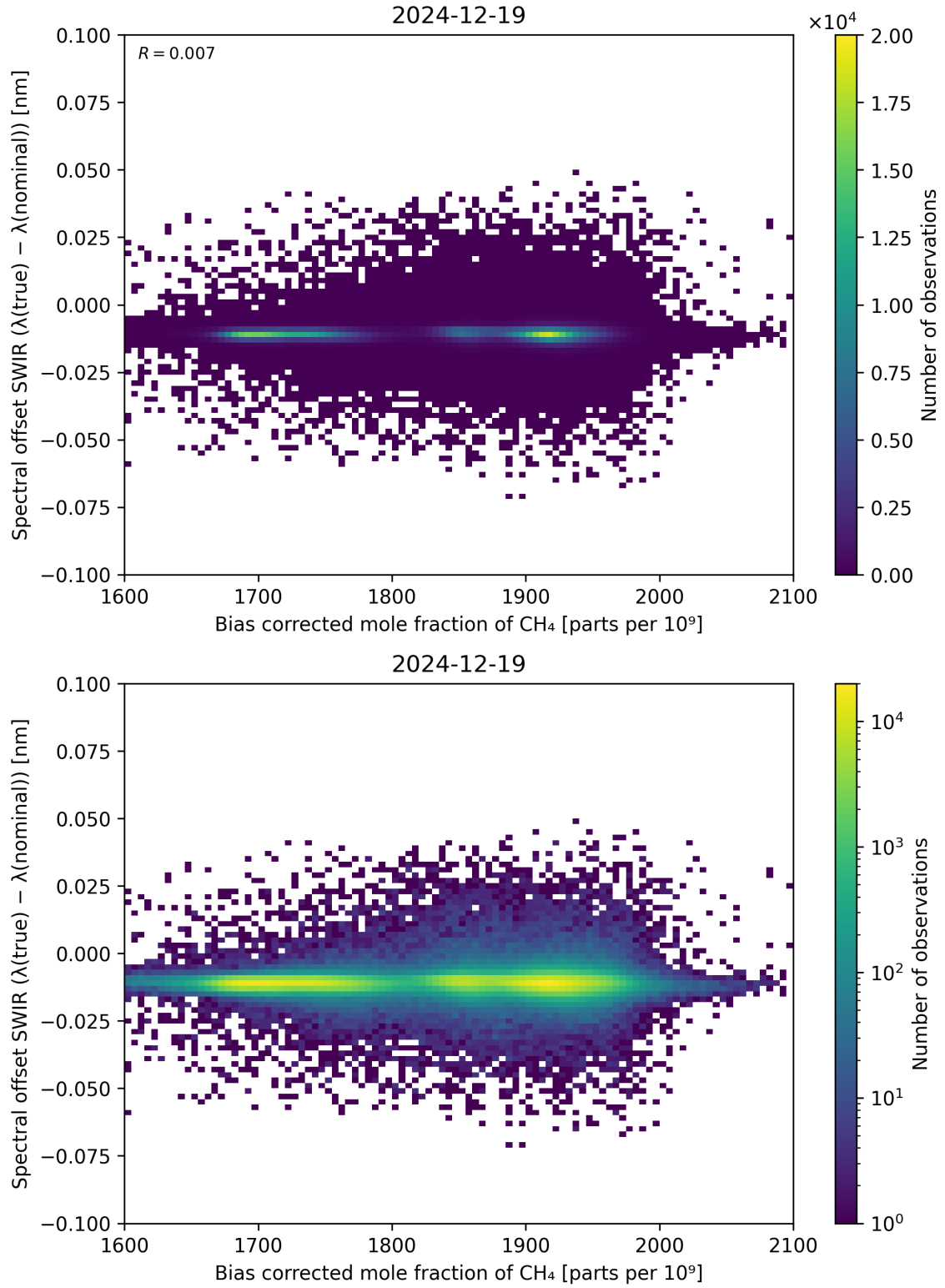
Figure 69: Scatter density plot of “Bias corrected mole fraction of \text{CH}_4 ” against “Spectral offset SWIR ( \lambda_{\text{true}} - \lambda_{\text{nominal}} )” for 2024-12-18 to 2024-12-20.
