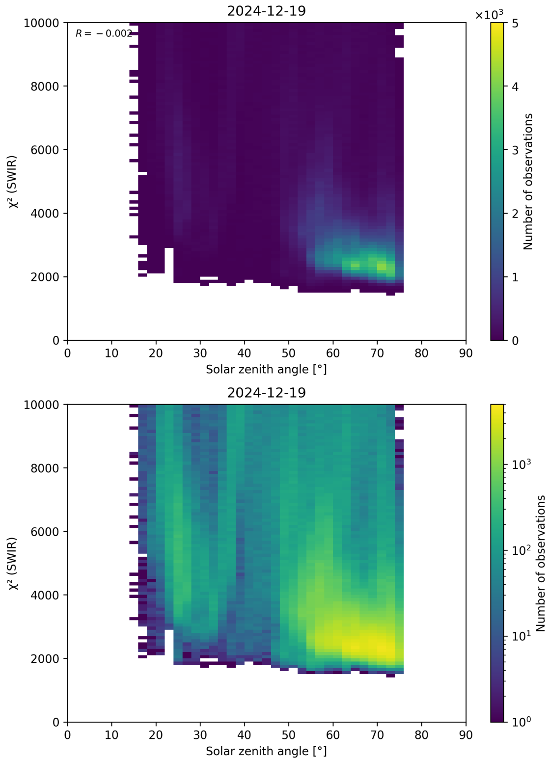
Figure 95: Scatter density plot of “Solar zenith angle” against “ \chi^2 (SWIR)” for 2024-12-18 to 2024-12-20.
