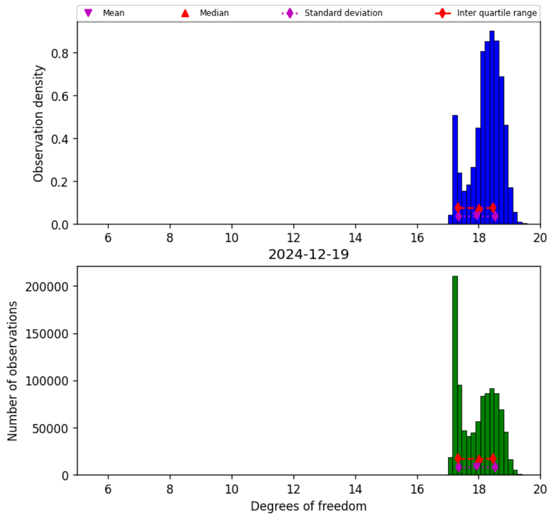
Figure 30: Histogram of “Degrees of freedom” for 2024-12-18 to 2024-12-20
