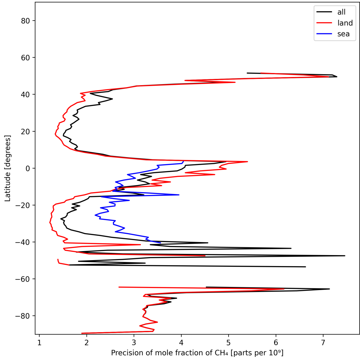
Figure 13: Zonal average of “Precision of mole fraction of CH 4 ” for 2024-12-18 to 2024-12-20.
