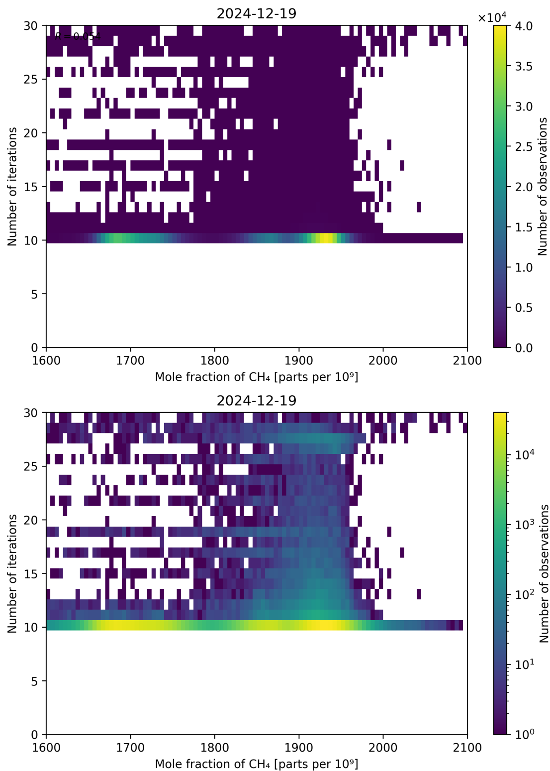
Figure 76: Scatter density plot of “Mole fraction of CH 4 ” against “Number of iterations” for 2024-12-18 to 2024-12-20.
