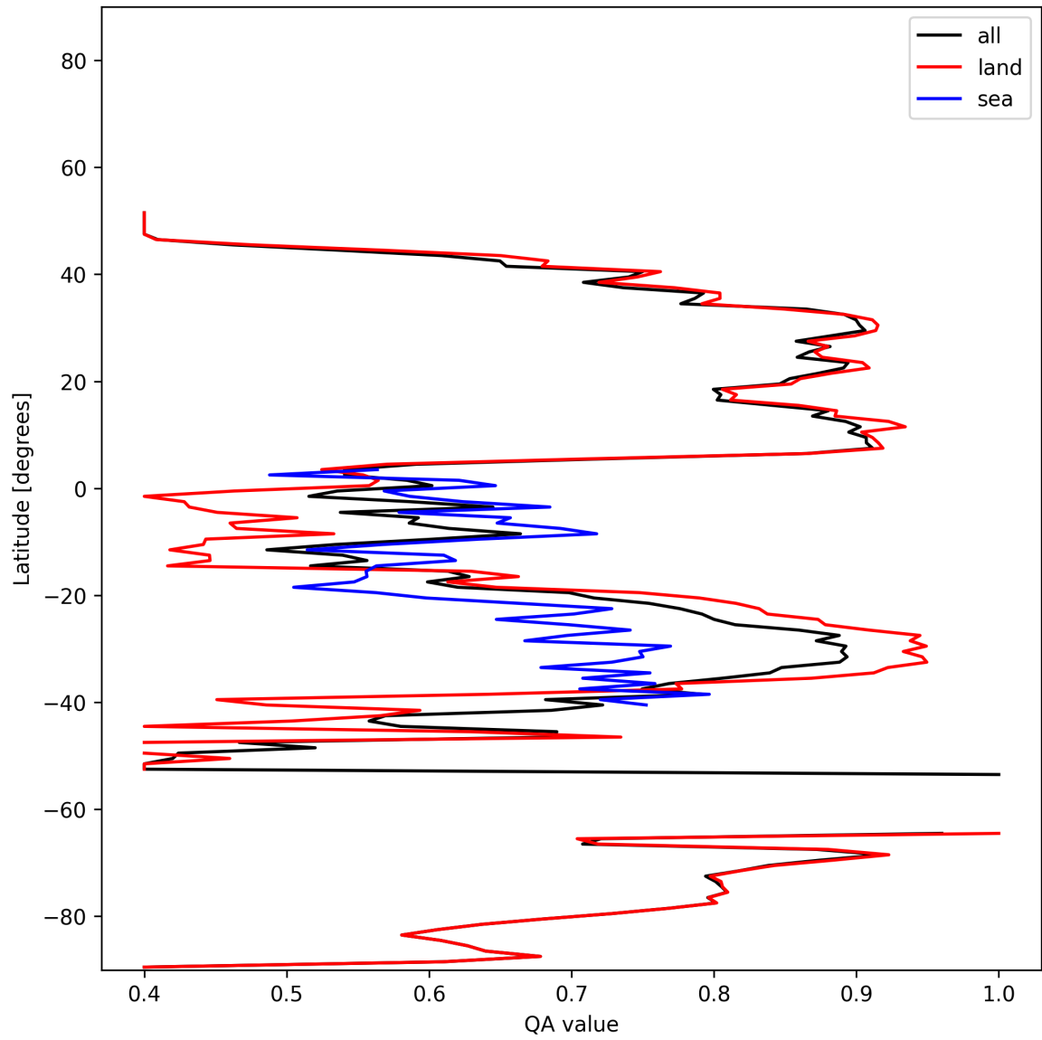
Figure 11: Zonal average of “QA value” for 2024-12-18 to 2024-12-20.
