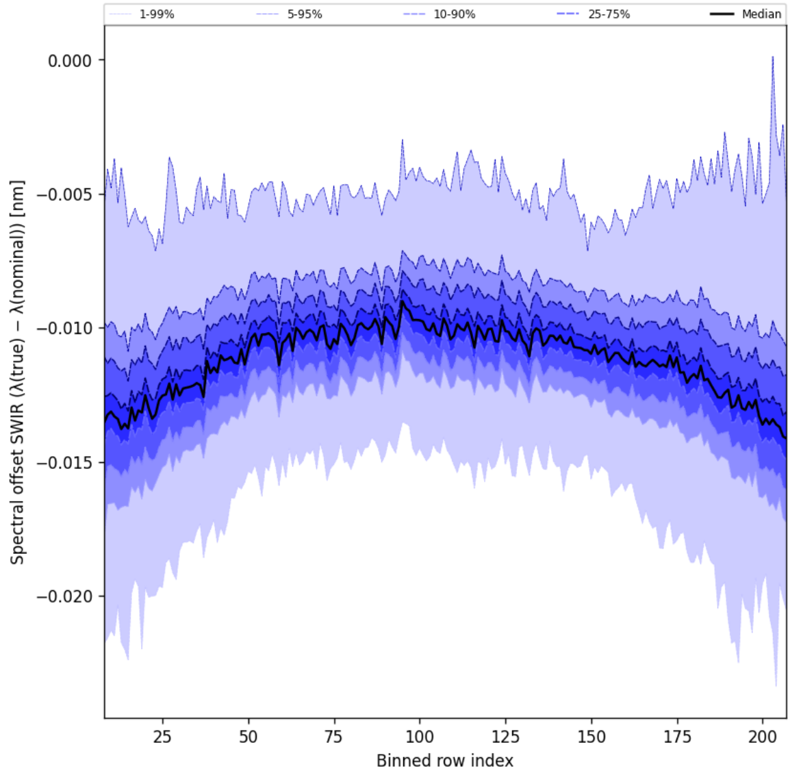
Figure 38: Along track statistics of “Spectral offset SWIR ( \lambda_{\text{true}} - \lambda_{\text{nominal}} )” for 2024-12-18 to 2024-12-20
