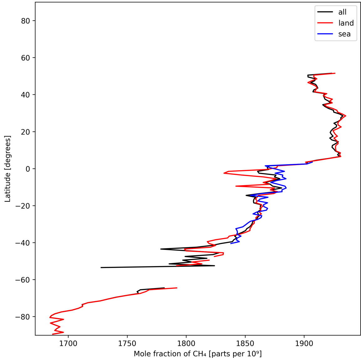
Figure 12: Zonal average of “Mole fraction of CH 4 ” for 2024-12-18 to 2024-12-20.
