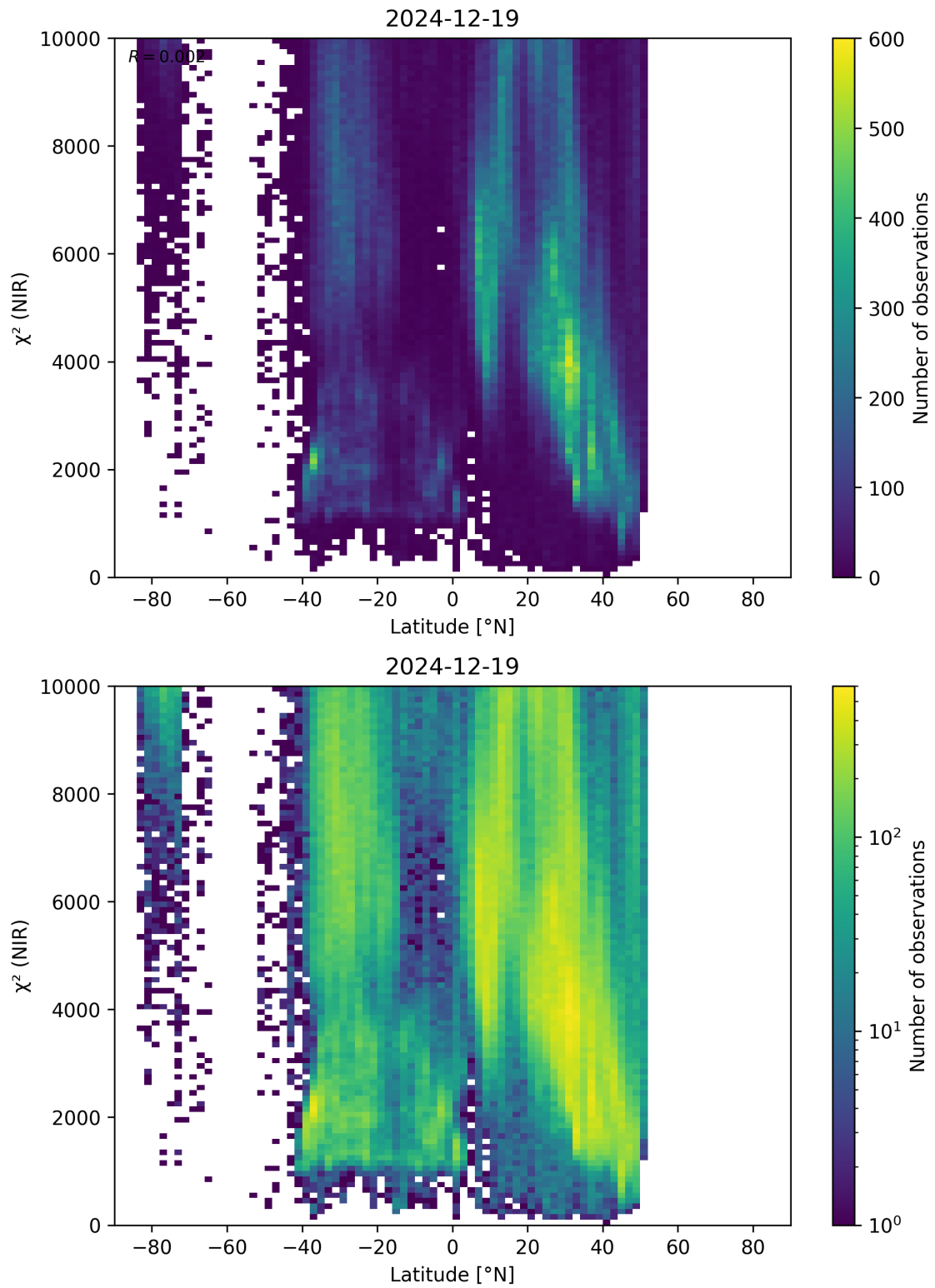
Figure 53: Scatter density plot of “Latitude” against “ \chi^2 (NIR)” for 2024-12-18 to 2024-12-20.
