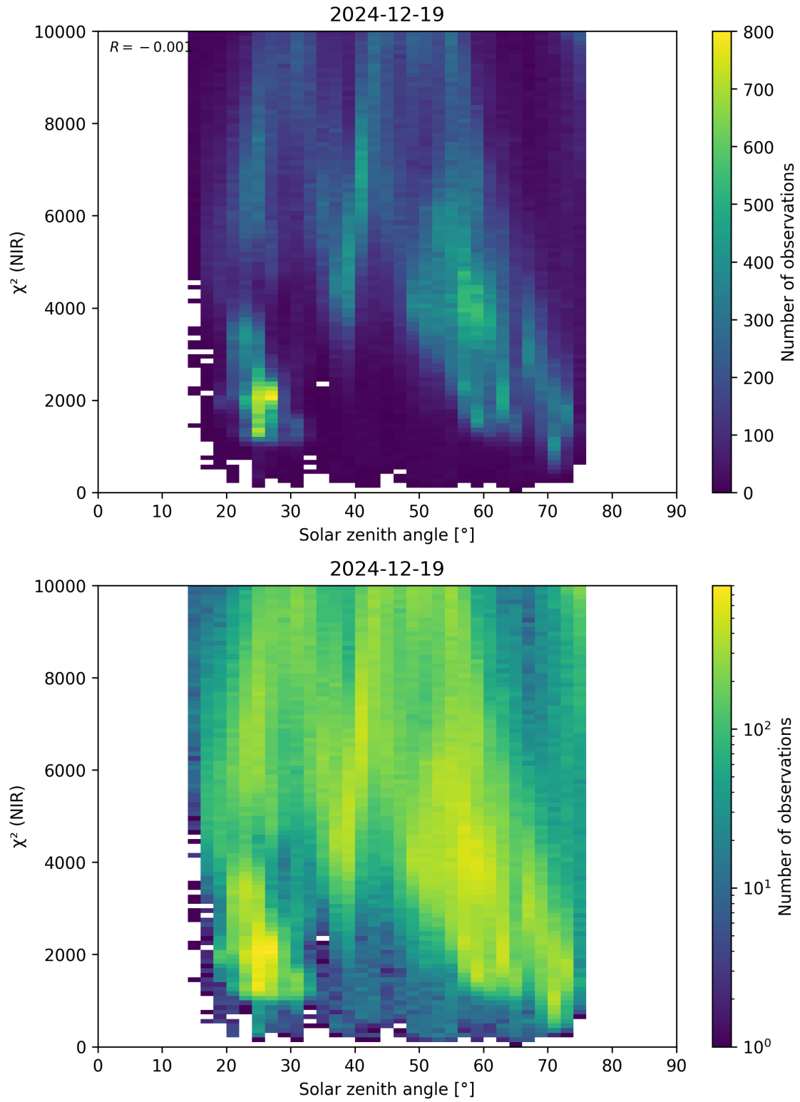
Figure 94: Scatter density plot of “Solar zenith angle” against “ \chi^2 (NIR)” for 2024-12-18 to 2024-12-20.
