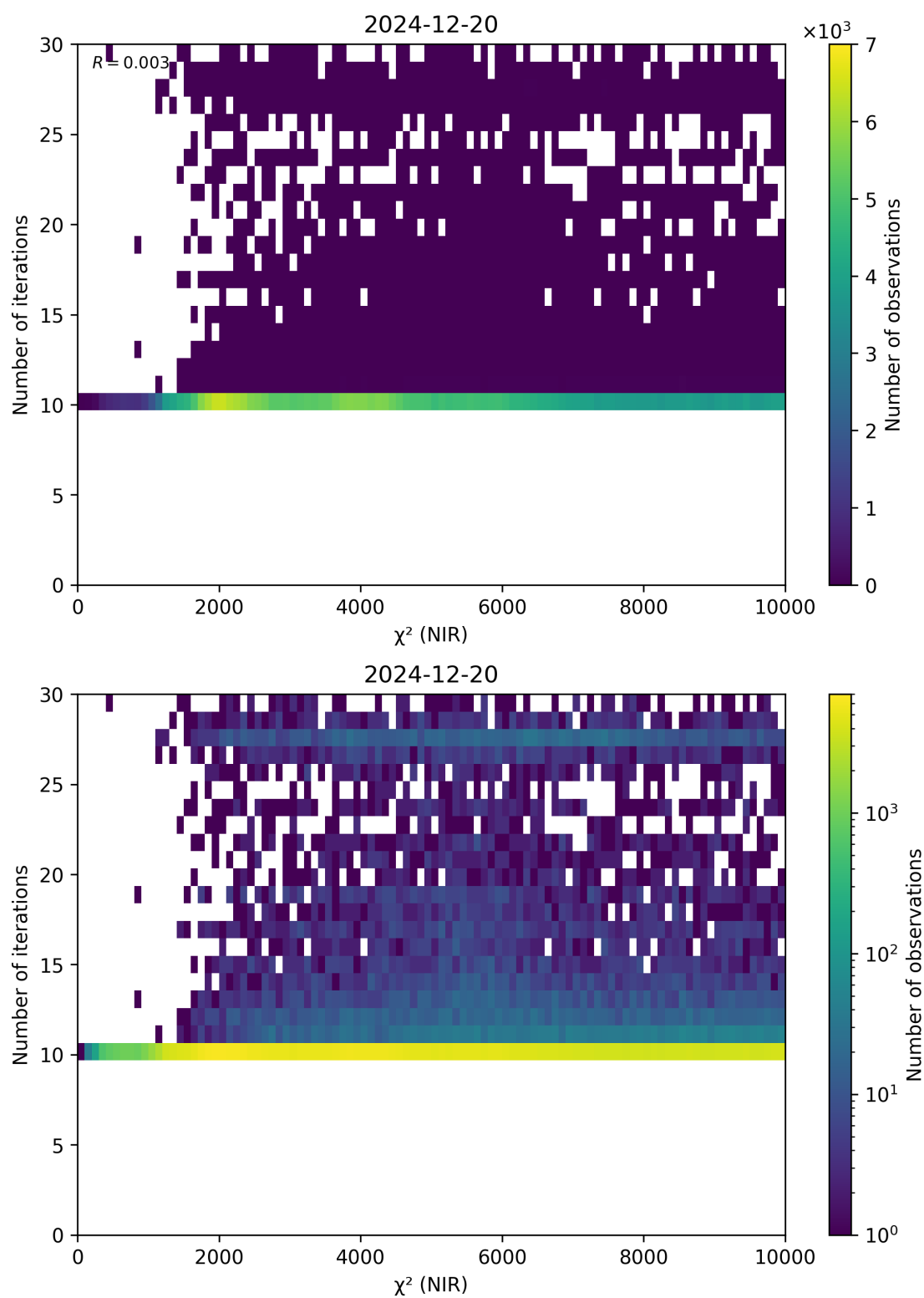
Figure 46: Scatter density plot of “ \chi^2 (NIR)” against “Number of iterations” for 2024-12-19 to 2024-12-21.
