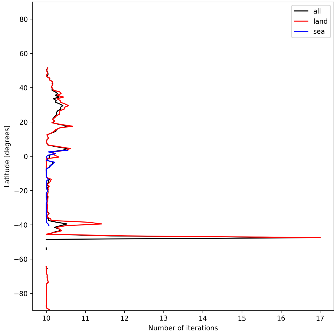
Figure 20: Zonal average of “Number of iterations” for 2024-12-19 to 2024-12-21.
