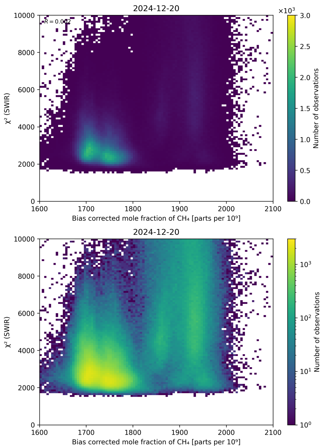
Figure 64: Scatter density plot of “Bias corrected mole fraction of \text{CH}_4 ” against “ \chi^2 (SWIR)” for 2024-12-19 to 2024-12-21.
