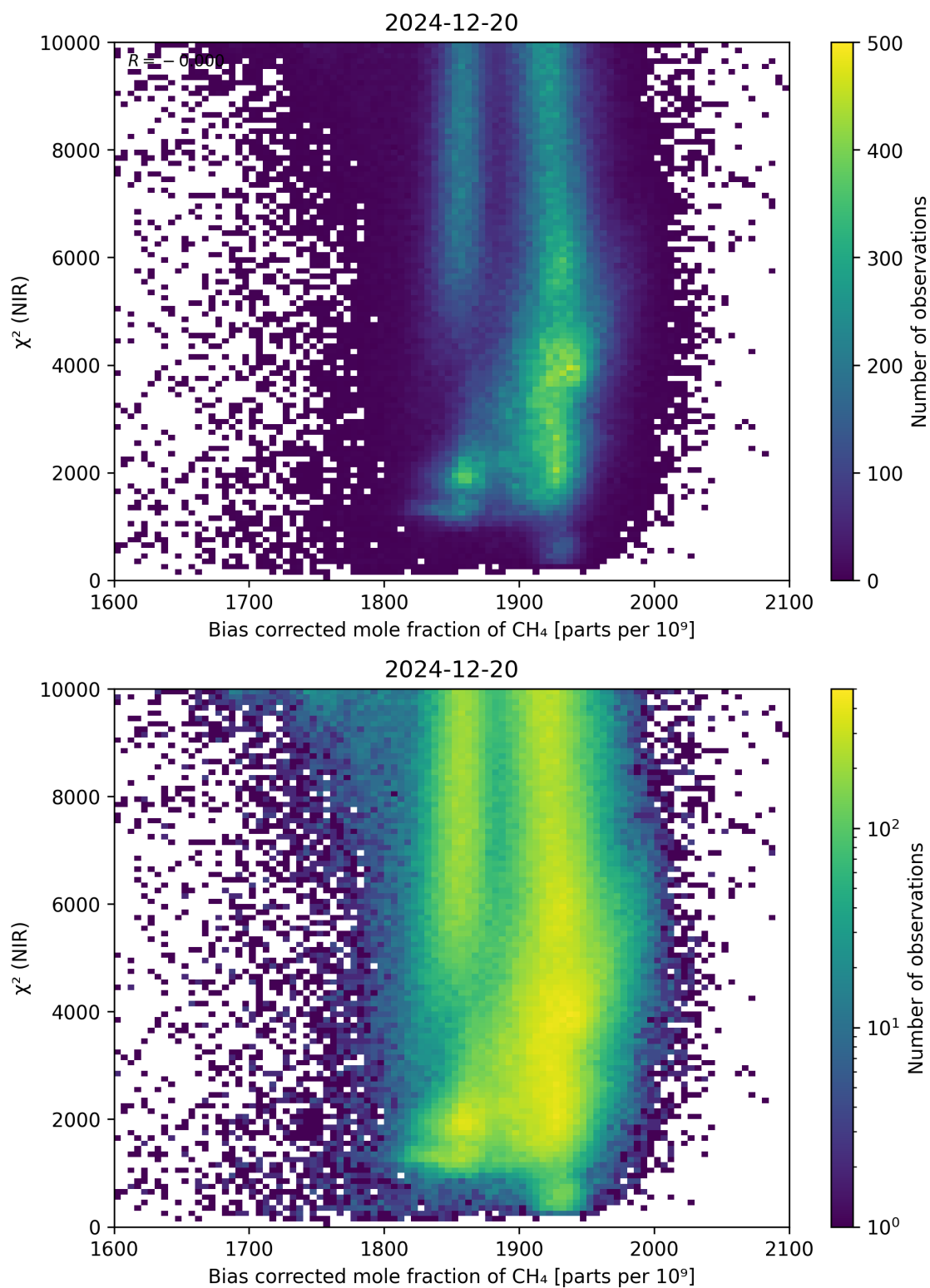
Figure 63: Scatter density plot of “Bias corrected mole fraction of \text{CH}_4 ” against “ \chi^2 (NIR)” for 2024-12-19 to 2024-12-21.
