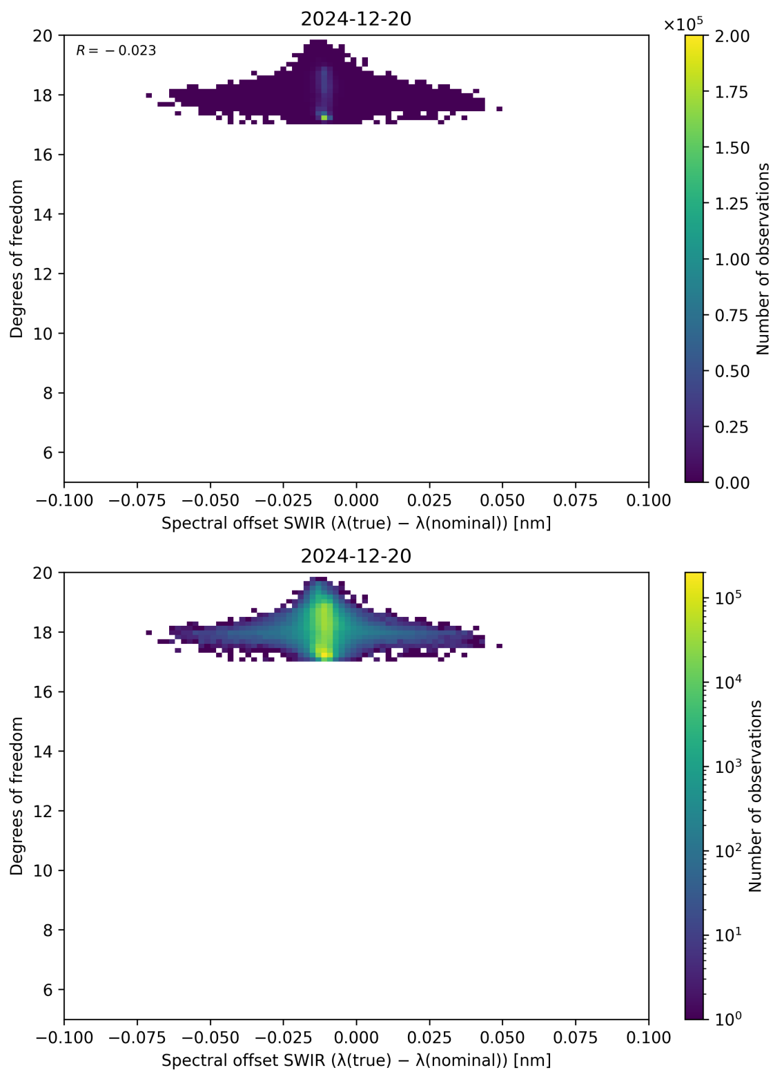
Figure 119: Scatter density plot of “Spectral offset SWIR ( \lambda_{\text{true}} - \lambda_{\text{nominal}} )” against “Degrees of freedom” for 2024-12-19 to 2024-12-21.
