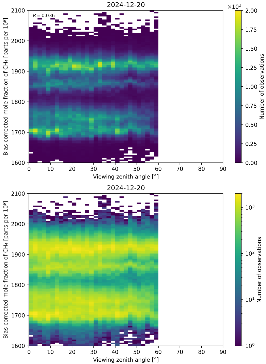
Figure 111: Scatter density plot of “Viewing zenith angle” against “Bias corrected mole fraction of CH 4 ” for 2024-12-19 to 2024-12-21.
