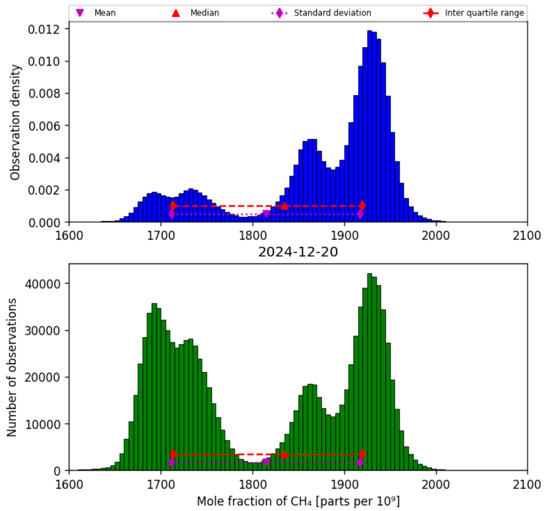
Figure 23: Histogram of “Mole fraction of CH 4 ” for 2024-12-19 to 2024-12-21
