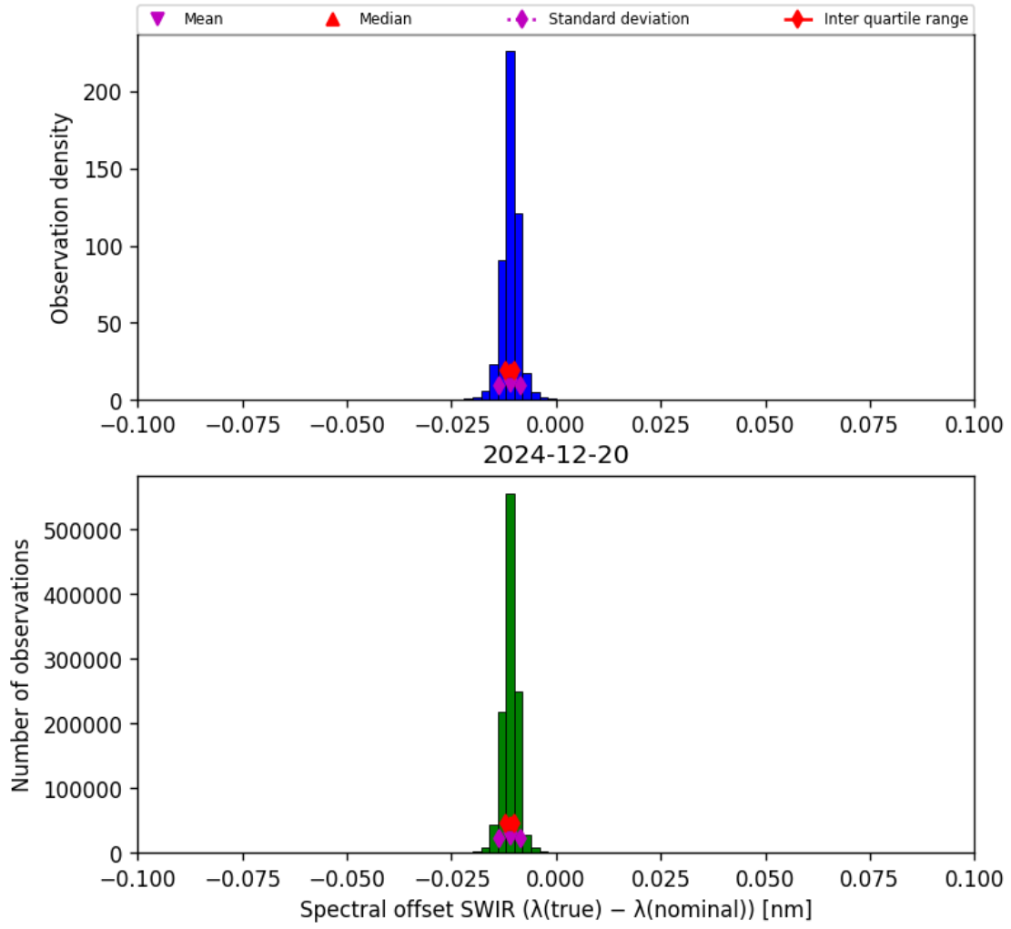
Figure 27: Histogram of “Spectral offset SWIR ( \lambda_{\text{true}} - \lambda_{\text{nominal}} )” for 2024-12-19 to 2024-12-21
