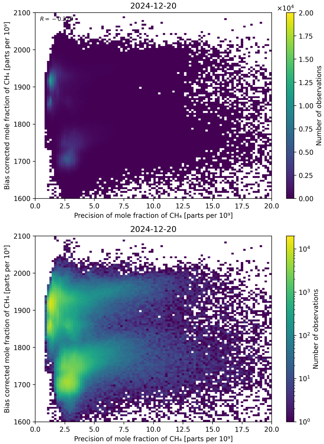
Figure 82: Scatter density plot of “Precision of mole fraction of \text{CH}_4 ” against “Bias corrected mole fraction of \text{CH}_4 ” for 2024-12-19 to 2024-12-21.
