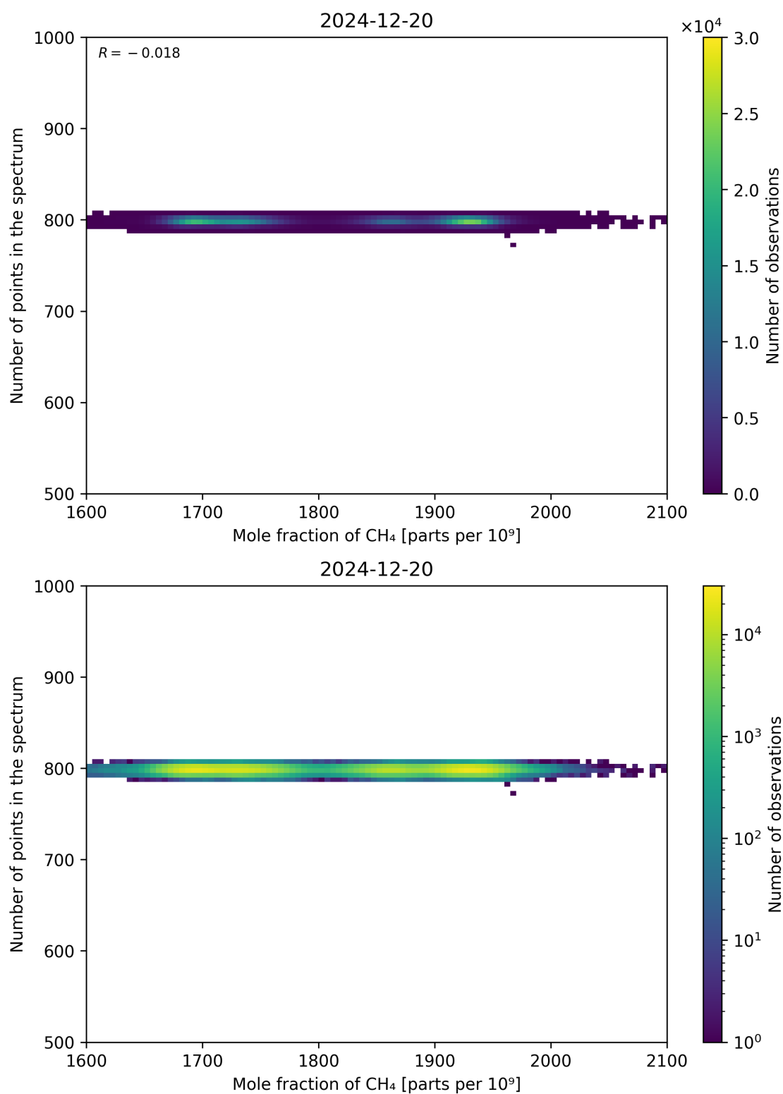
Figure 77: Scatter density plot of “Mole fraction of CH 4 ” against “Number of points in the spectrum” for 2024-12-19 to 2024-12-21.
