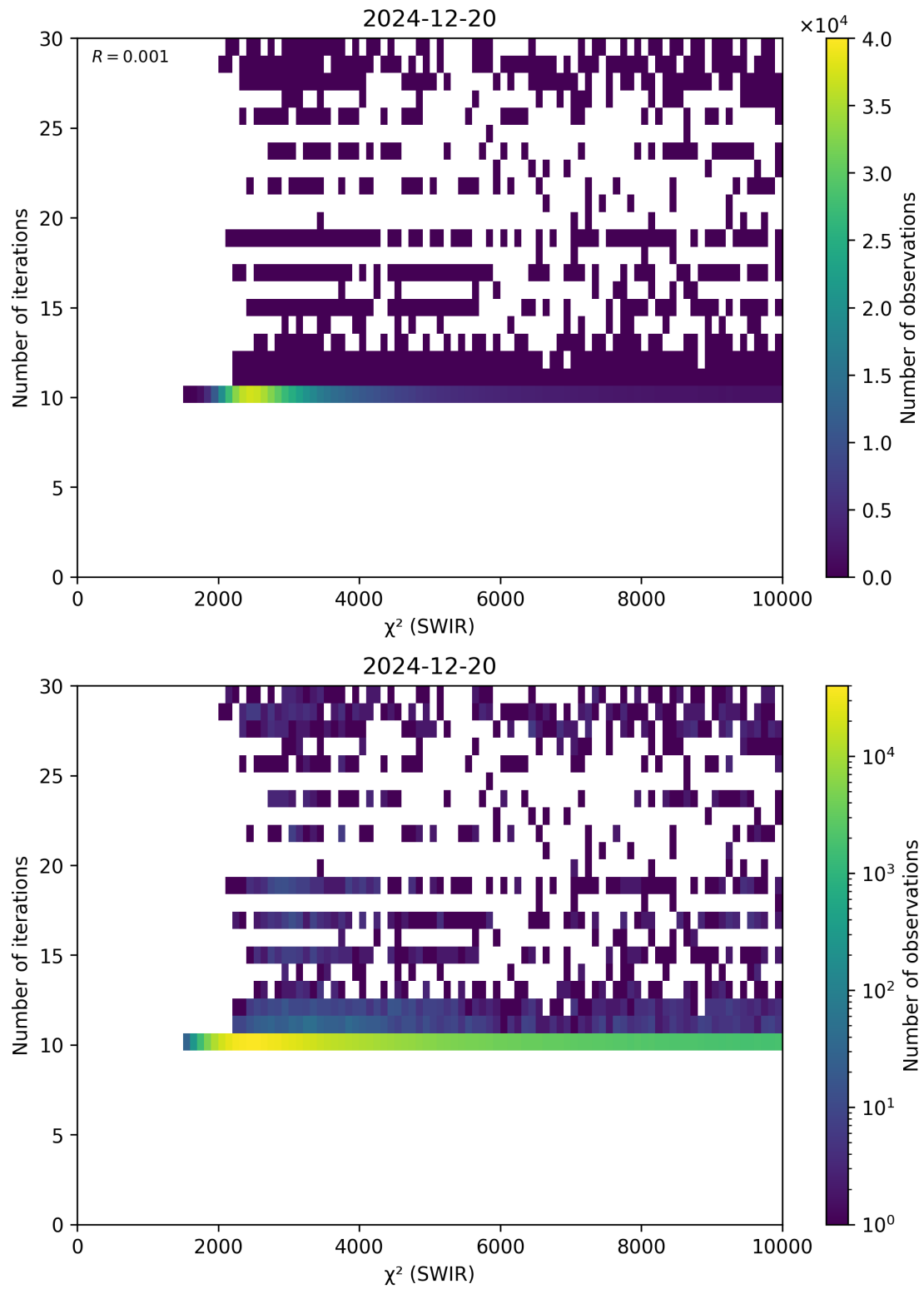
Figure 50: Scatter density plot of “ \chi^2 (SWIR)” against “Number of iterations” for 2024-12-19 to 2024-12-21.
