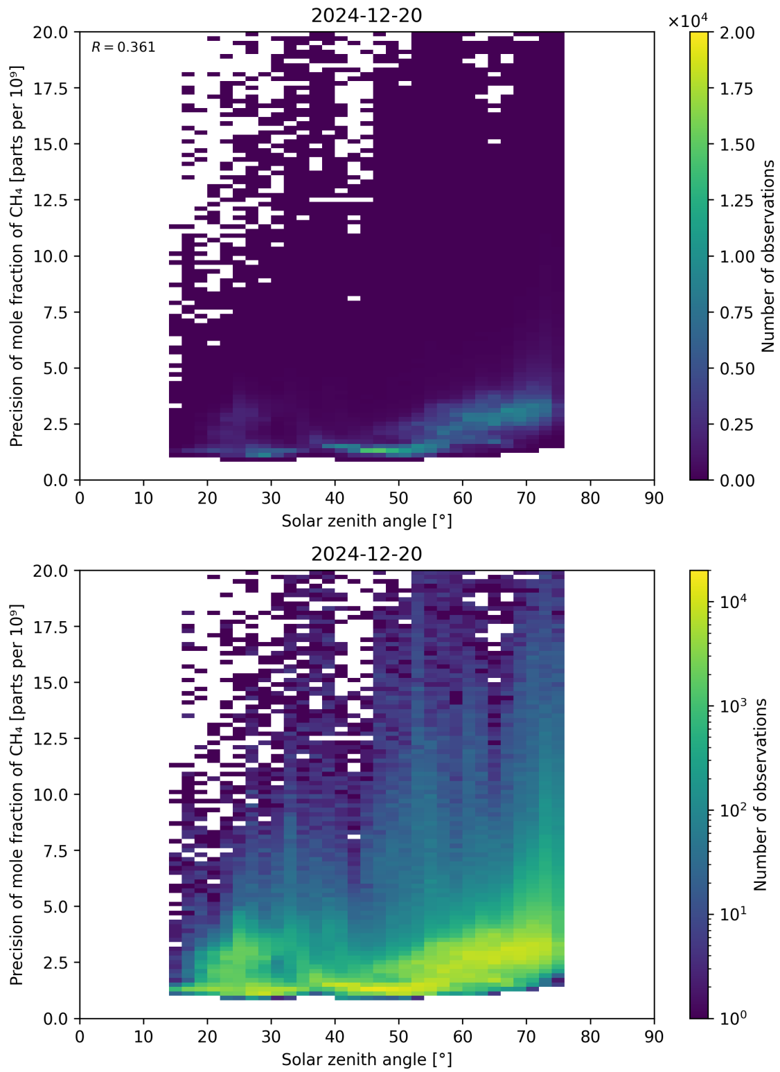
Figure 101: Scatter density plot of “Solar zenith angle” against “Precision of mole fraction of CH 4 ” for 2024-12-19 to 2024-12-21.
