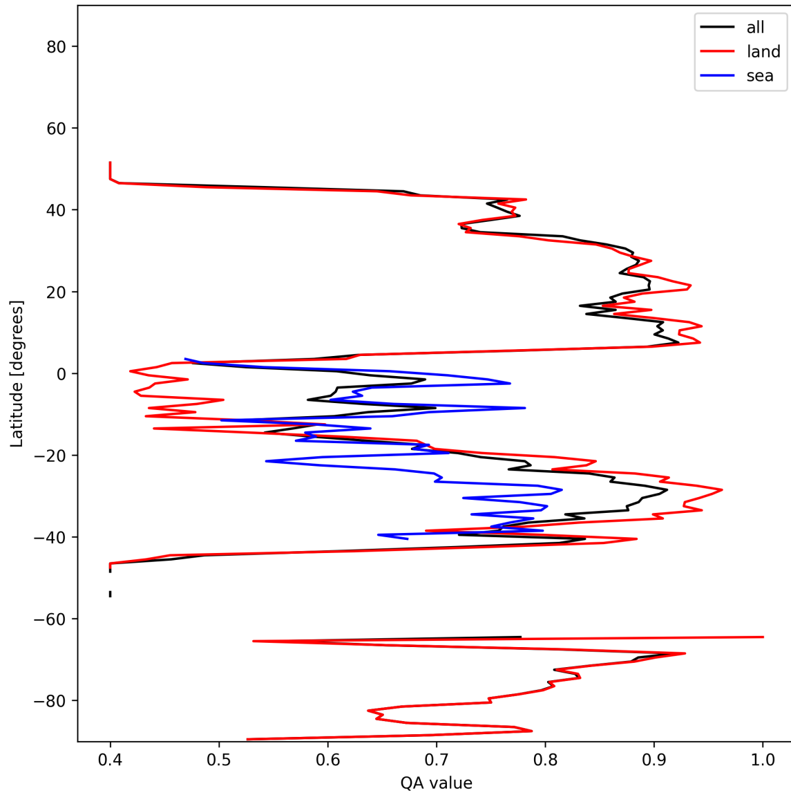
Figure 11: Zonal average of “QA value” for 2024-12-19 to 2024-12-21.
