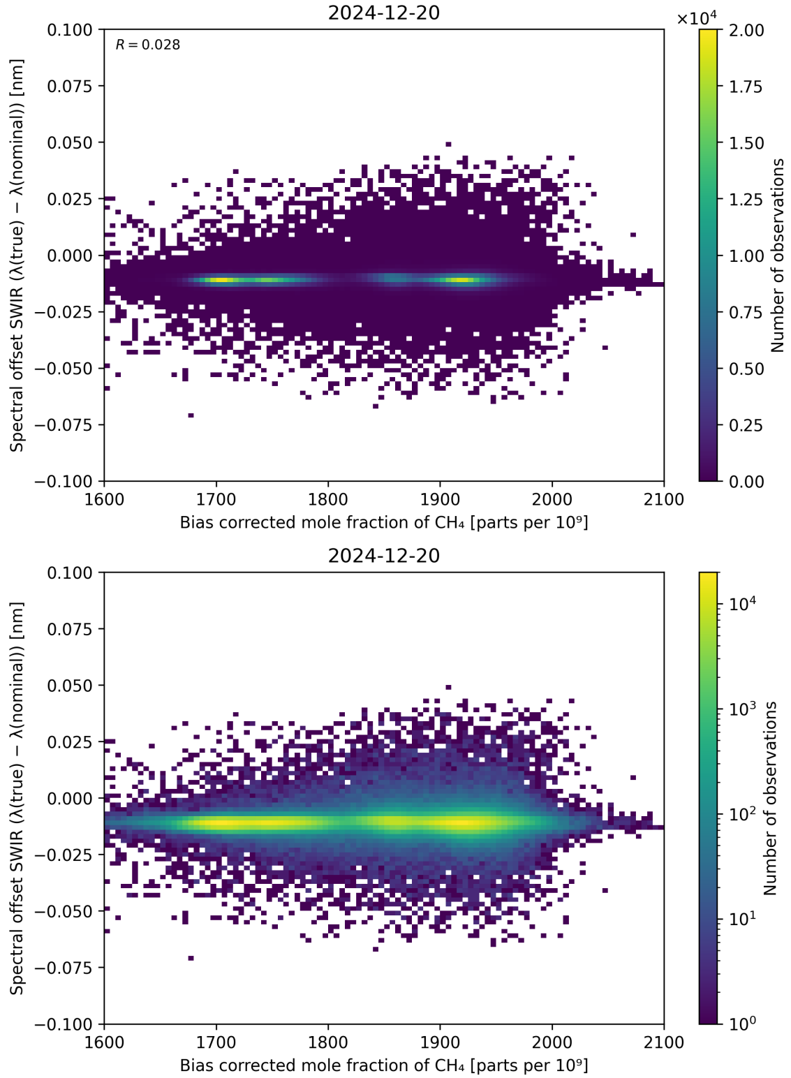
Figure 69: Scatter density plot of “Bias corrected mole fraction of \text{CH}_4 ” against “Spectral offset SWIR ( \lambda_{\text{true}} - \lambda_{\text{nominal}} )” for 2024-12-19 to 2024-12-21.
