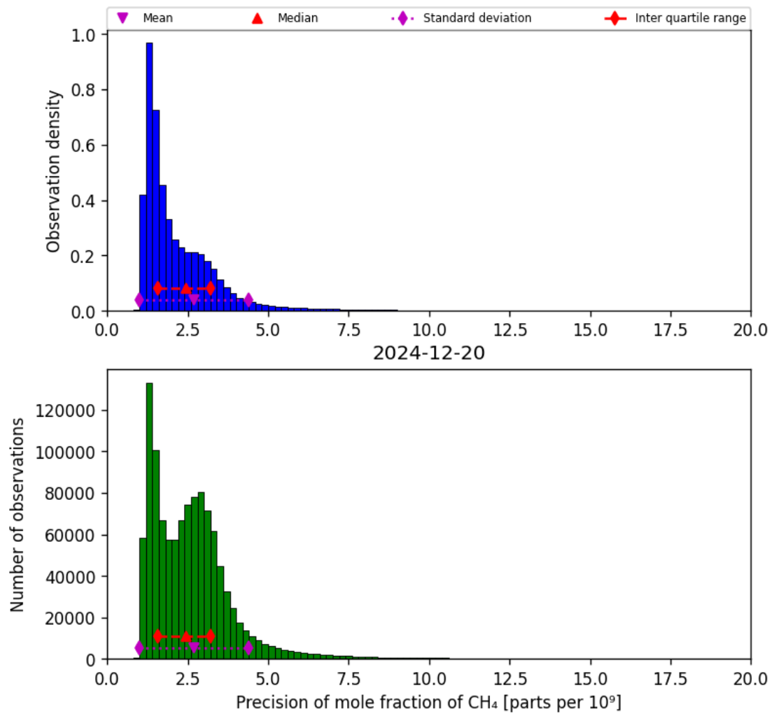
Figure 24: Histogram of “Precision of mole fraction of CH 4 ” for 2024-12-19 to 2024-12-21
