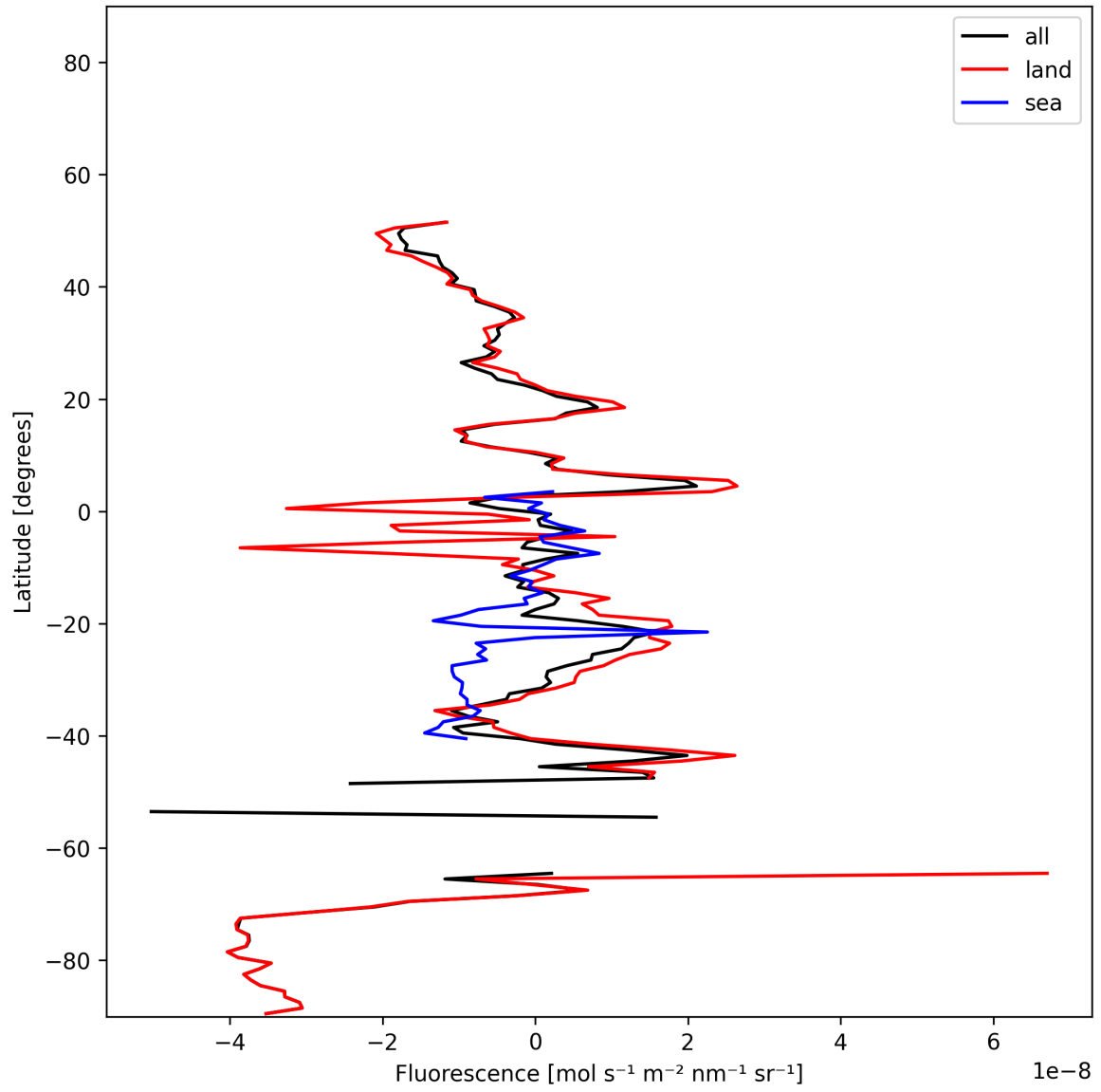
Figure 21: Zonal average of “Fluorescence” for 2024-12-19 to 2024-12-21.
