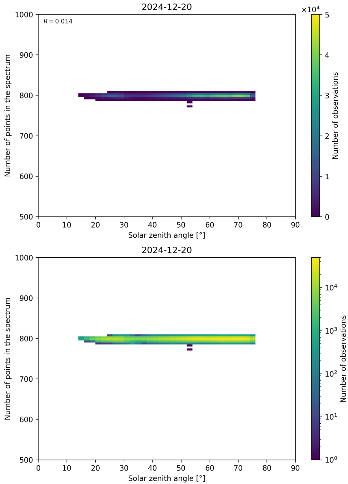
Figure 103: Scatter density plot of “Solar zenith angle” against “Number of points in the spectrum” for 2024-12-19 to 2024-12-21.
