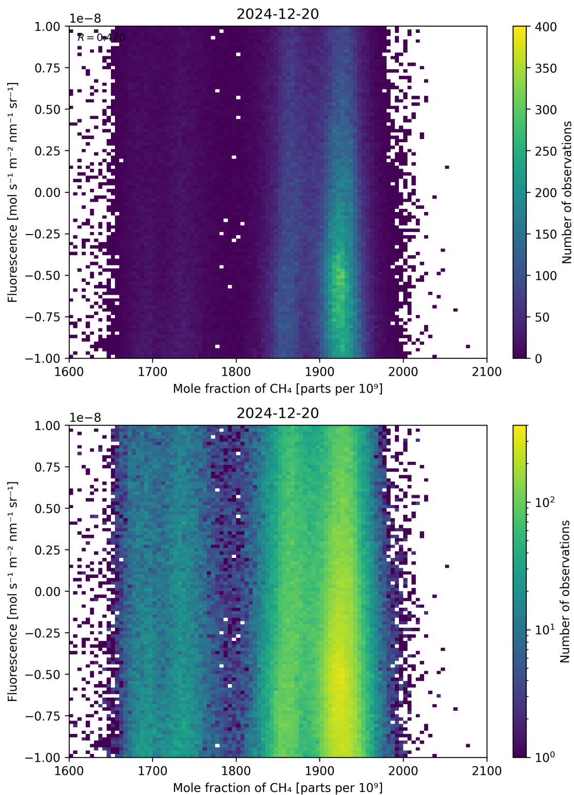
Figure 73: Scatter density plot of “Mole fraction of \text{CH}_4 ” against “Fluorescence” for 2024-12-19 to 2024-12-21.
