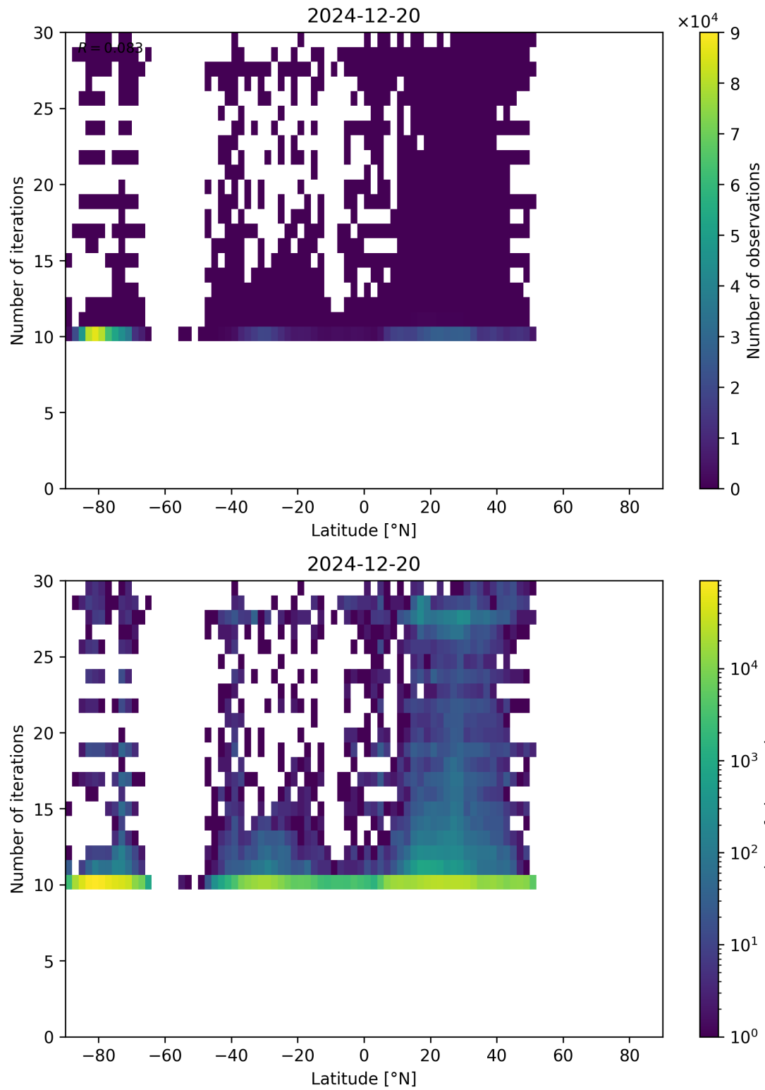
Figure 60: Scatter density plot of “Latitude” against “Number of iterations” for 2024-12-19 to 2024-12-21.
