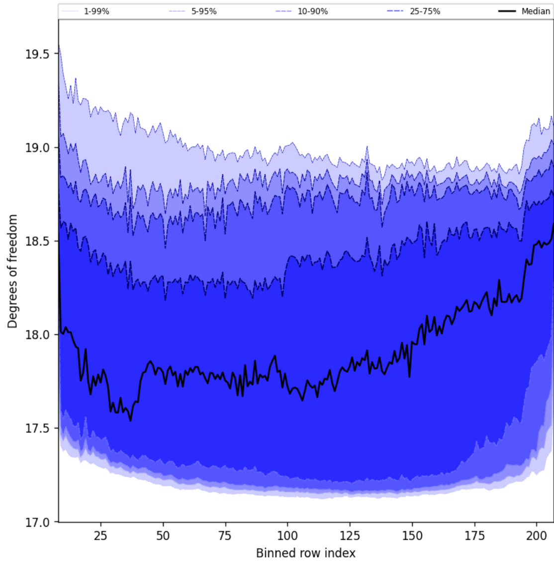
Figure 41: Along track statistics of “Degrees of freedom” for 2024-12-19 to 2024-12-21
