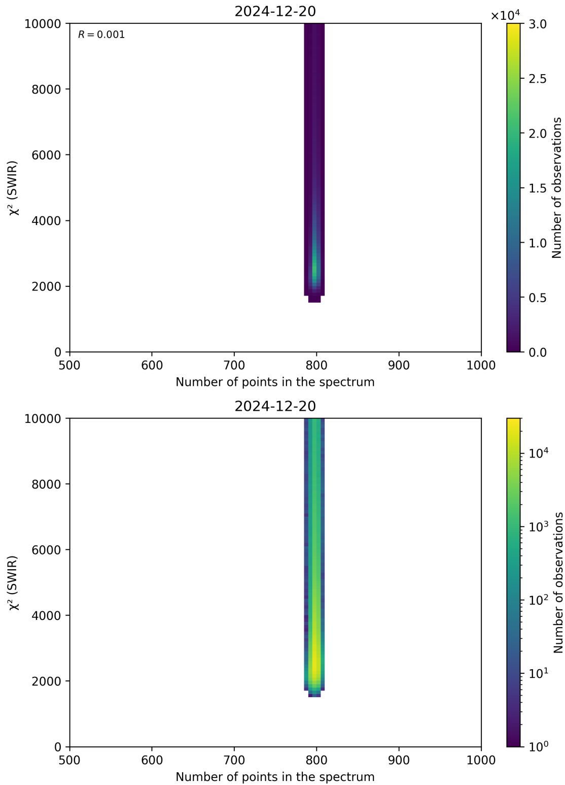
Figure 89: Scatter density plot of “Number of points in the spectrum” against “ \chi^2 (SWIR)” for 2024-12-19 to 2024-12-21.
