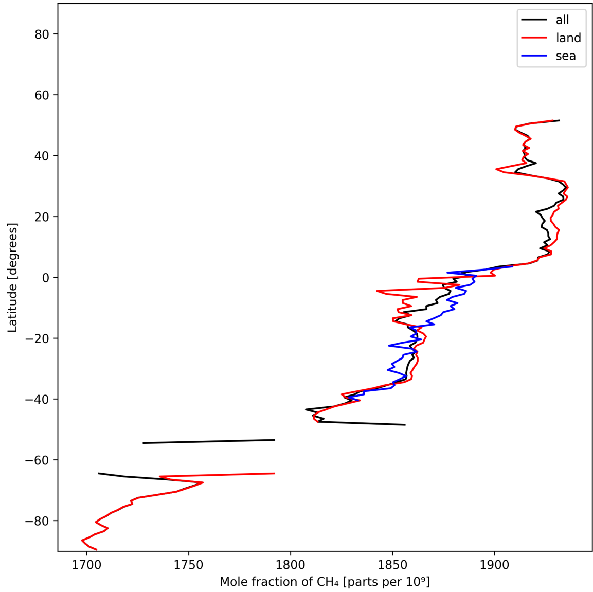
Figure 12: Zonal average of “Mole fraction of CH 4 ” for 2024-12-19 to 2024-12-21.
