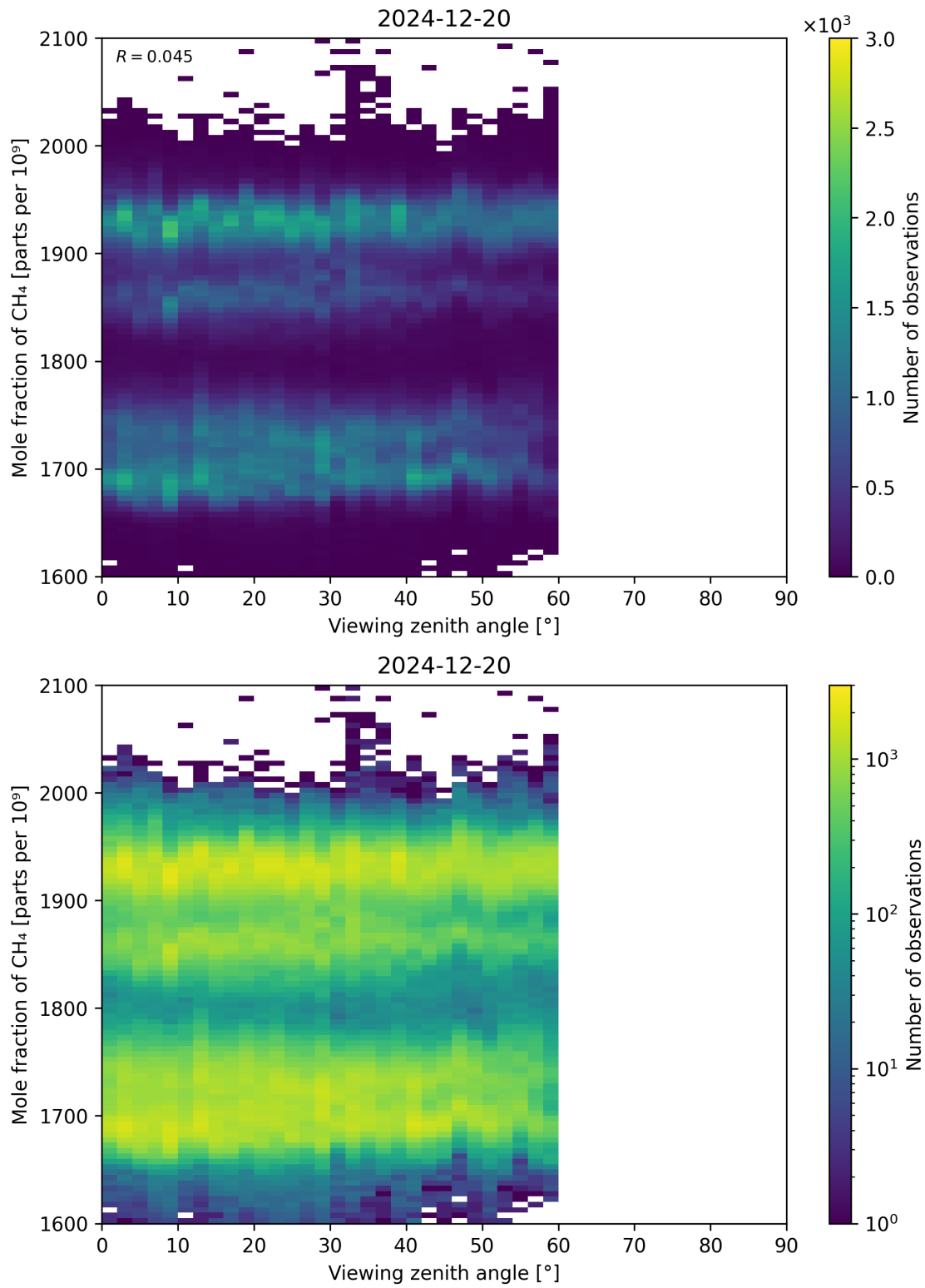
Figure 110: Scatter density plot of “Viewing zenith angle” against “Mole fraction of CH 4 ” for 2024-12-19 to 2024-12-21.
