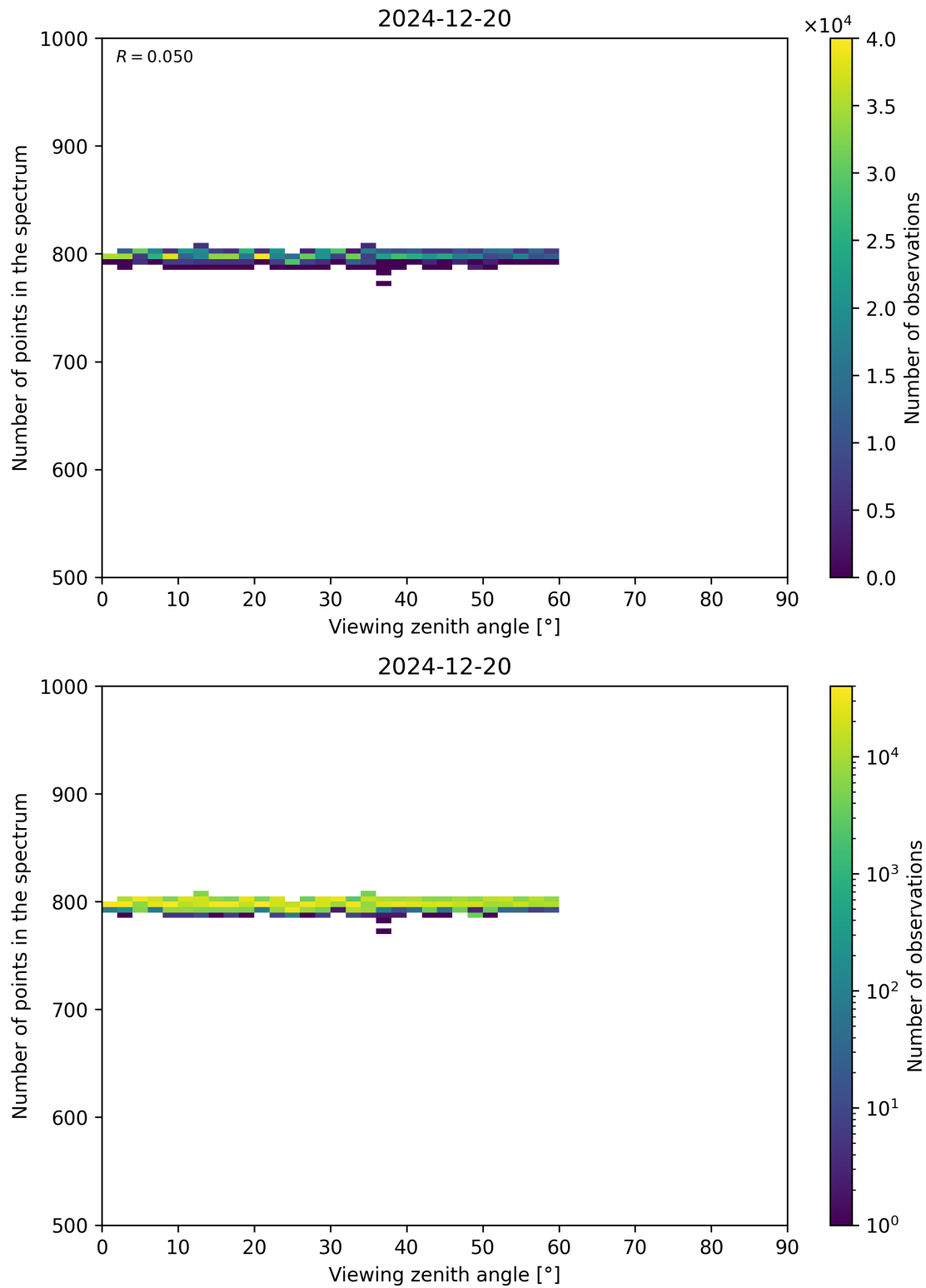
Figure 114: Scatter density plot of “Viewing zenith angle” against “Number of points in the spectrum” for 2024-12-19 to 2024-12-21.
