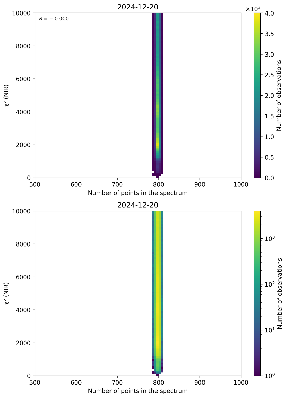
Figure 88: Scatter density plot of “Number of points in the spectrum” against “ \chi^2 (NIR)” for 2024-12-19 to 2024-12-21.
