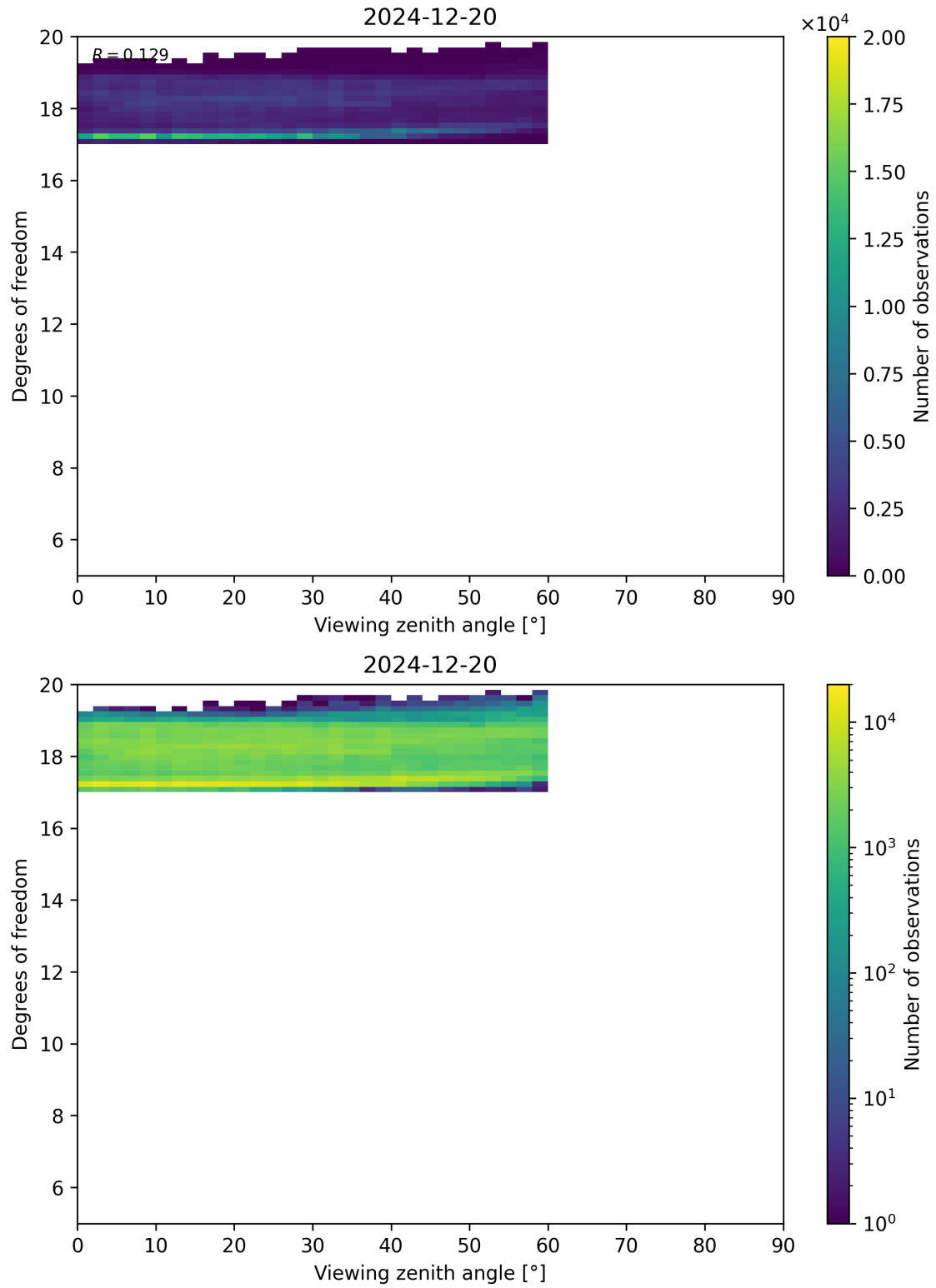
Figure 107: Scatter density plot of “Viewing zenith angle” against “Degrees of freedom” for 2024-12-19 to 2024-12-21.
