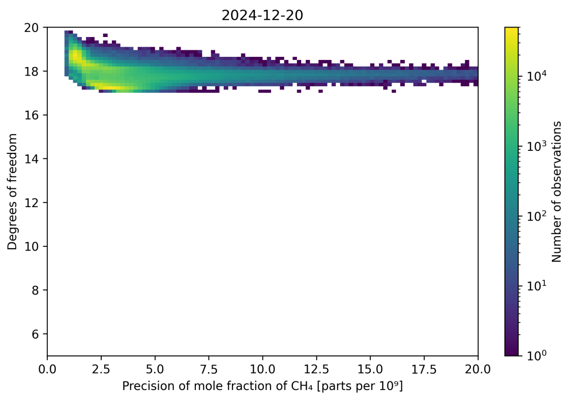
Figure 80: Scatter density plot of “Precision of mole fraction of CH 4 ” against “Degrees of freedom” for 2024-12-19 to 2024-12-21.
