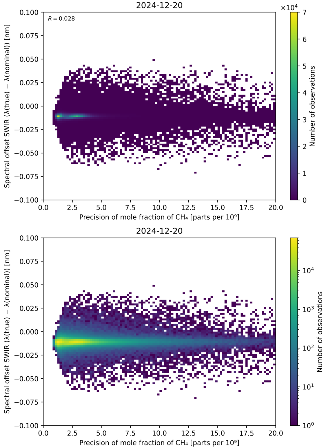
Figure 85: Scatter density plot of “Precision of mole fraction of \text{CH}_4 ” against “Spectral offset SWIR ( \lambda_{\text{true}} - \lambda_{\text{nominal}} )” for 2024-12-19 to 2024-12-21.
