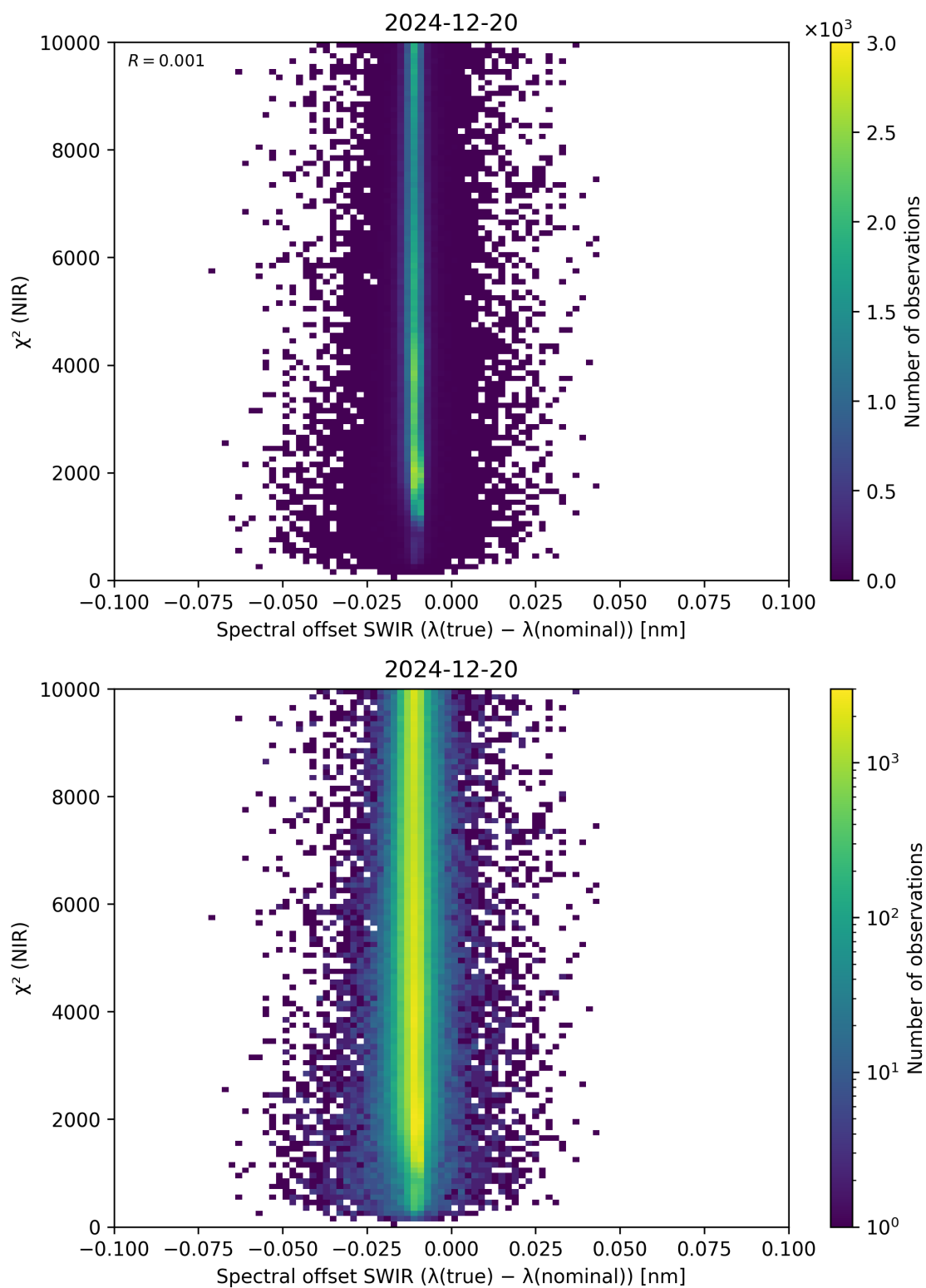
Figure 117: Scatter density plot of “Spectral offset SWIR ( \lambda_{\text{true}} - \lambda_{\text{nominal}} )” against “ \chi^2 (NIR)” for 2024-12-19 to 2024-12-21.
