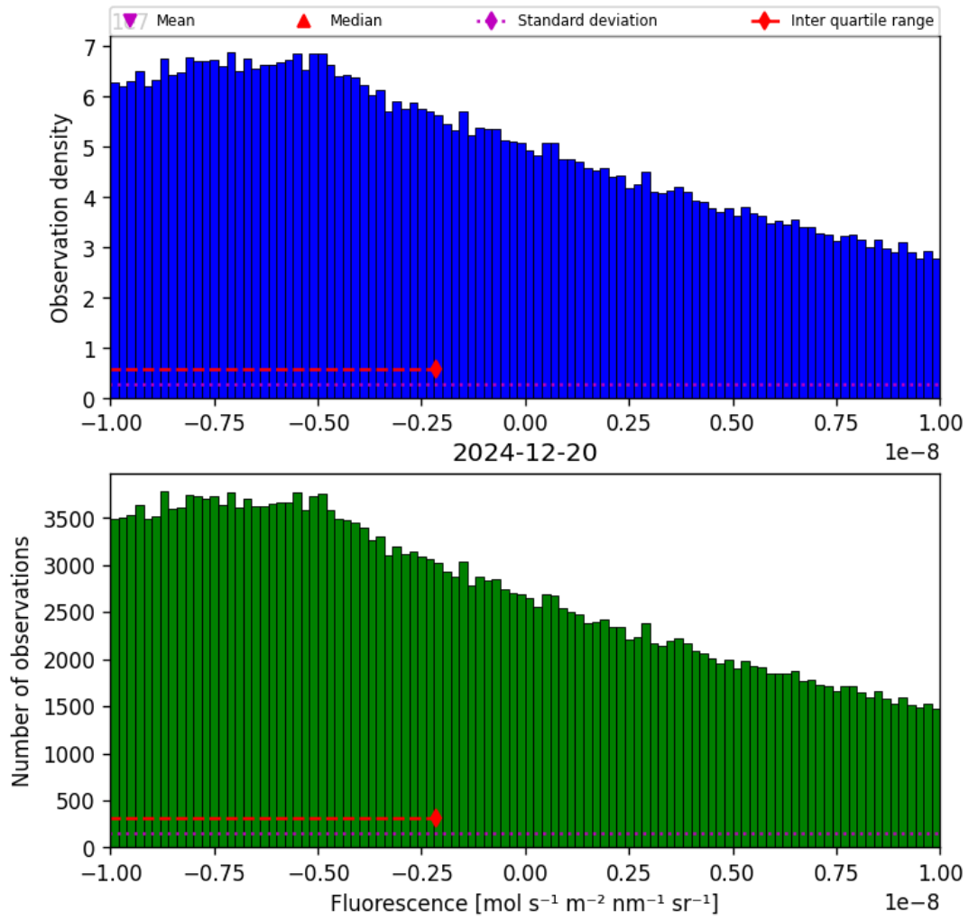
Figure 32: Histogram of “Fluorescence” for 2024-12-19 to 2024-12-21
