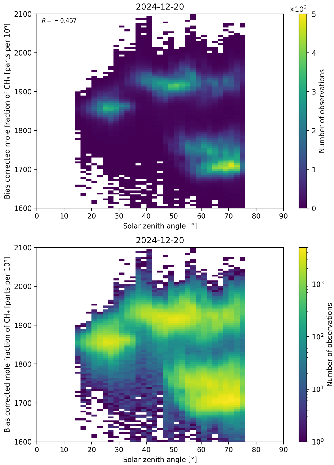
Figure 100: Scatter density plot of “Solar zenith angle” against “Bias corrected mole fraction of CH 4 ” for 2024-12-19 to 2024-12-21.
