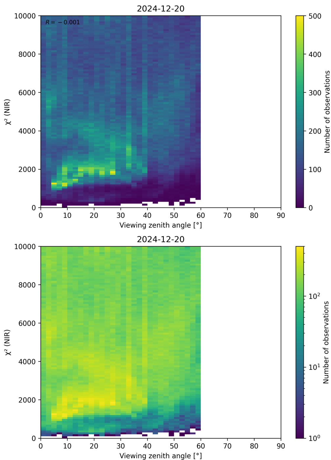
Figure 105: Scatter density plot of “Viewing zenith angle” against “ \chi^2 (NIR)” for 2024-12-19 to 2024-12-21.
