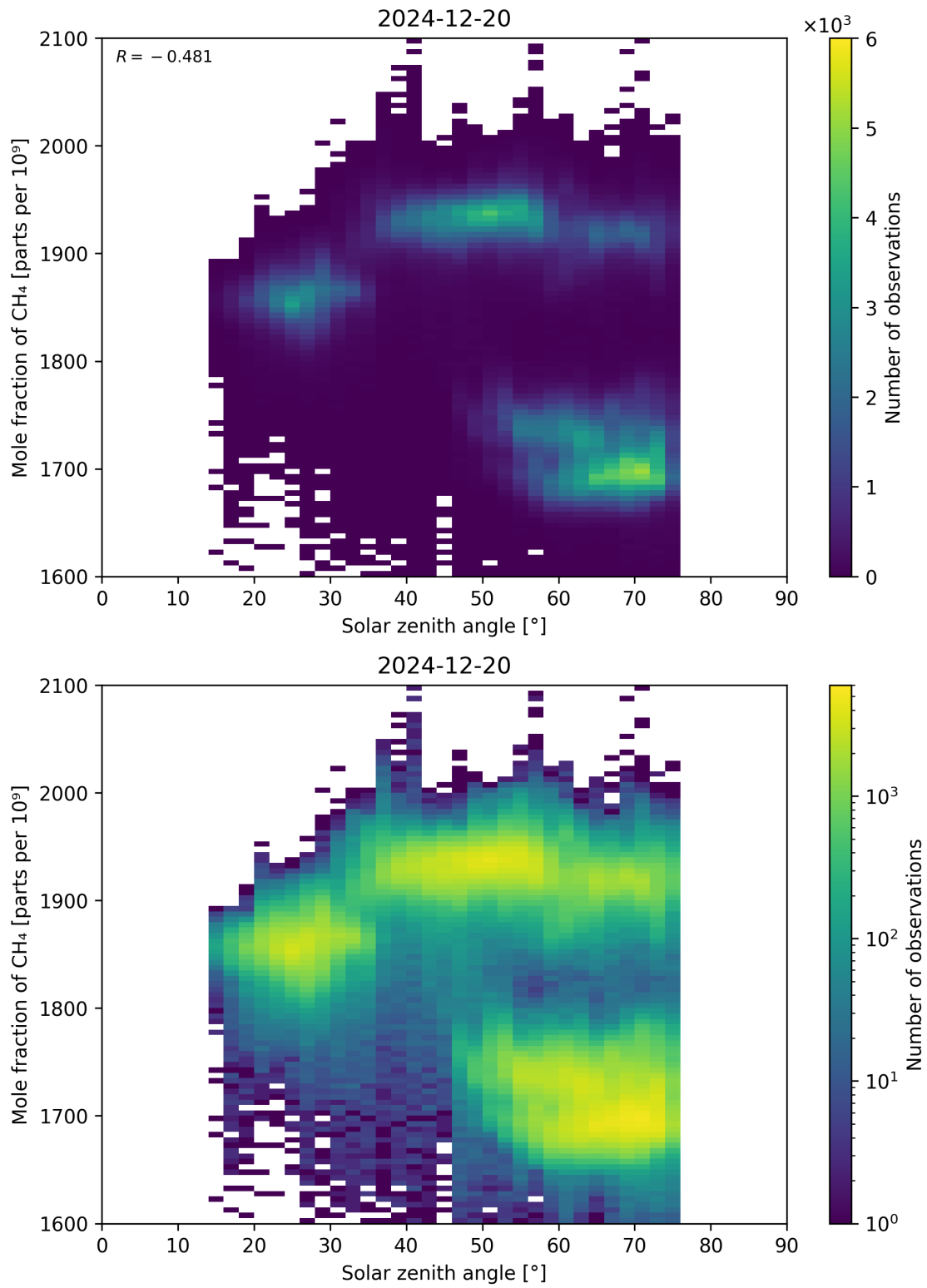
Figure 99: Scatter density plot of “Solar zenith angle” against “Mole fraction of \text{CH}_4 ” for 2024-12-19 to 2024-12-21.
