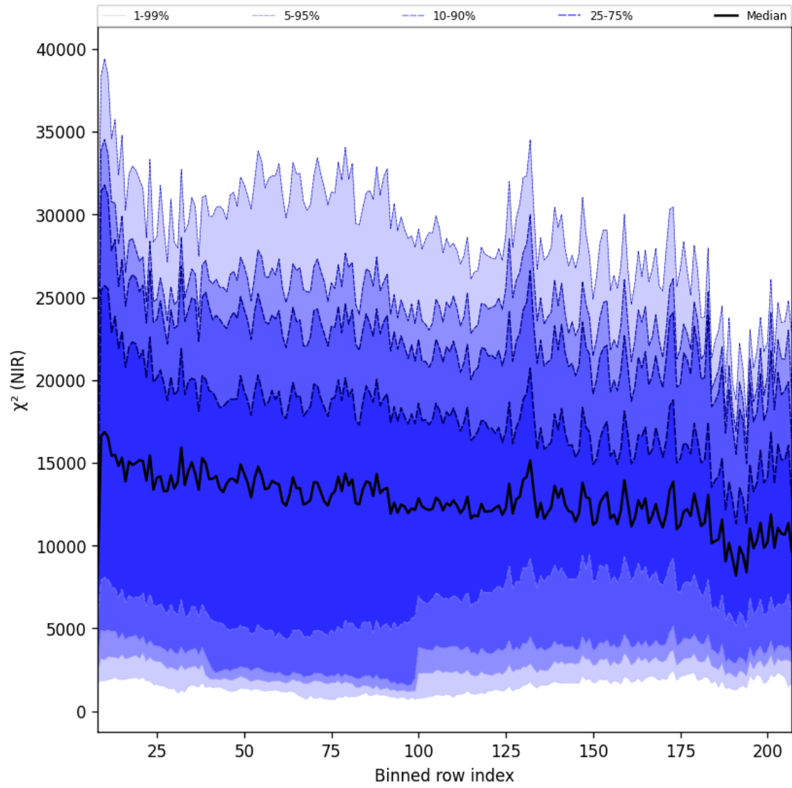
Figure 40: Along track statistics of “ \chi^2 (NIR)” for 2024-12-19 to 2024-12-21
