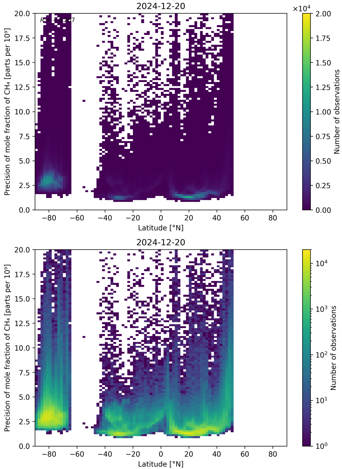
Figure 59: Scatter density plot of “Latitude” against “Precision of mole fraction of CH 4 ” for 2024-12-19 to 2024-12-21.
