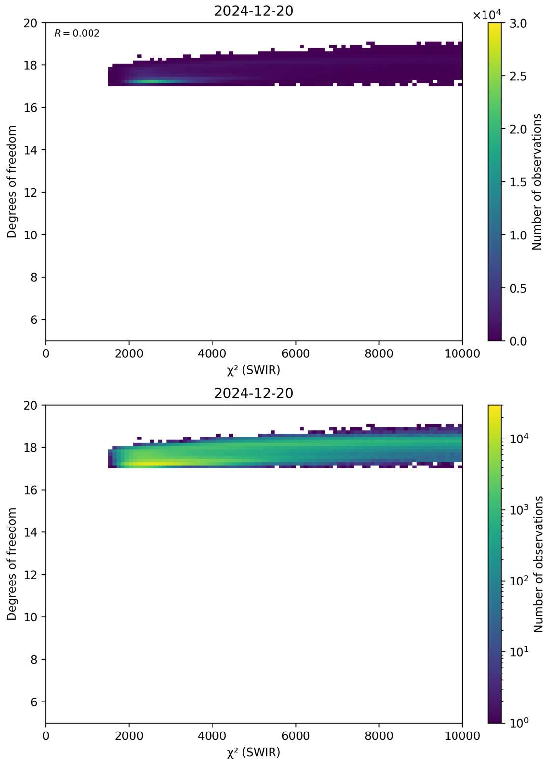
Figure 48: Scatter density plot of “ \chi^2 (SWIR)” against “Degrees of freedom” for 2024-12-19 to 2024-12-21.
