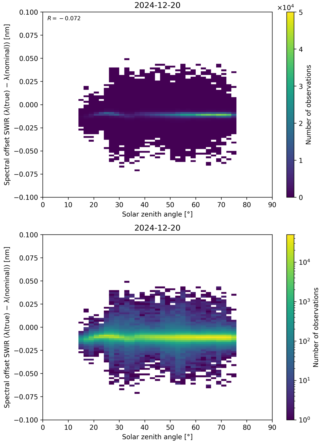
Figure 104: Scatter density plot of “Solar zenith angle” against “Spectral offset SWIR ( \lambda_{\text{true}} - \lambda_{\text{nominal}} )” for 2024-12-19 to 2024-12-21.
