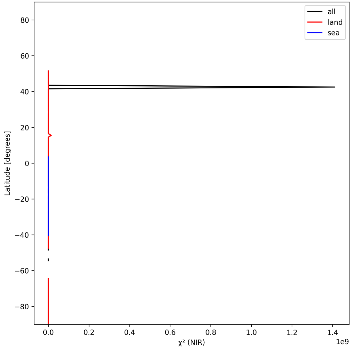
Figure 18: Zonal average of “ \chi^2 (NIR)” for 2024-12-19 to 2024-12-21.
