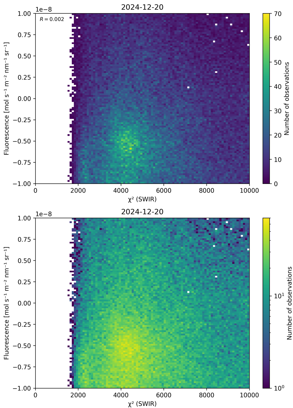
Figure 49: Scatter density plot of “ \chi^2 (SWIR)” against “Fluorescence” for 2024-12-19 to 2024-12-21.
