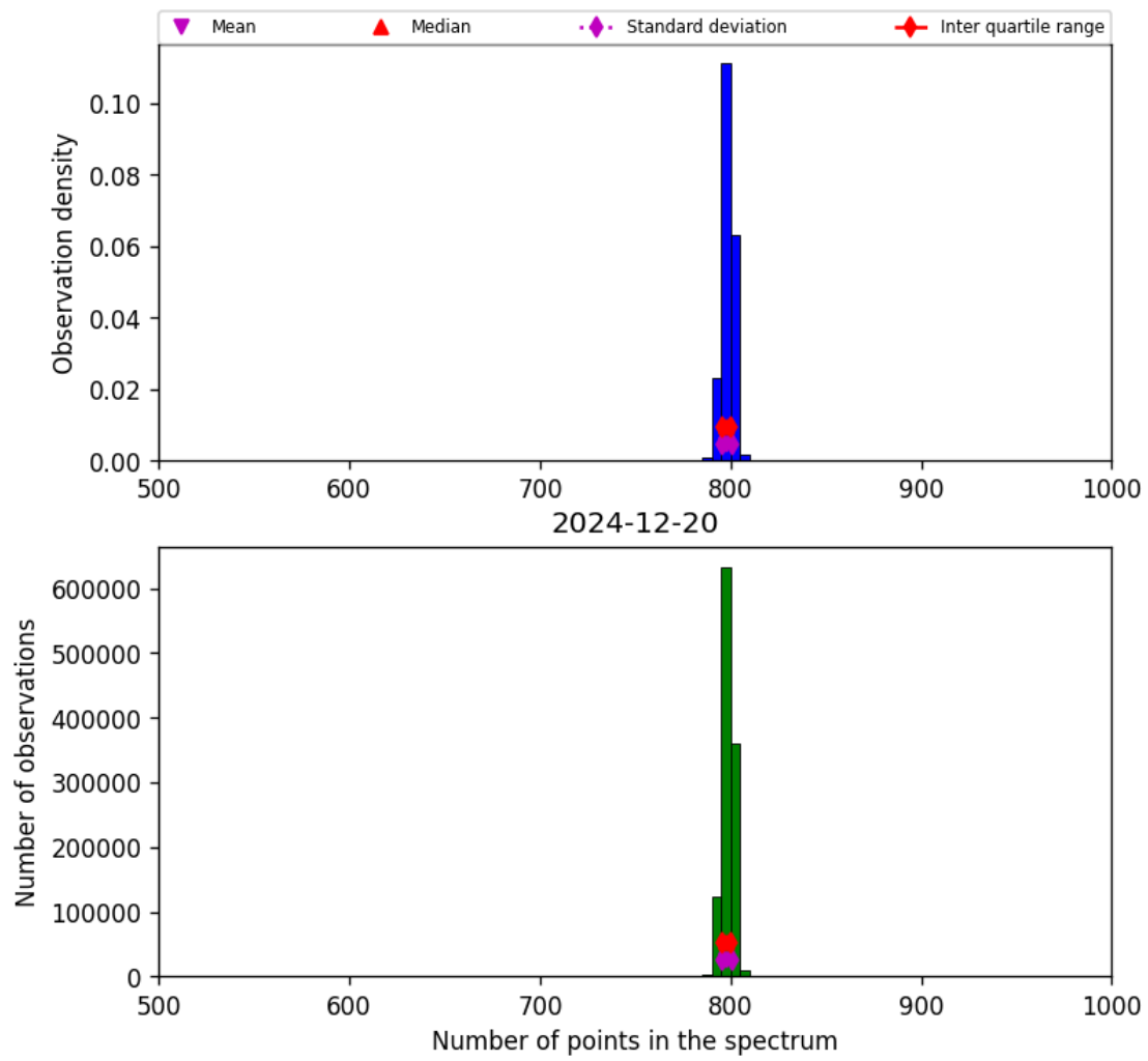
Figure 26: Histogram of “Number of points in the spectrum” for 2024-12-19 to 2024-12-21
