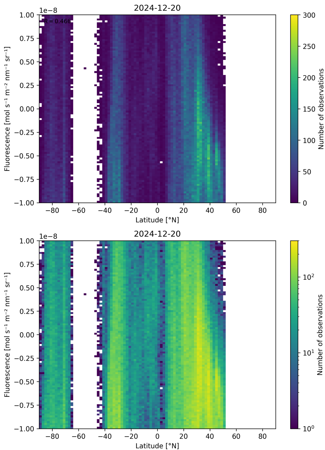
Figure 56: Scatter density plot of “Latitude” against “Fluorescence” for 2024-12-19 to 2024-12-21.
