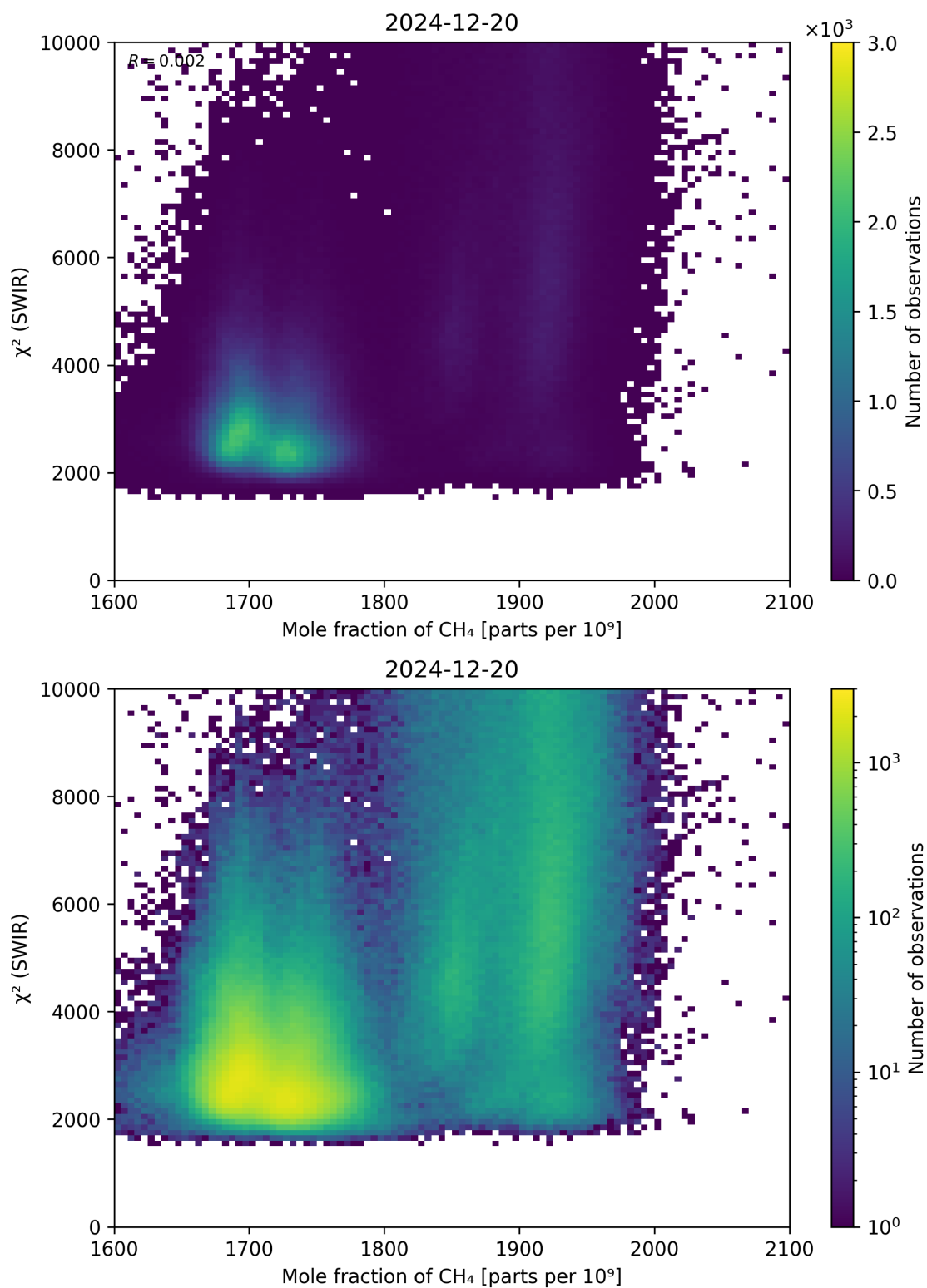
Figure 71: Scatter density plot of “Mole fraction of CH 4 ” against “ \chi^2 (SWIR)” for 2024-12-19 to 2024-12-21.
