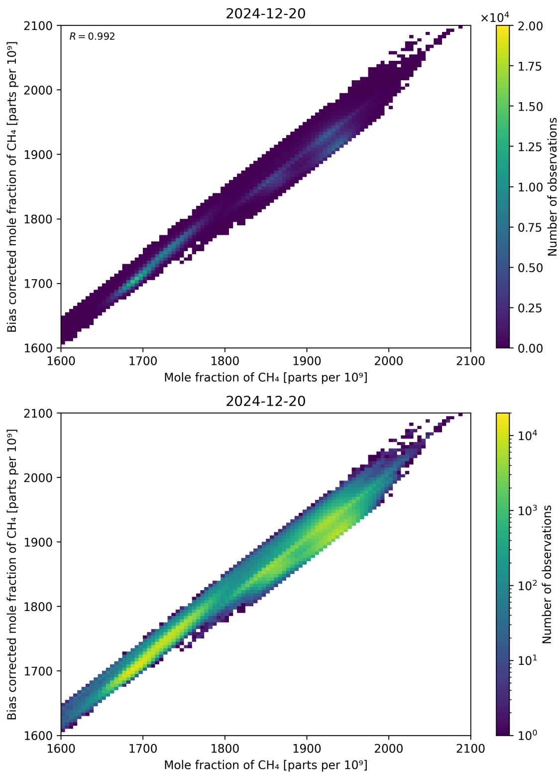
Figure 74: Scatter density plot of “Mole fraction of CH 4 ” against “Bias corrected mole fraction of CH 4 ” for 2024-12-19 to 2024-12-21.
