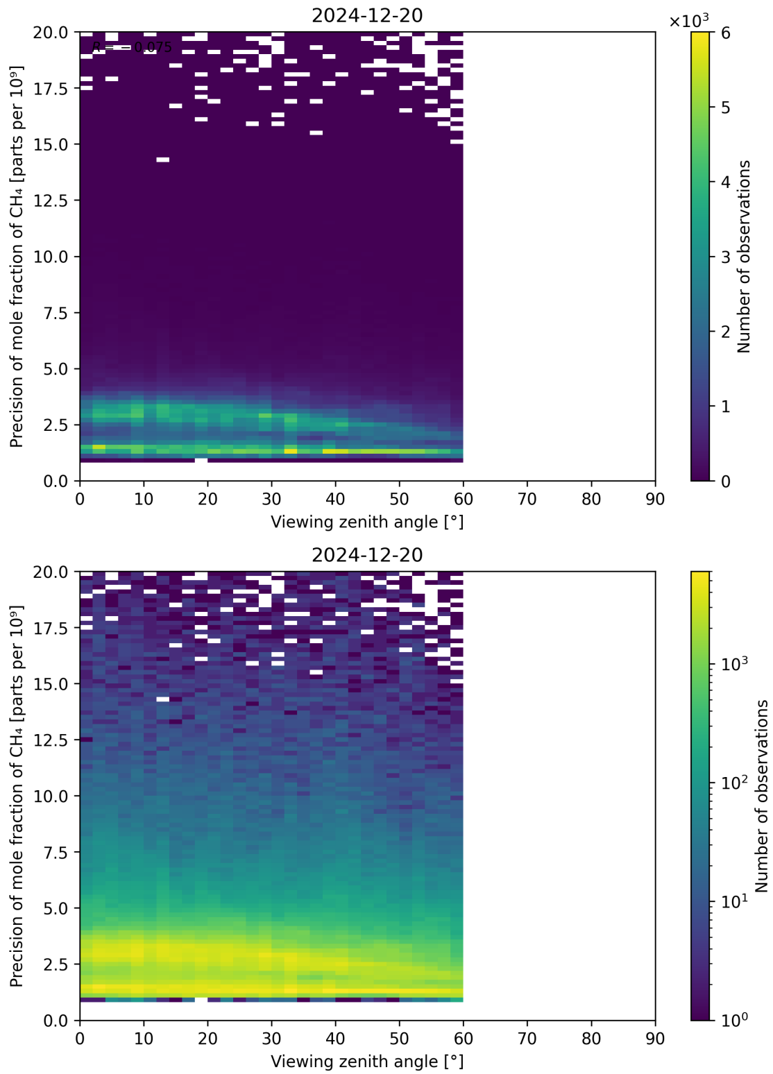
Figure 112: Scatter density plot of “Viewing zenith angle” against “Precision of mole fraction of CH 4 ” for 2024-12-19 to 2024-12-21.
