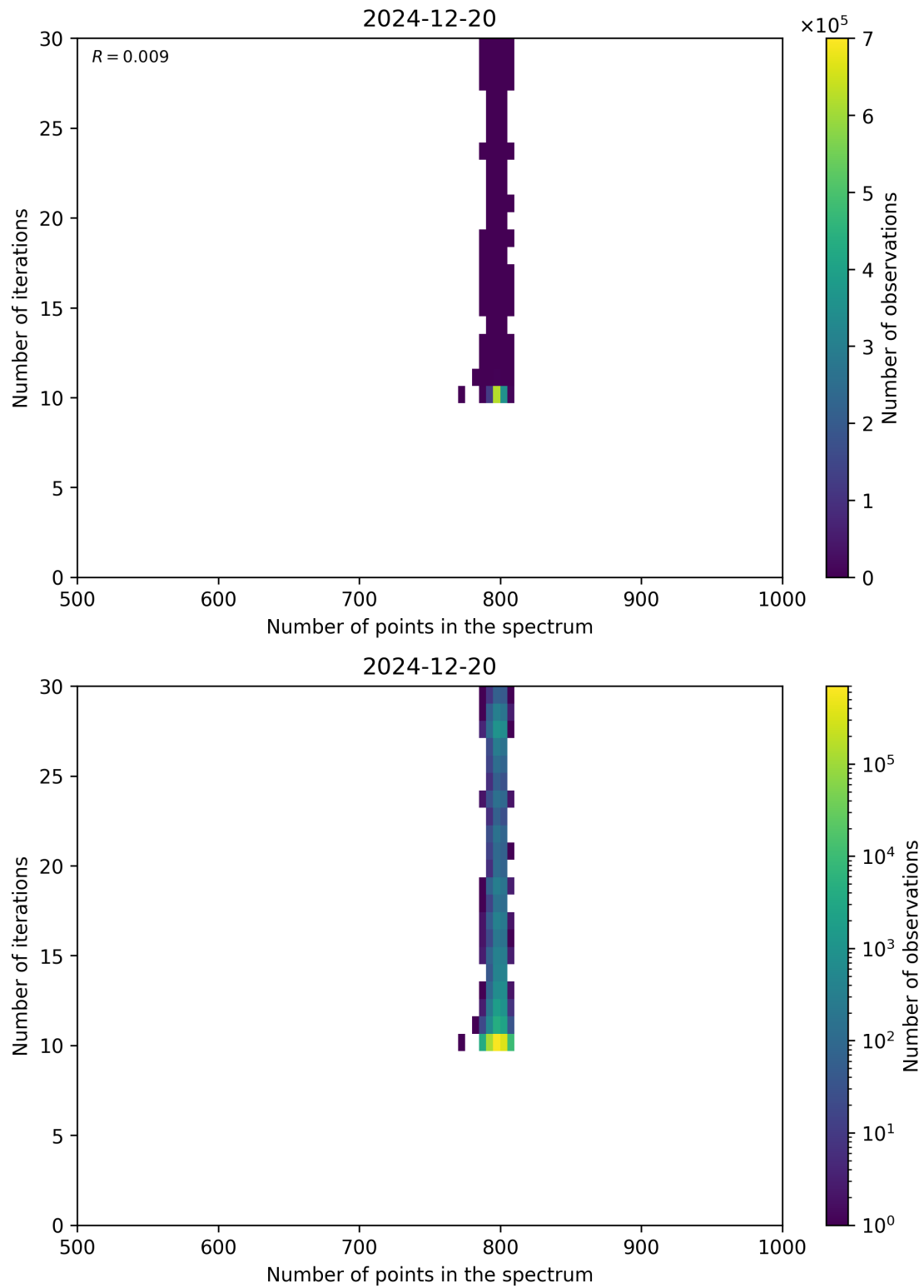
Figure 92: Scatter density plot of “Number of points in the spectrum” against “Number of iterations” for 2024-12-19 to 2024-12-21.
