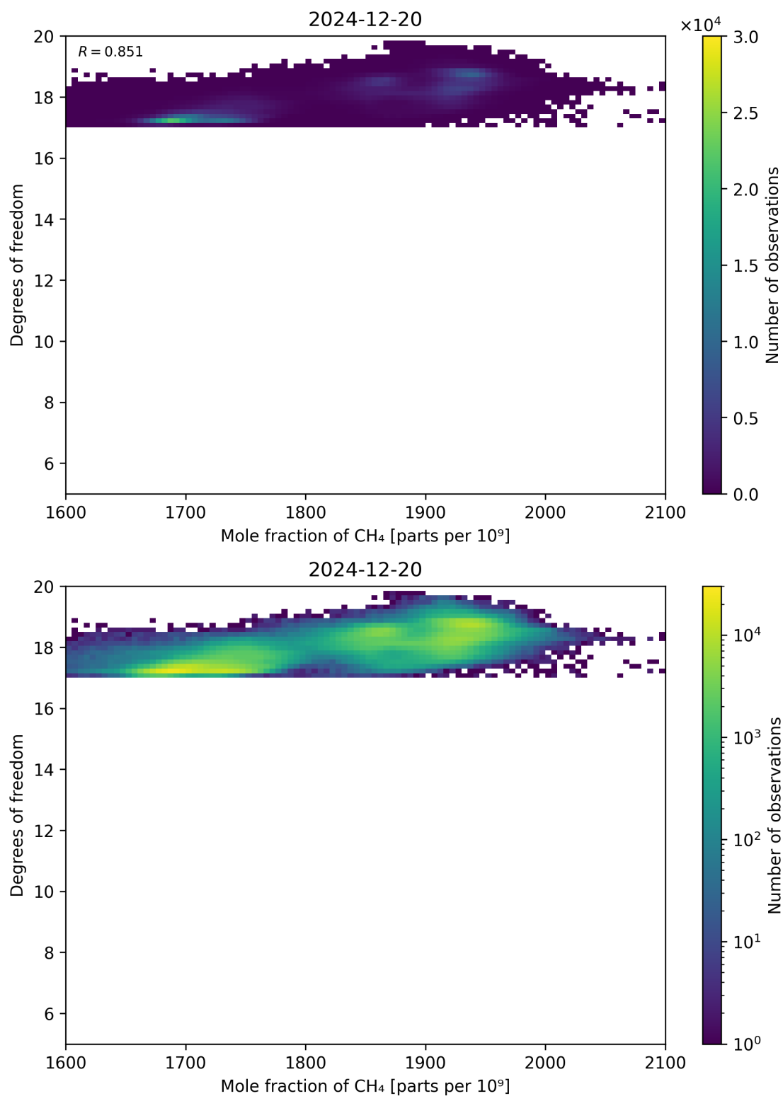
Figure 72: Scatter density plot of “Mole fraction of CH 4 ” against “Degrees of freedom” for 2024-12-19 to 2024-12-21.
