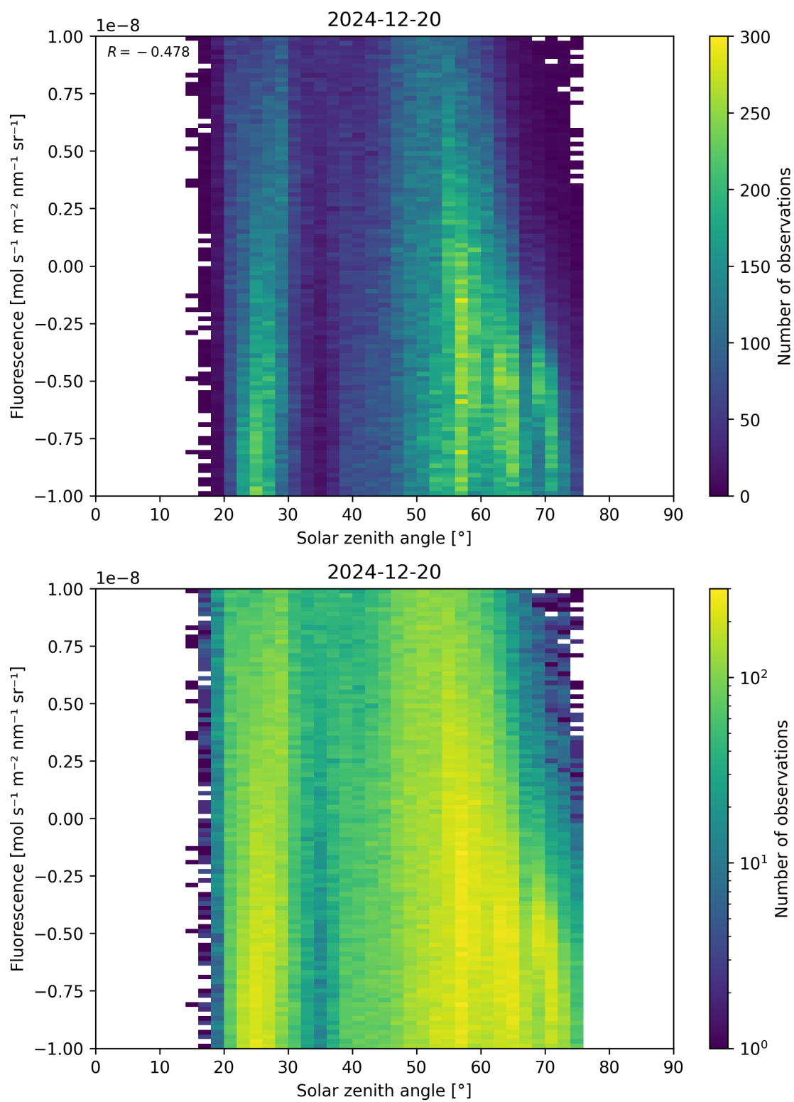
Figure 97: Scatter density plot of “Solar zenith angle” against “Fluorescence” for 2024-12-19 to 2024-12-21.
