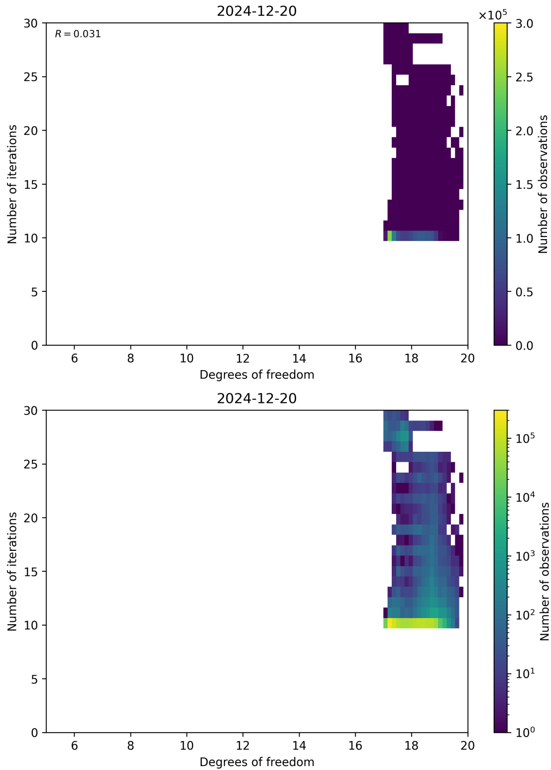
Figure 52: Scatter density plot of “Degrees of freedom” against “Number of iterations” for 2024-12-19 to 2024-12-21.
