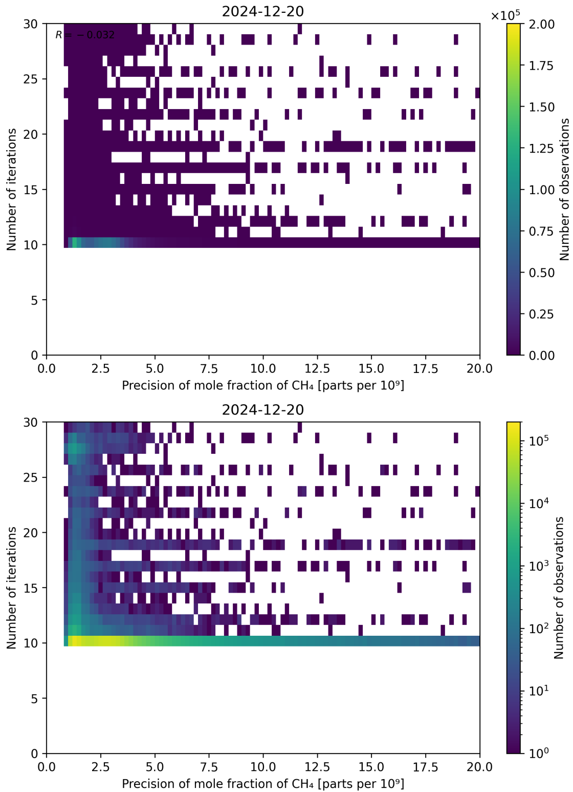
Figure 83: Scatter density plot of “Precision of mole fraction of CH 4 ” against “Number of iterations” for 2024-12-19 to 2024-12-21.
