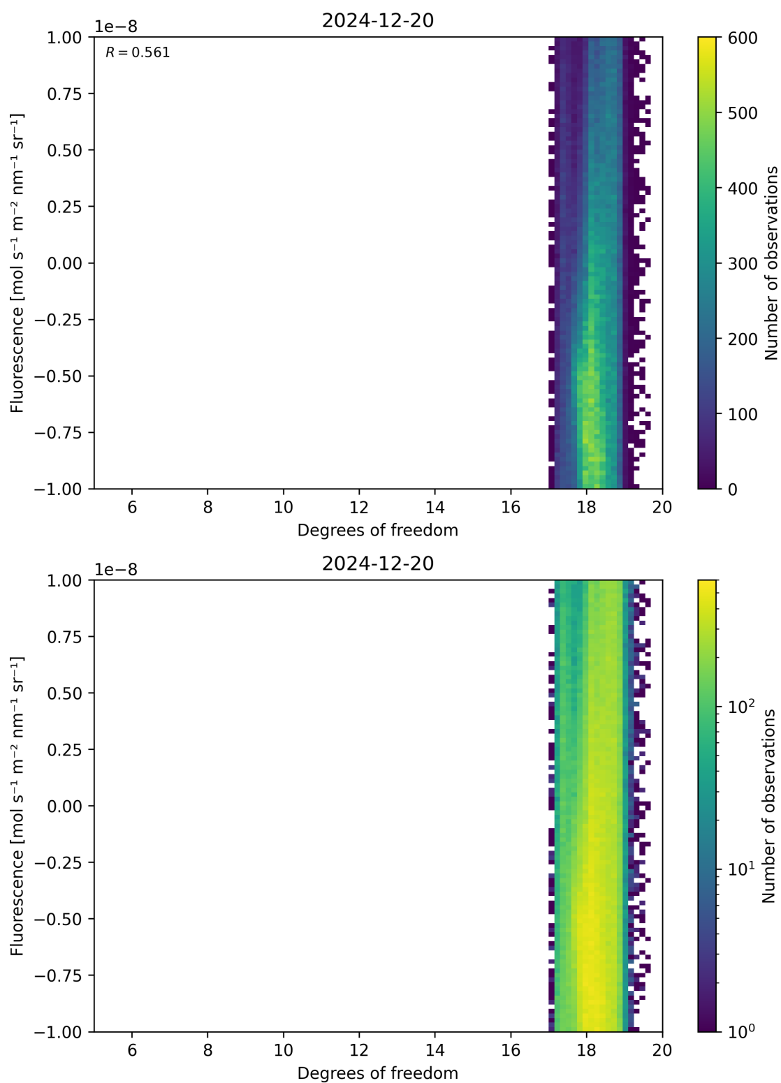
Figure 51: Scatter density plot of “Degrees of freedom” against “Fluorescence” for 2024-12-19 to 2024-12-21.
