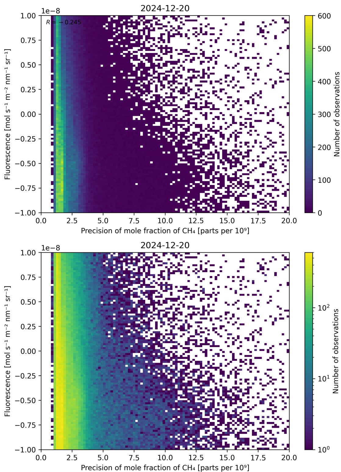
Figure 81: Scatter density plot of “Precision of mole fraction of \text{CH}_4 ” against “Fluorescence” for 2024-12-19 to 2024-12-21.
