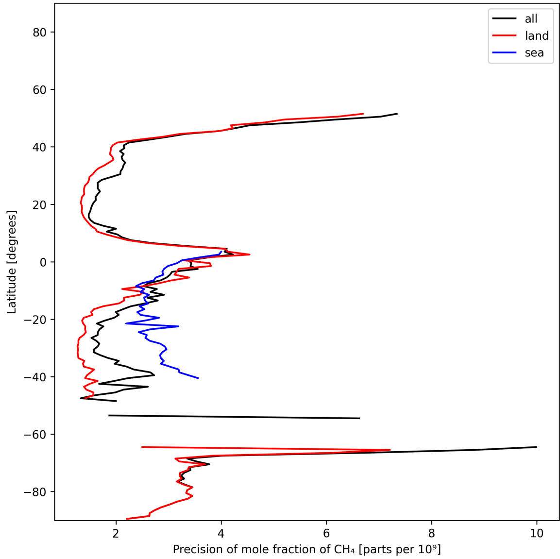
Figure 13: Zonal average of “Precision of mole fraction of CH 4 ” for 2024-12-19 to 2024-12-21.
