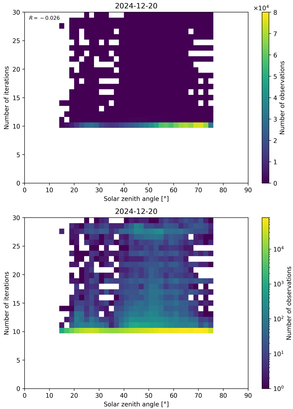
Figure 102: Scatter density plot of “Solar zenith angle” against “Number of iterations” for 2024-12-19 to 2024-12-21.
