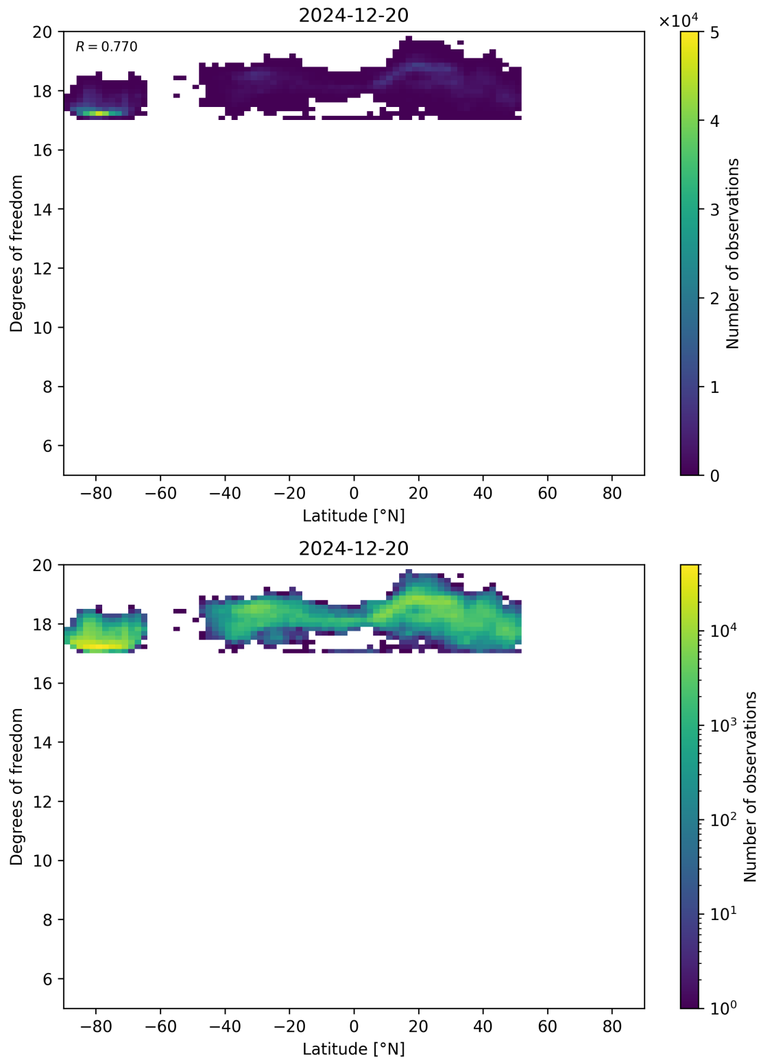
Figure 55: Scatter density plot of “Latitude” against “Degrees of freedom” for 2024-12-19 to 2024-12-21.
