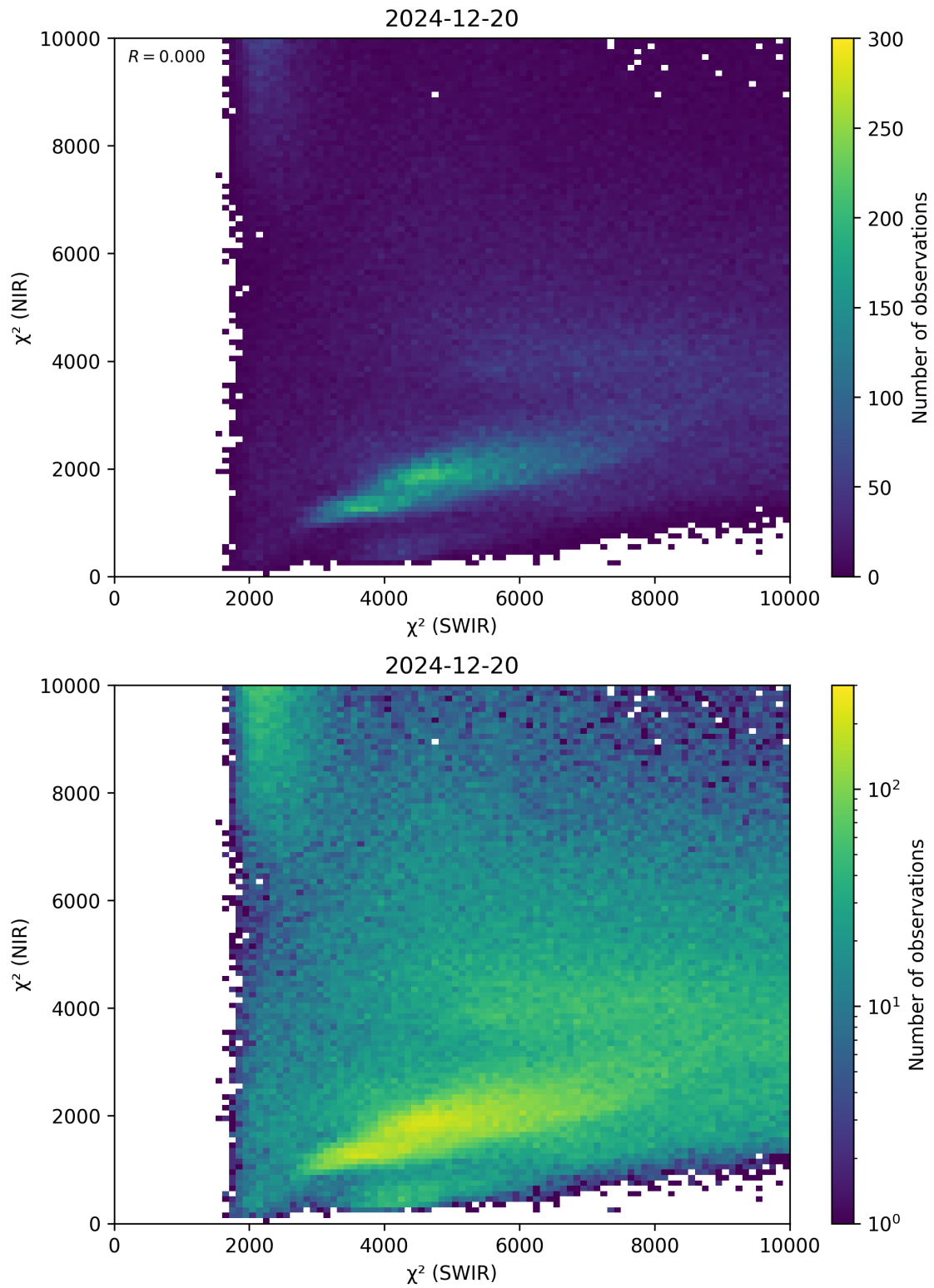
Figure 47: Scatter density plot of “ \chi^2 (SWIR)” against “ \chi^2 (NIR)” for 2024-12-19 to 2024-12-21.
