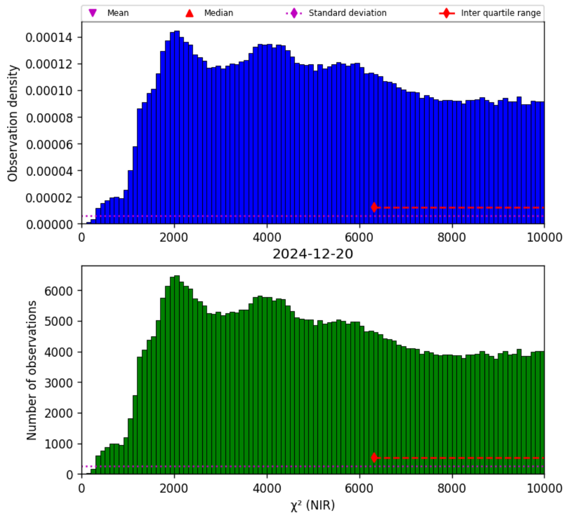
Figure 29: Histogram of “ \chi^2 (NIR)” for 2024-12-19 to 2024-12-21
