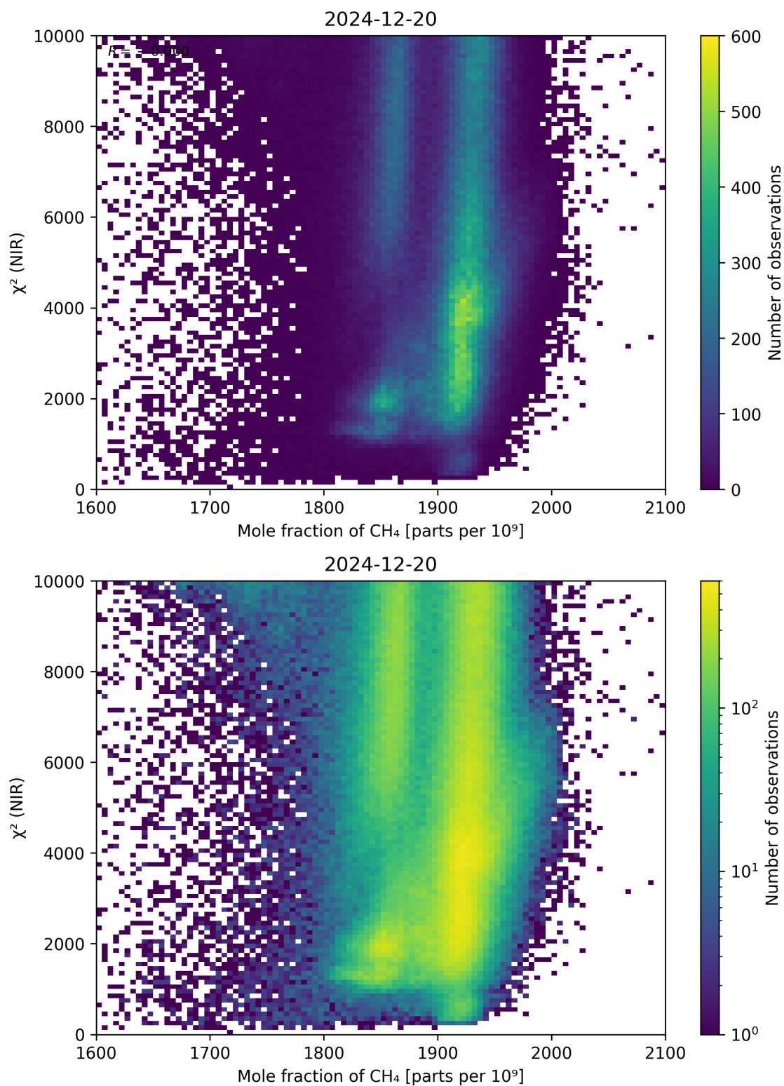
Figure 70: Scatter density plot of “Mole fraction of \text{CH}_4 ” against “ \chi^2 (NIR)” for 2024-12-19 to 2024-12-21.
