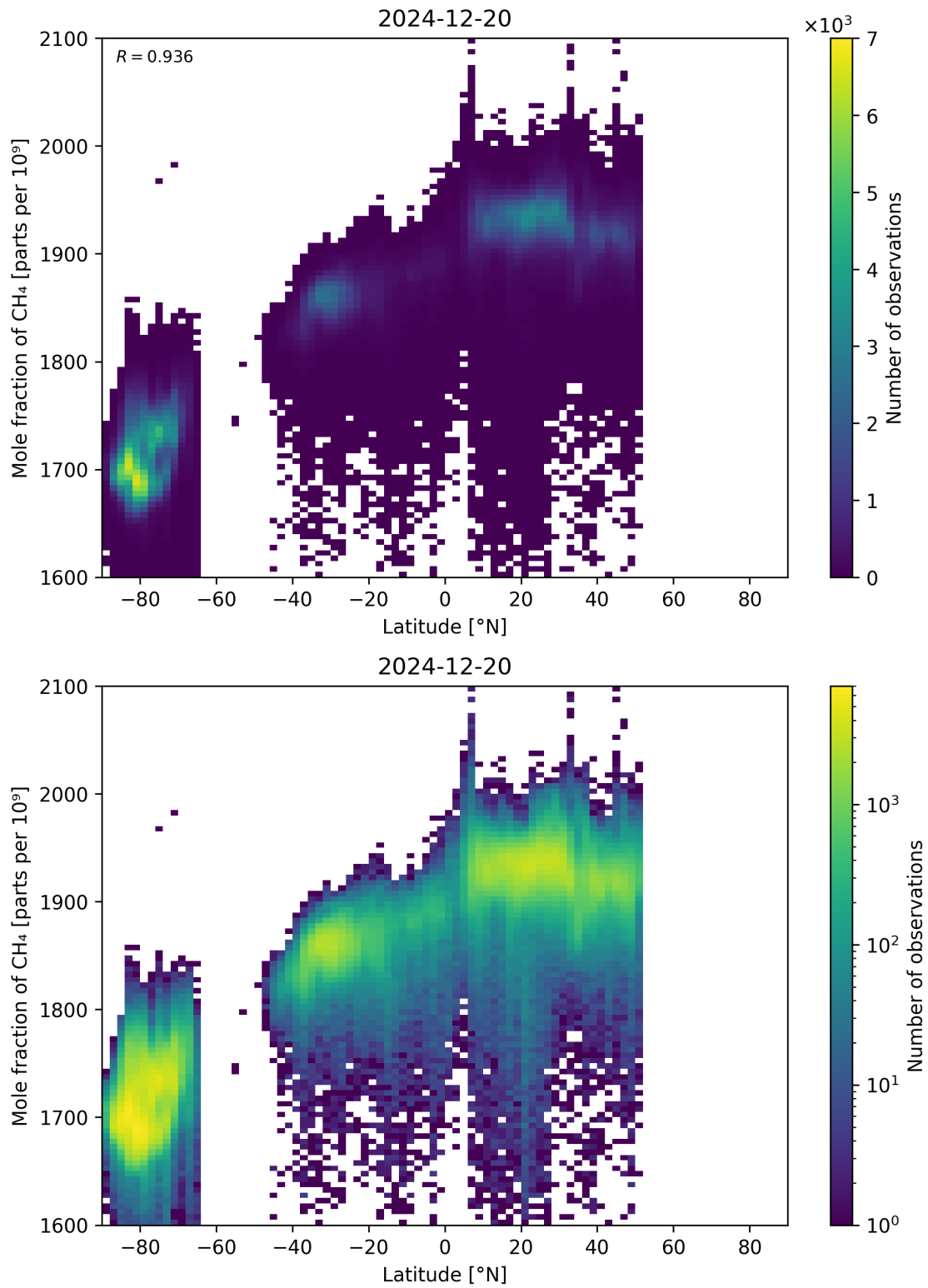
Figure 57: Scatter density plot of “Latitude” against “Mole fraction of CH 4 ” for 2024-12-19 to 2024-12-21.
