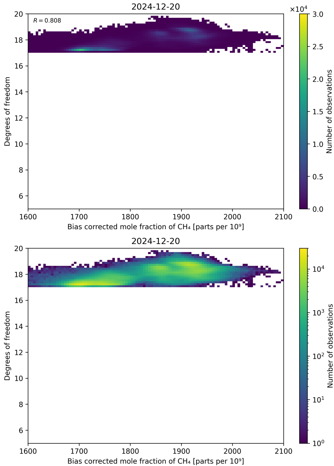
Figure 65: Scatter density plot of “Bias corrected mole fraction of CH 4 ” against “Degrees of freedom” for 2024-12-19 to 2024-12-21.
