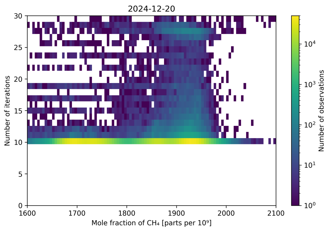
Figure 76: Scatter density plot of “Mole fraction of CH 4 ” against “Number of iterations” for 2024-12-19 to 2024-12-21.
