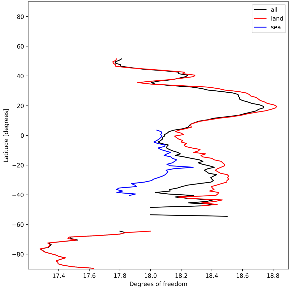
Figure 19: Zonal average of “Degrees of freedom” for 2024-12-19 to 2024-12-21.
