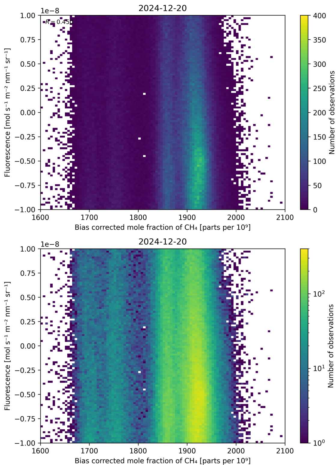
Figure 66: Scatter density plot of “Bias corrected mole fraction of \text{CH}_4 ” against “Fluorescence” for 2024-12-19 to 2024-12-21.
