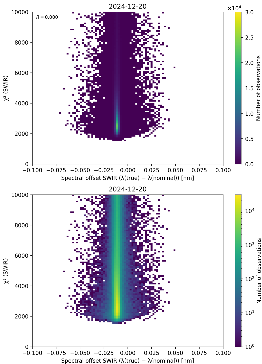
Figure 118: Scatter density plot of “Spectral offset SWIR ( \lambda_{\text{true}} - \lambda_{\text{nominal}} )” against “ \chi^2 (SWIR)” for 2024-12-19 to 2024-12-21.
