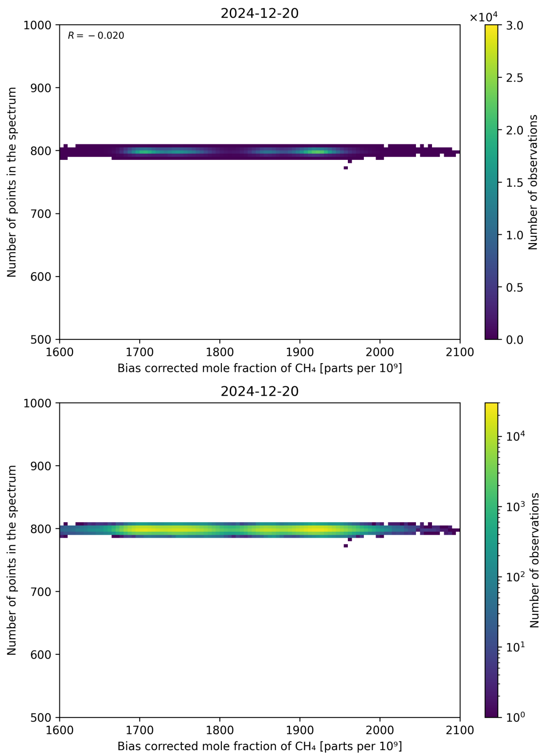
Figure 68: Scatter density plot of “Bias corrected mole fraction of CH 4 ” against “Number of points in the spectrum” for 2024-12-19 to 2024-12-21.
