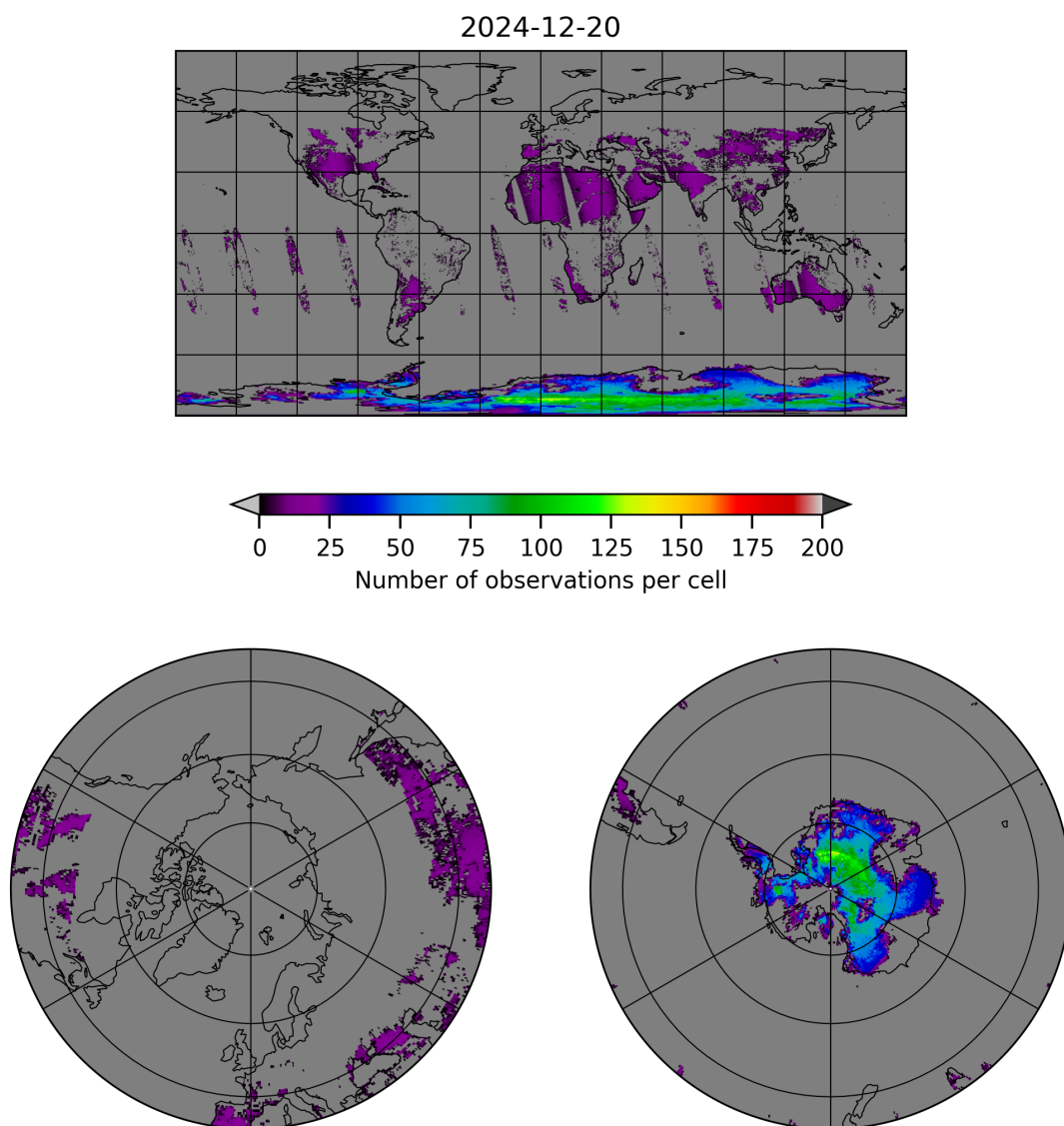
Figure 10: Map of the number of observations for 2024-12-19 to 2024-12-21
