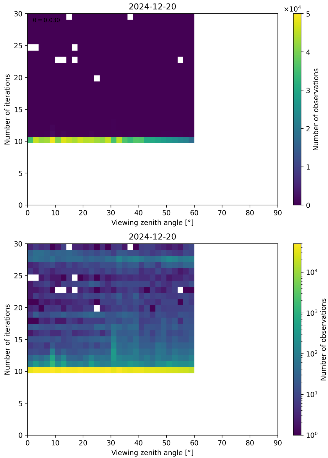
Figure 113: Scatter density plot of “Viewing zenith angle” against “Number of iterations” for 2024-12-19 to 2024-12-21.
