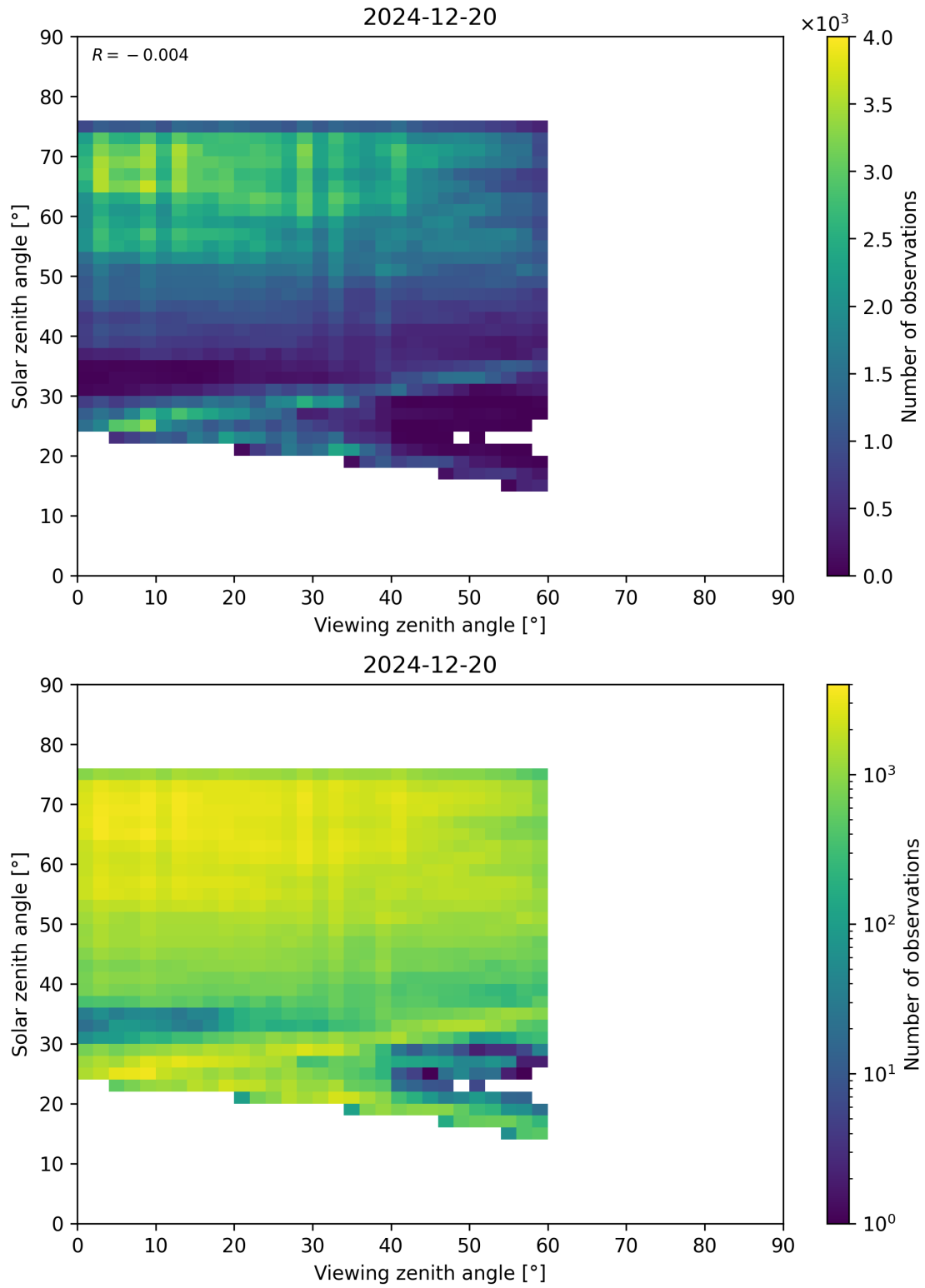
Figure 115: Scatter density plot of “Viewing zenith angle” against “Solar zenith angle” for 2024-12-19 to 2024-12-21.
