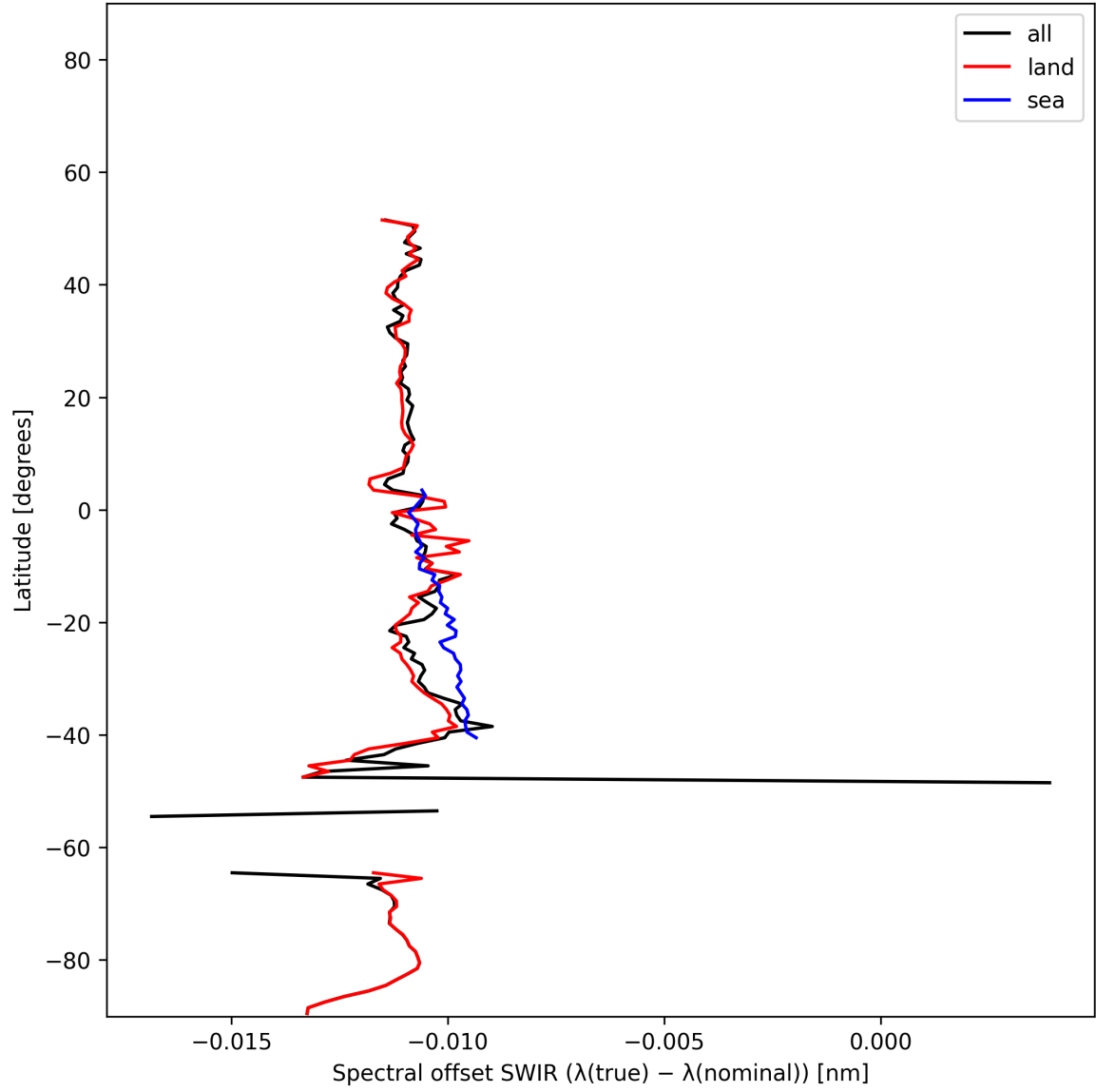
Figure 16: Zonal average of “Spectral offset SWIR ( \lambda_{\text{true}} - \lambda_{\text{nominal}} )” for 2024-12-19 to 2024-12-21.
