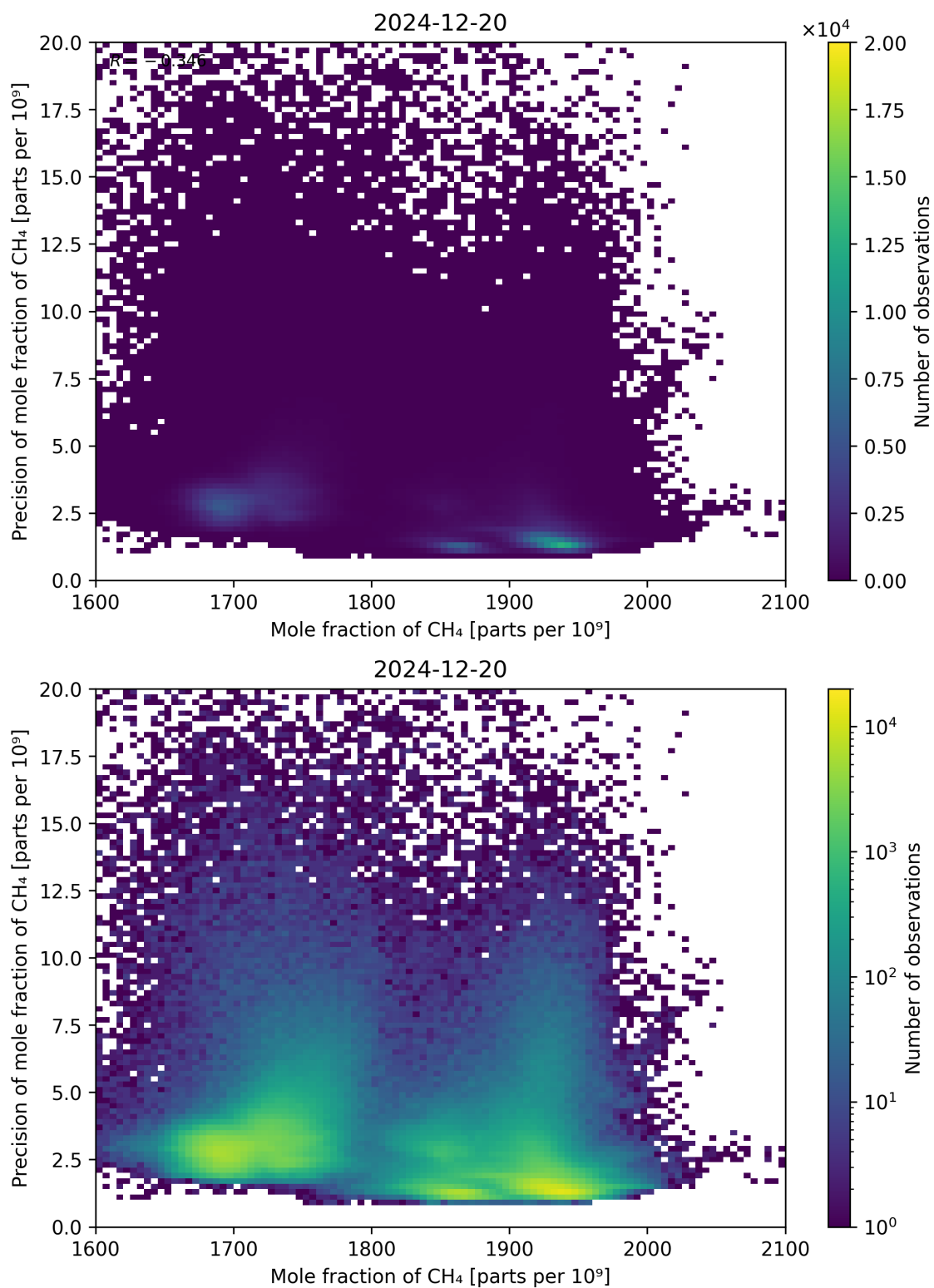
Figure 75: Scatter density plot of “Mole fraction of CH 4 ” against “Precision of mole fraction of CH 4 ” for 2024-12-19 to 2024-12-21.
