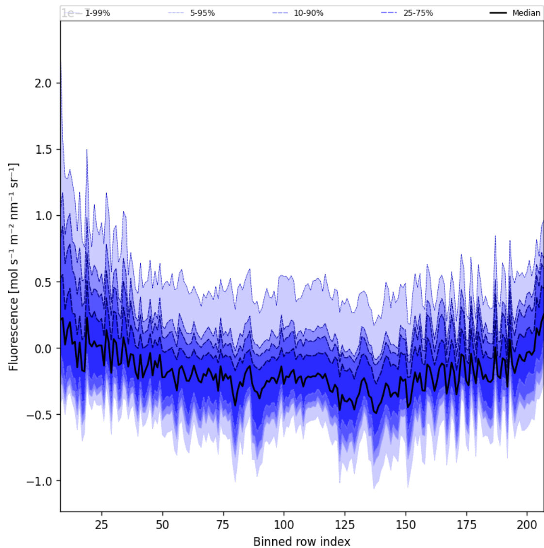
Figure 43: Along track statistics of “Fluorescence” for 2024-12-19 to 2024-12-21
