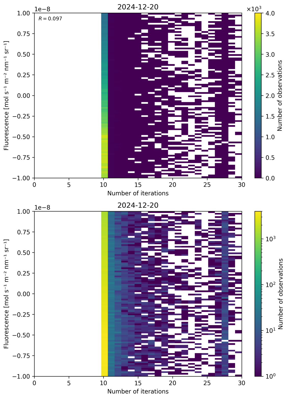
Figure 87: Scatter density plot of “Number of iterations” against “Fluorescence” for 2024-12-19 to 2024-12-21.
