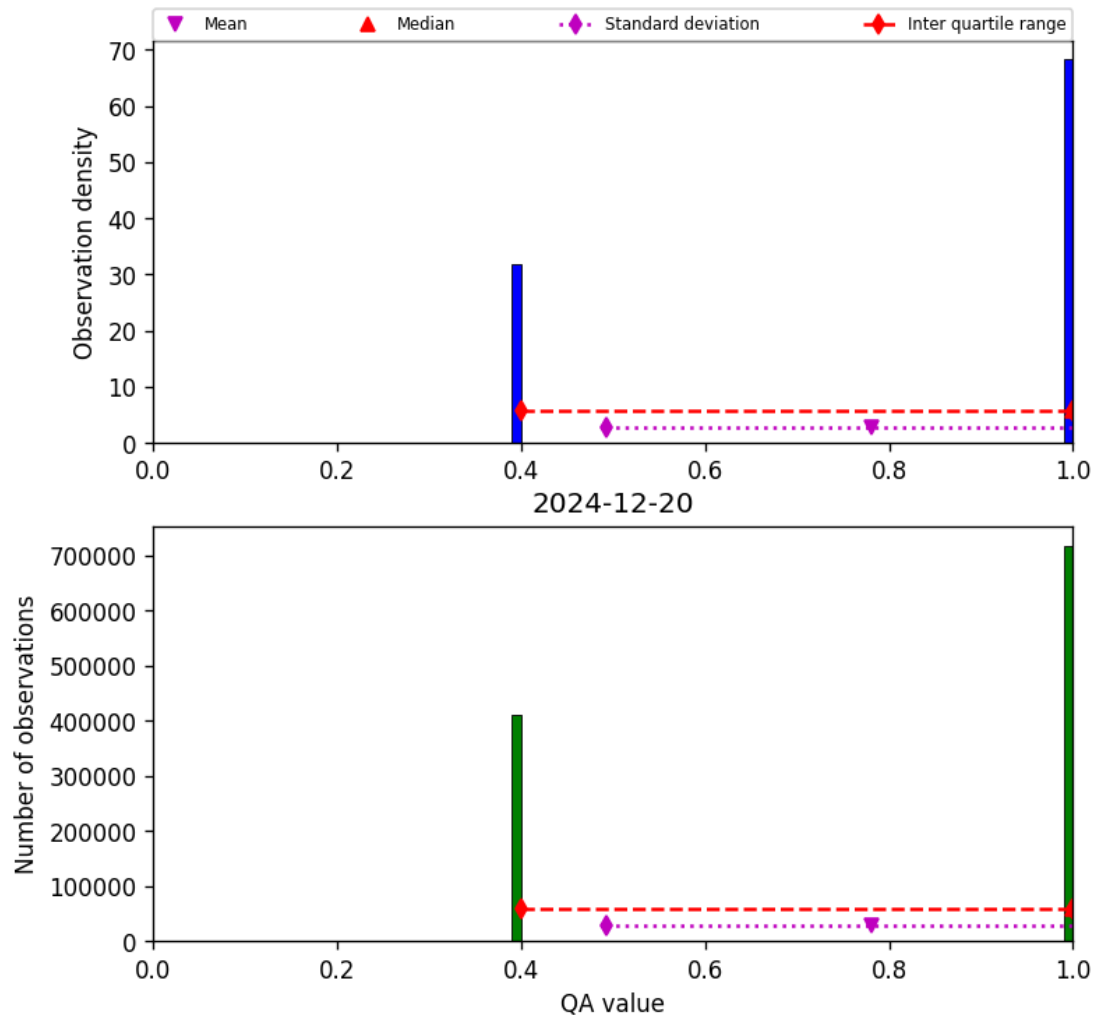
Figure 22: Histogram of “QA value” for 2024-12-19 to 2024-12-21
