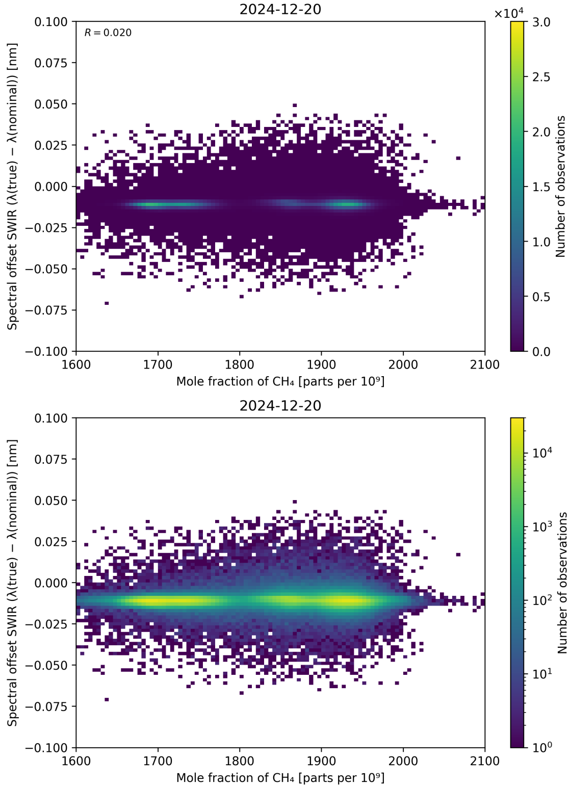
Figure 86: Scatter density plot of “Mole fraction of \text{CH}_4 ” against “Spectral offset SWIR ( \lambda_{\text{true}} - \lambda_{\text{nominal}} )” for 2024-12-19 to 2024-12-21.
