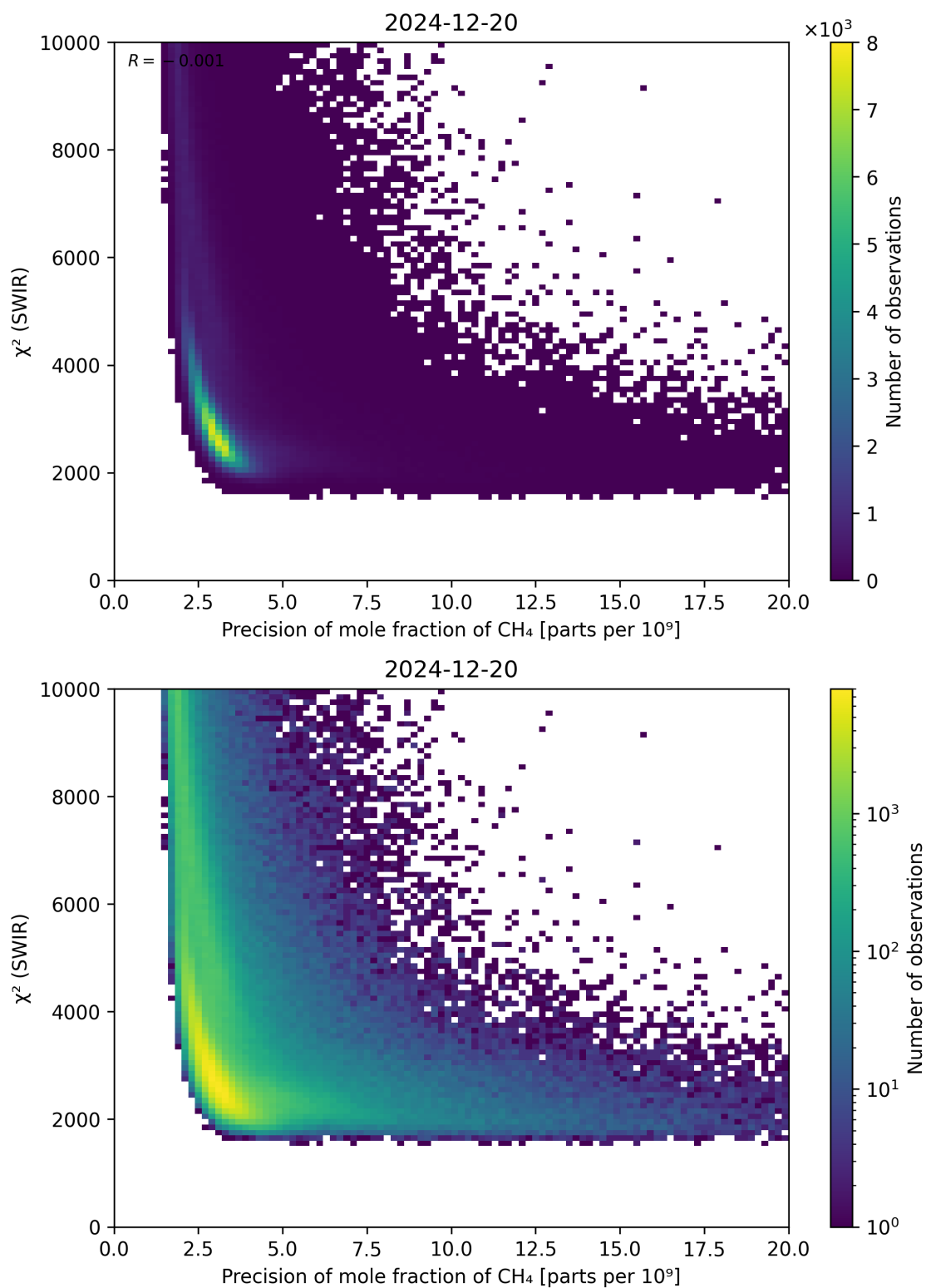
Figure 79: Scatter density plot of “Precision of mole fraction of CH 4 ” against “ \chi^2 (SWIR)” for 2024-12-19 to 2024-12-21.
