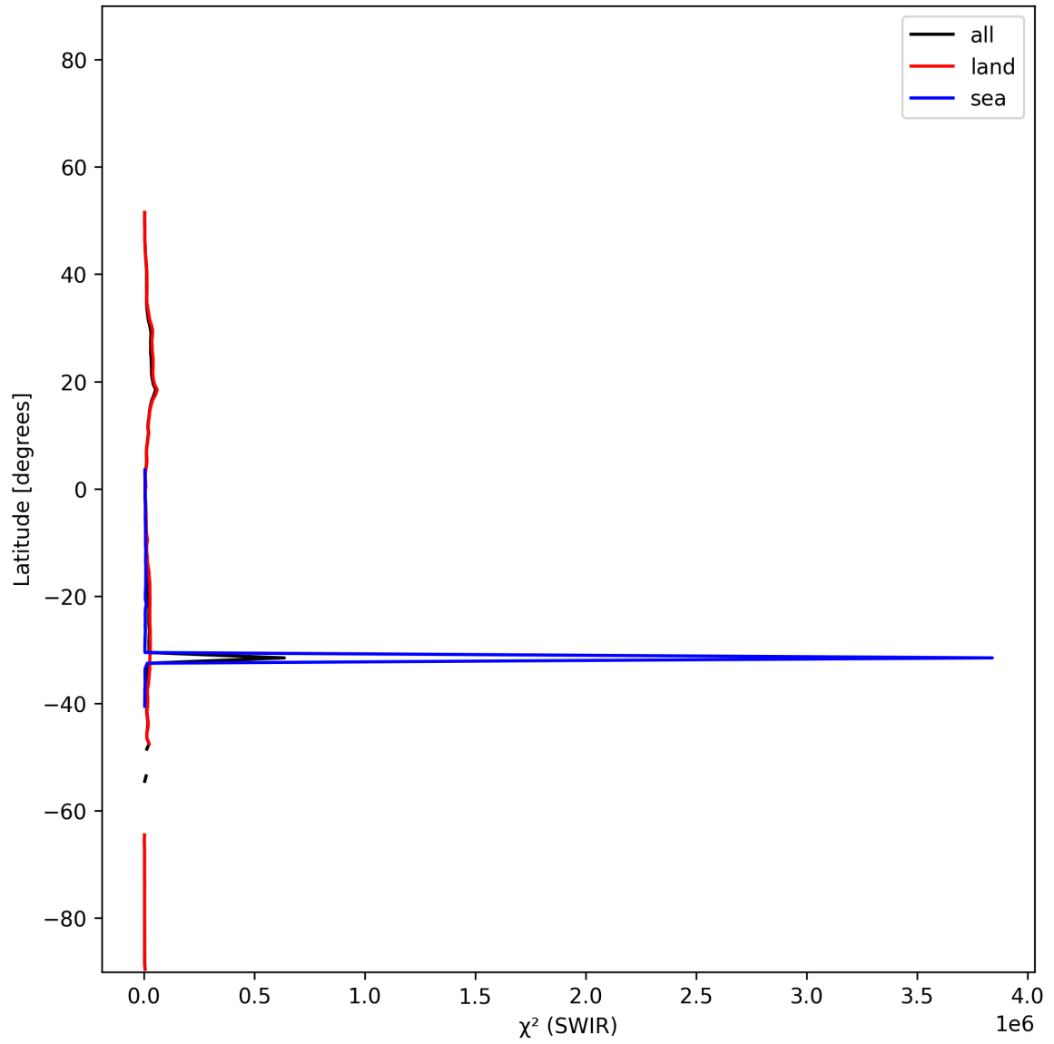
Figure 17: Zonal average of “ \chi^2 (SWIR)” for 2024-12-19 to 2024-12-21.
