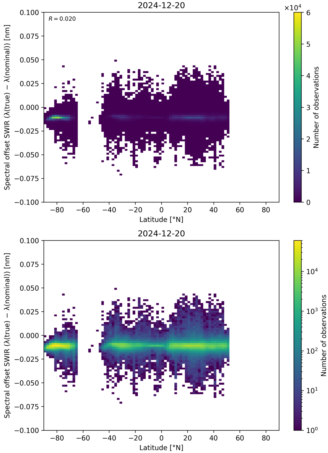
Figure 62: Scatter density plot of “Latitude” against “Spectral offset SWIR ( \lambda_{\text{true}} - \lambda_{\text{nominal}} )” for 2024-12-19 to 2024-12-21.
