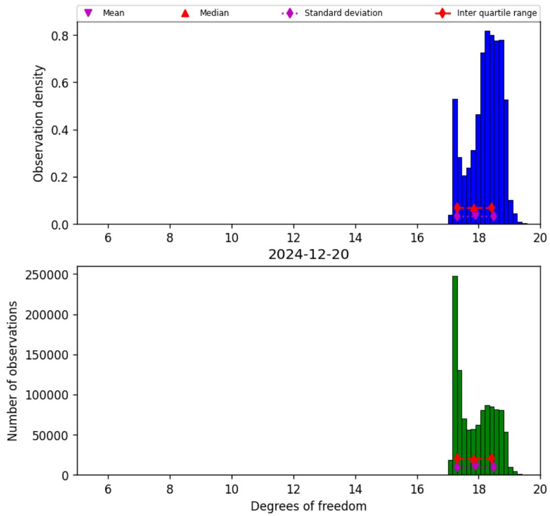
Figure 30: Histogram of “Degrees of freedom” for 2024-12-19 to 2024-12-21
