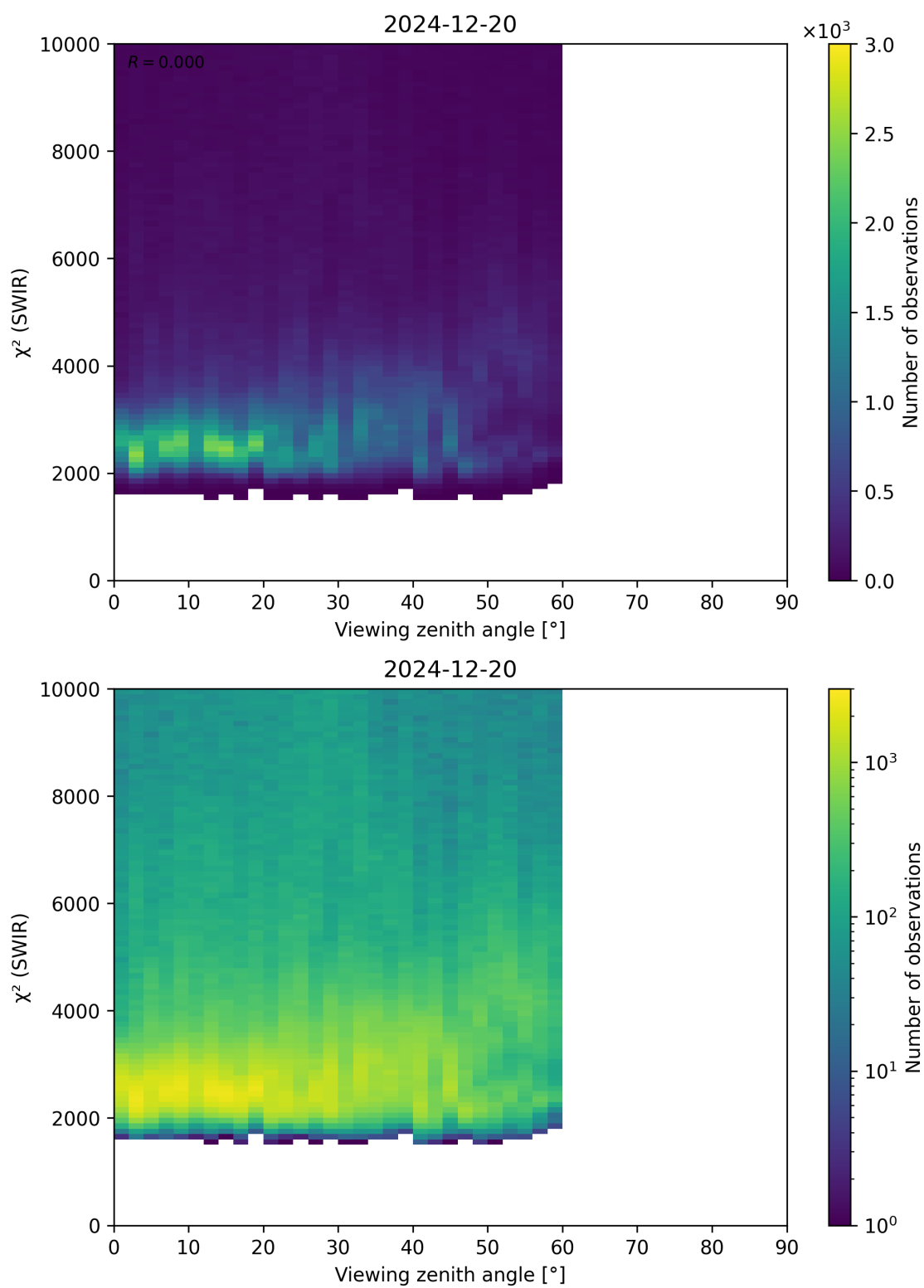
Figure 106: Scatter density plot of “Viewing zenith angle” against “ \chi^2 (SWIR)” for 2024-12-19 to 2024-12-21.
