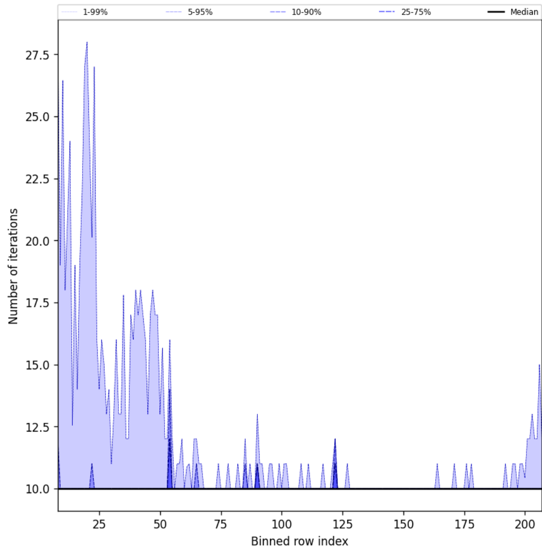
Figure 42: Along track statistics of “Number of iterations” for 2024-12-19 to 2024-12-21
