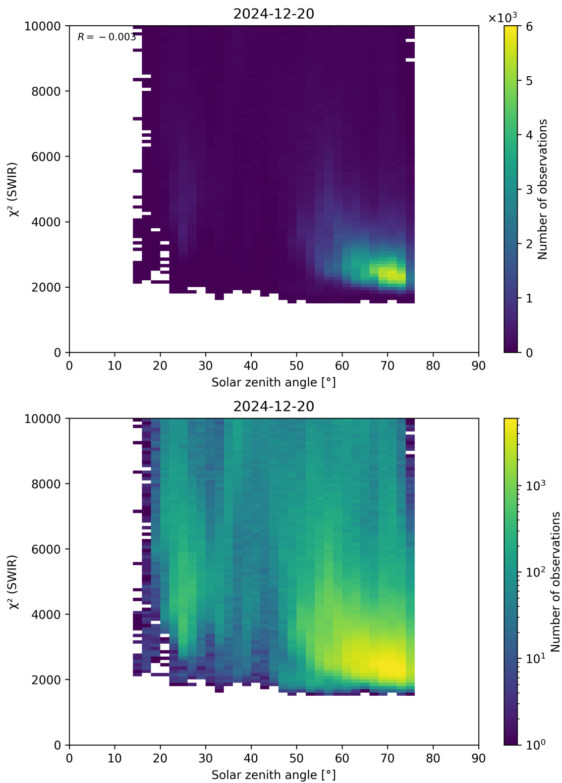
Figure 95: Scatter density plot of “Solar zenith angle” against “ \chi^2 (SWIR)” for 2024-12-19 to 2024-12-21.
