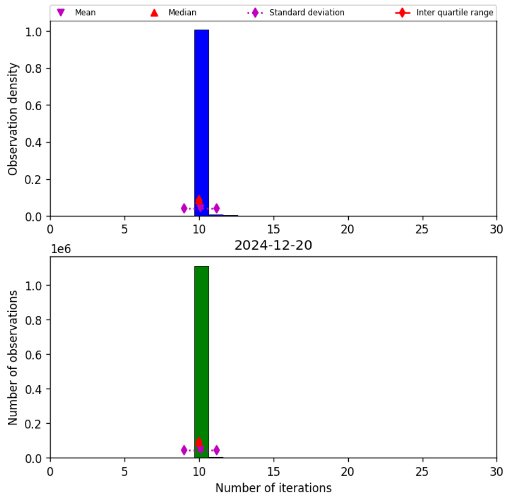
Figure 31: Histogram of “Number of iterations” for 2024-12-19 to 2024-12-21
