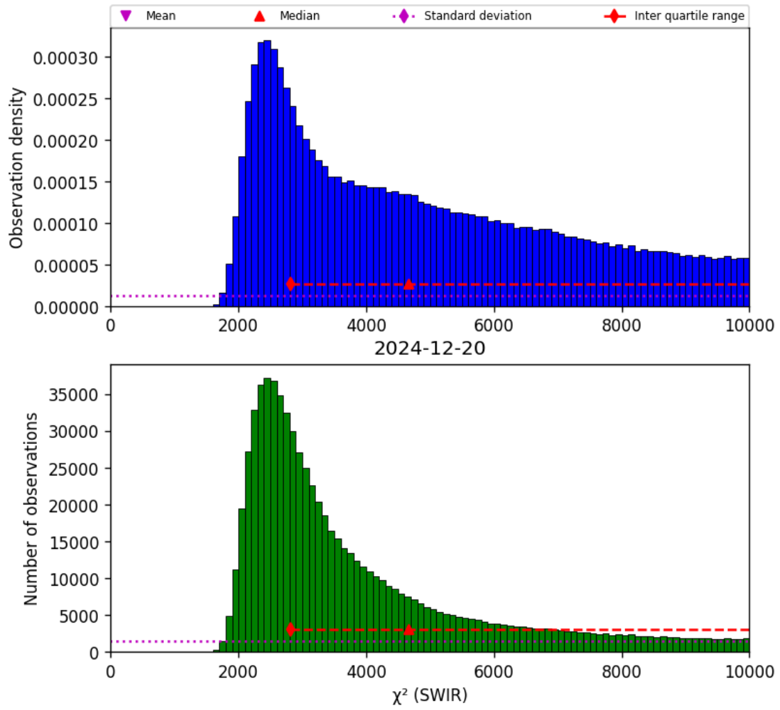
Figure 28: Histogram of “ \chi^2 (SWIR)” for 2024-12-19 to 2024-12-21
