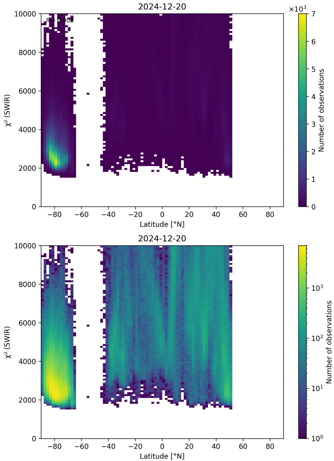
Figure 54: Scatter density plot of “Latitude” against “ \chi^2 (SWIR)” for 2024-12-19 to 2024-12-21.
