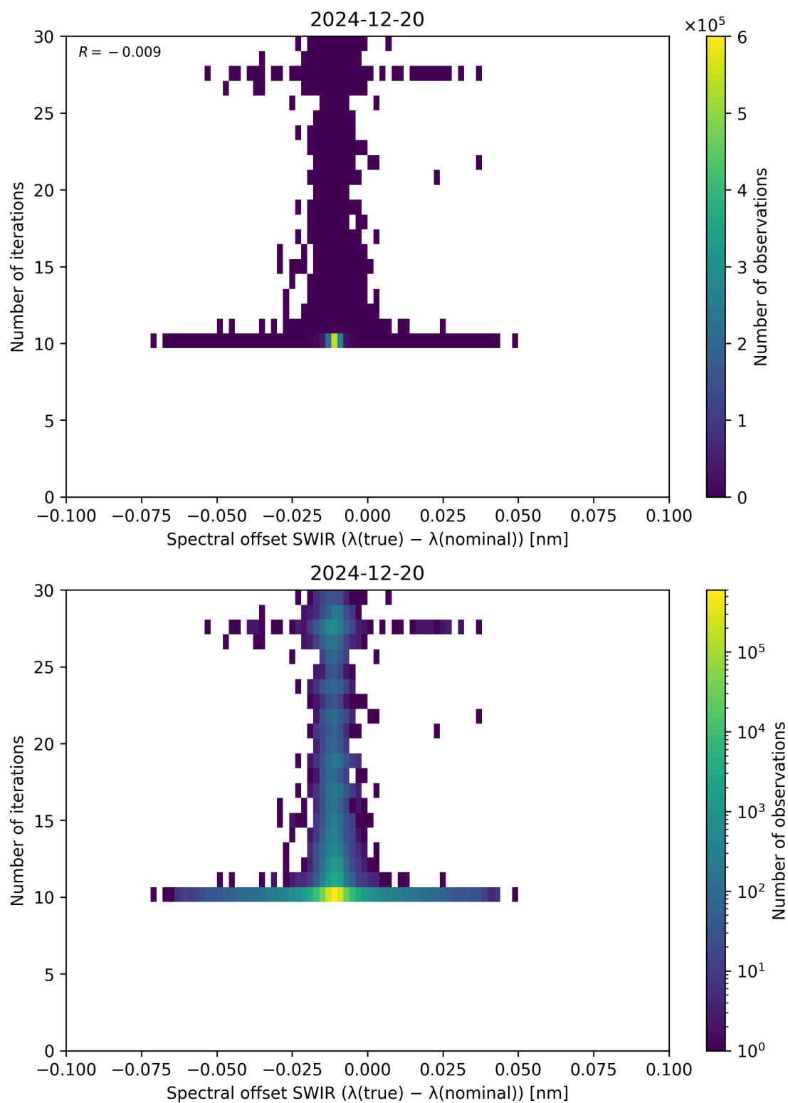
Figure 121: Scatter density plot of “Spectral offset SWIR ( \lambda_{\text{true}} - \lambda_{\text{nominal}} )” against “Number of iterations” for 2024-12-19 to 2024-12-21.
