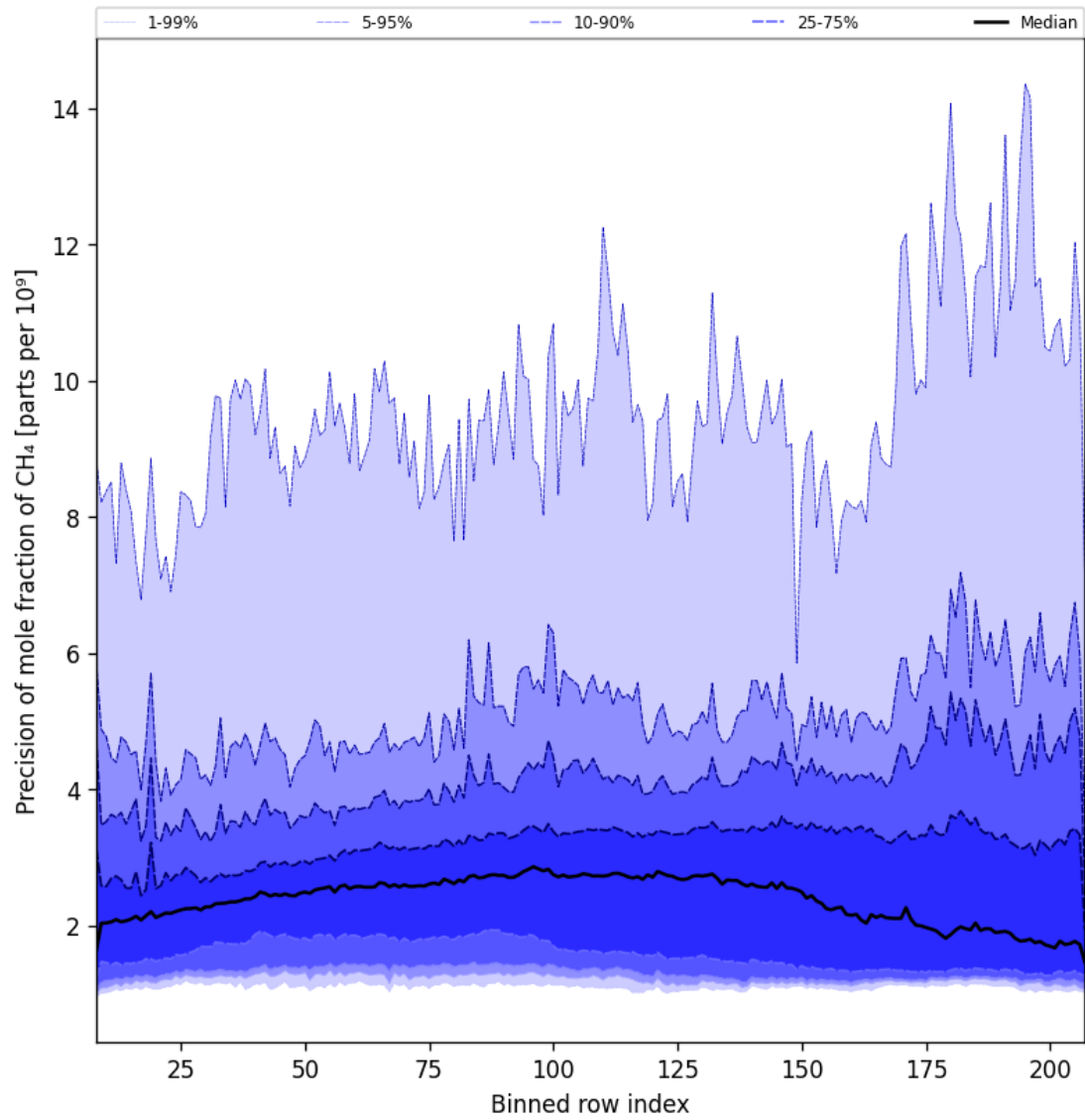
Figure 35: Along track statistics of “Precision of mole fraction of CH 4 ” for 2024-12-19 to 2024-12-21
