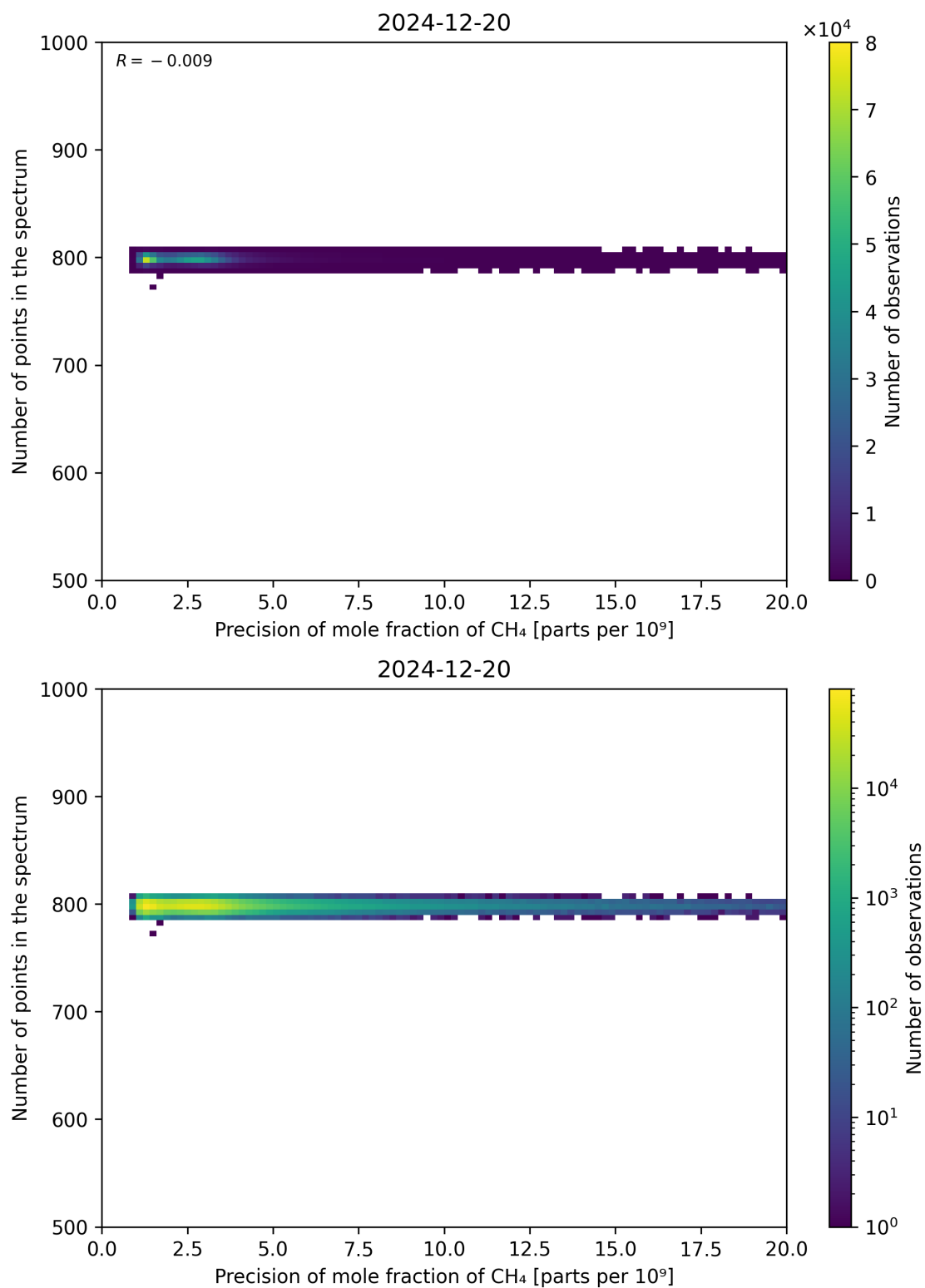
Figure 84: Scatter density plot of “Precision of mole fraction of CH 4 ” against “Number of points in the spectrum” for 2024-12-19 to 2024-12-21.
