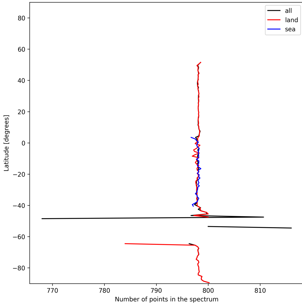
Figure 15: Zonal average of “Number of points in the spectrum” for 2024-12-19 to 2024-12-21.
