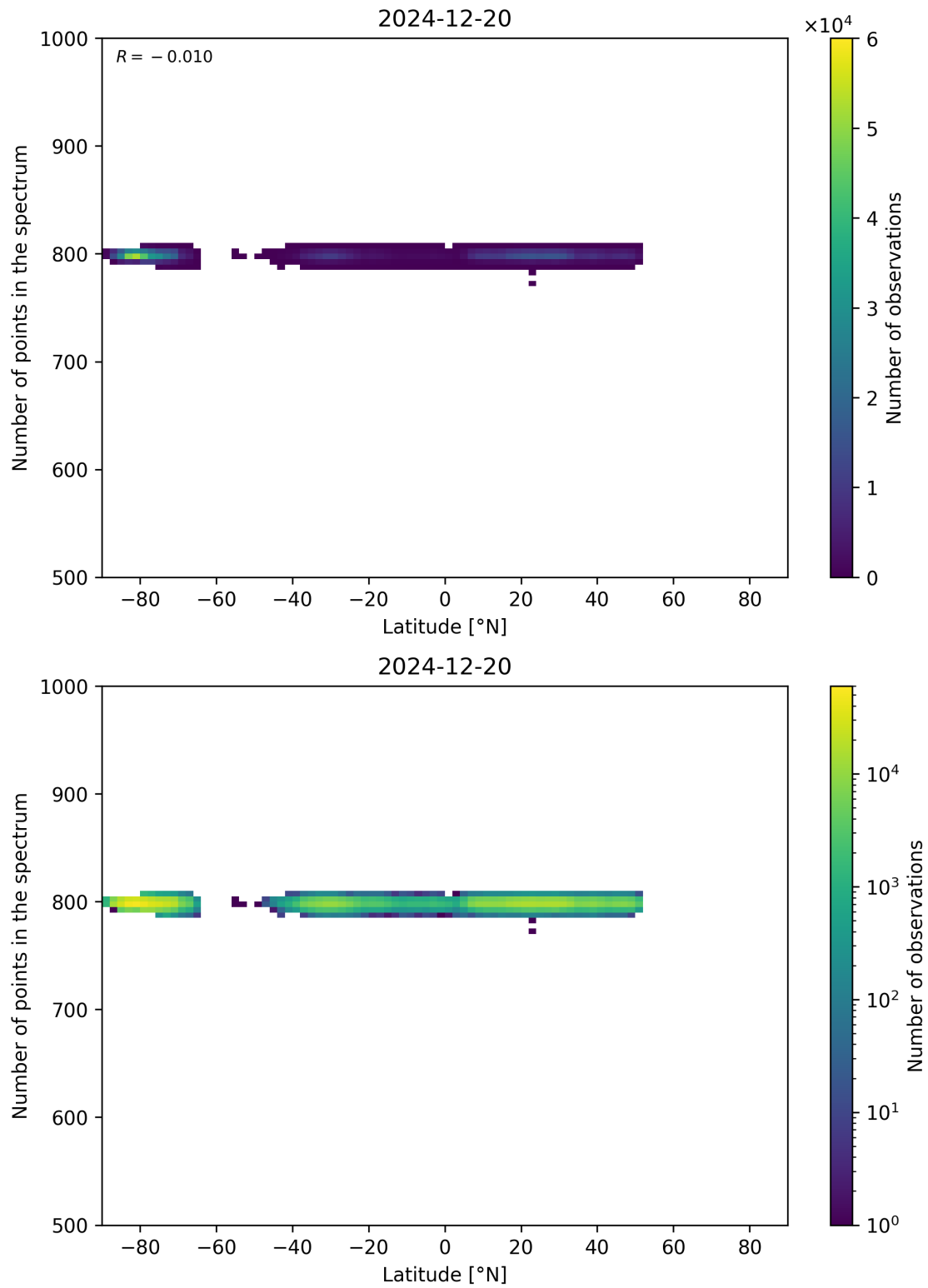
Figure 61: Scatter density plot of “Latitude” against “Number of points in the spectrum” for 2024-12-19 to 2024-12-21.
