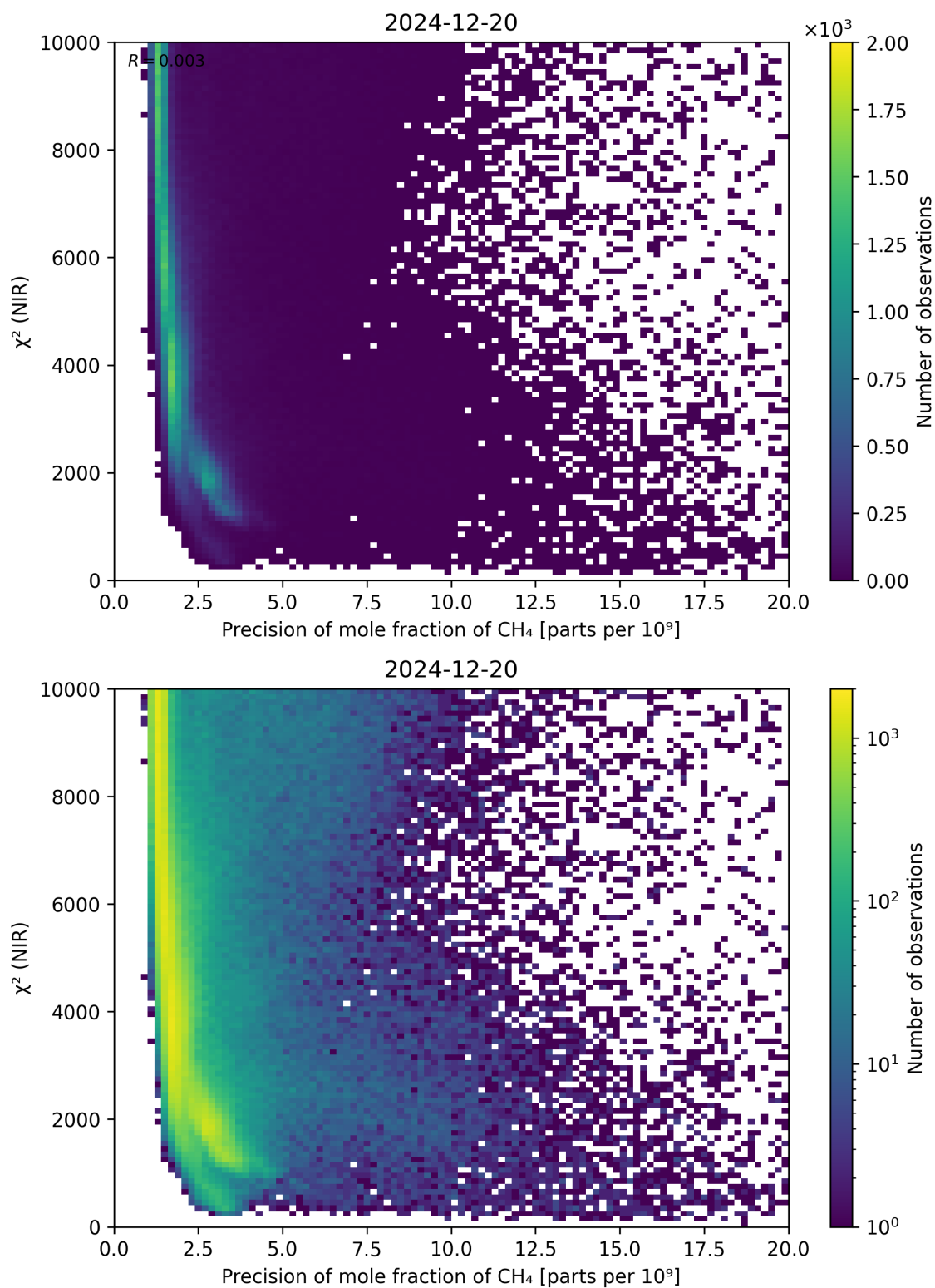
Figure 78: Scatter density plot of “Precision of mole fraction of \text{CH}_4 ” against “ \chi^2 (NIR)” for 2024-12-19 to 2024-12-21.
