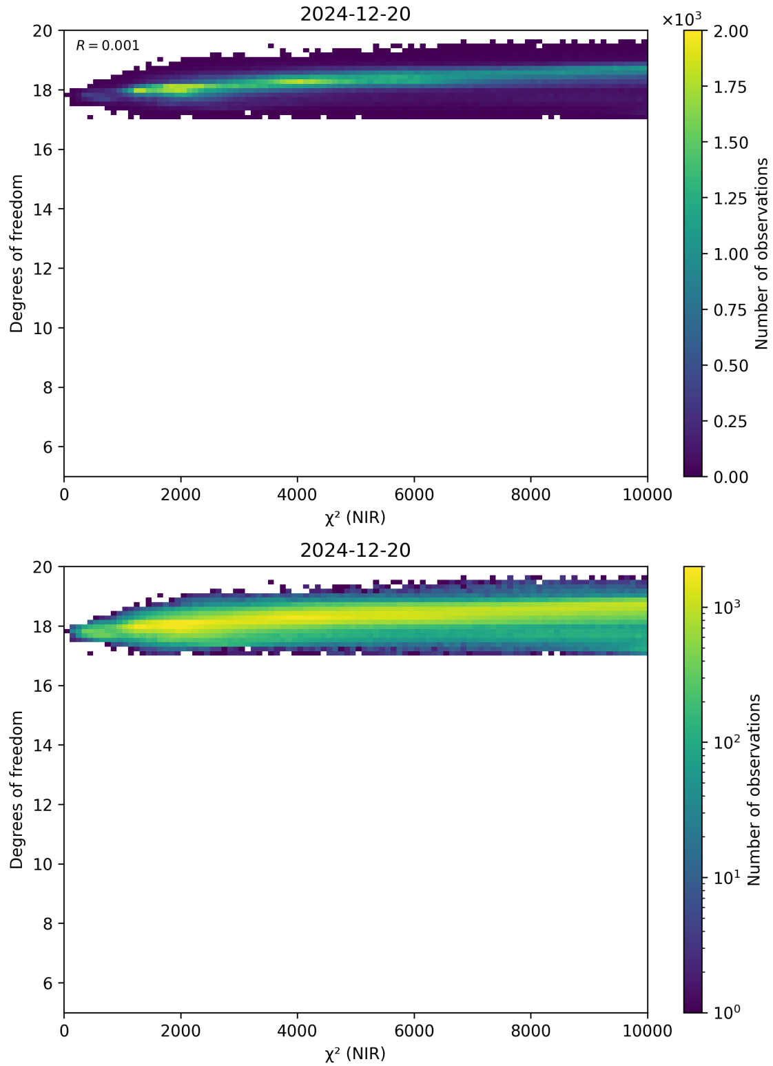
Figure 44: Scatter density plot of “ \chi^2 (NIR)” against “Degrees of freedom” for 2024-12-19 to 2024-12-21.
