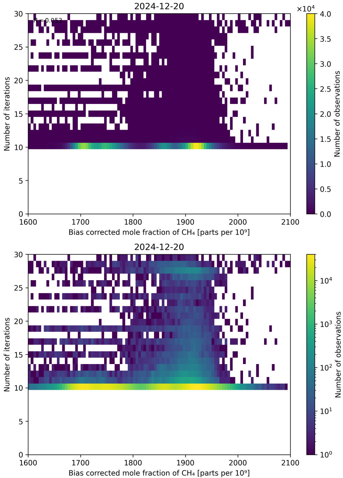
Figure 67: Scatter density plot of “Bias corrected mole fraction of CH 4 ” against “Number of iterations” for 2024-12-19 to 2024-12-21.
