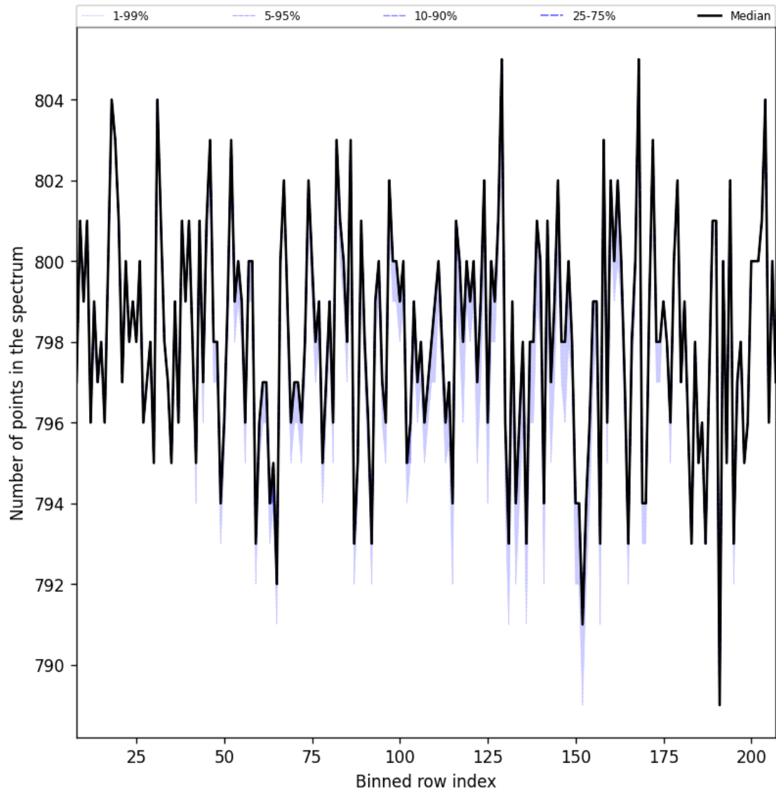
Figure 37: Along track statistics of “Number of points in the spectrum” for 2024-12-19 to 2024-12-21
