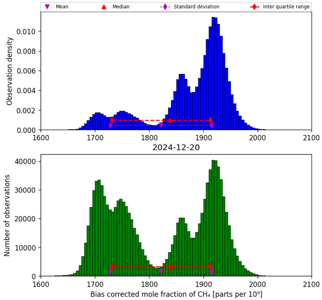
Figure 25: Histogram of “Bias corrected mole fraction of CH 4 ” for 2024-12-19 to 2024-12-21
