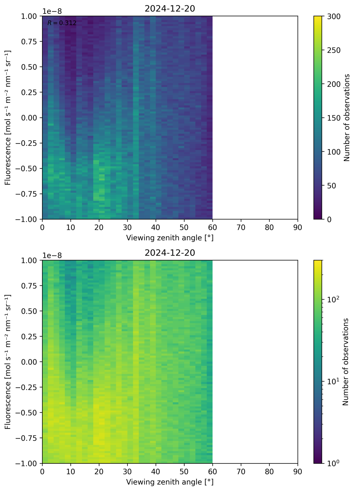
Figure 108: Scatter density plot of “Viewing zenith angle” against “Fluorescence” for 2024-12-19 to 2024-12-21.
