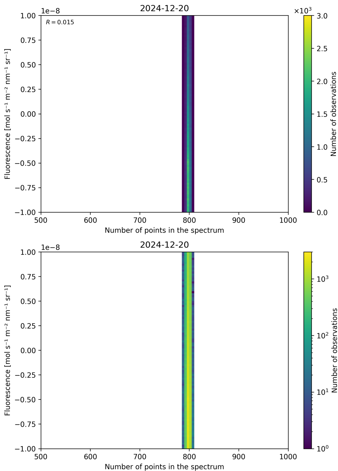
Figure 91: Scatter density plot of “Number of points in the spectrum” against “Fluorescence” for 2024-12-19 to 2024-12-21.
