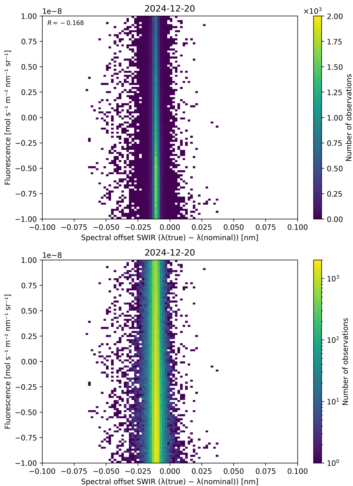
Figure 120: Scatter density plot of “Spectral offset SWIR ( \lambda_{\text{true}} - \lambda_{\text{nominal}} )” against “Fluorescence” for 2024-12-19 to 2024-12-21.
