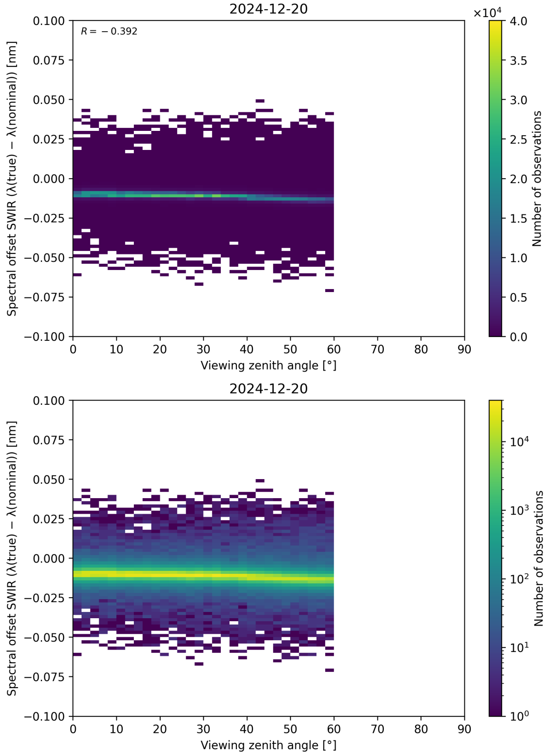
Figure 116: Scatter density plot of “Viewing zenith angle” against “Spectral offset SWIR ( \lambda_{\text{true}} - \lambda_{\text{nominal}} )” for 2024-12-19 to 2024-12-21.
