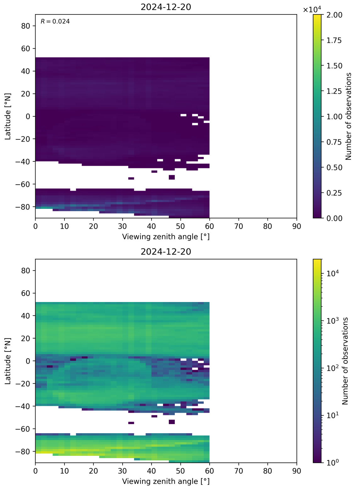
Figure 109: Scatter density plot of “Viewing zenith angle” against “Latitude” for 2024-12-19 to 2024-12-21.
