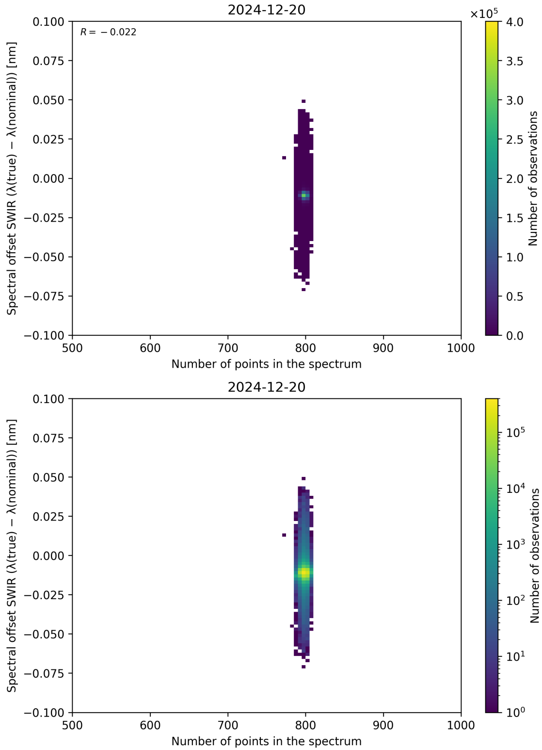
Figure 93: Scatter density plot of “Number of points in the spectrum” against “Spectral offset SWIR ( \lambda_{\text{true}} - \lambda_{\text{nominal}} )” for 2024-12-19 to 2024-12-21.
