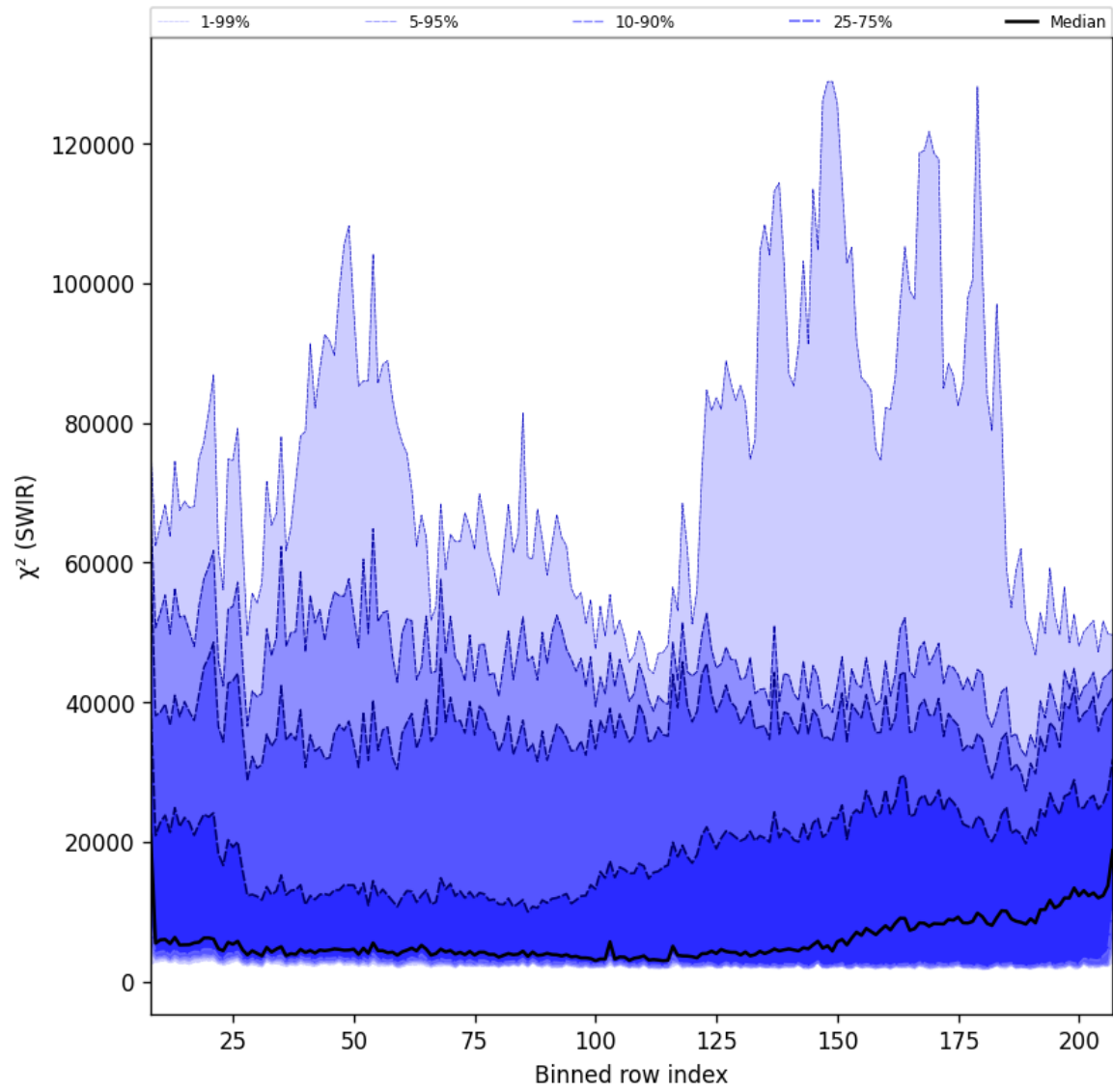
Figure 39: Along track statistics of “ \chi^2 (SWIR)” for 2024-12-19 to 2024-12-21
