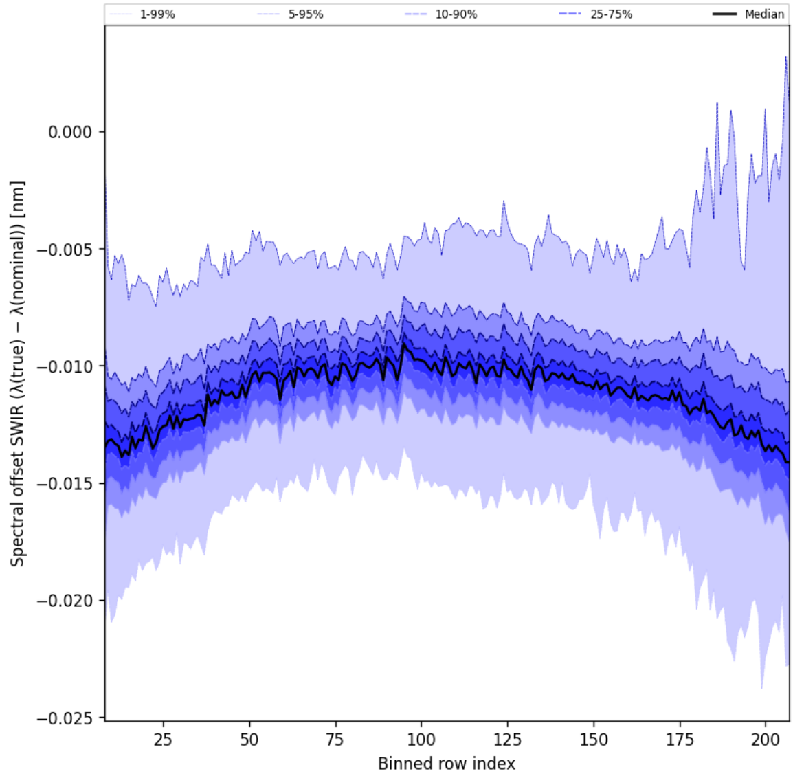
Figure 38: Along track statistics of “Spectral offset SWIR ( \lambda_{\text{true}} - \lambda_{\text{nominal}} )” for 2024-12-19 to 2024-12-21
