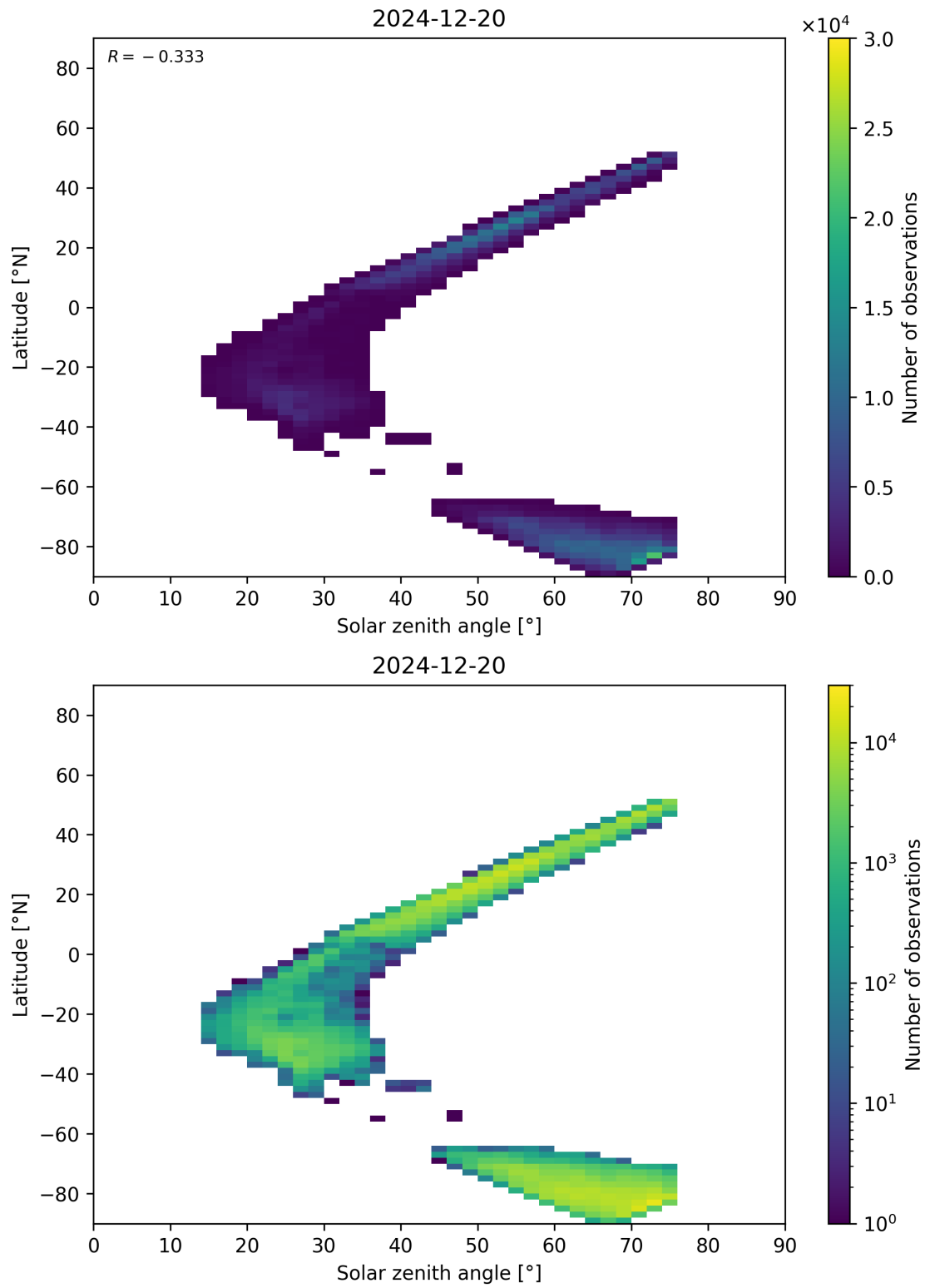
Figure 98: Scatter density plot of “Solar zenith angle” against “Latitude” for 2024-12-19 to 2024-12-21.
