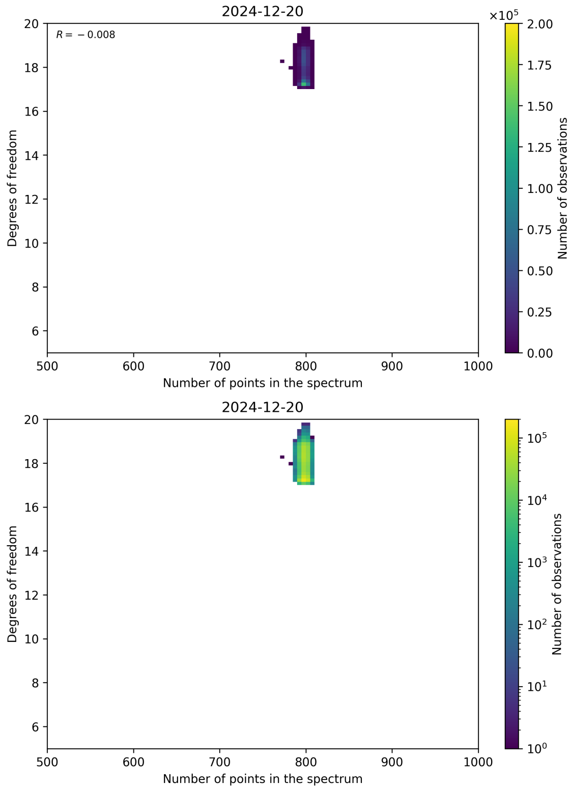
Figure 90: Scatter density plot of “Number of points in the spectrum” against “Degrees of freedom” for 2024-12-19 to 2024-12-21.
