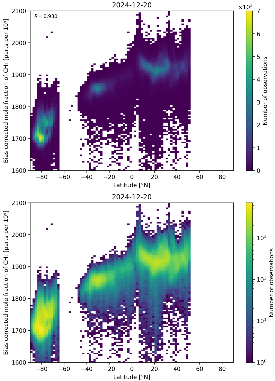
Figure 58: Scatter density plot of “Latitude” against “Bias corrected mole fraction of CH 4 ” for 2024-12-19 to 2024-12-21.
