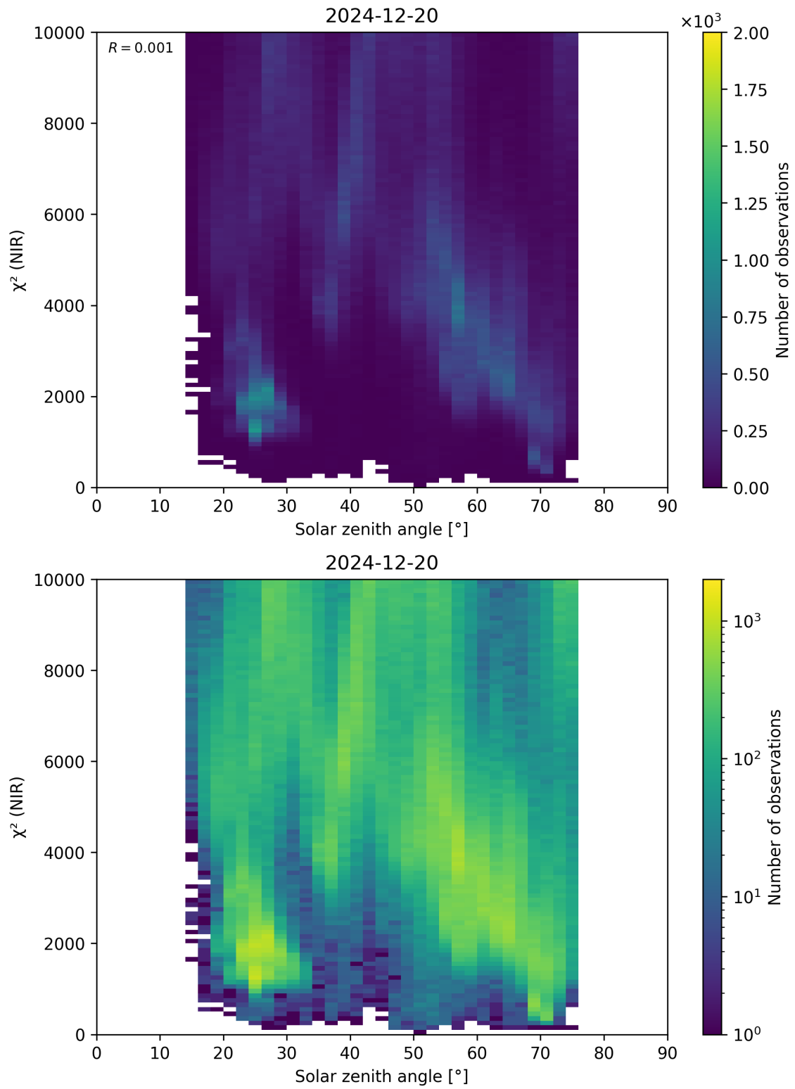
Figure 94: Scatter density plot of “Solar zenith angle” against “ \chi^2 (NIR)” for 2024-12-19 to 2024-12-21.
