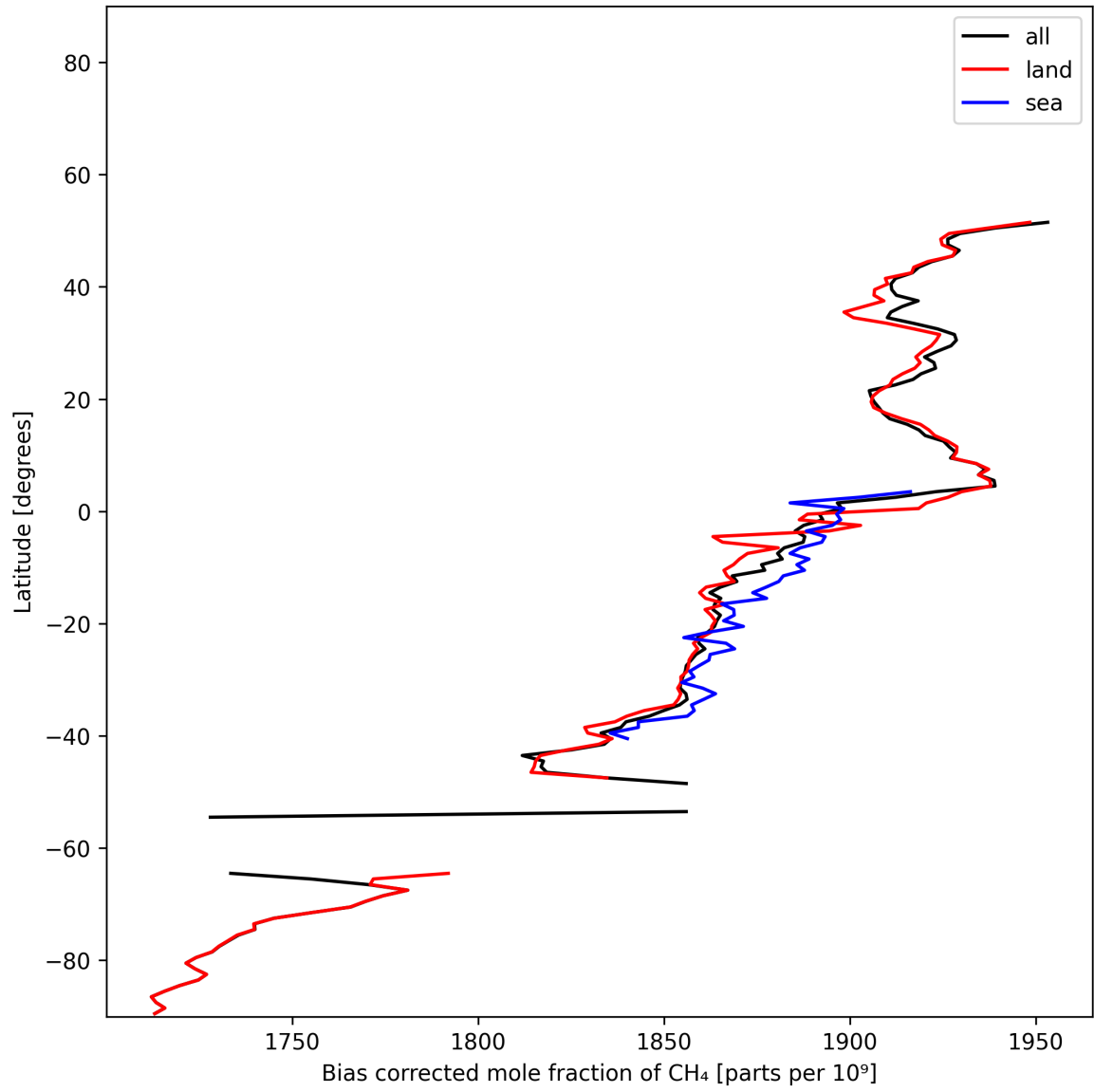
Figure 14: Zonal average of “Bias corrected mole fraction of CH 4 ” for 2024-12-19 to 2024-12-21.
