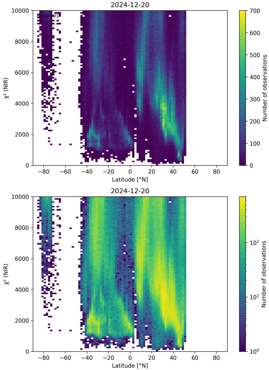
Figure 53: Scatter density plot of “Latitude” against “ \chi^2 (NIR)” for 2024-12-19 to 2024-12-21.
