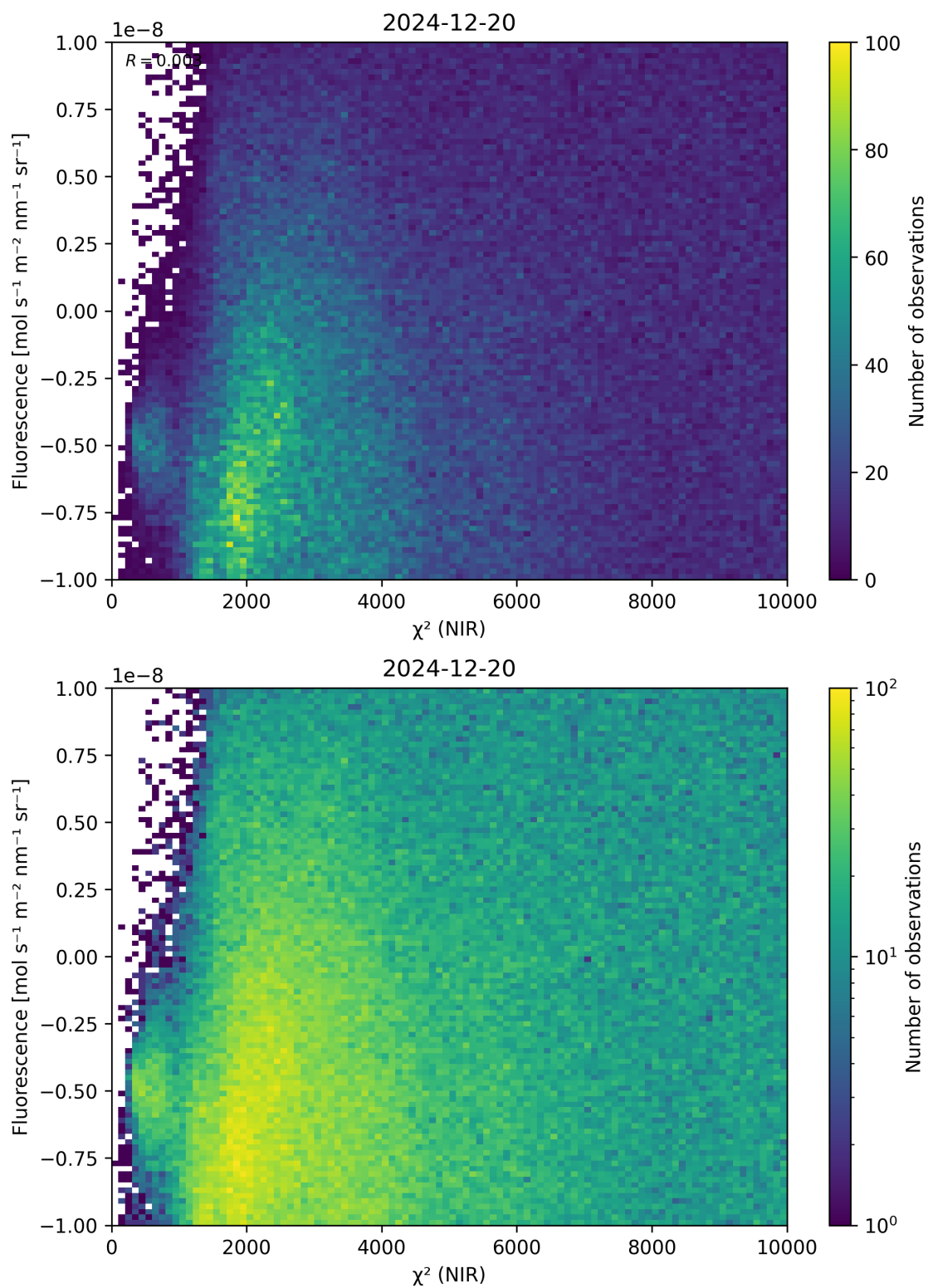
Figure 45: Scatter density plot of “ \chi^2 (NIR)” against “Fluorescence” for 2024-12-19 to 2024-12-21.
