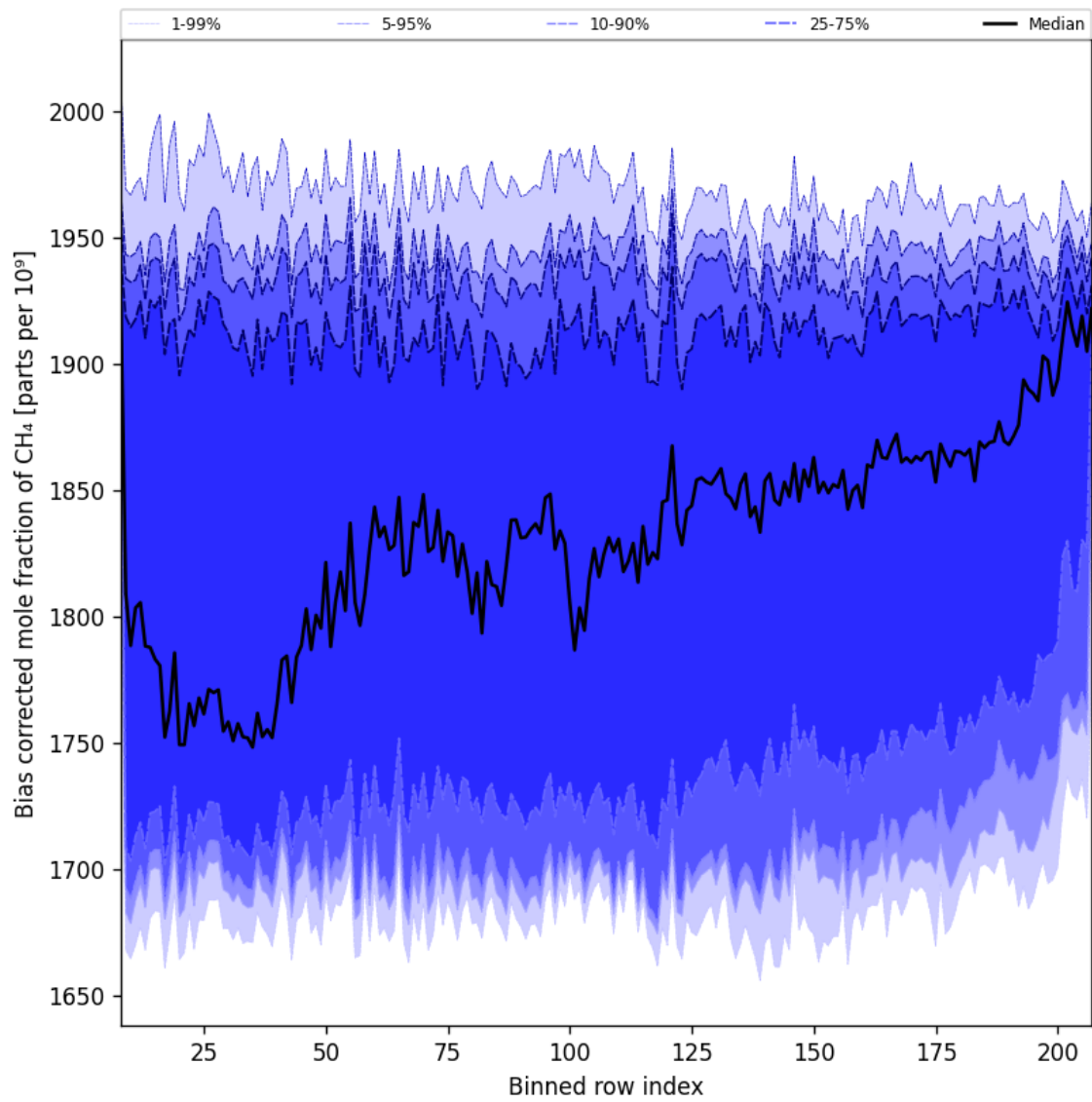
Figure 36: Along track statistics of “Bias corrected mole fraction of CH 4 ” for 2024-12-19 to 2024-12-21
