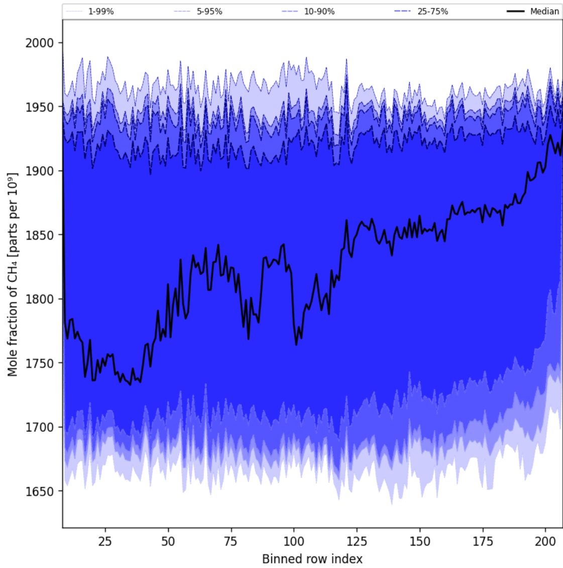
Figure 34: Along track statistics of “Mole fraction of CH 4 ” for 2024-12-19 to 2024-12-21
