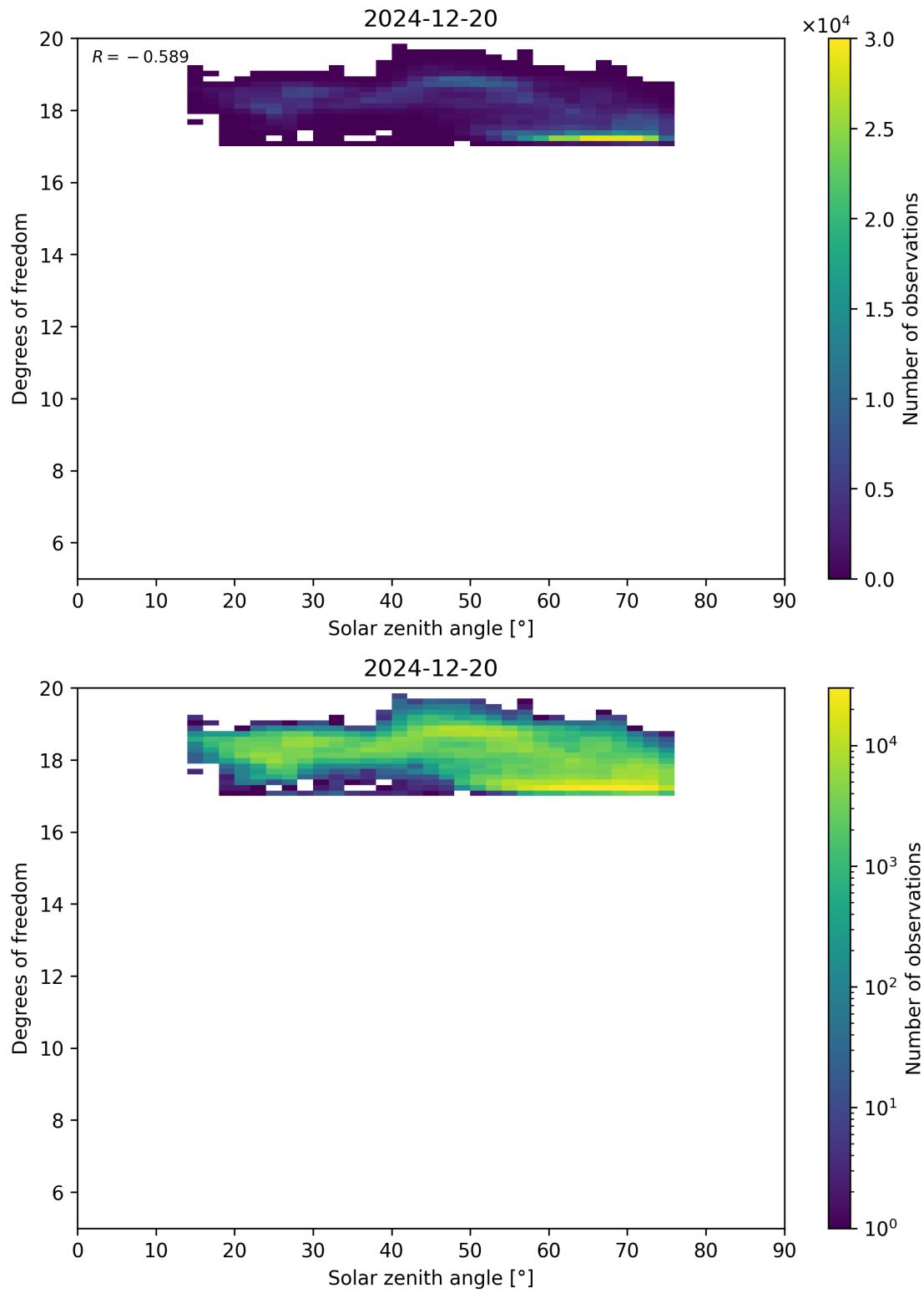
Figure 96: Scatter density plot of “Solar zenith angle” against “Degrees of freedom” for 2024-12-19 to 2024-12-21.
