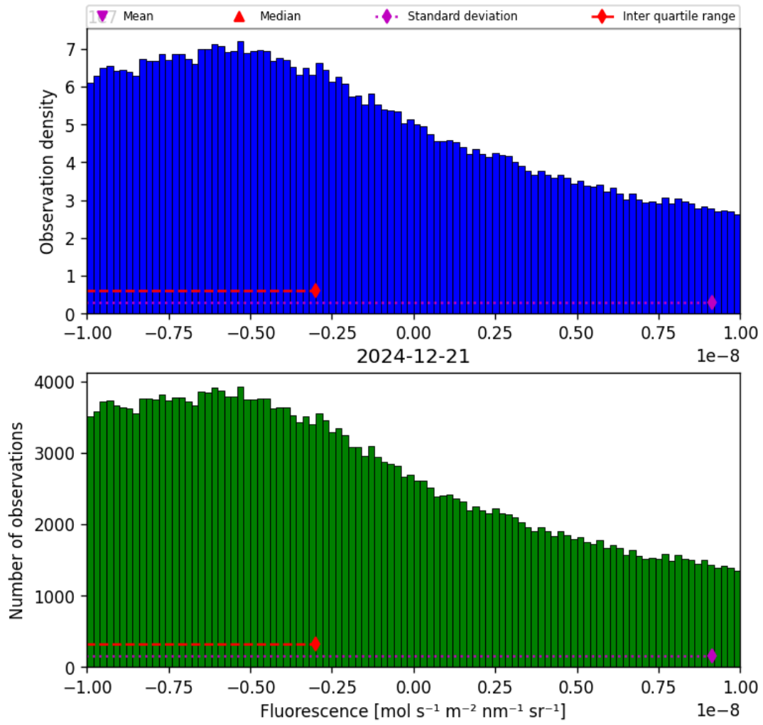
Figure 32: Histogram of “Fluorescence” for 2024-12-20 to 2024-12-22
