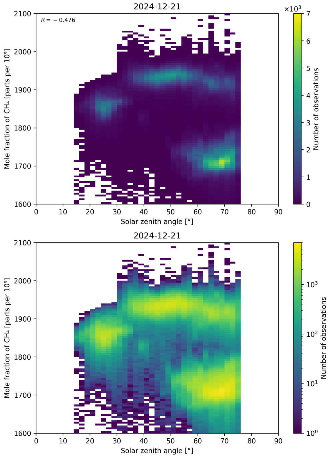
Figure 99: Scatter density plot of “Solar zenith angle” against “Mole fraction of CH 4 ” for 2024-12-20 to 2024-12-22.
