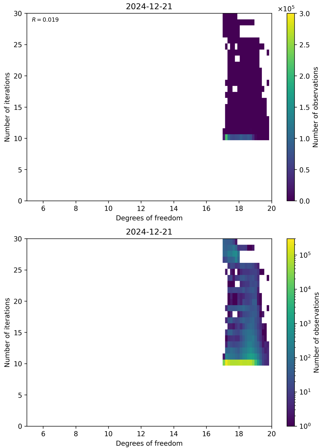
Figure 52: Scatter density plot of “Degrees of freedom” against “Number of iterations” for 2024-12-20 to 2024-12-22.
