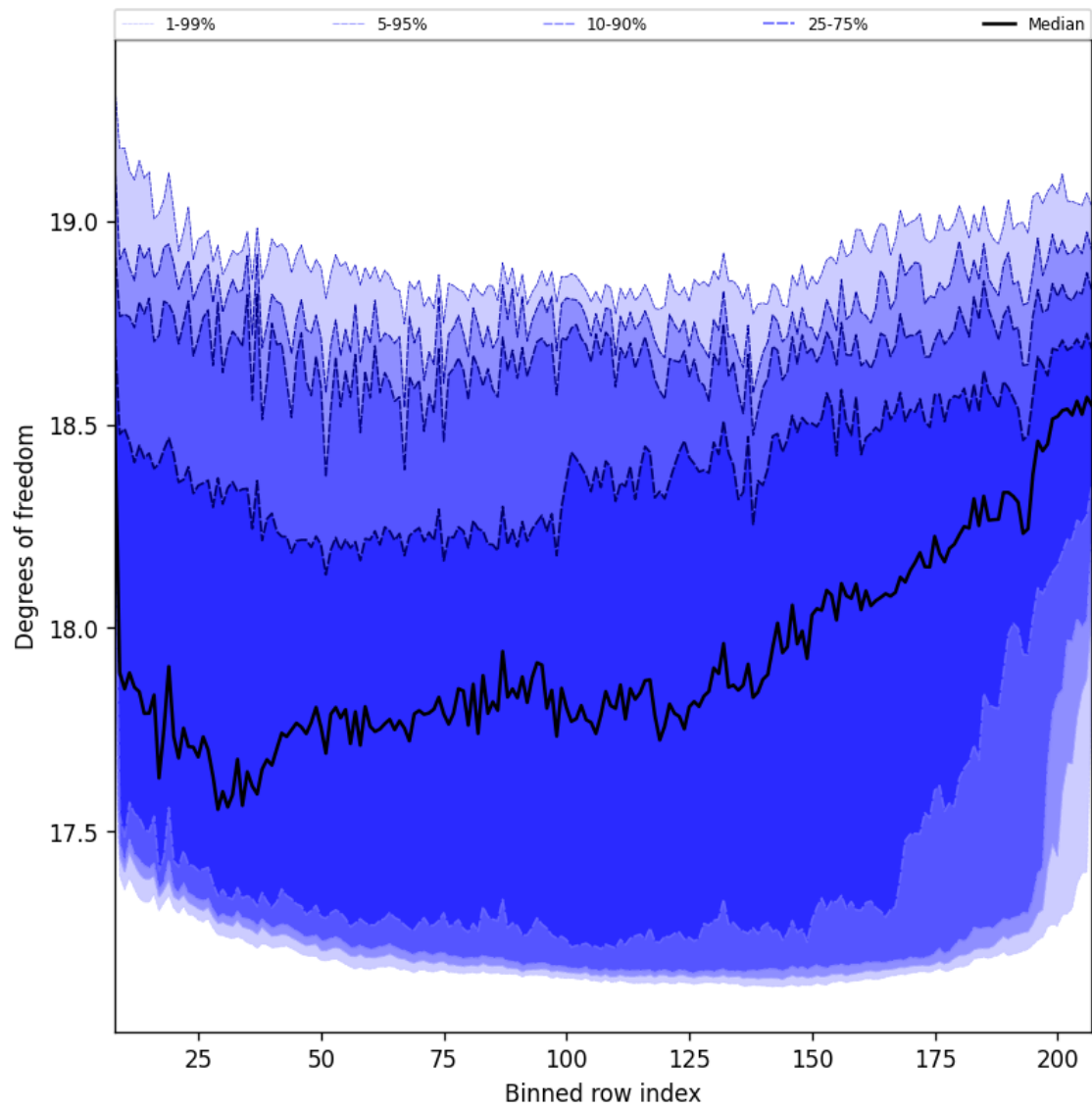
Figure 41: Along track statistics of “Degrees of freedom” for 2024-12-20 to 2024-12-22
