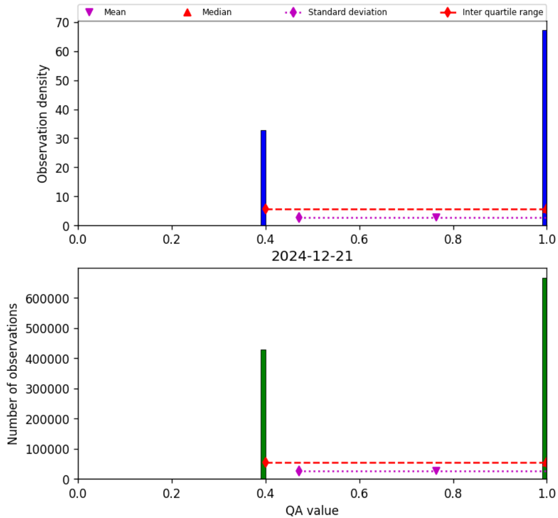
Figure 22: Histogram of “QA value” for 2024-12-20 to 2024-12-22
