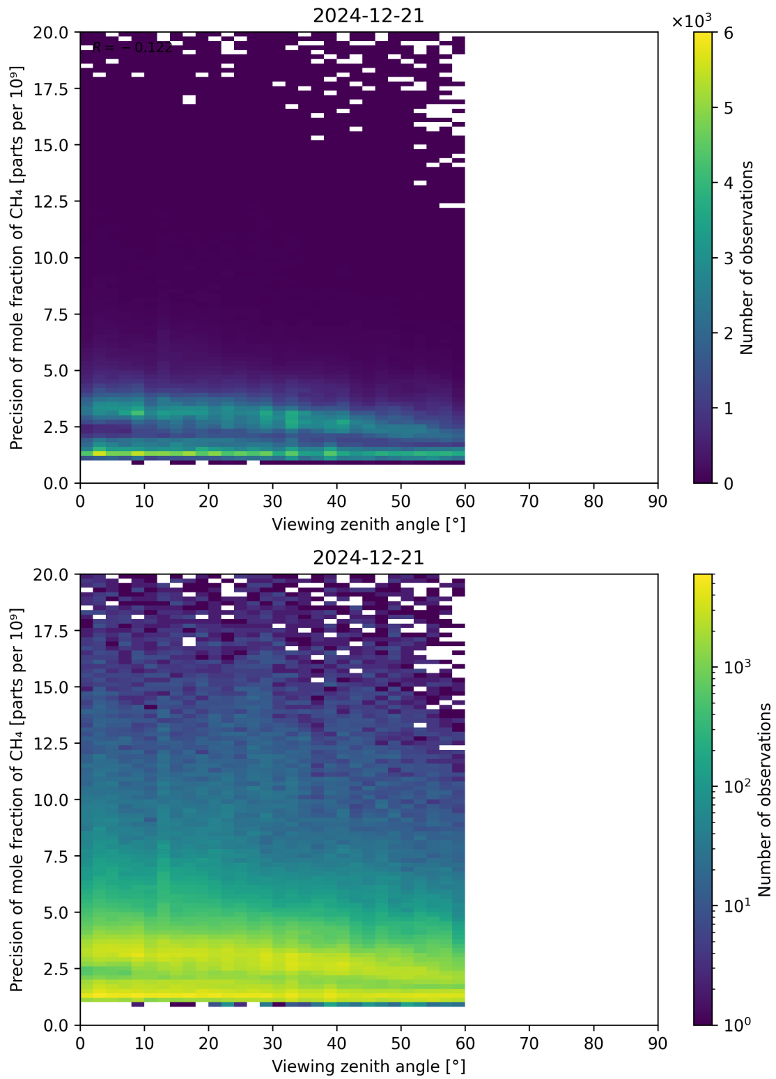
Figure 112: Scatter density plot of “Viewing zenith angle” against “Precision of mole fraction of CH 4 ” for 2024-12-20 to 2024-12-22.
