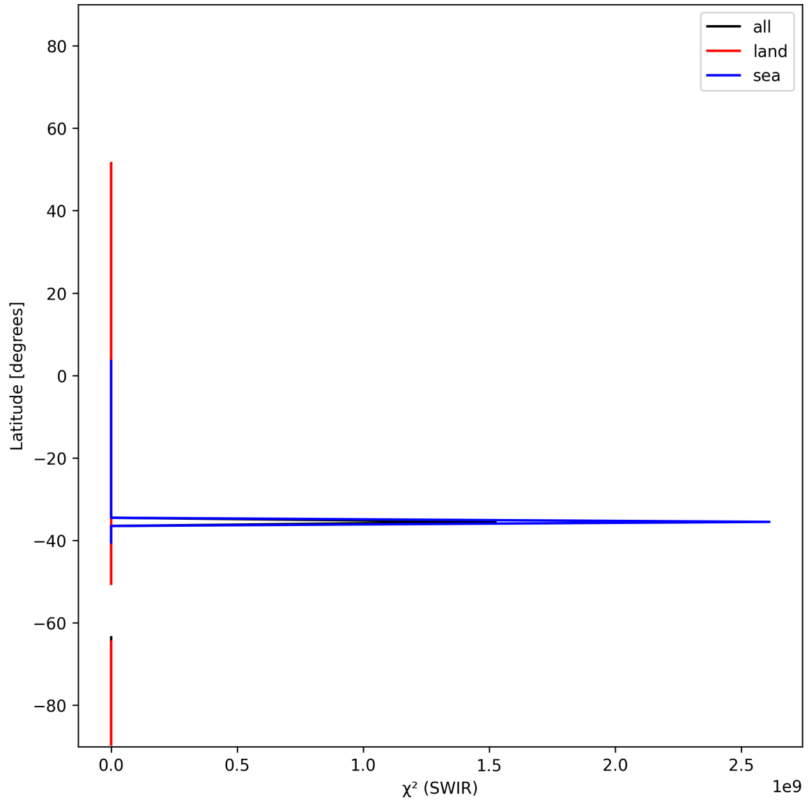
Figure 17: Zonal average of “ \chi^2 (SWIR)” for 2024-12-20 to 2024-12-22.
