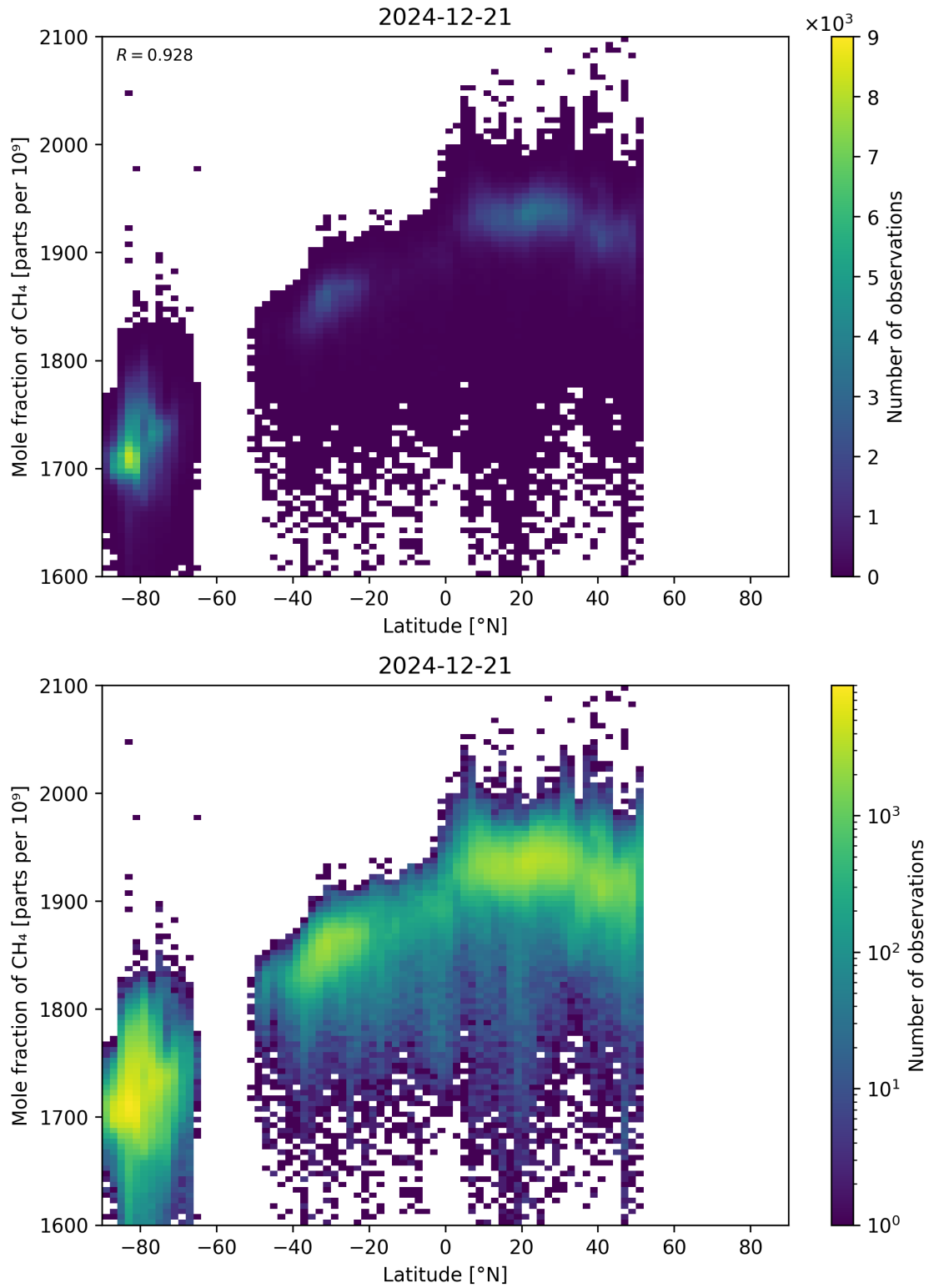
Figure 57: Scatter density plot of “Latitude” against “Mole fraction of CH 4 ” for 2024-12-20 to 2024-12-22.
