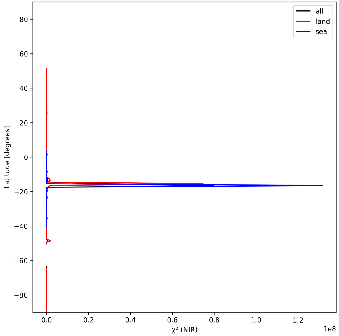
Figure 18: Zonal average of “ \chi^2 (NIR)” for 2024-12-20 to 2024-12-22.
