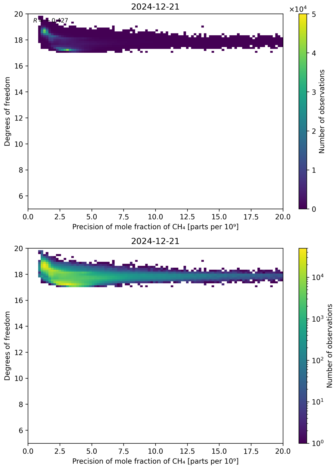
Figure 80: Scatter density plot of “Precision of mole fraction of CH 4 ” against “Degrees of freedom” for 2024-12-20 to 2024-12-22.
