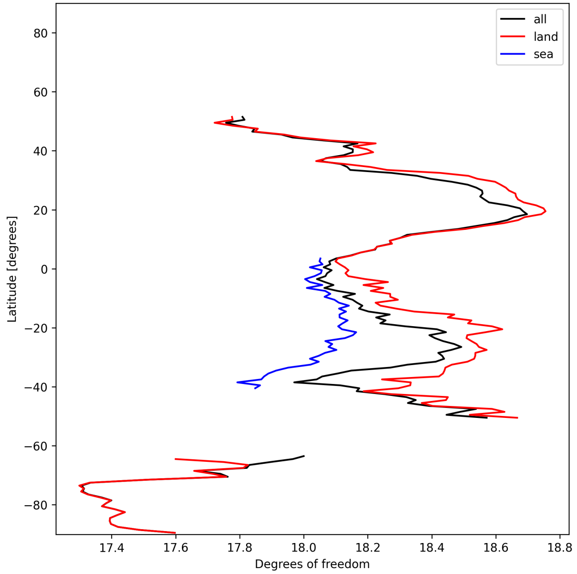
Figure 19: Zonal average of “Degrees of freedom” for 2024-12-20 to 2024-12-22.
