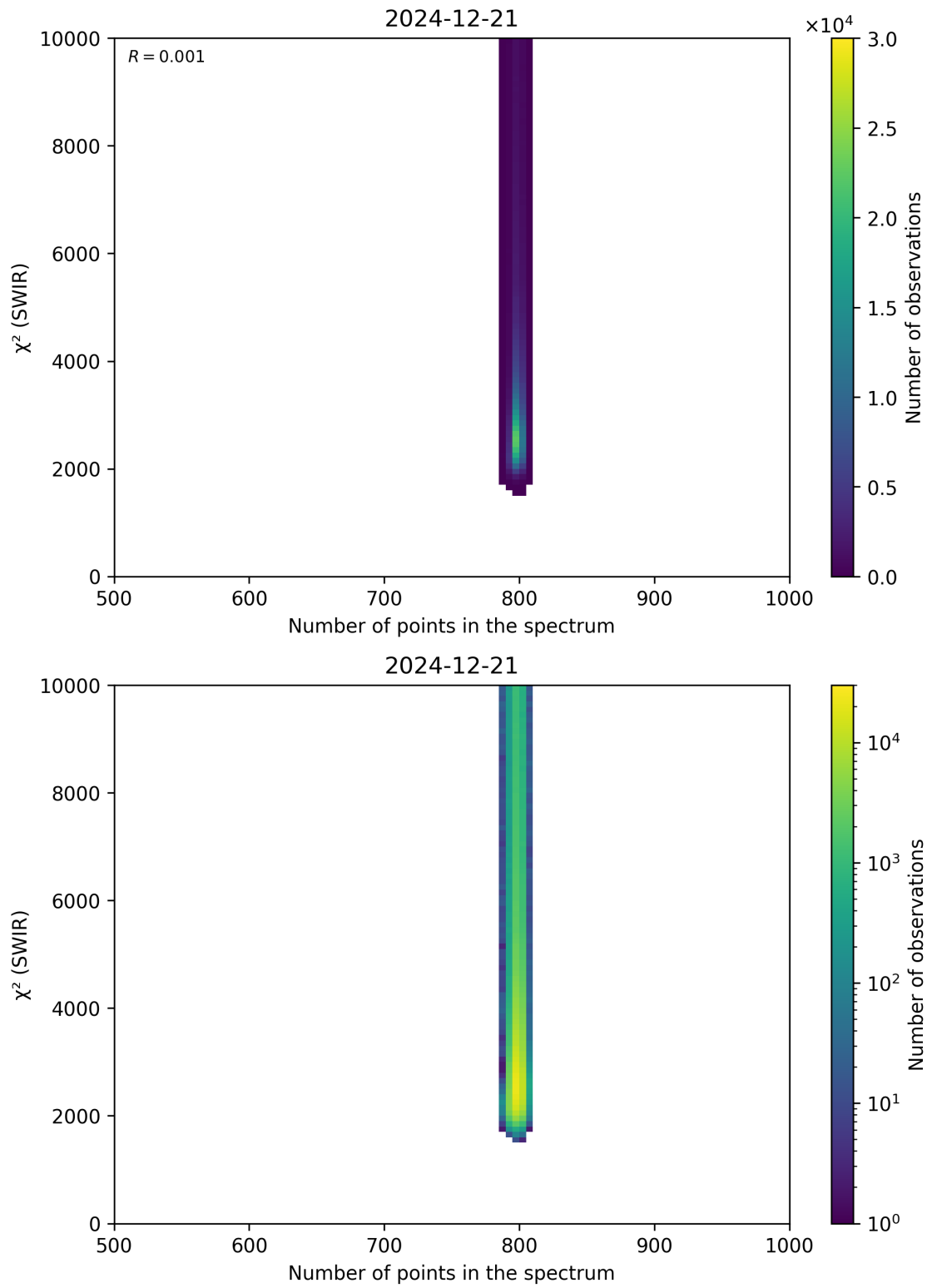
Figure 89: Scatter density plot of “Number of points in the spectrum” against “ \chi^2 (SWIR)” for 2024-12-20 to 2024-12-22.
