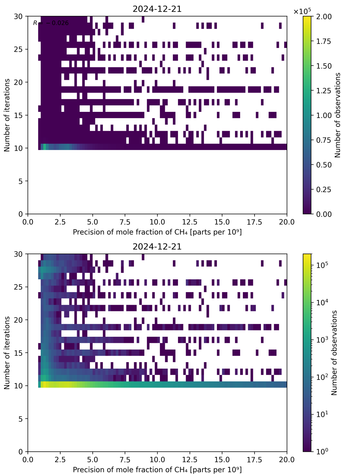
Figure 83: Scatter density plot of “Precision of mole fraction of CH 4 ” against “Number of iterations” for 2024-12-20 to 2024-12-22.
