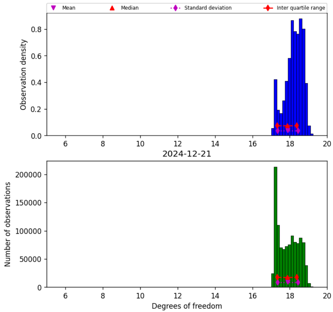
Figure 30: Histogram of “Degrees of freedom” for 2024-12-20 to 2024-12-22
