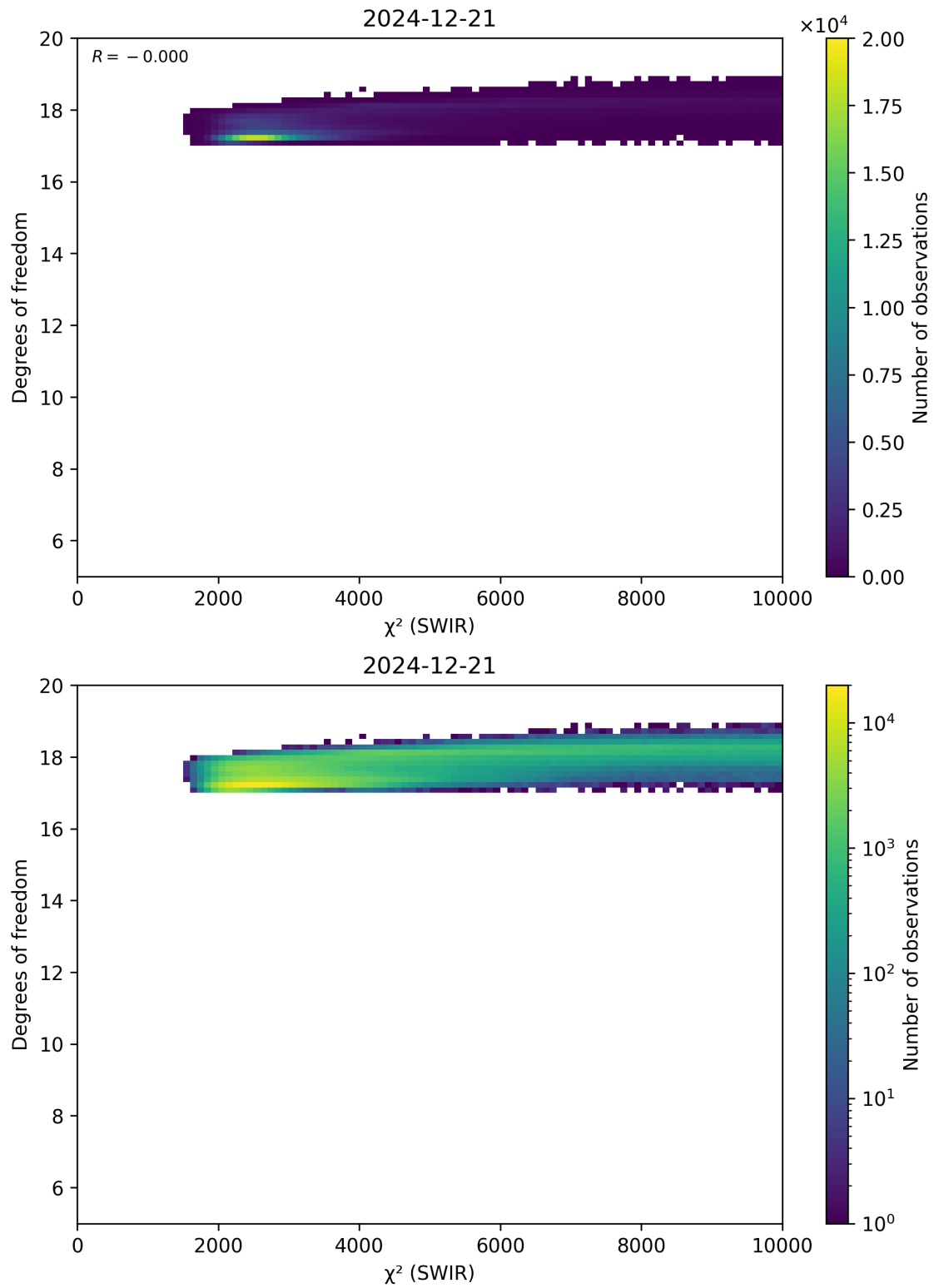
Figure 48: Scatter density plot of “ \chi^2 (SWIR)” against “Degrees of freedom” for 2024-12-20 to 2024-12-22.
