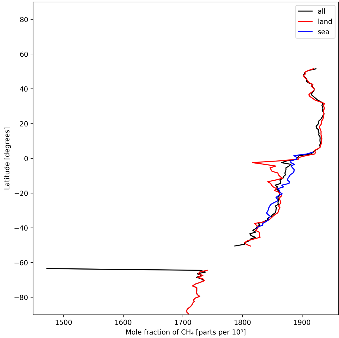
Figure 12: Zonal average of “Mole fraction of \text{CH}_4 ” for 2024-12-20 to 2024-12-22.
