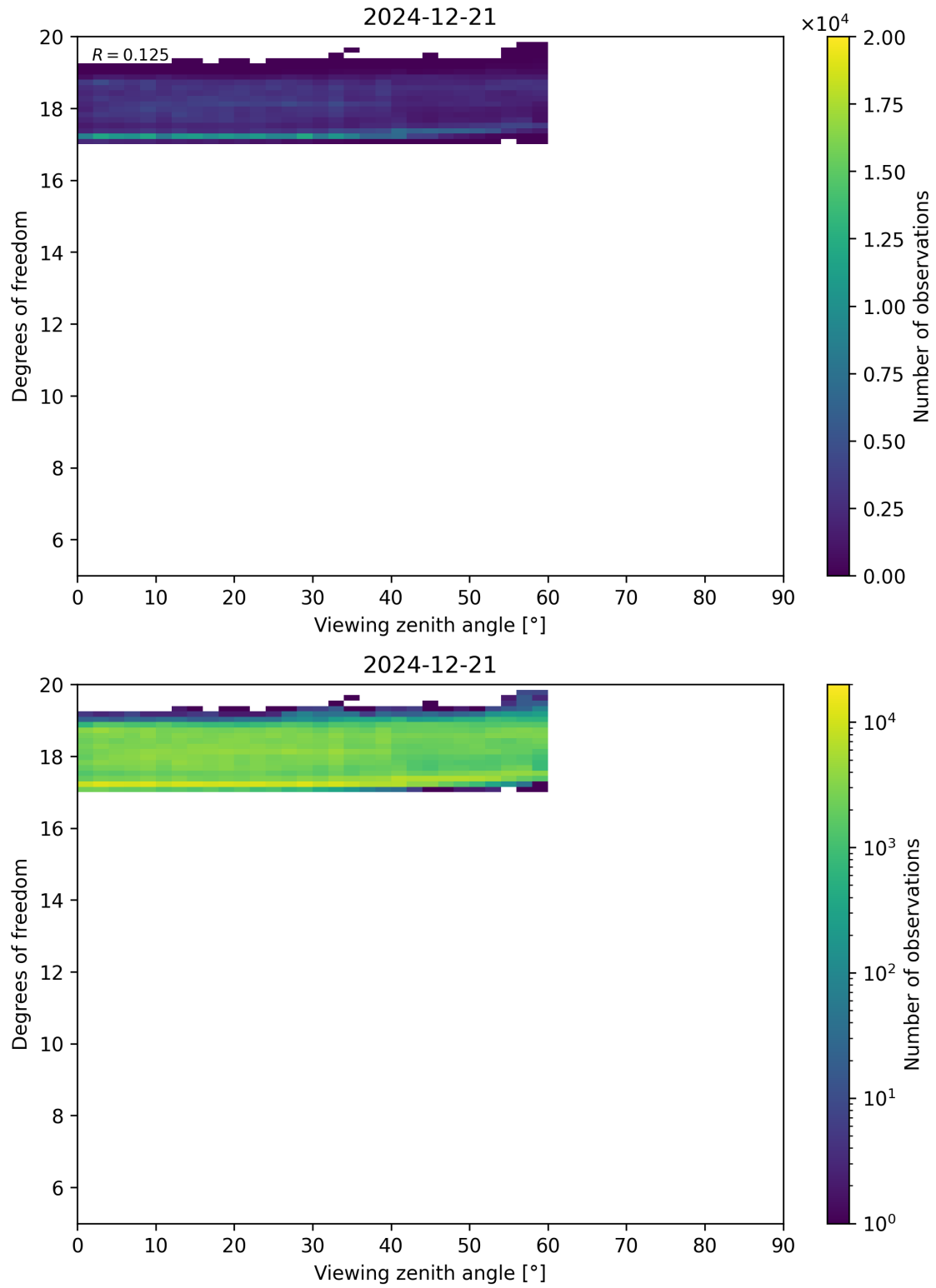
Figure 107: Scatter density plot of “Viewing zenith angle” against “Degrees of freedom” for 2024-12-20 to 2024-12-22.
