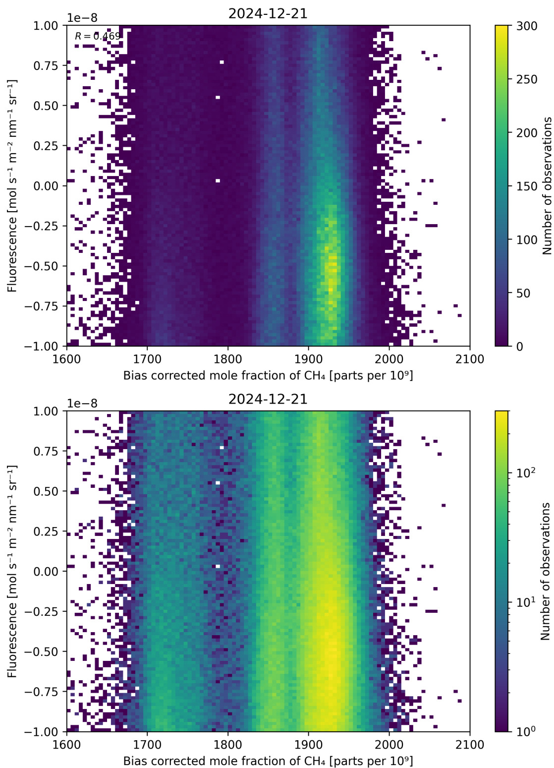
Figure 66: Scatter density plot of “Bias corrected mole fraction of \text{CH}_4 ” against “Fluorescence” for 2024-12-20 to 2024-12-22.
