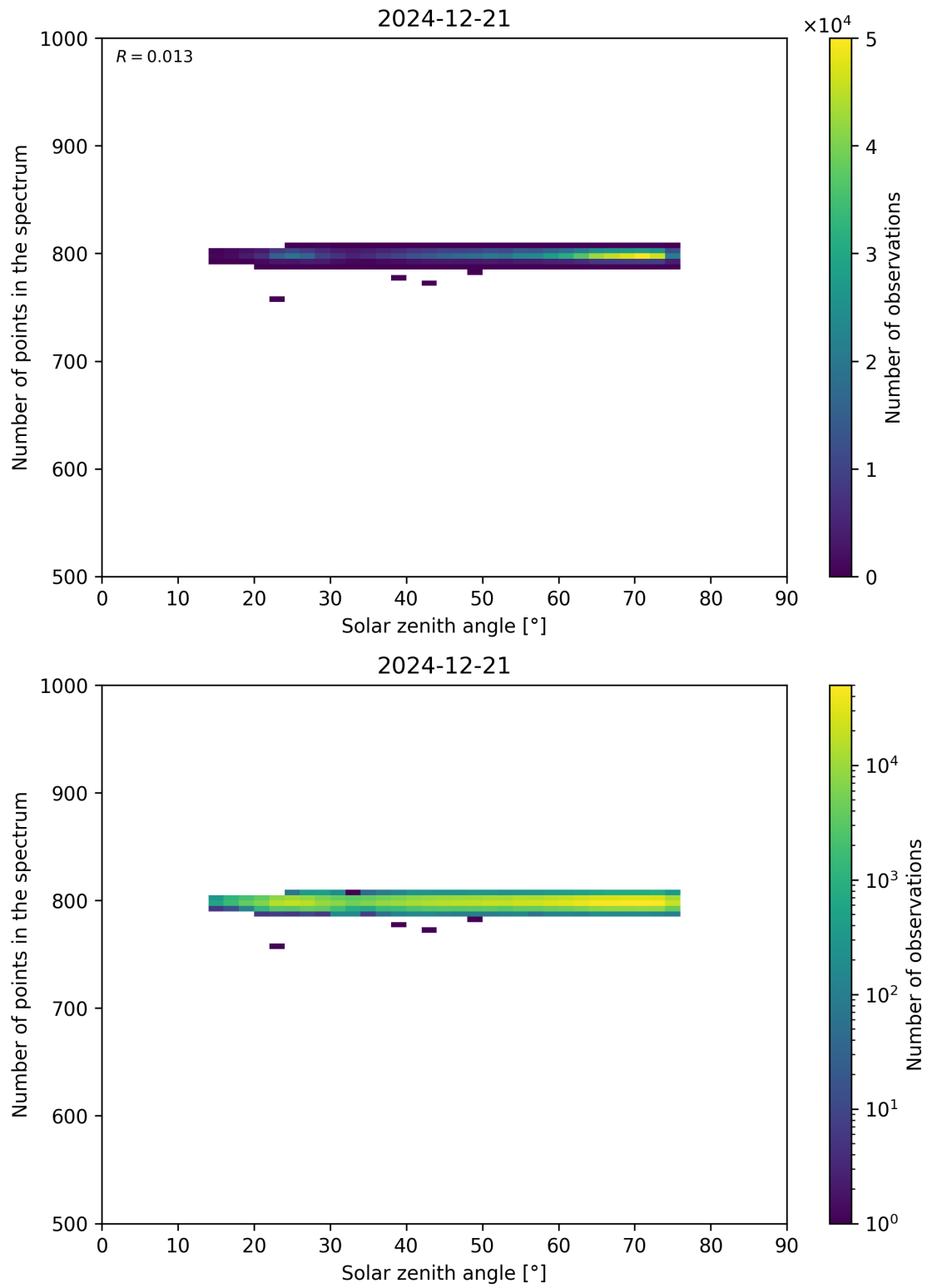
Figure 103: Scatter density plot of “Solar zenith angle” against “Number of points in the spectrum” for 2024-12-20 to 2024-12-22.
