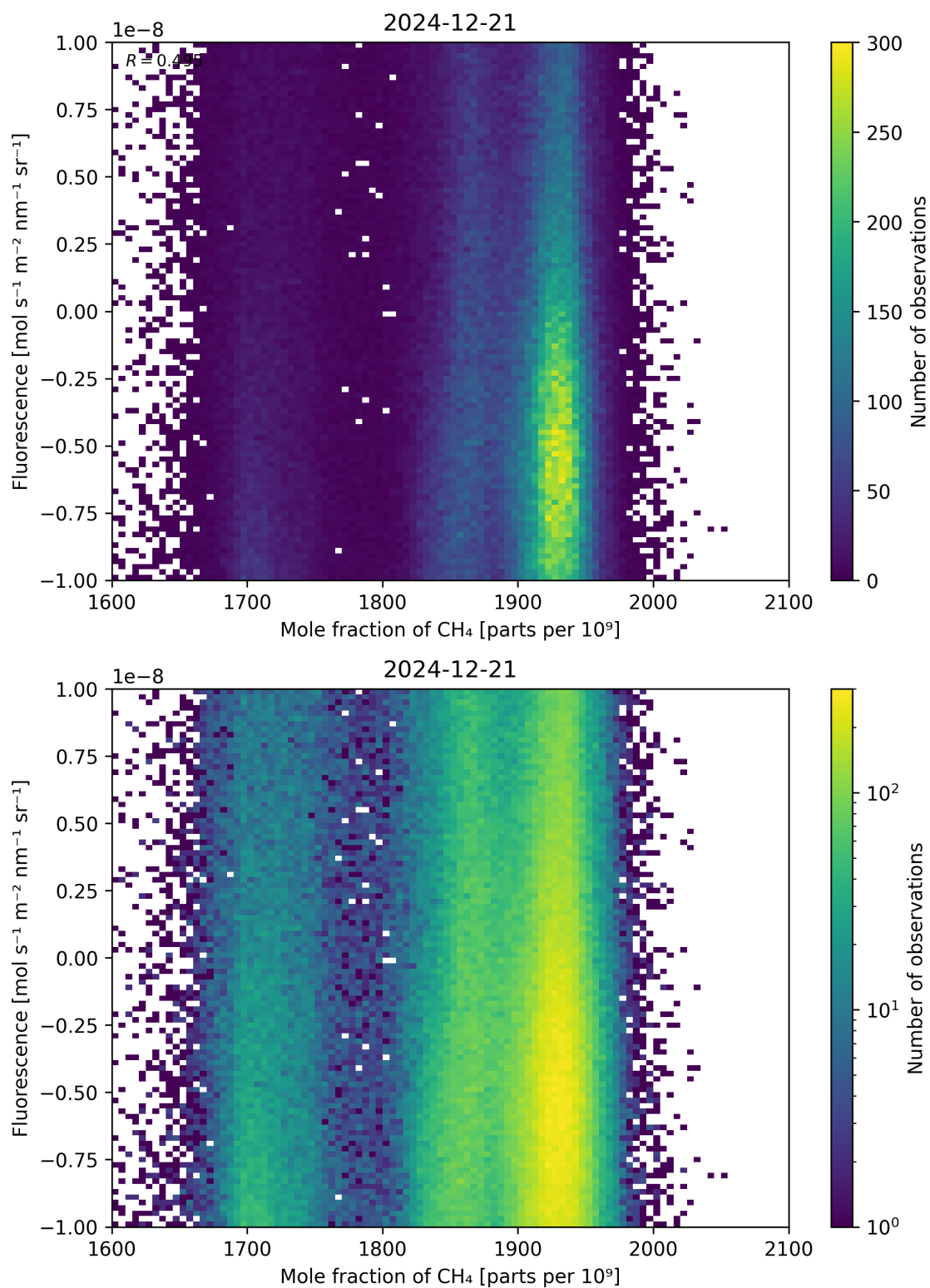
Figure 73: Scatter density plot of “Mole fraction of \text{CH}_4 ” against “Fluorescence” for 2024-12-20 to 2024-12-22.
