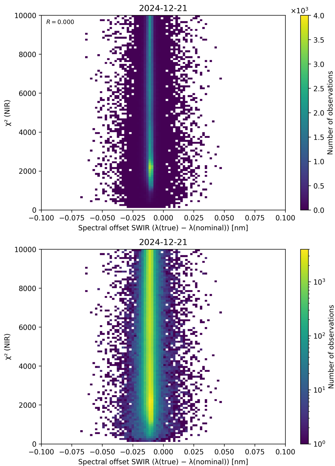
Figure 117: Scatter density plot of “Spectral offset SWIR ( \lambda_{\text{true}} - \lambda_{\text{nominal}} )” against “ \chi^2 (NIR)” for 2024-12-20 to 2024-12-22.
