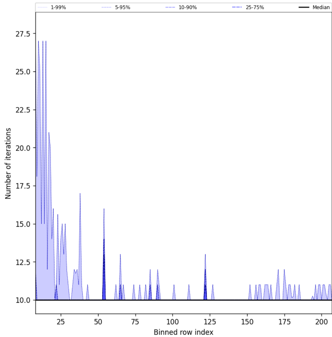
Figure 42: Along track statistics of “Number of iterations” for 2024-12-20 to 2024-12-22
