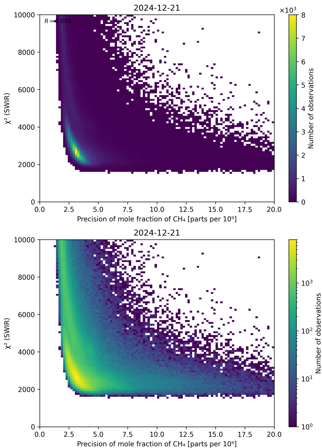
Figure 79: Scatter density plot of “Precision of mole fraction of CH 4 ” against “ \chi^2 (SWIR)” for 2024-12-20 to 2024-12-22.
