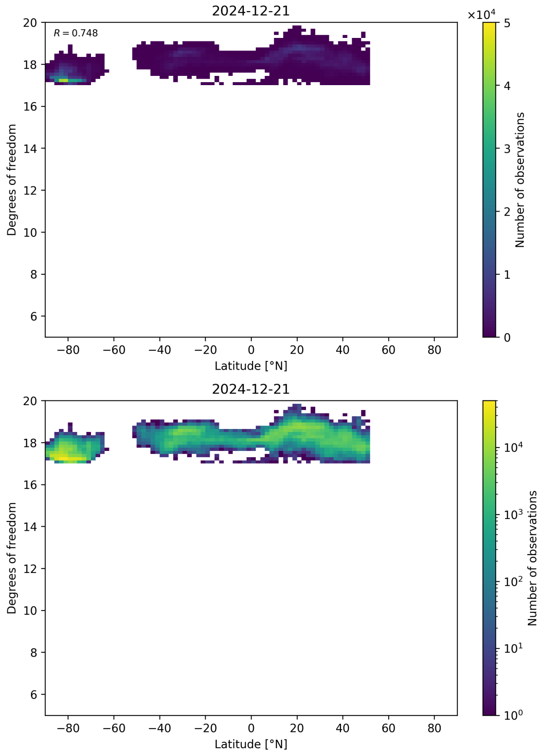
Figure 55: Scatter density plot of “Latitude” against “Degrees of freedom” for 2024-12-20 to 2024-12-22.
