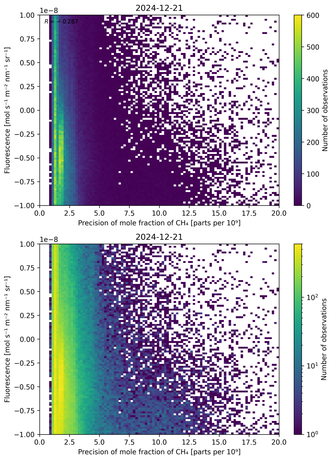
Figure 81: Scatter density plot of “Precision of mole fraction of \text{CH}_4 ” against “Fluorescence” for 2024-12-20 to 2024-12-22.
