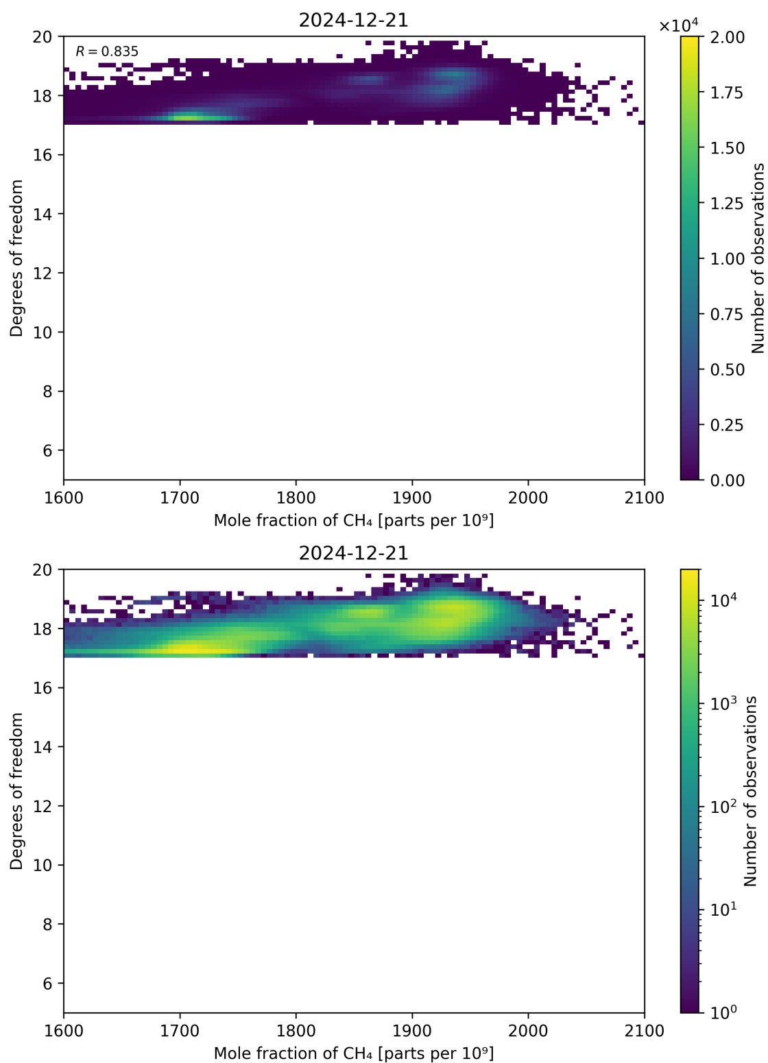
Figure 72: Scatter density plot of “Mole fraction of CH 4 ” against “Degrees of freedom” for 2024-12-20 to 2024-12-22.
