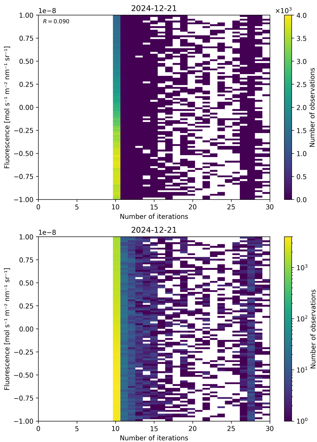
Figure 87: Scatter density plot of “Number of iterations” against “Fluorescence” for 2024-12-20 to 2024-12-22.
