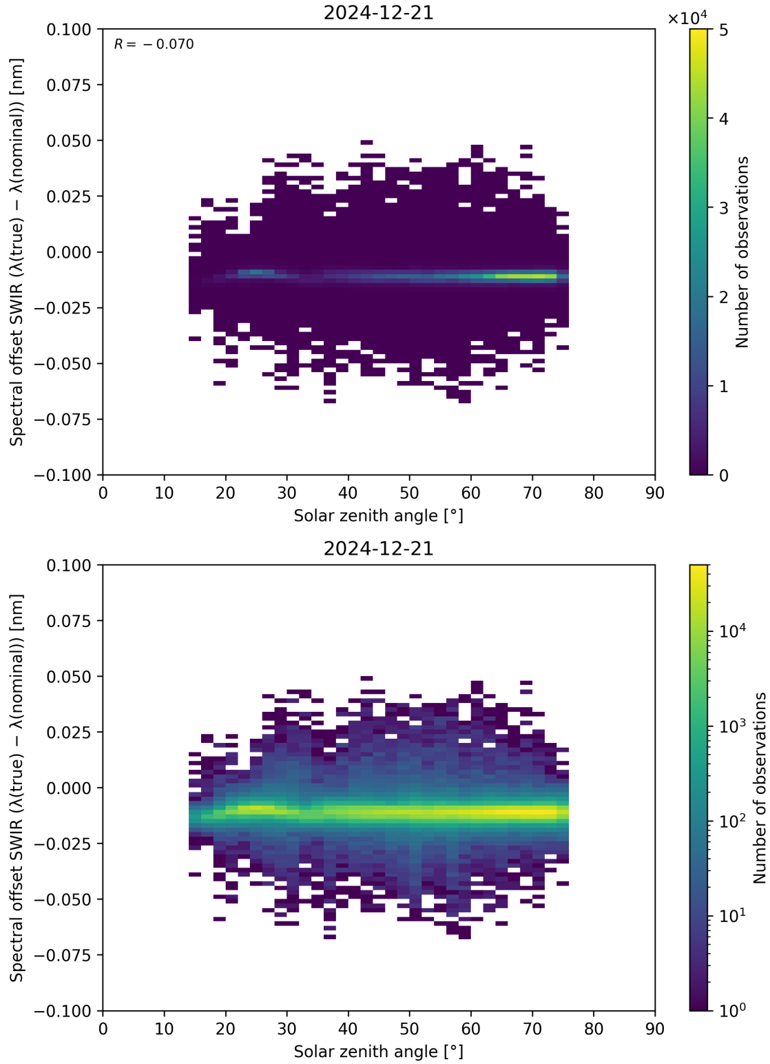
Figure 104: Scatter density plot of “Solar zenith angle” against “Spectral offset SWIR ( \lambda_{\text{true}} - \lambda_{\text{nominal}} )” for 2024-12-20 to 2024-12-22.
