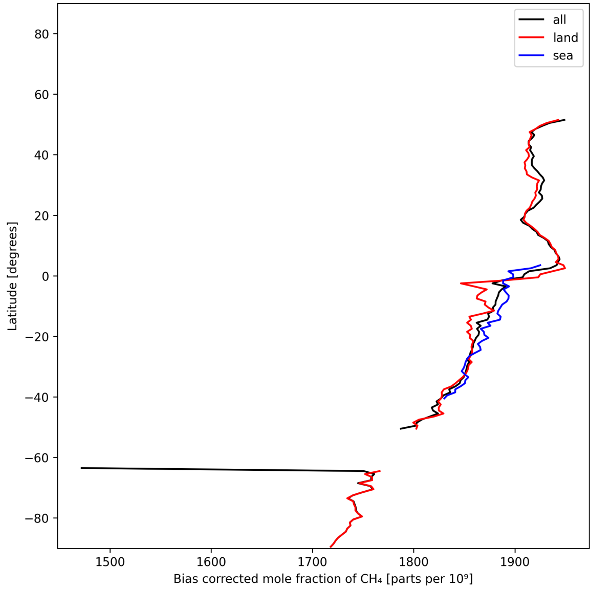
Figure 14: Zonal average of “Bias corrected mole fraction of CH 4 ” for 2024-12-20 to 2024-12-22.
