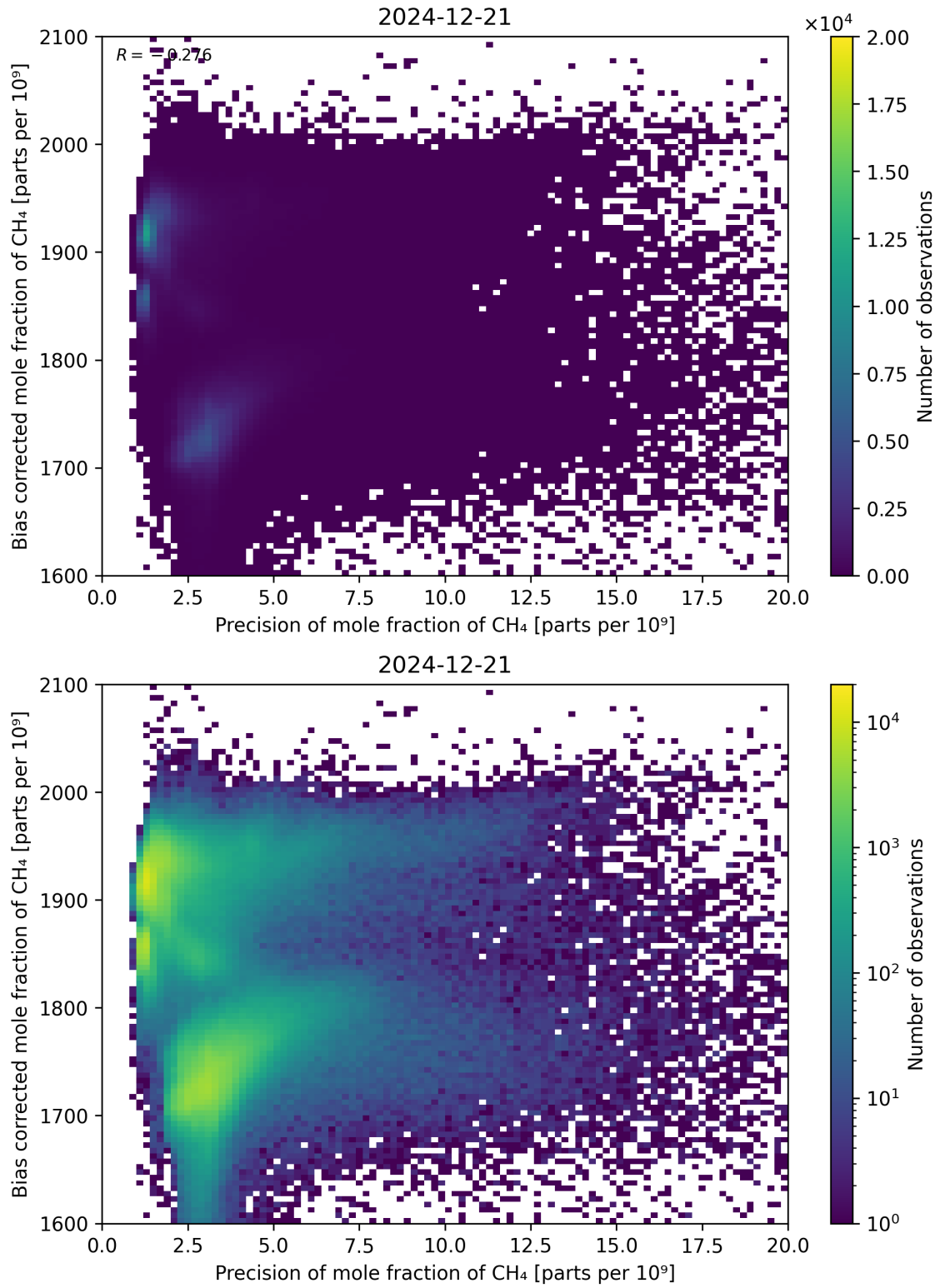
Figure 82: Scatter density plot of “Precision of mole fraction of \text{CH}_4 ” against “Bias corrected mole fraction of \text{CH}_4 ” for 2024-12-20 to 2024-12-22.
