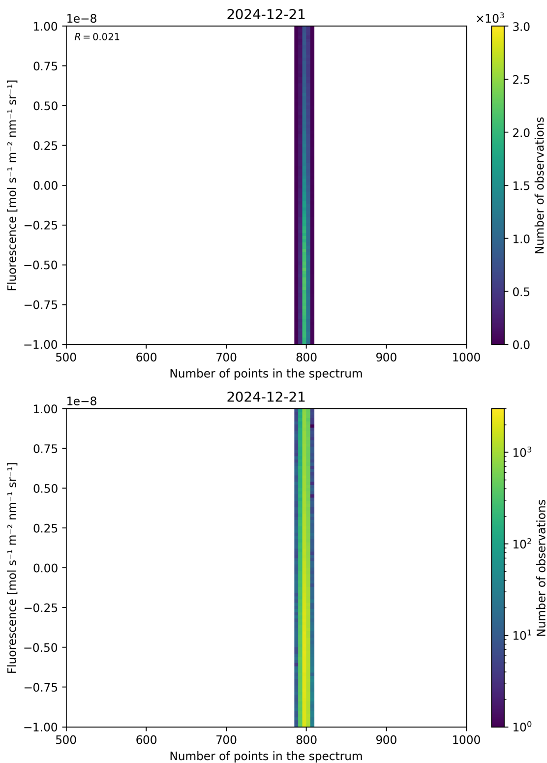
Figure 91: Scatter density plot of “Number of points in the spectrum” against “Fluorescence” for 2024-12-20 to 2024-12-22.
