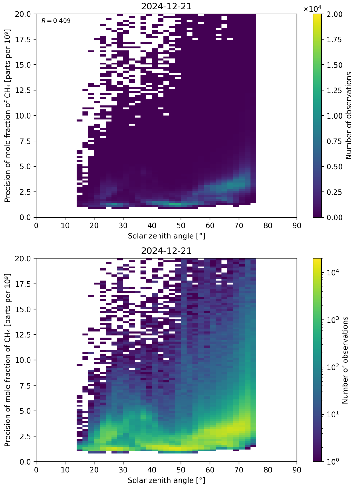
Figure 101: Scatter density plot of “Solar zenith angle” against “Precision of mole fraction of \text{CH}_4 ” for 2024-12-20 to 2024-12-22.
