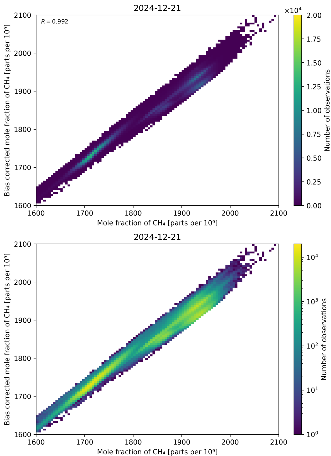
Figure 74: Scatter density plot of “Mole fraction of CH 4 ” against “Bias corrected mole fraction of CH 4 ” for 2024-12-20 to 2024-12-22.
