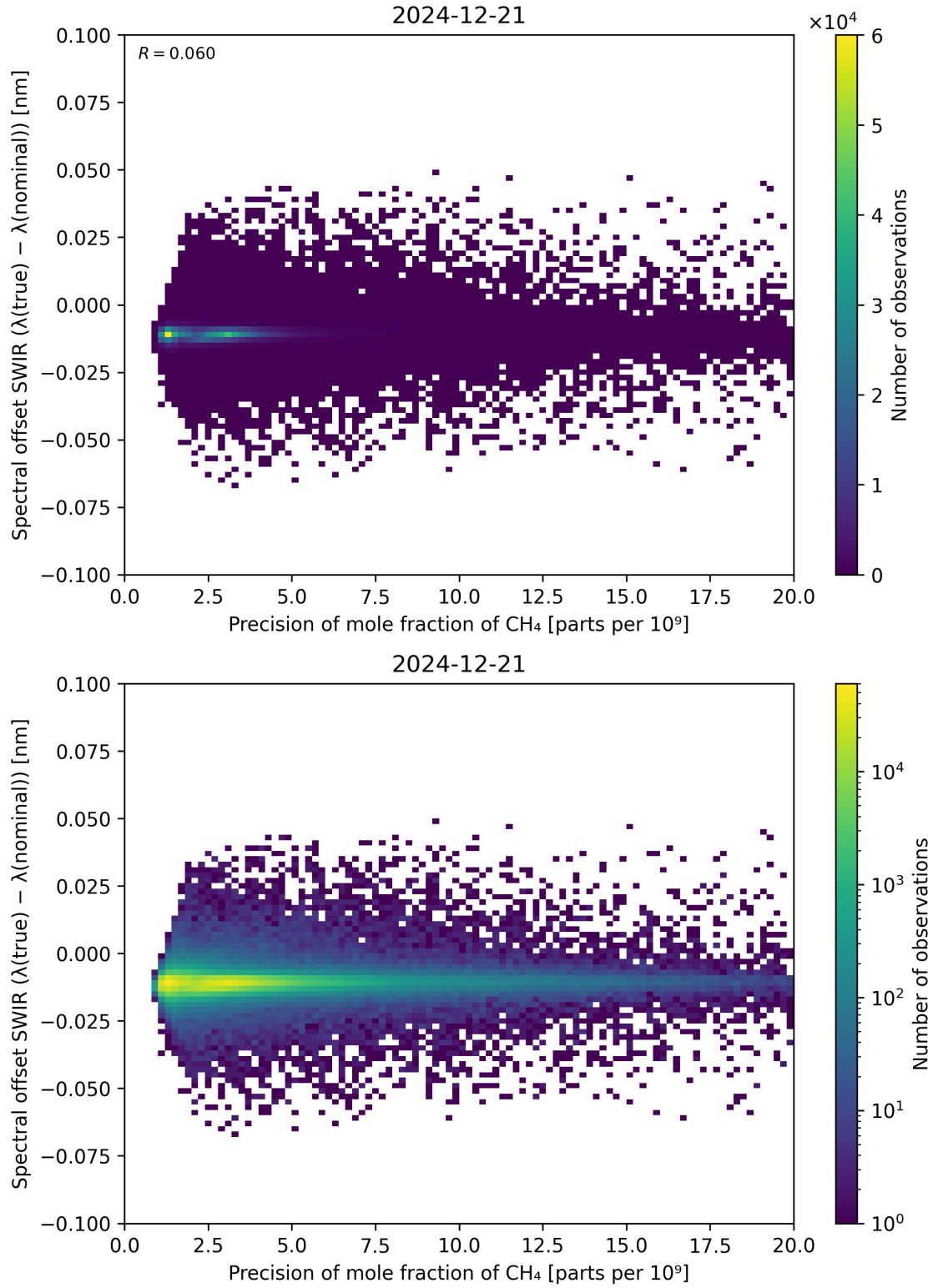
Figure 85: Scatter density plot of “Precision of mole fraction of \text{CH}_4 ” against “Spectral offset SWIR ( \lambda_{\text{true}} - \lambda_{\text{nominal}} )” for 2024-12-20 to 2024-12-22.
