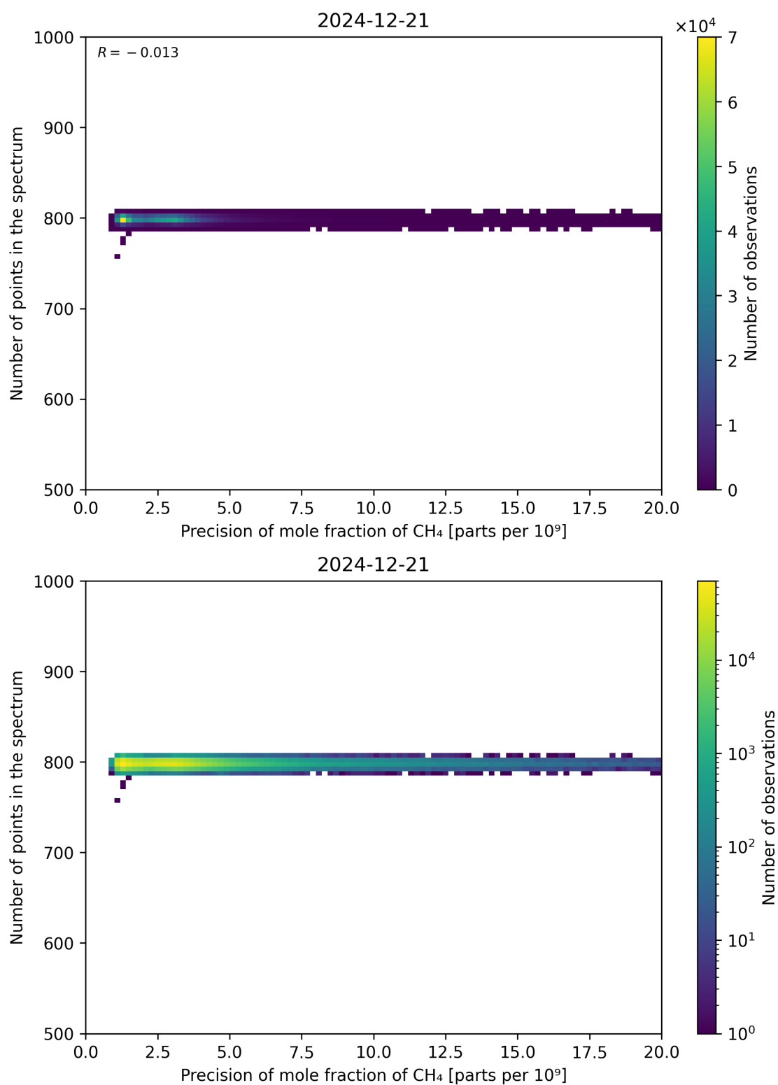
Figure 84: Scatter density plot of “Precision of mole fraction of CH 4 ” against “Number of points in the spectrum” for 2024-12-20 to 2024-12-22.
