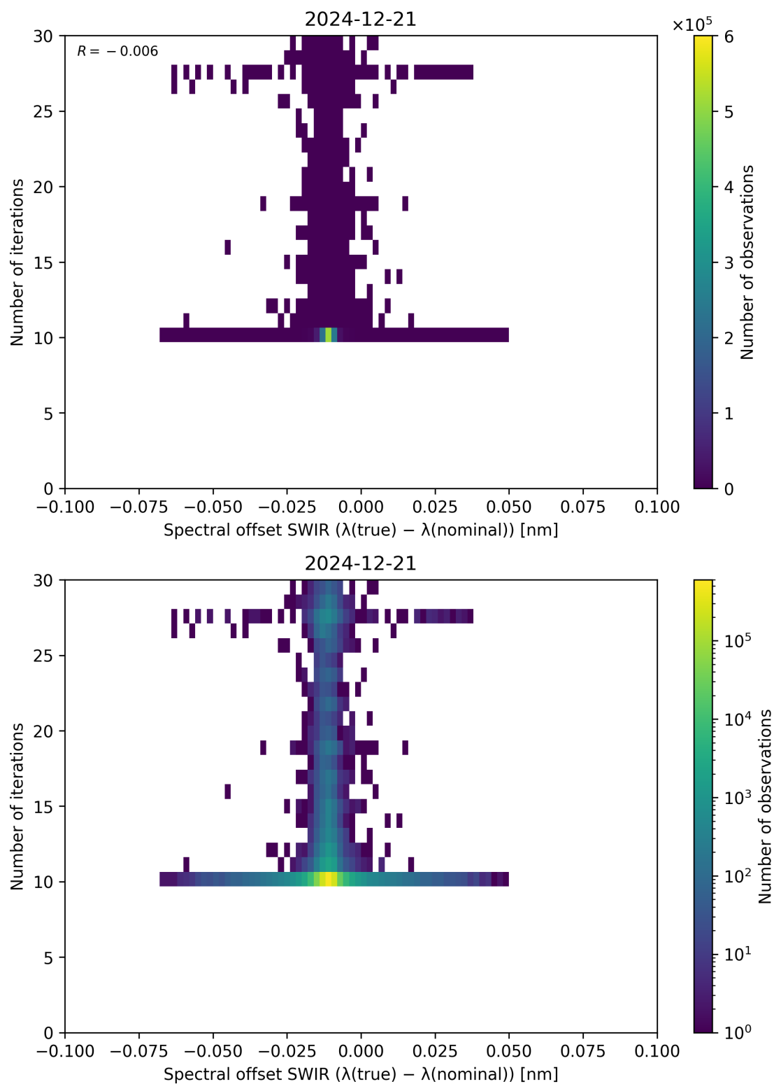
Figure 121: Scatter density plot of “Spectral offset SWIR ( \lambda_{\text{true}} - \lambda_{\text{nominal}} )” against “Number of iterations” for 2024-12-20 to 2024-12-22.
