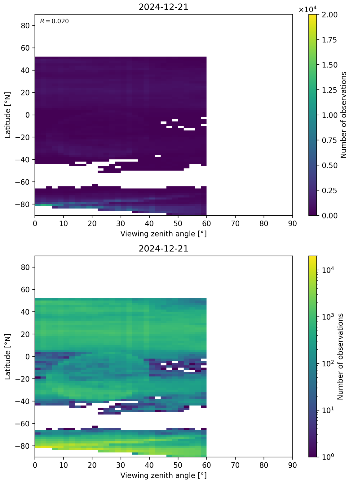
Figure 109: Scatter density plot of “Viewing zenith angle” against “Latitude” for 2024-12-20 to 2024-12-22.
