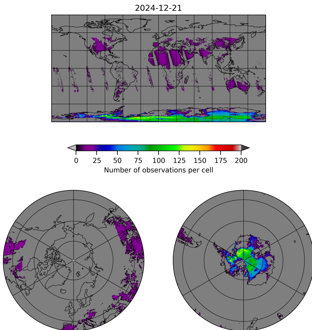
Figure 10: Map of the number of observations for 2024-12-20 to 2024-12-22
