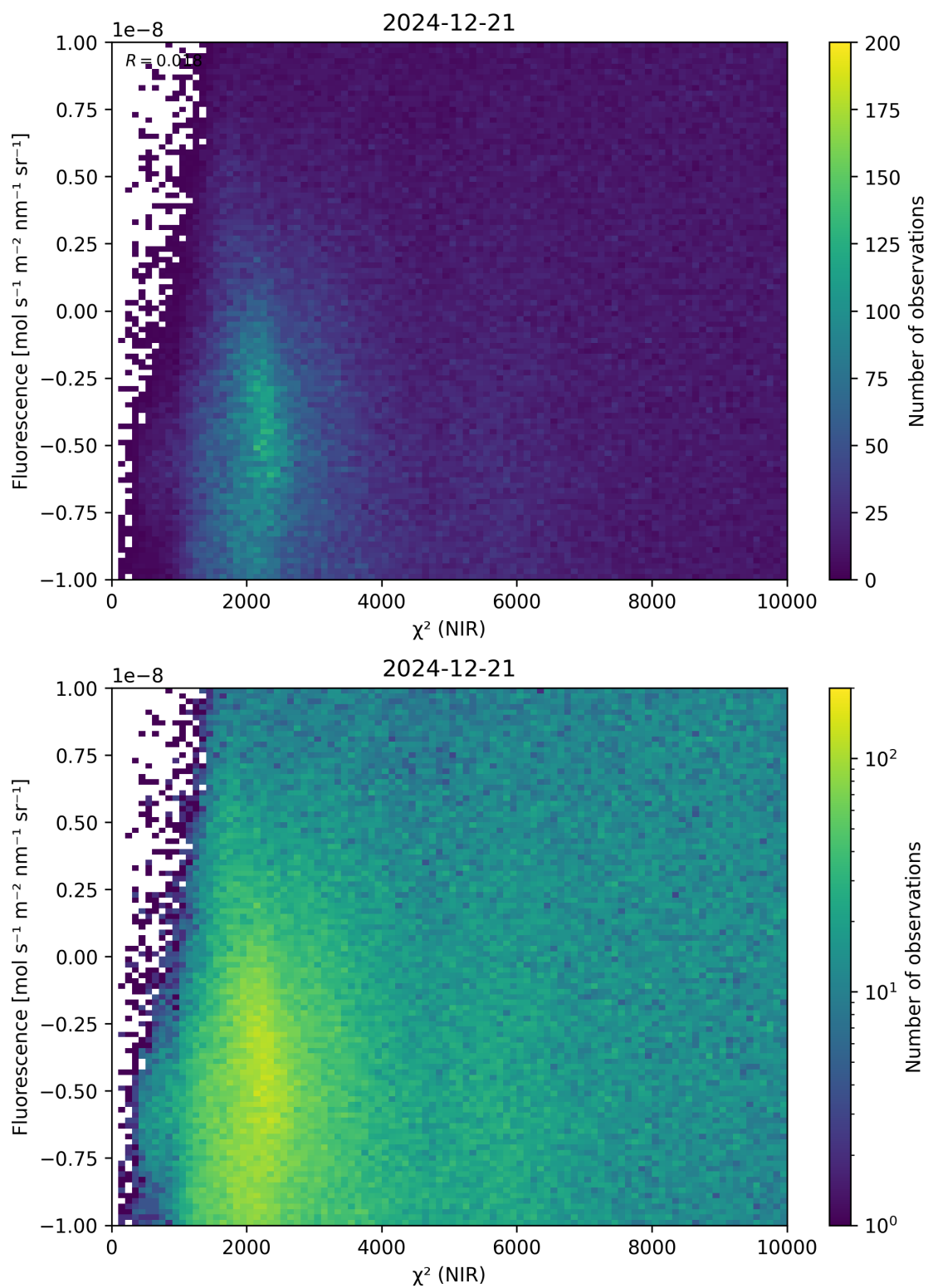
Figure 45: Scatter density plot of “ \chi^2 (NIR)” against “Fluorescence” for 2024-12-20 to 2024-12-22.
