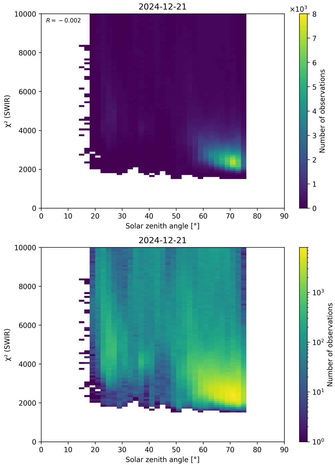
Figure 95: Scatter density plot of “Solar zenith angle” against “ \chi^2 (SWIR)” for 2024-12-20 to 2024-12-22.
