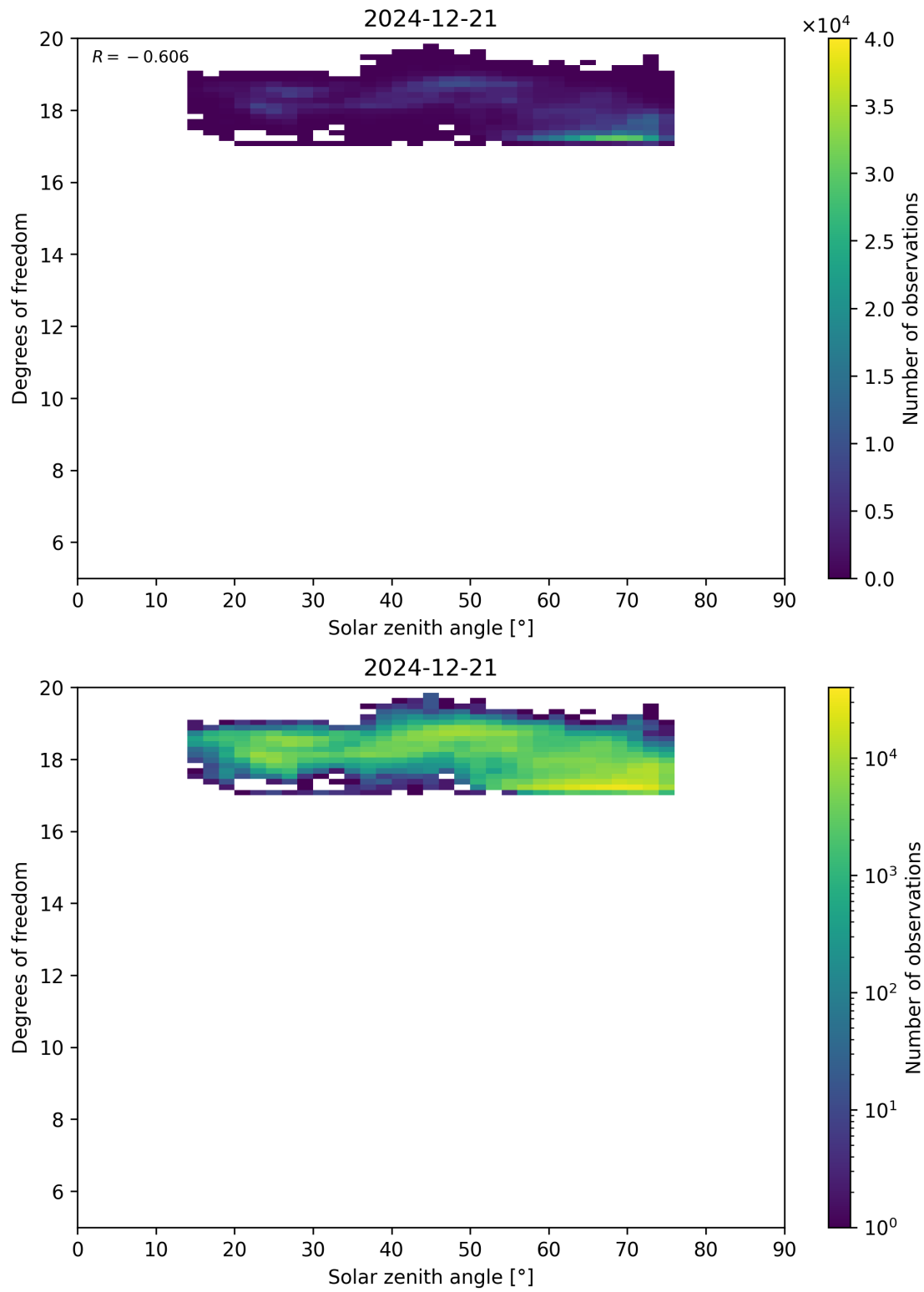
Figure 96: Scatter density plot of “Solar zenith angle” against “Degrees of freedom” for 2024-12-20 to 2024-12-22.
