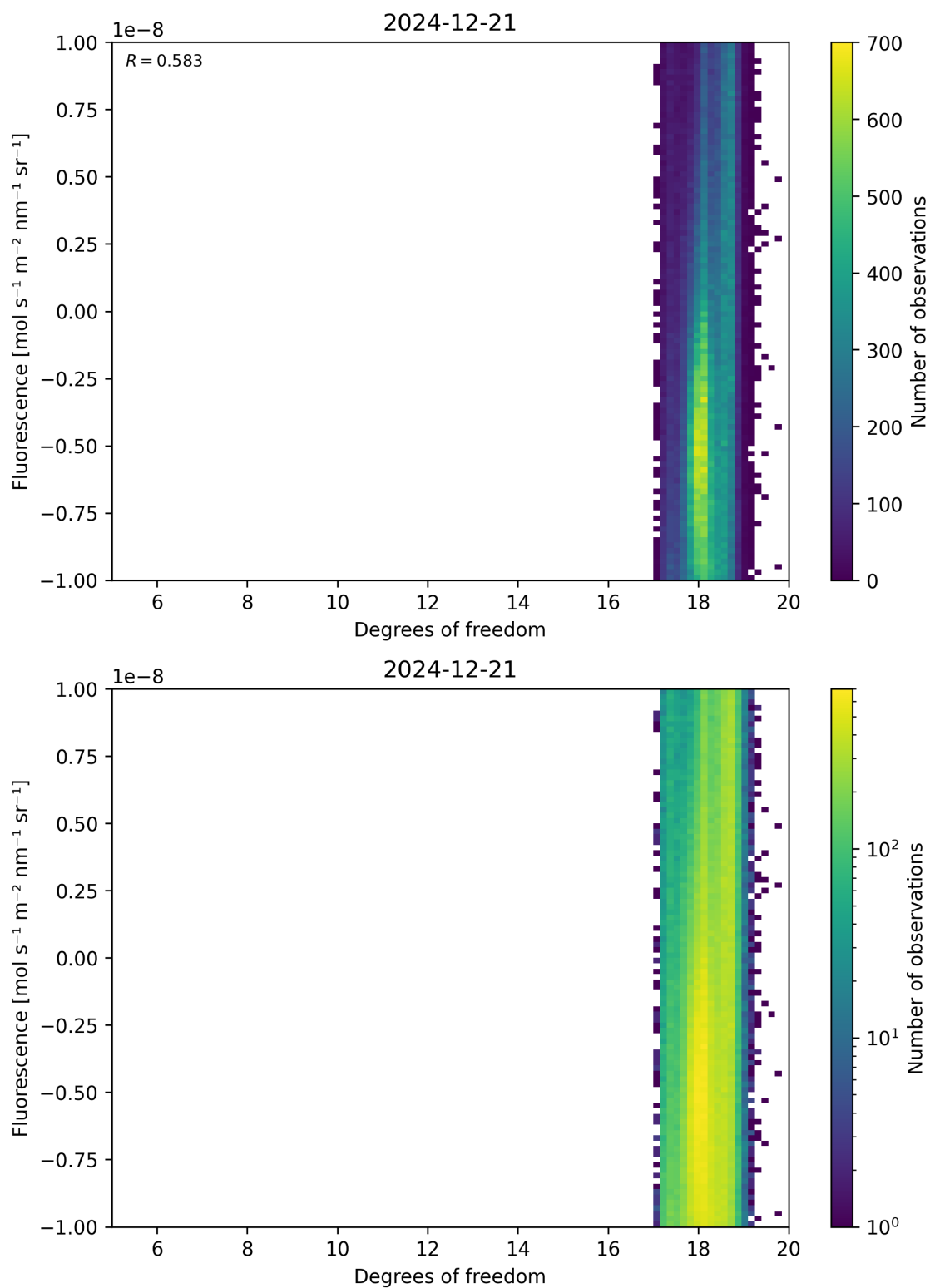
Figure 51: Scatter density plot of “Degrees of freedom” against “Fluorescence” for 2024-12-20 to 2024-12-22.
