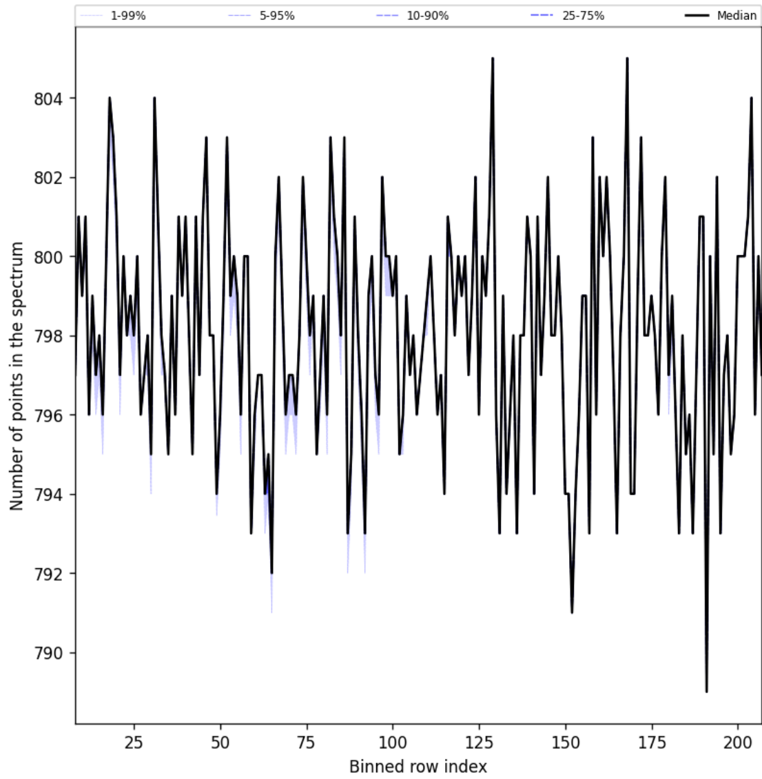
Figure 37: Along track statistics of “Number of points in the spectrum” for 2024-12-20 to 2024-12-22
