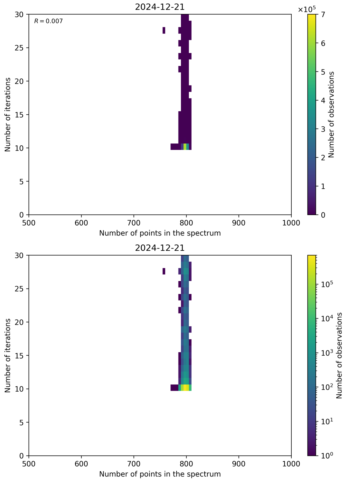
Figure 92: Scatter density plot of “Number of points in the spectrum” against “Number of iterations” for 2024-12-20 to 2024-12-22.
