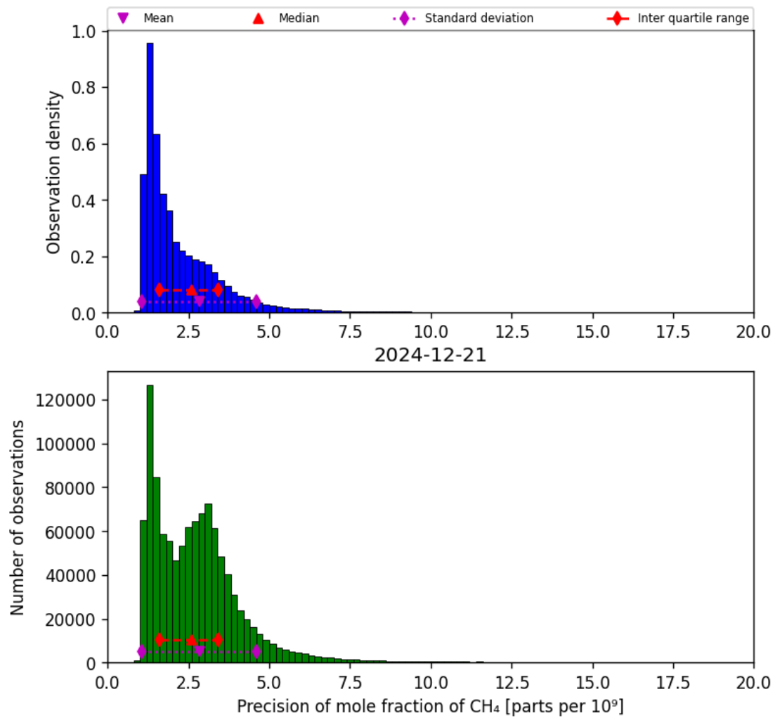
Figure 24: Histogram of “Precision of mole fraction of CH 4 ” for 2024-12-20 to 2024-12-22
