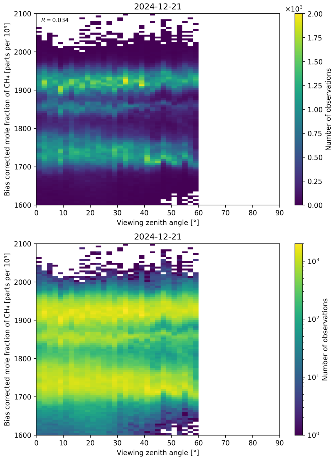
Figure 111: Scatter density plot of “Viewing zenith angle” against “Bias corrected mole fraction of CH 4 ” for 2024-12-20 to 2024-12-22.
