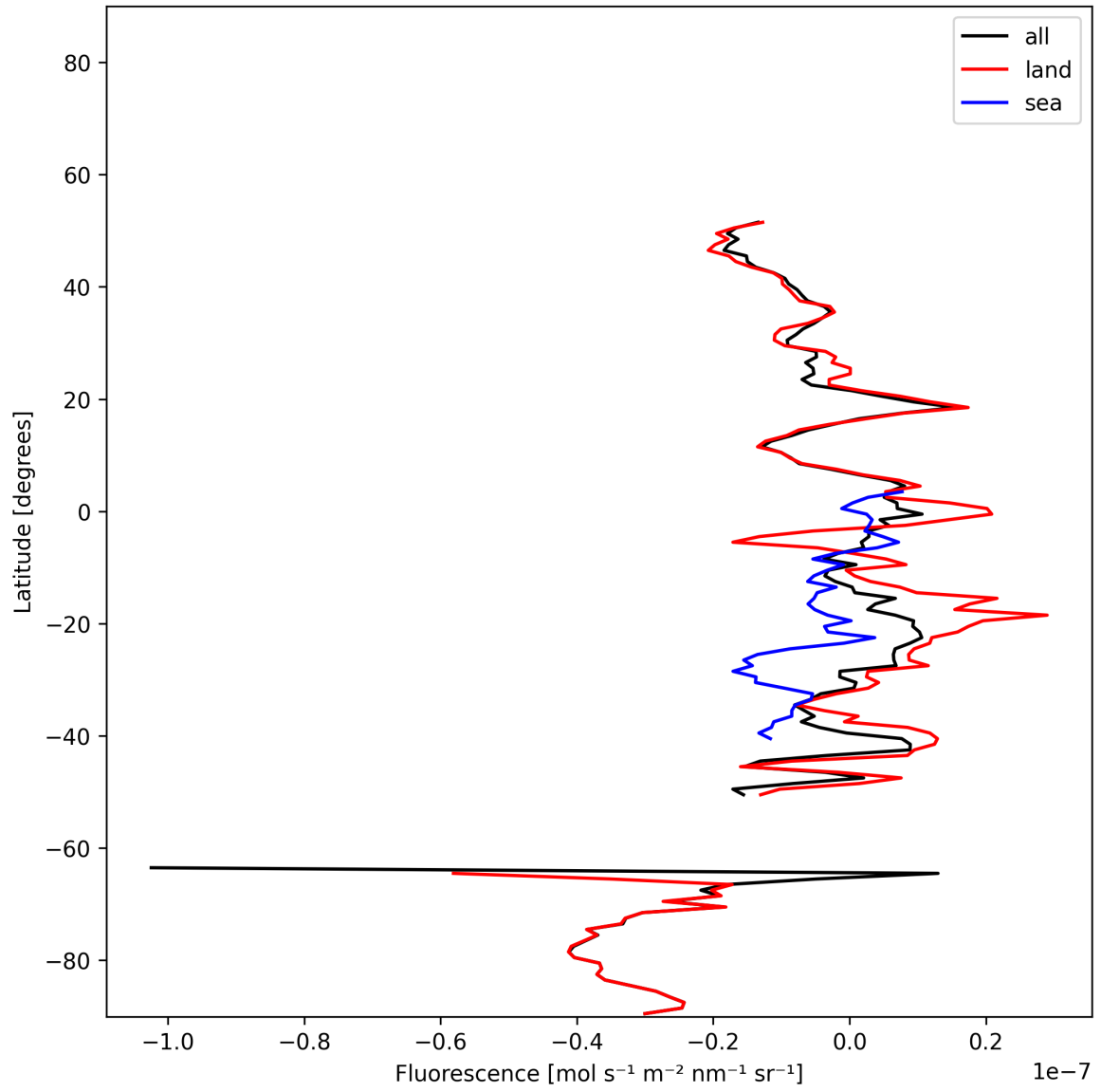
Figure 21: Zonal average of “Fluorescence” for 2024-12-20 to 2024-12-22.
