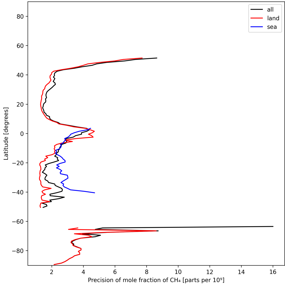
Figure 13: Zonal average of “Precision of mole fraction of CH 4 ” for 2024-12-20 to 2024-12-22.
