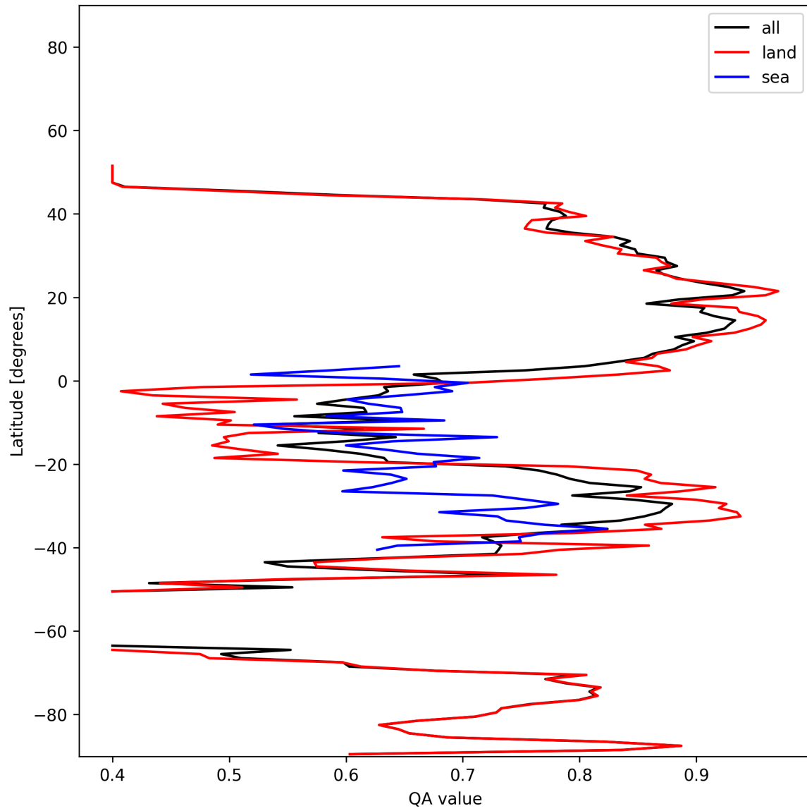
Figure 11: Zonal average of “QA value” for 2024-12-20 to 2024-12-22.
