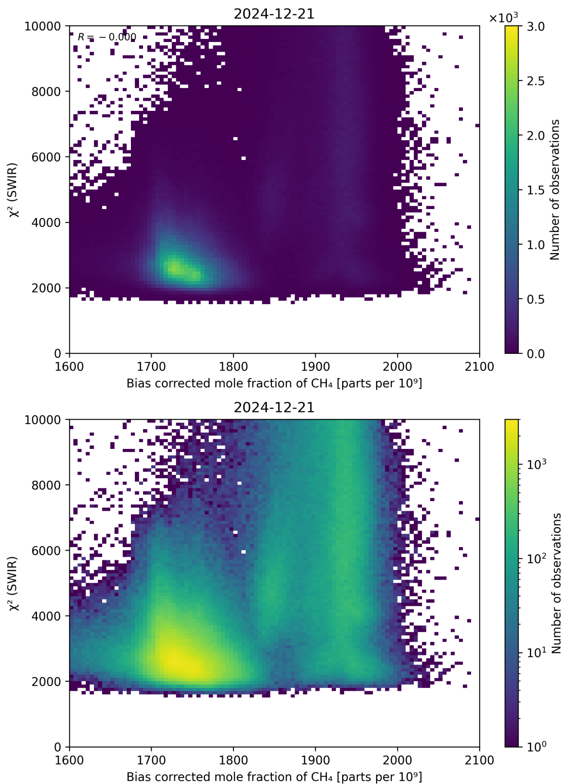
Figure 64: Scatter density plot of “Bias corrected mole fraction of CH 4 ” against “ \chi^2 (SWIR)” for 2024-12-20 to 2024-12-22.
