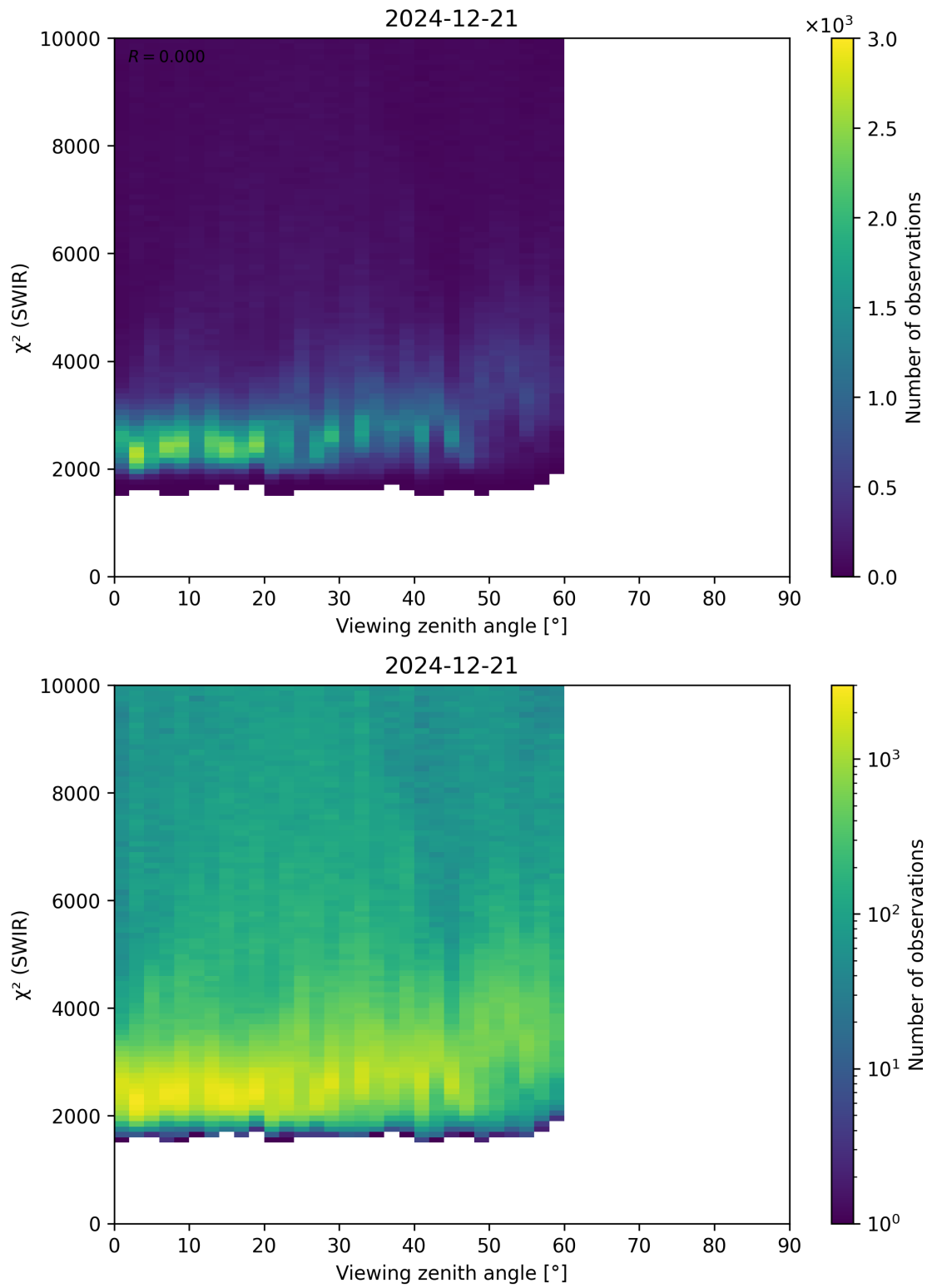
Figure 106: Scatter density plot of “Viewing zenith angle” against “ \chi^2 (SWIR)” for 2024-12-20 to 2024-12-22.
