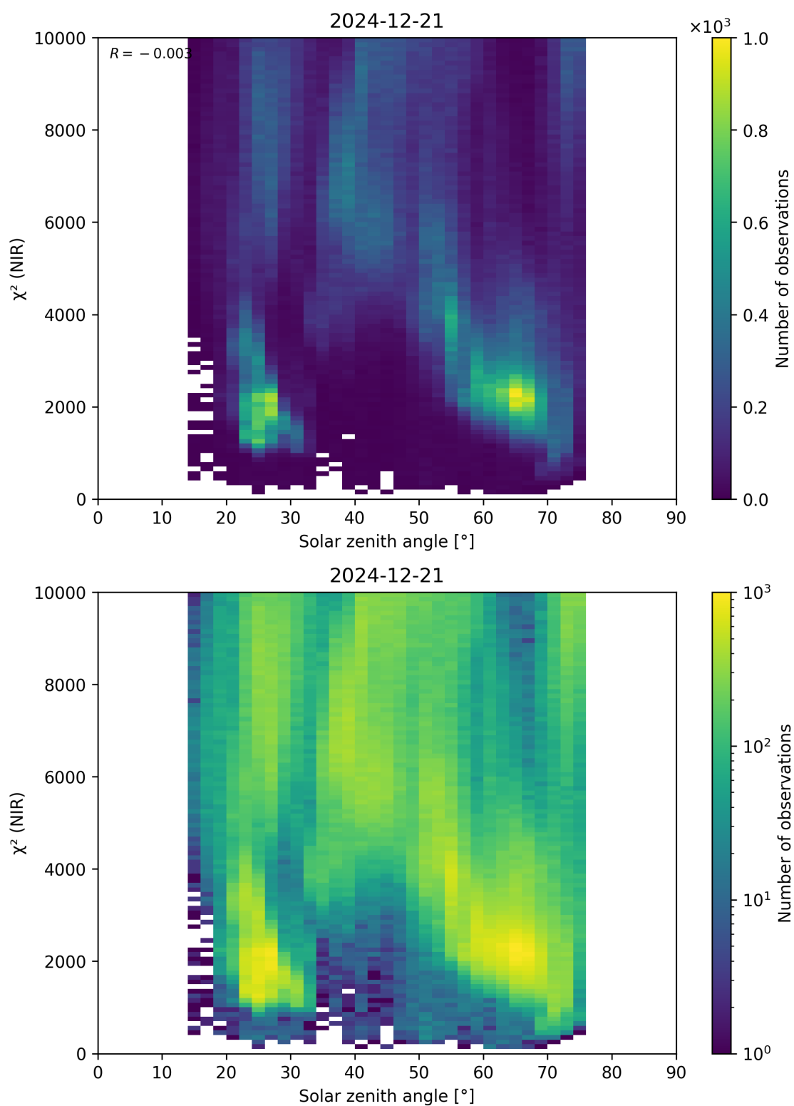
Figure 94: Scatter density plot of “Solar zenith angle” against “ \chi^2 (NIR)” for 2024-12-20 to 2024-12-22.
