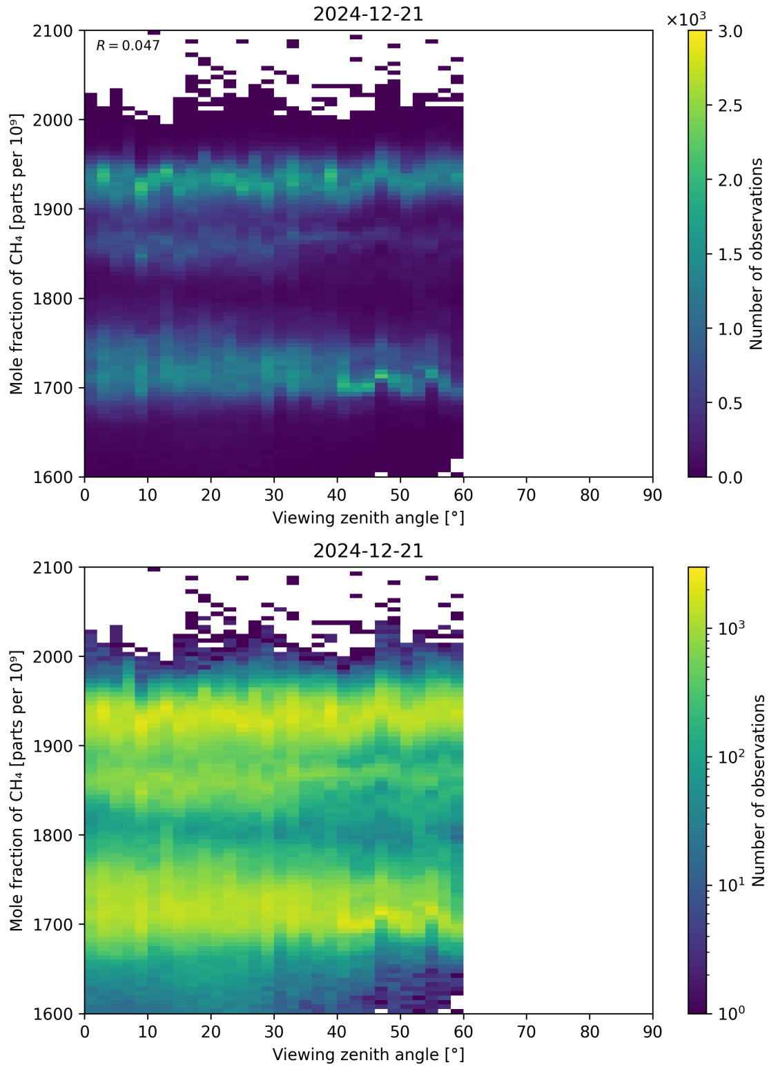
Figure 110: Scatter density plot of “Viewing zenith angle” against “Mole fraction of CH 4 ” for 2024-12-20 to 2024-12-22.
