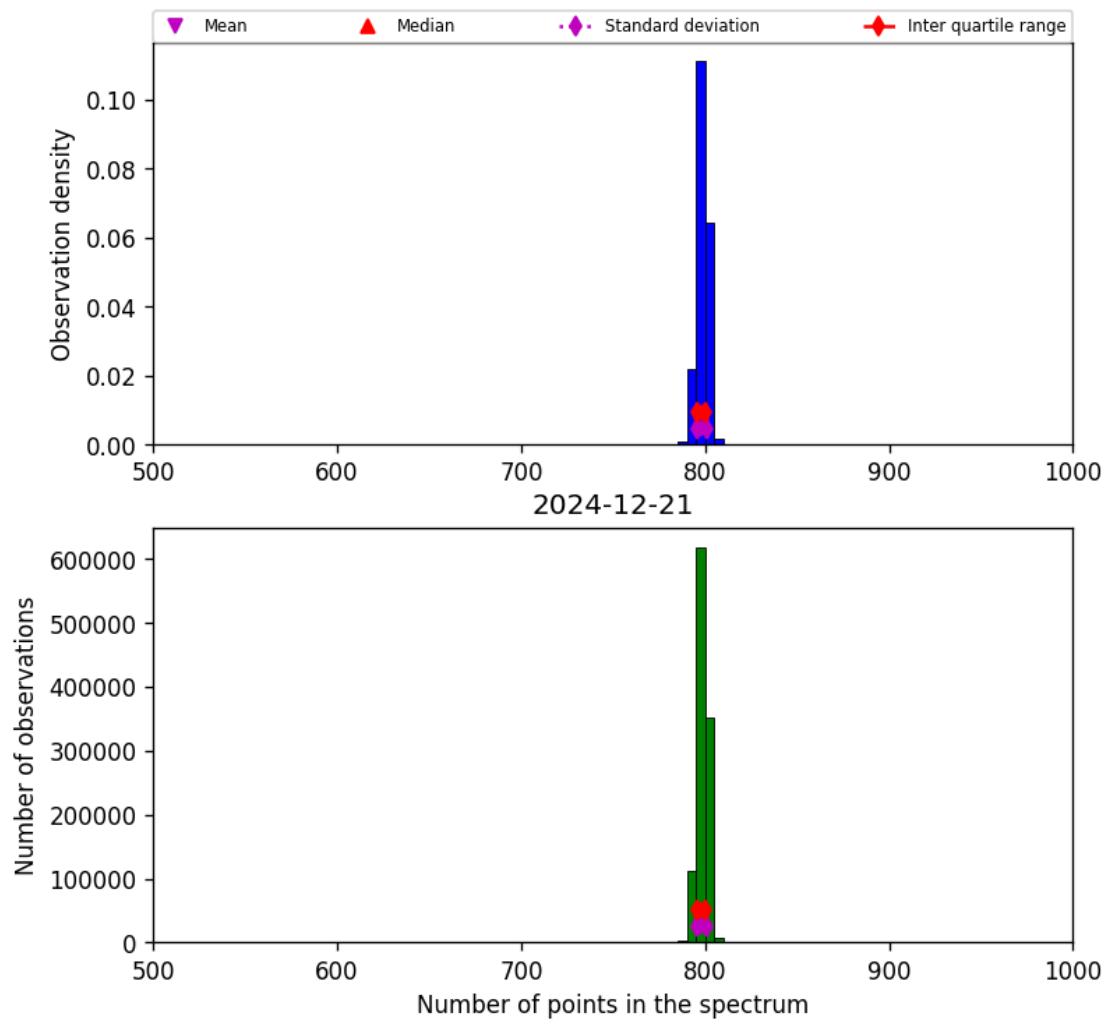
Figure 26: Histogram of “Number of points in the spectrum” for 2024-12-20 to 2024-12-22
