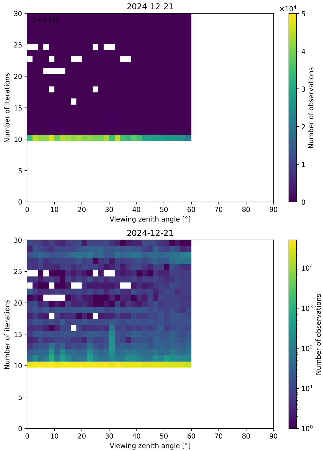
Figure 113: Scatter density plot of “Viewing zenith angle” against “Number of iterations” for 2024-12-20 to 2024-12-22.
