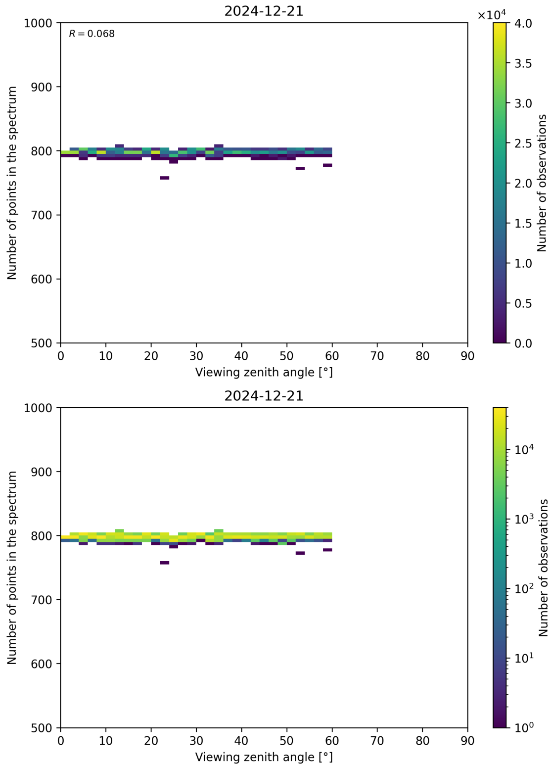
Figure 114: Scatter density plot of “Viewing zenith angle” against “Number of points in the spectrum” for 2024-12-20 to 2024-12-22.
