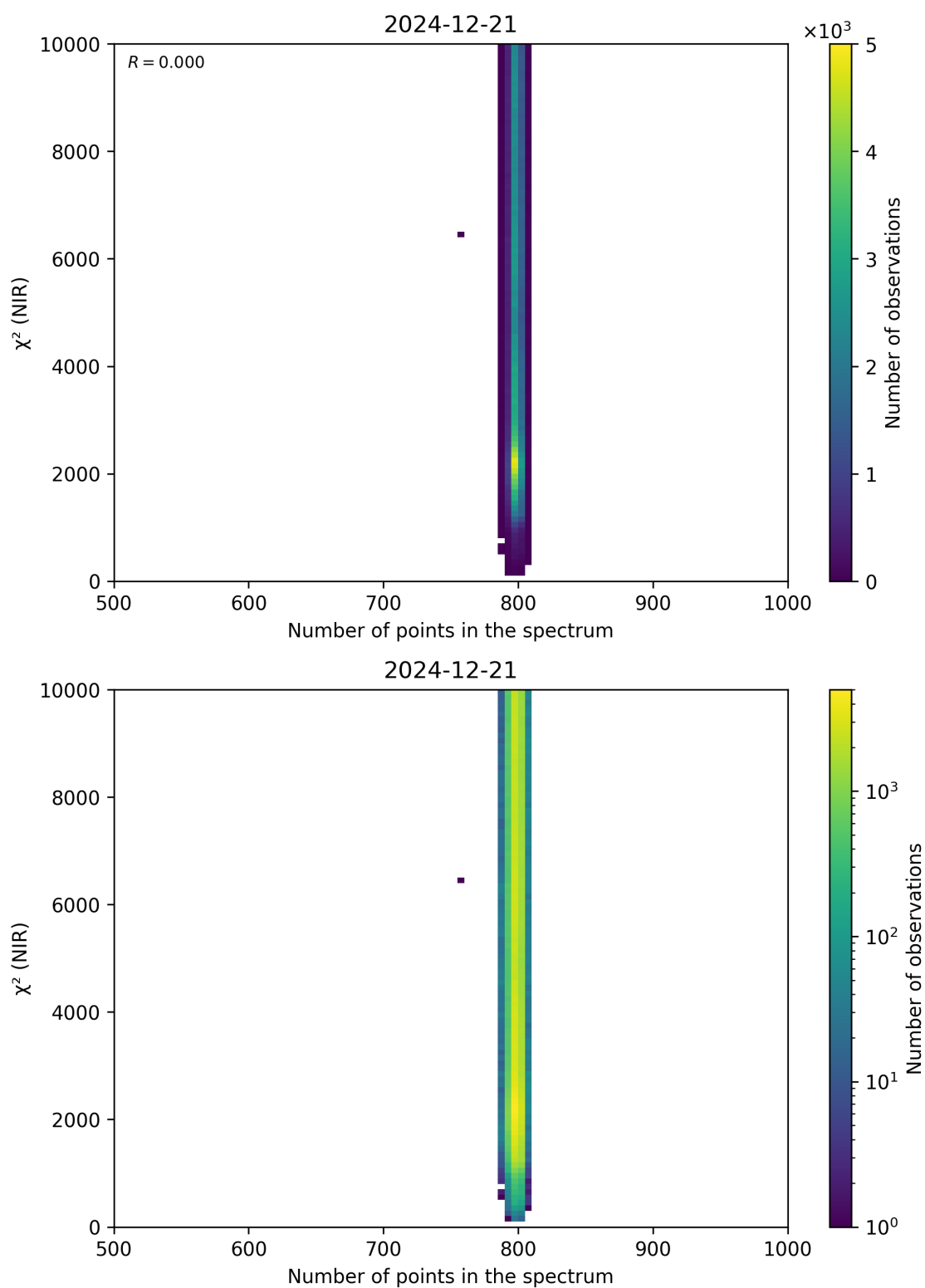
Figure 88: Scatter density plot of “Number of points in the spectrum” against “ \chi^2 (NIR)” for 2024-12-20 to 2024-12-22.
