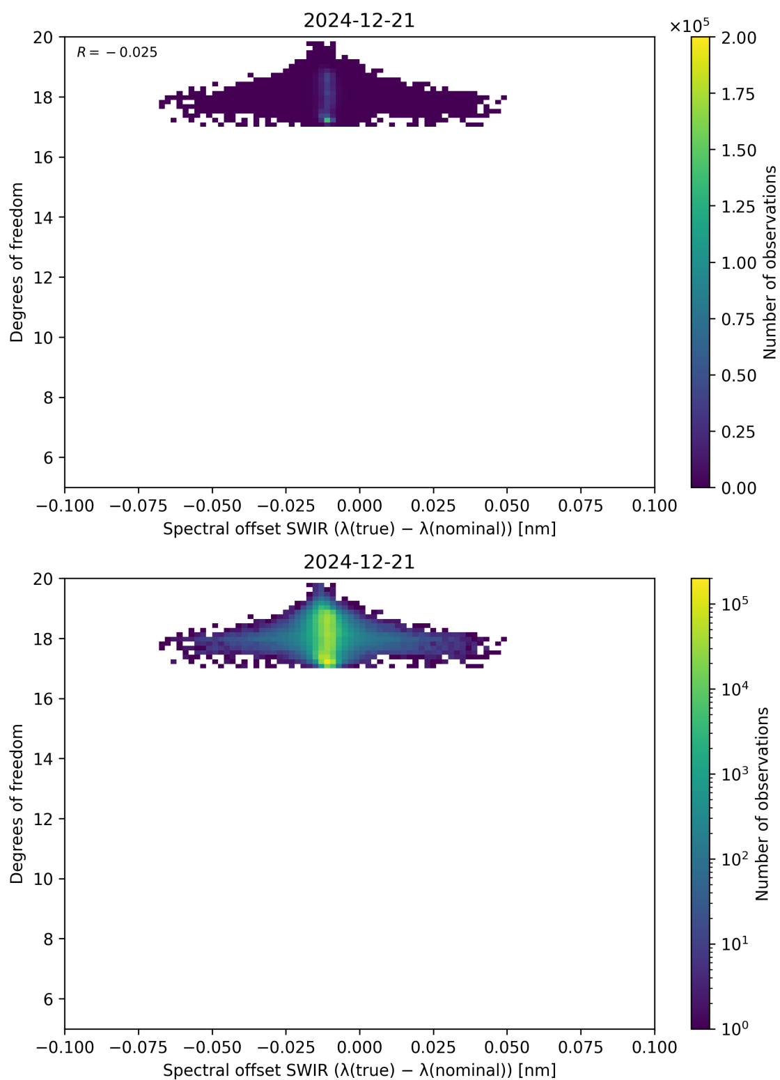
Figure 119: Scatter density plot of “Spectral offset SWIR ( \lambda_{\text{true}} - \lambda_{\text{nominal}} )” against “Degrees of freedom” for 2024-12-20 to 2024-12-22.
