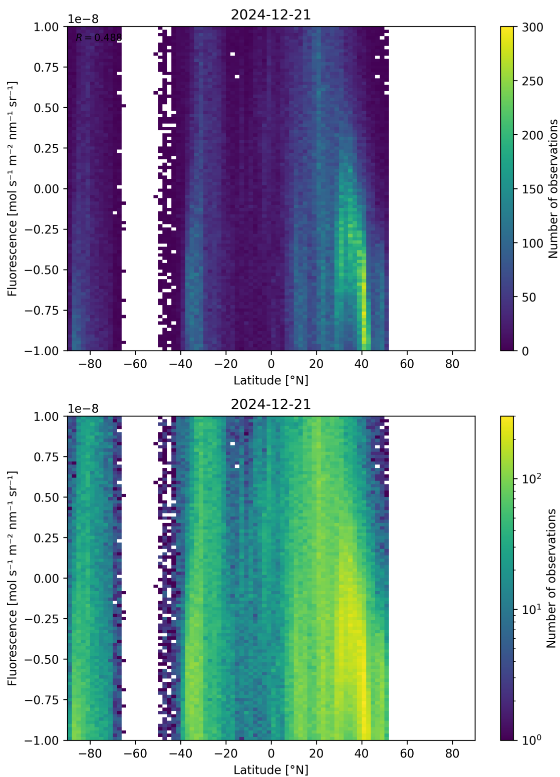
Figure 56: Scatter density plot of “Latitude” against “Fluorescence” for 2024-12-20 to 2024-12-22.
