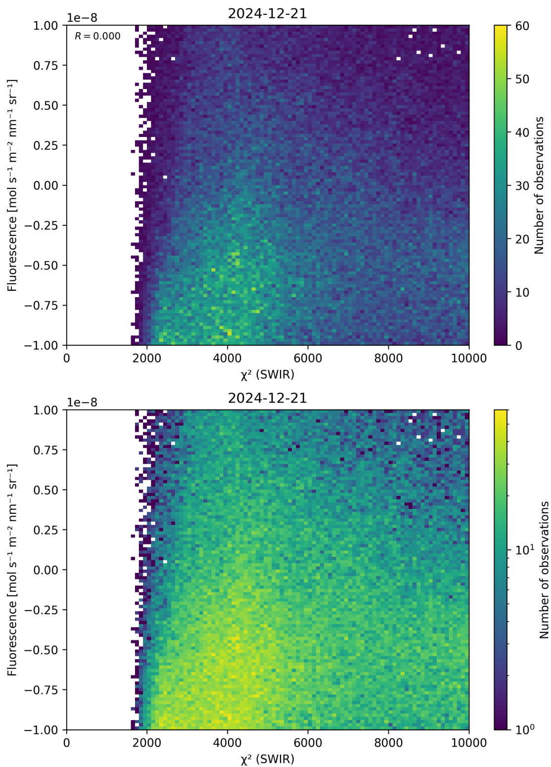
Figure 49: Scatter density plot of “ \chi^2 (SWIR)” against “Fluorescence” for 2024-12-20 to 2024-12-22.
