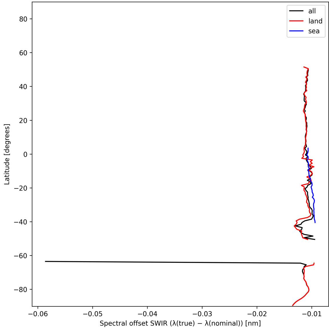
Figure 16: Zonal average of “Spectral offset SWIR ( \lambda_{\text{true}} - \lambda_{\text{nominal}} )” for 2024-12-20 to 2024-12-22.
