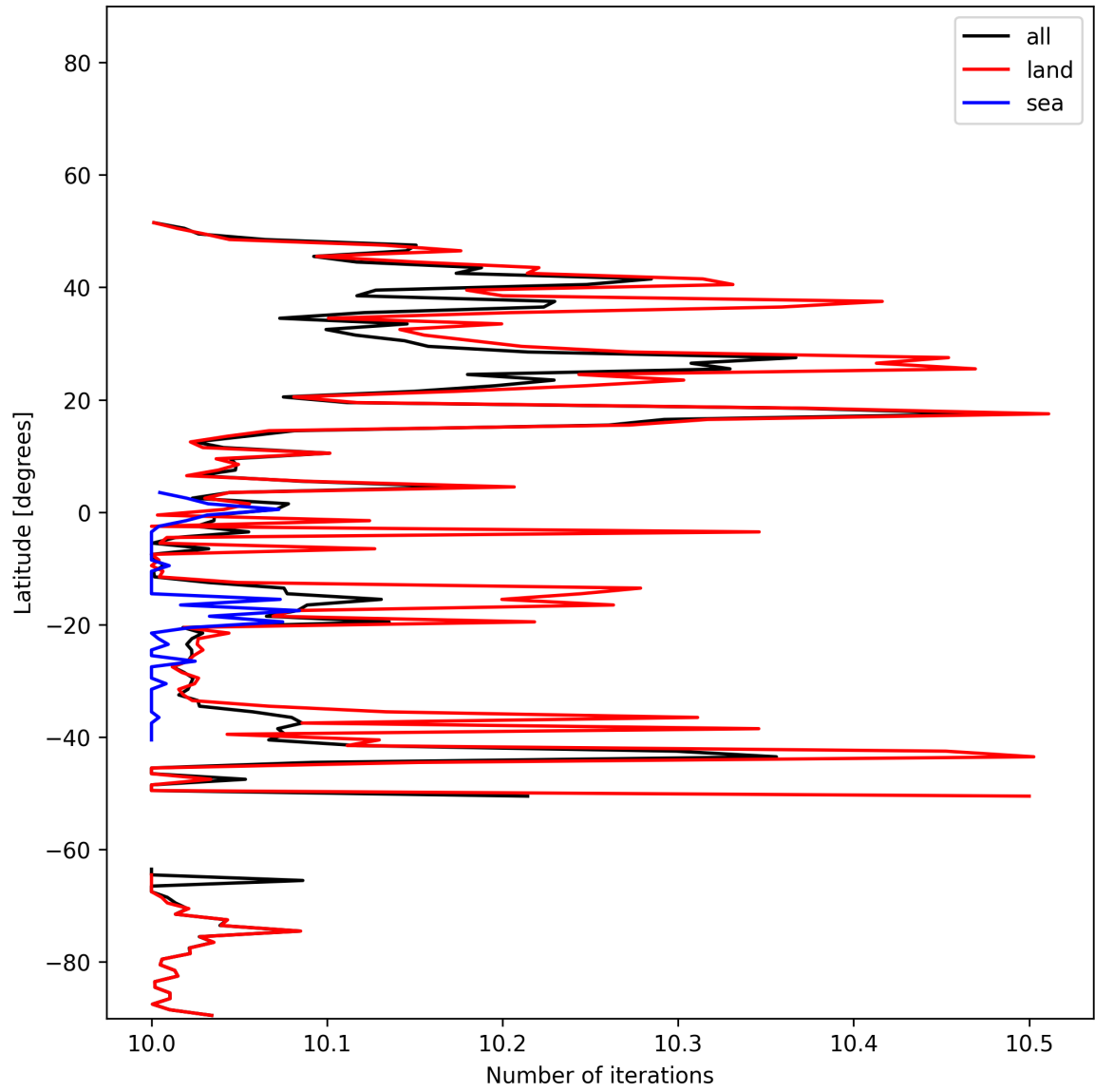
Figure 20: Zonal average of “Number of iterations” for 2024-12-20 to 2024-12-22.
