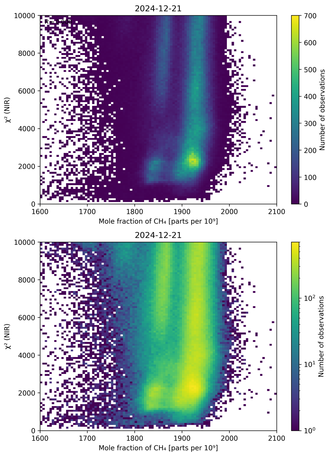
Figure 70: Scatter density plot of “Mole fraction of CH 4 ” against “ \chi^2 (NIR)” for 2024-12-20 to 2024-12-22.
