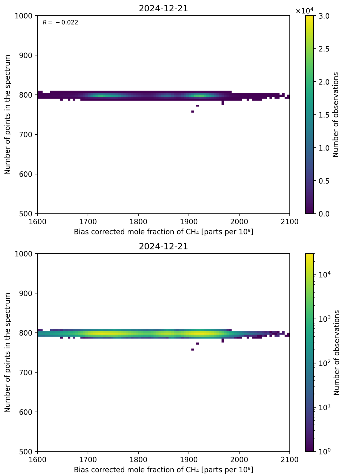
Figure 68: Scatter density plot of “Bias corrected mole fraction of CH 4 ” against “Number of points in the spectrum” for 2024-12-20 to 2024-12-22.
