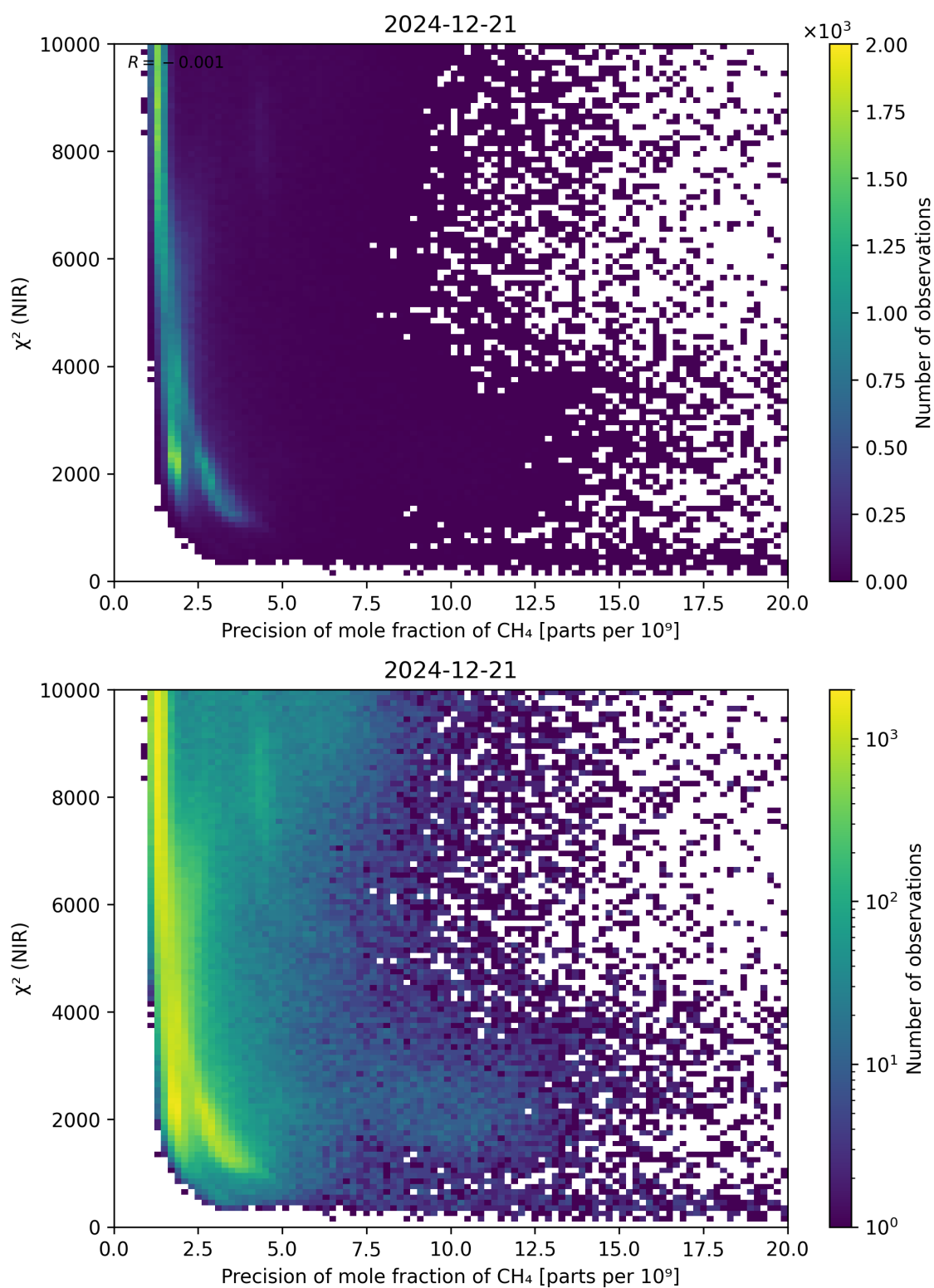
Figure 78: Scatter density plot of “Precision of mole fraction of CH 4 ” against “ \chi^2 (NIR)” for 2024-12-20 to 2024-12-22.
