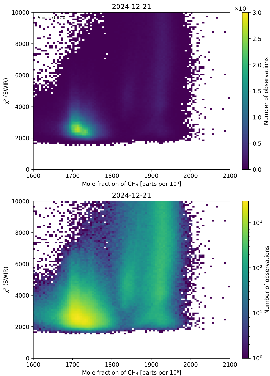
Figure 71: Scatter density plot of “Mole fraction of \text{CH}_4 ” against “ \chi^2 (SWIR)” for 2024-12-20 to 2024-12-22.
