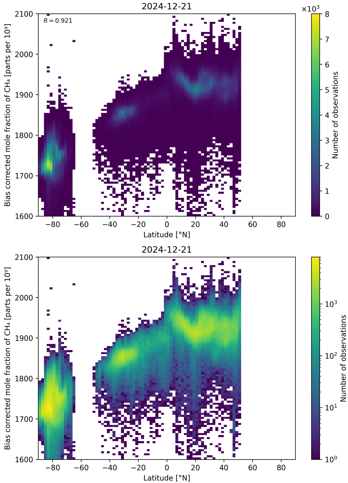
Figure 58: Scatter density plot of “Latitude” against “Bias corrected mole fraction of CH 4 ” for 2024-12-20 to 2024-12-22.
