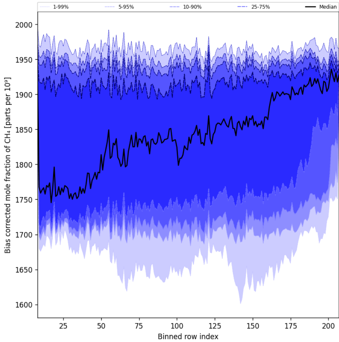
Figure 36: Along track statistics of “Bias corrected mole fraction of CH 4 ” for 2024-12-20 to 2024-12-22
