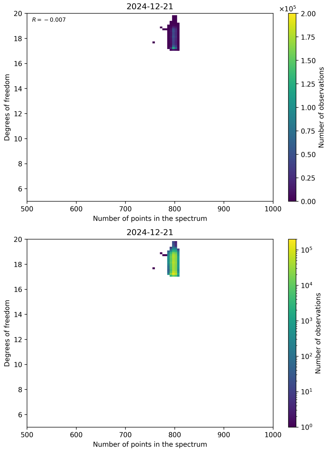
Figure 90: Scatter density plot of “Number of points in the spectrum” against “Degrees of freedom” for 2024-12-20 to 2024-12-22.
