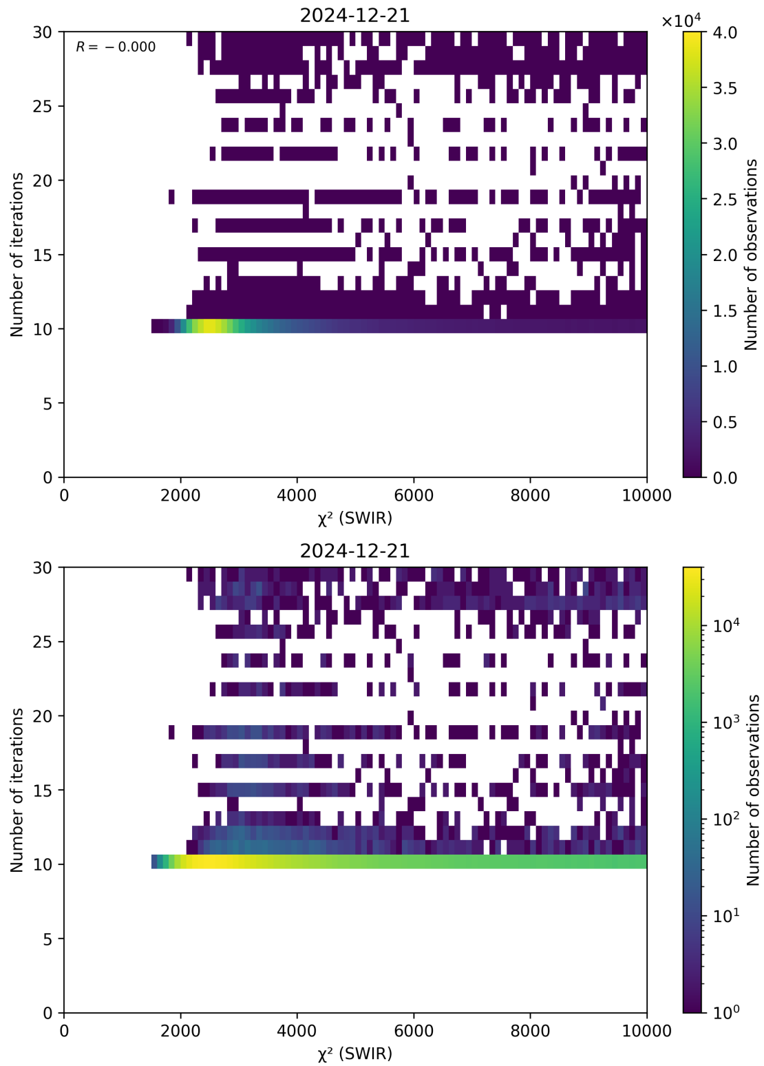
Figure 50: Scatter density plot of “ \chi^2 (SWIR)” against “Number of iterations” for 2024-12-20 to 2024-12-22.
