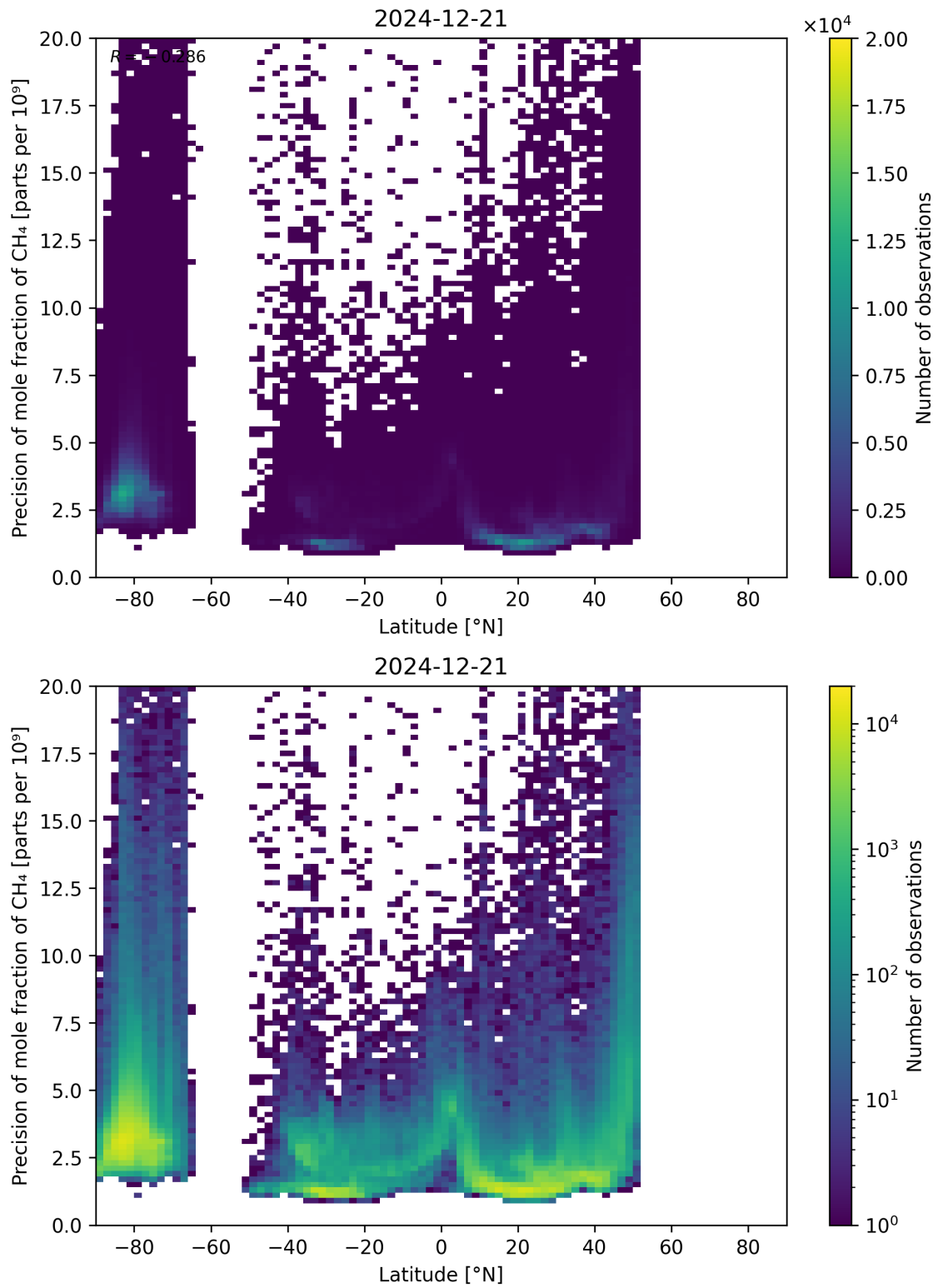
Figure 59: Scatter density plot of “Latitude” against “Precision of mole fraction of CH 4 ” for 2024-12-20 to 2024-12-22.
