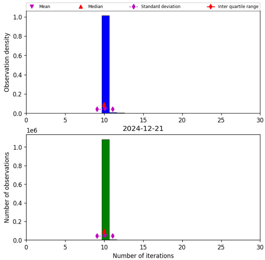
Figure 31: Histogram of “Number of iterations” for 2024-12-20 to 2024-12-22
