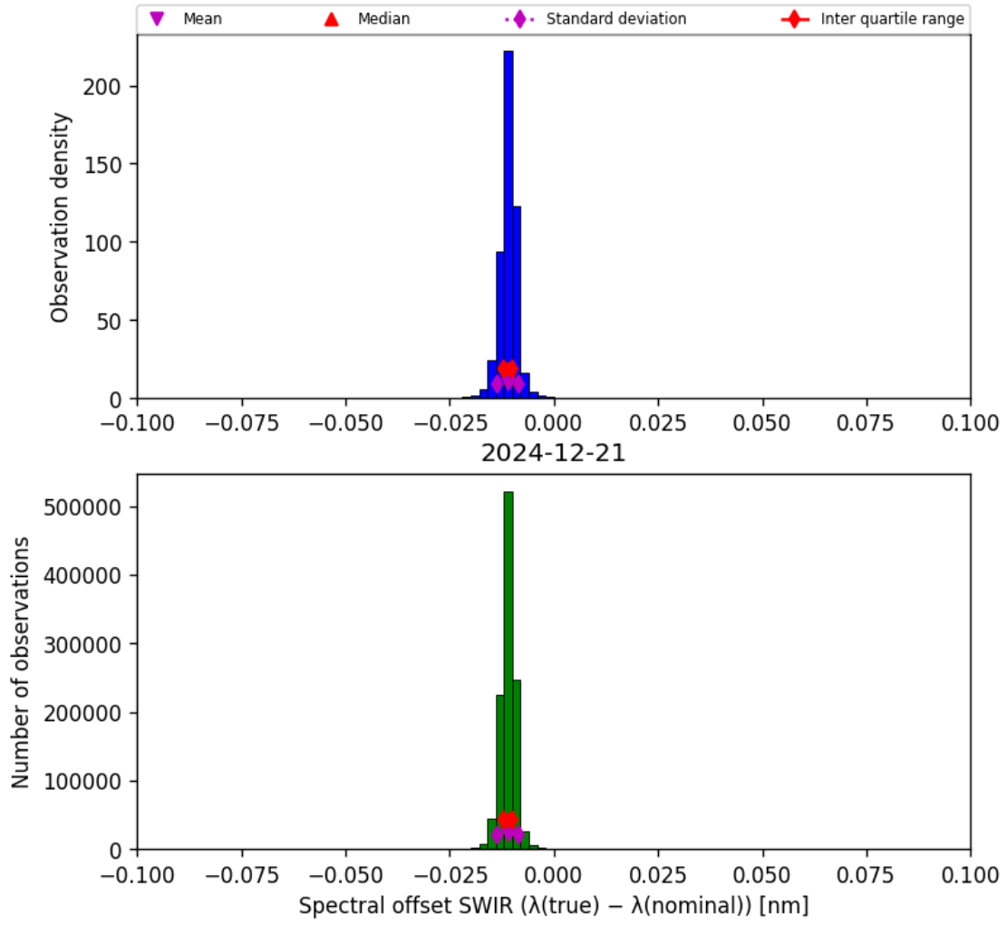
Figure 27: Histogram of “Spectral offset SWIR ( \lambda_{\text{true}} - \lambda_{\text{nominal}} )” for 2024-12-20 to 2024-12-22
