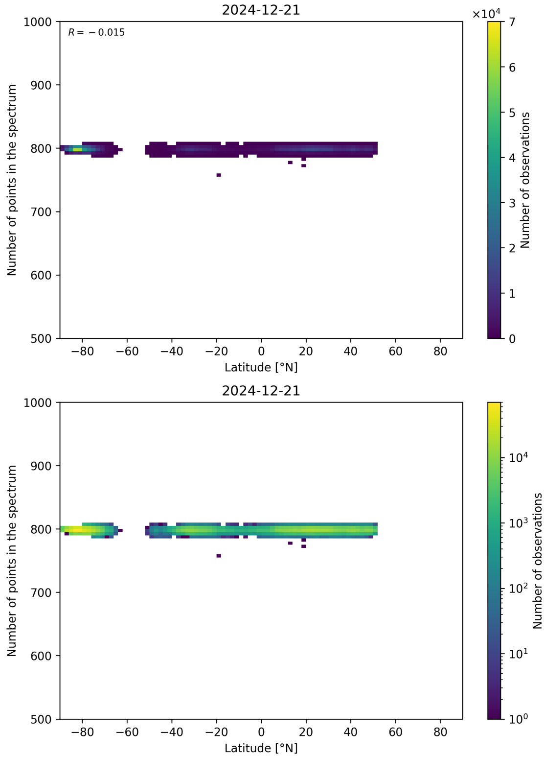
Figure 61: Scatter density plot of “Latitude” against “Number of points in the spectrum” for 2024-12-20 to 2024-12-22.
