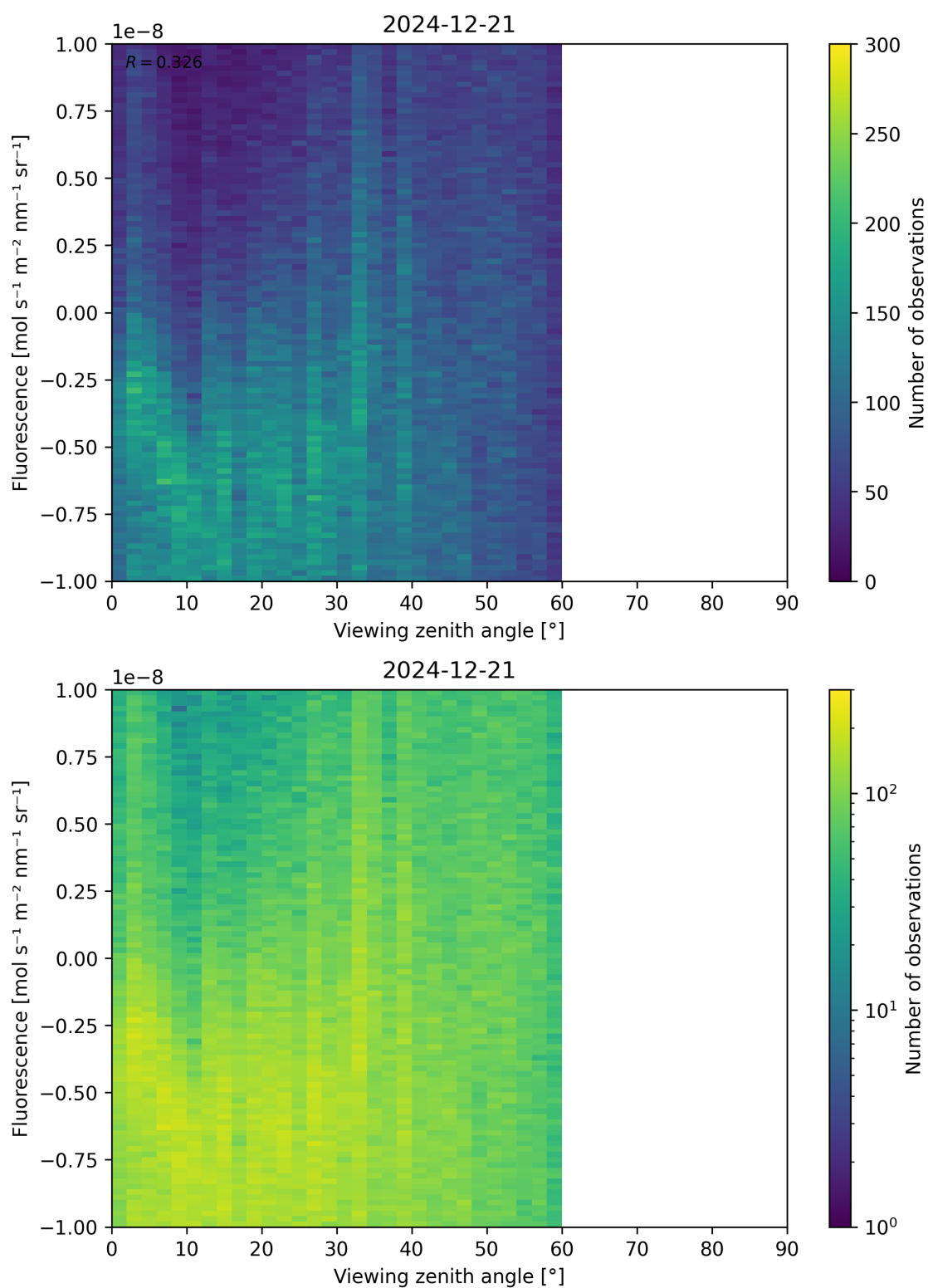
Figure 108: Scatter density plot of “Viewing zenith angle” against “Fluorescence” for 2024-12-20 to 2024-12-22.
