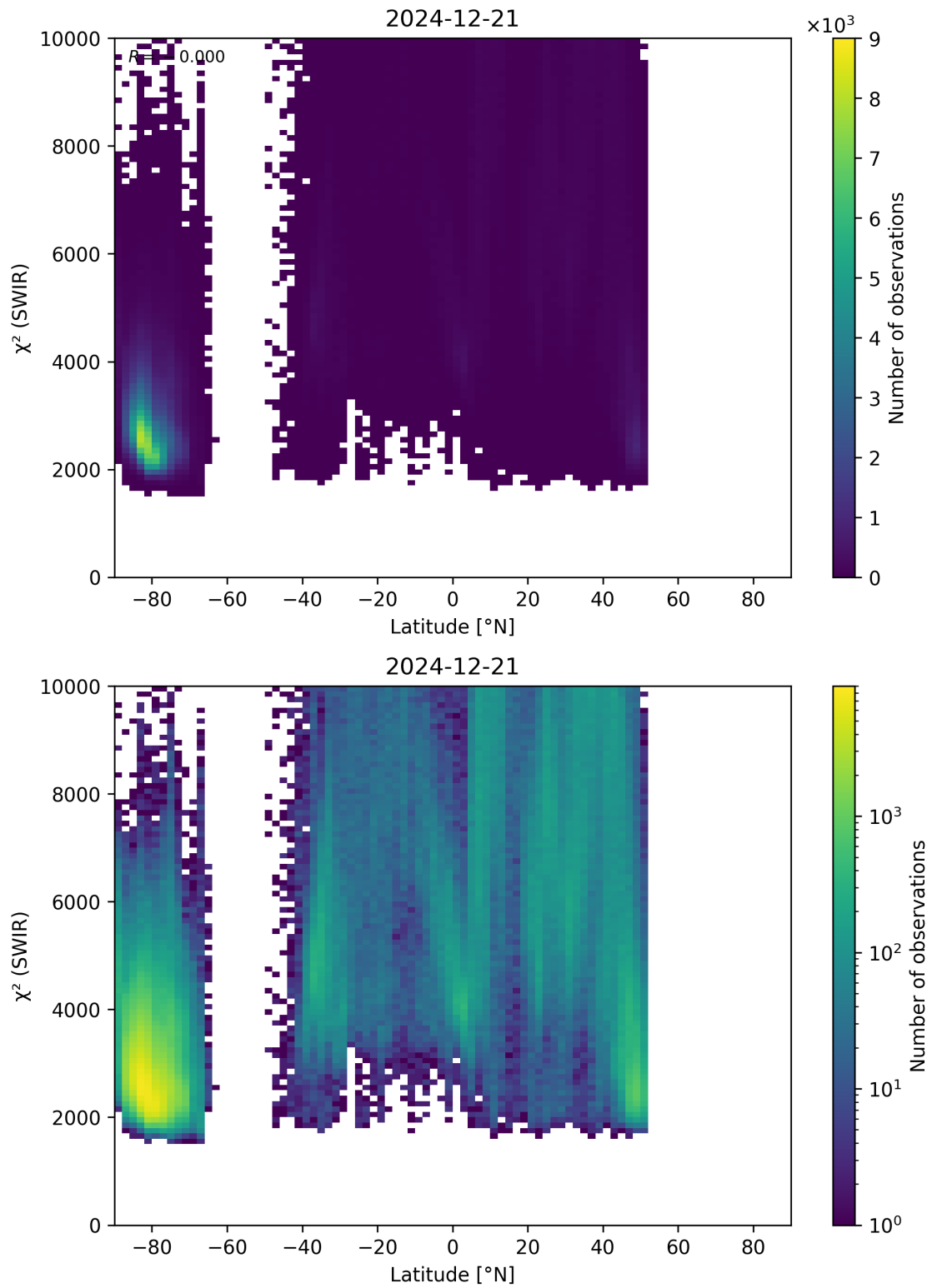
Figure 54: Scatter density plot of “Latitude” against “ \chi^2 (SWIR)” for 2024-12-20 to 2024-12-22.
