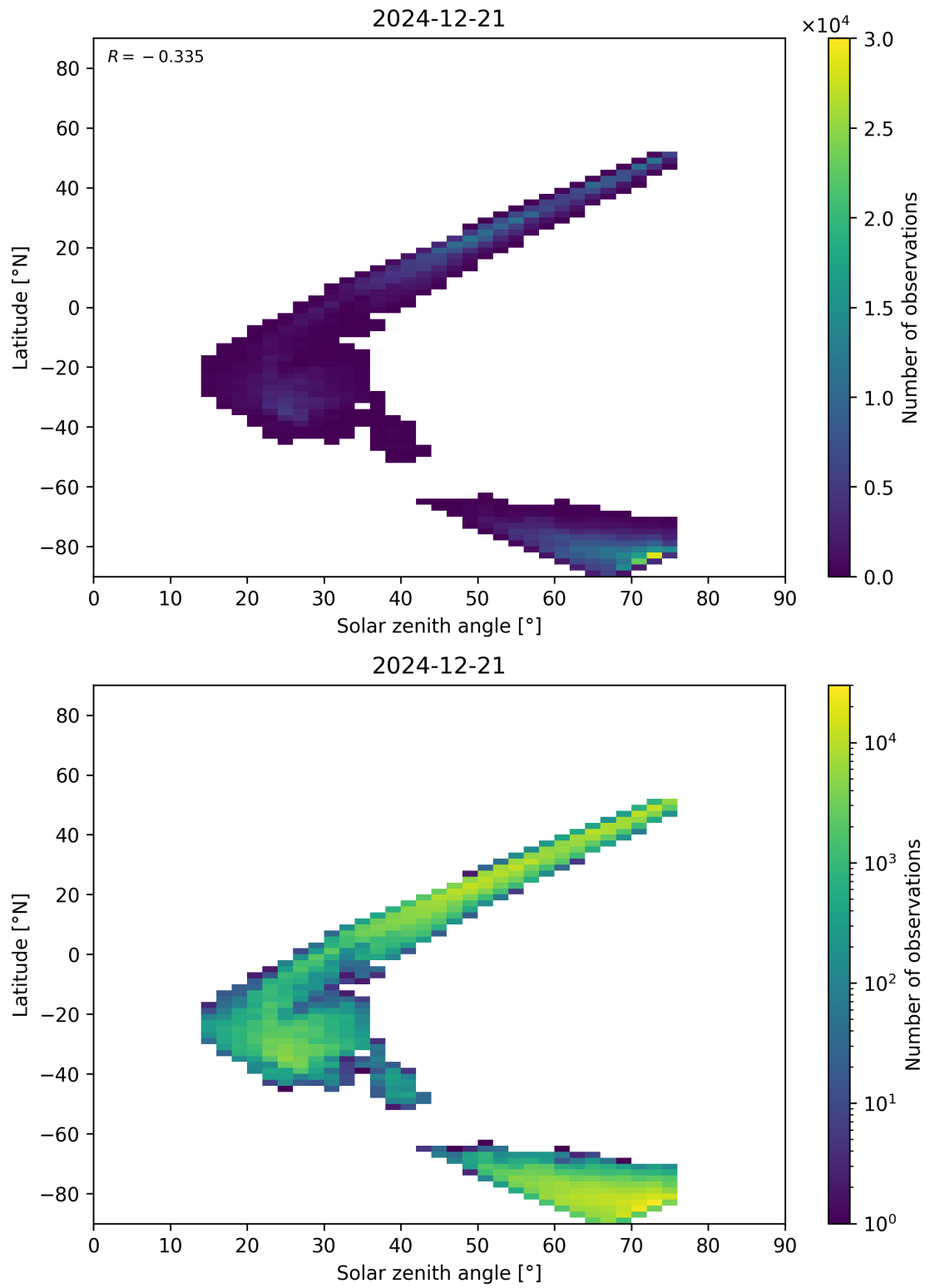
Figure 98: Scatter density plot of “Solar zenith angle” against “Latitude” for 2024-12-20 to 2024-12-22.
