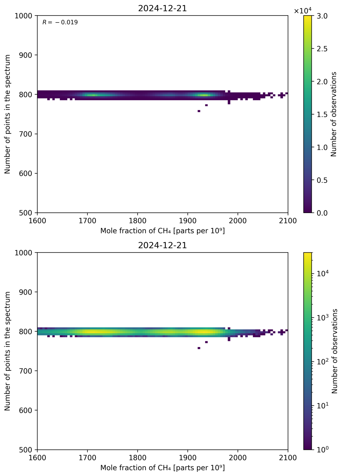
Figure 77: Scatter density plot of “Mole fraction of CH 4 ” against “Number of points in the spectrum” for 2024-12-20 to 2024-12-22.
