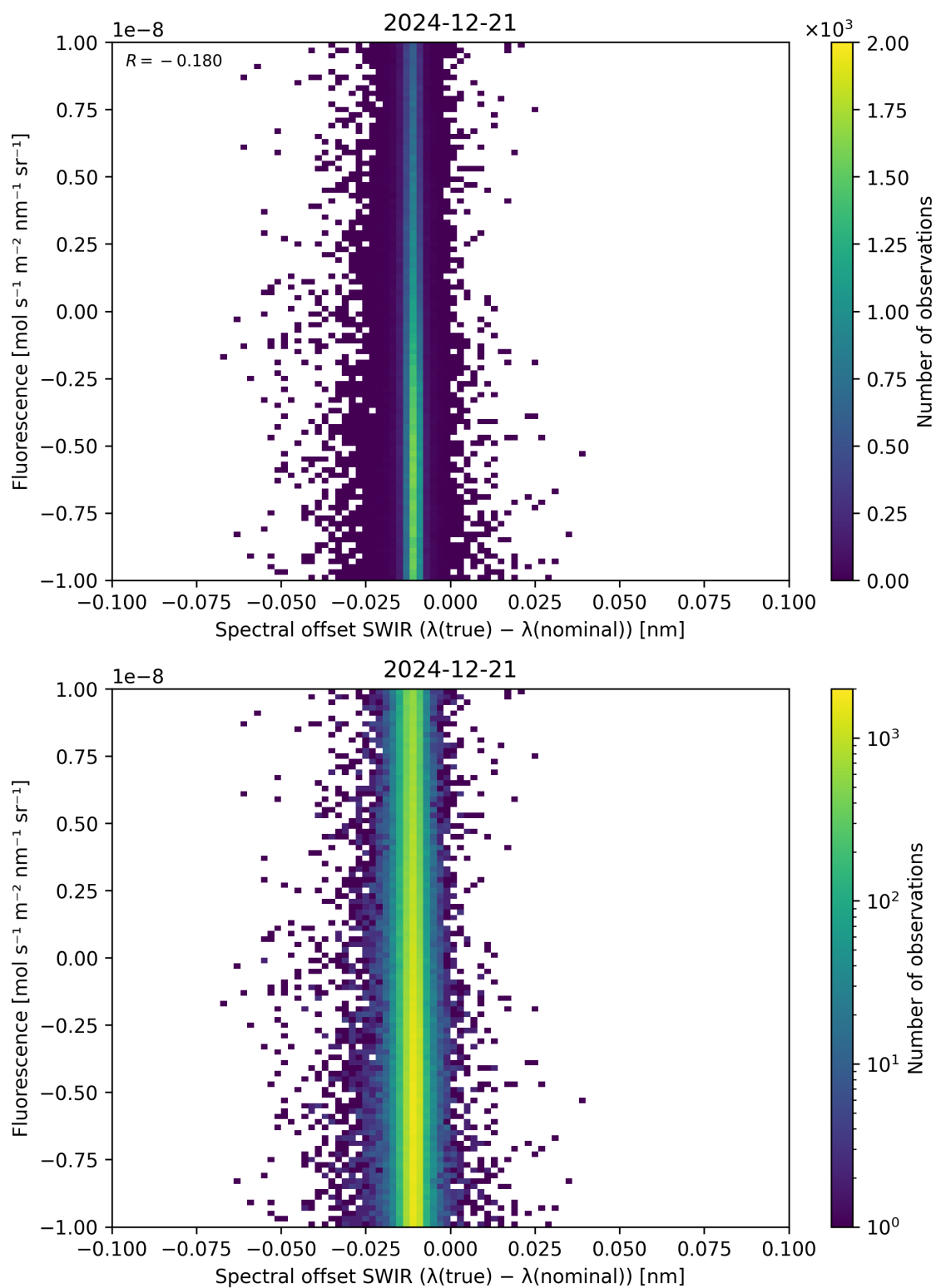
Figure 120: Scatter density plot of “Spectral offset SWIR ( \lambda_{\text{true}} - \lambda_{\text{nominal}} )” against “Fluorescence” for 2024-12-20 to 2024-12-22.
