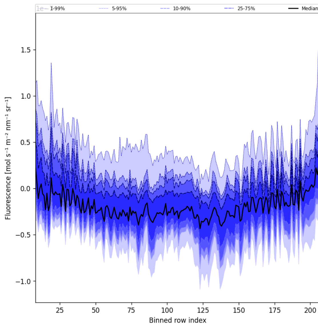
Figure 43: Along track statistics of “Fluorescence” for 2024-12-20 to 2024-12-22
