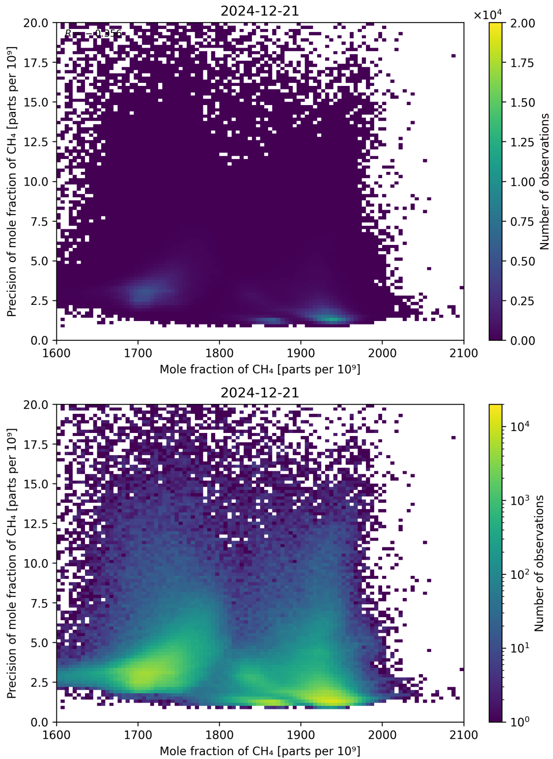
Figure 75: Scatter density plot of “Mole fraction of CH 4 ” against “Precision of mole fraction of CH 4 ” for 2024-12-20 to 2024-12-22.
