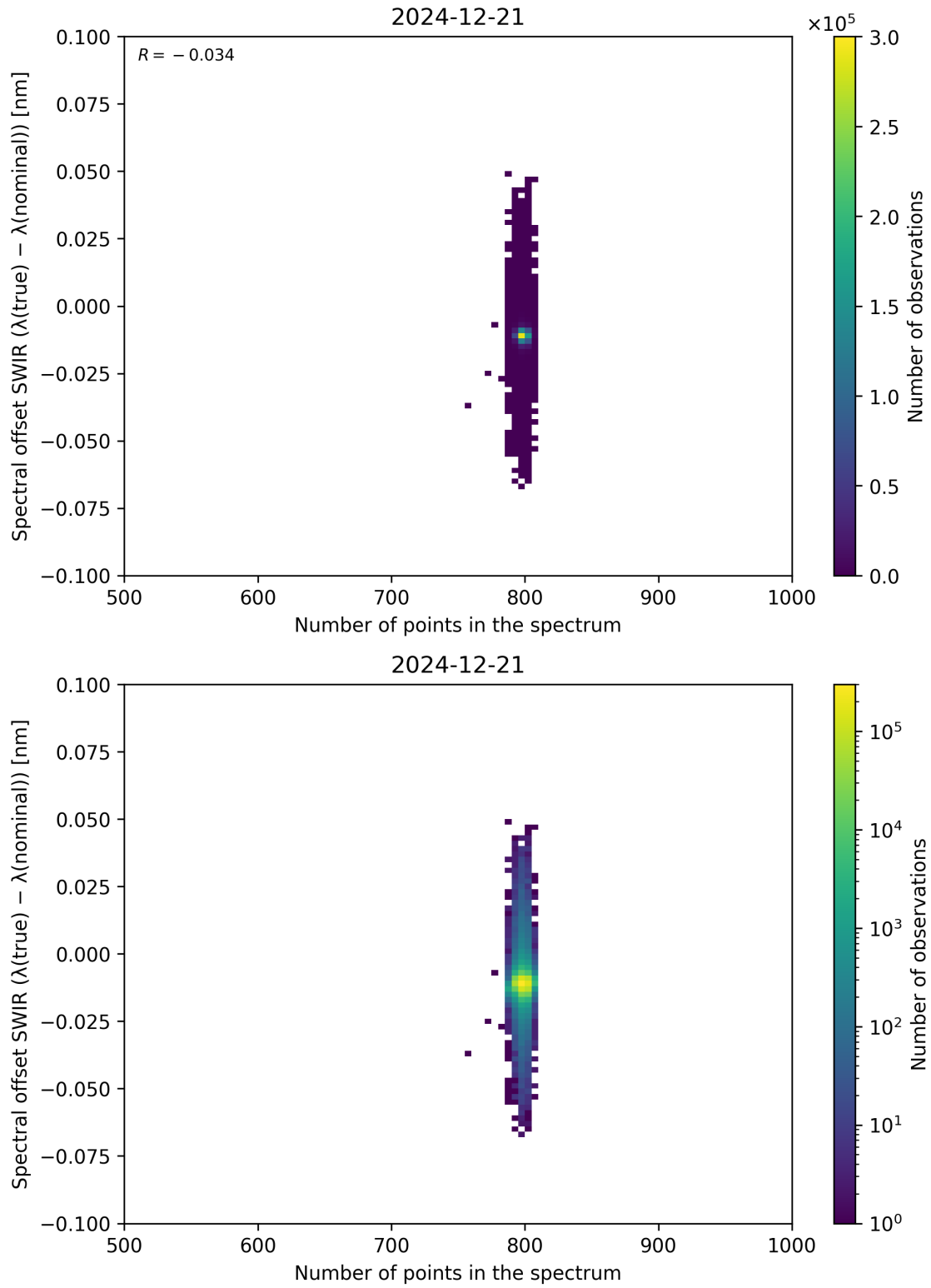
Figure 93: Scatter density plot of “Number of points in the spectrum” against “Spectral offset SWIR ( \lambda_{\text{true}} - \lambda_{\text{nominal}} )” for 2024-12-20 to 2024-12-22.
