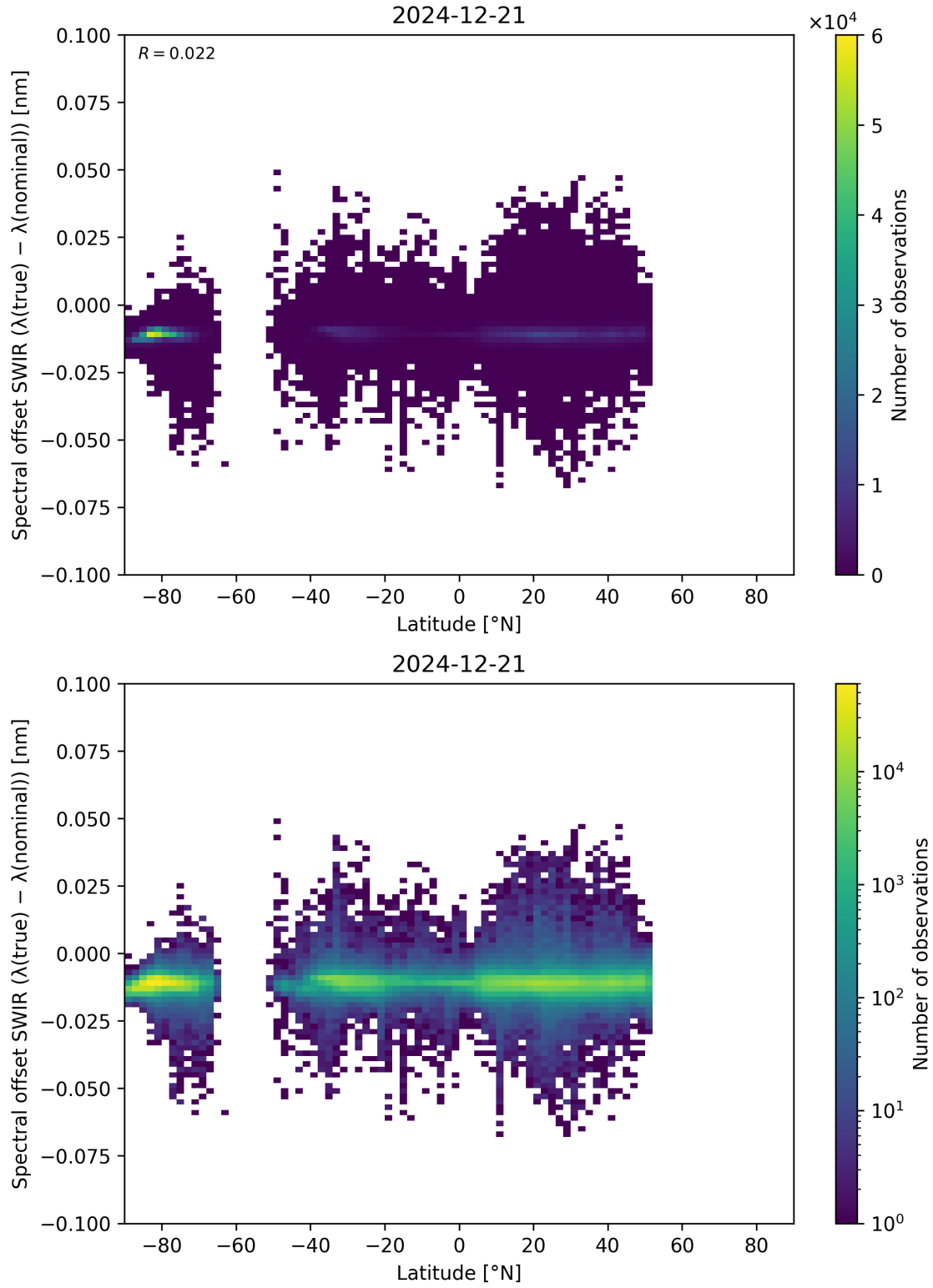
Figure 62: Scatter density plot of “Latitude” against “Spectral offset SWIR ( \lambda_{\text{true}} - \lambda_{\text{nominal}} )” for 2024-12-20 to 2024-12-22.
