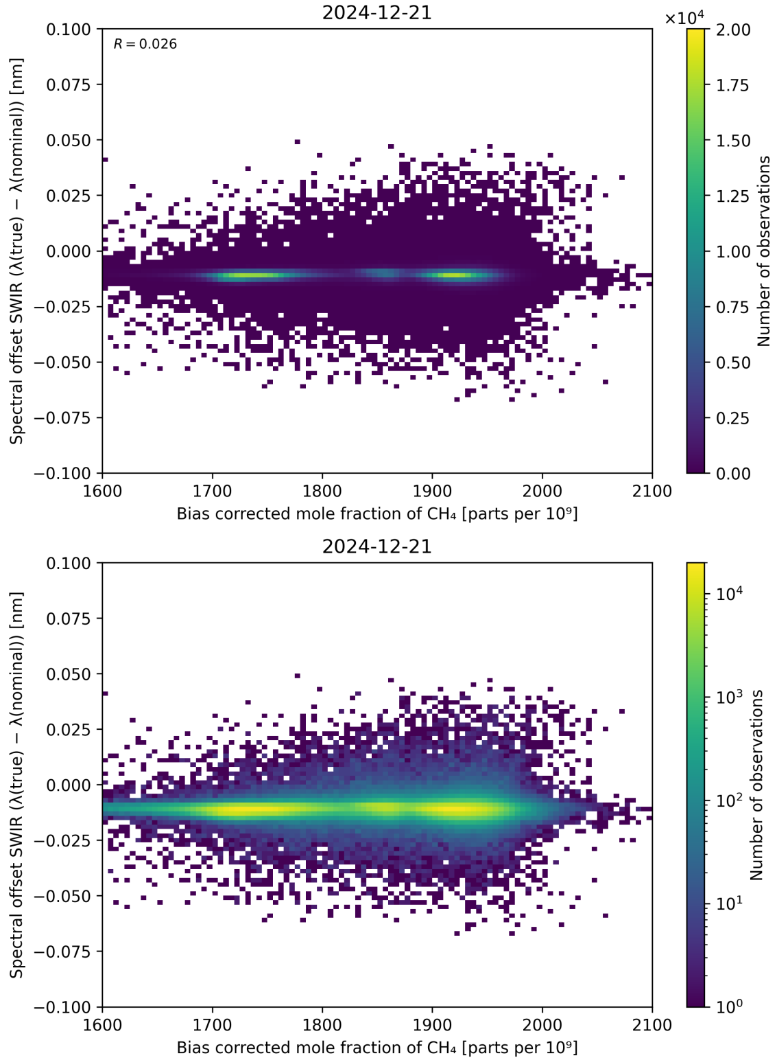
Figure 69: Scatter density plot of “Bias corrected mole fraction of \text{CH}_4 ” against “Spectral offset SWIR ( \lambda_{\text{true}} - \lambda_{\text{nominal}} )” for 2024-12-20 to 2024-12-22.
