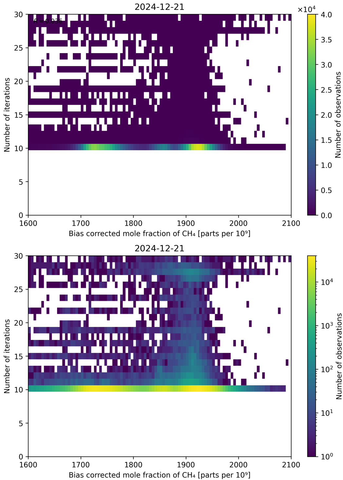
Figure 67: Scatter density plot of “Bias corrected mole fraction of \text{CH}_4 ” against “Number of iterations” for 2024-12-20 to 2024-12-22.
