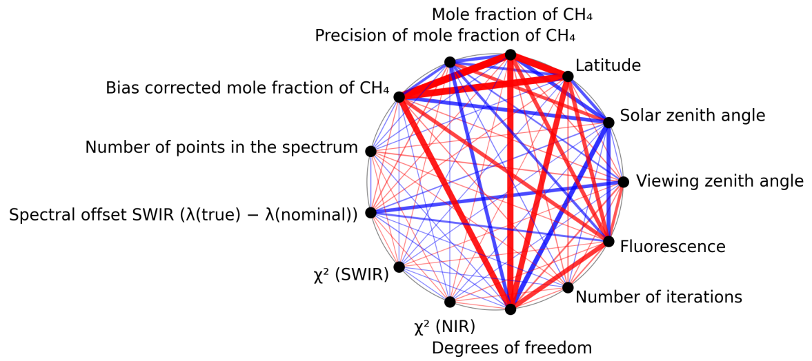
Figure 1: Map of correlation graph for 2024-12-20 to 2024-12-22.
