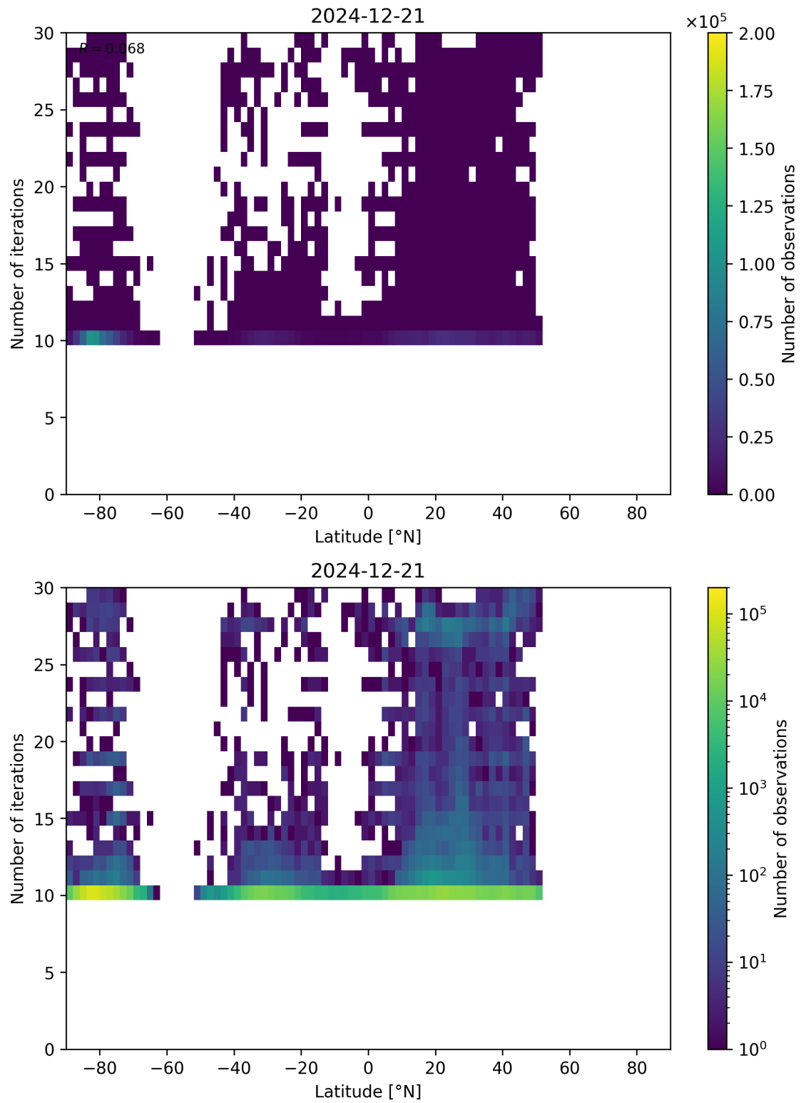
Figure 60: Scatter density plot of “Latitude” against “Number of iterations” for 2024-12-20 to 2024-12-22.
