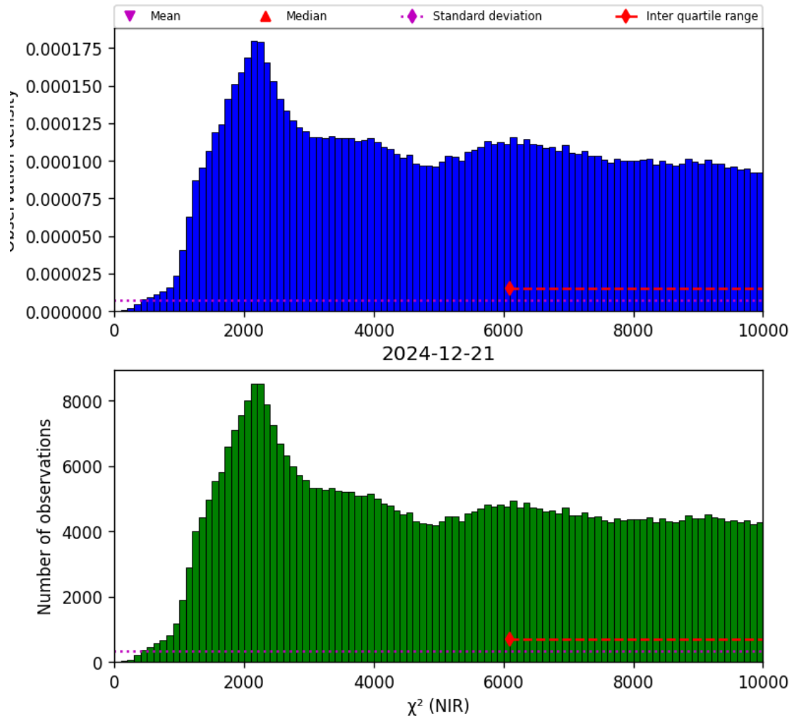
Figure 29: Histogram of “ \chi^2 (NIR)” for 2024-12-20 to 2024-12-22
