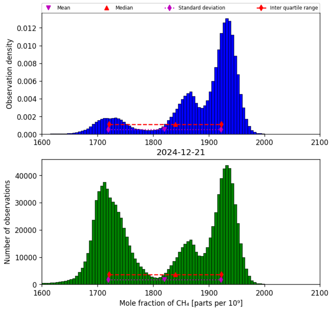
Figure 23: Histogram of “Mole fraction of CH 4 ” for 2024-12-20 to 2024-12-22
