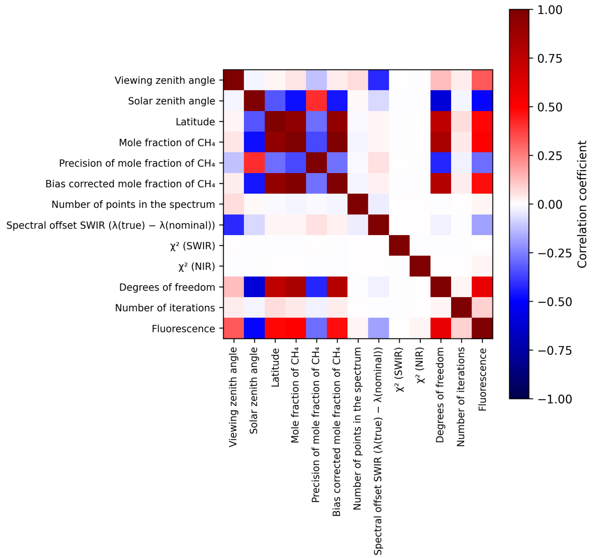
Figure 2: Map of correlation matrix for 2024-12-20 to 2024-12-22.
