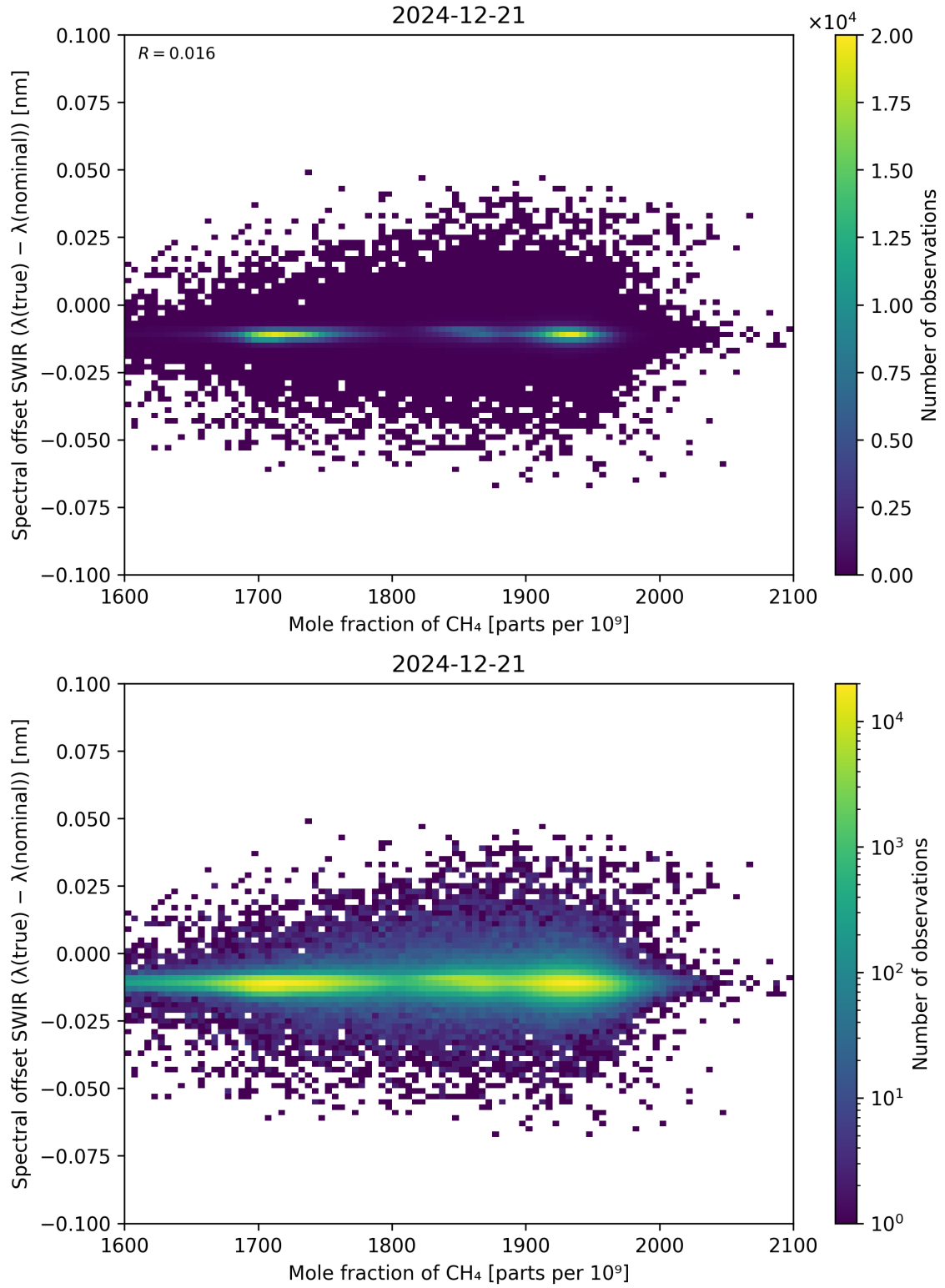
Figure 86: Scatter density plot of “Mole fraction of CH 4 ” against “Spectral offset SWIR ( \lambda_{\text{true}} - \lambda_{\text{nominal}} )” for 2024-12-20 to 2024-12-22.
