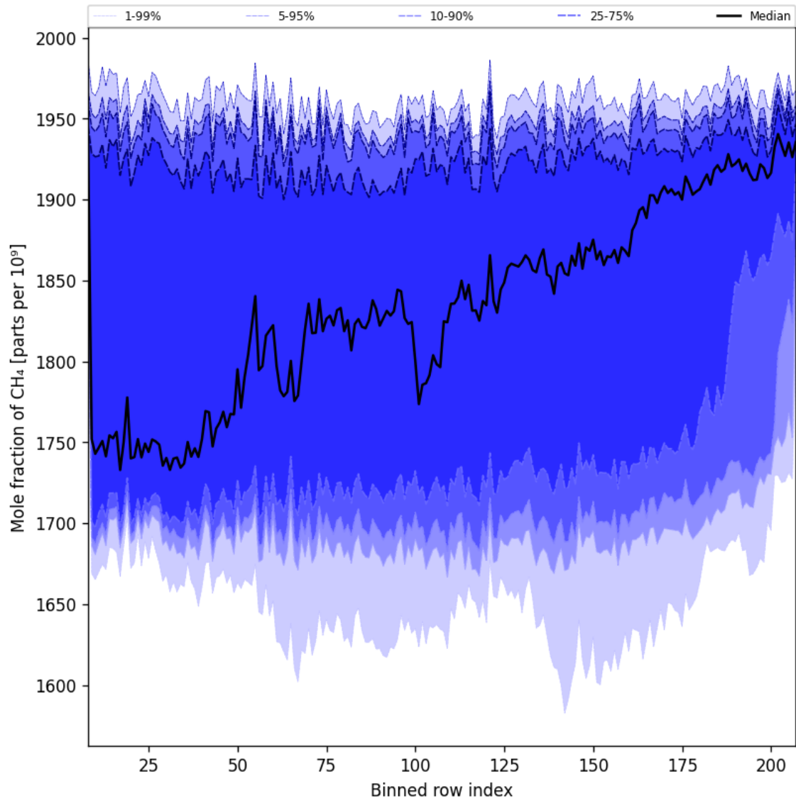
Figure 34: Along track statistics of “Mole fraction of CH 4 ” for 2024-12-20 to 2024-12-22
