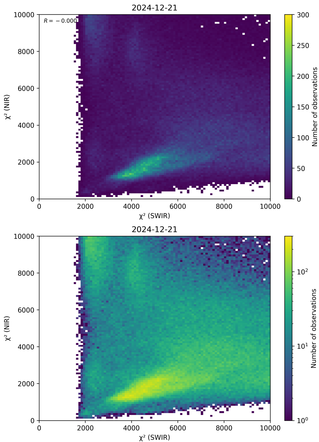
Figure 47: Scatter density plot of “ \chi^2 (SWIR)” against “ \chi^2 (NIR)” for 2024-12-20 to 2024-12-22.
