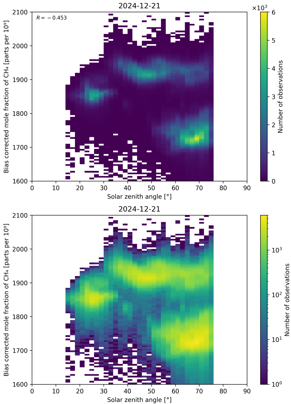
Figure 100: Scatter density plot of “Solar zenith angle” against “Bias corrected mole fraction of CH 4 ” for 2024-12-20 to 2024-12-22.
