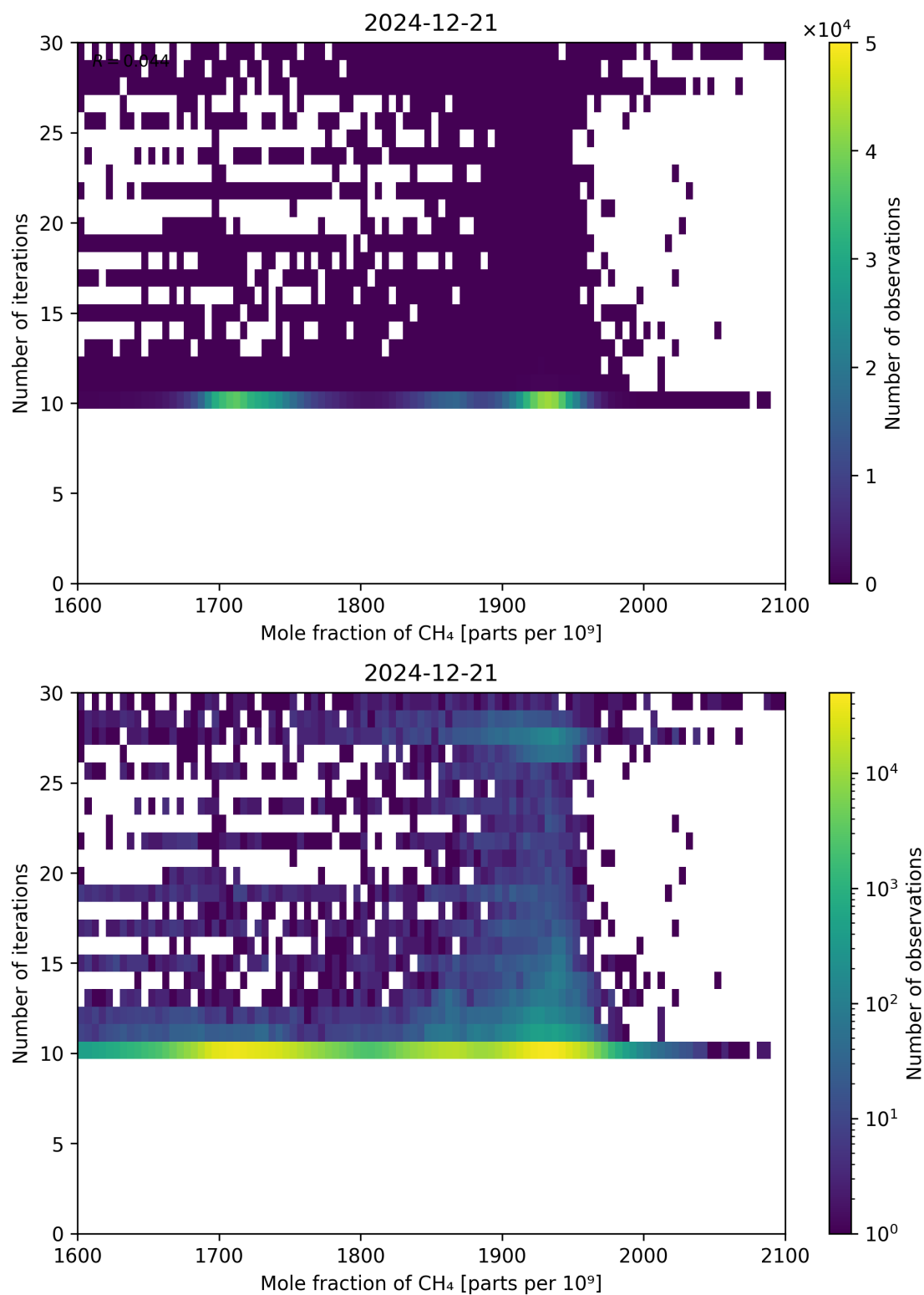
Figure 76: Scatter density plot of “Mole fraction of CH 4 ” against “Number of iterations” for 2024-12-20 to 2024-12-22.
