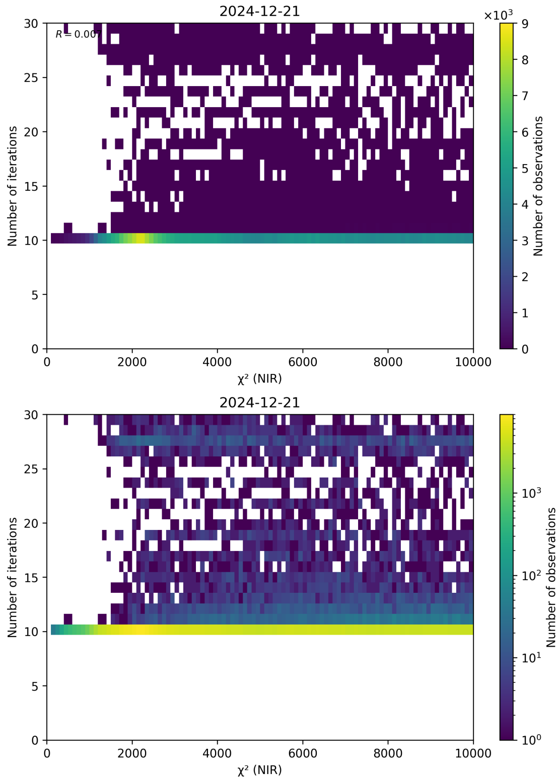
Figure 46: Scatter density plot of “ \chi^2 (NIR)” against “Number of iterations” for 2024-12-20 to 2024-12-22.
