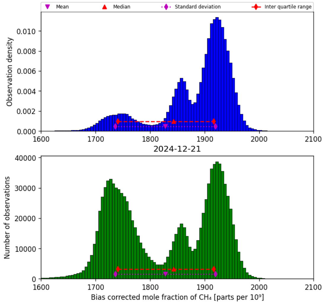
Figure 25: Histogram of “Bias corrected mole fraction of CH 4 ” for 2024-12-20 to 2024-12-22
