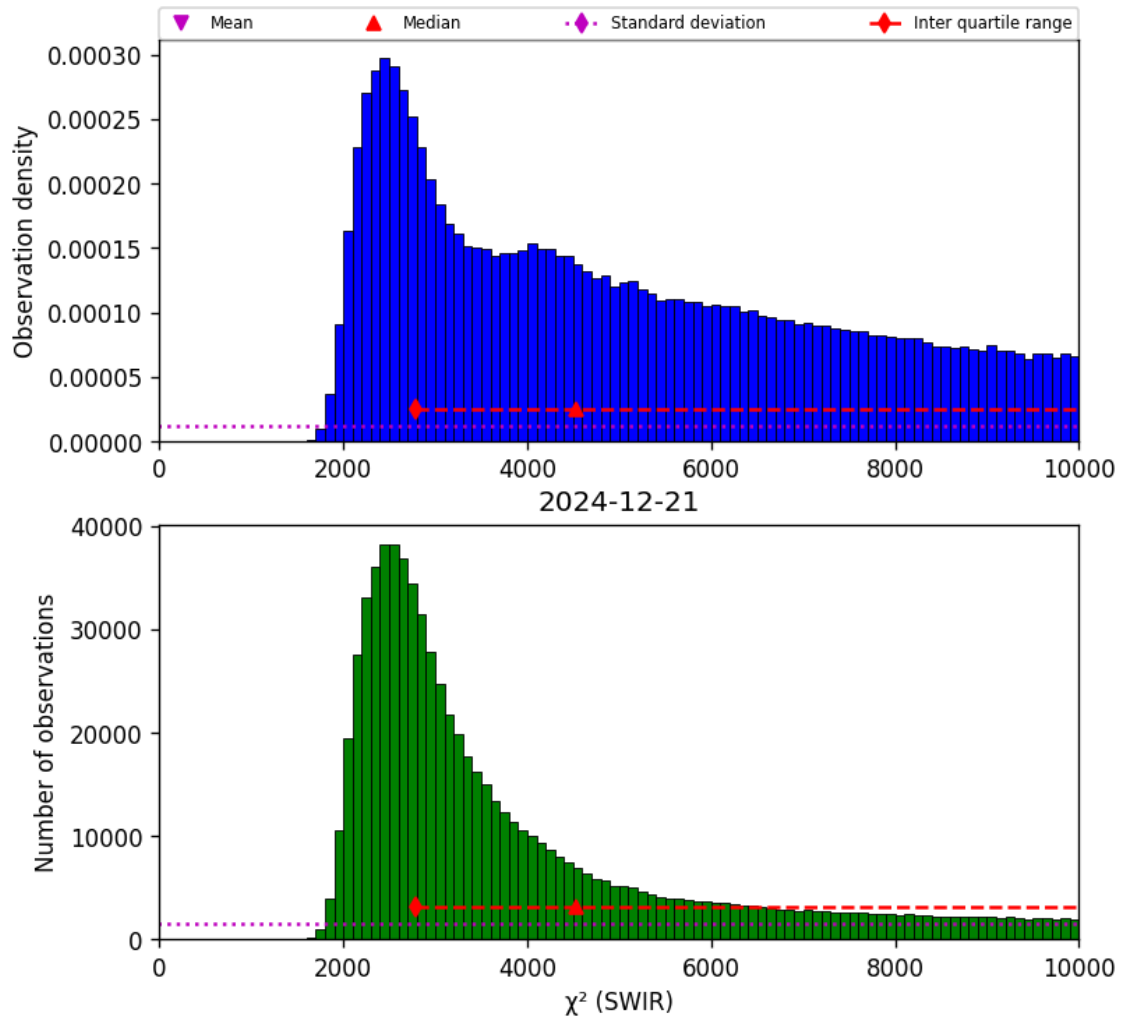
Figure 28: Histogram of “ \chi^2 (SWIR)” for 2024-12-20 to 2024-12-22
