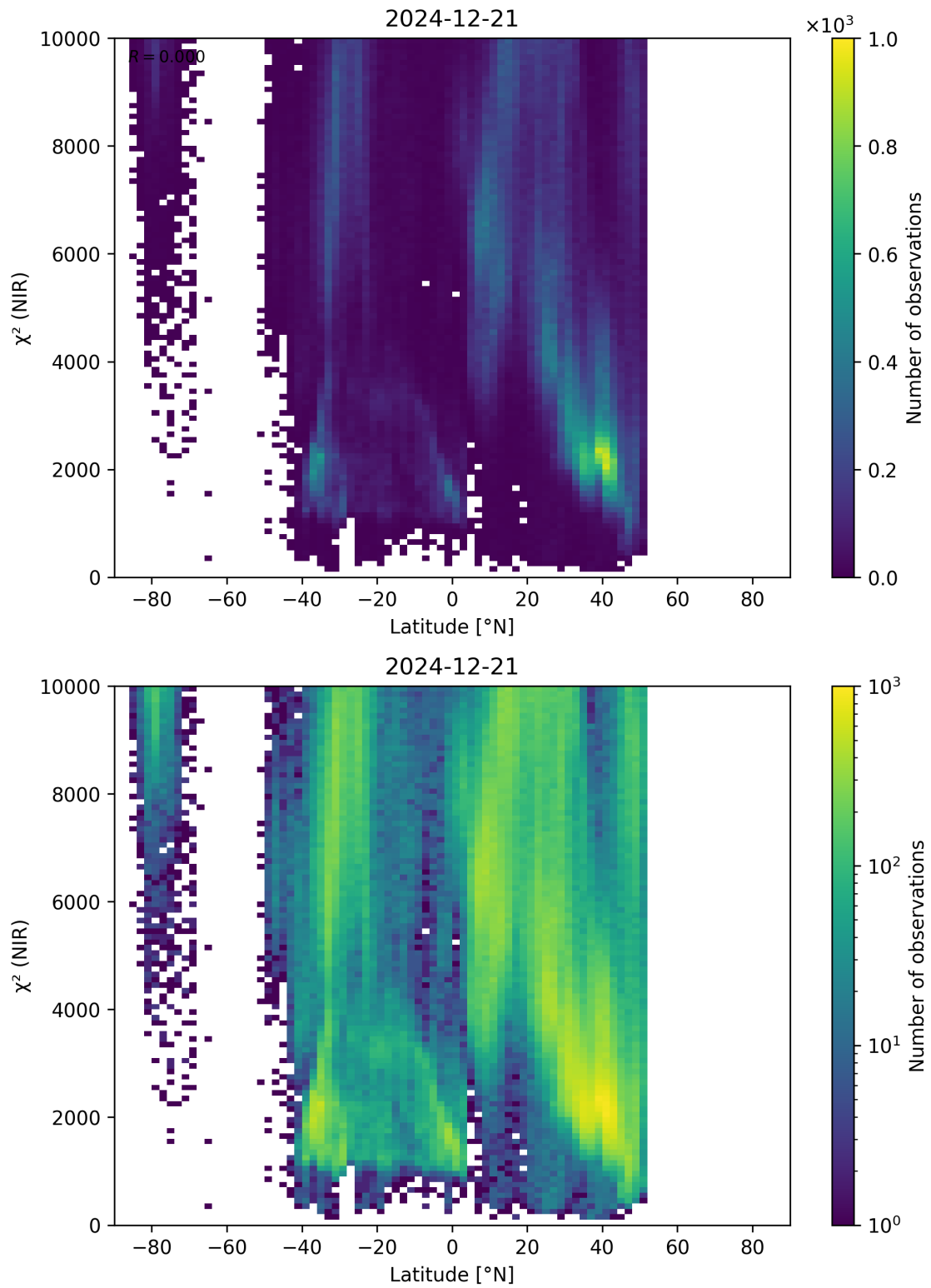
Figure 53: Scatter density plot of “Latitude” against “ \chi^2 (NIR)” for 2024-12-20 to 2024-12-22.
