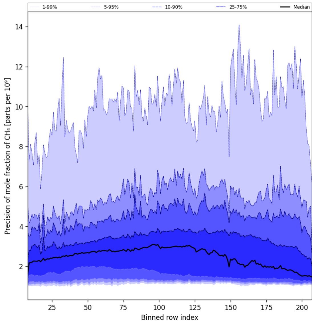
Figure 35: Along track statistics of “Precision of mole fraction of CH 4 ” for 2024-12-20 to 2024-12-22
