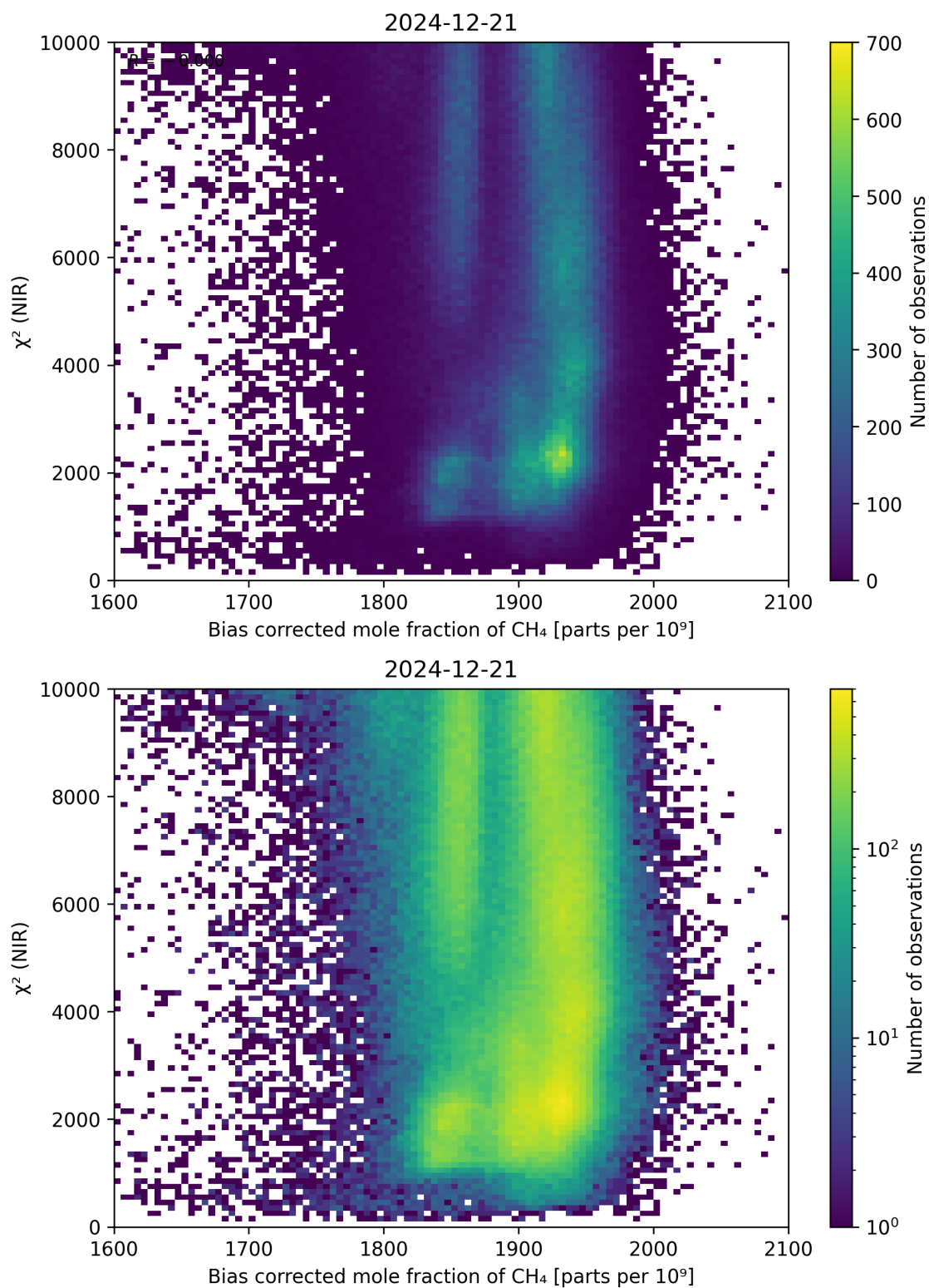
Figure 63: Scatter density plot of “Bias corrected mole fraction of \text{CH}_4 ” against “ \chi^2 (NIR)” for 2024-12-20 to 2024-12-22.
