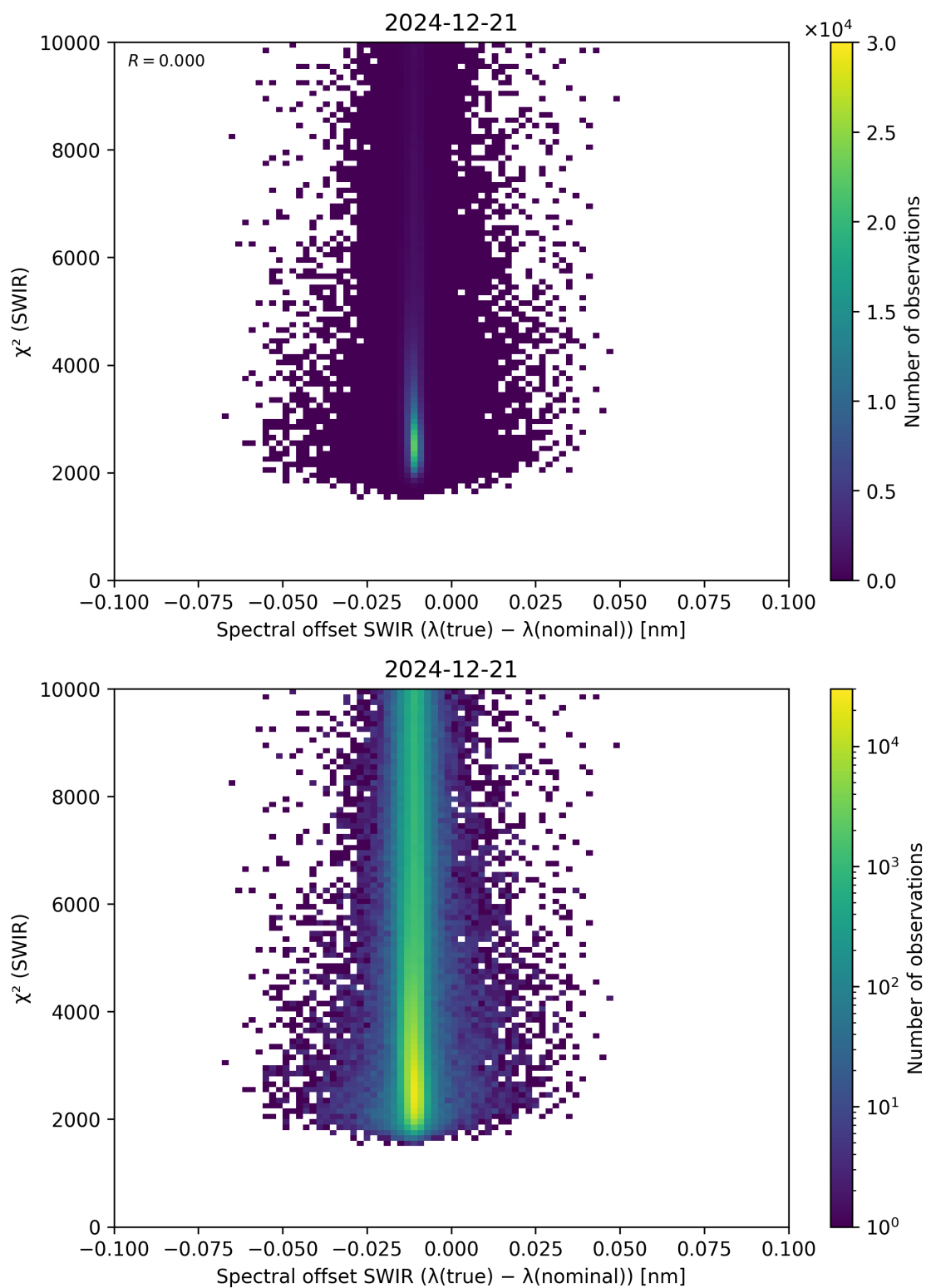
Figure 118: Scatter density plot of “Spectral offset SWIR ( \lambda_{\text{true}} - \lambda_{\text{nominal}} )” against “ \chi^2 (SWIR)” for 2024-12-20 to 2024-12-22.
