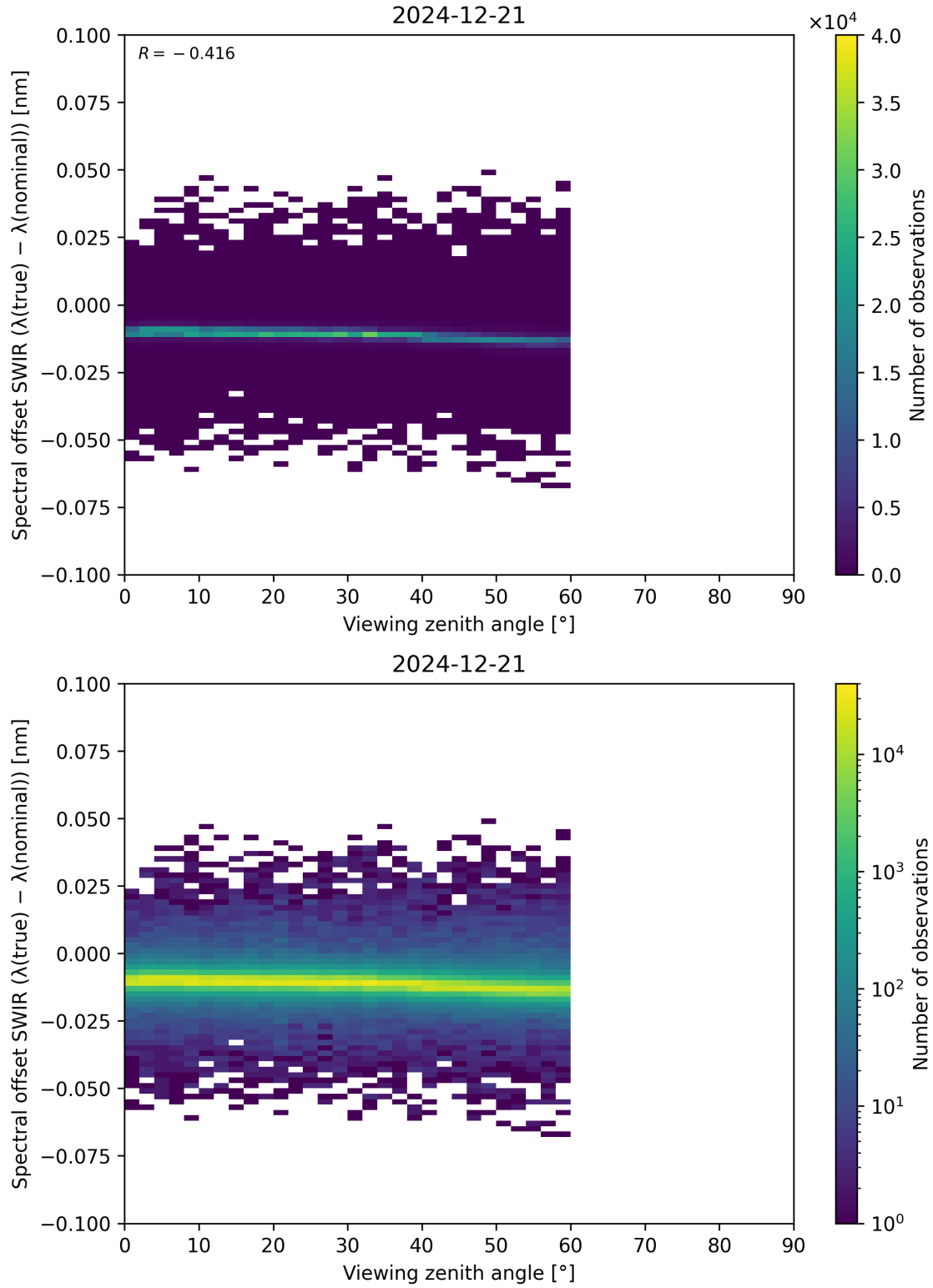
Figure 116: Scatter density plot of “Viewing zenith angle” against “Spectral offset SWIR ( \lambda_{\text{true}} - \lambda_{\text{nominal}} )” for 2024-12-20 to 2024-12-22.
