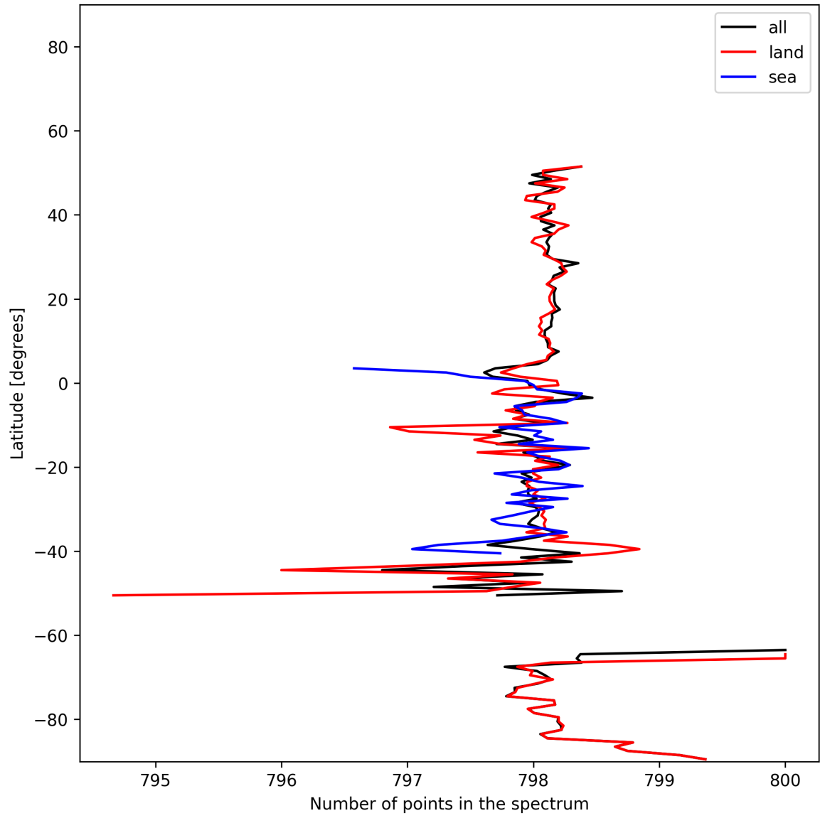
Figure 15: Zonal average of “Number of points in the spectrum” for 2024-12-20 to 2024-12-22.
