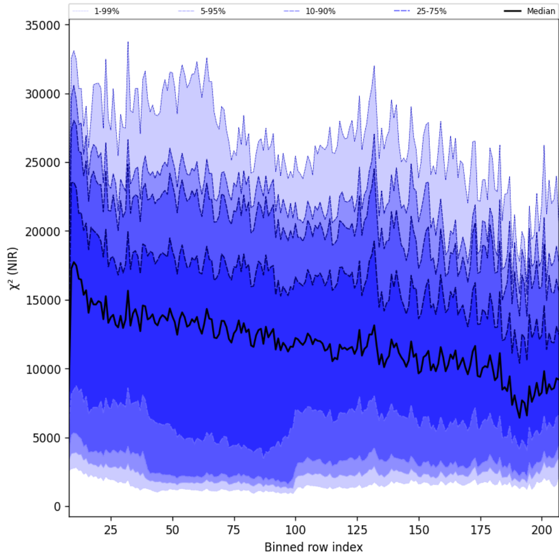
Figure 40: Along track statistics of “ \chi^2 (NIR)” for 2024-12-20 to 2024-12-22
