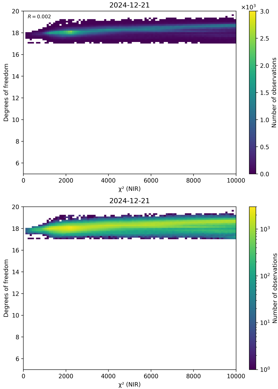
Figure 44: Scatter density plot of “ \chi^2 (NIR)” against “Degrees of freedom” for 2024-12-20 to 2024-12-22.
