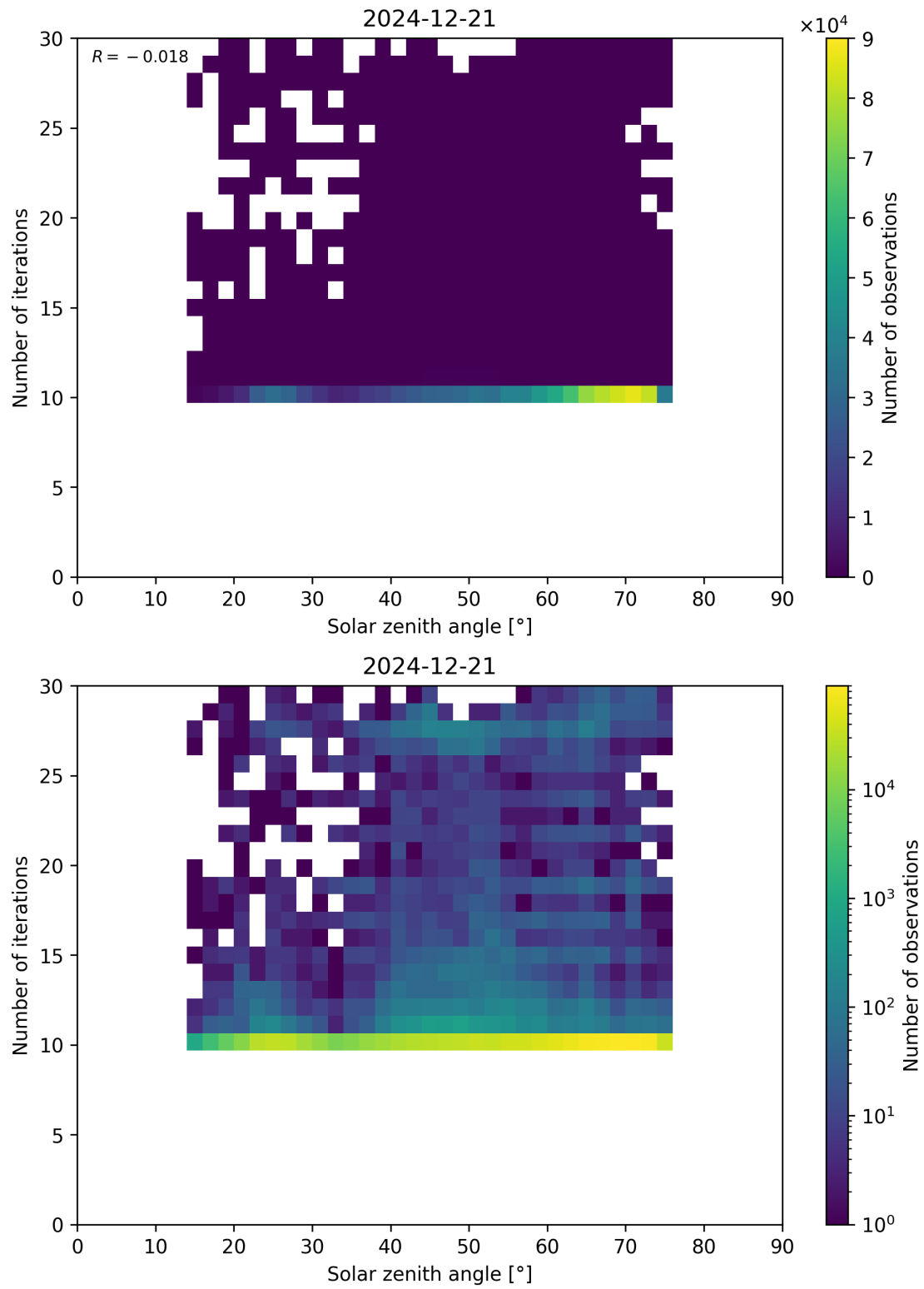
Figure 102: Scatter density plot of “Solar zenith angle” against “Number of iterations” for 2024-12-20 to 2024-12-22.
