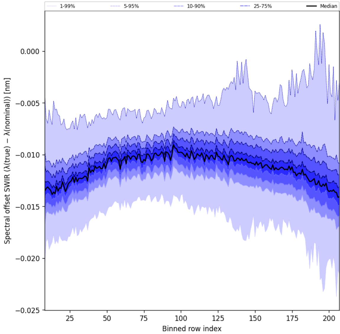
Figure 38: Along track statistics of “Spectral offset SWIR ( \lambda_{\text{true}} - \lambda_{\text{nominal}} )” for 2024-12-20 to 2024-12-22
