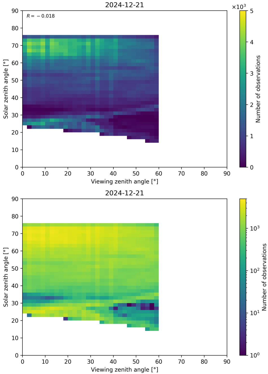
Figure 115: Scatter density plot of “Viewing zenith angle” against “Solar zenith angle” for 2024-12-20 to 2024-12-22.
