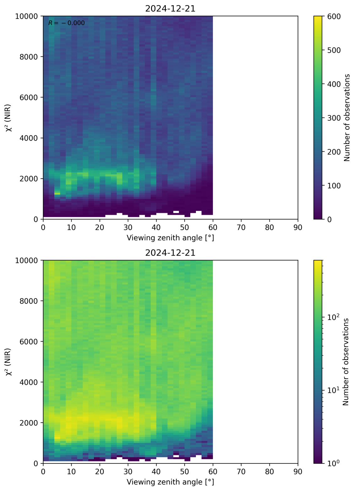
Figure 105: Scatter density plot of “Viewing zenith angle” against “ \chi^2 (NIR)” for 2024-12-20 to 2024-12-22.
