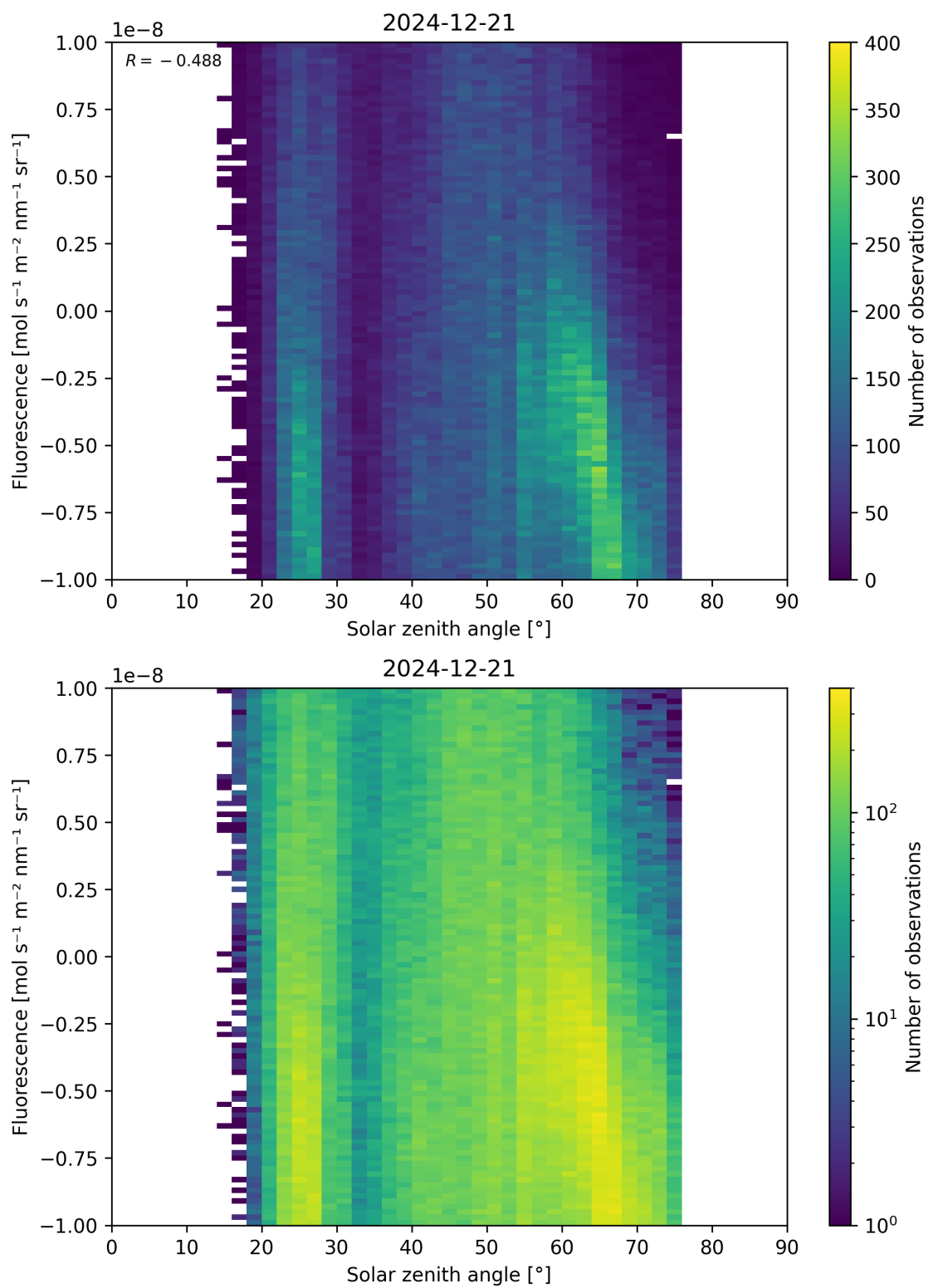
Figure 97: Scatter density plot of “Solar zenith angle” against “Fluorescence” for 2024-12-20 to 2024-12-22.
