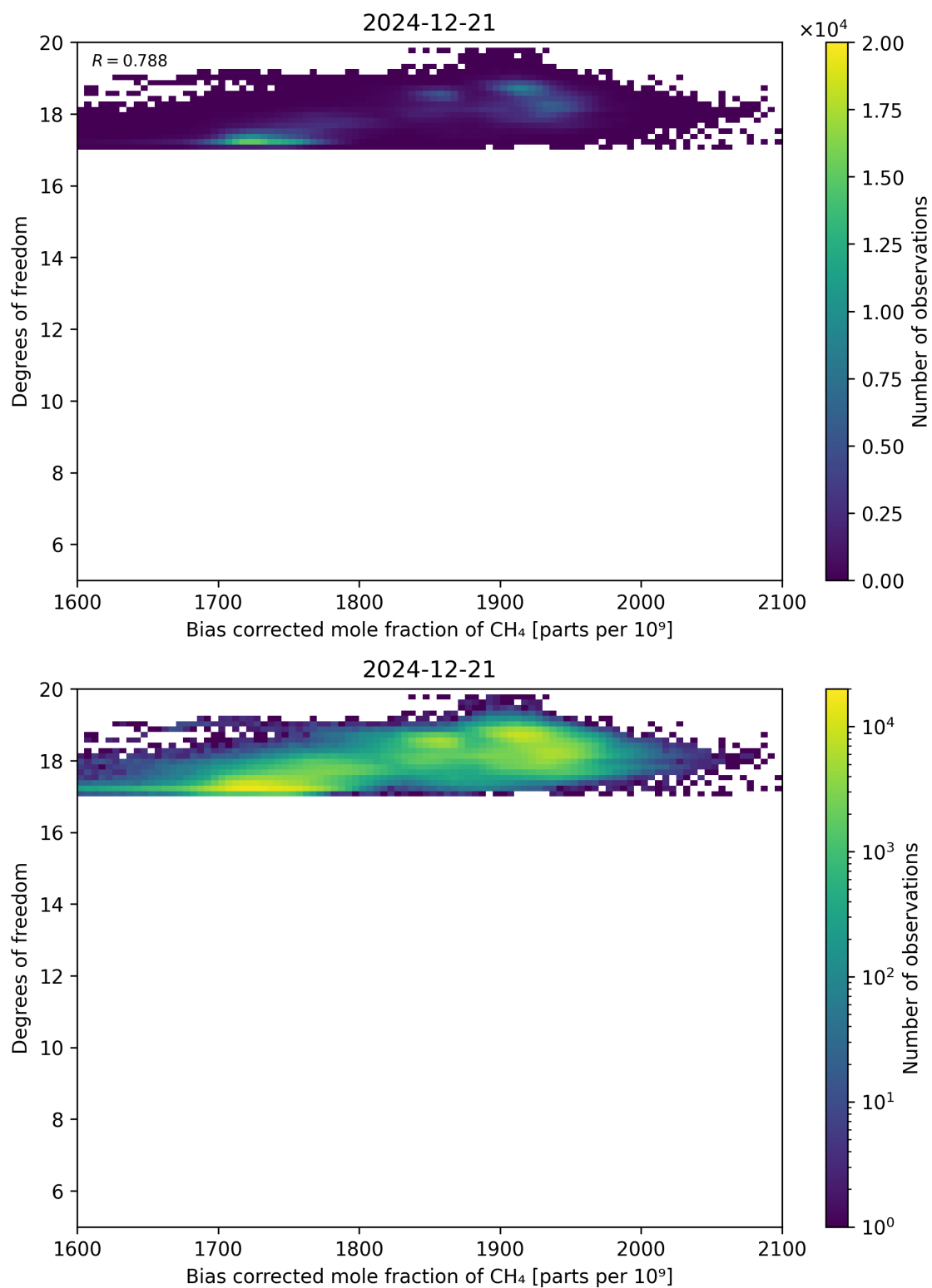
Figure 65: Scatter density plot of “Bias corrected mole fraction of \text{CH}_4 ” against “Degrees of freedom” for 2024-12-20 to 2024-12-22.
