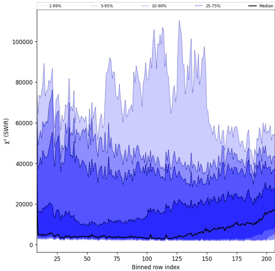
Figure 39: Along track statistics of “ \chi^2 (SWIR)” for 2024-12-20 to 2024-12-22
