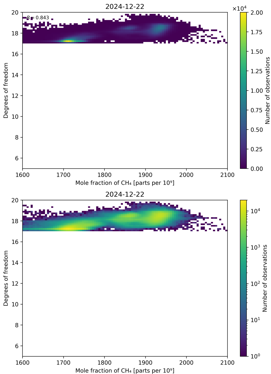
Figure 72: Scatter density plot of “Mole fraction of CH 4 ” against “Degrees of freedom” for 2024-12-22 to 2024-12-23.
