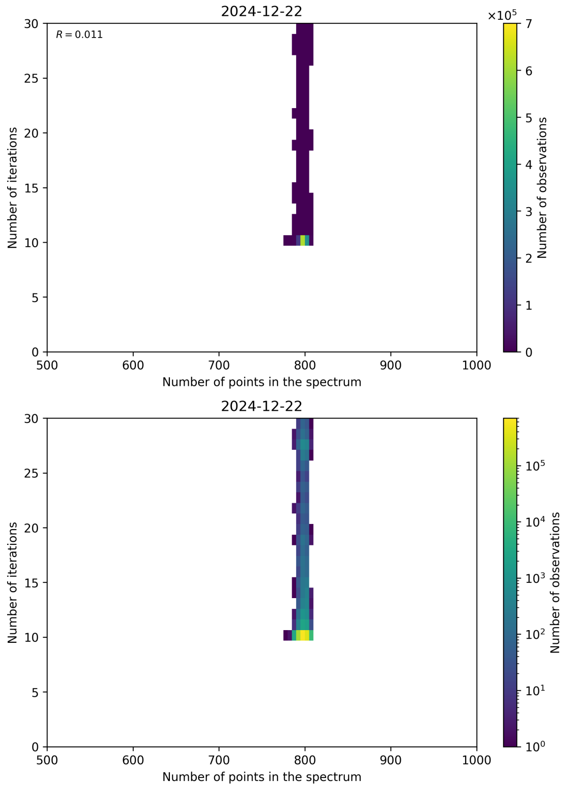
Figure 92: Scatter density plot of “Number of points in the spectrum” against “Number of iterations” for 2024-12-22 to 2024-12-23.
