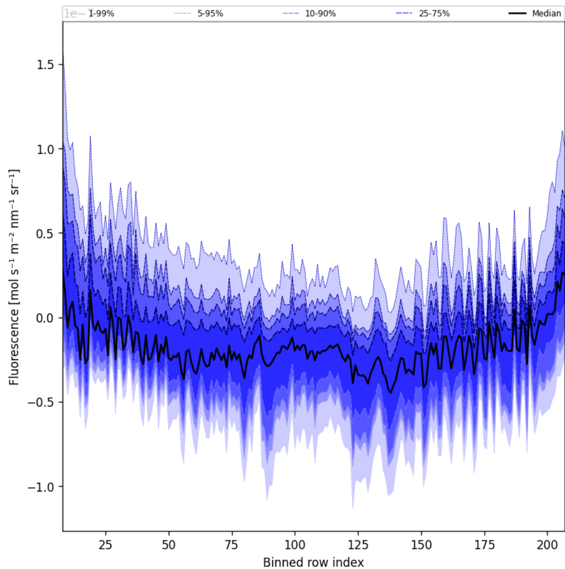
Figure 43: Along track statistics of “Fluorescence” for 2024-12-22 to 2024-12-23
