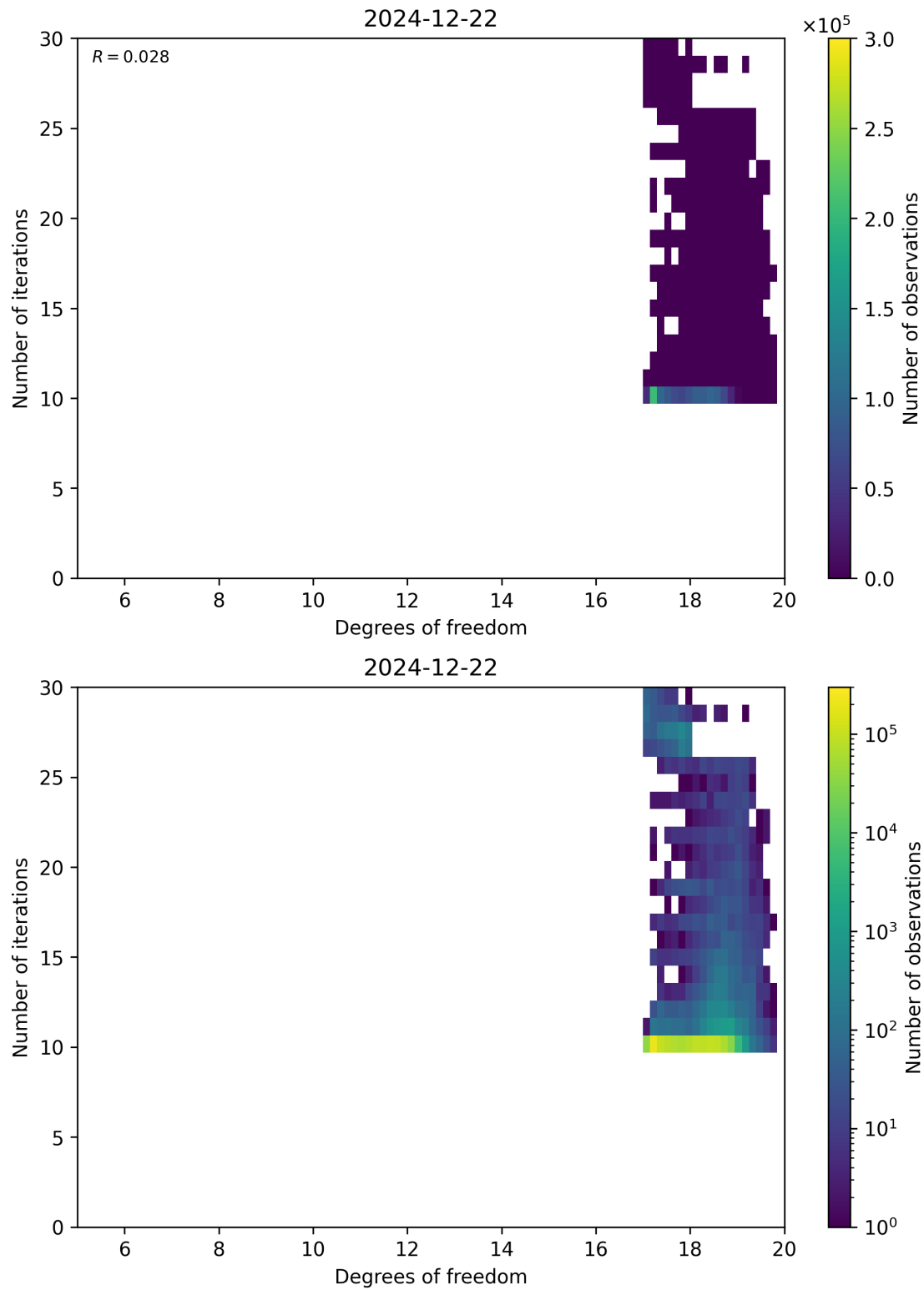
Figure 52: Scatter density plot of “Degrees of freedom” against “Number of iterations” for 2024-12-22 to 2024-12-23.
