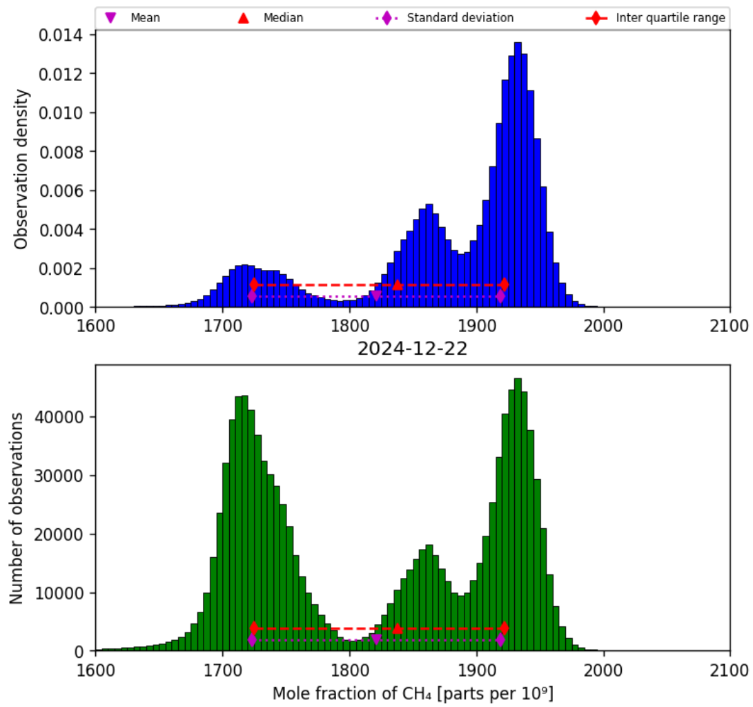
Figure 23: Histogram of “Mole fraction of CH 4 ” for 2024-12-22 to 2024-12-23
