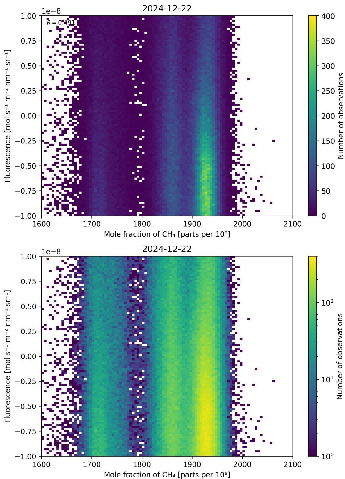
Figure 73: Scatter density plot of “Mole fraction of \text{CH}_4 ” against “Fluorescence” for 2024-12-22 to 2024-12-23.
