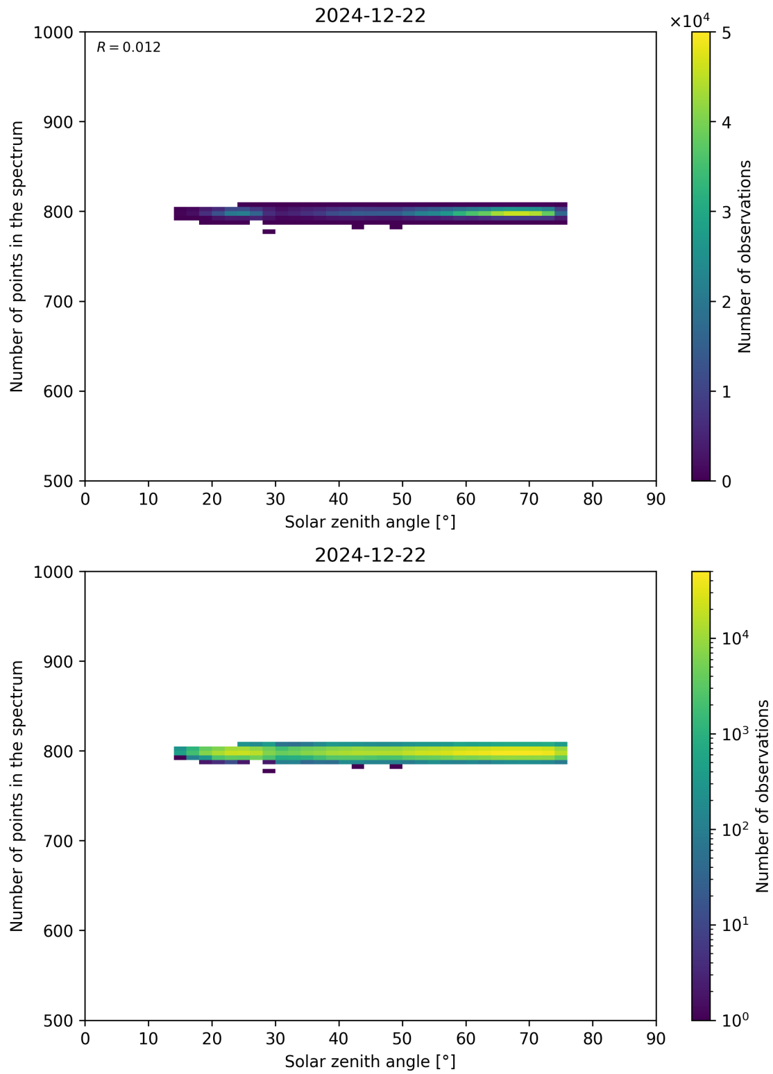
Figure 103: Scatter density plot of “Solar zenith angle” against “Number of points in the spectrum” for 2024-12-22 to 2024-12-23.
