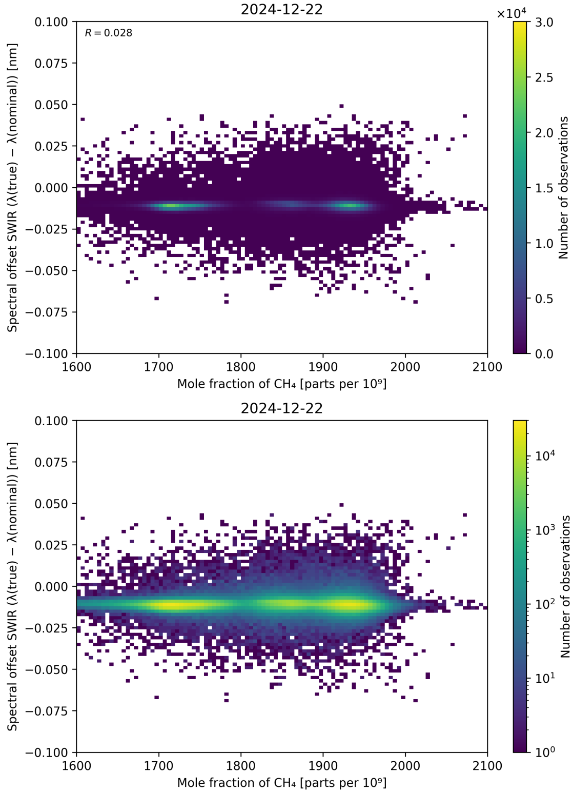
Figure 86: Scatter density plot of “Mole fraction of CH 4 ” against “Spectral offset SWIR ( \lambda_{\text{true}} - \lambda_{\text{nominal}} )” for 2024-12-22 to 2024-12-23.
