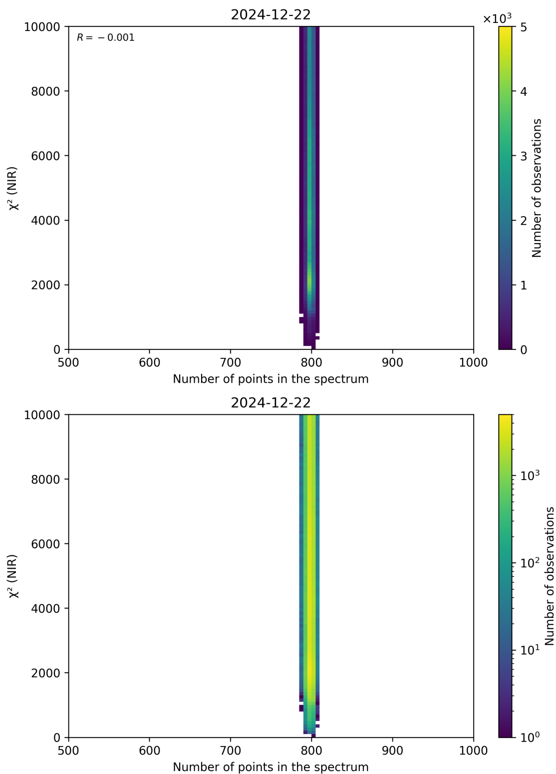
Figure 88: Scatter density plot of “Number of points in the spectrum” against “ \chi^2 (NIR)” for 2024-12-22 to 2024-12-23.
