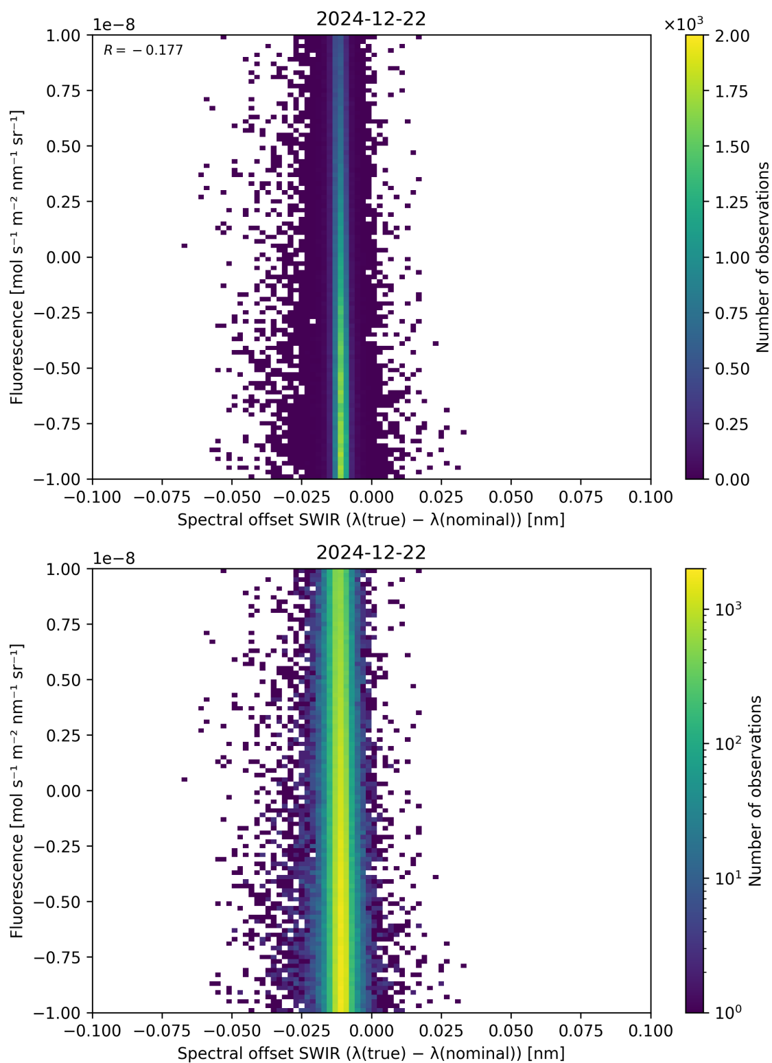
Figure 120: Scatter density plot of “Spectral offset SWIR ( \lambda_{\text{true}} - \lambda_{\text{nominal}} )” against “Fluorescence” for 2024-12-22 to 2024-12-23.
