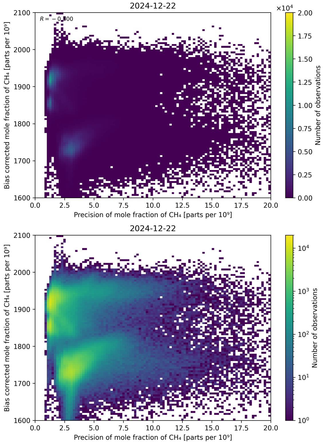
Figure 82: Scatter density plot of “Precision of mole fraction of \text{CH}_4 ” against “Bias corrected mole fraction of \text{CH}_4 ” for 2024-12-22 to 2024-12-23.
