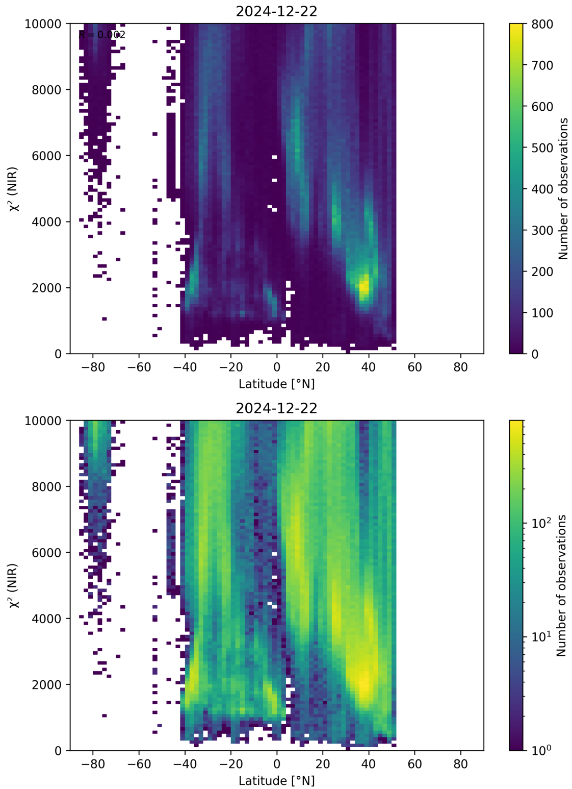
Figure 53: Scatter density plot of “Latitude” against “ \chi^2 (NIR)” for 2024-12-22 to 2024-12-23.
