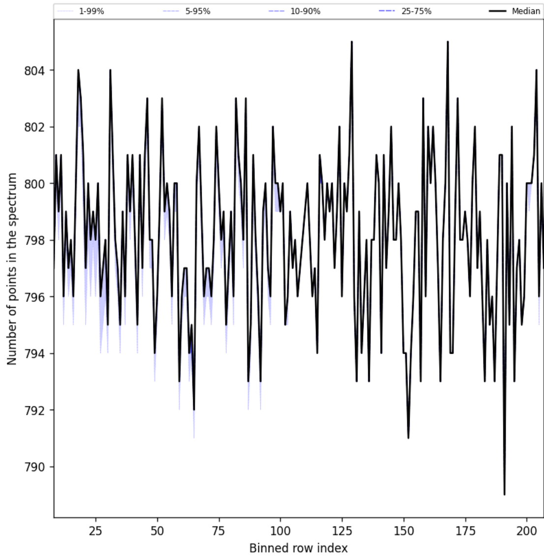
Figure 37: Along track statistics of “Number of points in the spectrum” for 2024-12-22 to 2024-12-23
