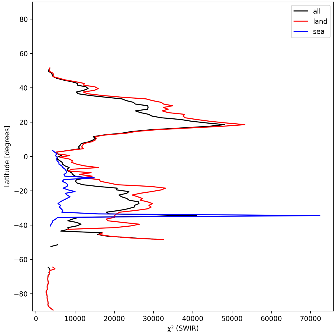
Figure 17: Zonal average of “ \chi^2 (SWIR)” for 2024-12-22 to 2024-12-23.
