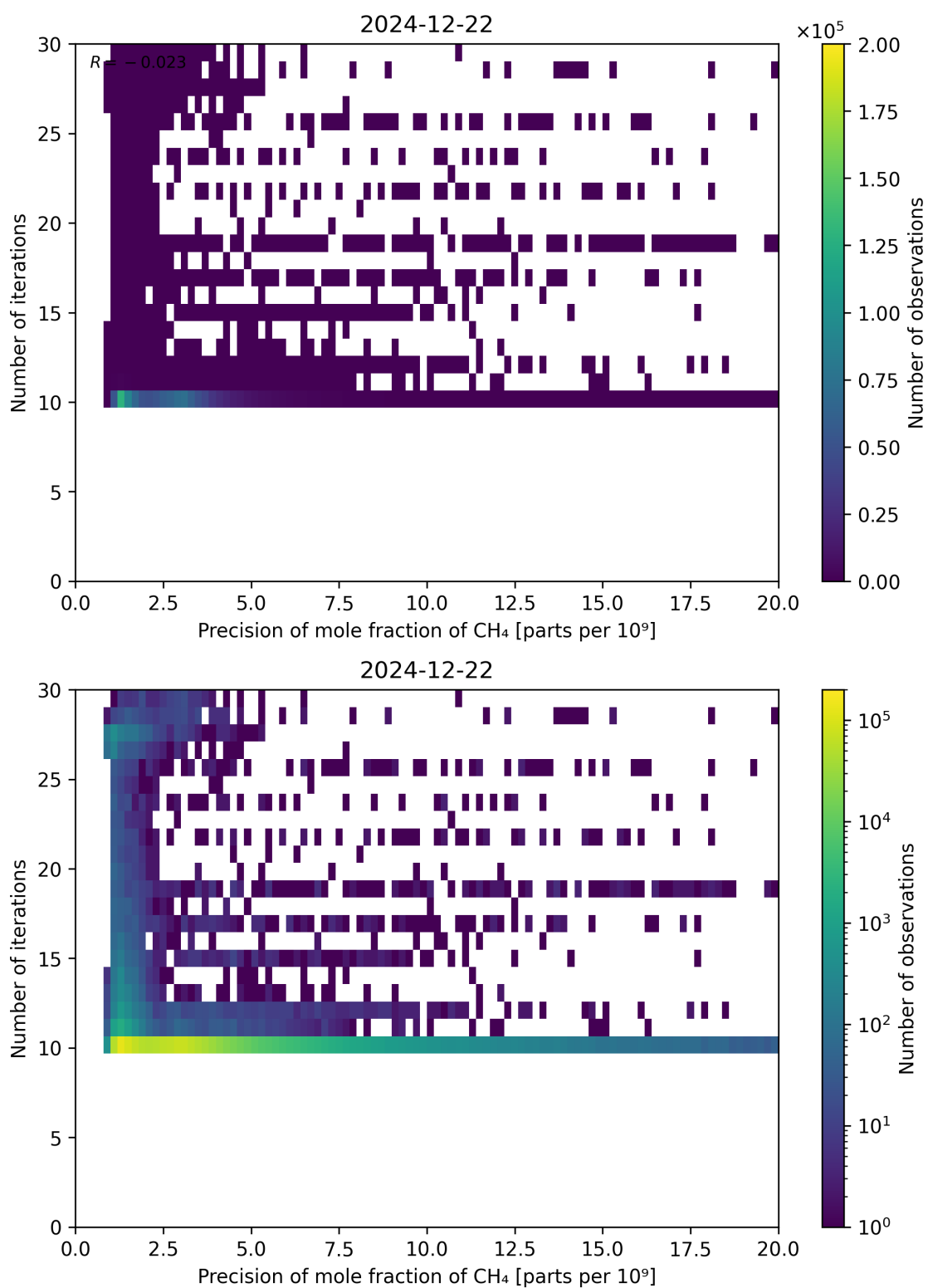
Figure 83: Scatter density plot of “Precision of mole fraction of CH 4 ” against “Number of iterations” for 2024-12-22 to 2024-12-23.
