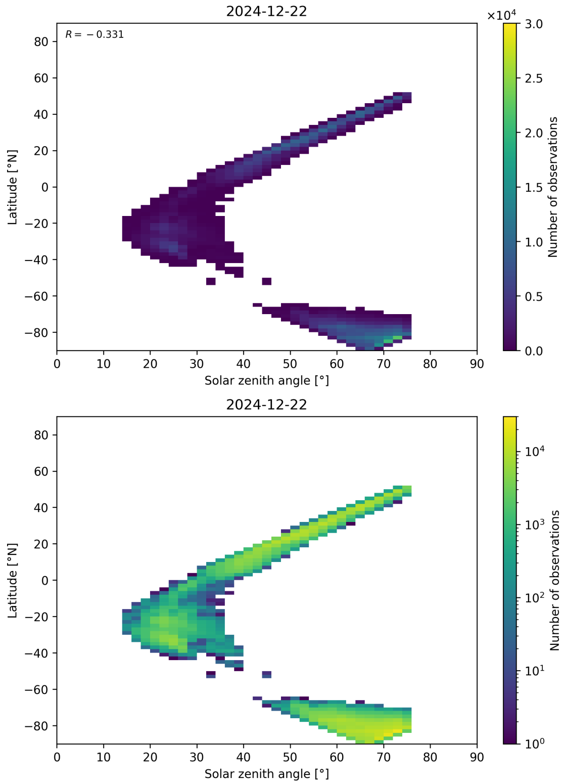
Figure 98: Scatter density plot of “Solar zenith angle” against “Latitude” for 2024-12-22 to 2024-12-23.
