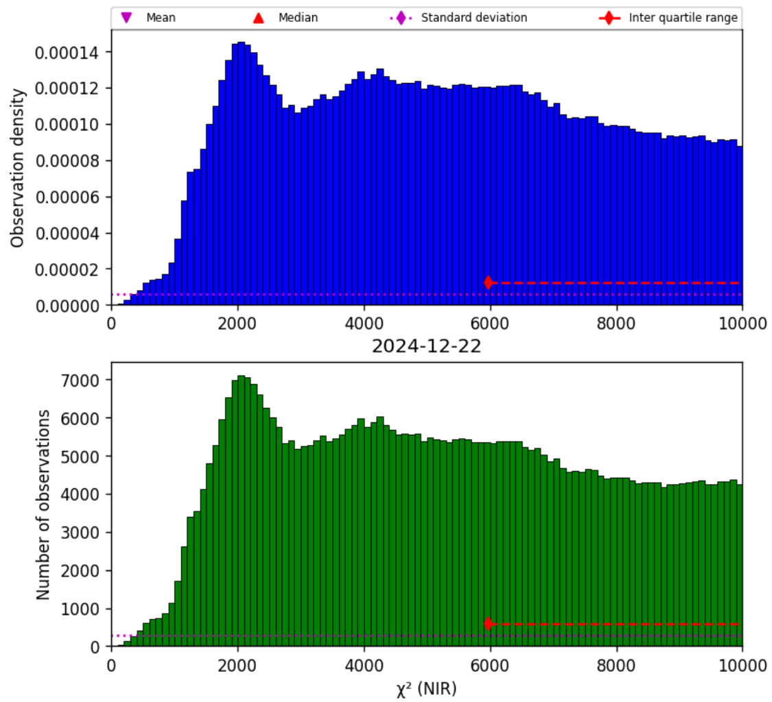
Figure 29: Histogram of " \chi^2 (NIR)" for 2024-12-22 to 2024-12-23
