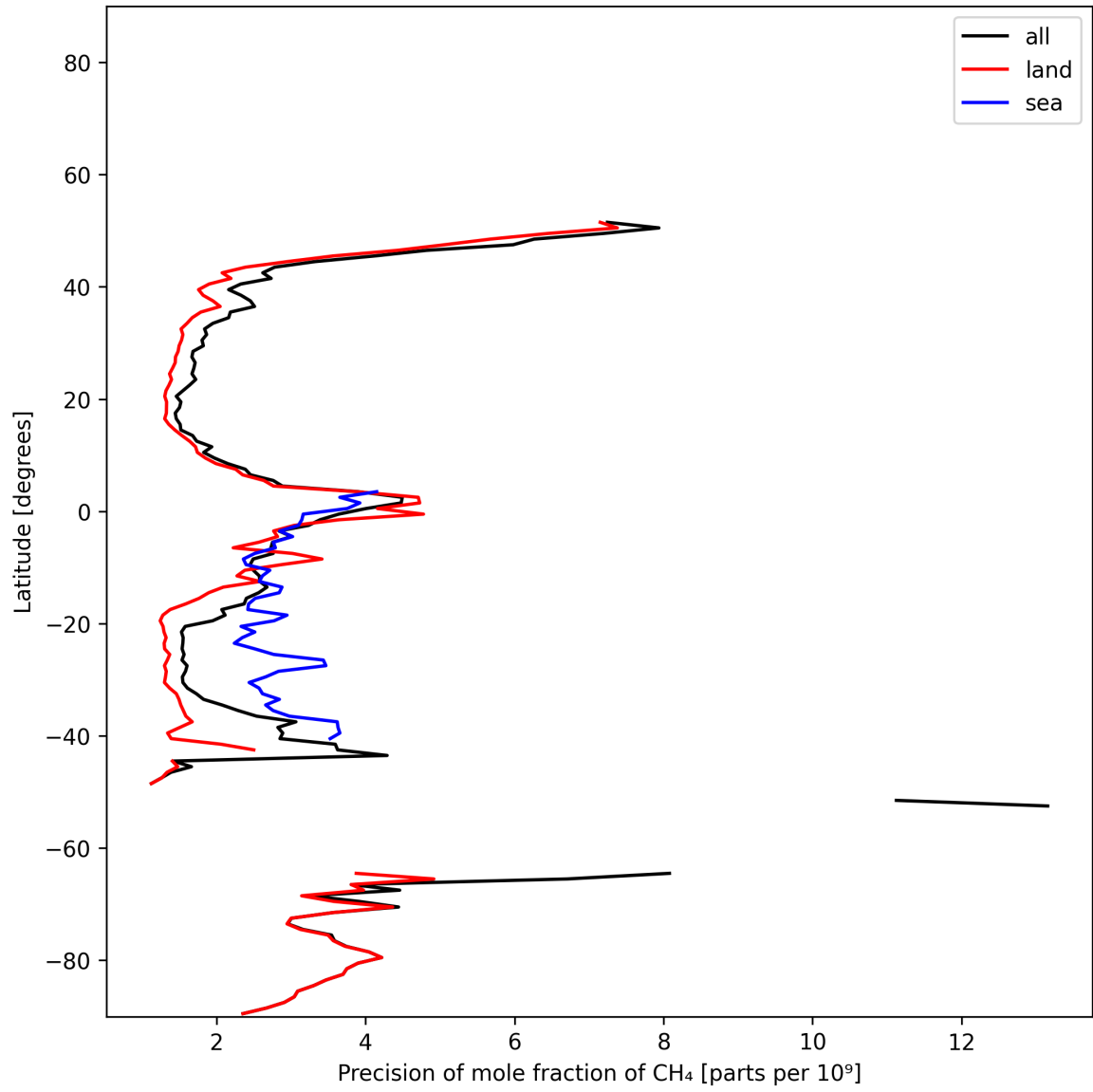
Figure 13: Zonal average of “Precision of mole fraction of CH 4 ” for 2024-12-22 to 2024-12-23.
