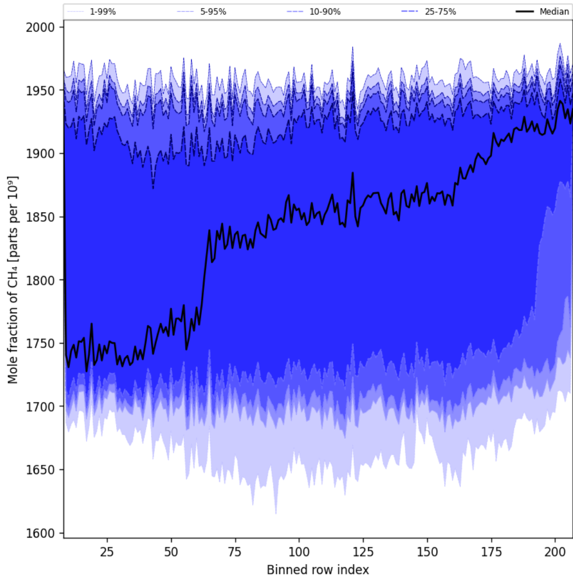
Figure 34: Along track statistics of “Mole fraction of CH 4 ” for 2024-12-22 to 2024-12-23
