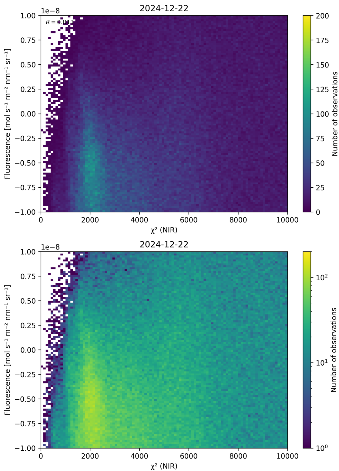
Figure 45: Scatter density plot of “ \chi^2 (NIR)” against “Fluorescence” for 2024-12-22 to 2024-12-23.
