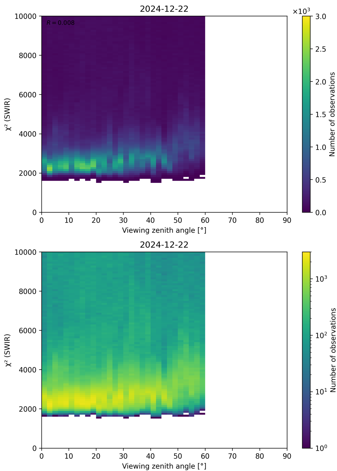
Figure 106: Scatter density plot of “Viewing zenith angle” against “ \chi^2 (SWIR)” for 2024-12-22 to 2024-12-23.
