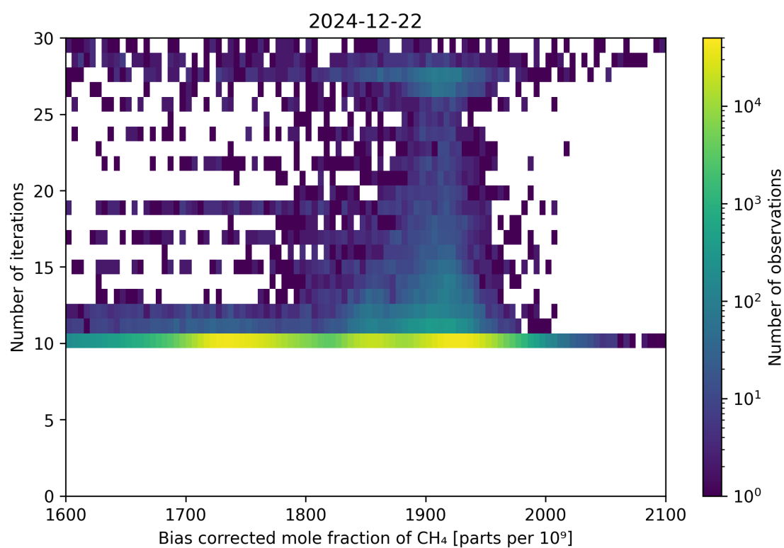
Figure 67: Scatter density plot of “Bias corrected mole fraction of \text{CH}_4 ” against “Number of iterations” for 2024-12-22 to 2024-12-23.
