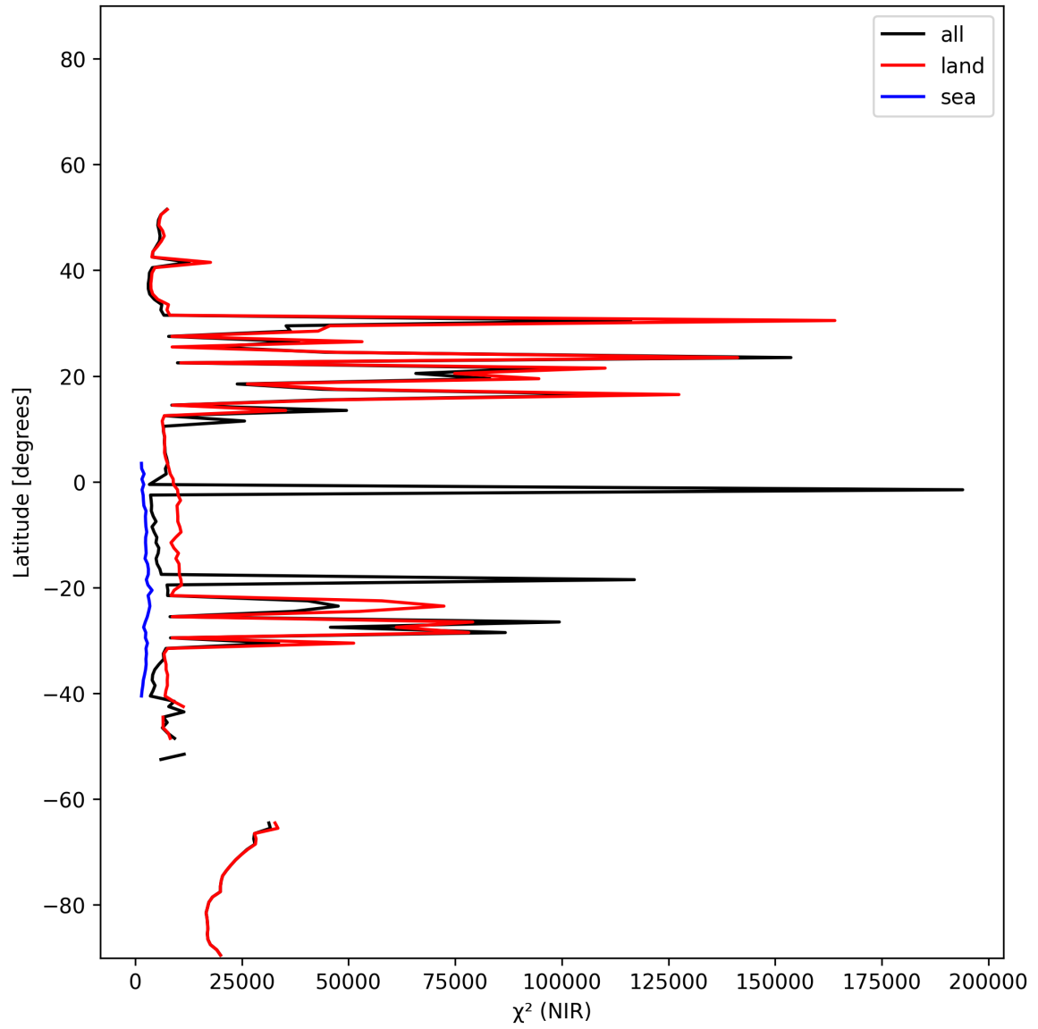
Figure 18: Zonal average of “ \chi^2 (NIR)” for 2024-12-22 to 2024-12-23.
