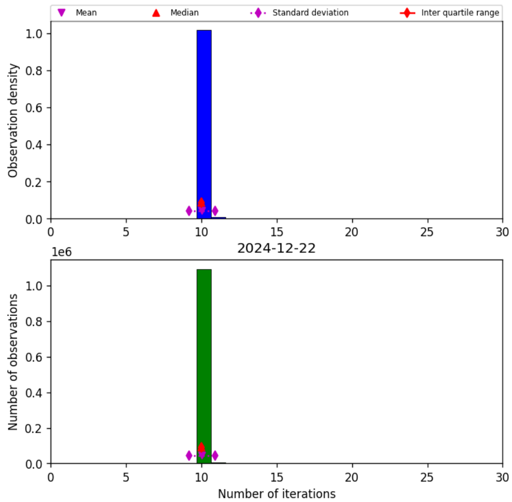
Figure 31: Histogram of “Number of iterations” for 2024-12-22 to 2024-12-23
