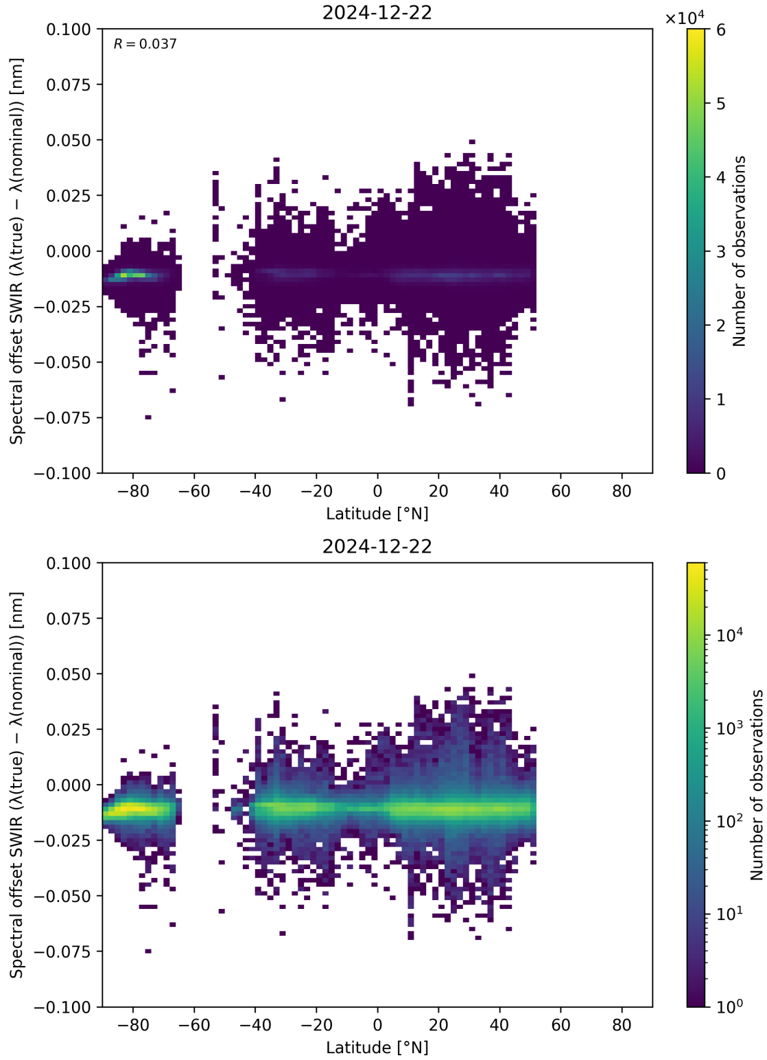
Figure 62: Scatter density plot of “Latitude” against “Spectral offset SWIR ( \lambda_{\text{true}} - \lambda_{\text{nominal}} )” for 2024-12-22 to 2024-12-23.
