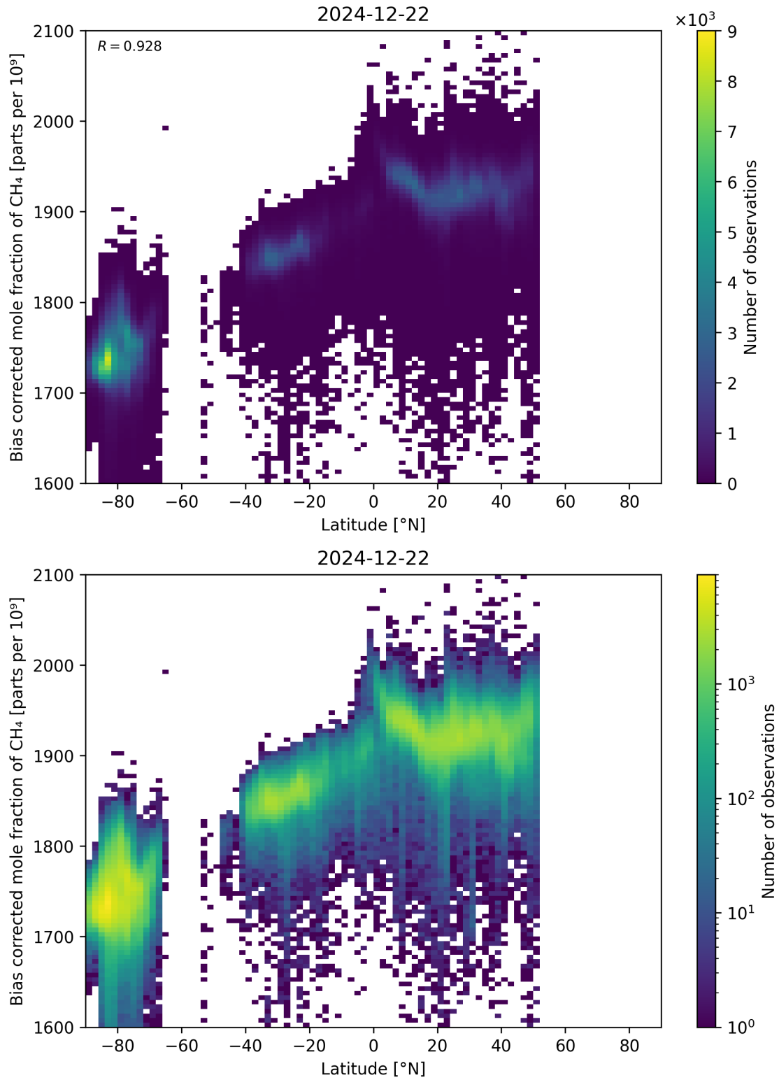
Figure 58: Scatter density plot of “Latitude” against “Bias corrected mole fraction of CH 4 ” for 2024-12-22 to 2024-12-23.
