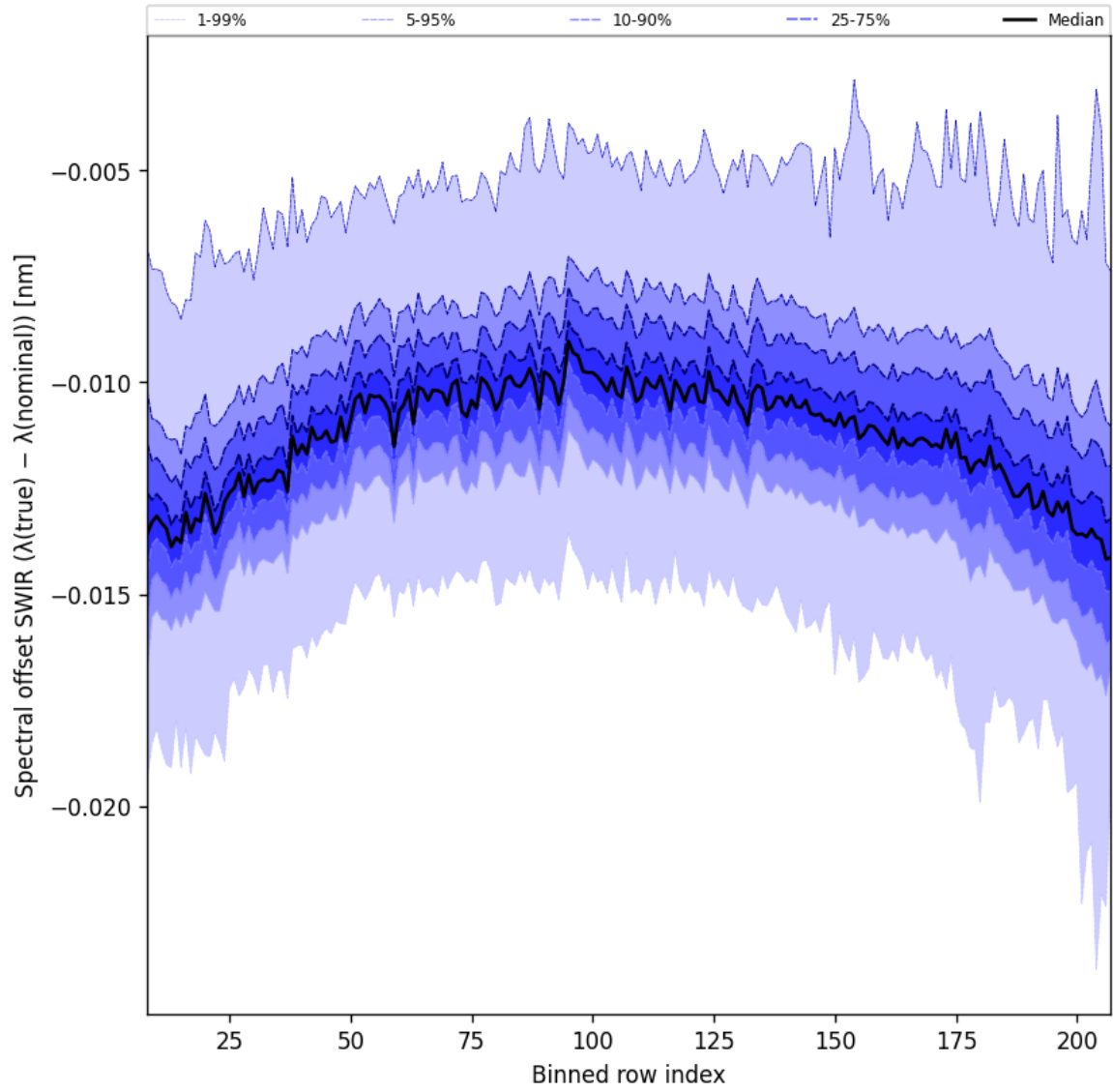
Figure 38: Along track statistics of “Spectral offset SWIR ( \lambda_{\text{true}} - \lambda_{\text{nominal}} )” for 2024-12-22 to 2024-12-23
