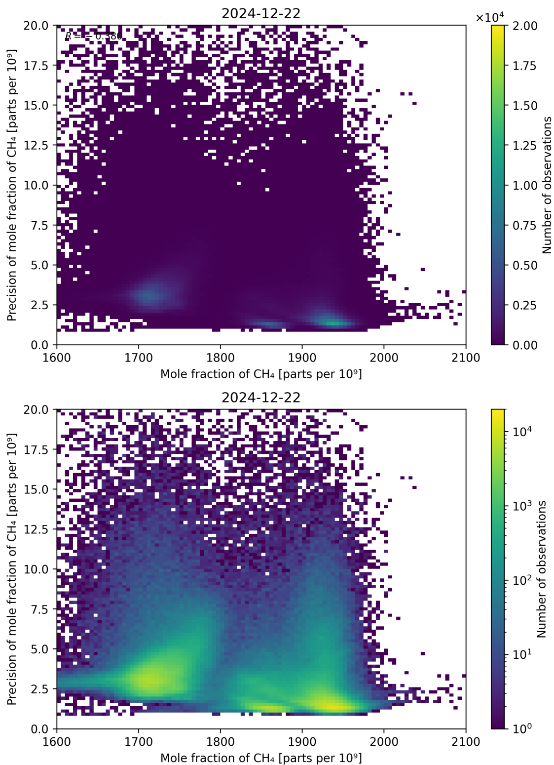
Figure 75: Scatter density plot of “Mole fraction of CH 4 ” against “Precision of mole fraction of CH 4 ” for 2024-12-22 to 2024-12-23.
