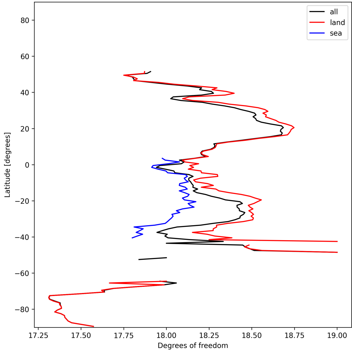
Figure 19: Zonal average of “Degrees of freedom” for 2024-12-22 to 2024-12-23.
