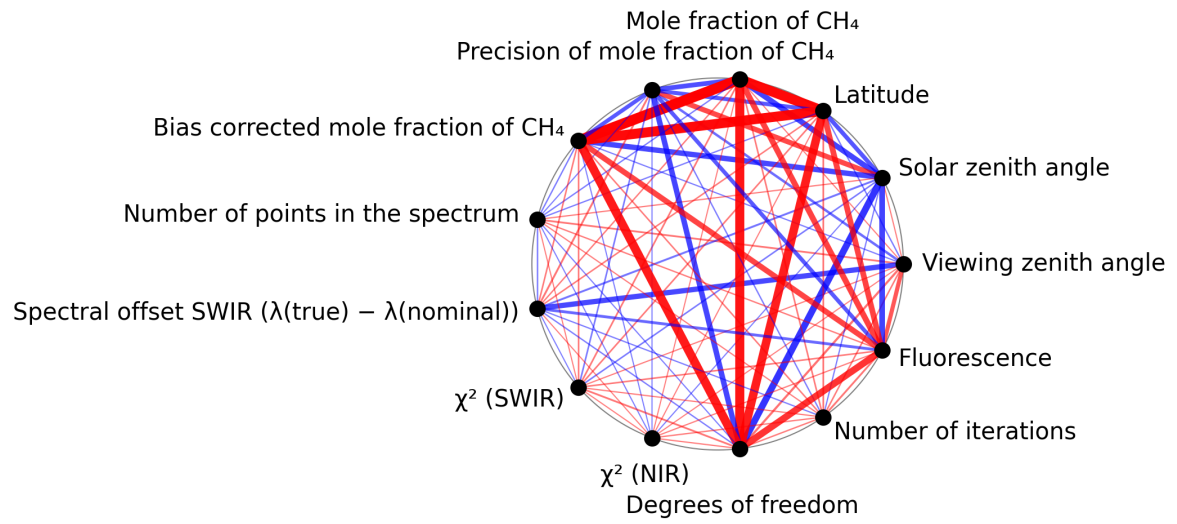
Figure 1: Map of correlation graph for 2024-12-22 to 2024-12-23.
