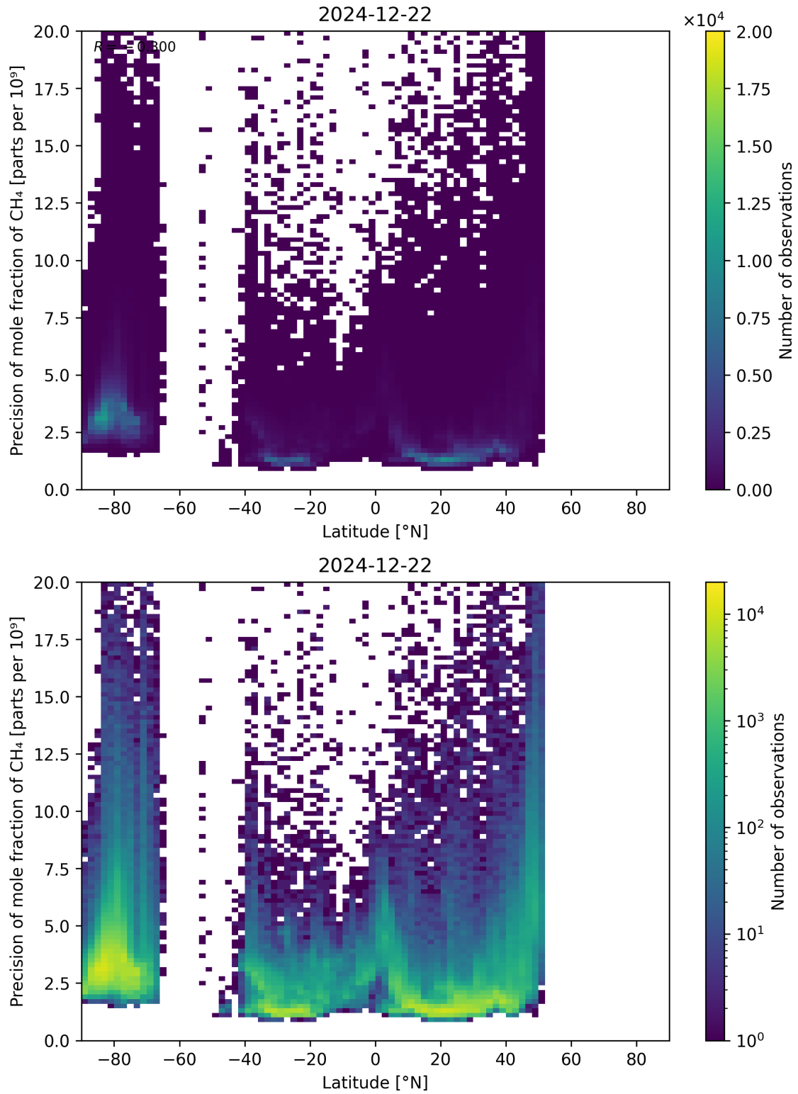
Figure 59: Scatter density plot of “Latitude” against “Precision of mole fraction of CH 4 ” for 2024-12-22 to 2024-12-23.
