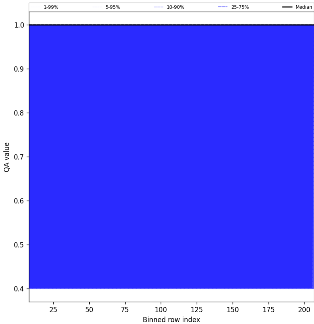
Figure 33: Along track statistics of “QA value” for 2024-12-22 to 2024-12-23
