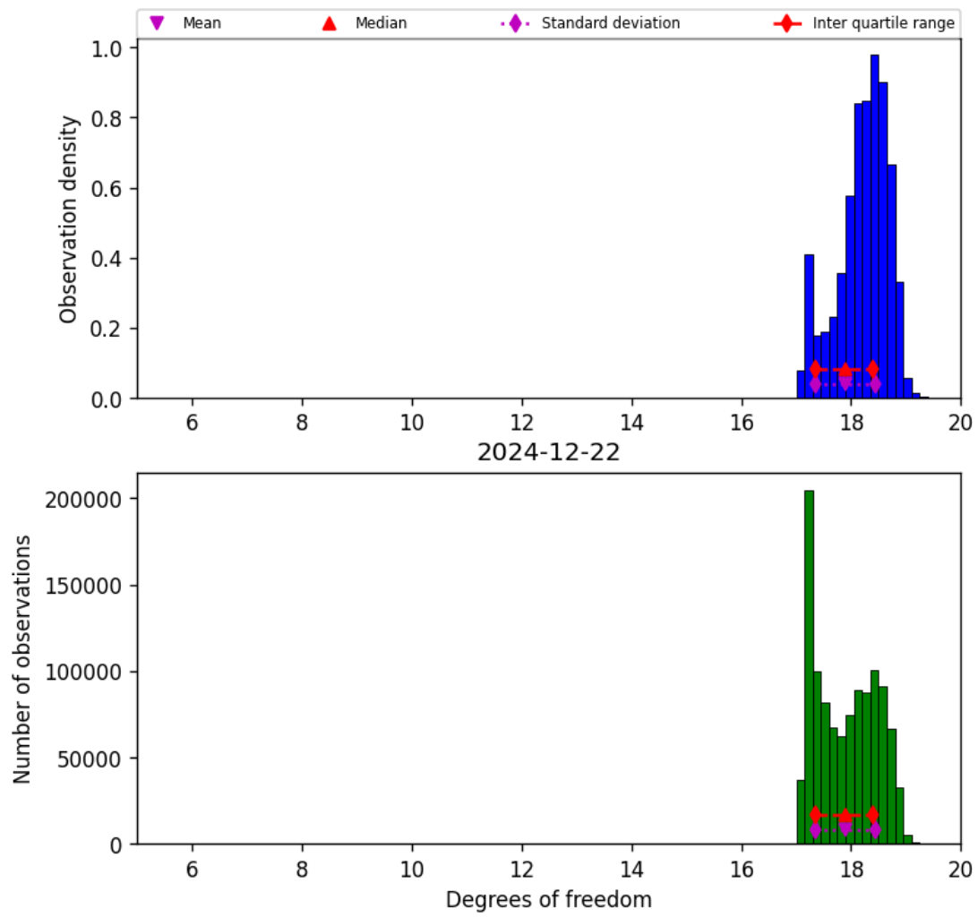
Figure 30: Histogram of “Degrees of freedom” for 2024-12-22 to 2024-12-23
