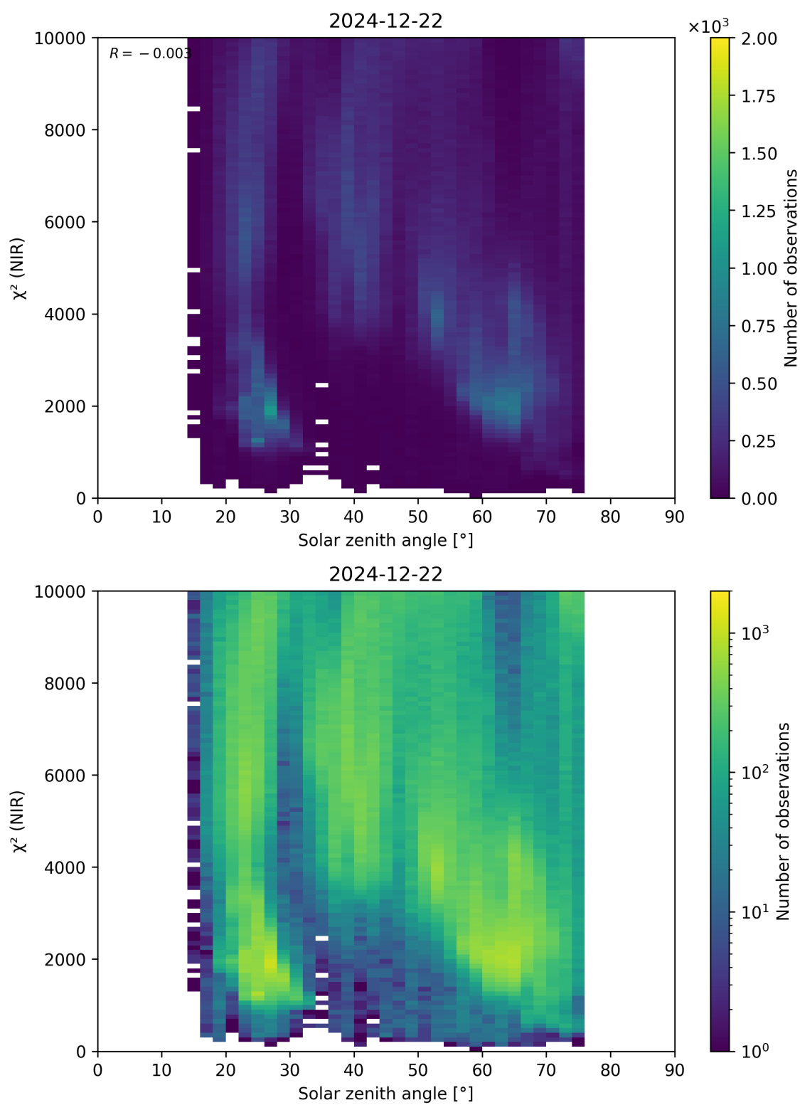
Figure 94: Scatter density plot of “Solar zenith angle” against “ \chi^2 (NIR)” for 2024-12-22 to 2024-12-23.
