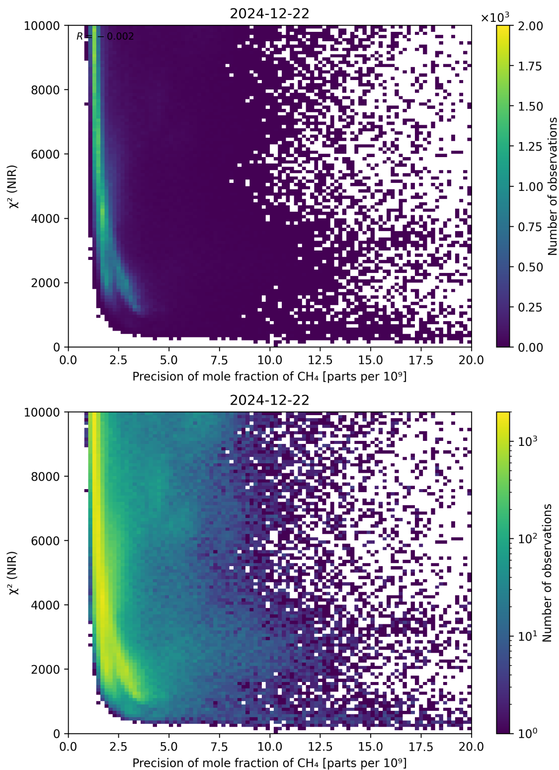
Figure 78: Scatter density plot of “Precision of mole fraction of \text{CH}_4 ” against “ \chi^2 (NIR)” for 2024-12-22 to 2024-12-23.
