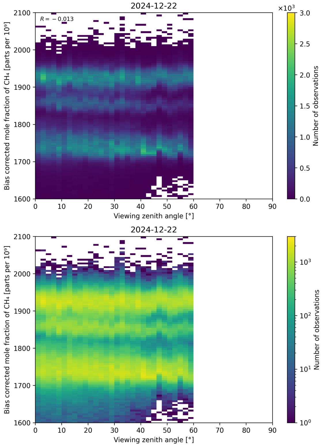
Figure 111: Scatter density plot of “Viewing zenith angle” against “Bias corrected mole fraction of CH 4 ” for 2024-12-22 to 2024-12-23.
