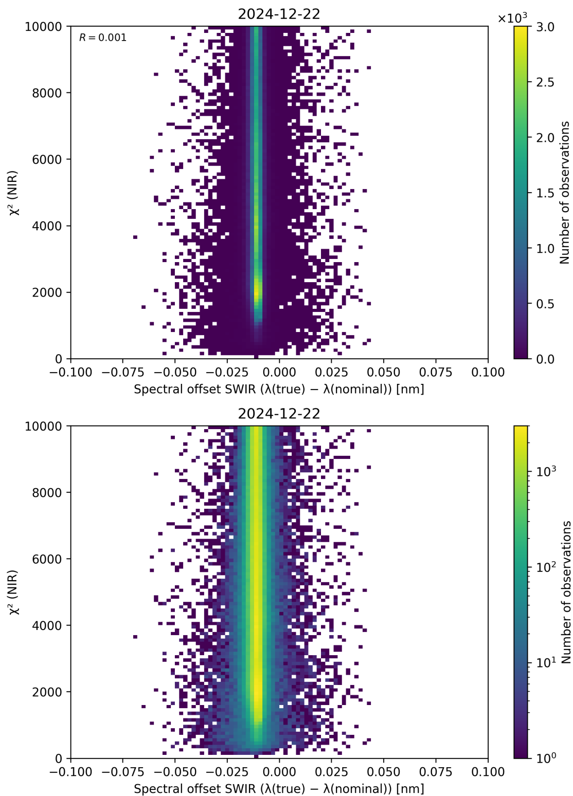
Figure 117: Scatter density plot of “Spectral offset SWIR ( \lambda_{\text{true}} - \lambda_{\text{nominal}} )” against “ \chi^2 (NIR)” for 2024-12-22 to 2024-12-23.
