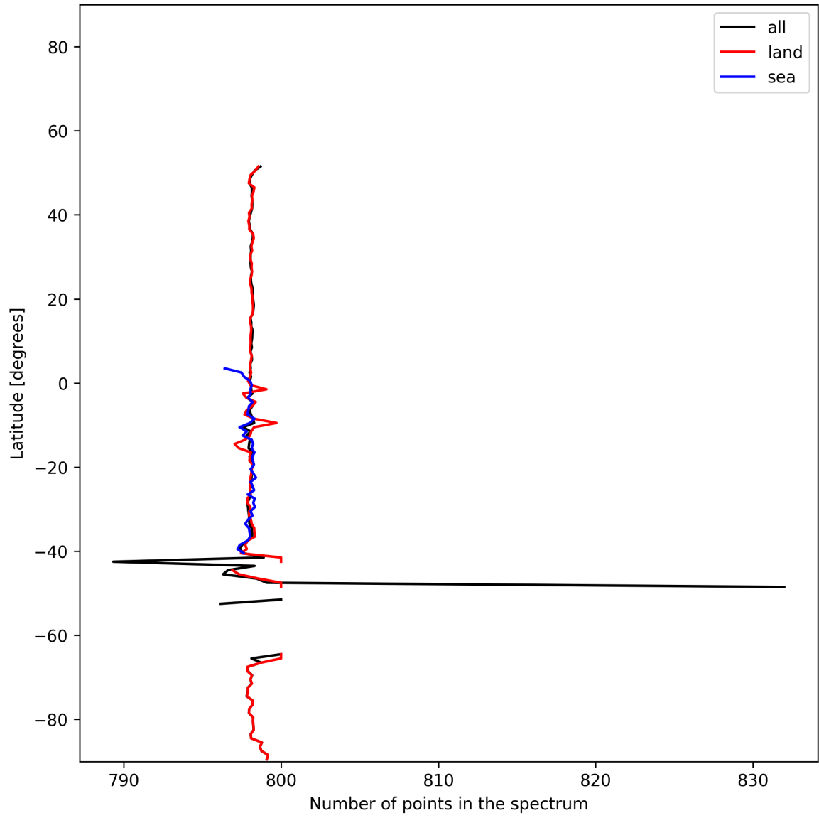
Figure 15: Zonal average of “Number of points in the spectrum” for 2024-12-22 to 2024-12-23.
