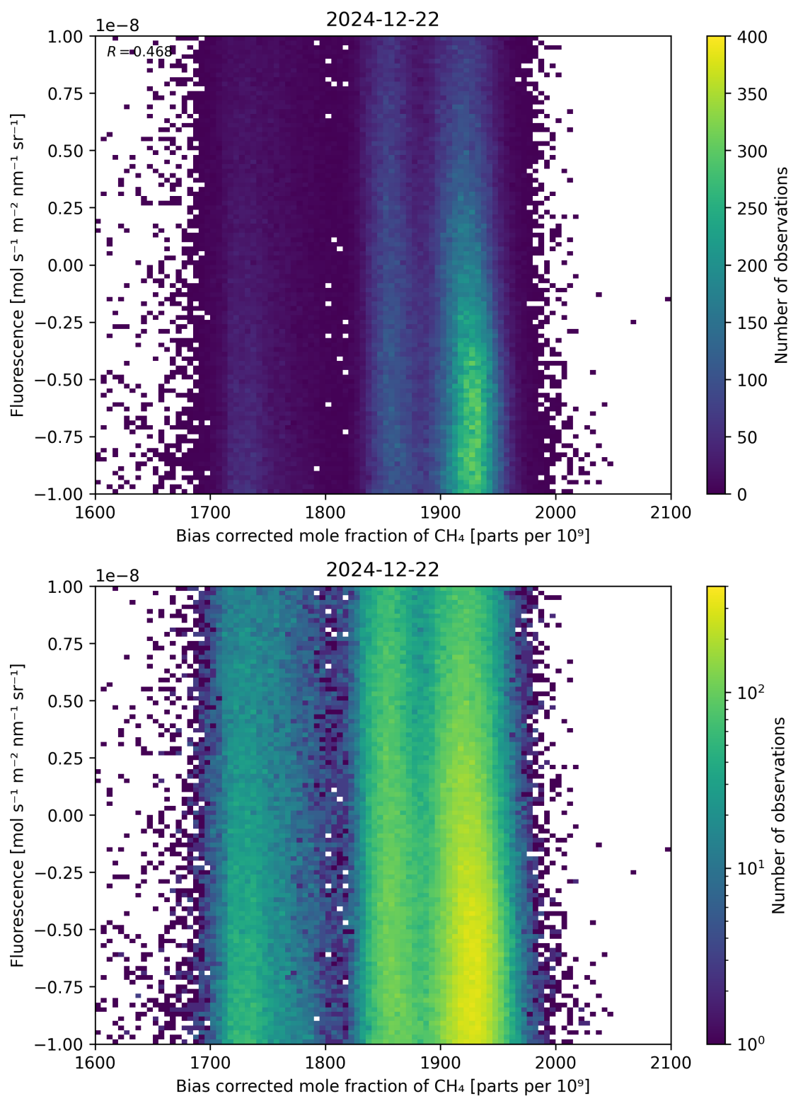
Figure 66: Scatter density plot of “Bias corrected mole fraction of CH 4 ” against “Fluorescence” for 2024-12-22 to 2024-12-23.
