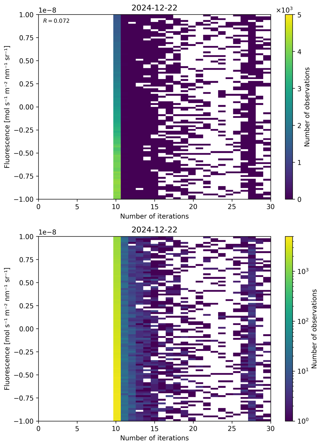
Figure 87: Scatter density plot of “Number of iterations” against “Fluorescence” for 2024-12-22 to 2024-12-23.
