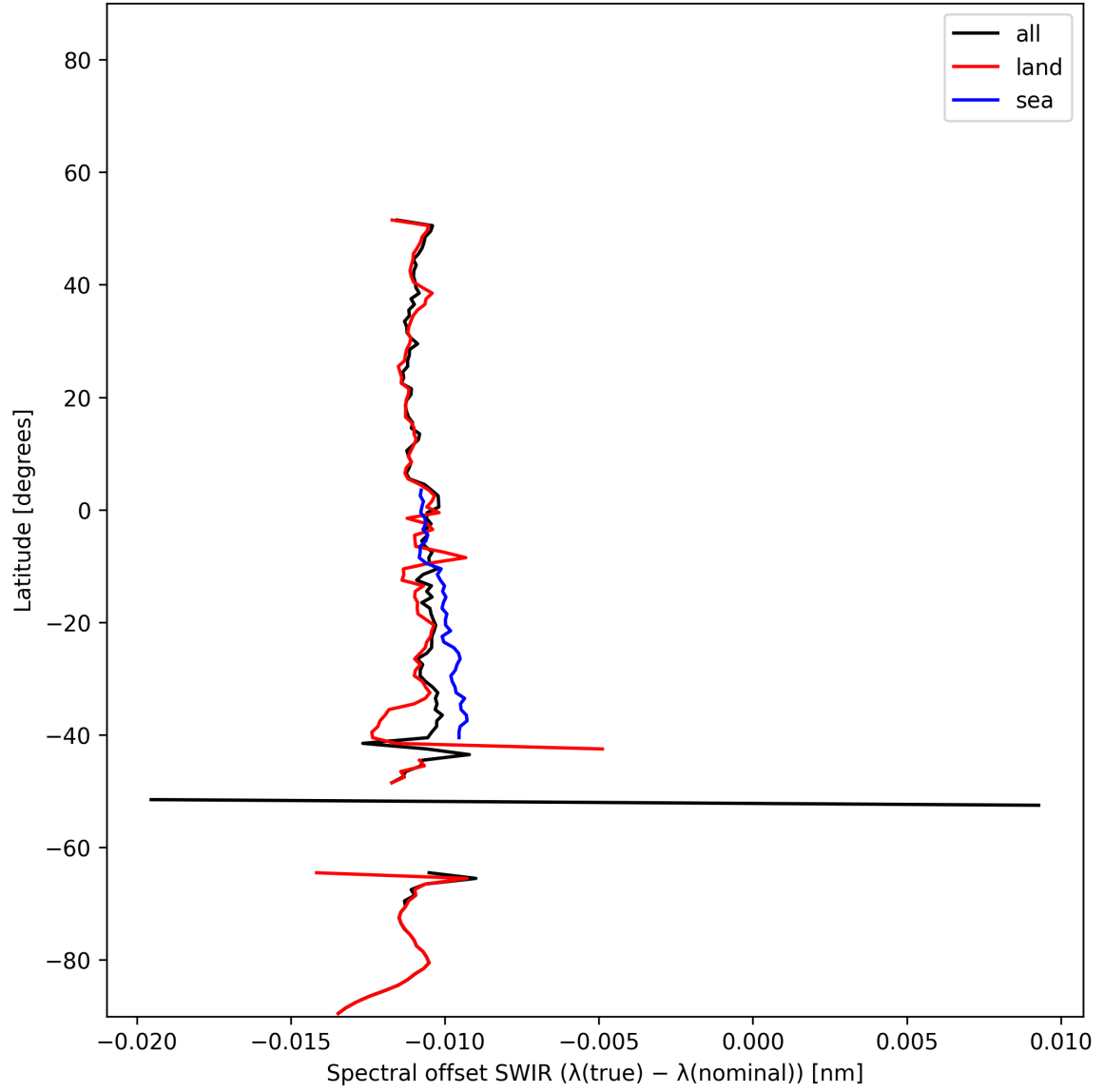
Figure 16: Zonal average of “Spectral offset SWIR ( \lambda_{\text{true}} - \lambda_{\text{nominal}} )” for 2024-12-22 to 2024-12-23.
