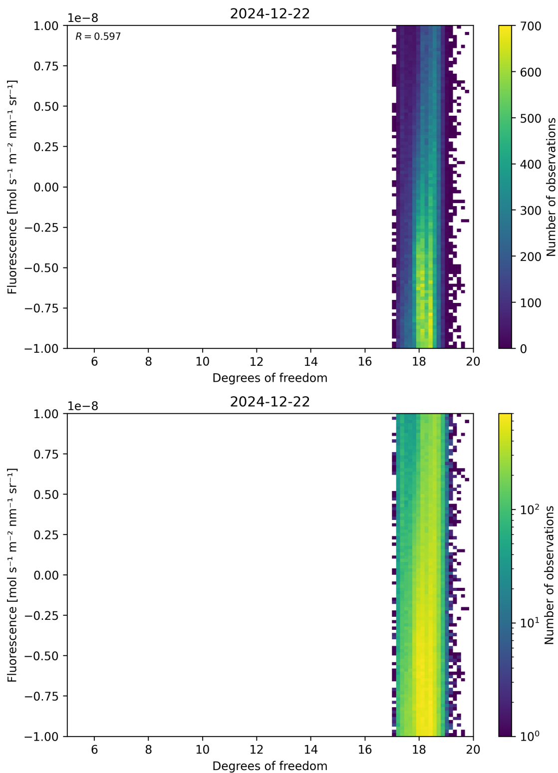
Figure 51: Scatter density plot of “Degrees of freedom” against “Fluorescence” for 2024-12-22 to 2024-12-23.
