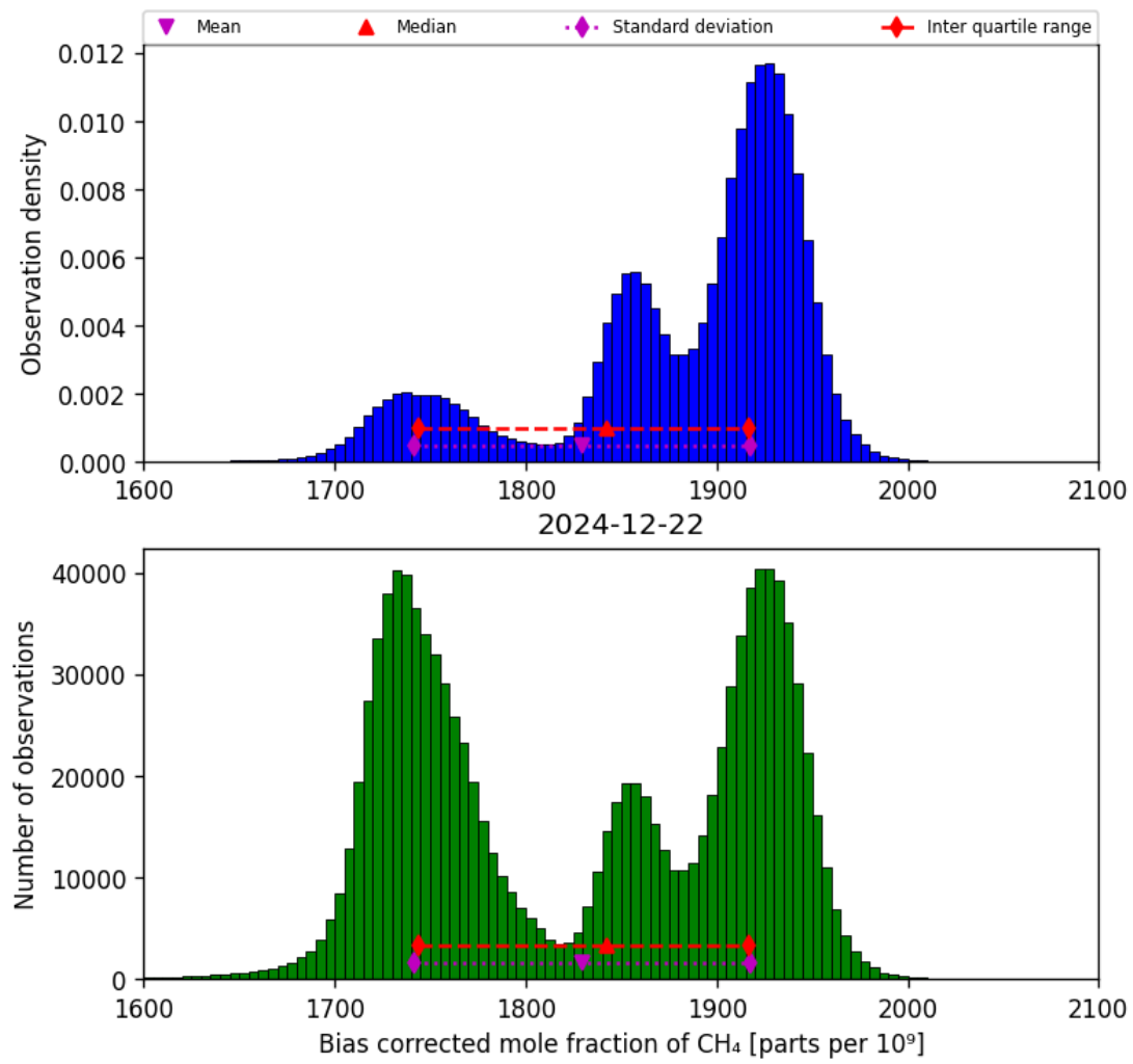
Figure 25: Histogram of “Bias corrected mole fraction of CH 4 ” for 2024-12-22 to 2024-12-23
