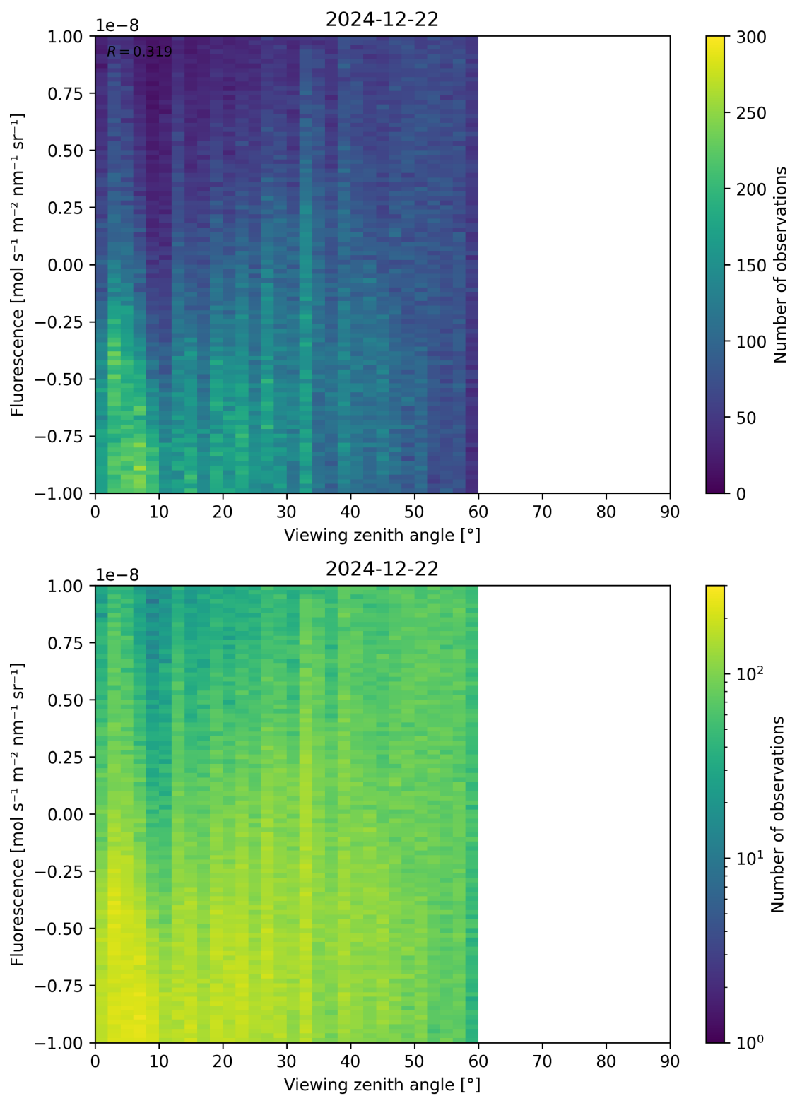
Figure 108: Scatter density plot of “Viewing zenith angle” against “Fluorescence” for 2024-12-22 to 2024-12-23.
