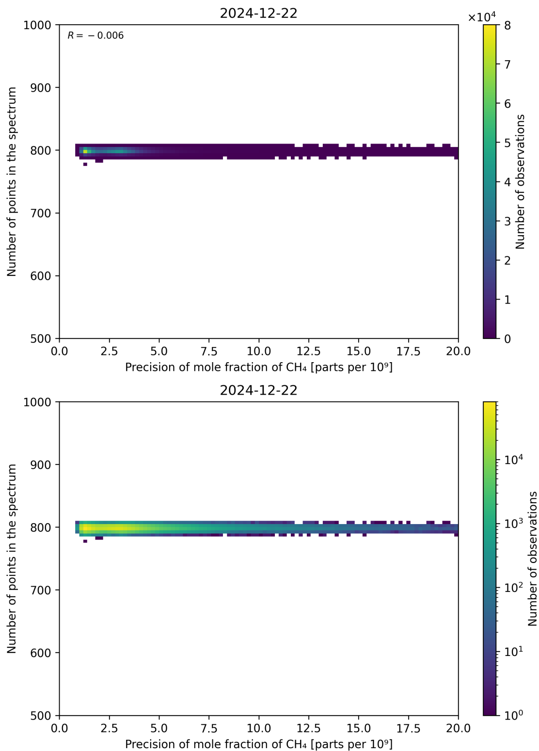
Figure 84: Scatter density plot of “Precision of mole fraction of CH 4 ” against “Number of points in the spectrum” for 2024-12-22 to 2024-12-23.
