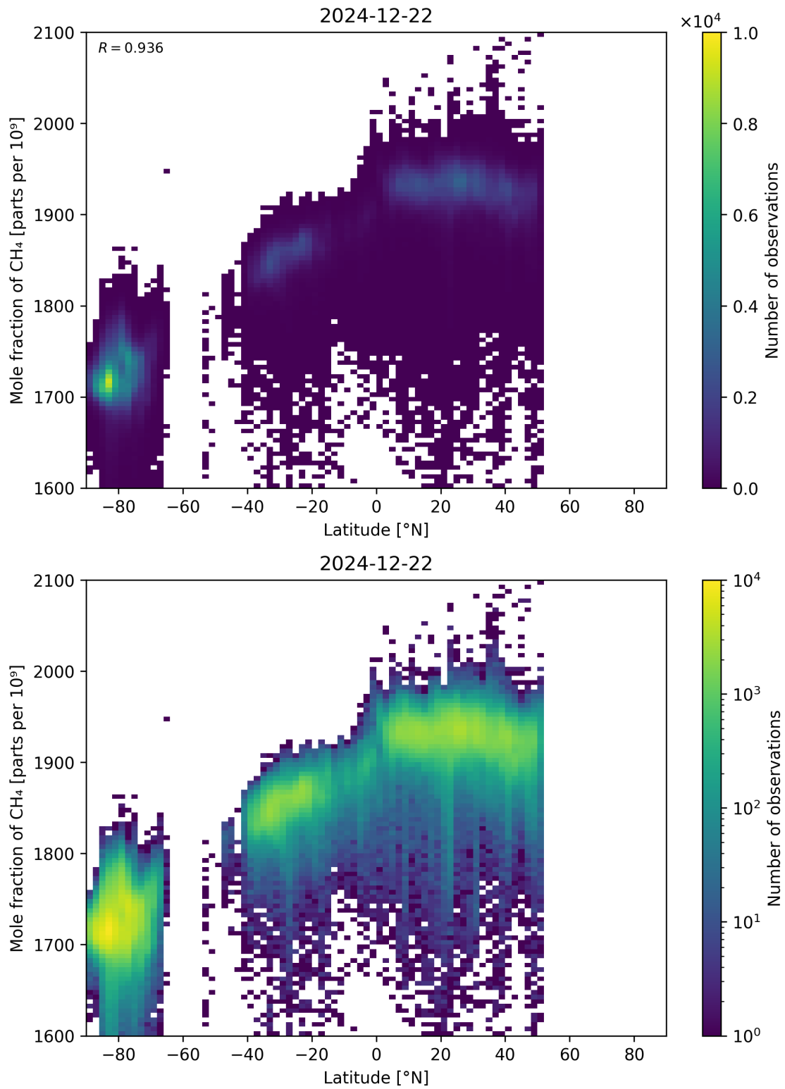
Figure 57: Scatter density plot of “Latitude” against “Mole fraction of CH 4 ” for 2024-12-22 to 2024-12-23.
