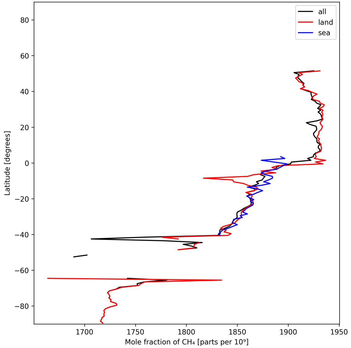
Figure 12: Zonal average of “Mole fraction of \text{CH}_4 ” for 2024-12-22 to 2024-12-23.
