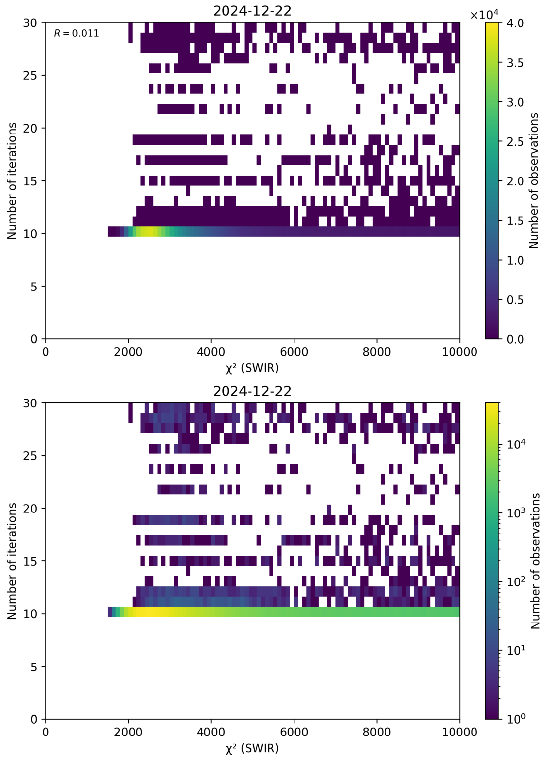
Figure 50: Scatter density plot of “ \chi^2 (SWIR)” against “Number of iterations” for 2024-12-22 to 2024-12-23.
