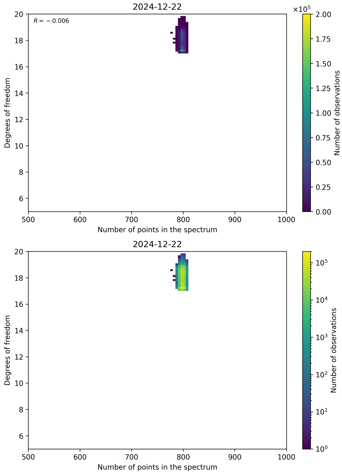
Figure 90: Scatter density plot of “Number of points in the spectrum” against “Degrees of freedom” for 2024-12-22 to 2024-12-23.
