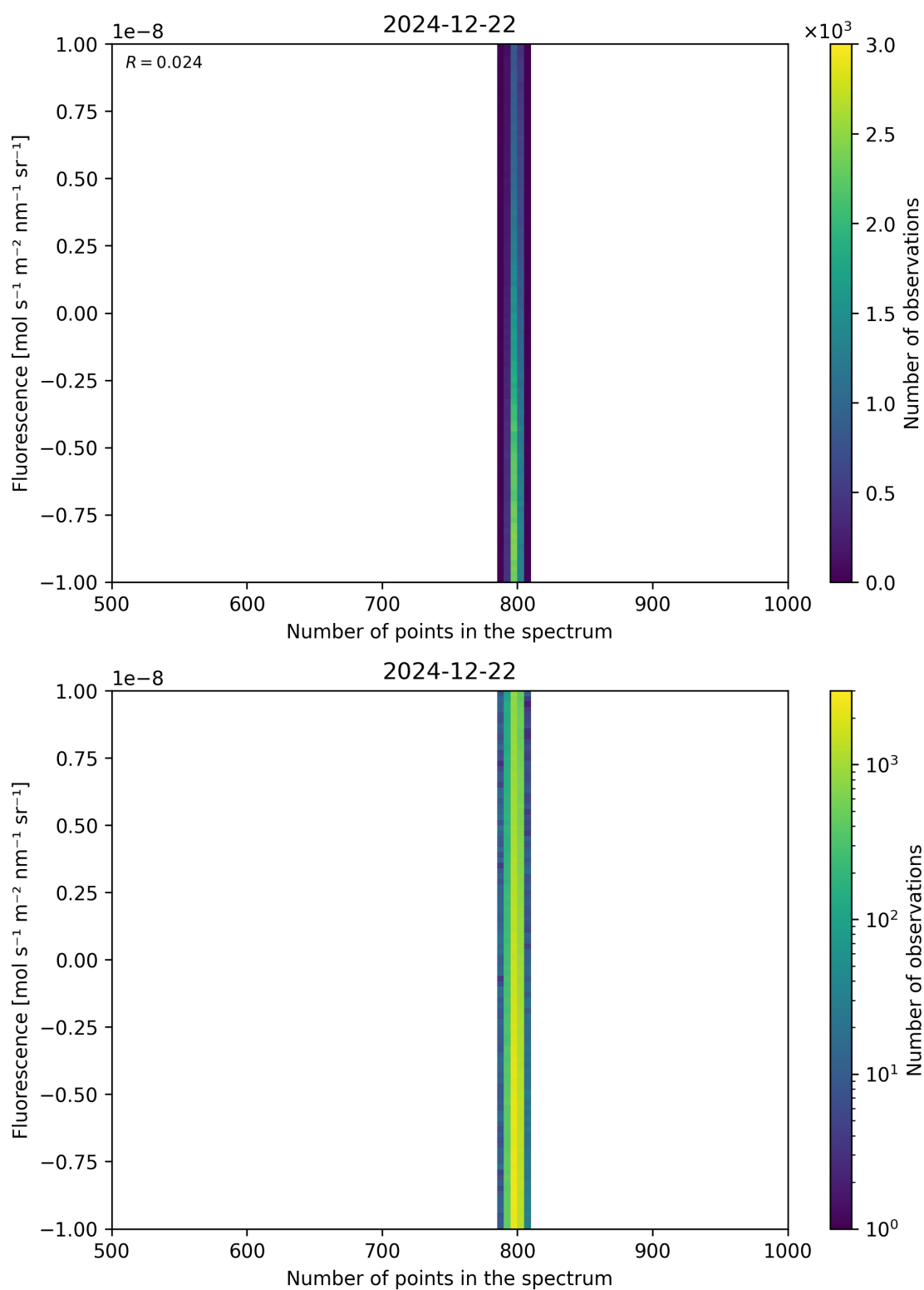
Figure 91: Scatter density plot of “Number of points in the spectrum” against “Fluorescence” for 2024-12-22 to 2024-12-23.
