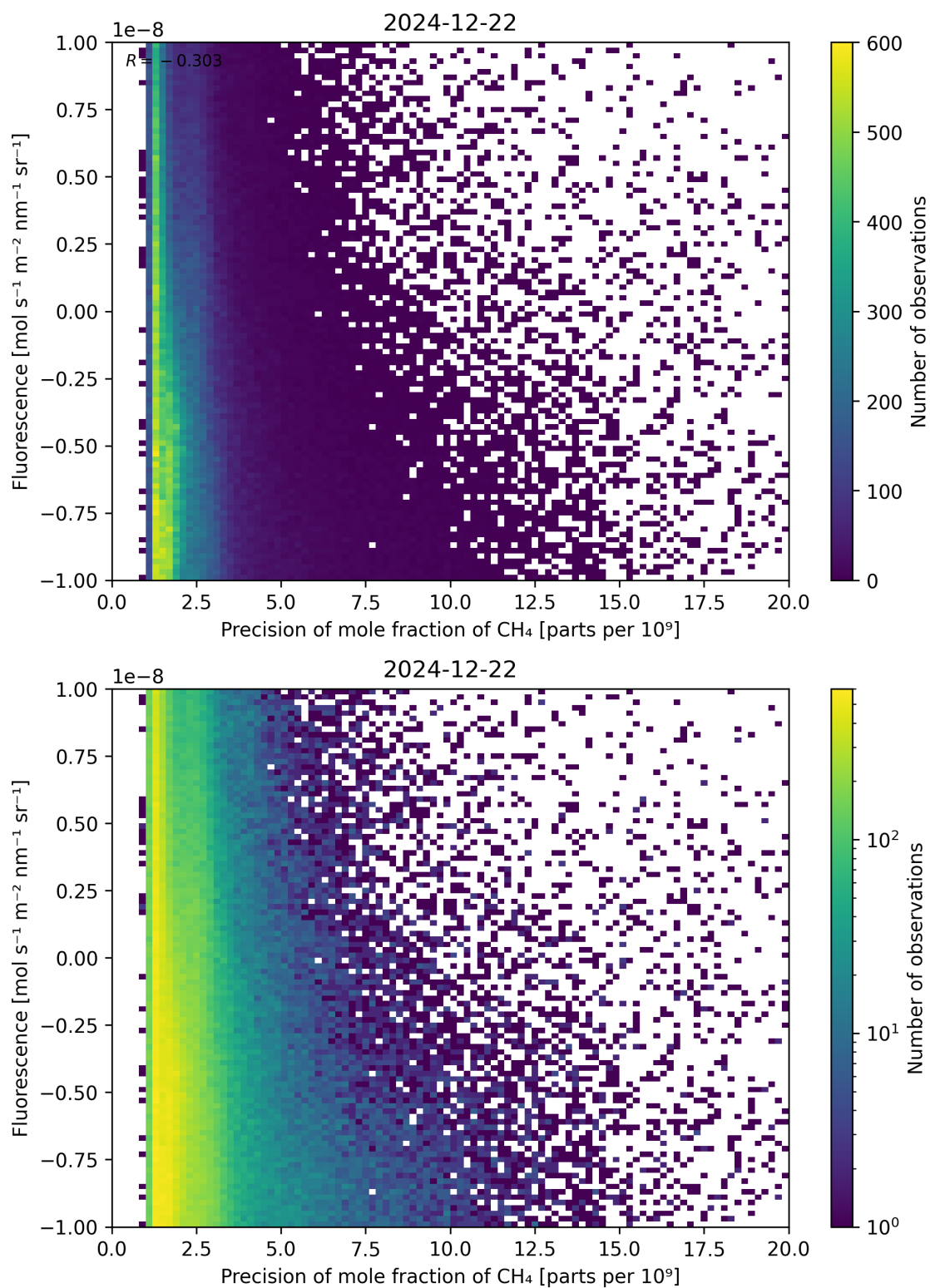
Figure 81: Scatter density plot of “Precision of mole fraction of CH 4 ” against “Fluorescence” for 2024-12-22 to 2024-12-23.
