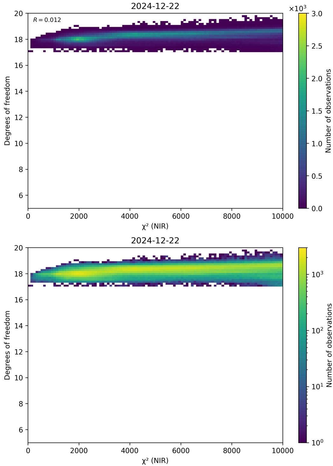
Figure 44: Scatter density plot of “ \chi^2 (NIR)” against “Degrees of freedom” for 2024-12-22 to 2024-12-23.
