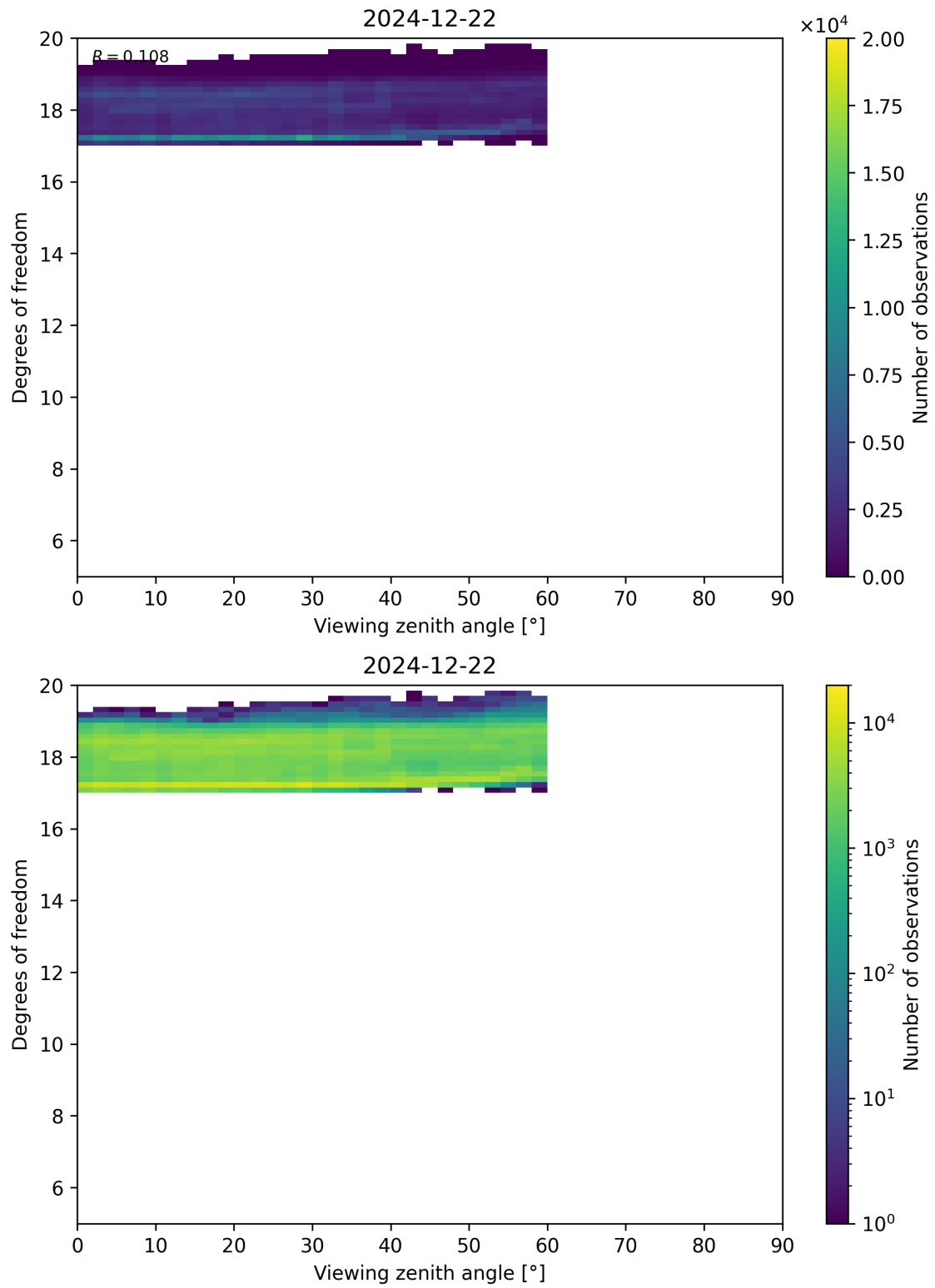
Figure 107: Scatter density plot of “Viewing zenith angle” against “Degrees of freedom” for 2024-12-22 to 2024-12-23.
