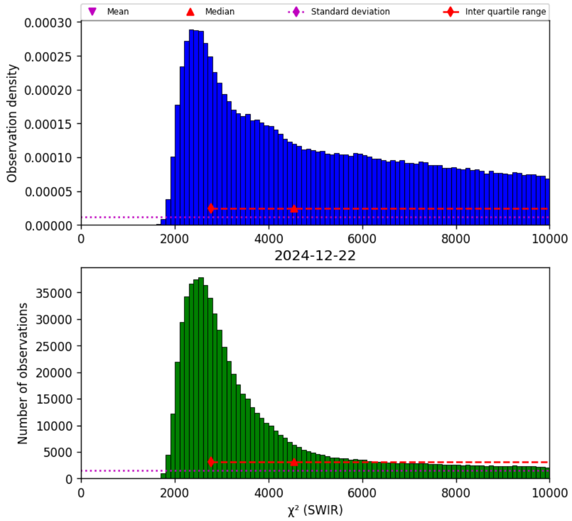
Figure 28: Histogram of “ \chi^2 (SWIR)” for 2024-12-22 to 2024-12-23
