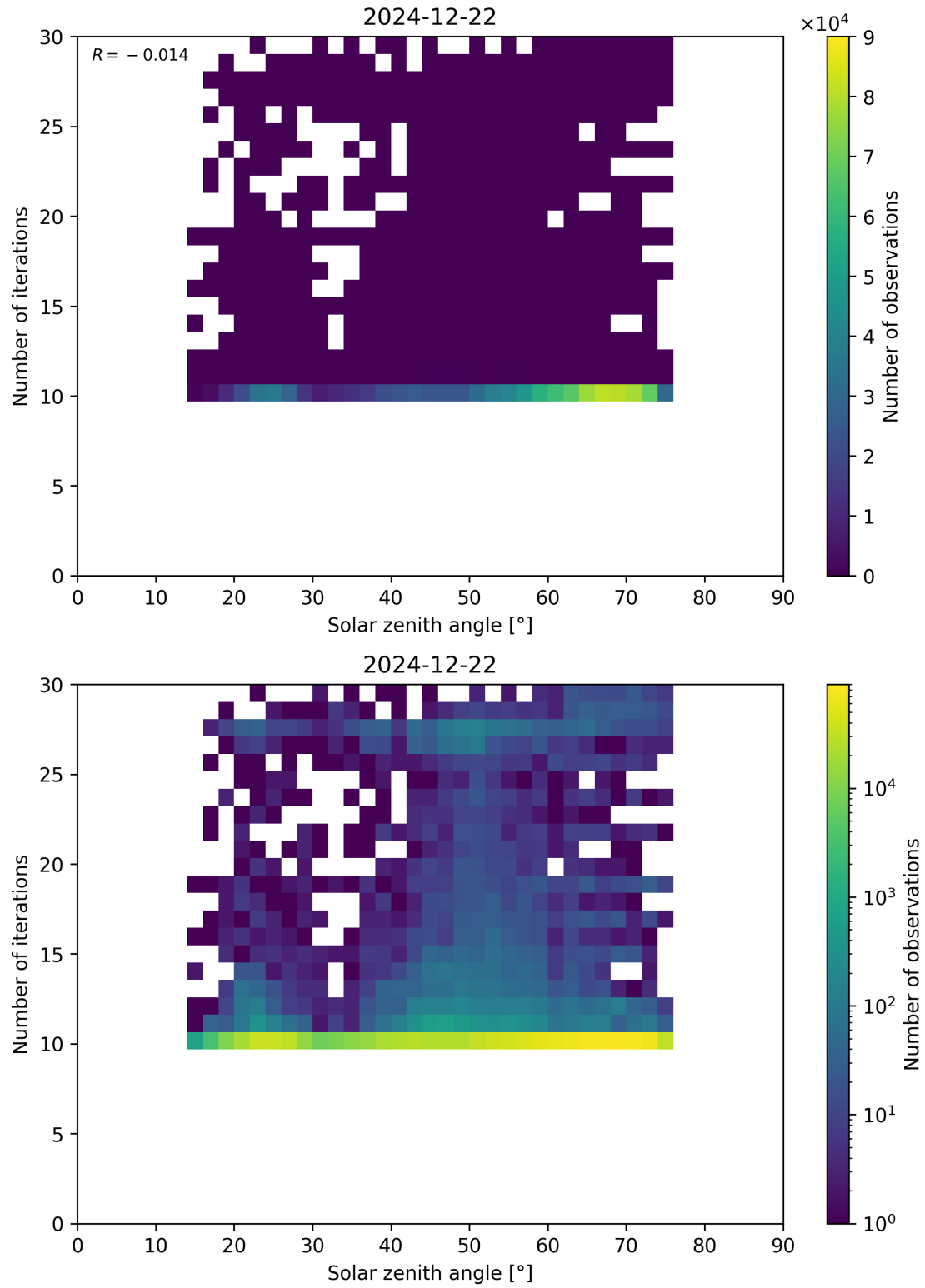
Figure 102: Scatter density plot of “Solar zenith angle” against “Number of iterations” for 2024-12-22 to 2024-12-23.
