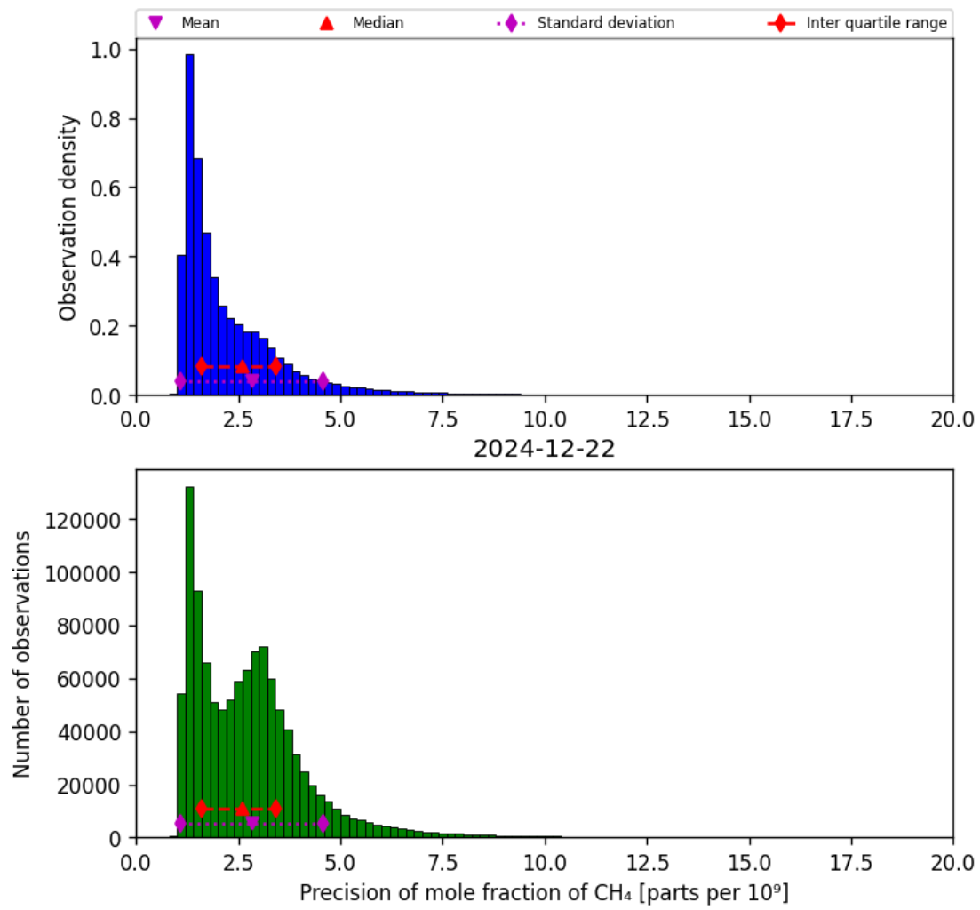
Figure 24: Histogram of “Precision of mole fraction of CH 4 ” for 2024-12-22 to 2024-12-23
