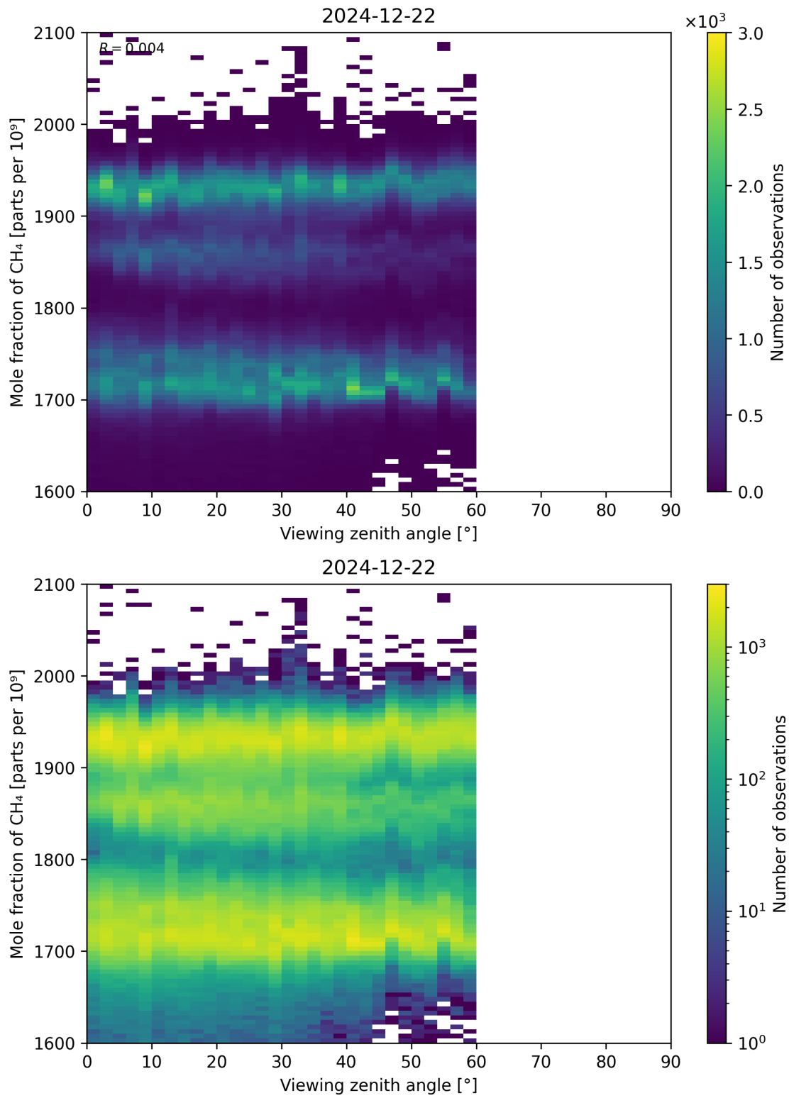
Figure 110: Scatter density plot of “Viewing zenith angle” against “Mole fraction of CH 4 ” for 2024-12-22 to 2024-12-23.
