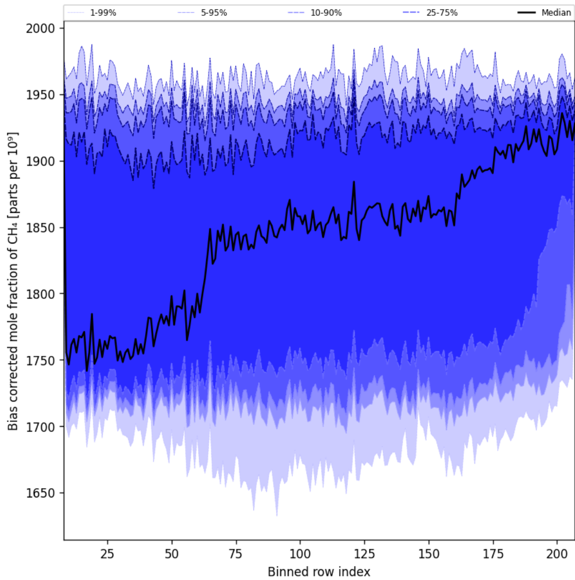
Figure 36: Along track statistics of “Bias corrected mole fraction of CH 4 ” for 2024-12-22 to 2024-12-23
