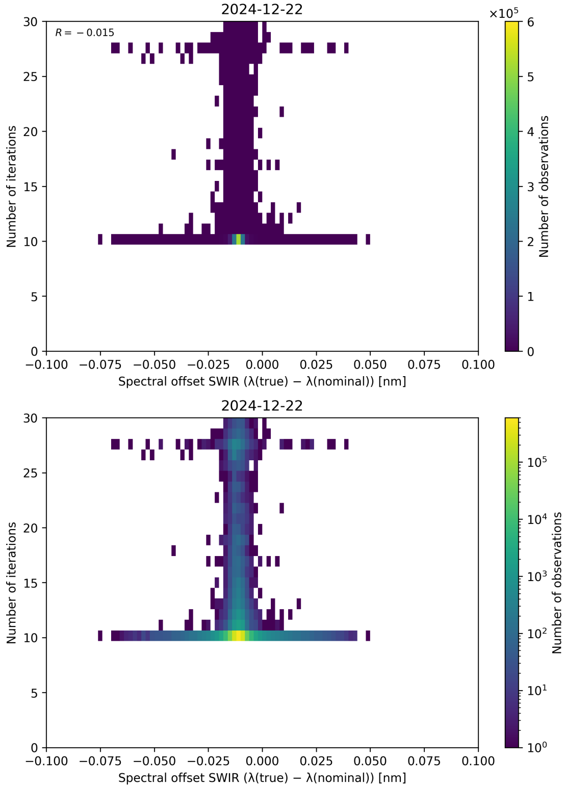
Figure 121: Scatter density plot of “Spectral offset SWIR ( \lambda_{\text{true}} - \lambda_{\text{nominal}} )” against “Number of iterations” for 2024-12-22 to 2024-12-23.
