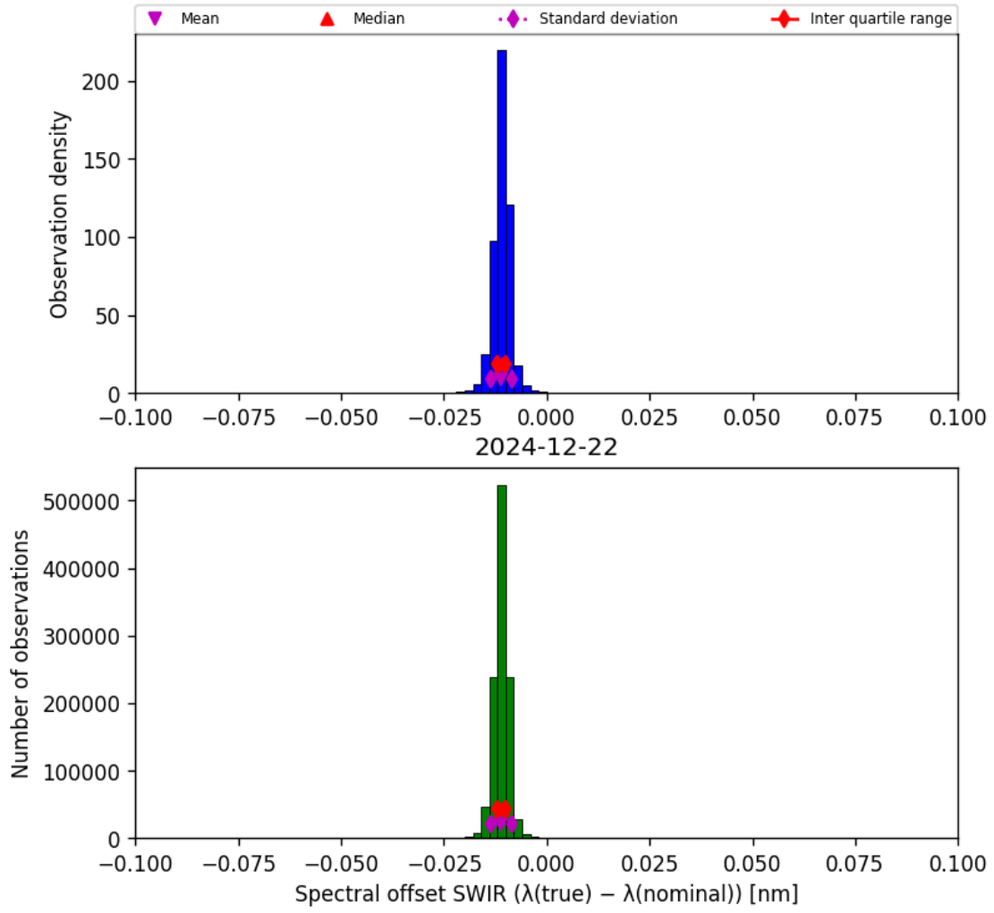
Figure 27: Histogram of “Spectral offset SWIR ( \lambda_{\text{true}} - \lambda_{\text{nominal}} )” for 2024-12-22 to 2024-12-23
