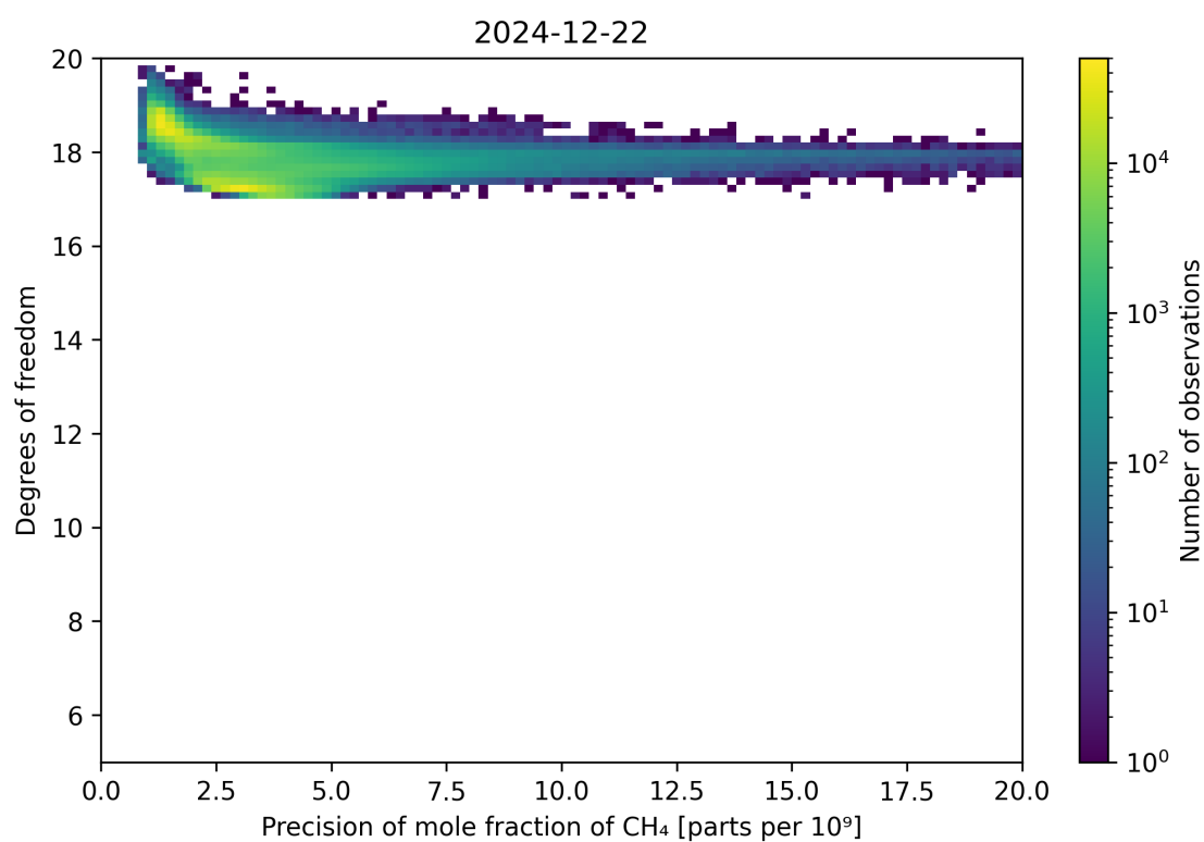
Figure 80: Scatter density plot of “Precision of mole fraction of CH 4 ” against “Degrees of freedom” for 2024-12-22 to 2024-12-23.
