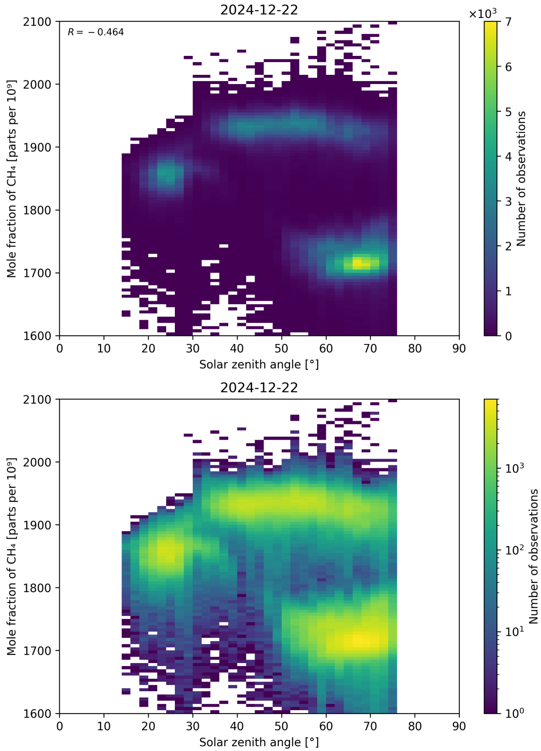
Figure 99: Scatter density plot of “Solar zenith angle” against “Mole fraction of \text{CH}_4 ” for 2024-12-22 to 2024-12-23.
