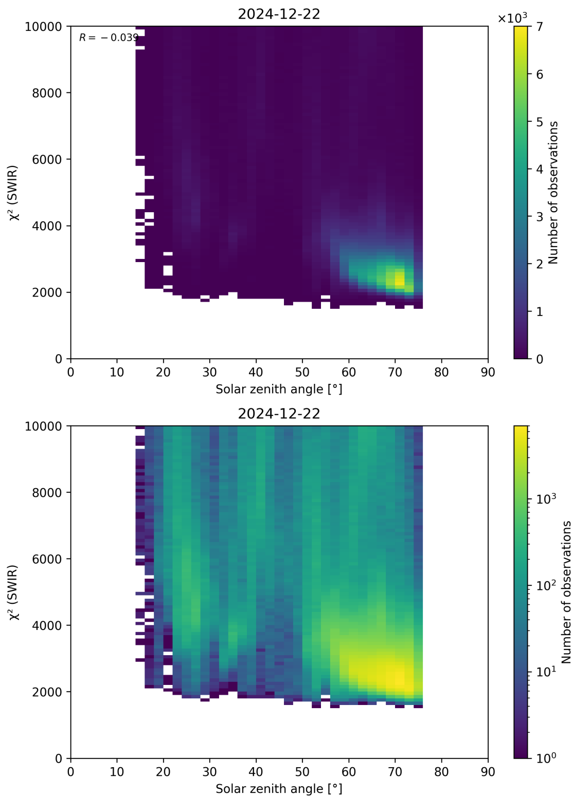
Figure 95: Scatter density plot of “Solar zenith angle” against “ \chi^2 (SWIR)” for 2024-12-22 to 2024-12-23.
