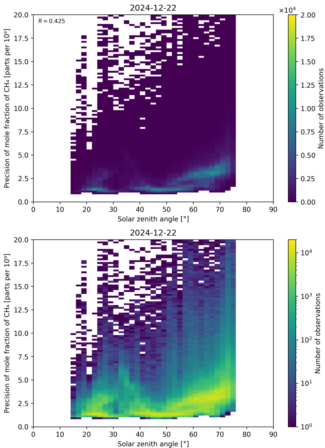
Figure 101: Scatter density plot of “Solar zenith angle” against “Precision of mole fraction of \text{CH}_4 ” for 2024-12-22 to 2024-12-23.
