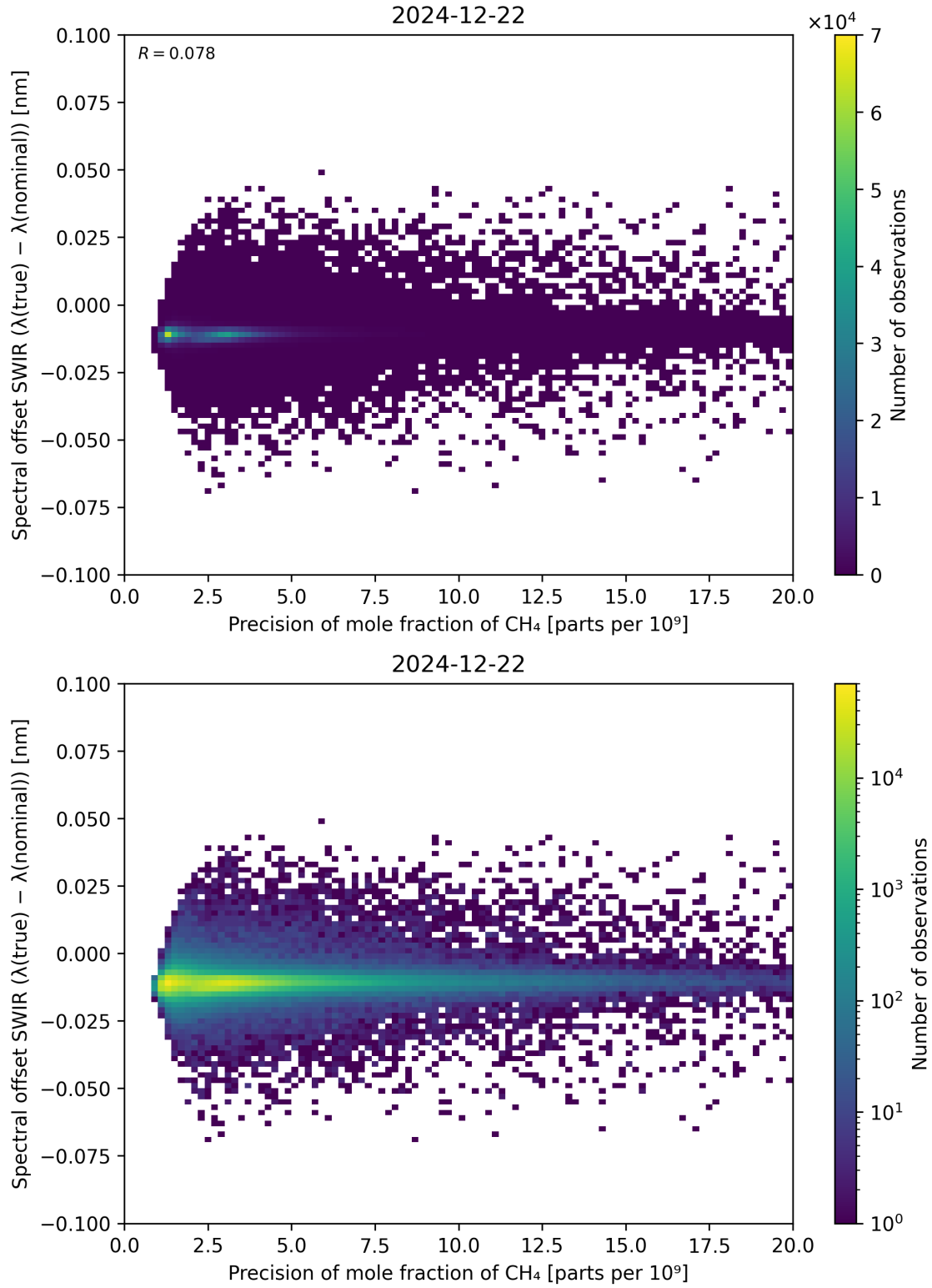
Figure 85: Scatter density plot of “Precision of mole fraction of \text{CH}_4 ” against “Spectral offset SWIR ( \lambda_{\text{true}} - \lambda_{\text{nominal}} )” for 2024-12-22 to 2024-12-23.
