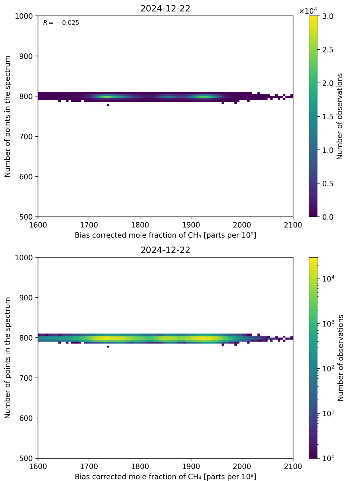
Figure 68: Scatter density plot of “Bias corrected mole fraction of CH 4 ” against “Number of points in the spectrum” for 2024-12-22 to 2024-12-23.
