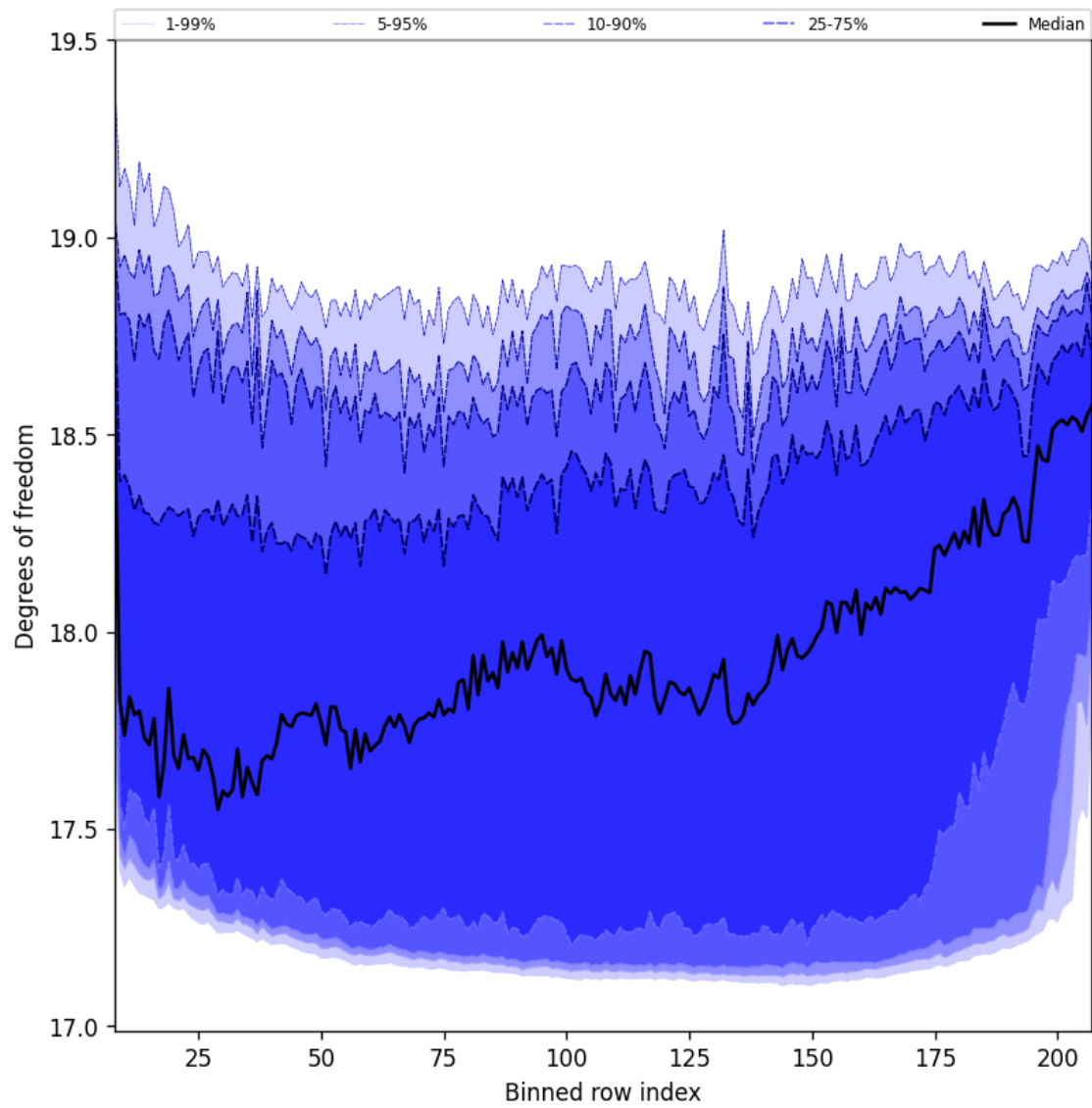
Figure 41: Along track statistics of “Degrees of freedom” for 2024-12-22 to 2024-12-23
