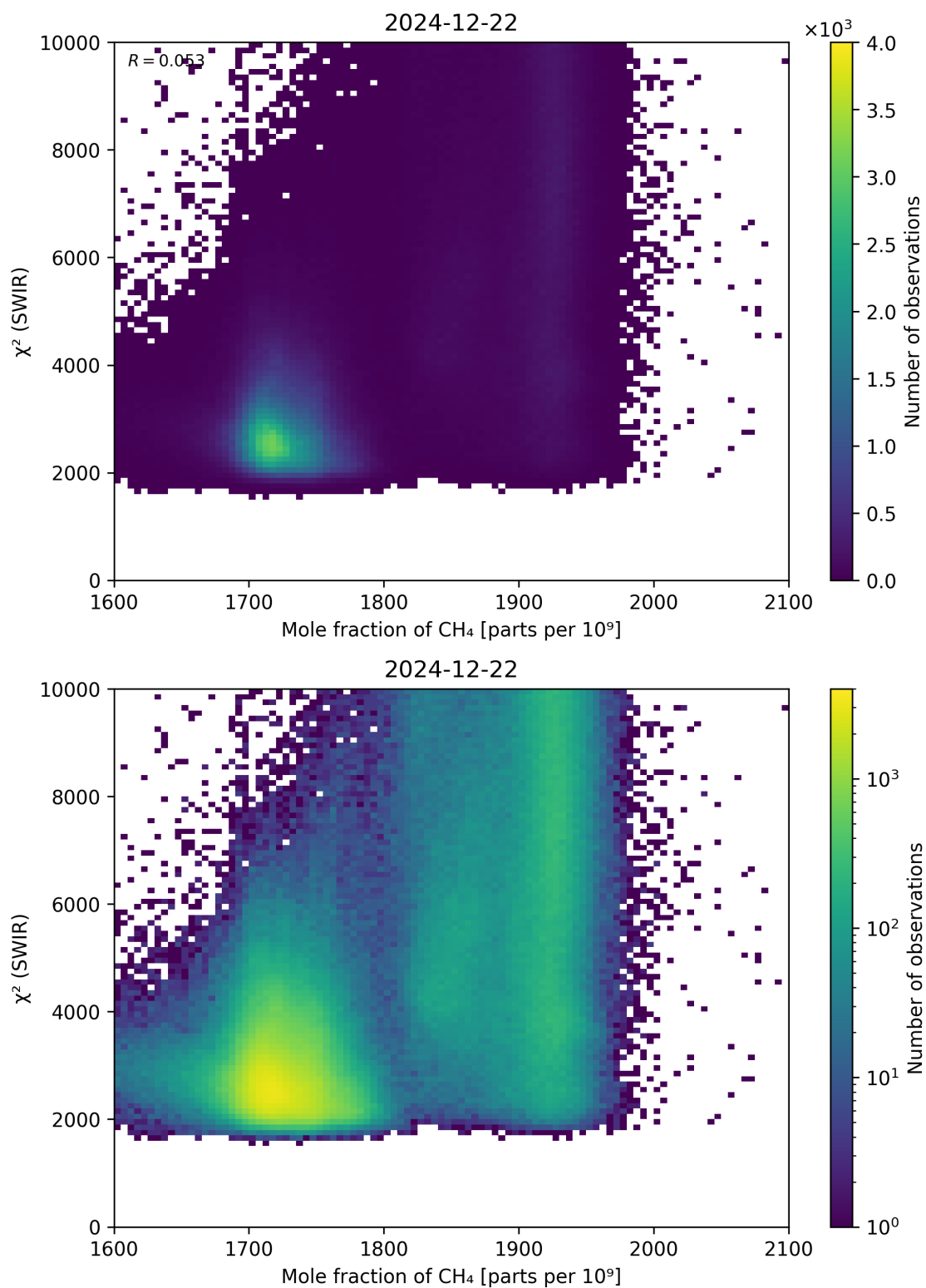
Figure 71: Scatter density plot of “Mole fraction of \text{CH}_4 ” against “ \chi^2 (SWIR)” for 2024-12-22 to 2024-12-23.
