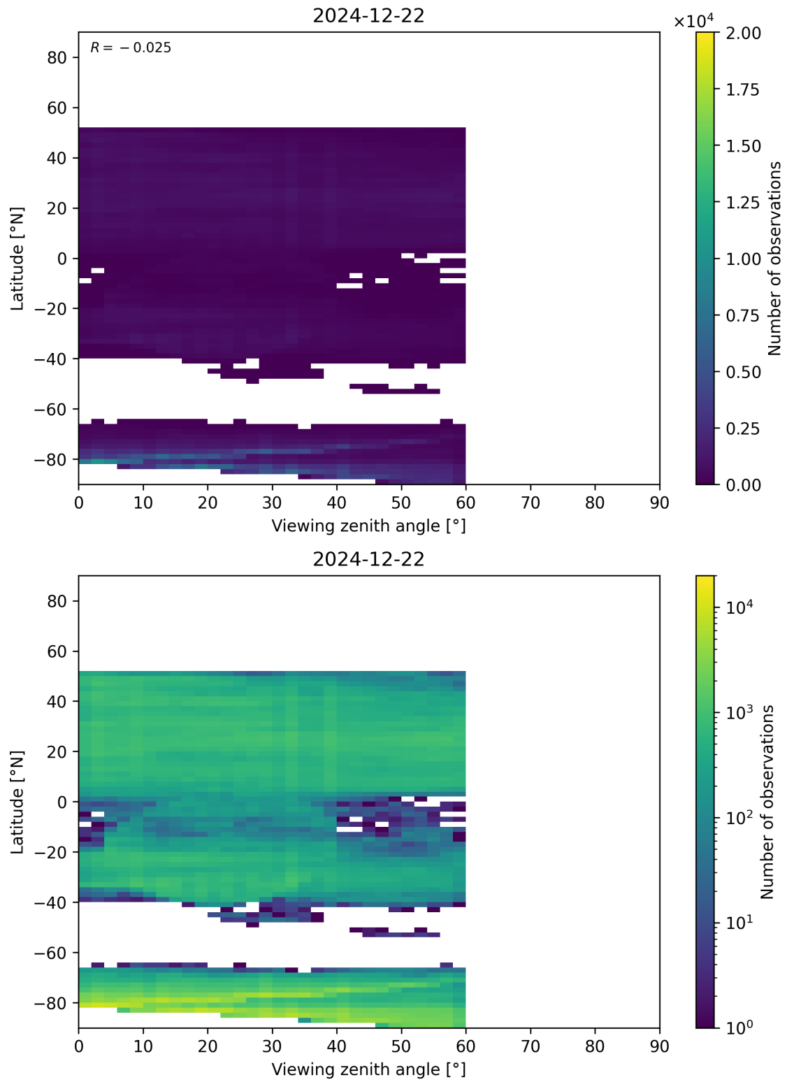
Figure 109: Scatter density plot of “Viewing zenith angle” against “Latitude” for 2024-12-22 to 2024-12-23.
