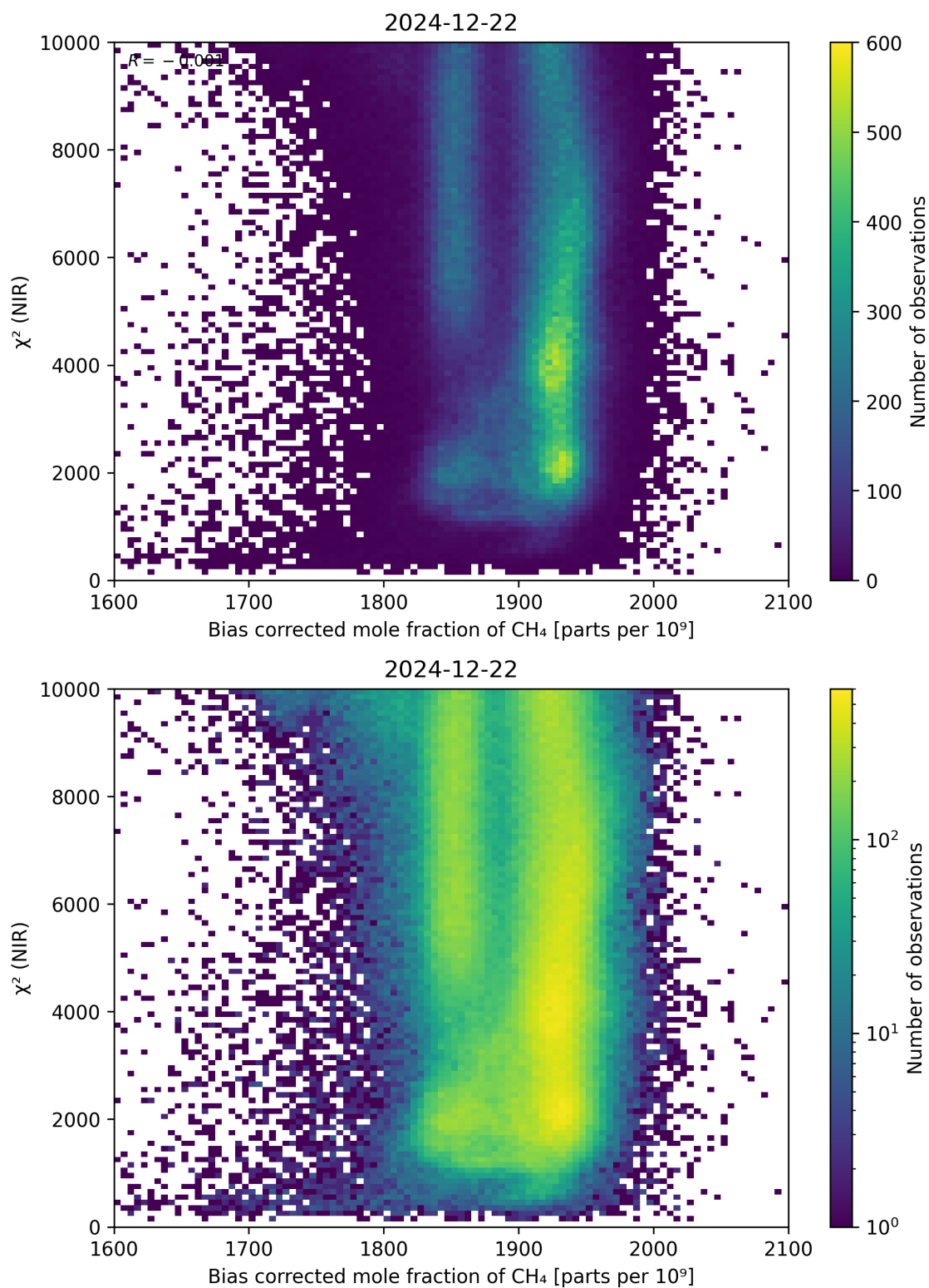
Figure 63: Scatter density plot of “Bias corrected mole fraction of \text{CH}_4 ” against “ \chi^2 (NIR)” for 2024-12-22 to 2024-12-23.
