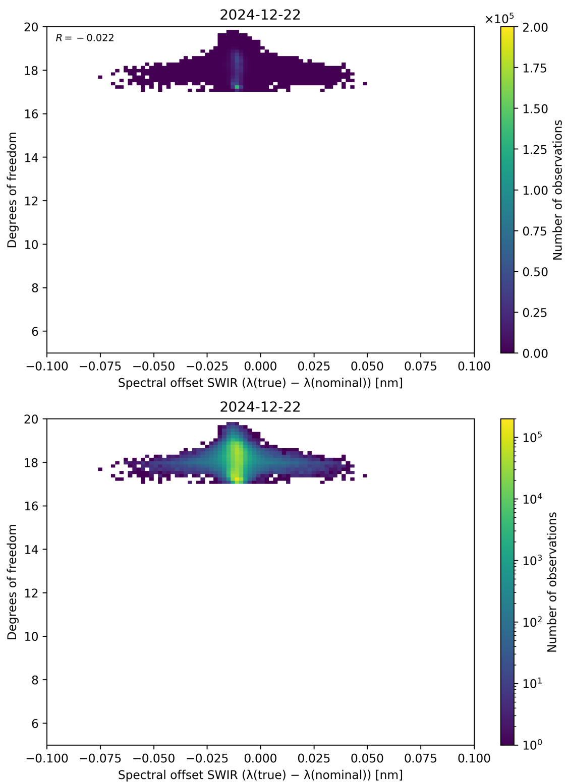
Figure 119: Scatter density plot of “Spectral offset SWIR ( \lambda_{\text{true}} - \lambda_{\text{nominal}} )” against “Degrees of freedom” for 2024-12-22 to 2024-12-23.
