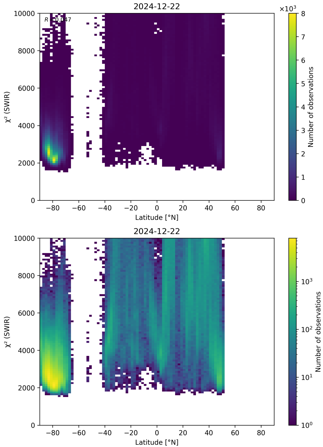
Figure 54: Scatter density plot of “Latitude” against “ \chi^2 (SWIR)” for 2024-12-22 to 2024-12-23.
