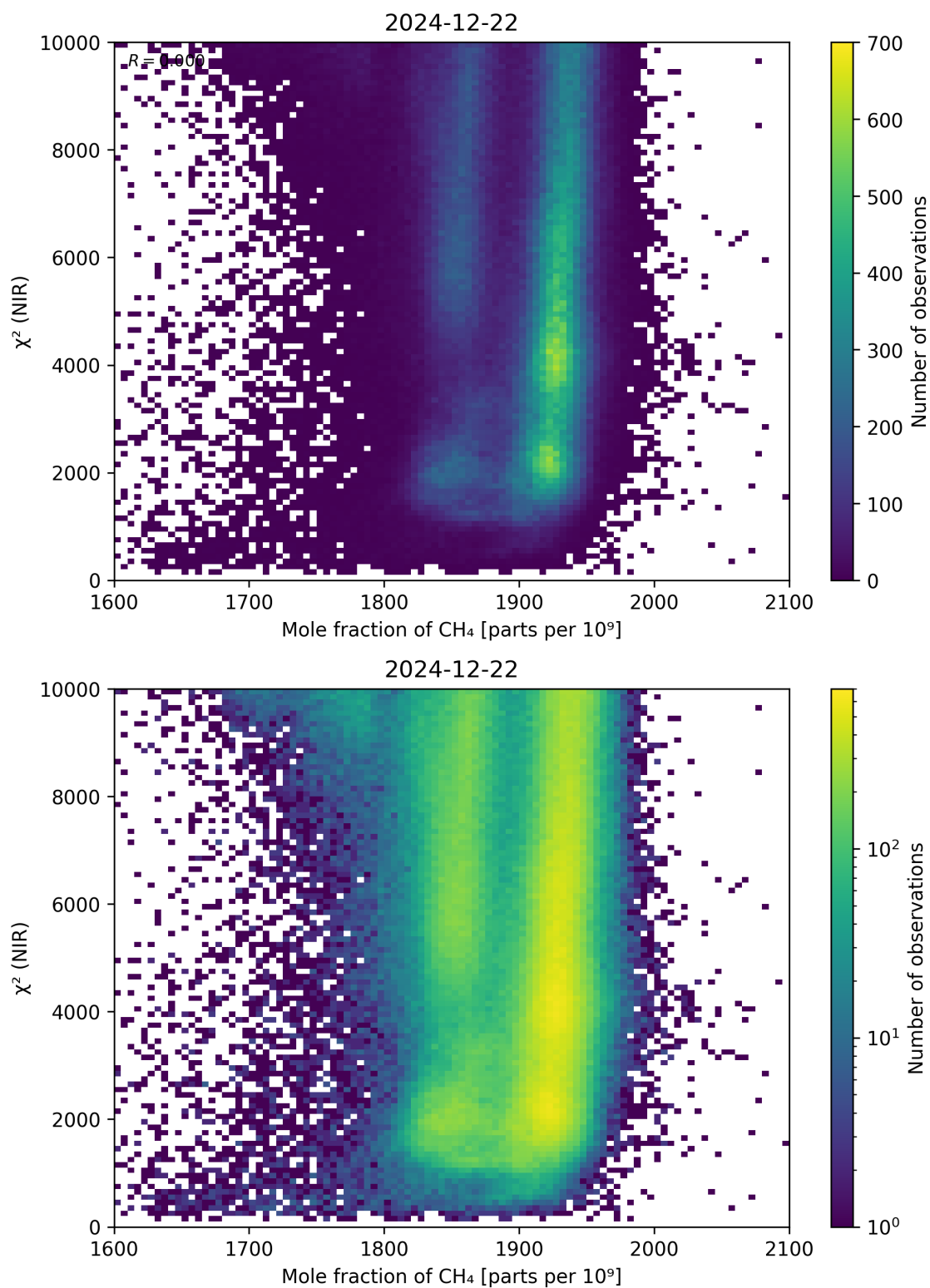
Figure 70: Scatter density plot of “Mole fraction of \text{CH}_4 ” against “ \chi^2 (NIR)” for 2024-12-22 to 2024-12-23.
