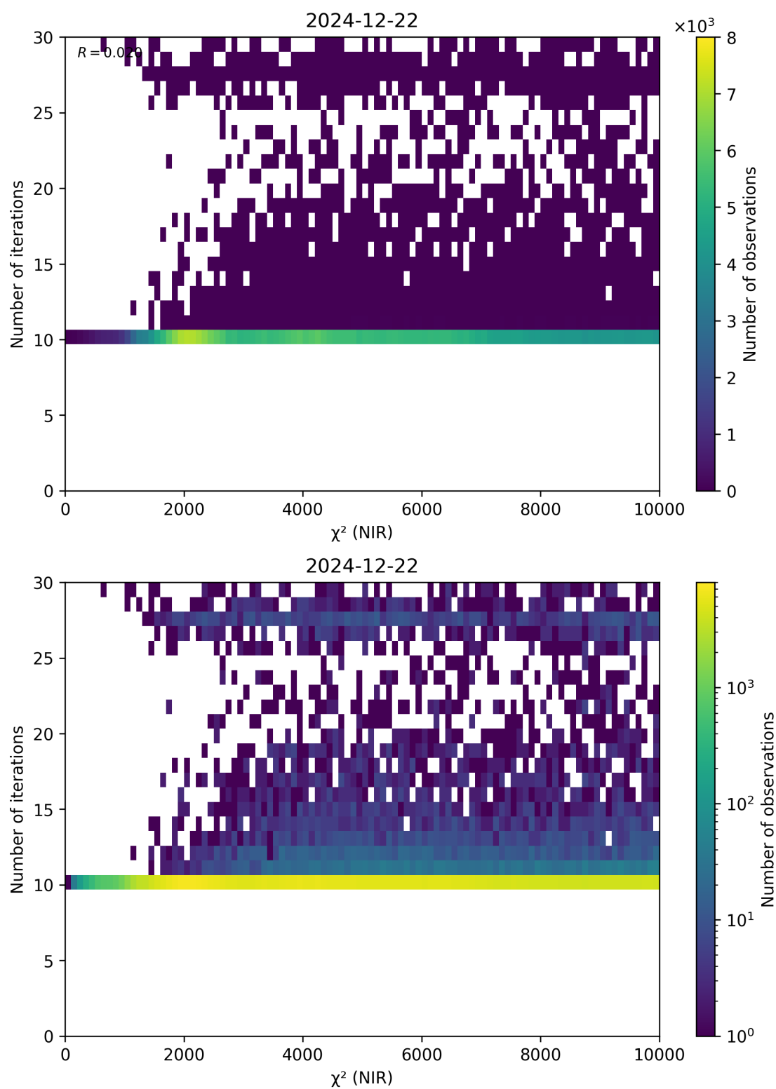
Figure 46: Scatter density plot of “ \chi^2 (NIR)” against “Number of iterations” for 2024-12-22 to 2024-12-23.
