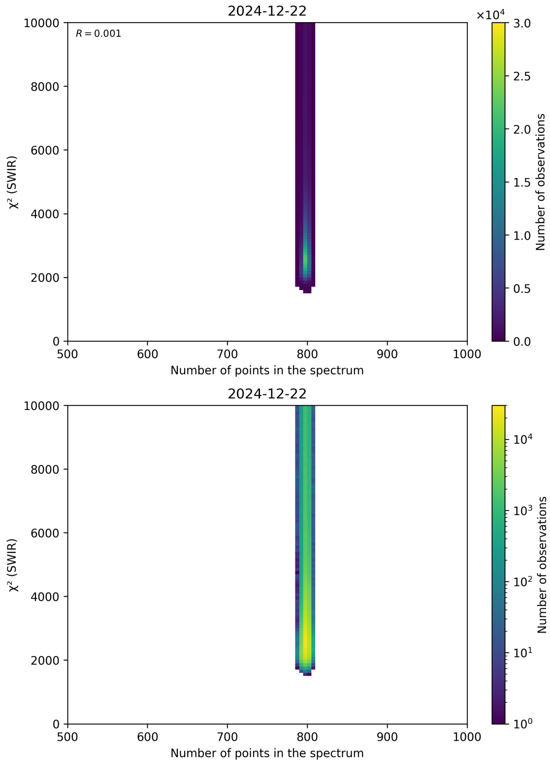
Figure 89: Scatter density plot of “Number of points in the spectrum” against “ \chi^2 (SWIR)” for 2024-12-22 to 2024-12-23.
