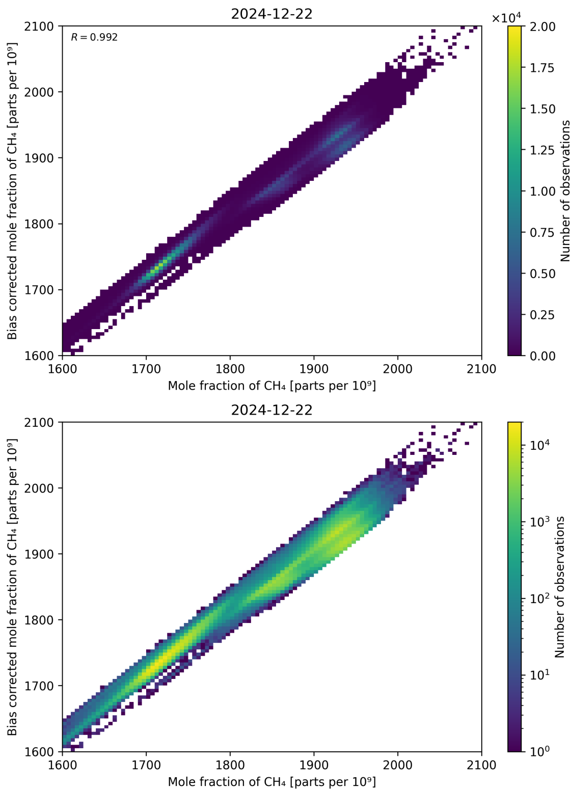
Figure 74: Scatter density plot of “Mole fraction of CH 4 ” against “Bias corrected mole fraction of CH 4 ” for 2024-12-22 to 2024-12-23.
