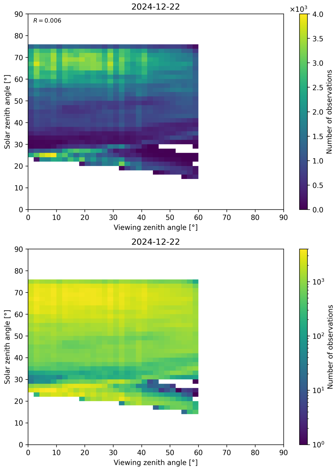
Figure 115: Scatter density plot of “Viewing zenith angle” against “Solar zenith angle” for 2024-12-22 to 2024-12-23.
