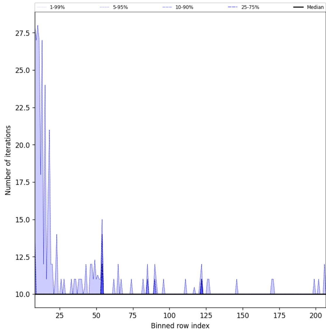
Figure 42: Along track statistics of “Number of iterations” for 2024-12-22 to 2024-12-23
