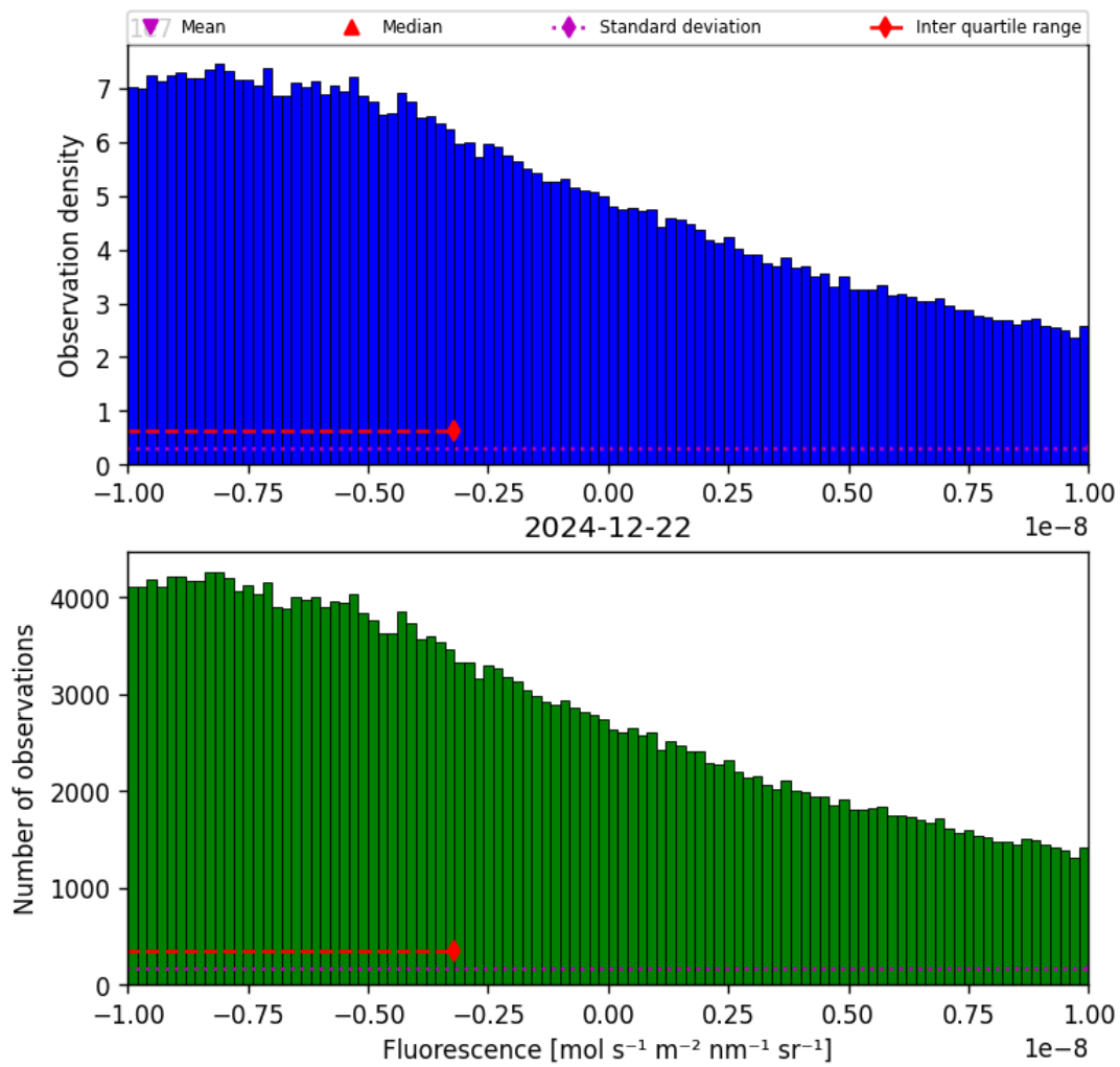
Figure 32: Histogram of “Fluorescence” for 2024-12-22 to 2024-12-23
