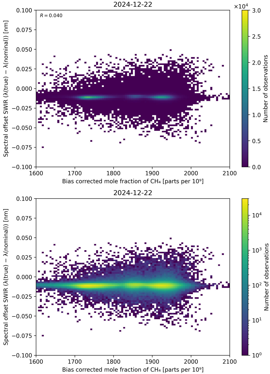
Figure 69: Scatter density plot of “Bias corrected mole fraction of \text{CH}_4 ” against “Spectral offset SWIR ( \lambda_{\text{true}} - \lambda_{\text{nominal}} )” for 2024-12-22 to 2024-12-23.
