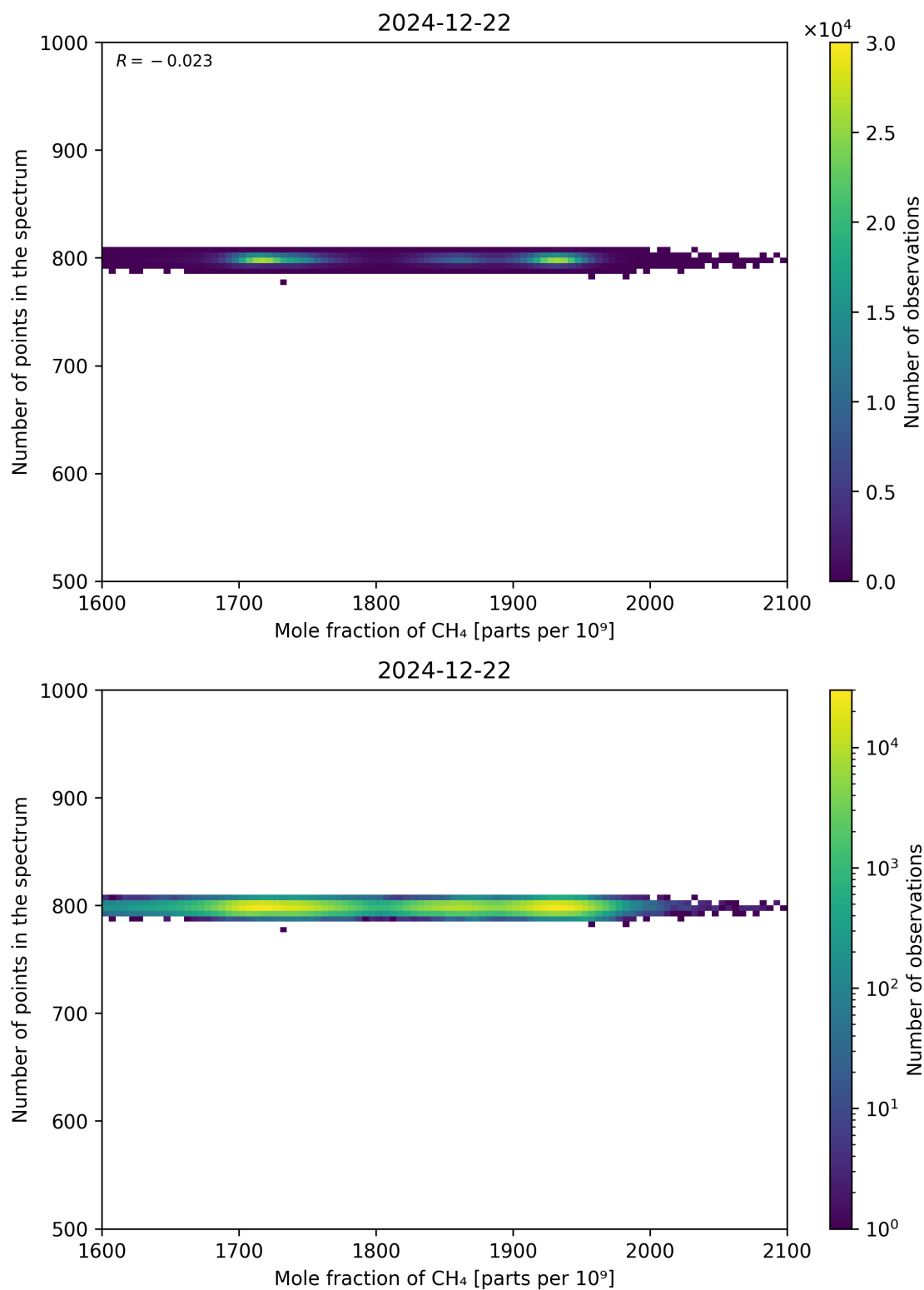
Figure 77: Scatter density plot of “Mole fraction of CH 4 ” against “Number of points in the spectrum” for 2024-12-22 to 2024-12-23.
