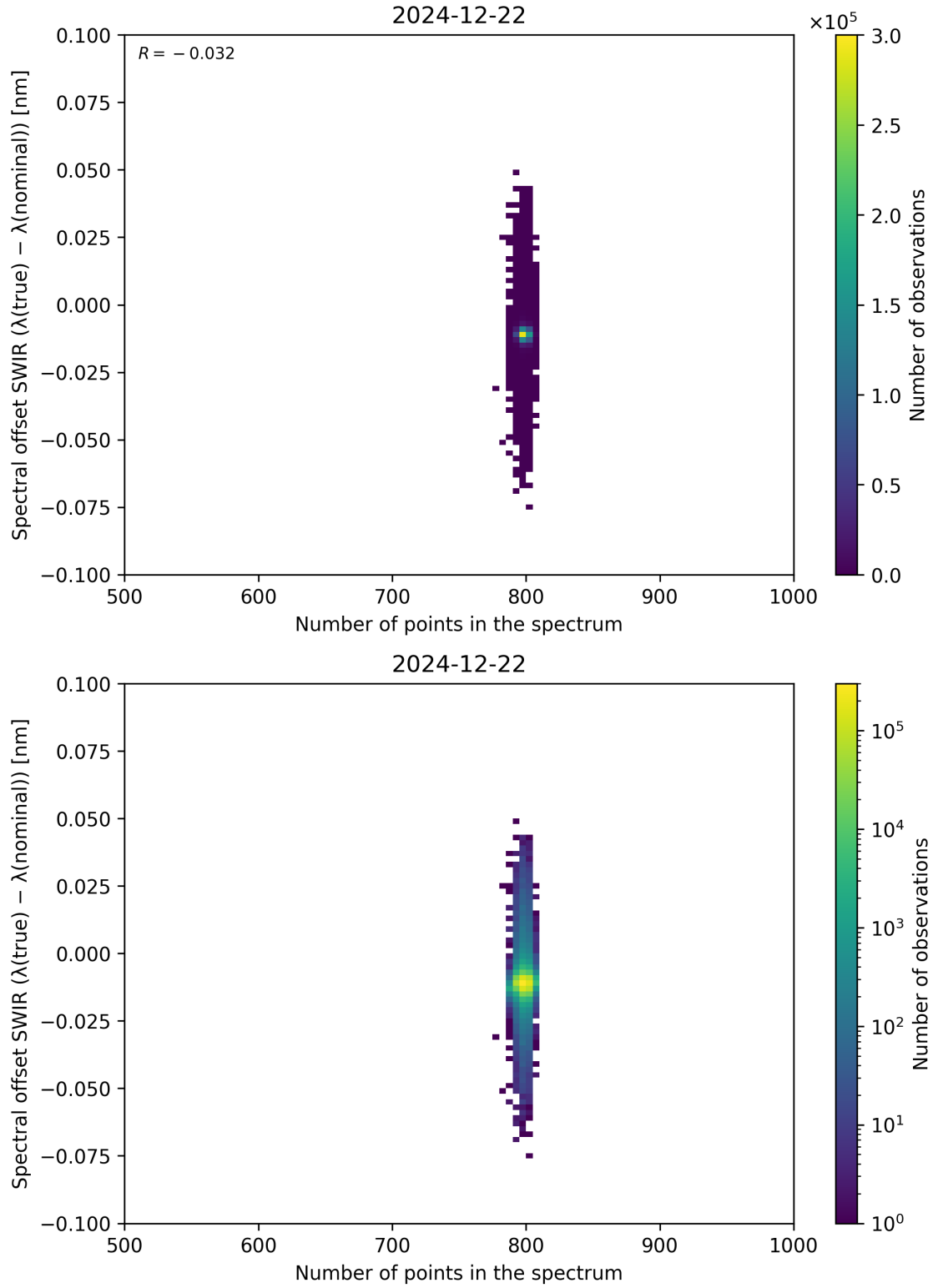
Figure 93: Scatter density plot of “Number of points in the spectrum” against “Spectral offset SWIR ( \lambda_{\text{true}} - \lambda_{\text{nominal}} )” for 2024-12-22 to 2024-12-23.
