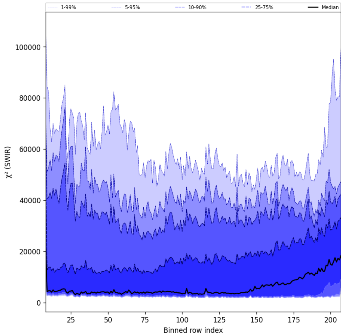
Figure 39: Along track statistics of “ \chi^2 (SWIR)” for 2024-12-22 to 2024-12-23
