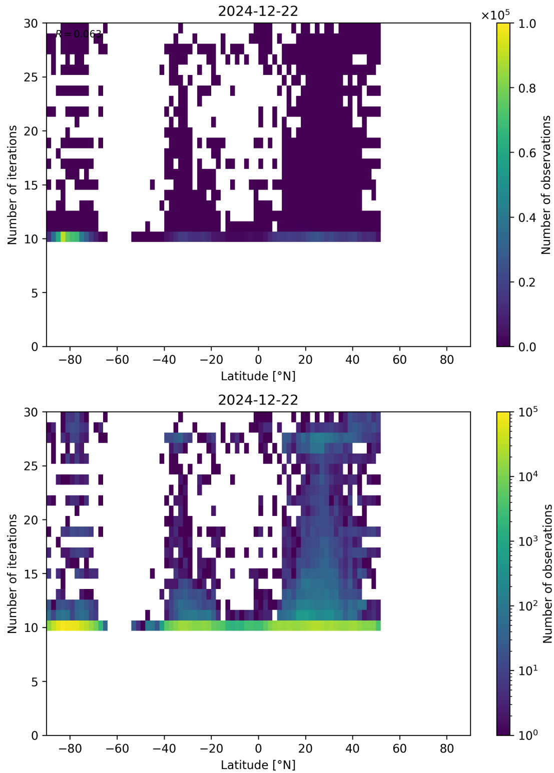
Figure 60: Scatter density plot of “Latitude” against “Number of iterations” for 2024-12-22 to 2024-12-23.
