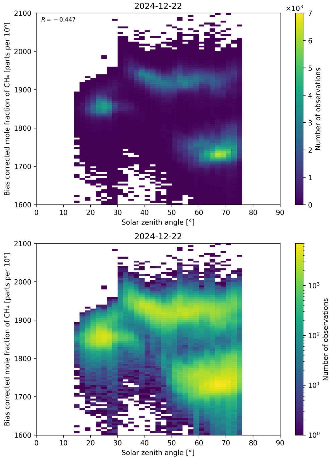
Figure 100: Scatter density plot of “Solar zenith angle” against “Bias corrected mole fraction of CH 4 ” for 2024-12-22 to 2024-12-23.
