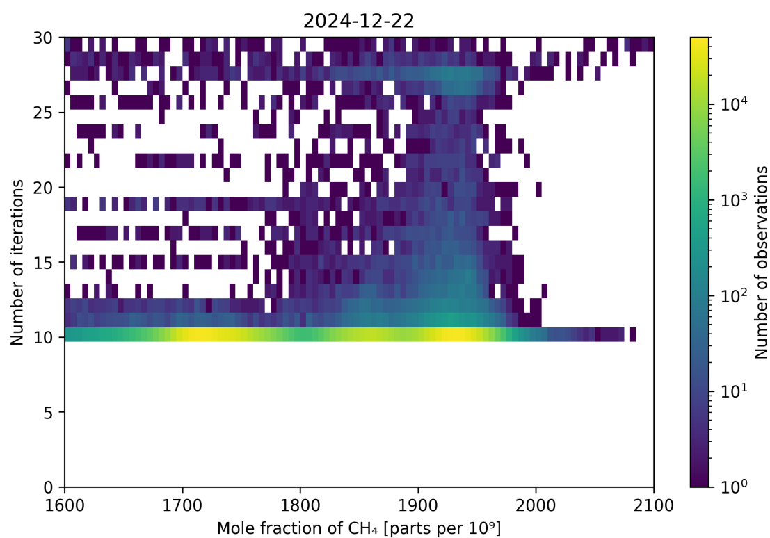
Figure 76: Scatter density plot of “Mole fraction of CH 4 ” against “Number of iterations” for 2024-12-22 to 2024-12-23.
