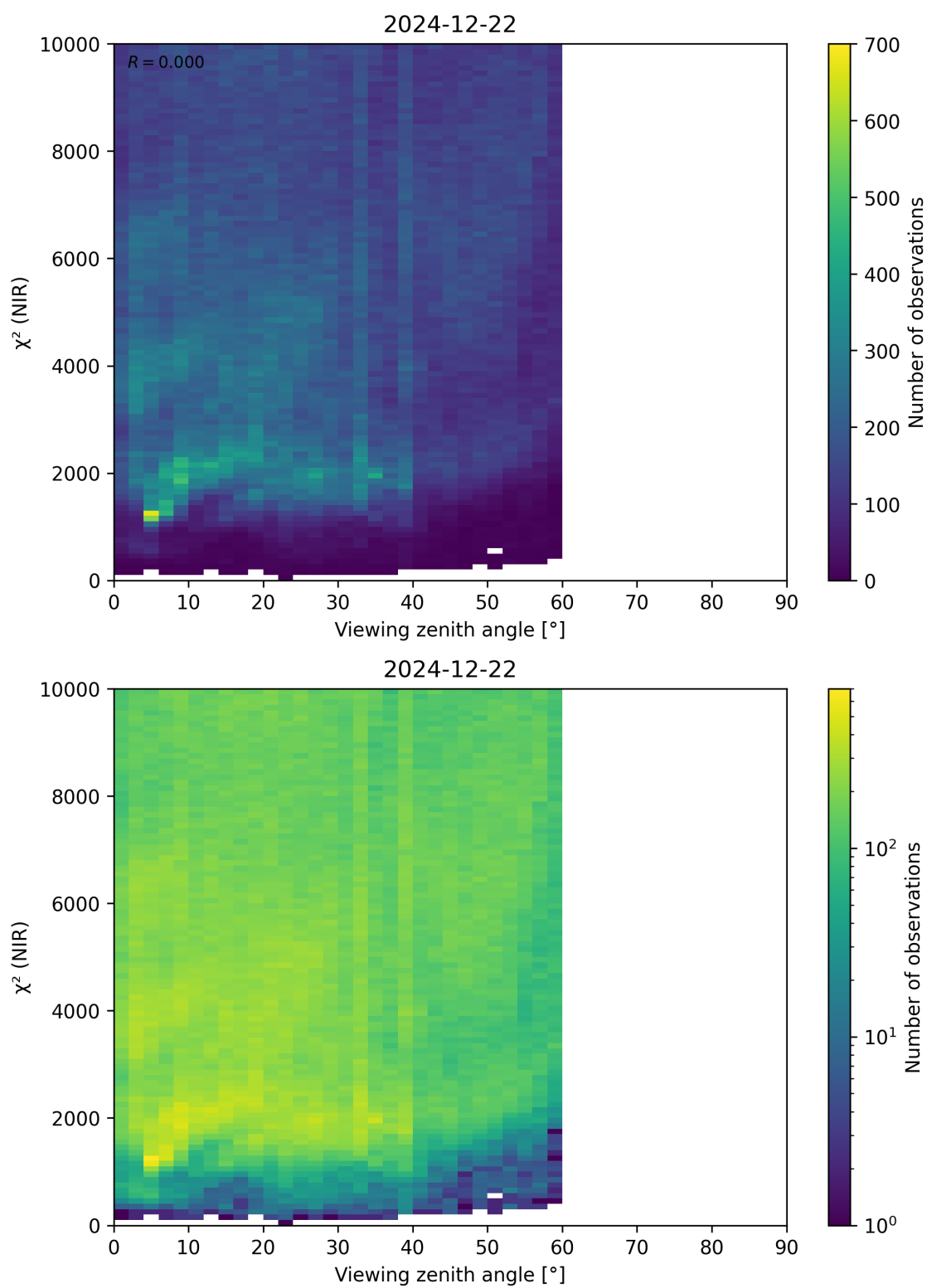
Figure 105: Scatter density plot of “Viewing zenith angle” against “ \chi^2 (NIR)” for 2024-12-22 to 2024-12-23.
