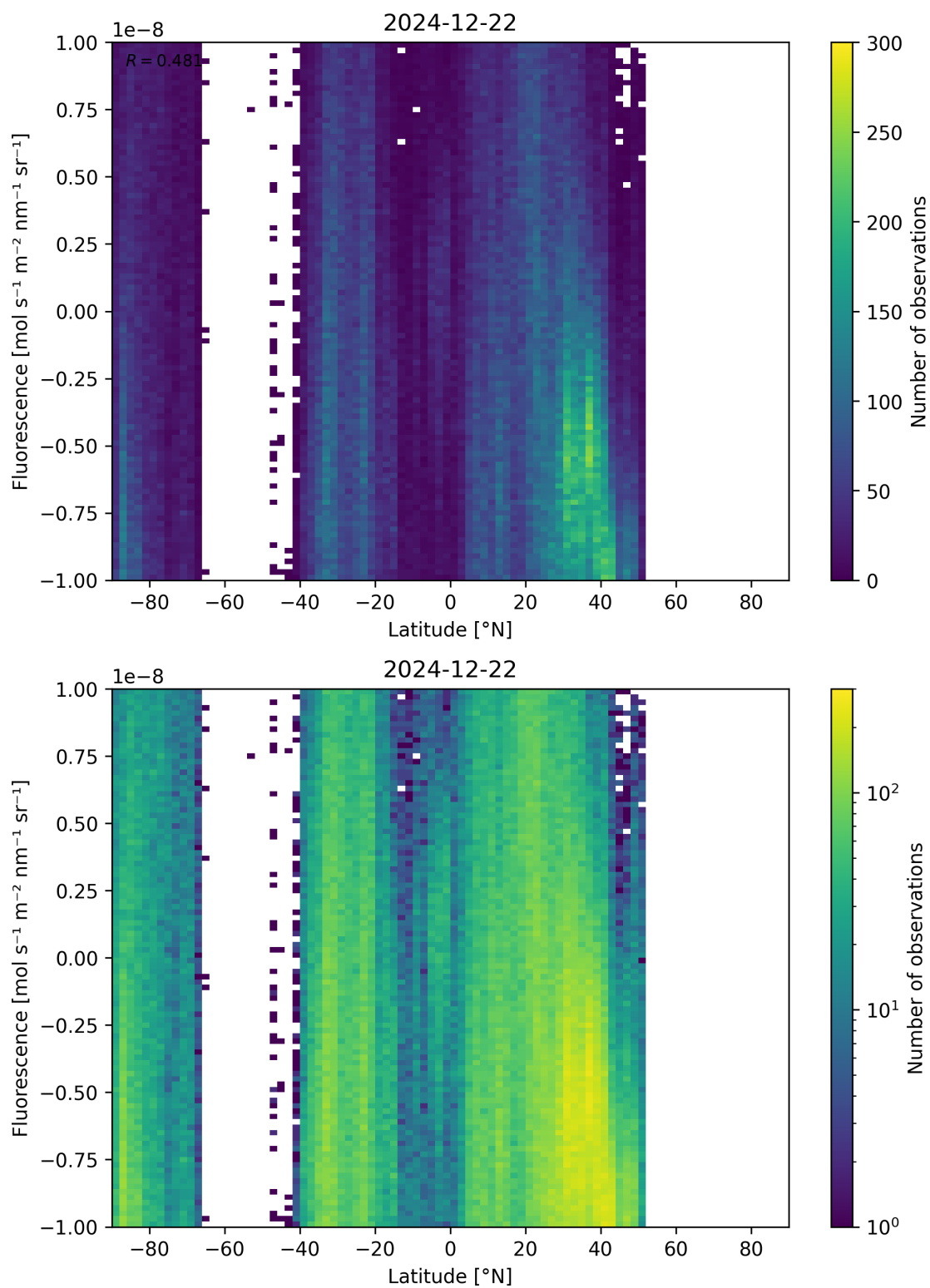
Figure 56: Scatter density plot of “Latitude” against “Fluorescence” for 2024-12-22 to 2024-12-23.
