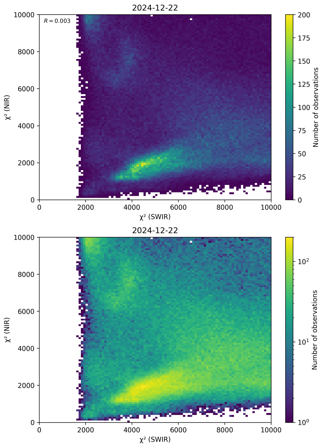
Figure 47: Scatter density plot of “ \chi^2 (SWIR)” against “ \chi^2 (NIR)” for 2024-12-22 to 2024-12-23.
