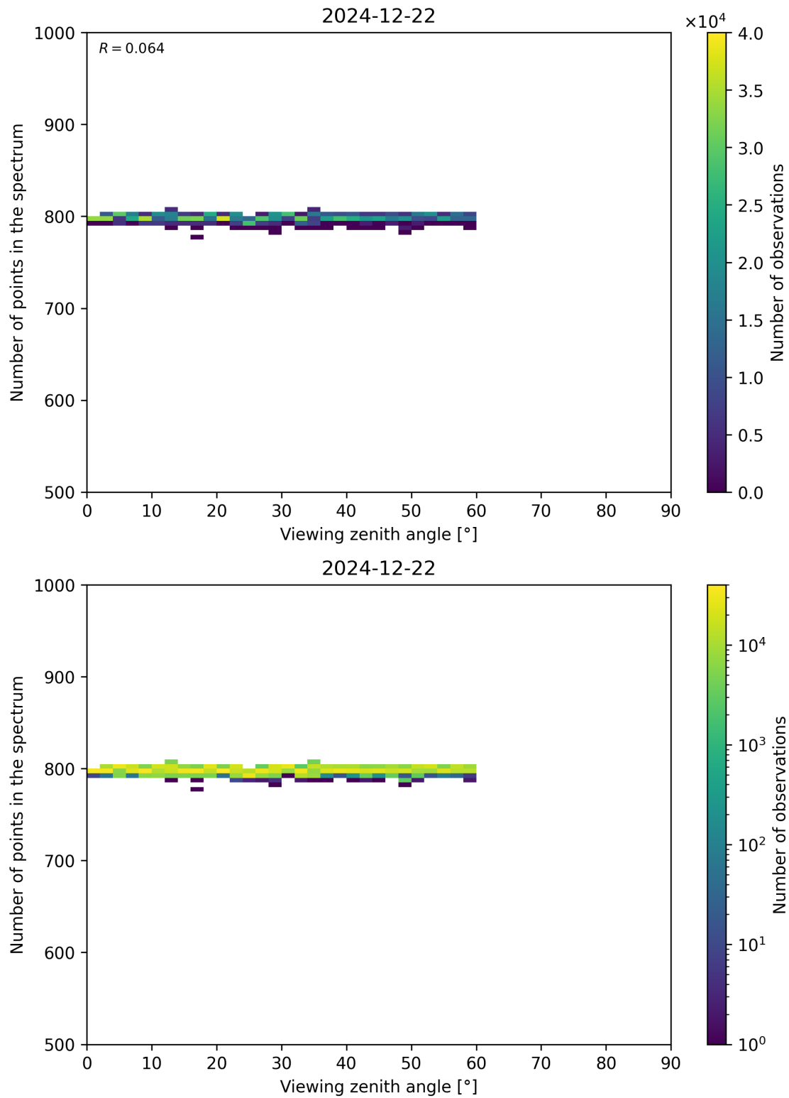
Figure 114: Scatter density plot of “Viewing zenith angle” against “Number of points in the spectrum” for 2024-12-22 to 2024-12-23.
