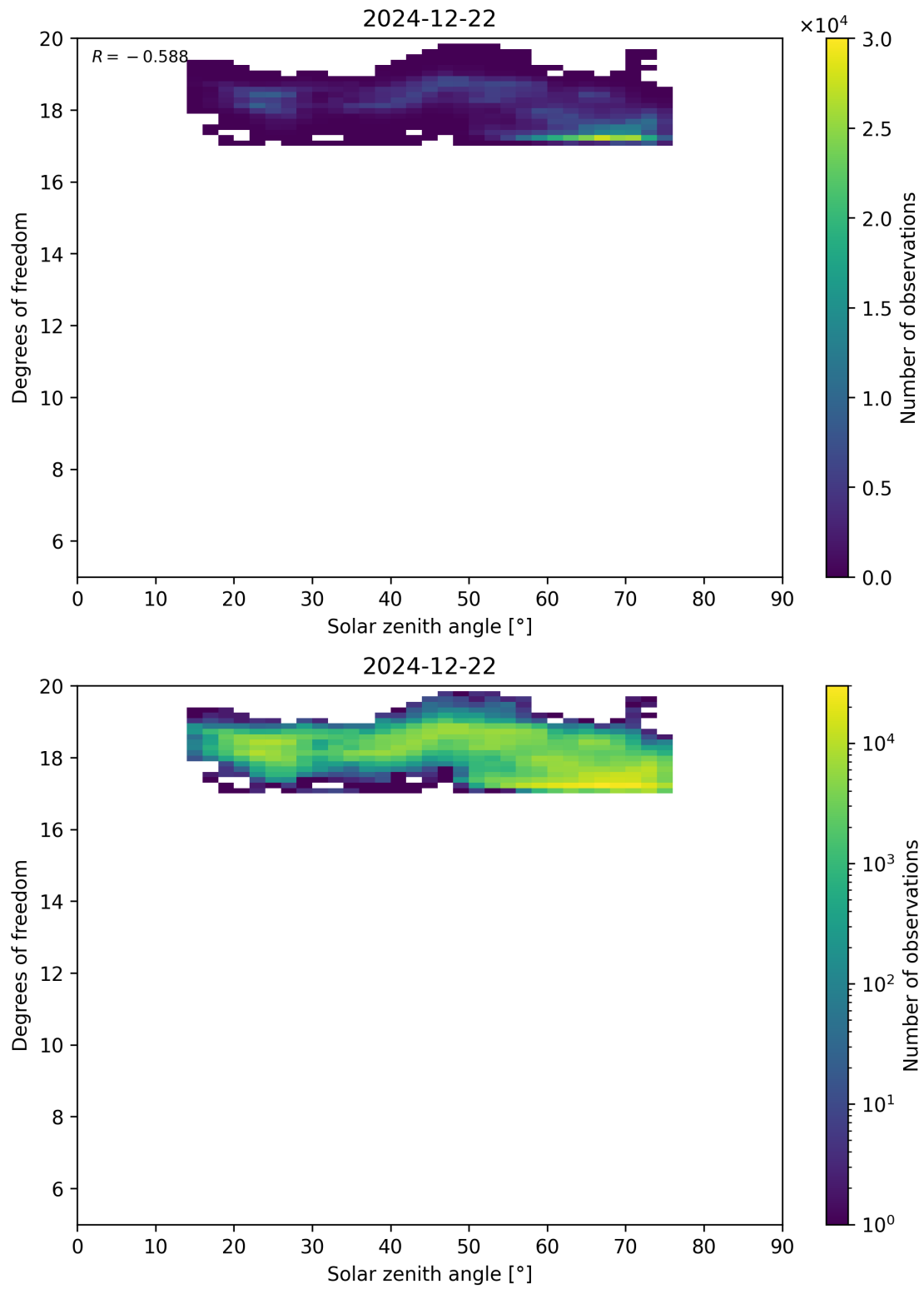
Figure 96: Scatter density plot of “Solar zenith angle” against “Degrees of freedom” for 2024-12-22 to 2024-12-23.
