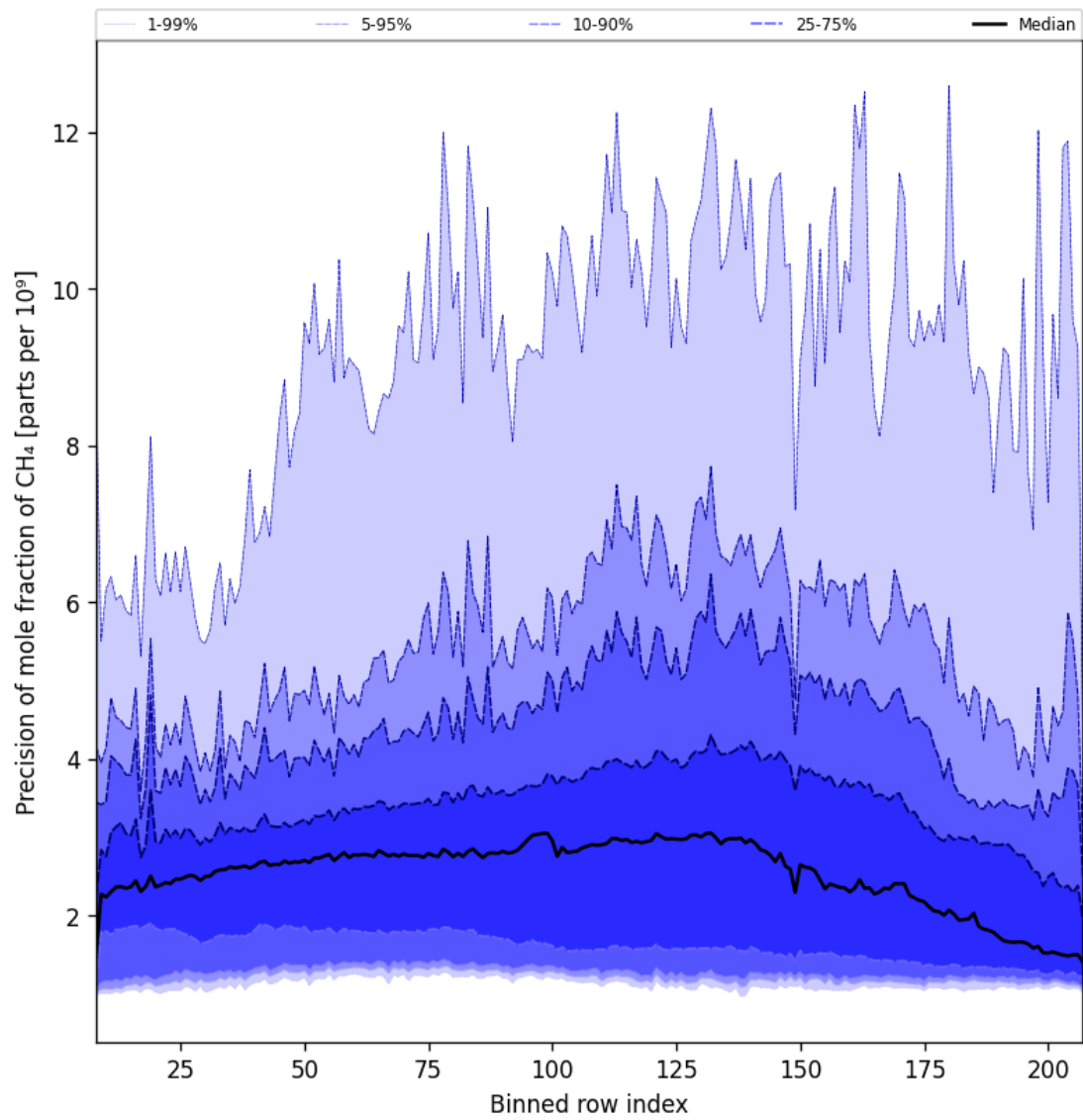
Figure 35: Along track statistics of “Precision of mole fraction of CH 4 ” for 2024-12-22 to 2024-12-23
