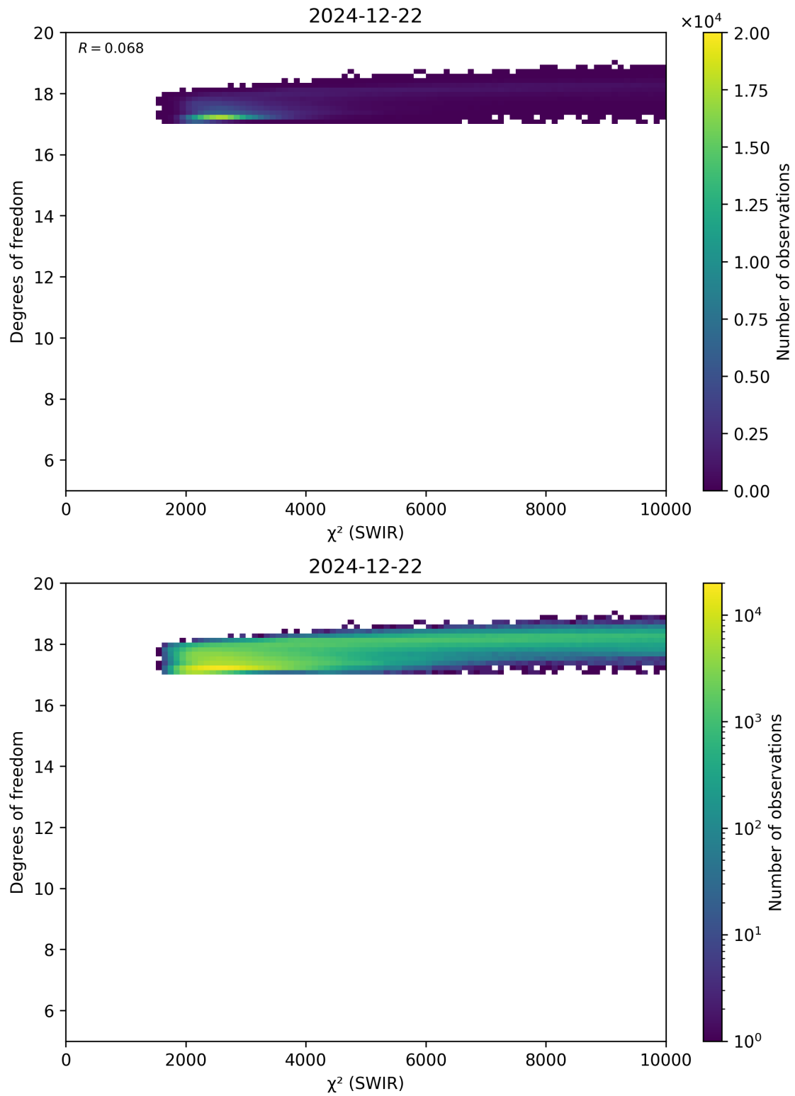
Figure 48: Scatter density plot of “ \chi^2 (SWIR)” against “Degrees of freedom” for 2024-12-22 to 2024-12-23.
