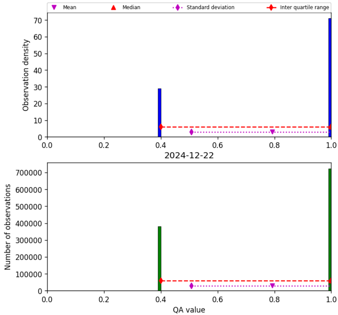
Figure 22: Histogram of “QA value” for 2024-12-22 to 2024-12-23
