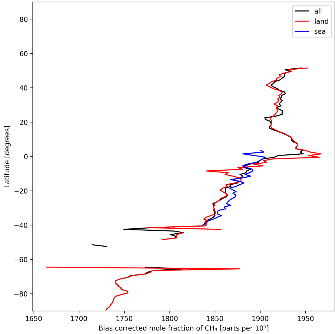
Figure 14: Zonal average of “Bias corrected mole fraction of CH 4 ” for 2024-12-22 to 2024-12-23.
