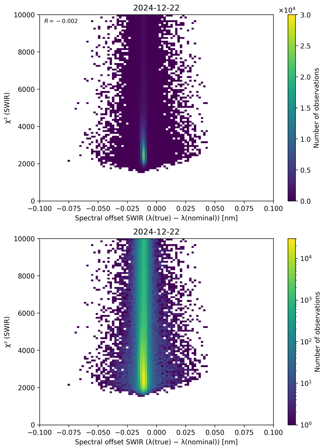
Figure 118: Scatter density plot of “Spectral offset SWIR ( \lambda_{\text{true}} - \lambda_{\text{nominal}} )” against “ \chi^2 (SWIR)” for 2024-12-22 to 2024-12-23.
