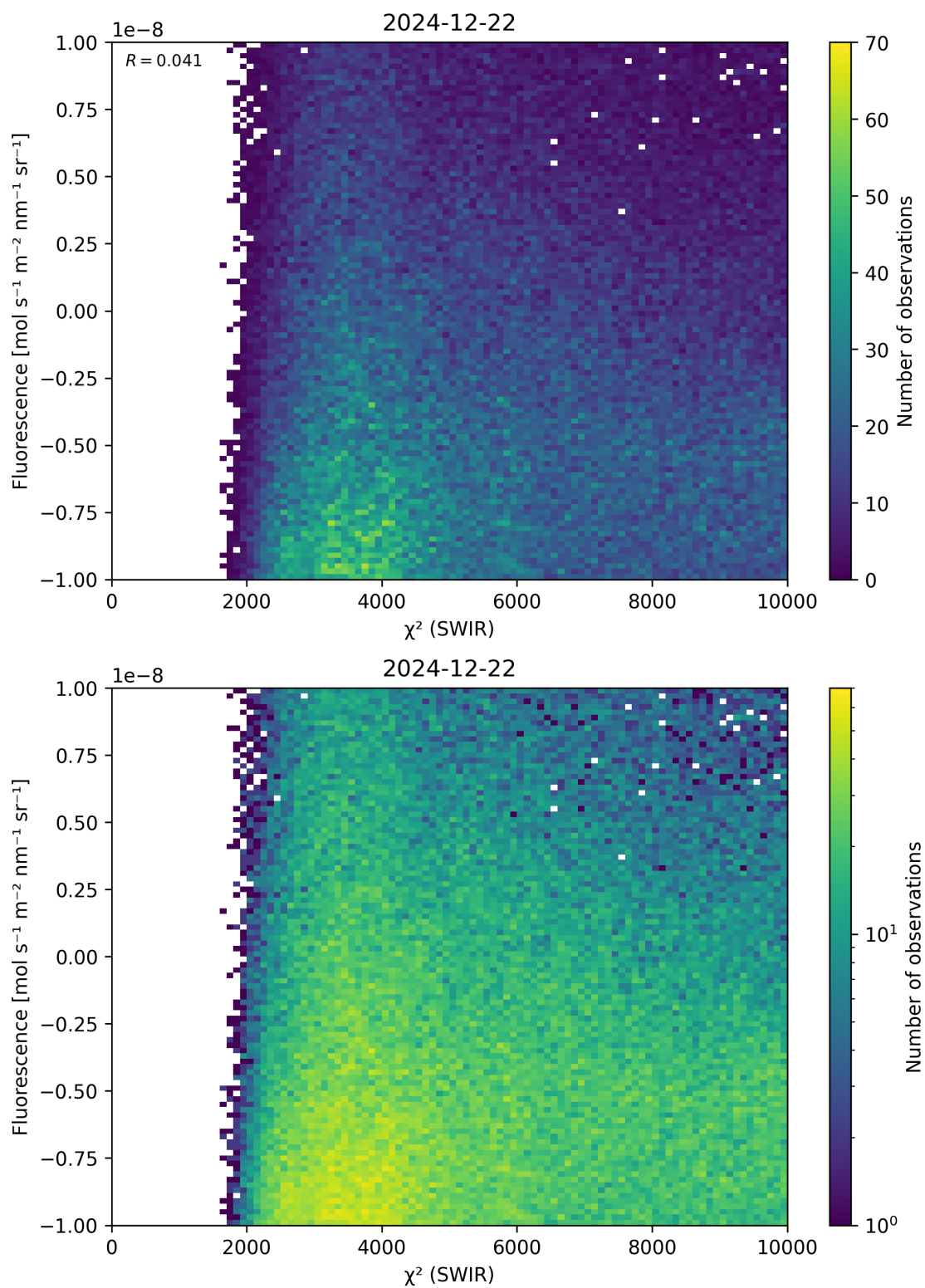
Figure 49: Scatter density plot of “ \chi^2 (SWIR)” against “Fluorescence” for 2024-12-22 to 2024-12-23.
