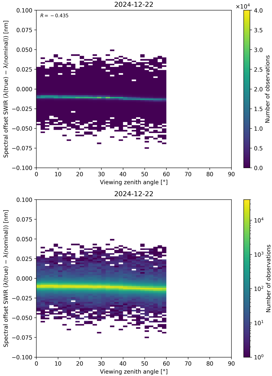
Figure 116: Scatter density plot of “Viewing zenith angle” against “Spectral offset SWIR ( \lambda_{\text{true}} - \lambda_{\text{nominal}} )” for 2024-12-22 to 2024-12-23.
