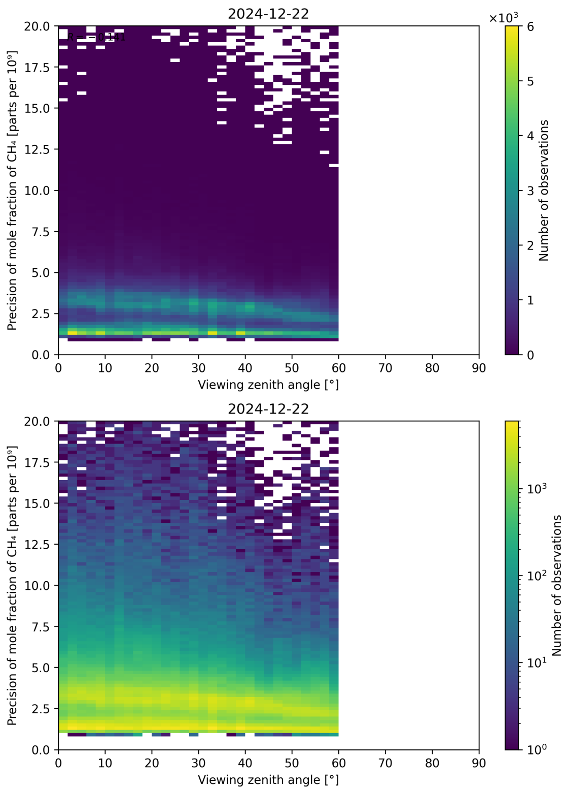
Figure 112: Scatter density plot of “Viewing zenith angle” against “Precision of mole fraction of CH 4 ” for 2024-12-22 to 2024-12-23.
