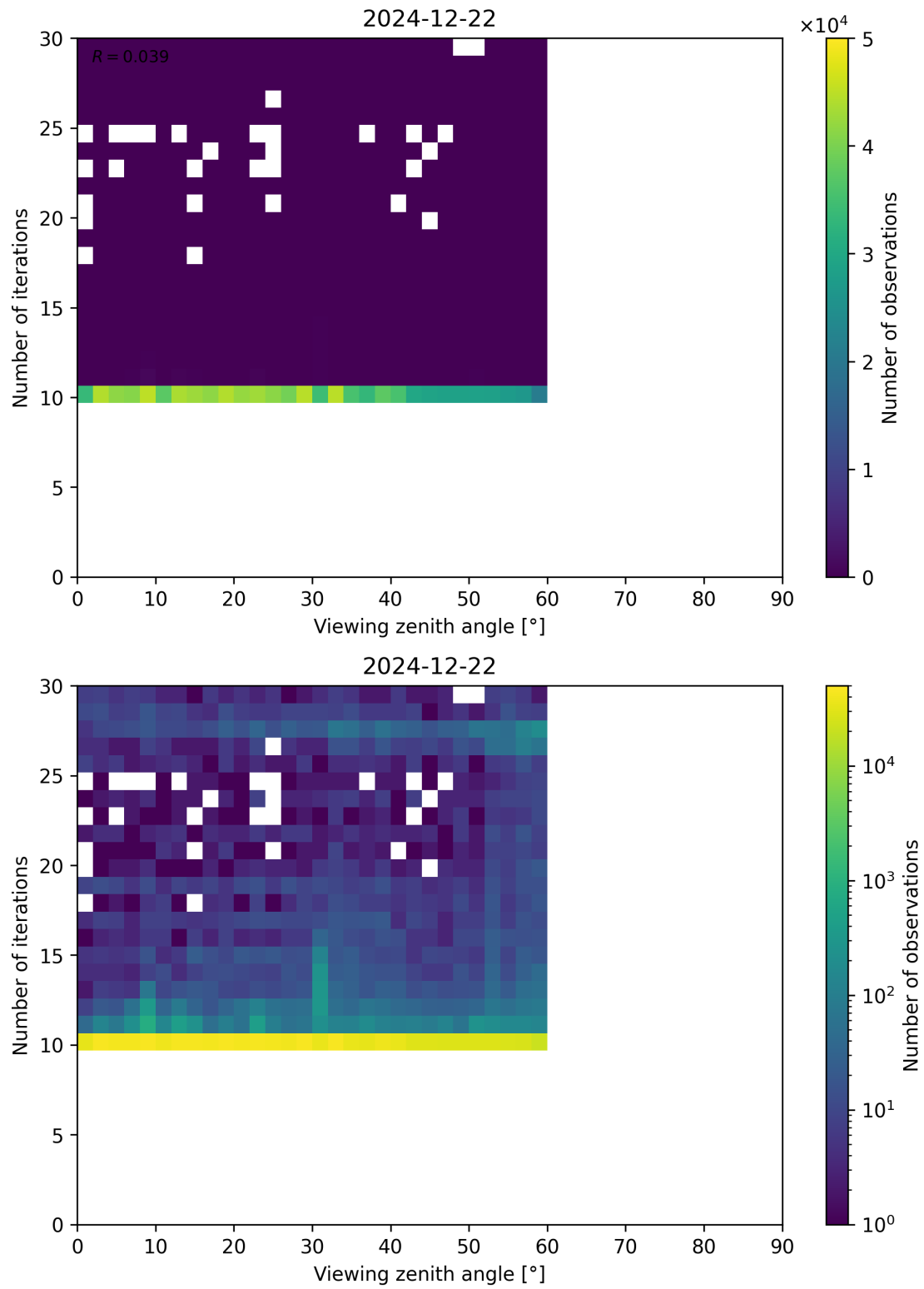
Figure 113: Scatter density plot of “Viewing zenith angle” against “Number of iterations” for 2024-12-22 to 2024-12-23.
