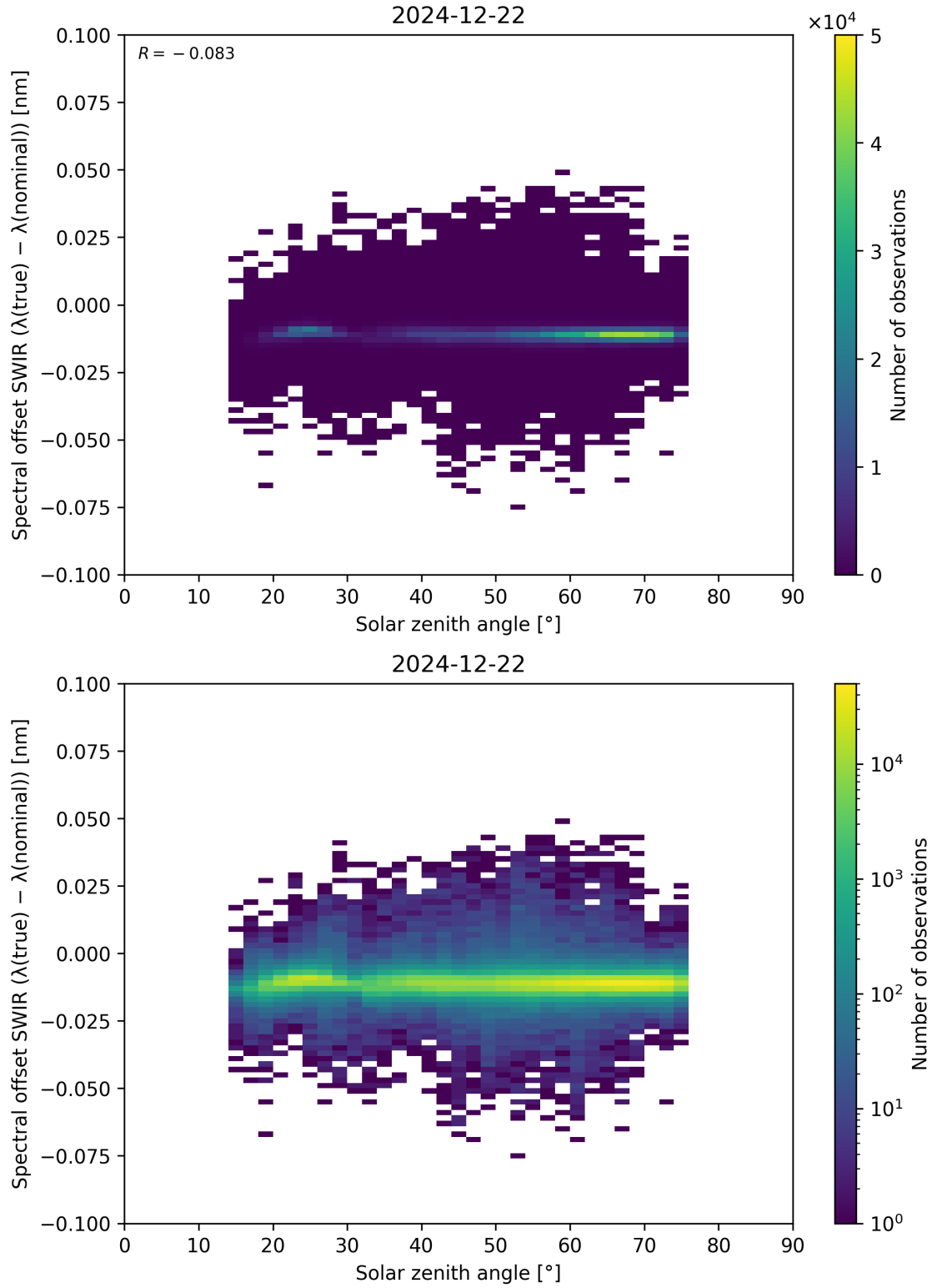
Figure 104: Scatter density plot of “Solar zenith angle” against “Spectral offset SWIR ( \lambda_{\text{true}} - \lambda_{\text{nominal}} )” for 2024-12-22 to 2024-12-23.
