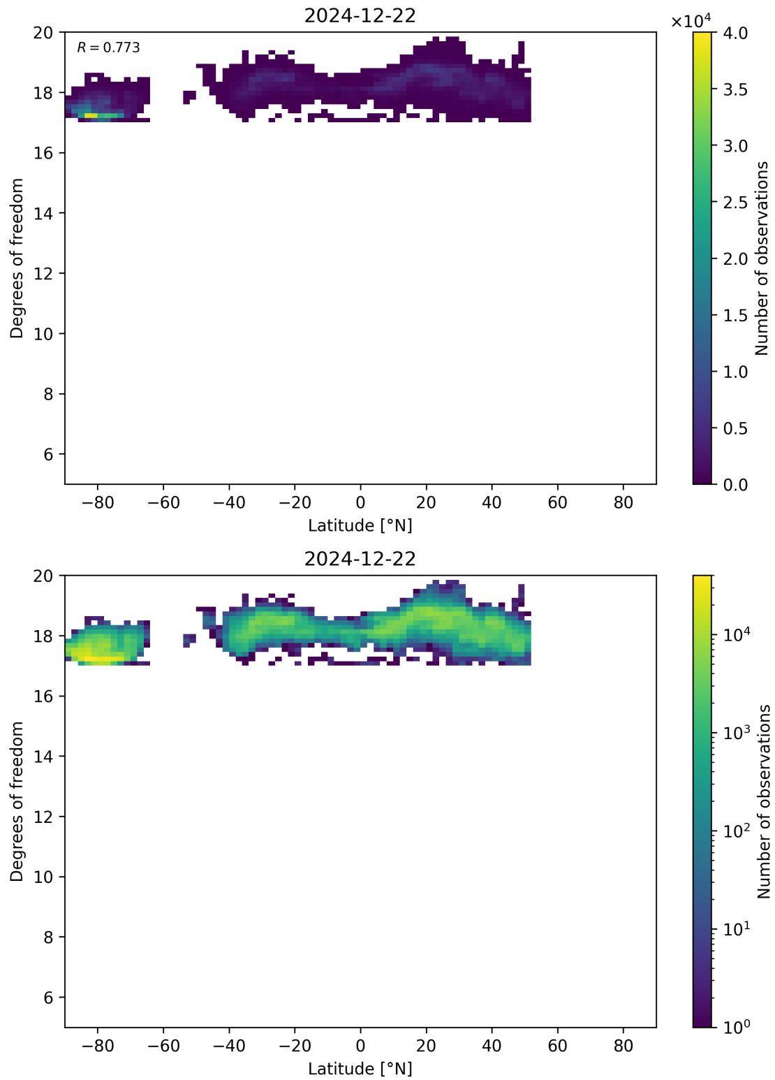
Figure 55: Scatter density plot of “Latitude” against “Degrees of freedom” for 2024-12-22 to 2024-12-23.
