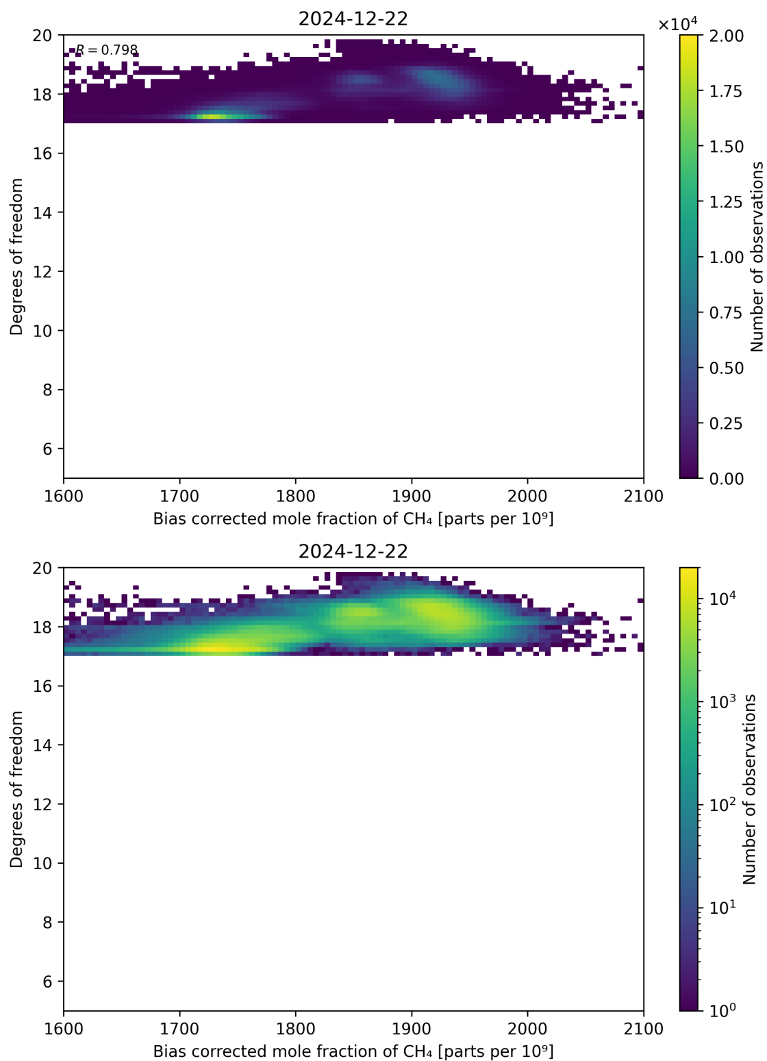
Figure 65: Scatter density plot of “Bias corrected mole fraction of CH 4 ” against “Degrees of freedom” for 2024-12-22 to 2024-12-23.
