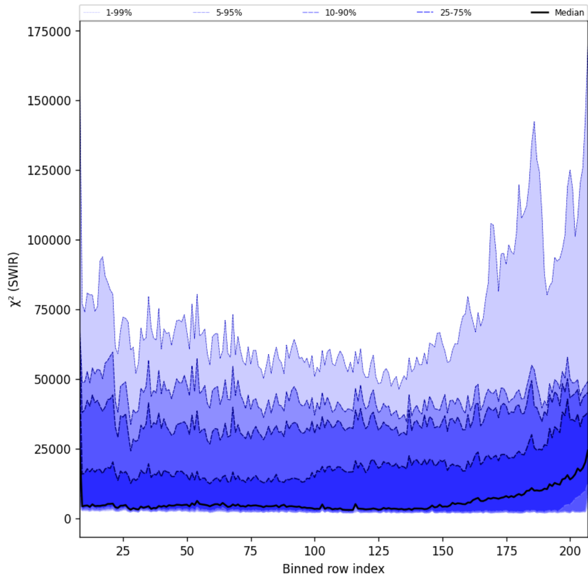
Figure 39: Along track statistics of “ \chi^2 (SWIR)” for 2024-12-22 to 2024-12-24
