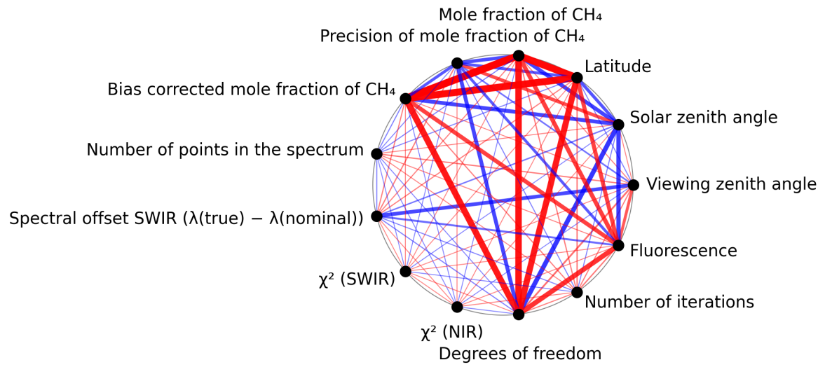
Figure 1: Map of correlation graph for 2024-12-22 to 2024-12-24.
