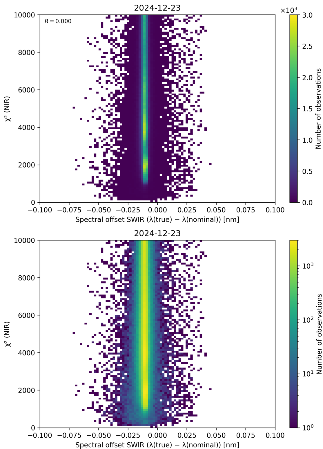
Figure 117: Scatter density plot of “Spectral offset SWIR ( \lambda_{\text{true}} - \lambda_{\text{nominal}} )” against “ \chi^2 (NIR)” for 2024-12-22 to 2024-12-24.
