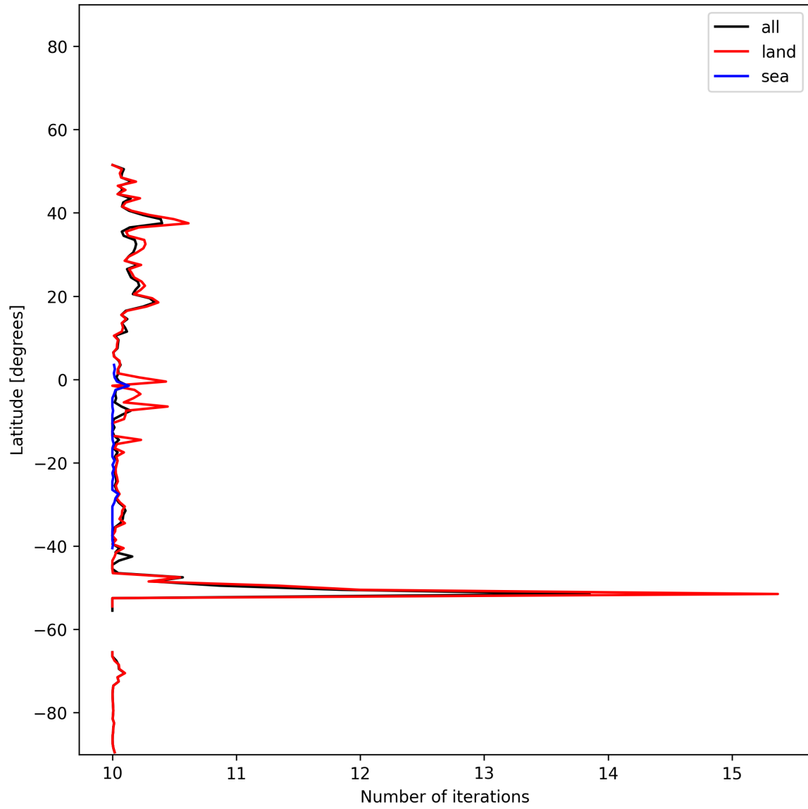
Figure 20: Zonal average of “Number of iterations” for 2024-12-22 to 2024-12-24.
