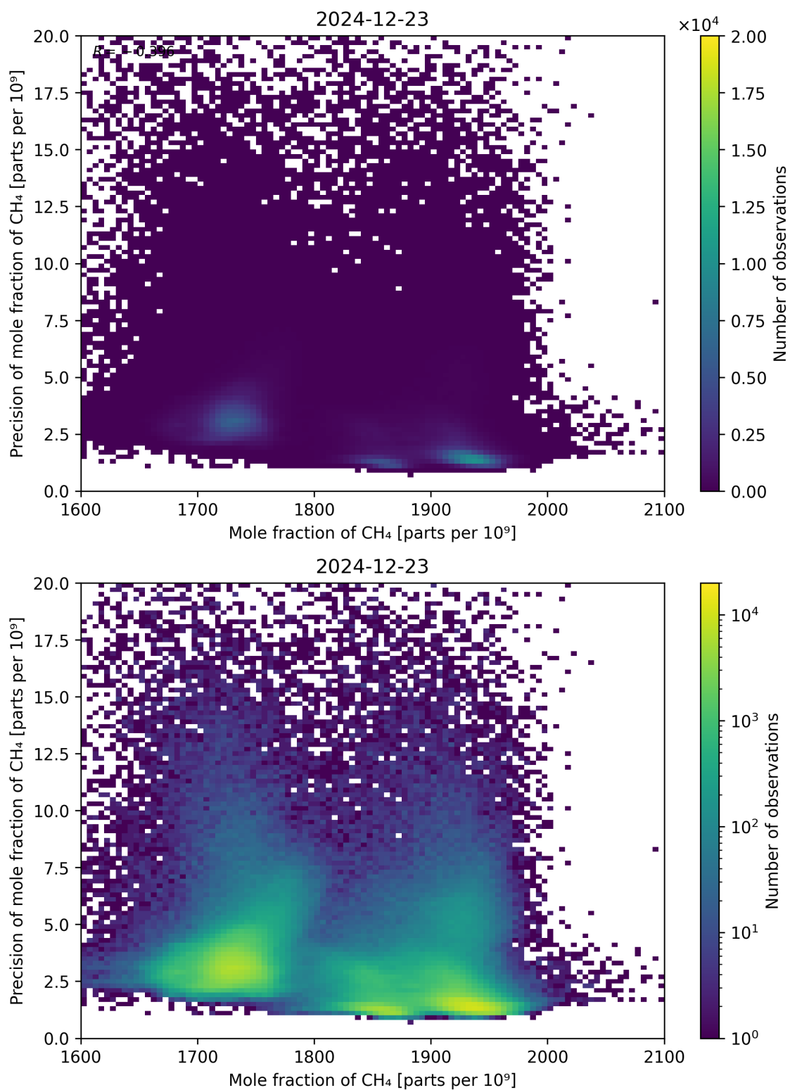
Figure 75: Scatter density plot of “Mole fraction of CH 4 ” against “Precision of mole fraction of CH 4 ” for 2024-12-22 to 2024-12-24.
