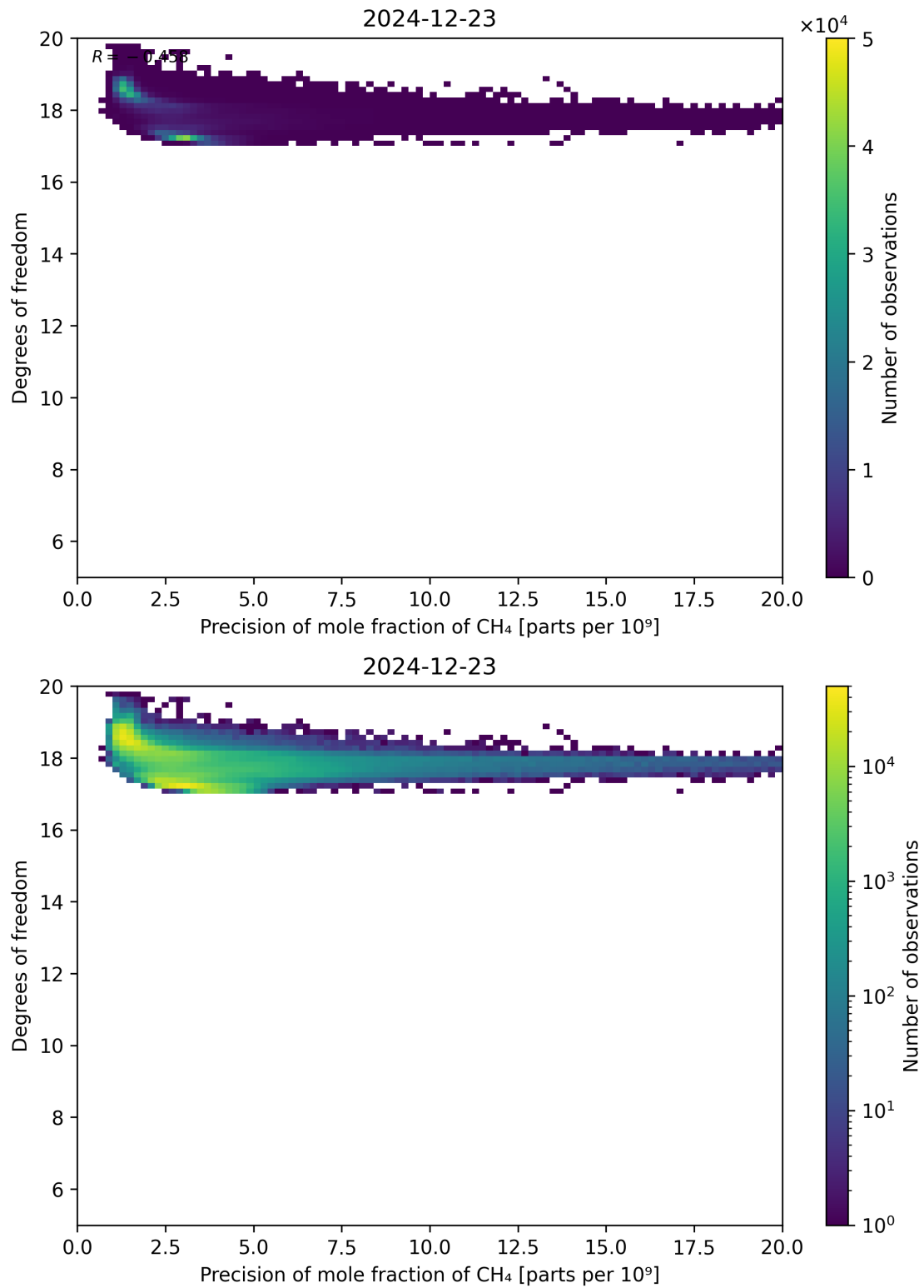
Figure 80: Scatter density plot of “Precision of mole fraction of CH 4 ” against “Degrees of freedom” for 2024-12-22 to 2024-12-24.
