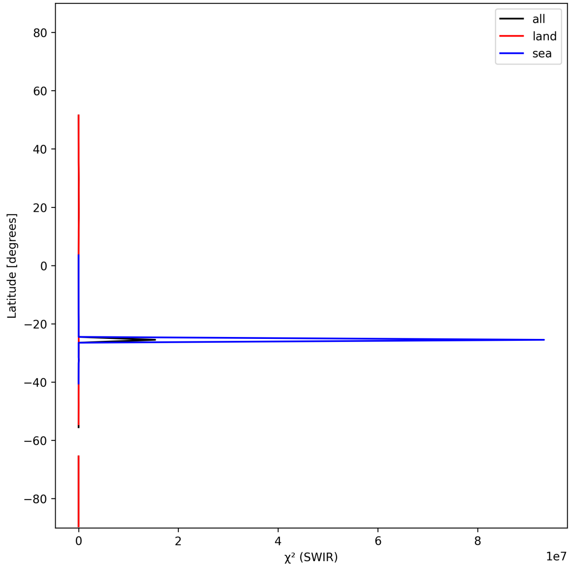
Figure 17: Zonal average of “ \chi^2 (SWIR)” for 2024-12-22 to 2024-12-24.
