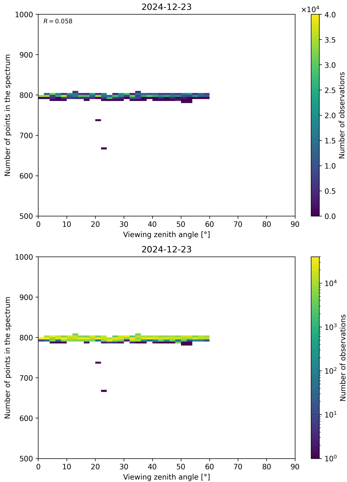
Figure 114: Scatter density plot of “Viewing zenith angle” against “Number of points in the spectrum” for 2024-12-22 to 2024-12-24.
