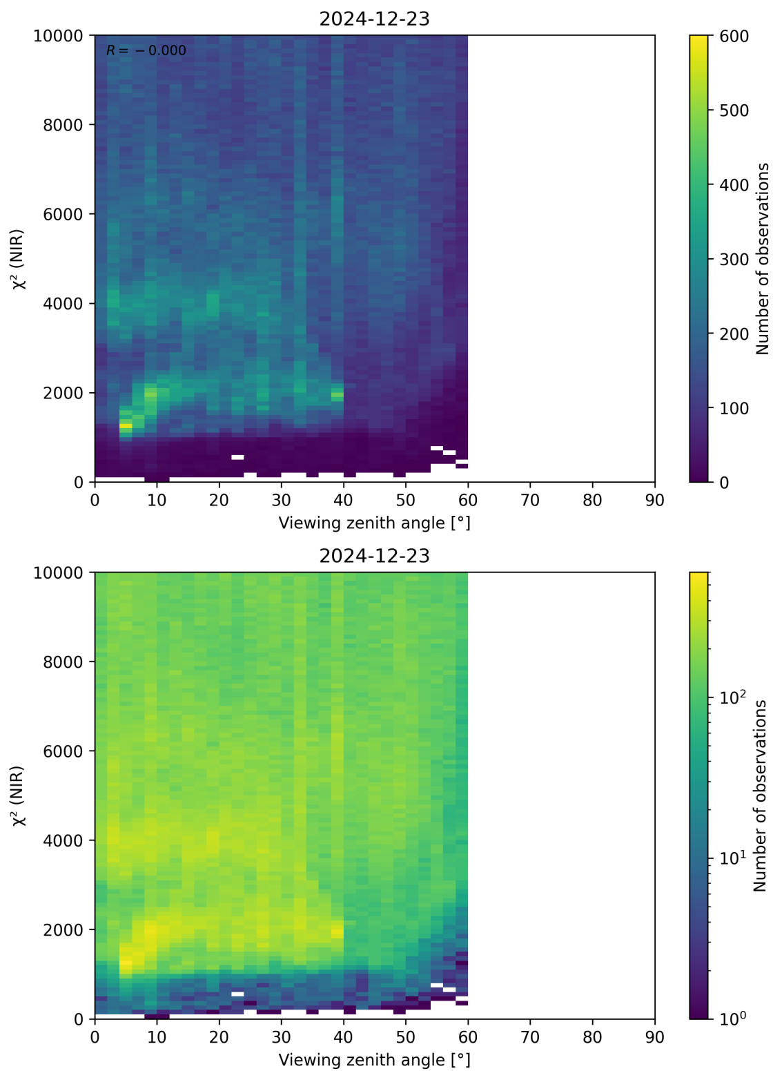
Figure 105: Scatter density plot of “Viewing zenith angle” against “ \chi^2 (NIR)” for 2024-12-22 to 2024-12-24.
