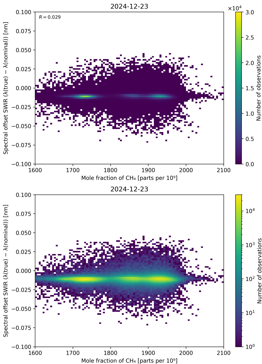
Figure 86: Scatter density plot of “Mole fraction of \text{CH}_4 ” against “Spectral offset SWIR ( \lambda_{\text{true}} - \lambda_{\text{nominal}} )” for 2024-12-22 to 2024-12-24.
