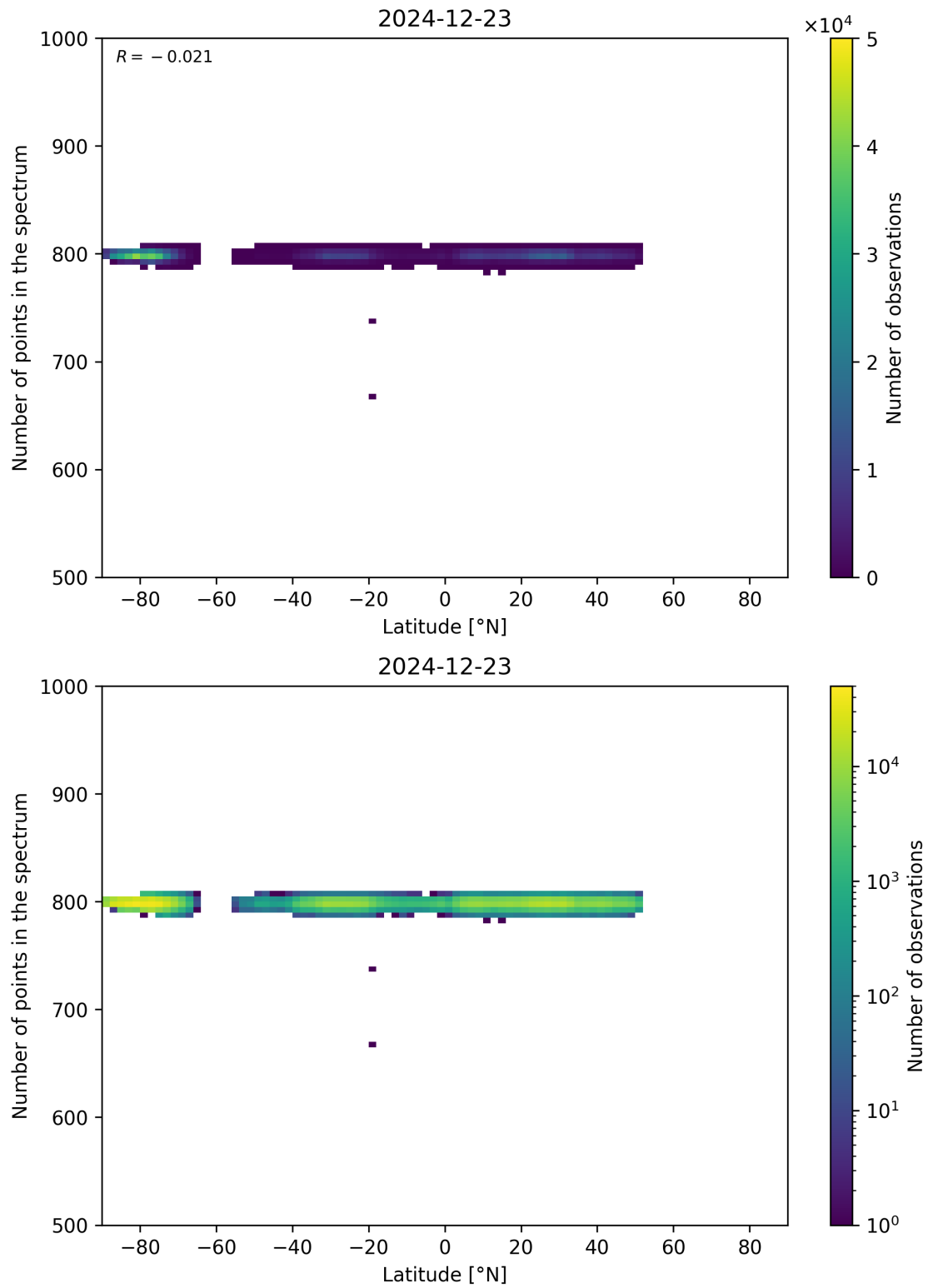
Figure 61: Scatter density plot of “Latitude” against “Number of points in the spectrum” for 2024-12-22 to 2024-12-24.
