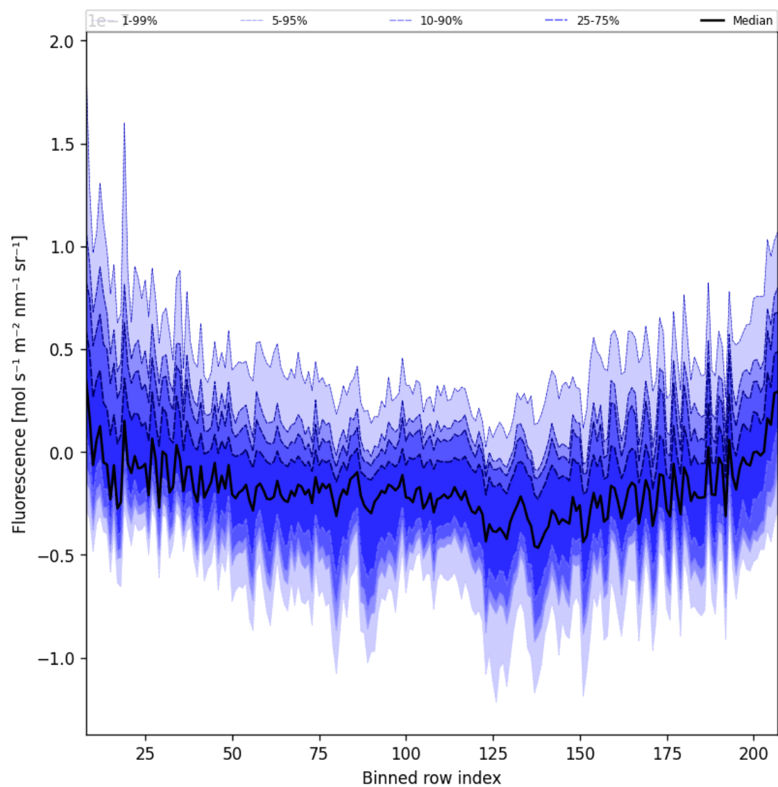
Figure 43: Along track statistics of “Fluorescence” for 2024-12-22 to 2024-12-24
