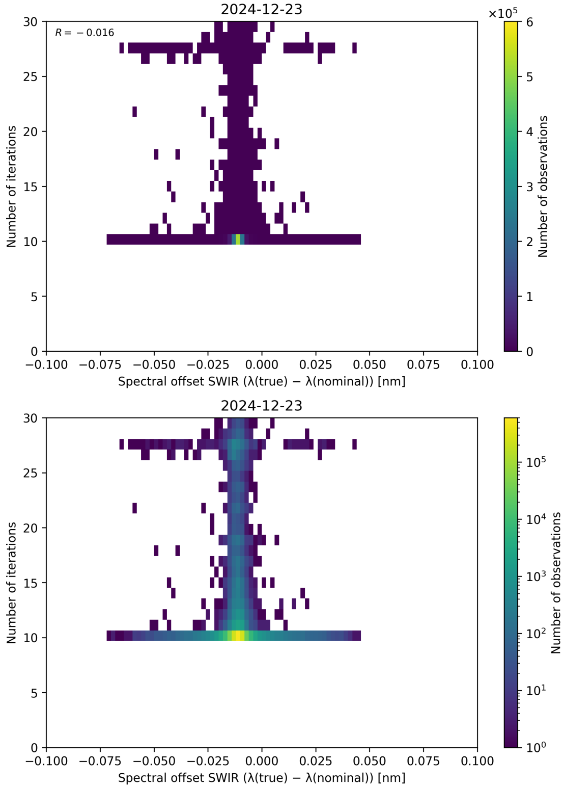
Figure 121: Scatter density plot of “Spectral offset SWIR ( \lambda_{\text{true}} - \lambda_{\text{nominal}} )” against “Number of iterations” for 2024-12-22 to 2024-12-24.
