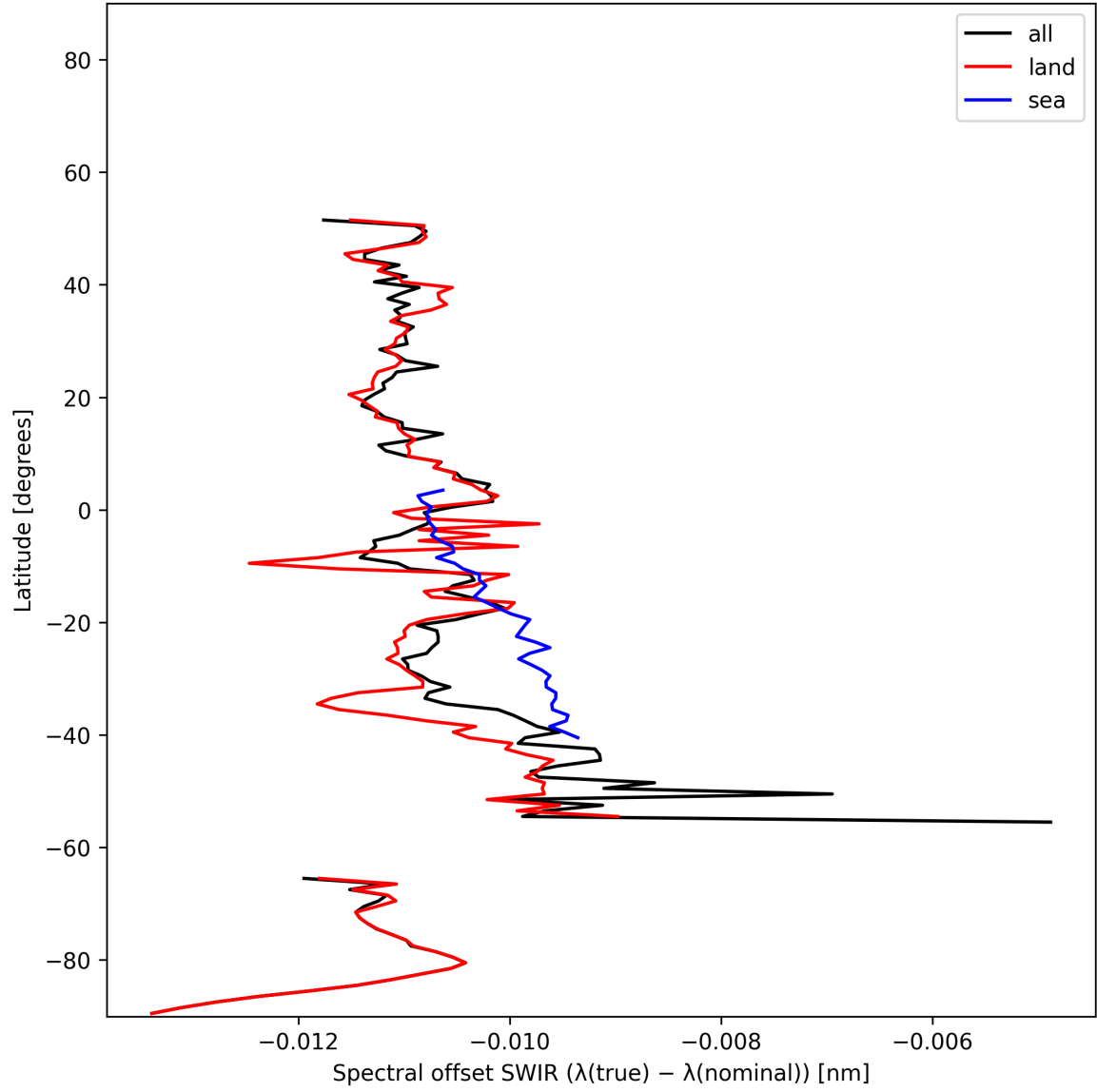
Figure 16: Zonal average of “Spectral offset SWIR ( \lambda_{\text{true}} - \lambda_{\text{nominal}} )” for 2024-12-22 to 2024-12-24.
