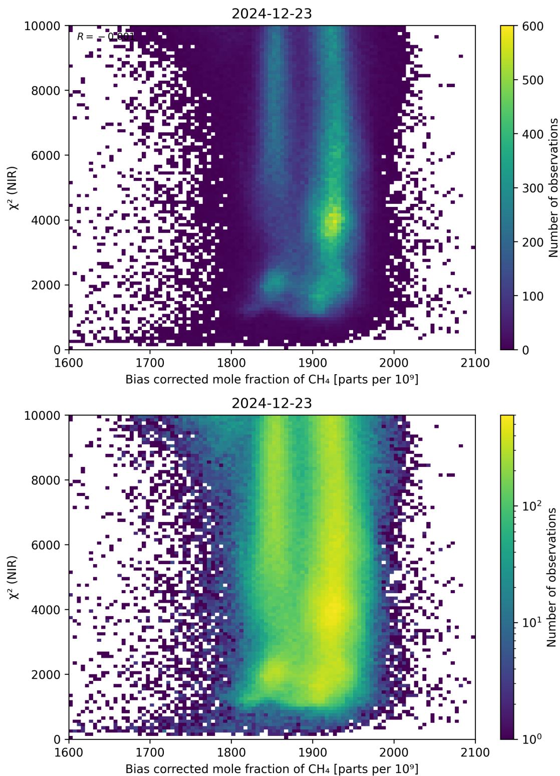
Figure 63: Scatter density plot of “Bias corrected mole fraction of CH 4 ” against “ \chi^2 (NIR)” for 2024-12-22 to 2024-12-24.
