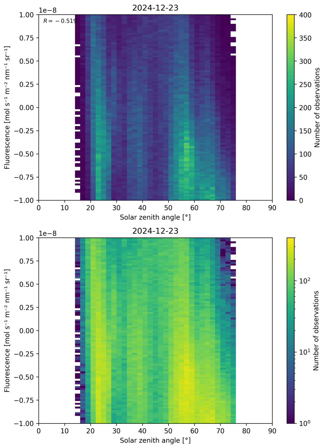
Figure 97: Scatter density plot of “Solar zenith angle” against “Fluorescence” for 2024-12-22 to 2024-12-24.
