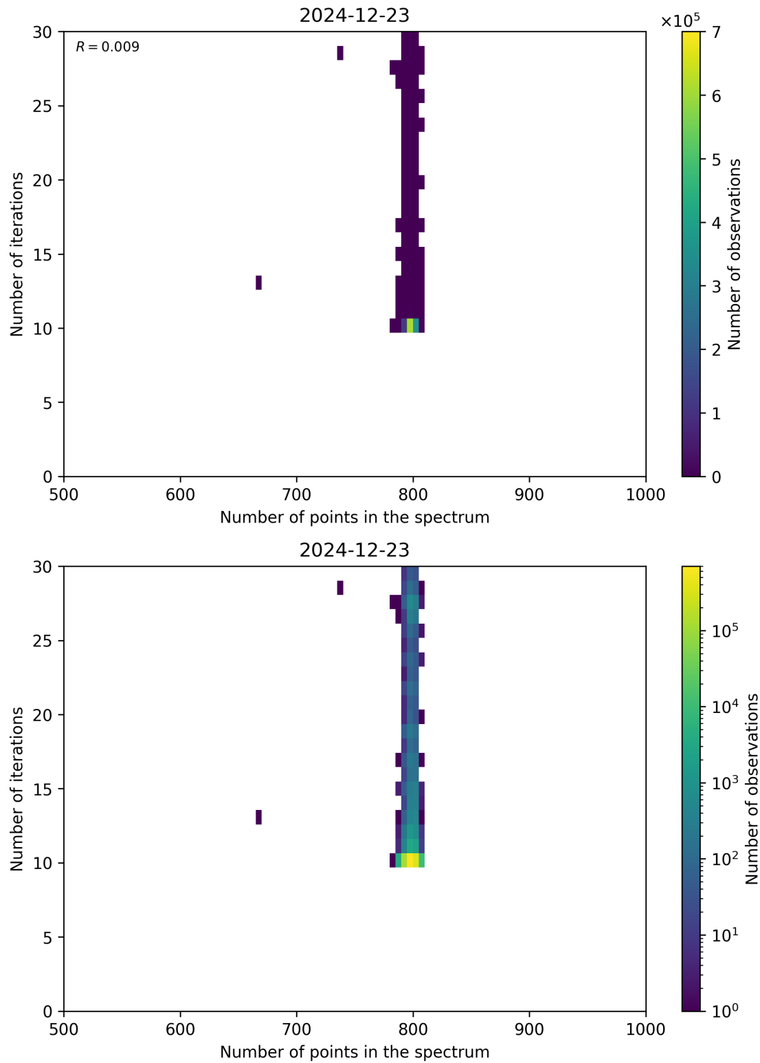
Figure 92: Scatter density plot of “Number of points in the spectrum” against “Number of iterations” for 2024-12-22 to 2024-12-24.
