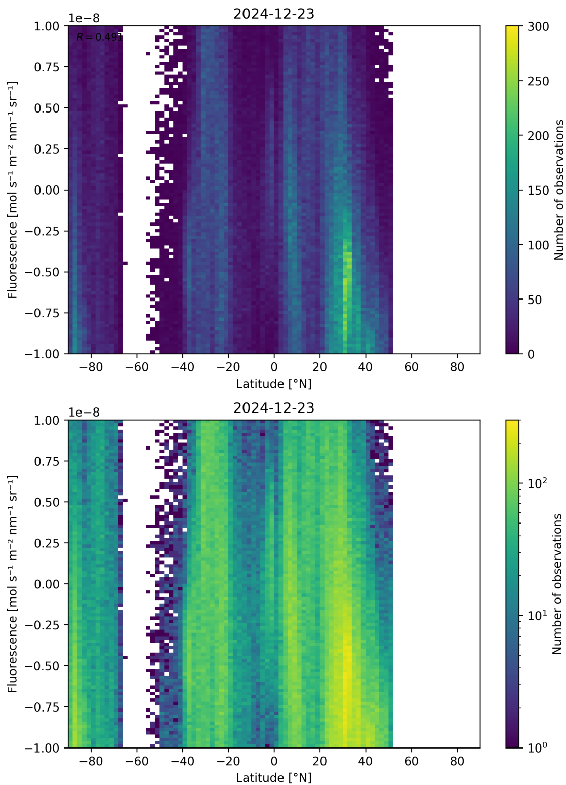
Figure 56: Scatter density plot of “Latitude” against “Fluorescence” for 2024-12-22 to 2024-12-24.
