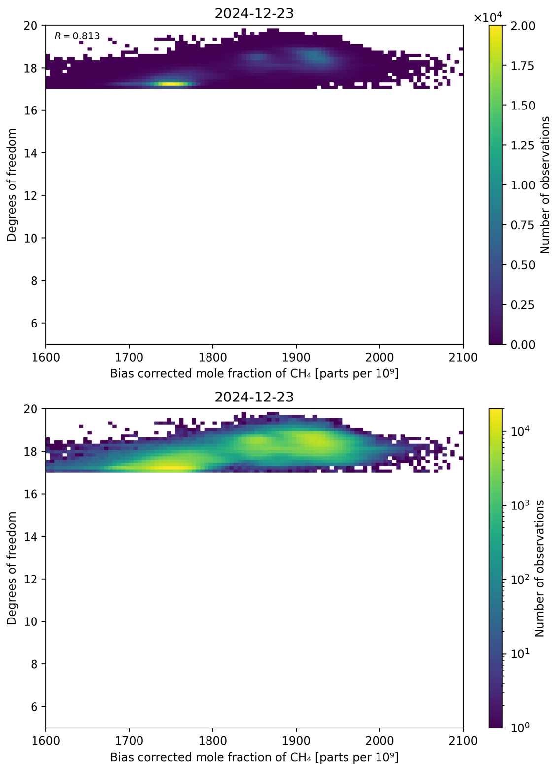
Figure 65: Scatter density plot of “Bias corrected mole fraction of CH 4 ” against “Degrees of freedom” for 2024-12-22 to 2024-12-24.
