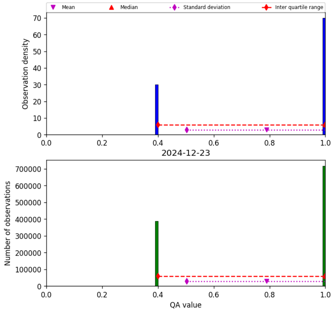
Figure 22: Histogram of “QA value” for 2024-12-22 to 2024-12-24
