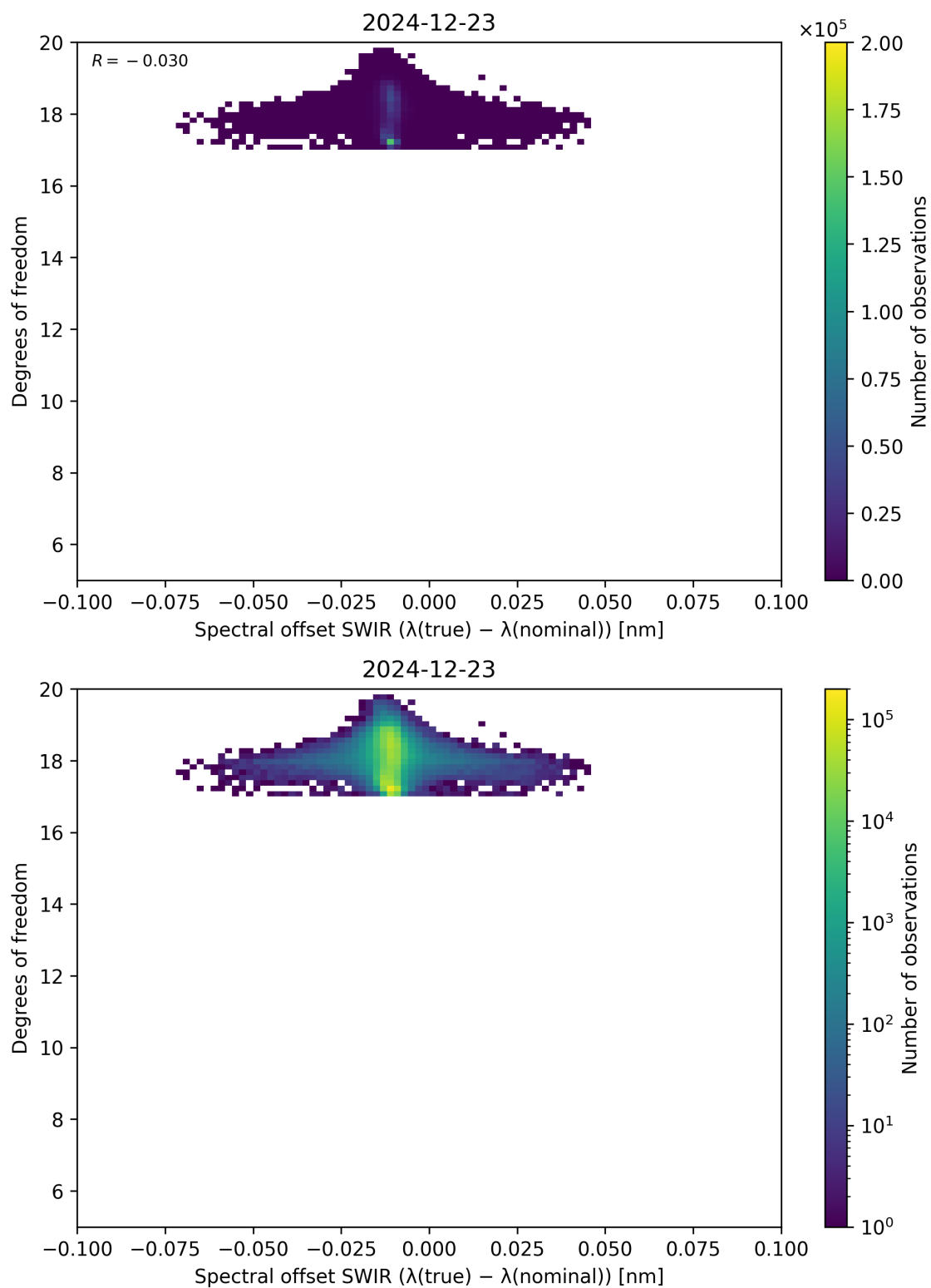
Figure 119: Scatter density plot of “Spectral offset SWIR ( \lambda_{\text{true}} - \lambda_{\text{nominal}} )” against “Degrees of freedom” for 2024-12-22 to 2024-12-24.
