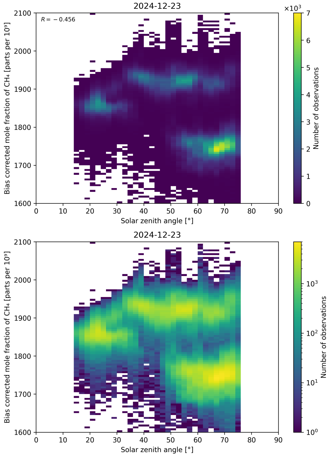
Figure 100: Scatter density plot of “Solar zenith angle” against “Bias corrected mole fraction of \text{CH}_4 ” for 2024-12-22 to 2024-12-24.
