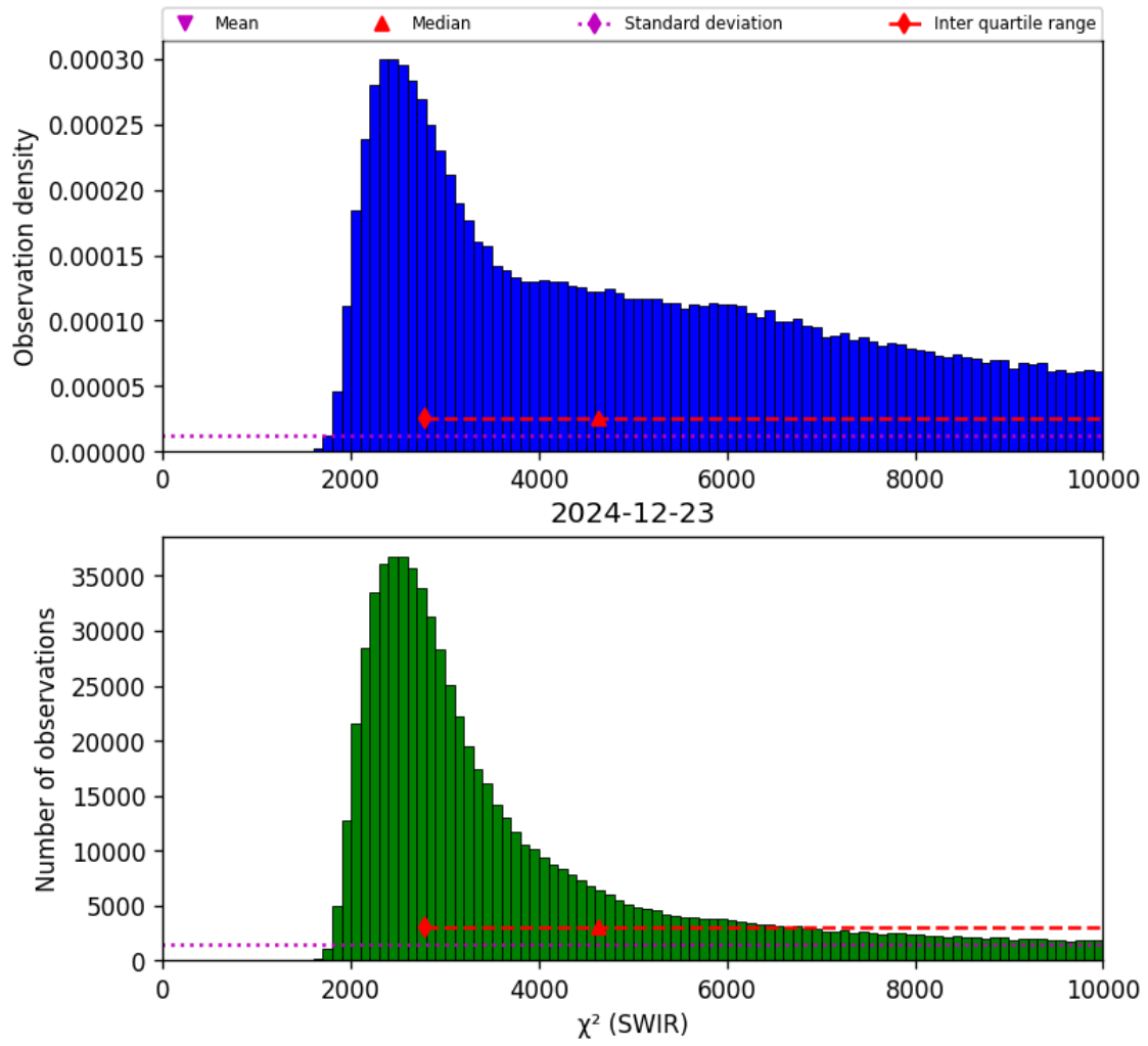
Figure 28: Histogram of “ \chi^2 (SWIR)” for 2024-12-22 to 2024-12-24
