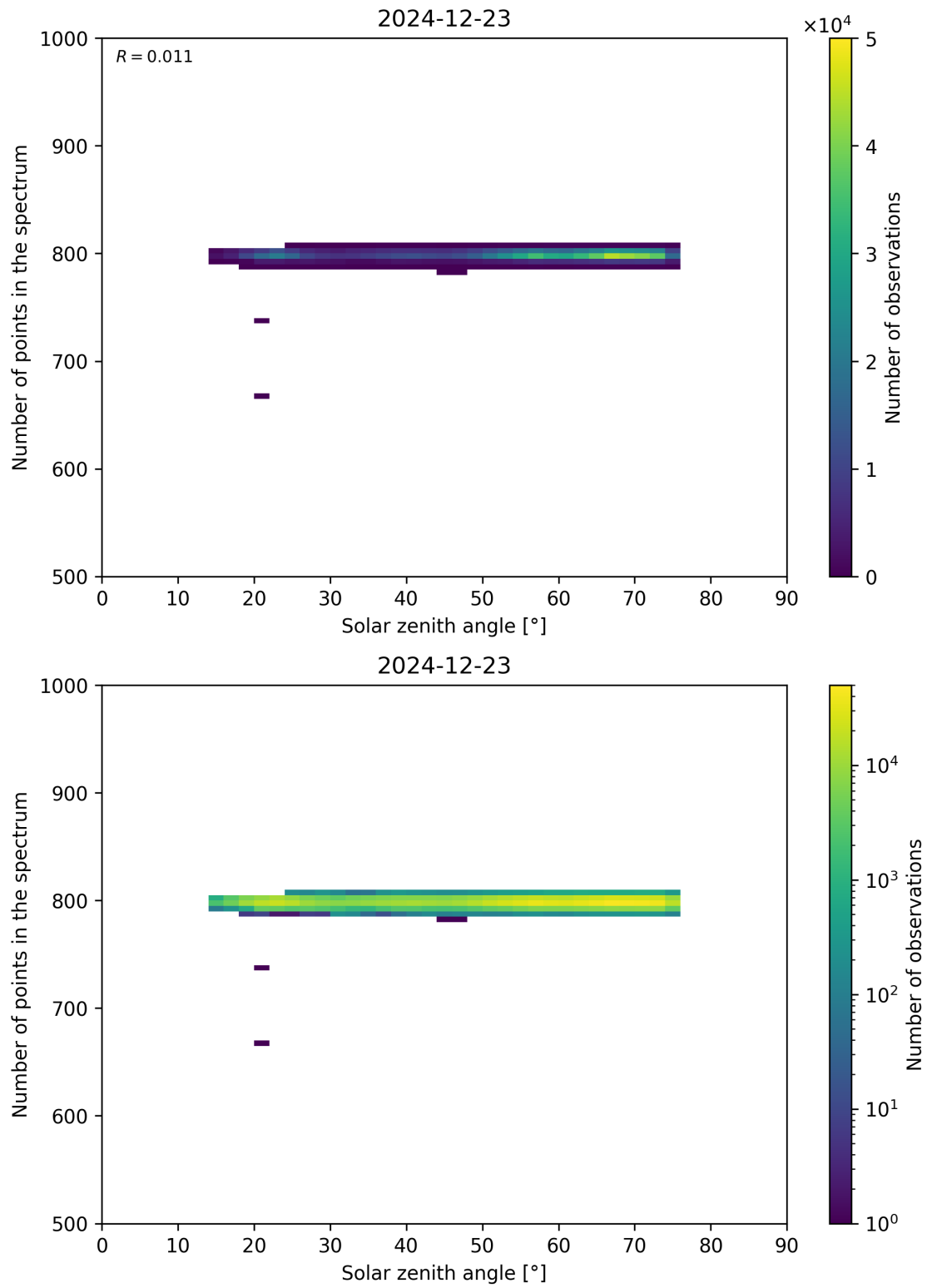
Figure 103: Scatter density plot of “Solar zenith angle” against “Number of points in the spectrum” for 2024-12-22 to 2024-12-24.
