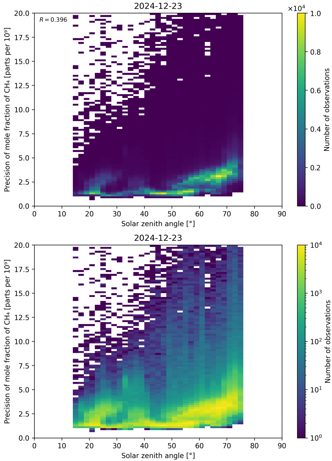
Figure 101: Scatter density plot of “Solar zenith angle” against “Precision of mole fraction of \text{CH}_4 ” for 2024-12-22 to 2024-12-24.
