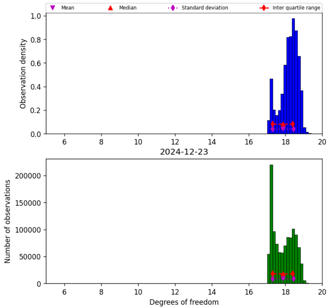
Figure 30: Histogram of “Degrees of freedom” for 2024-12-22 to 2024-12-24
