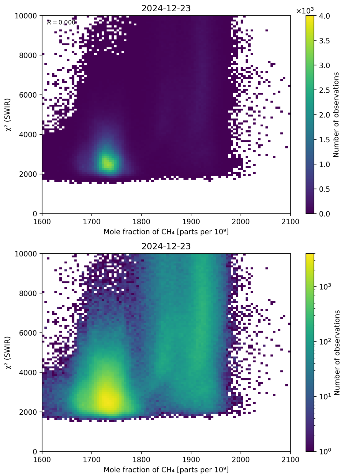
Figure 71: Scatter density plot of “Mole fraction of \text{CH}_4 ” against “ \chi^2 (SWIR)” for 2024-12-22 to 2024-12-24.
