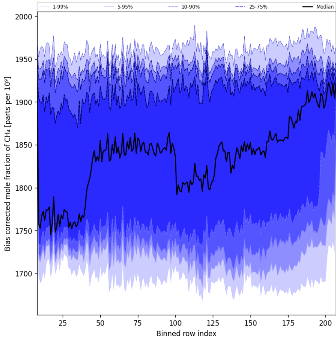
Figure 36: Along track statistics of “Bias corrected mole fraction of CH 4 ” for 2024-12-22 to 2024-12-24
