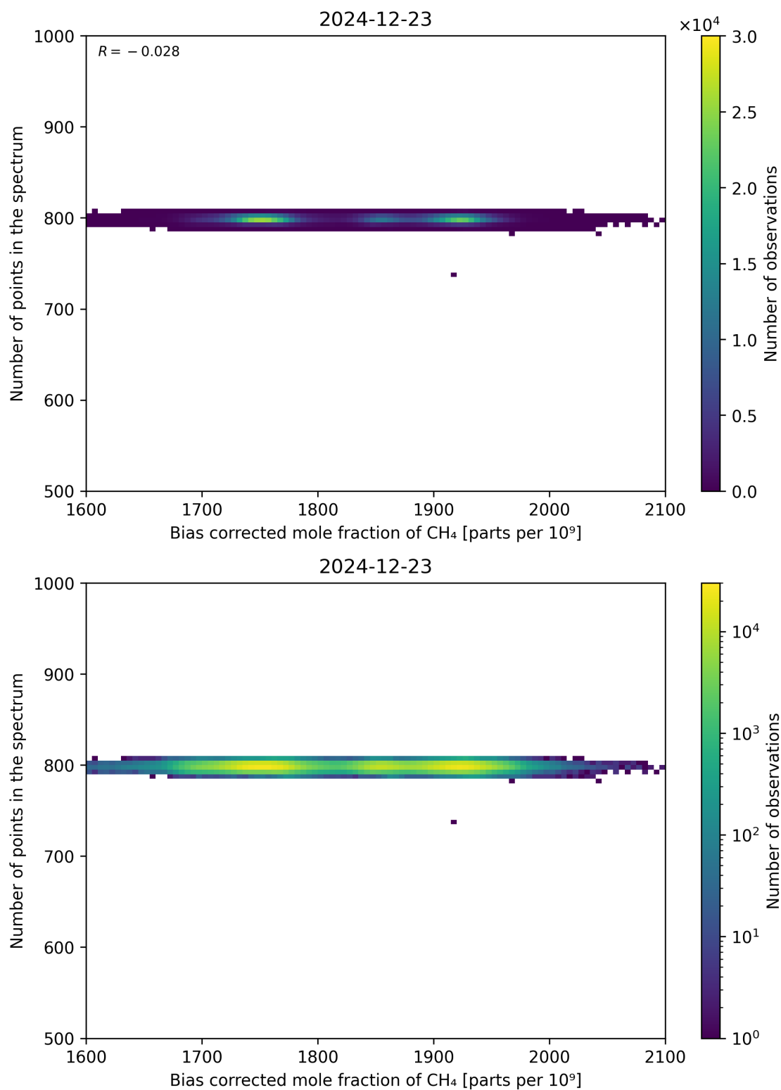
Figure 68: Scatter density plot of “Bias corrected mole fraction of CH 4 ” against “Number of points in the spectrum” for 2024-12-22 to 2024-12-24.
