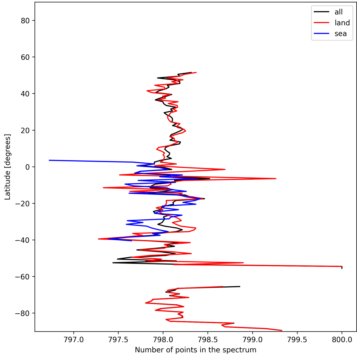
Figure 15: Zonal average of “Number of points in the spectrum” for 2024-12-22 to 2024-12-24.
