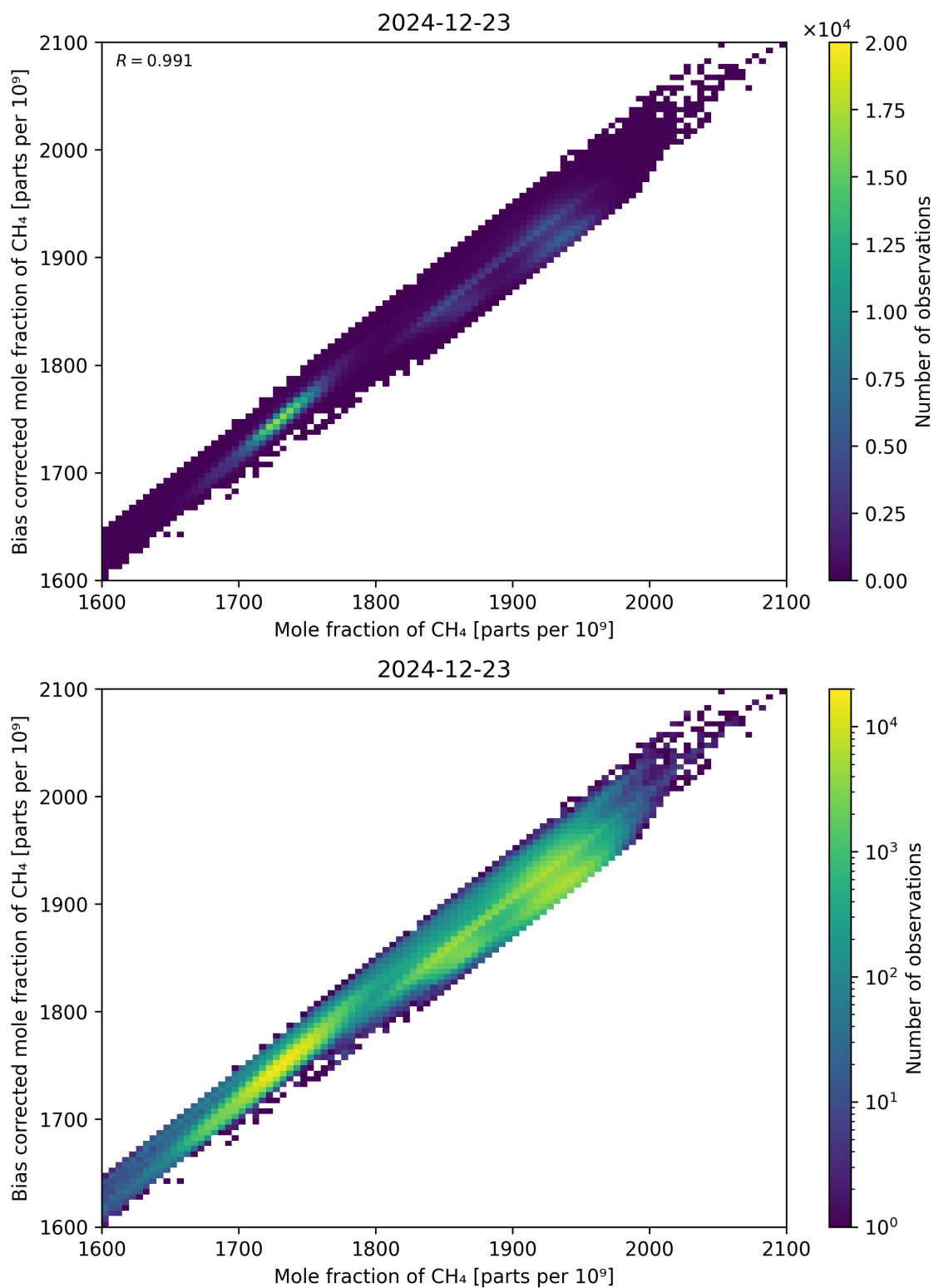
Figure 74: Scatter density plot of “Mole fraction of CH 4 ” against “Bias corrected mole fraction of CH 4 ” for 2024-12-22 to 2024-12-24.
