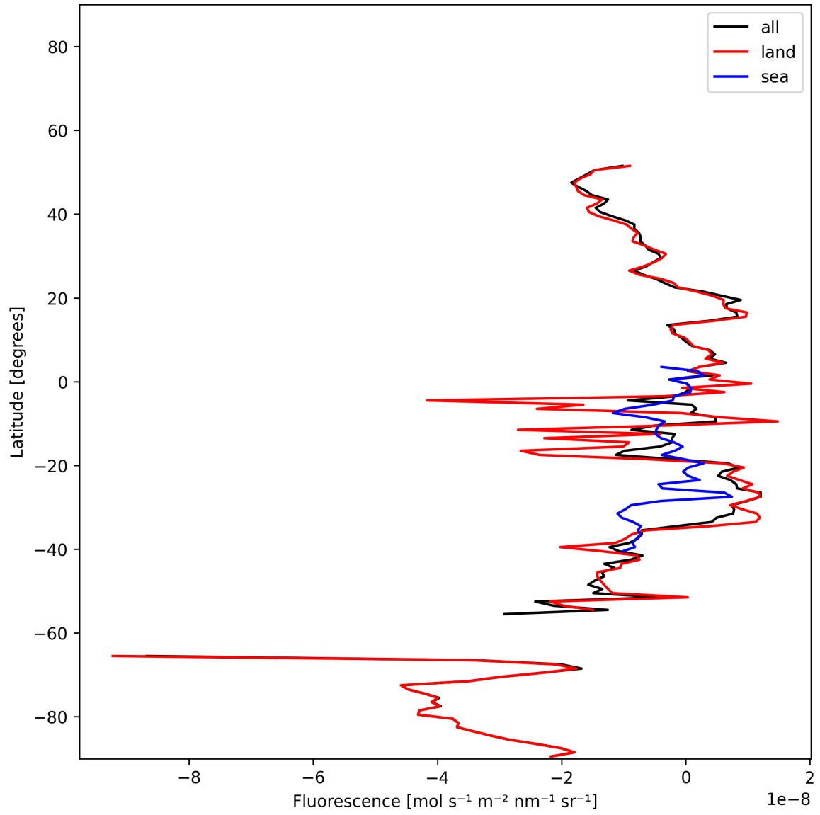
Figure 21: Zonal average of “Fluorescence” for 2024-12-22 to 2024-12-24.
