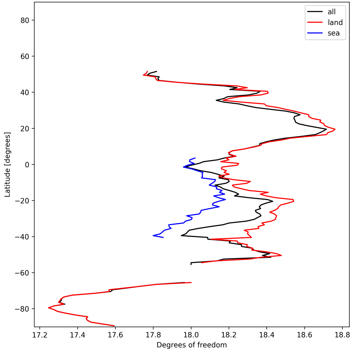
Figure 19: Zonal average of “Degrees of freedom” for 2024-12-22 to 2024-12-24.
