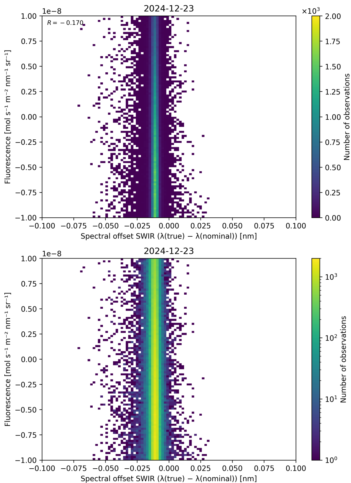
Figure 120: Scatter density plot of “Spectral offset SWIR ( \lambda_{\text{true}} - \lambda_{\text{nominal}} )” against “Fluorescence” for 2024-12-22 to 2024-12-24.
