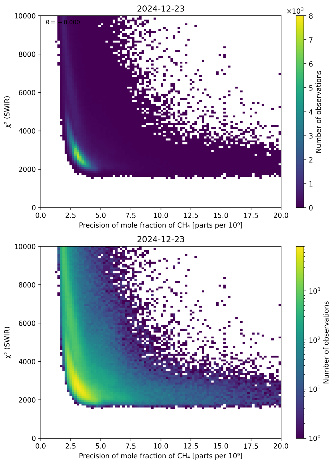
Figure 79: Scatter density plot of “Precision of mole fraction of CH 4 ” against “ \chi^2 (SWIR)” for 2024-12-22 to 2024-12-24.
