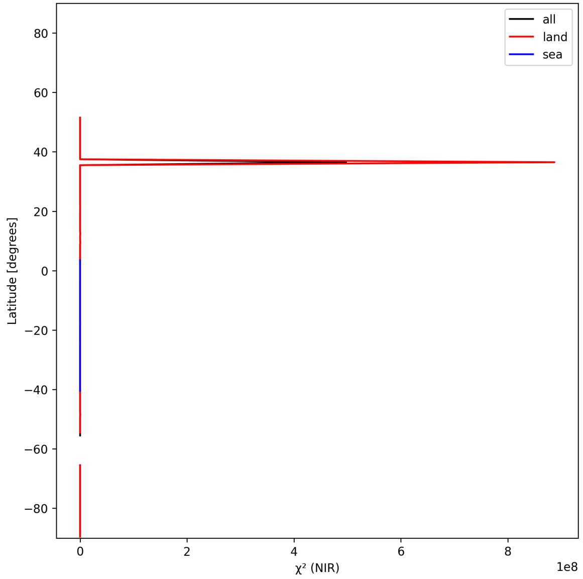
Figure 18: Zonal average of “ \chi^2 (NIR)” for 2024-12-22 to 2024-12-24.
