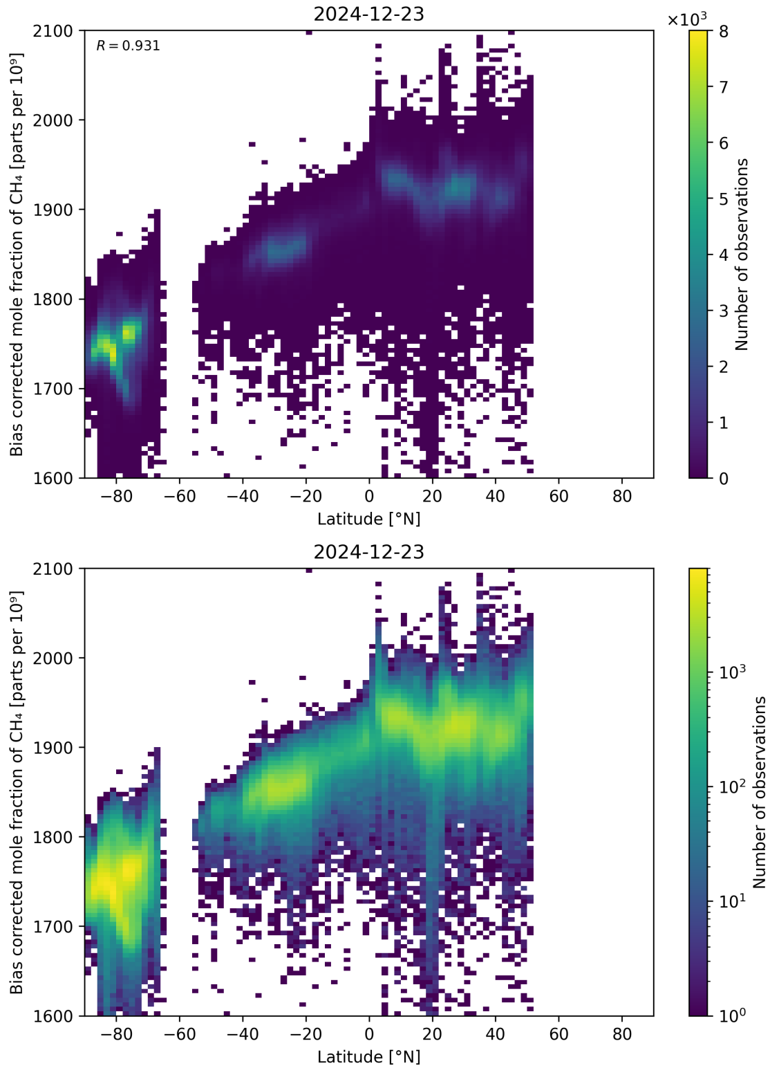
Figure 58: Scatter density plot of “Latitude” against “Bias corrected mole fraction of CH 4 ” for 2024-12-22 to 2024-12-24.
