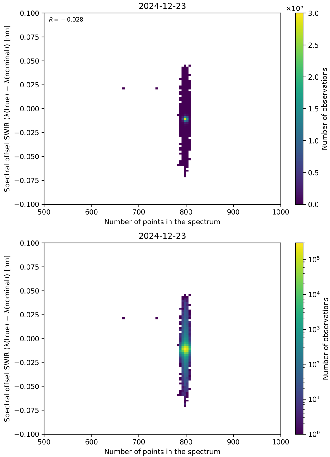
Figure 93: Scatter density plot of “Number of points in the spectrum” against “Spectral offset SWIR ( \lambda_{\text{true}} - \lambda_{\text{nominal}} )” for 2024-12-22 to 2024-12-24.
