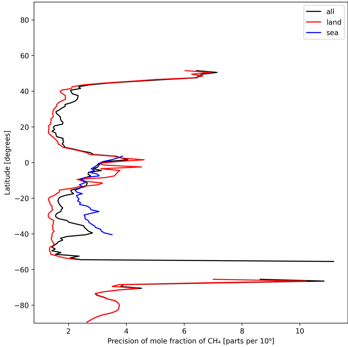
Figure 13: Zonal average of “Precision of mole fraction of CH 4 ” for 2024-12-22 to 2024-12-24.
