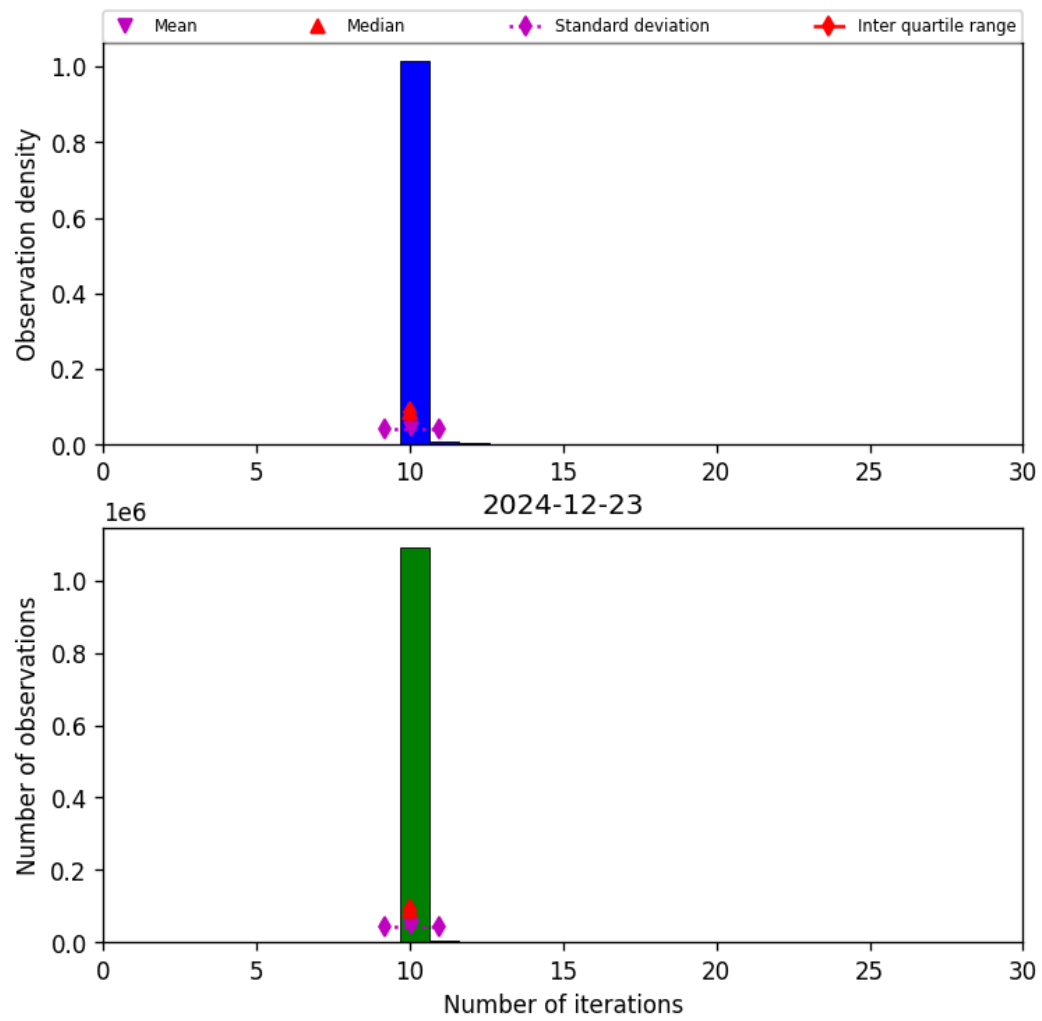
Figure 31: Histogram of “Number of iterations” for 2024-12-22 to 2024-12-24
