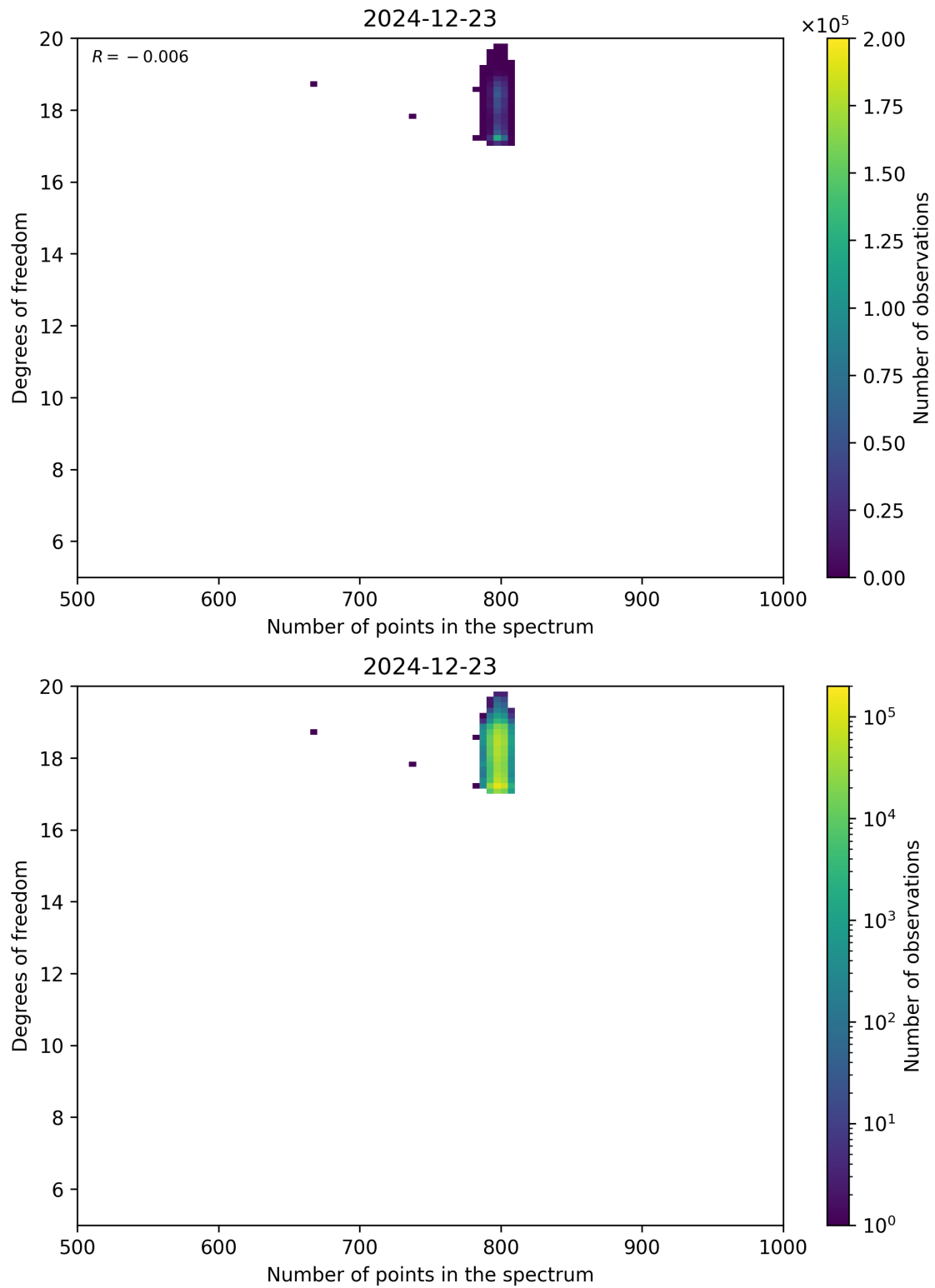
Figure 90: Scatter density plot of “Number of points in the spectrum” against “Degrees of freedom” for 2024-12-22 to 2024-12-24.
