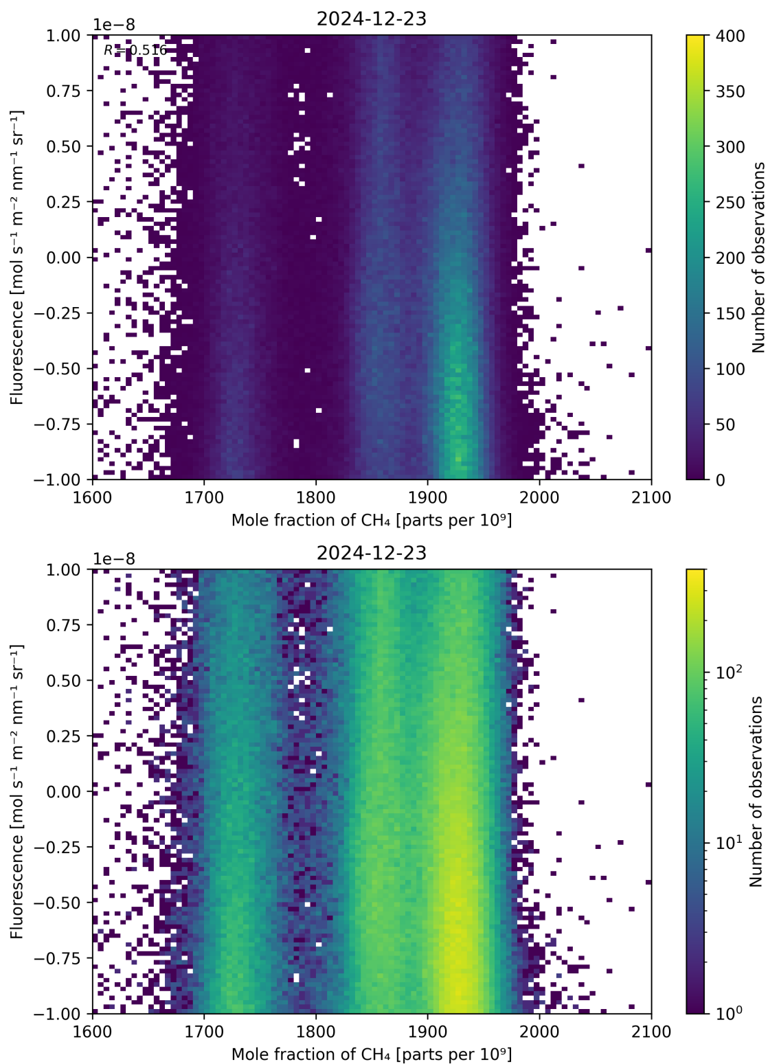
Figure 73: Scatter density plot of “Mole fraction of \text{CH}_4 ” against “Fluorescence” for 2024-12-22 to 2024-12-24.
