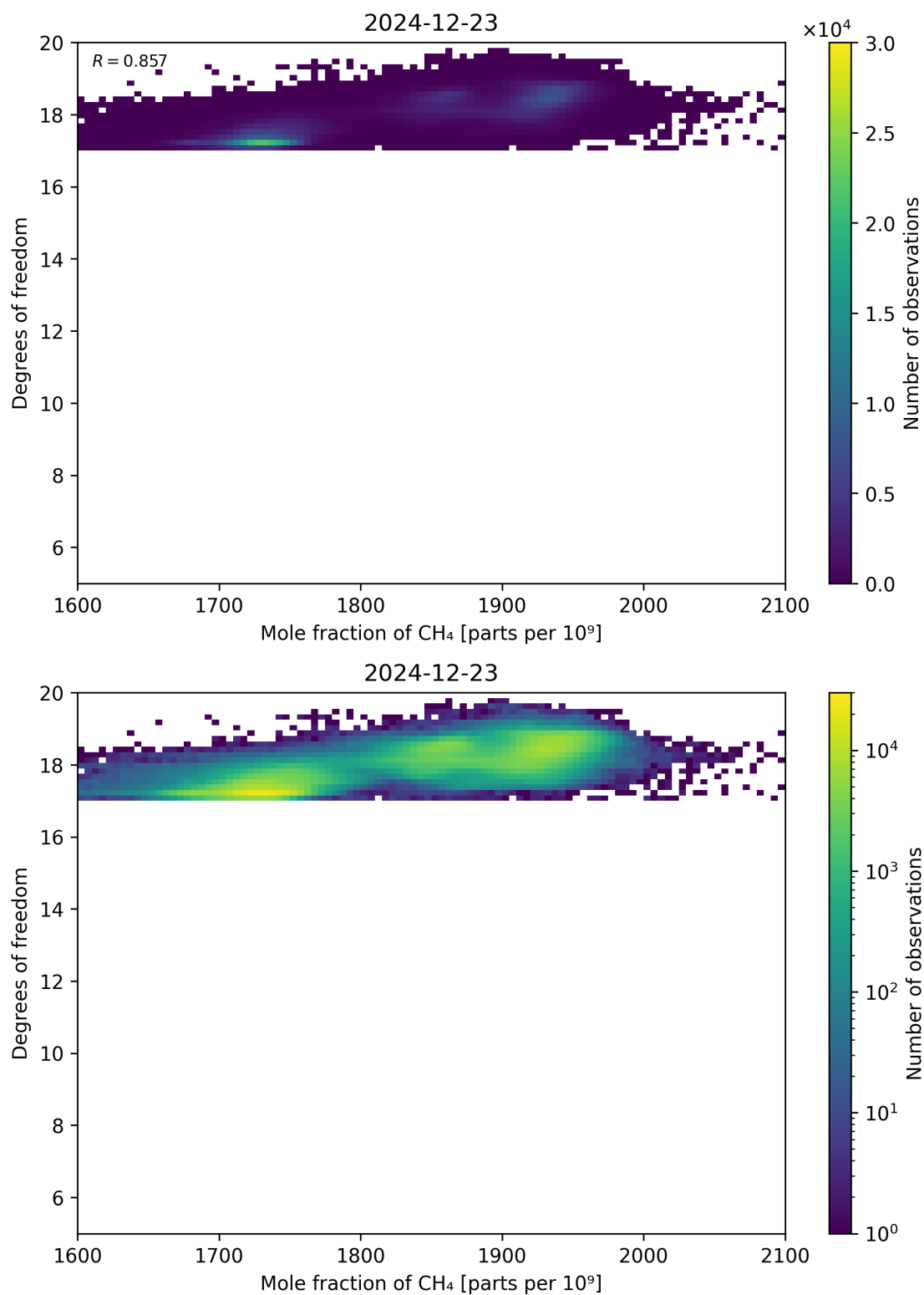
Figure 72: Scatter density plot of “Mole fraction of CH 4 ” against “Degrees of freedom” for 2024-12-22 to 2024-12-24.
