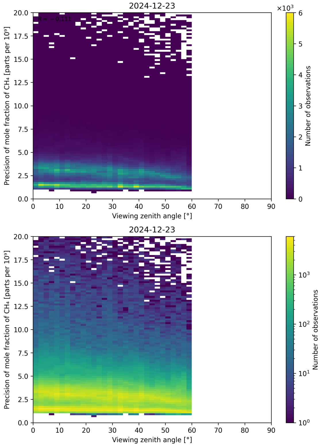
Figure 112: Scatter density plot of “Viewing zenith angle” against “Precision of mole fraction of \text{CH}_4 ” for 2024-12-22 to 2024-12-24.
