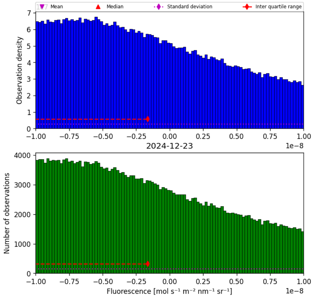
Figure 32: Histogram of “Fluorescence” for 2024-12-22 to 2024-12-24
