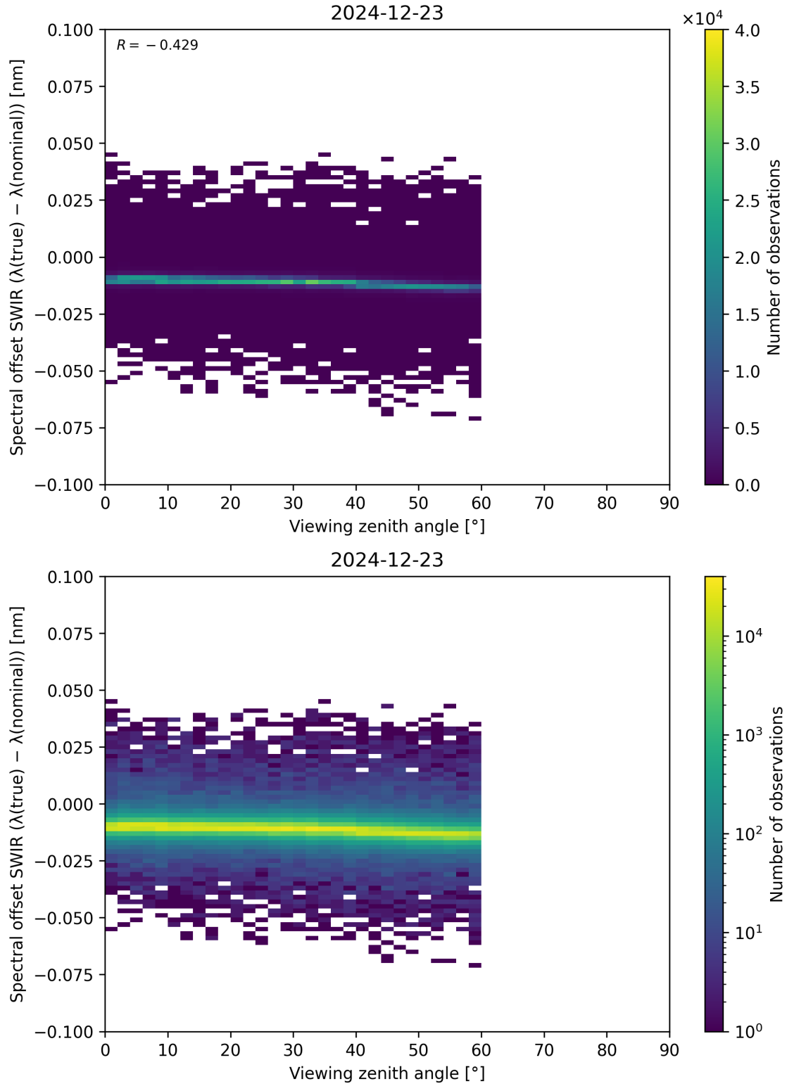
Figure 116: Scatter density plot of “Viewing zenith angle” against “Spectral offset SWIR ( \lambda_{\text{true}} - \lambda_{\text{nominal}} )” for 2024-12-22 to 2024-12-24.
