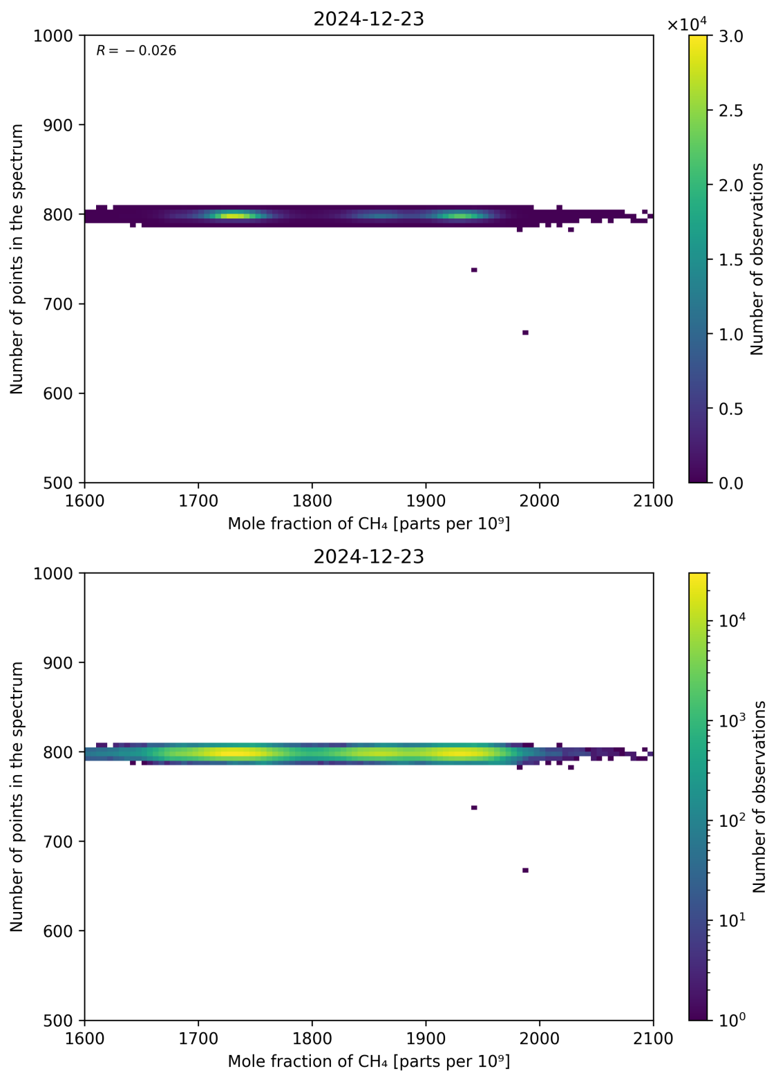
Figure 77: Scatter density plot of “Mole fraction of CH 4 ” against “Number of points in the spectrum” for 2024-12-22 to 2024-12-24.
