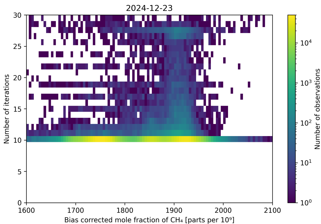
Figure 67: Scatter density plot of “Bias corrected mole fraction of CH 4 ” against “Number of iterations” for 2024-12-22 to 2024-12-24.
