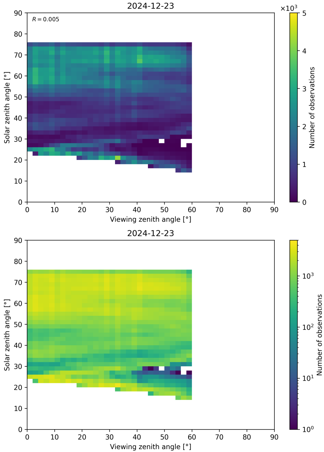
Figure 115: Scatter density plot of “Viewing zenith angle” against “Solar zenith angle” for 2024-12-22 to 2024-12-24.
