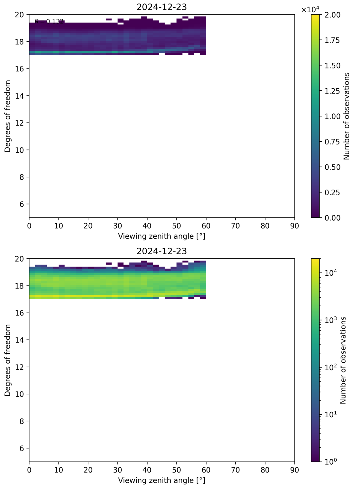
Figure 107: Scatter density plot of “Viewing zenith angle” against “Degrees of freedom” for 2024-12-22 to 2024-12-24.
