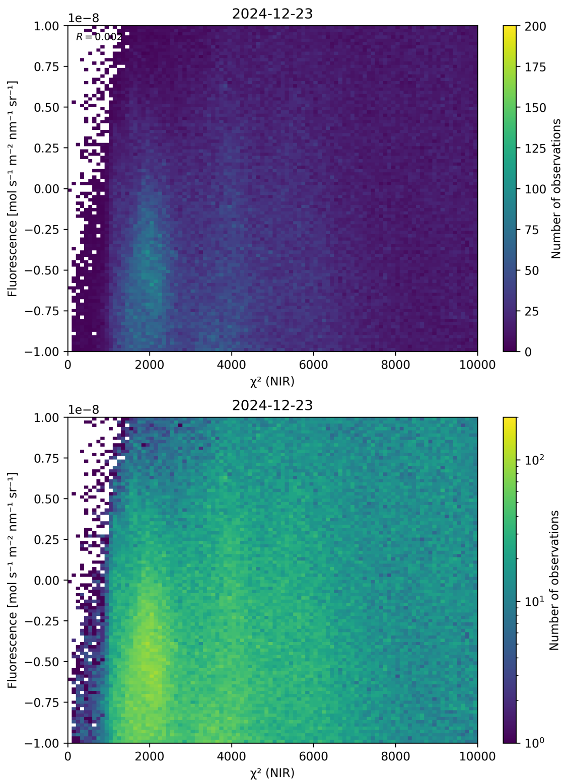
Figure 45: Scatter density plot of “ \chi^2 (NIR)” against “Fluorescence” for 2024-12-22 to 2024-12-24.
