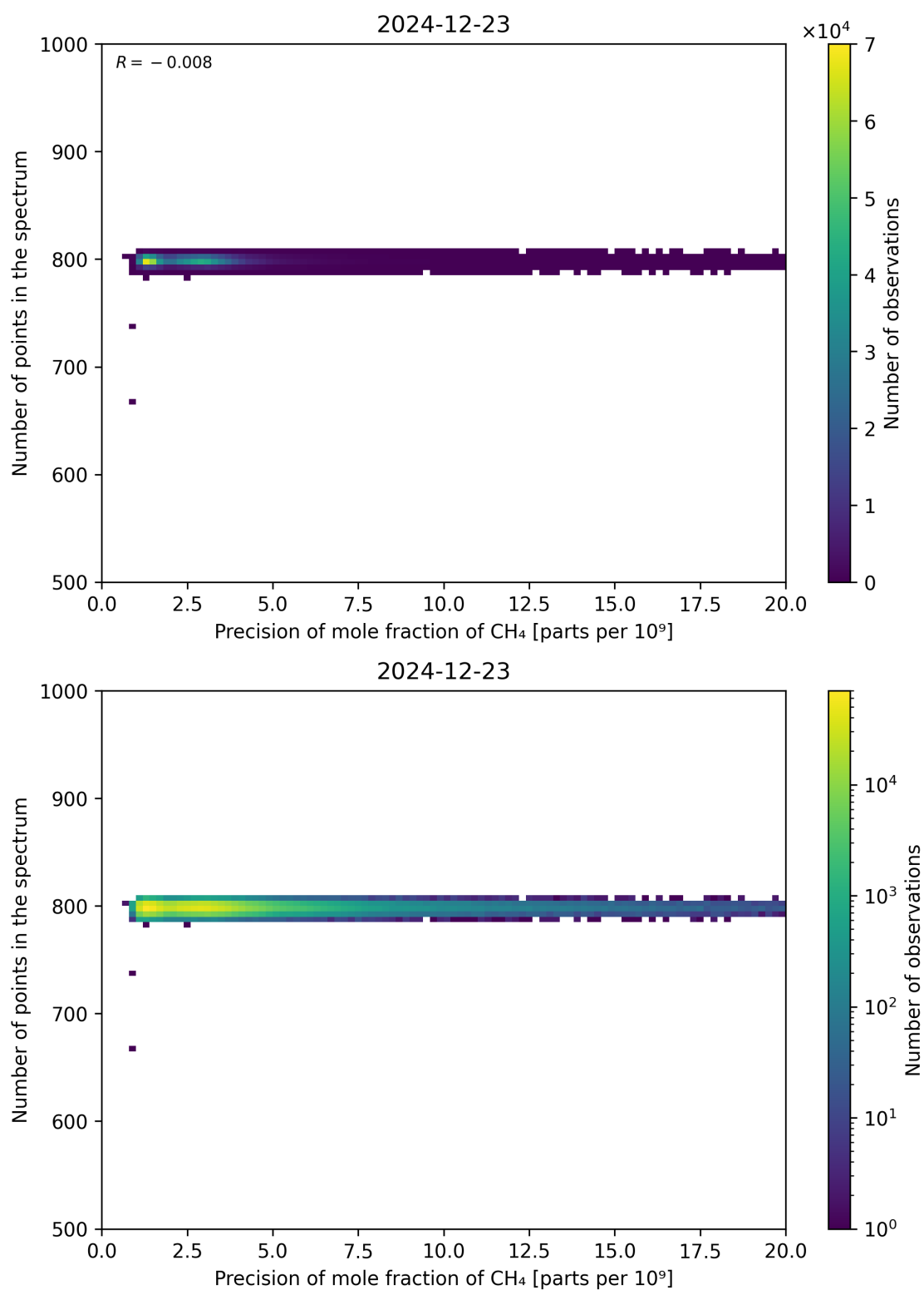
Figure 84: Scatter density plot of “Precision of mole fraction of CH 4 ” against “Number of points in the spectrum” for 2024-12-22 to 2024-12-24.
