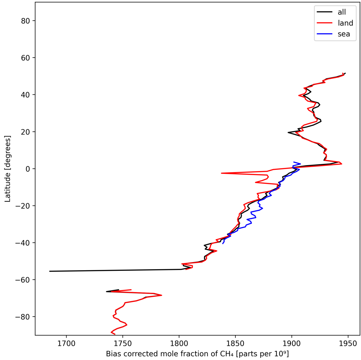
Figure 14: Zonal average of “Bias corrected mole fraction of CH 4 ” for 2024-12-22 to 2024-12-24.
