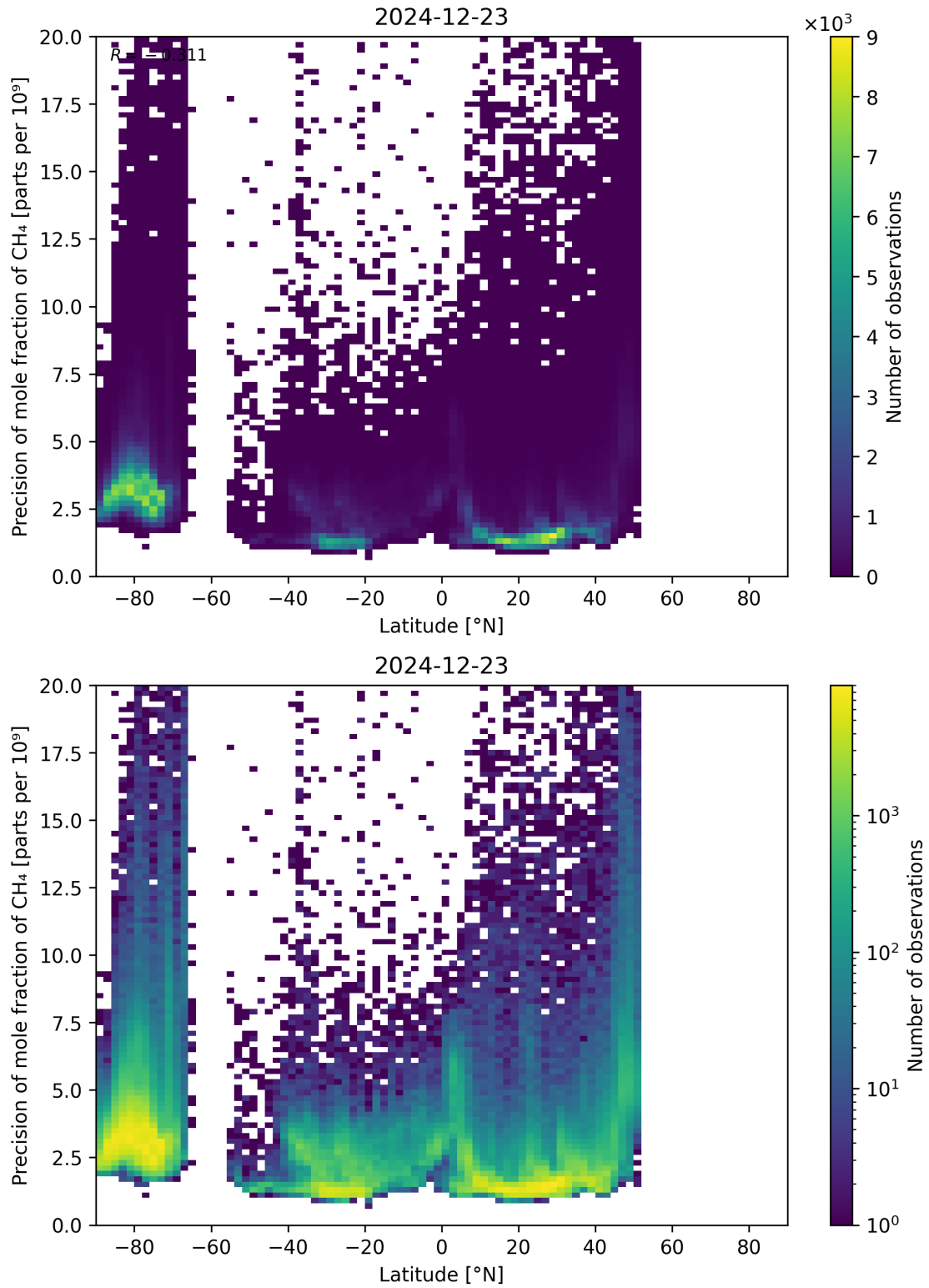
Figure 59: Scatter density plot of “Latitude” against “Precision of mole fraction of CH 4 ” for 2024-12-22 to 2024-12-24.
