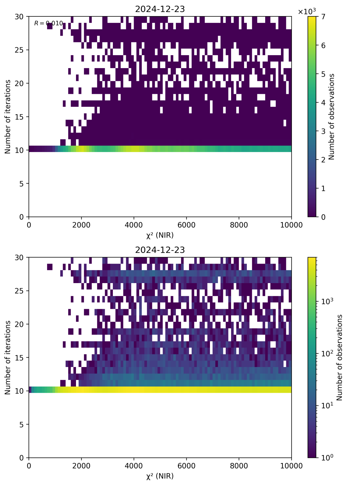
Figure 46: Scatter density plot of “ \chi^2 (NIR)” against “Number of iterations” for 2024-12-22 to 2024-12-24.
