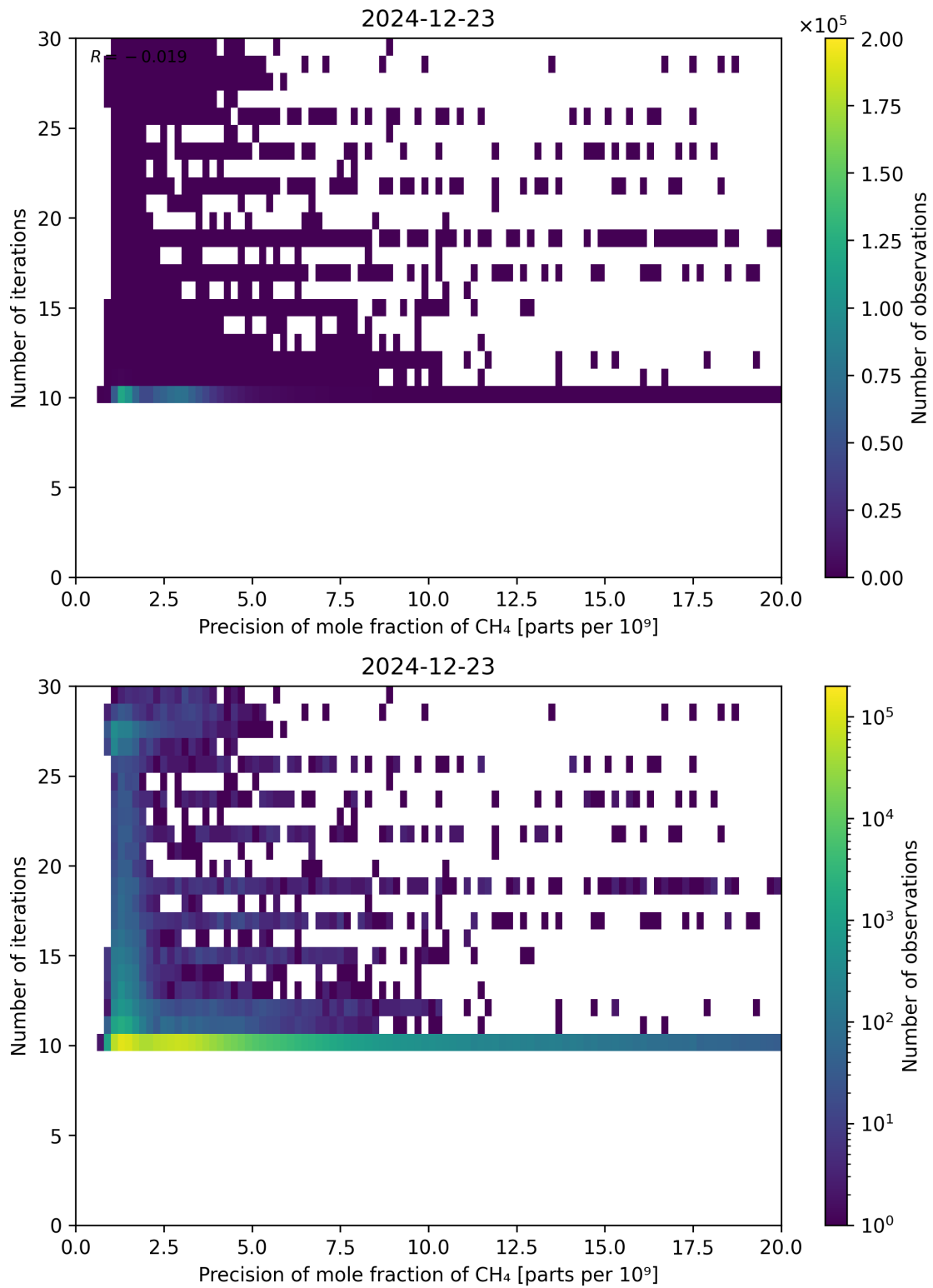
Figure 83: Scatter density plot of “Precision of mole fraction of \text{CH}_4 ” against “Number of iterations” for 2024-12-22 to 2024-12-24.
