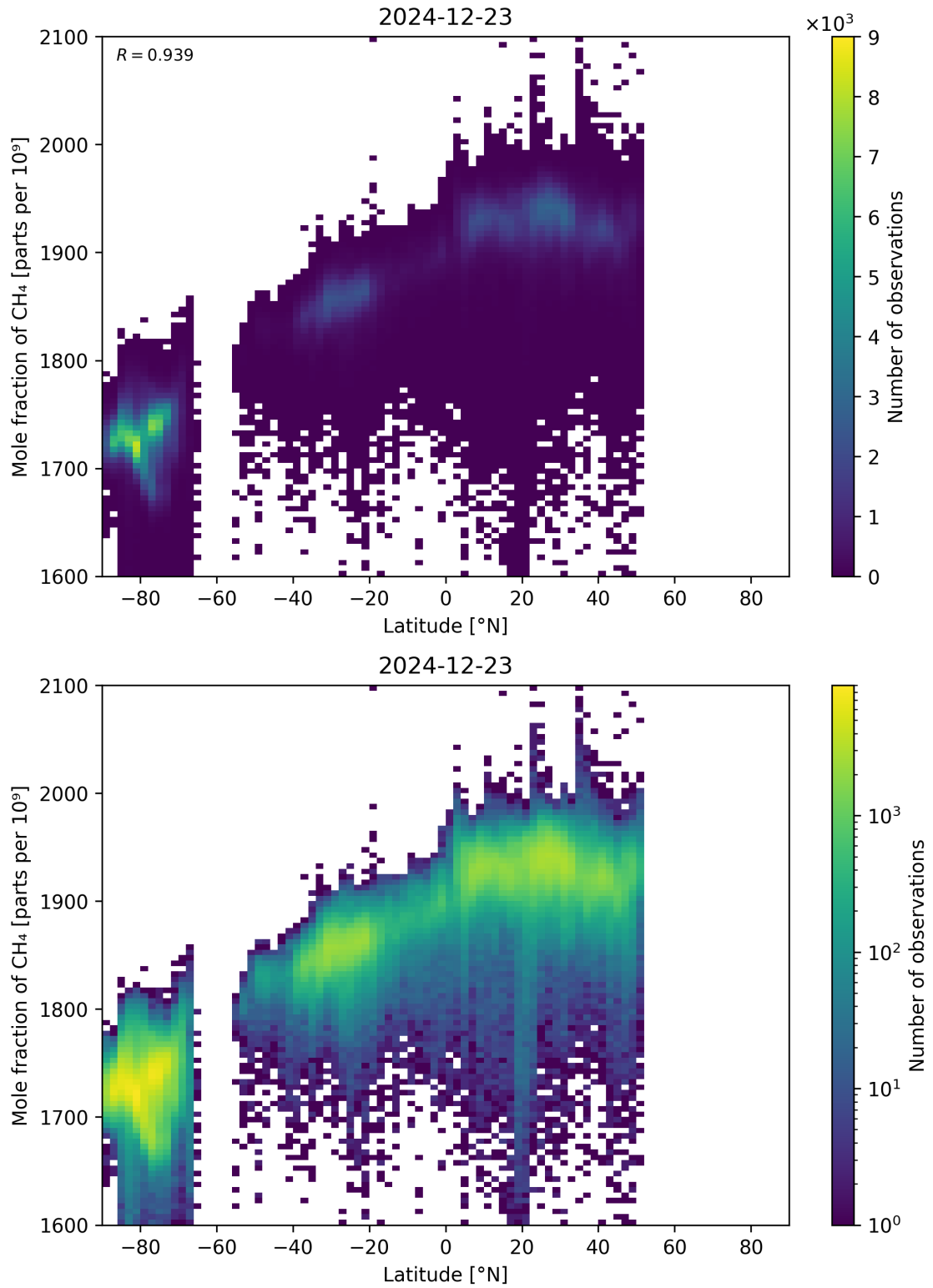
Figure 57: Scatter density plot of “Latitude” against “Mole fraction of CH 4 ” for 2024-12-22 to 2024-12-24.
