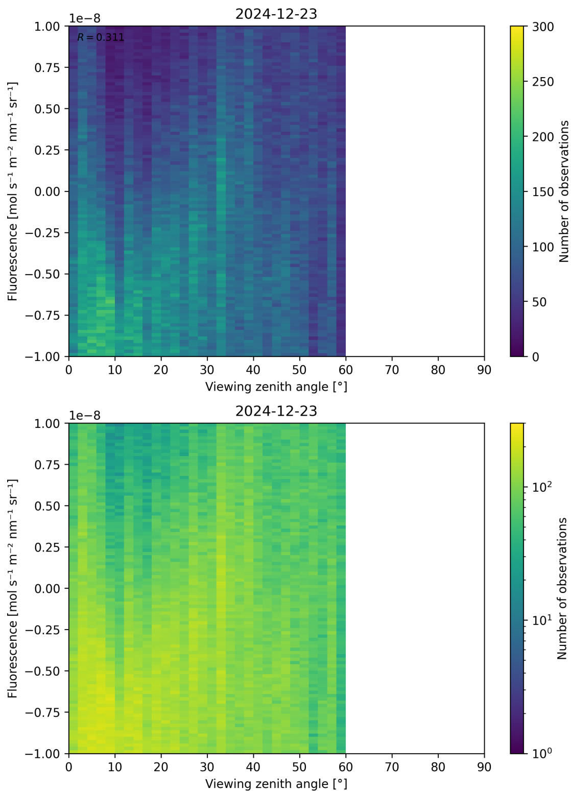
Figure 108: Scatter density plot of “Viewing zenith angle” against “Fluorescence” for 2024-12-22 to 2024-12-24.
