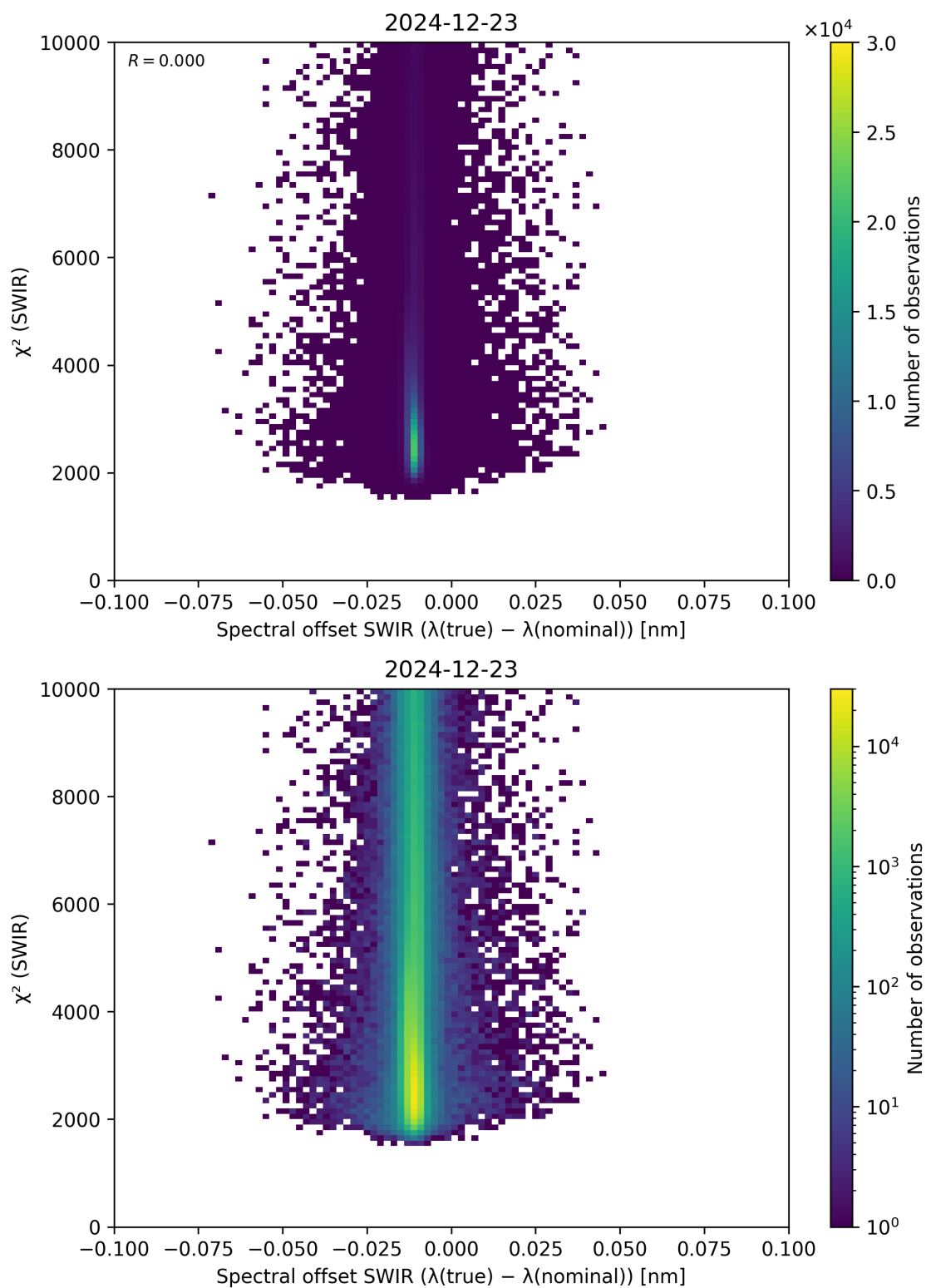
Figure 118: Scatter density plot of “Spectral offset SWIR ( \lambda_{\text{true}} - \lambda_{\text{nominal}} )” against “ \chi^2 (SWIR)” for 2024-12-22 to 2024-12-24.
