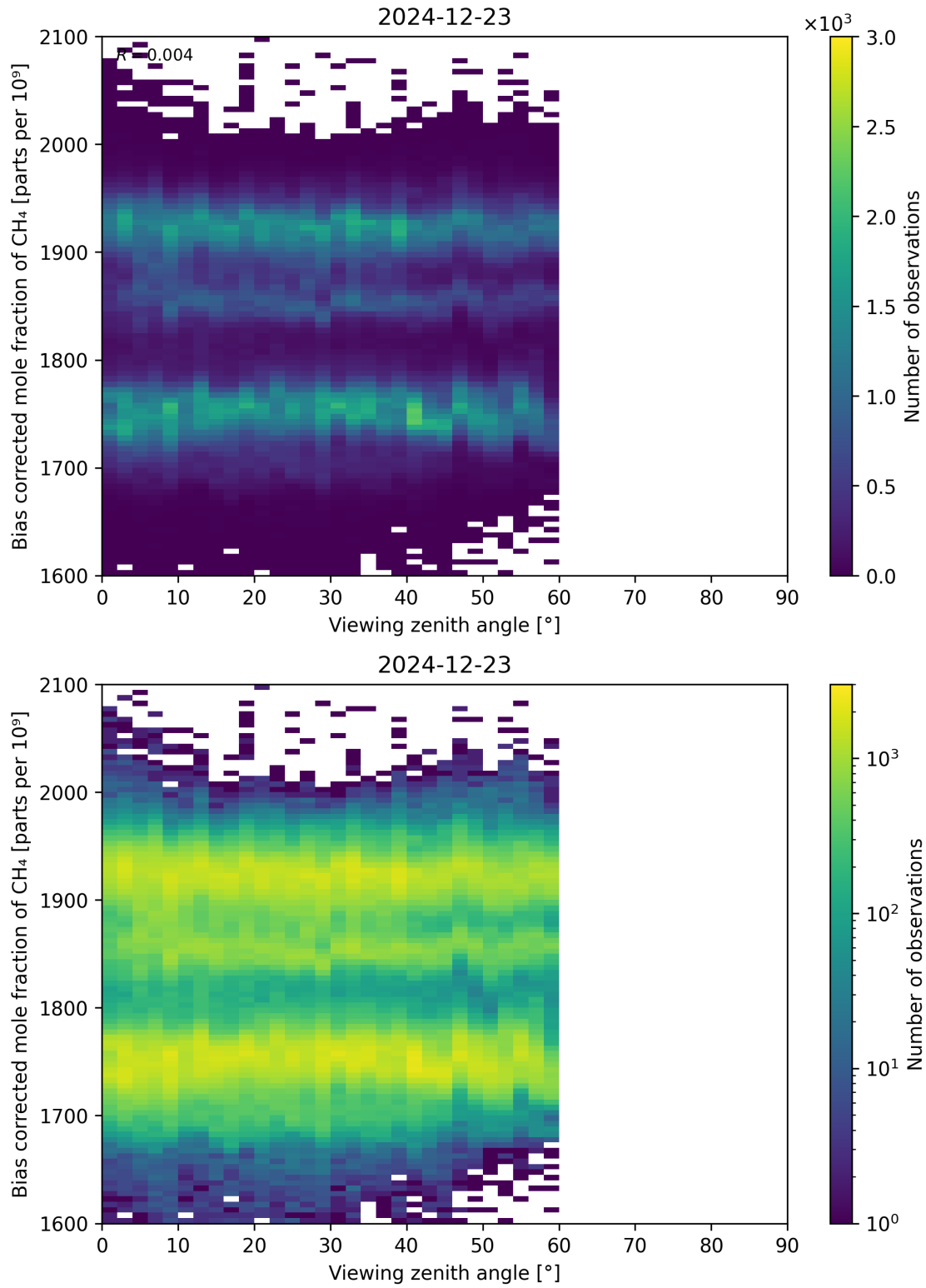
Figure 111: Scatter density plot of “Viewing zenith angle” against “Bias corrected mole fraction of CH 4 ” for 2024-12-22 to 2024-12-24.
