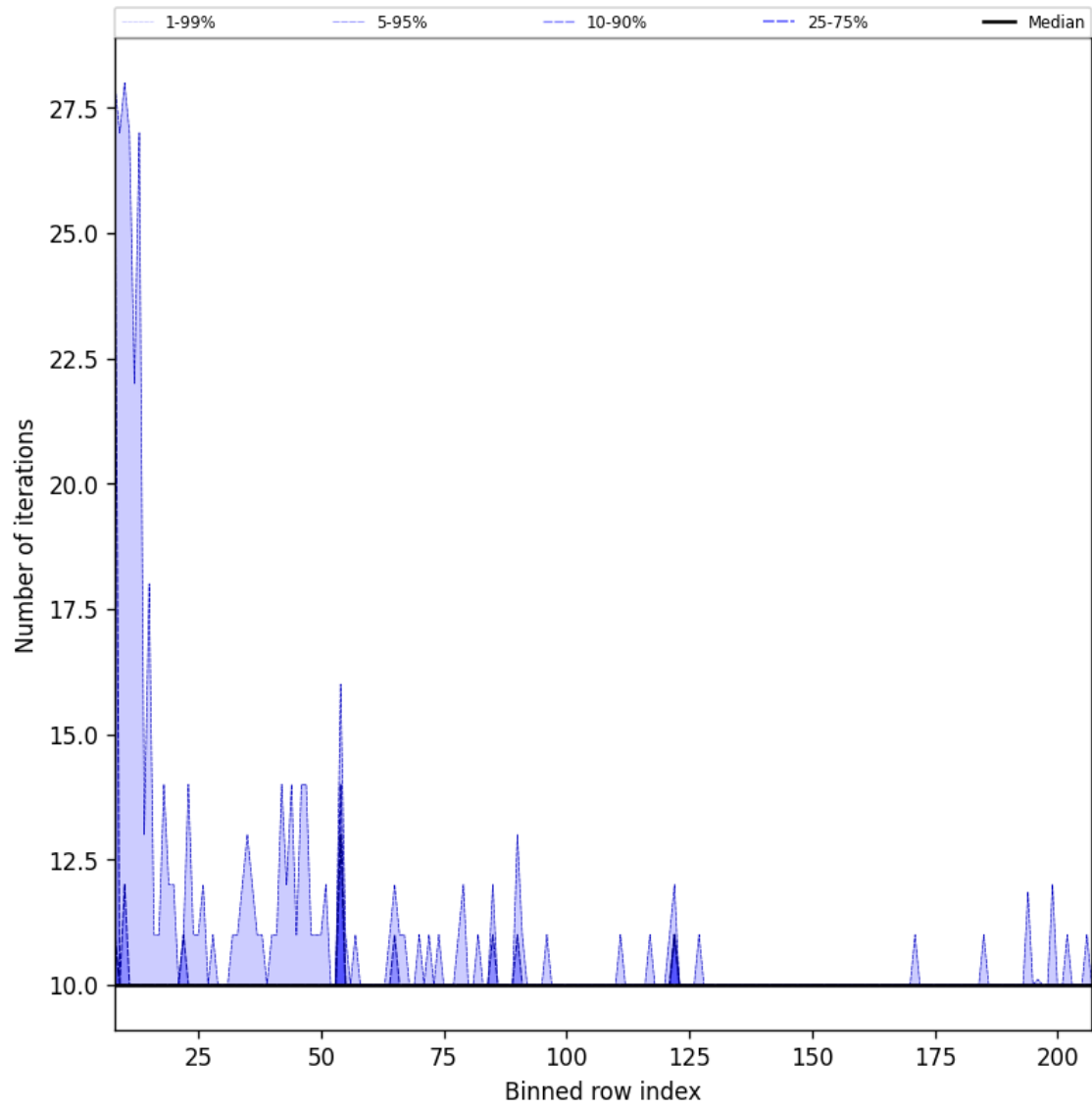
Figure 42: Along track statistics of “Number of iterations” for 2024-12-22 to 2024-12-24
