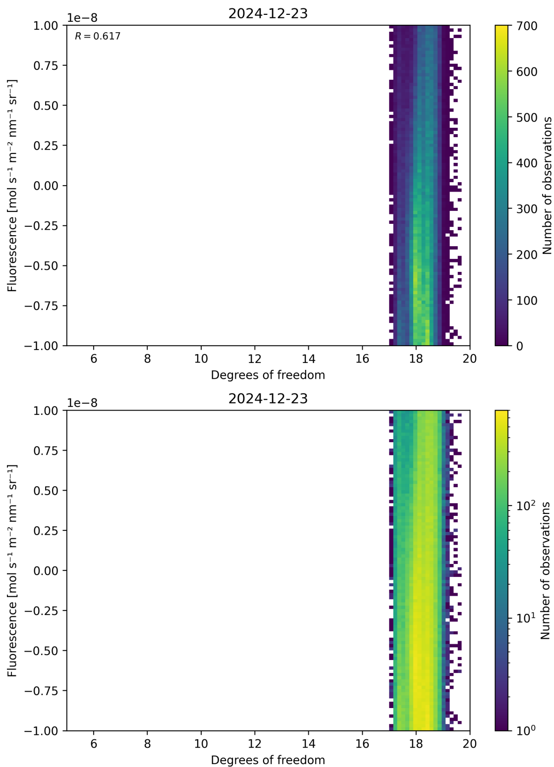
Figure 51: Scatter density plot of “Degrees of freedom” against “Fluorescence” for 2024-12-22 to 2024-12-24.
