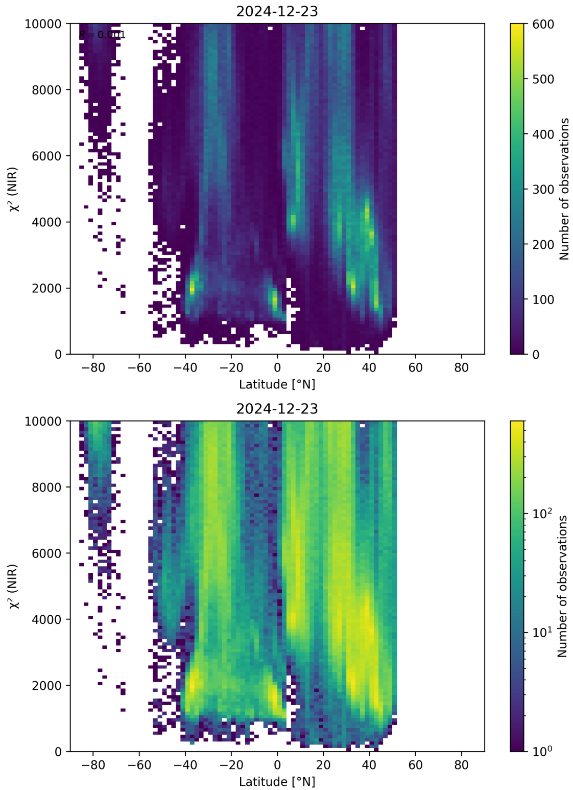
Figure 53: Scatter density plot of “Latitude” against “ \chi^2 (NIR)” for 2024-12-22 to 2024-12-24.
