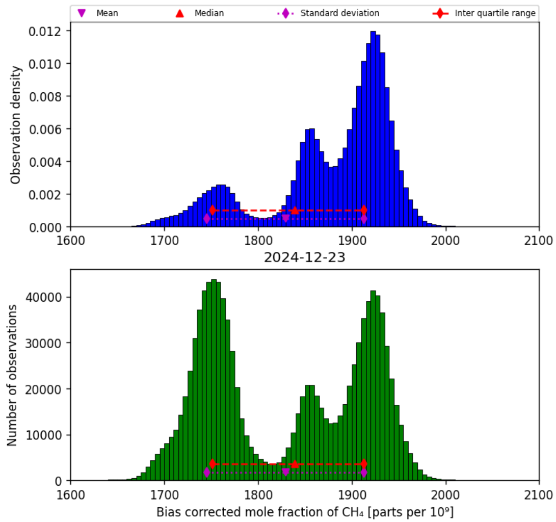
Figure 25: Histogram of “Bias corrected mole fraction of CH 4 ” for 2024-12-22 to 2024-12-24
