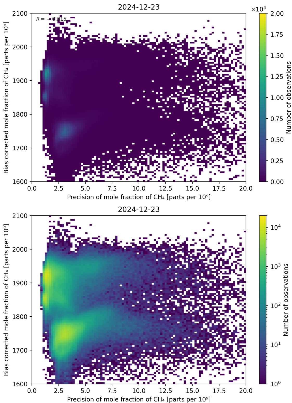
Figure 82: Scatter density plot of “Precision of mole fraction of CH 4 ” against “Bias corrected mole fraction of CH 4 ” for 2024-12-22 to 2024-12-24.
