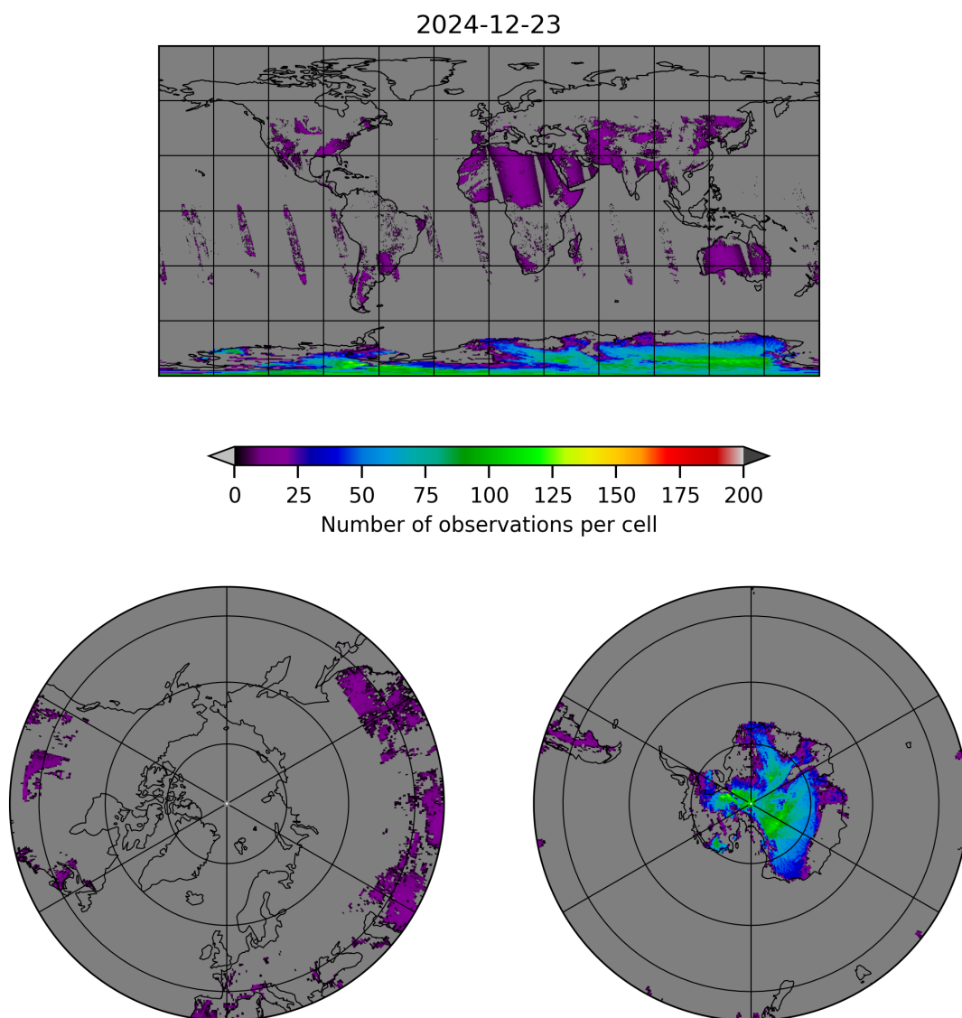
Figure 10: Map of the number of observations for 2024-12-22 to 2024-12-24
