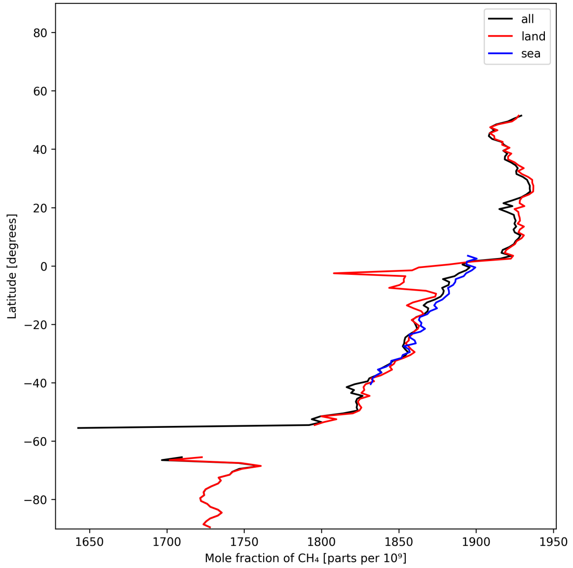
Figure 12: Zonal average of “Mole fraction of CH 4 ” for 2024-12-22 to 2024-12-24.
