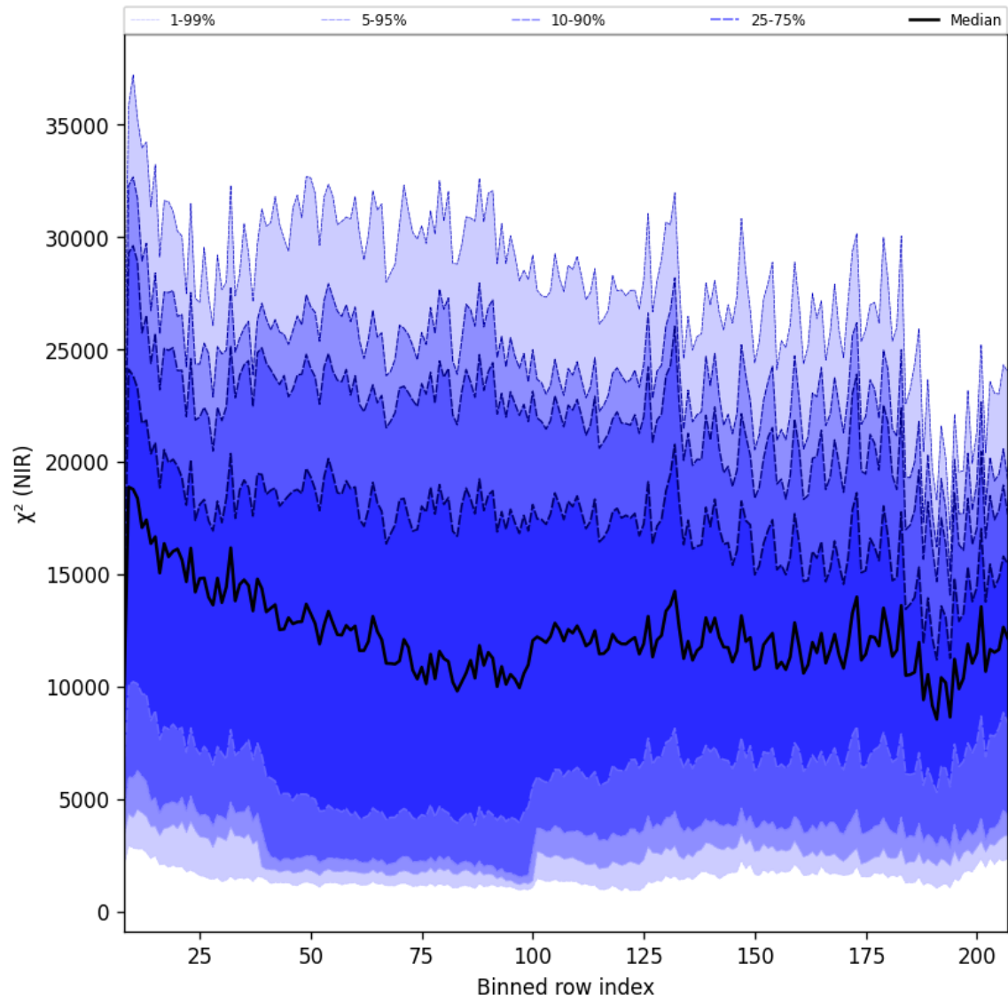
Figure 40: Along track statistics of “ \chi^2 (NIR)” for 2024-12-22 to 2024-12-24
