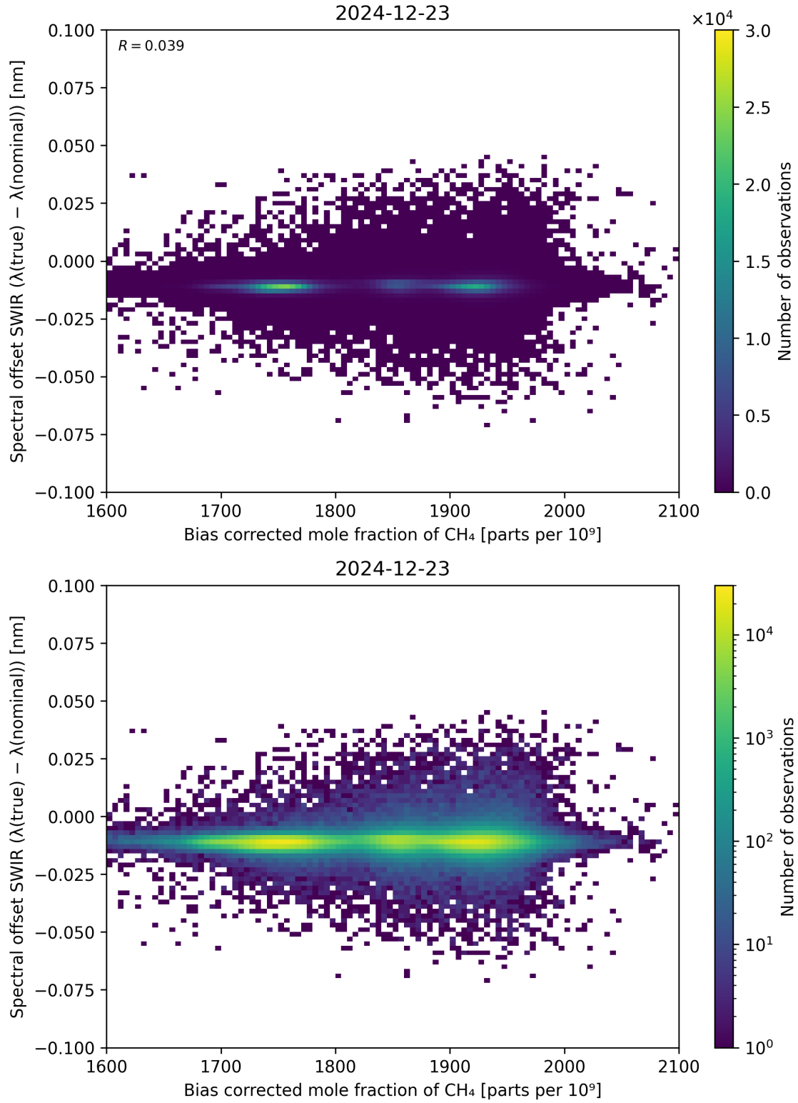
Figure 69: Scatter density plot of “Bias corrected mole fraction of \text{CH}_4 ” against “Spectral offset SWIR ( \lambda_{\text{true}} - \lambda_{\text{nominal}} )” for 2024-12-22 to 2024-12-24.
