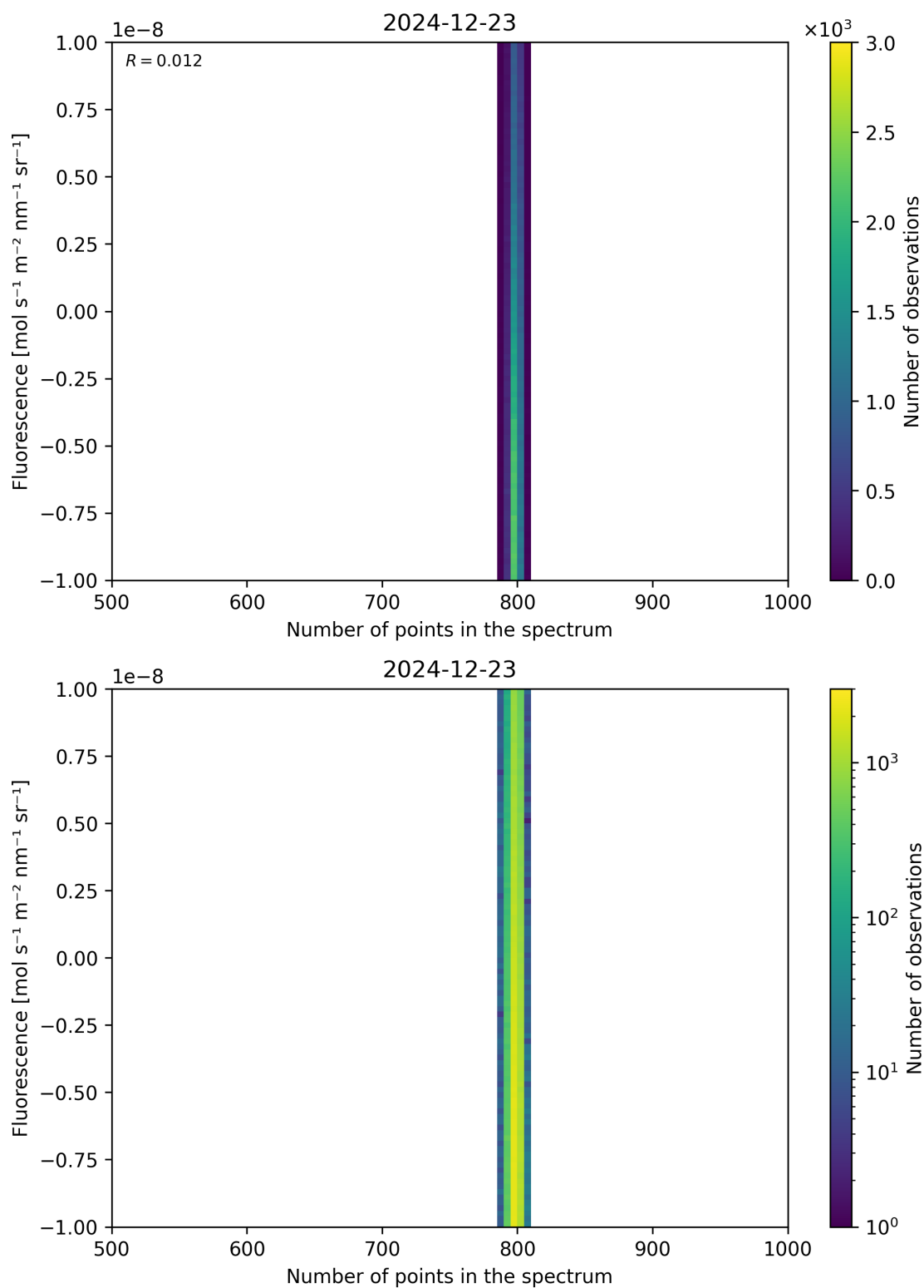
Figure 91: Scatter density plot of “Number of points in the spectrum” against “Fluorescence” for 2024-12-22 to 2024-12-24.
