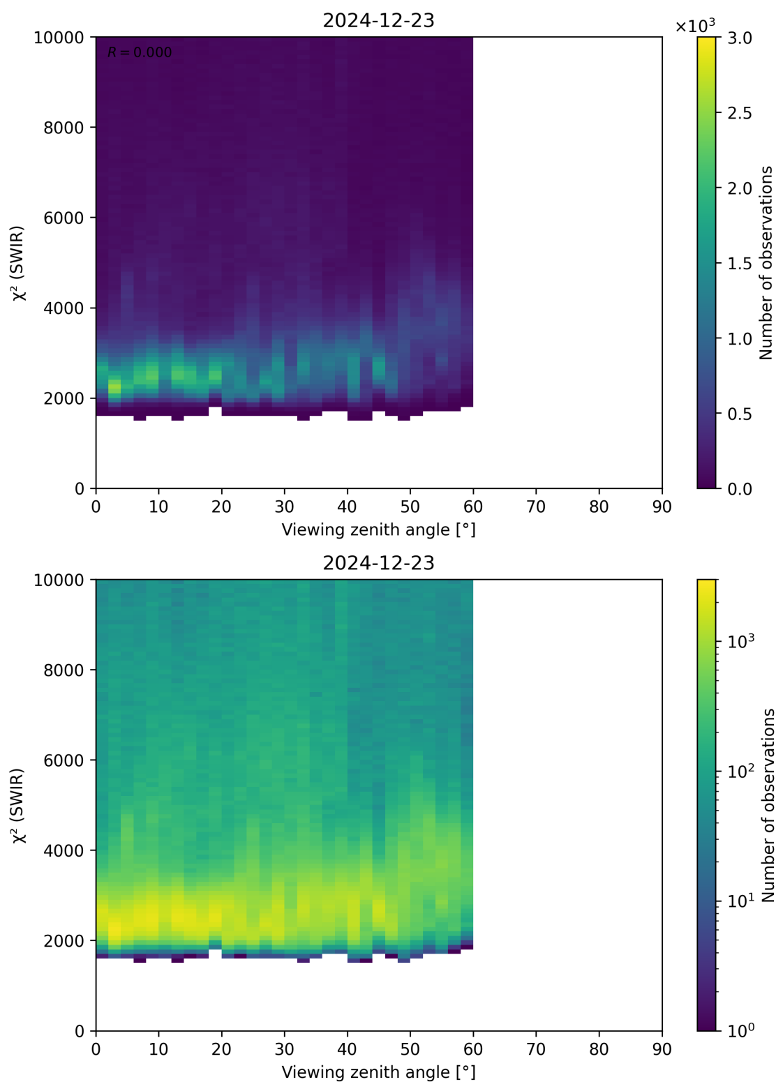
Figure 106: Scatter density plot of “Viewing zenith angle” against “ \chi^2 (SWIR)” for 2024-12-22 to 2024-12-24.
