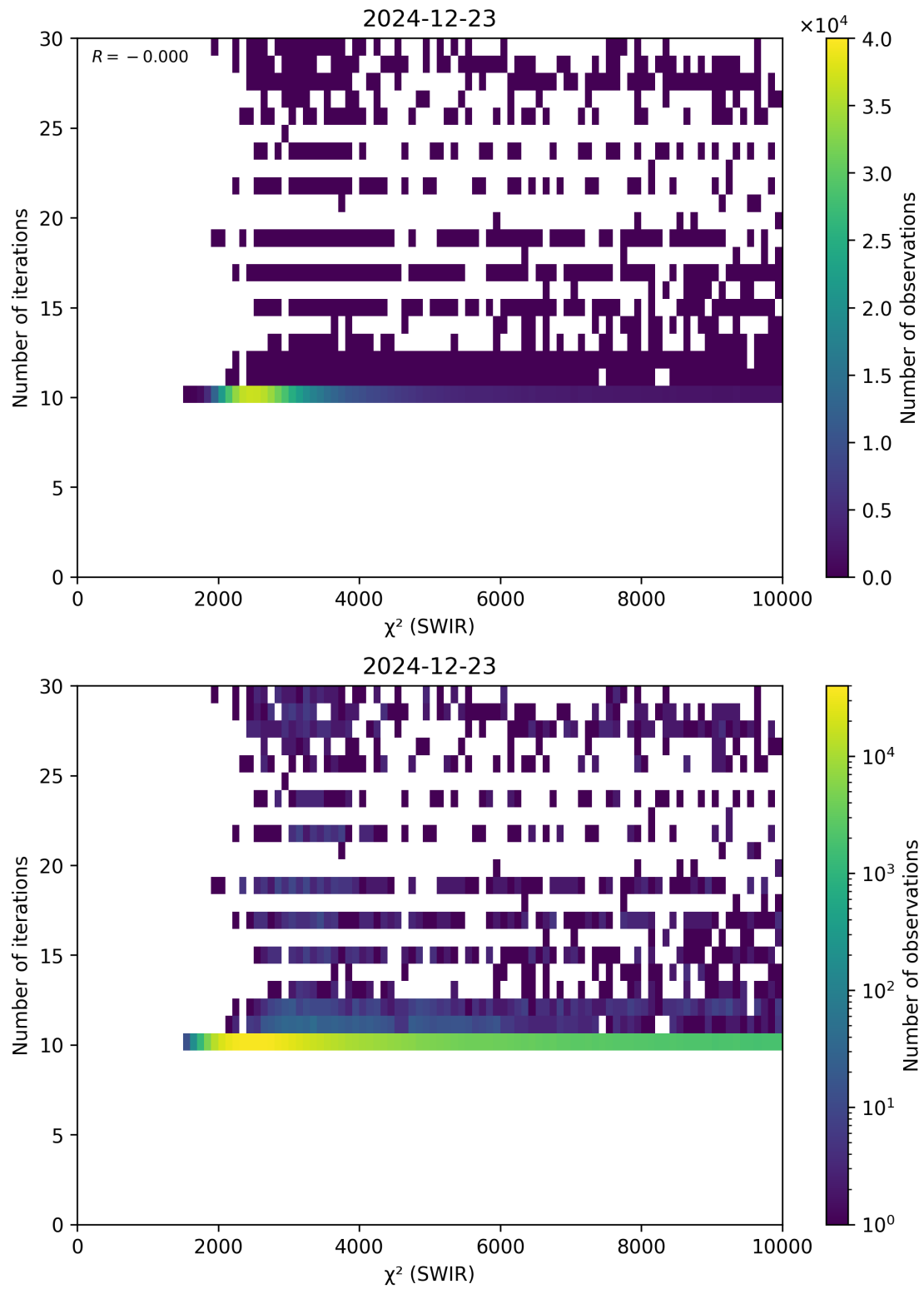
Figure 50: Scatter density plot of “ \chi^2 (SWIR)” against “Number of iterations” for 2024-12-22 to 2024-12-24.
