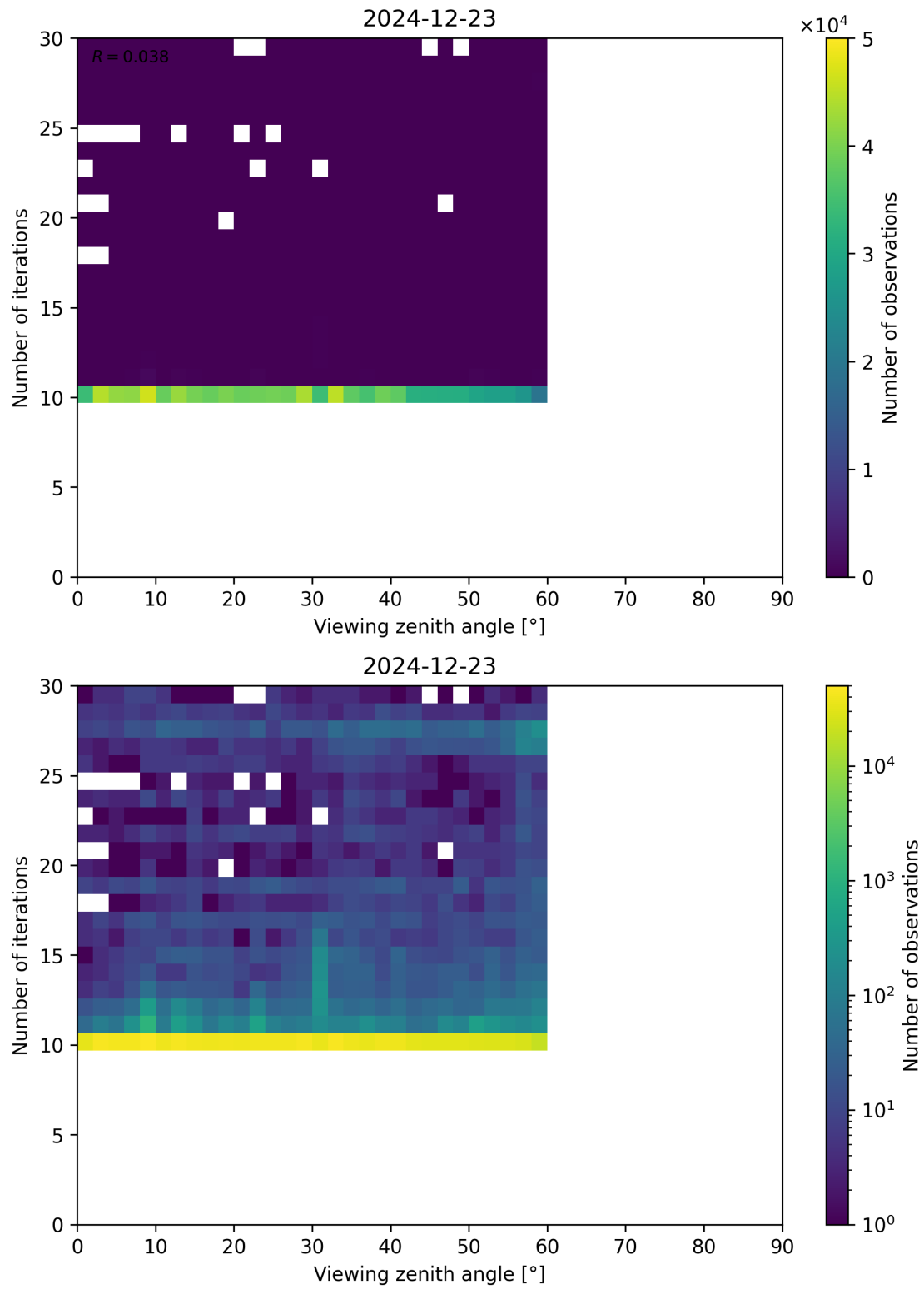
Figure 113: Scatter density plot of “Viewing zenith angle” against “Number of iterations” for 2024-12-22 to 2024-12-24.
