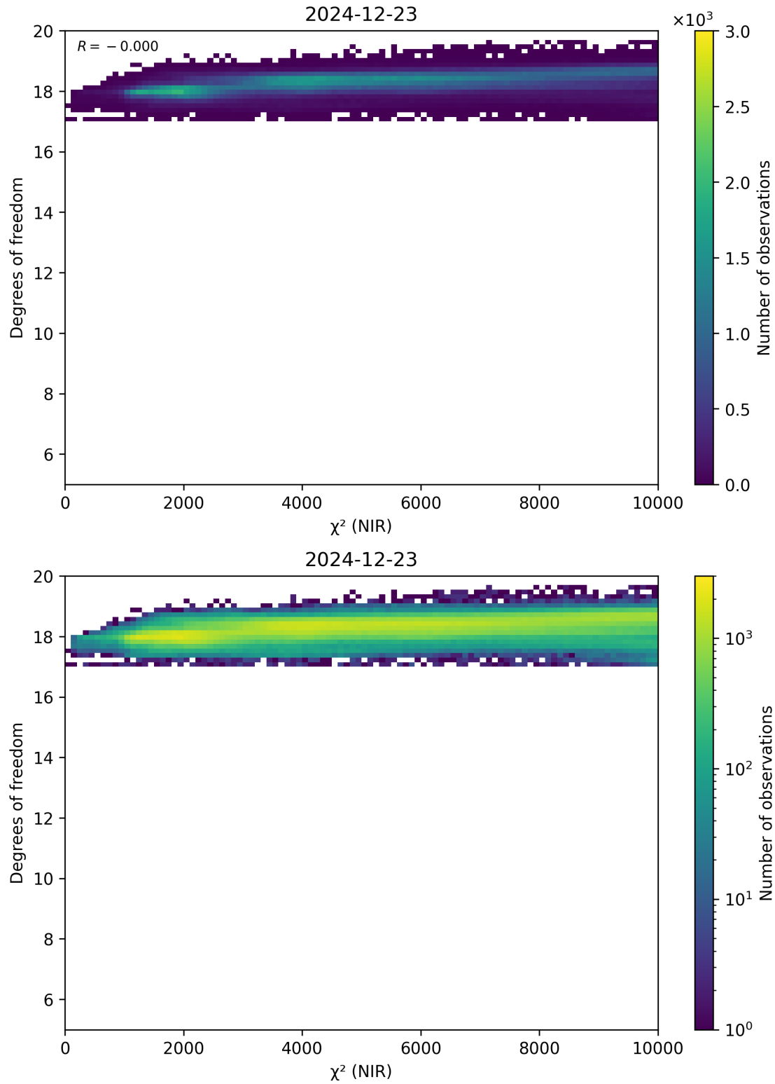
Figure 44: Scatter density plot of “ \chi^2 (NIR)” against “Degrees of freedom” for 2024-12-22 to 2024-12-24.
