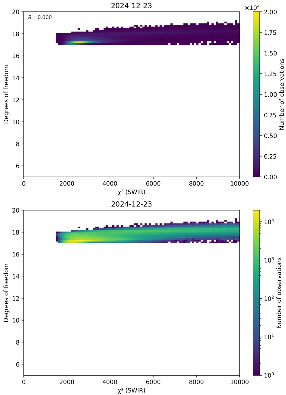
Figure 48: Scatter density plot of “ \chi^2 (SWIR)” against “Degrees of freedom” for 2024-12-22 to 2024-12-24.
