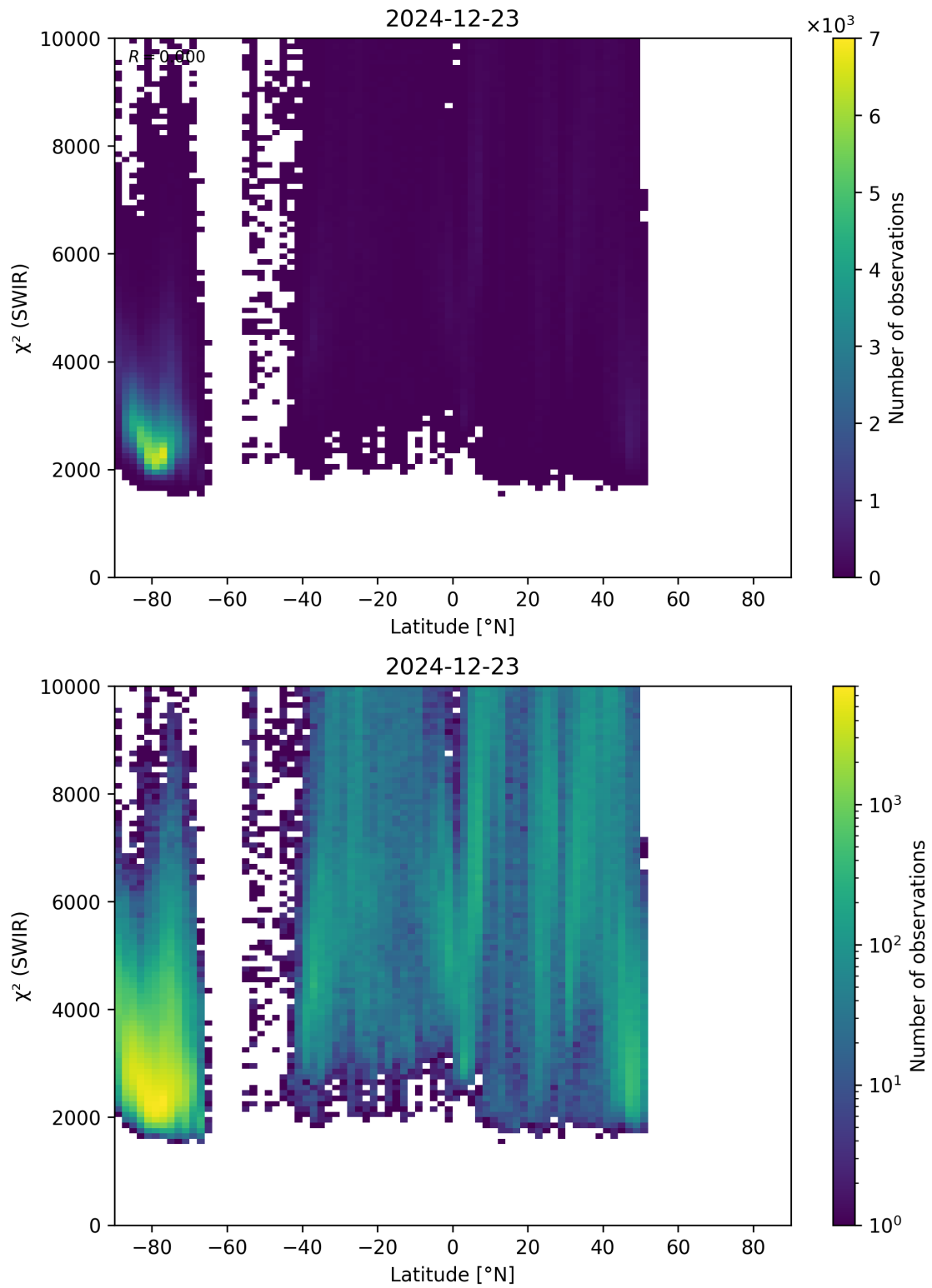
Figure 54: Scatter density plot of “Latitude” against “ \chi^2 (SWIR)” for 2024-12-22 to 2024-12-24.
