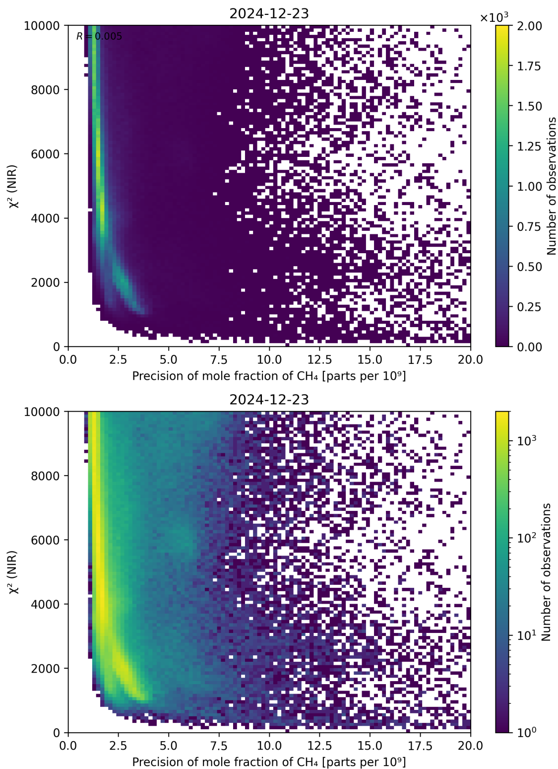
Figure 78: Scatter density plot of “Precision of mole fraction of \text{CH}_4 ” against “ \chi^2 (NIR)” for 2024-12-22 to 2024-12-24.
