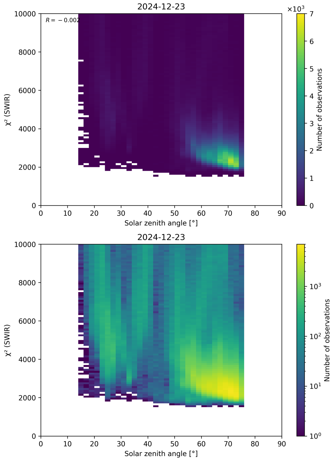
Figure 95: Scatter density plot of “Solar zenith angle” against “ \chi^2 (SWIR)” for 2024-12-22 to 2024-12-24.
