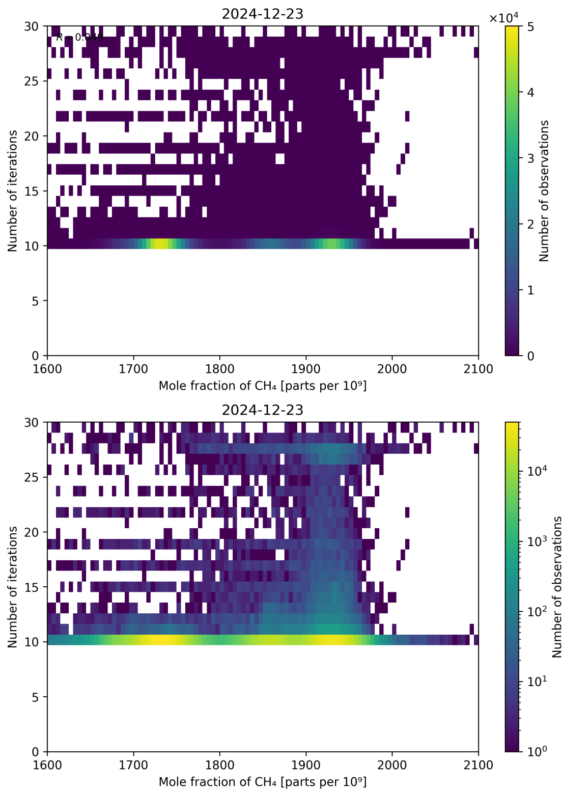
Figure 76: Scatter density plot of “Mole fraction of CH 4 ” against “Number of iterations” for 2024-12-22 to 2024-12-24.
