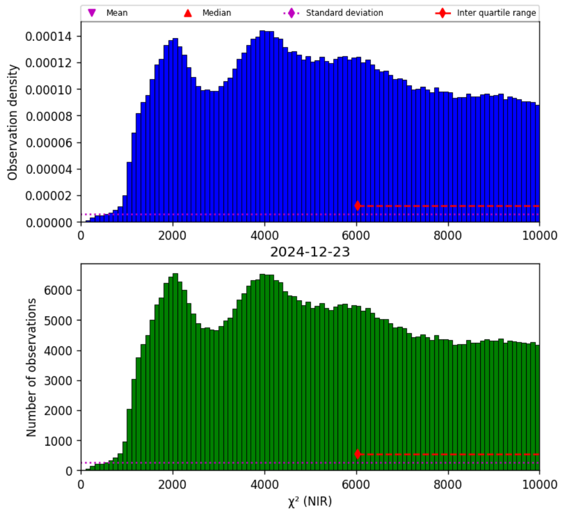
Figure 29: Histogram of “ \chi^2 (NIR)” for 2024-12-22 to 2024-12-24
