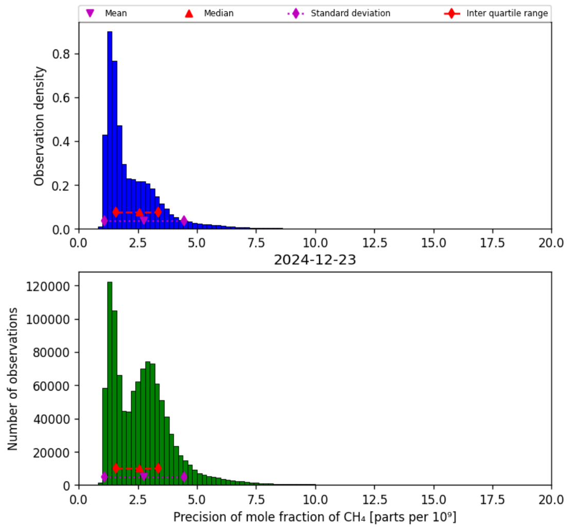
Figure 24: Histogram of “Precision of mole fraction of CH 4 ” for 2024-12-22 to 2024-12-24
