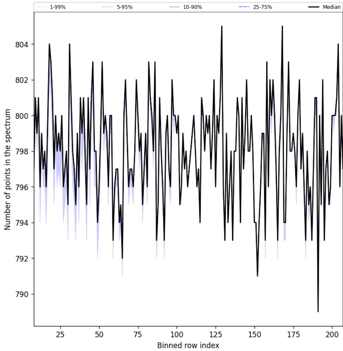
Figure 37: Along track statistics of “Number of points in the spectrum” for 2024-12-22 to 2024-12-24
