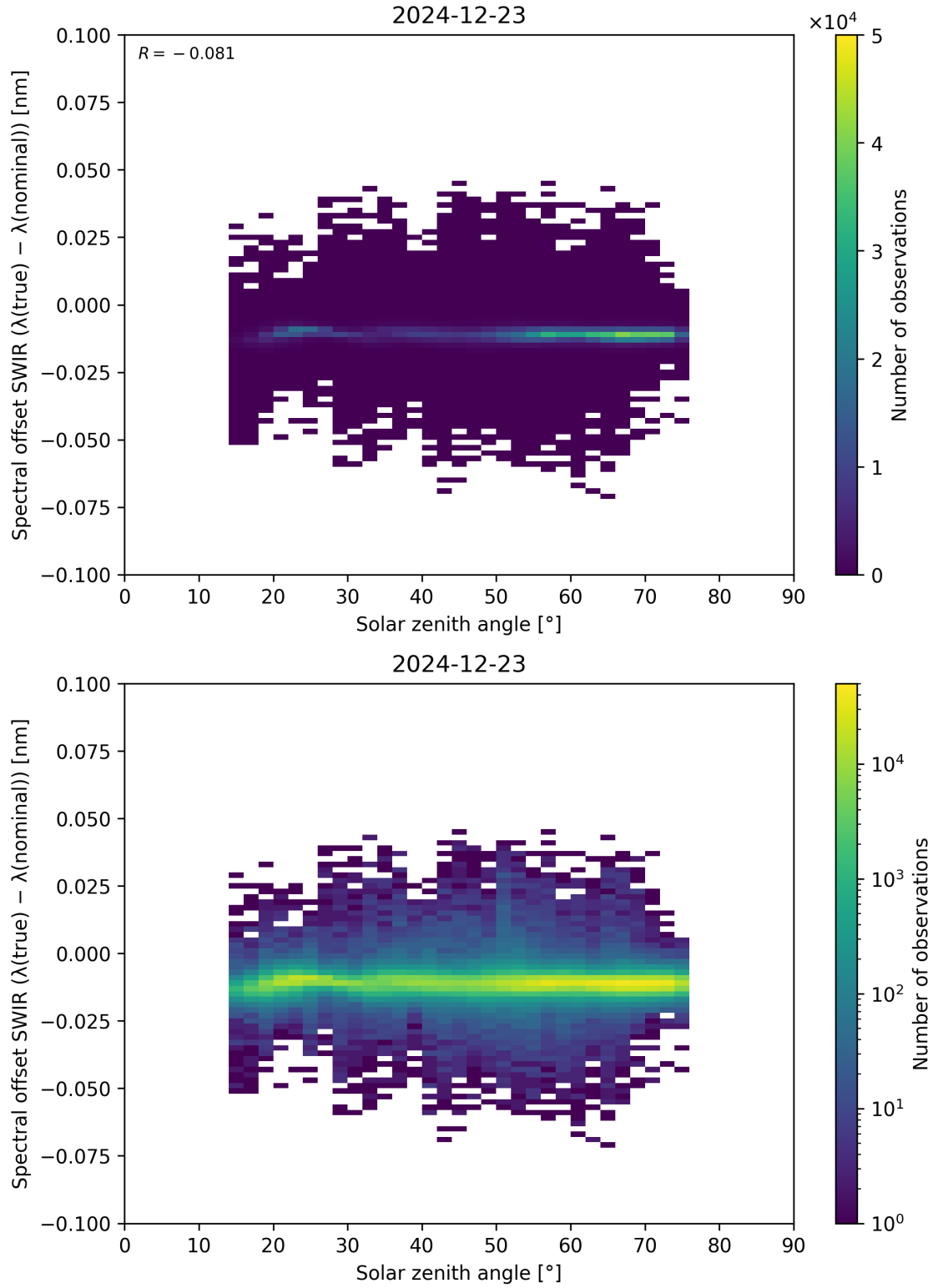
Figure 104: Scatter density plot of “Solar zenith angle” against “Spectral offset SWIR ( \lambda_{\text{true}} - \lambda_{\text{nominal}} )” for 2024-12-22 to 2024-12-24.
