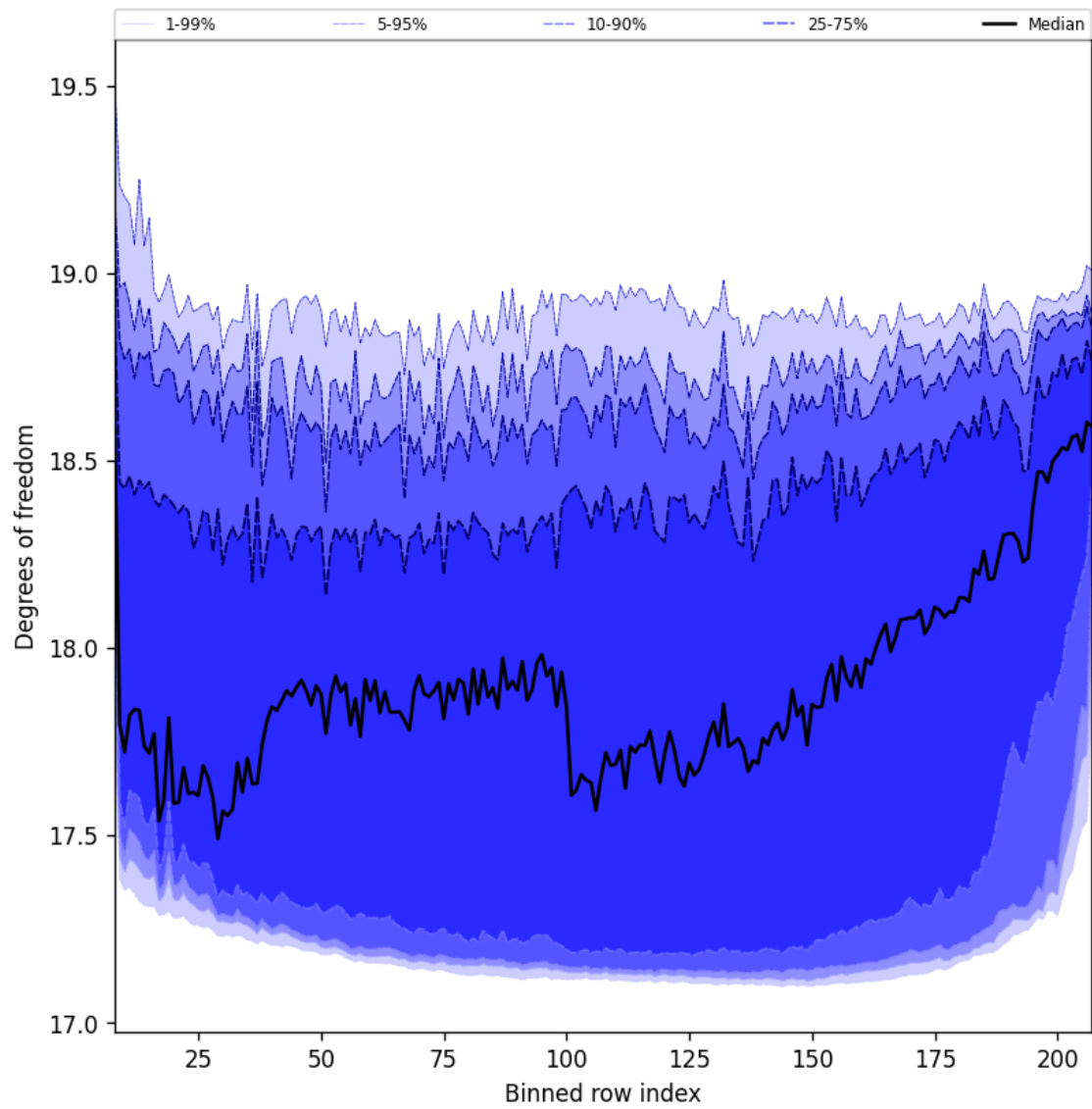
Figure 41: Along track statistics of “Degrees of freedom” for 2024-12-22 to 2024-12-24
