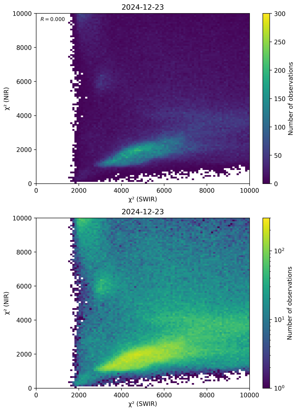
Figure 47: Scatter density plot of “ \chi^2 (SWIR)” against “ \chi^2 (NIR)” for 2024-12-22 to 2024-12-24.
