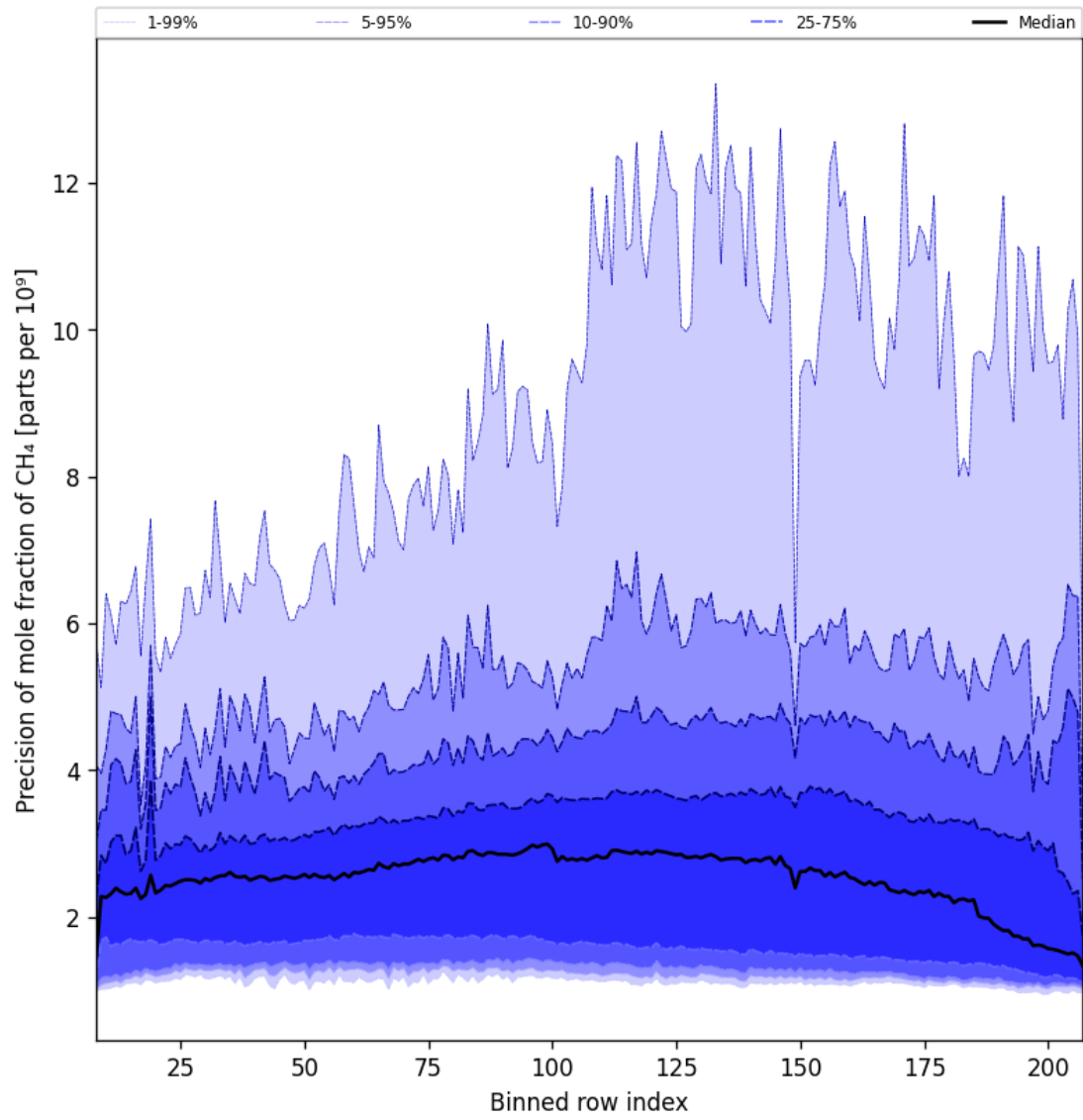
Figure 35: Along track statistics of “Precision of mole fraction of CH 4 ” for 2024-12-22 to 2024-12-24
