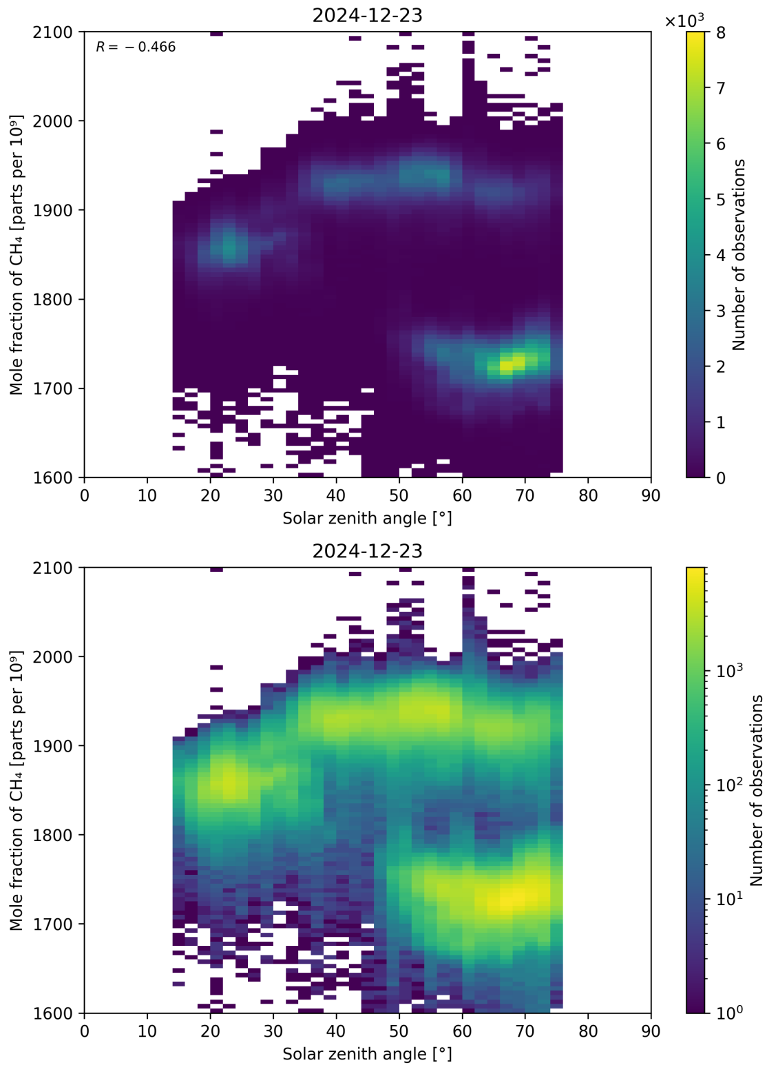
Figure 99: Scatter density plot of “Solar zenith angle” against “Mole fraction of CH 4 ” for 2024-12-22 to 2024-12-24.
