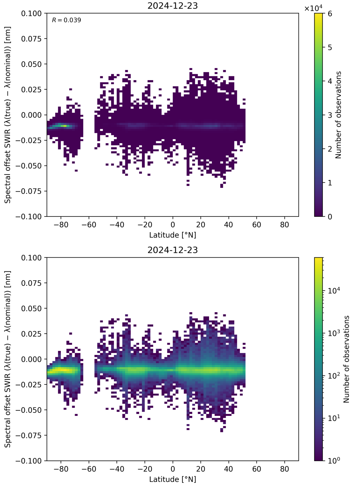
Figure 62: Scatter density plot of “Latitude” against “Spectral offset SWIR ( \lambda_{\text{true}} - \lambda_{\text{nominal}} )” for 2024-12-22 to 2024-12-24.
