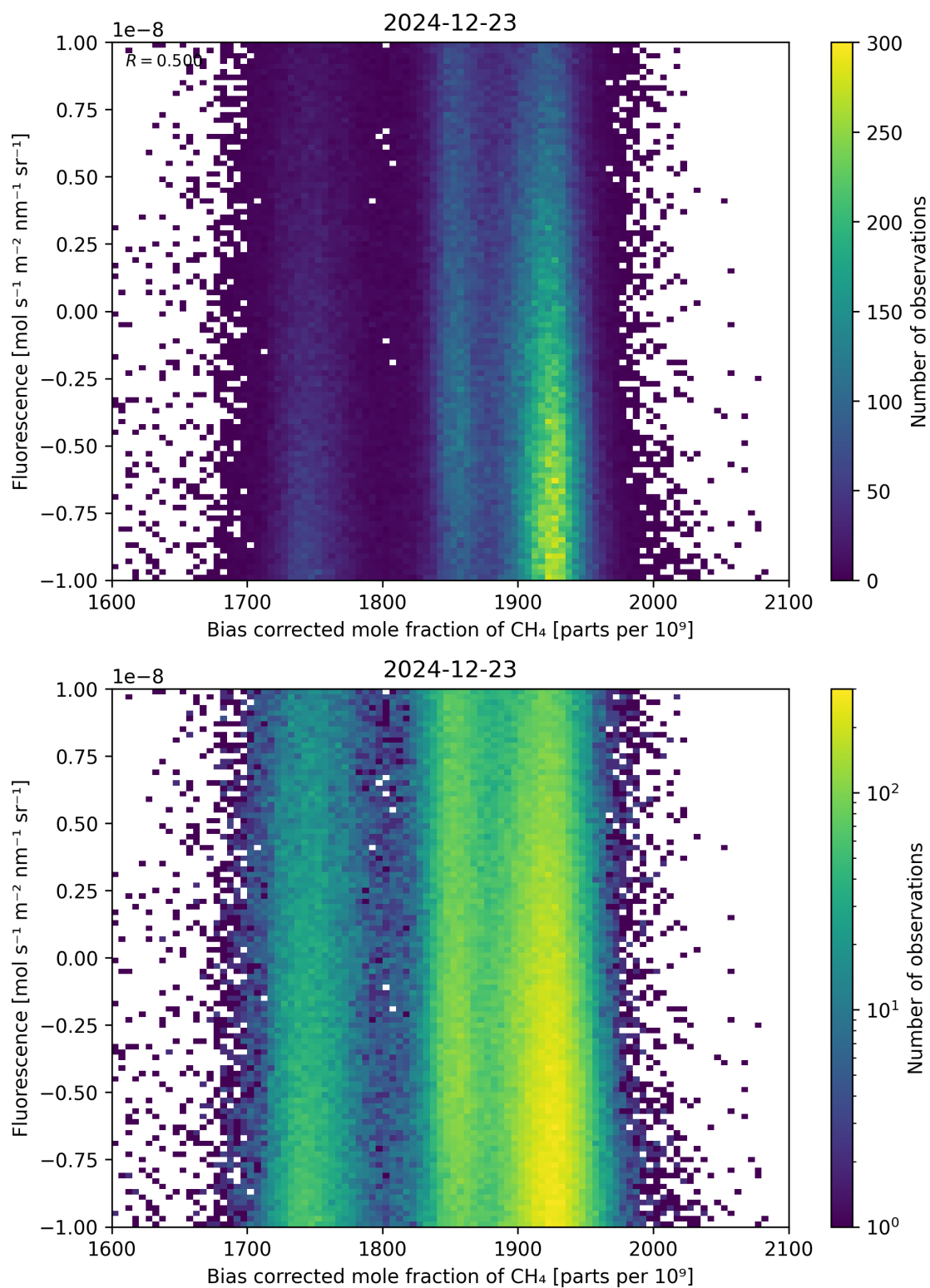
Figure 66: Scatter density plot of “Bias corrected mole fraction of \text{CH}_4 ” against “Fluorescence” for 2024-12-22 to 2024-12-24.
