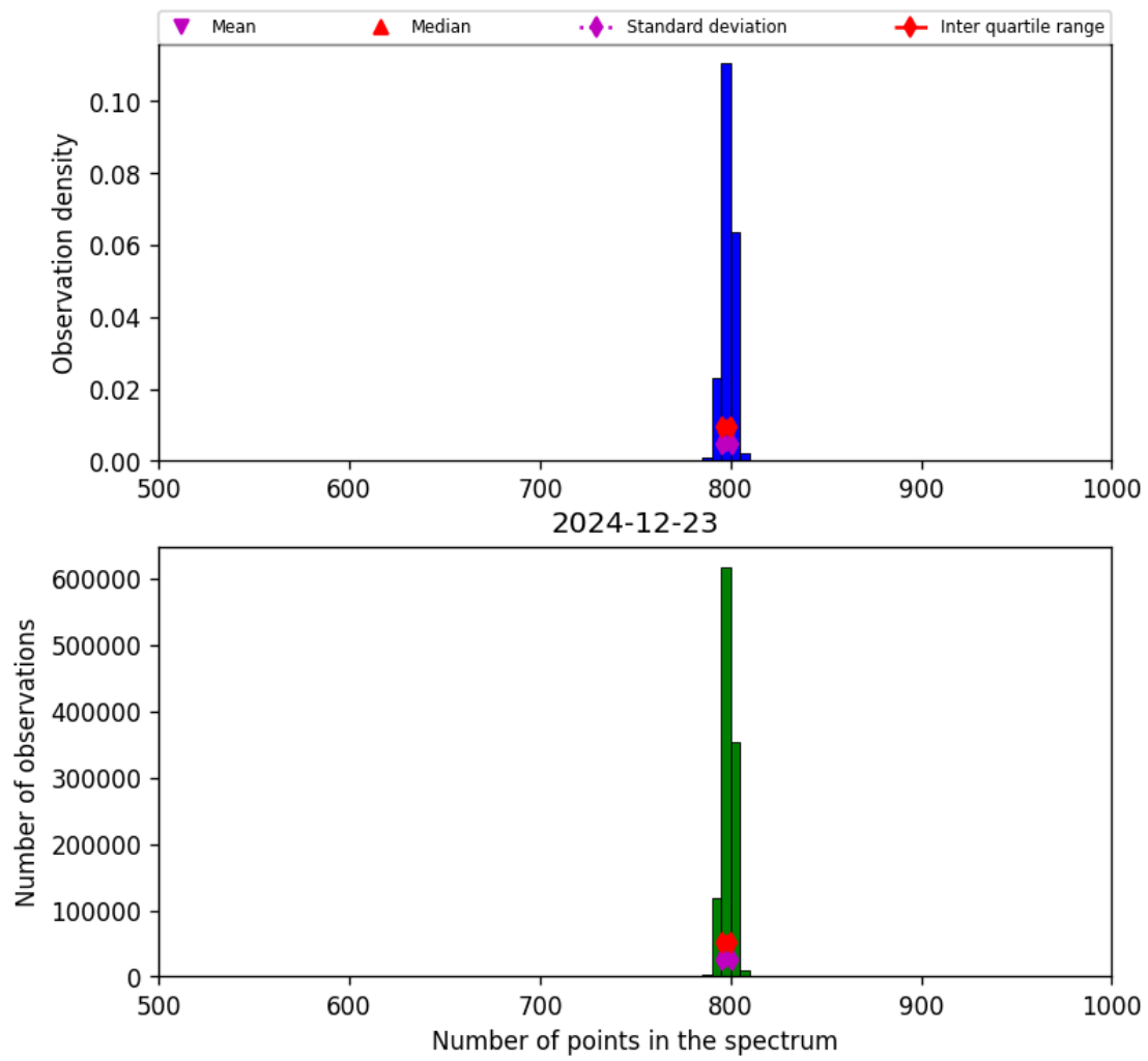
Figure 26: Histogram of “Number of points in the spectrum” for 2024-12-22 to 2024-12-24
