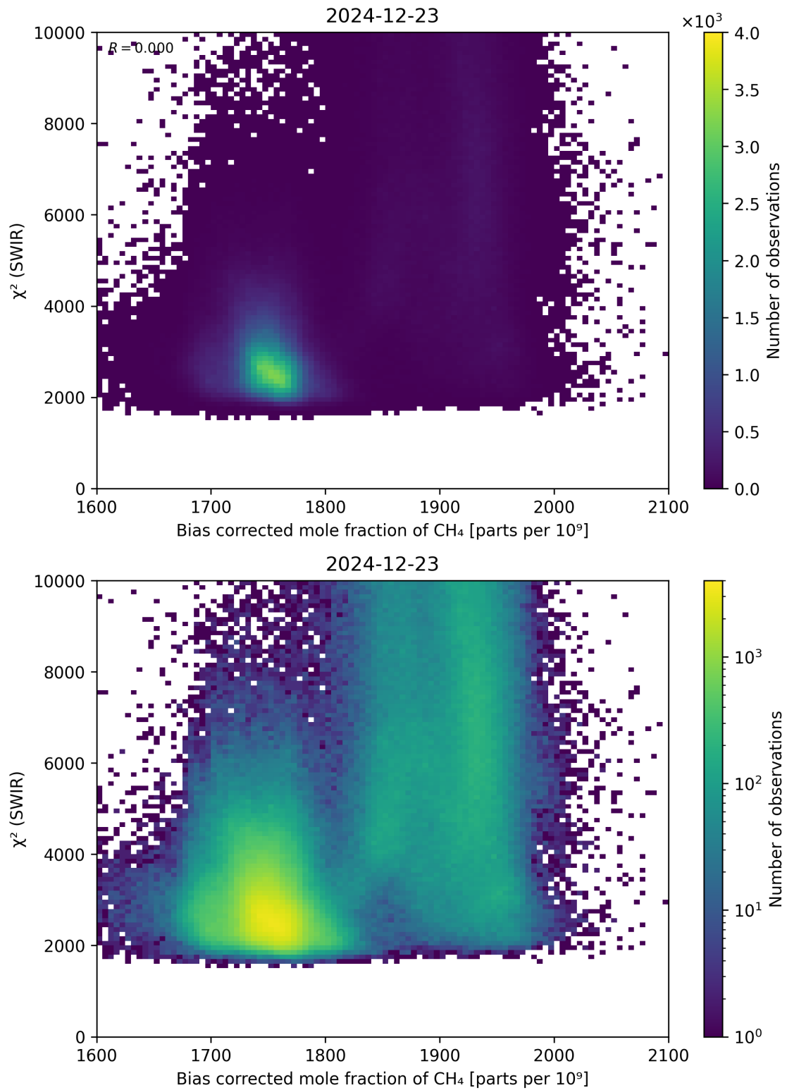
Figure 64: Scatter density plot of “Bias corrected mole fraction of \text{CH}_4 ” against “ \chi^2 (SWIR)” for 2024-12-22 to 2024-12-24.
