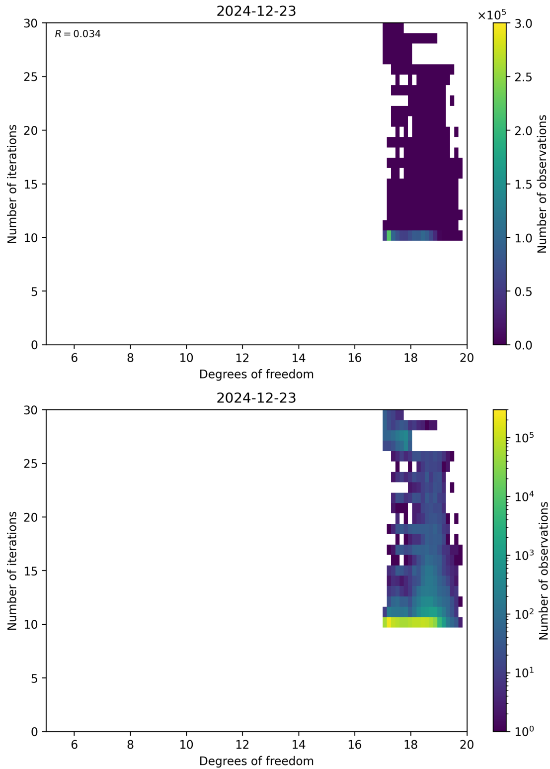
Figure 52: Scatter density plot of “Degrees of freedom” against “Number of iterations” for 2024-12-22 to 2024-12-24.
