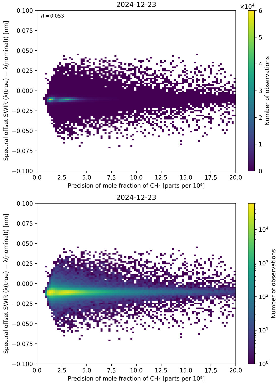
Figure 85: Scatter density plot of “Precision of mole fraction of CH 4 ” against “Spectral offset SWIR ( \lambda_{\text{true}} - \lambda_{\text{nominal}} )” for 2024-12-22 to 2024-12-24.
