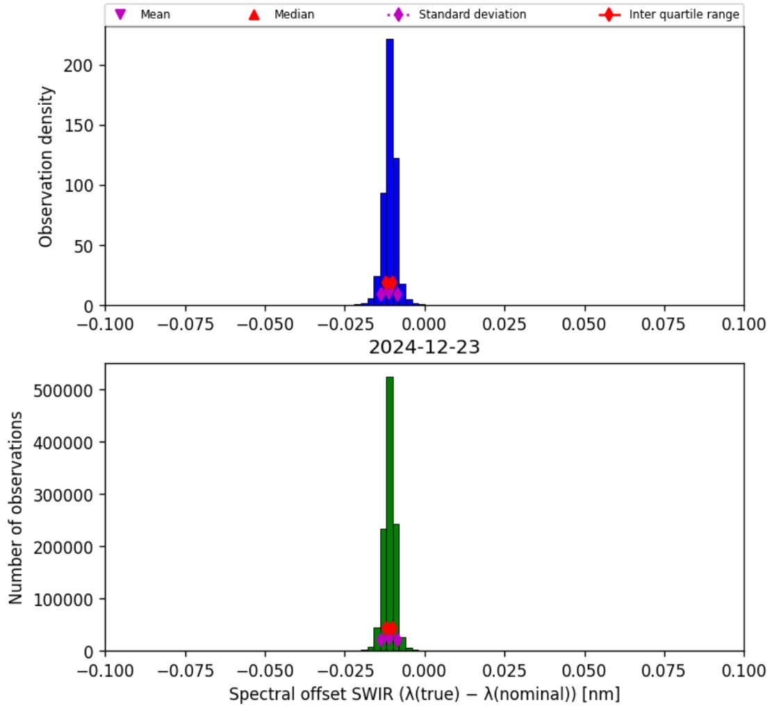
Figure 27: Histogram of “Spectral offset SWIR ( \lambda_{\text{true}} - \lambda_{\text{nominal}} )” for 2024-12-22 to 2024-12-24
