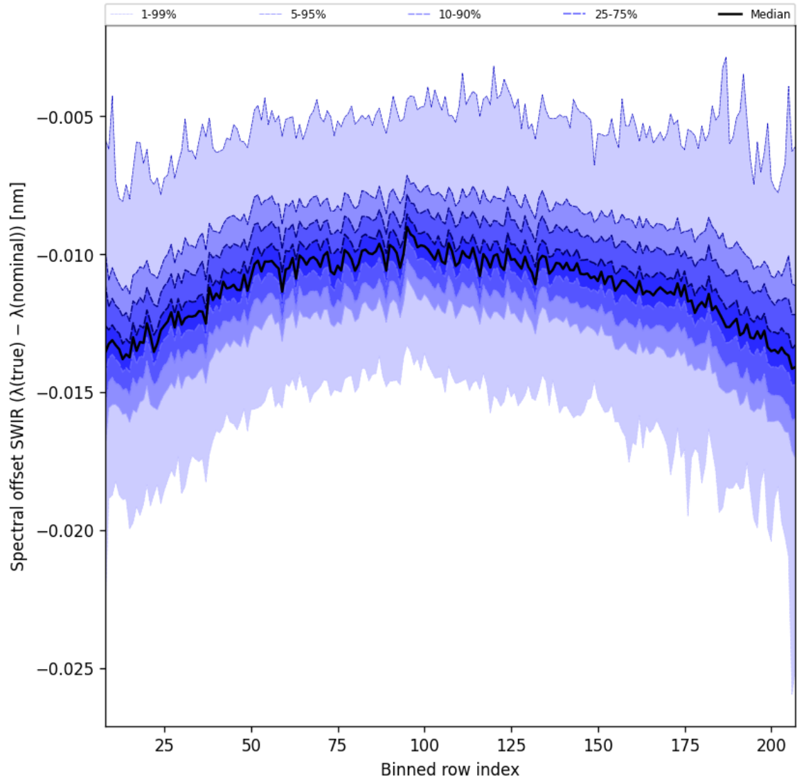
Figure 38: Along track statistics of “Spectral offset SWIR ( \lambda_{\text{true}} - \lambda_{\text{nominal}} )” for 2024-12-22 to 2024-12-24
