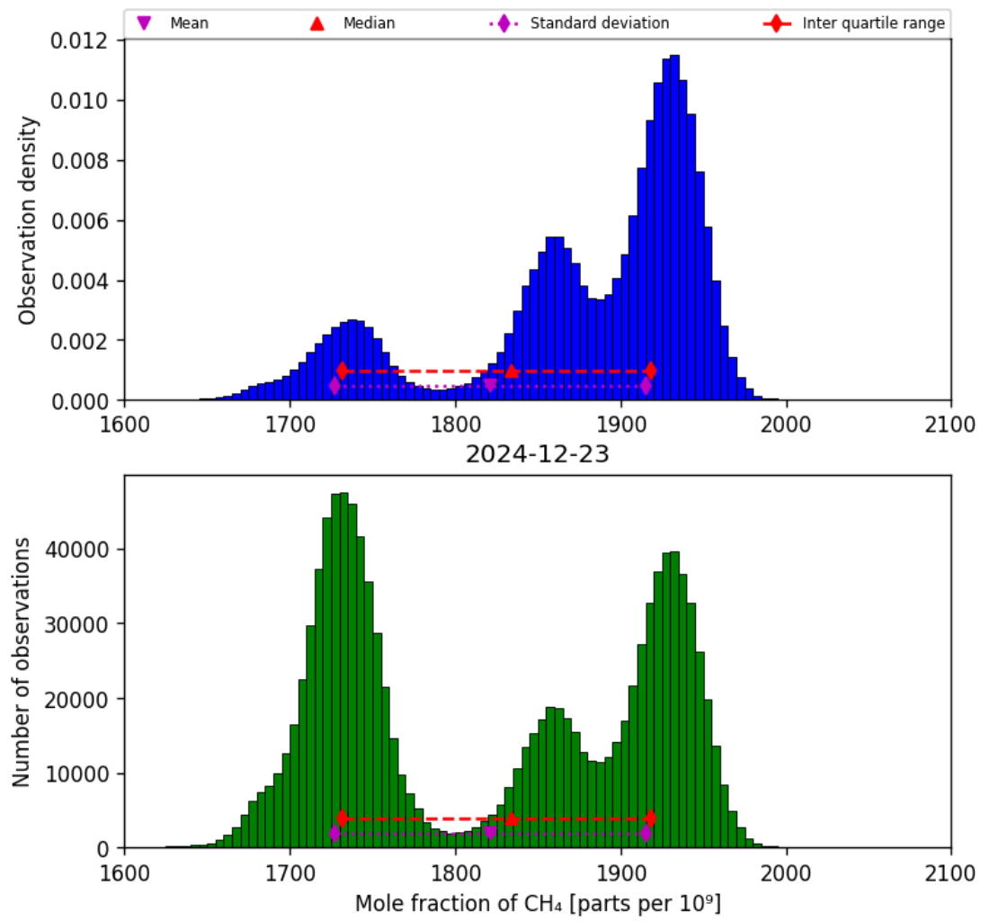
Figure 23: Histogram of “Mole fraction of CH 4 ” for 2024-12-22 to 2024-12-24
