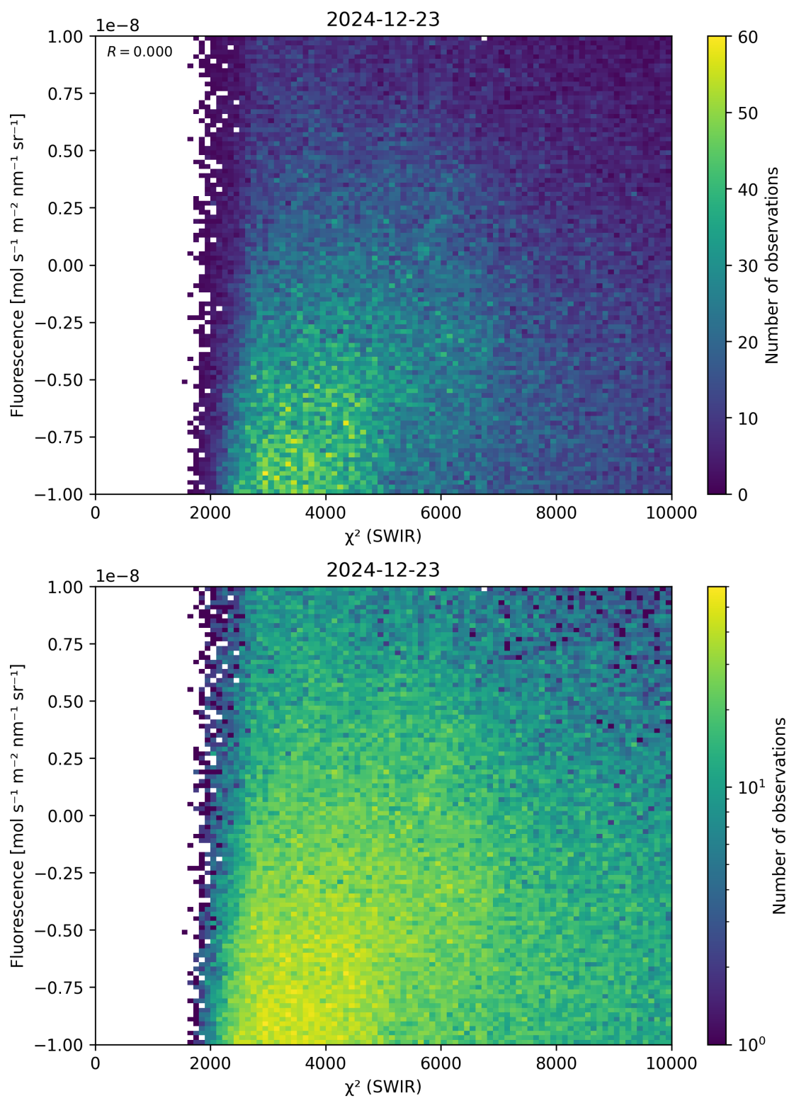
Figure 49: Scatter density plot of “ \chi^2 (SWIR)” against “Fluorescence” for 2024-12-22 to 2024-12-24.
