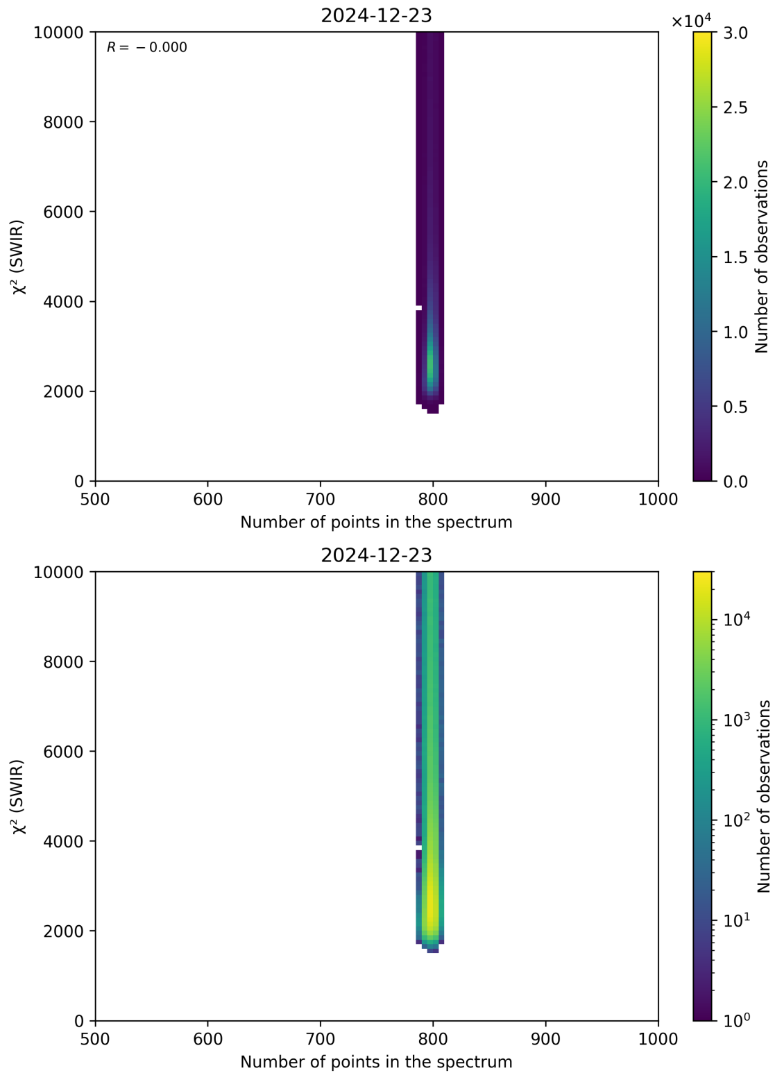
Figure 89: Scatter density plot of “Number of points in the spectrum” against “ \chi^2 (SWIR)” for 2024-12-22 to 2024-12-24.
