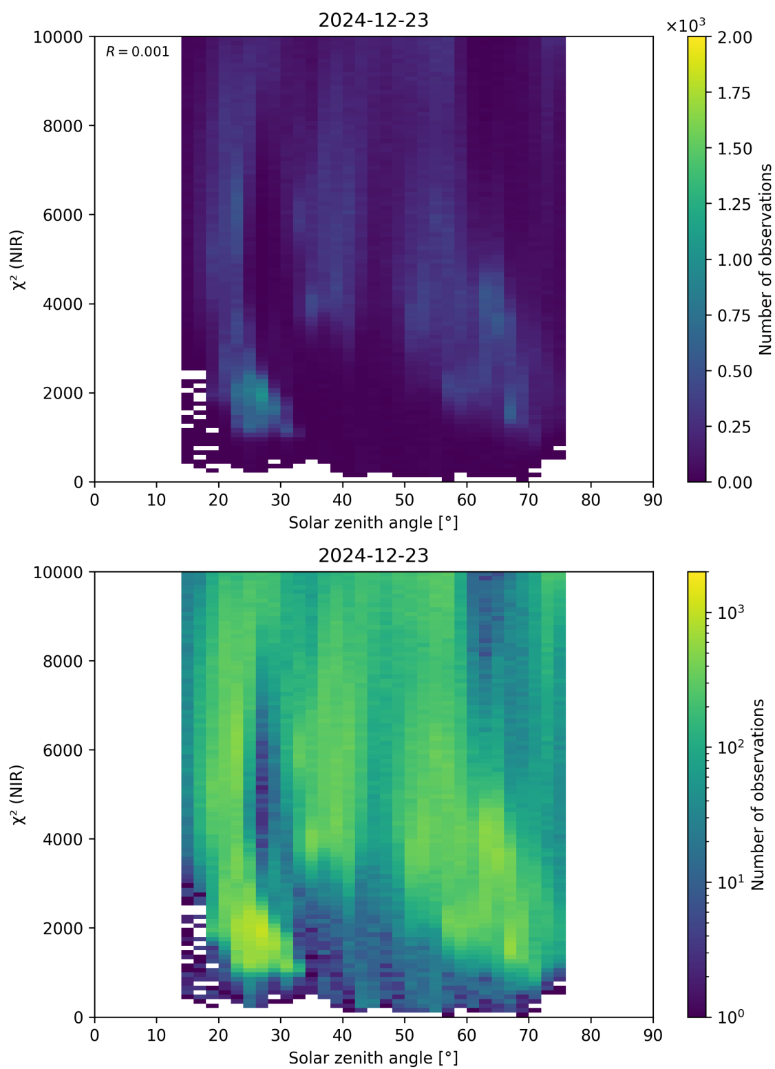
Figure 94: Scatter density plot of “Solar zenith angle” against “ \chi^2 (NIR)” for 2024-12-22 to 2024-12-24.
