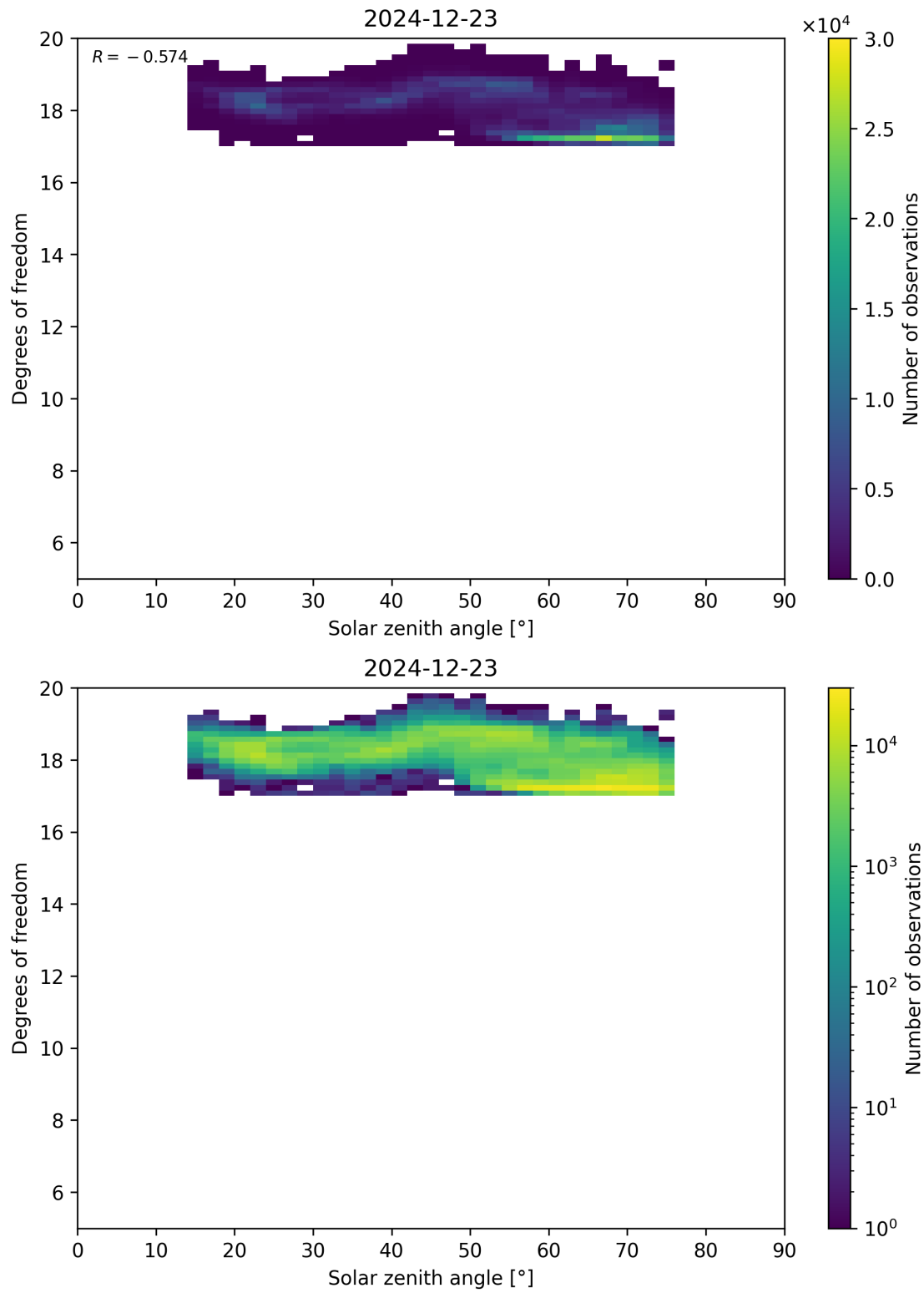
Figure 96: Scatter density plot of “Solar zenith angle” against “Degrees of freedom” for 2024-12-22 to 2024-12-24.
