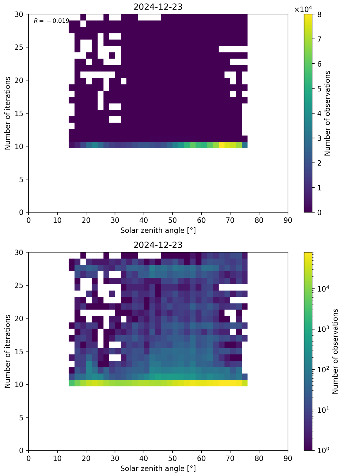
Figure 102: Scatter density plot of “Solar zenith angle” against “Number of iterations” for 2024-12-22 to 2024-12-24.
