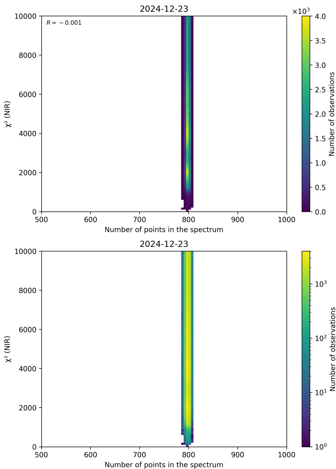
Figure 88: Scatter density plot of “Number of points in the spectrum” against “ \chi^2 (NIR)” for 2024-12-22 to 2024-12-24.
