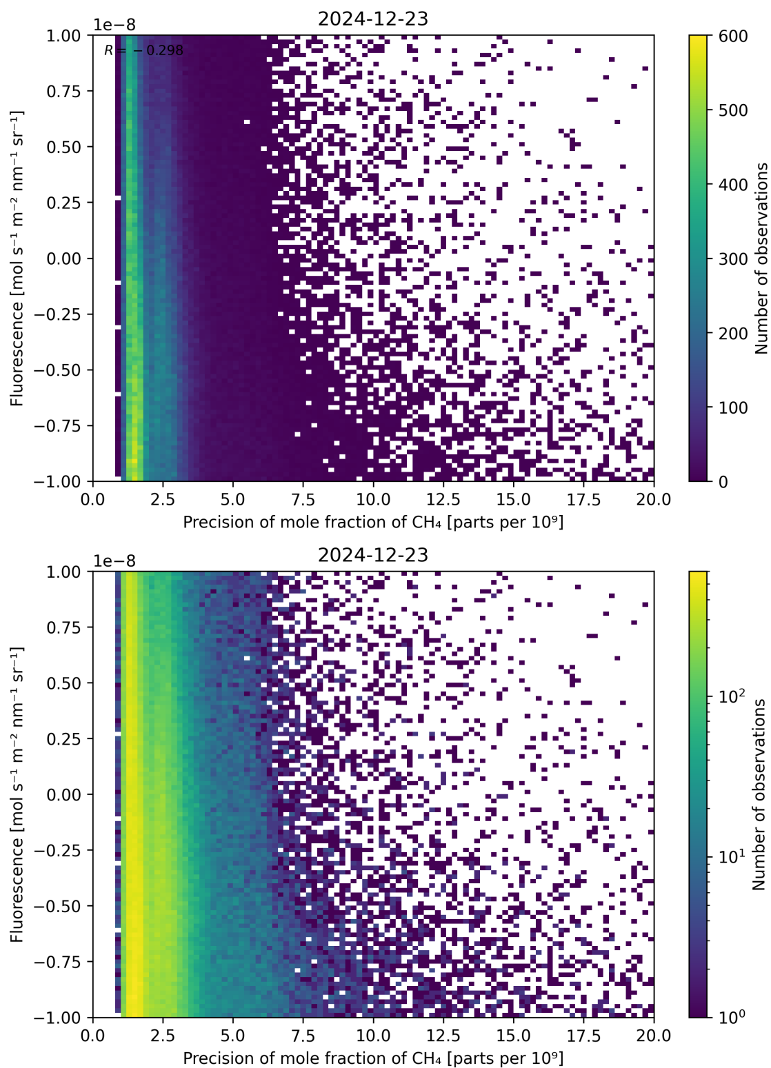
Figure 81: Scatter density plot of “Precision of mole fraction of \text{CH}_4 ” against “Fluorescence” for 2024-12-22 to 2024-12-24.
