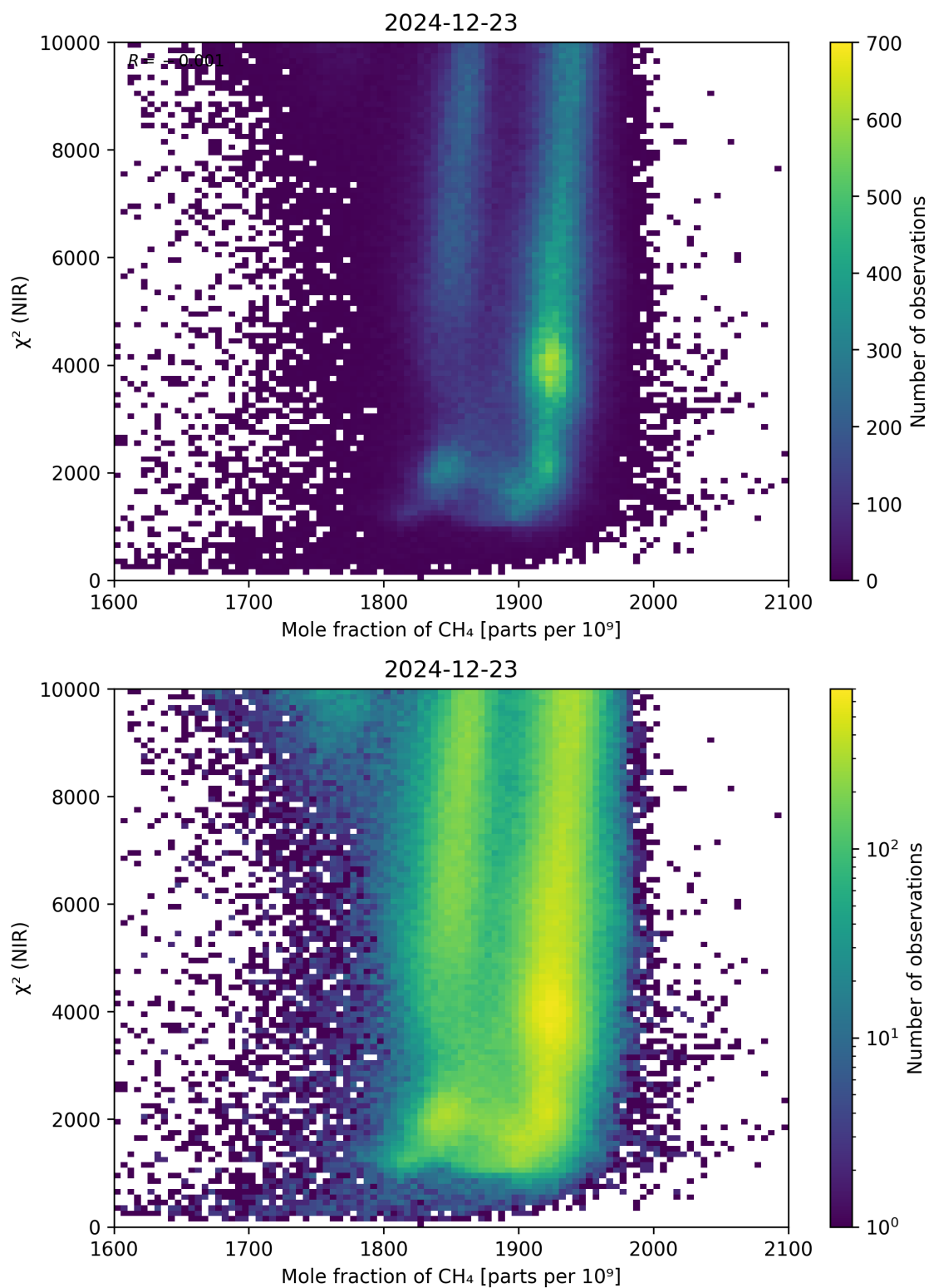
Figure 70: Scatter density plot of “Mole fraction of \text{CH}_4 ” against “ \chi^2 (NIR)” for 2024-12-22 to 2024-12-24.
