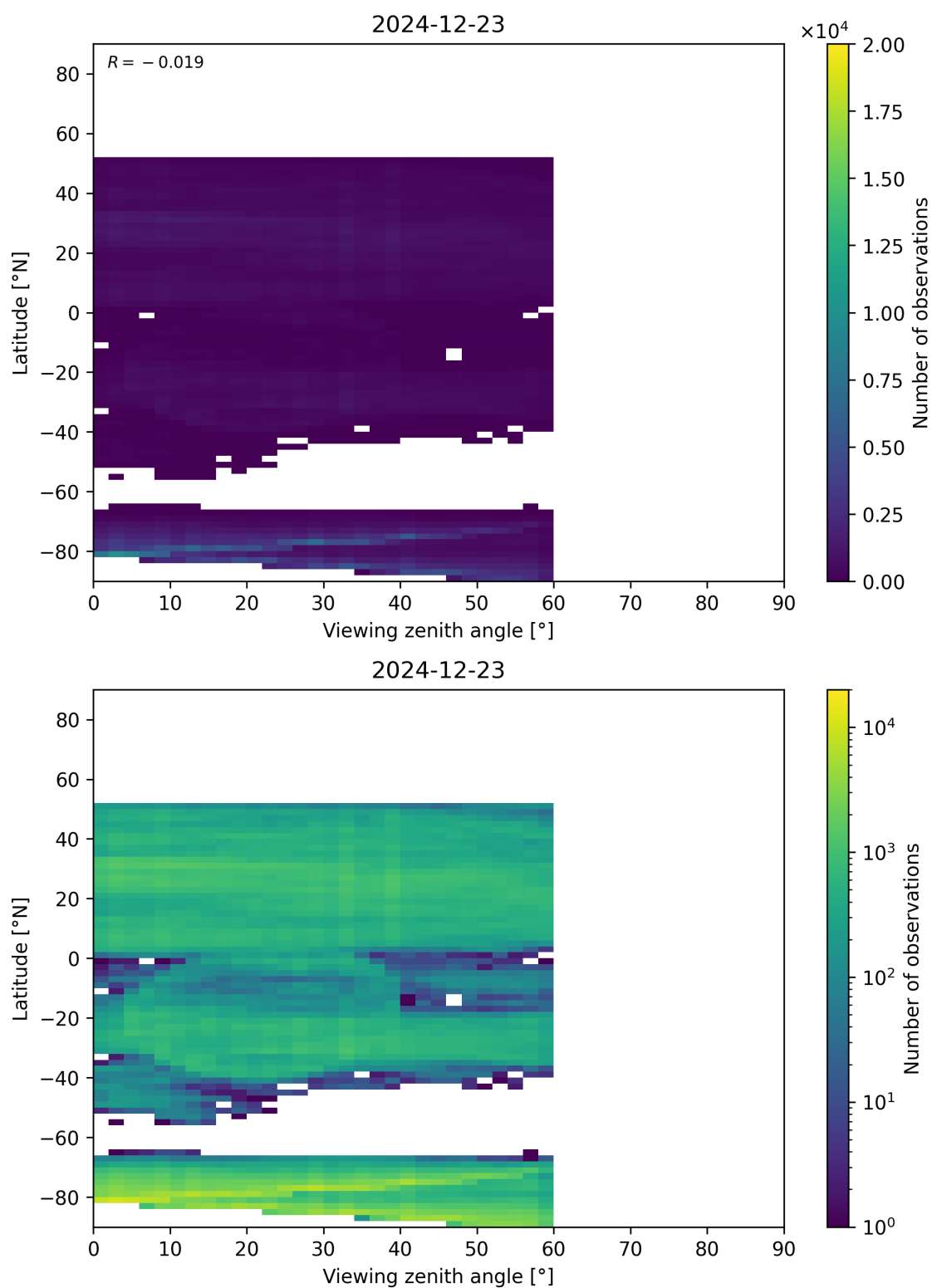
Figure 109: Scatter density plot of “Viewing zenith angle” against “Latitude” for 2024-12-22 to 2024-12-24.
