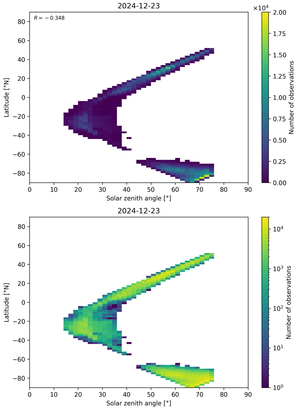
Figure 98: Scatter density plot of “Solar zenith angle” against “Latitude” for 2024-12-22 to 2024-12-24.
