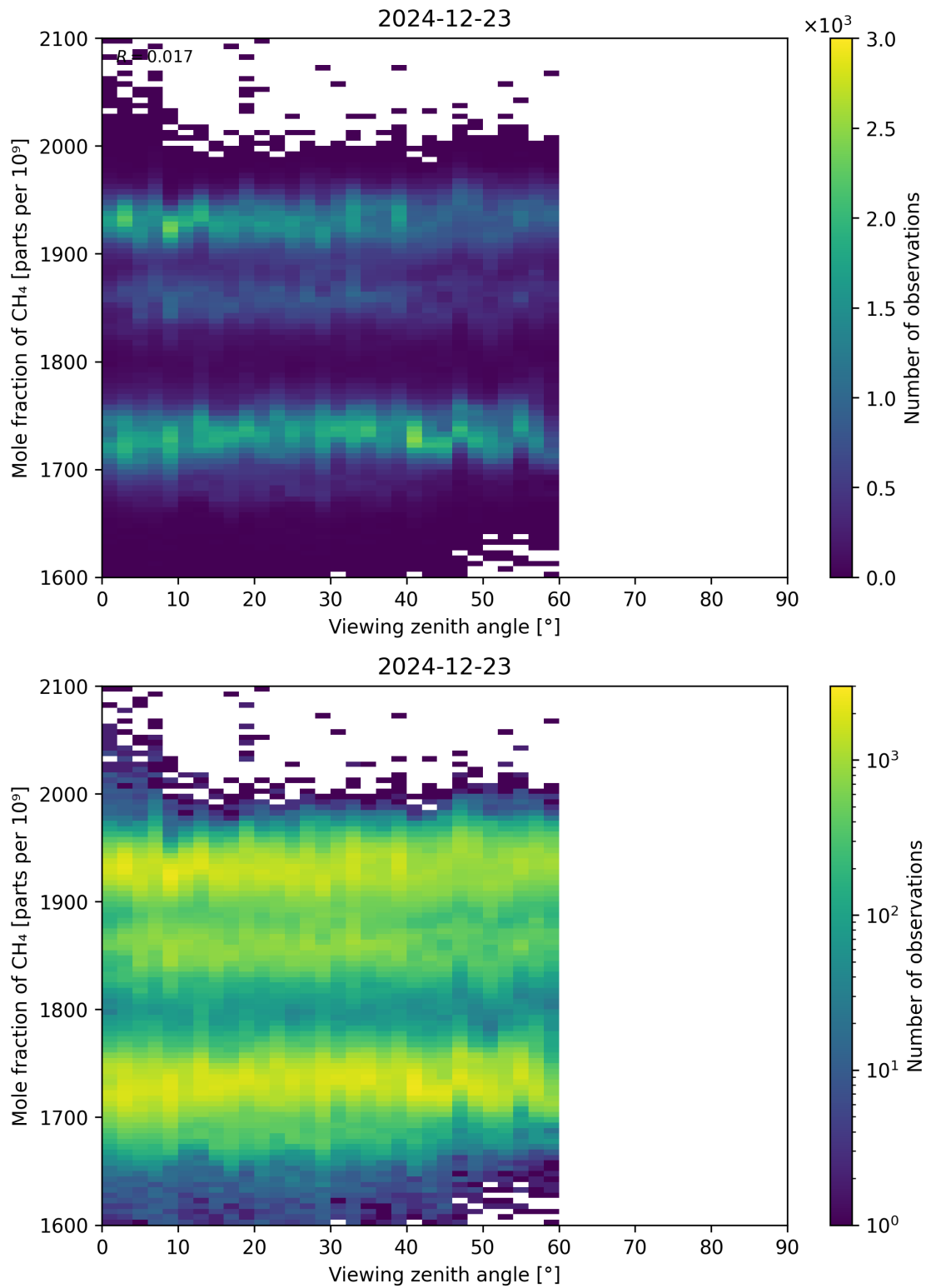
Figure 110: Scatter density plot of “Viewing zenith angle” against “Mole fraction of CH 4 ” for 2024-12-22 to 2024-12-24.
