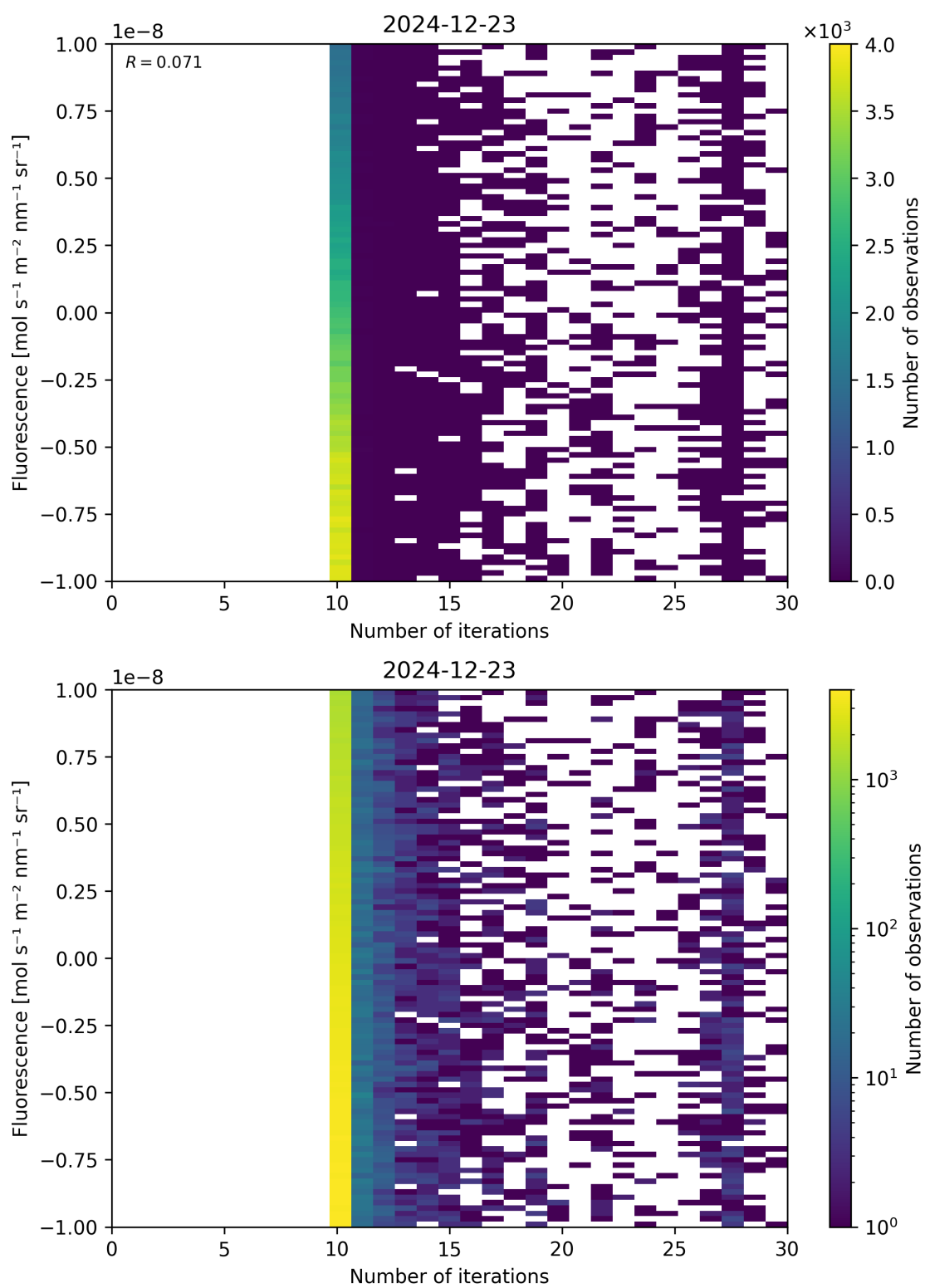
Figure 87: Scatter density plot of “Number of iterations” against “Fluorescence” for 2024-12-22 to 2024-12-24.
