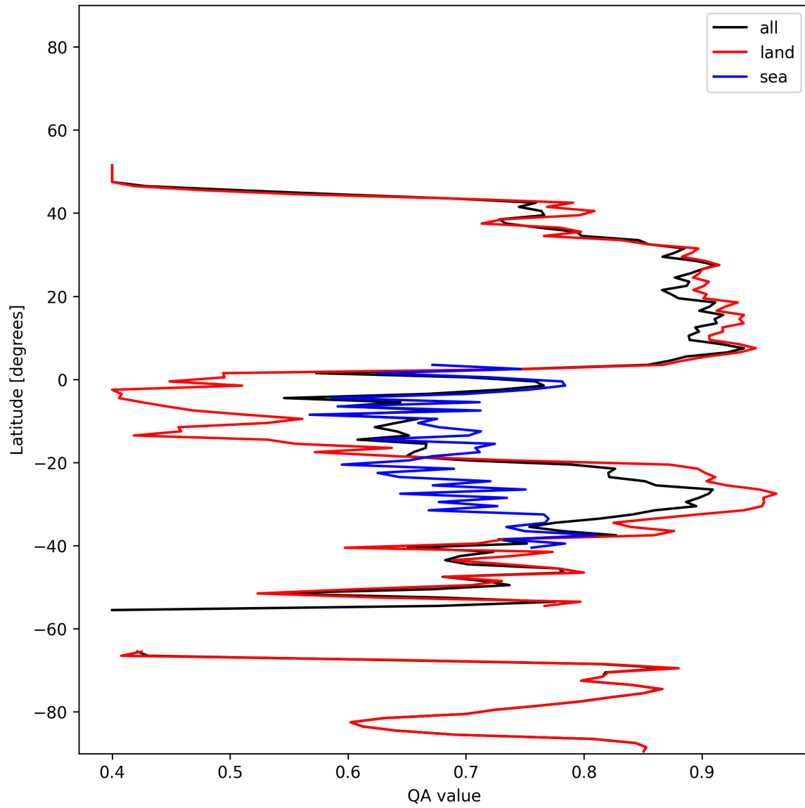
Figure 11: Zonal average of “QA value” for 2024-12-22 to 2024-12-24.
