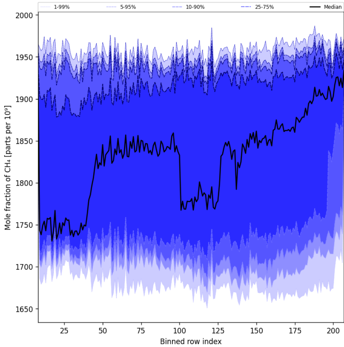
Figure 34: Along track statistics of “Mole fraction of CH 4 ” for 2024-12-22 to 2024-12-24
