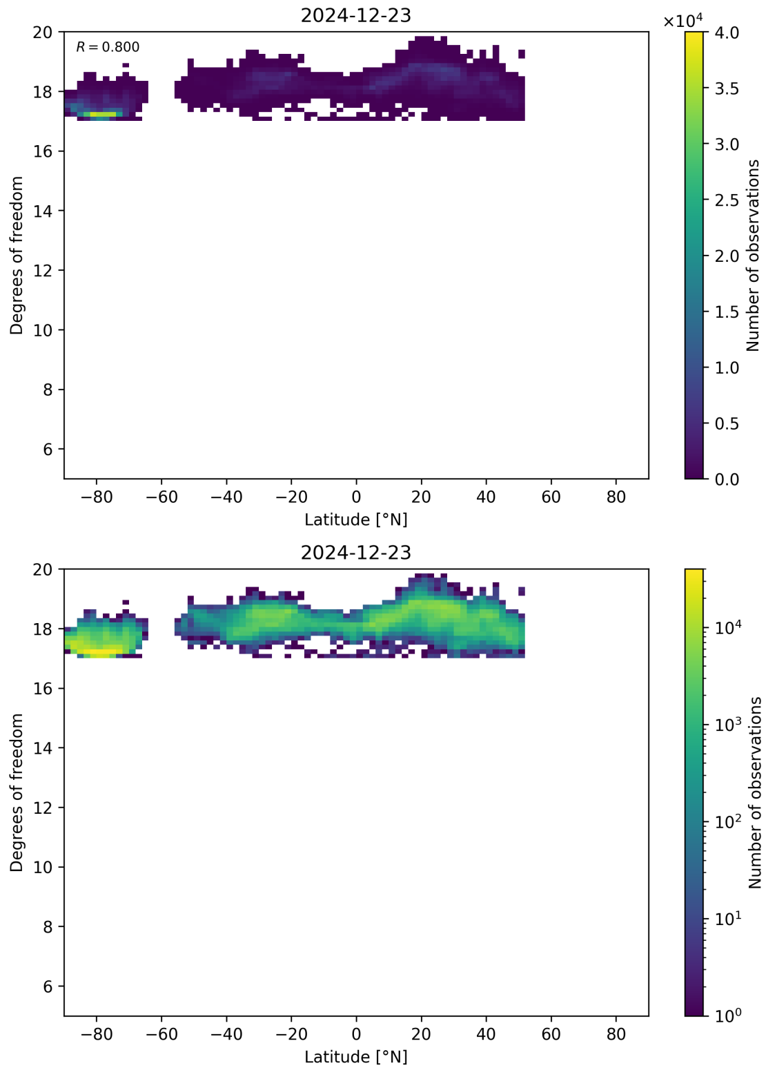
Figure 55: Scatter density plot of “Latitude” against “Degrees of freedom” for 2024-12-22 to 2024-12-24.
