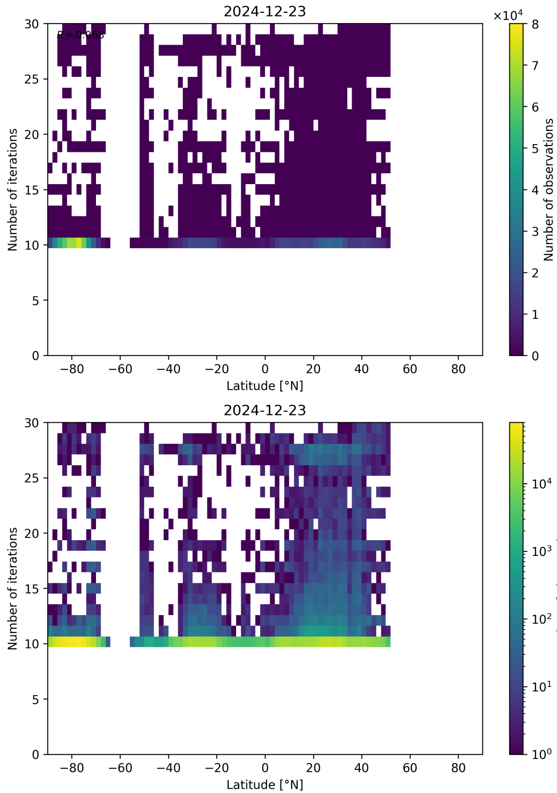
Figure 60: Scatter density plot of “Latitude” against “Number of iterations” for 2024-12-22 to 2024-12-24.
