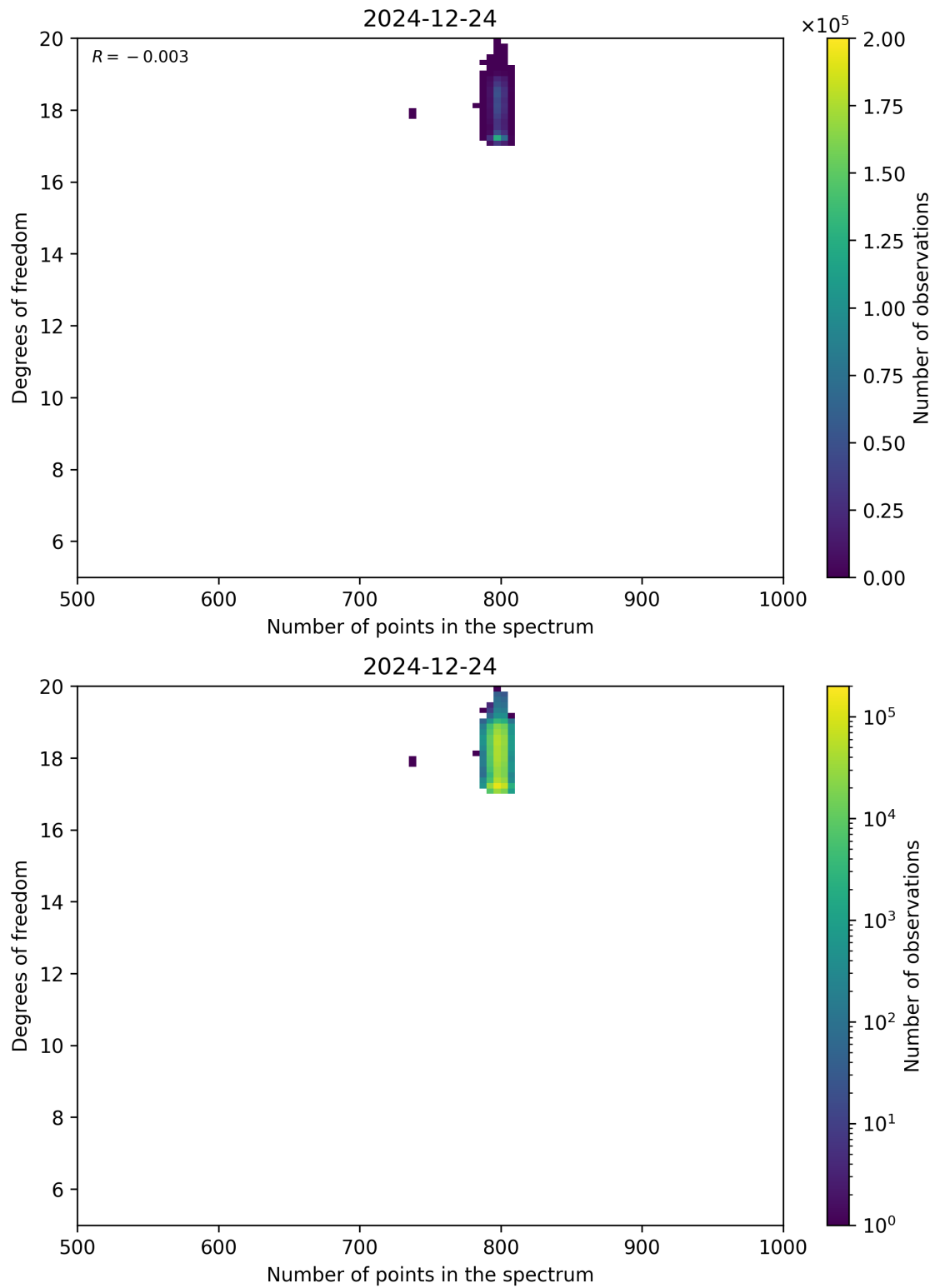
Figure 90: Scatter density plot of “Number of points in the spectrum” against “Degrees of freedom” for 2024-12-23 to 2024-12-25.
