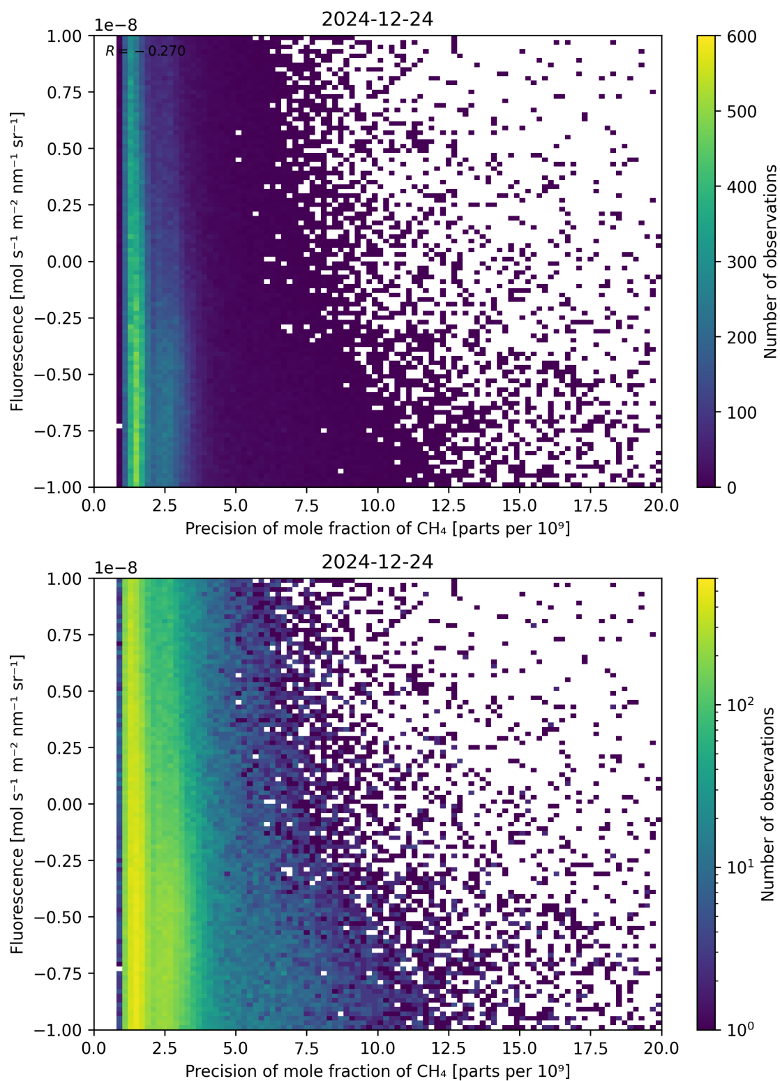
Figure 81: Scatter density plot of “Precision of mole fraction of \text{CH}_4 ” against “Fluorescence” for 2024-12-23 to 2024-12-25.
