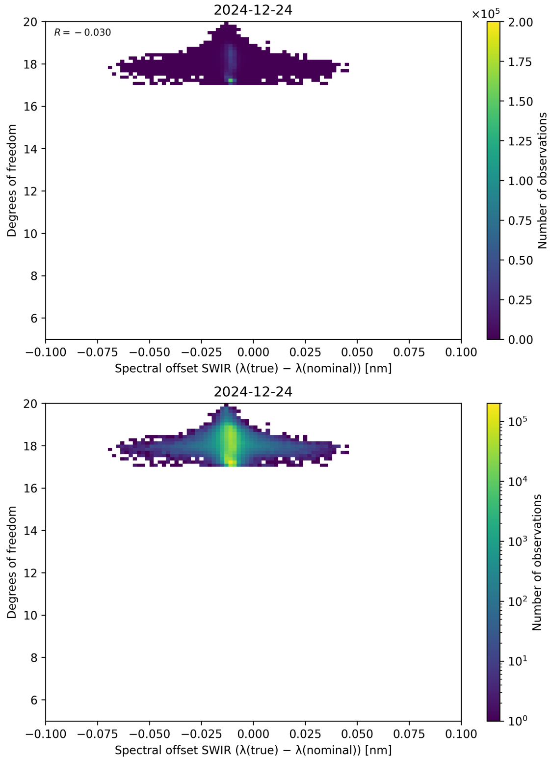
Figure 119: Scatter density plot of “Spectral offset SWIR ( \lambda_{\text{true}} - \lambda_{\text{nominal}} )” against “Degrees of freedom” for 2024-12-23 to 2024-12-25.
