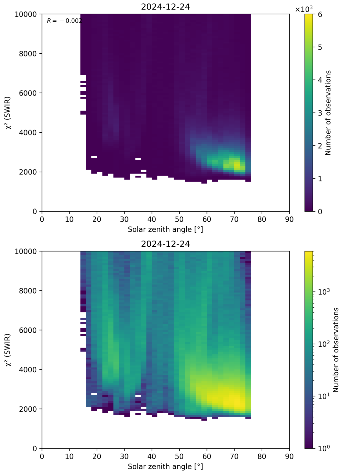
Figure 95: Scatter density plot of “Solar zenith angle” against “ \chi^2 (SWIR)” for 2024-12-23 to 2024-12-25.
