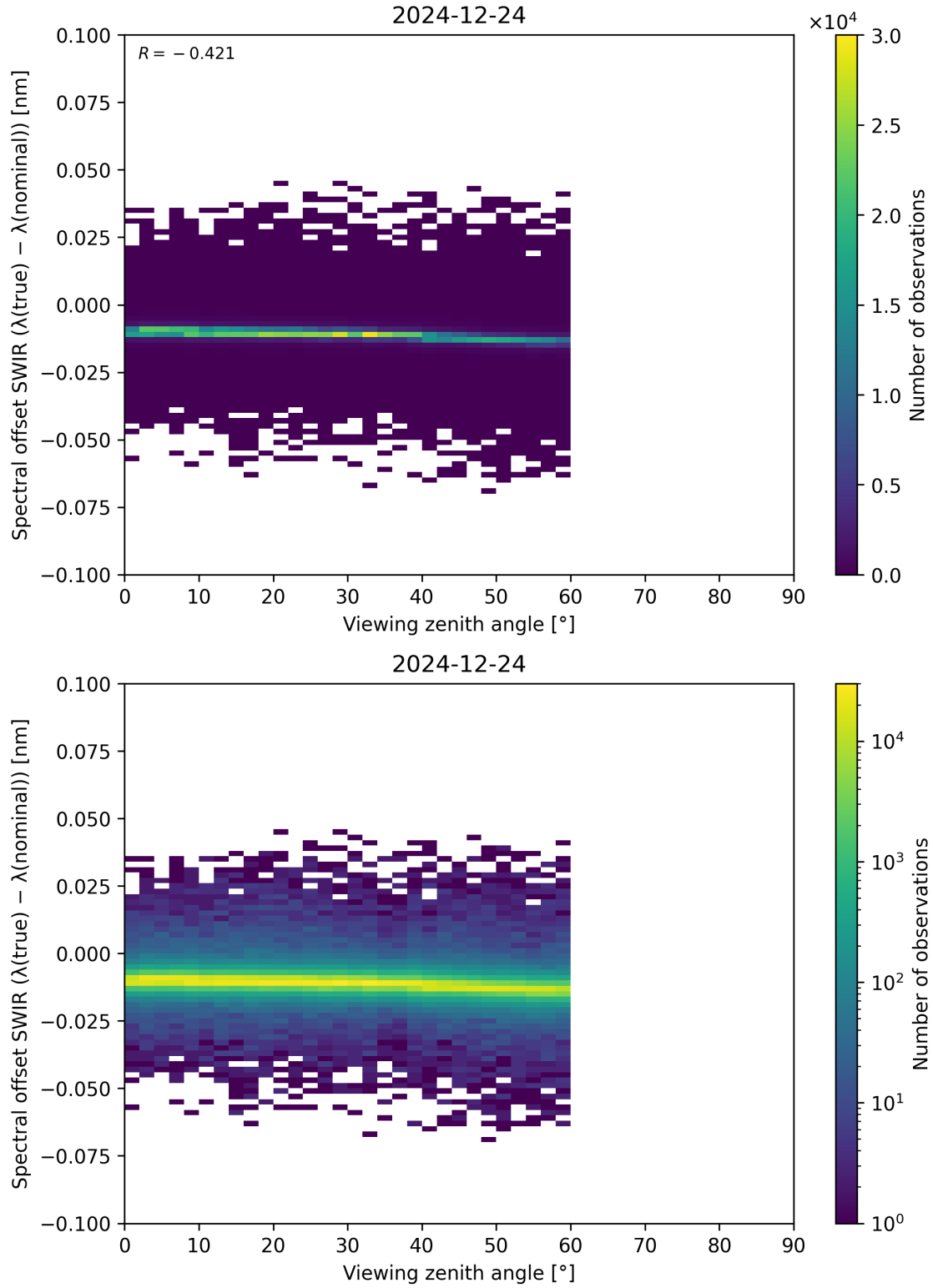
Figure 116: Scatter density plot of “Viewing zenith angle” against “Spectral offset SWIR ( \lambda_{\text{true}} - \lambda_{\text{nominal}} )” for 2024-12-23 to 2024-12-25.
