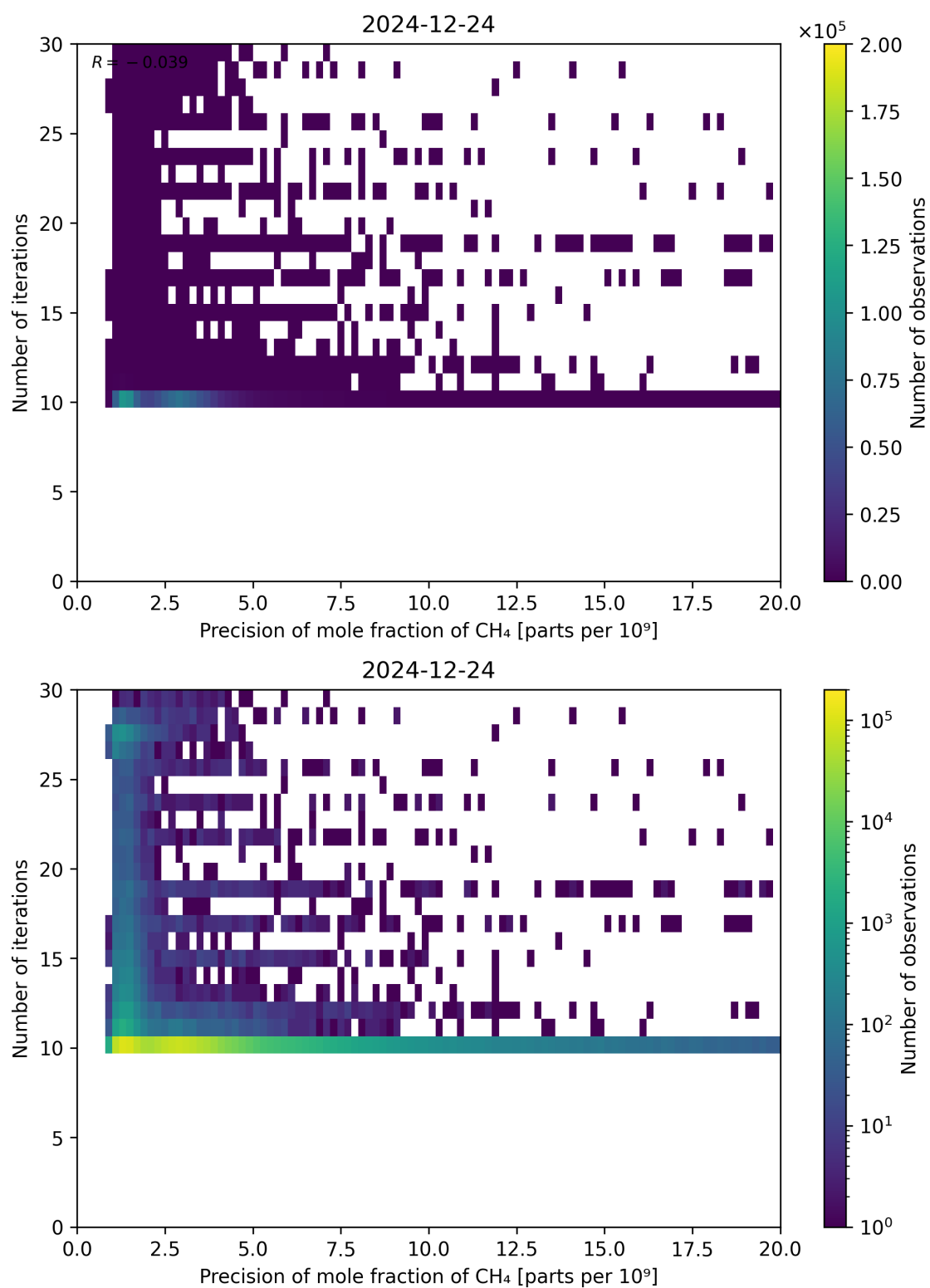
Figure 83: Scatter density plot of “Precision of mole fraction of CH 4 ” against “Number of iterations” for 2024-12-23 to 2024-12-25.
