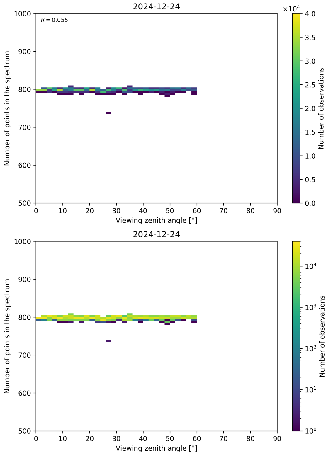
Figure 114: Scatter density plot of “Viewing zenith angle” against “Number of points in the spectrum” for 2024-12-23 to 2024-12-25.
