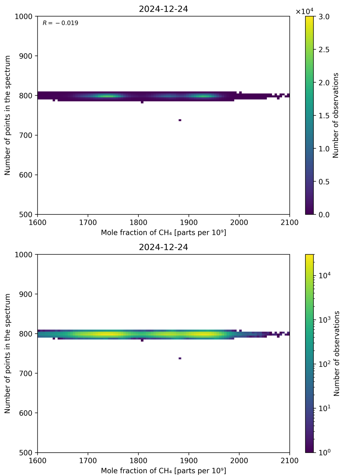
Figure 77: Scatter density plot of “Mole fraction of CH 4 ” against “Number of points in the spectrum” for 2024-12-23 to 2024-12-25.
