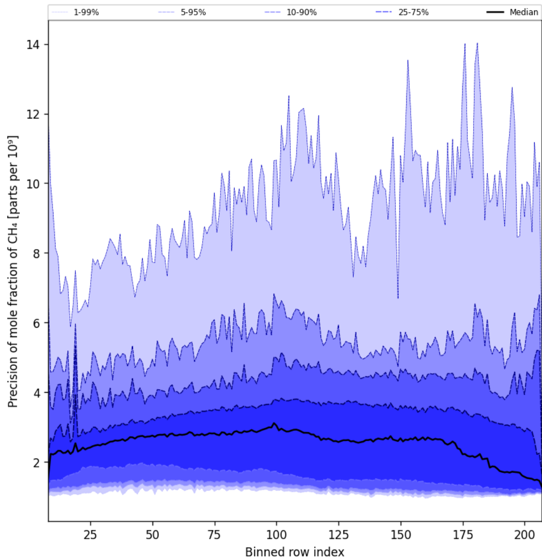
Figure 35: Along track statistics of “Precision of mole fraction of CH 4 ” for 2024-12-23 to 2024-12-25
