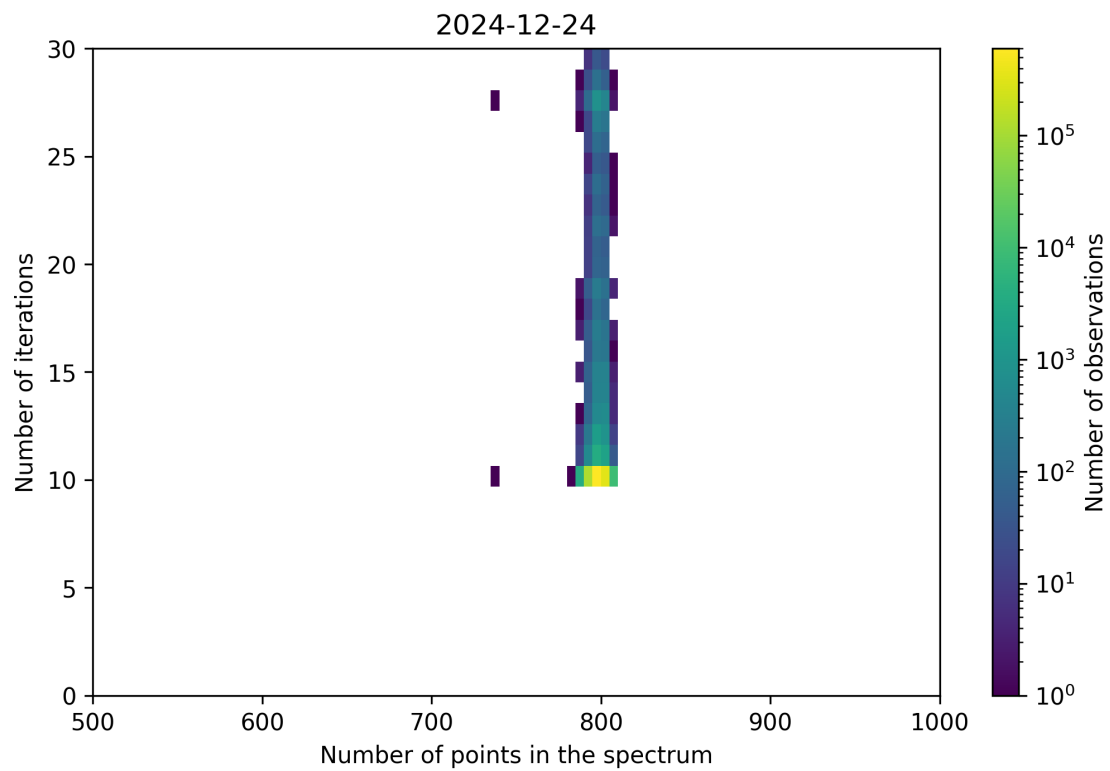
Figure 92: Scatter density plot of “Number of points in the spectrum” against “Number of iterations” for 2024-12-23 to 2024-12-25.
