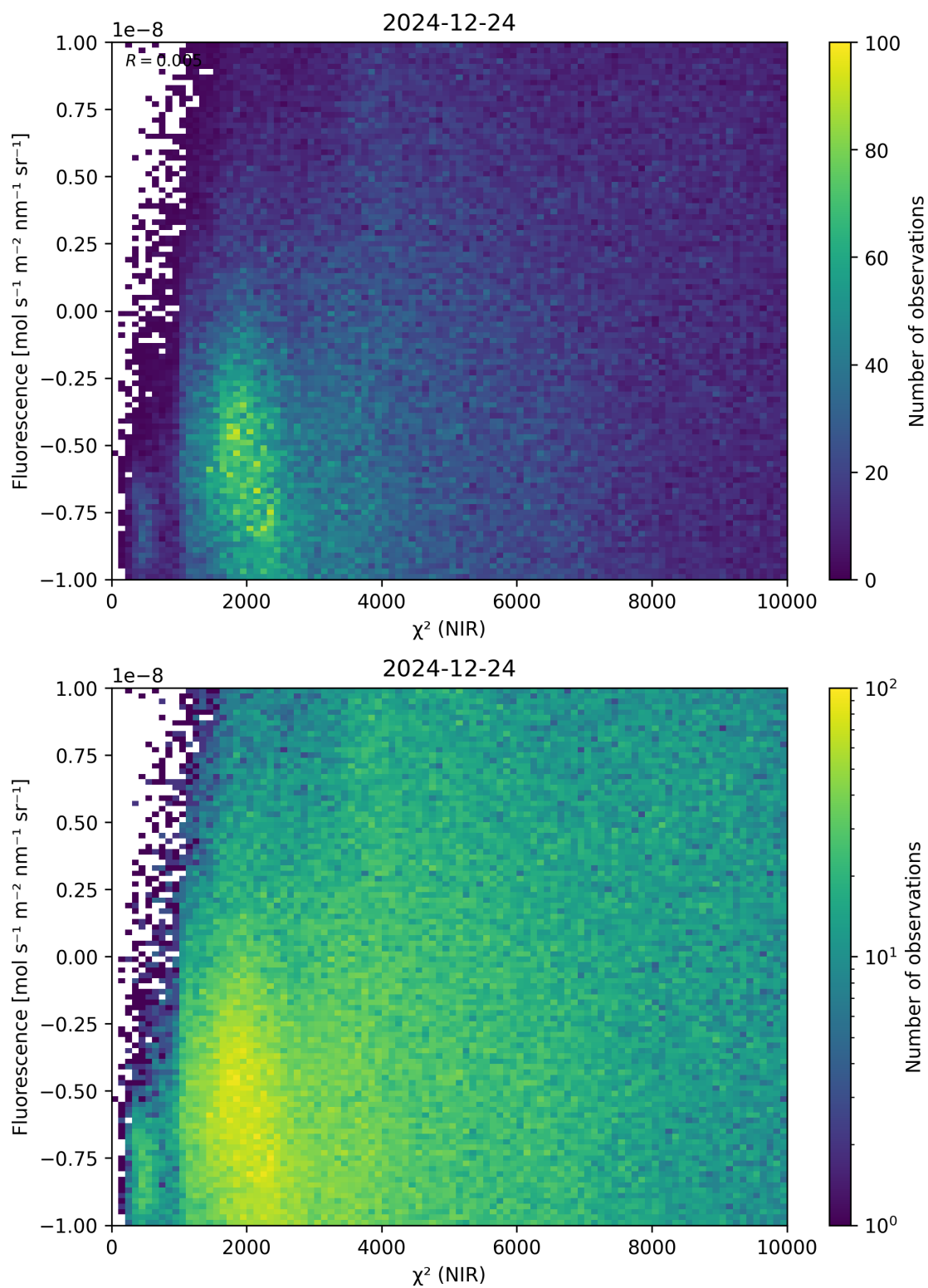
Figure 45: Scatter density plot of “ \chi^2 (NIR)” against “Fluorescence” for 2024-12-23 to 2024-12-25.
