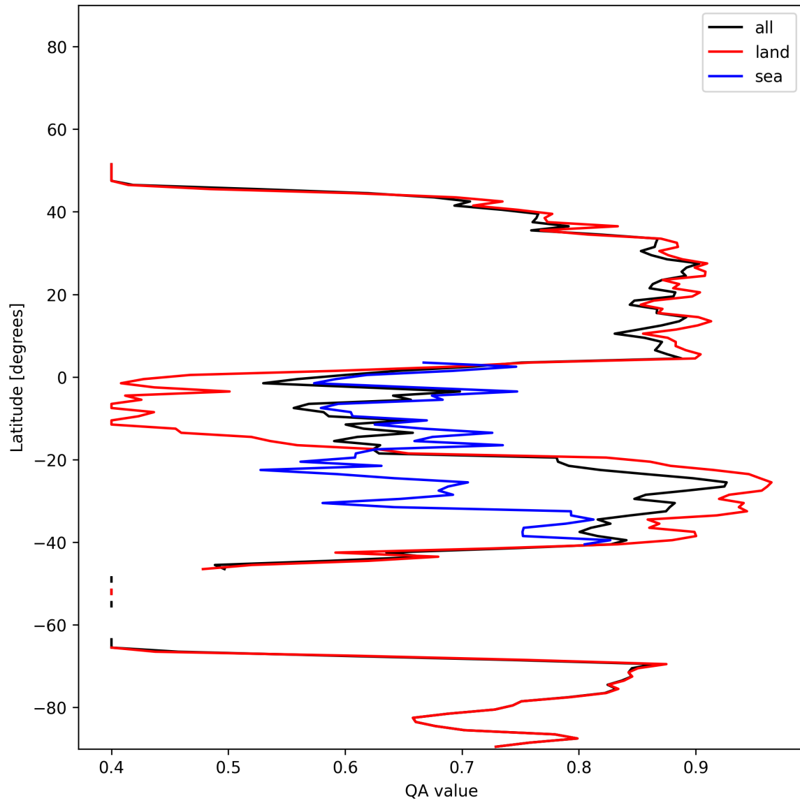
Figure 11: Zonal average of “QA value” for 2024-12-23 to 2024-12-25.
