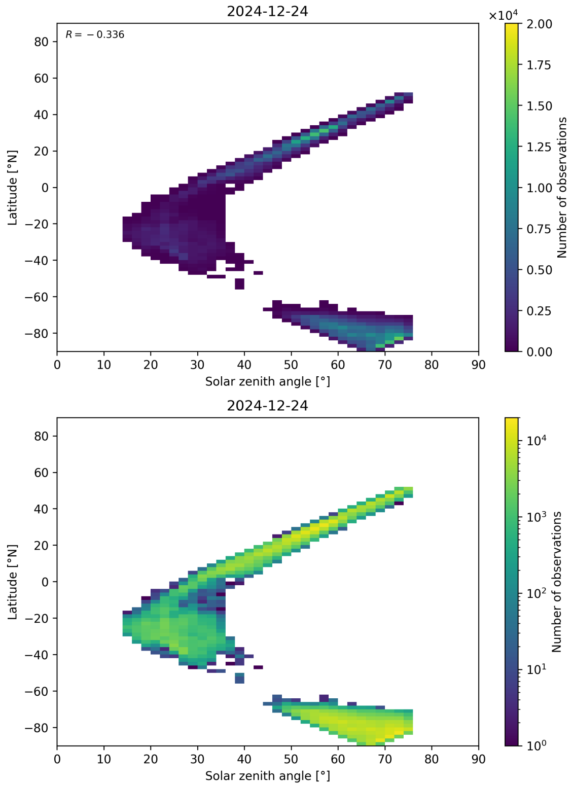
Figure 98: Scatter density plot of “Solar zenith angle” against “Latitude” for 2024-12-23 to 2024-12-25.
