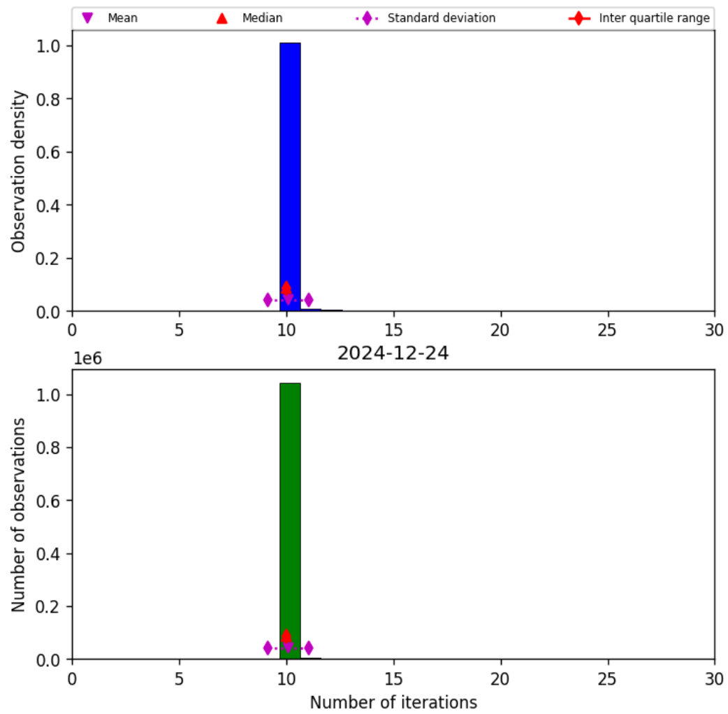
Figure 31: Histogram of “Number of iterations” for 2024-12-23 to 2024-12-25
