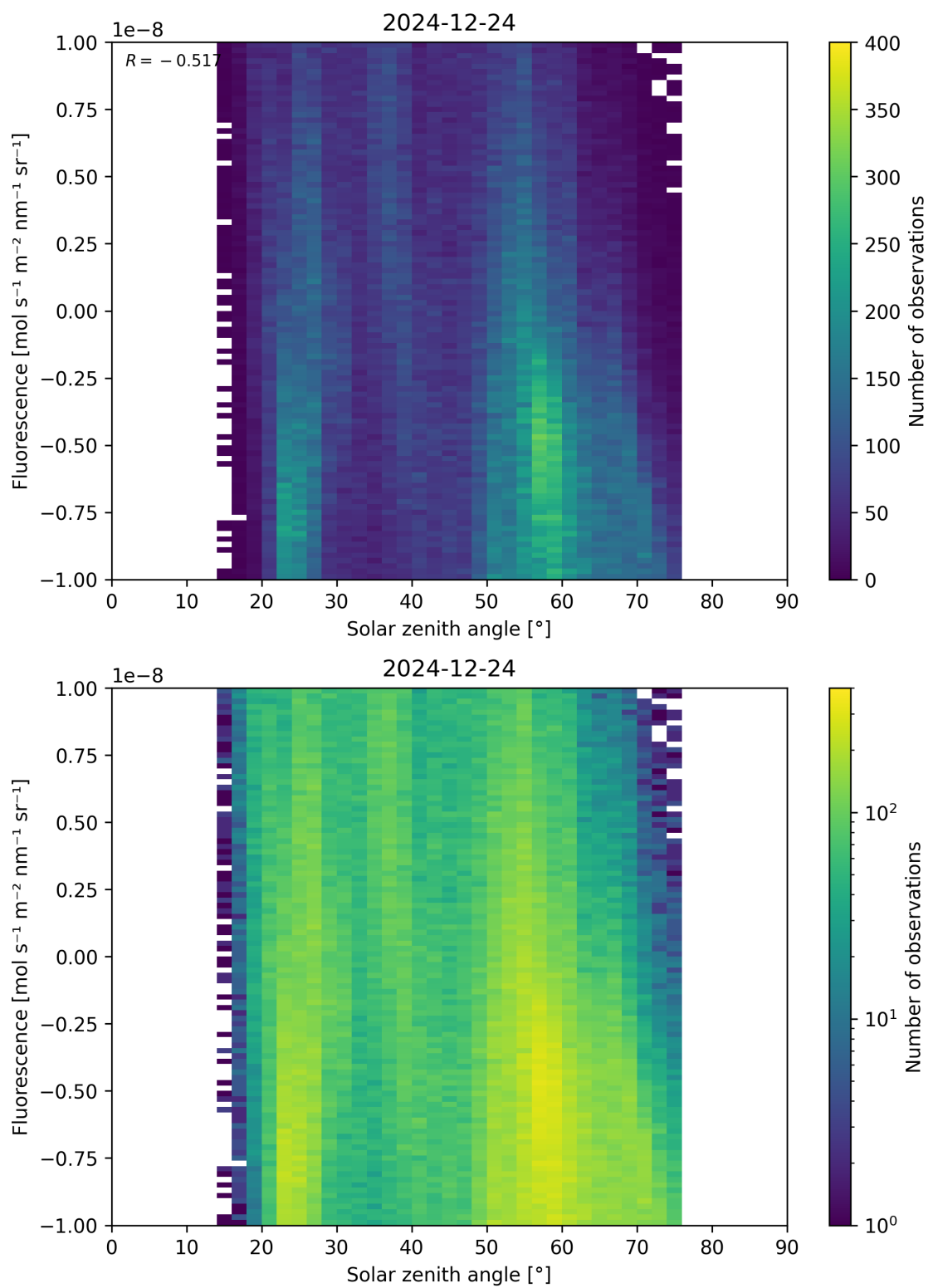
Figure 97: Scatter density plot of “Solar zenith angle” against “Fluorescence” for 2024-12-23 to 2024-12-25.
