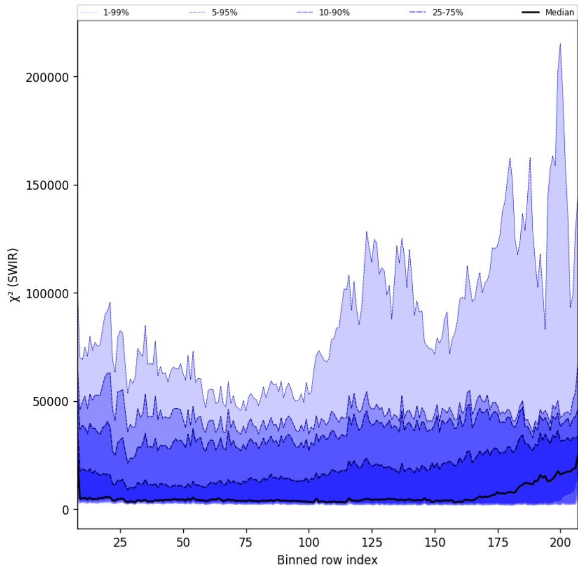
Figure 39: Along track statistics of “ \chi^2 (SWIR)” for 2024-12-23 to 2024-12-25
