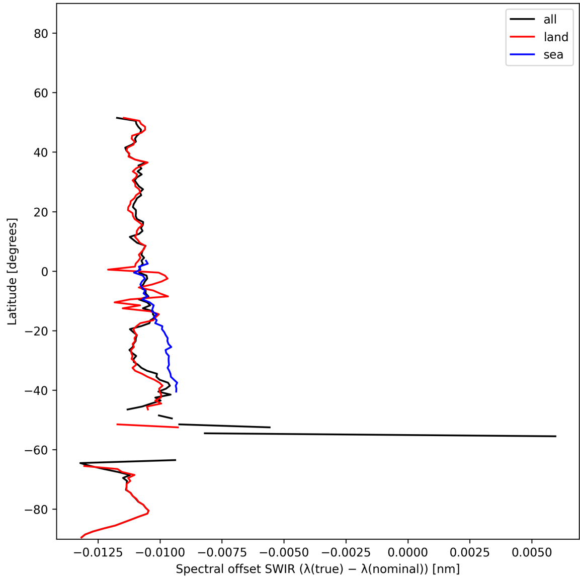
Figure 16: Zonal average of “Spectral offset SWIR ( \lambda_{\text{true}} - \lambda_{\text{nominal}} )” for 2024-12-23 to 2024-12-25.
