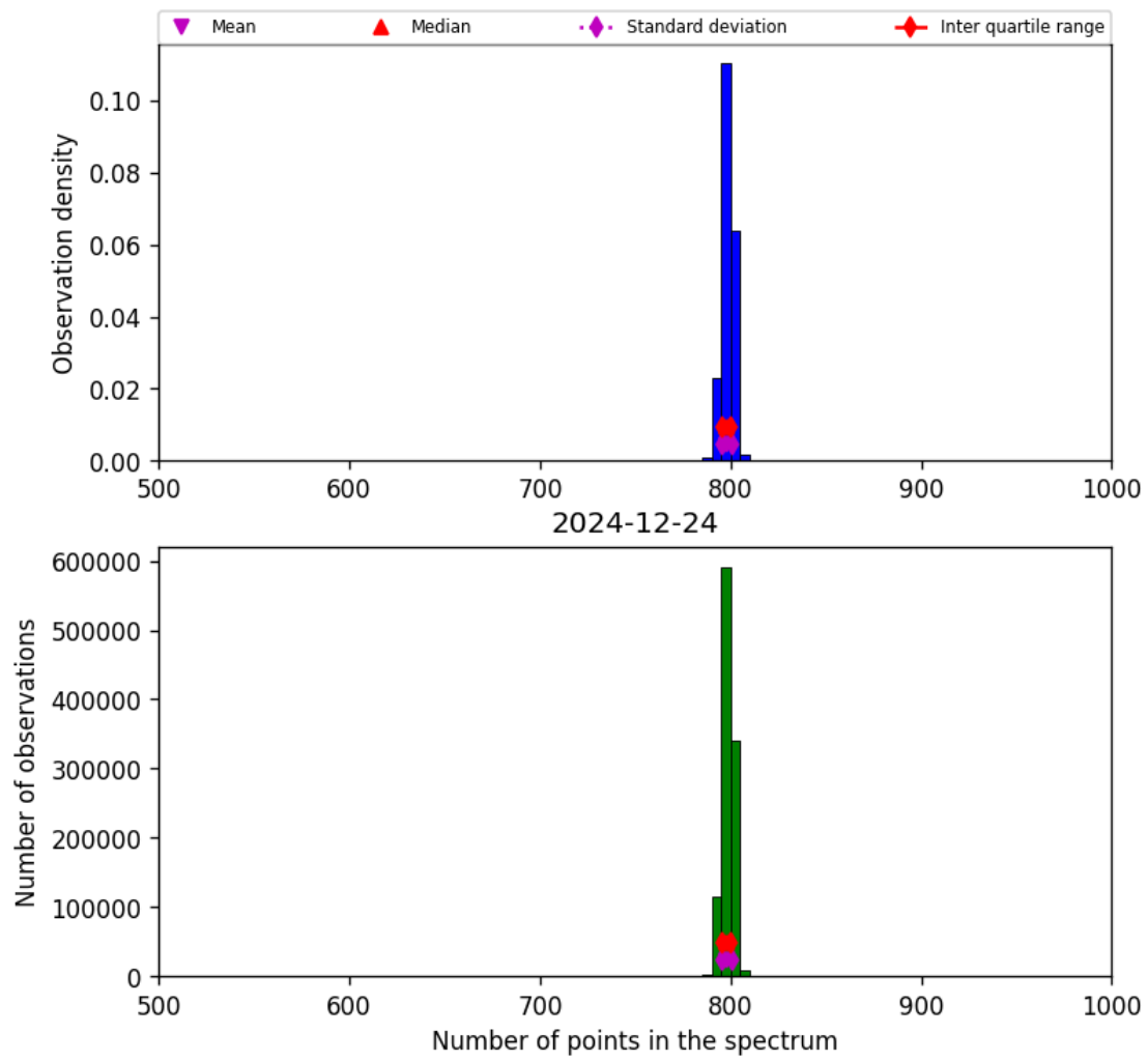
Figure 26: Histogram of “Number of points in the spectrum” for 2024-12-23 to 2024-12-25
