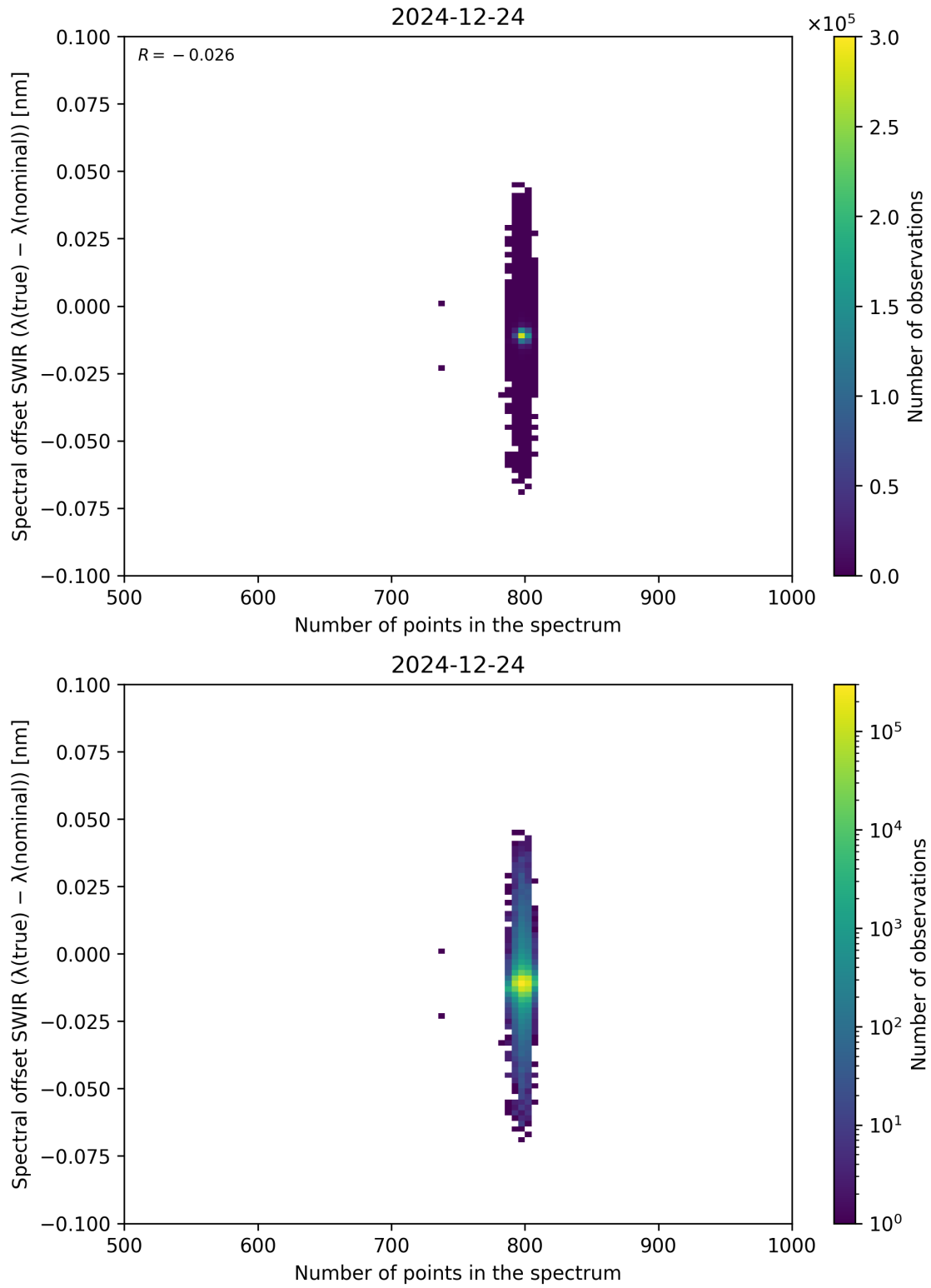
Figure 93: Scatter density plot of “Number of points in the spectrum” against “Spectral offset SWIR ( \lambda_{\text{true}} - \lambda_{\text{nominal}} )” for 2024-12-23 to 2024-12-25.
