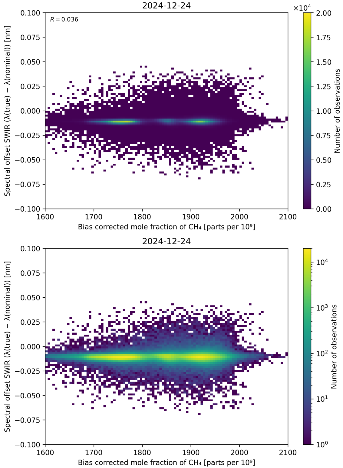
Figure 69: Scatter density plot of “Bias corrected mole fraction of \text{CH}_4 ” against “Spectral offset SWIR ( \lambda_{\text{true}} - \lambda_{\text{nominal}} )” for 2024-12-23 to 2024-12-25.
