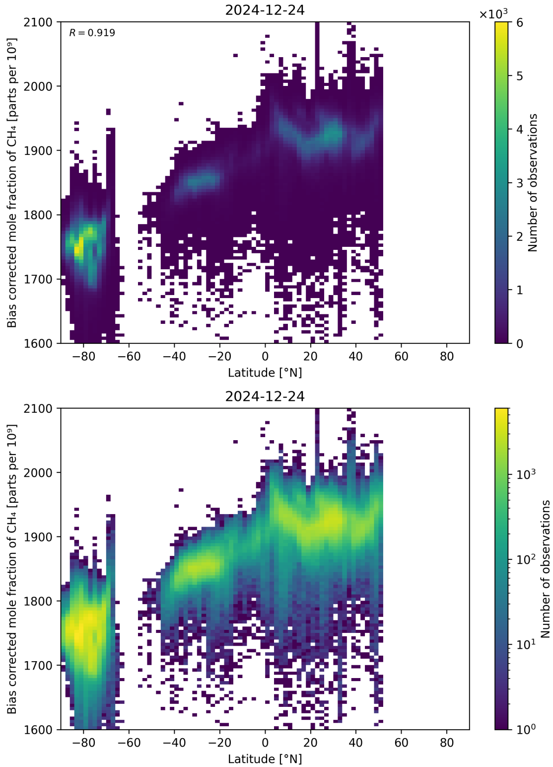
Figure 58: Scatter density plot of “Latitude” against “Bias corrected mole fraction of CH 4 ” for 2024-12-23 to 2024-12-25.
