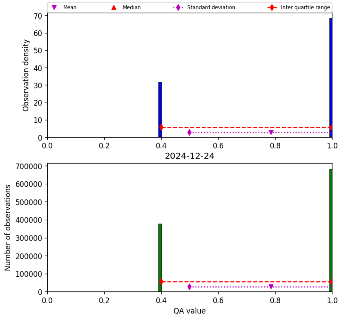
Figure 22: Histogram of “QA value” for 2024-12-23 to 2024-12-25
