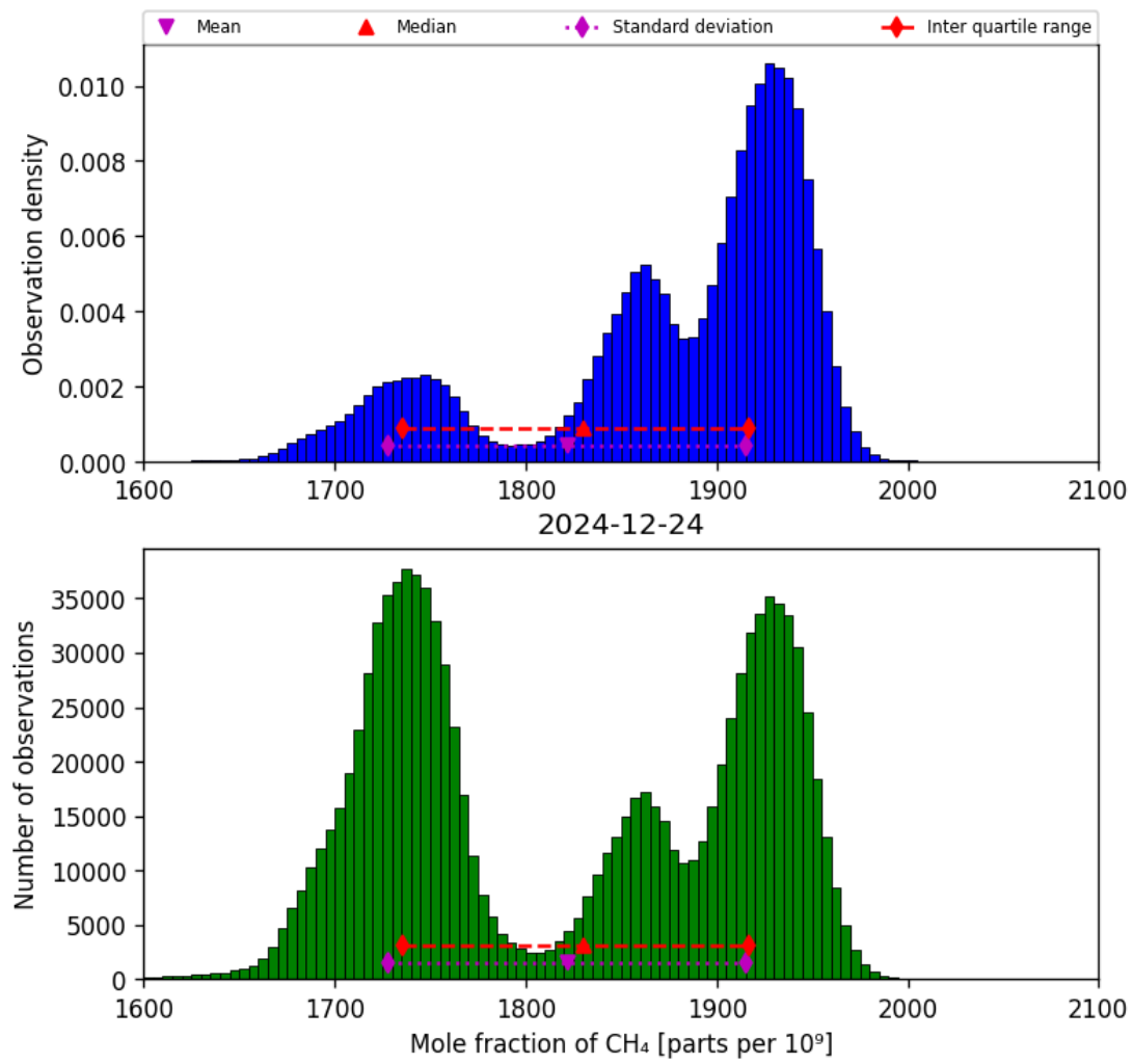
Figure 23: Histogram of “Mole fraction of CH 4 ” for 2024-12-23 to 2024-12-25
