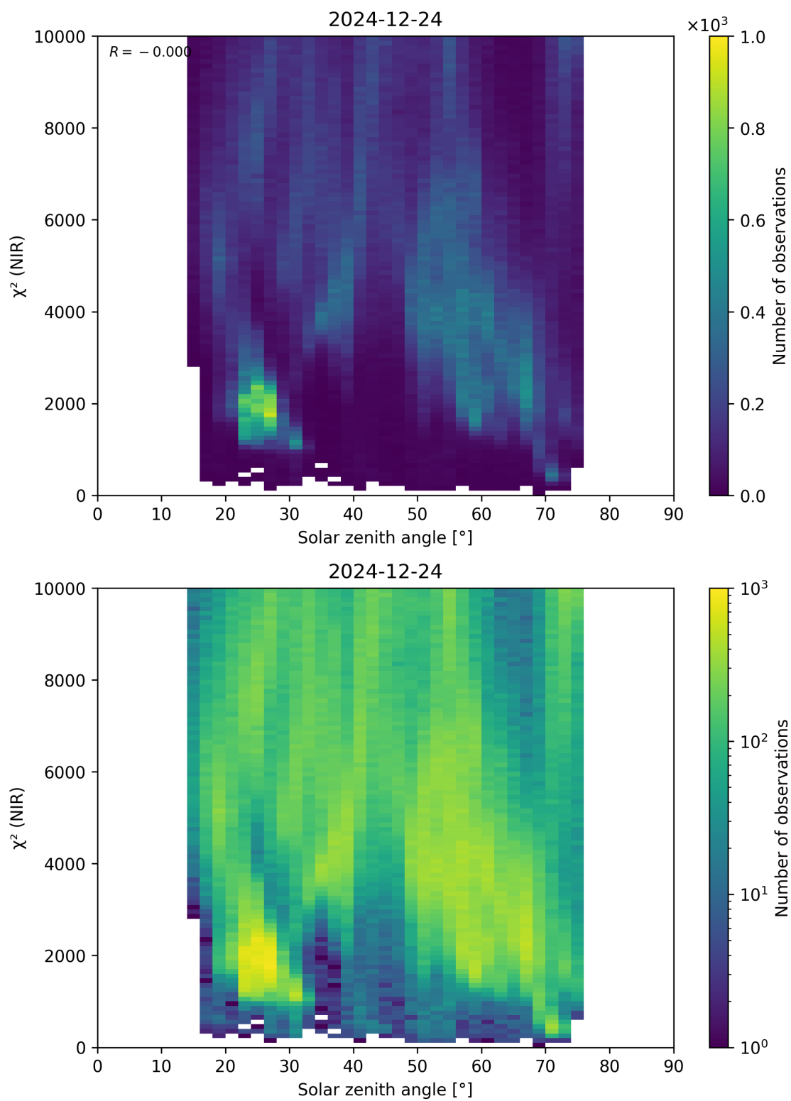
Figure 94: Scatter density plot of “Solar zenith angle” against “ \chi^2 (NIR)” for 2024-12-23 to 2024-12-25.
