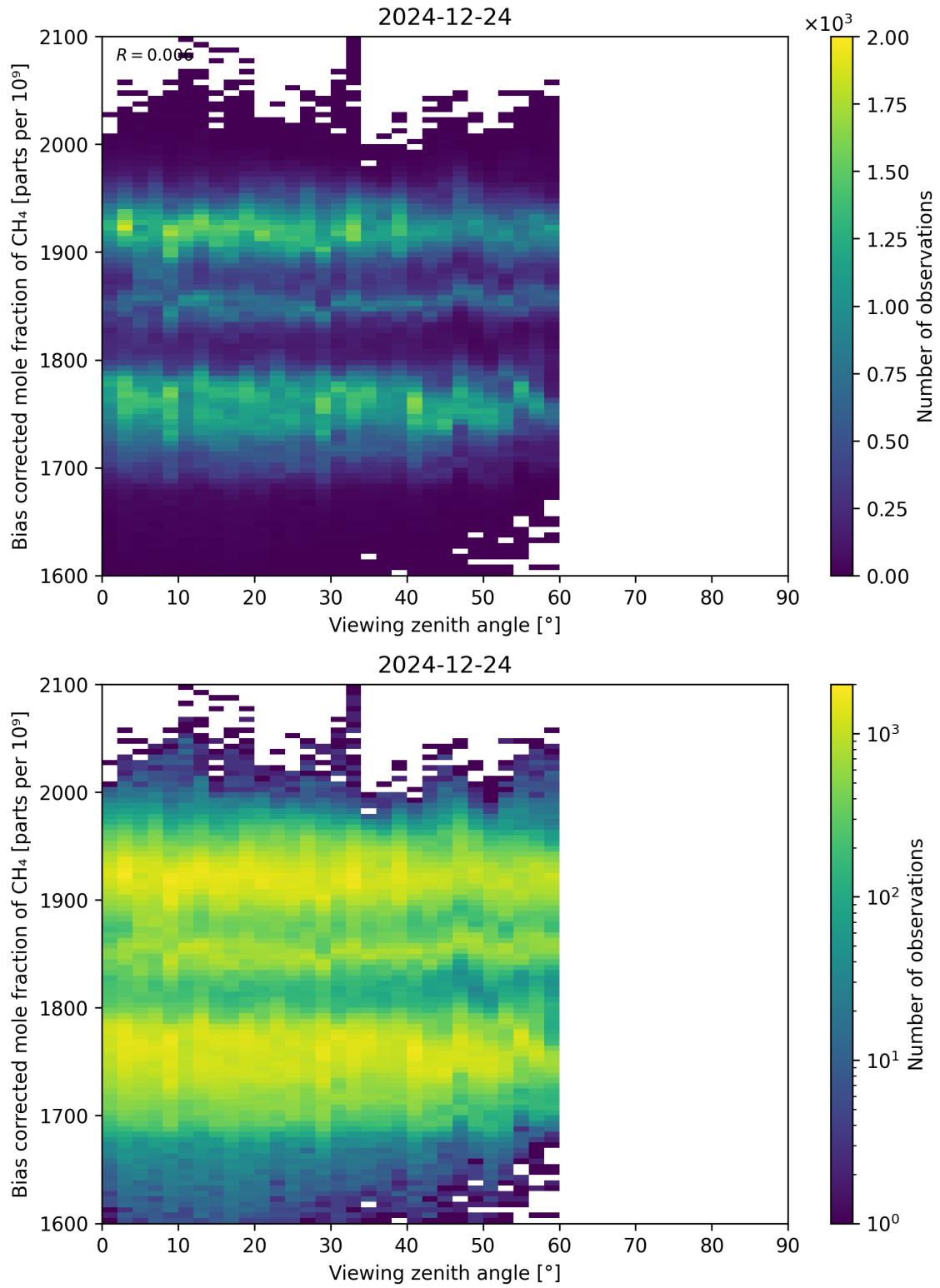
Figure 111: Scatter density plot of “Viewing zenith angle” against “Bias corrected mole fraction of CH 4 ” for 2024-12-23 to 2024-12-25.
