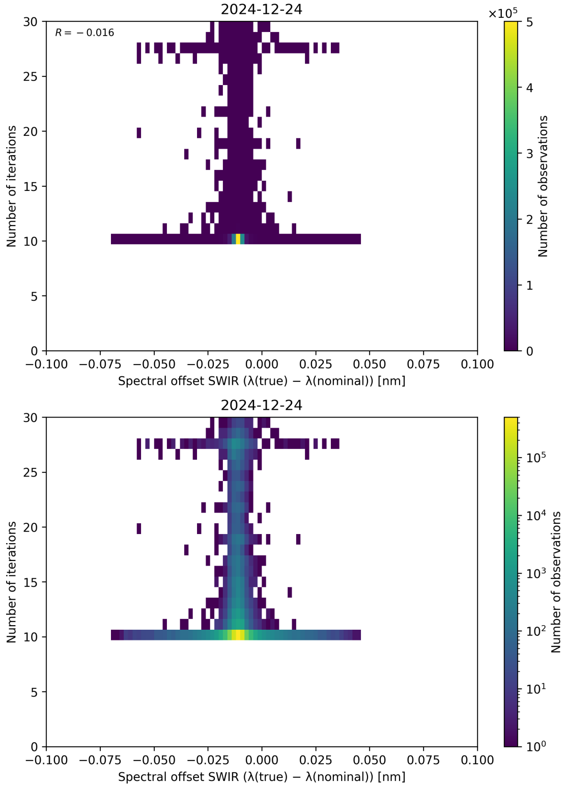
Figure 121: Scatter density plot of “Spectral offset SWIR ( \lambda_{\text{true}} - \lambda_{\text{nominal}} )” against “Number of iterations” for 2024-12-23 to 2024-12-25.
