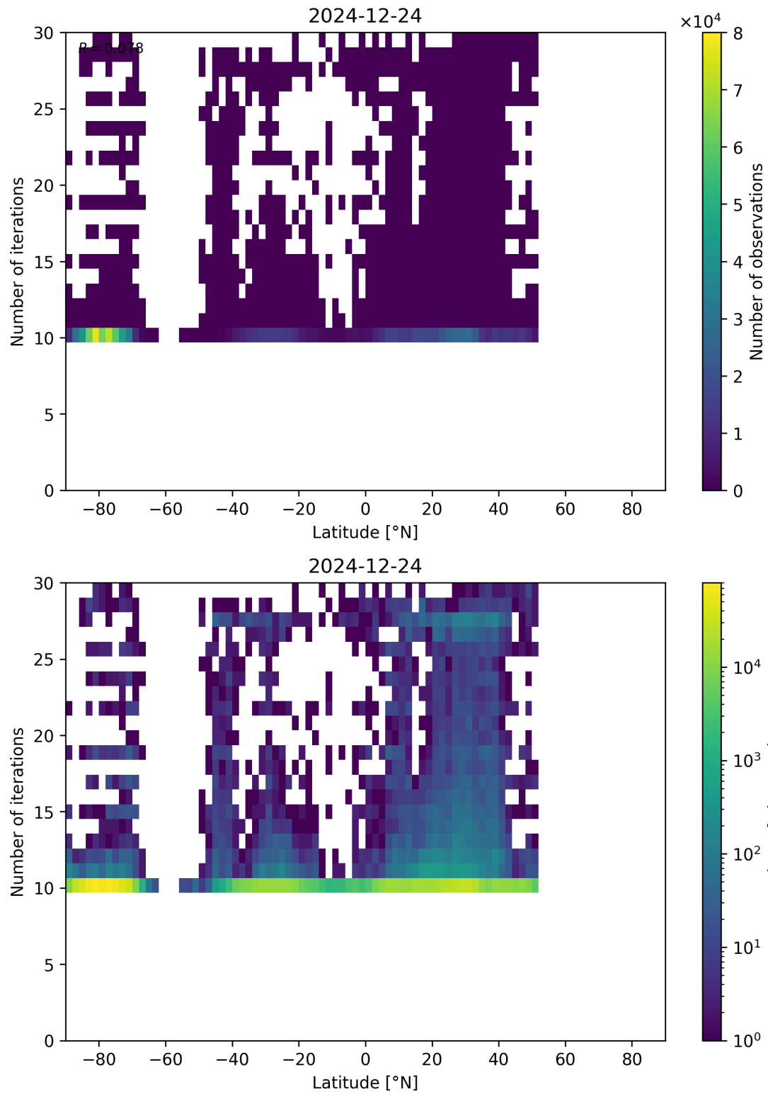
Figure 60: Scatter density plot of “Latitude” against “Number of iterations” for 2024-12-23 to 2024-12-25.
