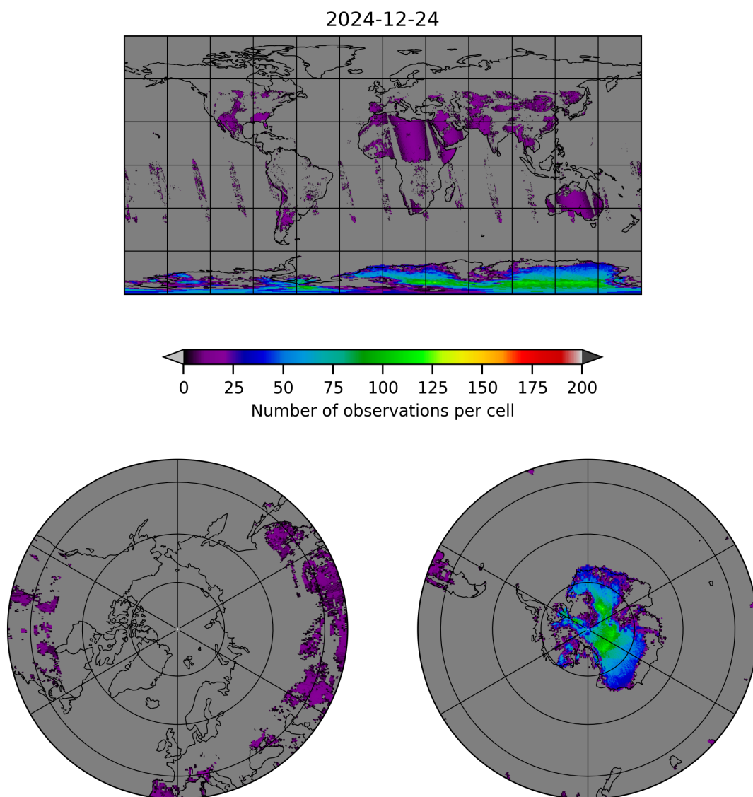
Figure 10: Map of the number of observations for 2024-12-23 to 2024-12-25
