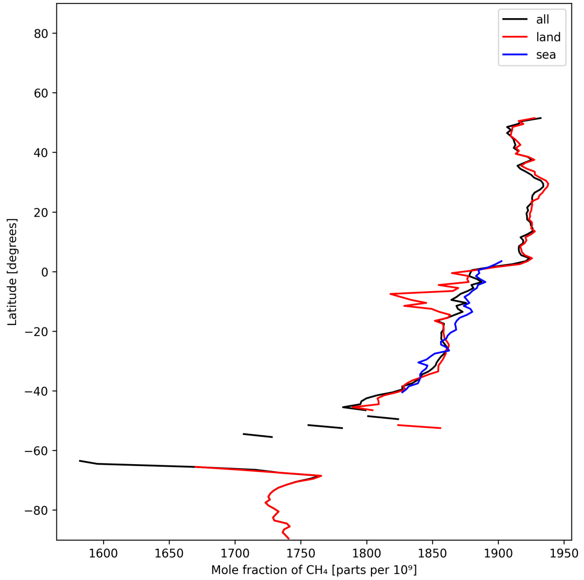
Figure 12: Zonal average of “Mole fraction of \text{CH}_4 ” for 2024-12-23 to 2024-12-25.
