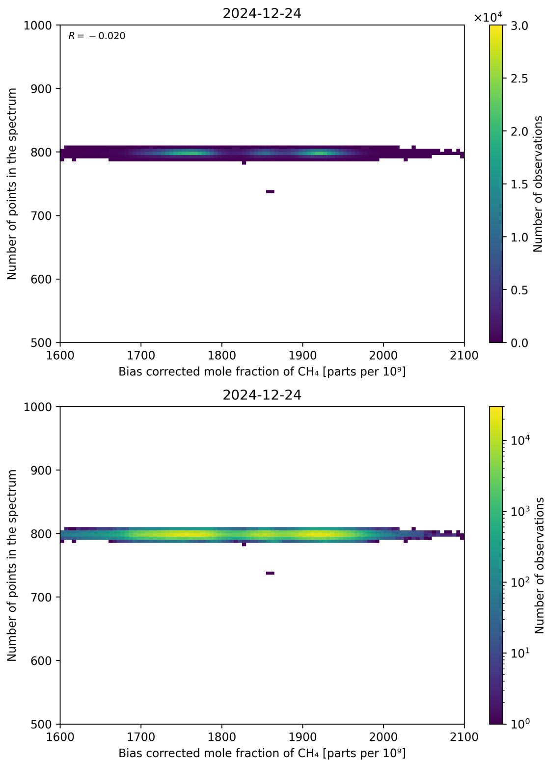
Figure 68: Scatter density plot of “Bias corrected mole fraction of CH 4 ” against “Number of points in the spectrum” for 2024-12-23 to 2024-12-25.
