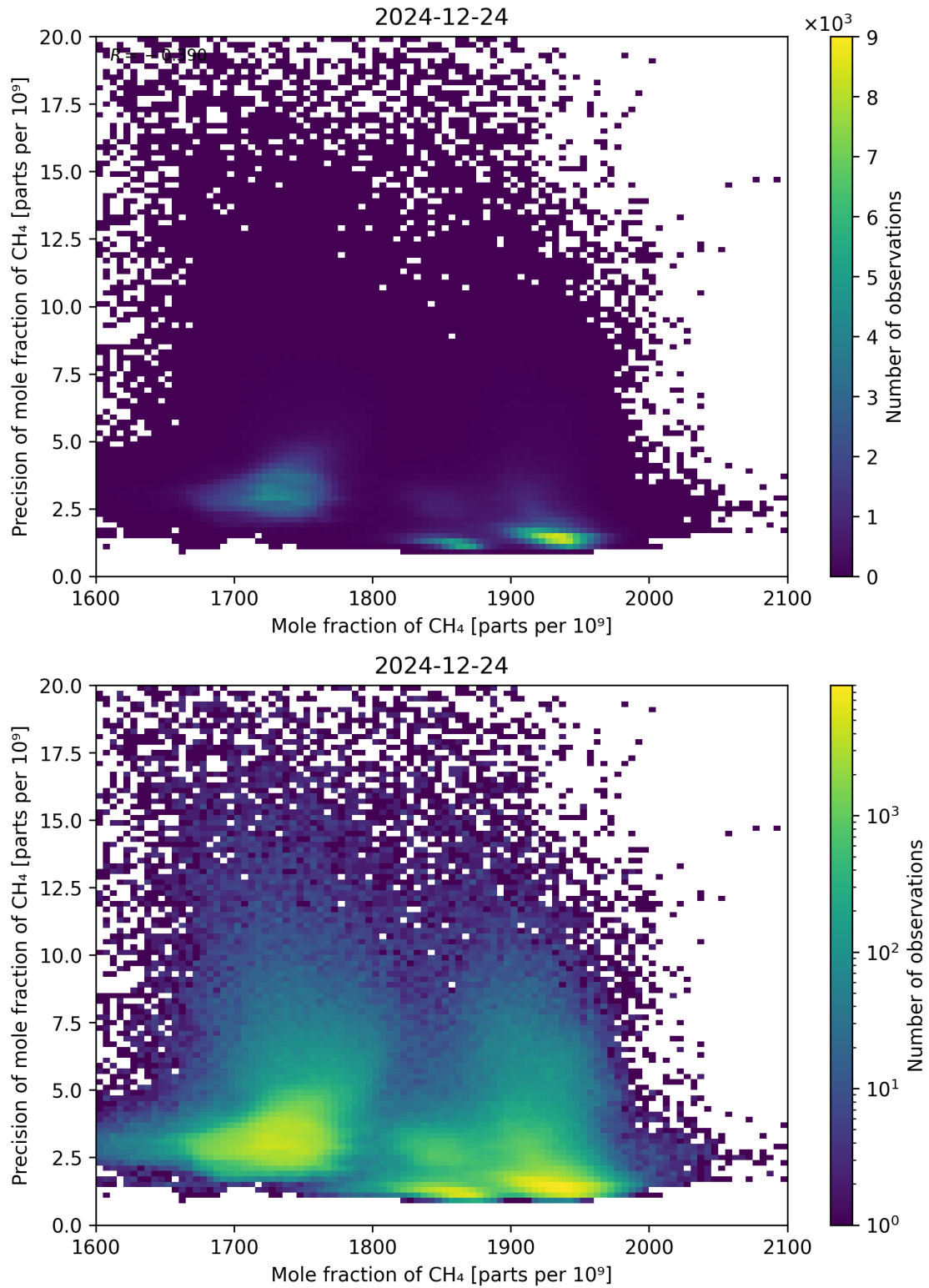
Figure 75: Scatter density plot of “Mole fraction of CH 4 ” against “Precision of mole fraction of CH 4 ” for 2024-12-23 to 2024-12-25.
