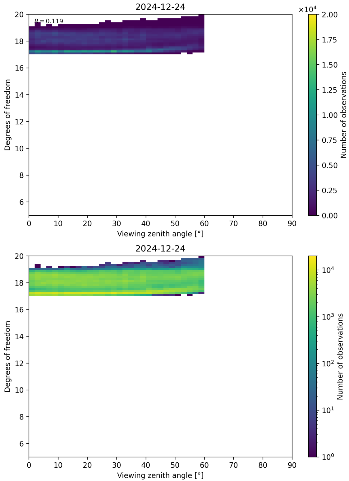
Figure 107: Scatter density plot of “Viewing zenith angle” against “Degrees of freedom” for 2024-12-23 to 2024-12-25.
