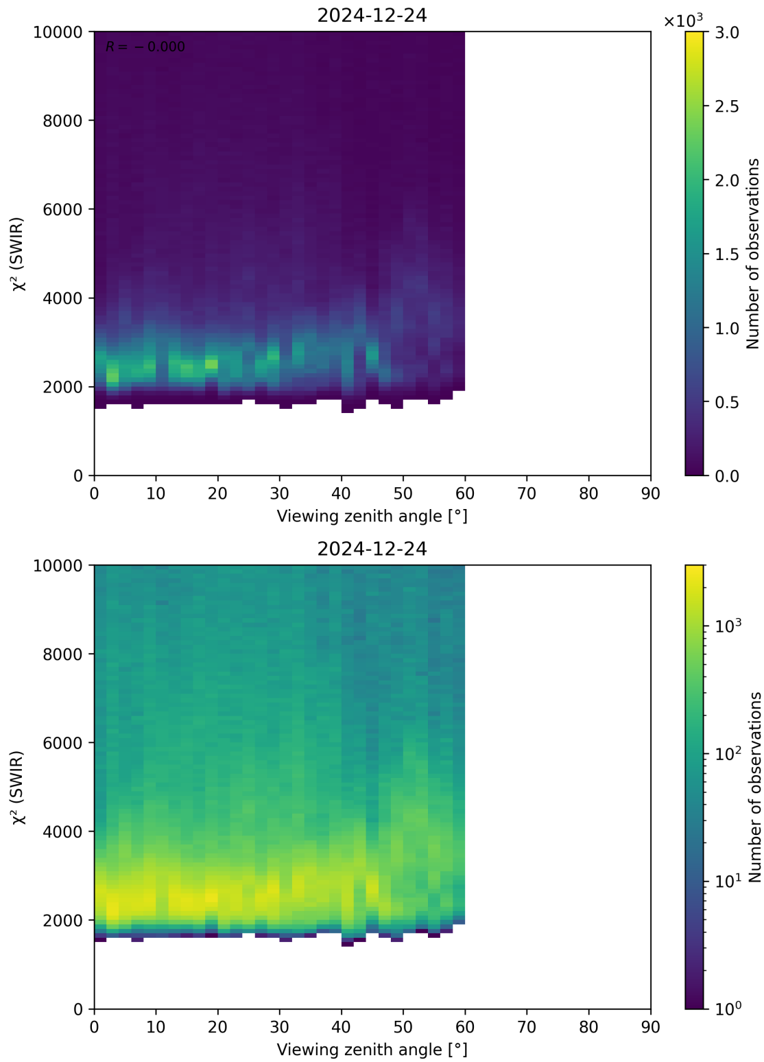
Figure 106: Scatter density plot of “Viewing zenith angle” against “ \chi^2 (SWIR)” for 2024-12-23 to 2024-12-25.
