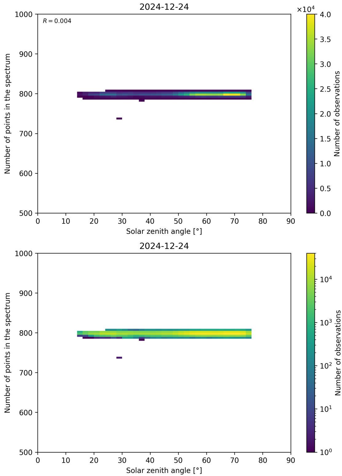
Figure 103: Scatter density plot of “Solar zenith angle” against “Number of points in the spectrum” for 2024-12-23 to 2024-12-25.
