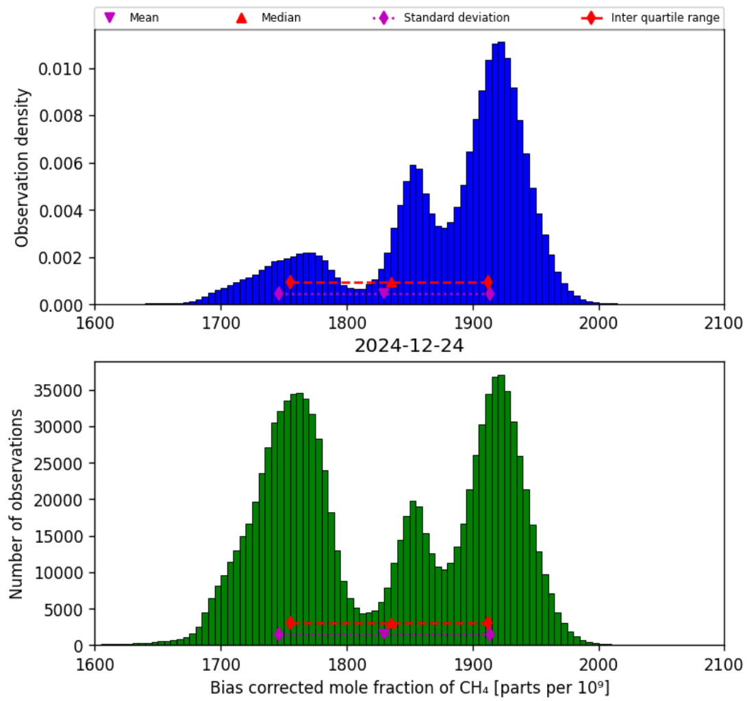
Figure 25: Histogram of “Bias corrected mole fraction of CH 4 ” for 2024-12-23 to 2024-12-25
