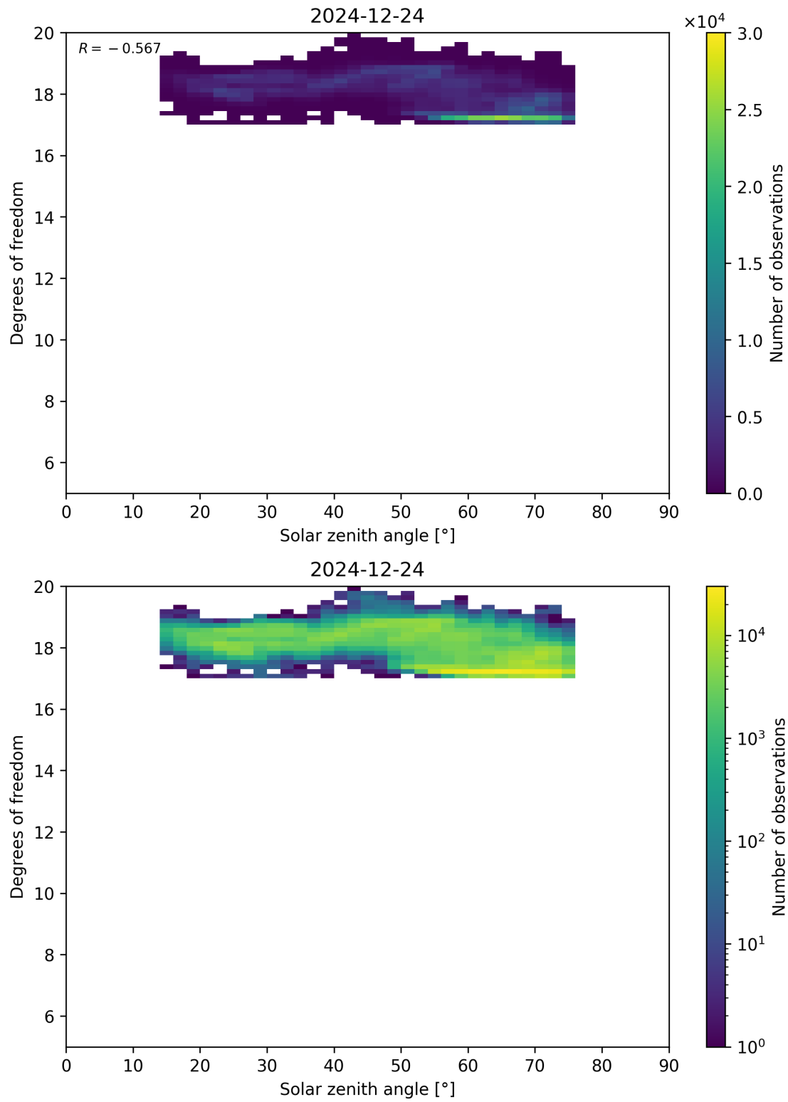
Figure 96: Scatter density plot of “Solar zenith angle” against “Degrees of freedom” for 2024-12-23 to 2024-12-25.
