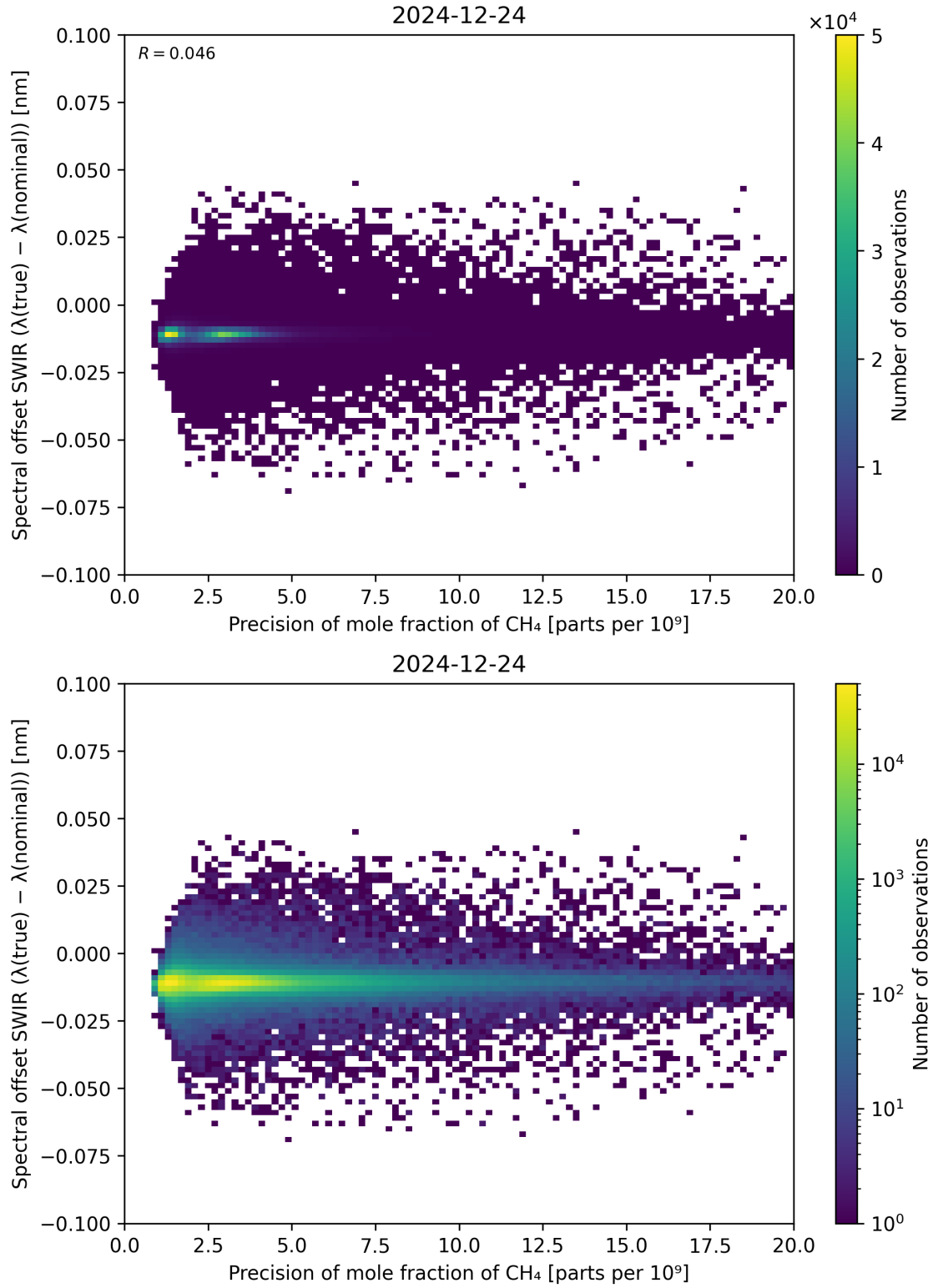
Figure 85: Scatter density plot of “Precision of mole fraction of CH 4 ” against “Spectral offset SWIR ( \lambda_{\text{true}} - \lambda_{\text{nominal}} )” for 2024-12-23 to 2024-12-25.
