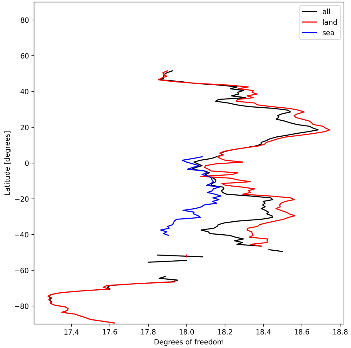
Figure 19: Zonal average of “Degrees of freedom” for 2024-12-23 to 2024-12-25.
