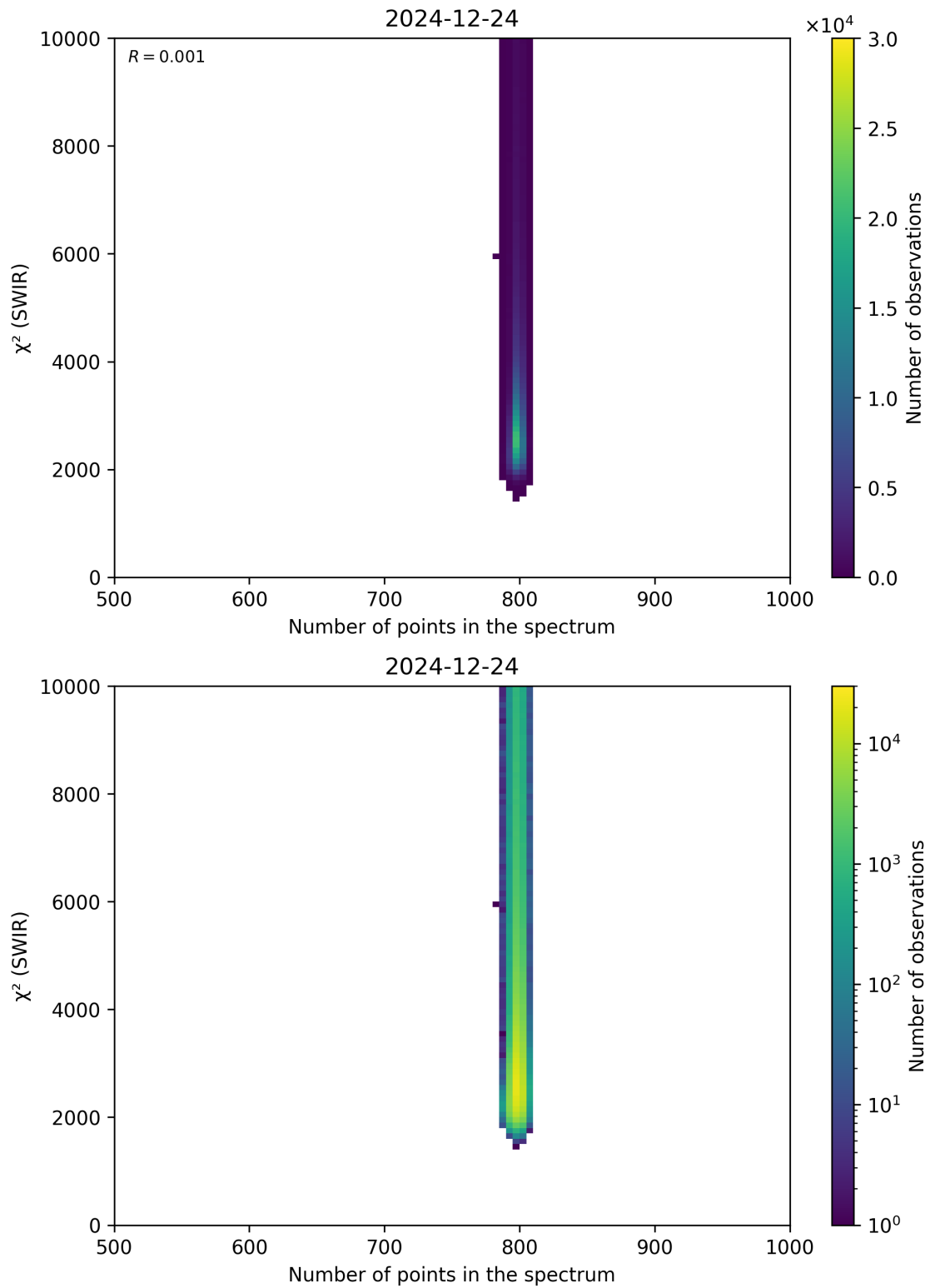
Figure 89: Scatter density plot of “Number of points in the spectrum” against “ \chi^2 (SWIR)” for 2024-12-23 to 2024-12-25.
