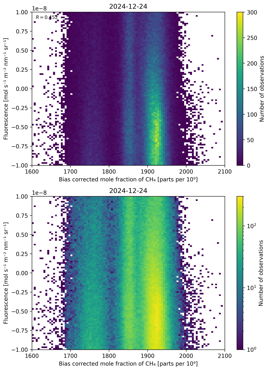
Figure 66: Scatter density plot of “Bias corrected mole fraction of \text{CH}_4 ” against “Fluorescence” for 2024-12-23 to 2024-12-25.
