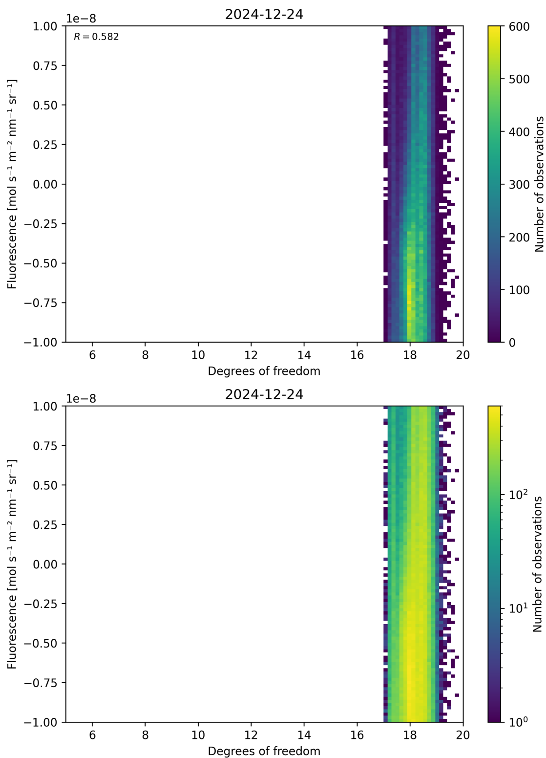
Figure 51: Scatter density plot of “Degrees of freedom” against “Fluorescence” for 2024-12-23 to 2024-12-25.
