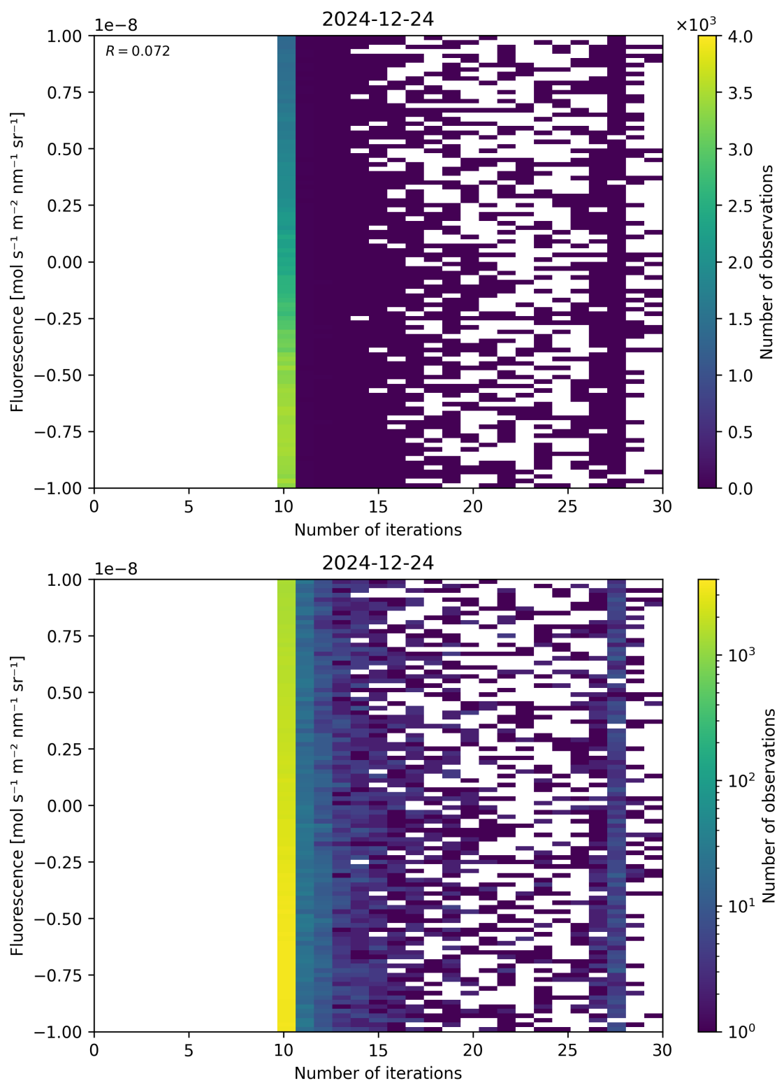
Figure 87: Scatter density plot of “Number of iterations” against “Fluorescence” for 2024-12-23 to 2024-12-25.
