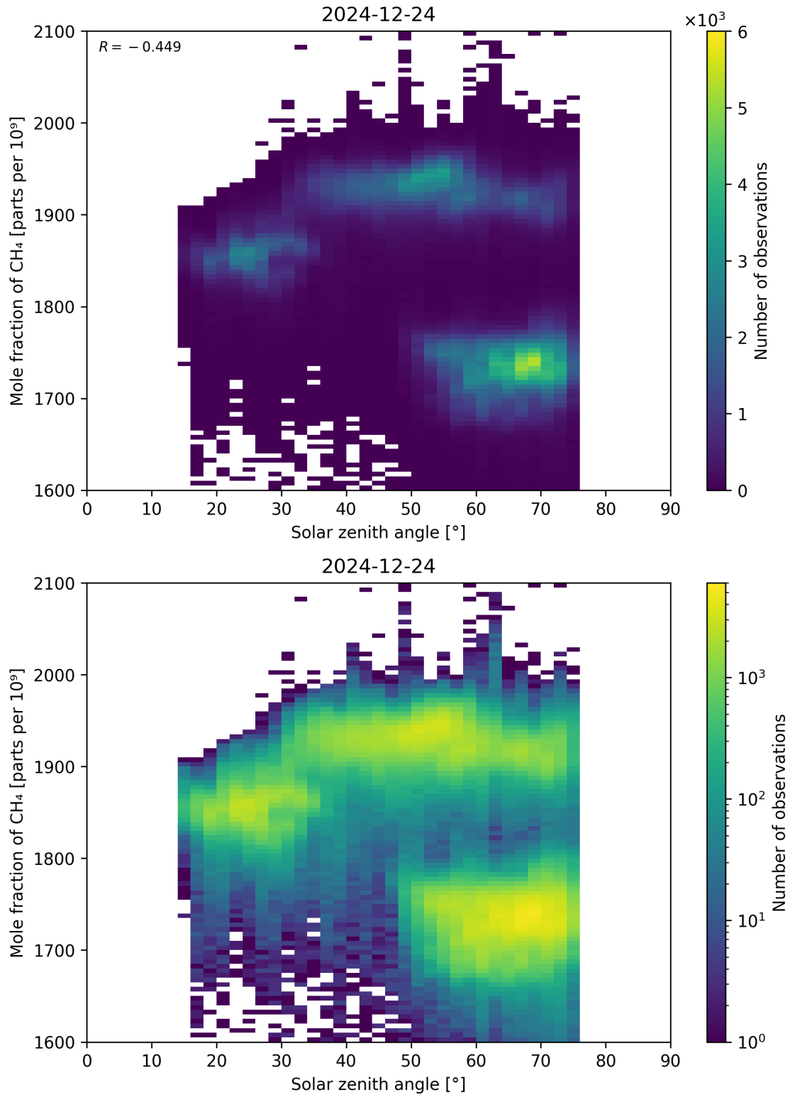
Figure 99: Scatter density plot of “Solar zenith angle” against “Mole fraction of \text{CH}_4 ” for 2024-12-23 to 2024-12-25.
