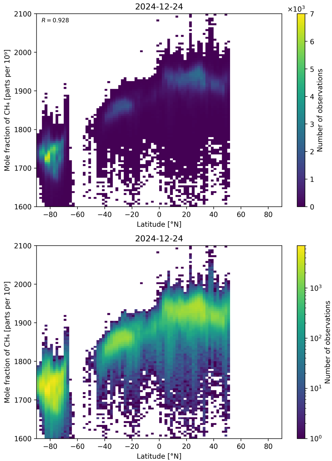
Figure 57: Scatter density plot of “Latitude” against “Mole fraction of CH 4 ” for 2024-12-23 to 2024-12-25.
