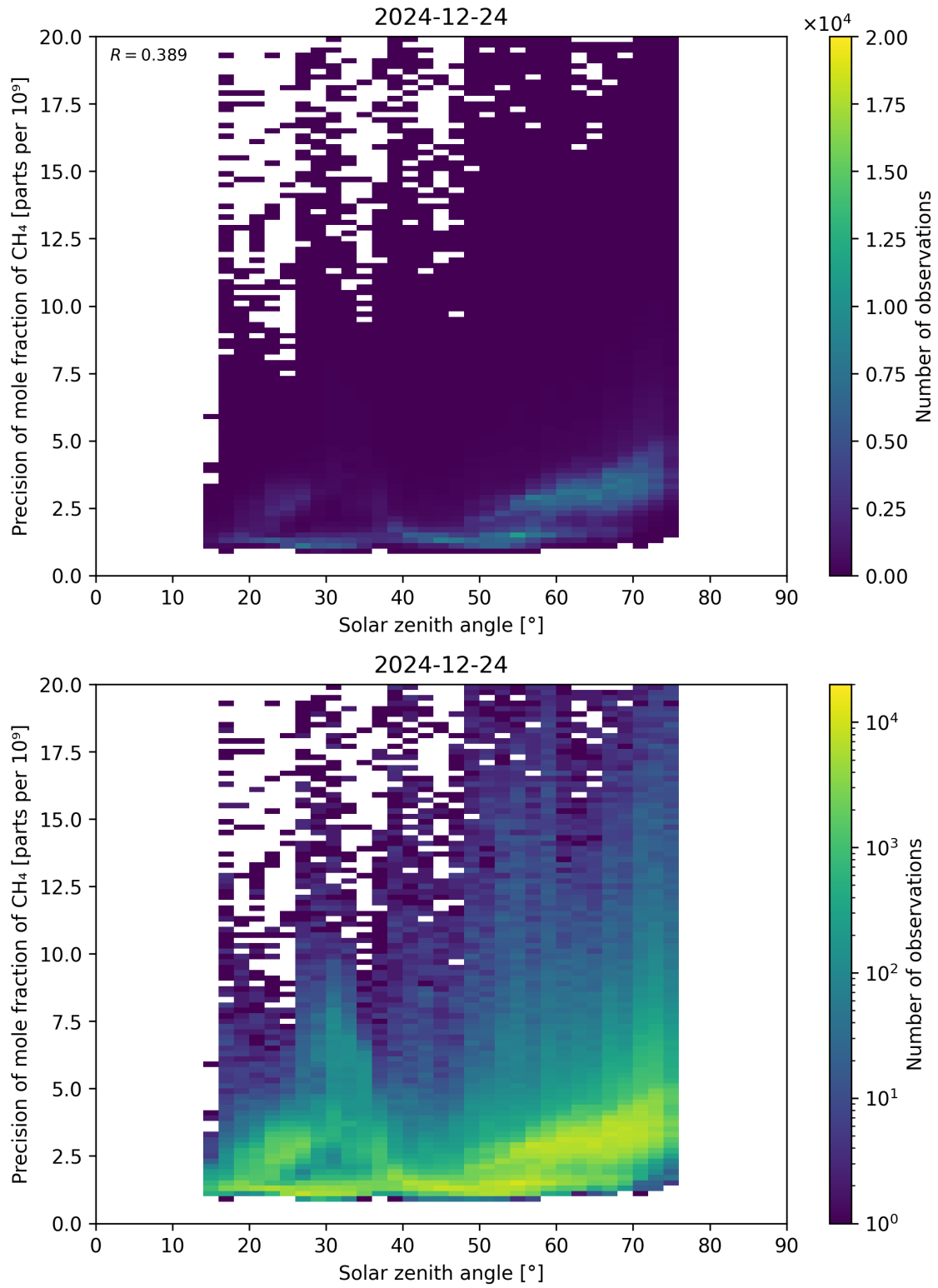
Figure 101: Scatter density plot of “Solar zenith angle” against “Precision of mole fraction of \text{CH}_4 ” for 2024-12-23 to 2024-12-25.
