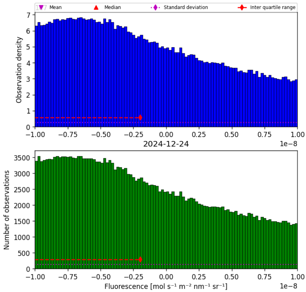
Figure 32: Histogram of “Fluorescence” for 2024-12-23 to 2024-12-25
