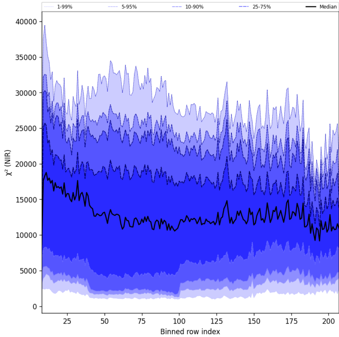
Figure 40: Along track statistics of “ \chi^2 (NIR)” for 2024-12-23 to 2024-12-25
