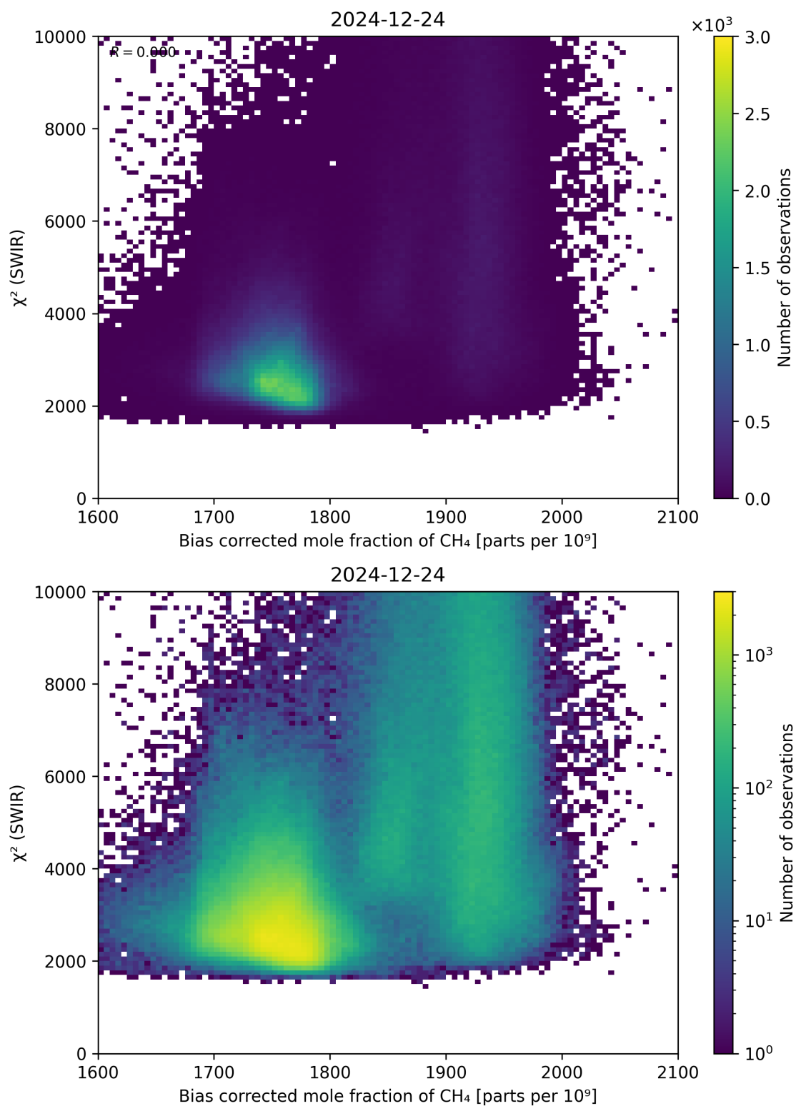
Figure 64: Scatter density plot of “Bias corrected mole fraction of \text{CH}_4 ” against “ \chi^2 (SWIR)” for 2024-12-23 to 2024-12-25.
