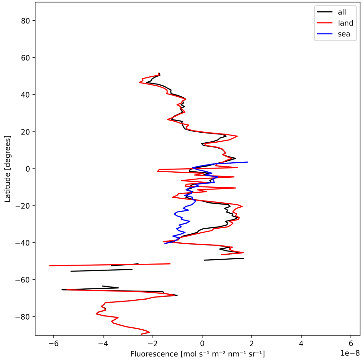
Figure 21: Zonal average of “Fluorescence” for 2024-12-23 to 2024-12-25.
