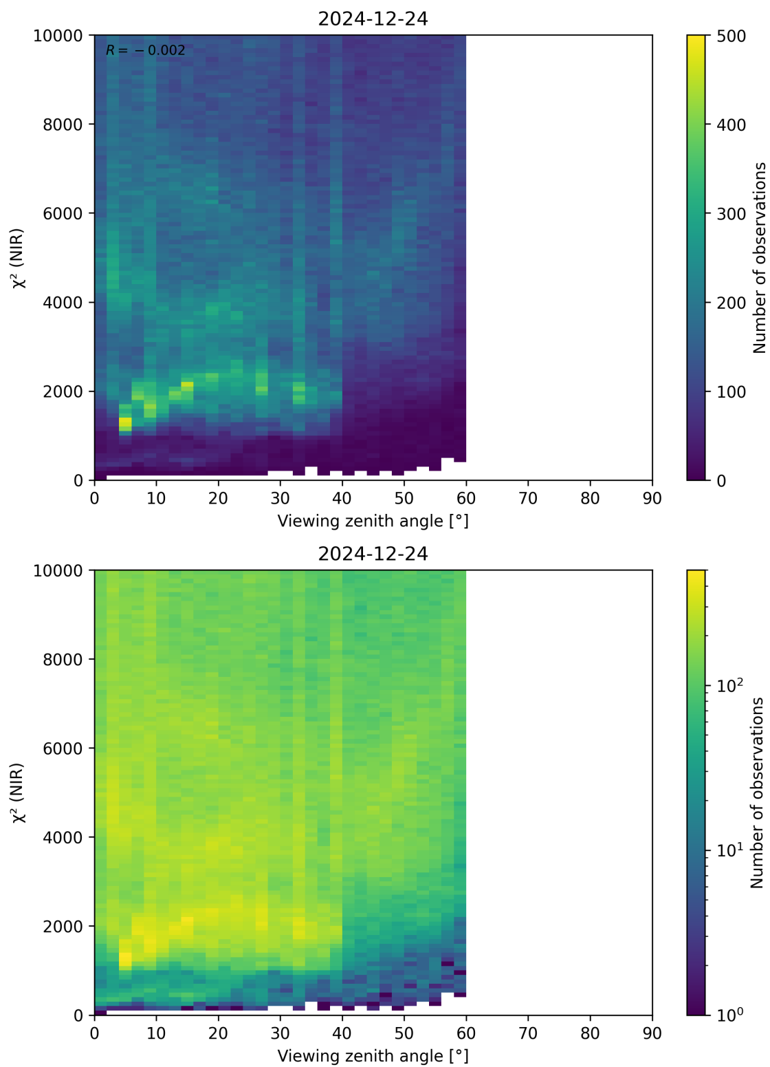
Figure 105: Scatter density plot of “Viewing zenith angle” against “ \chi^2 (NIR)” for 2024-12-23 to 2024-12-25.
