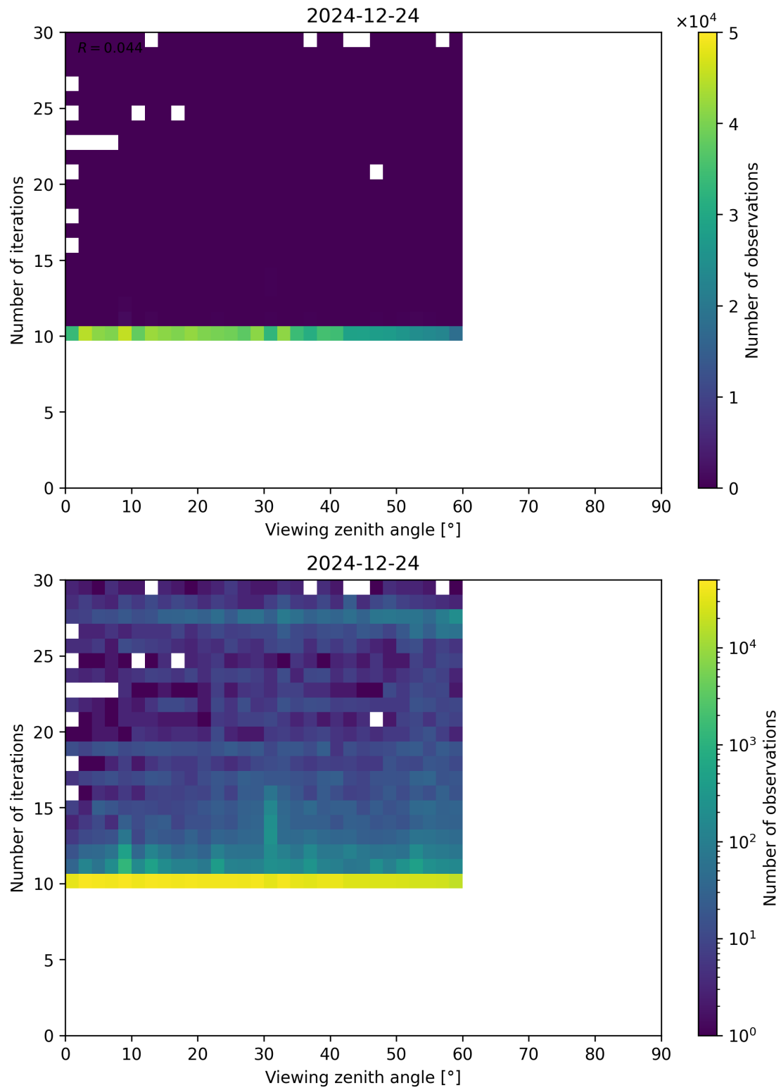
Figure 113: Scatter density plot of “Viewing zenith angle” against “Number of iterations” for 2024-12-23 to 2024-12-25.
