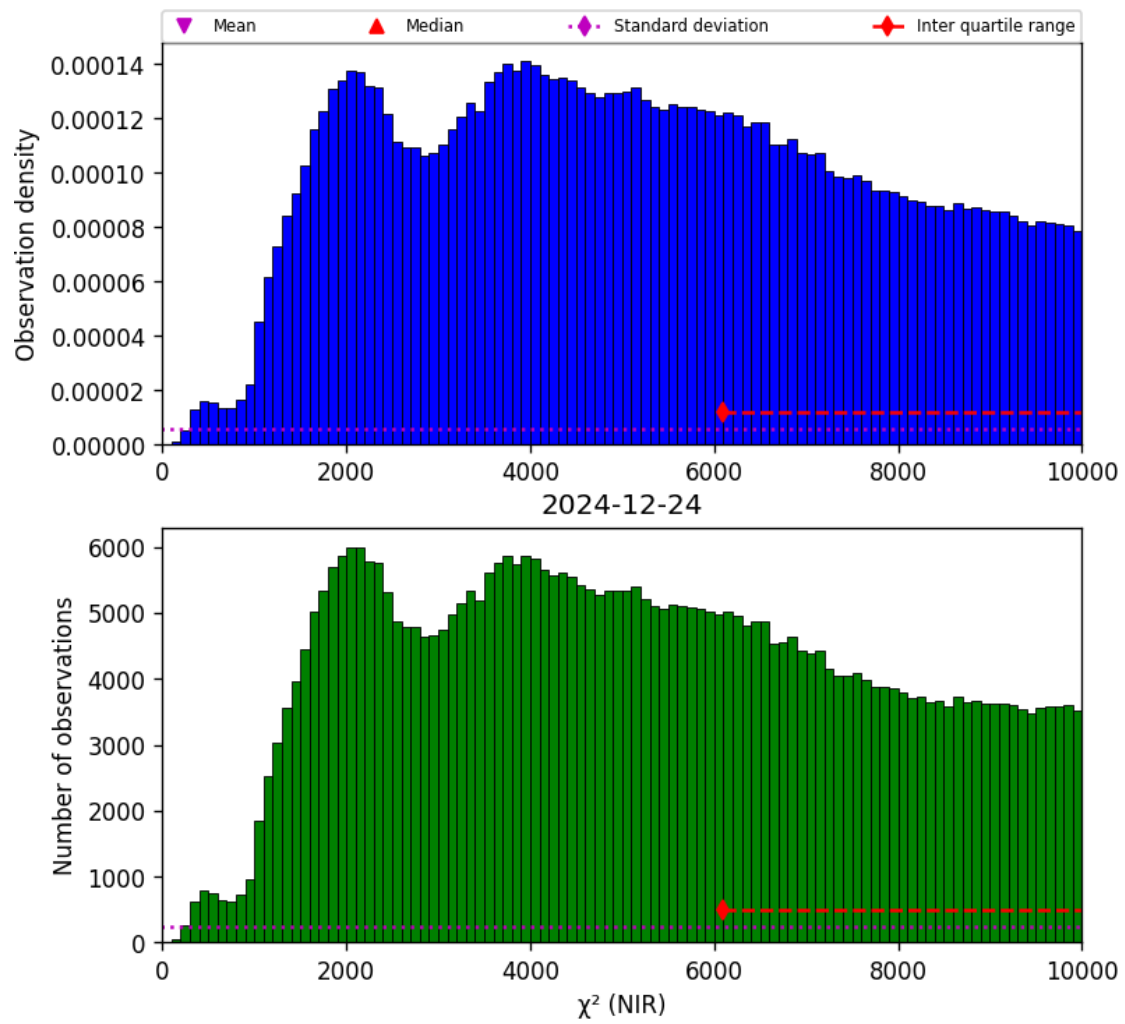
Figure 29: Histogram of “ \chi^2 (NIR)” for 2024-12-23 to 2024-12-25
