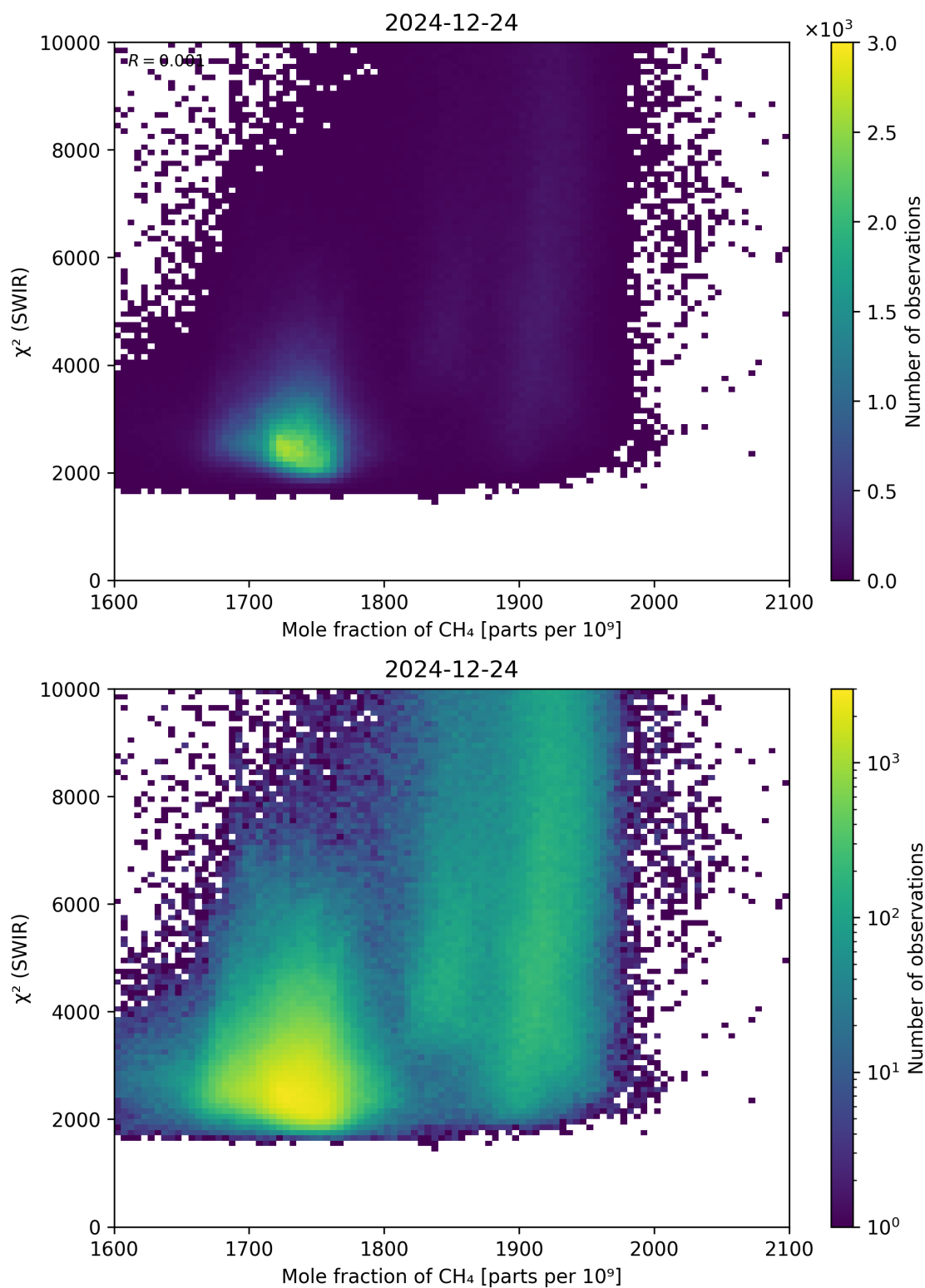
Figure 71: Scatter density plot of “Mole fraction of CH 4 ” against “ \chi^2 (SWIR)” for 2024-12-23 to 2024-12-25.
