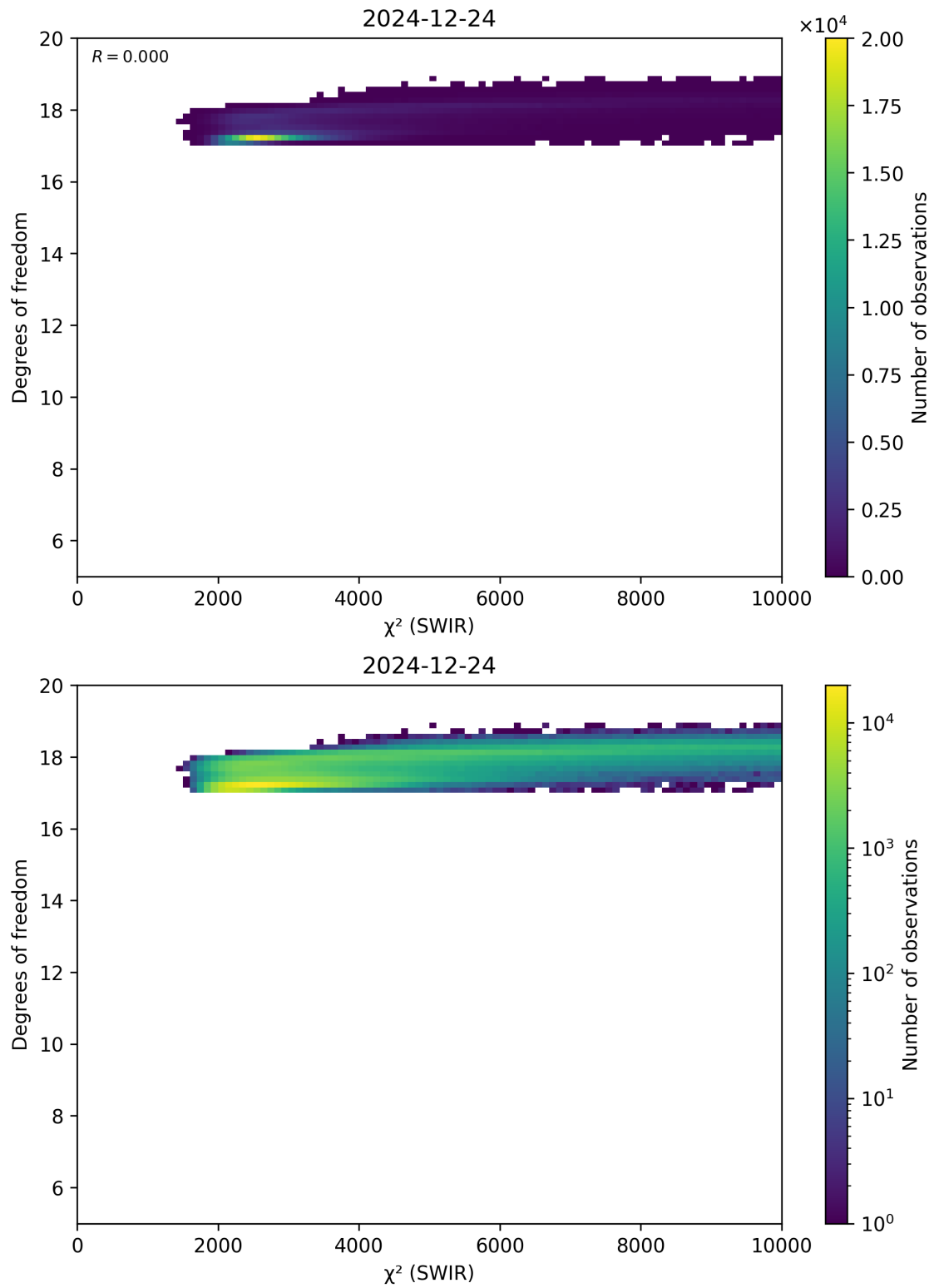
Figure 48: Scatter density plot of “ \chi^2 (SWIR)” against “Degrees of freedom” for 2024-12-23 to 2024-12-25.
