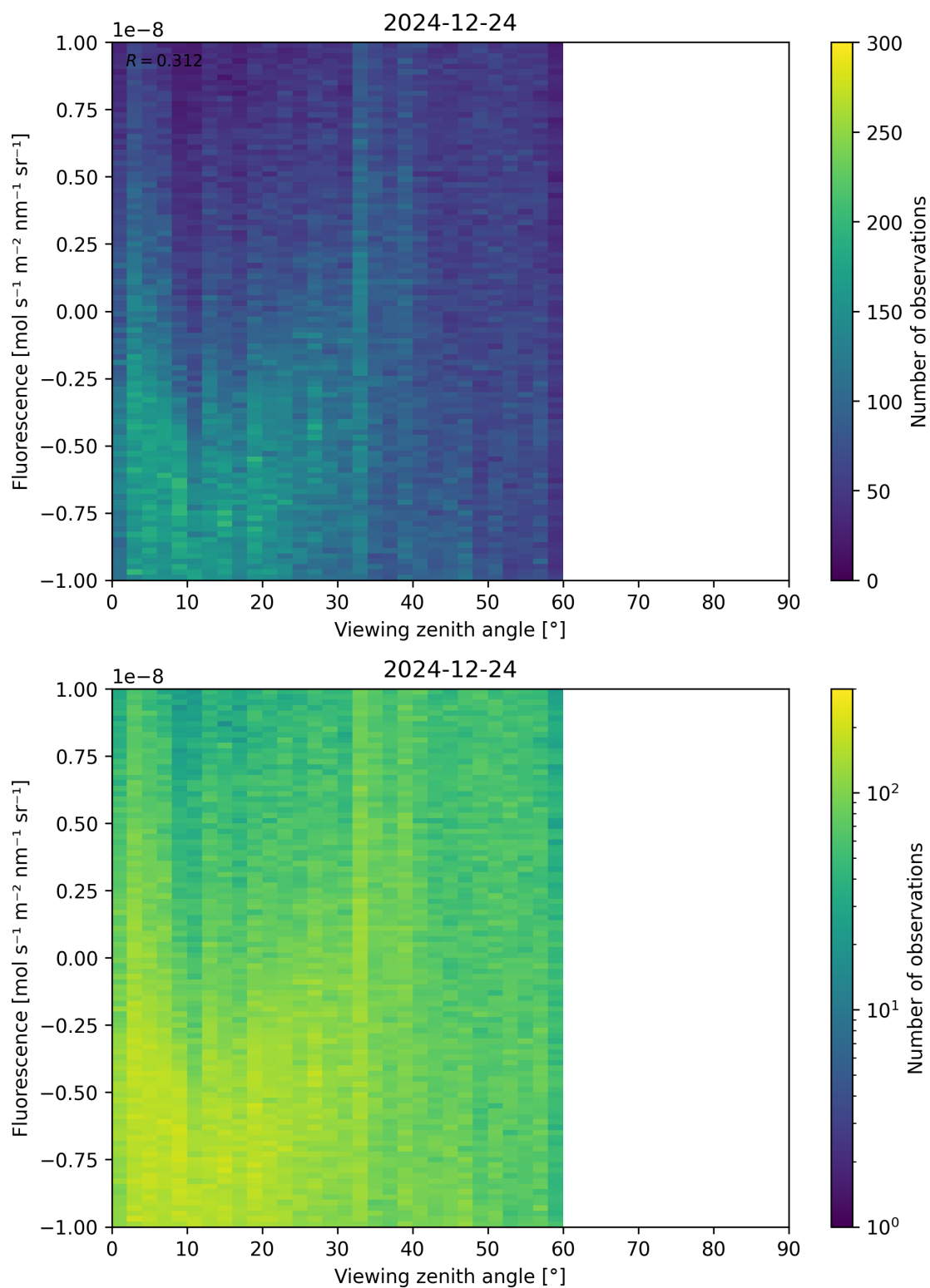
Figure 108: Scatter density plot of “Viewing zenith angle” against “Fluorescence” for 2024-12-23 to 2024-12-25.
