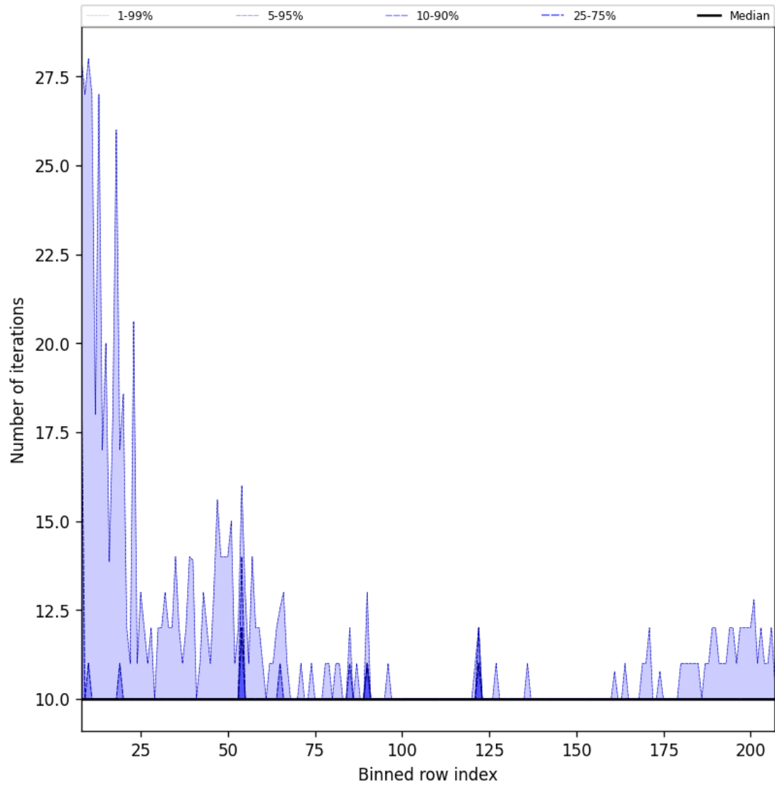
Figure 42: Along track statistics of “Number of iterations” for 2024-12-23 to 2024-12-25
