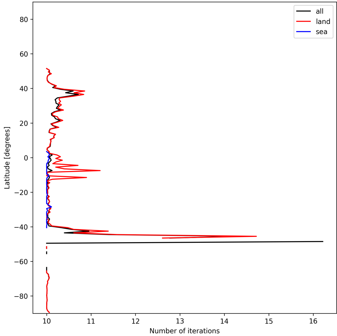
Figure 20: Zonal average of “Number of iterations” for 2024-12-23 to 2024-12-25.
