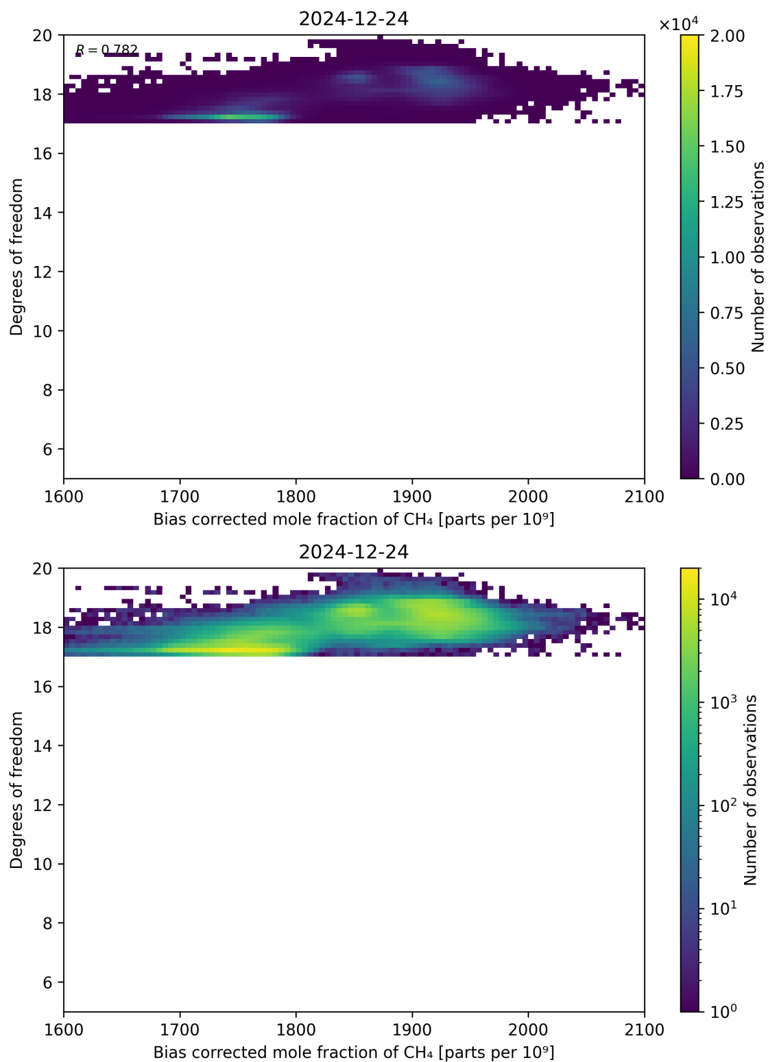
Figure 65: Scatter density plot of “Bias corrected mole fraction of CH 4 ” against “Degrees of freedom” for 2024-12-23 to 2024-12-25.
