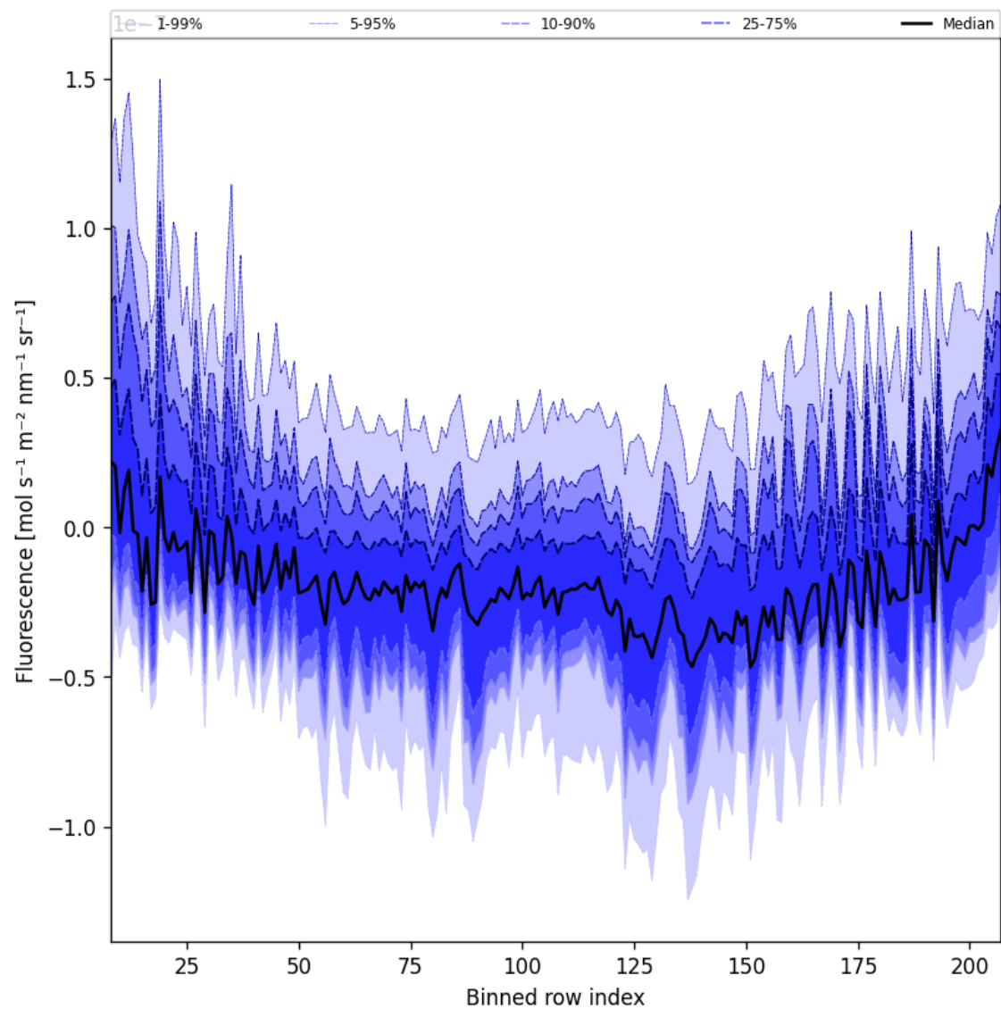
Figure 43: Along track statistics of “Fluorescence” for 2024-12-23 to 2024-12-25
