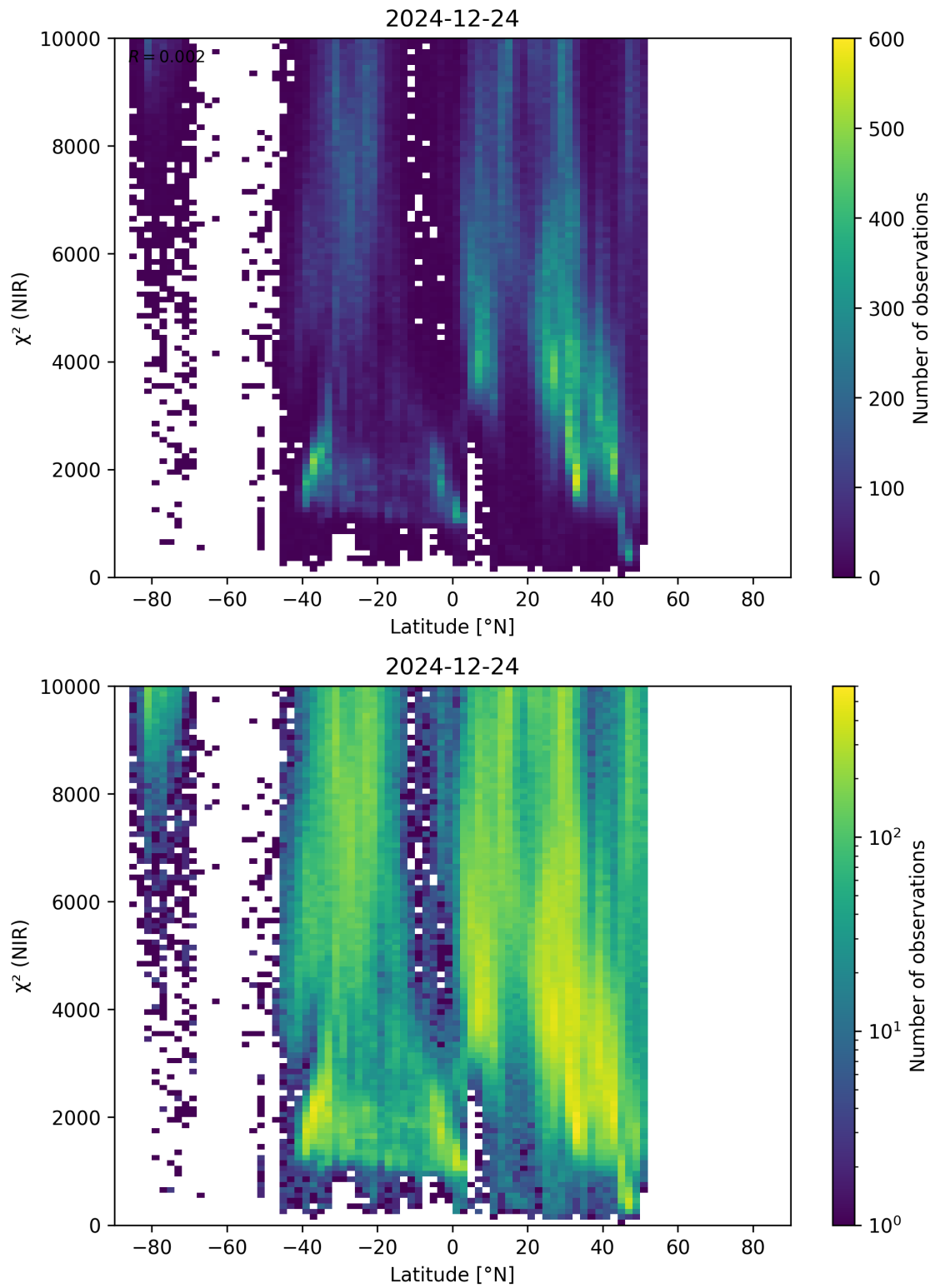
Figure 53: Scatter density plot of “Latitude” against “ \chi^2 (NIR)” for 2024-12-23 to 2024-12-25.
