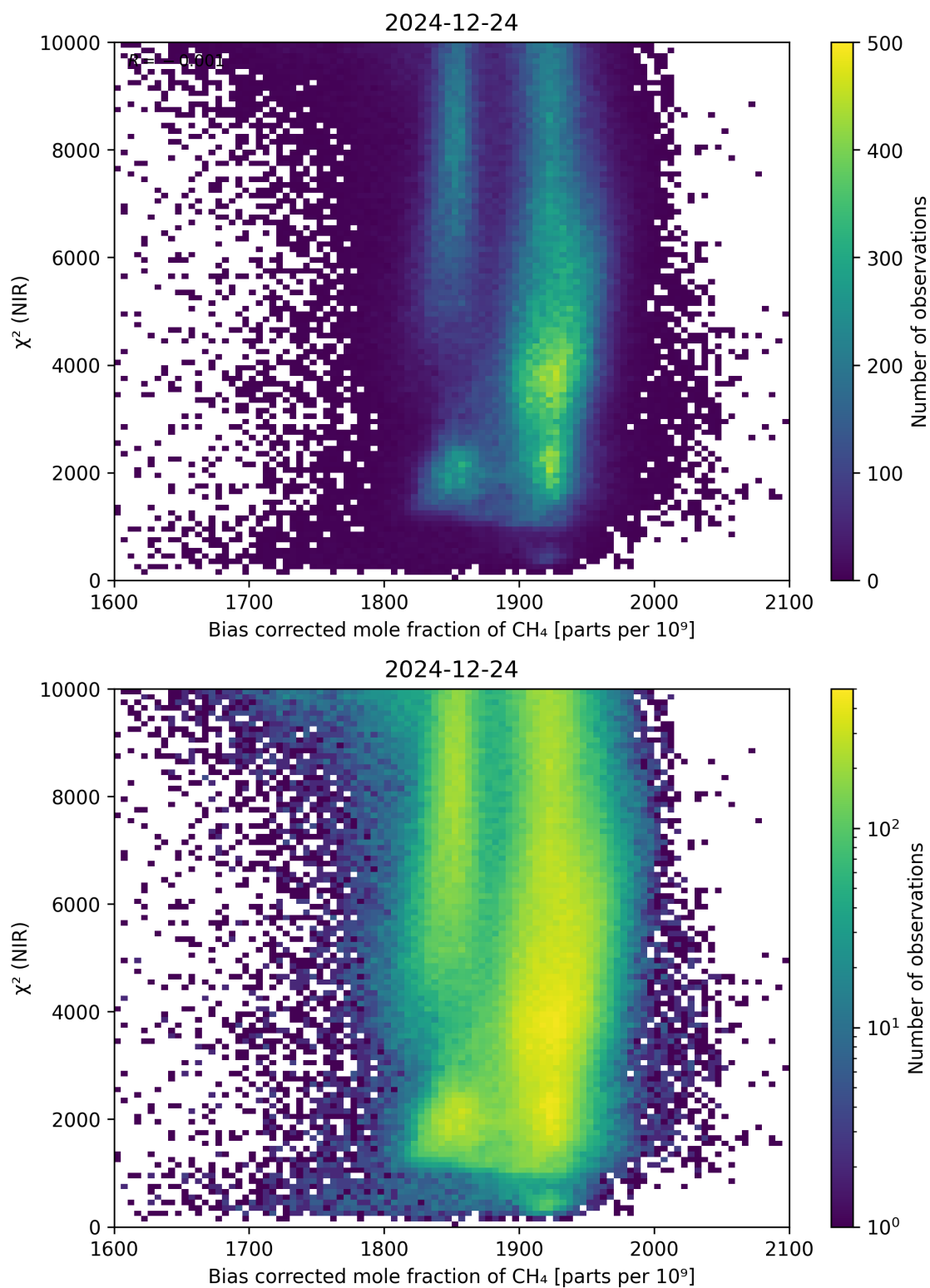
Figure 63: Scatter density plot of “Bias corrected mole fraction of CH 4 ” against “ \chi^2 (NIR)” for 2024-12-23 to 2024-12-25.
