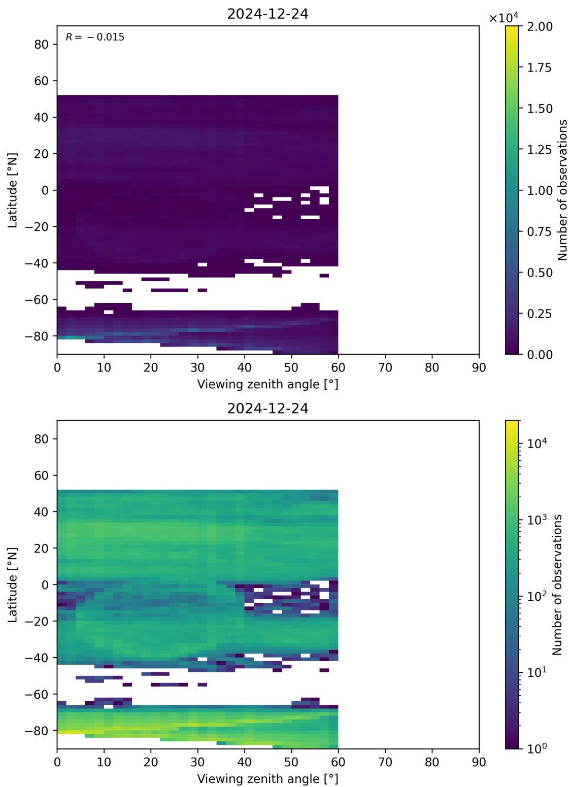
Figure 109: Scatter density plot of “Viewing zenith angle” against “Latitude” for 2024-12-23 to 2024-12-25.
