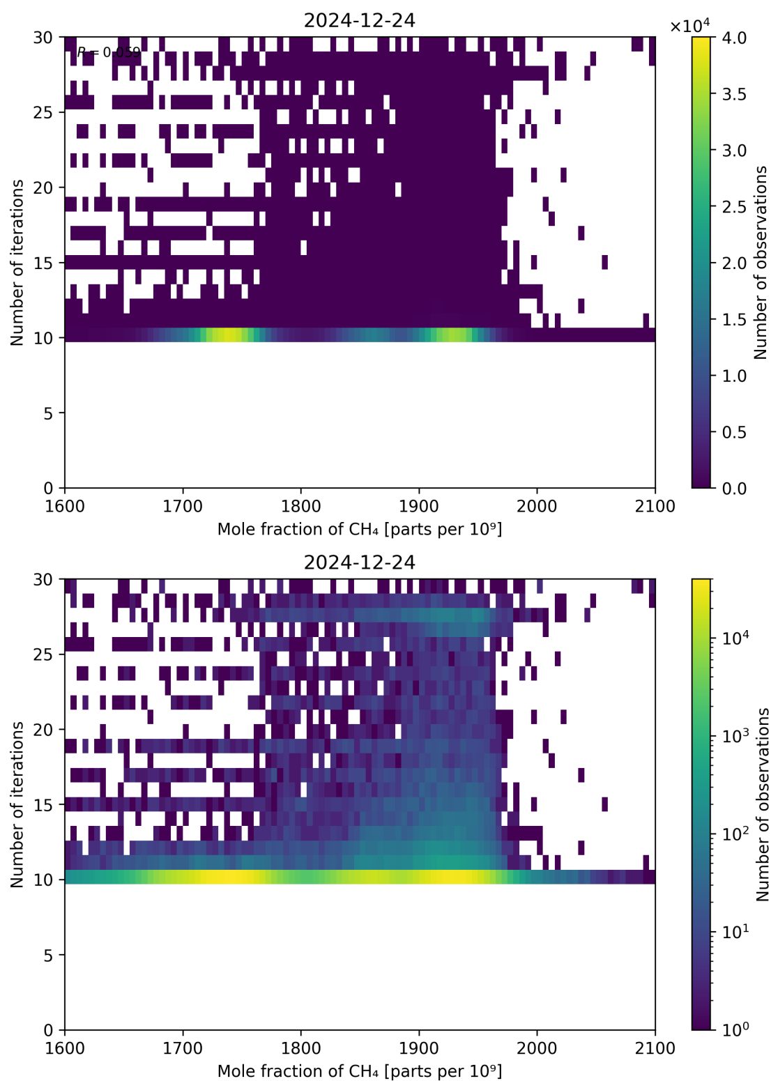
Figure 76: Scatter density plot of “Mole fraction of CH 4 ” against “Number of iterations” for 2024-12-23 to 2024-12-25.
