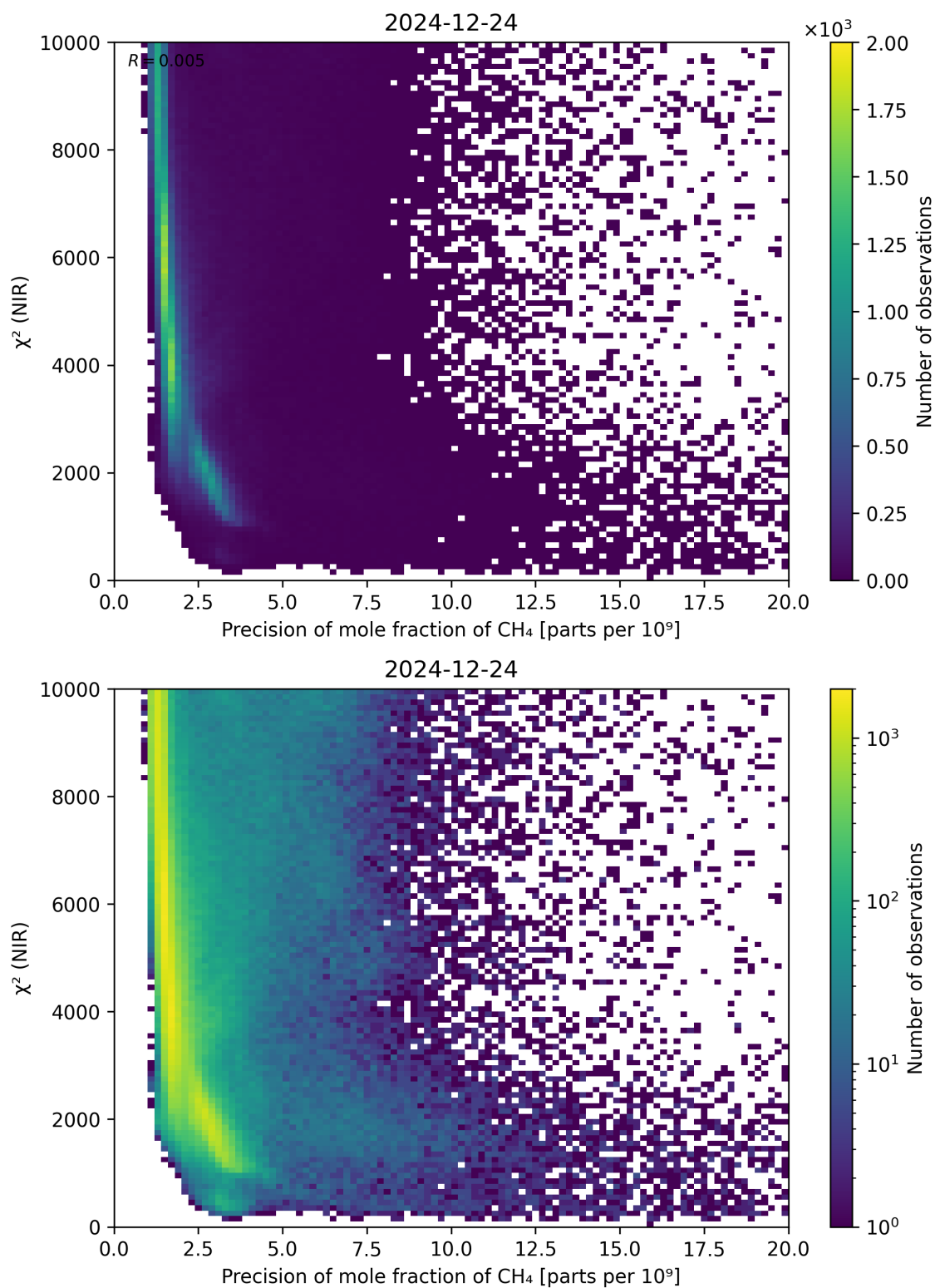
Figure 78: Scatter density plot of “Precision of mole fraction of \text{CH}_4 ” against “ \chi^2 (NIR)” for 2024-12-23 to 2024-12-25.
