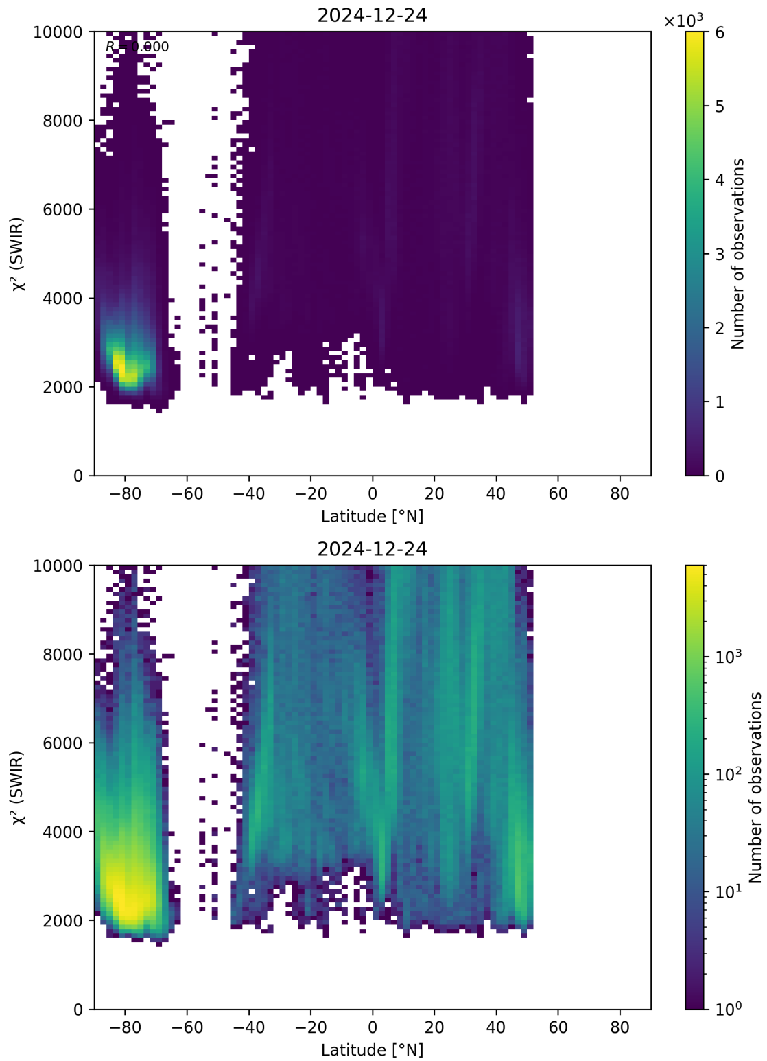
Figure 54: Scatter density plot of “Latitude” against “ \chi^2 (SWIR)” for 2024-12-23 to 2024-12-25.
