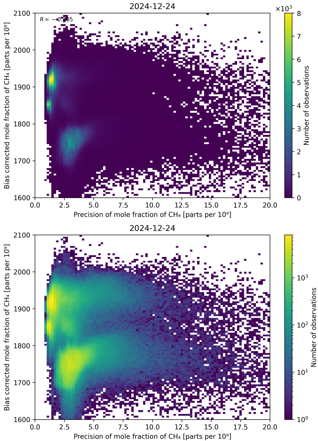
Figure 82: Scatter density plot of “Precision of mole fraction of CH 4 ” against “Bias corrected mole fraction of CH 4 ” for 2024-12-23 to 2024-12-25.
