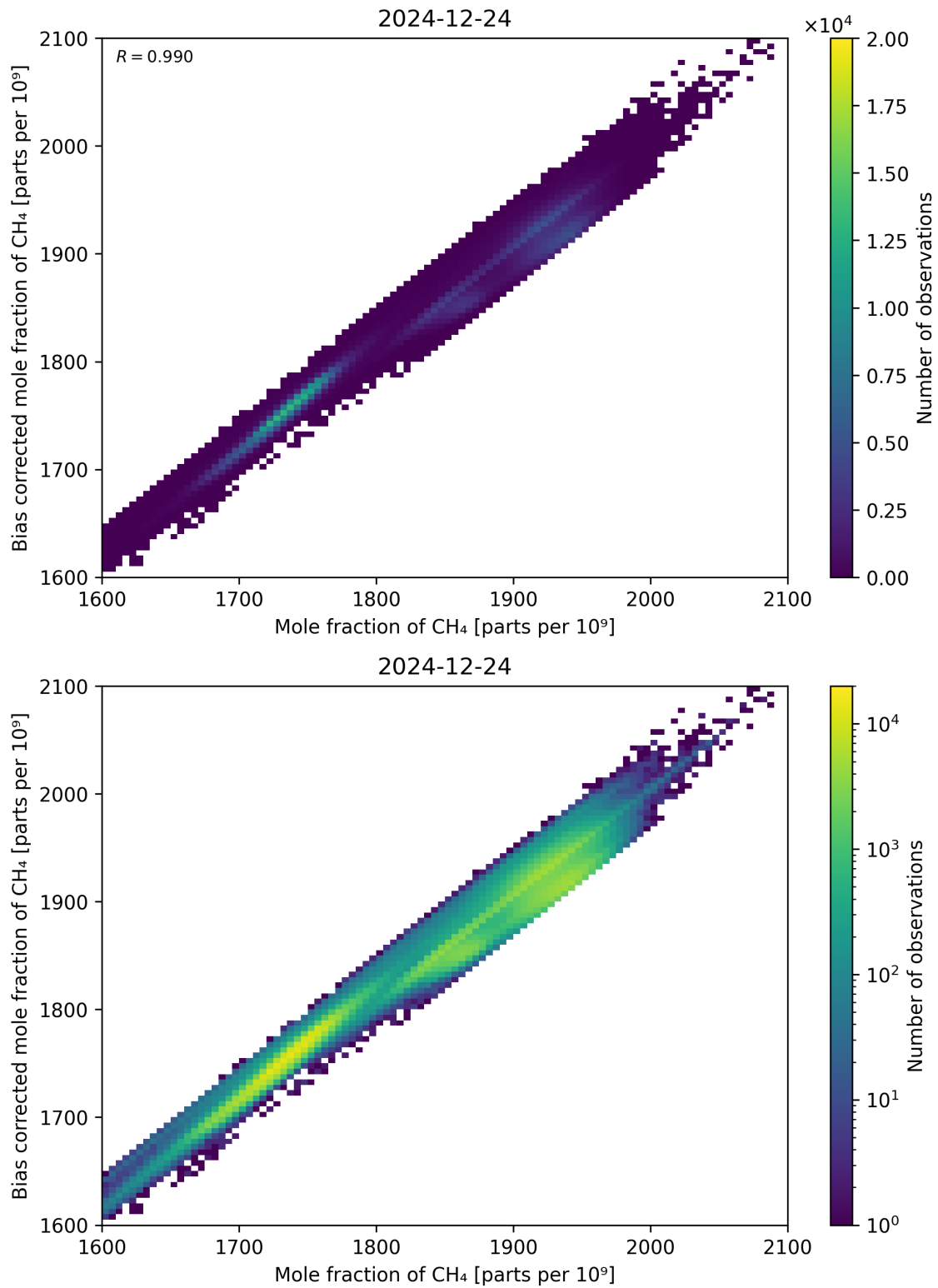
Figure 74: Scatter density plot of “Mole fraction of CH 4 ” against “Bias corrected mole fraction of CH 4 ” for 2024-12-23 to 2024-12-25.
