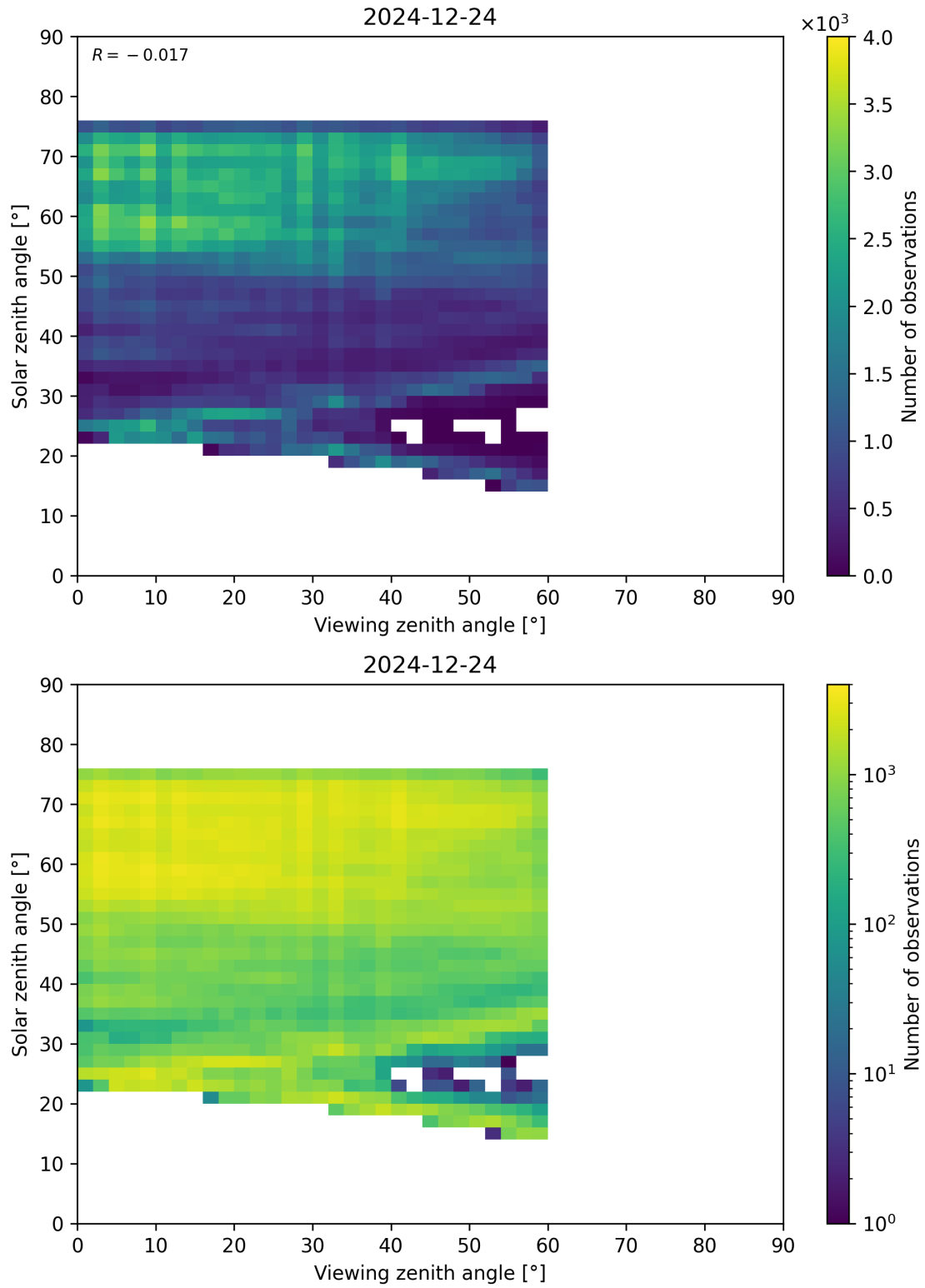
Figure 115: Scatter density plot of “Viewing zenith angle” against “Solar zenith angle” for 2024-12-23 to 2024-12-25.
