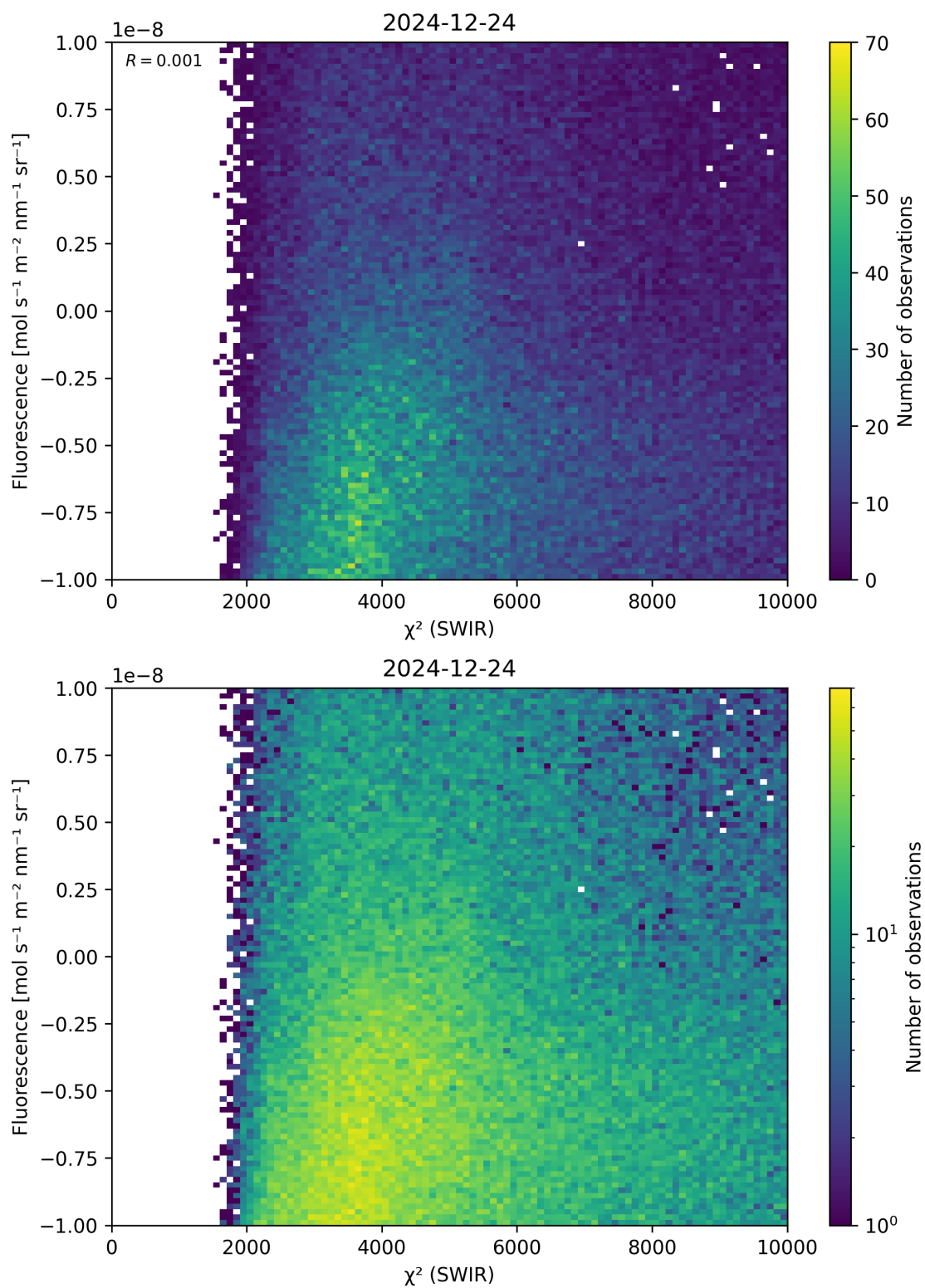
Figure 49: Scatter density plot of “ \chi^2 (SWIR)” against “Fluorescence” for 2024-12-23 to 2024-12-25.
