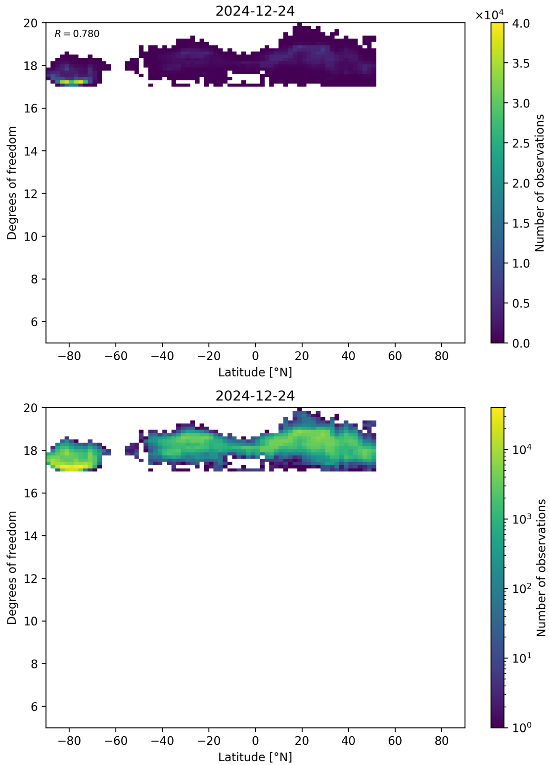
Figure 55: Scatter density plot of “Latitude” against “Degrees of freedom” for 2024-12-23 to 2024-12-25.
