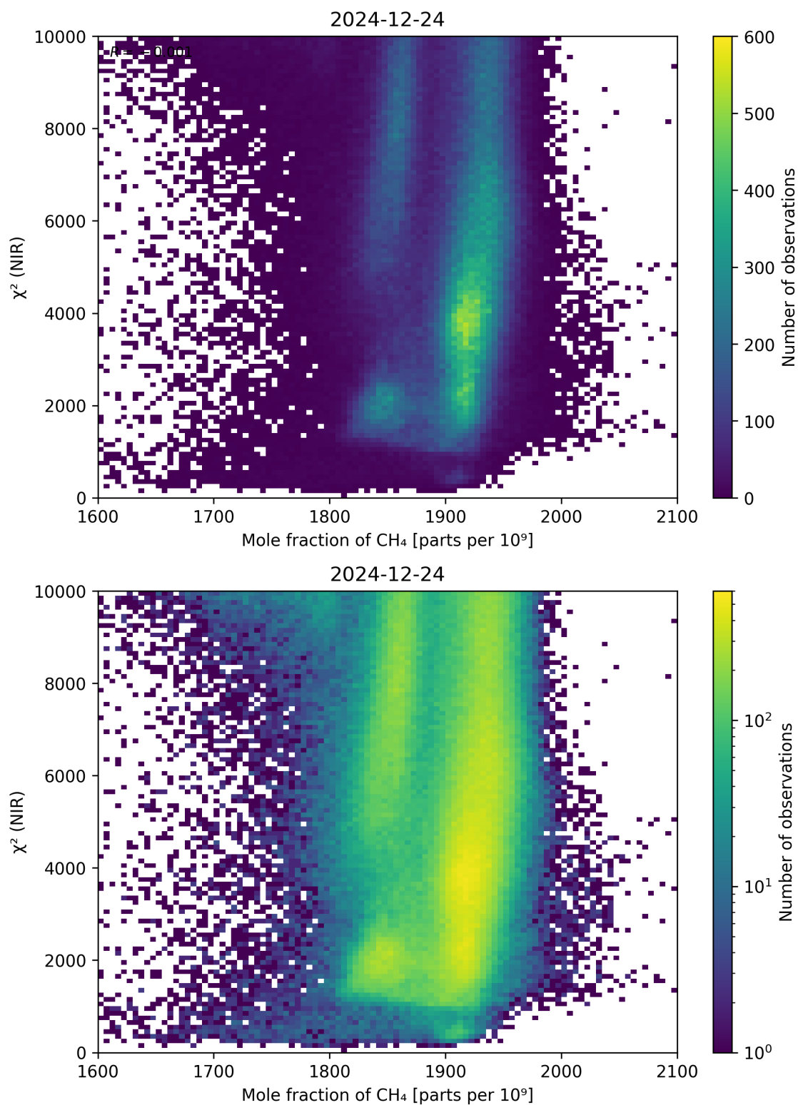
Figure 70: Scatter density plot of “Mole fraction of \text{CH}_4 ” against “ \chi^2 (NIR)” for 2024-12-23 to 2024-12-25.
