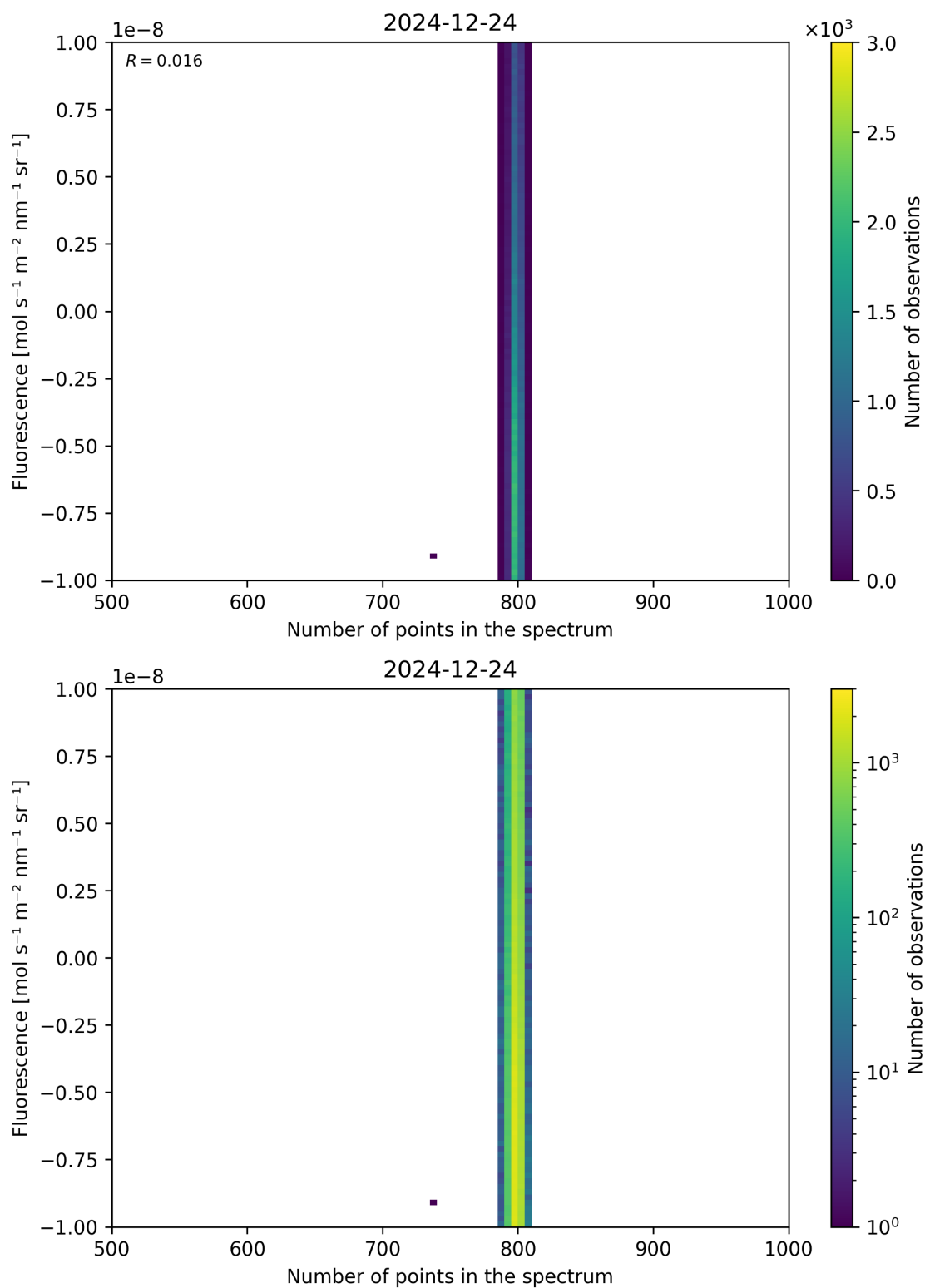
Figure 91: Scatter density plot of “Number of points in the spectrum” against “Fluorescence” for 2024-12-23 to 2024-12-25.
