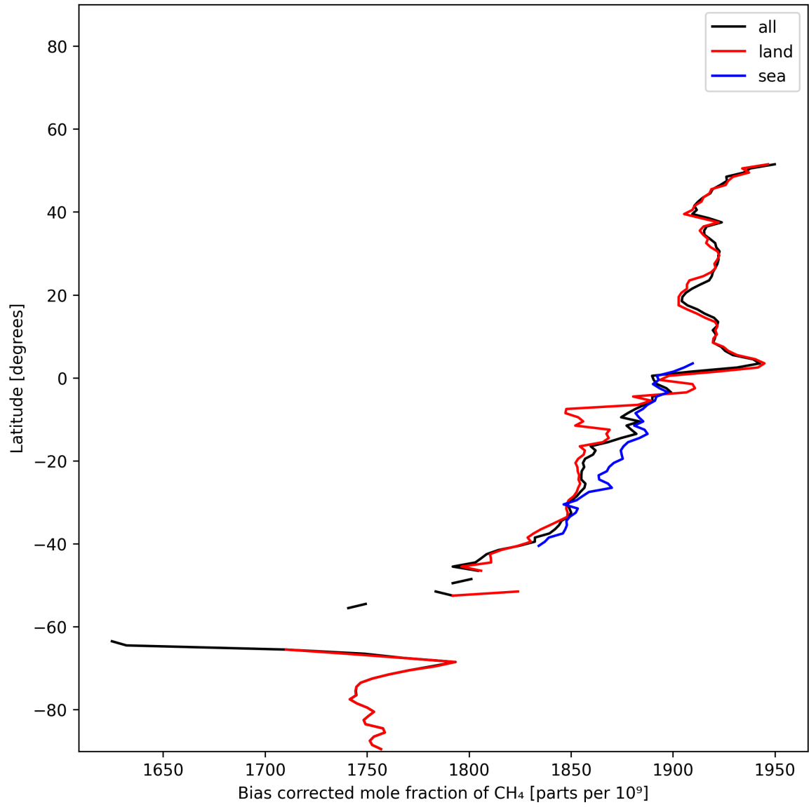
Figure 14: Zonal average of “Bias corrected mole fraction of CH 4 ” for 2024-12-23 to 2024-12-25.
