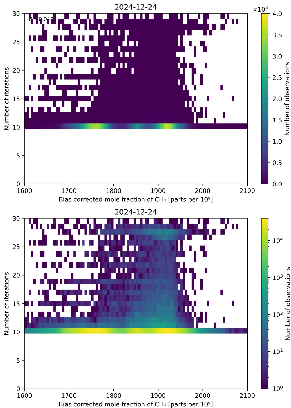
Figure 67: Scatter density plot of “Bias corrected mole fraction of \text{CH}_4 ” against “Number of iterations” for 2024-12-23 to 2024-12-25.
