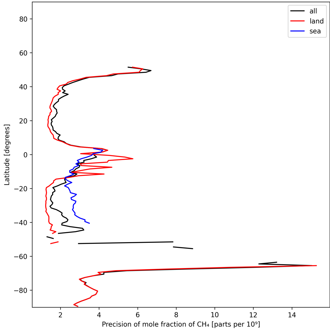
Figure 13: Zonal average of “Precision of mole fraction of CH 4 ” for 2024-12-23 to 2024-12-25.
