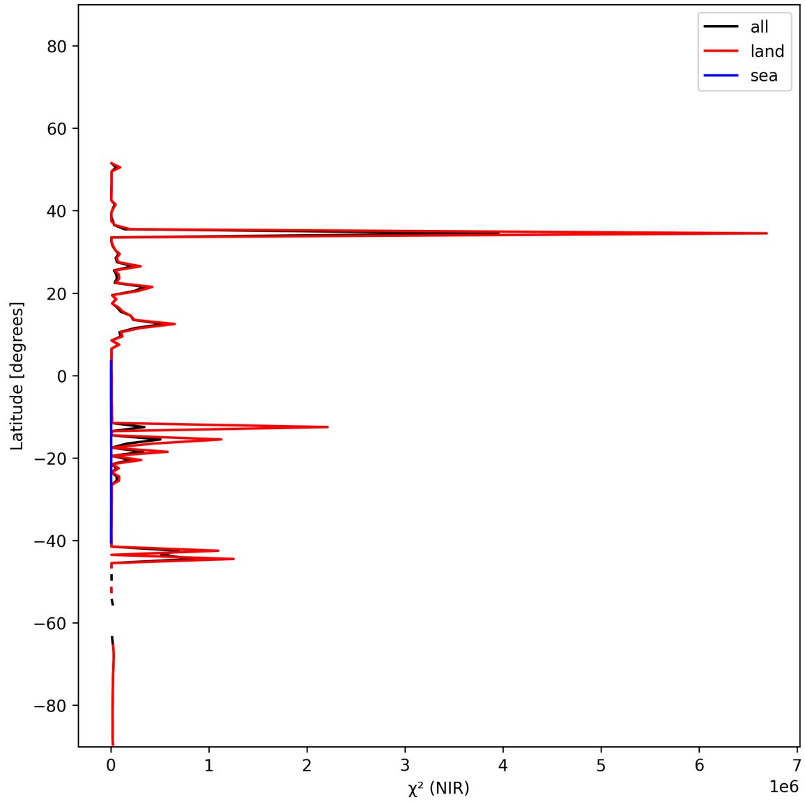
Figure 18: Zonal average of “ \chi^2 (NIR)” for 2024-12-23 to 2024-12-25.
