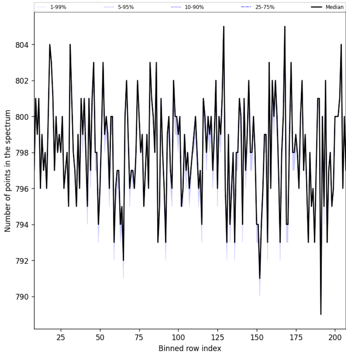
Figure 37: Along track statistics of “Number of points in the spectrum” for 2024-12-23 to 2024-12-25
