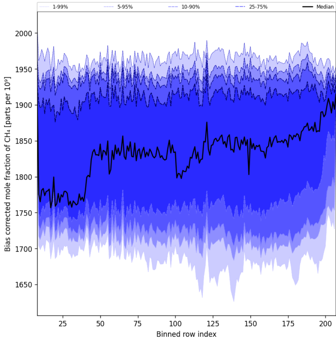
Figure 36: Along track statistics of “Bias corrected mole fraction of CH 4 ” for 2024-12-23 to 2024-12-25
