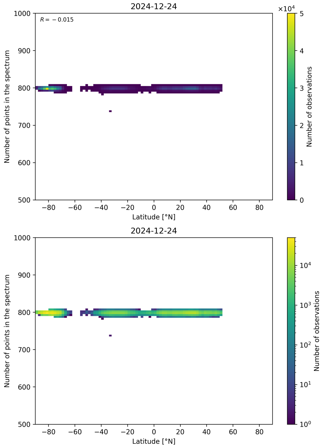
Figure 61: Scatter density plot of “Latitude” against “Number of points in the spectrum” for 2024-12-23 to 2024-12-25.
