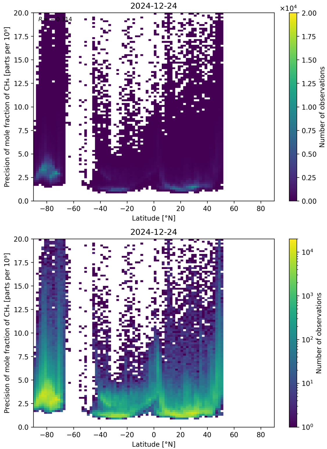
Figure 59: Scatter density plot of “Latitude” against “Precision of mole fraction of CH 4 ” for 2024-12-23 to 2024-12-25.
