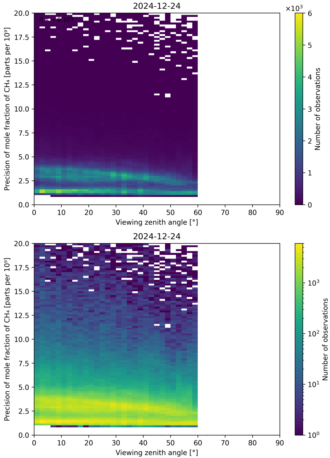
Figure 112: Scatter density plot of “Viewing zenith angle” against “Precision of mole fraction of CH 4 ” for 2024-12-23 to 2024-12-25.
