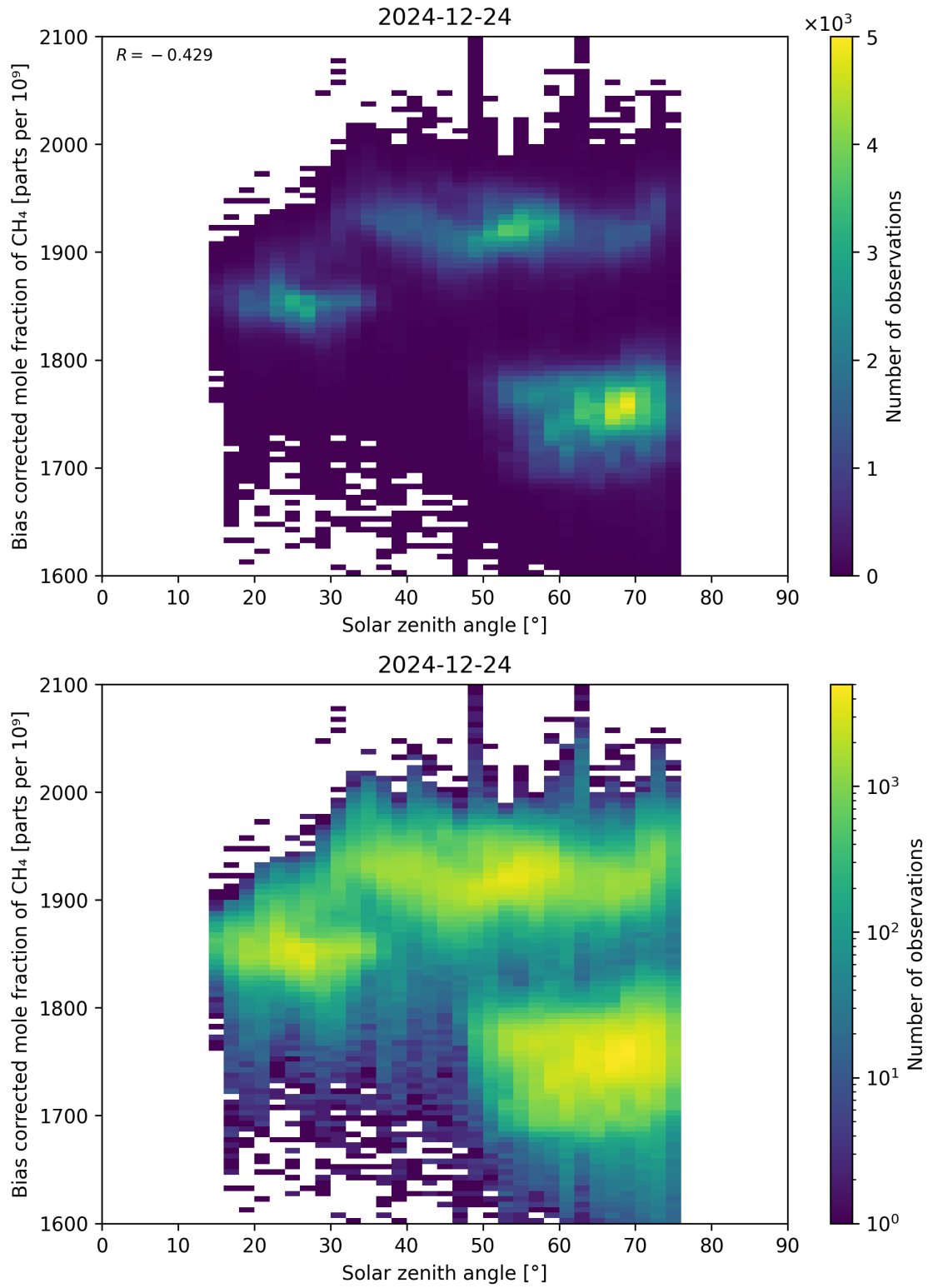
Figure 100: Scatter density plot of “Solar zenith angle” against “Bias corrected mole fraction of CH 4 ” for 2024-12-23 to 2024-12-25.
