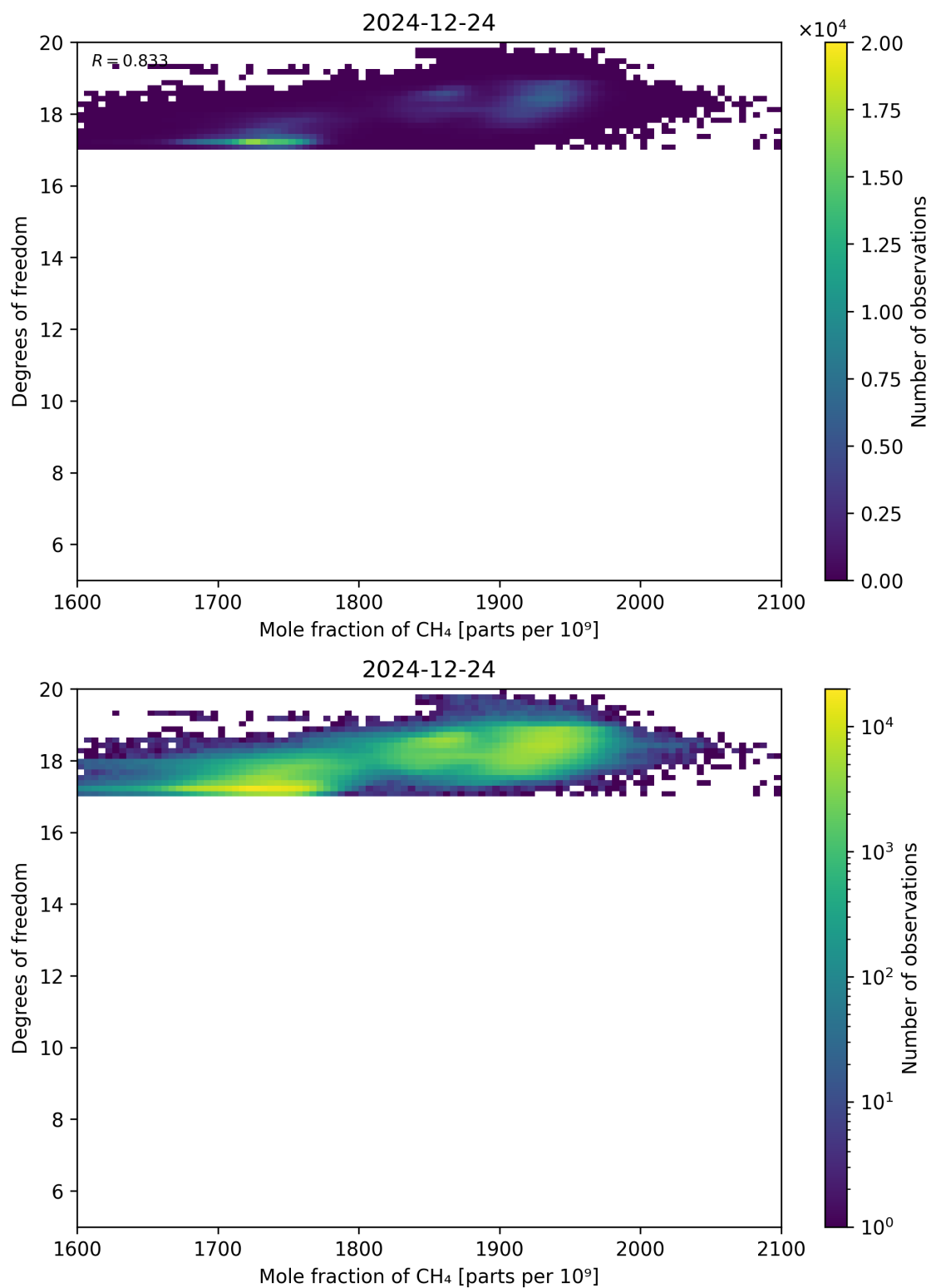
Figure 72: Scatter density plot of “Mole fraction of CH 4 ” against “Degrees of freedom” for 2024-12-23 to 2024-12-25.
