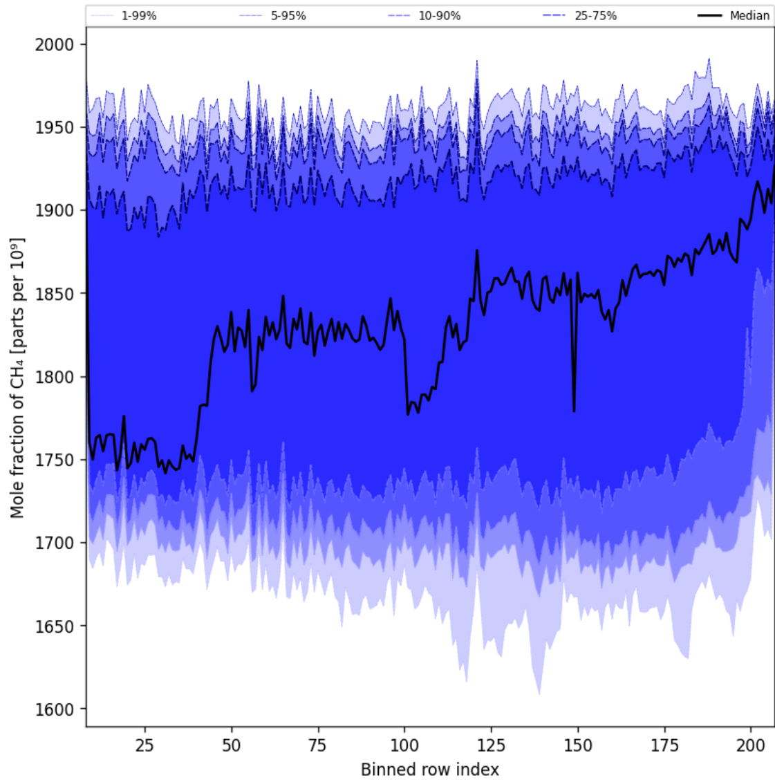
Figure 34: Along track statistics of “Mole fraction of CH 4 ” for 2024-12-23 to 2024-12-25
