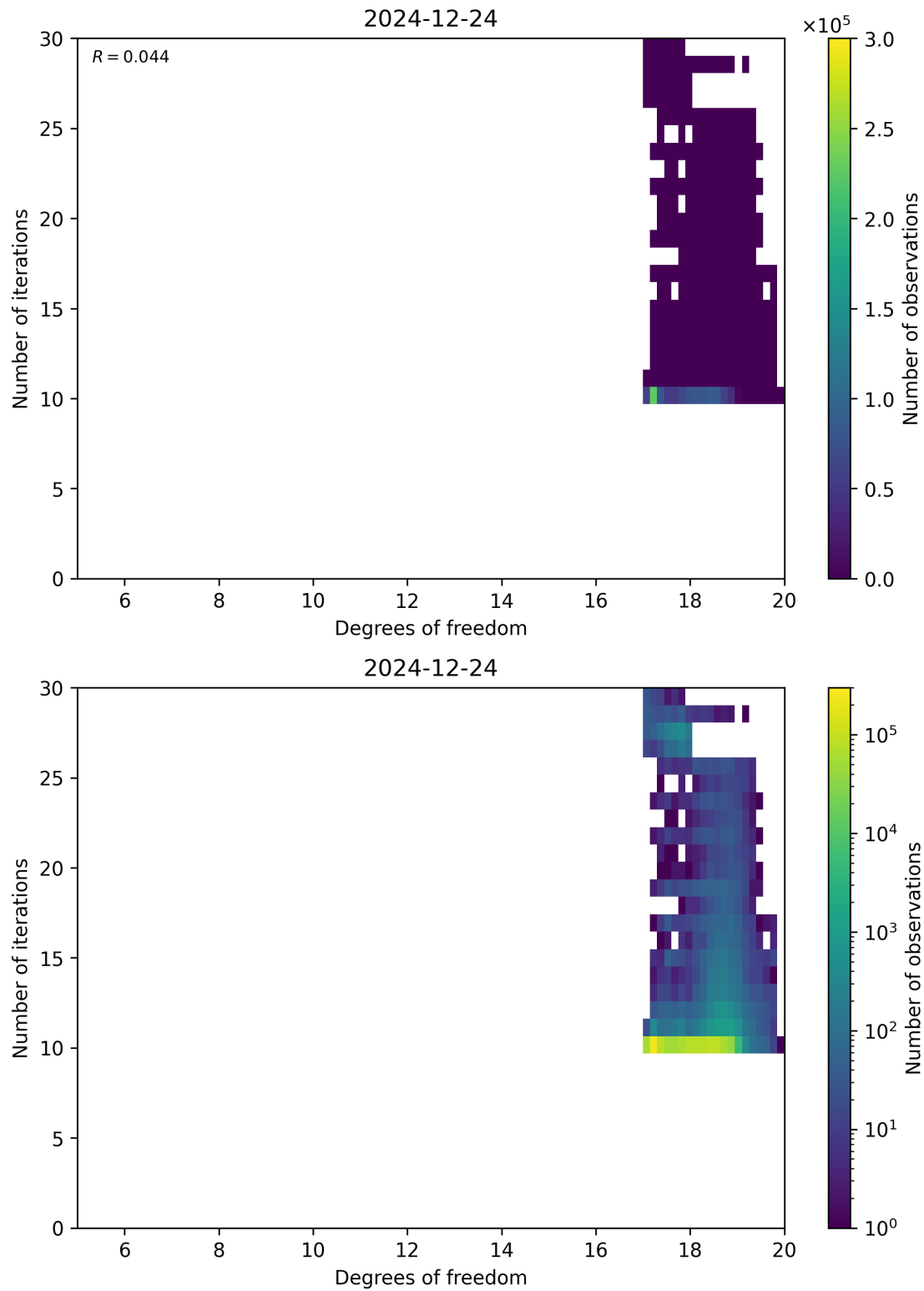
Figure 52: Scatter density plot of “Degrees of freedom” against “Number of iterations” for 2024-12-23 to 2024-12-25.
