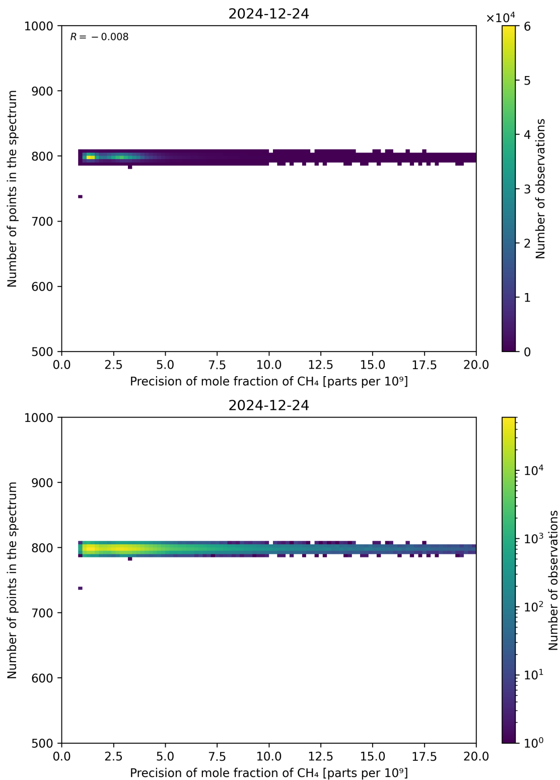
Figure 84: Scatter density plot of “Precision of mole fraction of CH 4 ” against “Number of points in the spectrum” for 2024-12-23 to 2024-12-25.
