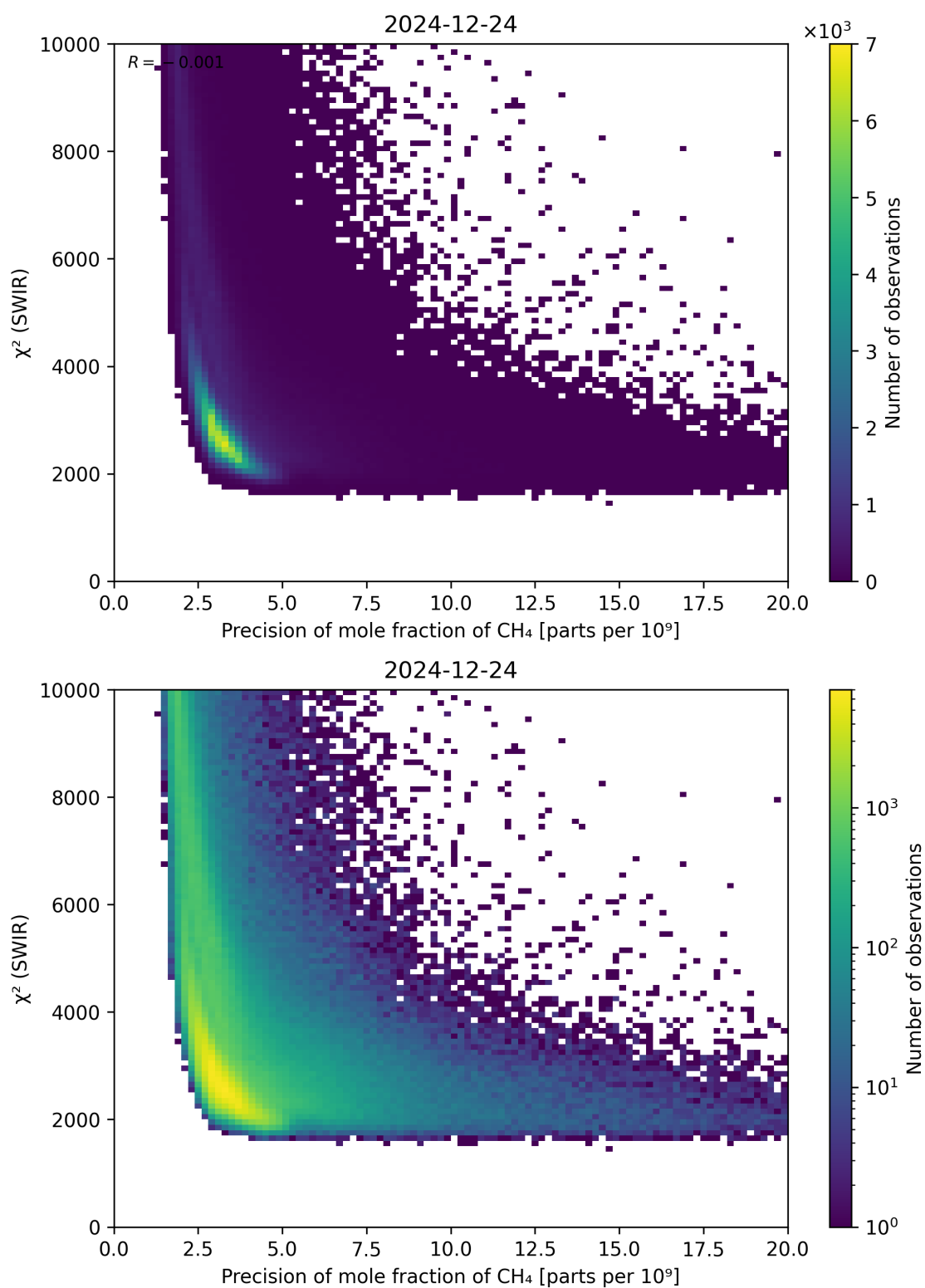
Figure 79: Scatter density plot of “Precision of mole fraction of \text{CH}_4 ” against “ \chi^2 (SWIR)” for 2024-12-23 to 2024-12-25.
