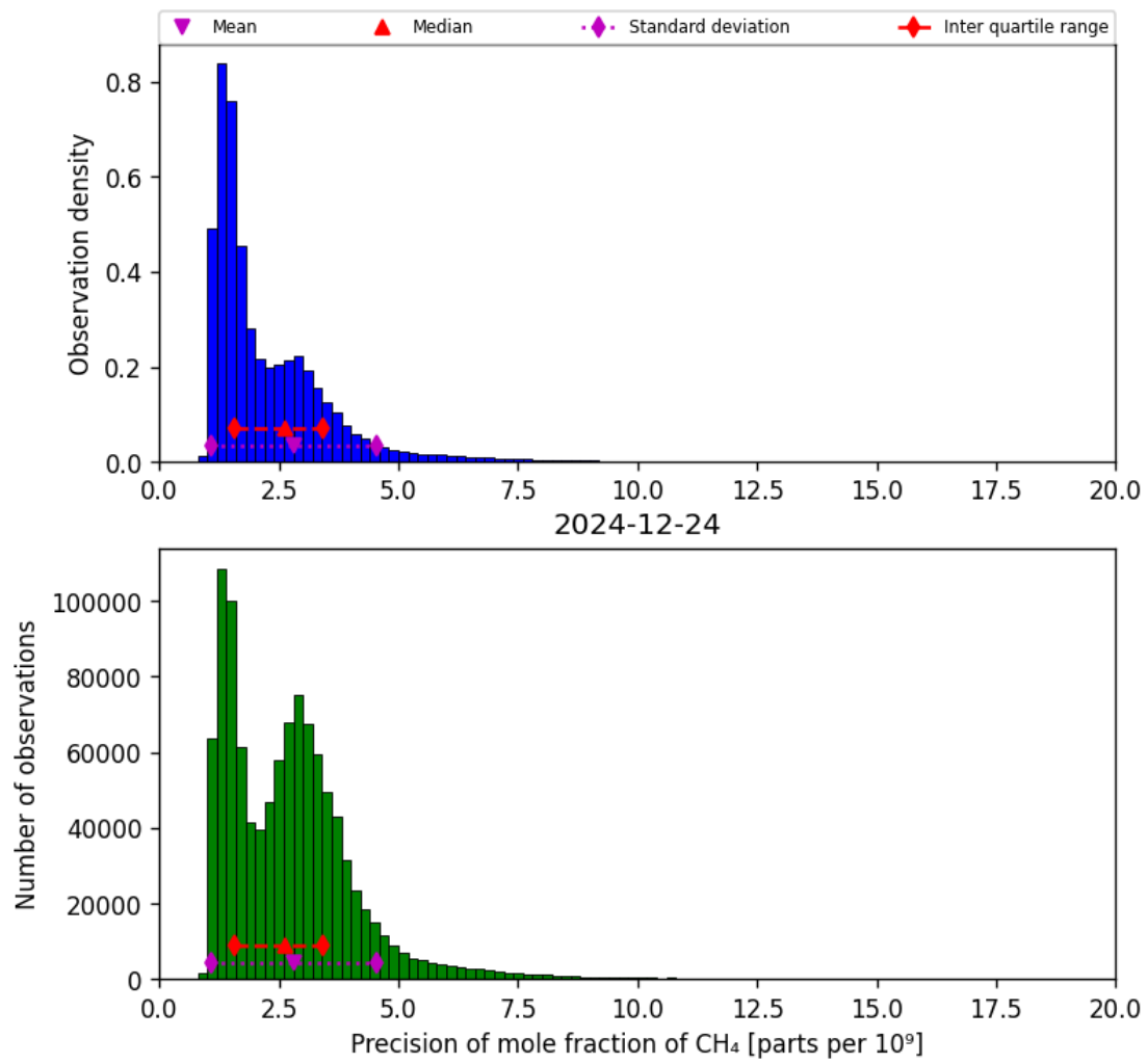
Figure 24: Histogram of “Precision of mole fraction of CH 4 ” for 2024-12-23 to 2024-12-25
