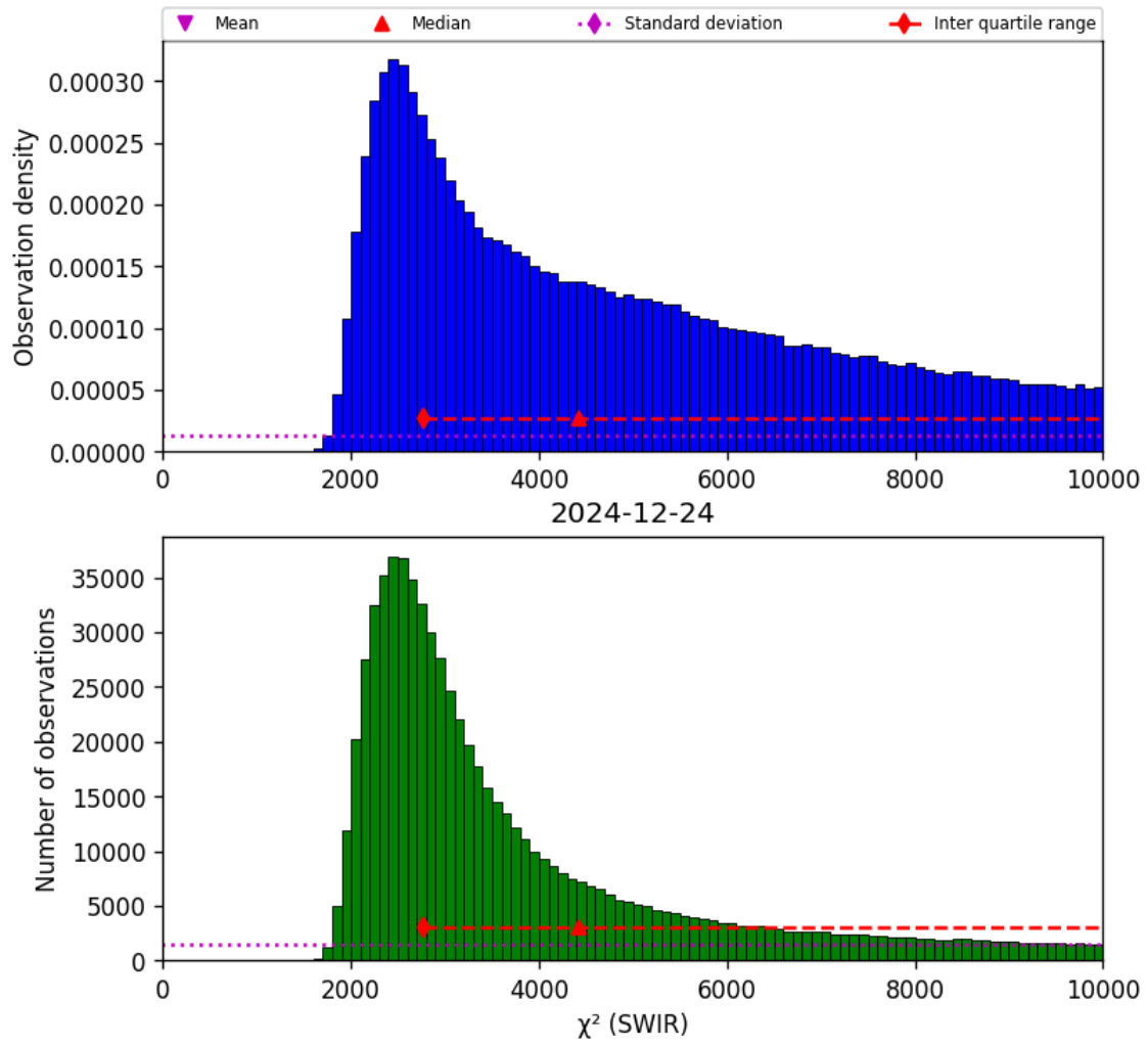
Figure 28: Histogram of “ \chi^2 (SWIR)” for 2024-12-23 to 2024-12-25
