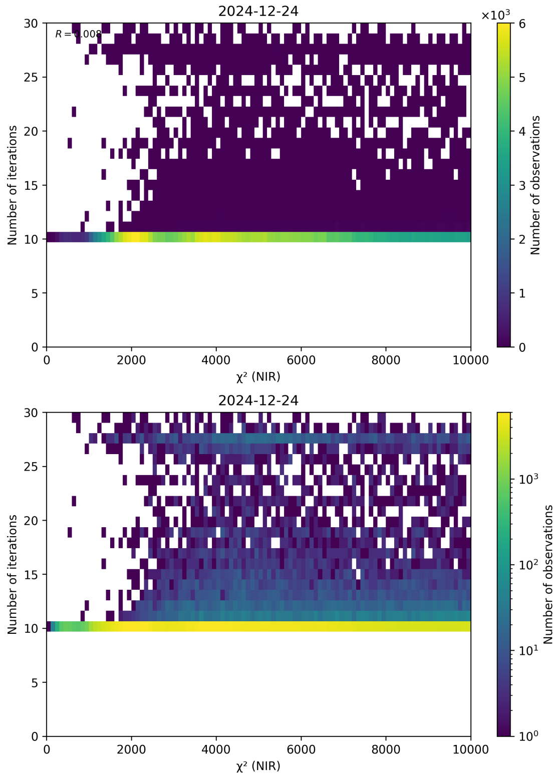
Figure 46: Scatter density plot of “ \chi^2 (NIR)” against “Number of iterations” for 2024-12-23 to 2024-12-25.
