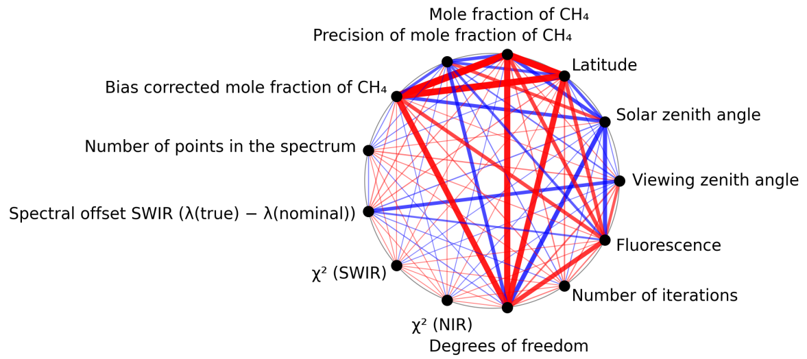
Figure 1: Map of correlation graph for 2024-12-23 to 2024-12-25.
