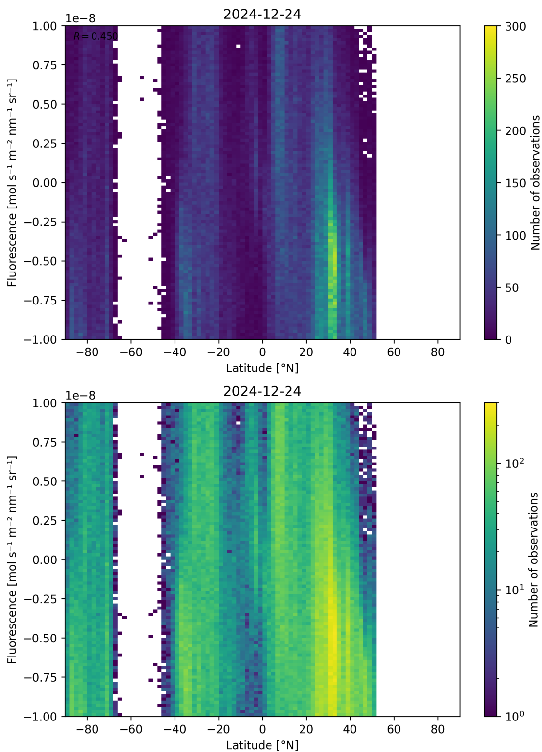
Figure 56: Scatter density plot of “Latitude” against “Fluorescence” for 2024-12-23 to 2024-12-25.
