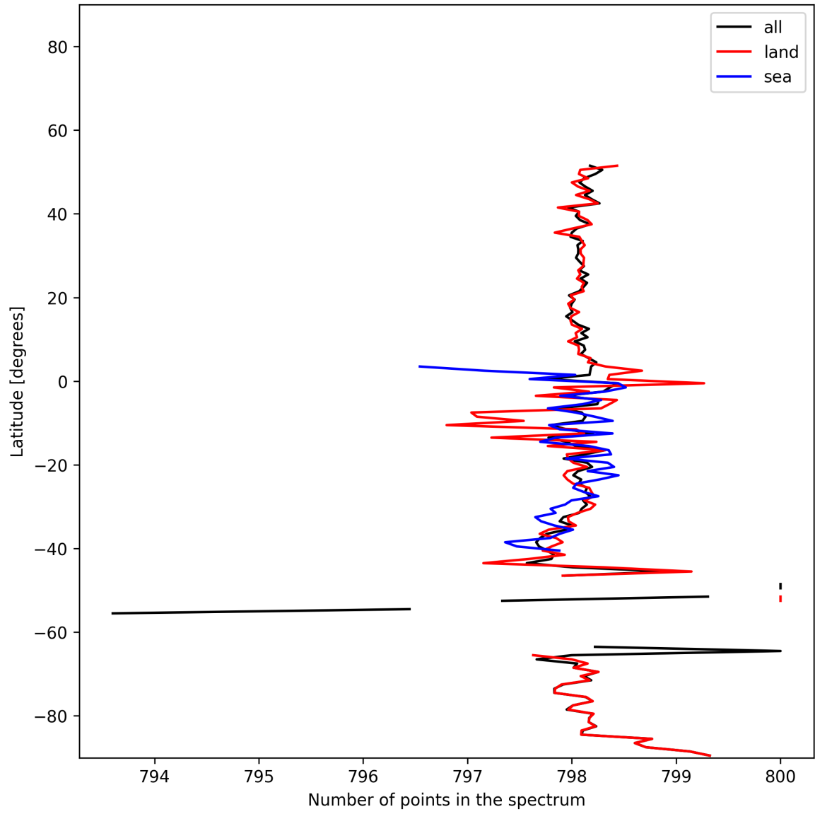
Figure 15: Zonal average of “Number of points in the spectrum” for 2024-12-23 to 2024-12-25.
