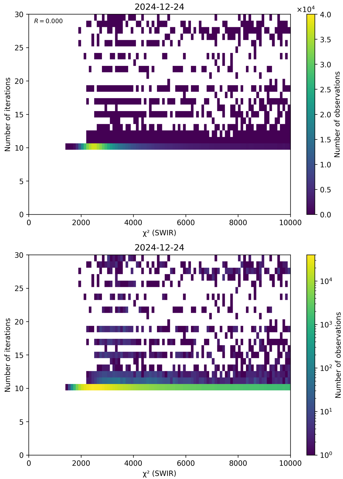
Figure 50: Scatter density plot of “ \chi^2 (SWIR)” against “Number of iterations” for 2024-12-23 to 2024-12-25.
