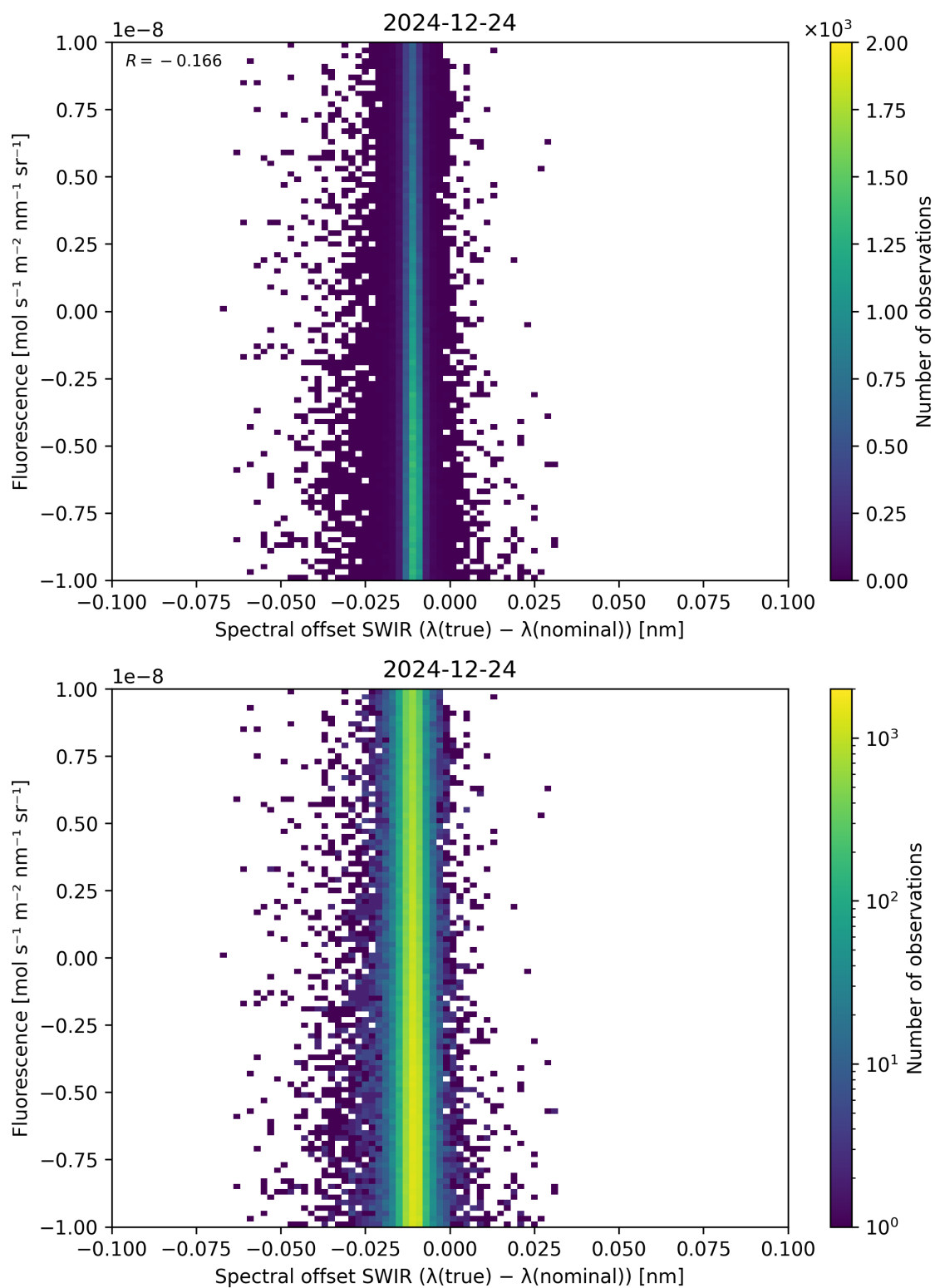
Figure 120: Scatter density plot of “Spectral offset SWIR ( \lambda_{\text{true}} - \lambda_{\text{nominal}} )” against “Fluorescence” for 2024-12-23 to 2024-12-25.
