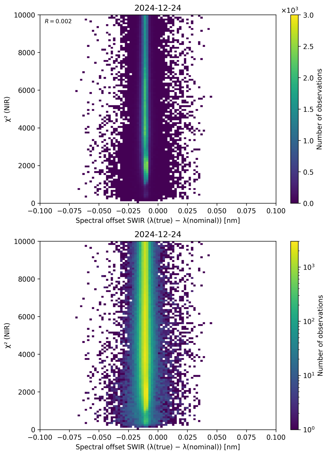
Figure 117: Scatter density plot of “Spectral offset SWIR ( \lambda_{\text{true}} - \lambda_{\text{nominal}} )” against “ \chi^2 (NIR)” for 2024-12-23 to 2024-12-25.
