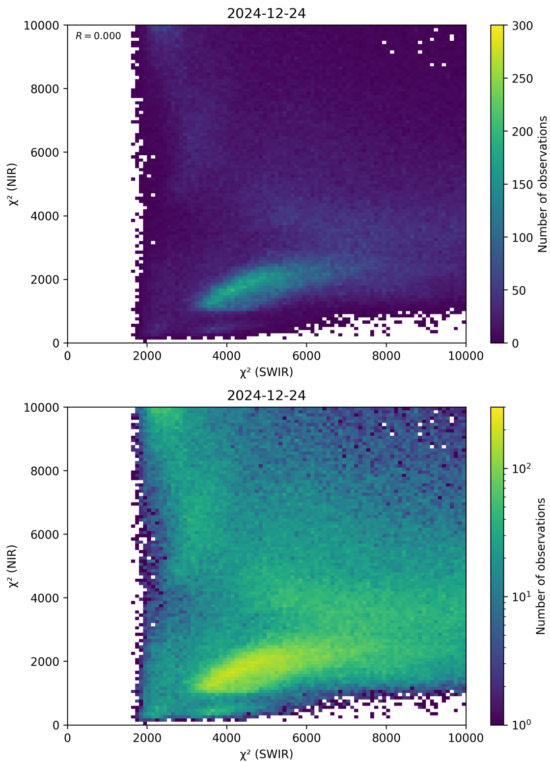
Figure 47: Scatter density plot of “ \chi^2 (SWIR)” against “ \chi^2 (NIR)” for 2024-12-23 to 2024-12-25.
