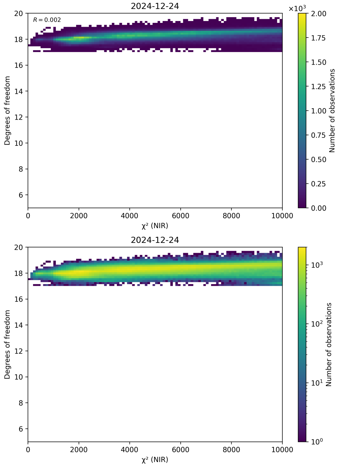
Figure 44: Scatter density plot of “ \chi^2 (NIR)” against “Degrees of freedom” for 2024-12-23 to 2024-12-25.
