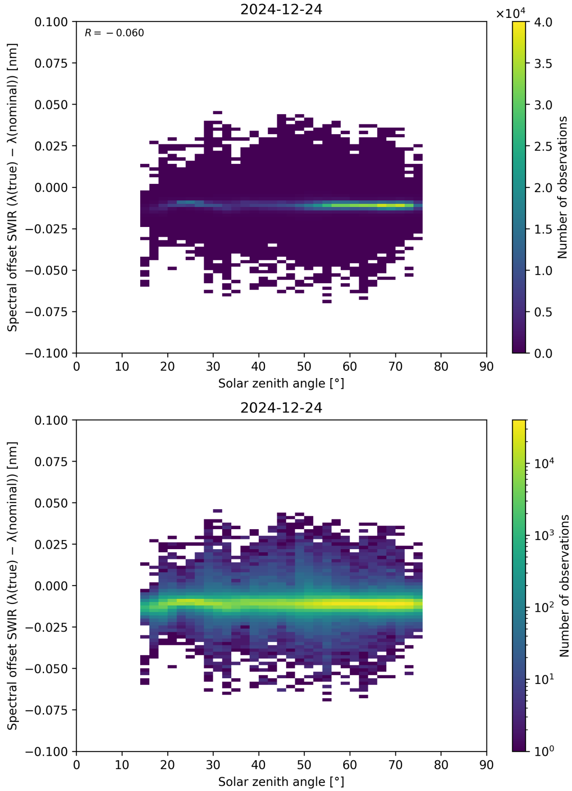
Figure 104: Scatter density plot of “Solar zenith angle” against “Spectral offset SWIR ( \lambda_{\text{true}} - \lambda_{\text{nominal}} )” for 2024-12-23 to 2024-12-25.
