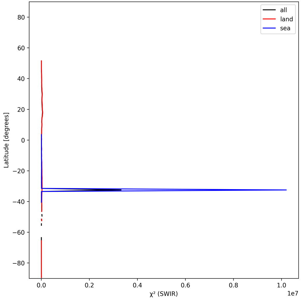
Figure 17: Zonal average of “ \chi^2 (SWIR)” for 2024-12-23 to 2024-12-25.
