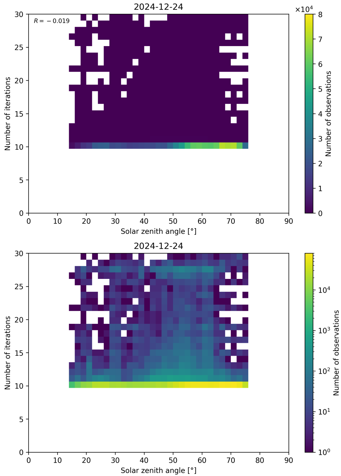
Figure 102: Scatter density plot of “Solar zenith angle” against “Number of iterations” for 2024-12-23 to 2024-12-25.
