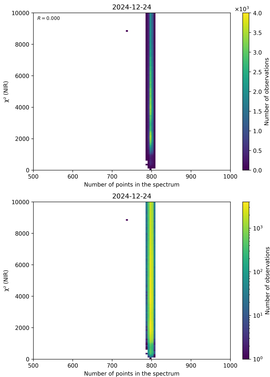
Figure 88: Scatter density plot of “Number of points in the spectrum” against “ \chi^2 (NIR)” for 2024-12-23 to 2024-12-25.
