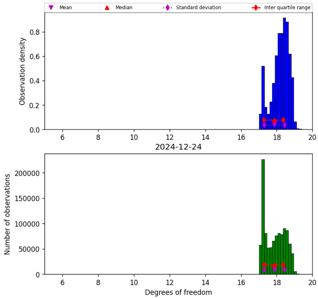
Figure 30: Histogram of “Degrees of freedom” for 2024-12-23 to 2024-12-25
