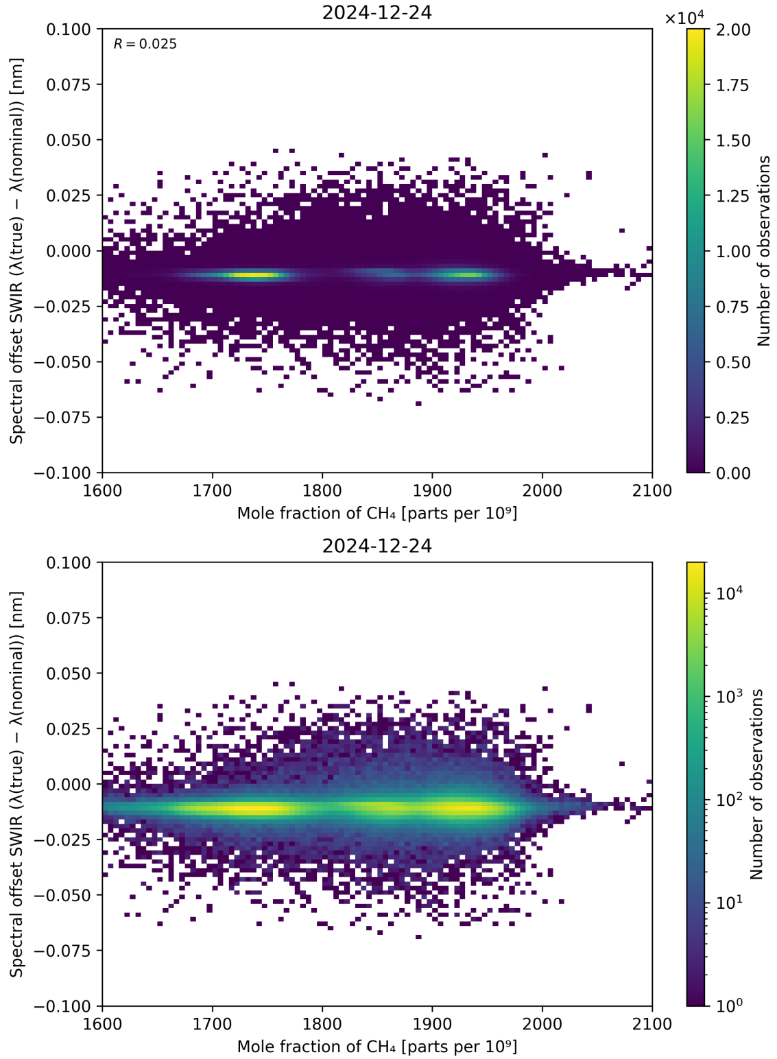
Figure 86: Scatter density plot of “Mole fraction of \text{CH}_4 ” against “Spectral offset SWIR ( \lambda_{\text{true}} - \lambda_{\text{nominal}} )” for 2024-12-23 to 2024-12-25.
