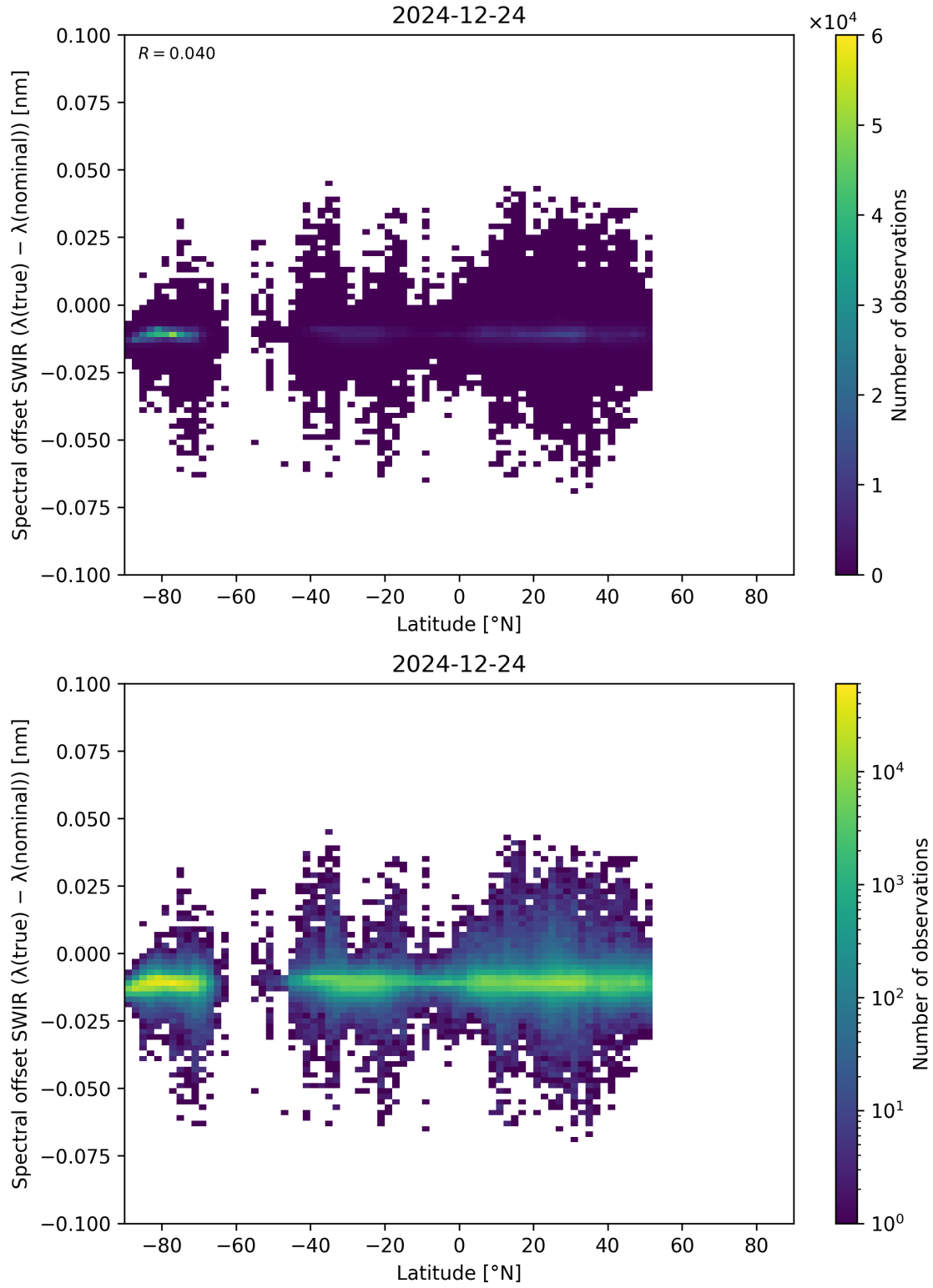
Figure 62: Scatter density plot of “Latitude” against “Spectral offset SWIR ( \lambda_{\text{true}} - \lambda_{\text{nominal}} )” for 2024-12-23 to 2024-12-25.
