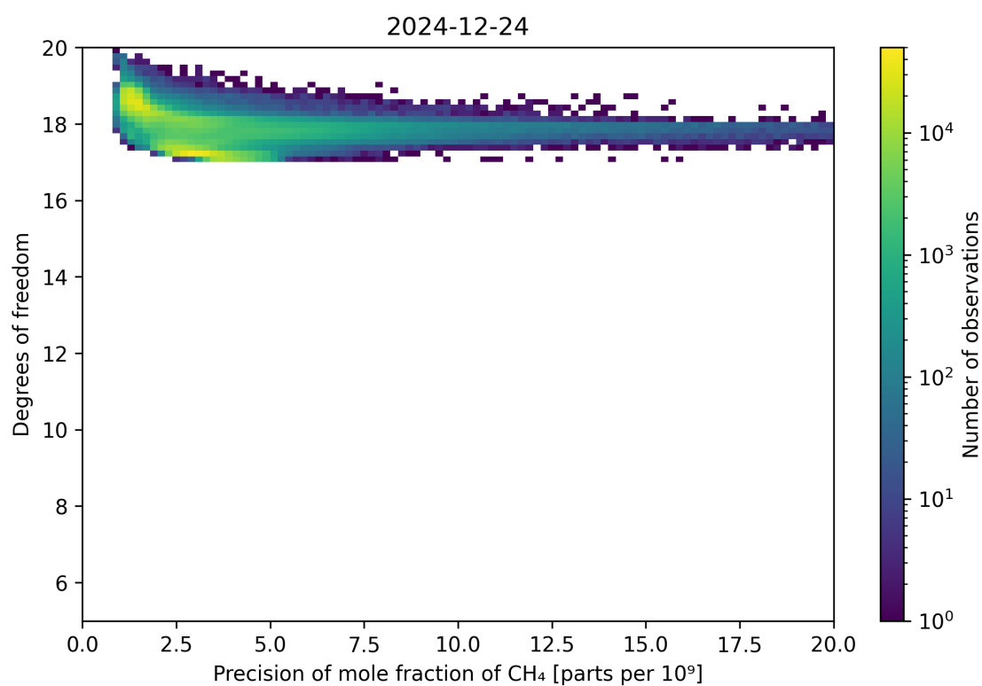
Figure 80: Scatter density plot of “Precision of mole fraction of CH 4 ” against “Degrees of freedom” for 2024-12-23 to 2024-12-25.
