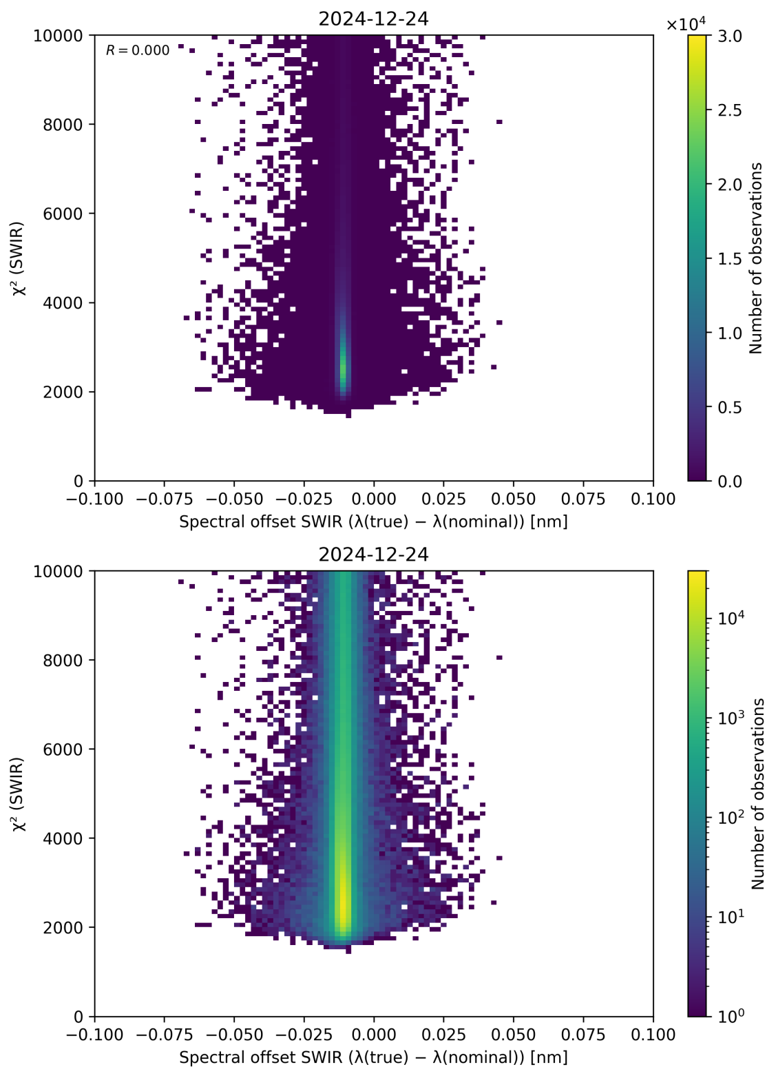
Figure 118: Scatter density plot of “Spectral offset SWIR ( \lambda_{\text{true}} - \lambda_{\text{nominal}} )” against “ \chi^2 (SWIR)” for 2024-12-23 to 2024-12-25.
