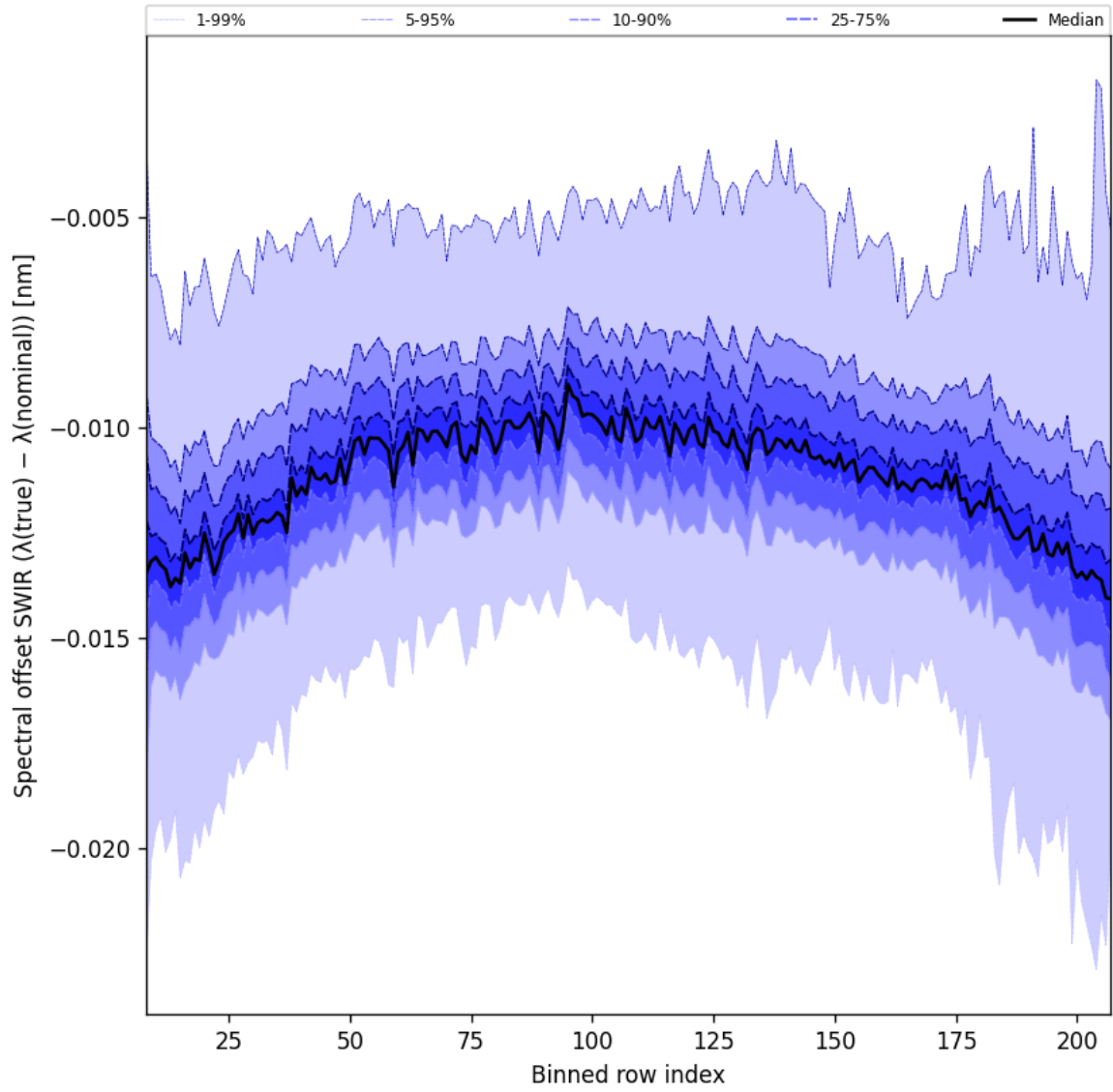
Figure 38: Along track statistics of “Spectral offset SWIR ( \lambda_{\text{true}} - \lambda_{\text{nominal}} )” for 2024-12-23 to 2024-12-25
