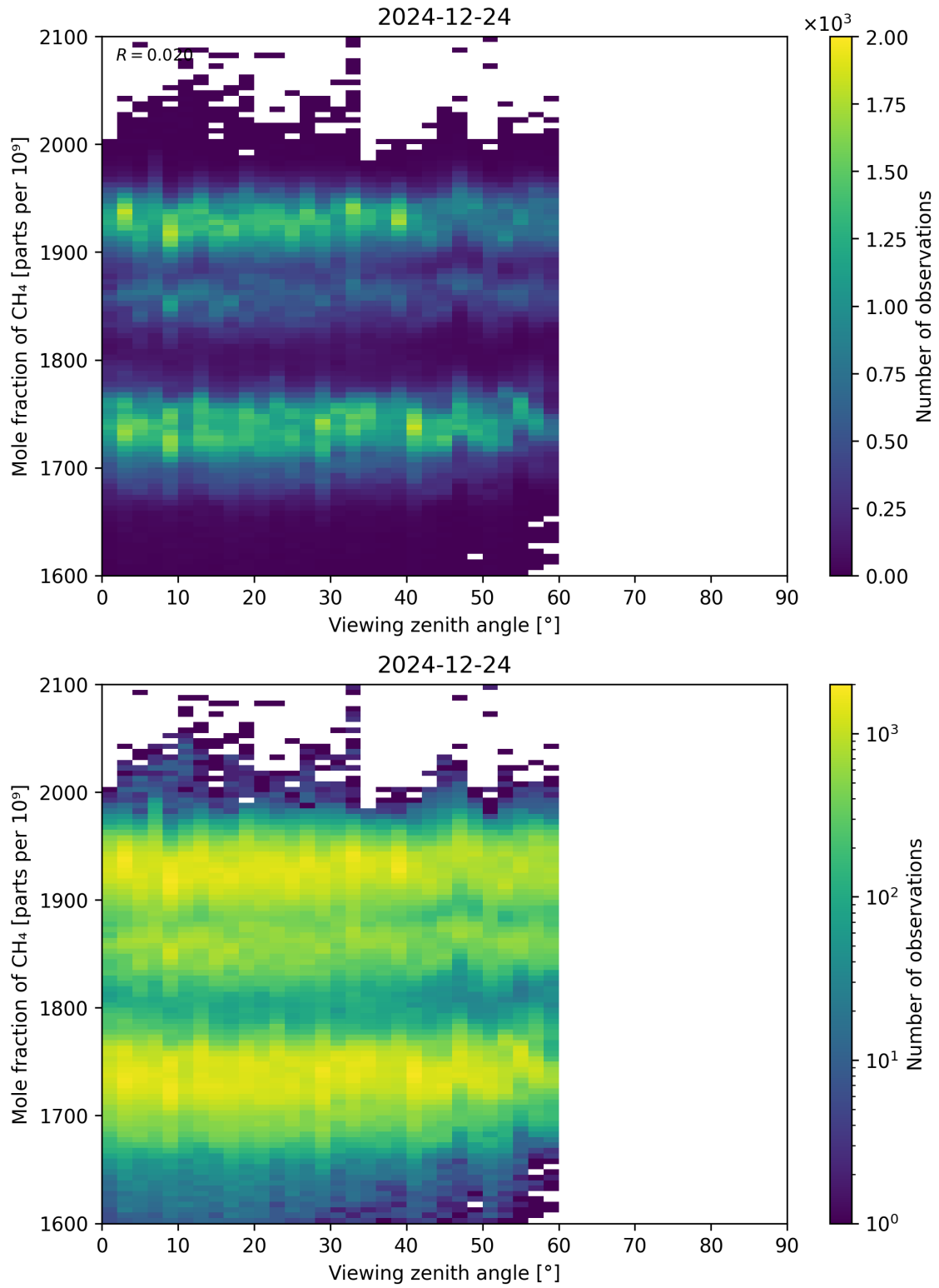
Figure 110: Scatter density plot of “Viewing zenith angle” against “Mole fraction of CH 4 ” for 2024-12-23 to 2024-12-25.
