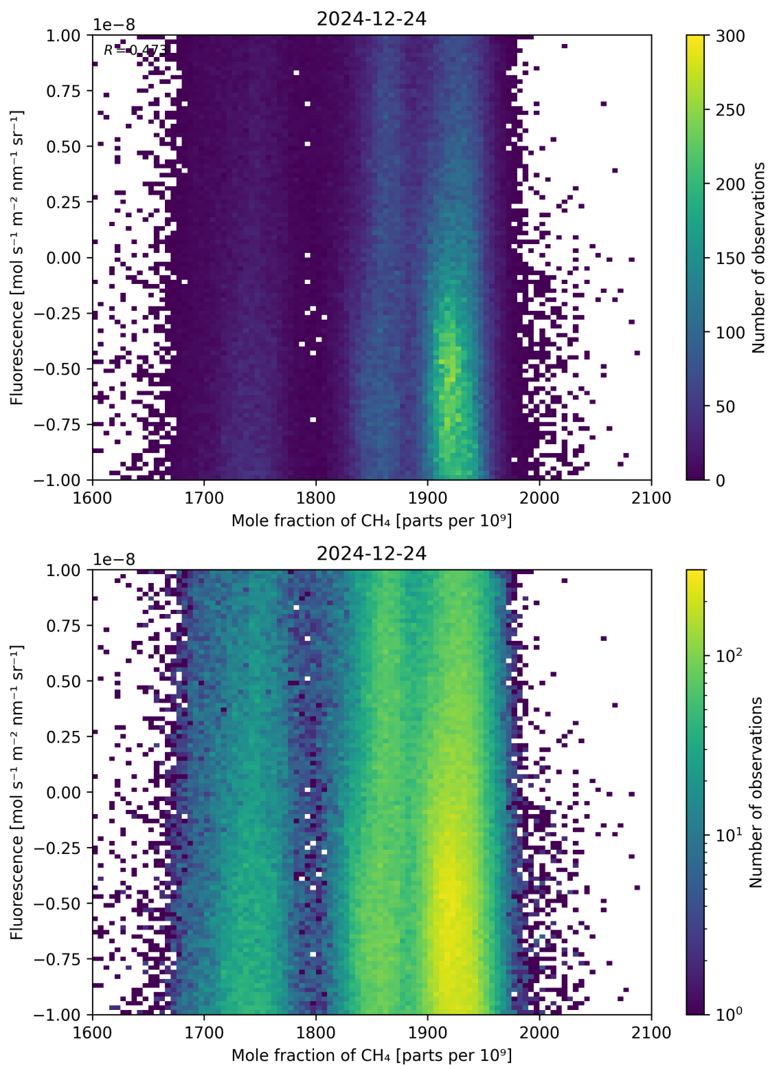
Figure 73: Scatter density plot of “Mole fraction of \text{CH}_4 ” against “Fluorescence” for 2024-12-23 to 2024-12-25.
