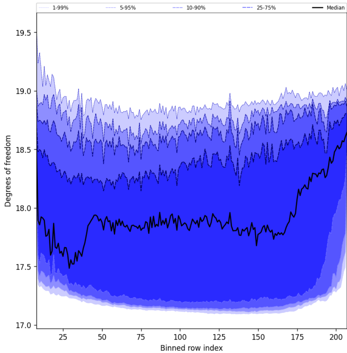
Figure 41: Along track statistics of “Degrees of freedom” for 2024-12-23 to 2024-12-25
