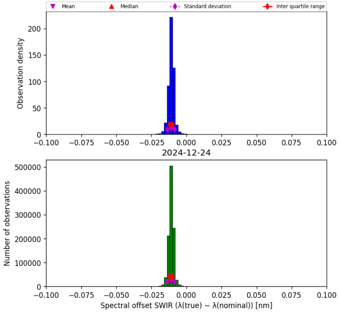
Figure 27: Histogram of “Spectral offset SWIR ( \lambda_{\text{true}} - \lambda_{\text{nominal}} )” for 2024-12-23 to 2024-12-25
