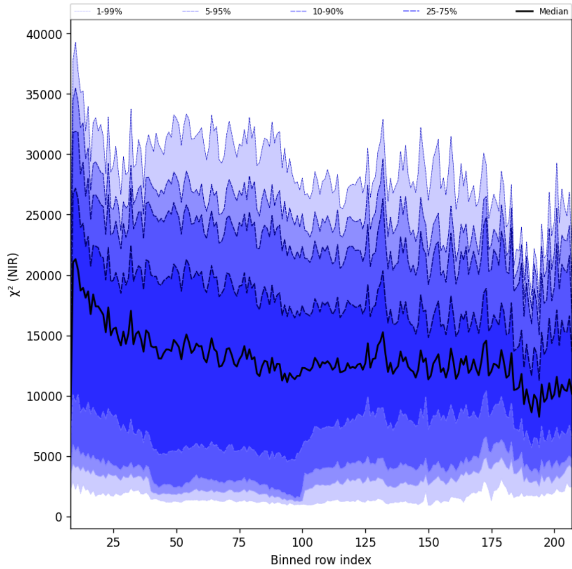
Figure 40: Along track statistics of “ \chi^2 (NIR)” for 2024-12-24 to 2024-12-26
