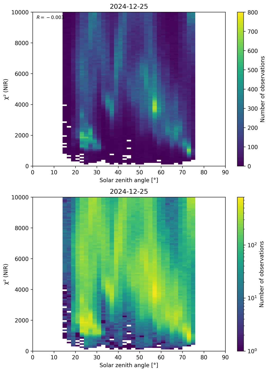
Figure 94: Scatter density plot of “Solar zenith angle” against “ \chi^2 (NIR)” for 2024-12-24 to 2024-12-26.
