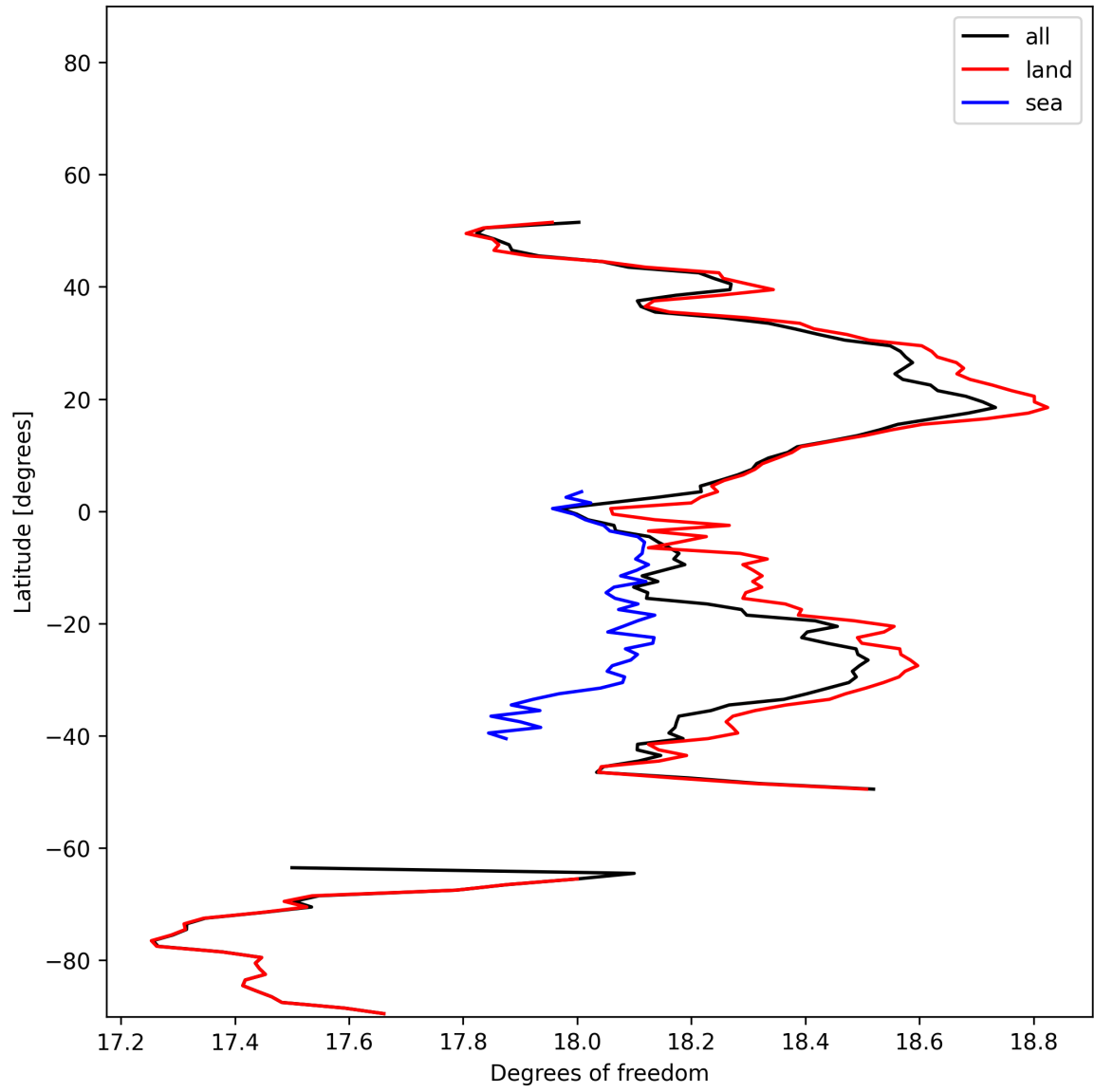
Figure 19: Zonal average of “Degrees of freedom” for 2024-12-24 to 2024-12-26.
