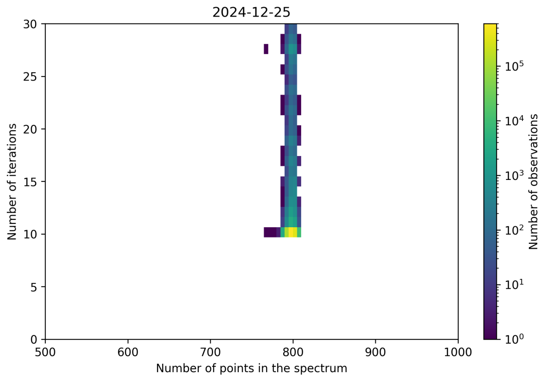
Figure 92: Scatter density plot of “Number of points in the spectrum” against “Number of iterations” for 2024-12-24 to 2024-12-26.
