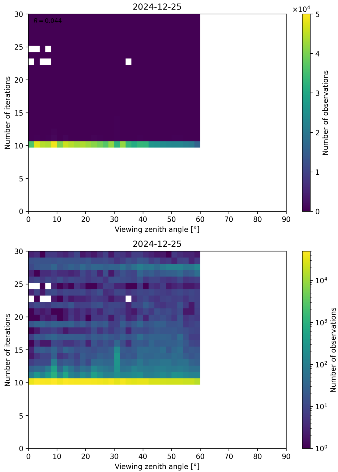
Figure 113: Scatter density plot of “Viewing zenith angle” against “Number of iterations” for 2024-12-24 to 2024-12-26.
