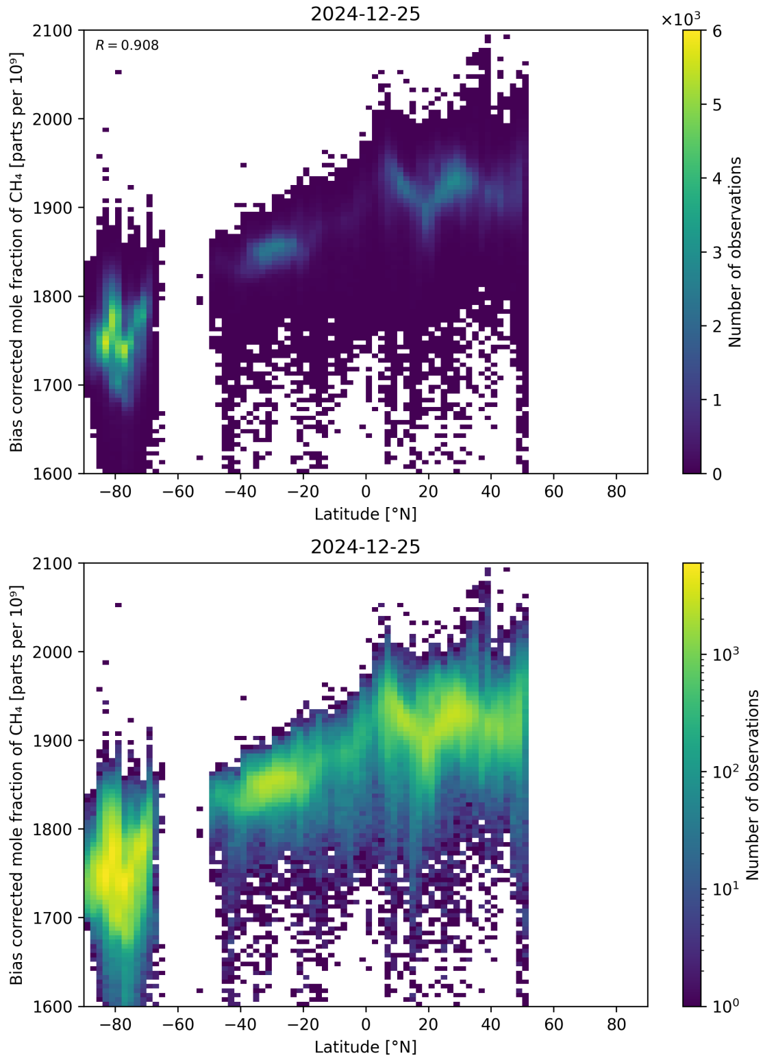
Figure 58: Scatter density plot of “Latitude” against “Bias corrected mole fraction of CH 4 ” for 2024-12-24 to 2024-12-26.
