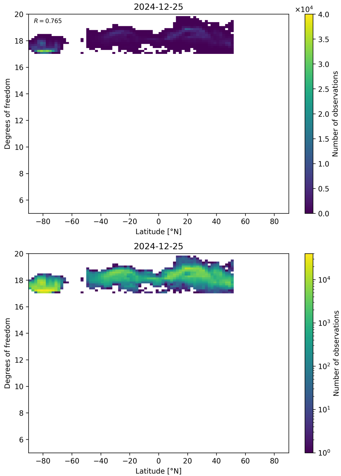
Figure 55: Scatter density plot of “Latitude” against “Degrees of freedom” for 2024-12-24 to 2024-12-26.
