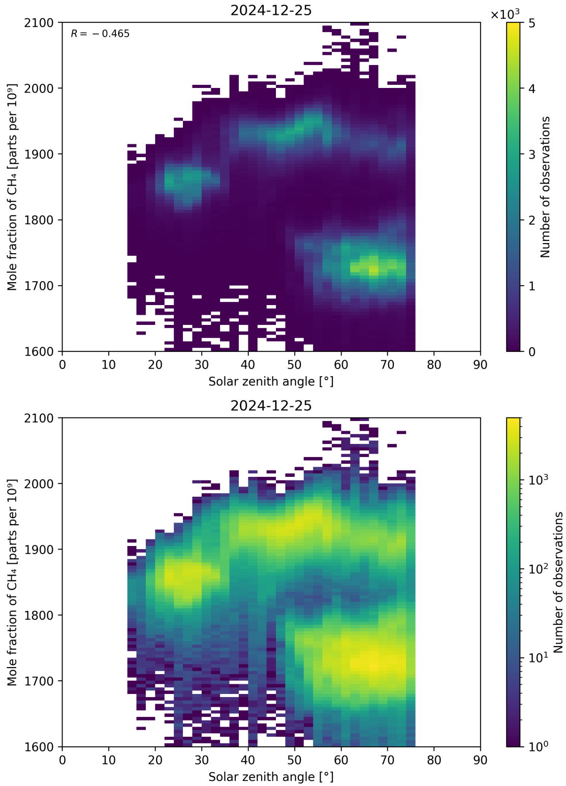
Figure 99: Scatter density plot of “Solar zenith angle” against “Mole fraction of CH 4 ” for 2024-12-24 to 2024-12-26.
