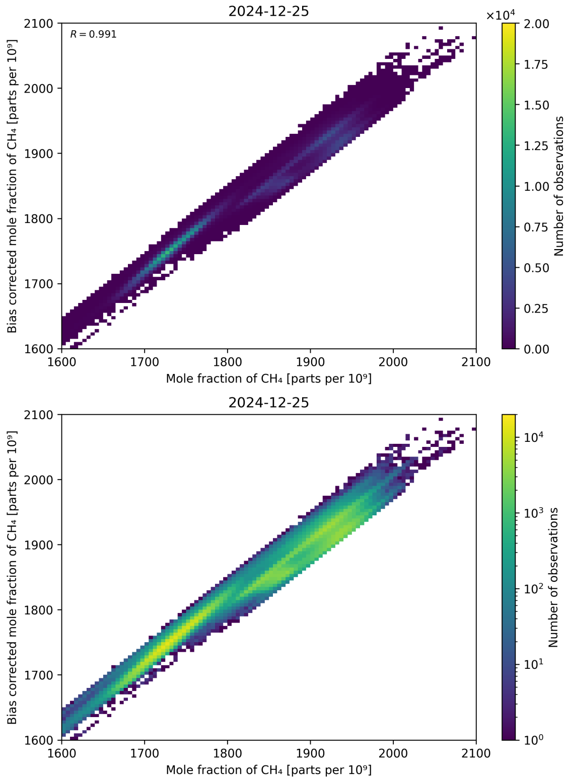
Figure 74: Scatter density plot of “Mole fraction of CH 4 ” against “Bias corrected mole fraction of CH 4 ” for 2024-12-24 to 2024-12-26.
