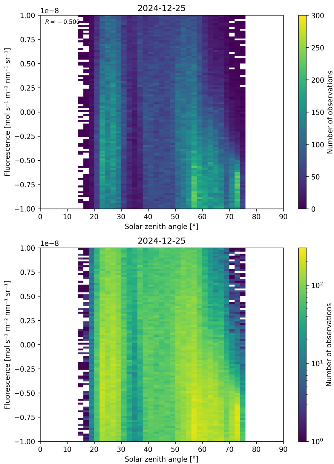
Figure 97: Scatter density plot of “Solar zenith angle” against “Fluorescence” for 2024-12-24 to 2024-12-26.
