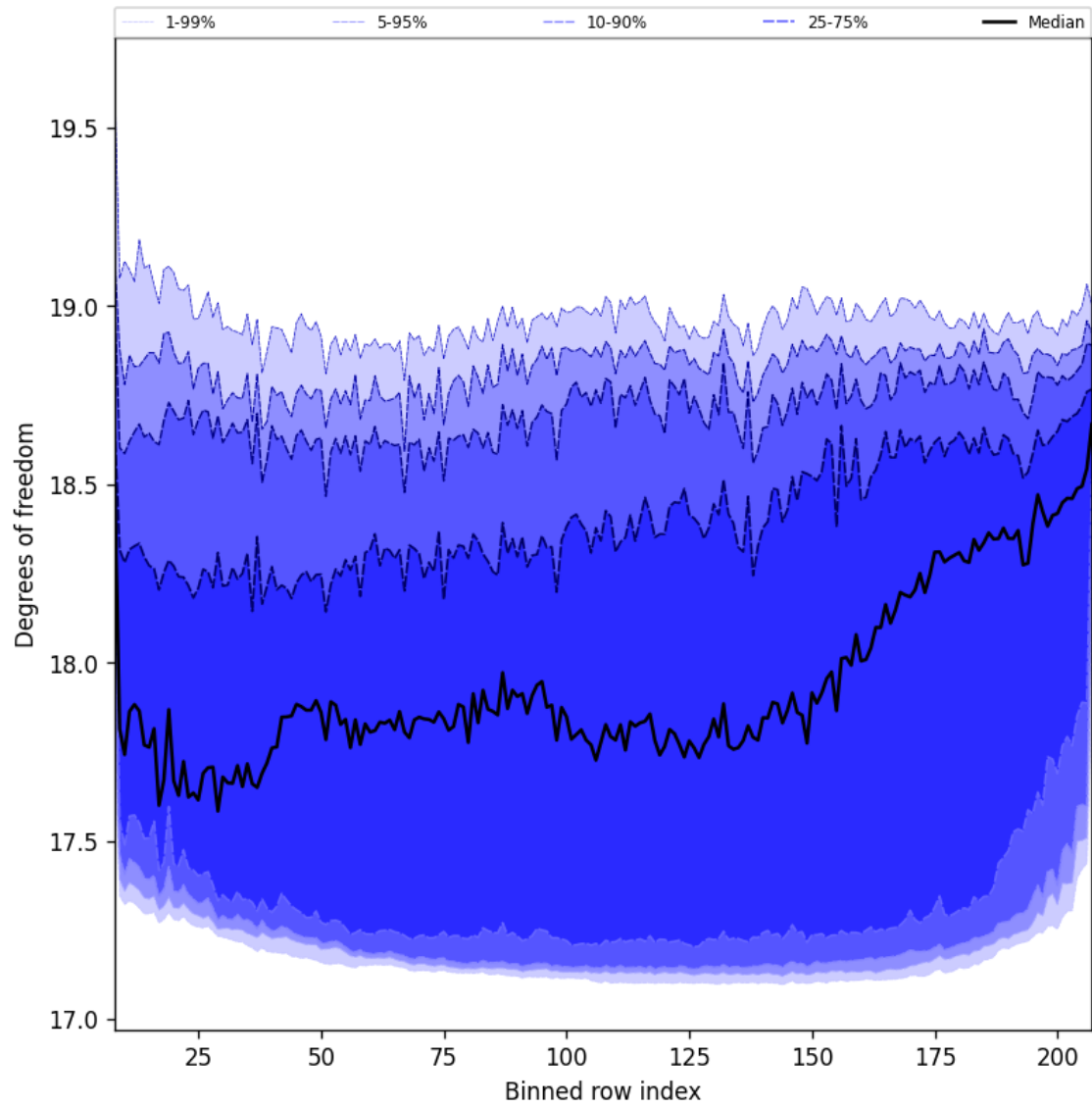
Figure 41: Along track statistics of “Degrees of freedom” for 2024-12-24 to 2024-12-26
