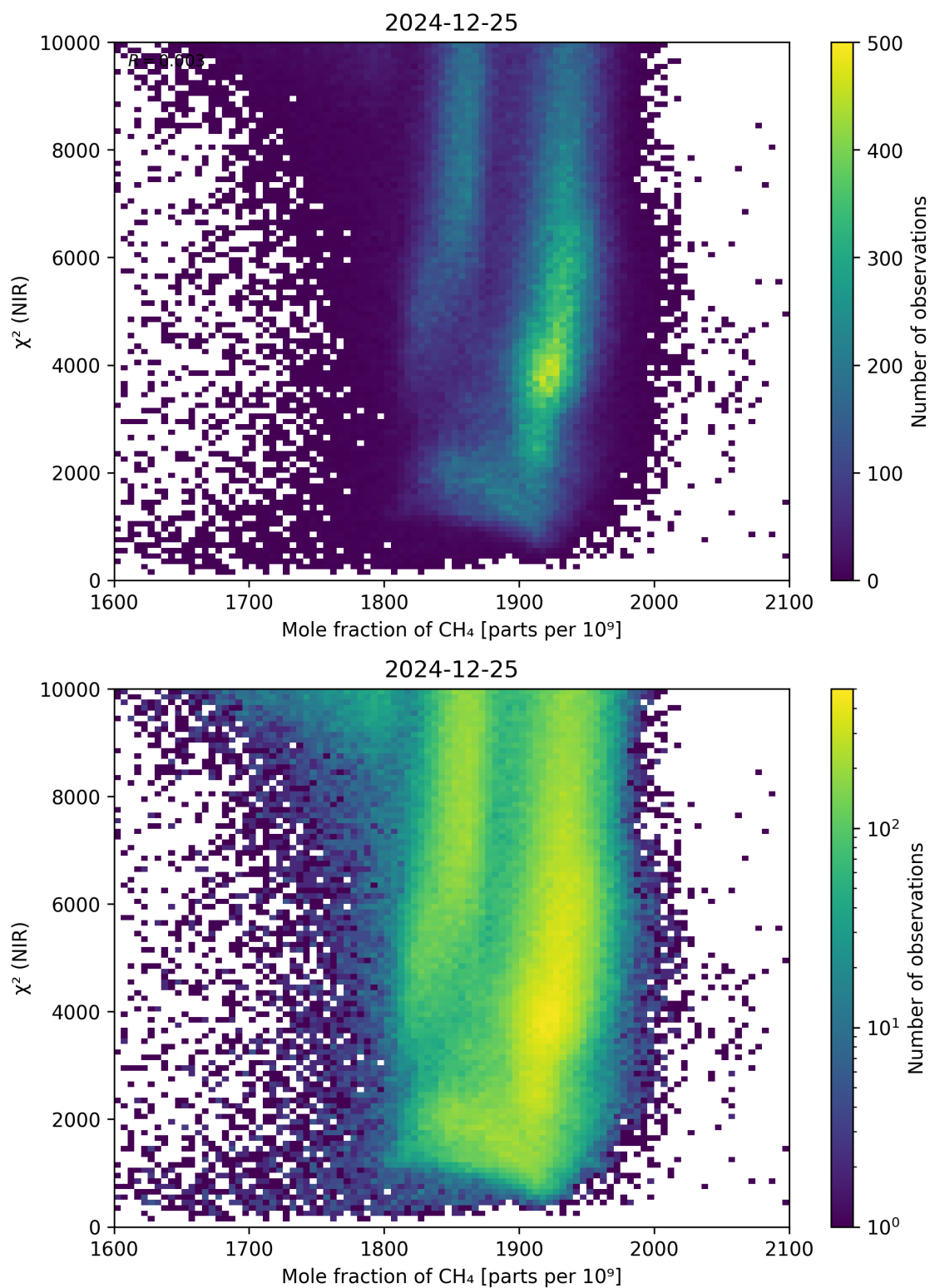
Figure 70: Scatter density plot of “Mole fraction of CH 4 ” against “ \chi^2 (NIR)” for 2024-12-24 to 2024-12-26.
