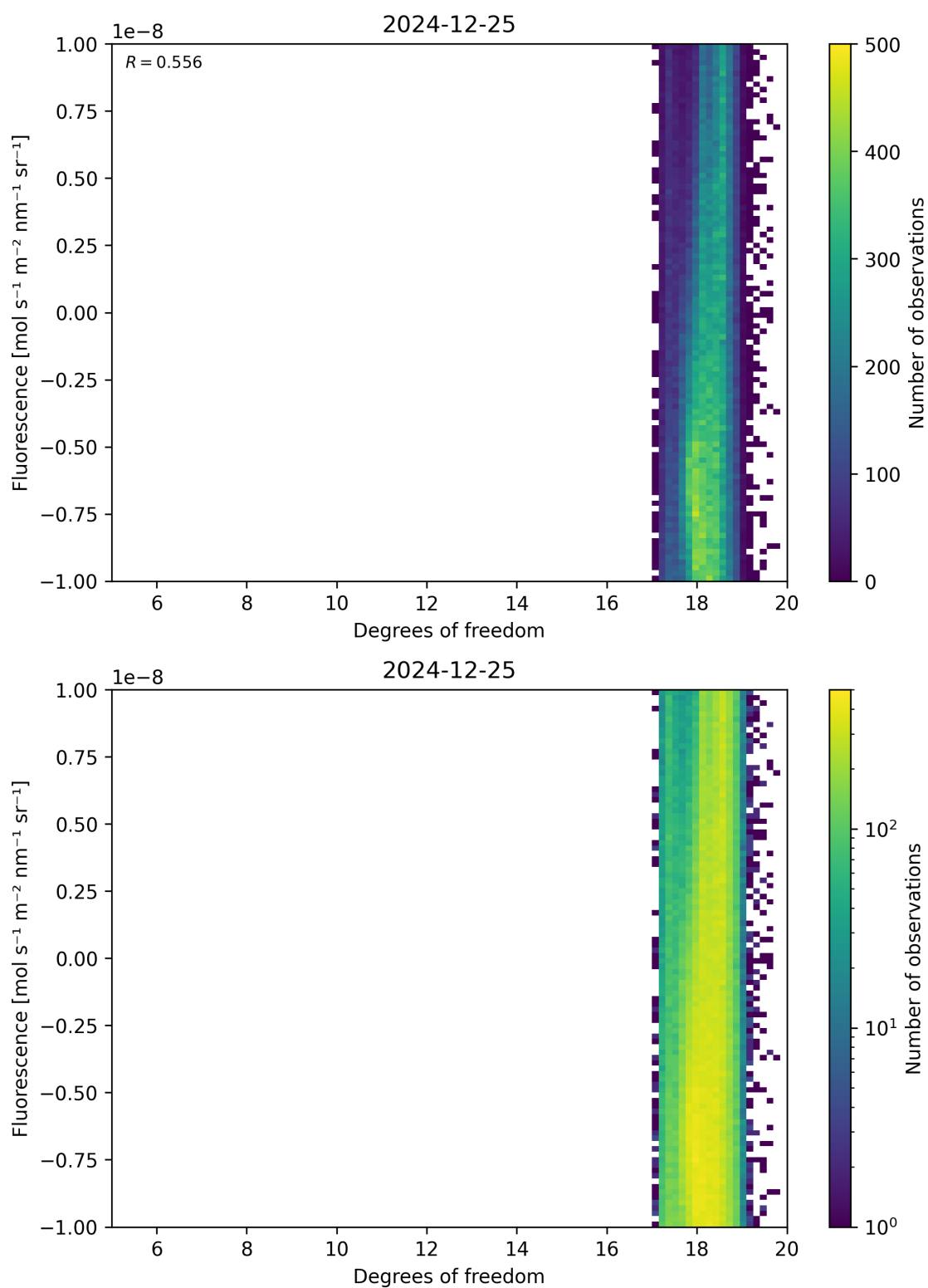
Figure 51: Scatter density plot of “Degrees of freedom” against “Fluorescence” for 2024-12-24 to 2024-12-26.
