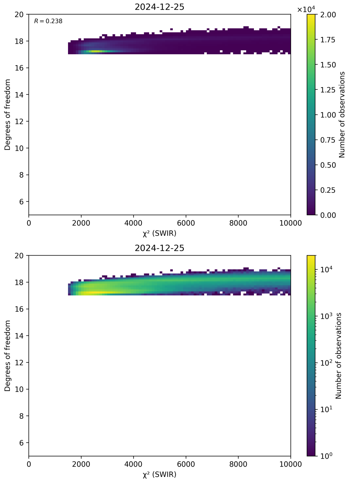
Figure 48: Scatter density plot of “ \chi^2 (SWIR)” against “Degrees of freedom” for 2024-12-24 to 2024-12-26.
