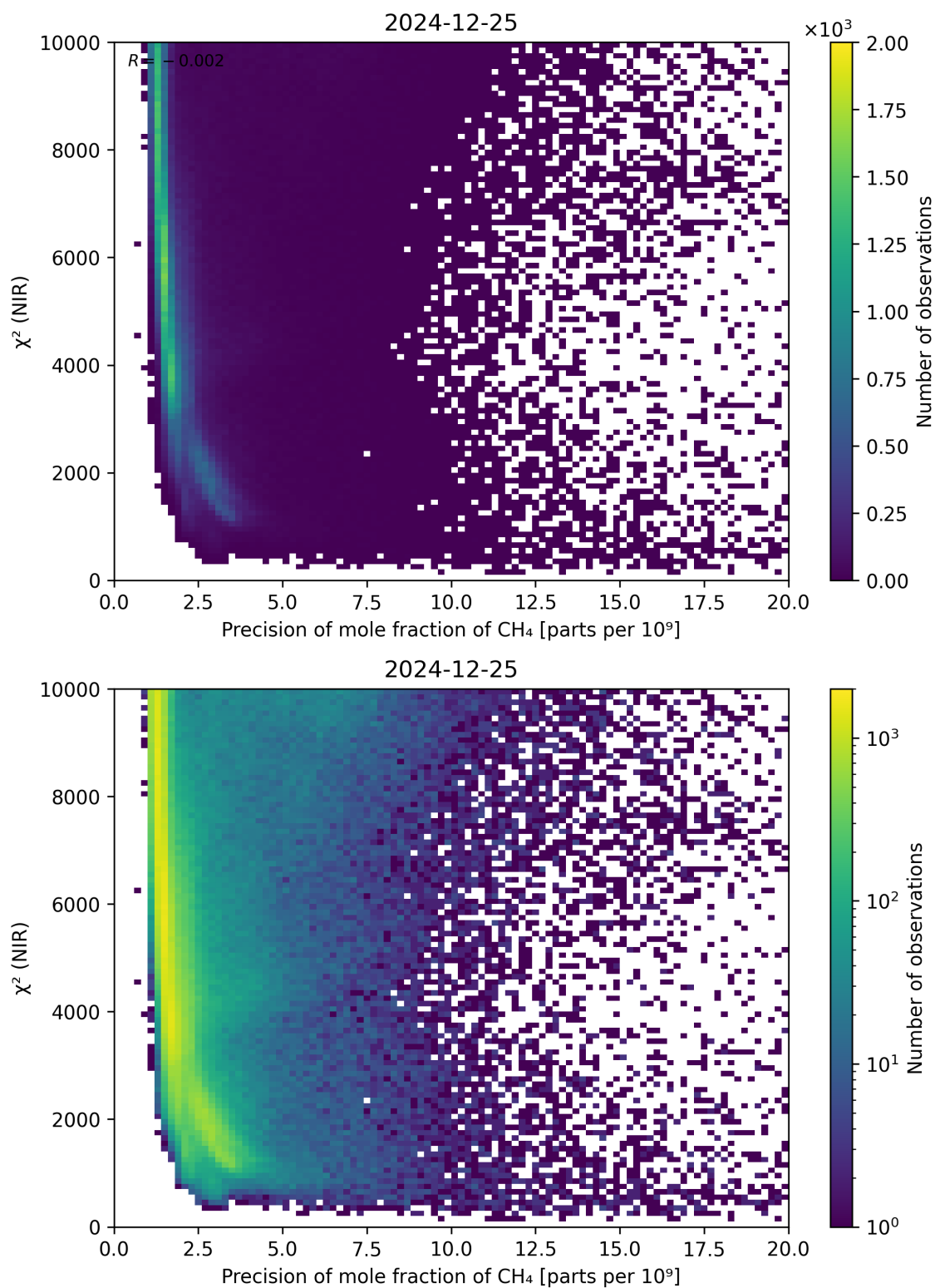
Figure 78: Scatter density plot of “Precision of mole fraction of CH 4 ” against “ \chi^2 (NIR)” for 2024-12-24 to 2024-12-26.
