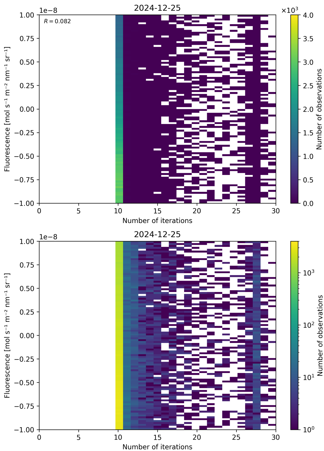
Figure 87: Scatter density plot of “Number of iterations” against “Fluorescence” for 2024-12-24 to 2024-12-26.
