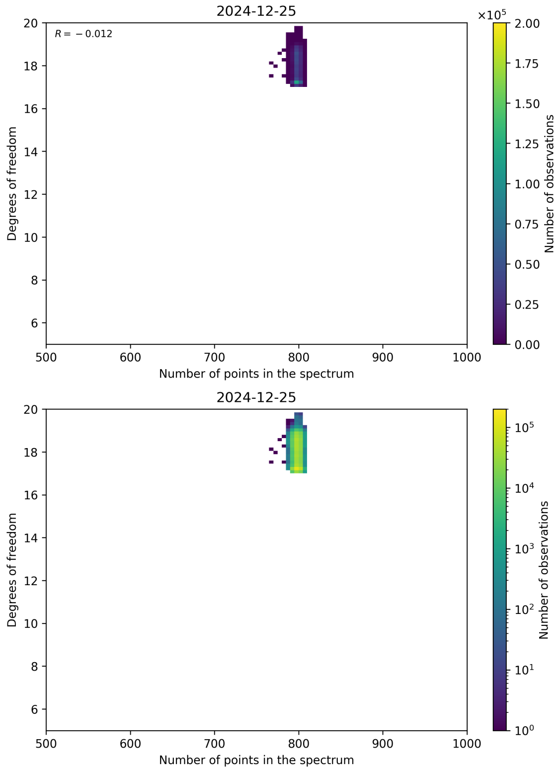
Figure 90: Scatter density plot of “Number of points in the spectrum” against “Degrees of freedom” for 2024-12-24 to 2024-12-26.
