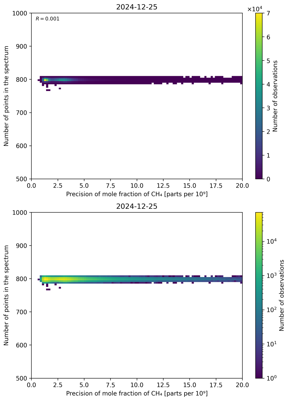
Figure 84: Scatter density plot of “Precision of mole fraction of CH 4 ” against “Number of points in the spectrum” for 2024-12-24 to 2024-12-26.
