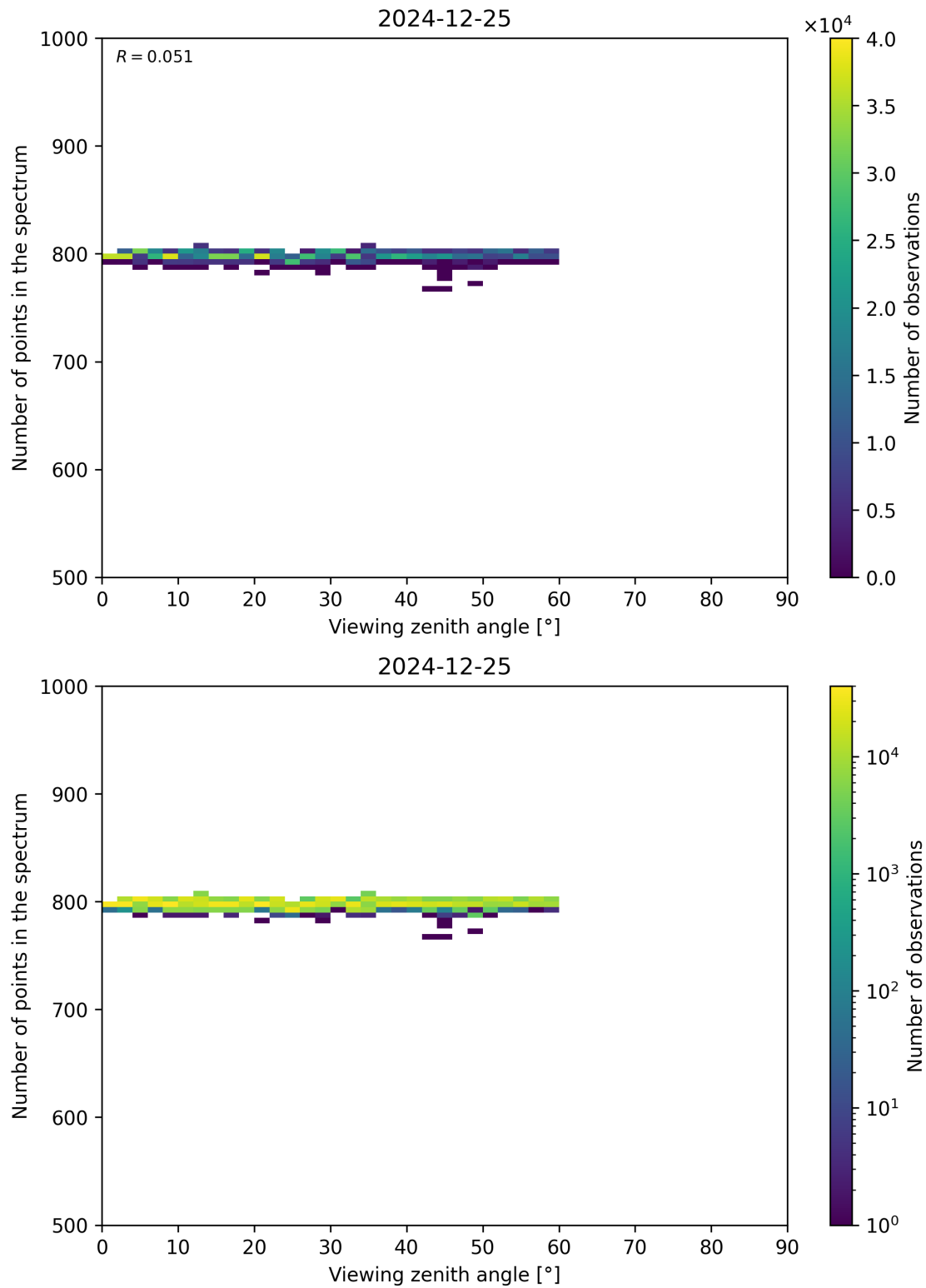
Figure 114: Scatter density plot of “Viewing zenith angle” against “Number of points in the spectrum” for 2024-12-24 to 2024-12-26.
