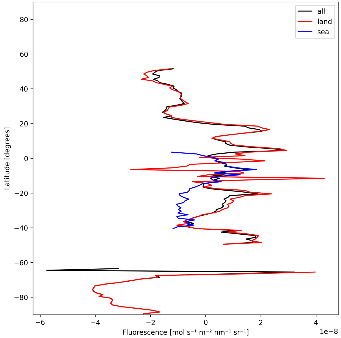
Figure 21: Zonal average of “Fluorescence” for 2024-12-24 to 2024-12-26.
