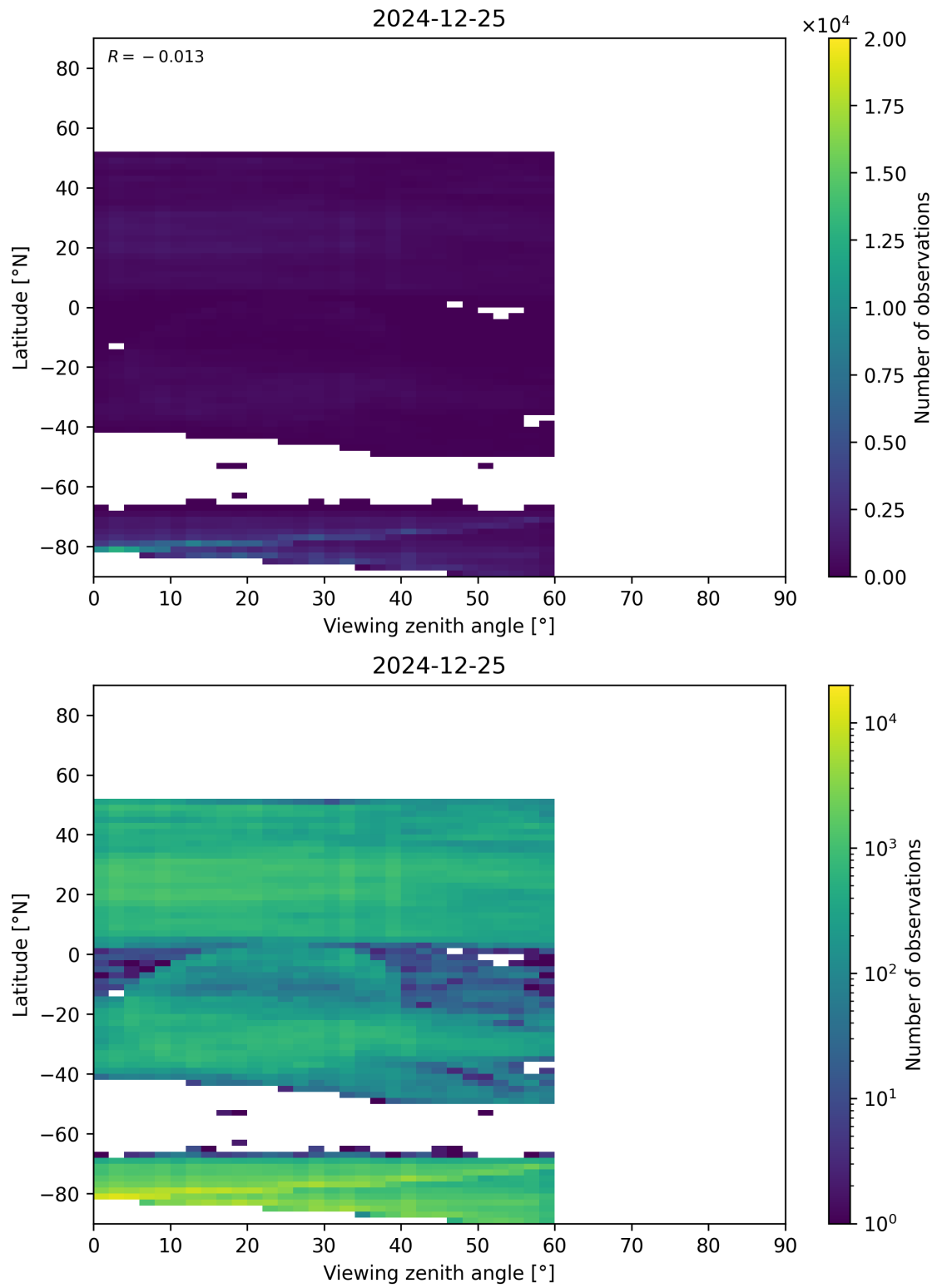
Figure 109: Scatter density plot of “Viewing zenith angle” against “Latitude” for 2024-12-24 to 2024-12-26.
