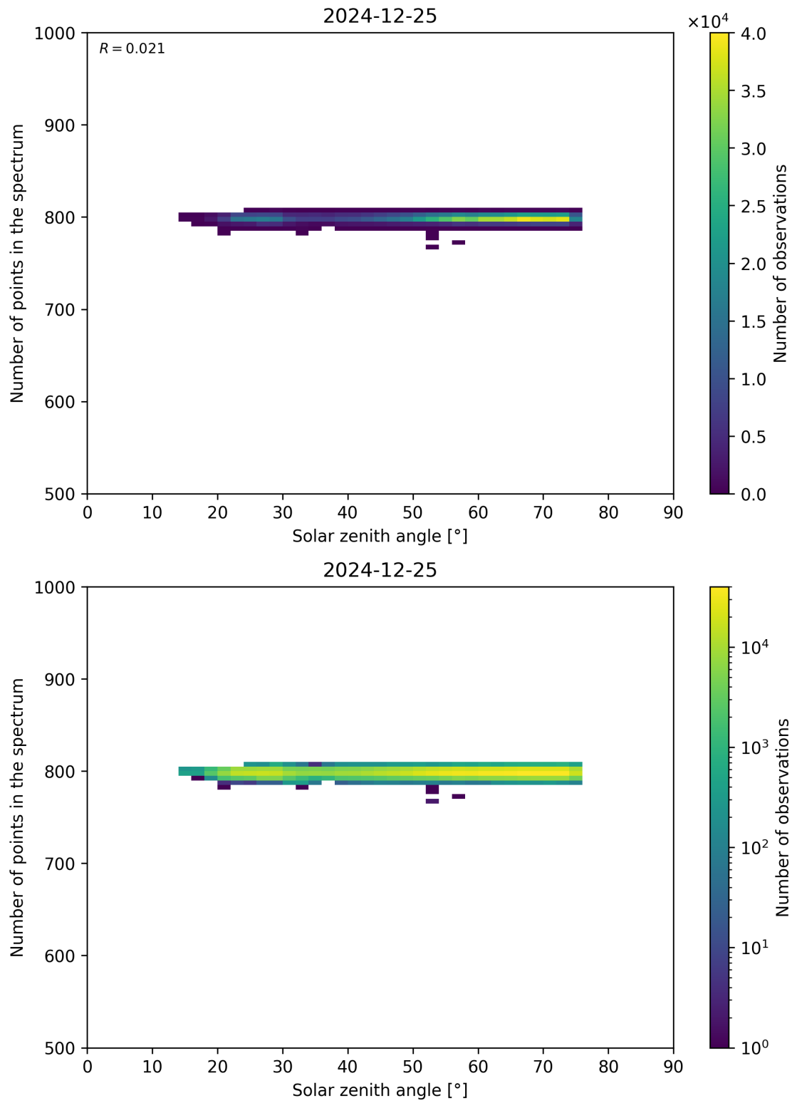
Figure 103: Scatter density plot of “Solar zenith angle” against “Number of points in the spectrum” for 2024-12-24 to 2024-12-26.
