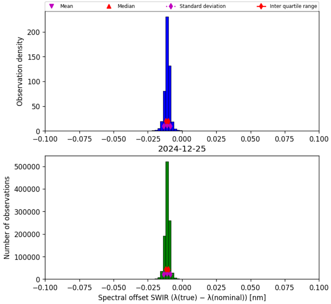
Figure 27: Histogram of “Spectral offset SWIR ( \lambda_{\text{true}} - \lambda_{\text{nominal}} )” for 2024-12-24 to 2024-12-26
