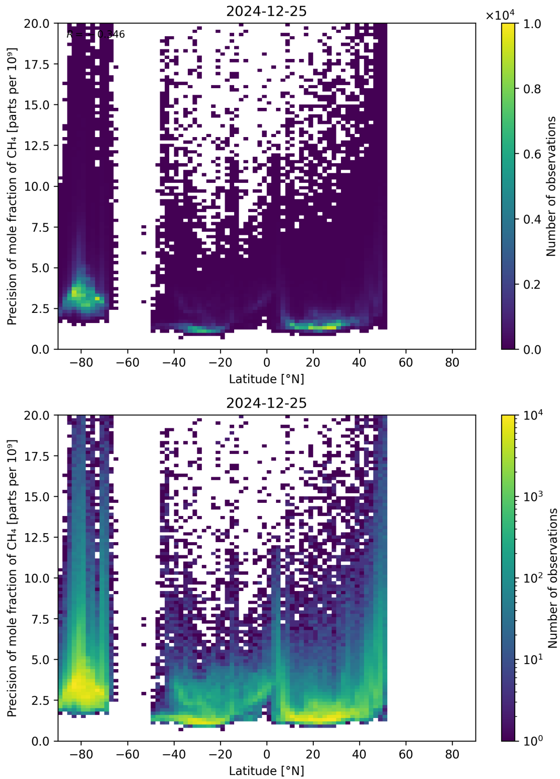
Figure 59: Scatter density plot of “Latitude” against “Precision of mole fraction of CH 4 ” for 2024-12-24 to 2024-12-26.
