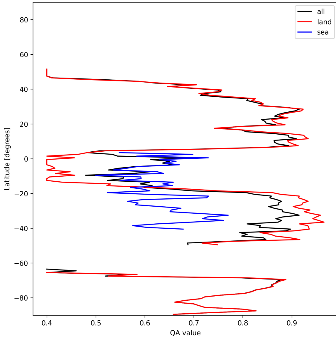
Figure 11: Zonal average of “QA value” for 2024-12-24 to 2024-12-26.
