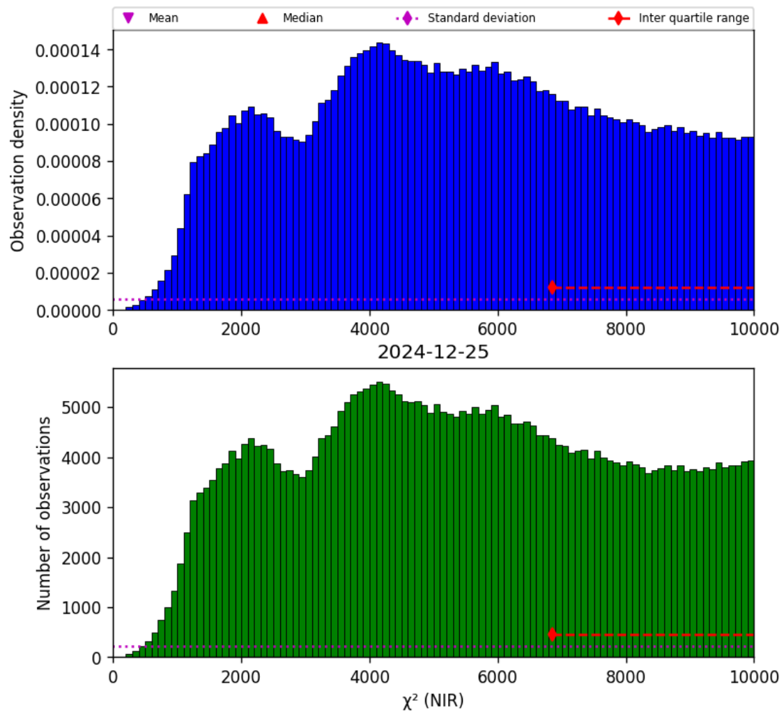
Figure 29: Histogram of “ \chi^2 (NIR)” for 2024-12-24 to 2024-12-26
