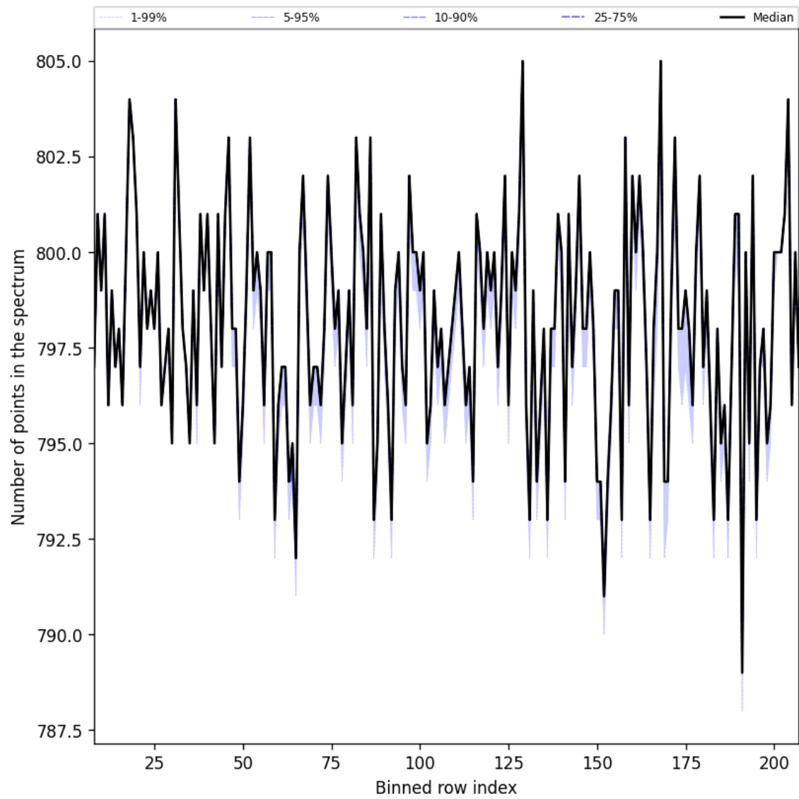
Figure 37: Along track statistics of “Number of points in the spectrum” for 2024-12-24 to 2024-12-26
