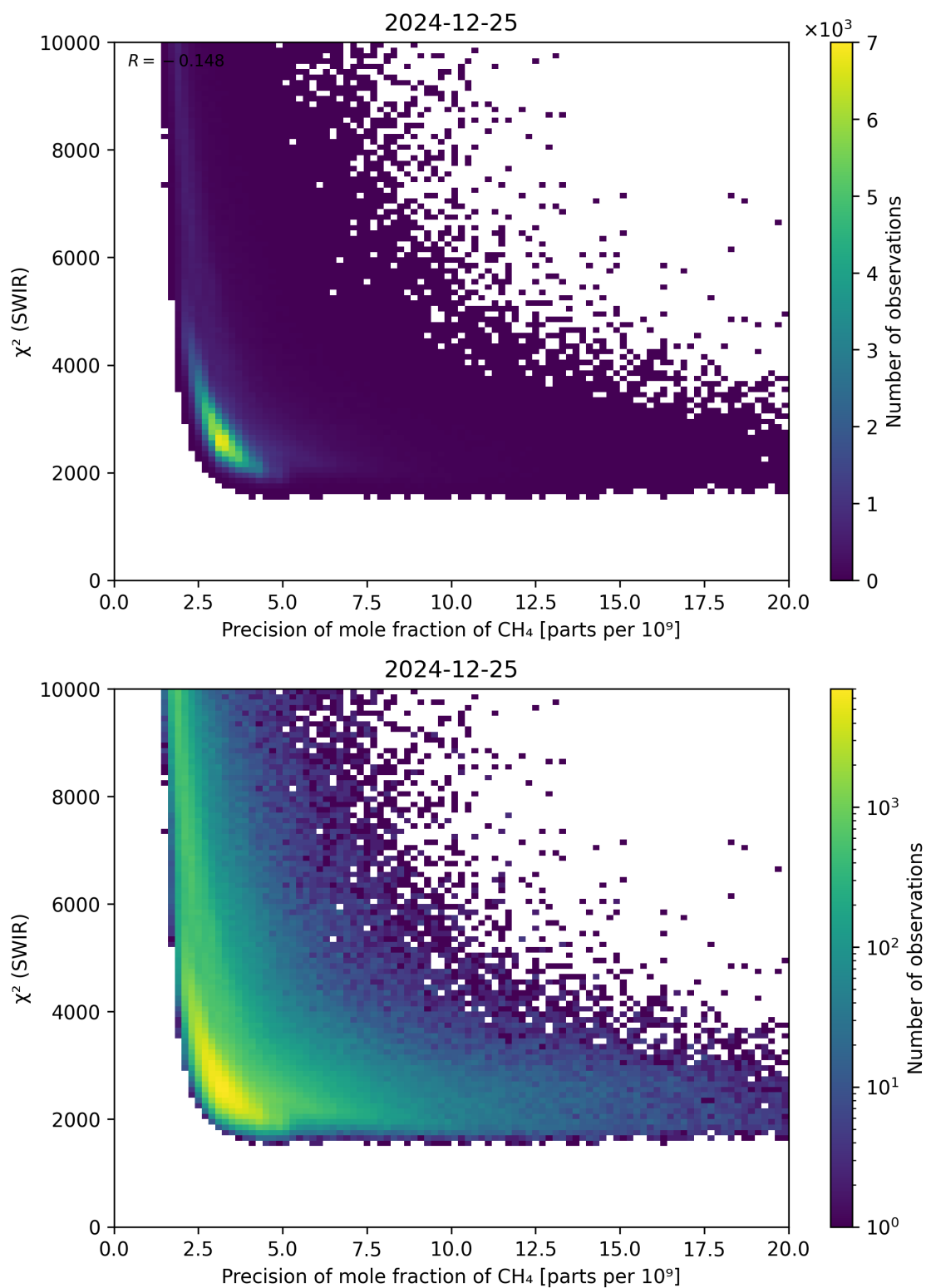
Figure 79: Scatter density plot of “Precision of mole fraction of CH 4 ” against “ \chi^2 (SWIR)” for 2024-12-24 to 2024-12-26.
