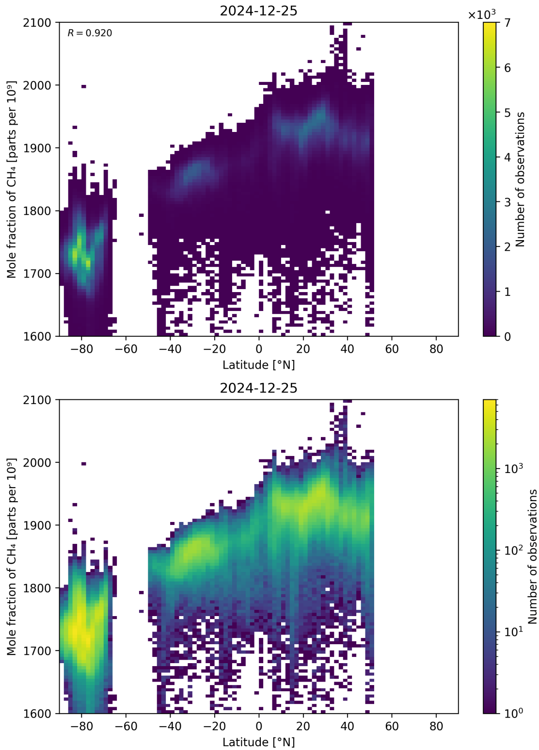
Figure 57: Scatter density plot of “Latitude” against “Mole fraction of CH 4 ” for 2024-12-24 to 2024-12-26.
