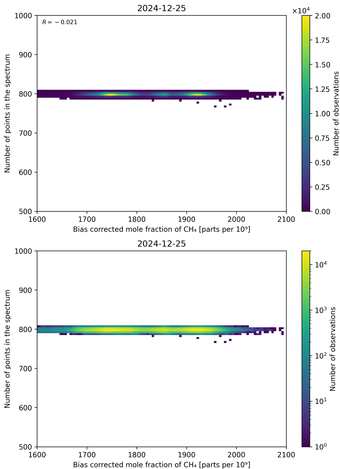
Figure 68: Scatter density plot of “Bias corrected mole fraction of CH 4 ” against “Number of points in the spectrum” for 2024-12-24 to 2024-12-26.
