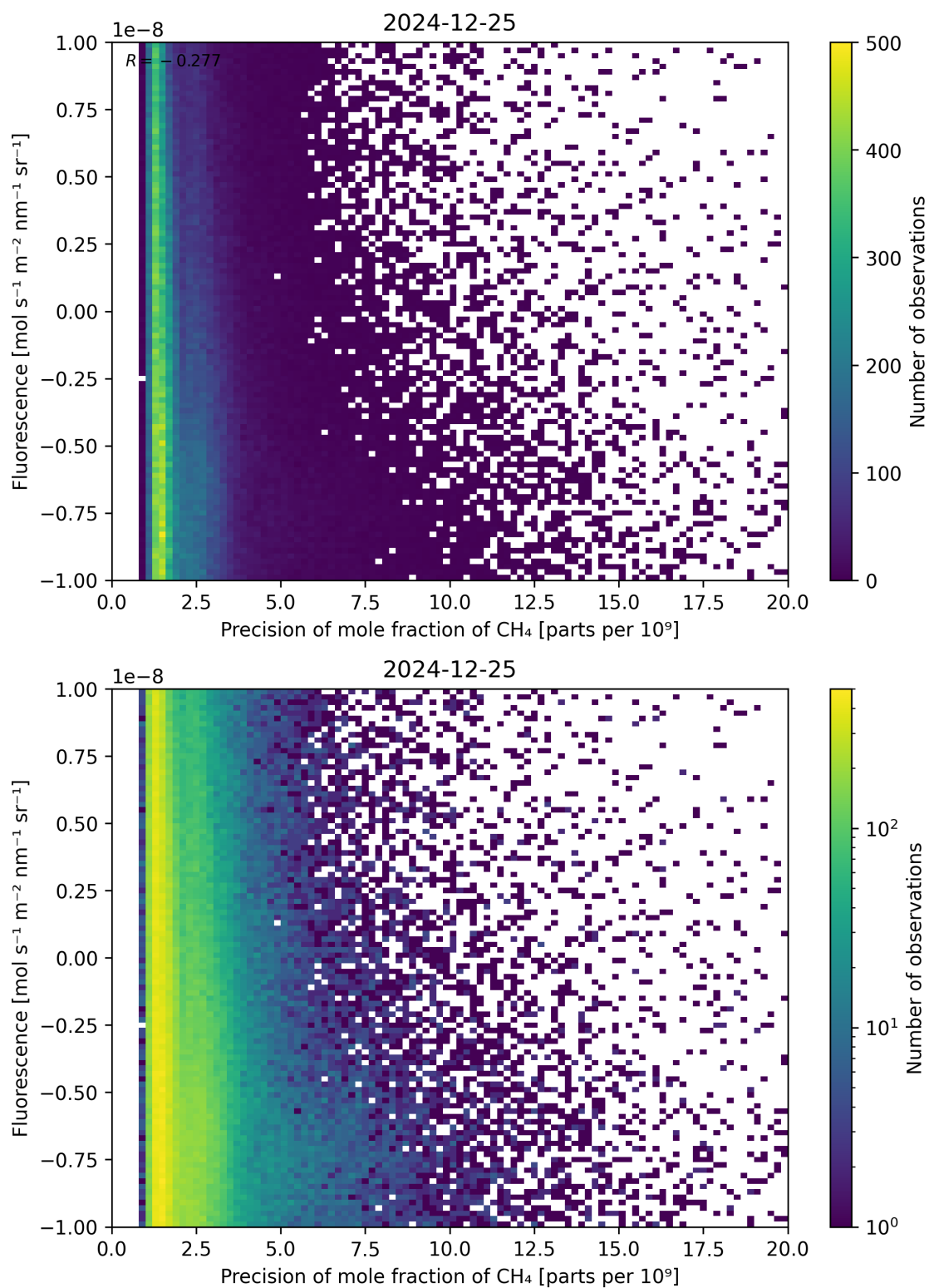
Figure 81: Scatter density plot of “Precision of mole fraction of CH 4 ” against “Fluorescence” for 2024-12-24 to 2024-12-26.
