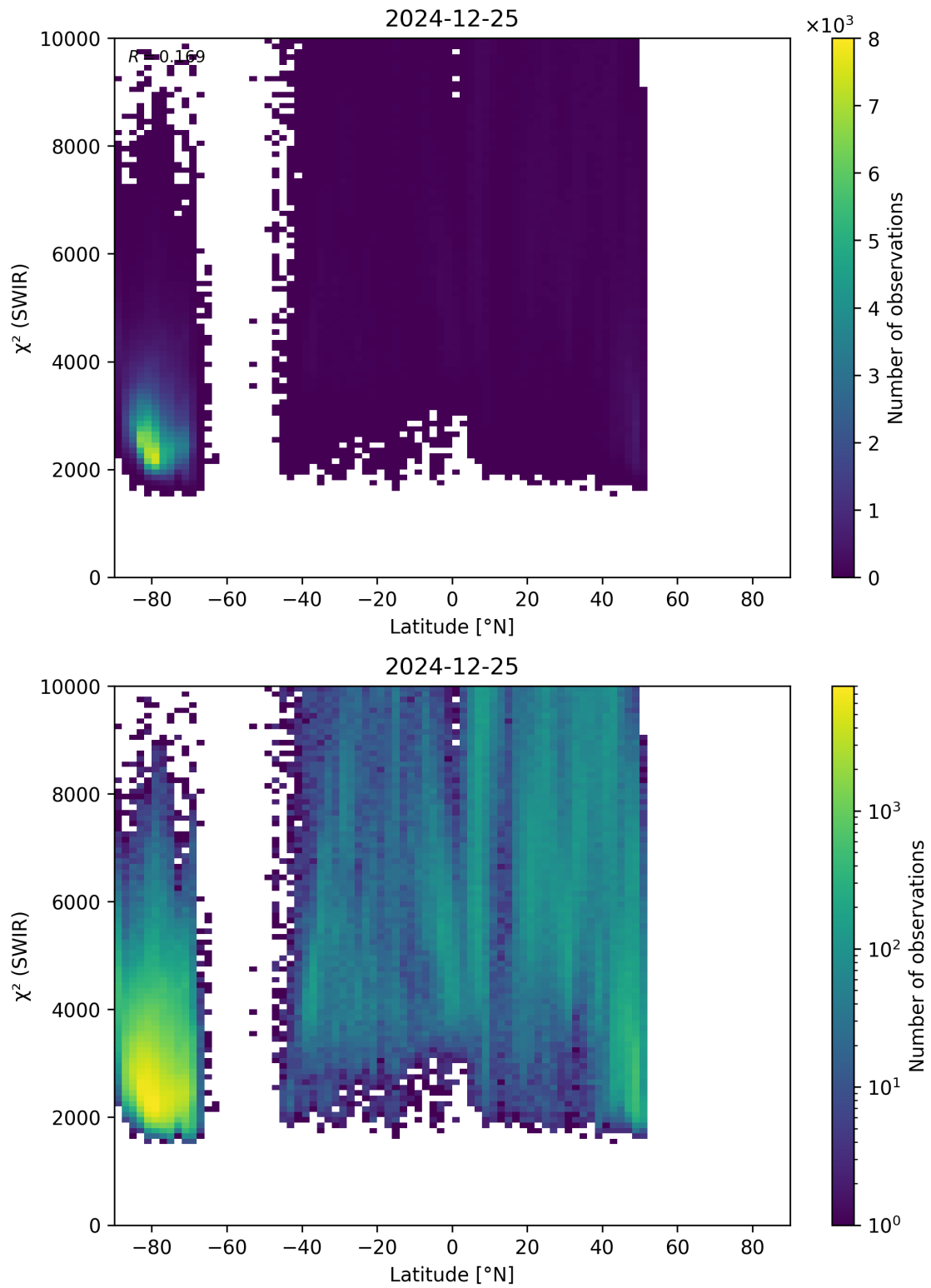
Figure 54: Scatter density plot of “Latitude” against “ \chi^2 (SWIR)” for 2024-12-24 to 2024-12-26.
