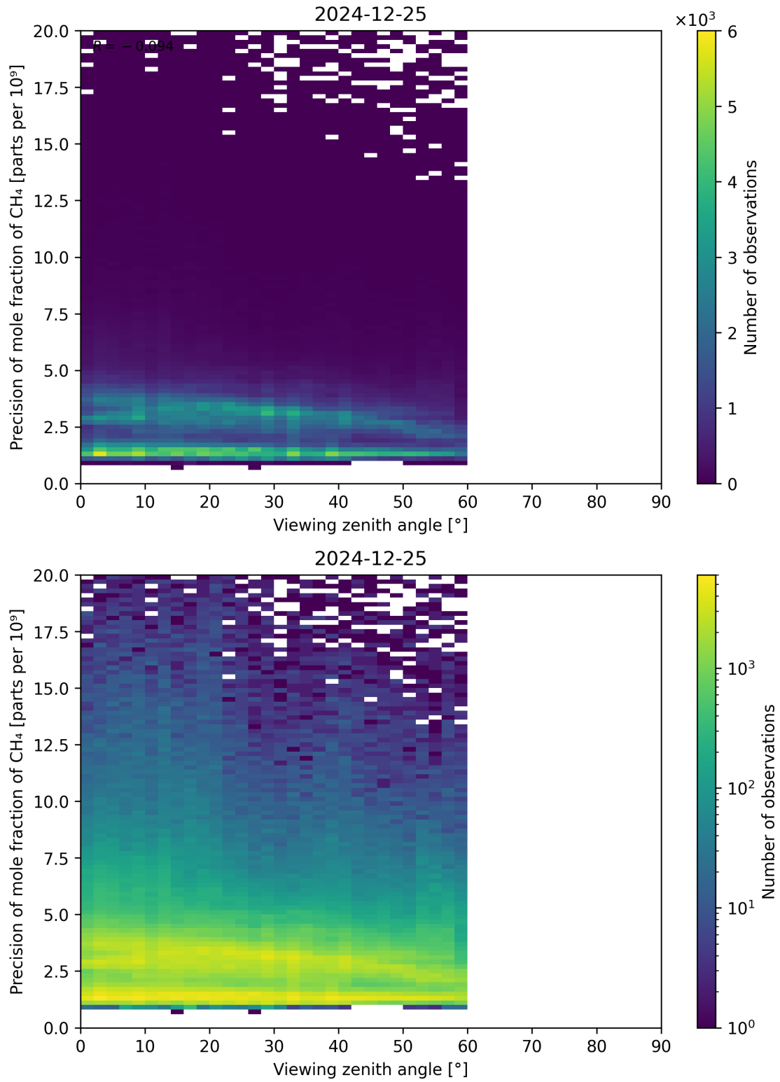
Figure 112: Scatter density plot of “Viewing zenith angle” against “Precision of mole fraction of CH 4 ” for 2024-12-24 to 2024-12-26.
