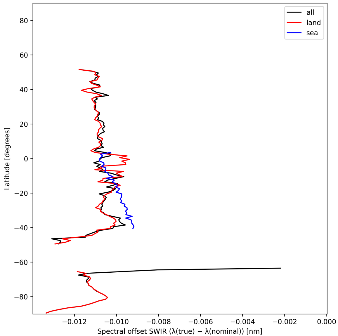
Figure 16: Zonal average of “Spectral offset SWIR ( \lambda_{\text{true}} - \lambda_{\text{nominal}} )” for 2024-12-24 to 2024-12-26.
