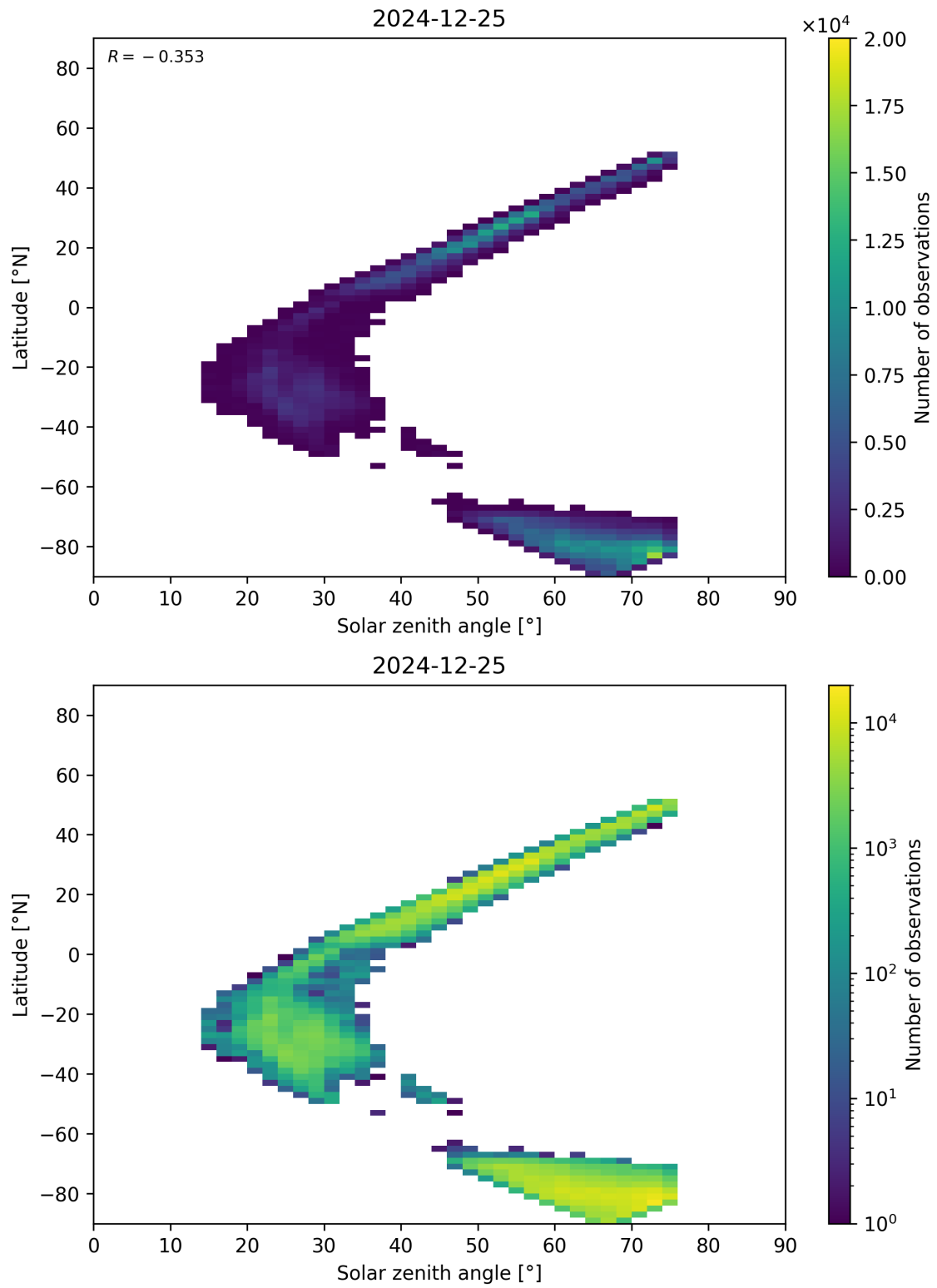
Figure 98: Scatter density plot of “Solar zenith angle” against “Latitude” for 2024-12-24 to 2024-12-26.
