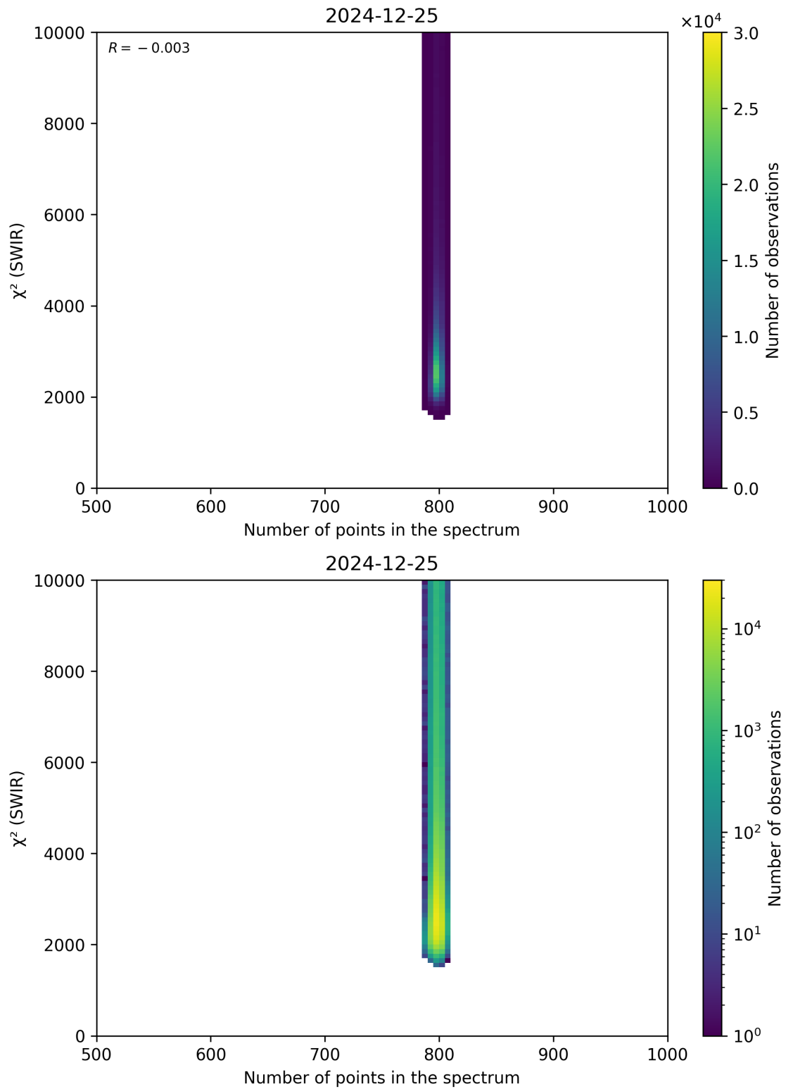
Figure 89: Scatter density plot of “Number of points in the spectrum” against “ \chi^2 (SWIR)” for 2024-12-24 to 2024-12-26.
