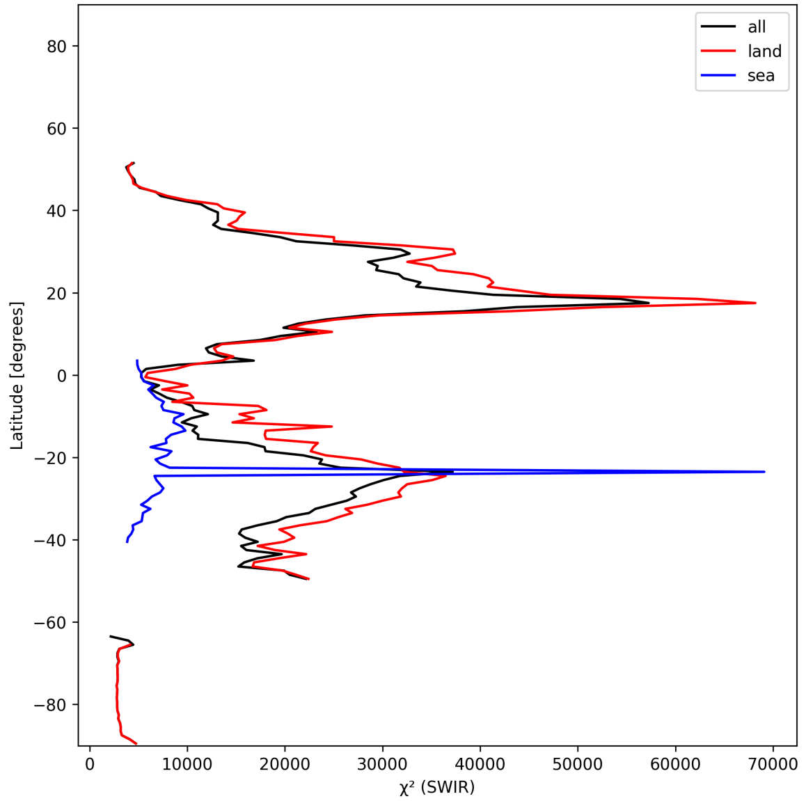
Figure 17: Zonal average of “ \chi^2 (SWIR)” for 2024-12-24 to 2024-12-26.
