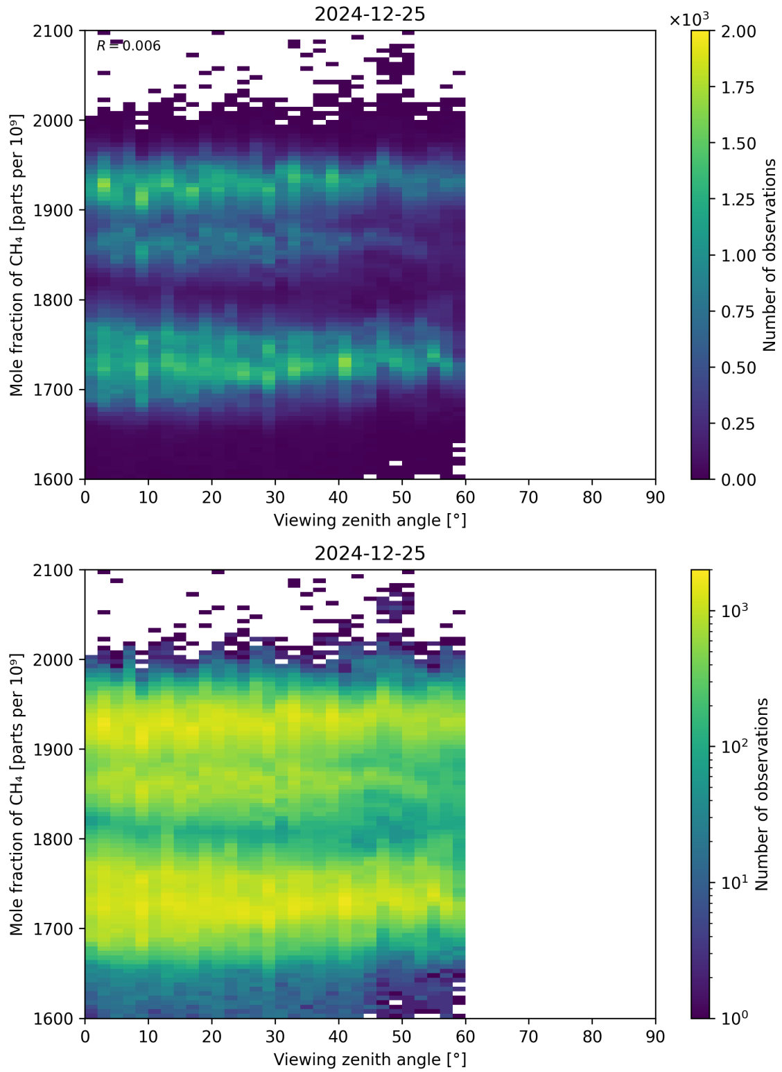
Figure 110: Scatter density plot of “Viewing zenith angle” against “Mole fraction of CH 4 ” for 2024-12-24 to 2024-12-26.
