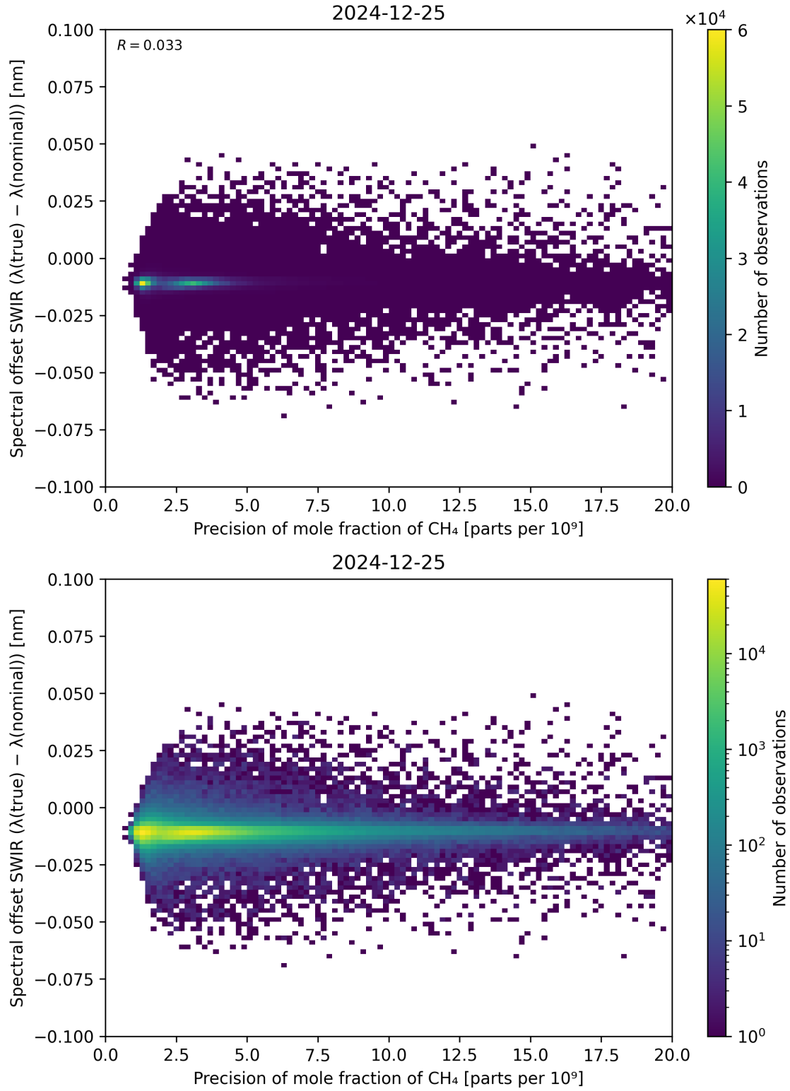
Figure 85: Scatter density plot of “Precision of mole fraction of CH 4 ” against “Spectral offset SWIR ( \lambda_{\text{true}} - \lambda_{\text{nominal}} )” for 2024-12-24 to 2024-12-26.
