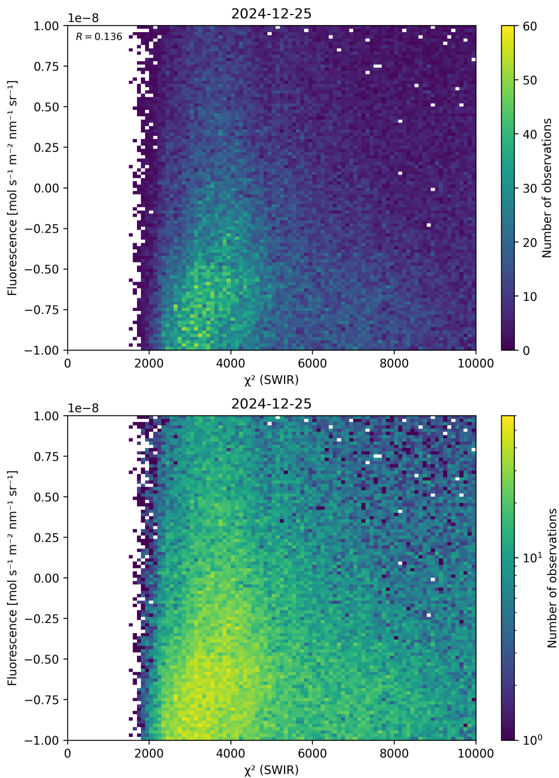
Figure 49: Scatter density plot of “ \chi^2 (SWIR)” against “Fluorescence” for 2024-12-24 to 2024-12-26.
