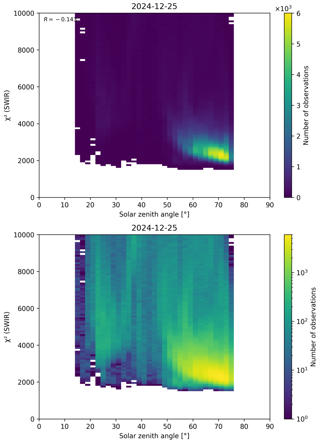
Figure 95: Scatter density plot of “Solar zenith angle” against “ \chi^2 (SWIR)” for 2024-12-24 to 2024-12-26.
