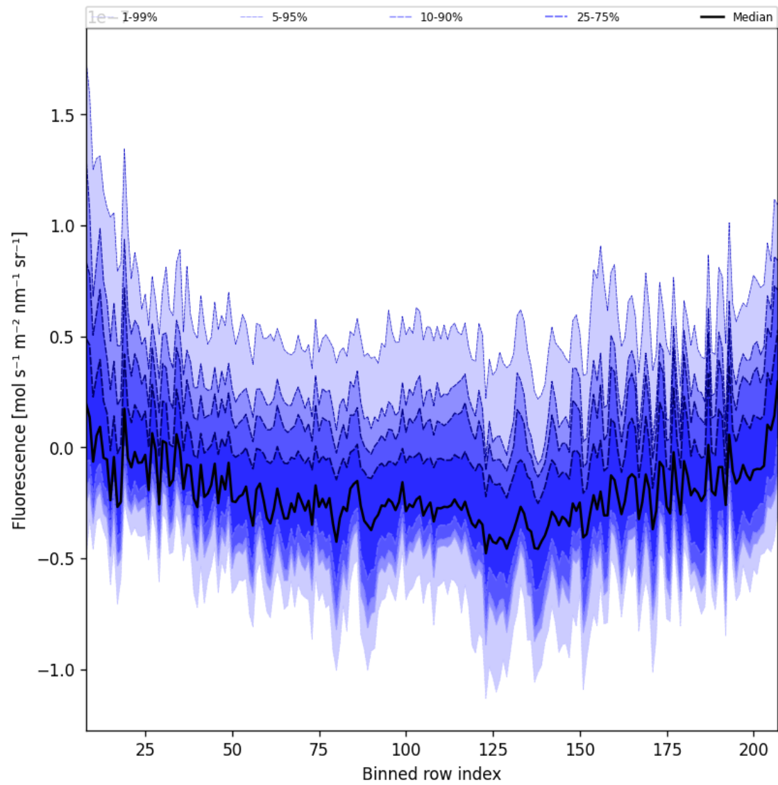
Figure 43: Along track statistics of “Fluorescence” for 2024-12-24 to 2024-12-26
