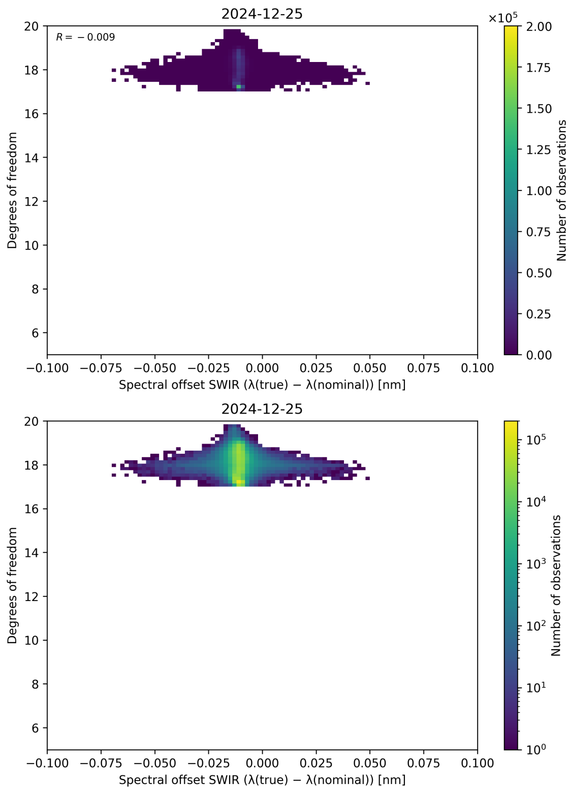
Figure 119: Scatter density plot of “Spectral offset SWIR ( \lambda_{\text{true}} - \lambda_{\text{nominal}} )” against “Degrees of freedom” for 2024-12-24 to 2024-12-26.
