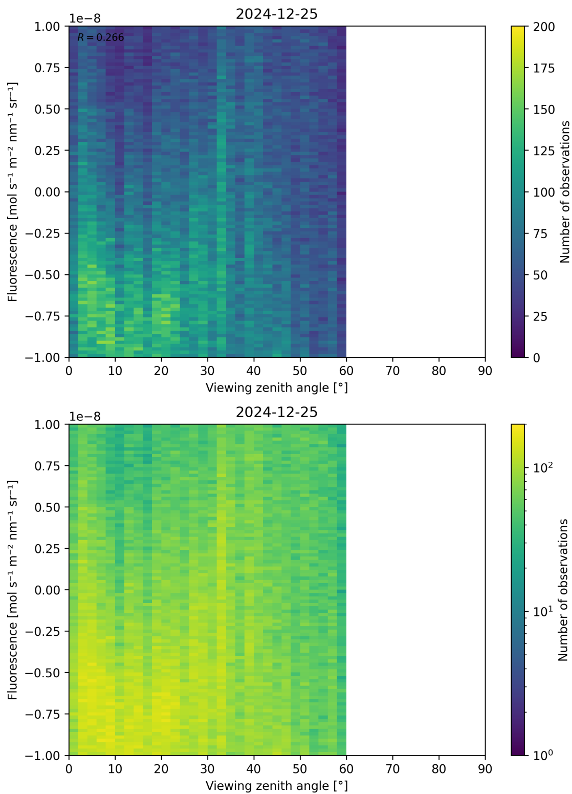
Figure 108: Scatter density plot of “Viewing zenith angle” against “Fluorescence” for 2024-12-24 to 2024-12-26.
