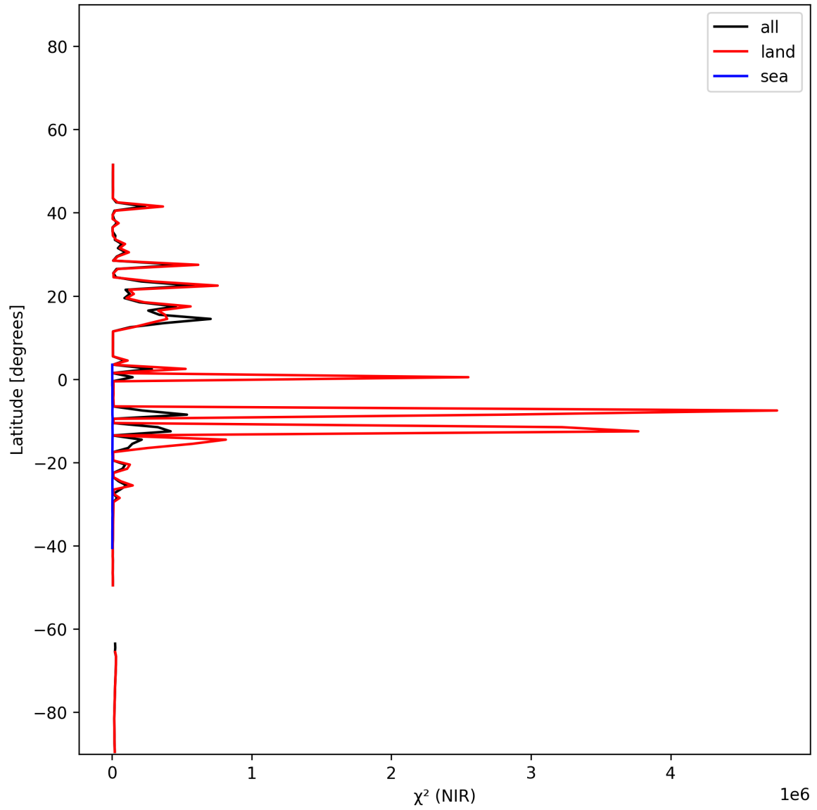
Figure 18: Zonal average of “ \chi^2 (NIR)” for 2024-12-24 to 2024-12-26.
