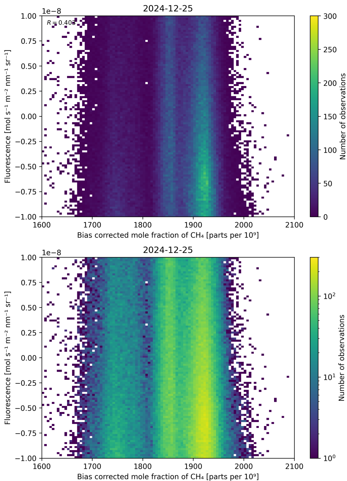
Figure 66: Scatter density plot of “Bias corrected mole fraction of \text{CH}_4 ” against “Fluorescence” for 2024-12-24 to 2024-12-26.
