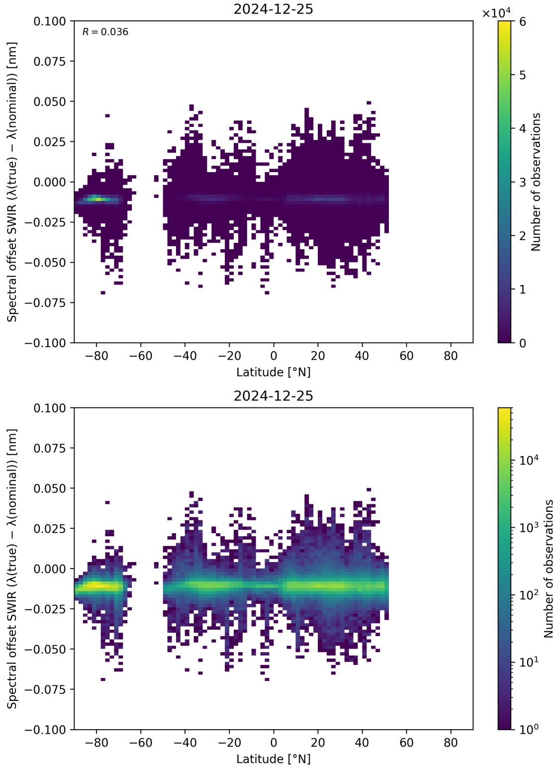
Figure 62: Scatter density plot of “Latitude” against “Spectral offset SWIR ( \lambda_{\text{true}} - \lambda_{\text{nominal}} )” for 2024-12-24 to 2024-12-26.
