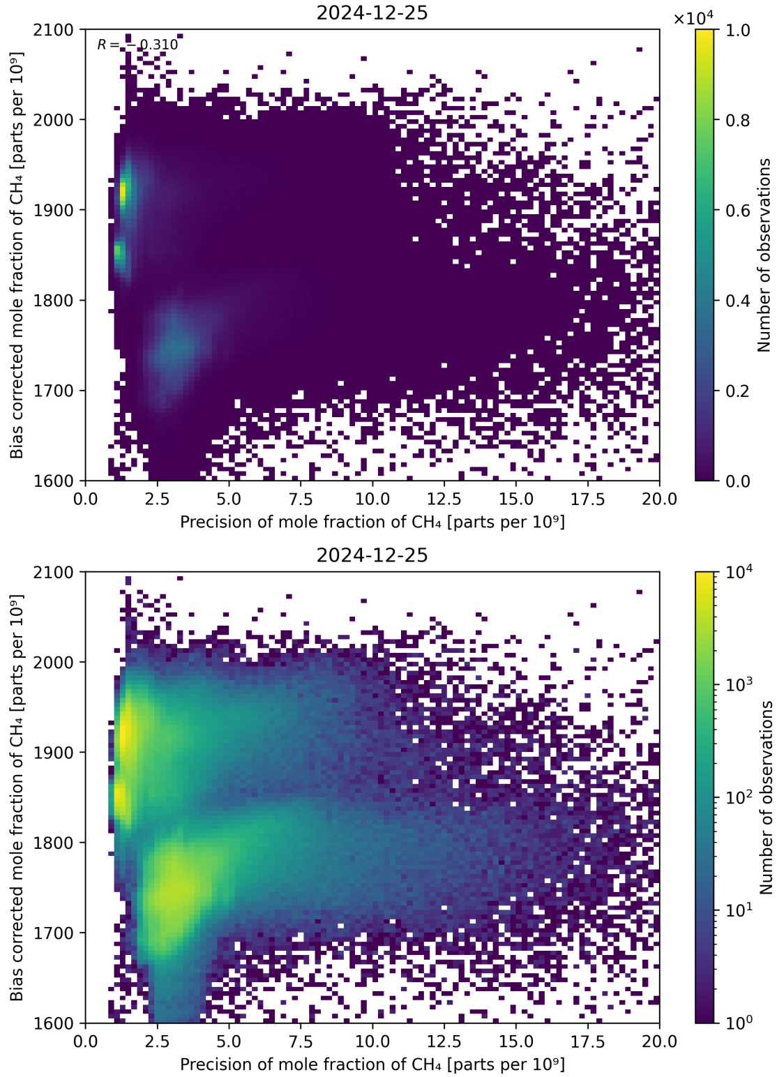
Figure 82: Scatter density plot of “Precision of mole fraction of \text{CH}_4 ” against “Bias corrected mole fraction of \text{CH}_4 ” for 2024-12-24 to 2024-12-26.
