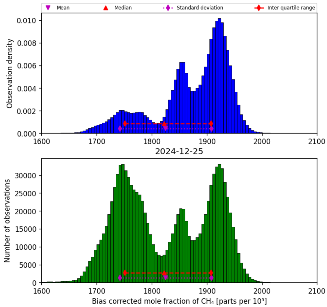
Figure 25: Histogram of “Bias corrected mole fraction of CH 4 ” for 2024-12-24 to 2024-12-26
