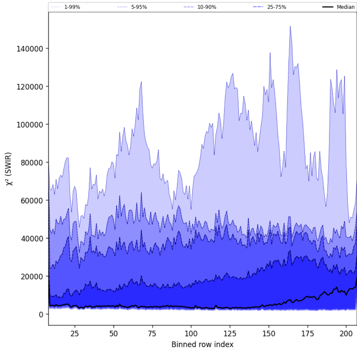
Figure 39: Along track statistics of “ \chi^2 (SWIR)” for 2024-12-24 to 2024-12-26
