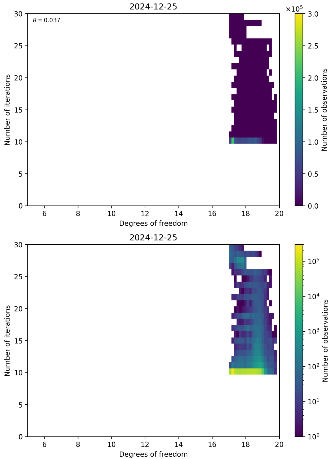
Figure 52: Scatter density plot of “Degrees of freedom” against “Number of iterations” for 2024-12-24 to 2024-12-26.
