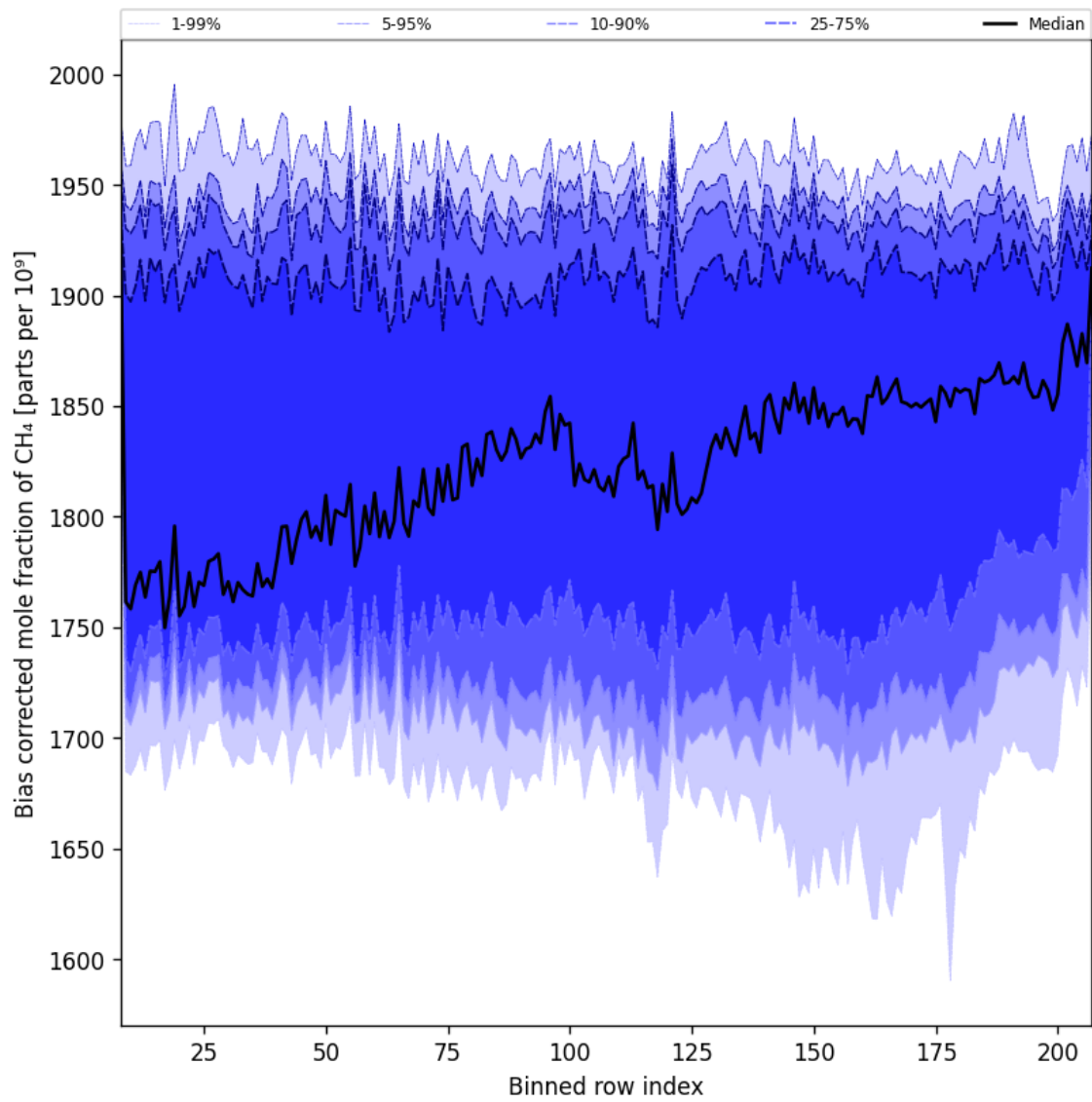
Figure 36: Along track statistics of “Bias corrected mole fraction of CH 4 ” for 2024-12-24 to 2024-12-26
