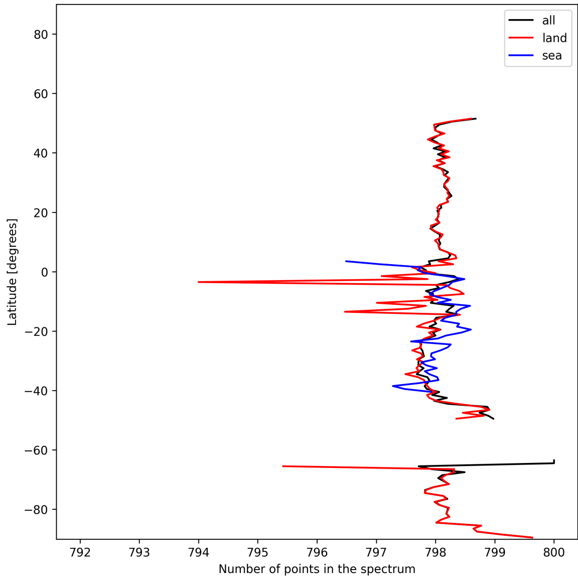
Figure 15: Zonal average of “Number of points in the spectrum” for 2024-12-24 to 2024-12-26.
