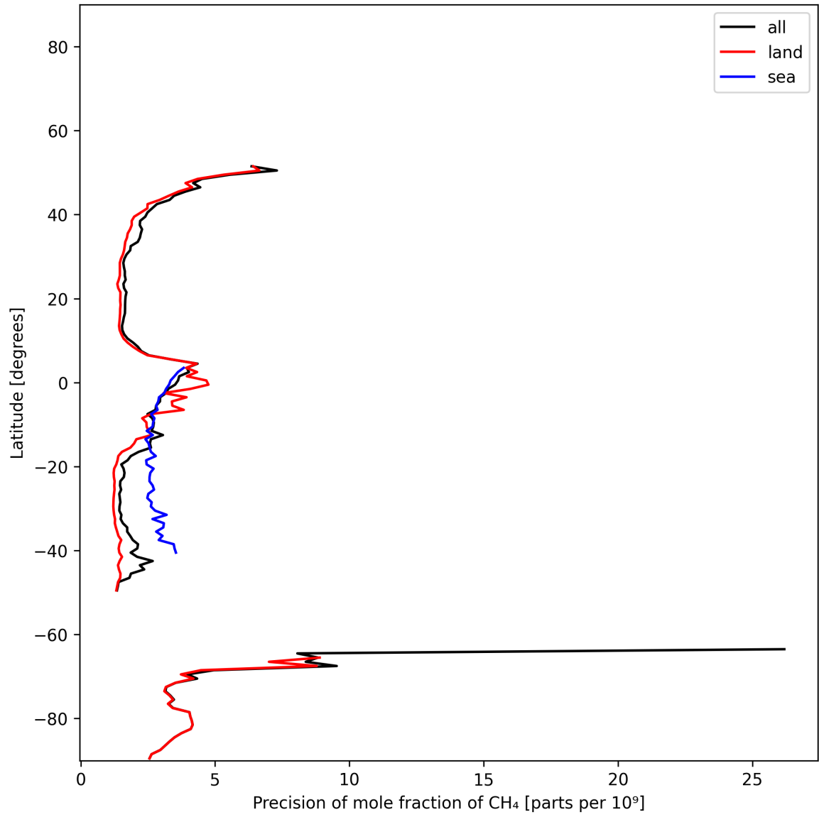
Figure 13: Zonal average of “Precision of mole fraction of CH 4 ” for 2024-12-24 to 2024-12-26.
