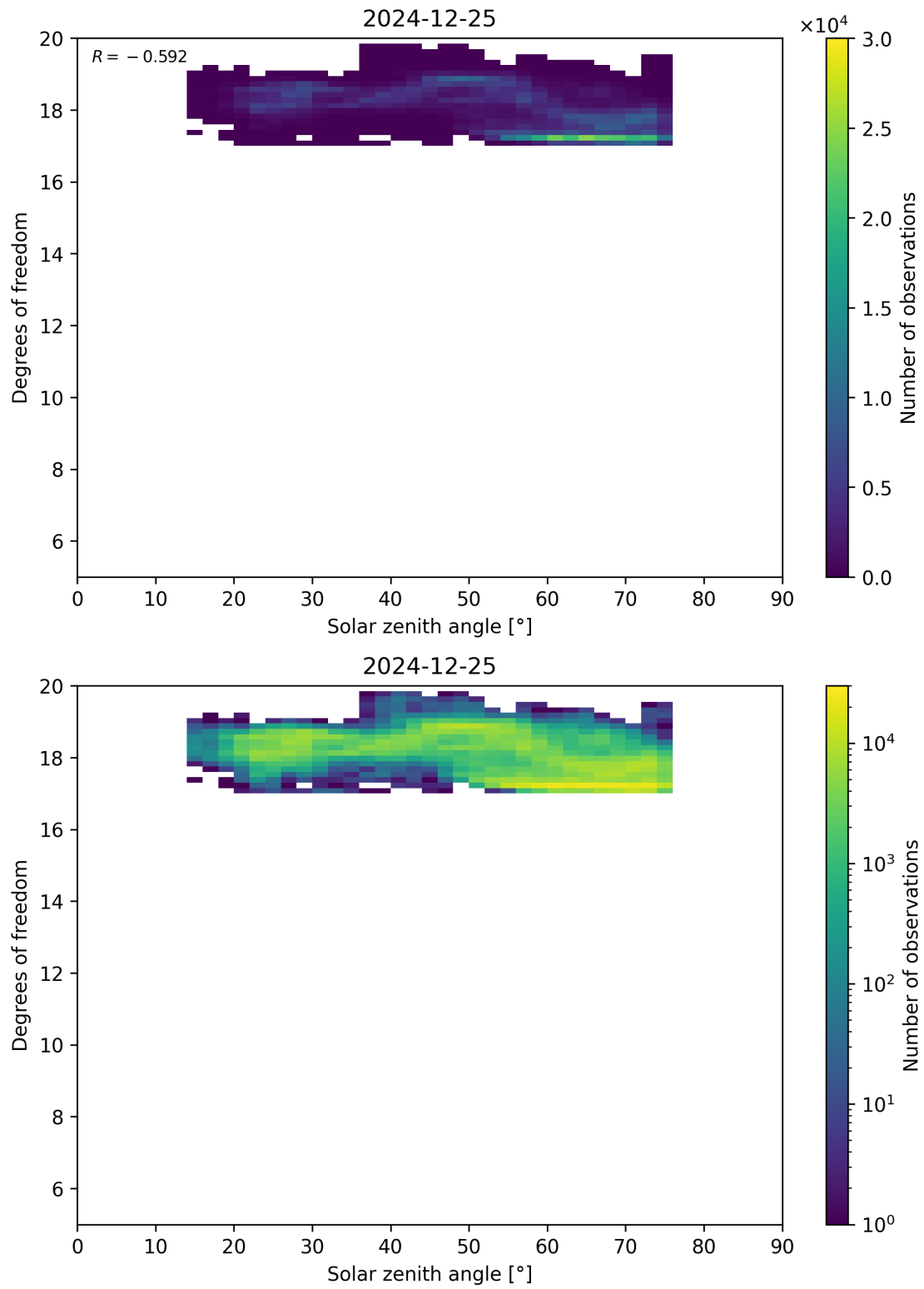
Figure 96: Scatter density plot of “Solar zenith angle” against “Degrees of freedom” for 2024-12-24 to 2024-12-26.
