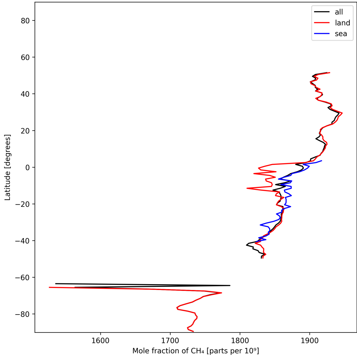
Figure 12: Zonal average of “Mole fraction of CH 4 ” for 2024-12-24 to 2024-12-26.
