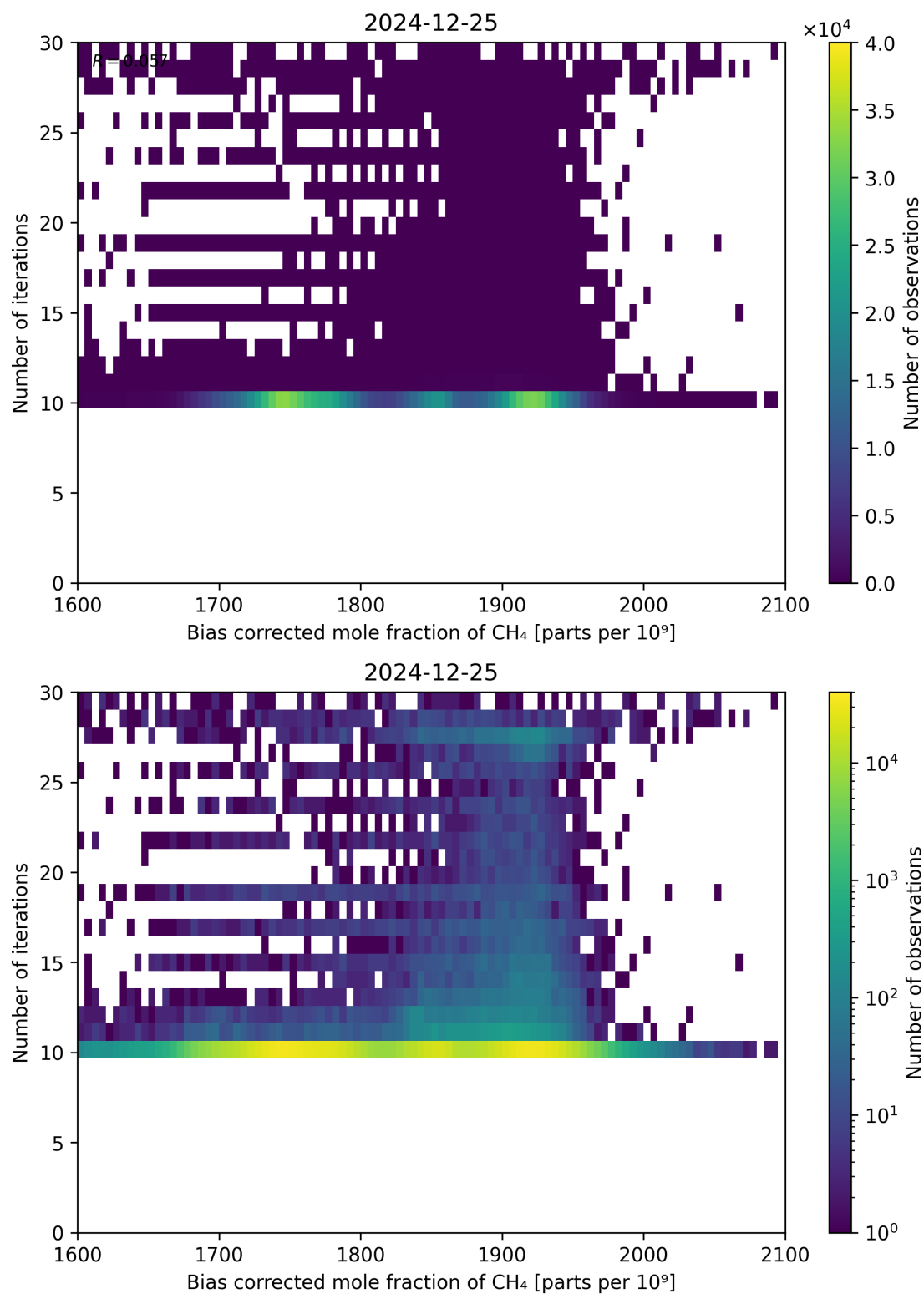
Figure 67: Scatter density plot of “Bias corrected mole fraction of \text{CH}_4 ” against “Number of iterations” for 2024-12-24 to 2024-12-26.
