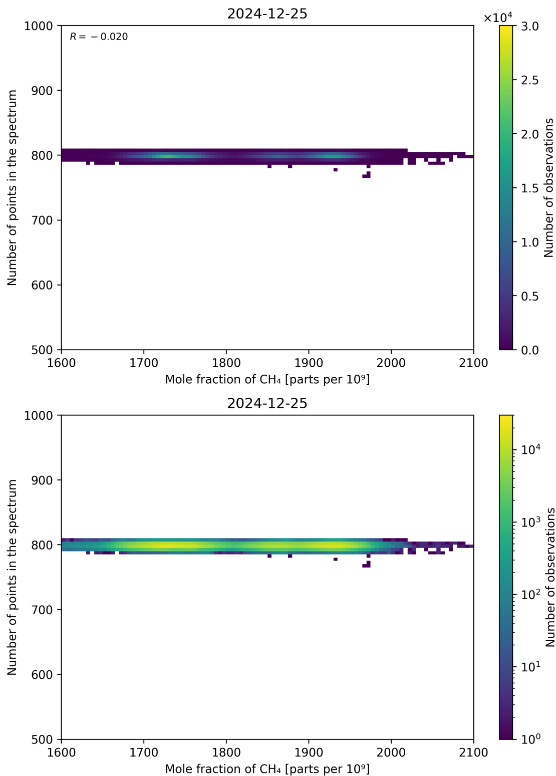
Figure 77: Scatter density plot of “Mole fraction of CH 4 ” against “Number of points in the spectrum” for 2024-12-24 to 2024-12-26.
