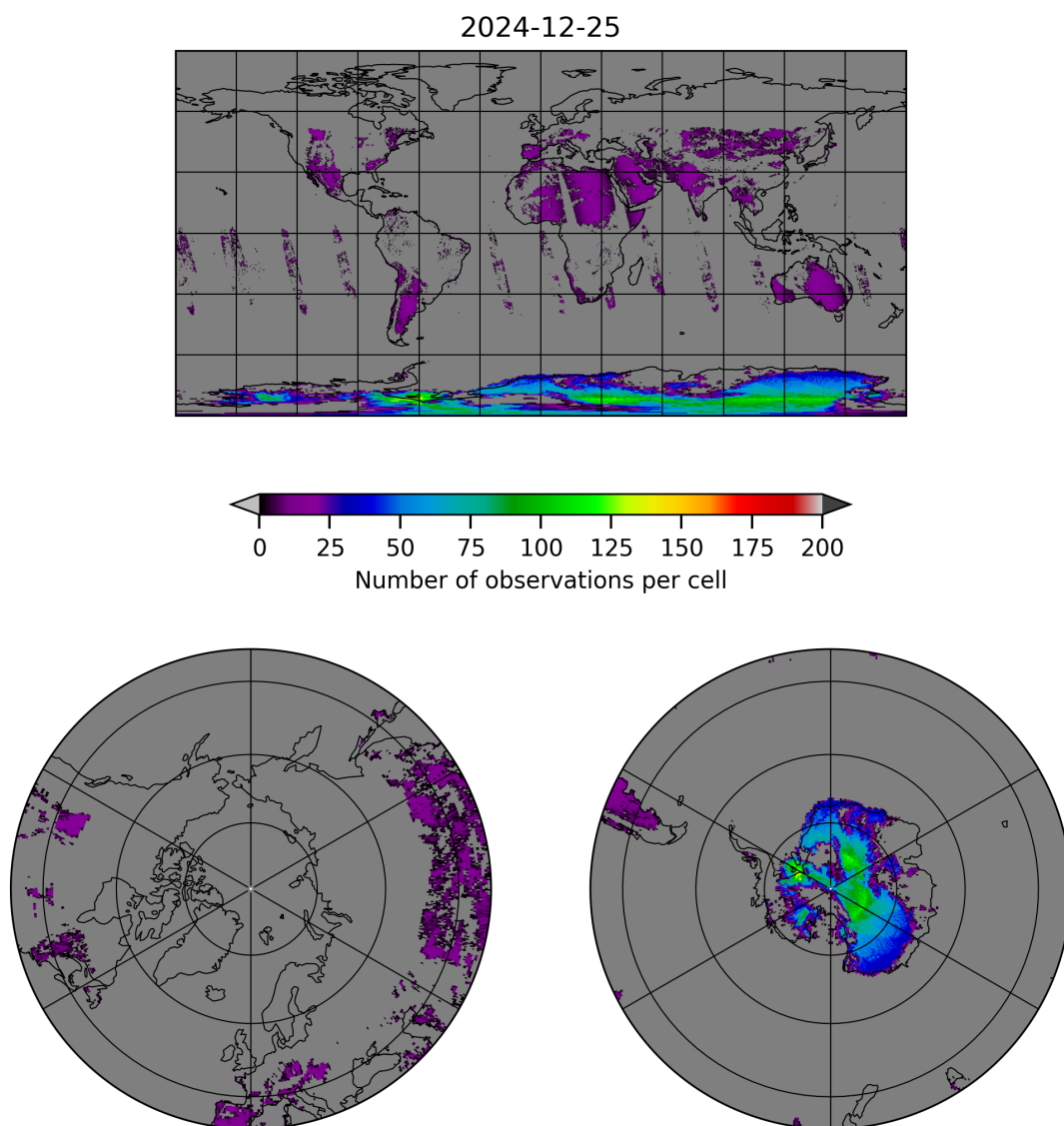
Figure 10: Map of the number of observations for 2024-12-24 to 2024-12-26
