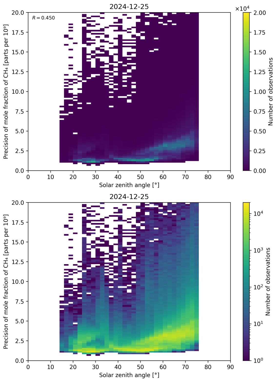
Figure 101: Scatter density plot of “Solar zenith angle” against “Precision of mole fraction of CH 4 ” for 2024-12-24 to 2024-12-26.
