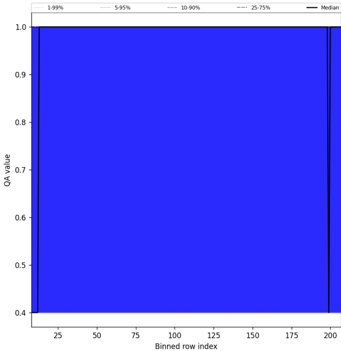
Figure 33: Along track statistics of “QA value” for 2024-12-24 to 2024-12-26
