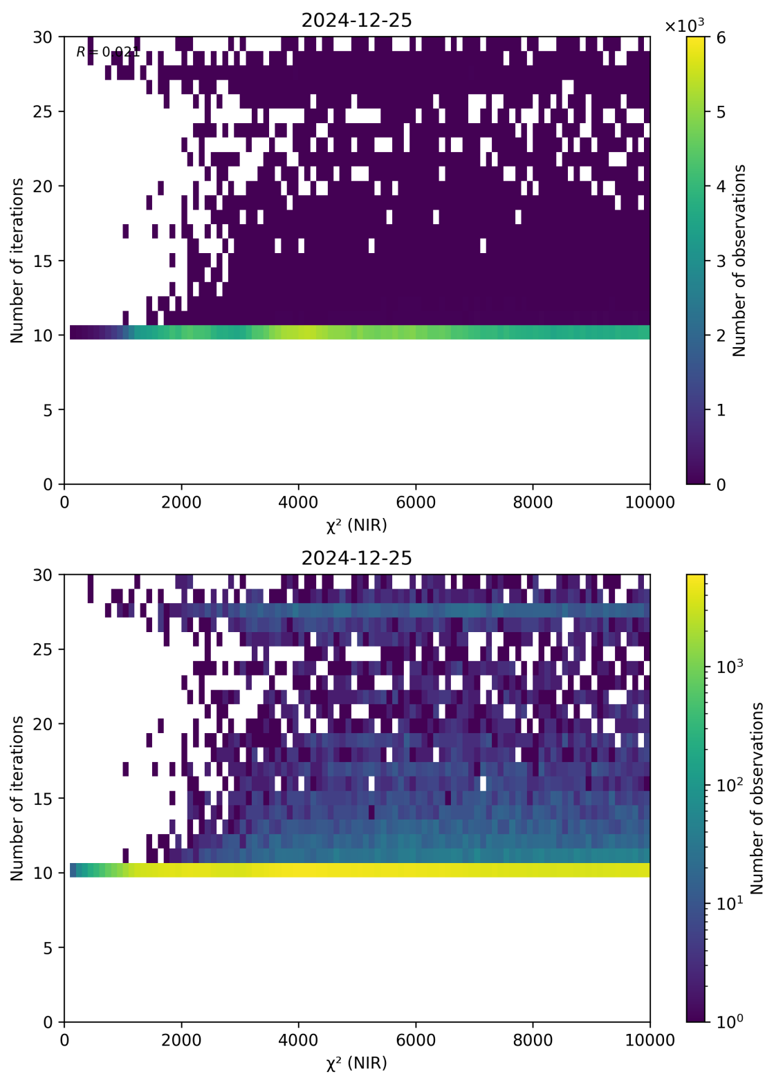
Figure 46: Scatter density plot of “ \chi^2 (NIR)” against “Number of iterations” for 2024-12-24 to 2024-12-26.
