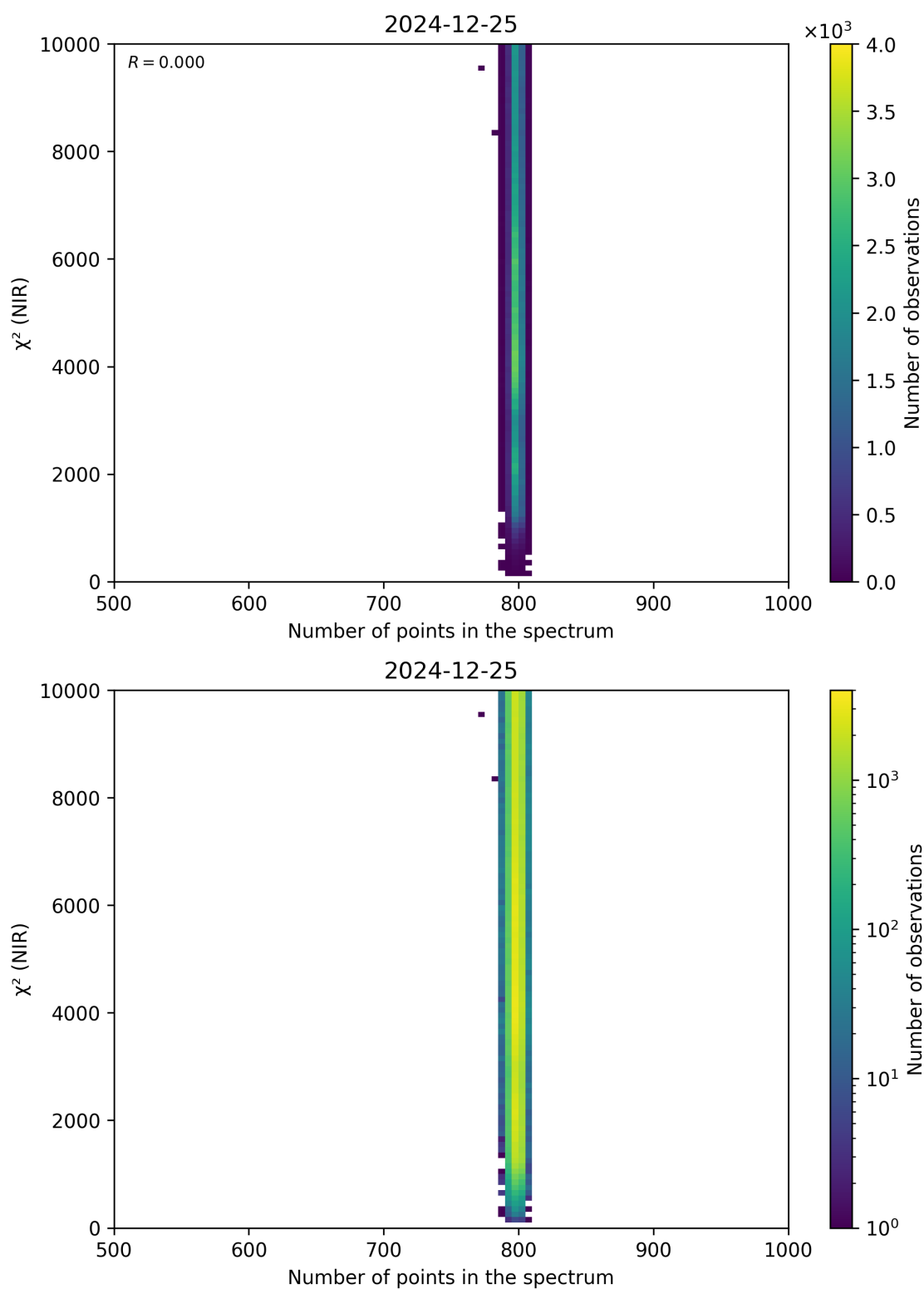
Figure 88: Scatter density plot of “Number of points in the spectrum” against “ \chi^2 (NIR)” for 2024-12-24 to 2024-12-26.
