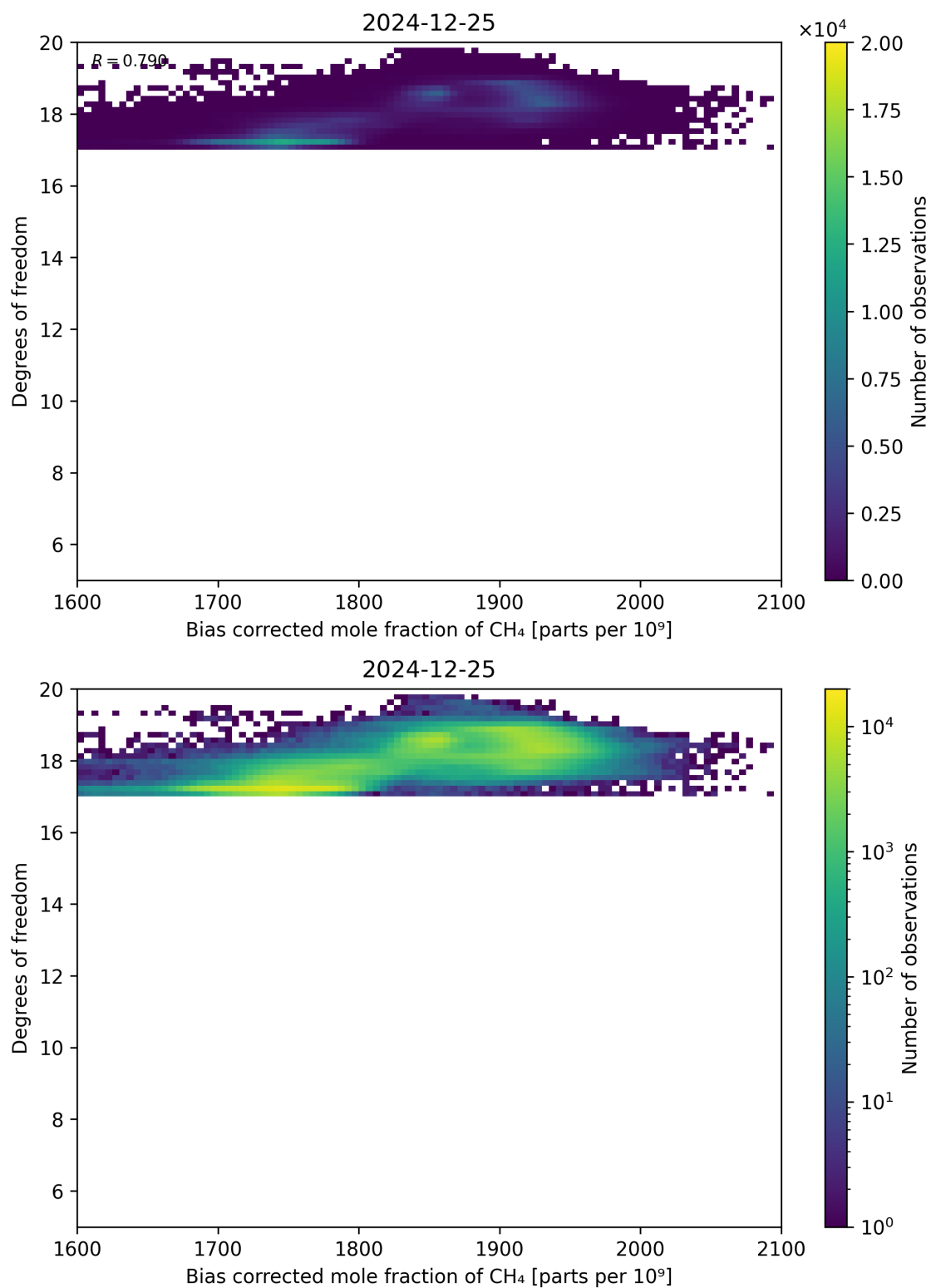
Figure 65: Scatter density plot of “Bias corrected mole fraction of CH 4 ” against “Degrees of freedom” for 2024-12-24 to 2024-12-26.
