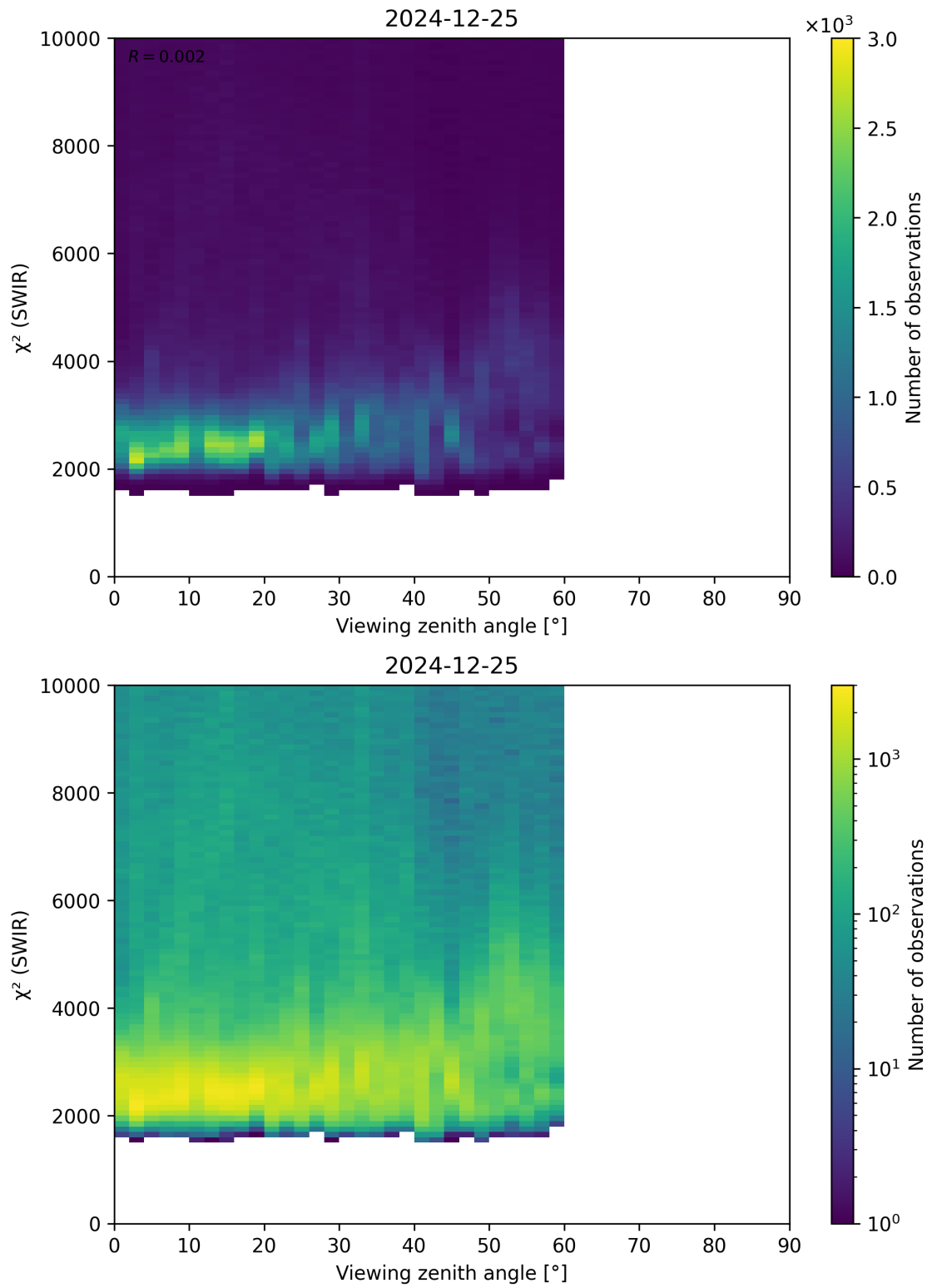
Figure 106: Scatter density plot of “Viewing zenith angle” against “ \chi^2 (SWIR)” for 2024-12-24 to 2024-12-26.
