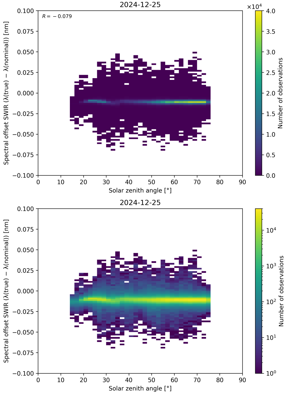
Figure 104: Scatter density plot of “Solar zenith angle” against “Spectral offset SWIR ( \lambda_{\text{true}} - \lambda_{\text{nominal}} )” for 2024-12-24 to 2024-12-26.
