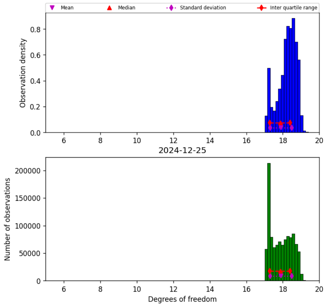
Figure 30: Histogram of “Degrees of freedom” for 2024-12-24 to 2024-12-26
