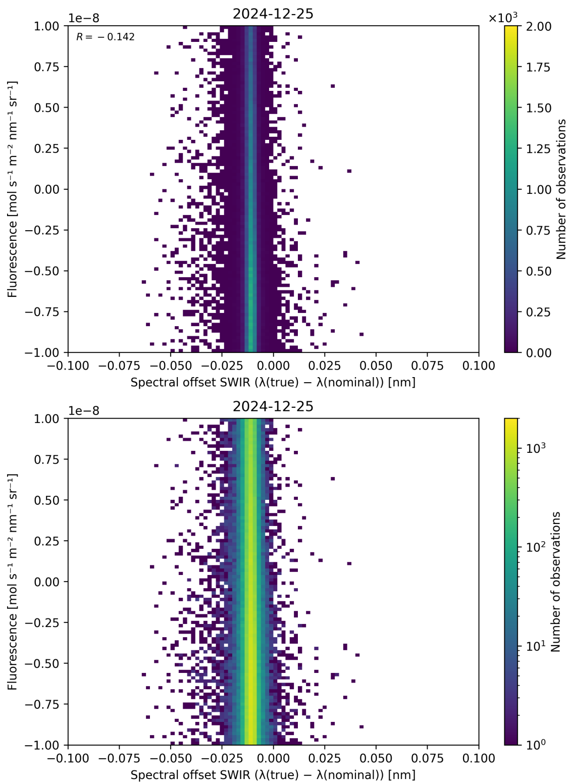
Figure 120: Scatter density plot of “Spectral offset SWIR ( \lambda_{\text{true}} - \lambda_{\text{nominal}} )” against “Fluorescence” for 2024-12-24 to 2024-12-26.
