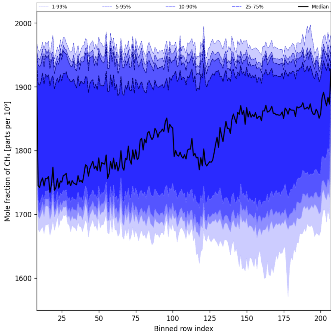
Figure 34: Along track statistics of “Mole fraction of CH 4 ” for 2024-12-24 to 2024-12-26
