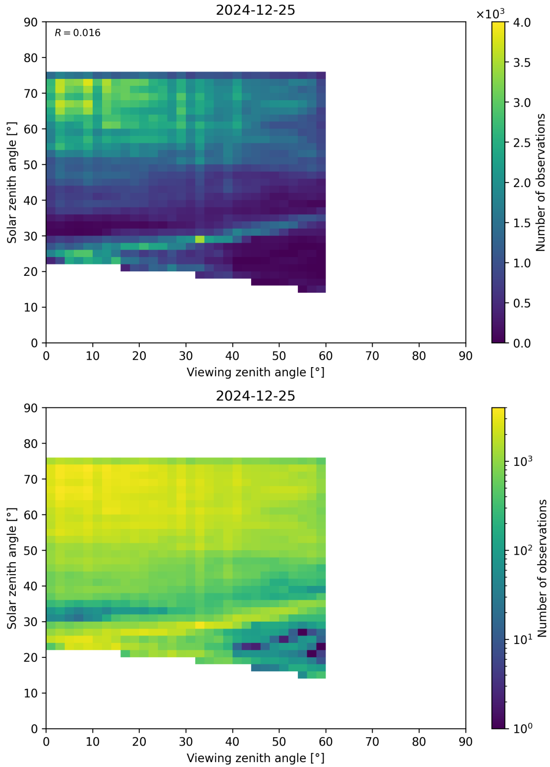
Figure 115: Scatter density plot of “Viewing zenith angle” against “Solar zenith angle” for 2024-12-24 to 2024-12-26.
