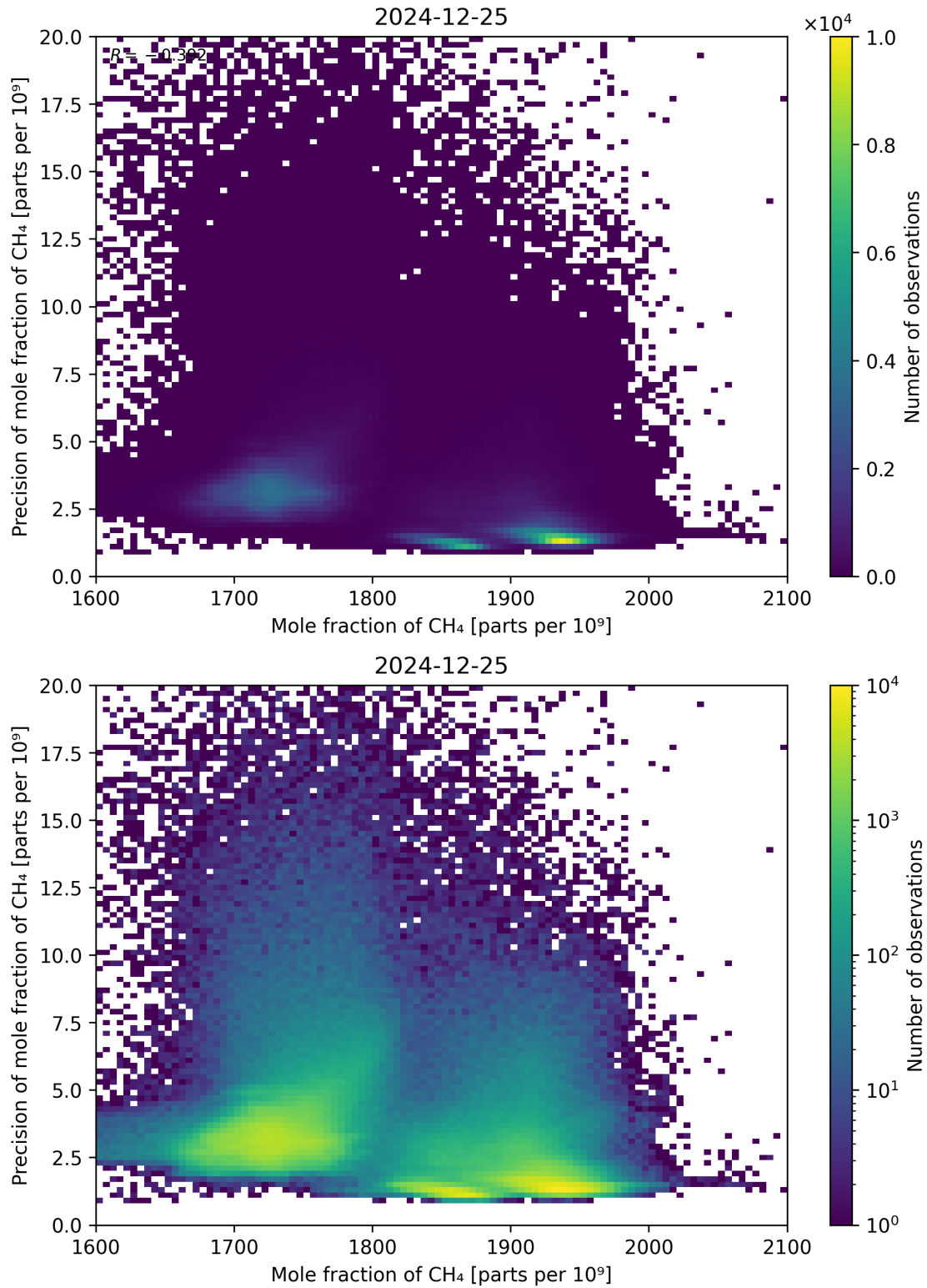
Figure 75: Scatter density plot of “Mole fraction of CH 4 ” against “Precision of mole fraction of CH 4 ” for 2024-12-24 to 2024-12-26.
