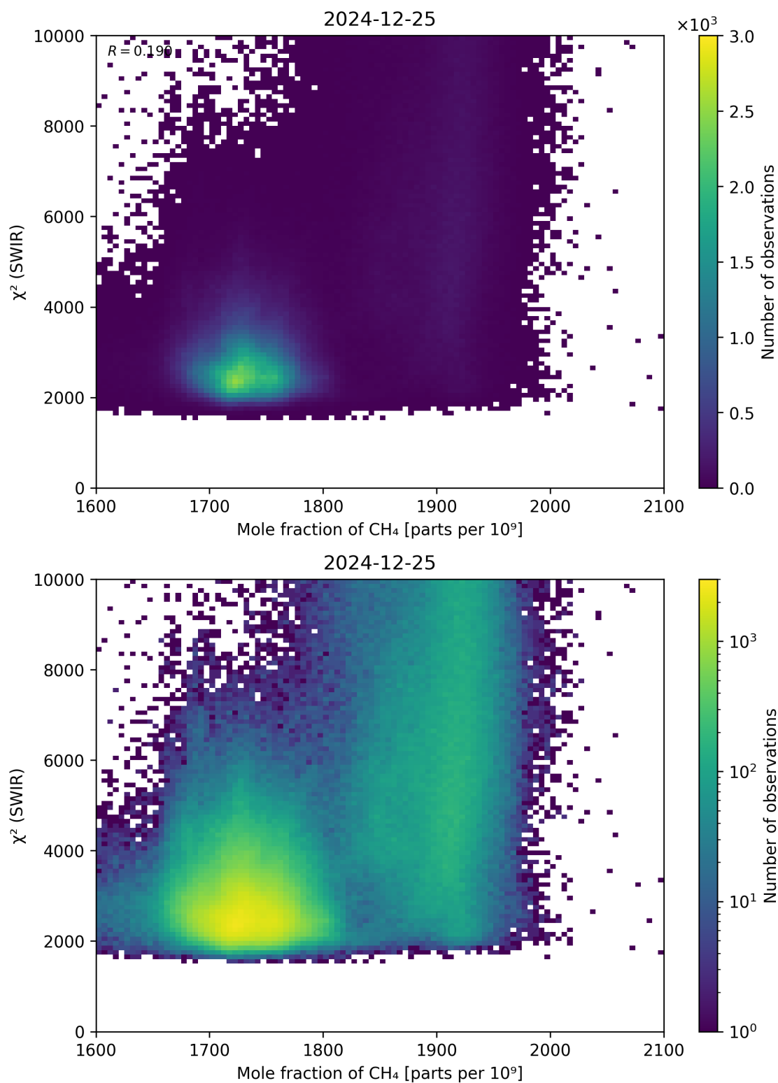
Figure 71: Scatter density plot of “Mole fraction of \text{CH}_4 ” against “ \chi^2 (SWIR)” for 2024-12-24 to 2024-12-26.
