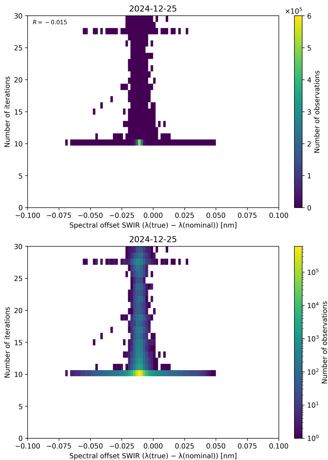
Figure 121: Scatter density plot of “Spectral offset SWIR ( \lambda_{\text{true}} - \lambda_{\text{nominal}} )” against “Number of iterations” for 2024-12-24 to 2024-12-26.
