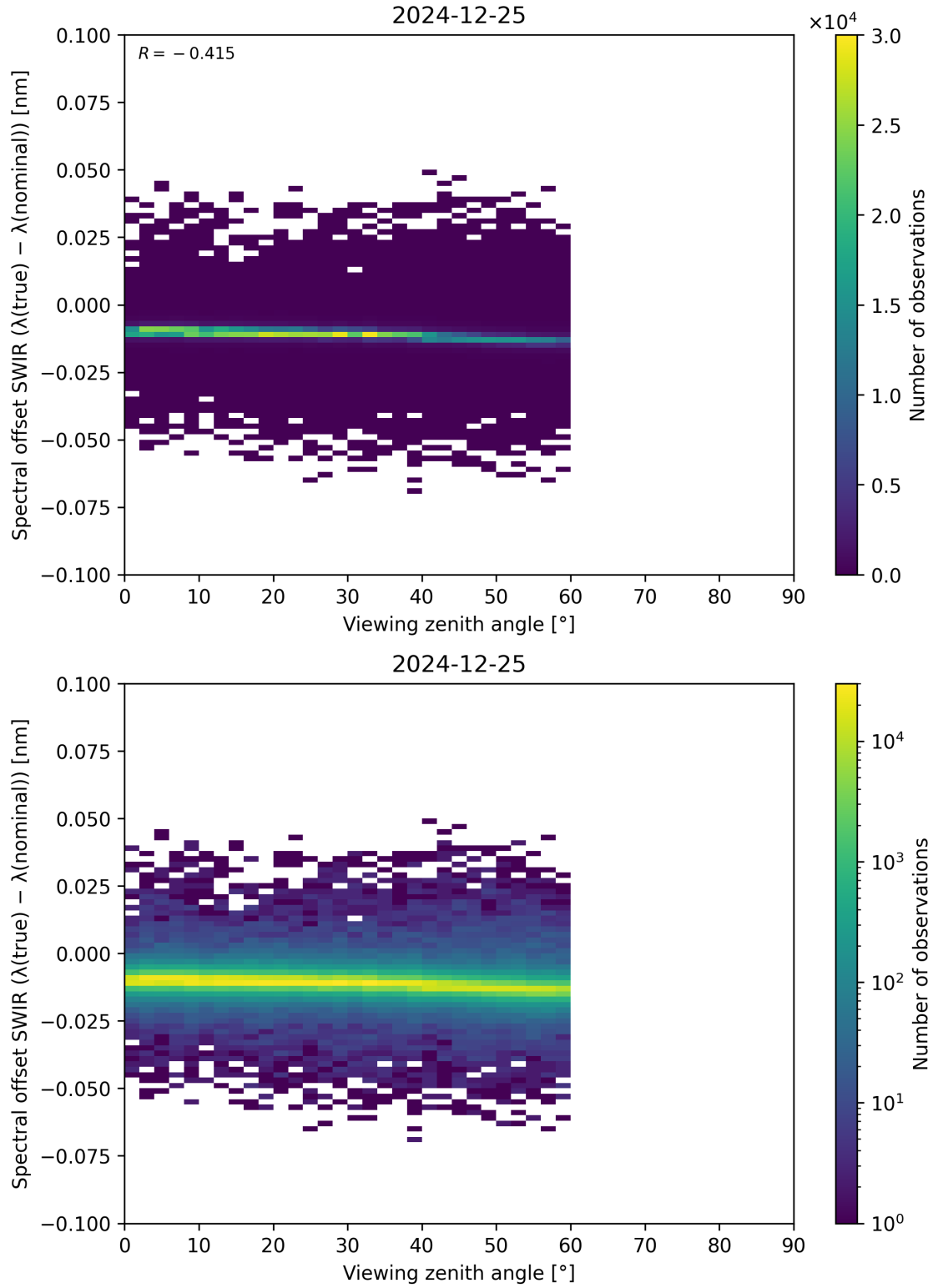
Figure 116: Scatter density plot of “Viewing zenith angle” against “Spectral offset SWIR ( \lambda_{\text{true}} - \lambda_{\text{nominal}} )” for 2024-12-24 to 2024-12-26.
