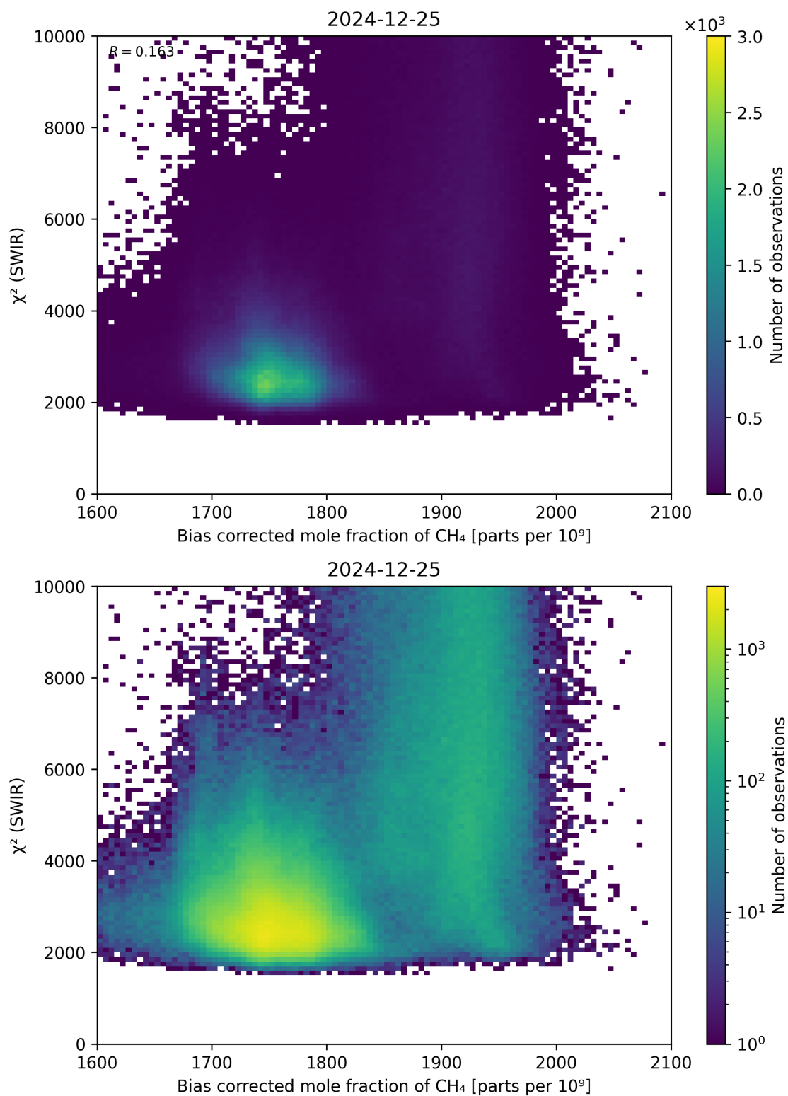
Figure 64: Scatter density plot of “Bias corrected mole fraction of \text{CH}_4 ” against “ \chi^2 (SWIR)” for 2024-12-24 to 2024-12-26.
