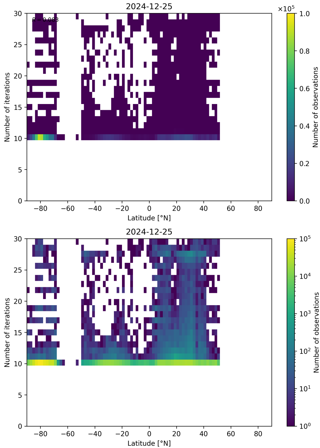
Figure 60: Scatter density plot of “Latitude” against “Number of iterations” for 2024-12-24 to 2024-12-26.
