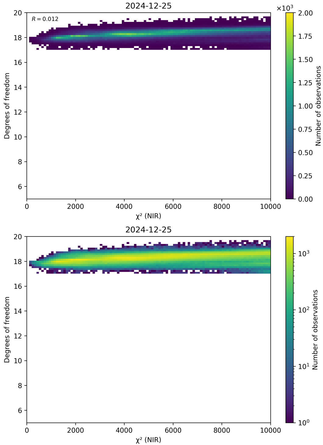
Figure 44: Scatter density plot of “ \chi^2 (NIR)” against “Degrees of freedom” for 2024-12-24 to 2024-12-26.
