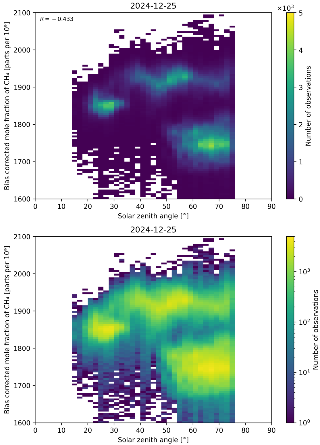
Figure 100: Scatter density plot of “Solar zenith angle” against “Bias corrected mole fraction of CH 4 ” for 2024-12-24 to 2024-12-26.
