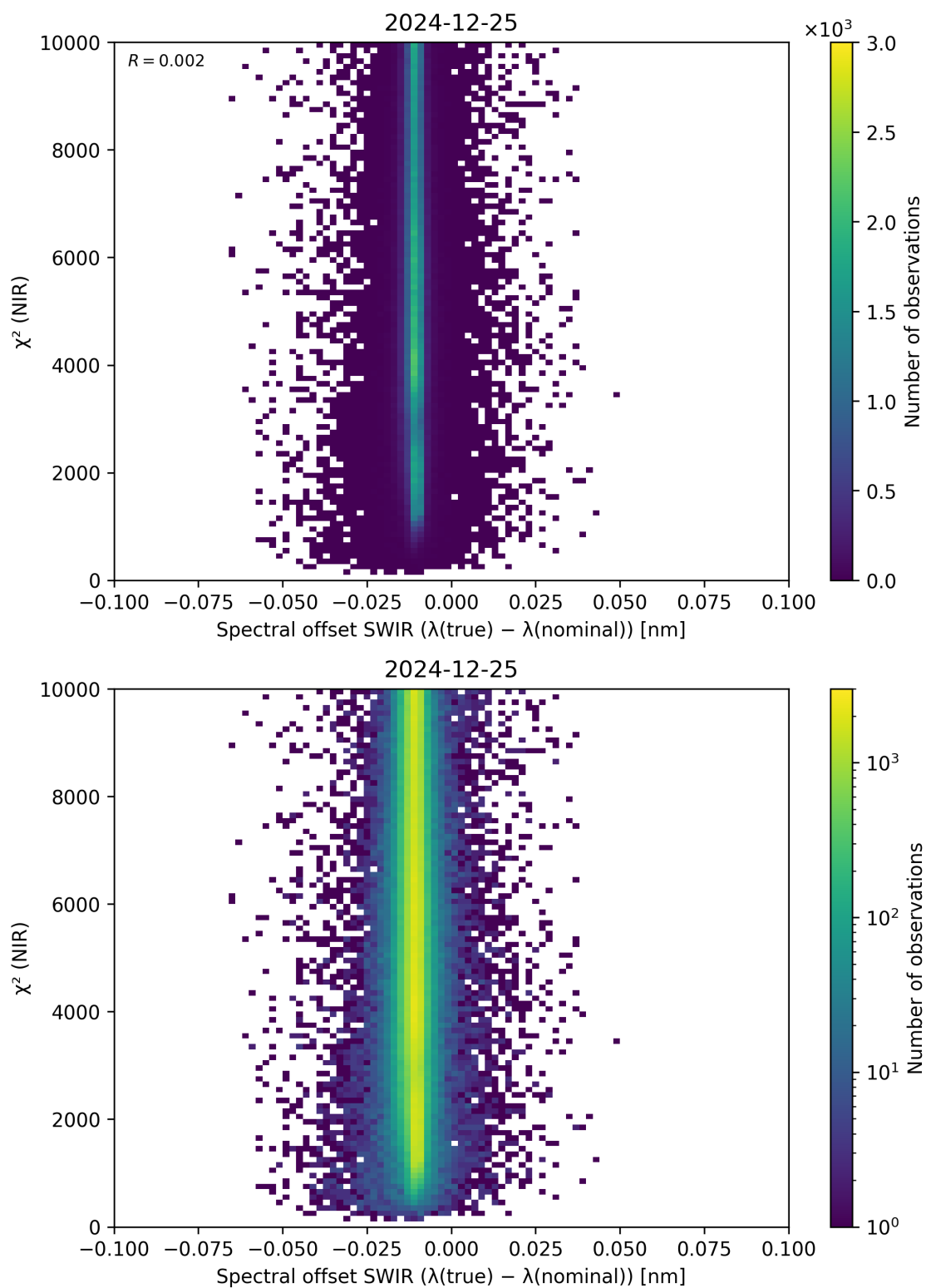
Figure 117: Scatter density plot of “Spectral offset SWIR ( \lambda_{\text{true}} - \lambda_{\text{nominal}} )” against “ \chi^2 (NIR)” for 2024-12-24 to 2024-12-26.
