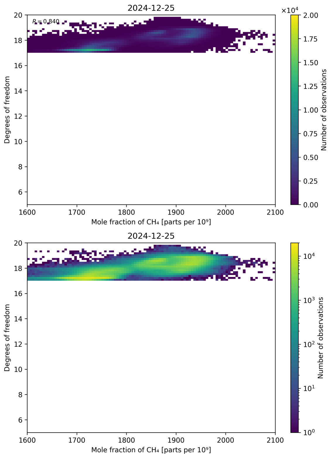
Figure 72: Scatter density plot of “Mole fraction of CH 4 ” against “Degrees of freedom” for 2024-12-24 to 2024-12-26.
