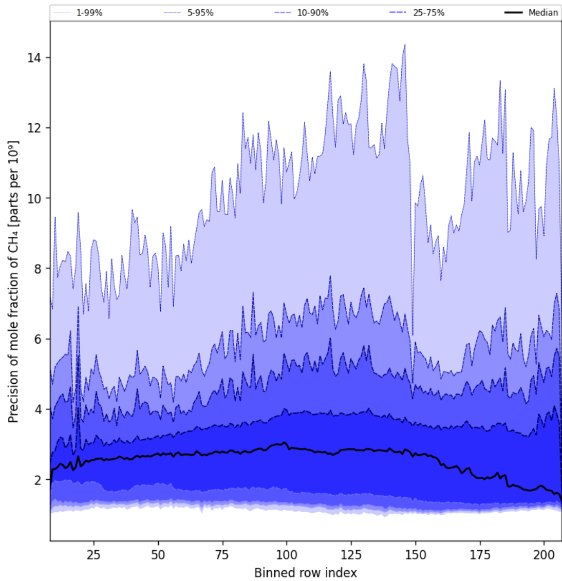
Figure 35: Along track statistics of “Precision of mole fraction of CH 4 ” for 2024-12-24 to 2024-12-26
