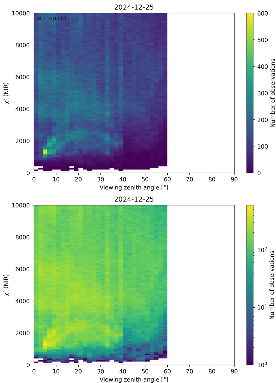
Figure 105: Scatter density plot of “Viewing zenith angle” against “ \chi^2 (NIR)” for 2024-12-24 to 2024-12-26.
