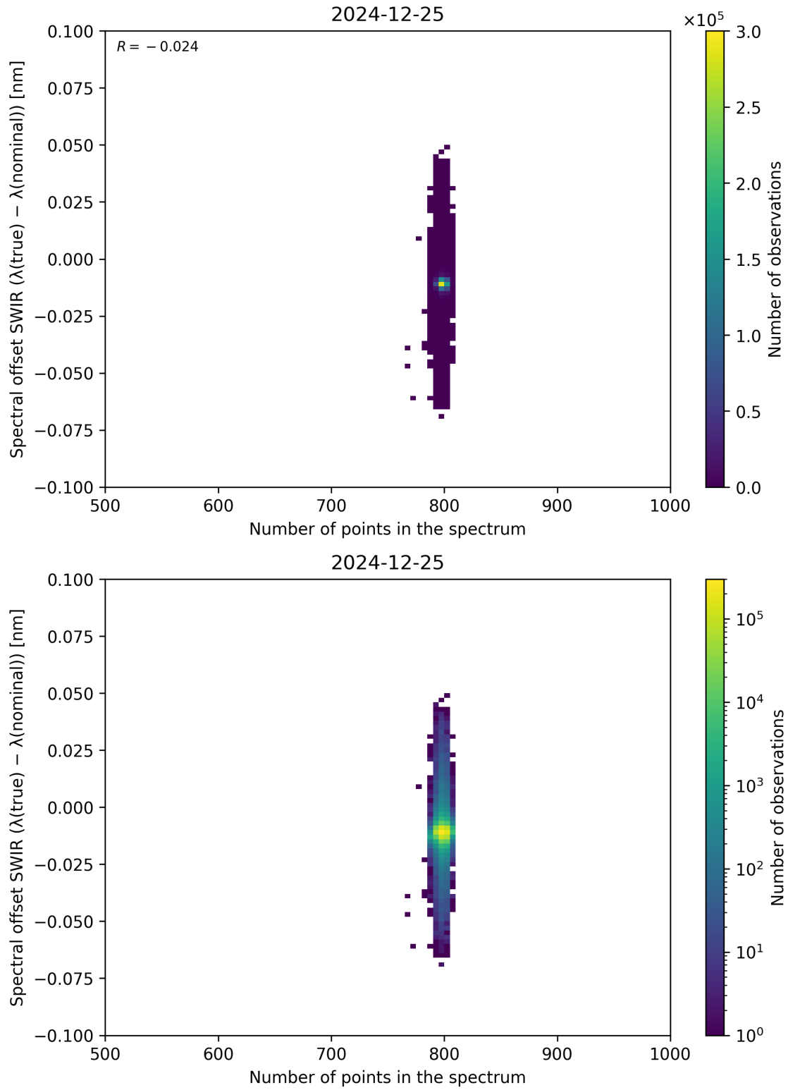
Figure 93: Scatter density plot of “Number of points in the spectrum” against “Spectral offset SWIR ( \lambda_{\text{true}} - \lambda_{\text{nominal}} )” for 2024-12-24 to 2024-12-26.
