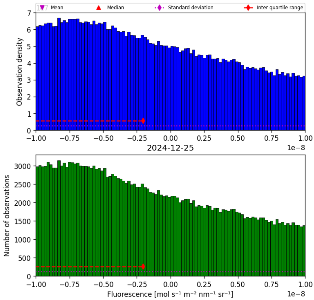
Figure 32: Histogram of “Fluorescence” for 2024-12-24 to 2024-12-26
