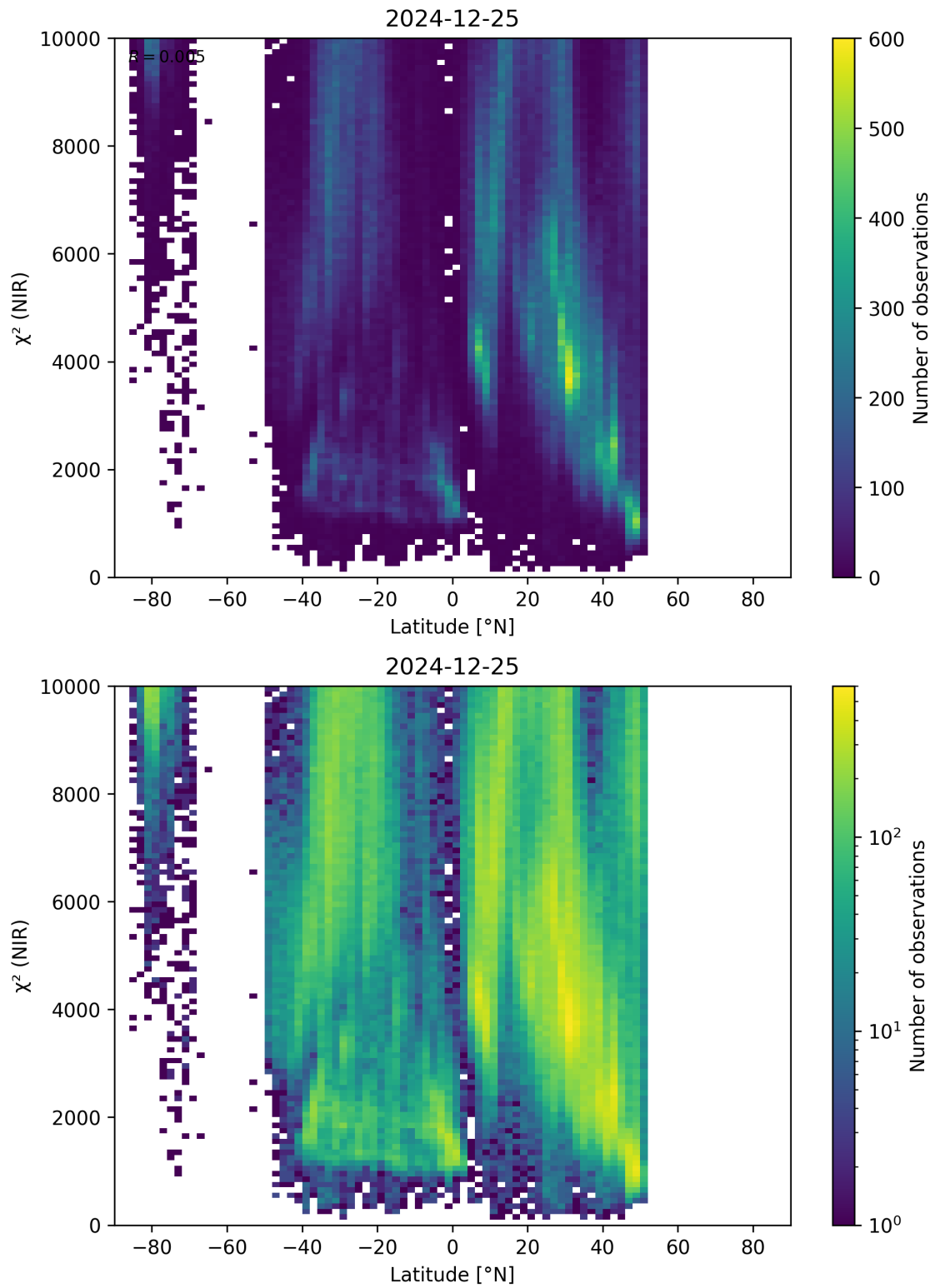
Figure 53: Scatter density plot of “Latitude” against “ \chi^2 (NIR)” for 2024-12-24 to 2024-12-26.
