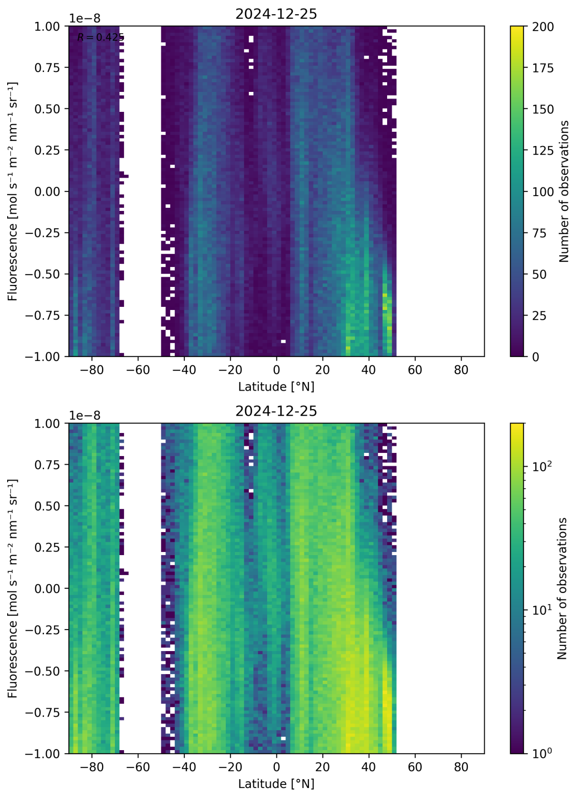
Figure 56: Scatter density plot of “Latitude” against “Fluorescence” for 2024-12-24 to 2024-12-26.
