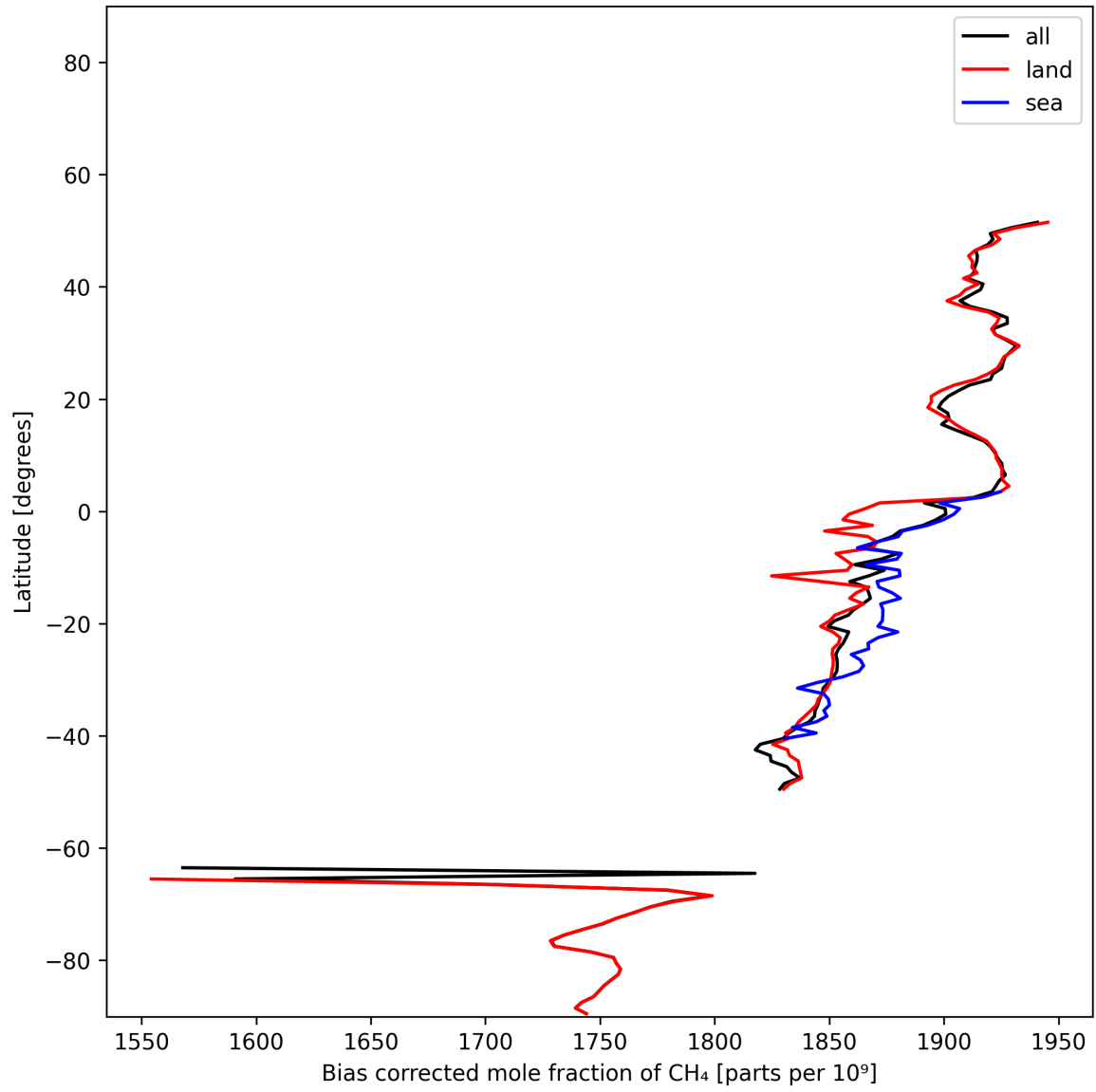
Figure 14: Zonal average of “Bias corrected mole fraction of CH 4 ” for 2024-12-24 to 2024-12-26.
