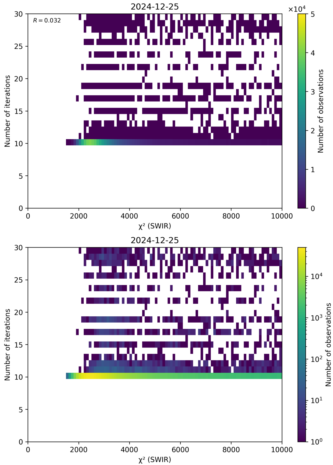
Figure 50: Scatter density plot of “ \chi^2 (SWIR)” against “Number of iterations” for 2024-12-24 to 2024-12-26.
