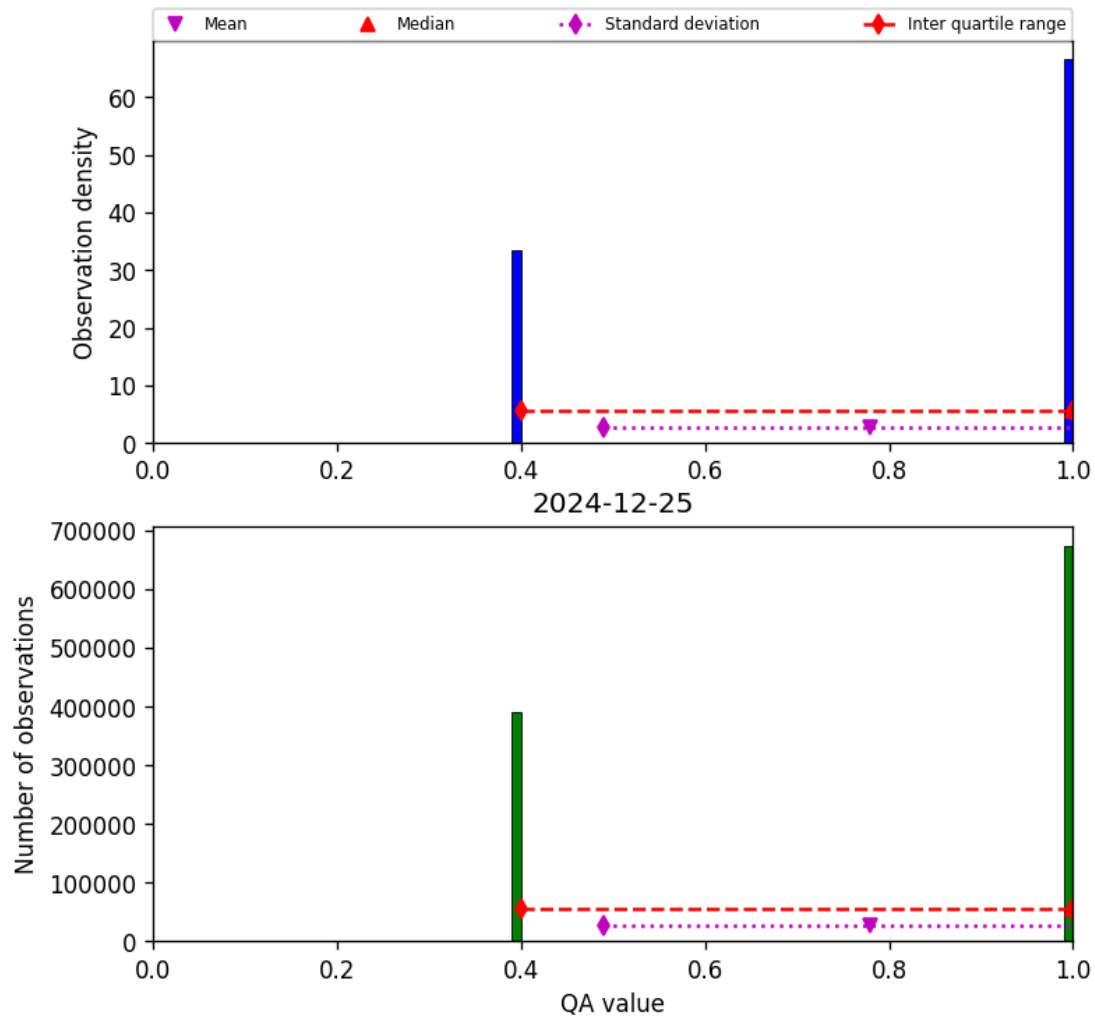
Figure 22: Histogram of “QA value” for 2024-12-24 to 2024-12-26
