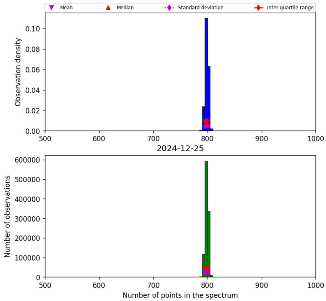
Figure 26: Histogram of “Number of points in the spectrum” for 2024-12-24 to 2024-12-26
