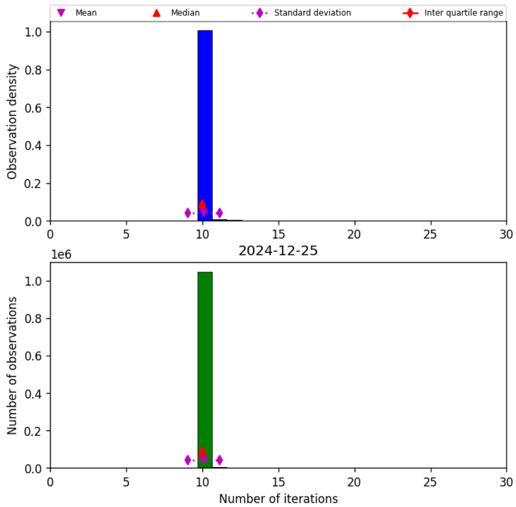
Figure 31: Histogram of “Number of iterations” for 2024-12-24 to 2024-12-26
