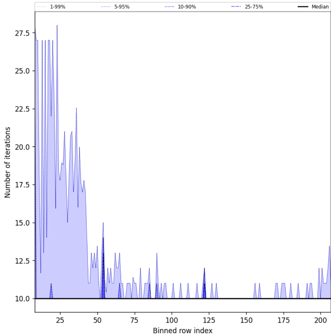
Figure 42: Along track statistics of “Number of iterations” for 2024-12-24 to 2024-12-26
