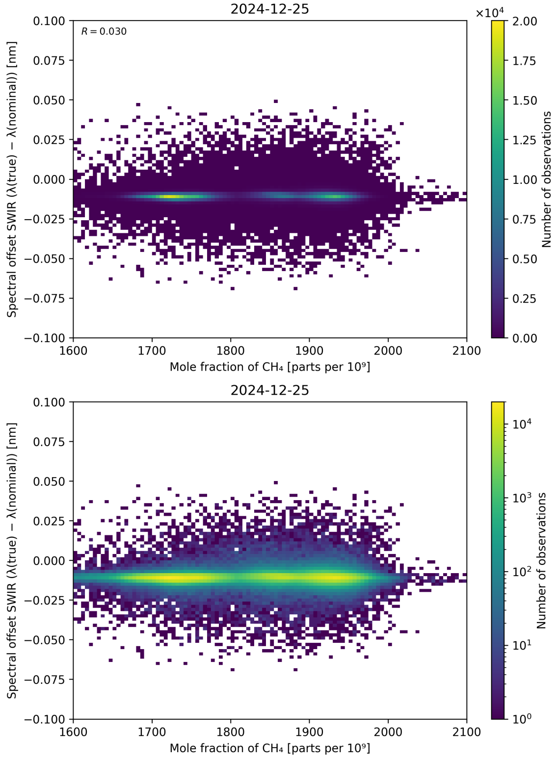
Figure 86: Scatter density plot of “Mole fraction of \text{CH}_4 ” against “Spectral offset SWIR ( \lambda_{\text{true}} - \lambda_{\text{nominal}} )” for 2024-12-24 to 2024-12-26.
