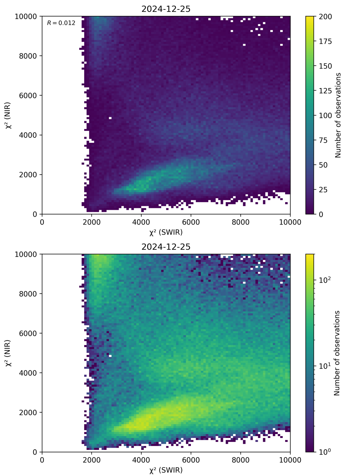
Figure 47: Scatter density plot of “ \chi^2 (SWIR)” against “ \chi^2 (NIR)” for 2024-12-24 to 2024-12-26.
