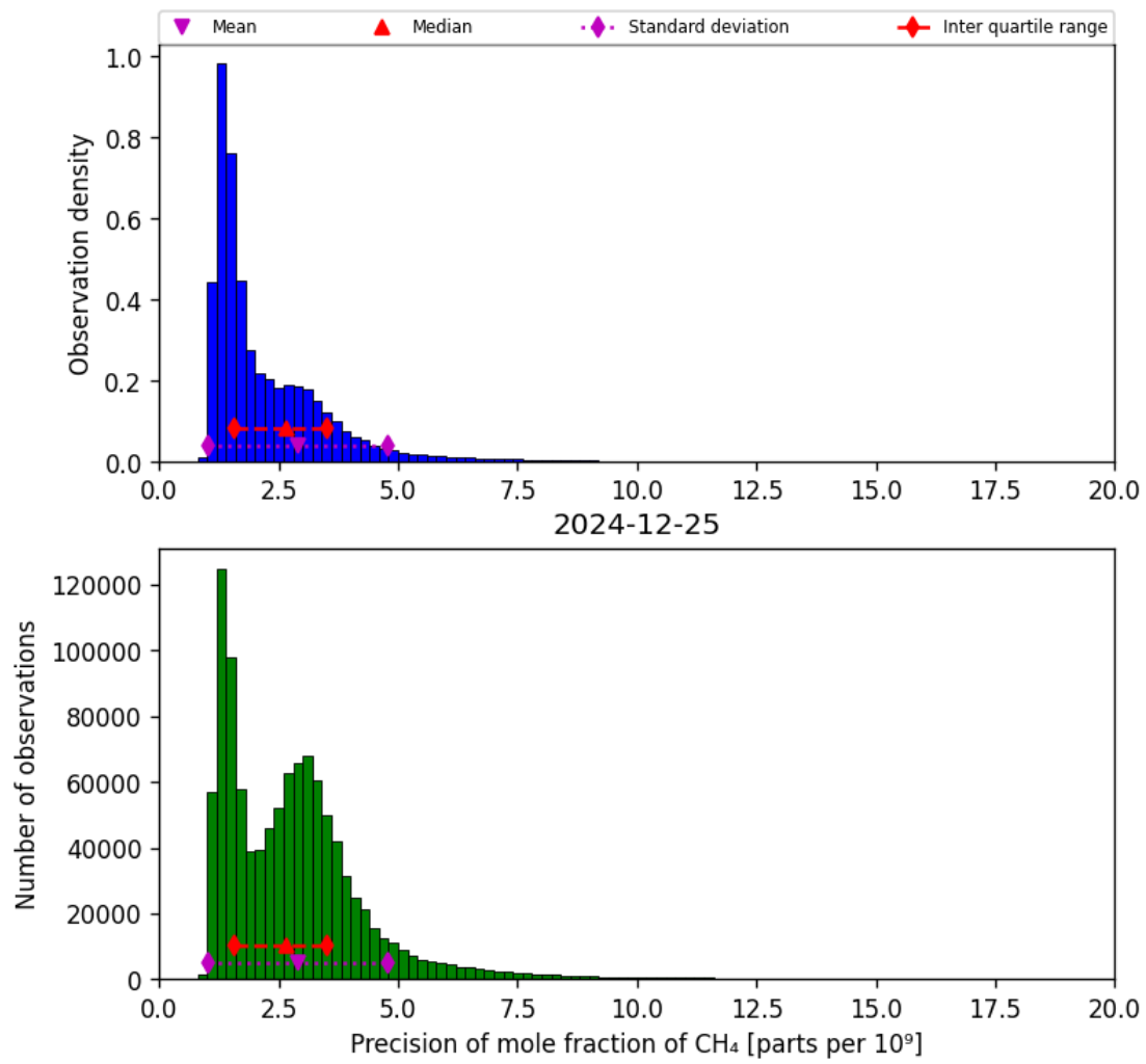
Figure 24: Histogram of “Precision of mole fraction of CH 4 ” for 2024-12-24 to 2024-12-26
