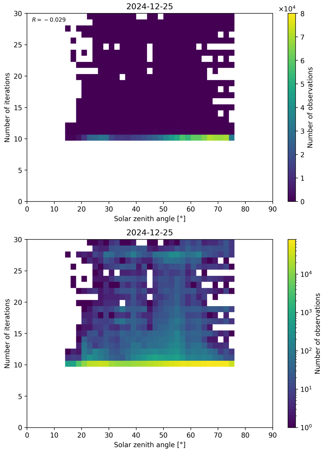
Figure 102: Scatter density plot of “Solar zenith angle” against “Number of iterations” for 2024-12-24 to 2024-12-26.
