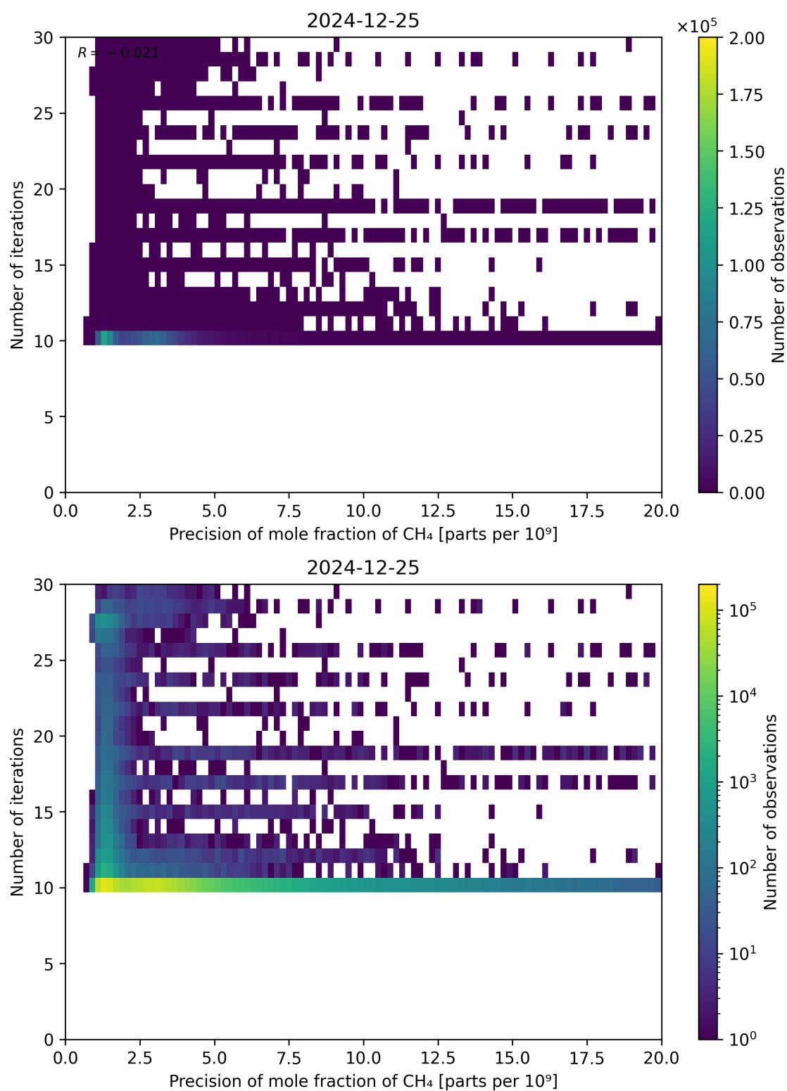
Figure 83: Scatter density plot of “Precision of mole fraction of CH 4 ” against “Number of iterations” for 2024-12-24 to 2024-12-26.
