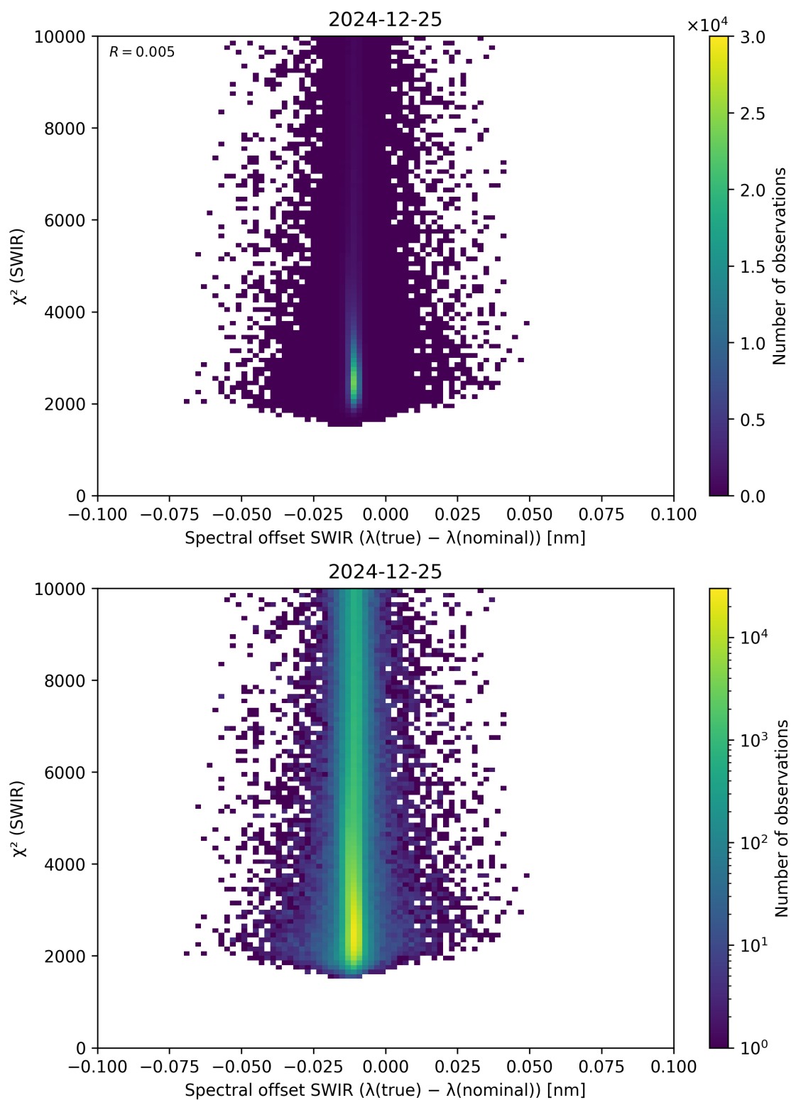
Figure 118: Scatter density plot of “Spectral offset SWIR ( \lambda_{\text{true}} - \lambda_{\text{nominal}} )” against “ \chi^2 (SWIR)” for 2024-12-24 to 2024-12-26.
