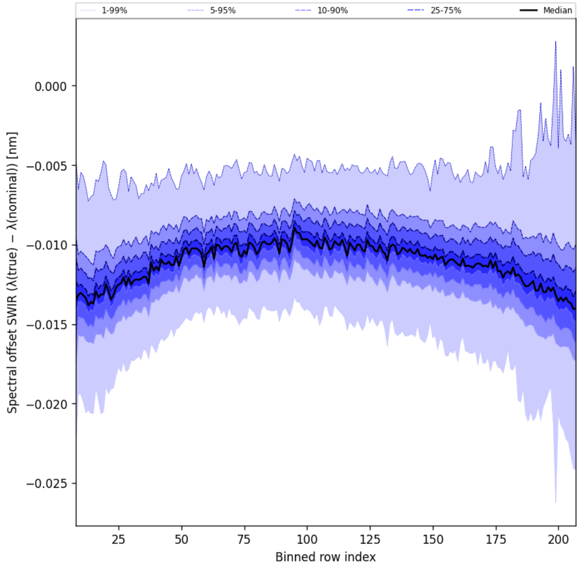
Figure 38: Along track statistics of “Spectral offset SWIR ( \lambda_{\text{true}} - \lambda_{\text{nominal}} )” for 2024-12-24 to 2024-12-26
