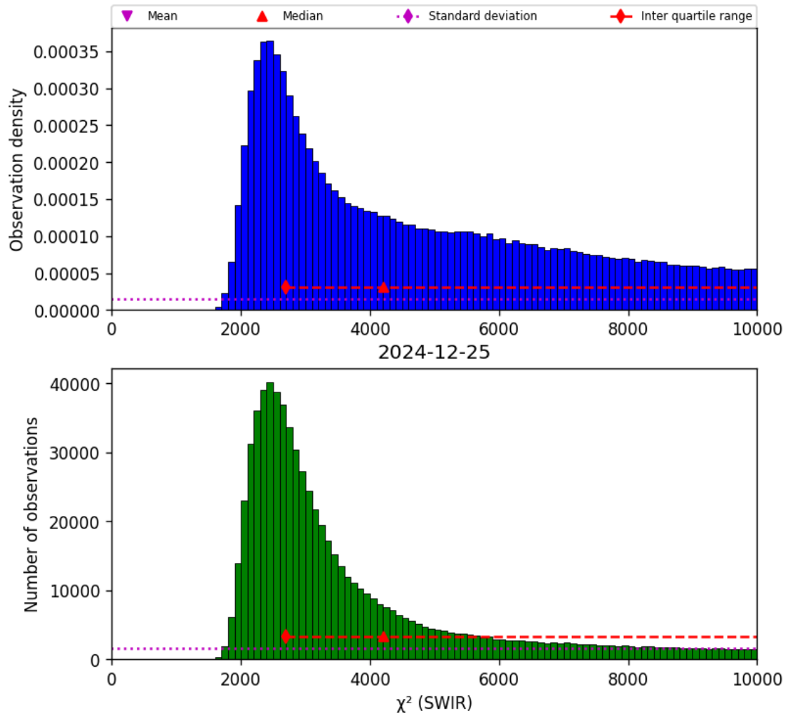
Figure 28: Histogram of “ \chi^2 (SWIR)” for 2024-12-24 to 2024-12-26
