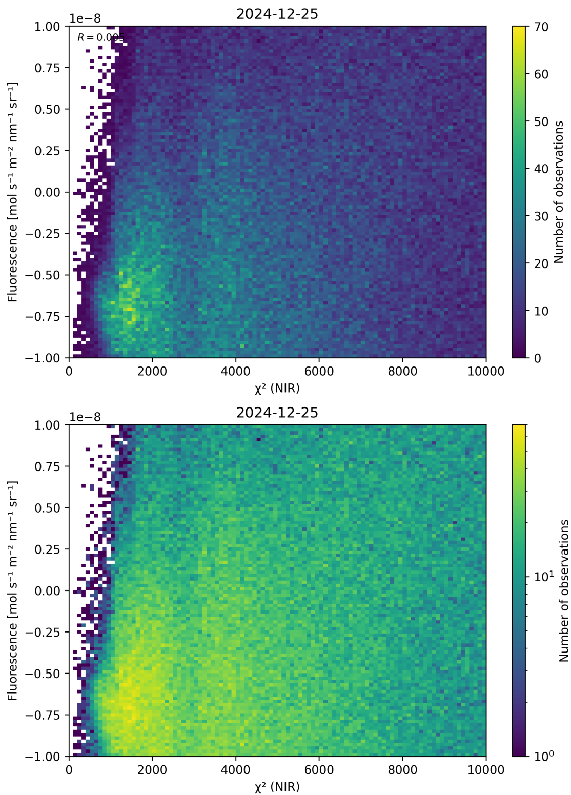
Figure 45: Scatter density plot of “ \chi^2 (NIR)” against “Fluorescence” for 2024-12-24 to 2024-12-26.
