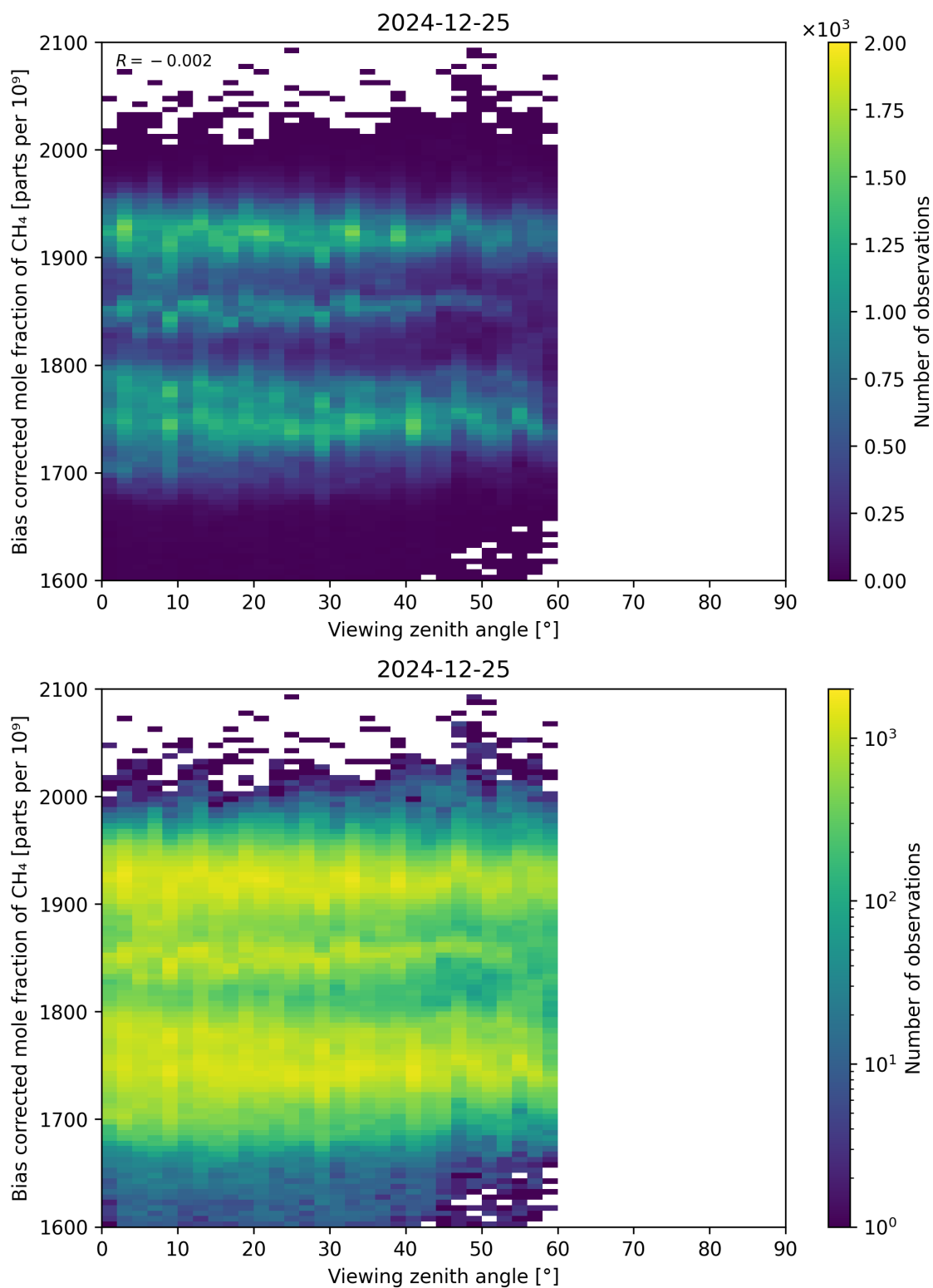
Figure 111: Scatter density plot of “Viewing zenith angle” against “Bias corrected mole fraction of CH 4 ” for 2024-12-24 to 2024-12-26.
