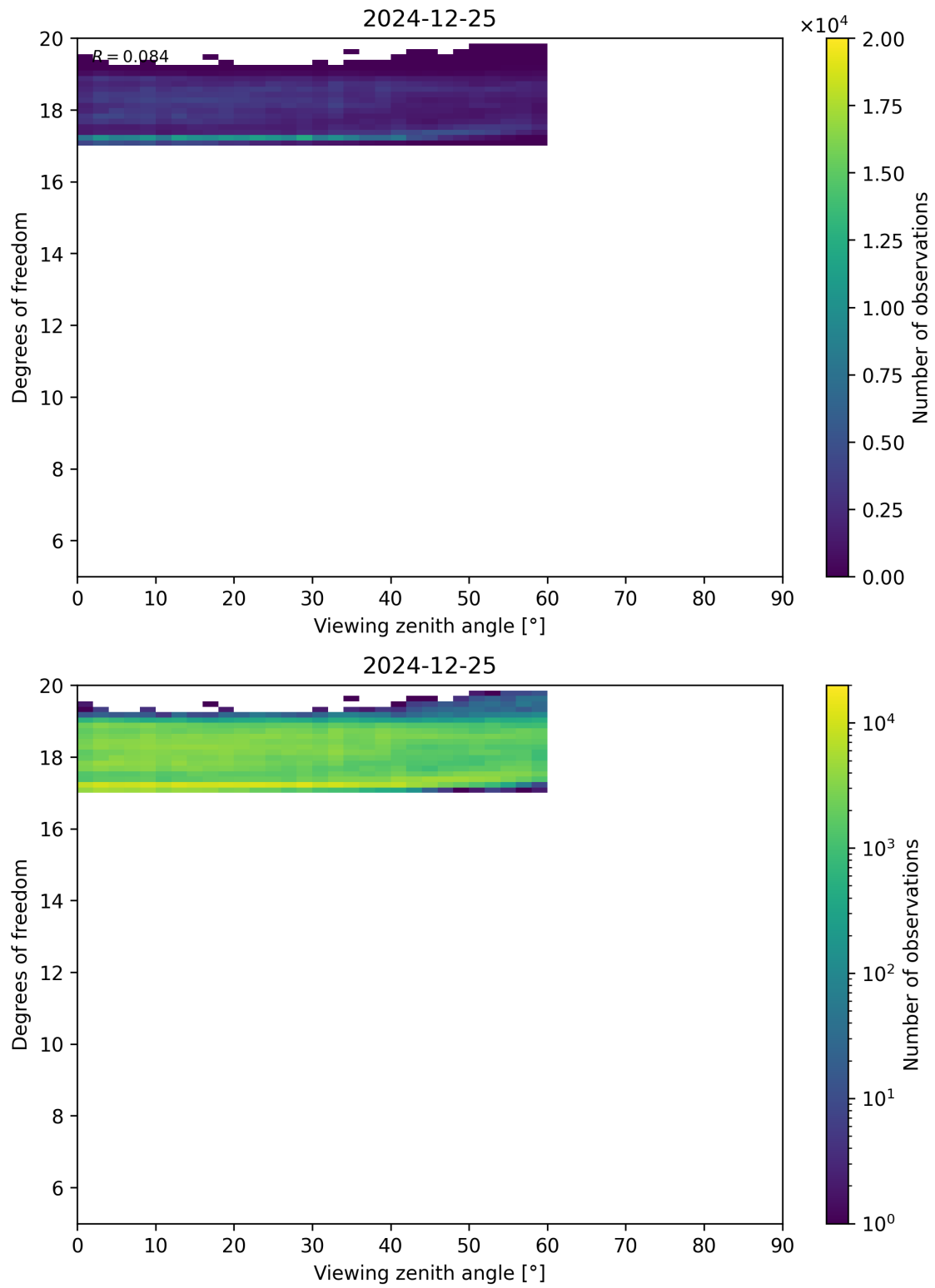
Figure 107: Scatter density plot of “Viewing zenith angle” against “Degrees of freedom” for 2024-12-24 to 2024-12-26.
