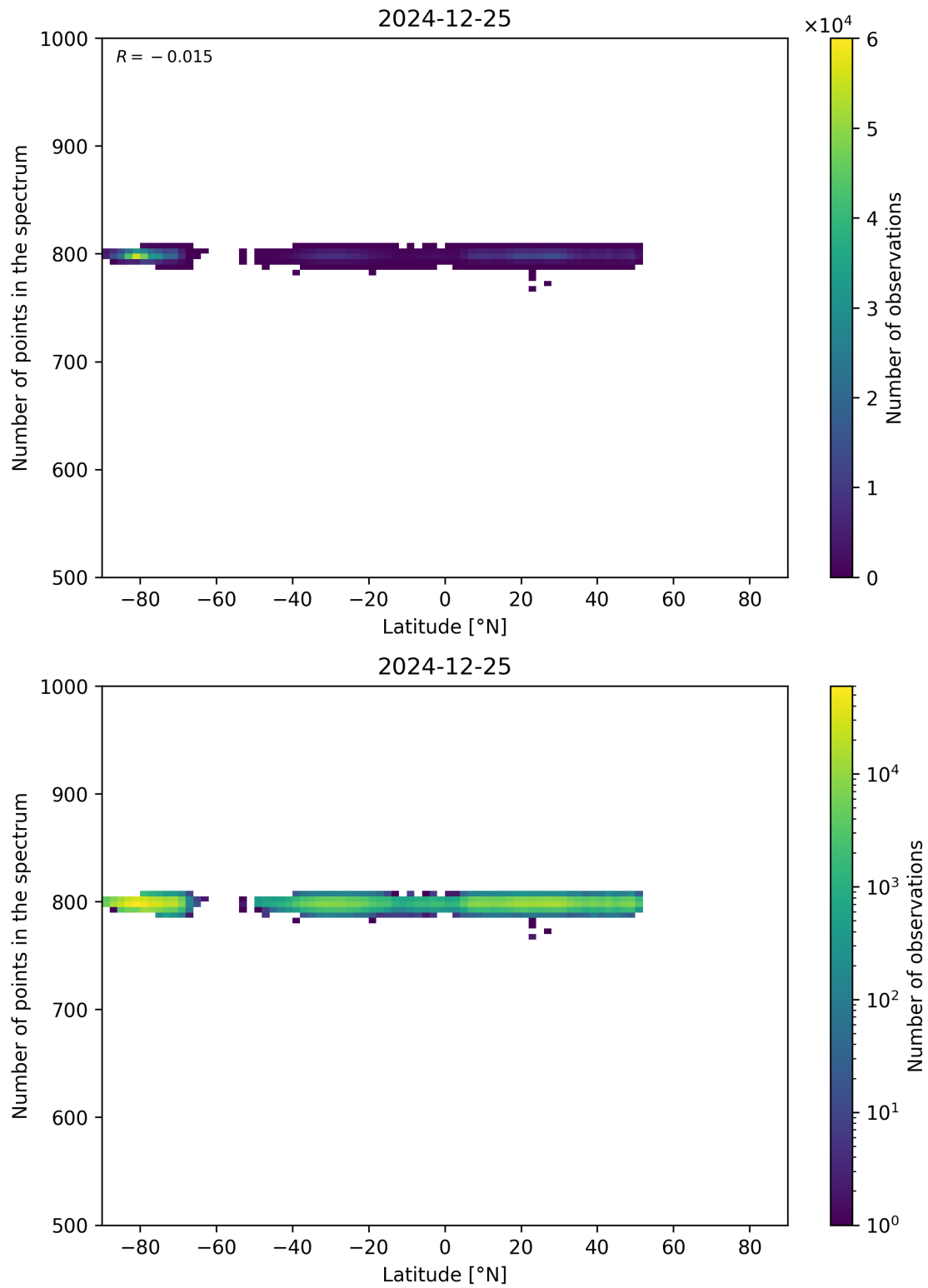
Figure 61: Scatter density plot of “Latitude” against “Number of points in the spectrum” for 2024-12-24 to 2024-12-26.
