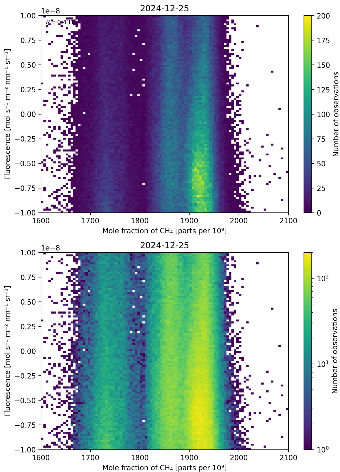
Figure 73: Scatter density plot of “Mole fraction of \text{CH}_4 ” against “Fluorescence” for 2024-12-24 to 2024-12-26.
