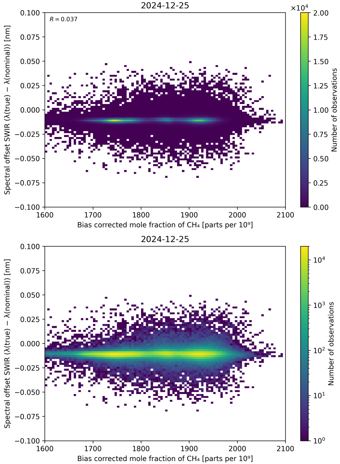
Figure 69: Scatter density plot of “Bias corrected mole fraction of \text{CH}_4 ” against “Spectral offset SWIR ( \lambda_{\text{true}} - \lambda_{\text{nominal}} )” for 2024-12-24 to 2024-12-26.
