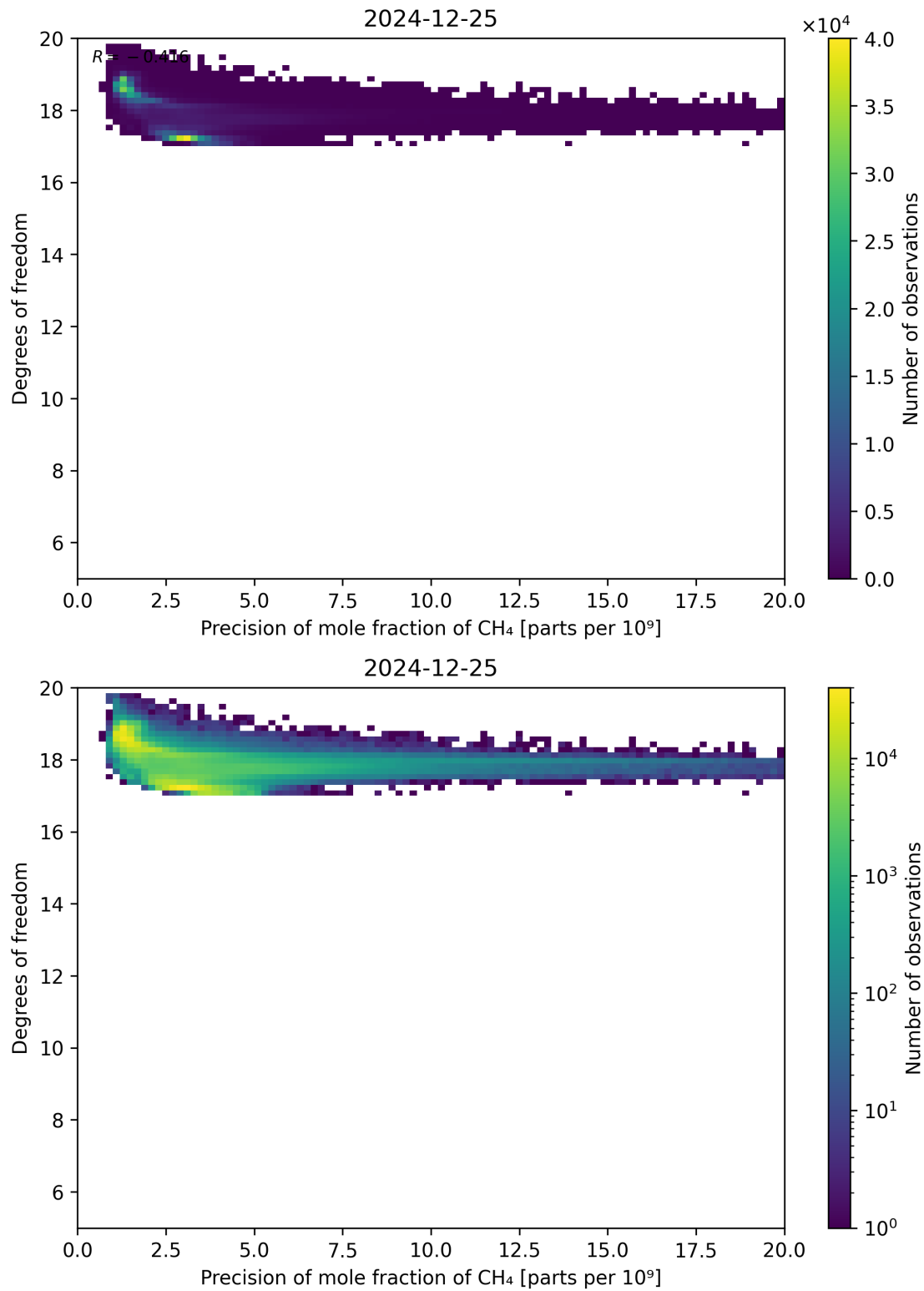
Figure 80: Scatter density plot of “Precision of mole fraction of CH 4 ” against “Degrees of freedom” for 2024-12-24 to 2024-12-26.
