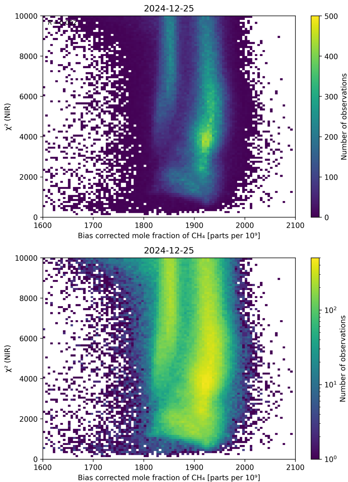
Figure 63: Scatter density plot of “Bias corrected mole fraction of \text{CH}_4 ” against “ \chi^2 (NIR)” for 2024-12-24 to 2024-12-26.
