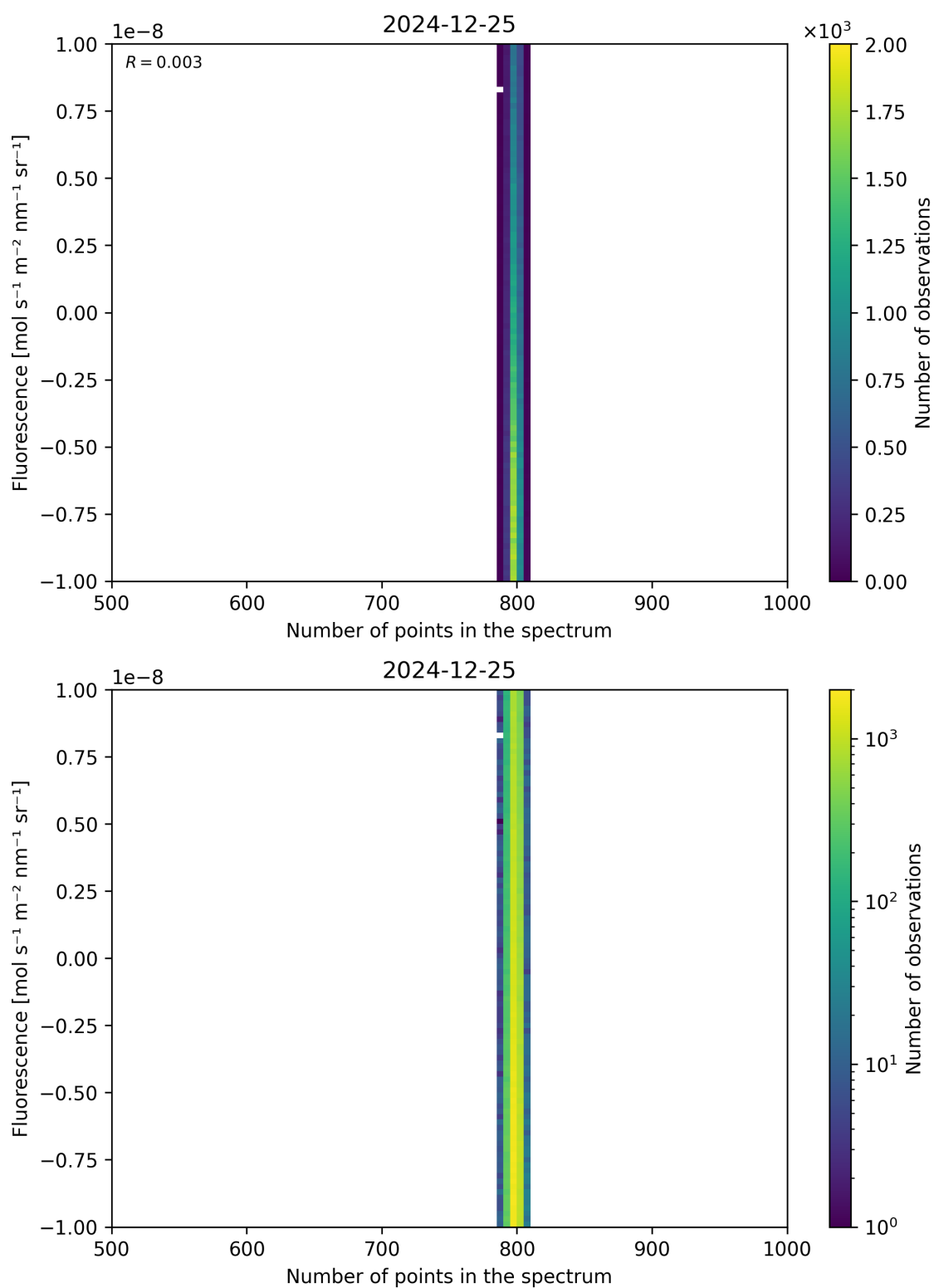
Figure 91: Scatter density plot of “Number of points in the spectrum” against “Fluorescence” for 2024-12-24 to 2024-12-26.
