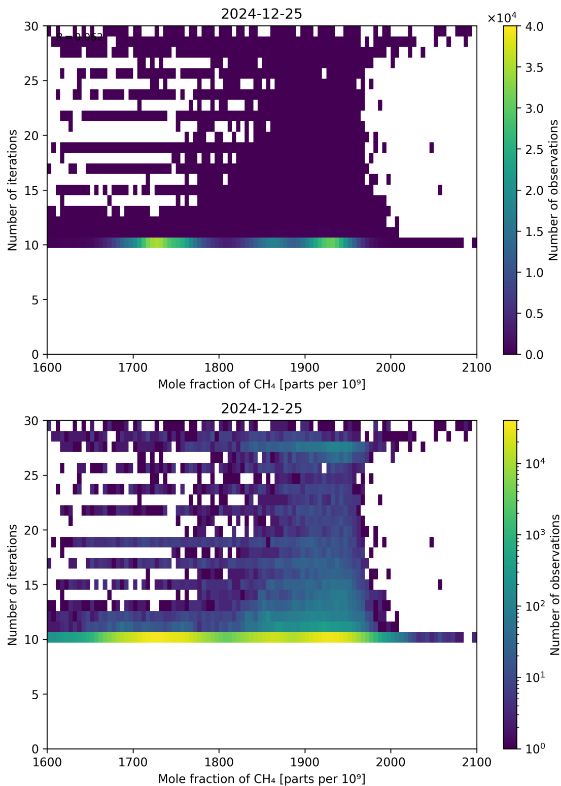
Figure 76: Scatter density plot of “Mole fraction of CH 4 ” against “Number of iterations” for 2024-12-24 to 2024-12-26.
