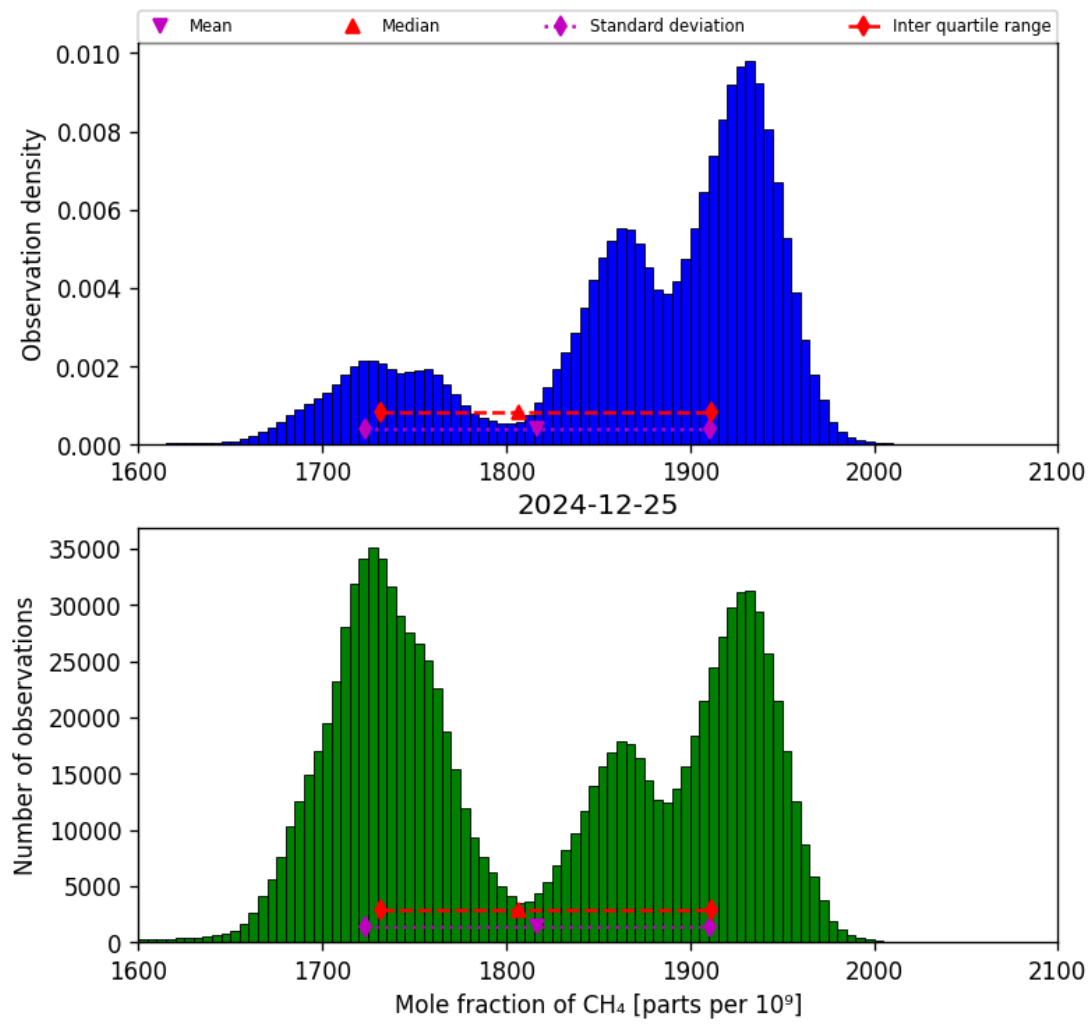
Figure 23: Histogram of “Mole fraction of CH 4 ” for 2024-12-24 to 2024-12-26
