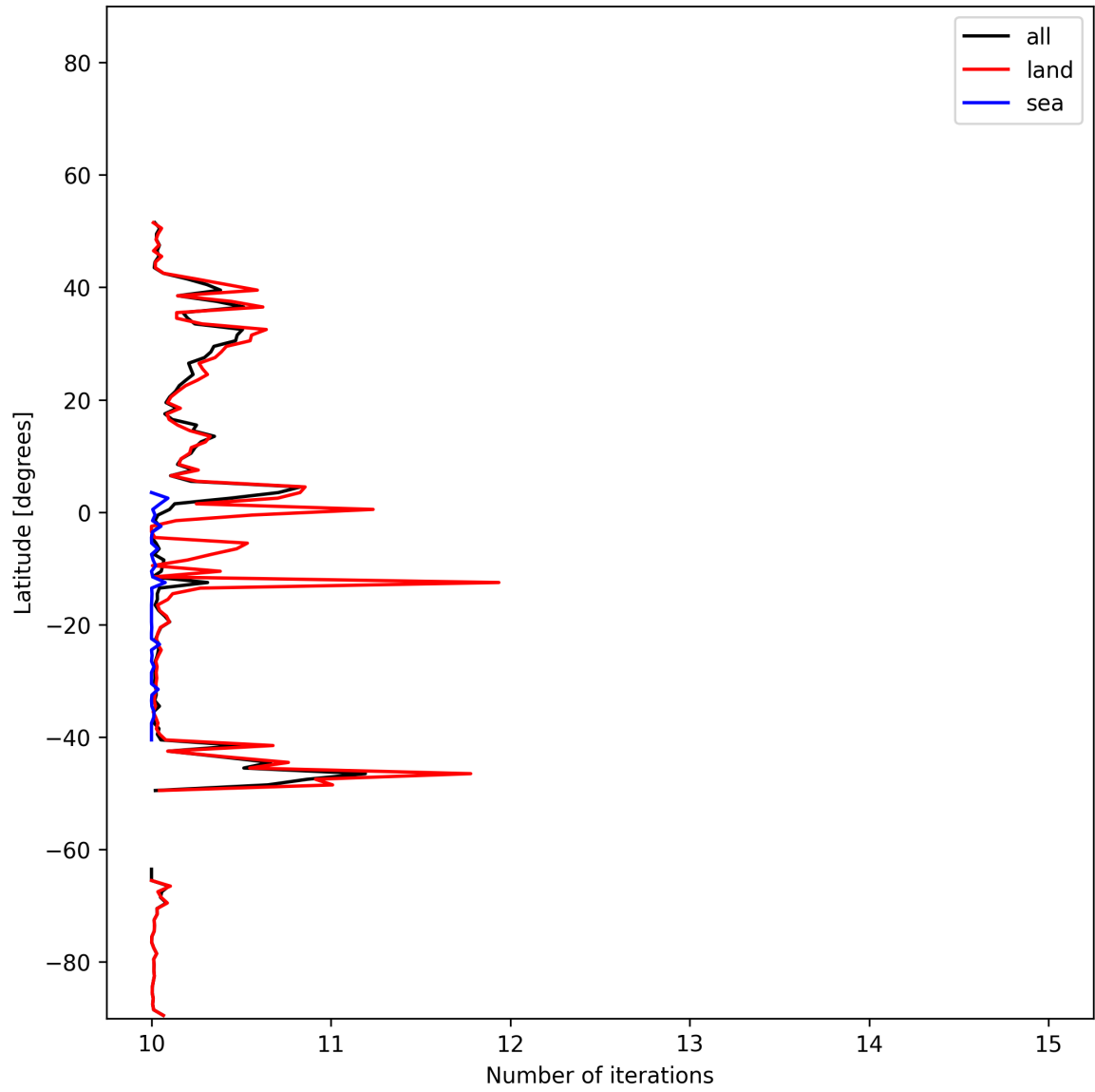
Figure 20: Zonal average of “Number of iterations” for 2024-12-24 to 2024-12-26.
