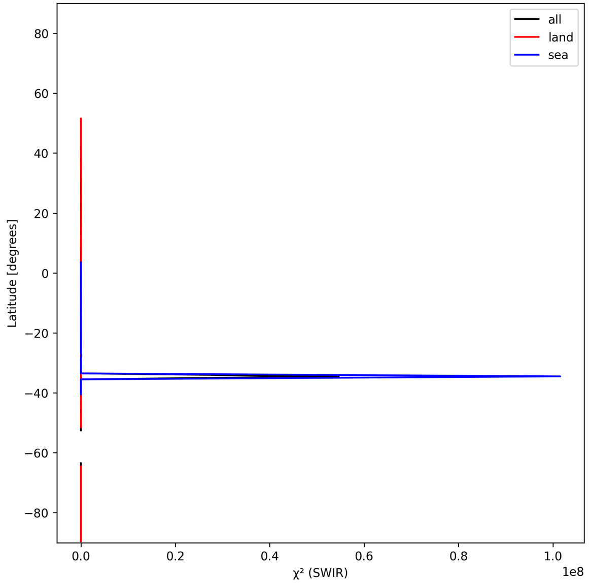
Figure 17: Zonal average of “ \chi^2 (SWIR)” for 2024-12-27 to 2024-12-28.
