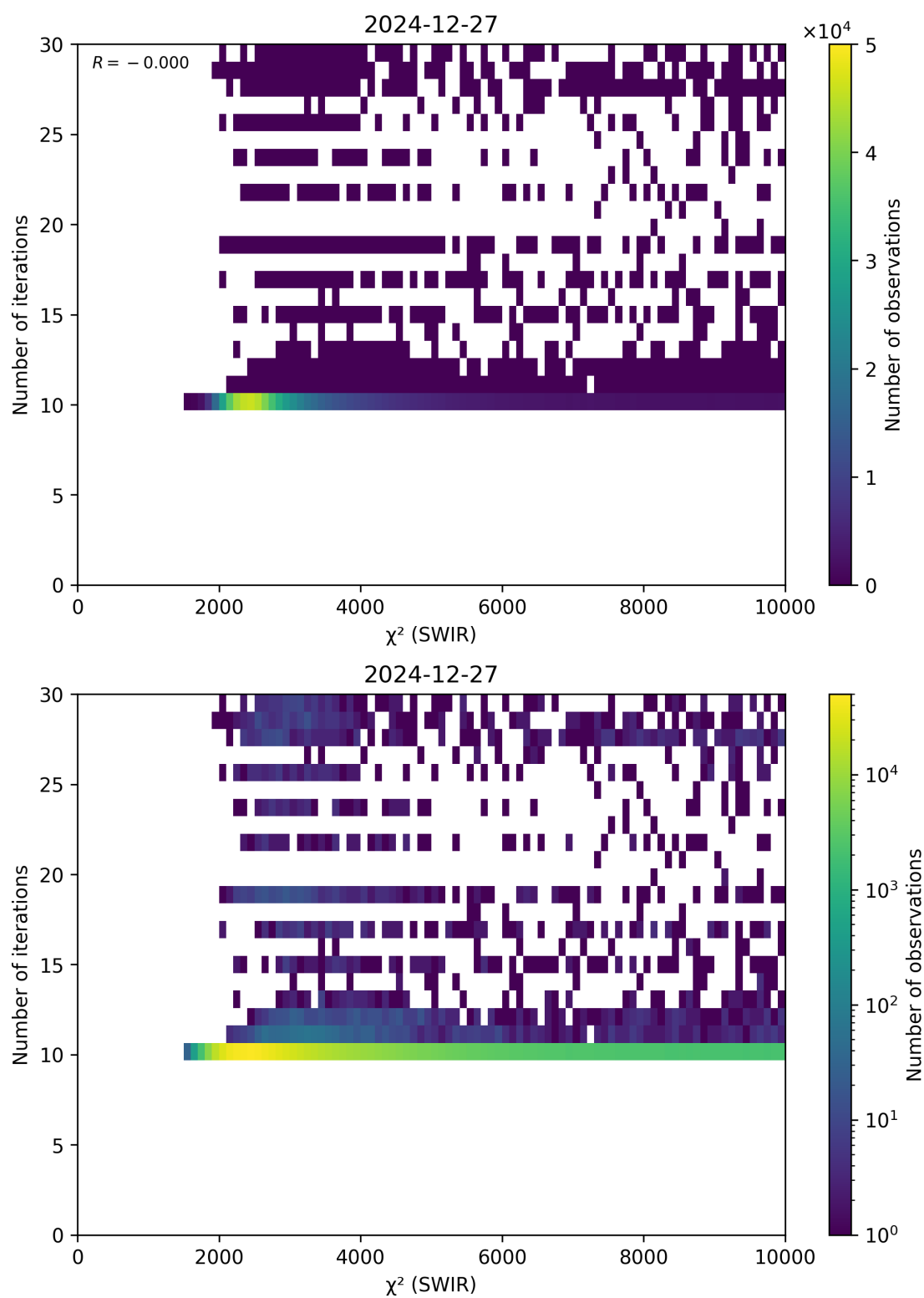
Figure 50: Scatter density plot of “ \chi^2 (SWIR)” against “Number of iterations” for 2024-12-27 to 2024-12-28.
