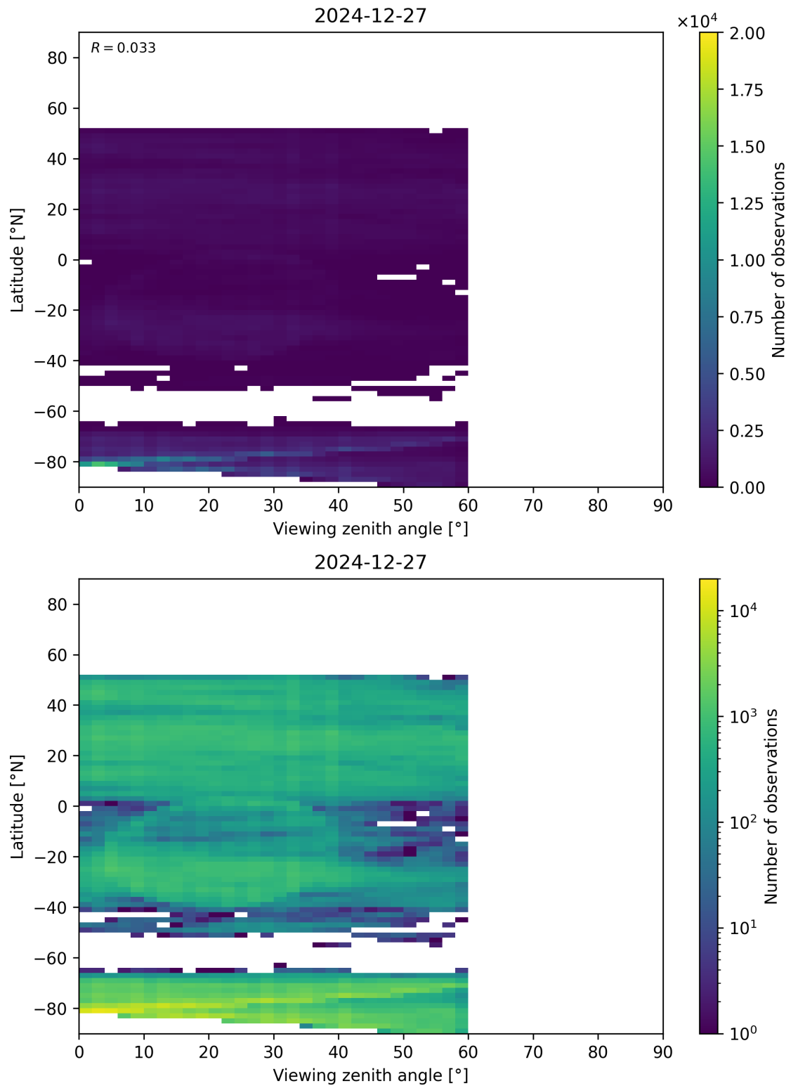
Figure 109: Scatter density plot of “Viewing zenith angle” against “Latitude” for 2024-12-27 to 2024-12-28.
