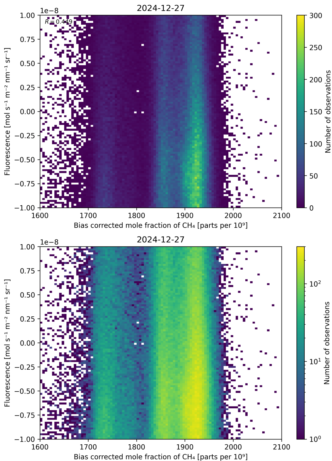
Figure 66: Scatter density plot of “Bias corrected mole fraction of \text{CH}_4 ” against “Fluorescence” for 2024-12-27 to 2024-12-28.
