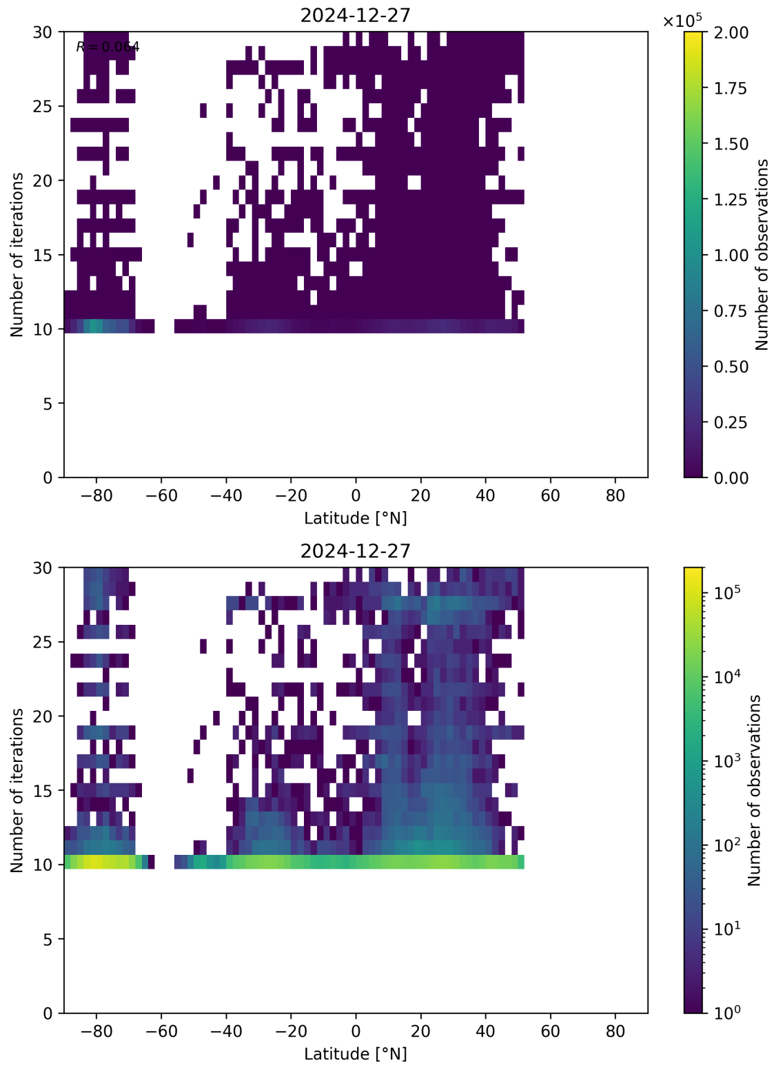
Figure 60: Scatter density plot of “Latitude” against “Number of iterations” for 2024-12-27 to 2024-12-28.
