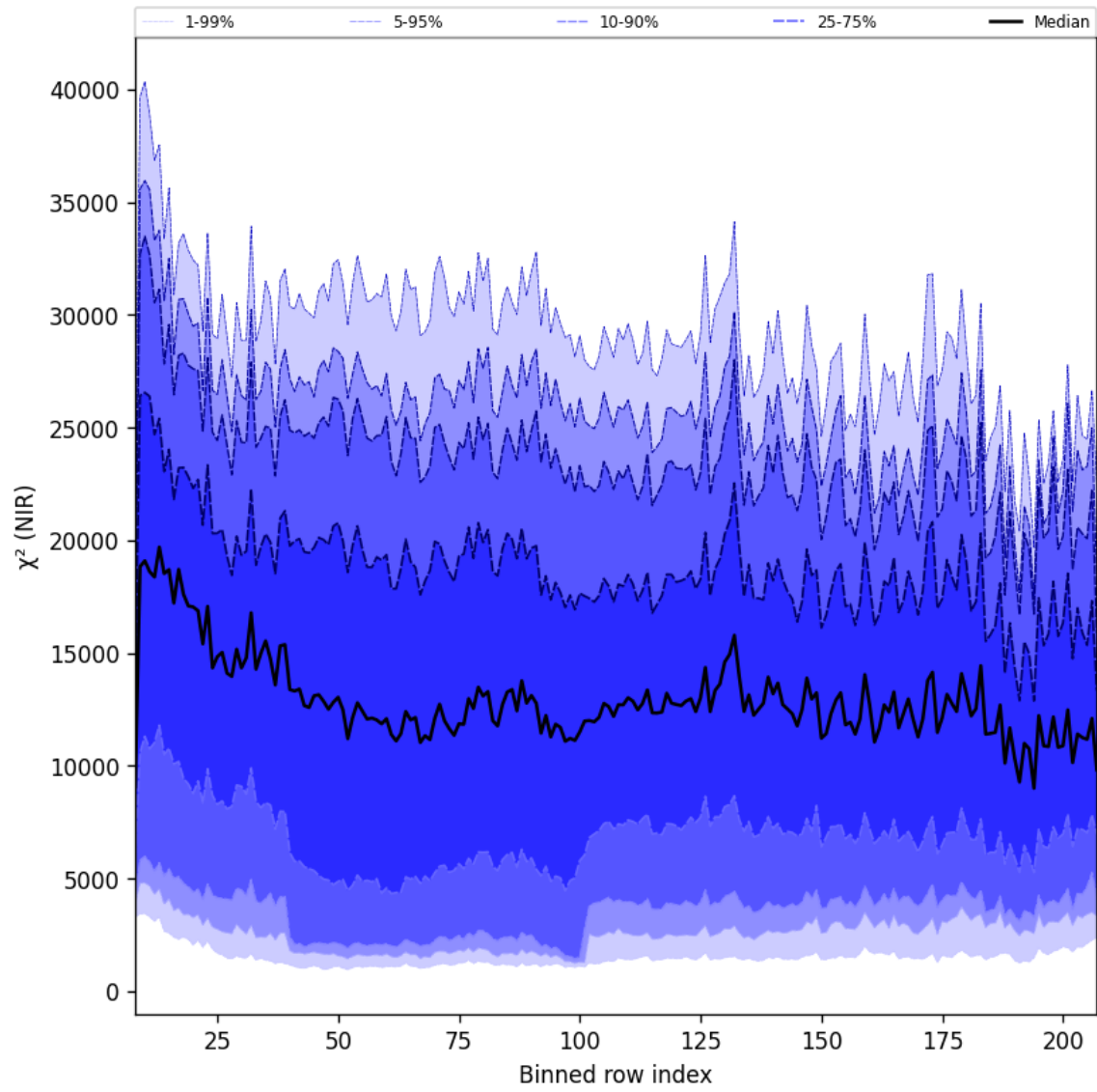
Figure 40: Along track statistics of “ \chi^2 (NIR)” for 2024-12-27 to 2024-12-28
