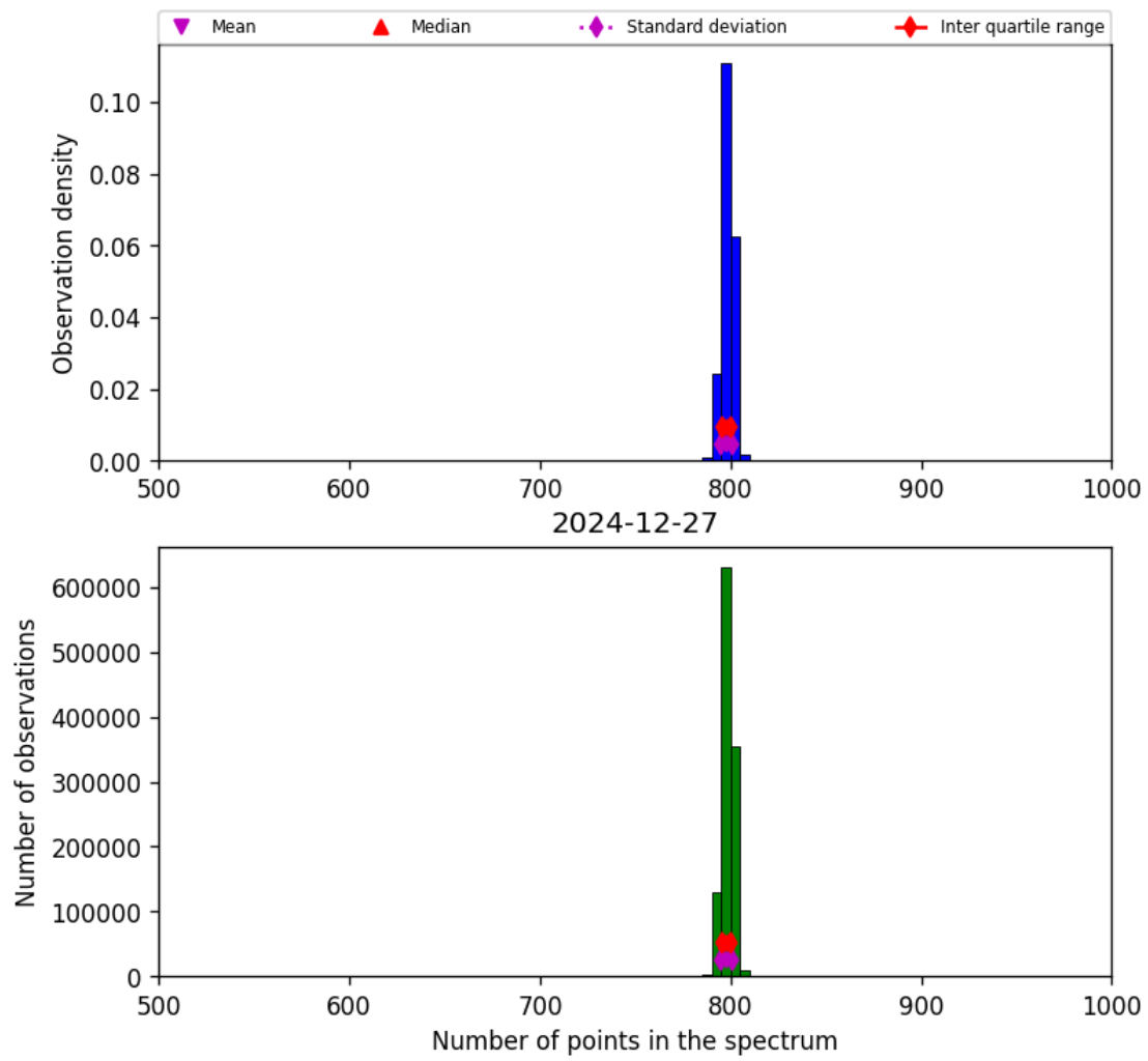
Figure 26: Histogram of “Number of points in the spectrum” for 2024-12-27 to 2024-12-28
