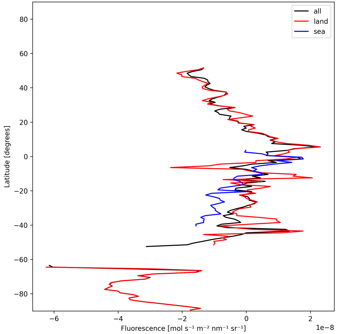
Figure 21: Zonal average of “Fluorescence” for 2024-12-27 to 2024-12-28.
