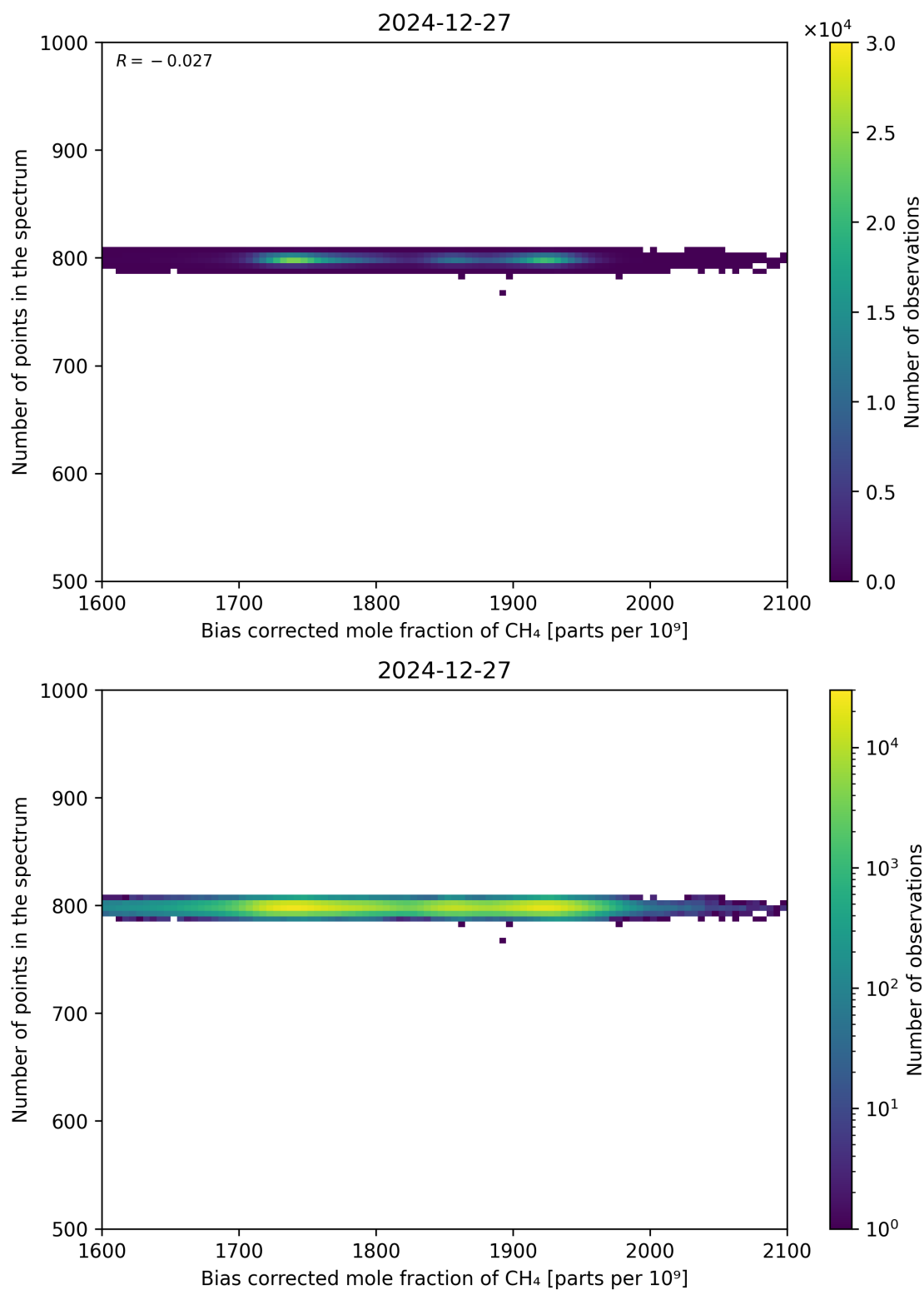
Figure 68: Scatter density plot of “Bias corrected mole fraction of CH 4 ” against “Number of points in the spectrum” for 2024-12-27 to 2024-12-28.
