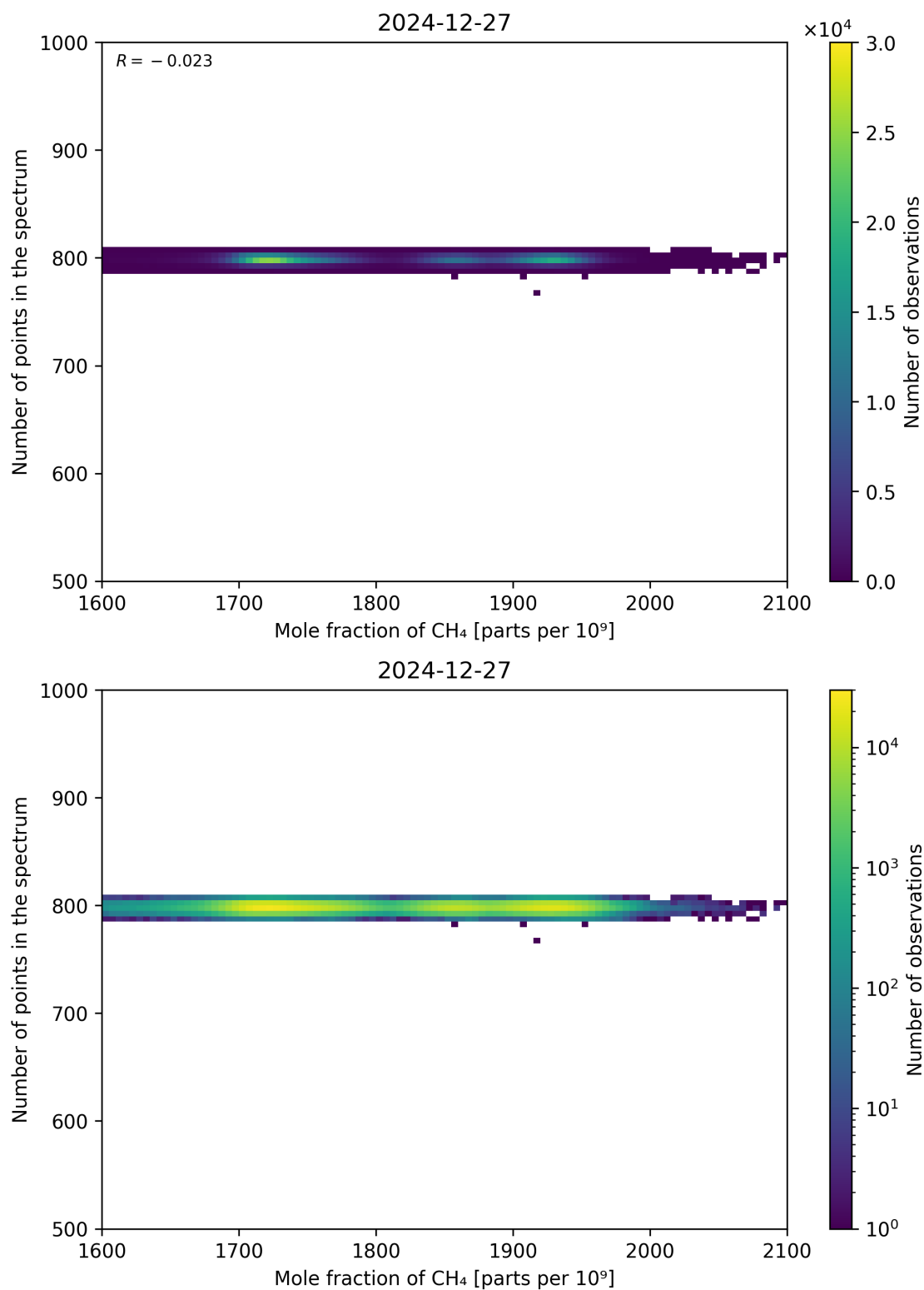
Figure 77: Scatter density plot of “Mole fraction of CH 4 ” against “Number of points in the spectrum” for 2024-12-27 to 2024-12-28.
