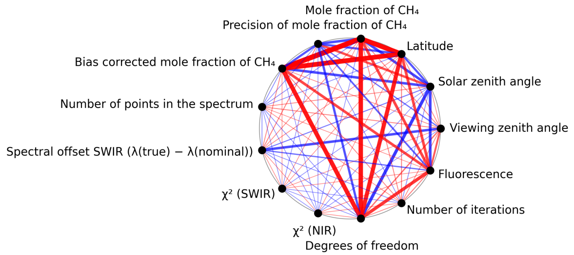
Figure 1: Map of correlation graph for 2024-12-27 to 2024-12-28.
