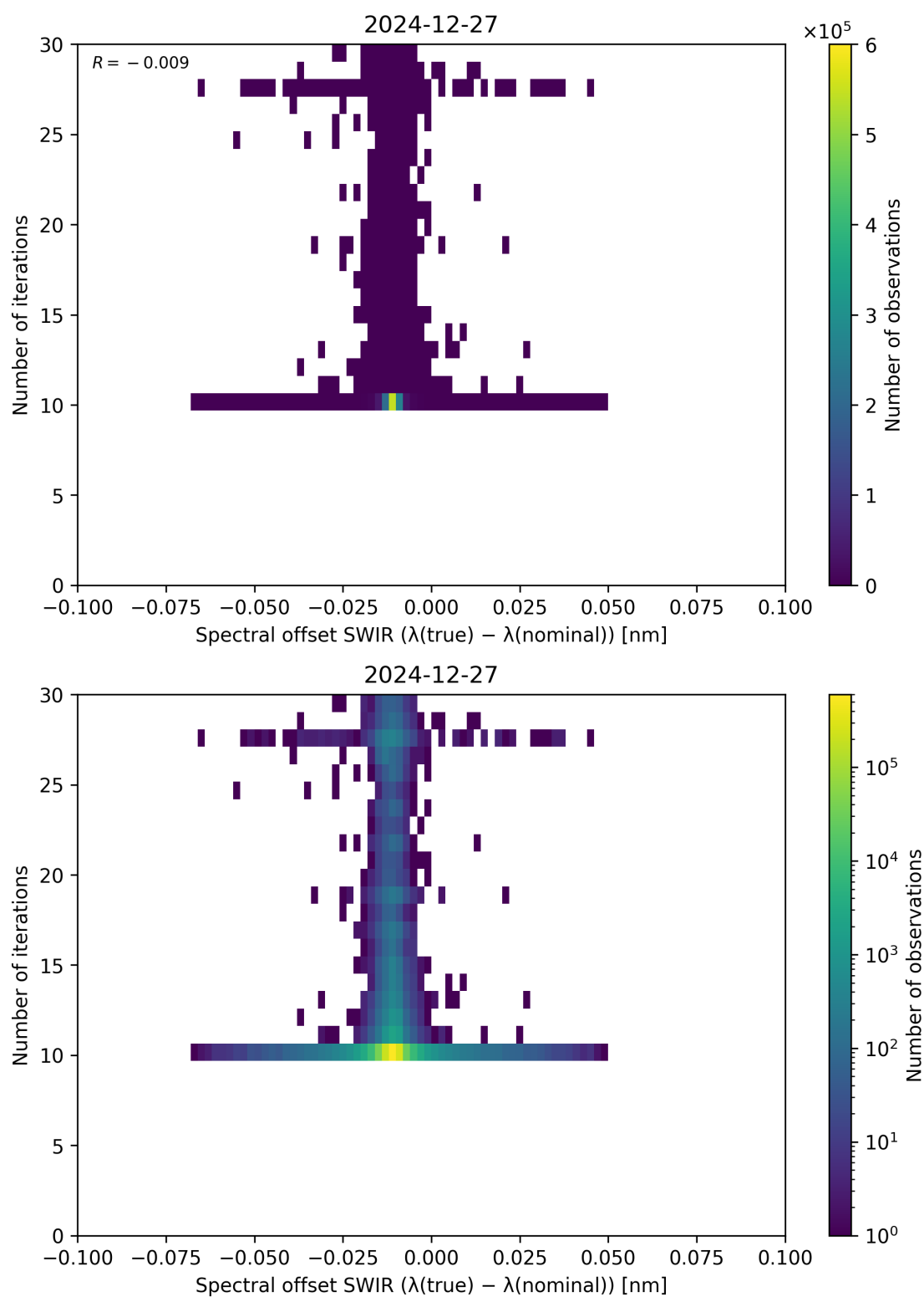
Figure 121: Scatter density plot of “Spectral offset SWIR ( \lambda_{\text{true}} - \lambda_{\text{nominal}} )” against “Number of iterations” for 2024-12-27 to 2024-12-28.
