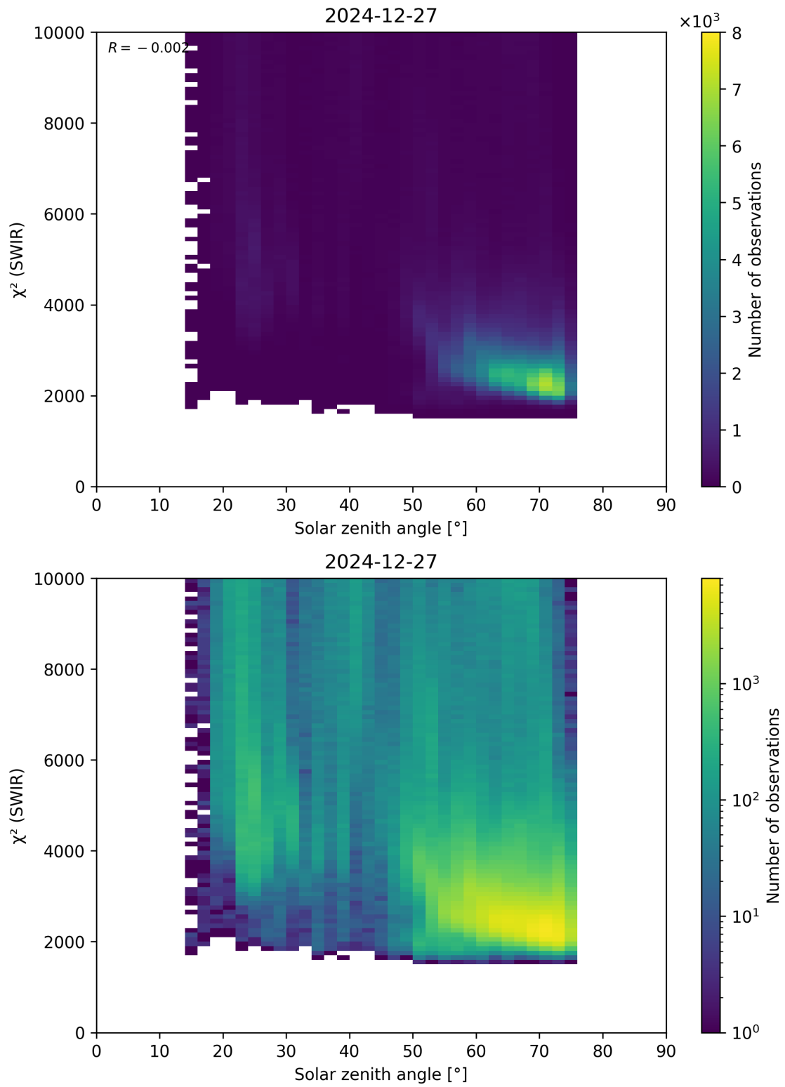
Figure 95: Scatter density plot of “Solar zenith angle” against “ \chi^2 (SWIR)” for 2024-12-27 to 2024-12-28.
