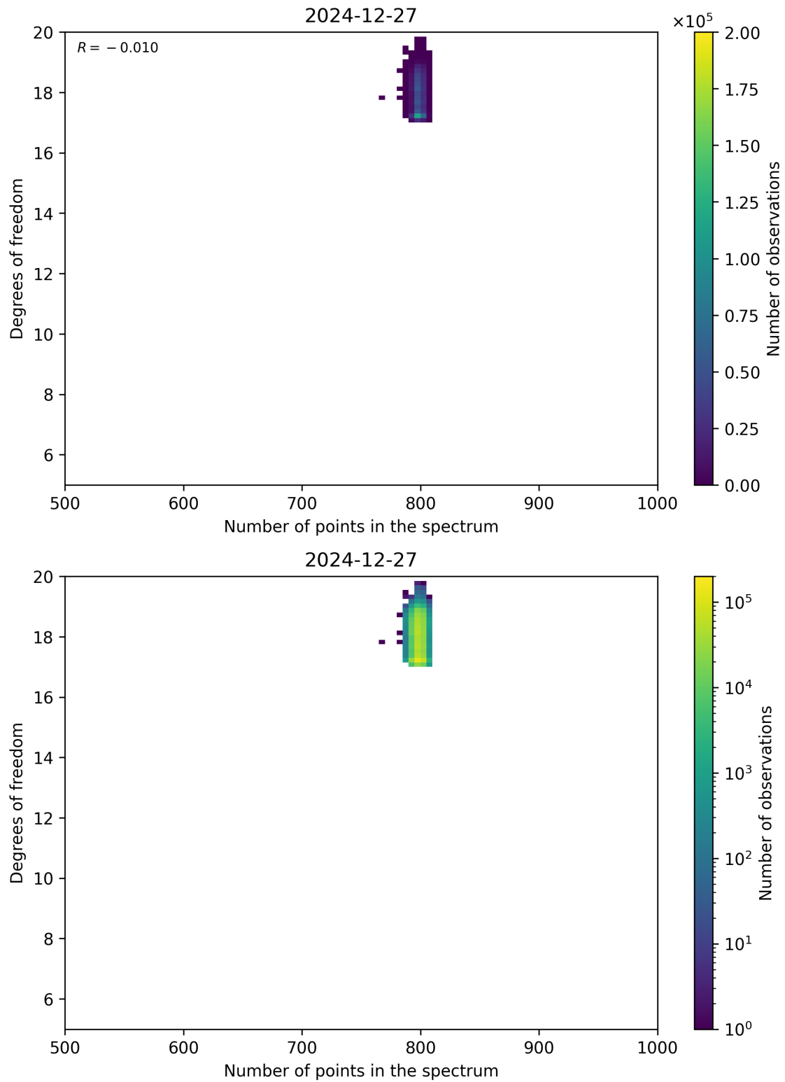
Figure 90: Scatter density plot of “Number of points in the spectrum” against “Degrees of freedom” for 2024-12-27 to 2024-12-28.
