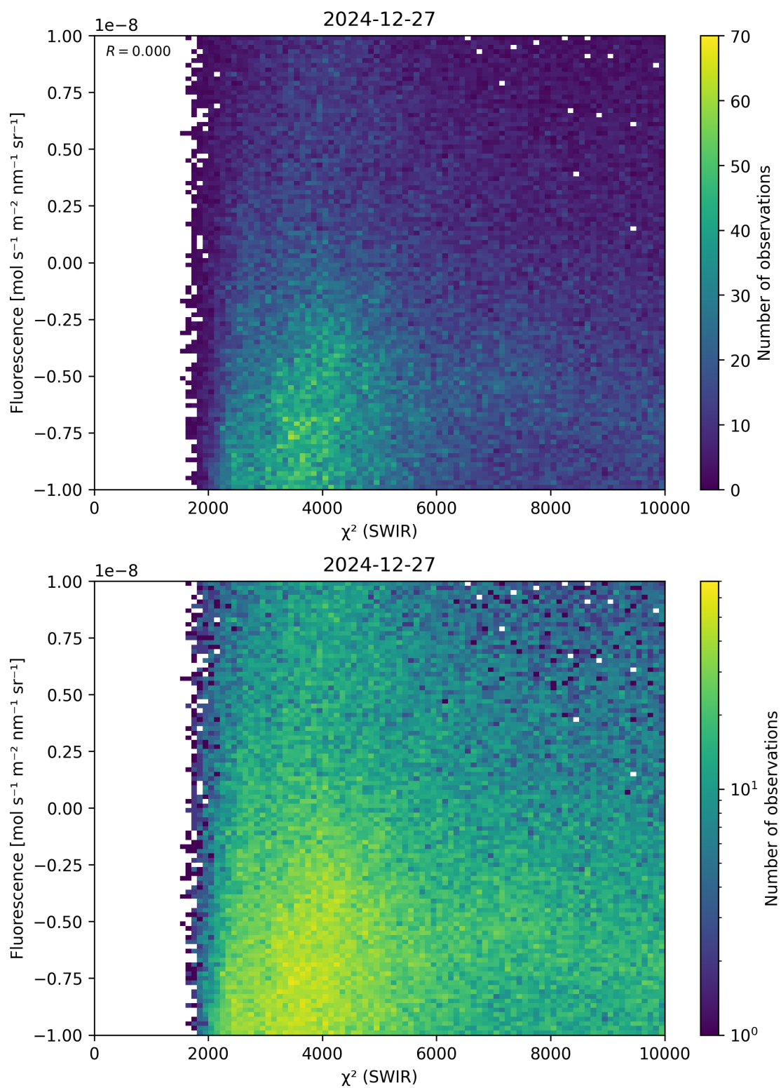
Figure 49: Scatter density plot of “ \chi^2 (SWIR)” against “Fluorescence” for 2024-12-27 to 2024-12-28.
