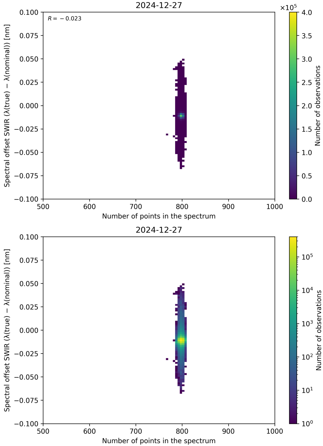
Figure 93: Scatter density plot of “Number of points in the spectrum” against “Spectral offset SWIR ( \lambda_{\text{true}} - \lambda_{\text{nominal}} )” for 2024-12-27 to 2024-12-28.
