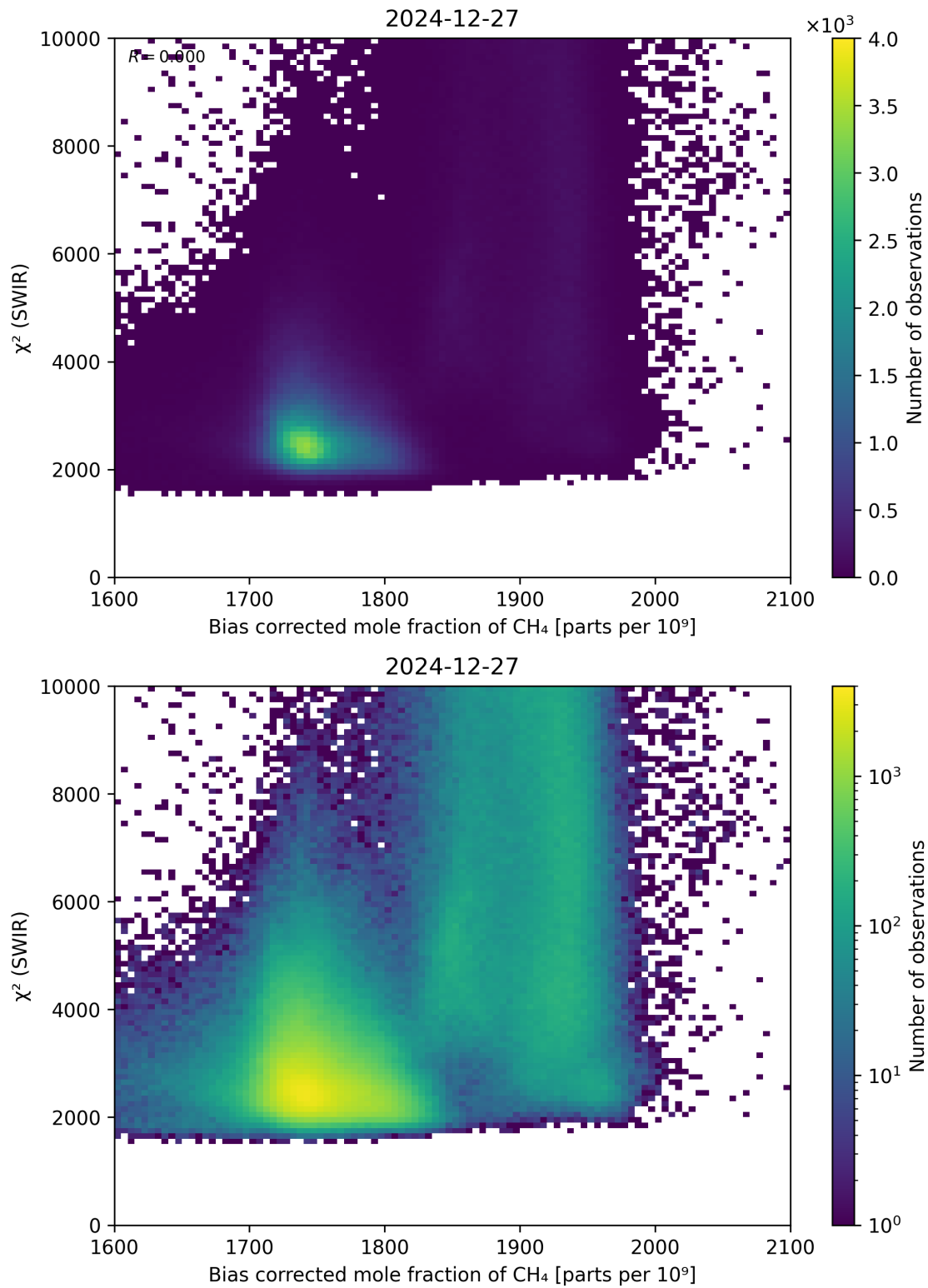
Figure 64: Scatter density plot of “Bias corrected mole fraction of \text{CH}_4 ” against “ \chi^2 (SWIR)” for 2024-12-27 to 2024-12-28.
