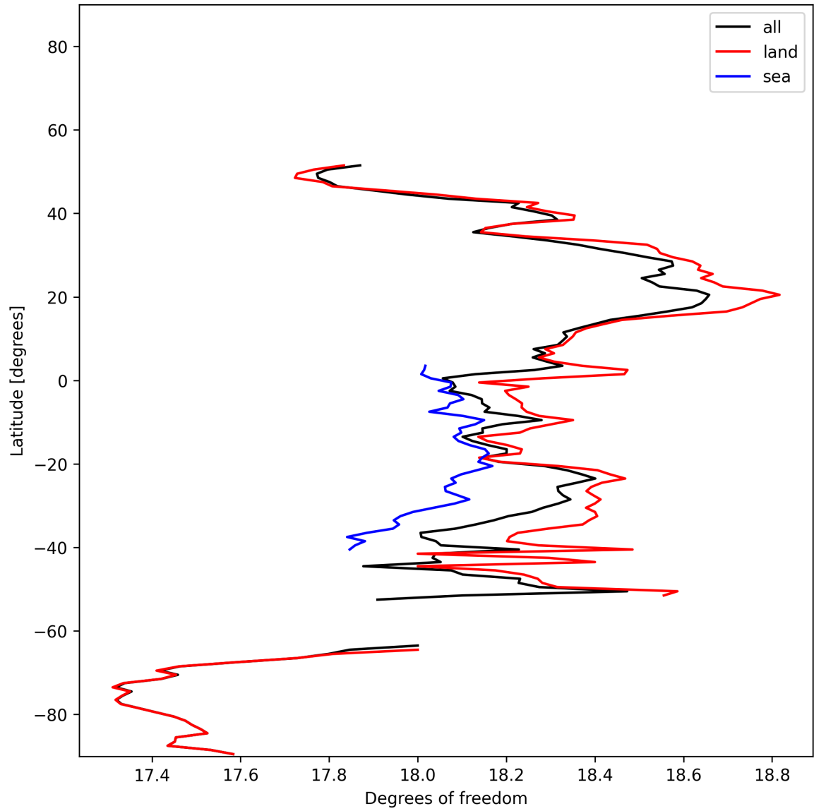
Figure 19: Zonal average of “Degrees of freedom” for 2024-12-27 to 2024-12-28.
