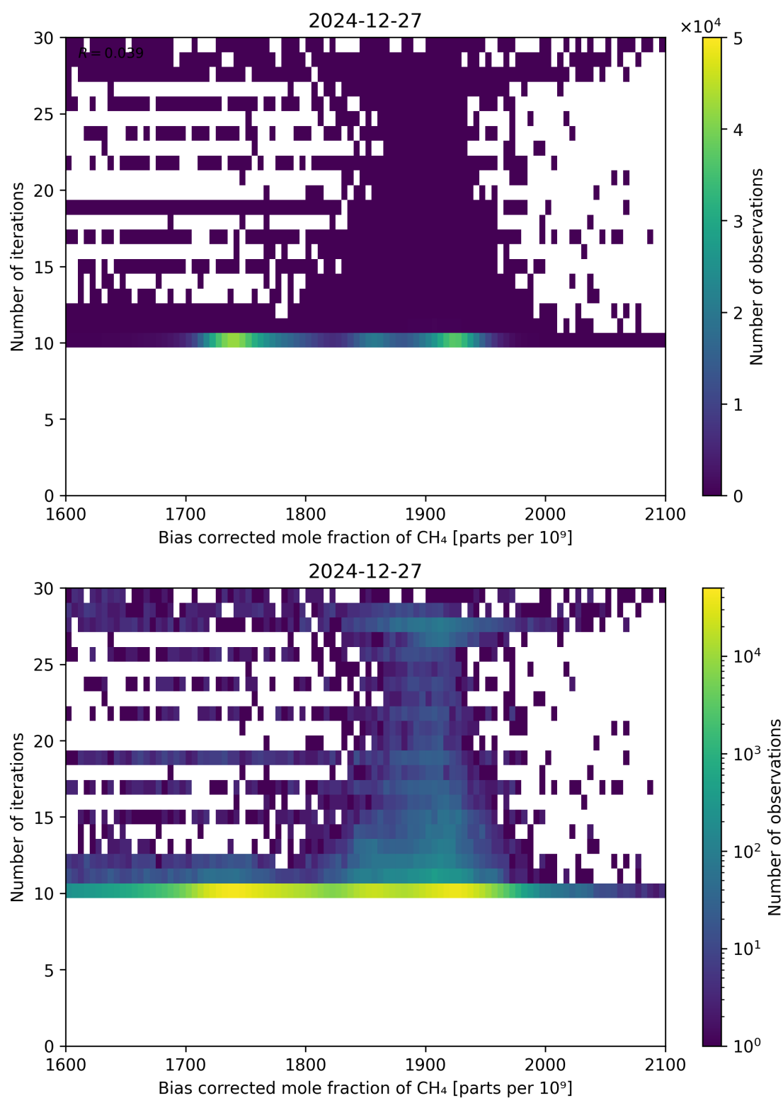
Figure 67: Scatter density plot of “Bias corrected mole fraction of \text{CH}_4 ” against “Number of iterations” for 2024-12-27 to 2024-12-28.
