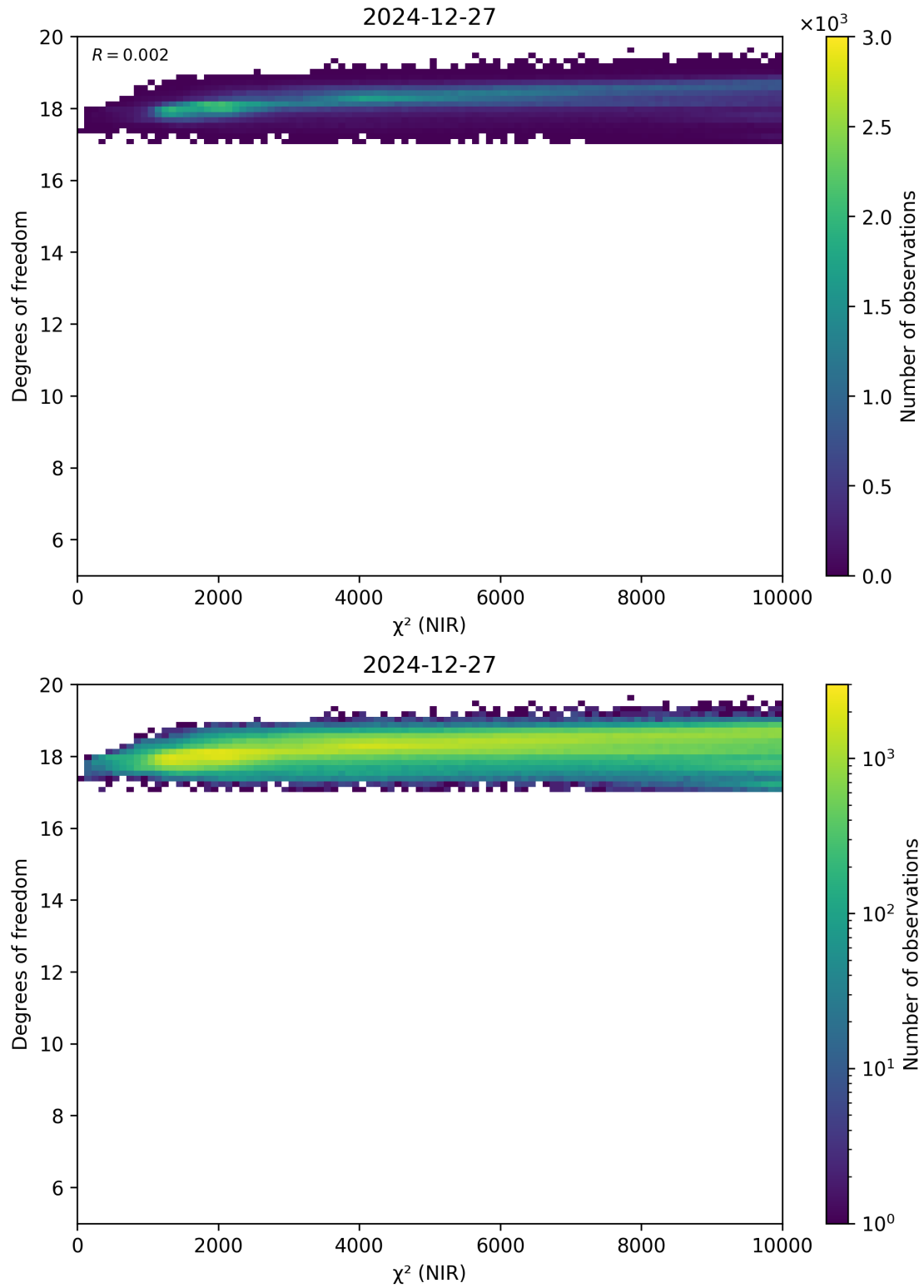
Figure 44: Scatter density plot of “ \chi^2 (NIR)” against “Degrees of freedom” for 2024-12-27 to 2024-12-28.
