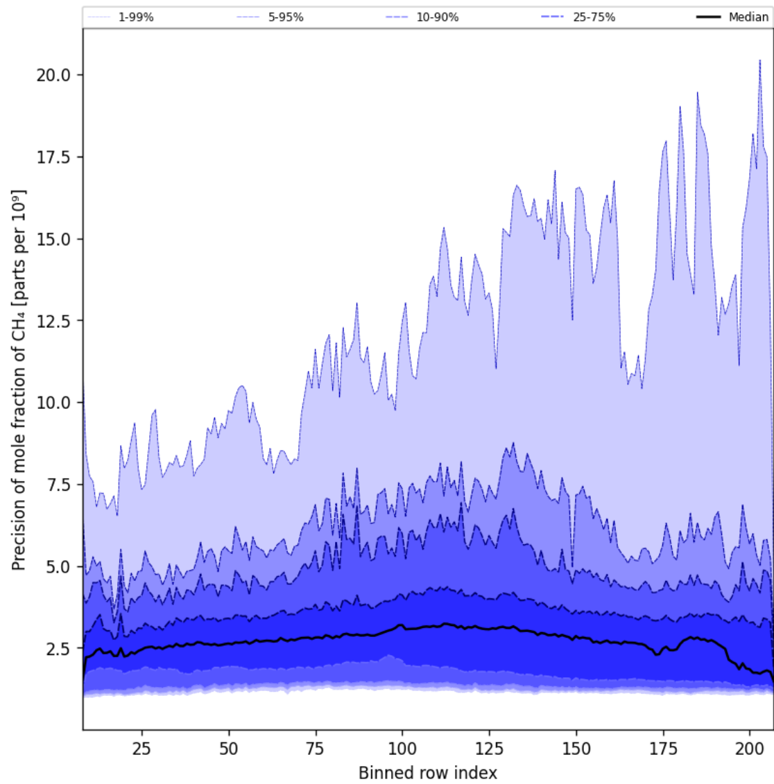
Figure 35: Along track statistics of “Precision of mole fraction of CH 4 ” for 2024-12-27 to 2024-12-28
