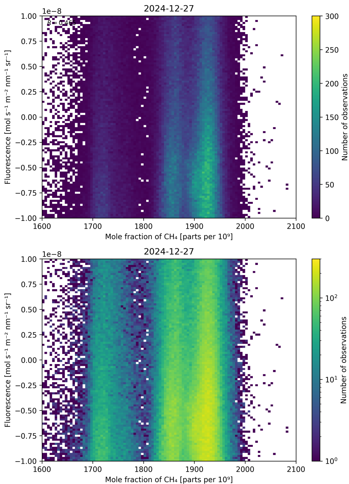
Figure 73: Scatter density plot of “Mole fraction of \text{CH}_4 ” against “Fluorescence” for 2024-12-27 to 2024-12-28.
