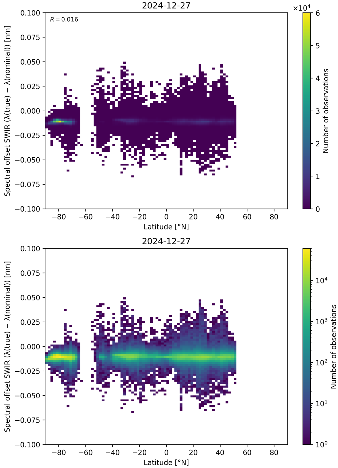
Figure 62: Scatter density plot of “Latitude” against “Spectral offset SWIR ( \lambda_{\text{true}} - \lambda_{\text{nominal}} )” for 2024-12-27 to 2024-12-28.
