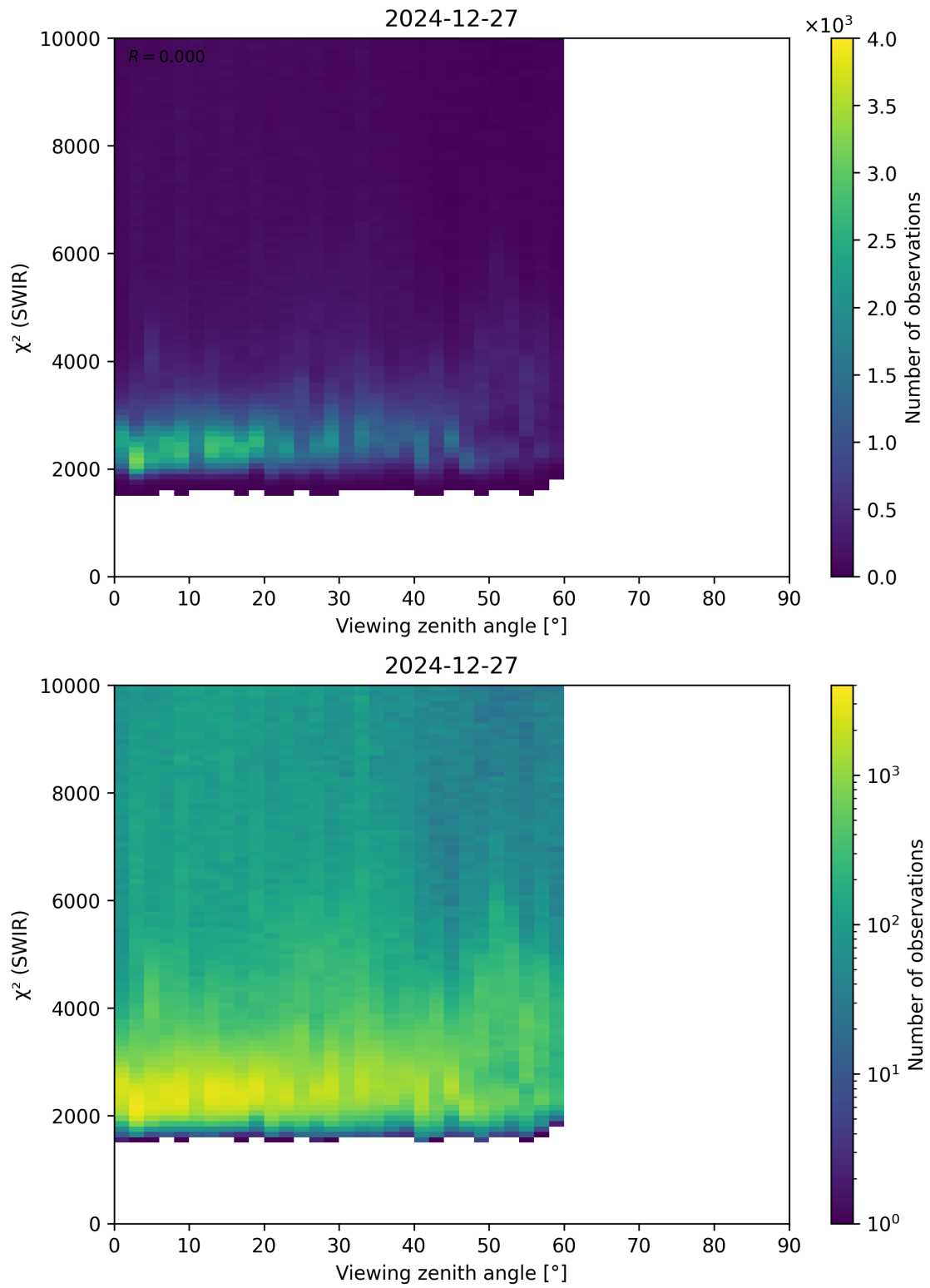
Figure 106: Scatter density plot of “Viewing zenith angle” against “ \chi^2 (SWIR)” for 2024-12-27 to 2024-12-28.
