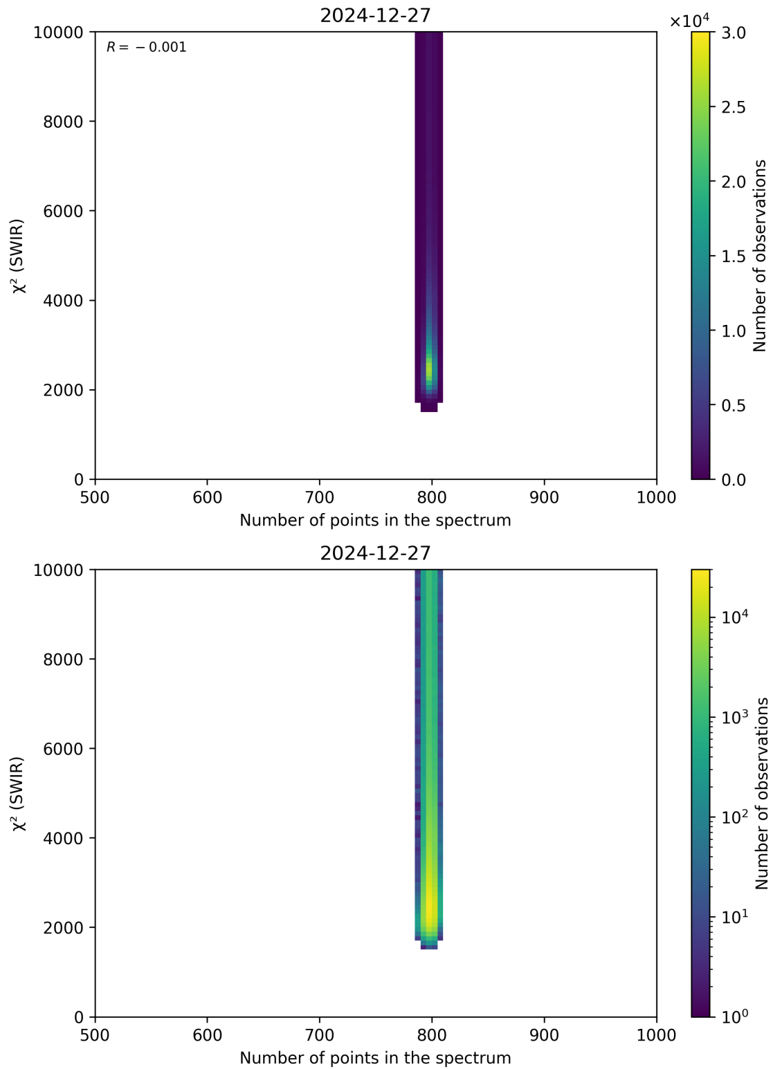
Figure 89: Scatter density plot of “Number of points in the spectrum” against “ \chi^2 (SWIR)” for 2024-12-27 to 2024-12-28.
