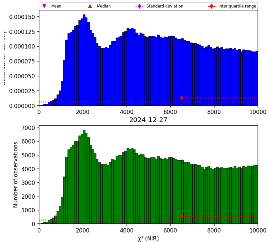
Figure 29: Histogram of “ \chi^2 (NIR)” for 2024-12-27 to 2024-12-28
