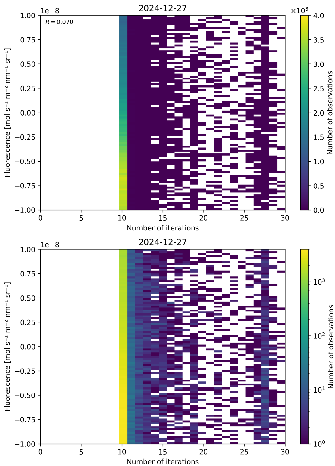
Figure 87: Scatter density plot of “Number of iterations” against “Fluorescence” for 2024-12-27 to 2024-12-28.
