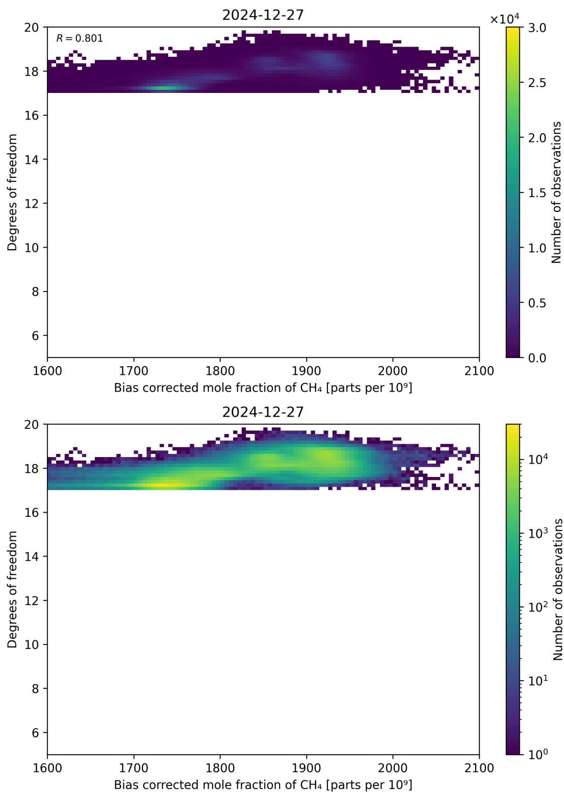
Figure 65: Scatter density plot of “Bias corrected mole fraction of \text{CH}_4 ” against “Degrees of freedom” for 2024-12-27 to 2024-12-28.
