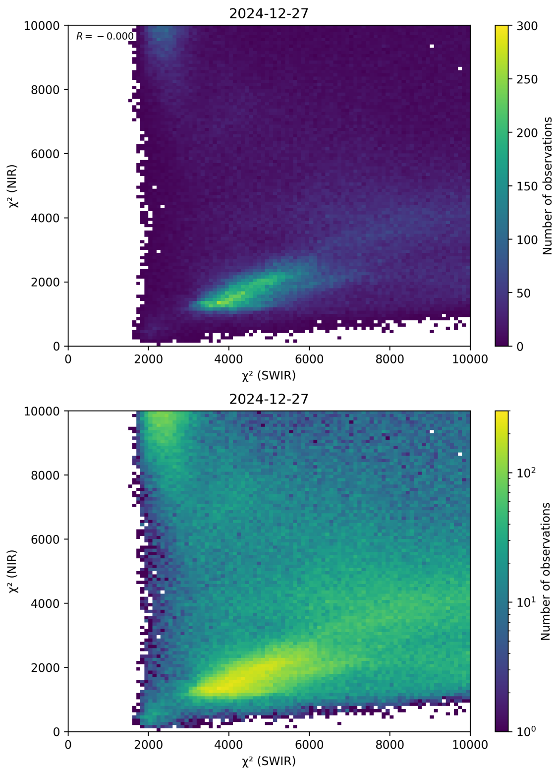
Figure 47: Scatter density plot of “ \chi^2 (SWIR)” against “ \chi^2 (NIR)” for 2024-12-27 to 2024-12-28.
