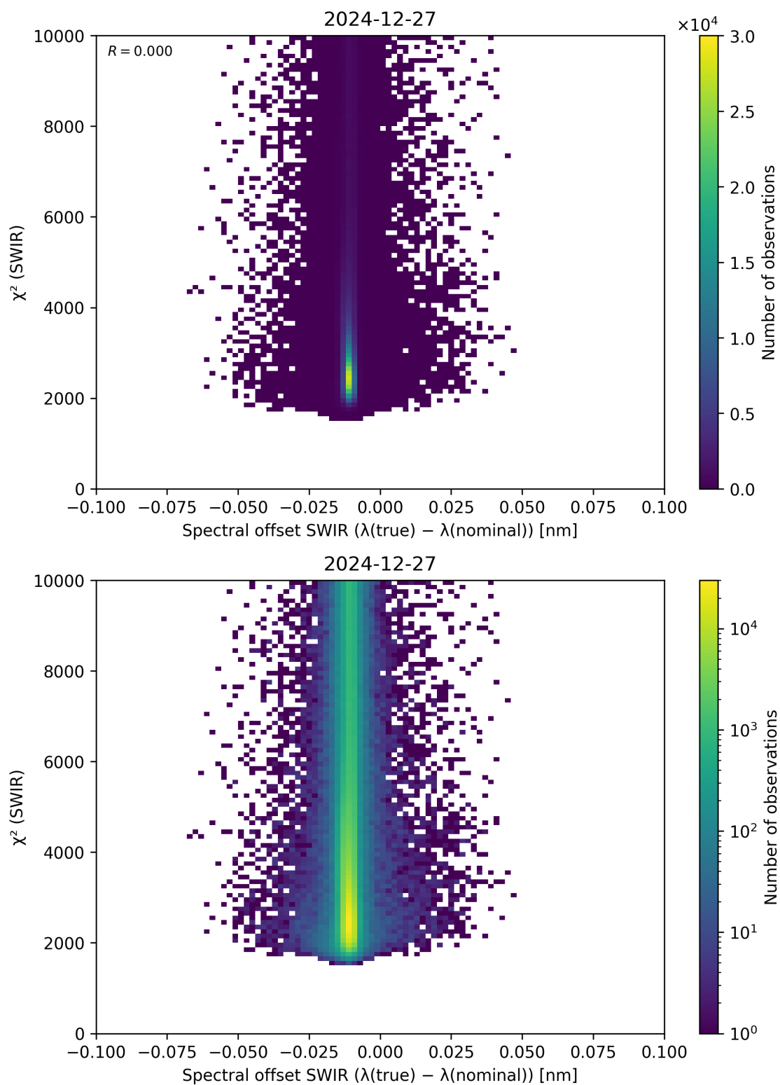
Figure 118: Scatter density plot of “Spectral offset SWIR ( \lambda_{\text{true}} - \lambda_{\text{nominal}} )” against “ \chi^2 (SWIR)” for 2024-12-27 to 2024-12-28.
