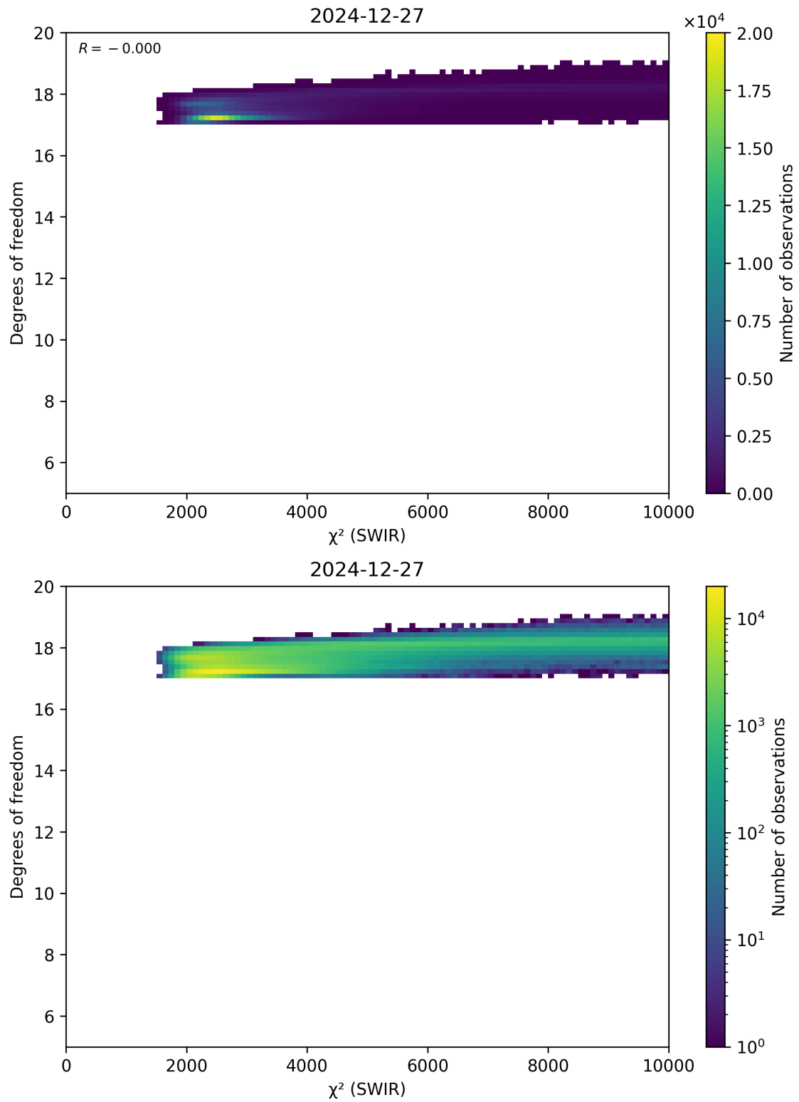
Figure 48: Scatter density plot of “ \chi^2 (SWIR)” against “Degrees of freedom” for 2024-12-27 to 2024-12-28.
