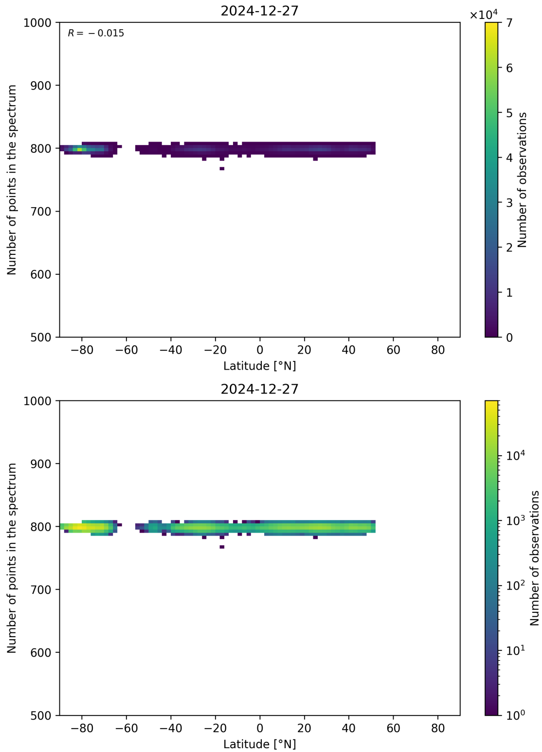
Figure 61: Scatter density plot of “Latitude” against “Number of points in the spectrum” for 2024-12-27 to 2024-12-28.
