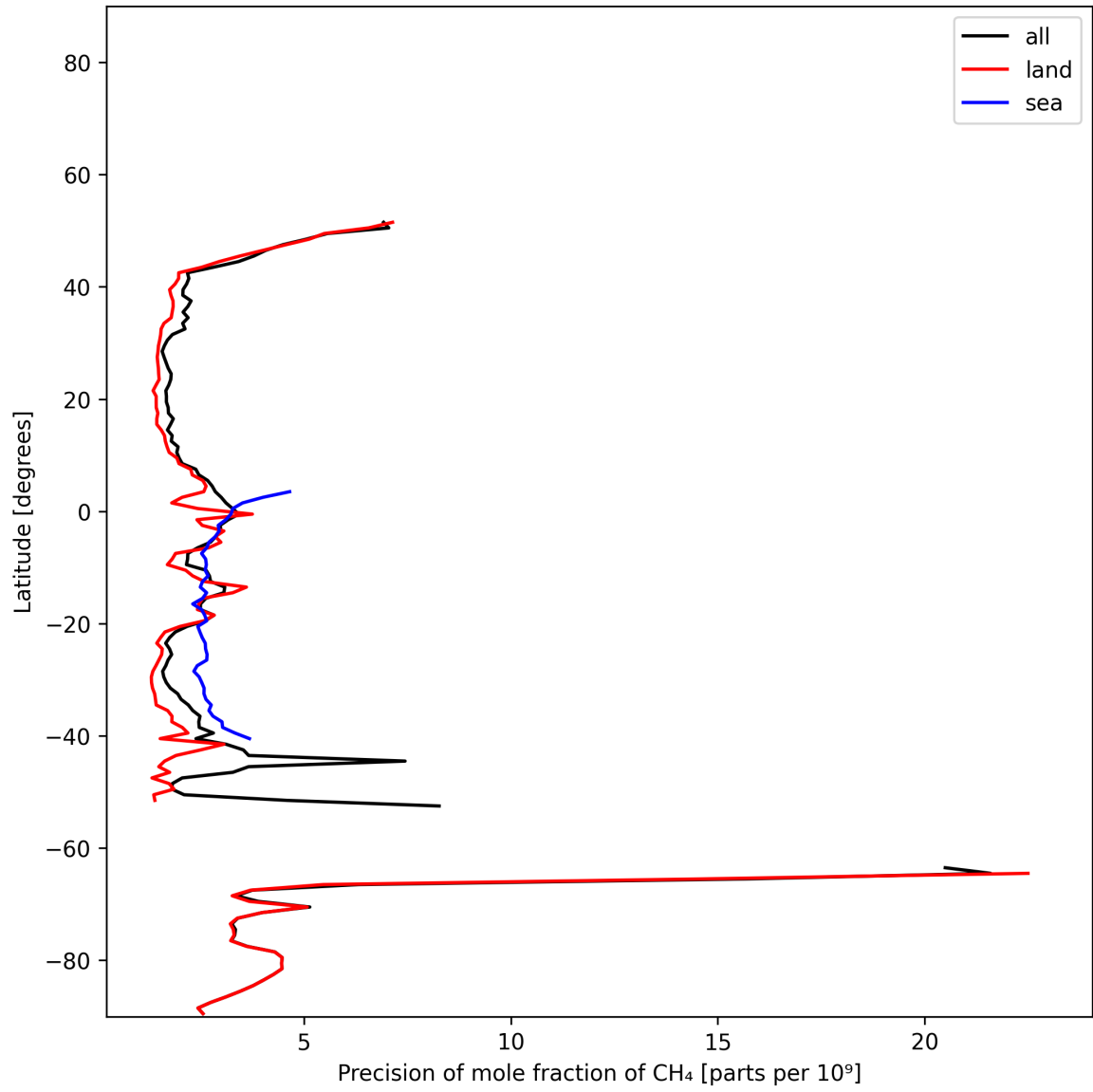
Figure 13: Zonal average of “Precision of mole fraction of CH 4 ” for 2024-12-27 to 2024-12-28.
