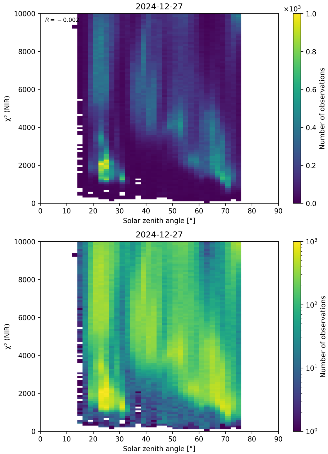
Figure 94: Scatter density plot of “Solar zenith angle” against “ \chi^2 (NIR)” for 2024-12-27 to 2024-12-28.
