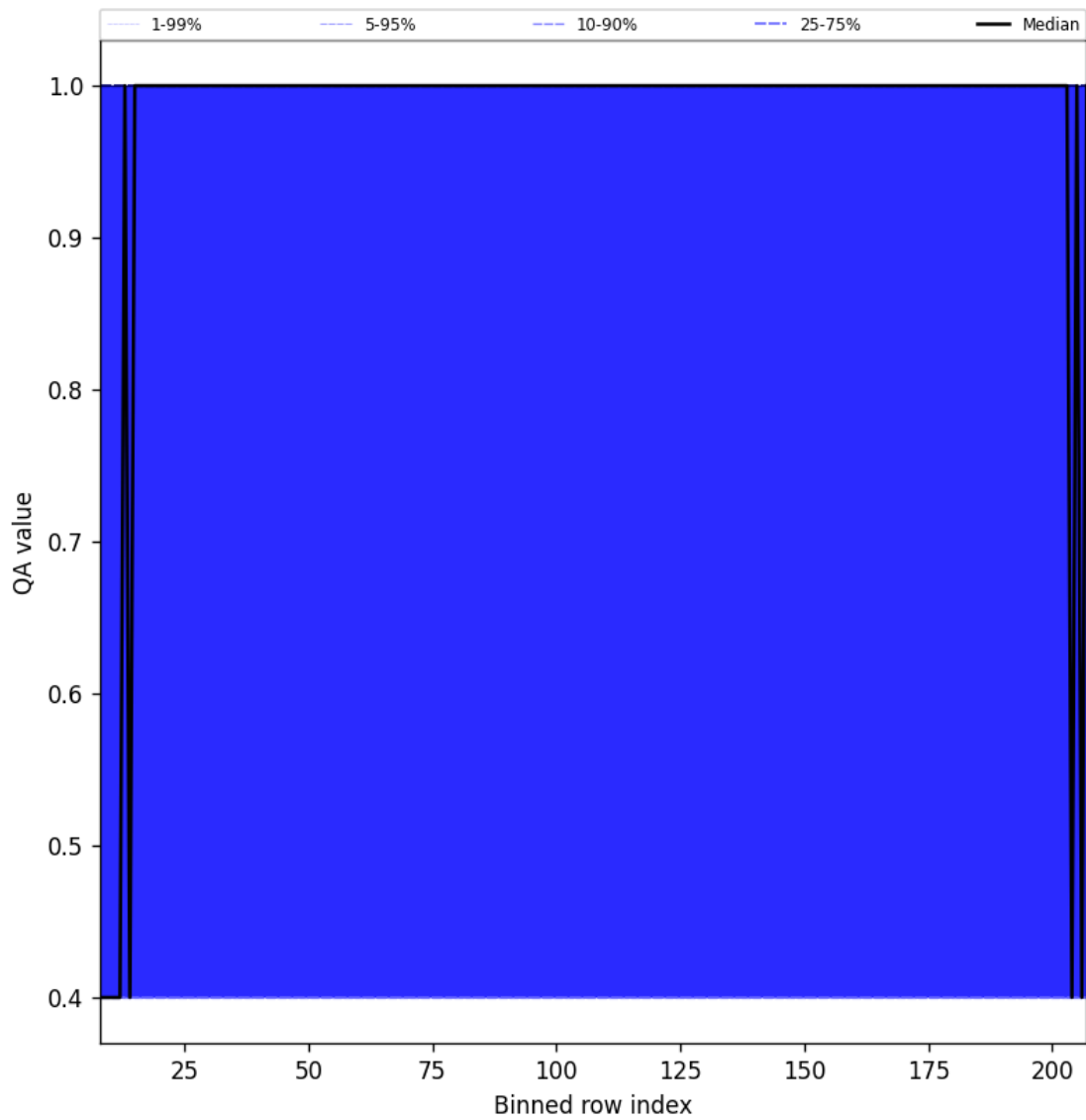
Figure 33: Along track statistics of “QA value” for 2024-12-27 to 2024-12-28
