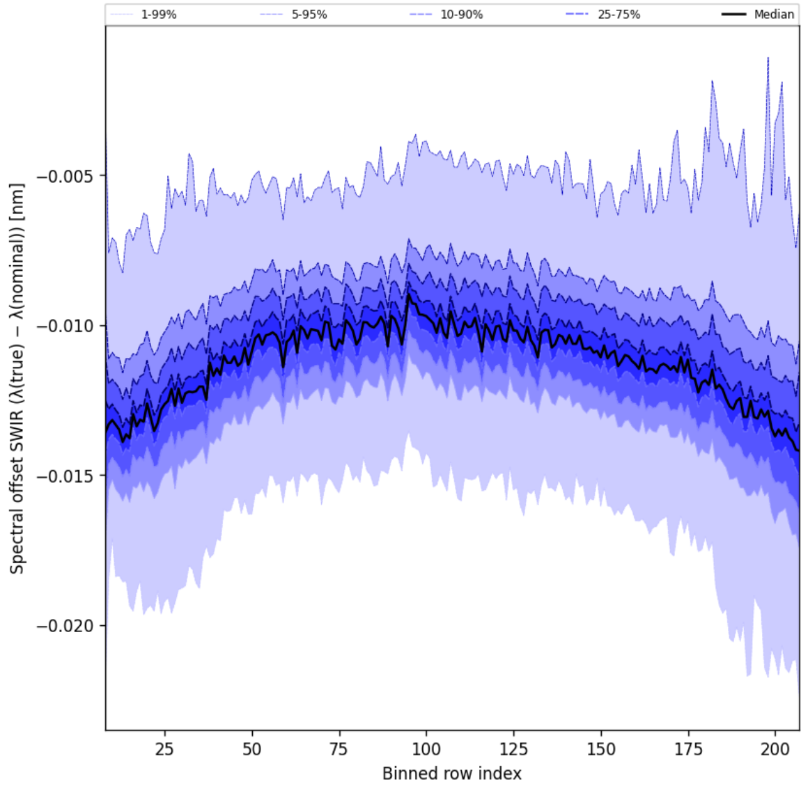
Figure 38: Along track statistics of “Spectral offset SWIR ( \lambda_{\text{true}} - \lambda_{\text{nominal}} )” for 2024-12-27 to 2024-12-28
