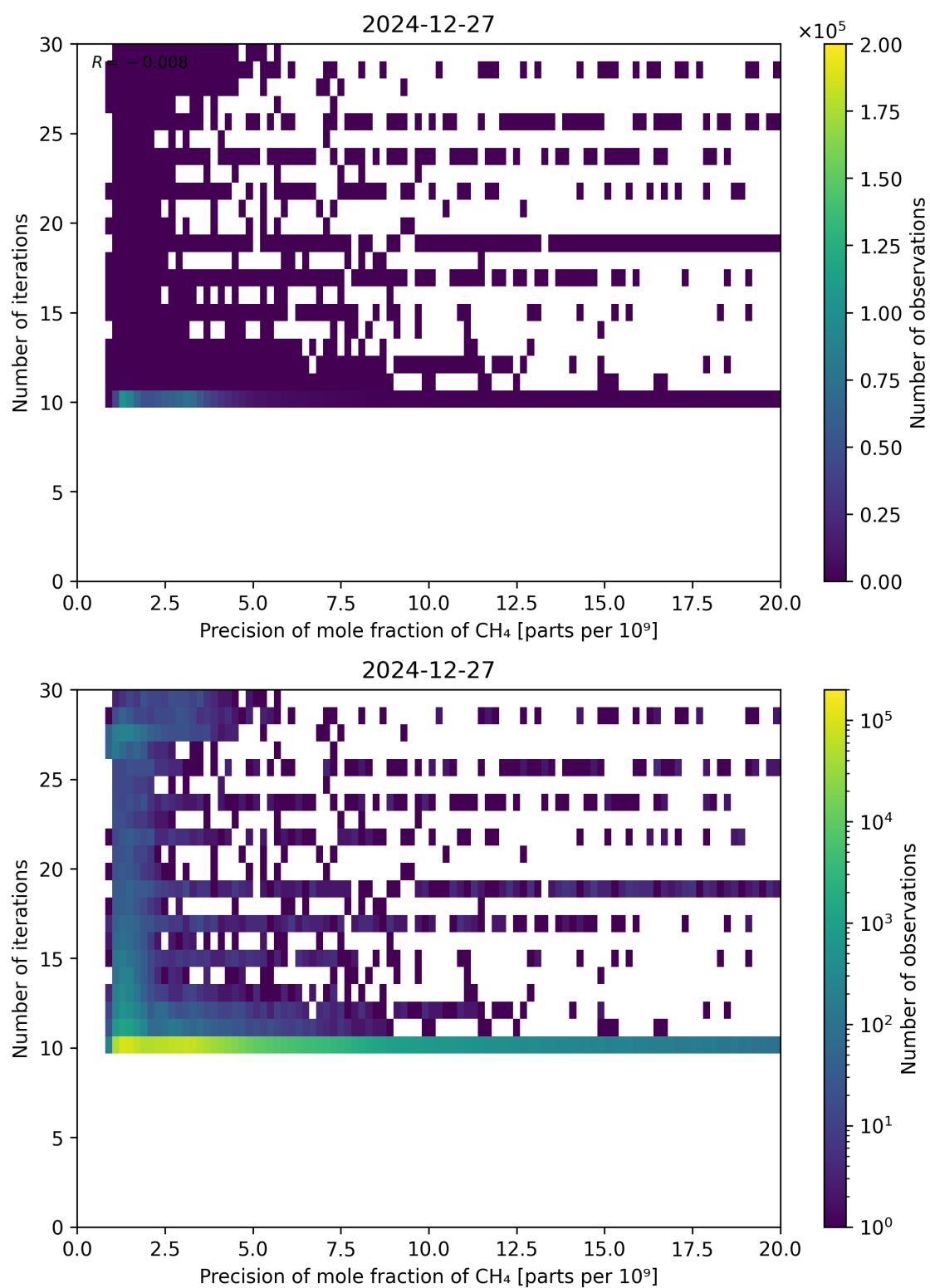
Figure 83: Scatter density plot of “Precision of mole fraction of CH 4 ” against “Number of iterations” for 2024-12-27 to 2024-12-28.
