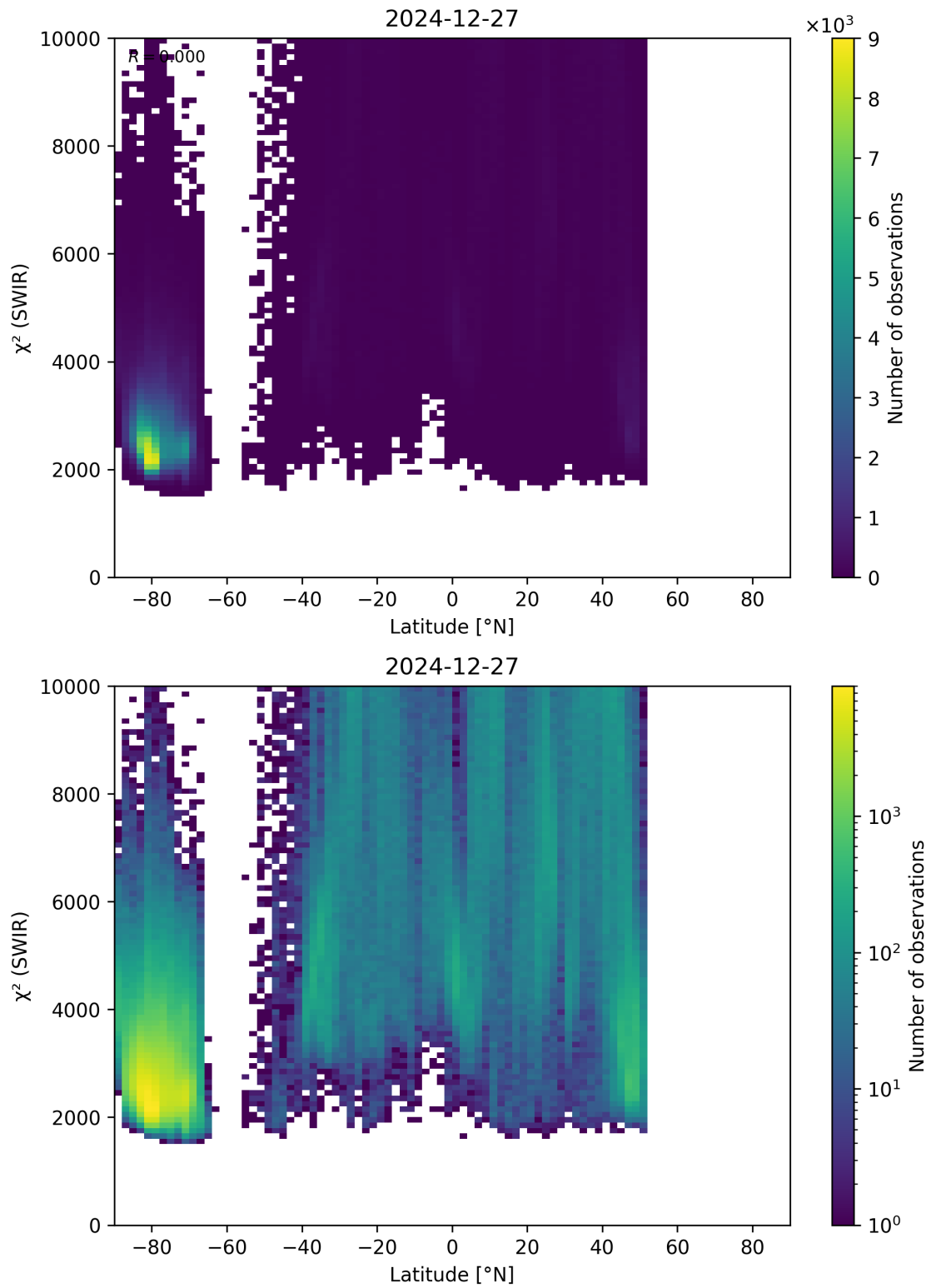
Figure 54: Scatter density plot of “Latitude” against “ \chi^2 (SWIR)” for 2024-12-27 to 2024-12-28.
