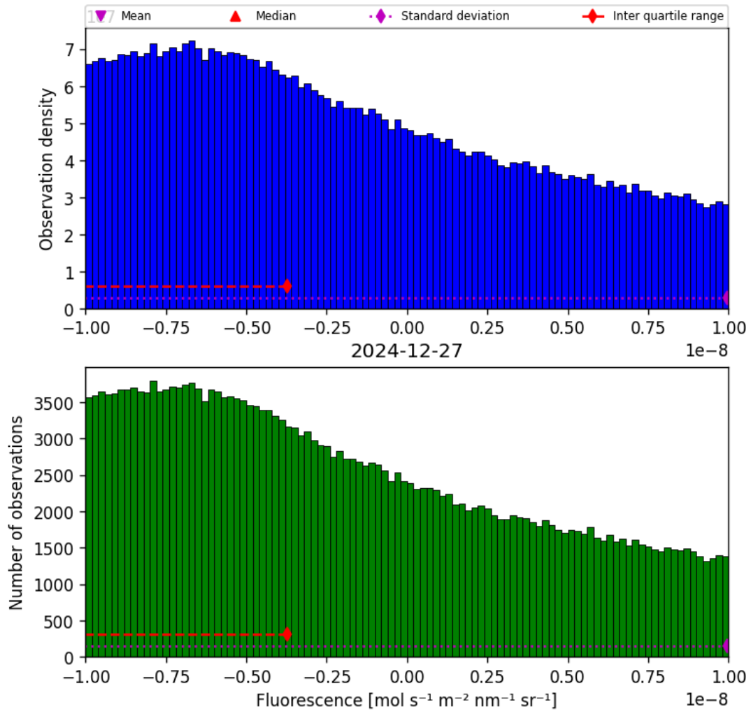
Figure 32: Histogram of “Fluorescence” for 2024-12-27 to 2024-12-28
