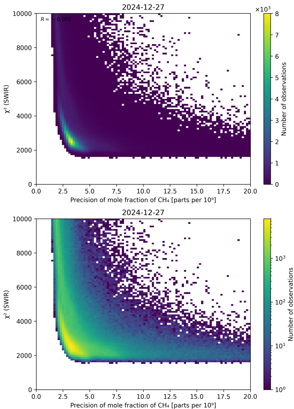
Figure 79: Scatter density plot of “Precision of mole fraction of \text{CH}_4 ” against “ \chi^2 (SWIR)” for 2024-12-27 to 2024-12-28.
