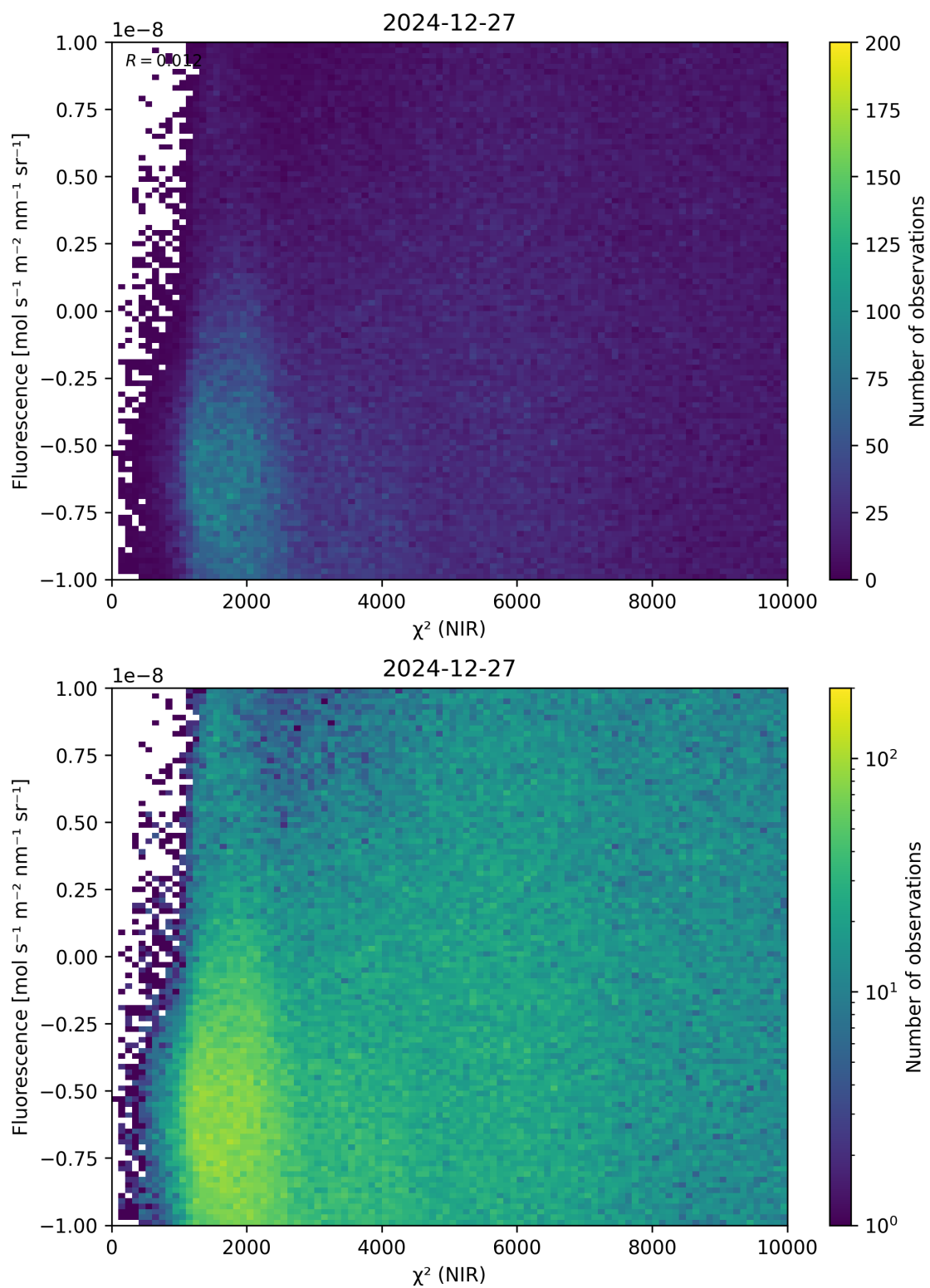
Figure 45: Scatter density plot of “ \chi^2 (NIR)” against “Fluorescence” for 2024-12-27 to 2024-12-28.
