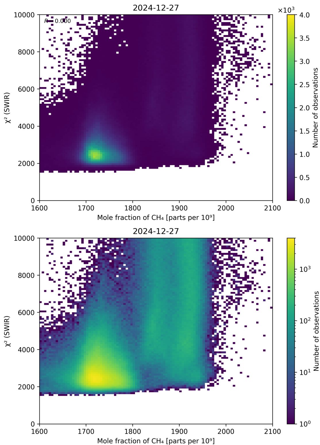
Figure 71: Scatter density plot of “Mole fraction of \text{CH}_4 ” against “ \chi^2 (SWIR)” for 2024-12-27 to 2024-12-28.
