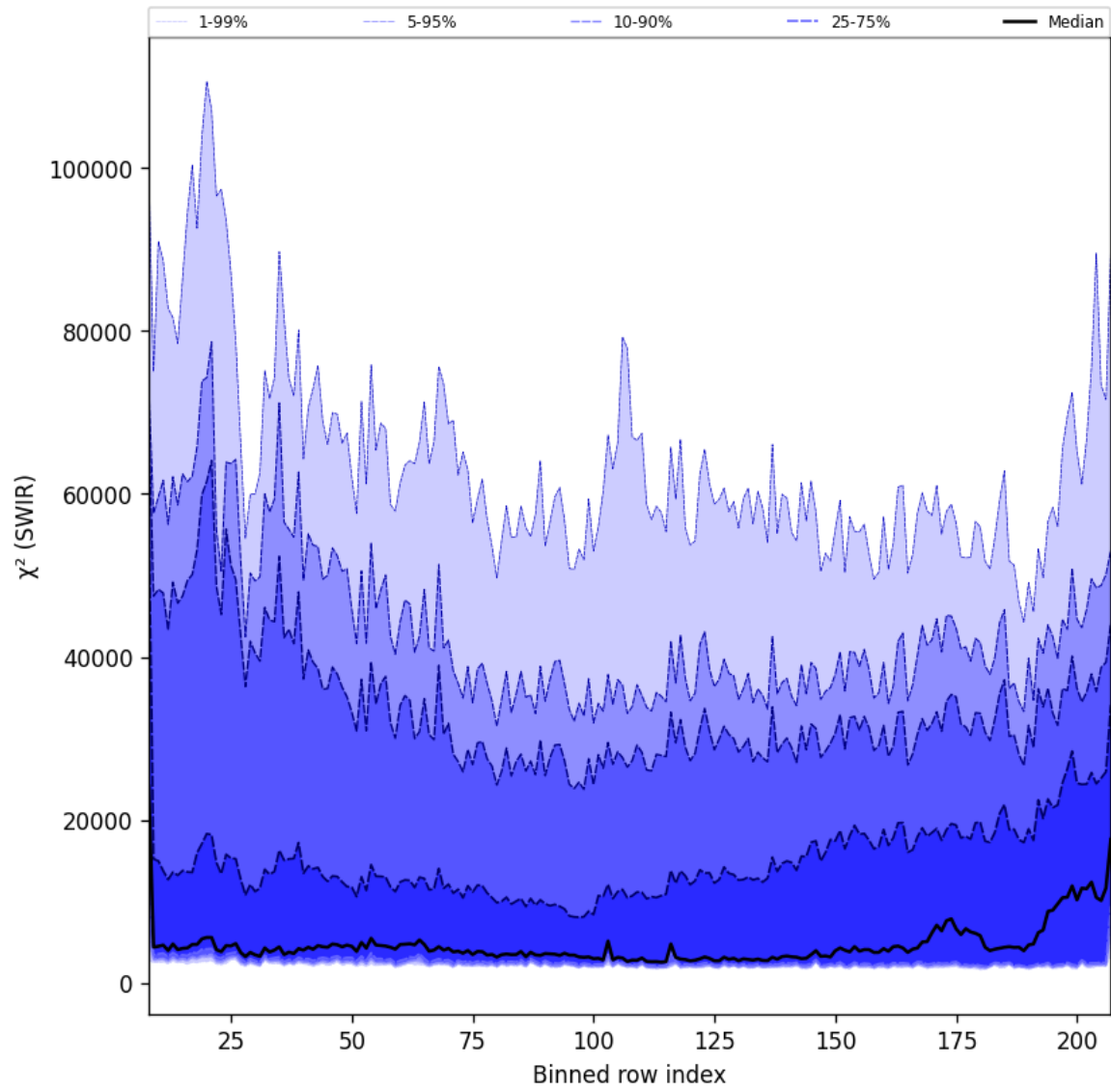
Figure 39: Along track statistics of “ \chi^2 (SWIR)” for 2024-12-27 to 2024-12-28
