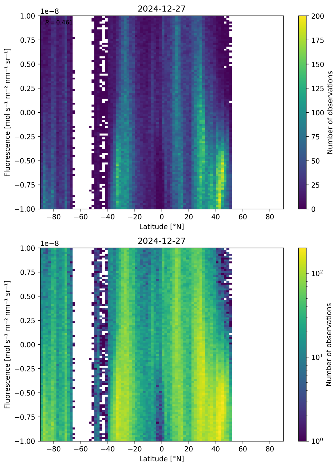
Figure 56: Scatter density plot of “Latitude” against “Fluorescence” for 2024-12-27 to 2024-12-28.
