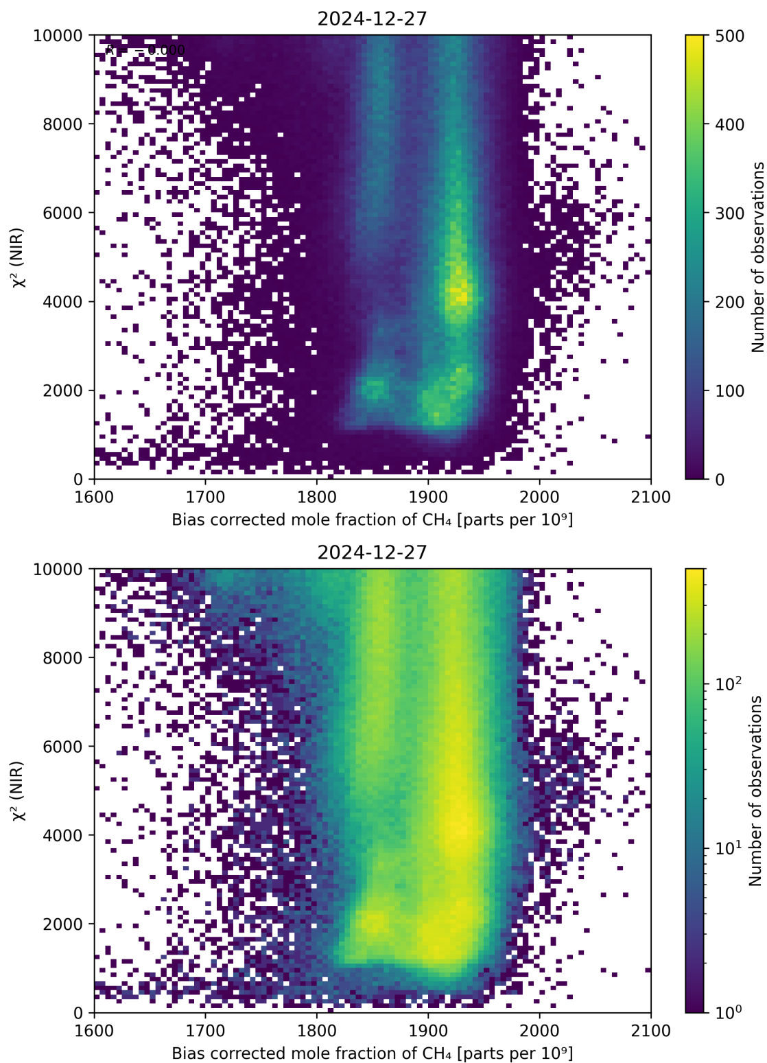
Figure 63: Scatter density plot of “Bias corrected mole fraction of CH 4 ” against “ \chi^2 (NIR)” for 2024-12-27 to 2024-12-28.
