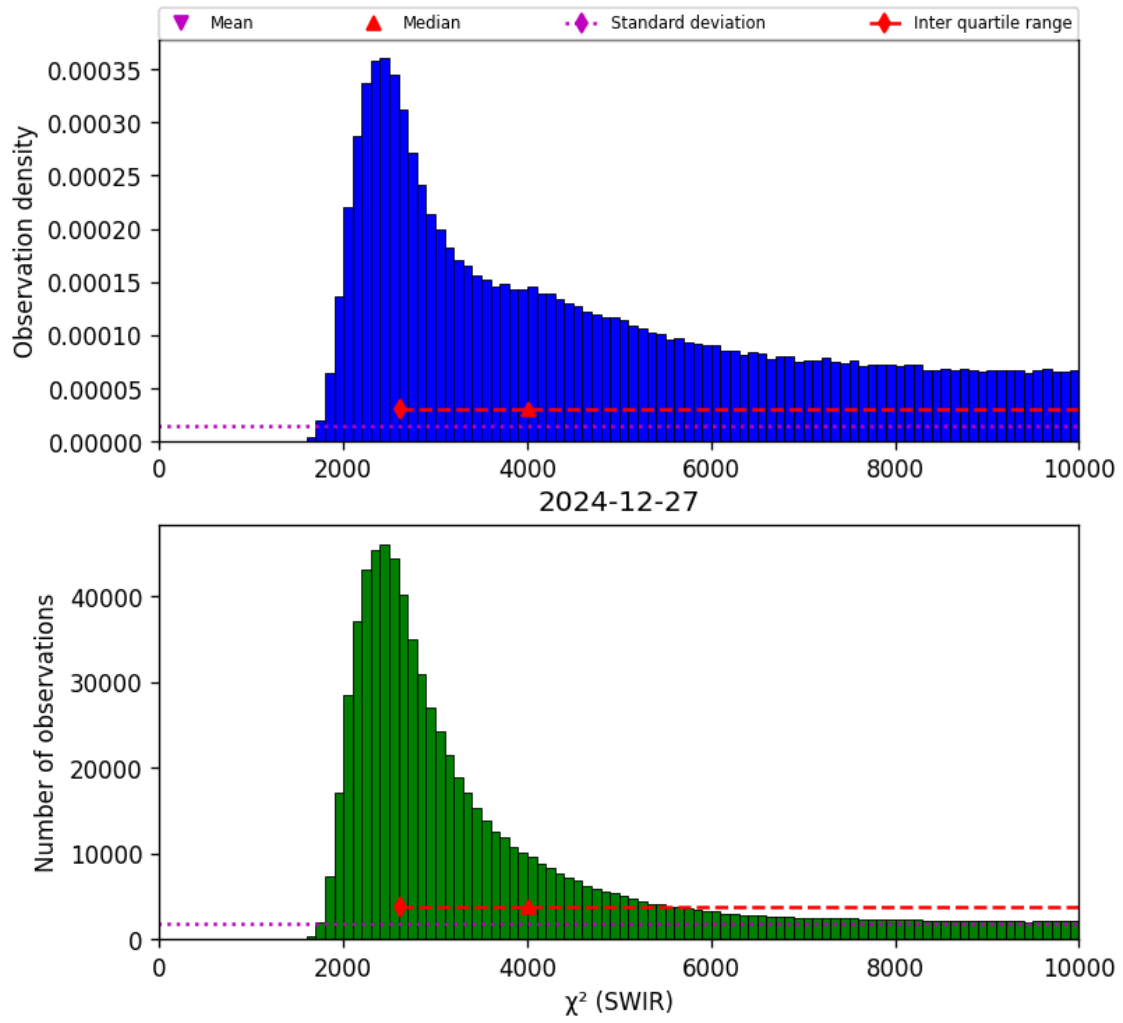
Figure 28: Histogram of “ \chi^2 (SWIR)” for 2024-12-27 to 2024-12-28
