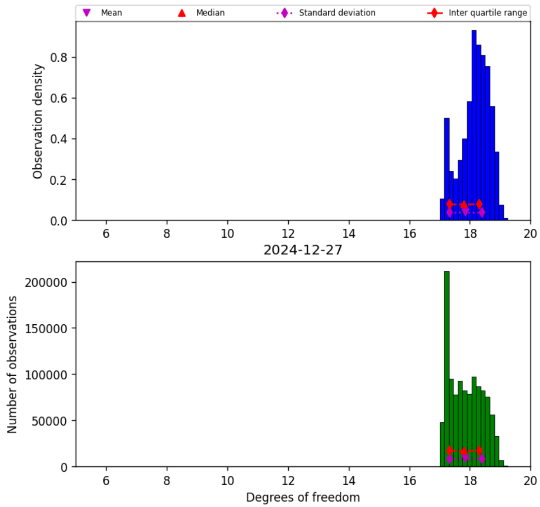
Figure 30: Histogram of “Degrees of freedom” for 2024-12-27 to 2024-12-28
