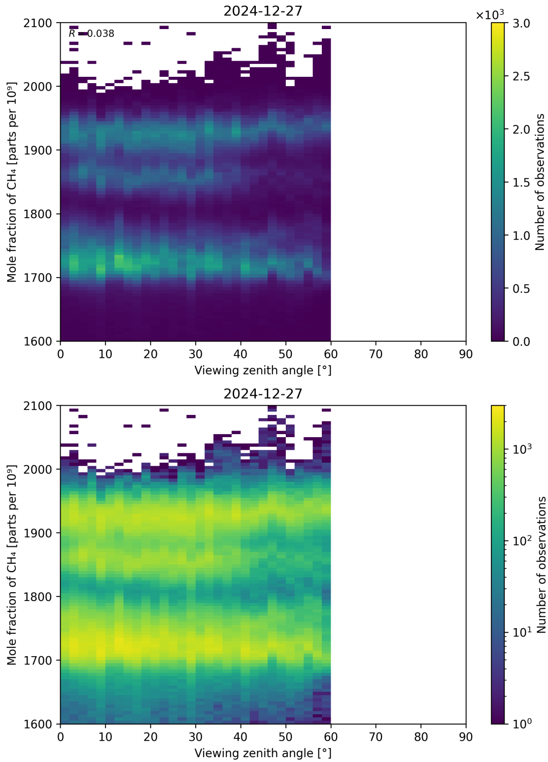
Figure 110: Scatter density plot of “Viewing zenith angle” against “Mole fraction of CH 4 ” for 2024-12-27 to 2024-12-28.
