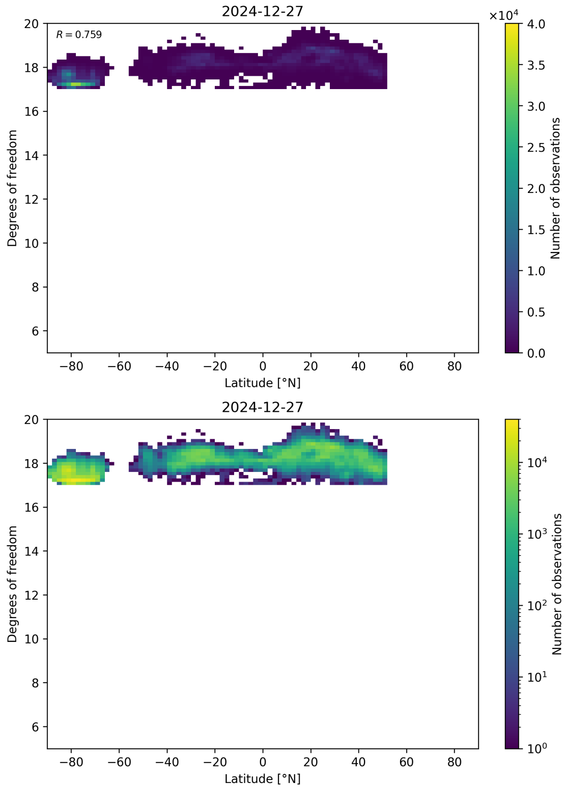
Figure 55: Scatter density plot of “Latitude” against “Degrees of freedom” for 2024-12-27 to 2024-12-28.
