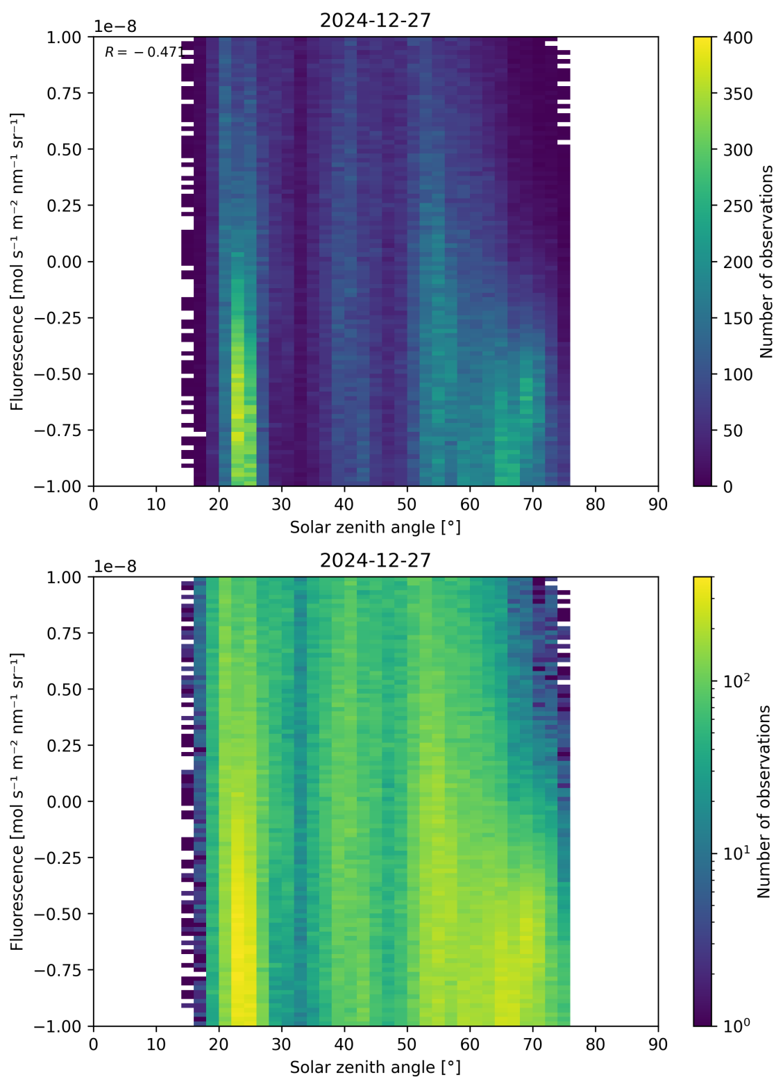
Figure 97: Scatter density plot of “Solar zenith angle” against “Fluorescence” for 2024-12-27 to 2024-12-28.
