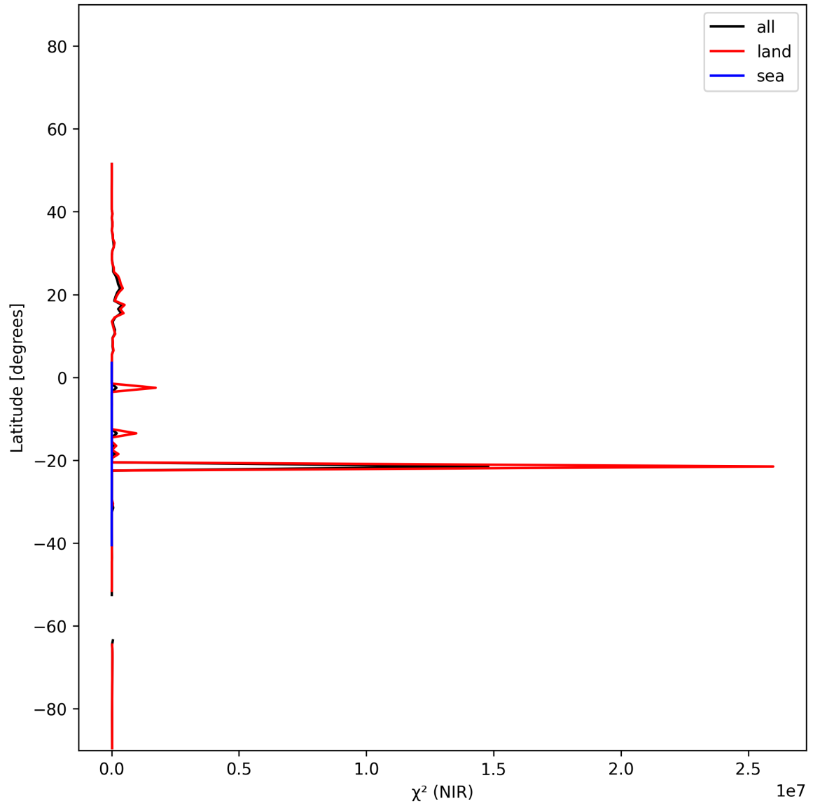
Figure 18: Zonal average of “ \chi^2 (NIR)” for 2024-12-27 to 2024-12-28.
