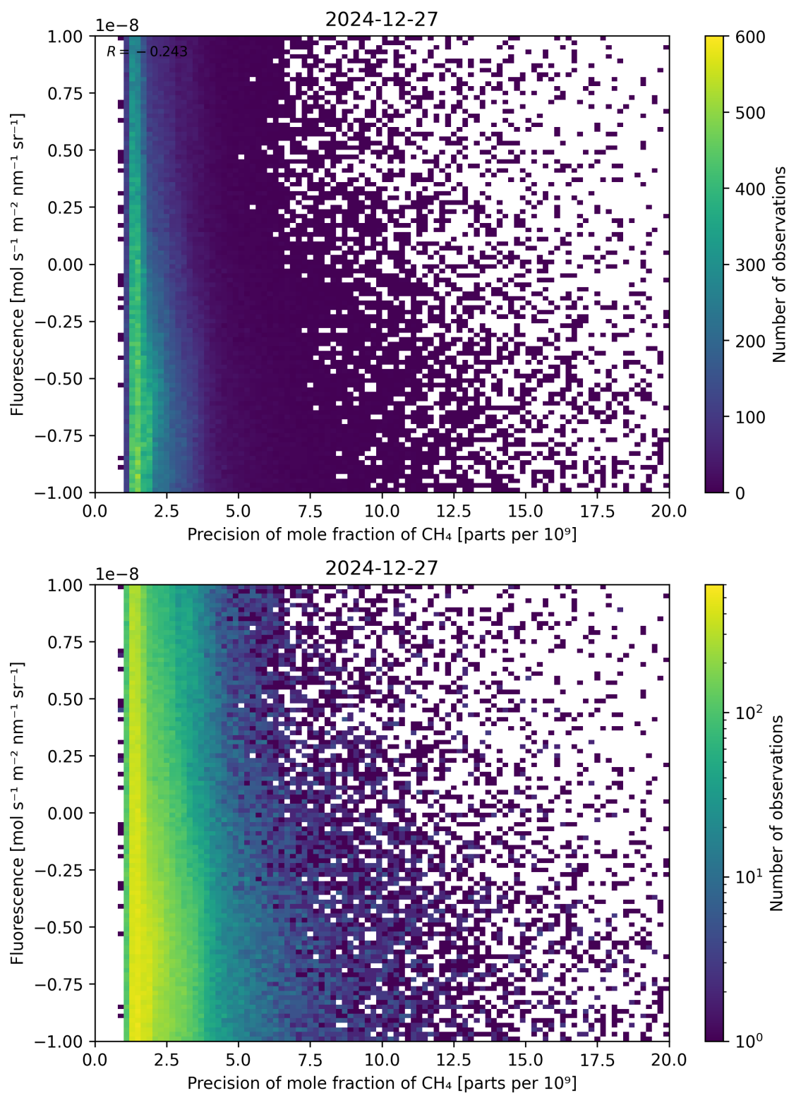
Figure 81: Scatter density plot of “Precision of mole fraction of \text{CH}_4 ” against “Fluorescence” for 2024-12-27 to 2024-12-28.
