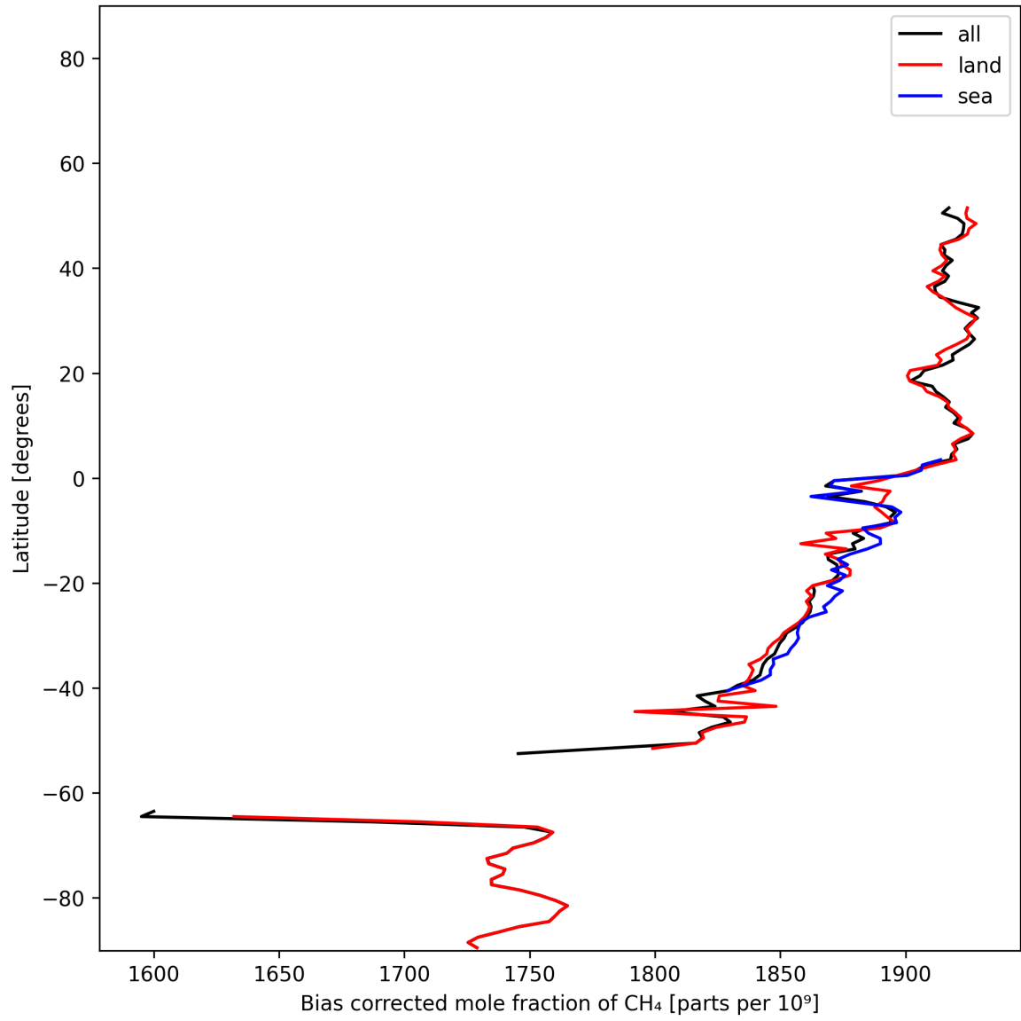
Figure 14: Zonal average of “Bias corrected mole fraction of CH 4 ” for 2024-12-27 to 2024-12-28.
