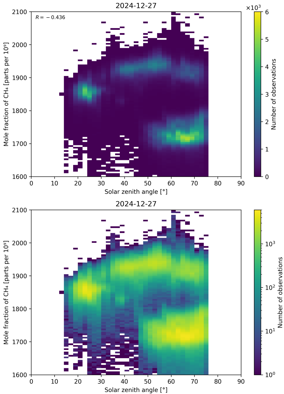
Figure 99: Scatter density plot of “Solar zenith angle” against “Mole fraction of CH 4 ” for 2024-12-27 to 2024-12-28.
