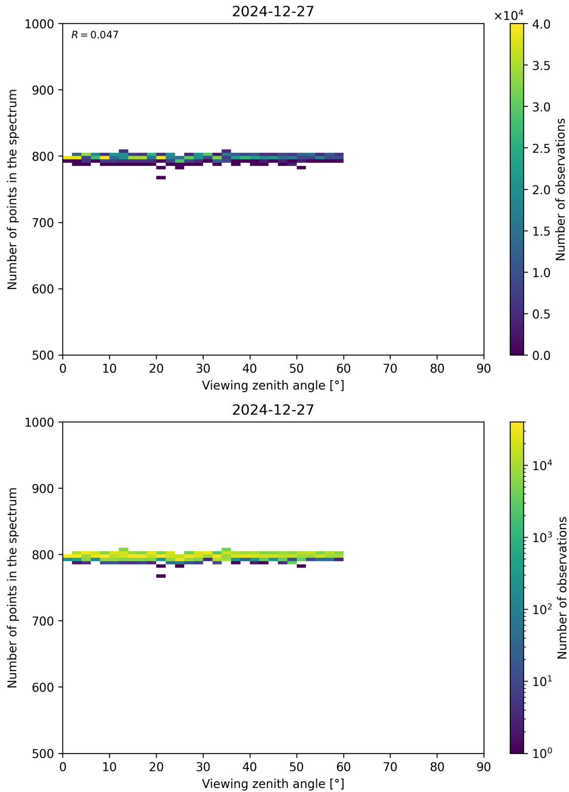
Figure 114: Scatter density plot of “Viewing zenith angle” against “Number of points in the spectrum” for 2024-12-27 to 2024-12-28.
