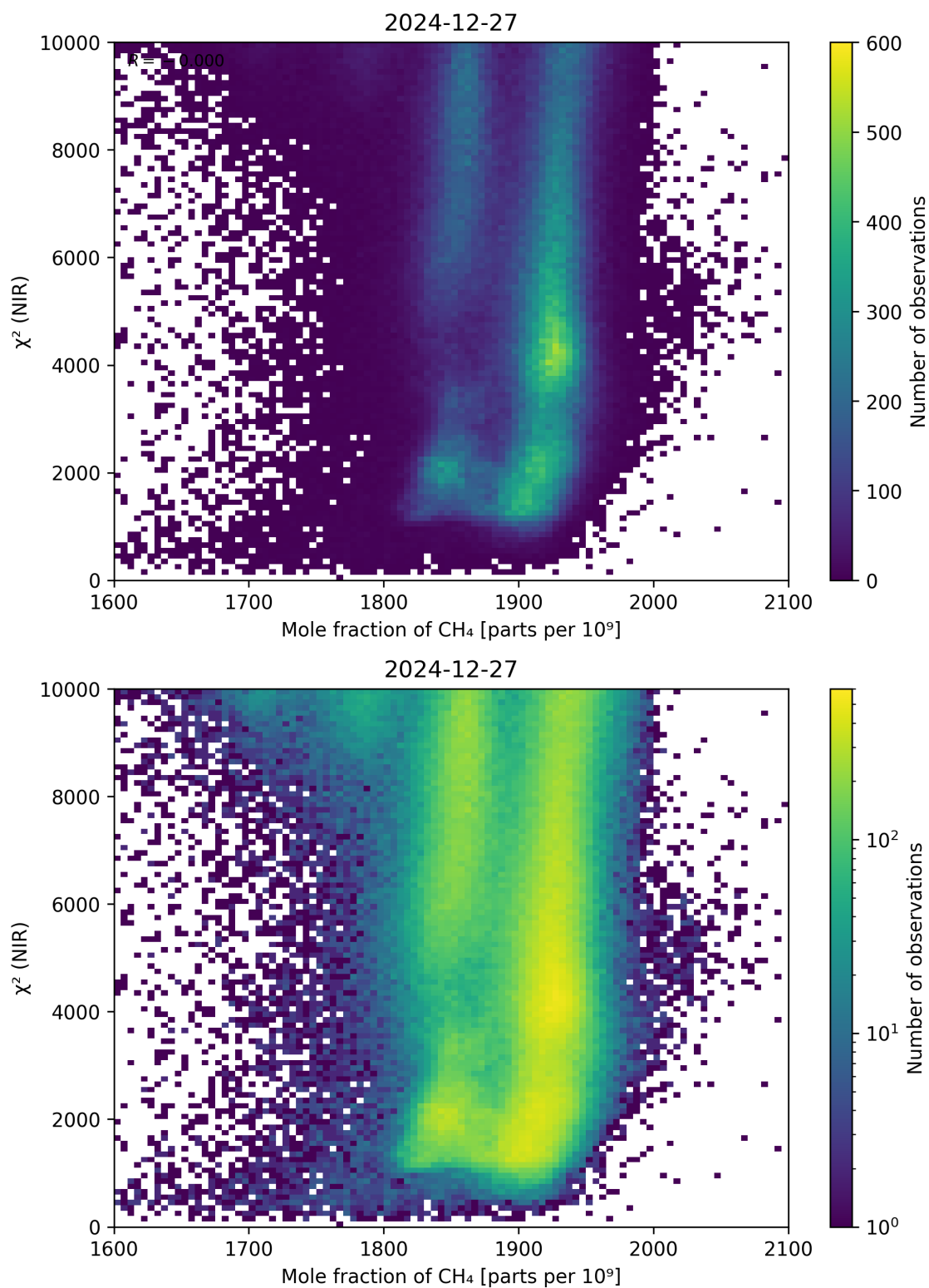
Figure 70: Scatter density plot of “Mole fraction of \text{CH}_4 ” against “ \chi^2 (NIR)” for 2024-12-27 to 2024-12-28.
