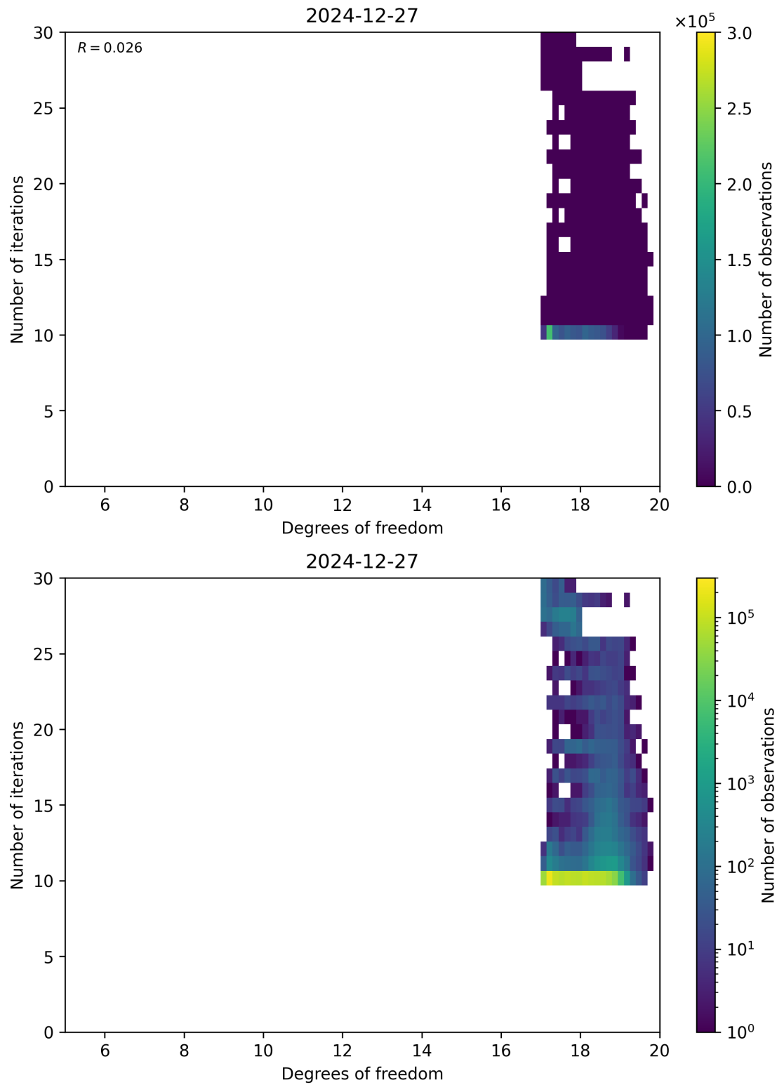
Figure 52: Scatter density plot of “Degrees of freedom” against “Number of iterations” for 2024-12-27 to 2024-12-28.
