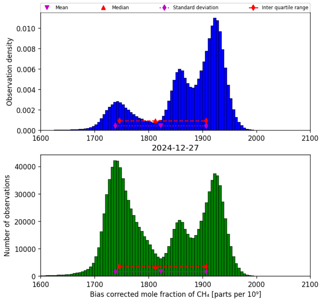
Figure 25: Histogram of “Bias corrected mole fraction of CH 4 ” for 2024-12-27 to 2024-12-28
