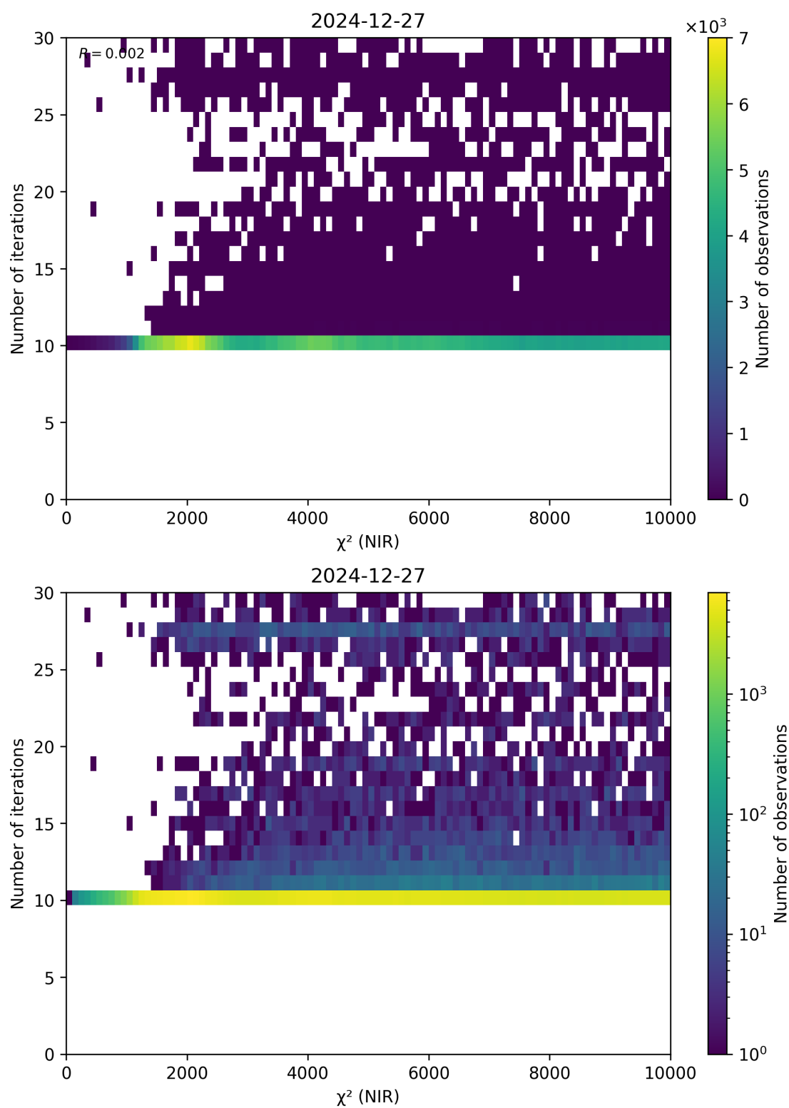
Figure 46: Scatter density plot of “ \chi^2 (NIR)” against “Number of iterations” for 2024-12-27 to 2024-12-28.
