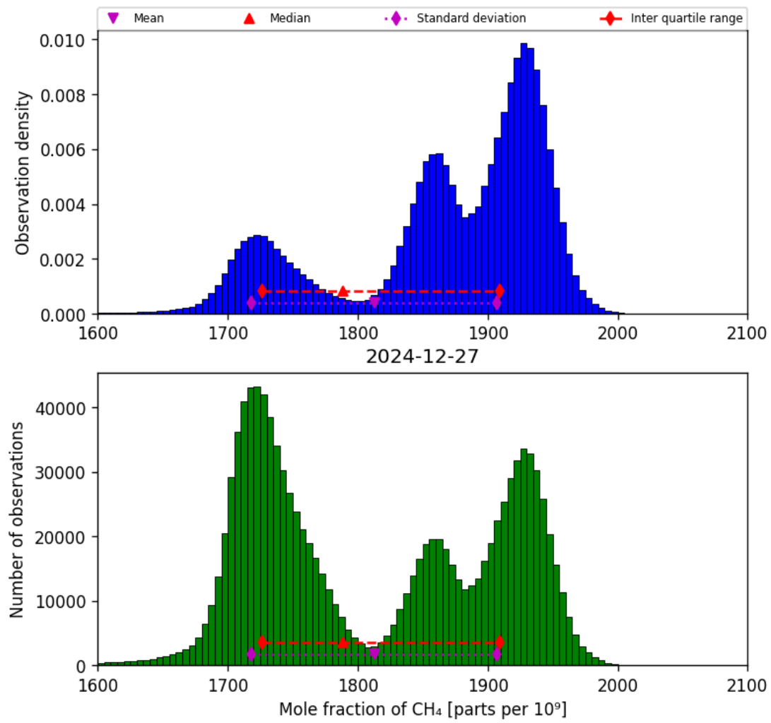
Figure 23: Histogram of “Mole fraction of CH 4 ” for 2024-12-27 to 2024-12-28
