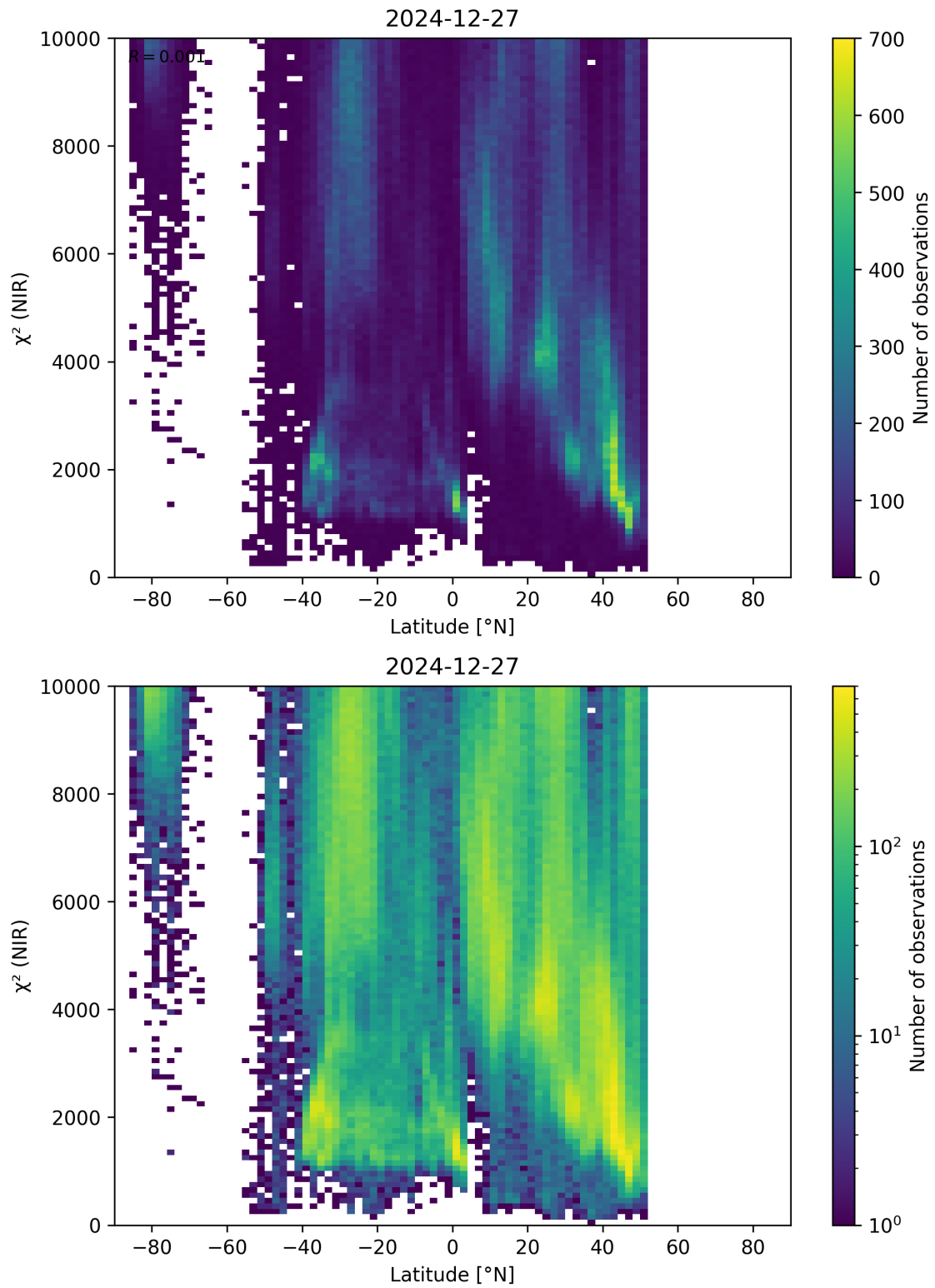
Figure 53: Scatter density plot of “Latitude” against “ \chi^2 (NIR)” for 2024-12-27 to 2024-12-28.
