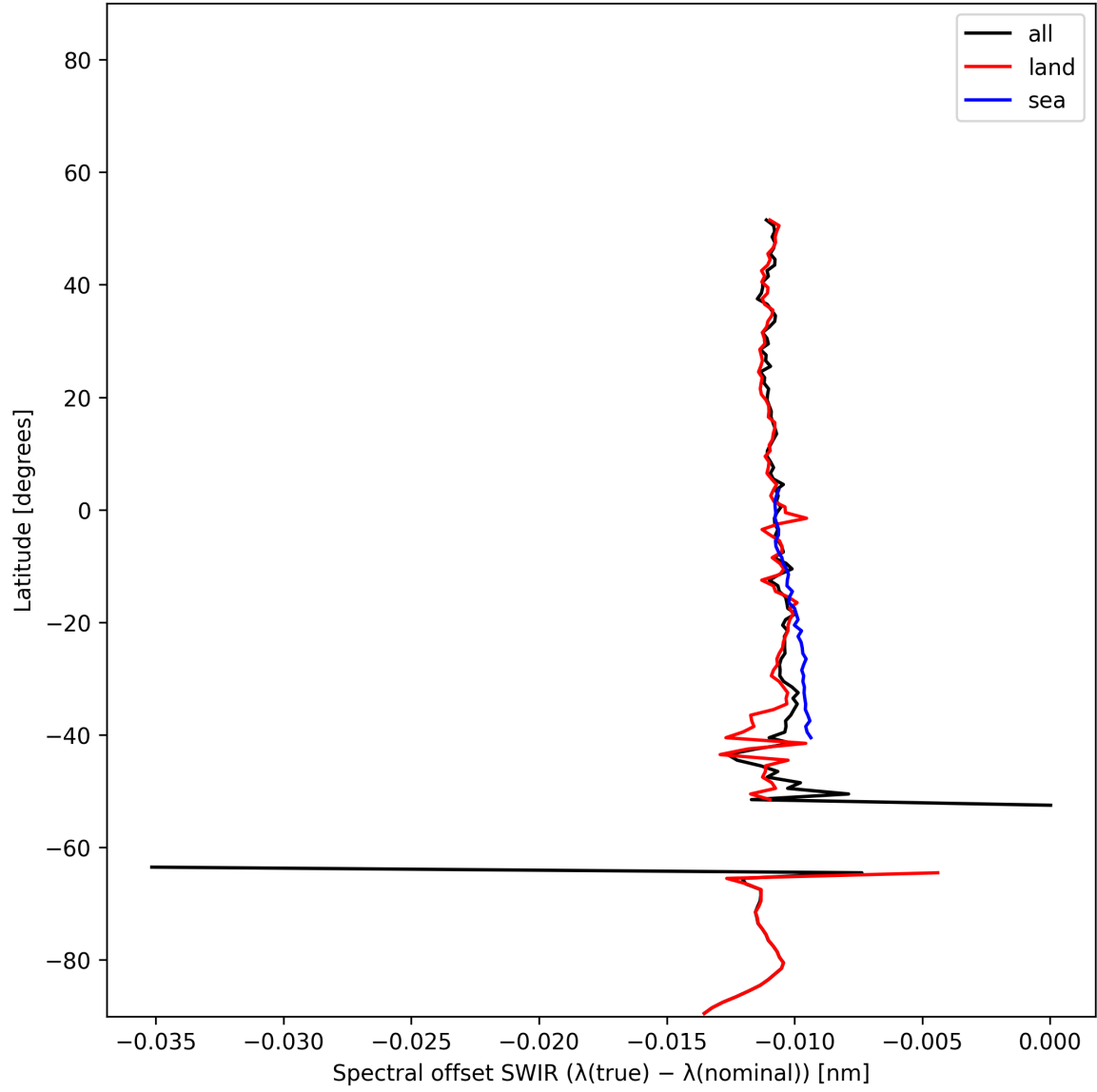
Figure 16: Zonal average of “Spectral offset SWIR ( \lambda_{\text{true}} - \lambda_{\text{nominal}} )” for 2024-12-27 to 2024-12-28.
