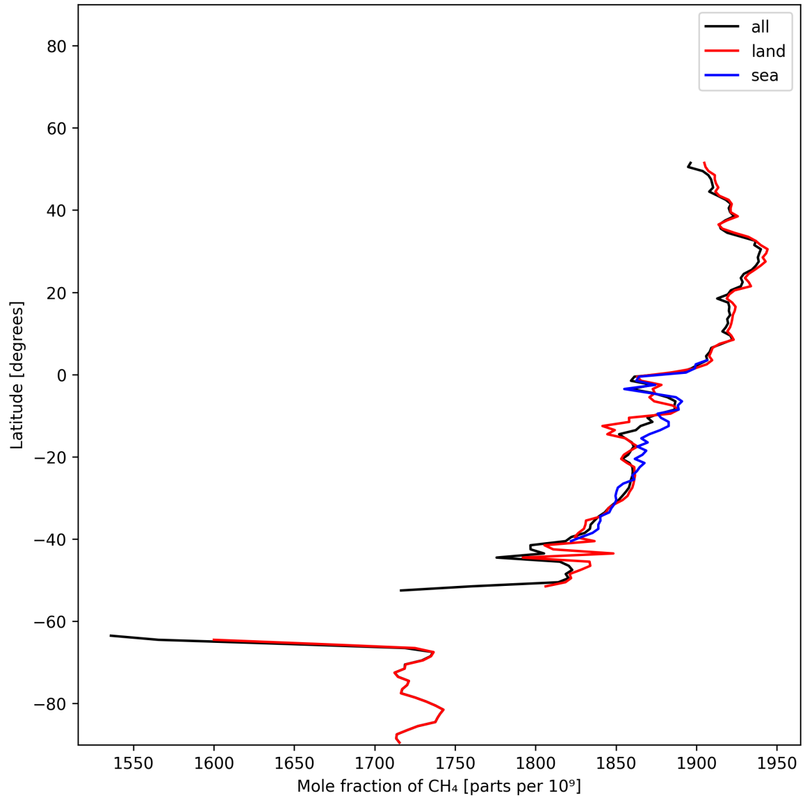
Figure 12: Zonal average of “Mole fraction of CH 4 ” for 2024-12-27 to 2024-12-28.
