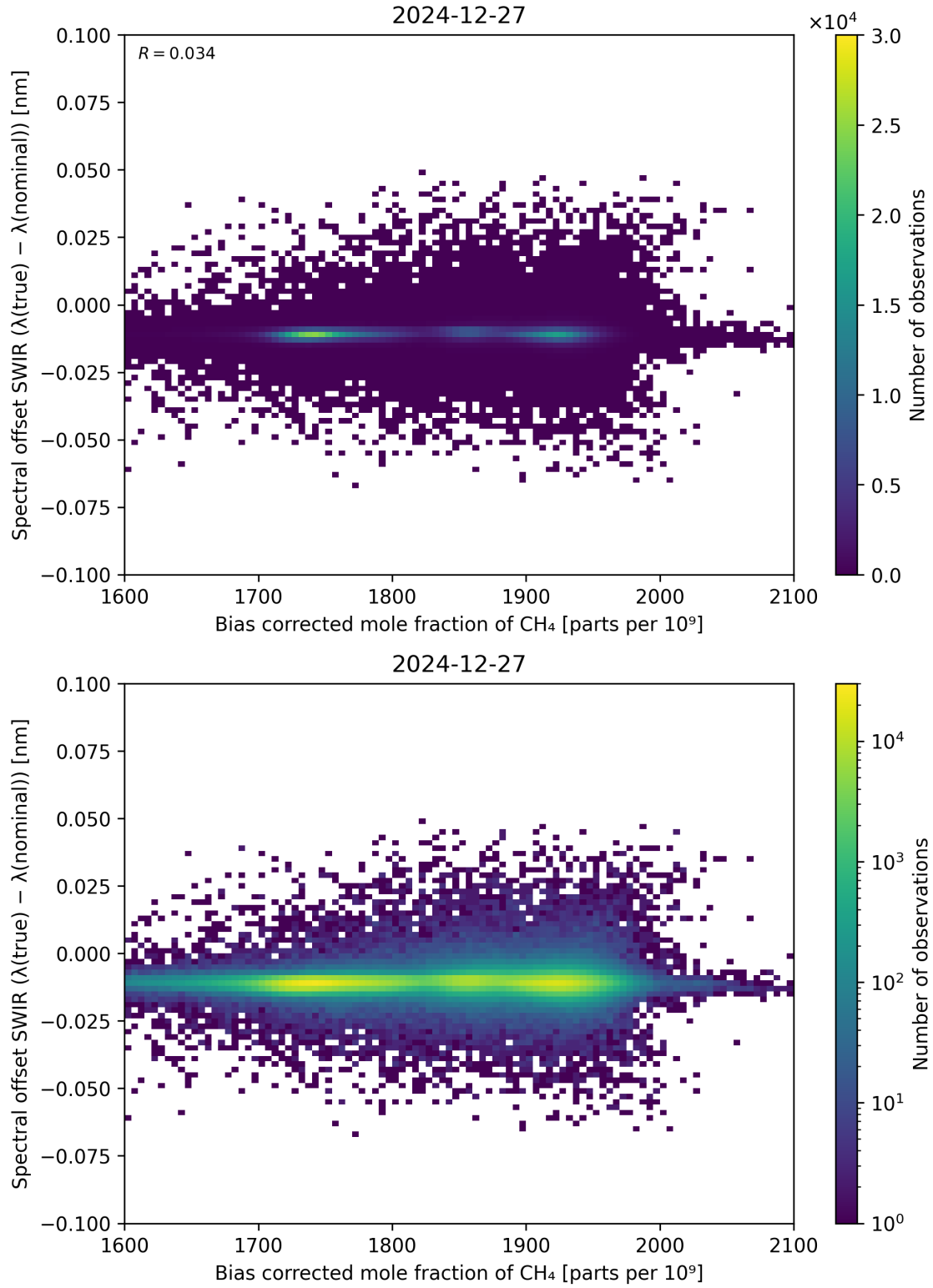
Figure 69: Scatter density plot of “Bias corrected mole fraction of \text{CH}_4 ” against “Spectral offset SWIR ( \lambda_{\text{true}} - \lambda_{\text{nominal}} )” for 2024-12-27 to 2024-12-28.
