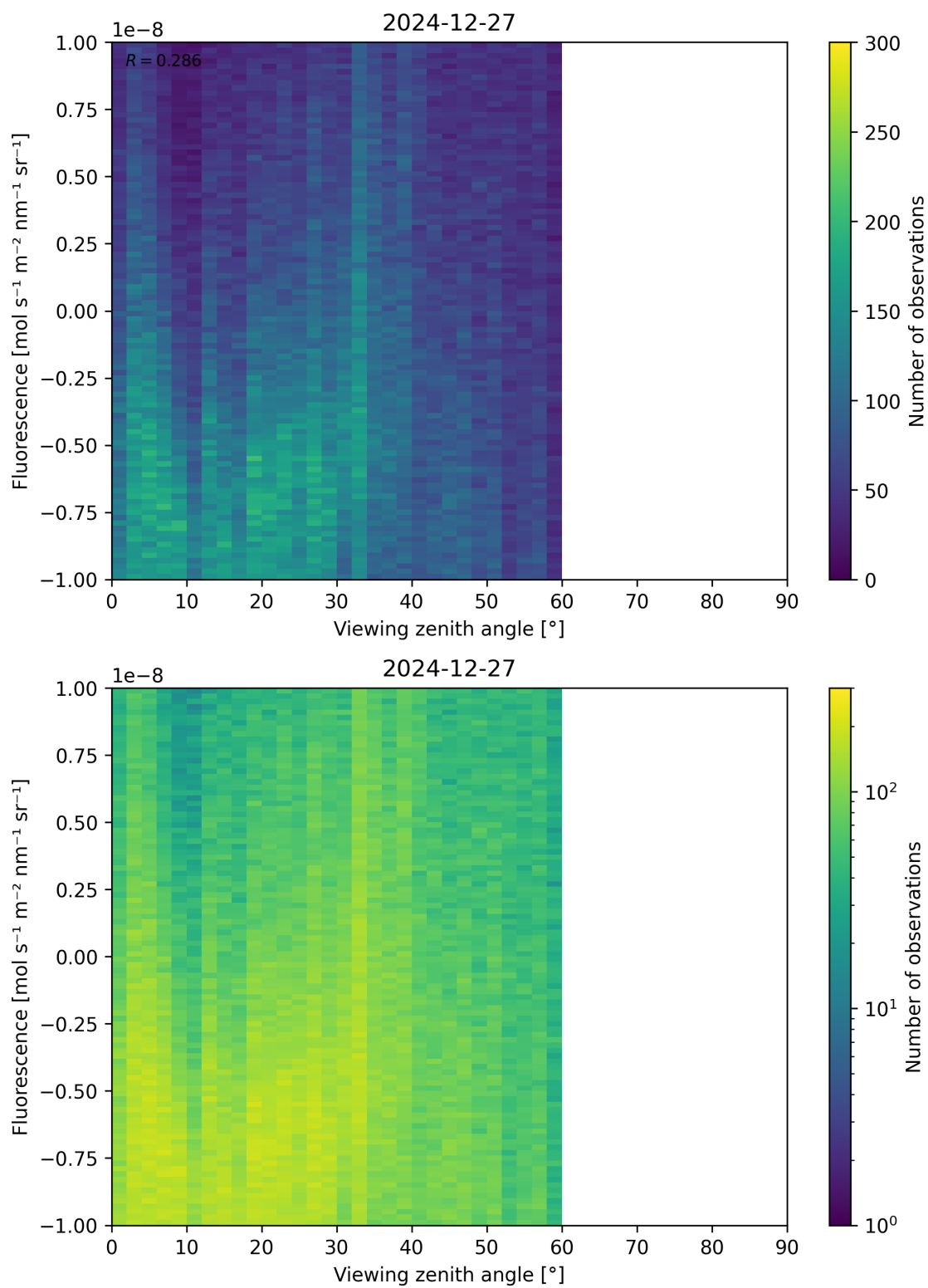
Figure 108: Scatter density plot of “Viewing zenith angle” against “Fluorescence” for 2024-12-27 to 2024-12-28.
