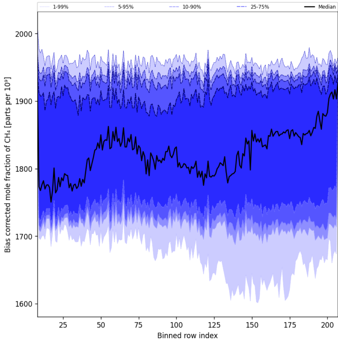
Figure 36: Along track statistics of “Bias corrected mole fraction of CH 4 ” for 2024-12-27 to 2024-12-28
