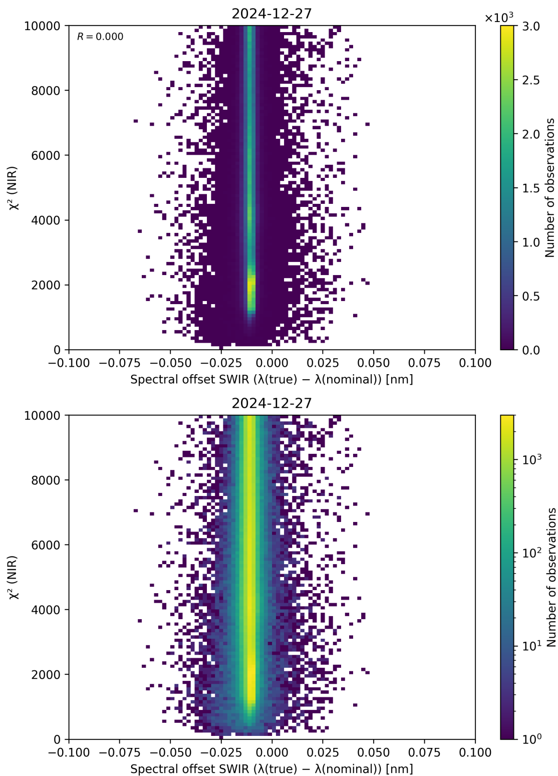
Figure 117: Scatter density plot of “Spectral offset SWIR ( \lambda_{\text{true}} - \lambda_{\text{nominal}} )” against “ \chi^2 (NIR)” for 2024-12-27 to 2024-12-28.
