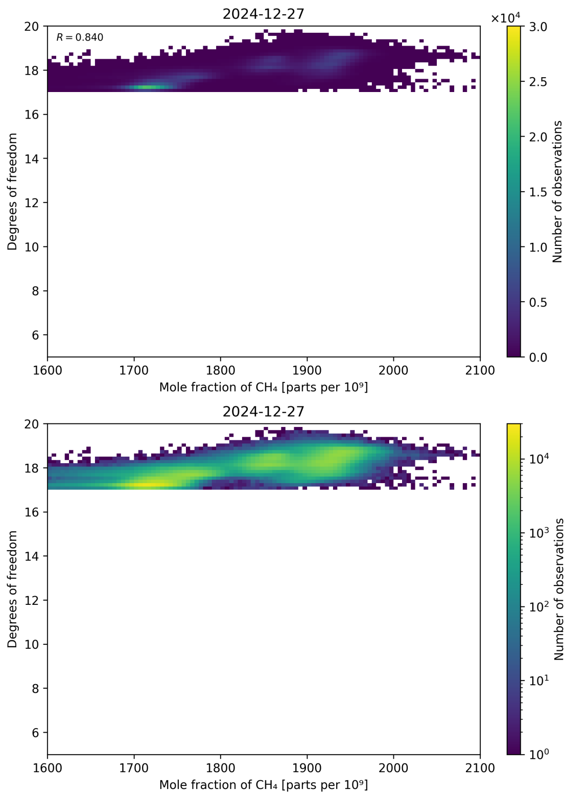
Figure 72: Scatter density plot of “Mole fraction of CH 4 ” against “Degrees of freedom” for 2024-12-27 to 2024-12-28.
