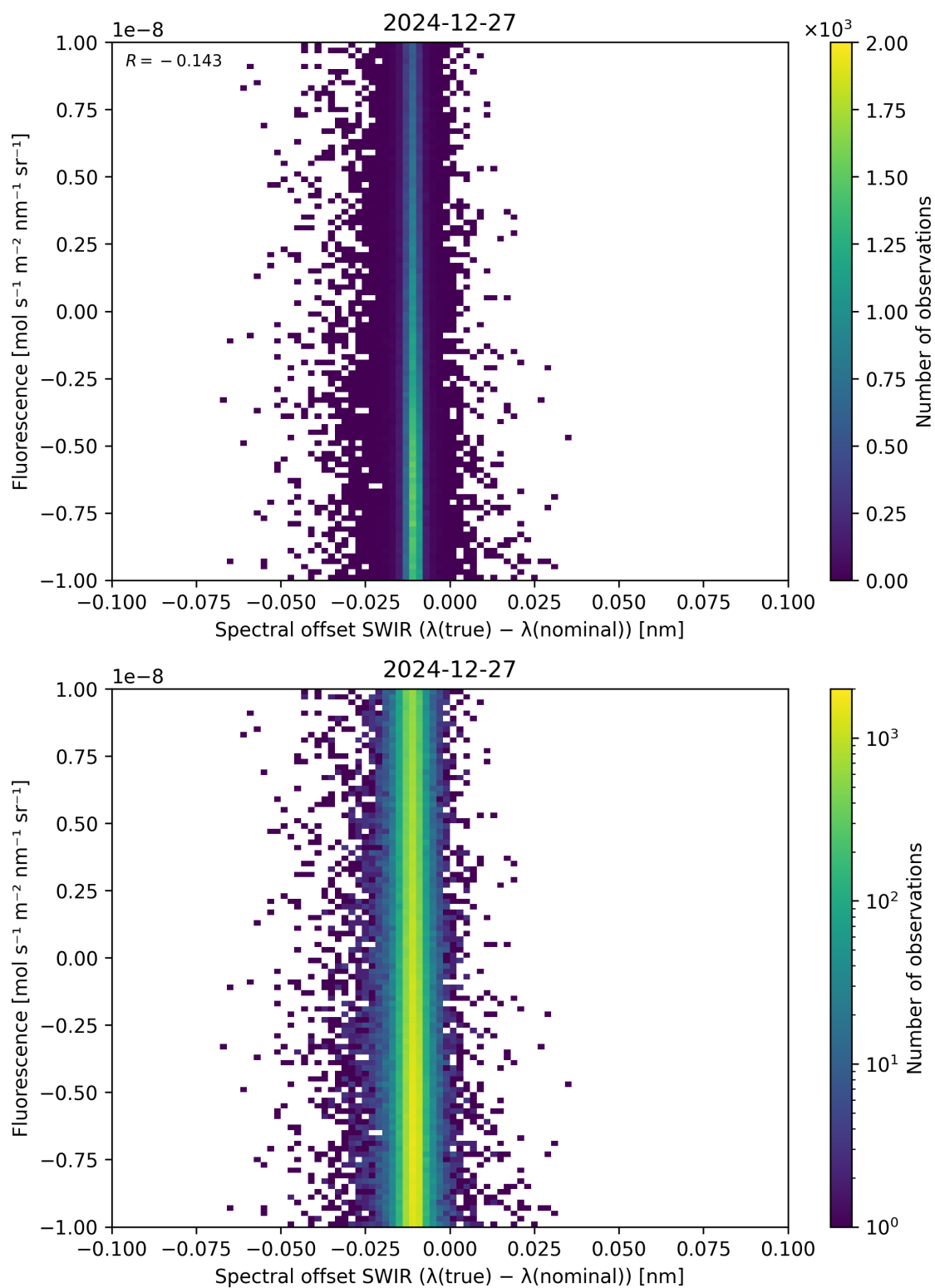
Figure 120: Scatter density plot of “Spectral offset SWIR ( \lambda_{\text{true}} - \lambda_{\text{nominal}} )” against “Fluorescence” for 2024-12-27 to 2024-12-28.
