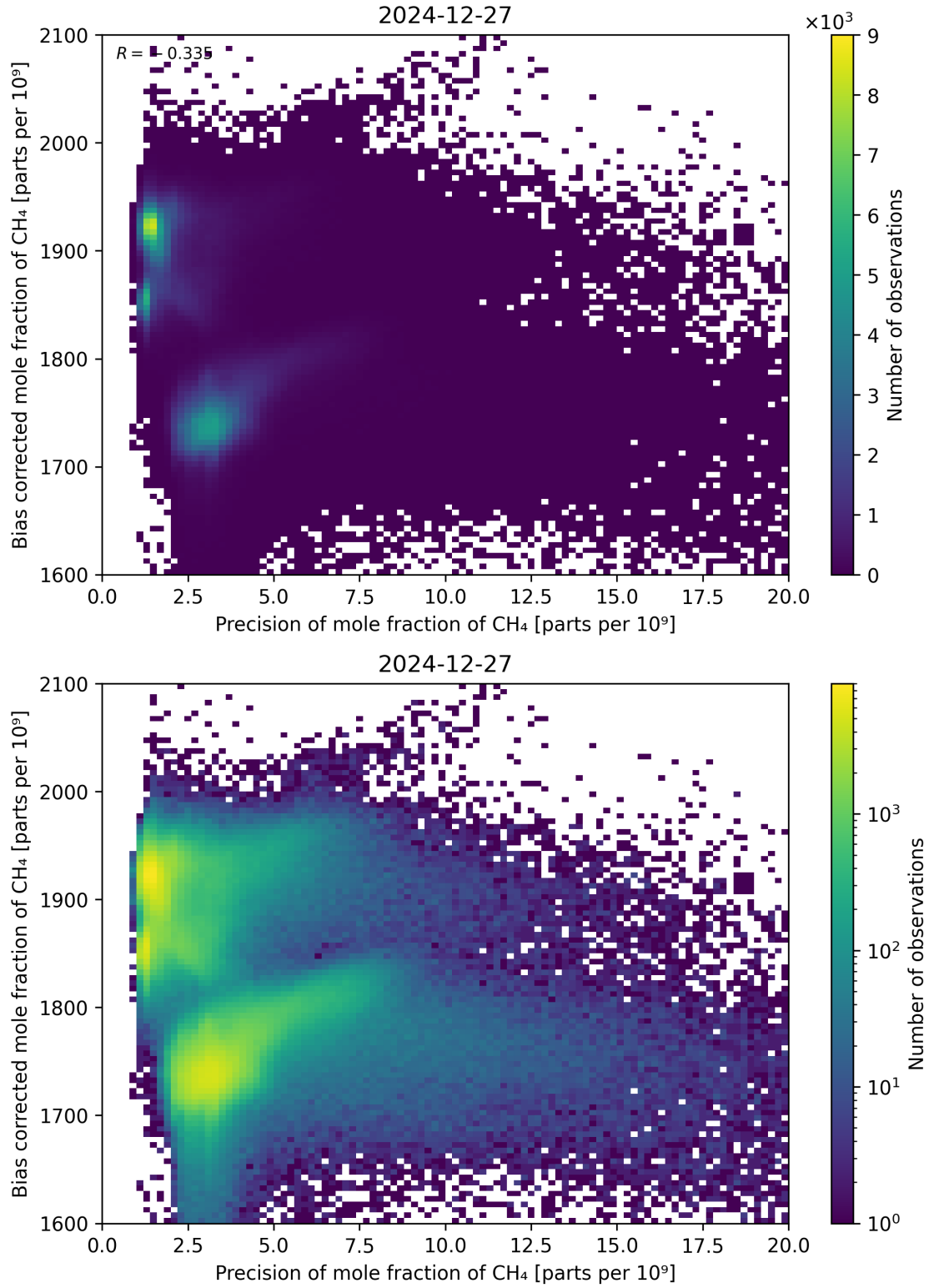
Figure 82: Scatter density plot of “Precision of mole fraction of \text{CH}_4 ” against “Bias corrected mole fraction of \text{CH}_4 ” for 2024-12-27 to 2024-12-28.
