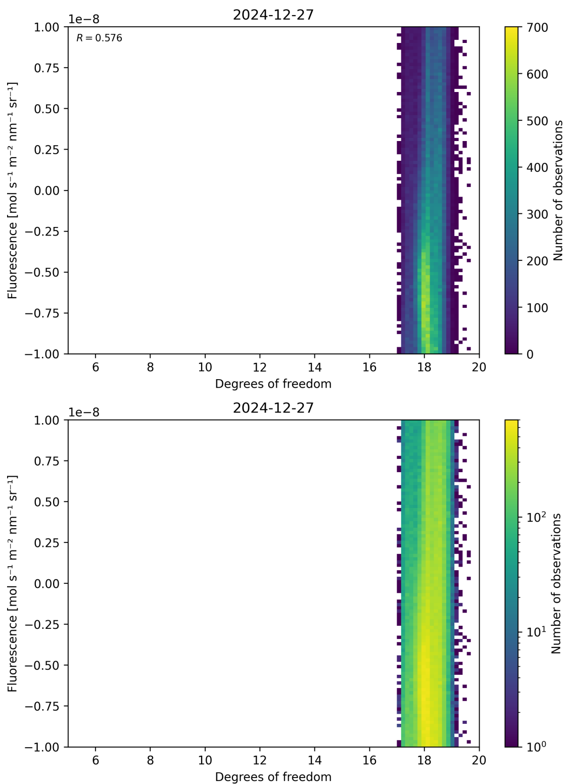
Figure 51: Scatter density plot of “Degrees of freedom” against “Fluorescence” for 2024-12-27 to 2024-12-28.
