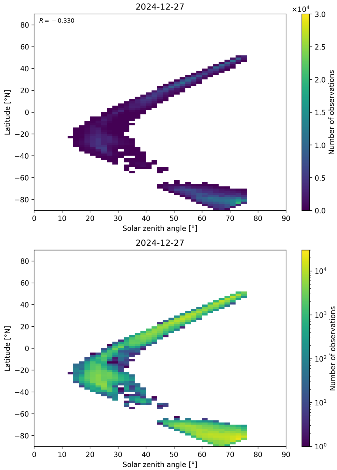
Figure 98: Scatter density plot of “Solar zenith angle” against “Latitude” for 2024-12-27 to 2024-12-28.
