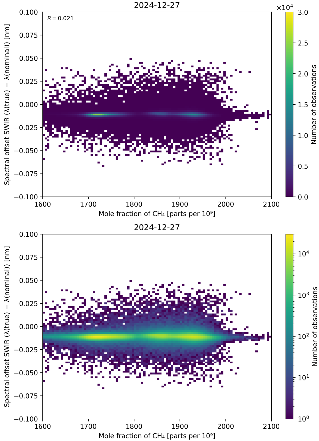
Figure 86: Scatter density plot of “Mole fraction of CH 4 ” against “Spectral offset SWIR ( \lambda_{\text{true}} - \lambda_{\text{nominal}} )” for 2024-12-27 to 2024-12-28.
