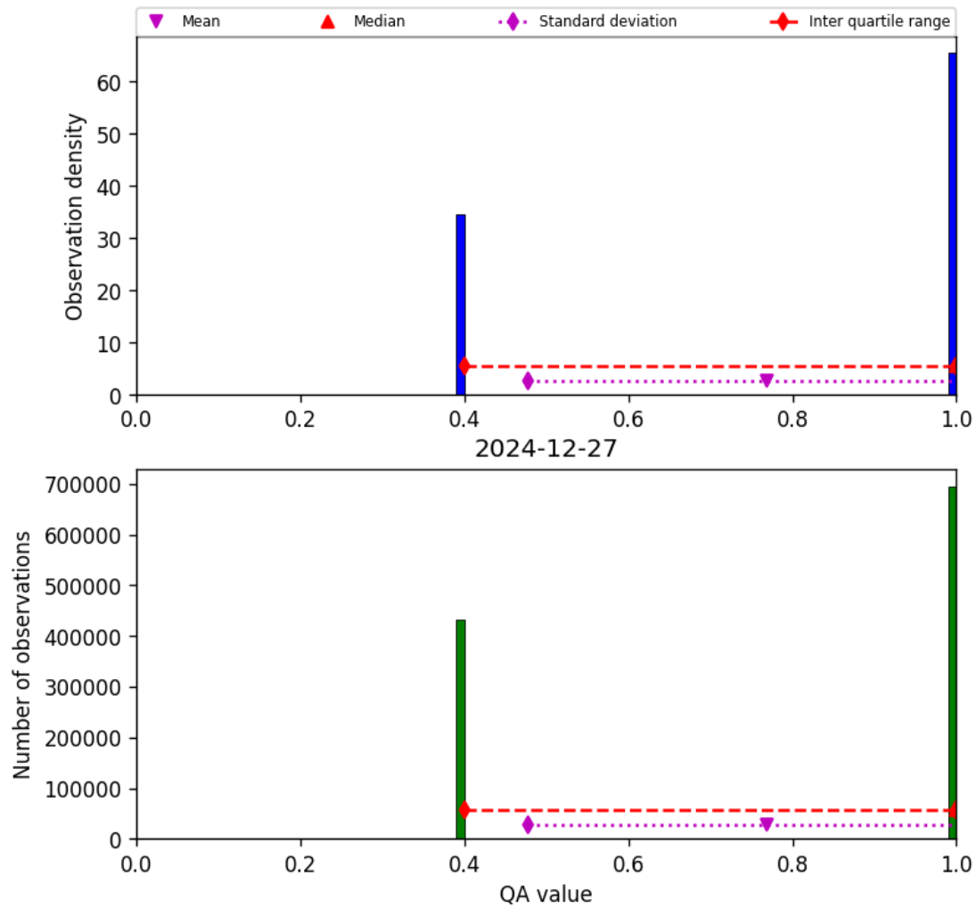
Figure 22: Histogram of “QA value” for 2024-12-27 to 2024-12-28
