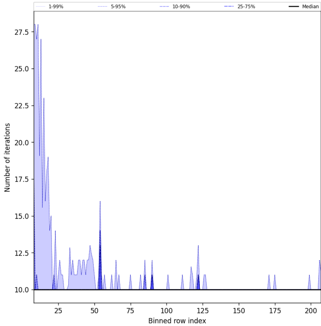
Figure 42: Along track statistics of “Number of iterations” for 2024-12-27 to 2024-12-28
