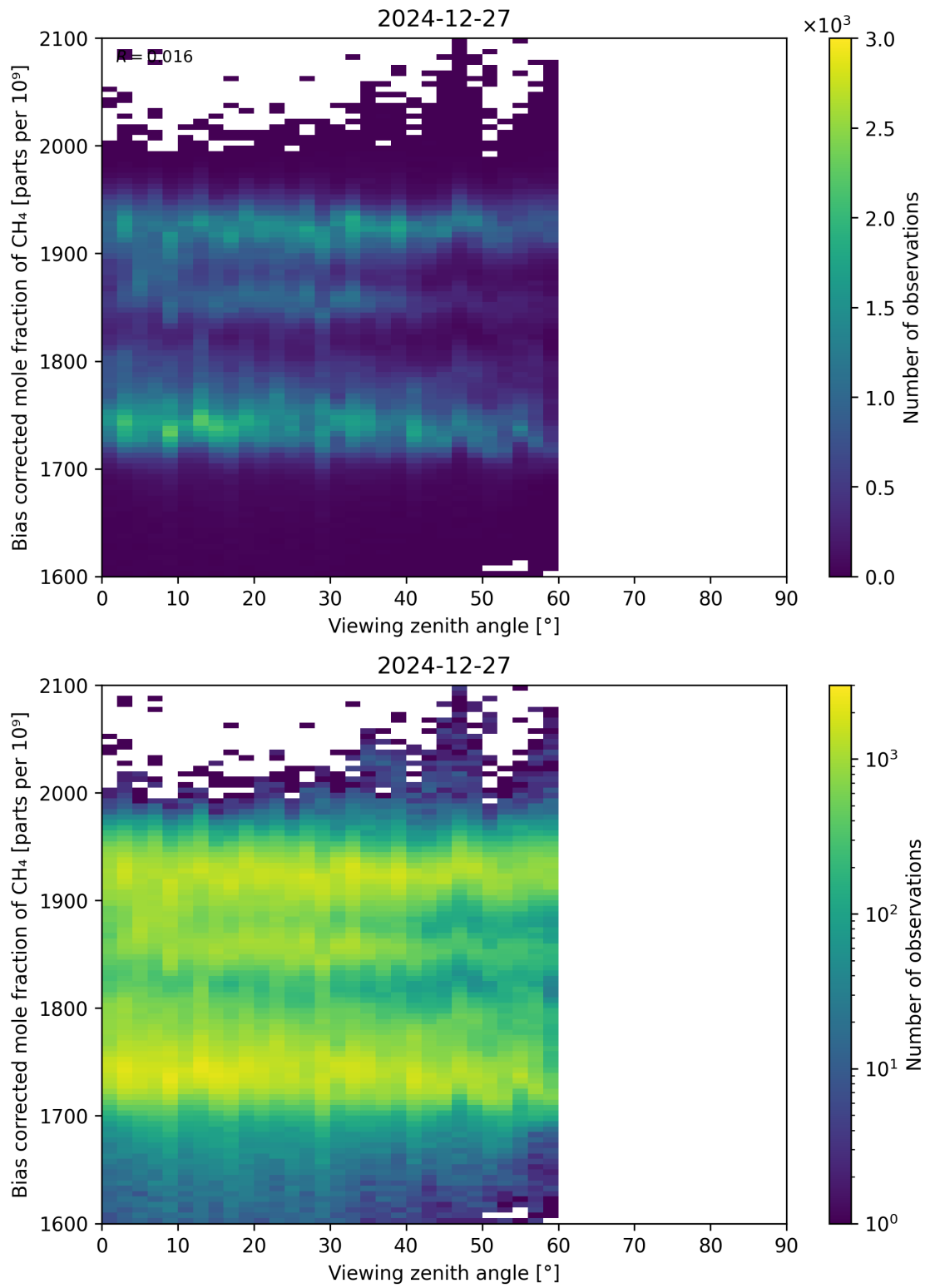
Figure 111: Scatter density plot of “Viewing zenith angle” against “Bias corrected mole fraction of CH 4 ” for 2024-12-27 to 2024-12-28.
