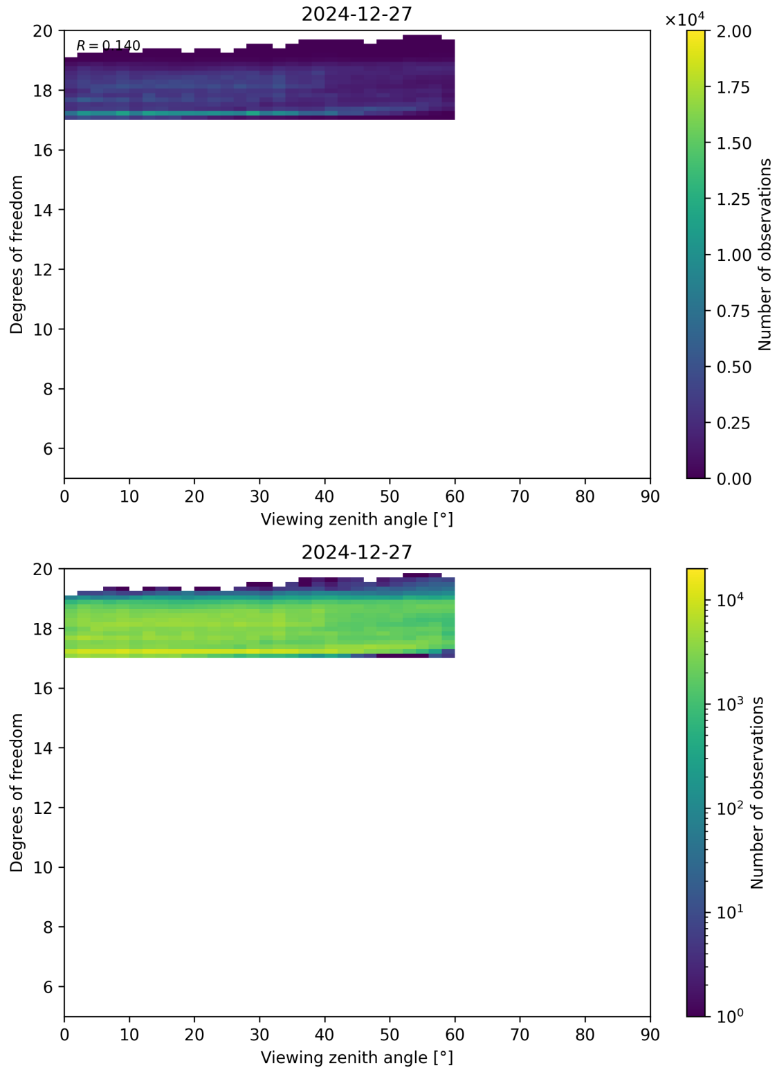
Figure 107: Scatter density plot of “Viewing zenith angle” against “Degrees of freedom” for 2024-12-27 to 2024-12-28.
