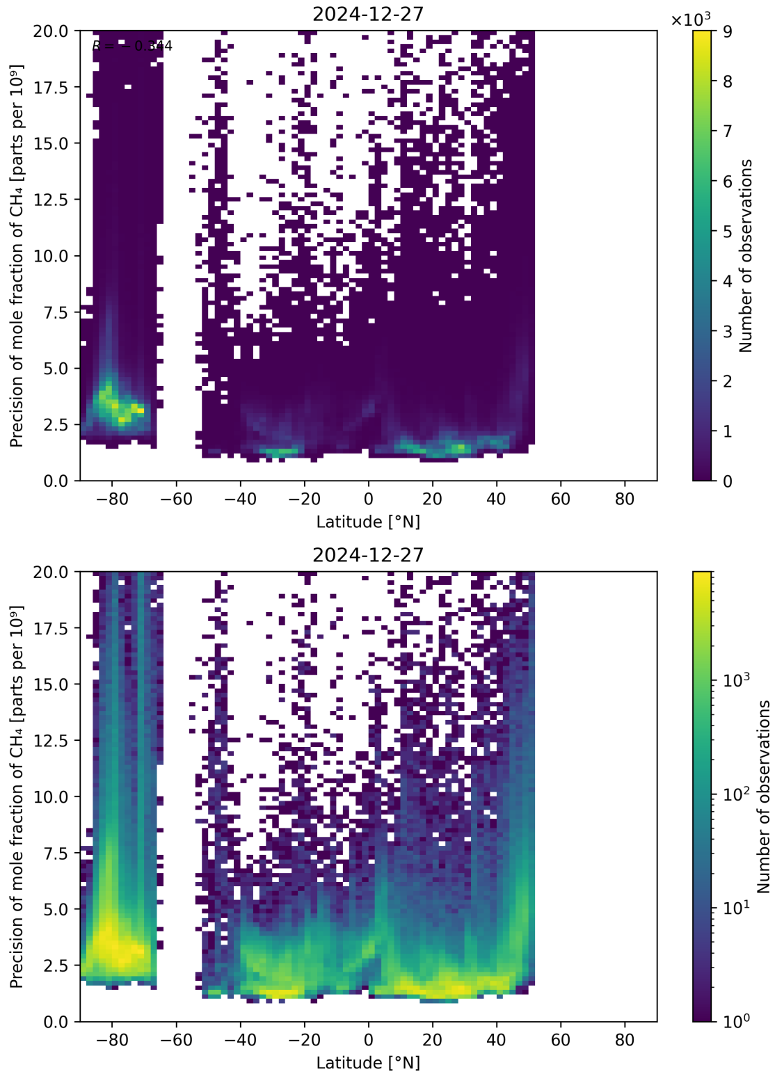
Figure 59: Scatter density plot of “Latitude” against “Precision of mole fraction of CH 4 ” for 2024-12-27 to 2024-12-28.
