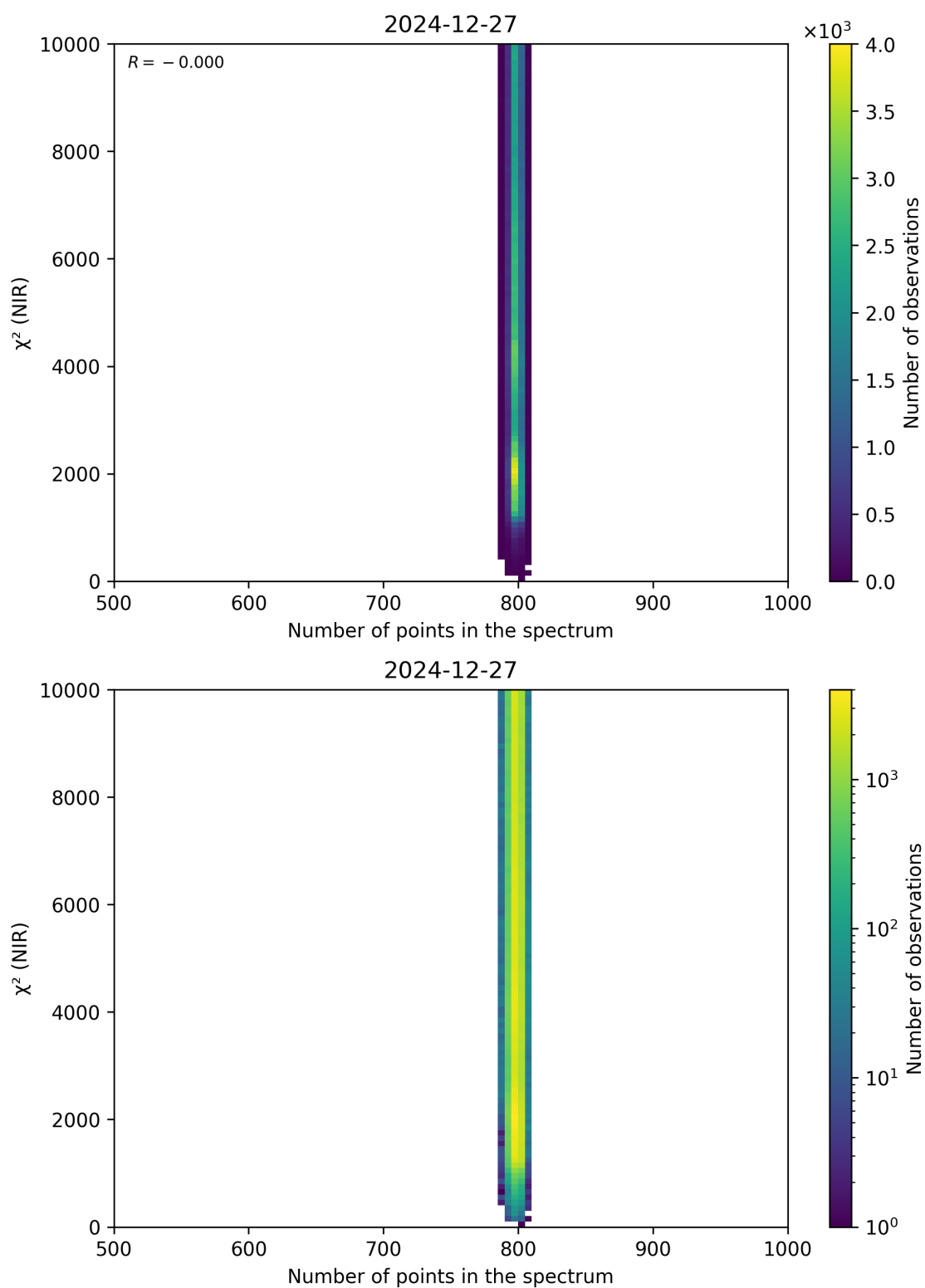
Figure 88: Scatter density plot of “Number of points in the spectrum” against “ \chi^2 (NIR)” for 2024-12-27 to 2024-12-28.
