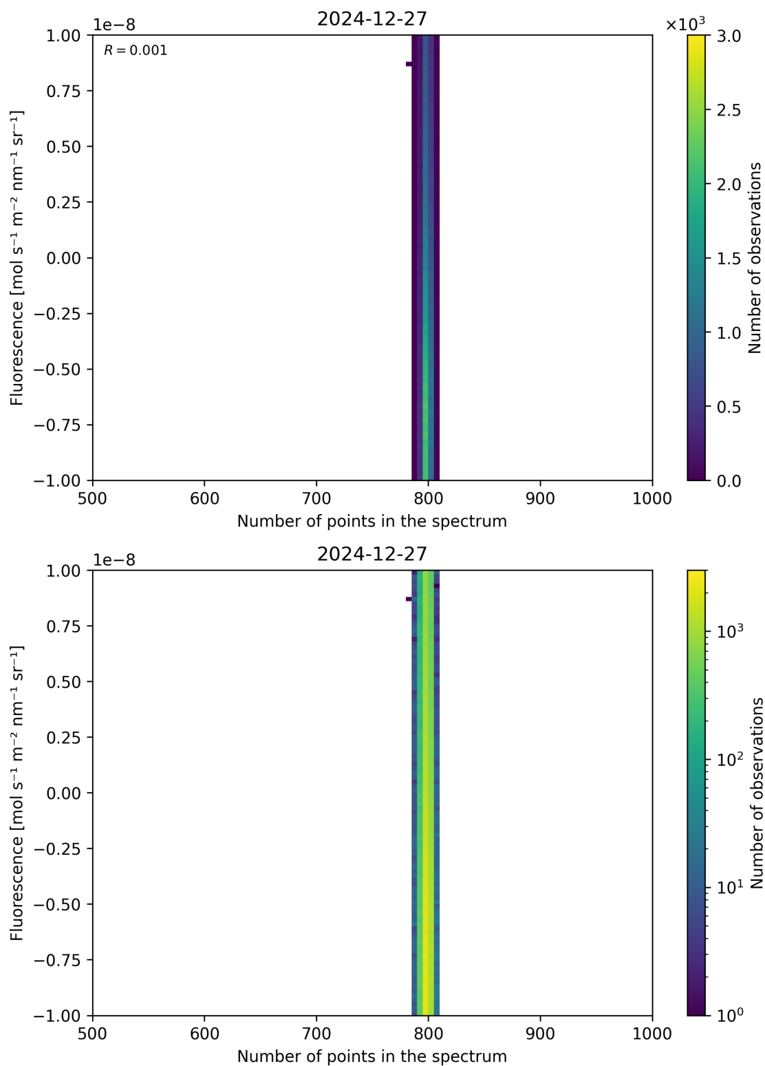
Figure 91: Scatter density plot of “Number of points in the spectrum” against “Fluorescence” for 2024-12-27 to 2024-12-28.
