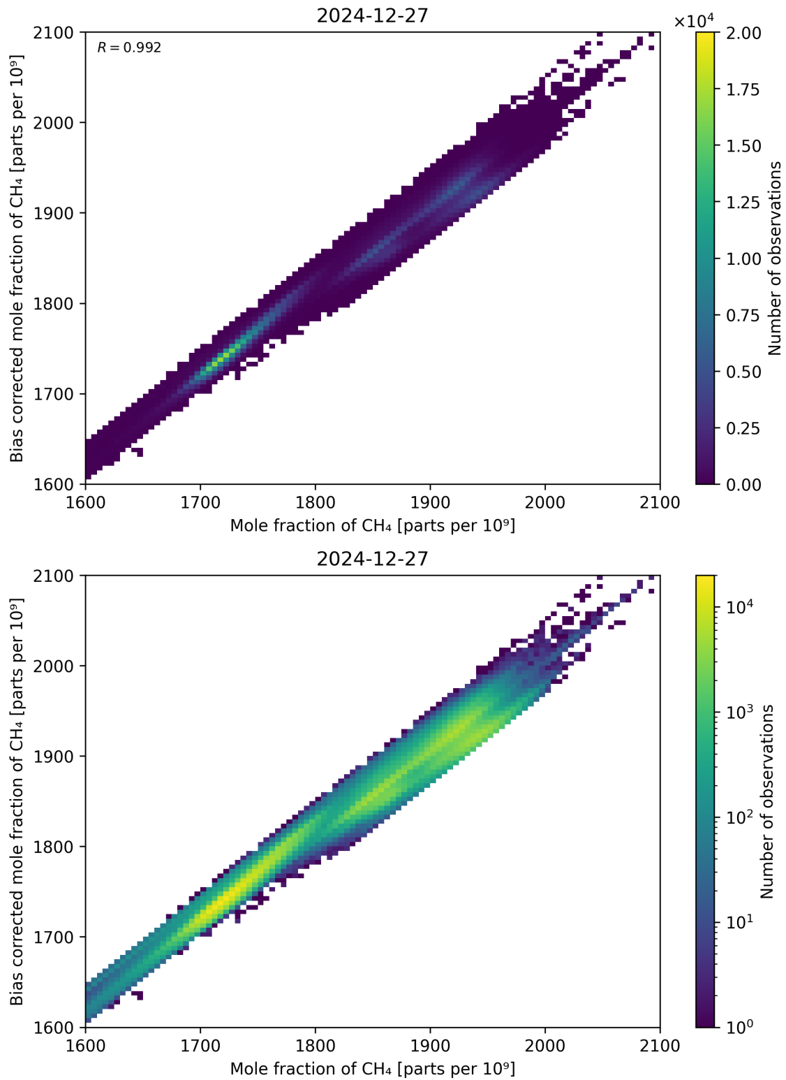
Figure 74: Scatter density plot of “Mole fraction of CH 4 ” against “Bias corrected mole fraction of CH 4 ” for 2024-12-27 to 2024-12-28.
