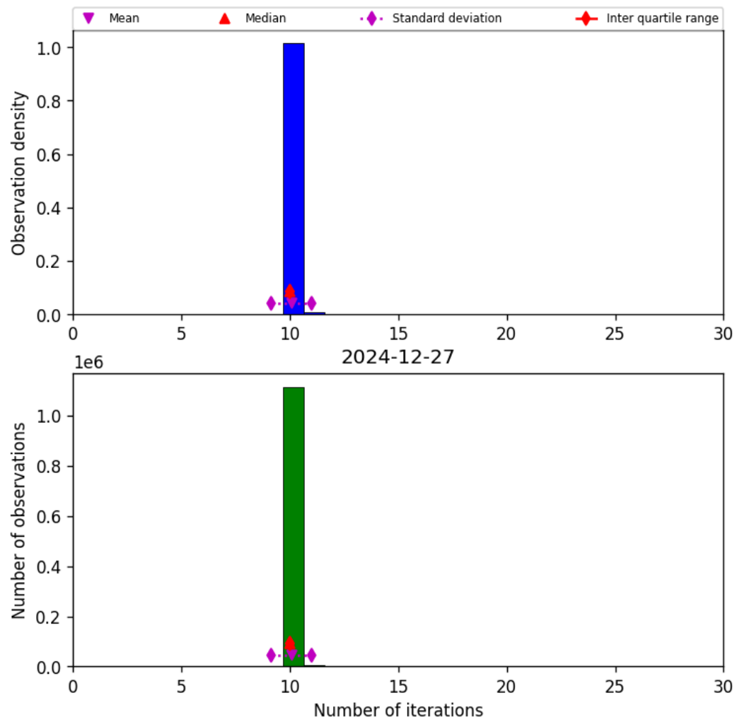
Figure 31: Histogram of “Number of iterations” for 2024-12-27 to 2024-12-28
