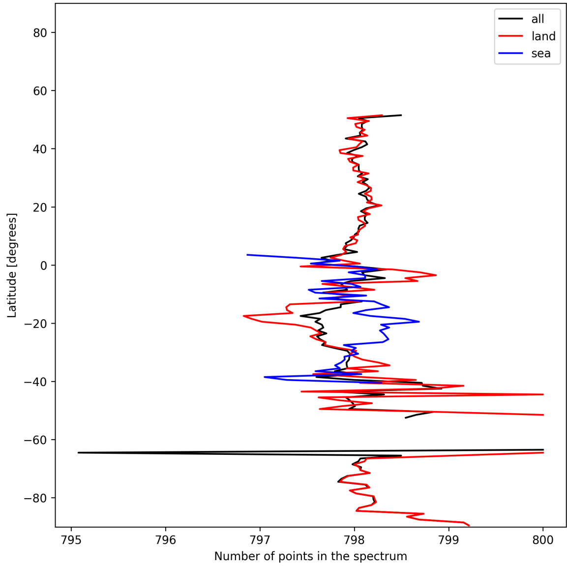
Figure 15: Zonal average of “Number of points in the spectrum” for 2024-12-27 to 2024-12-28.
