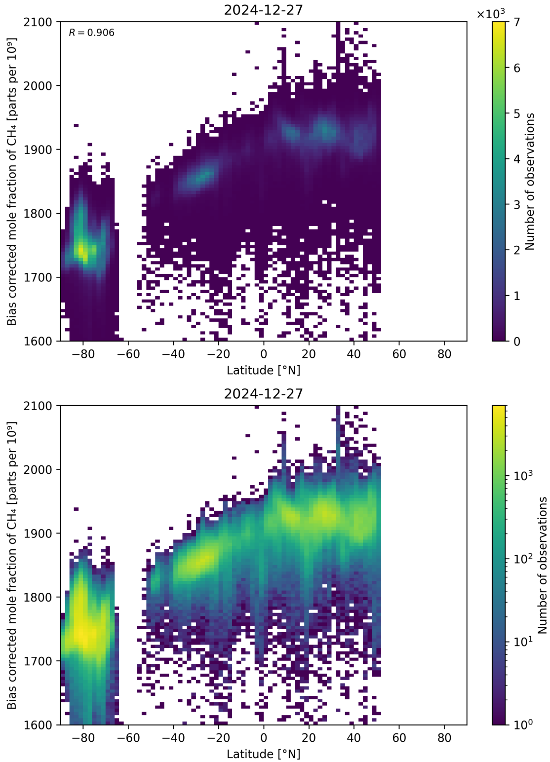
Figure 58: Scatter density plot of “Latitude” against “Bias corrected mole fraction of CH 4 ” for 2024-12-27 to 2024-12-28.
