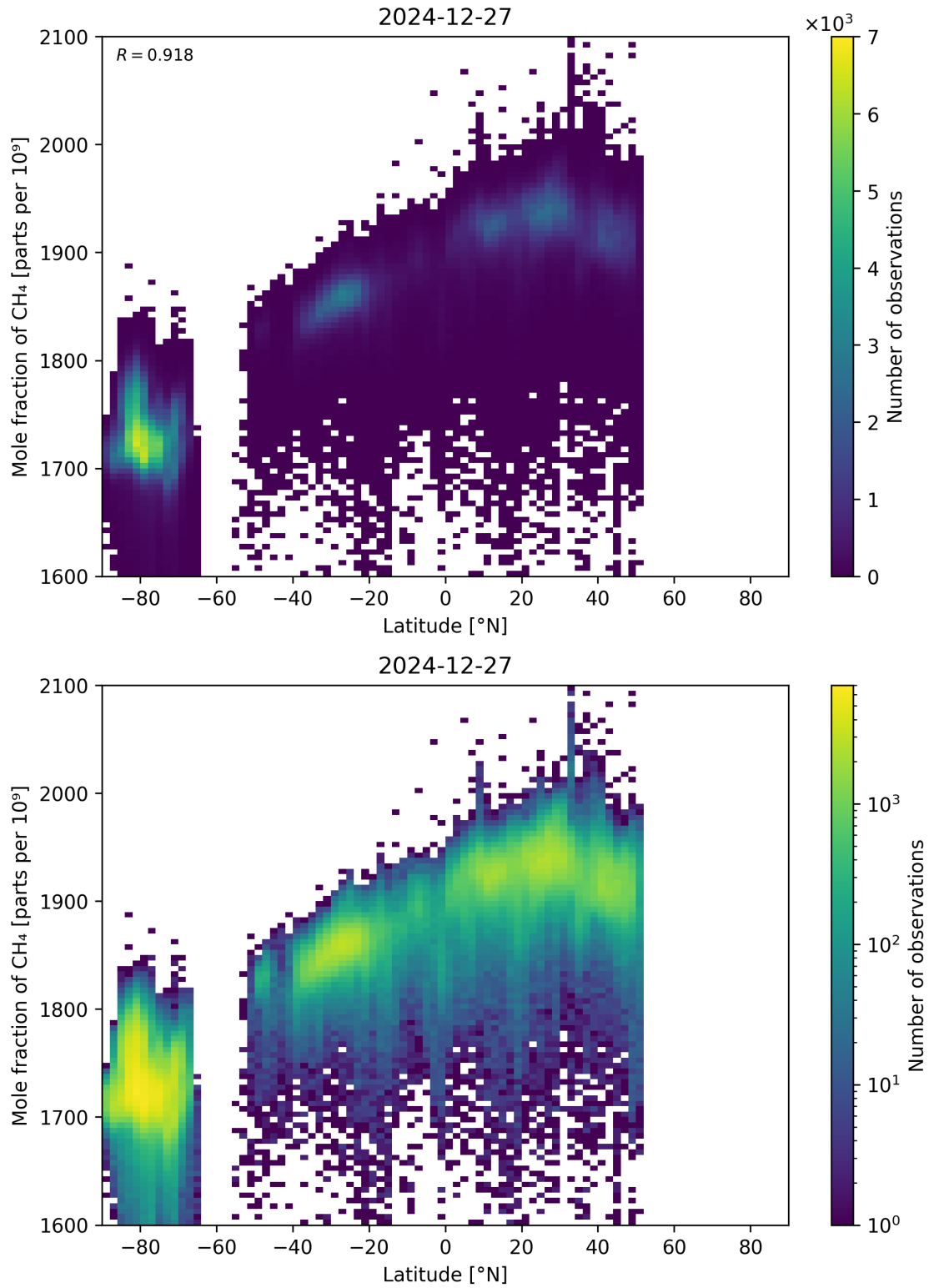
Figure 57: Scatter density plot of “Latitude” against “Mole fraction of CH 4 ” for 2024-12-27 to 2024-12-28.
