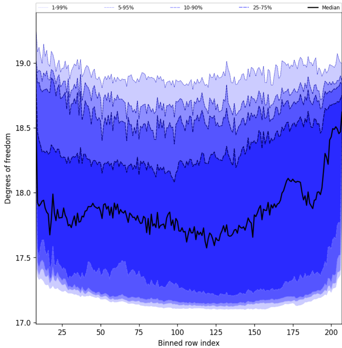
Figure 41: Along track statistics of “Degrees of freedom” for 2024-12-27 to 2024-12-28
