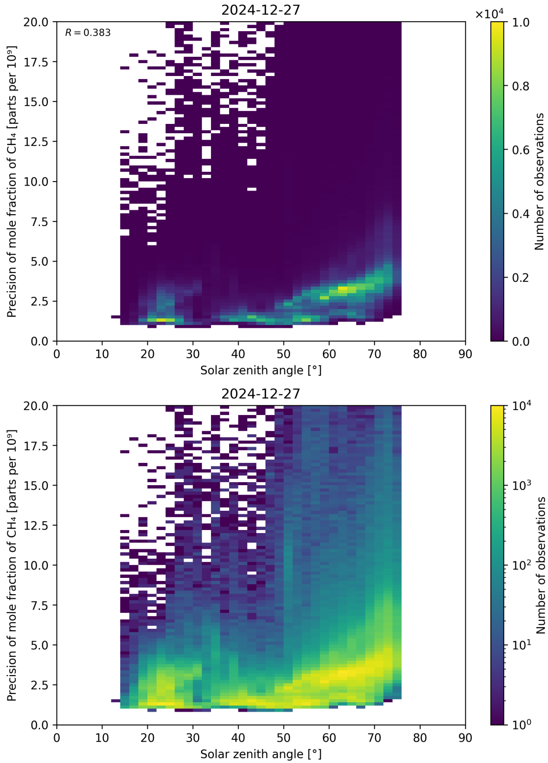
Figure 101: Scatter density plot of “Solar zenith angle” against “Precision of mole fraction of CH 4 ” for 2024-12-27 to 2024-12-28.
