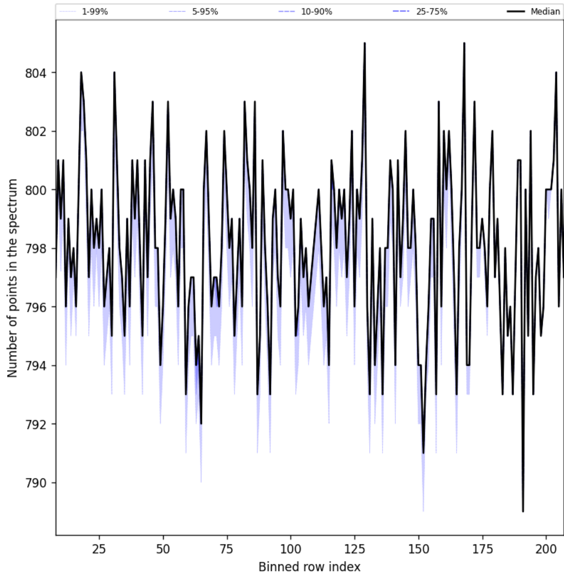
Figure 37: Along track statistics of “Number of points in the spectrum” for 2024-12-27 to 2024-12-28
