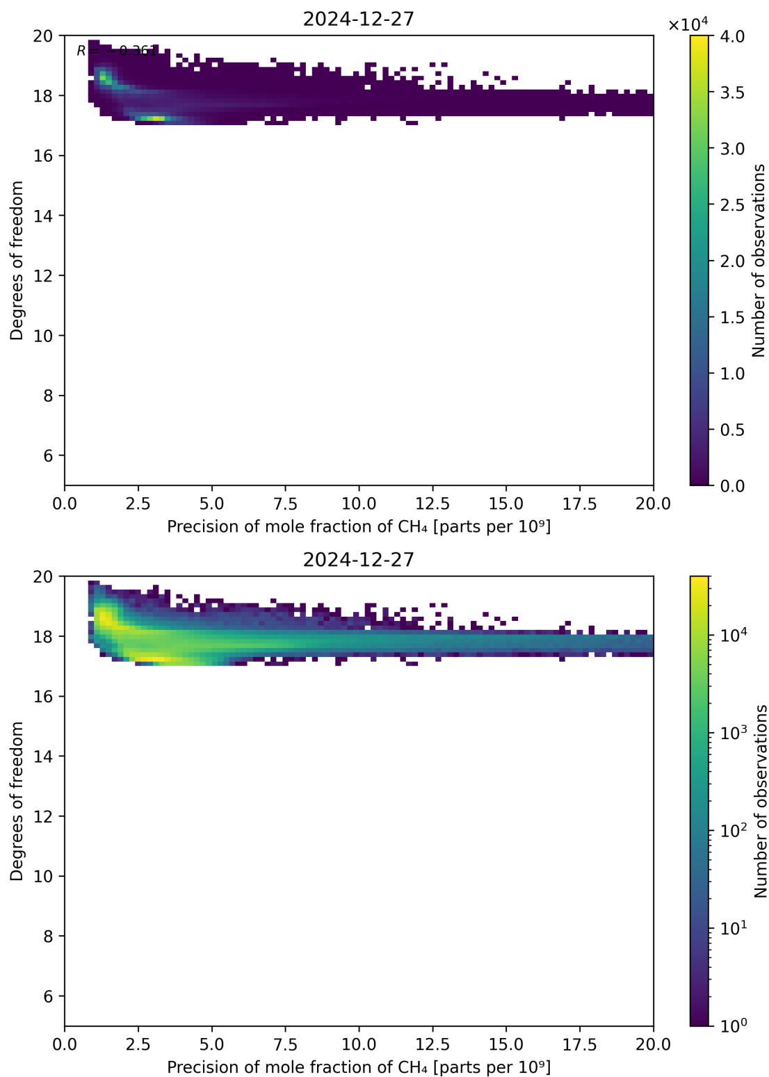
Figure 80: Scatter density plot of “Precision of mole fraction of \text{CH}_4 ” against “Degrees of freedom” for 2024-12-27 to 2024-12-28.
