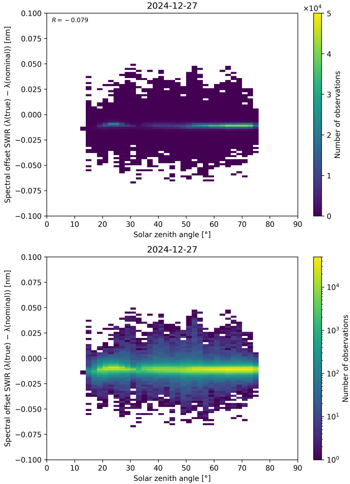
Figure 104: Scatter density plot of “Solar zenith angle” against “Spectral offset SWIR ( \lambda_{\text{true}} - \lambda_{\text{nominal}} )” for 2024-12-27 to 2024-12-28.
