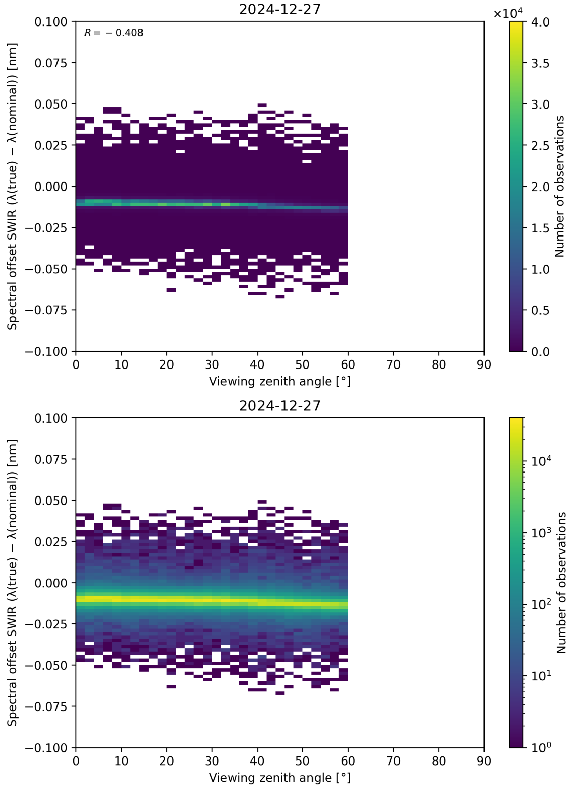
Figure 116: Scatter density plot of “Viewing zenith angle” against “Spectral offset SWIR ( \lambda_{\text{true}} - \lambda_{\text{nominal}} )” for 2024-12-27 to 2024-12-28.
