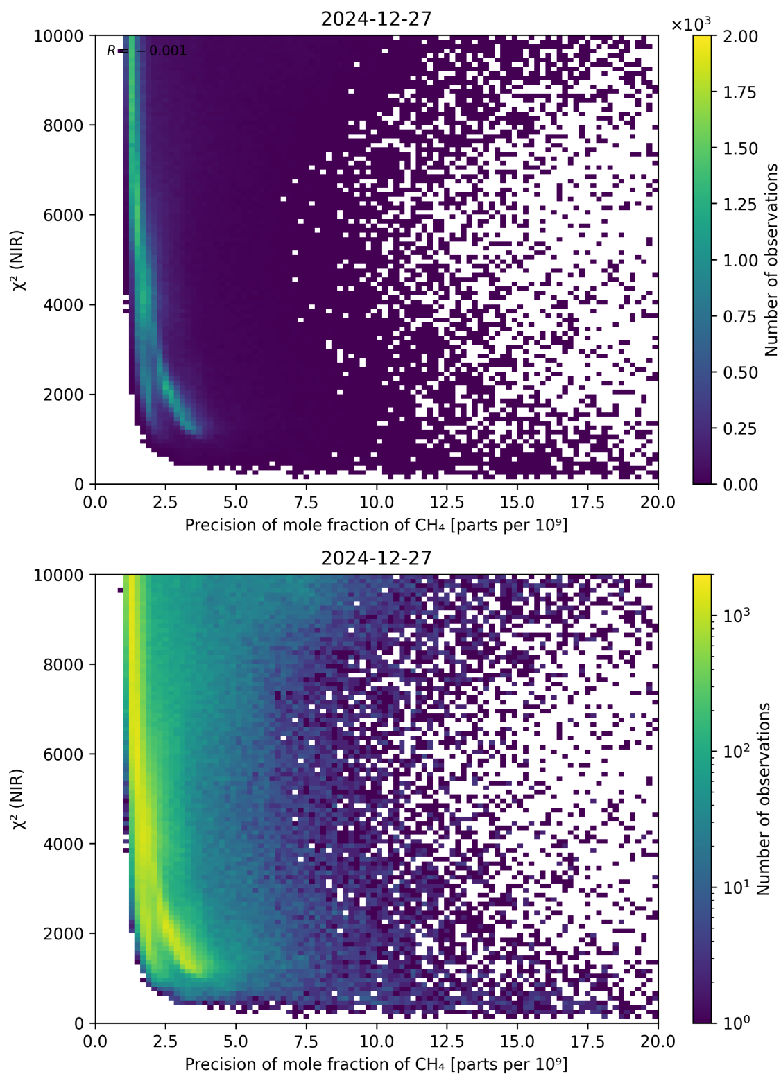
Figure 78: Scatter density plot of “Precision of mole fraction of CH 4 ” against “ \chi^2 (NIR)” for 2024-12-27 to 2024-12-28.
