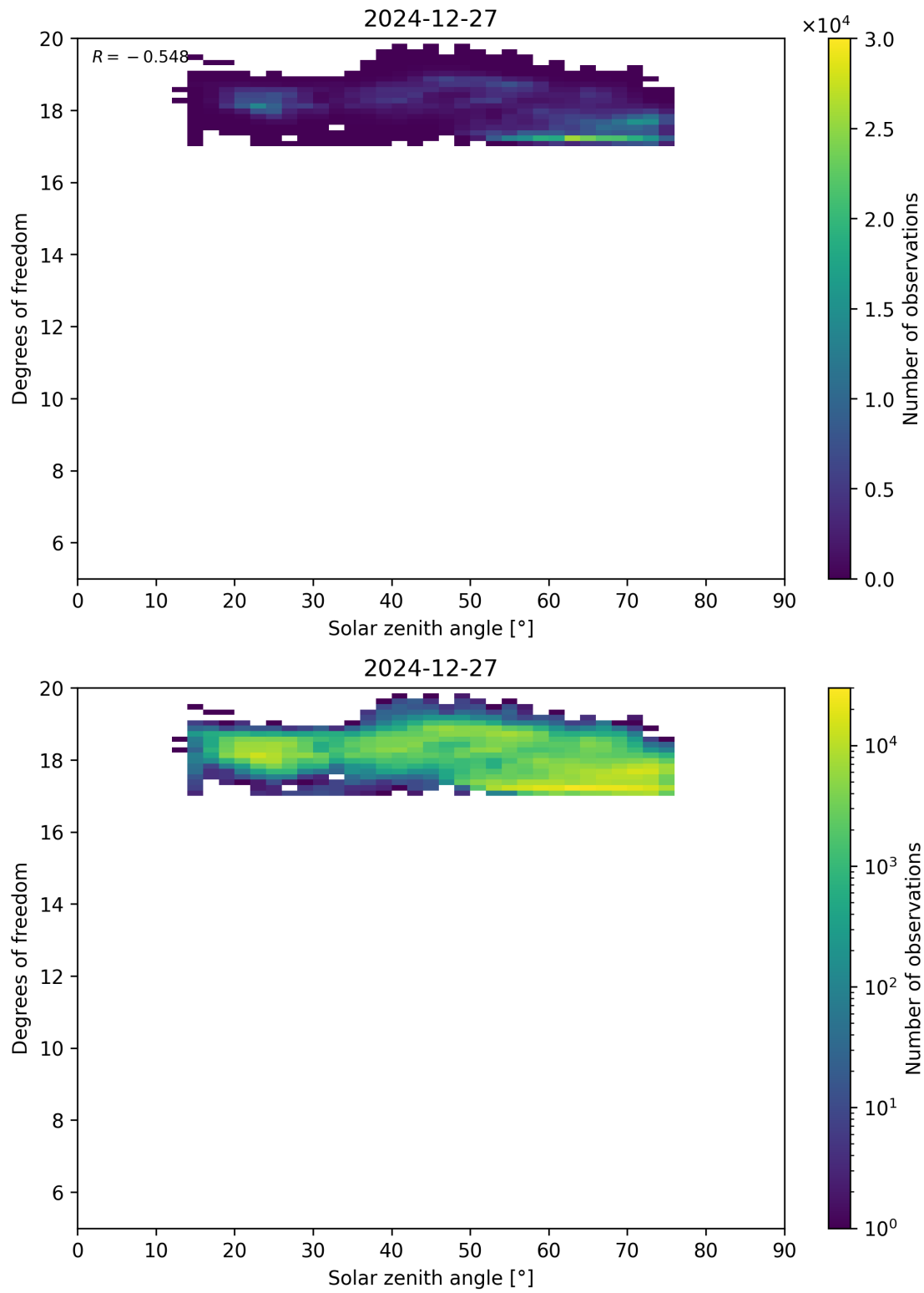
Figure 96: Scatter density plot of “Solar zenith angle” against “Degrees of freedom” for 2024-12-27 to 2024-12-28.
