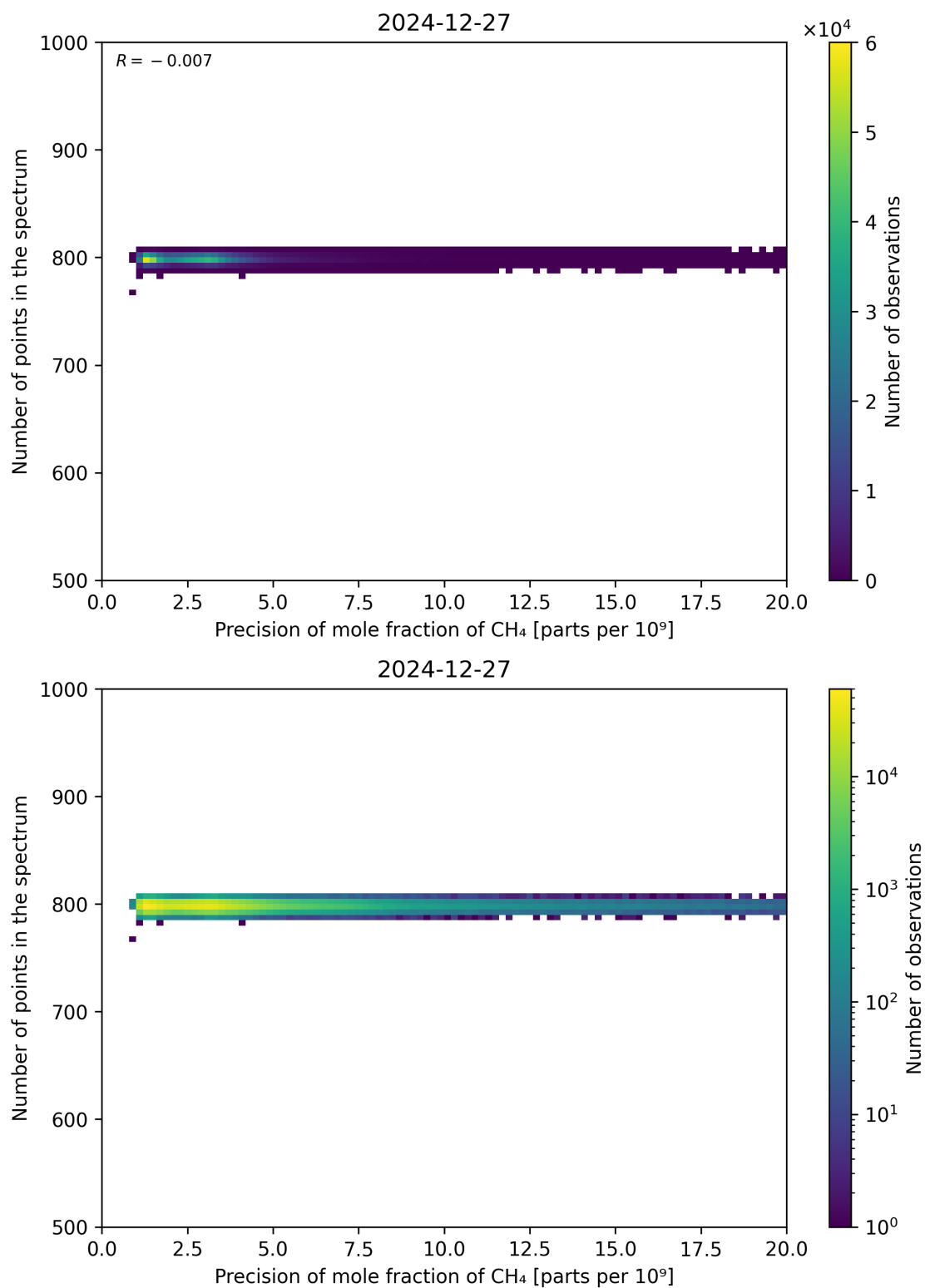
Figure 84: Scatter density plot of “Precision of mole fraction of CH 4 ” against “Number of points in the spectrum” for 2024-12-27 to 2024-12-28.
