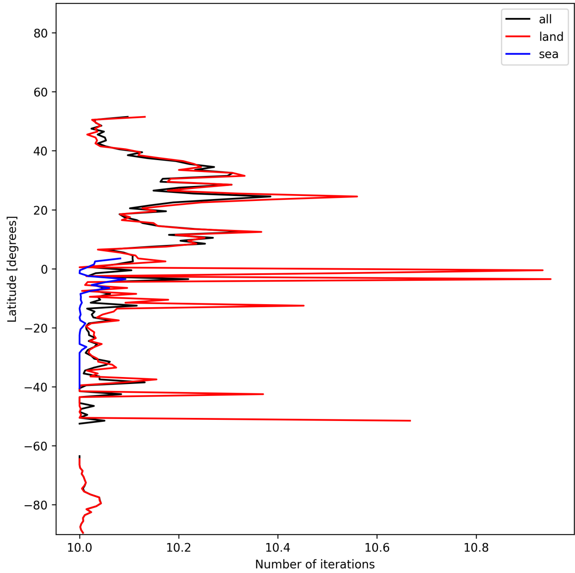
Figure 20: Zonal average of “Number of iterations” for 2024-12-27 to 2024-12-28.
