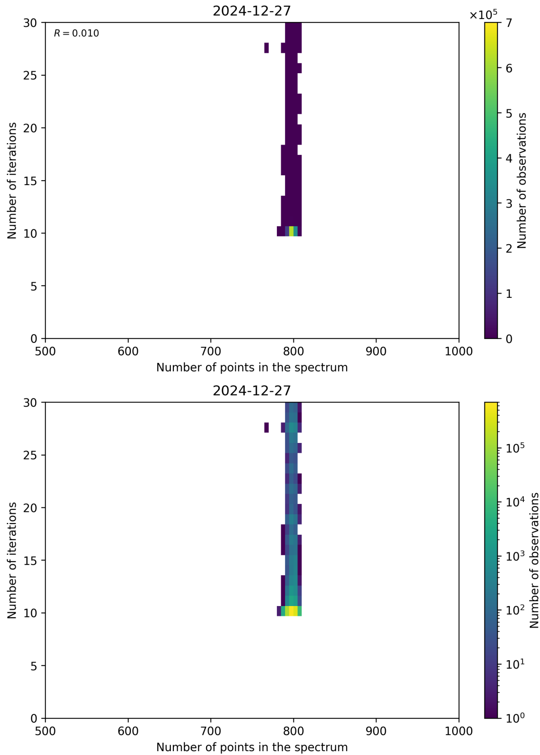
Figure 92: Scatter density plot of “Number of points in the spectrum” against “Number of iterations” for 2024-12-27 to 2024-12-28.
