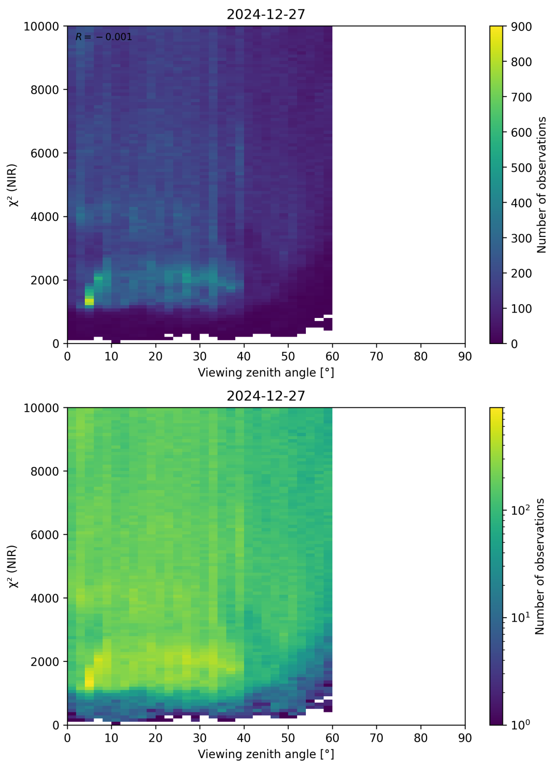
Figure 105: Scatter density plot of “Viewing zenith angle” against “ \chi^2 (NIR)” for 2024-12-27 to 2024-12-28.
