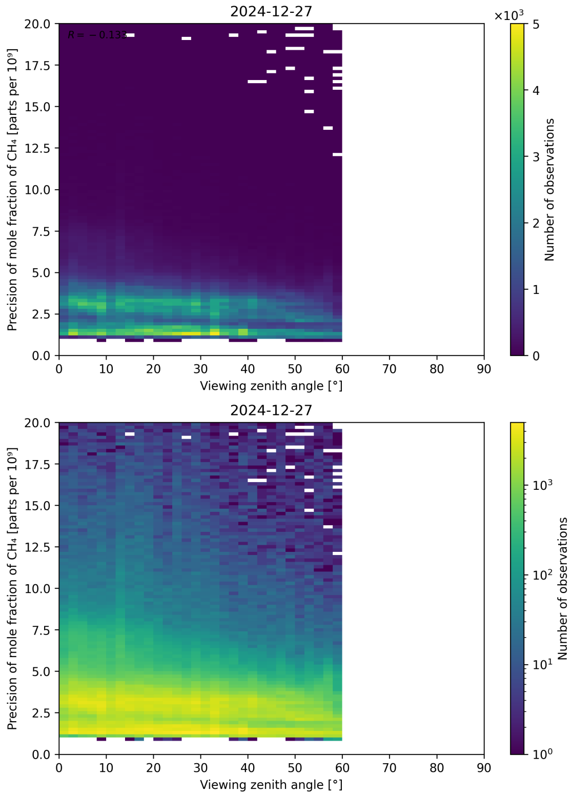
Figure 112: Scatter density plot of “Viewing zenith angle” against “Precision of mole fraction of CH 4 ” for 2024-12-27 to 2024-12-28.
