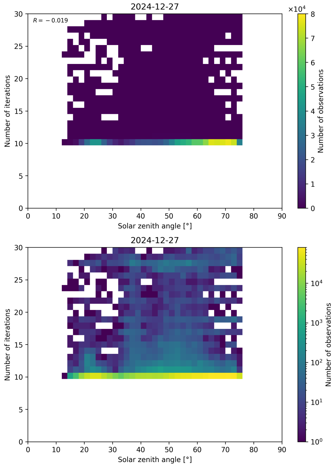
Figure 102: Scatter density plot of “Solar zenith angle” against “Number of iterations” for 2024-12-27 to 2024-12-28.
