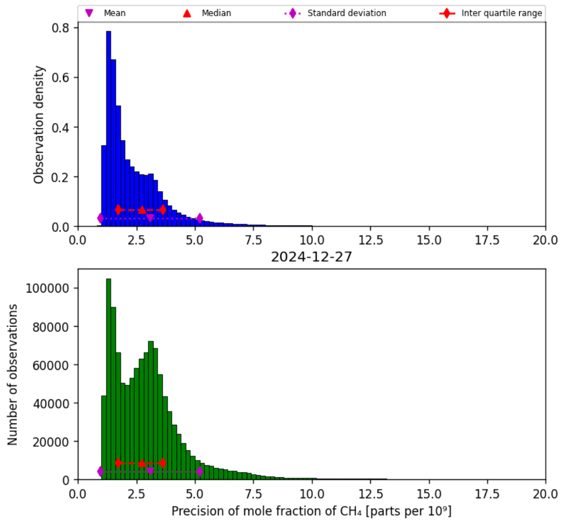
Figure 24: Histogram of “Precision of mole fraction of CH 4 ” for 2024-12-27 to 2024-12-28
