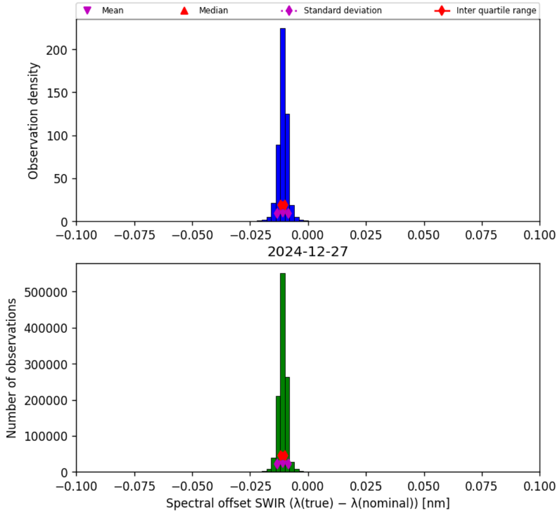
Figure 27: Histogram of “Spectral offset SWIR ( \lambda_{\text{true}} - \lambda_{\text{nominal}} )” for 2024-12-27 to 2024-12-28
