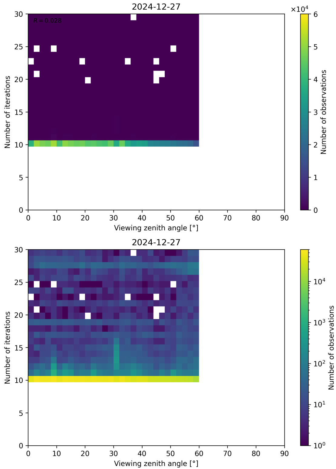
Figure 113: Scatter density plot of “Viewing zenith angle” against “Number of iterations” for 2024-12-27 to 2024-12-28.
