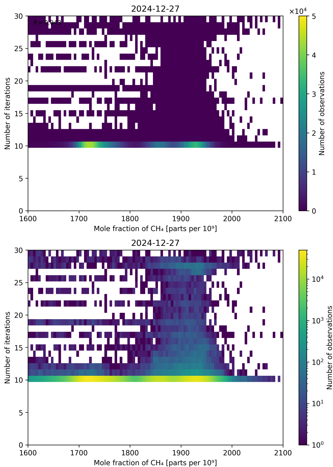
Figure 76: Scatter density plot of “Mole fraction of CH 4 ” against “Number of iterations” for 2024-12-27 to 2024-12-28.
