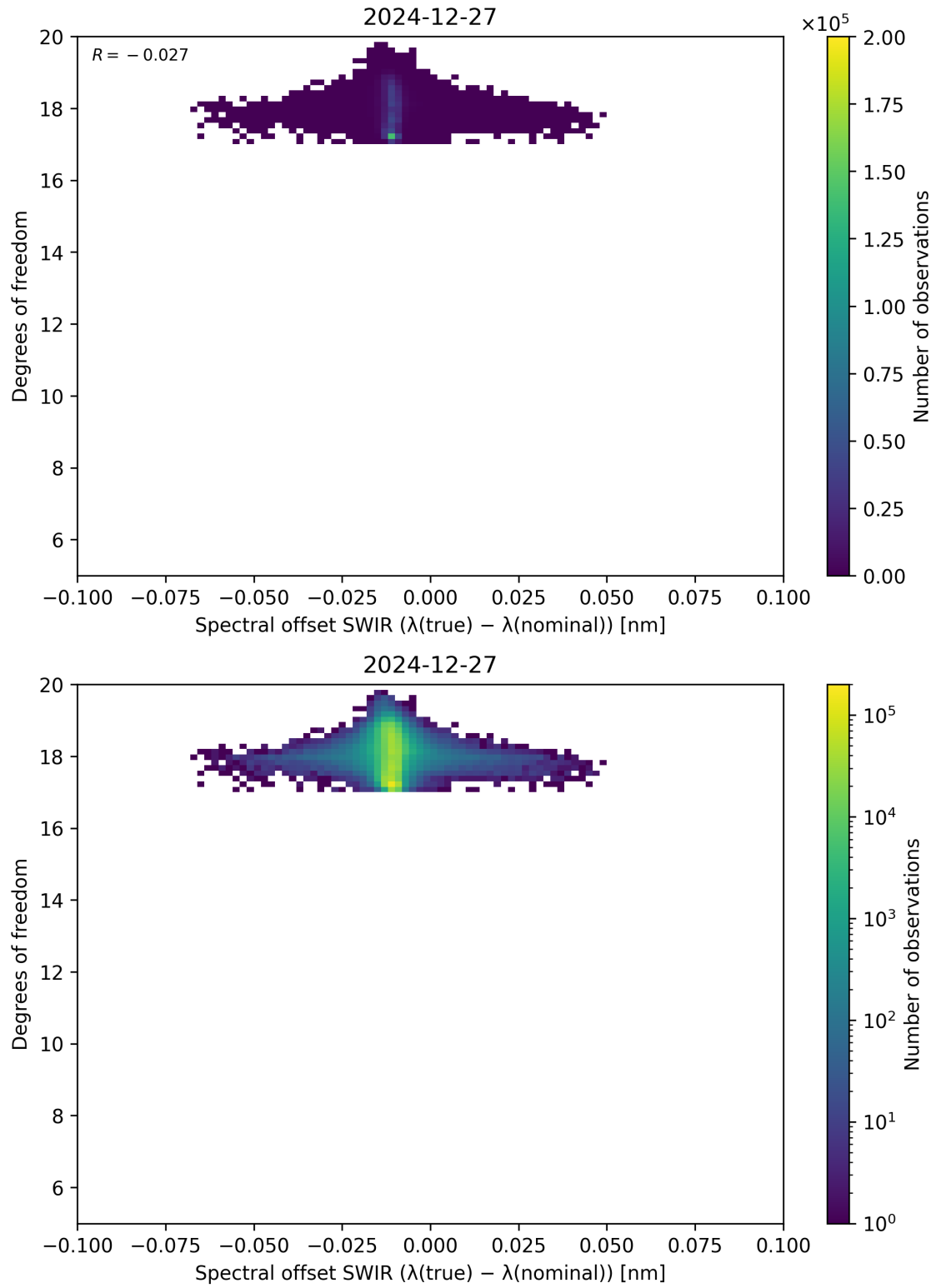
Figure 119: Scatter density plot of “Spectral offset SWIR ( \lambda_{\text{true}} - \lambda_{\text{nominal}} )” against “Degrees of freedom” for 2024-12-27 to 2024-12-28.
