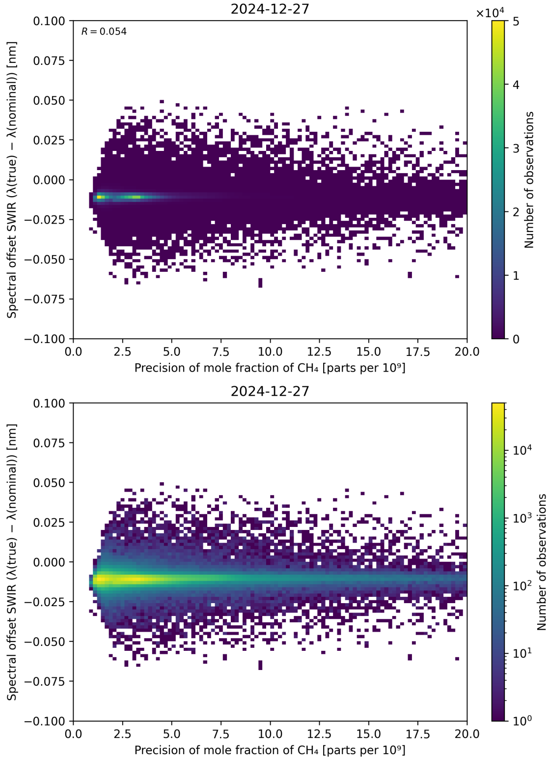
Figure 85: Scatter density plot of “Precision of mole fraction of \text{CH}_4 ” against “Spectral offset SWIR ( \lambda_{\text{true}} - \lambda_{\text{nominal}} )” for 2024-12-27 to 2024-12-28.
