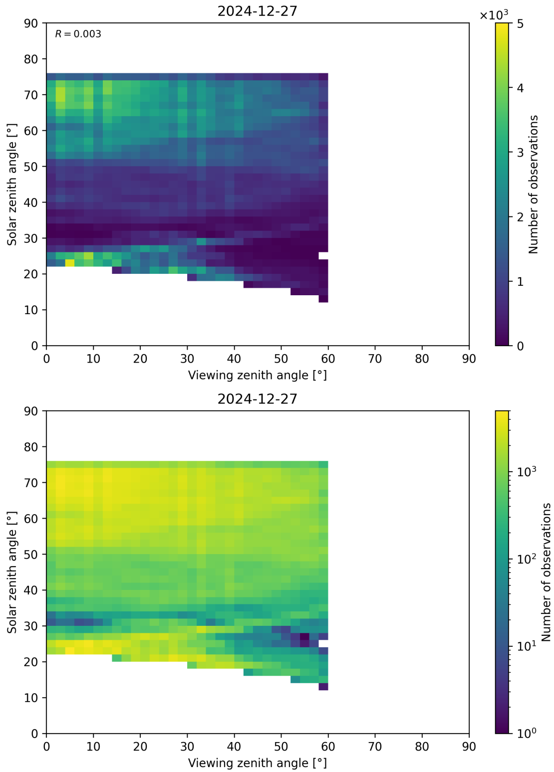
Figure 115: Scatter density plot of “Viewing zenith angle” against “Solar zenith angle” for 2024-12-27 to 2024-12-28.
