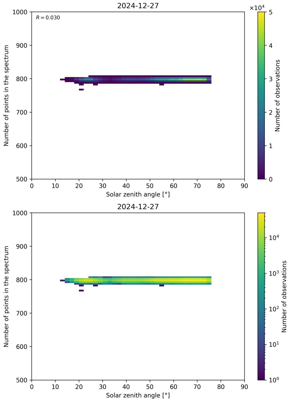
Figure 103: Scatter density plot of “Solar zenith angle” against “Number of points in the spectrum” for 2024-12-27 to 2024-12-28.
