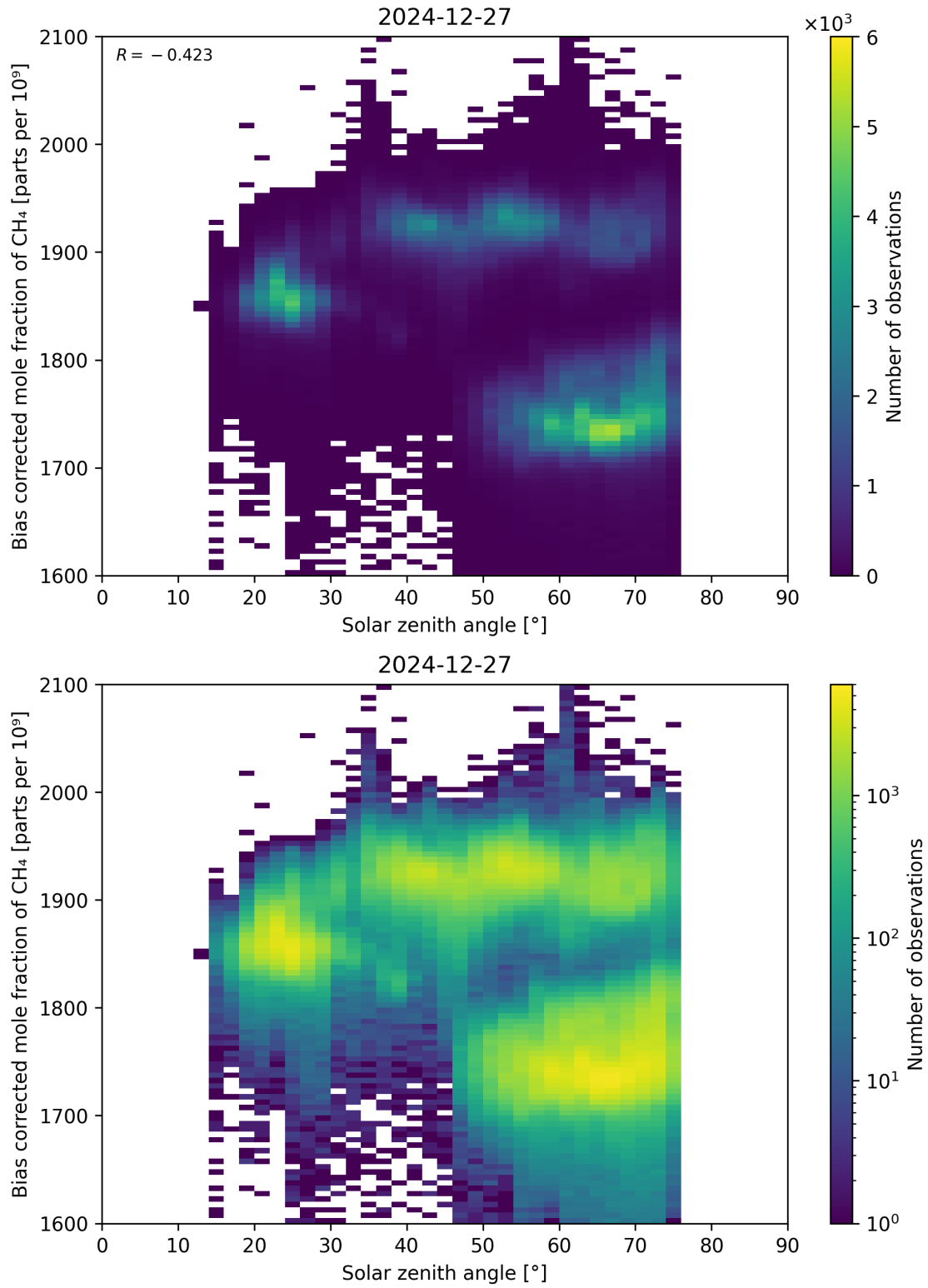
Figure 100: Scatter density plot of “Solar zenith angle” against “Bias corrected mole fraction of CH 4 ” for 2024-12-27 to 2024-12-28.
