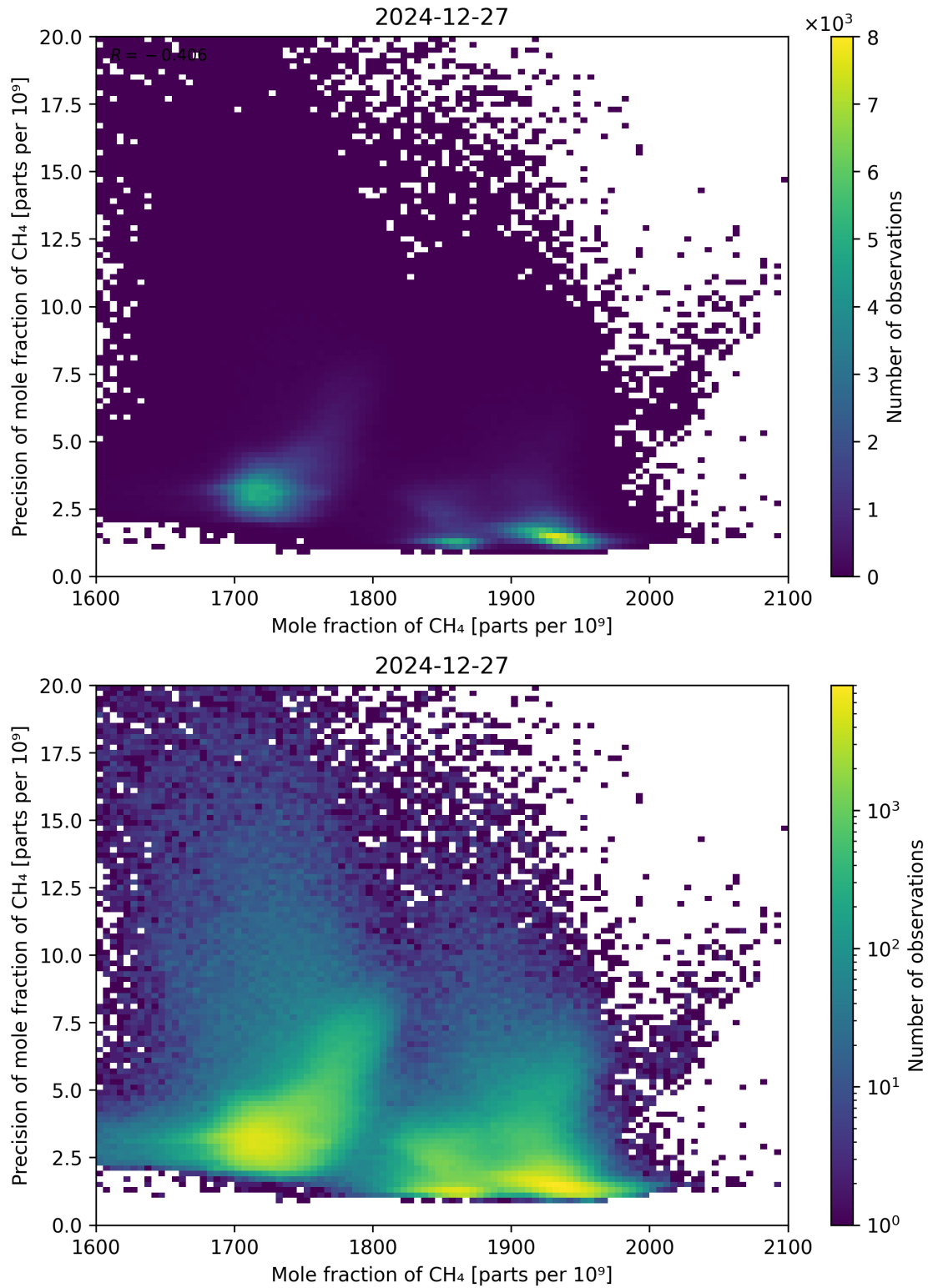
Figure 75: Scatter density plot of “Mole fraction of CH 4 ” against “Precision of mole fraction of CH 4 ” for 2024-12-27 to 2024-12-28.
