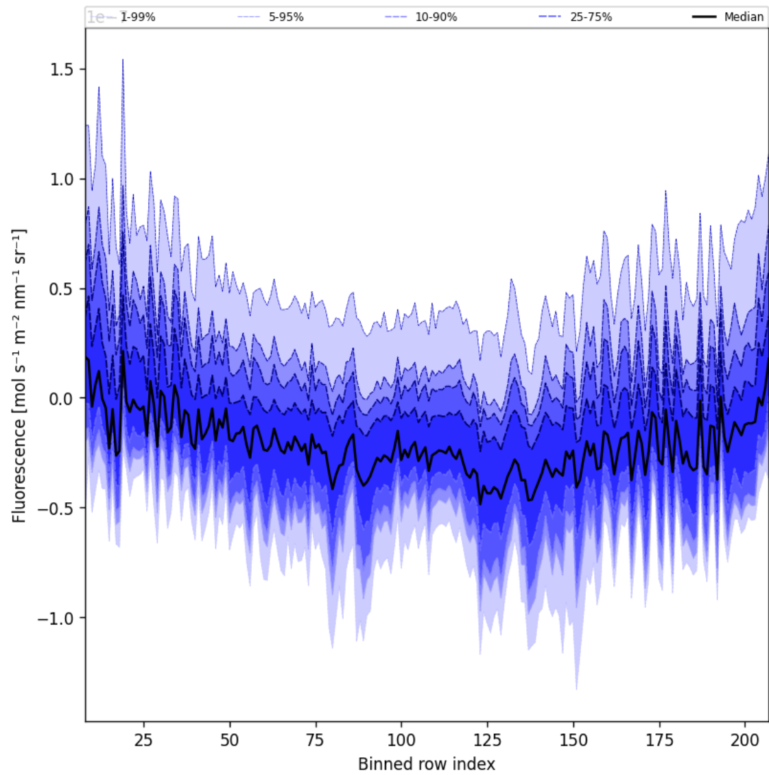
Figure 43: Along track statistics of “Fluorescence” for 2024-12-27 to 2024-12-28
