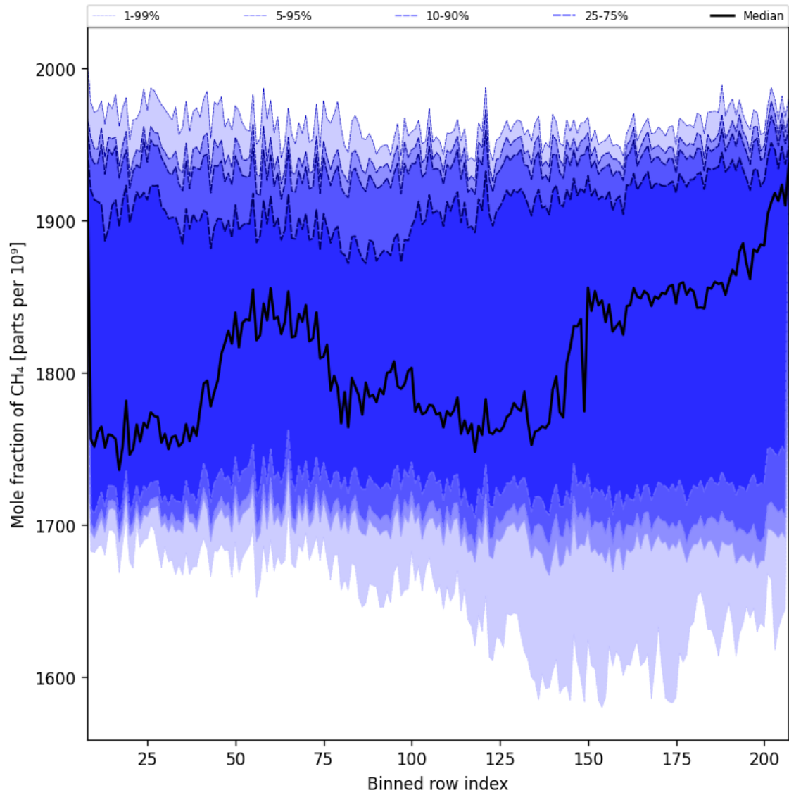
Figure 34: Along track statistics of “Mole fraction of CH 4 ” for 2024-12-27 to 2024-12-28
