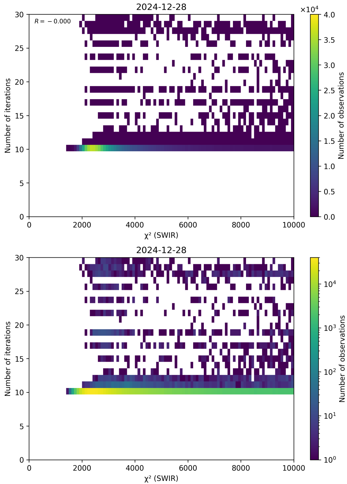
Figure 50: Scatter density plot of “ \chi^2 (SWIR)” against “Number of iterations” for 2024-12-27 to 2024-12-29.
