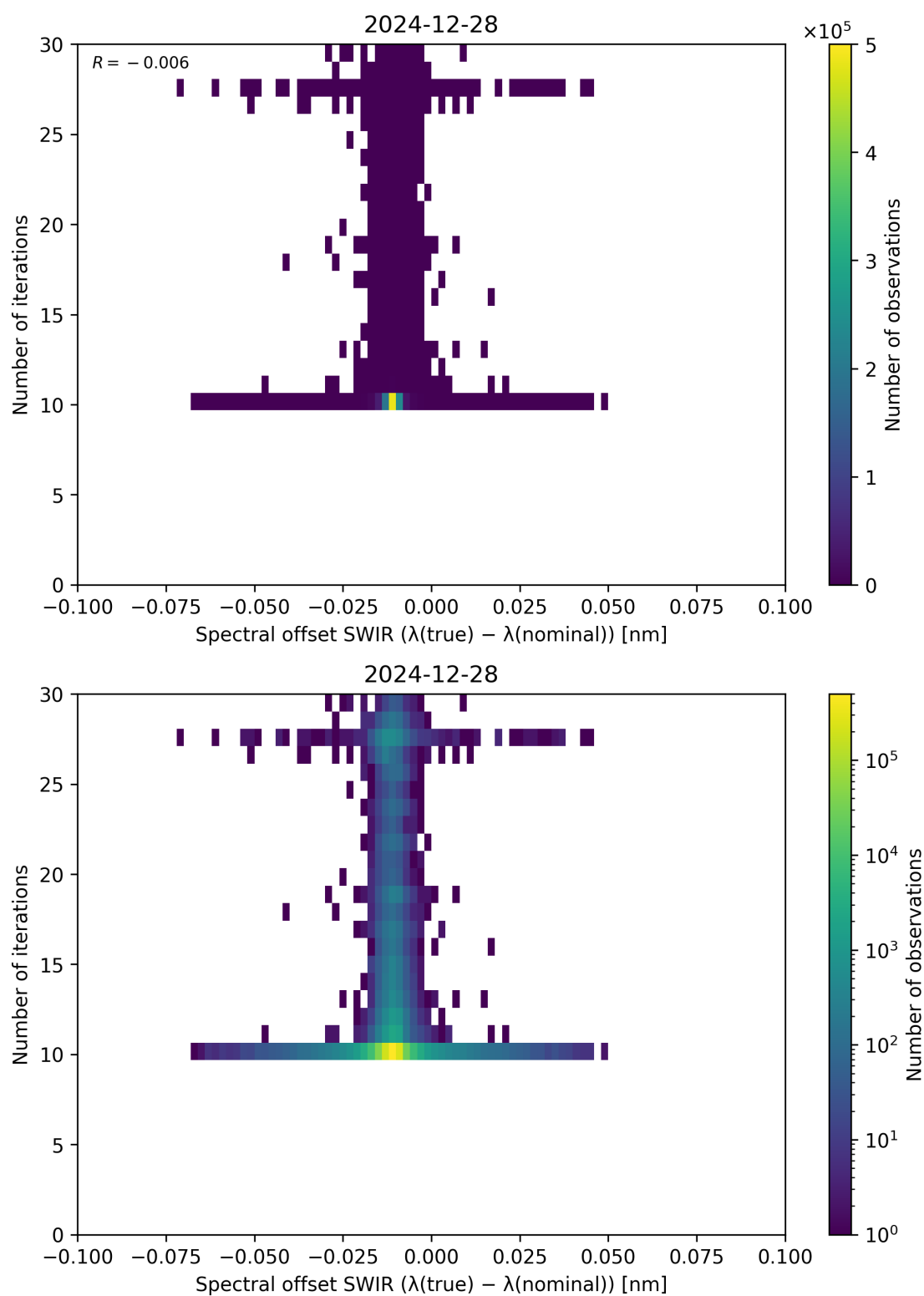
Figure 121: Scatter density plot of “Spectral offset SWIR ( \lambda_{\text{true}} - \lambda_{\text{nominal}} )” against “Number of iterations” for 2024-12-27 to 2024-12-29.
