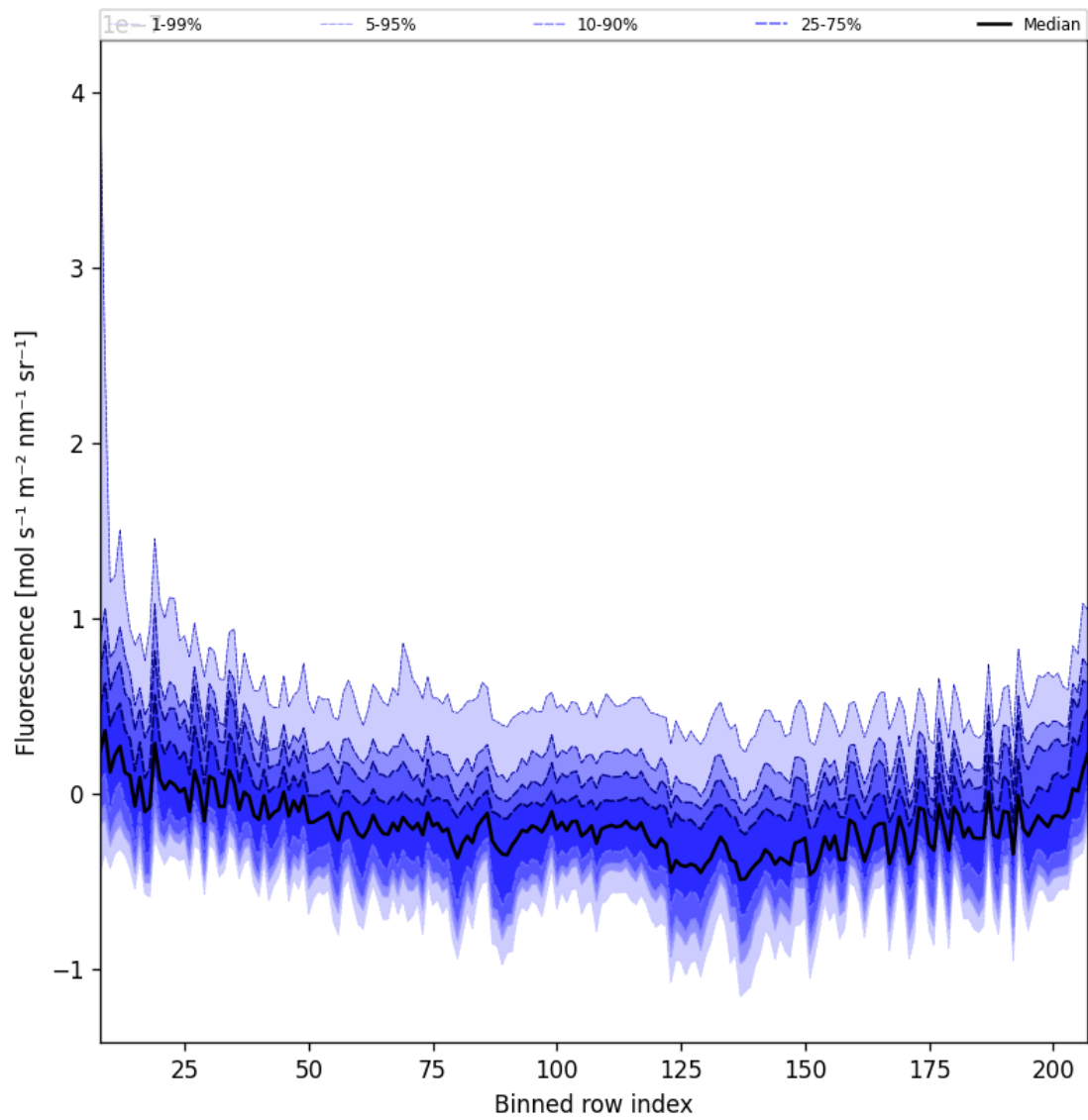
Figure 43: Along track statistics of “Fluorescence” for 2024-12-27 to 2024-12-29
