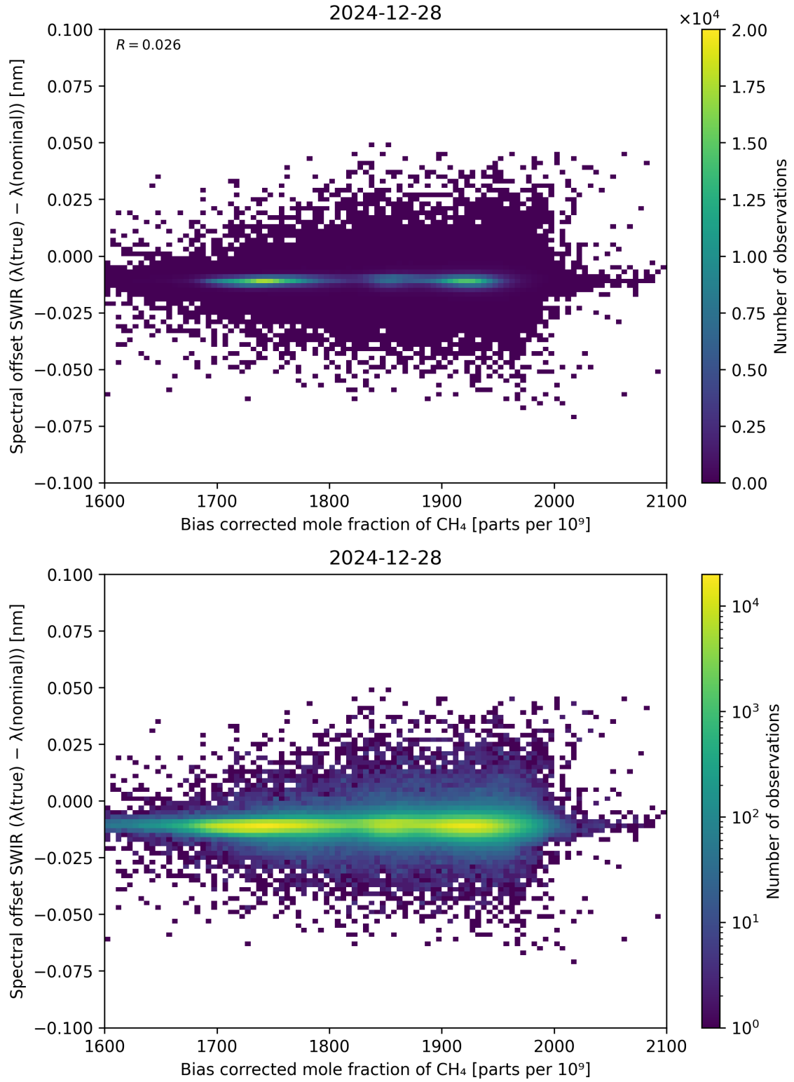
Figure 69: Scatter density plot of “Bias corrected mole fraction of \text{CH}_4 ” against “Spectral offset SWIR ( \lambda_{\text{true}} - \lambda_{\text{nominal}} )” for 2024-12-27 to 2024-12-29.
