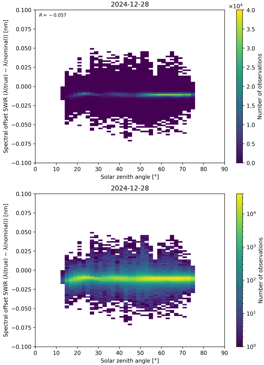
Figure 104: Scatter density plot of “Solar zenith angle” against “Spectral offset SWIR ( \lambda_{\text{true}} - \lambda_{\text{nominal}} )” for 2024-12-27 to 2024-12-29.
