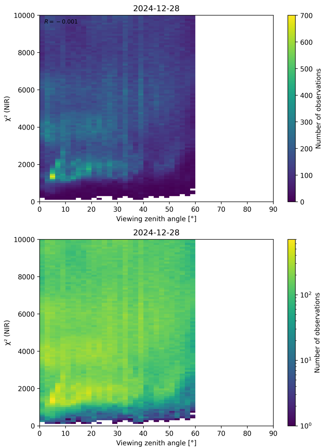
Figure 105: Scatter density plot of “Viewing zenith angle” against “ \chi^2 (NIR)” for 2024-12-27 to 2024-12-29.
