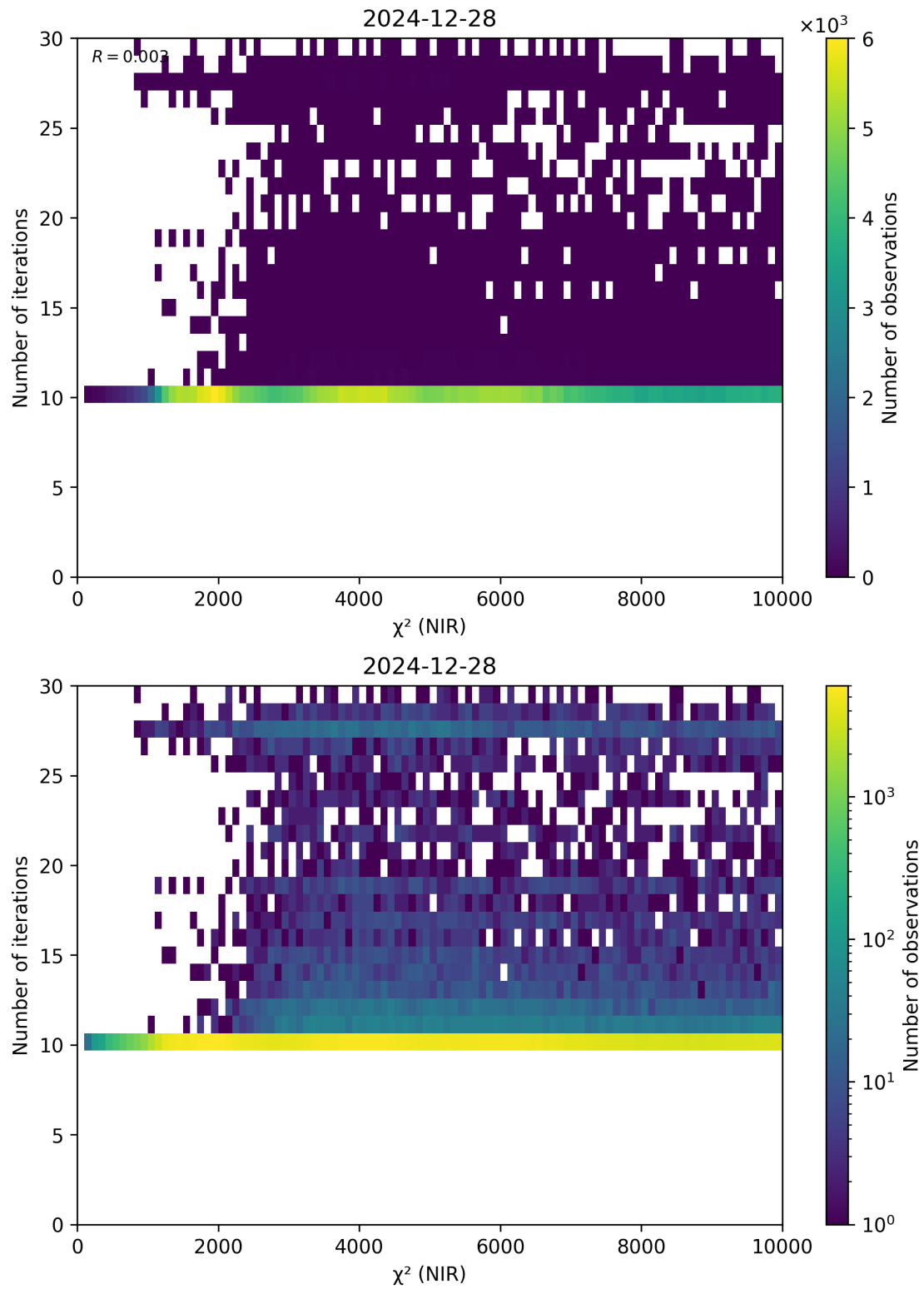
Figure 46: Scatter density plot of “ \chi^2 (NIR)” against “Number of iterations” for 2024-12-27 to 2024-12-29.
