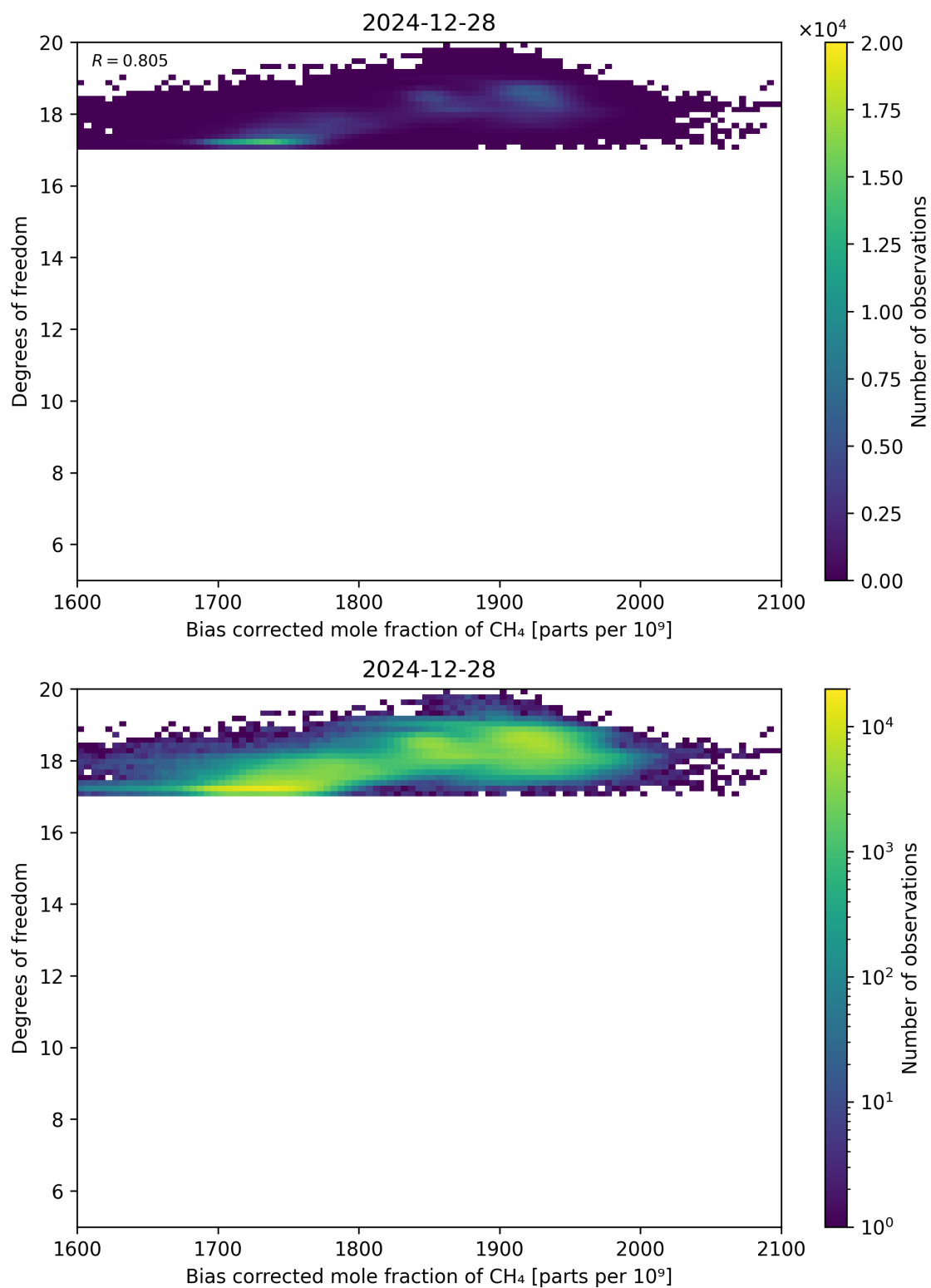
Figure 65: Scatter density plot of “Bias corrected mole fraction of CH 4 ” against “Degrees of freedom” for 2024-12-27 to 2024-12-29.
