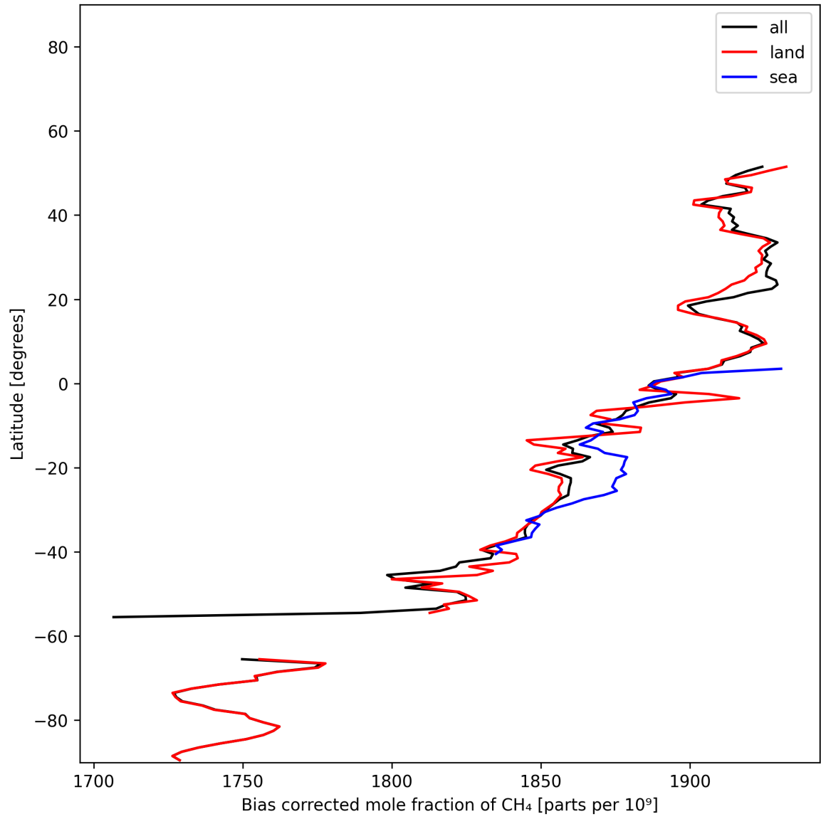
Figure 14: Zonal average of “Bias corrected mole fraction of CH 4 ” for 2024-12-27 to 2024-12-29.
