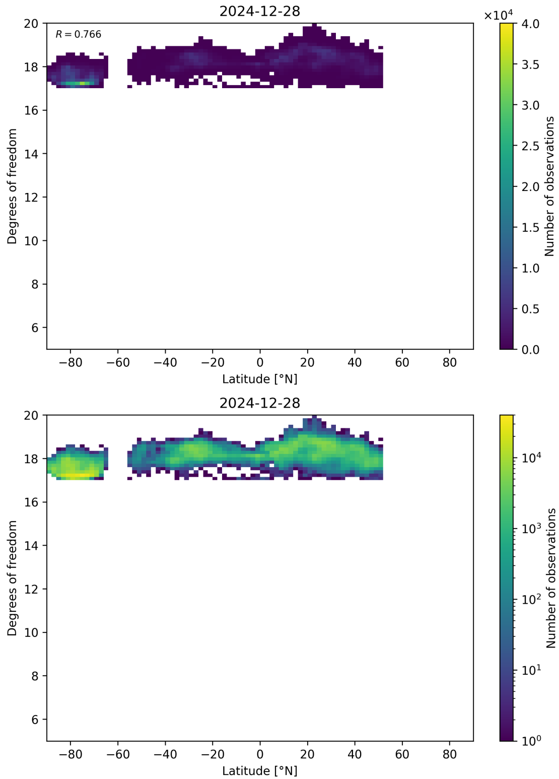
Figure 55: Scatter density plot of “Latitude” against “Degrees of freedom” for 2024-12-27 to 2024-12-29.
