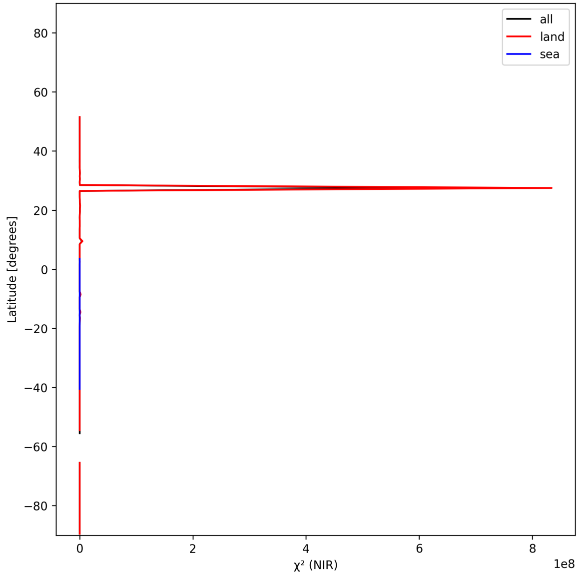
Figure 18: Zonal average of “ \chi^2 (NIR)” for 2024-12-27 to 2024-12-29.
