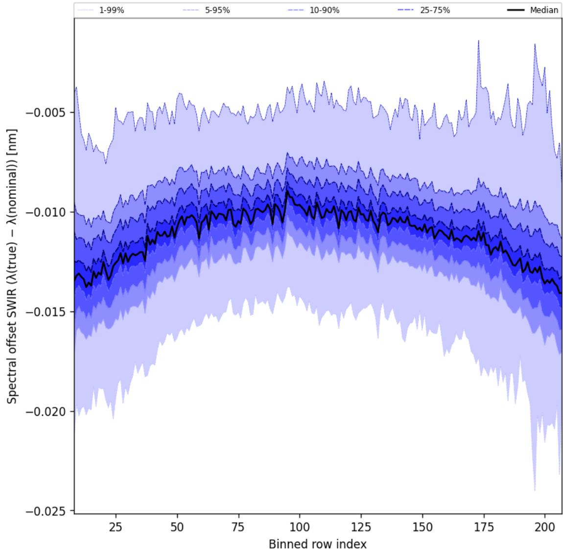
Figure 38: Along track statistics of “Spectral offset SWIR ( \lambda_{\text{true}} - \lambda_{\text{nominal}} )” for 2024-12-27 to 2024-12-29
