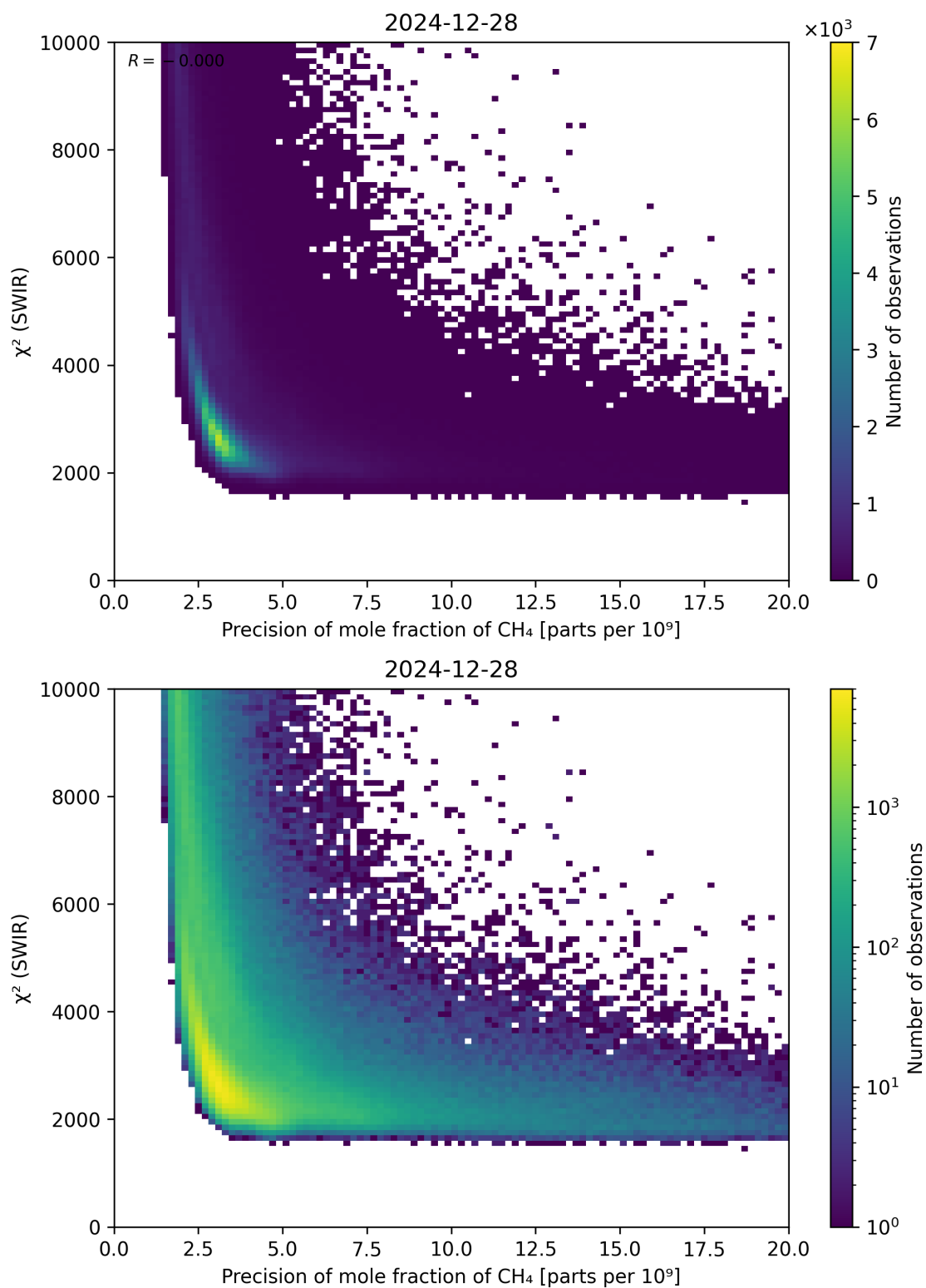
Figure 79: Scatter density plot of “Precision of mole fraction of CH 4 ” against “ \chi^2 (SWIR)” for 2024-12-27 to 2024-12-29.
