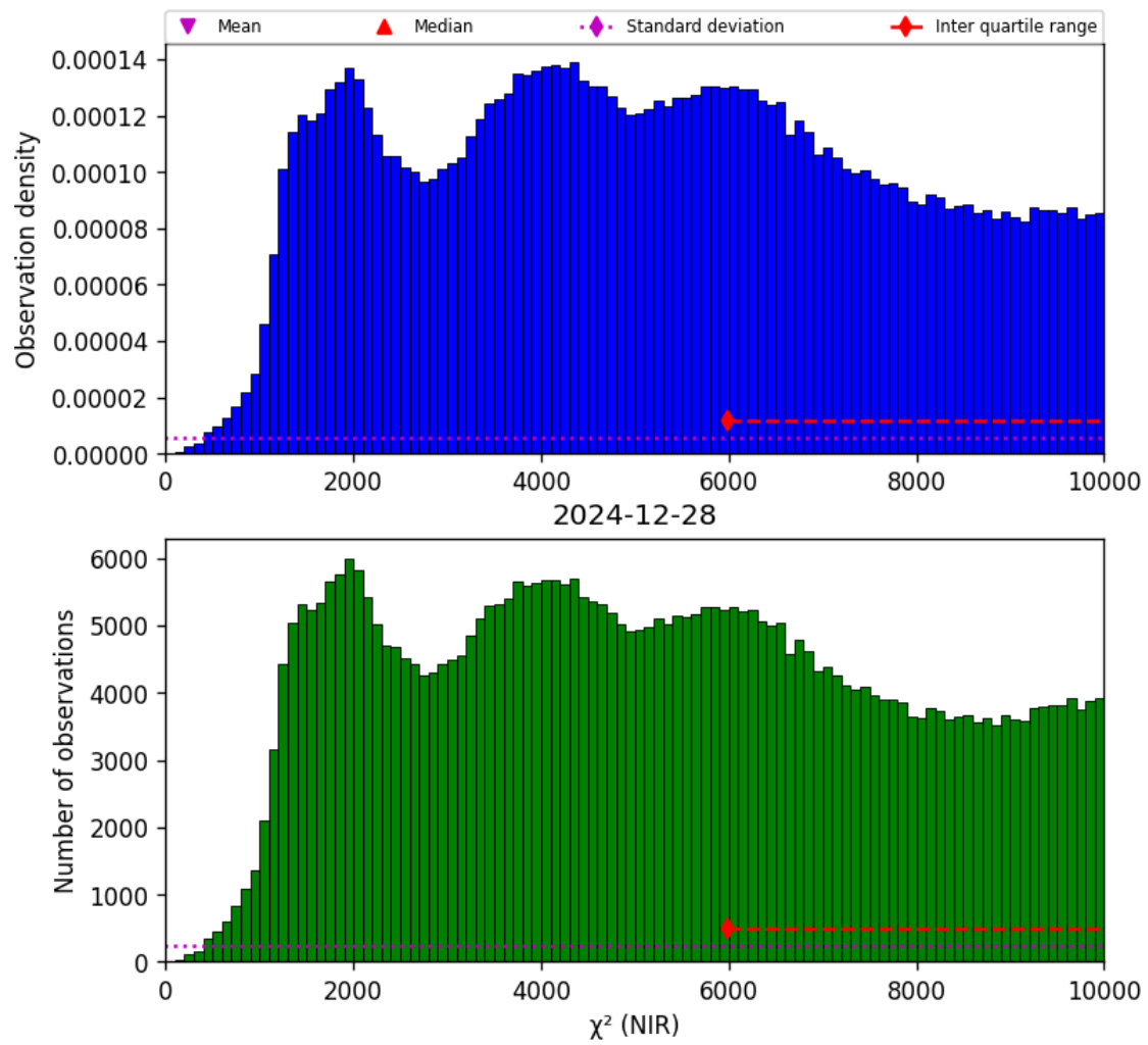
Figure 29: Histogram of " \chi^2 (NIR)" for 2024-12-27 to 2024-12-29
