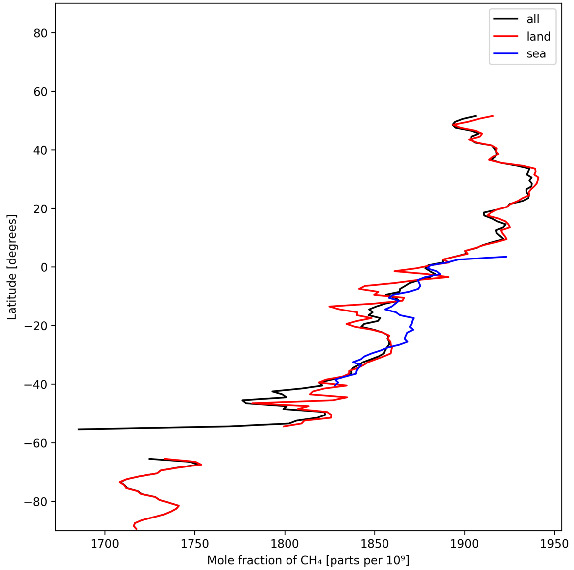
Figure 12: Zonal average of “Mole fraction of CH 4 ” for 2024-12-27 to 2024-12-29.
