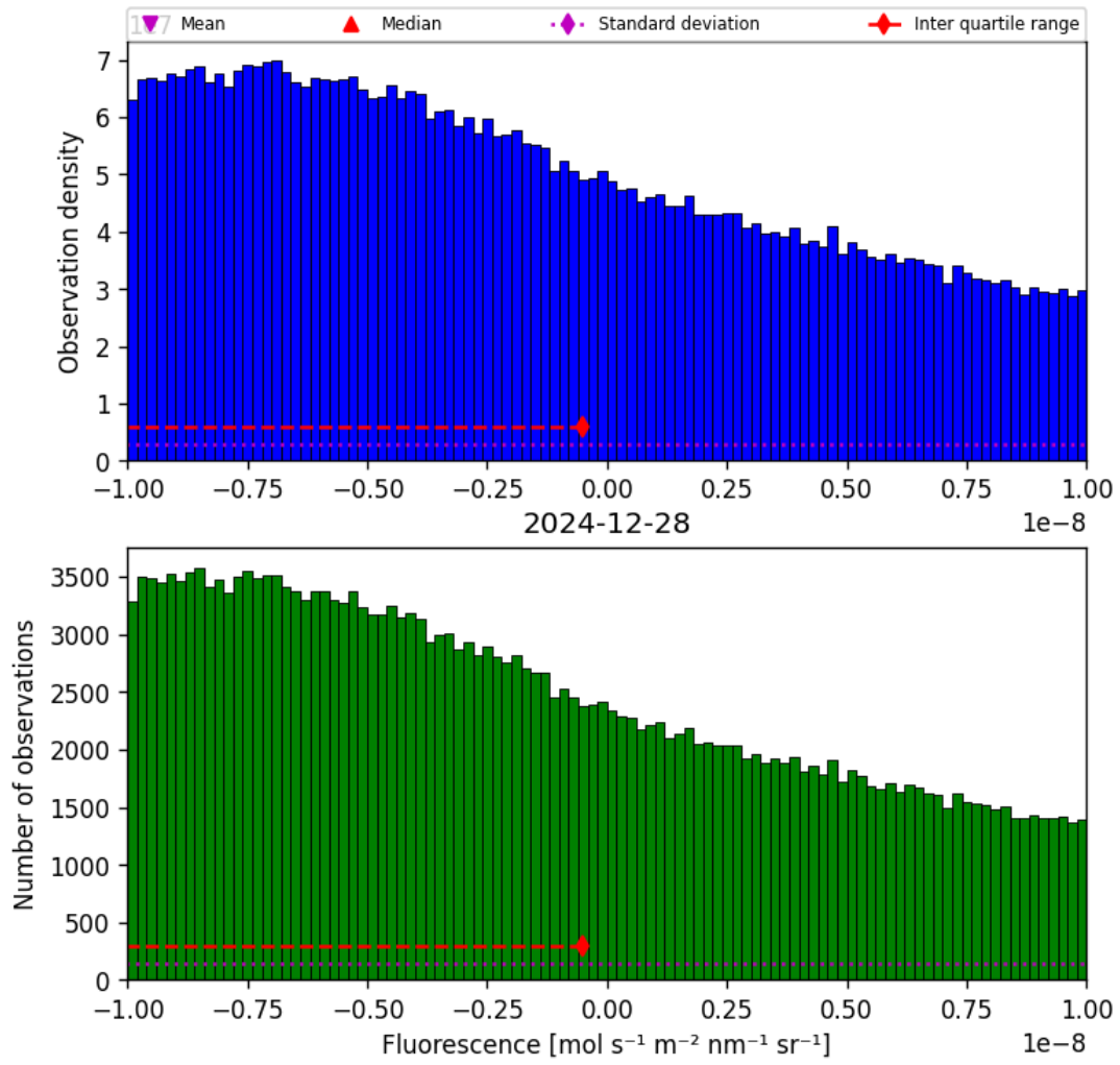
Figure 32: Histogram of “Fluorescence” for 2024-12-27 to 2024-12-29
