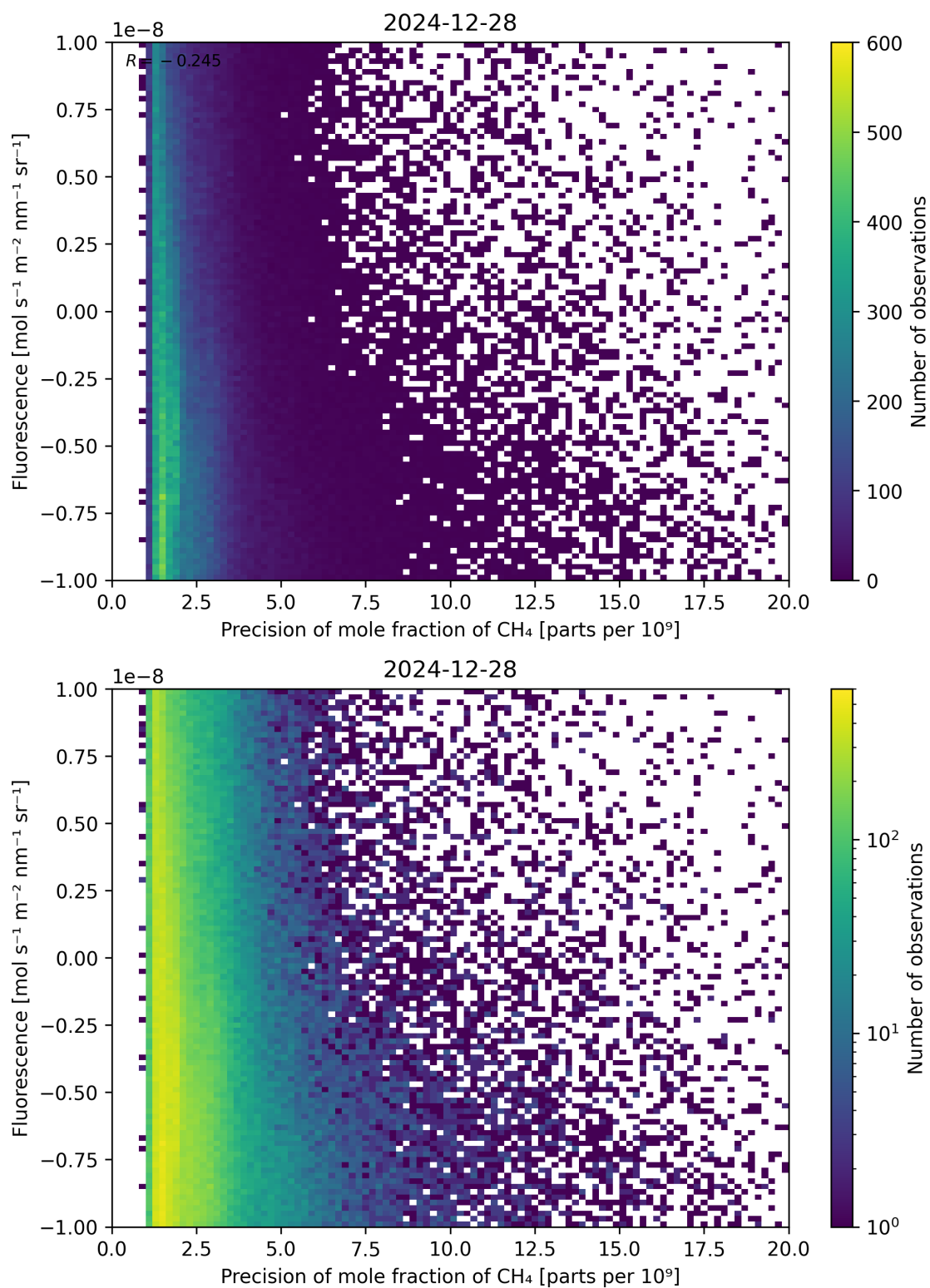
Figure 81: Scatter density plot of “Precision of mole fraction of \text{CH}_4 ” against “Fluorescence” for 2024-12-27 to 2024-12-29.
