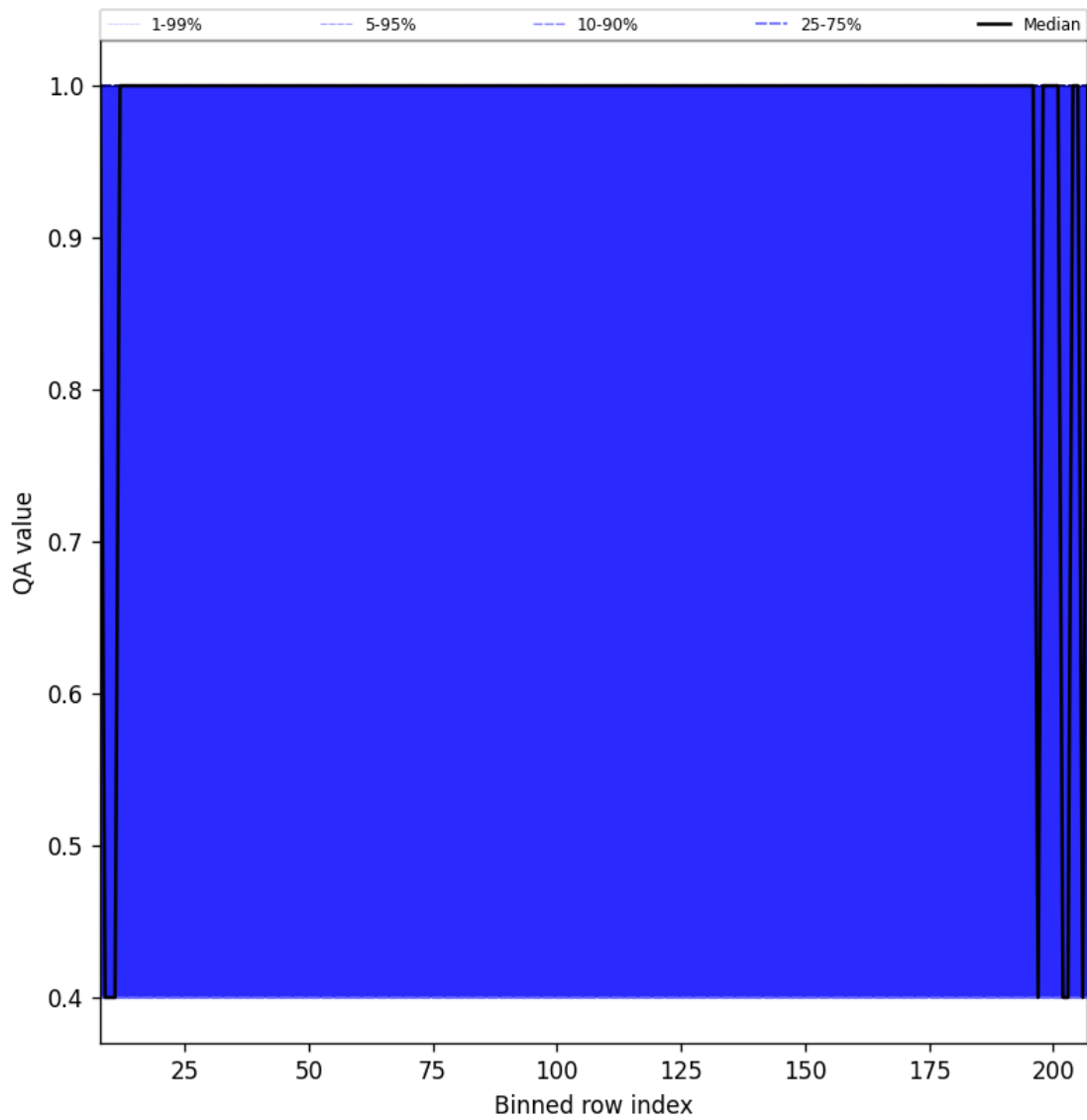
Figure 33: Along track statistics of “QA value” for 2024-12-27 to 2024-12-29
