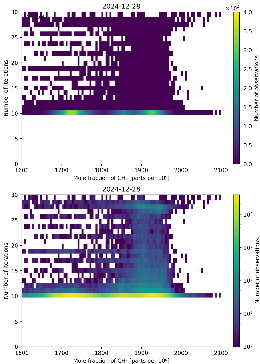
Figure 76: Scatter density plot of “Mole fraction of CH 4 ” against “Number of iterations” for 2024-12-27 to 2024-12-29.
