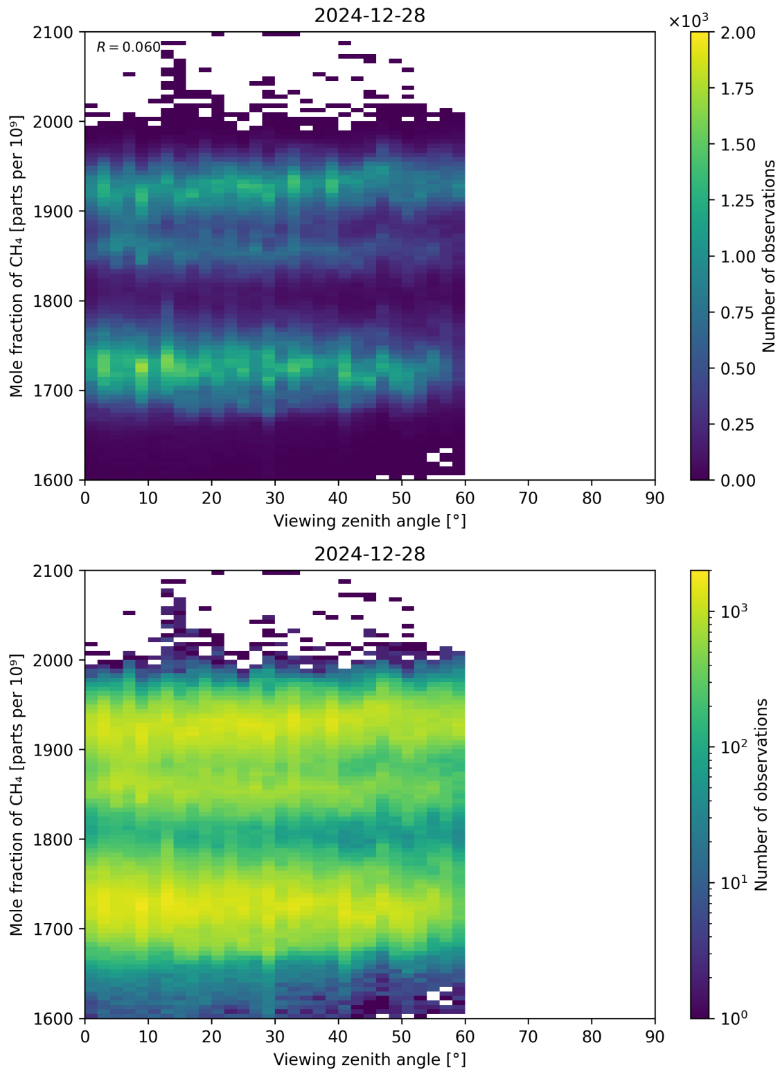
Figure 110: Scatter density plot of “Viewing zenith angle” against “Mole fraction of \text{CH}_4 ” for 2024-12-27 to 2024-12-29.
