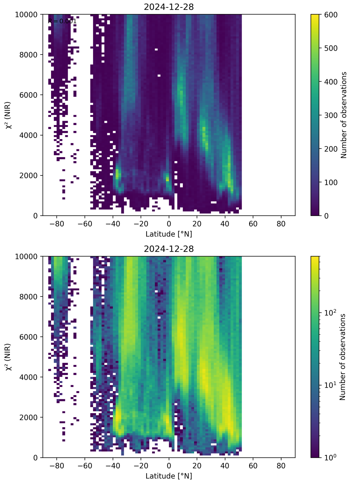
Figure 53: Scatter density plot of “Latitude” against “ \chi^2 (NIR)” for 2024-12-27 to 2024-12-29.
