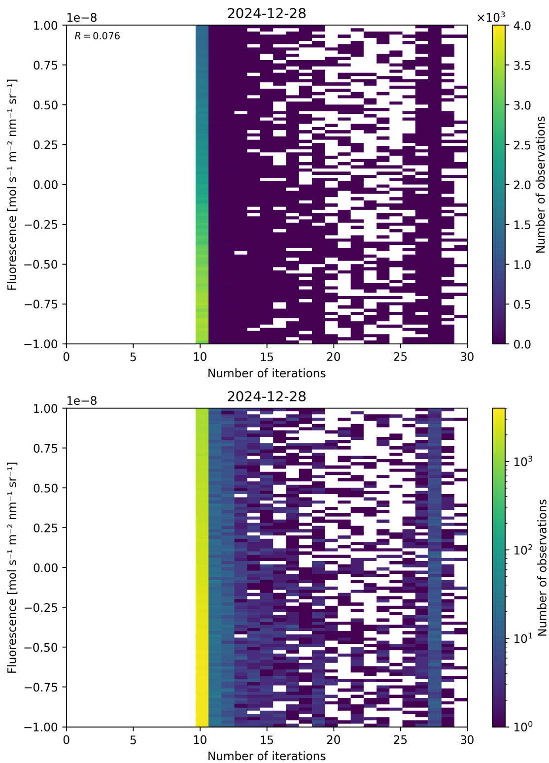
Figure 87: Scatter density plot of “Number of iterations” against “Fluorescence” for 2024-12-27 to 2024-12-29.
