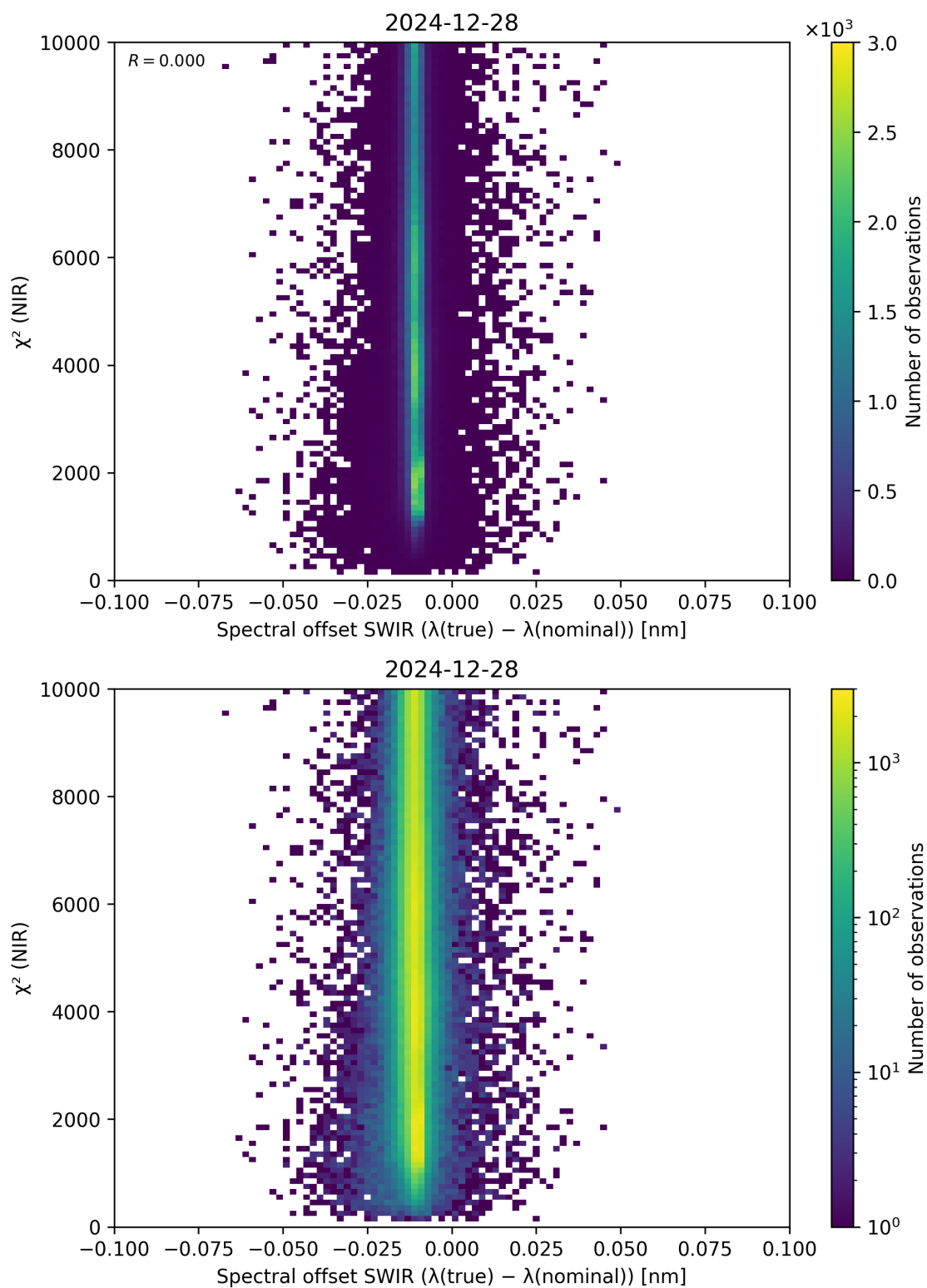
Figure 117: Scatter density plot of “Spectral offset SWIR ( \lambda_{\text{true}} - \lambda_{\text{nominal}} )” against “ \chi^2 (NIR)” for 2024-12-27 to 2024-12-29.
