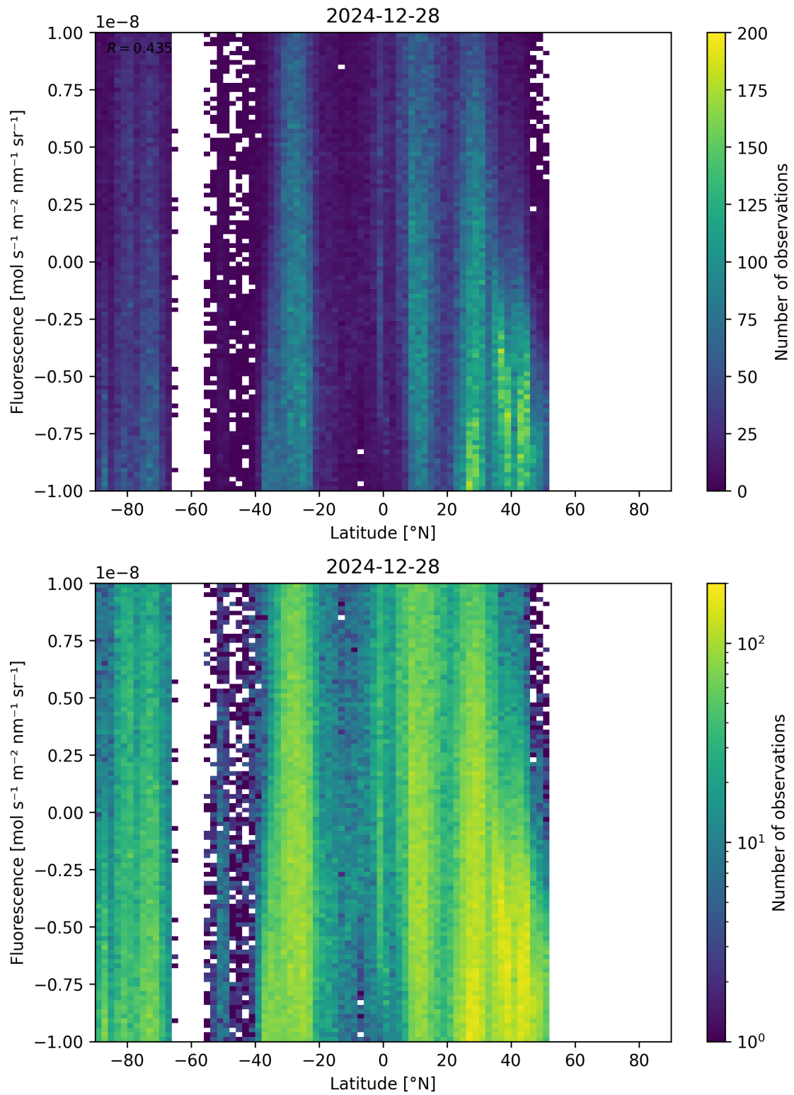
Figure 56: Scatter density plot of “Latitude” against “Fluorescence” for 2024-12-27 to 2024-12-29.
