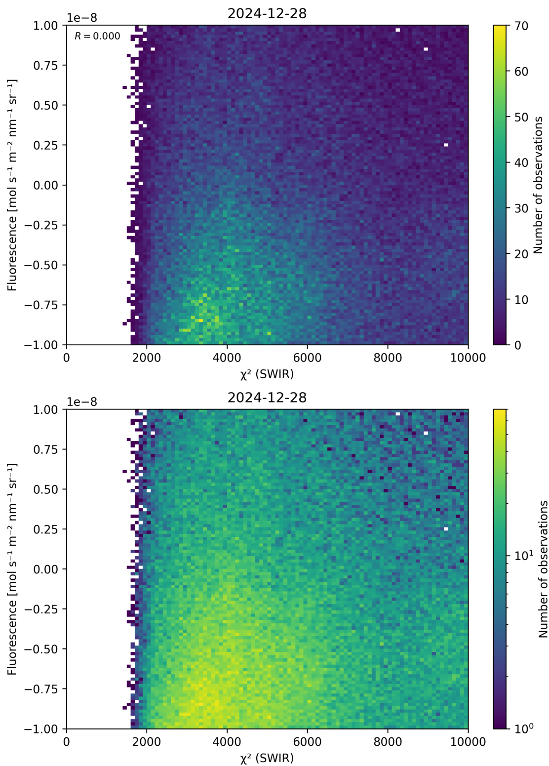
Figure 49: Scatter density plot of “ \chi^2 (SWIR)” against “Fluorescence” for 2024-12-27 to 2024-12-29.
