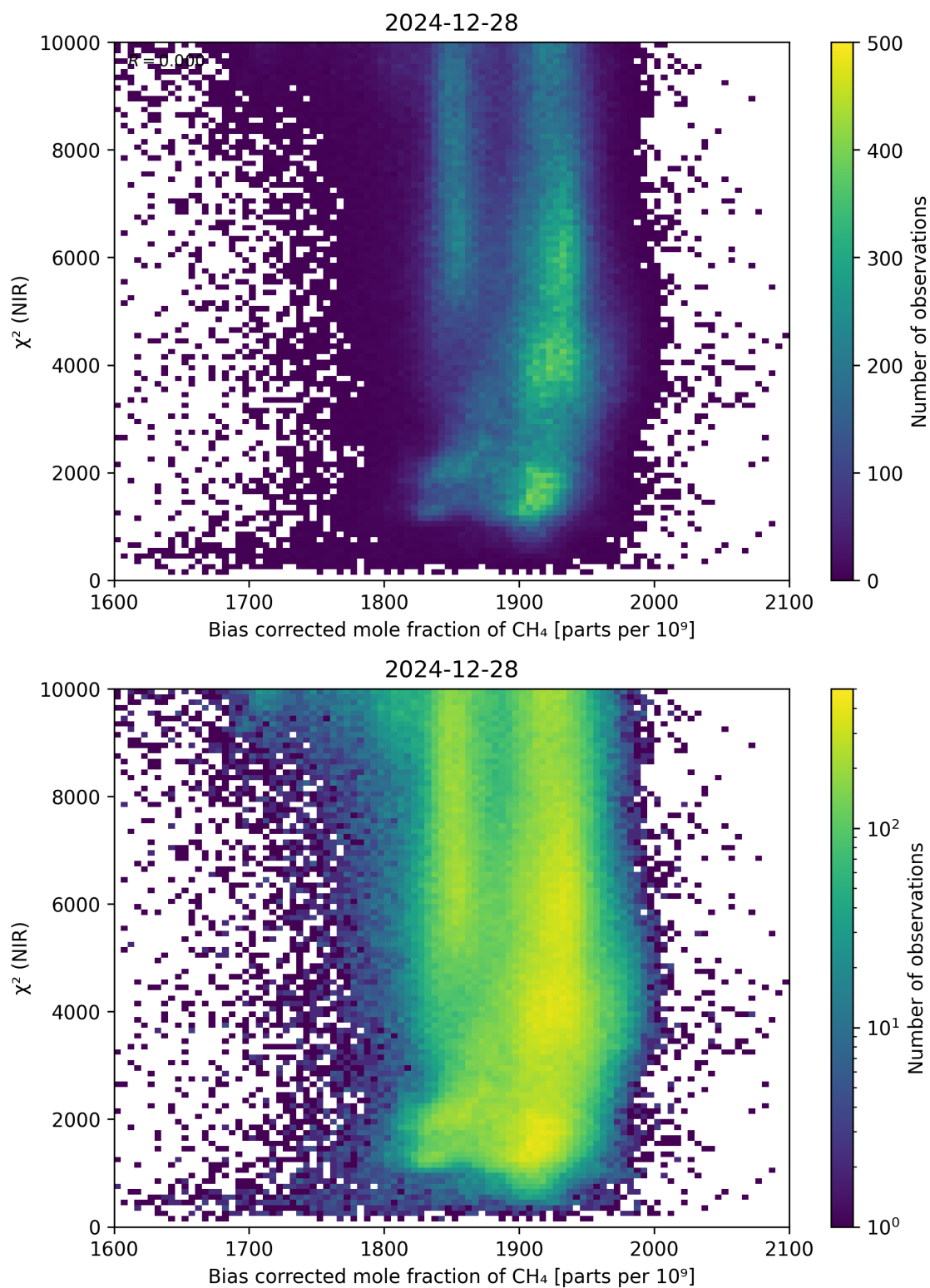
Figure 63: Scatter density plot of “Bias corrected mole fraction of CH 4 ” against “ \chi^2 (NIR)” for 2024-12-27 to 2024-12-29.
