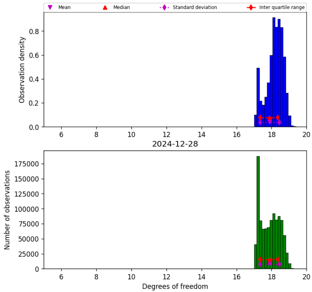
Figure 30: Histogram of “Degrees of freedom” for 2024-12-27 to 2024-12-29
