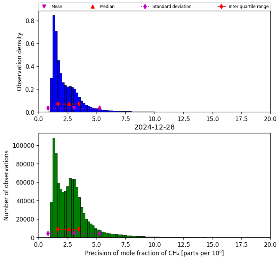
Figure 24: Histogram of “Precision of mole fraction of CH 4 ” for 2024-12-27 to 2024-12-29
