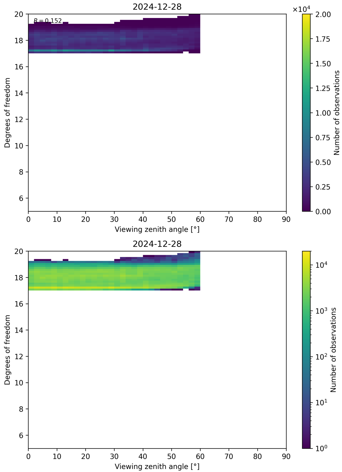
Figure 107: Scatter density plot of “Viewing zenith angle” against “Degrees of freedom” for 2024-12-27 to 2024-12-29.
