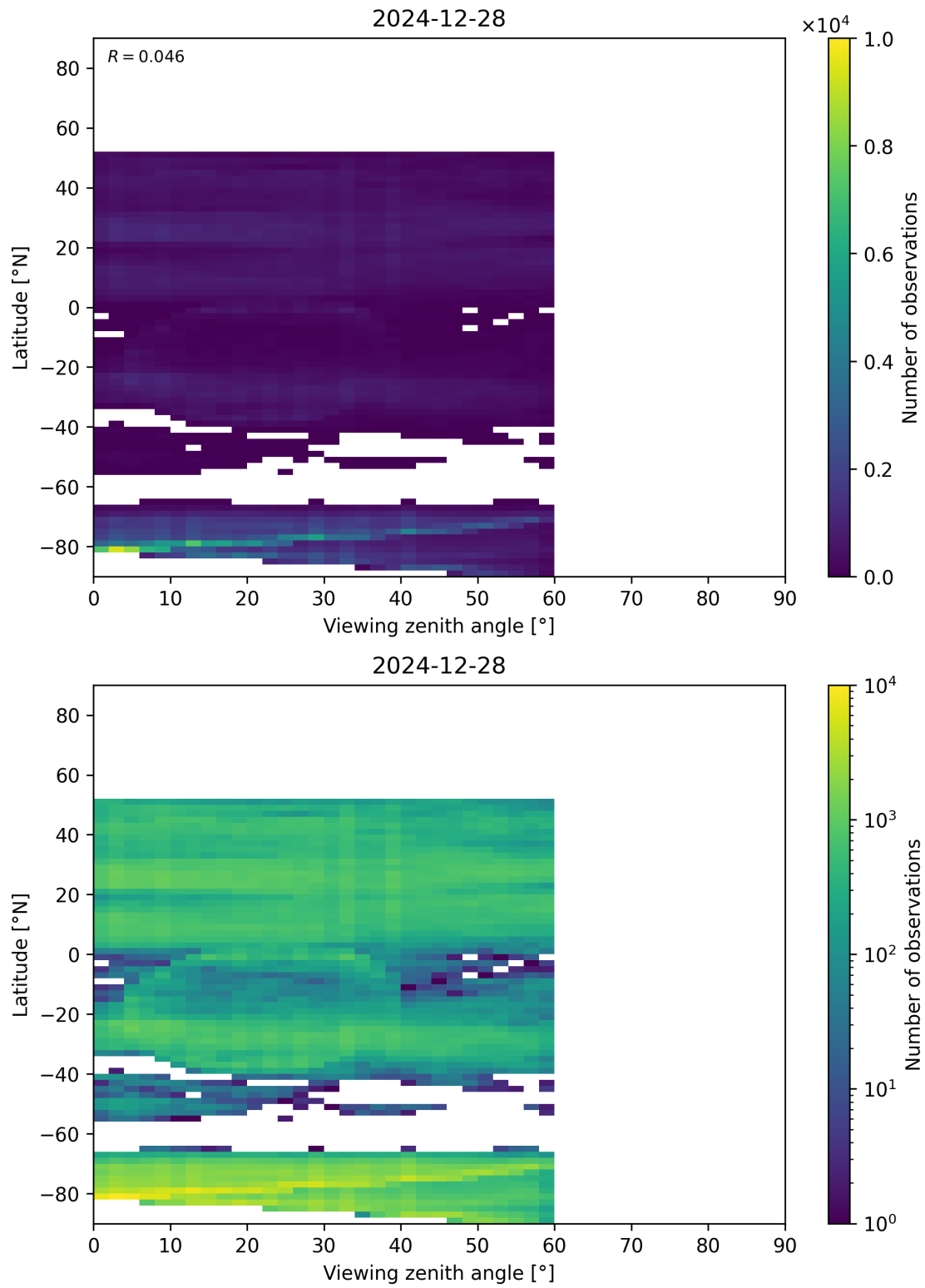
Figure 109: Scatter density plot of “Viewing zenith angle” against “Latitude” for 2024-12-27 to 2024-12-29.
