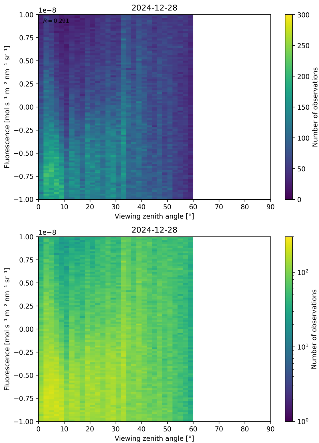
Figure 108: Scatter density plot of “Viewing zenith angle” against “Fluorescence” for 2024-12-27 to 2024-12-29.
