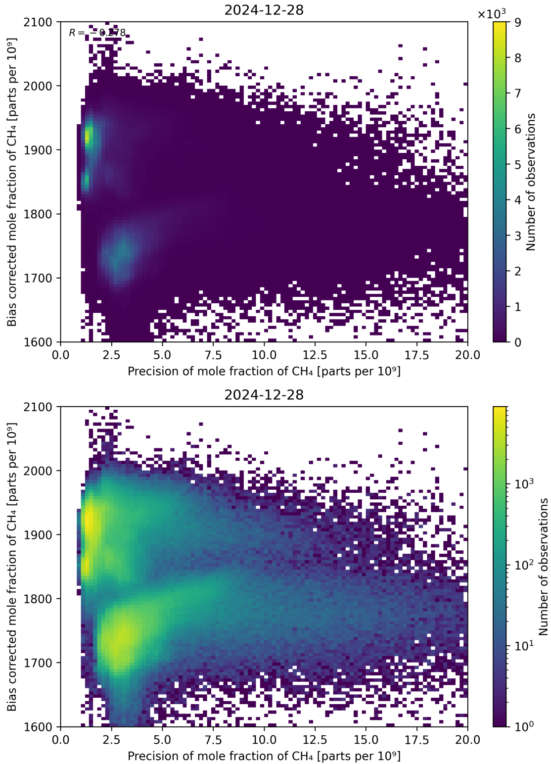
Figure 82: Scatter density plot of “Precision of mole fraction of CH 4 ” against “Bias corrected mole fraction of CH 4 ” for 2024-12-27 to 2024-12-29.
