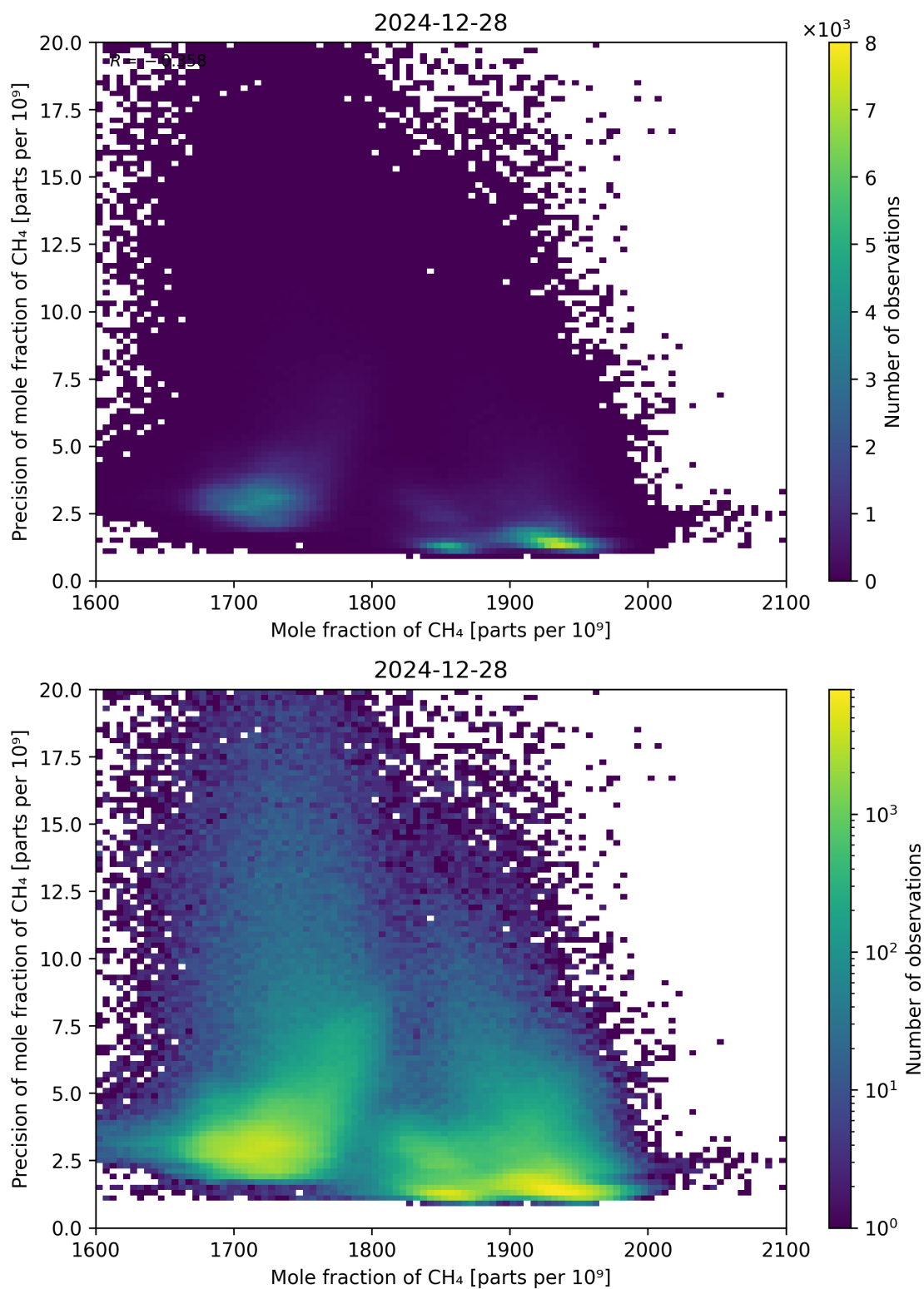
Figure 75: Scatter density plot of “Mole fraction of CH 4 ” against “Precision of mole fraction of CH 4 ” for 2024-12-27 to 2024-12-29.
