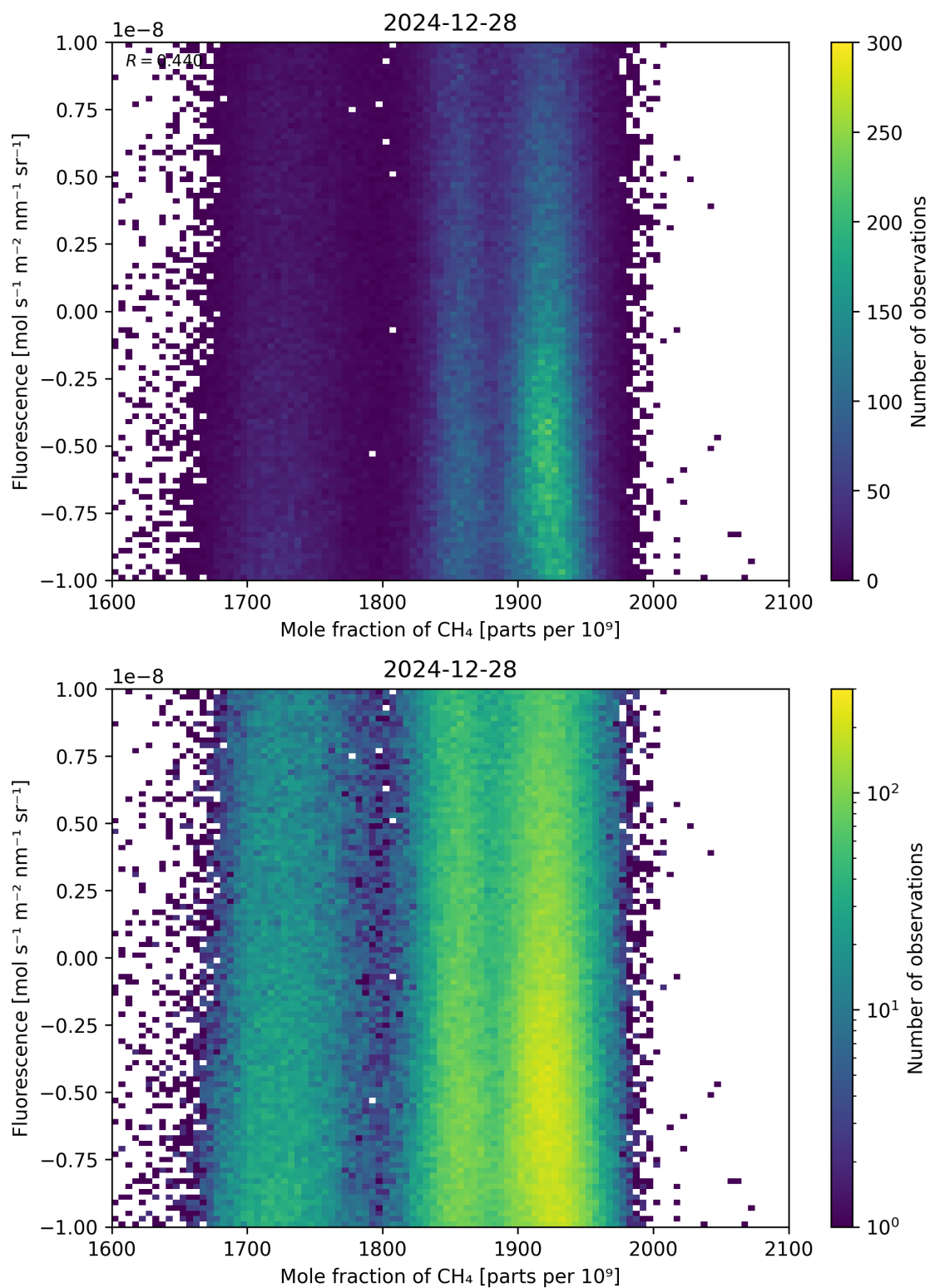
Figure 73: Scatter density plot of “Mole fraction of \text{CH}_4 ” against “Fluorescence” for 2024-12-27 to 2024-12-29.
