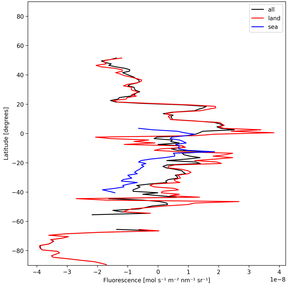
Figure 21: Zonal average of “Fluorescence” for 2024-12-27 to 2024-12-29.
