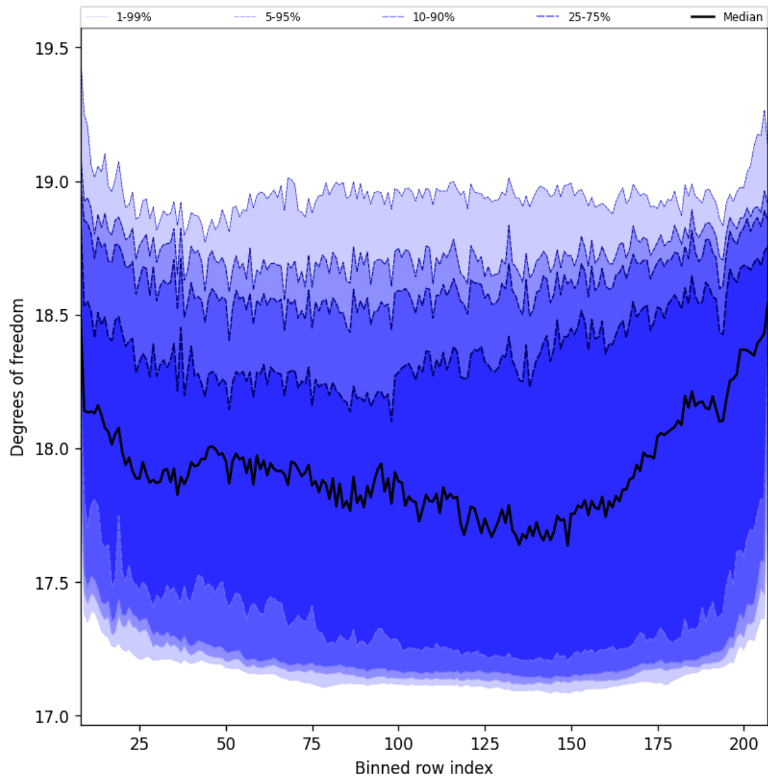
Figure 41: Along track statistics of “Degrees of freedom” for 2024-12-27 to 2024-12-29
