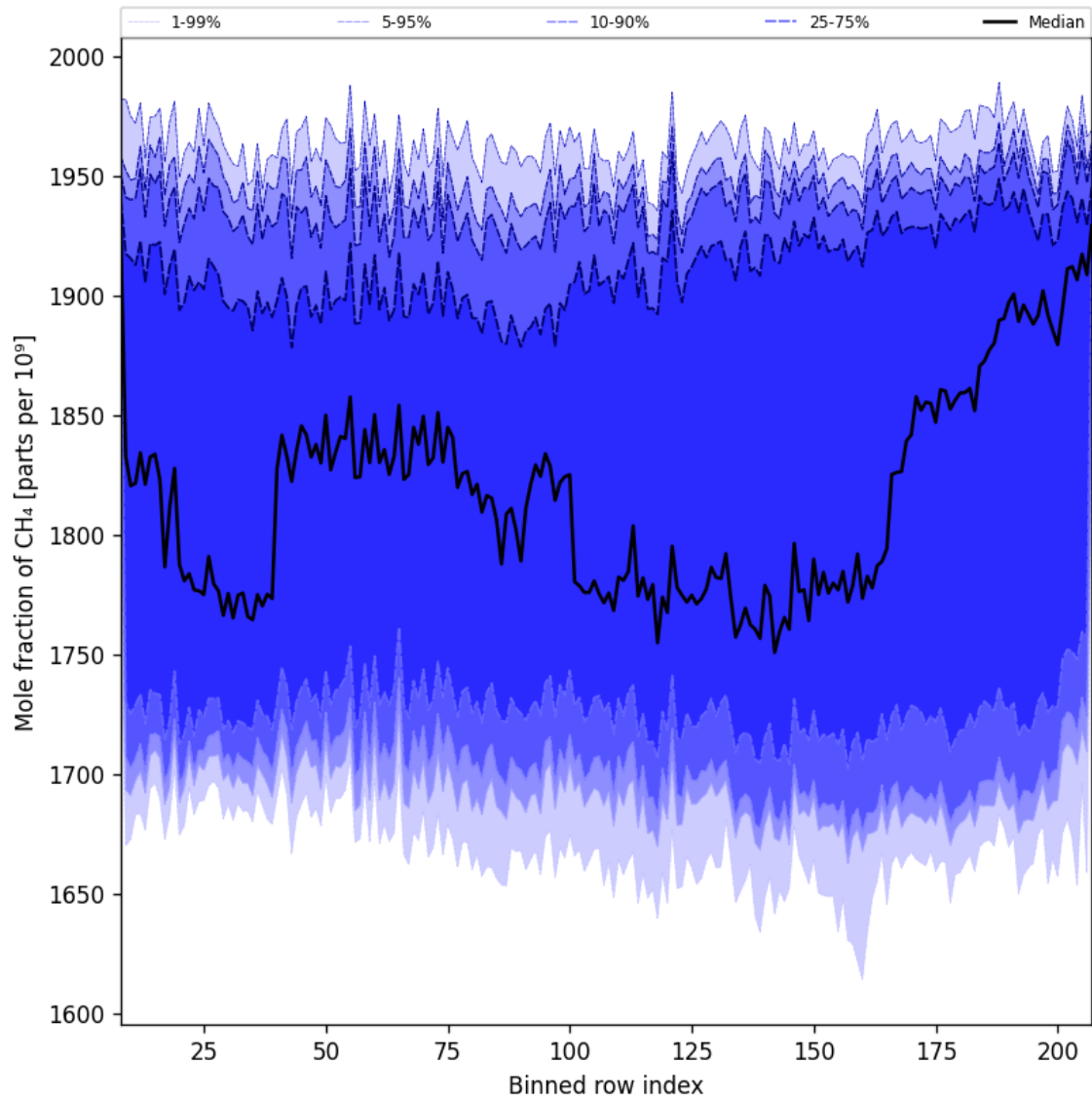
Figure 34: Along track statistics of “Mole fraction of CH 4 ” for 2024-12-27 to 2024-12-29
