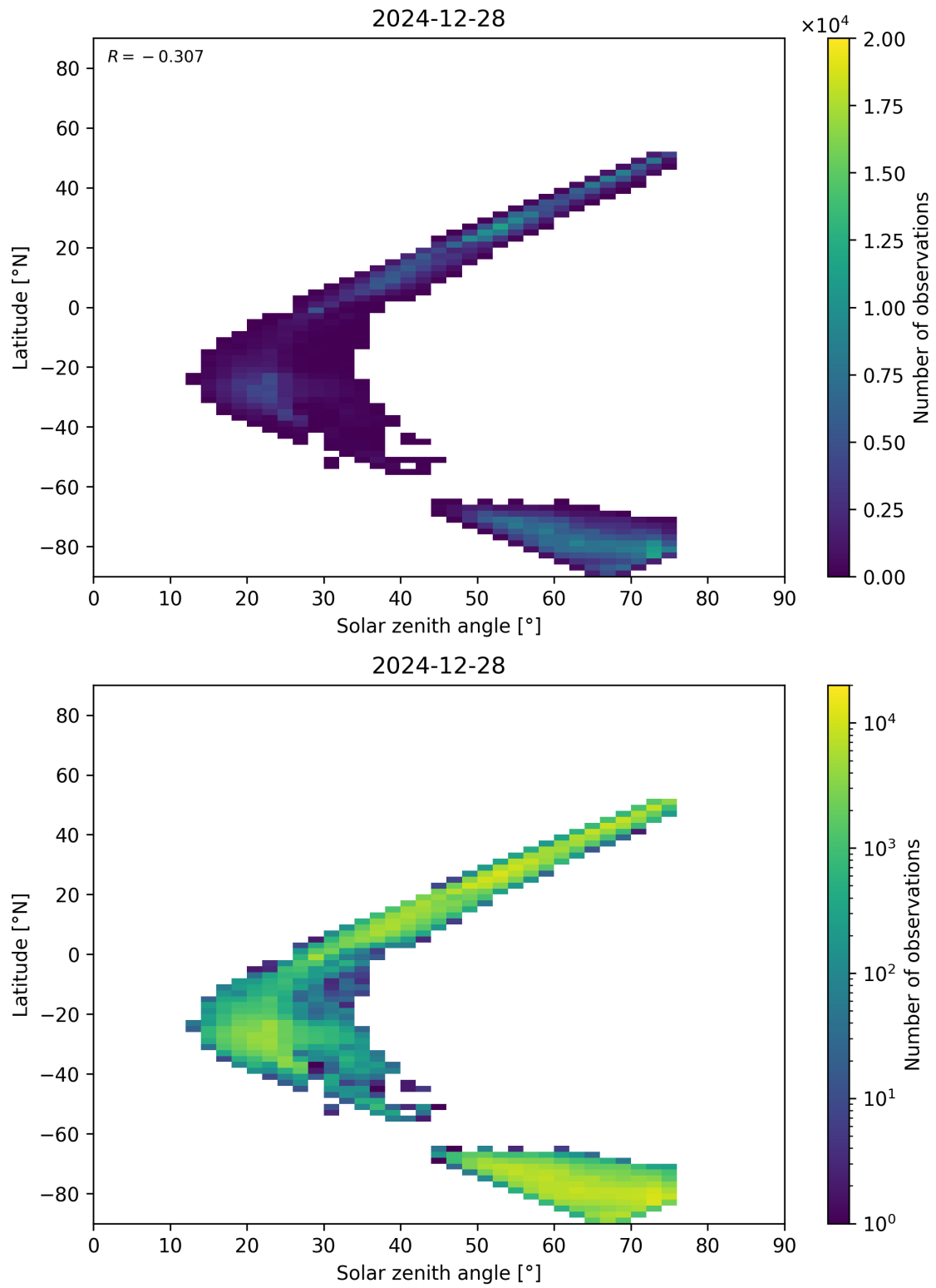
Figure 98: Scatter density plot of “Solar zenith angle” against “Latitude” for 2024-12-27 to 2024-12-29.
