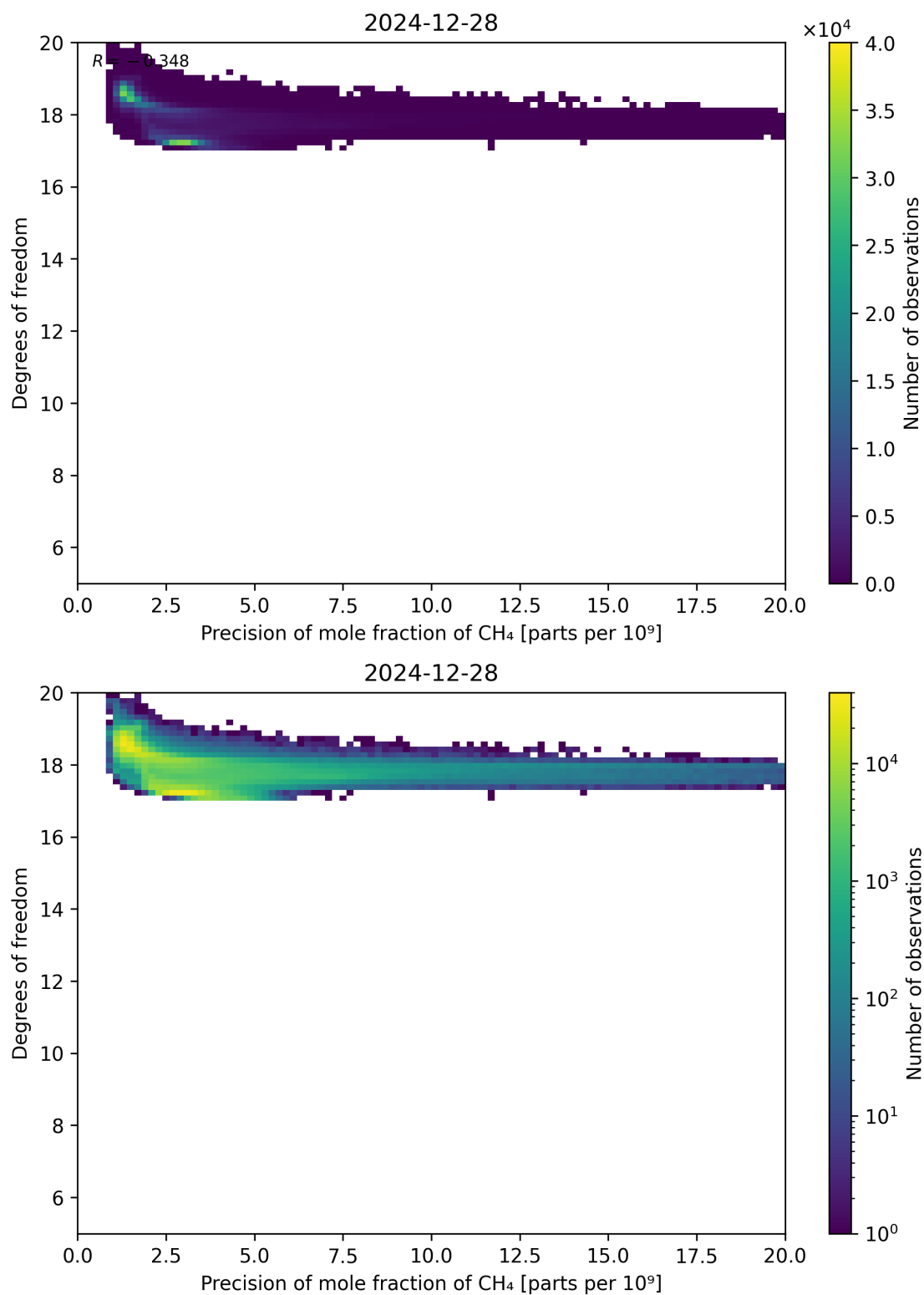
Figure 80: Scatter density plot of “Precision of mole fraction of \text{CH}_4 ” against “Degrees of freedom” for 2024-12-27 to 2024-12-29.
