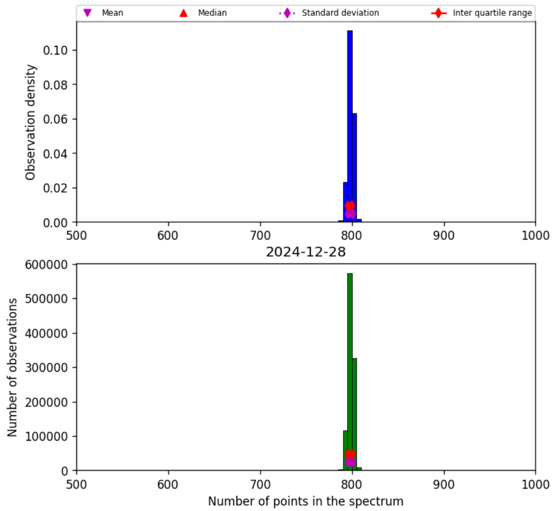
Figure 26: Histogram of “Number of points in the spectrum” for 2024-12-27 to 2024-12-29
