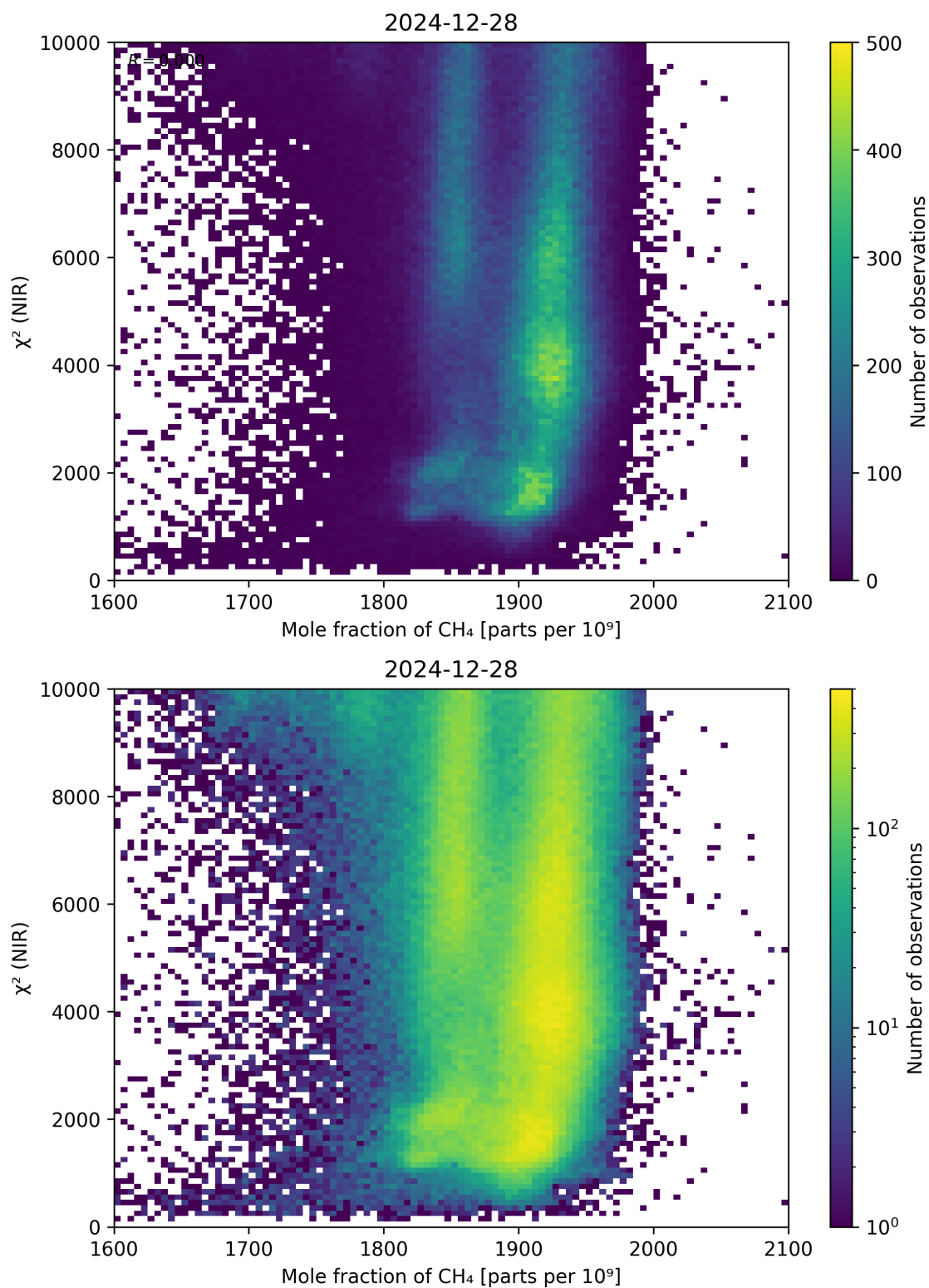
Figure 70: Scatter density plot of “Mole fraction of CH 4 ” against “ \chi^2 (NIR)” for 2024-12-27 to 2024-12-29.
