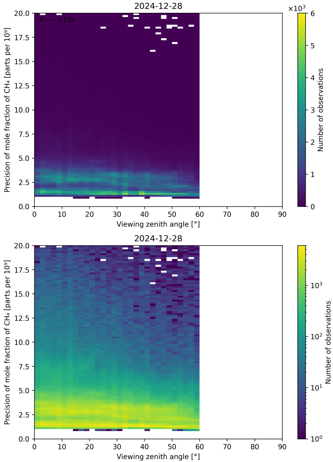
Figure 112: Scatter density plot of “Viewing zenith angle” against “Precision of mole fraction of CH 4 ” for 2024-12-27 to 2024-12-29.
