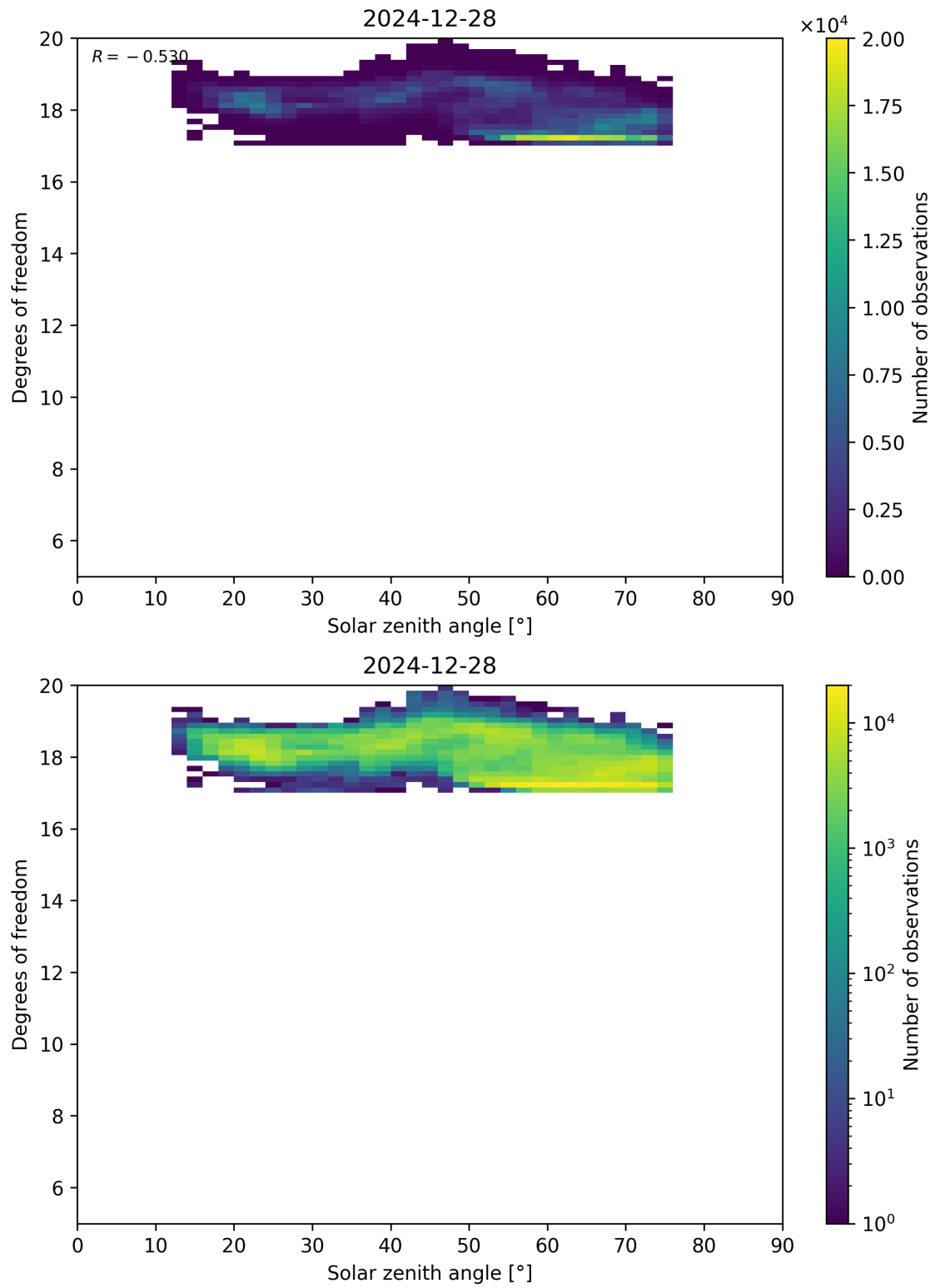
Figure 96: Scatter density plot of “Solar zenith angle” against “Degrees of freedom” for 2024-12-27 to 2024-12-29.
