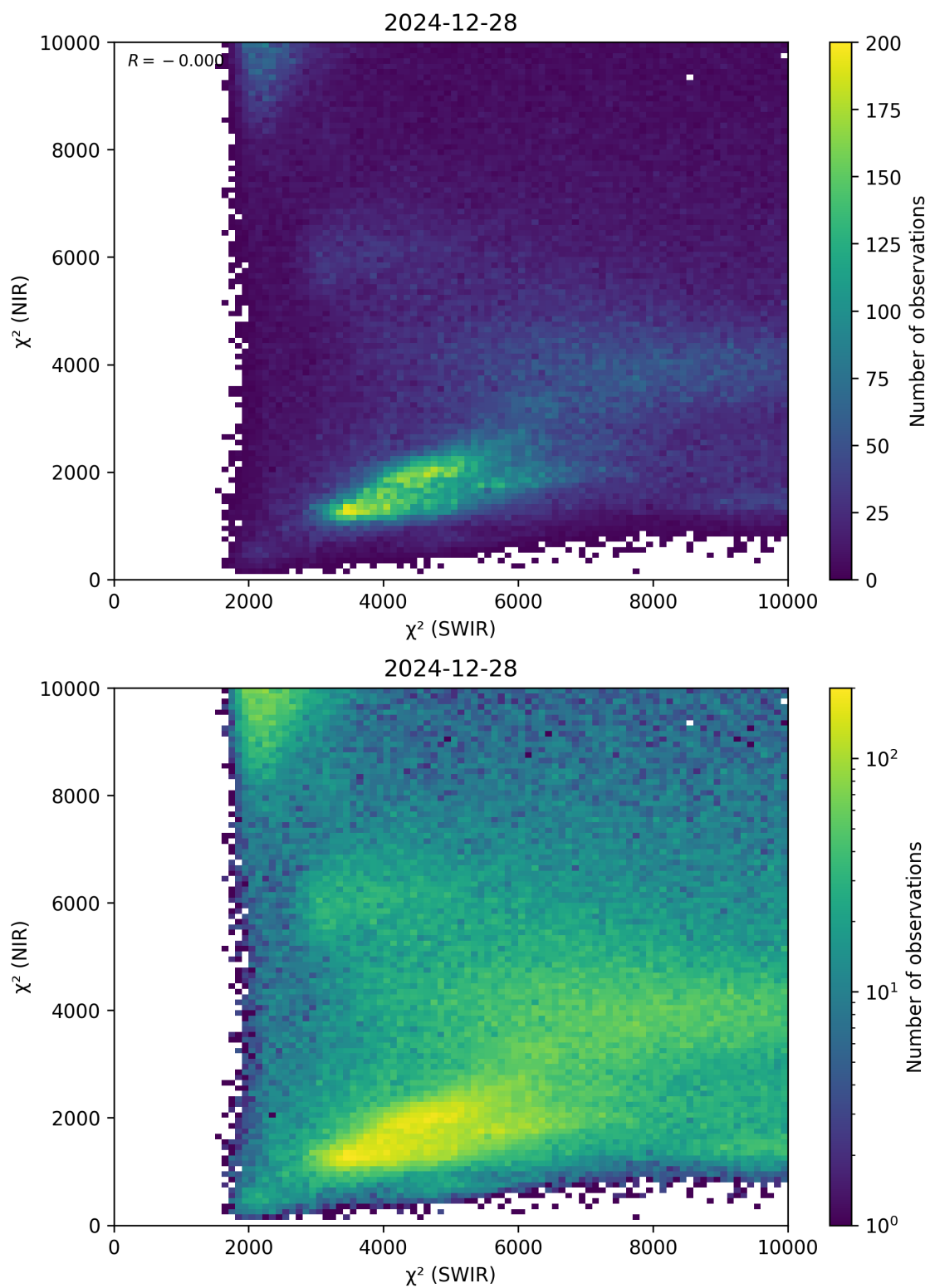
Figure 47: Scatter density plot of “ \chi^2 (SWIR)” against “ \chi^2 (NIR)” for 2024-12-27 to 2024-12-29.
