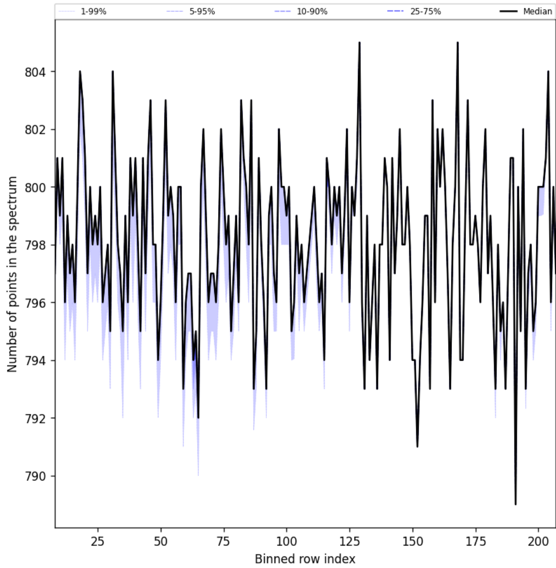
Figure 37: Along track statistics of “Number of points in the spectrum” for 2024-12-27 to 2024-12-29
