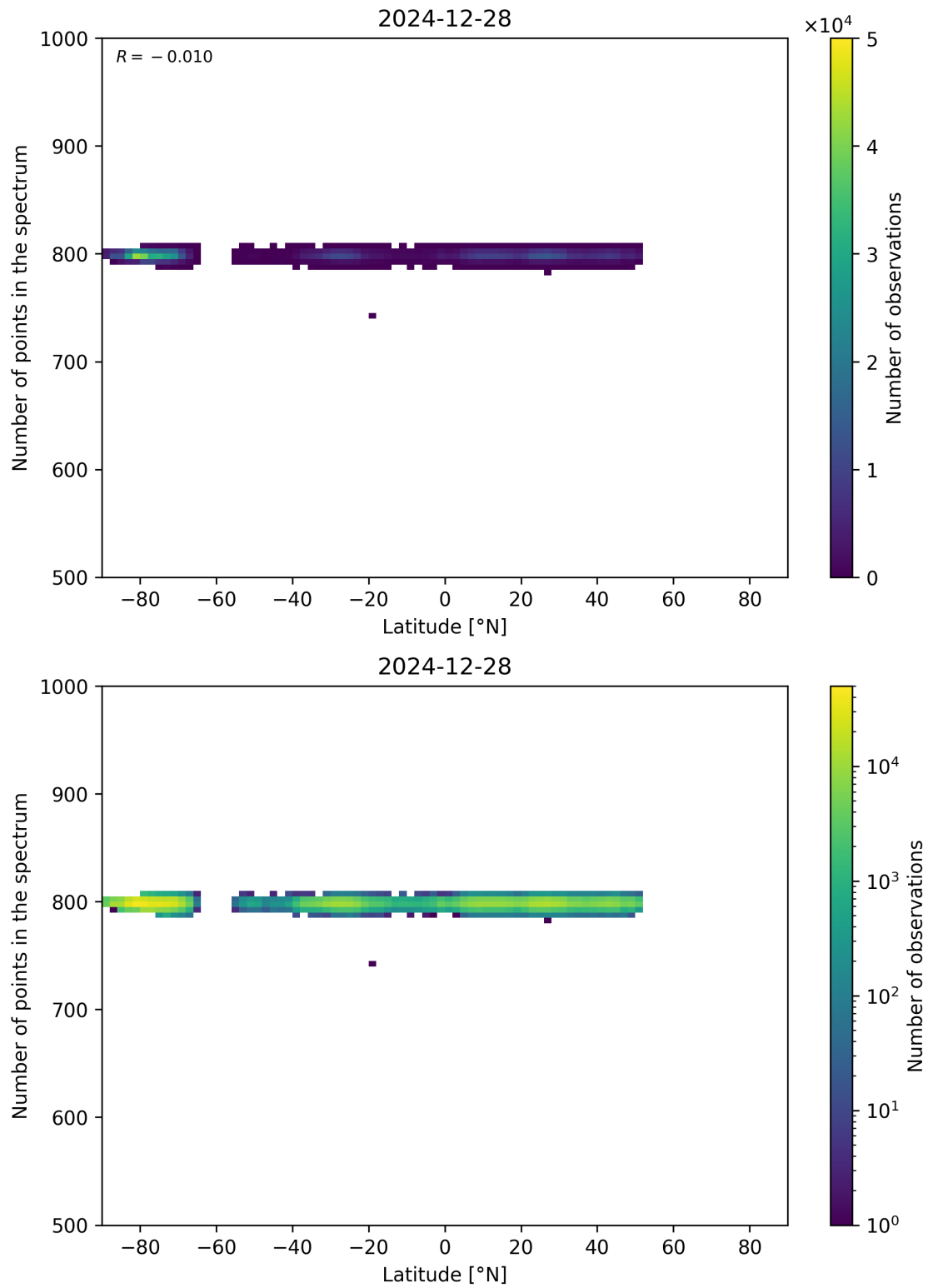
Figure 61: Scatter density plot of “Latitude” against “Number of points in the spectrum” for 2024-12-27 to 2024-12-29.
