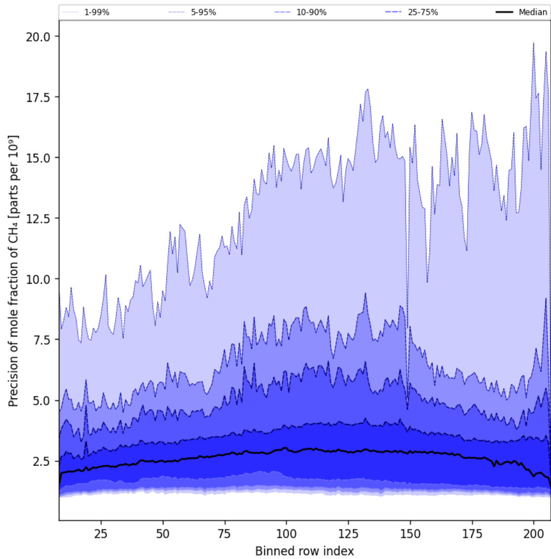
Figure 35: Along track statistics of “Precision of mole fraction of CH 4 ” for 2024-12-27 to 2024-12-29
