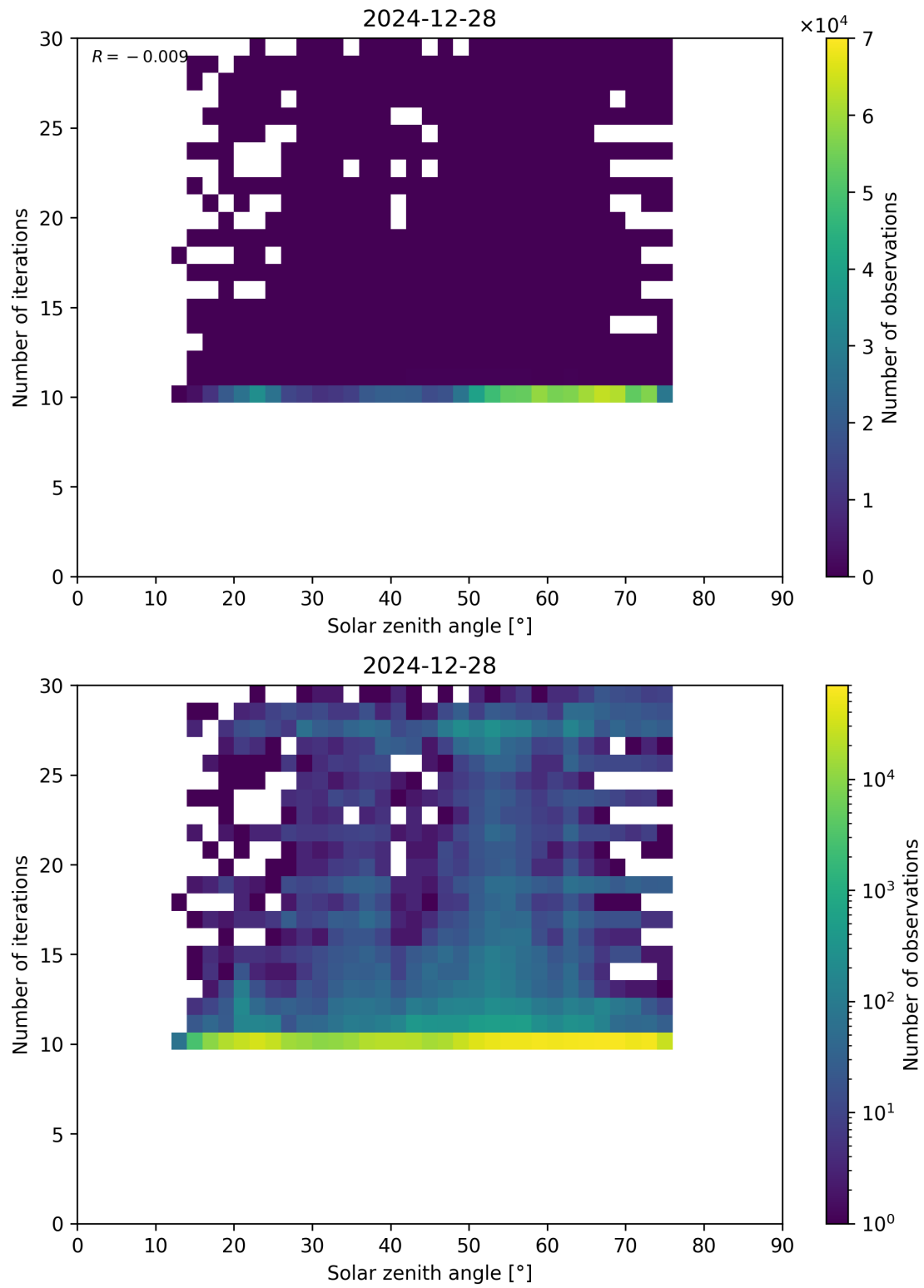
Figure 102: Scatter density plot of “Solar zenith angle” against “Number of iterations” for 2024-12-27 to 2024-12-29.
