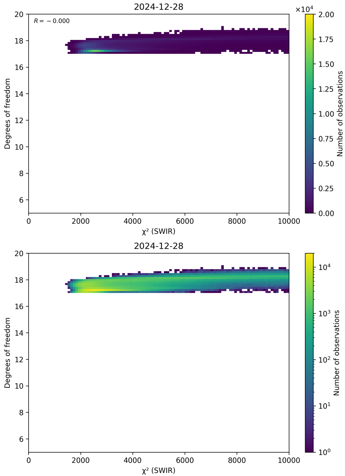
Figure 48: Scatter density plot of “ \chi^2 (SWIR)” against “Degrees of freedom” for 2024-12-27 to 2024-12-29.
