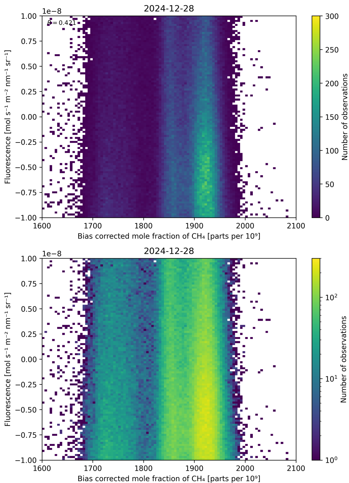
Figure 66: Scatter density plot of “Bias corrected mole fraction of \text{CH}_4 ” against “Fluorescence” for 2024-12-27 to 2024-12-29.
