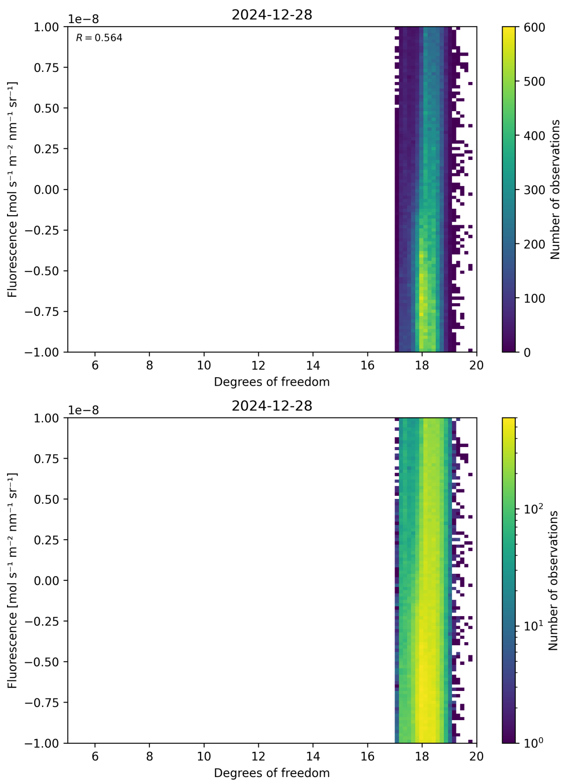
Figure 51: Scatter density plot of “Degrees of freedom” against “Fluorescence” for 2024-12-27 to 2024-12-29.
