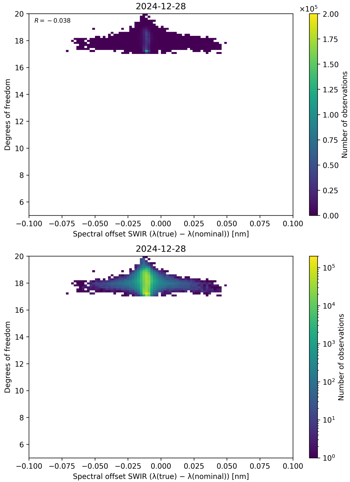
Figure 119: Scatter density plot of “Spectral offset SWIR ( \lambda_{\text{true}} - \lambda_{\text{nominal}} )” against “Degrees of freedom” for 2024-12-27 to 2024-12-29.
