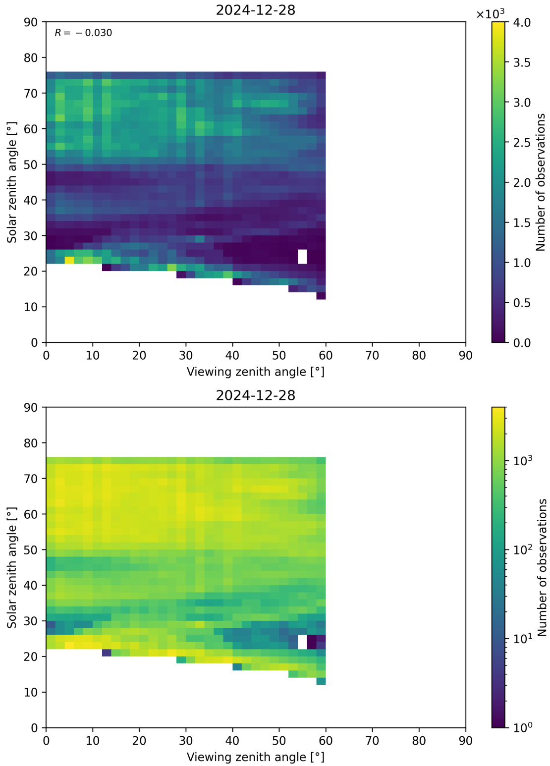
Figure 115: Scatter density plot of “Viewing zenith angle” against “Solar zenith angle” for 2024-12-27 to 2024-12-29.
