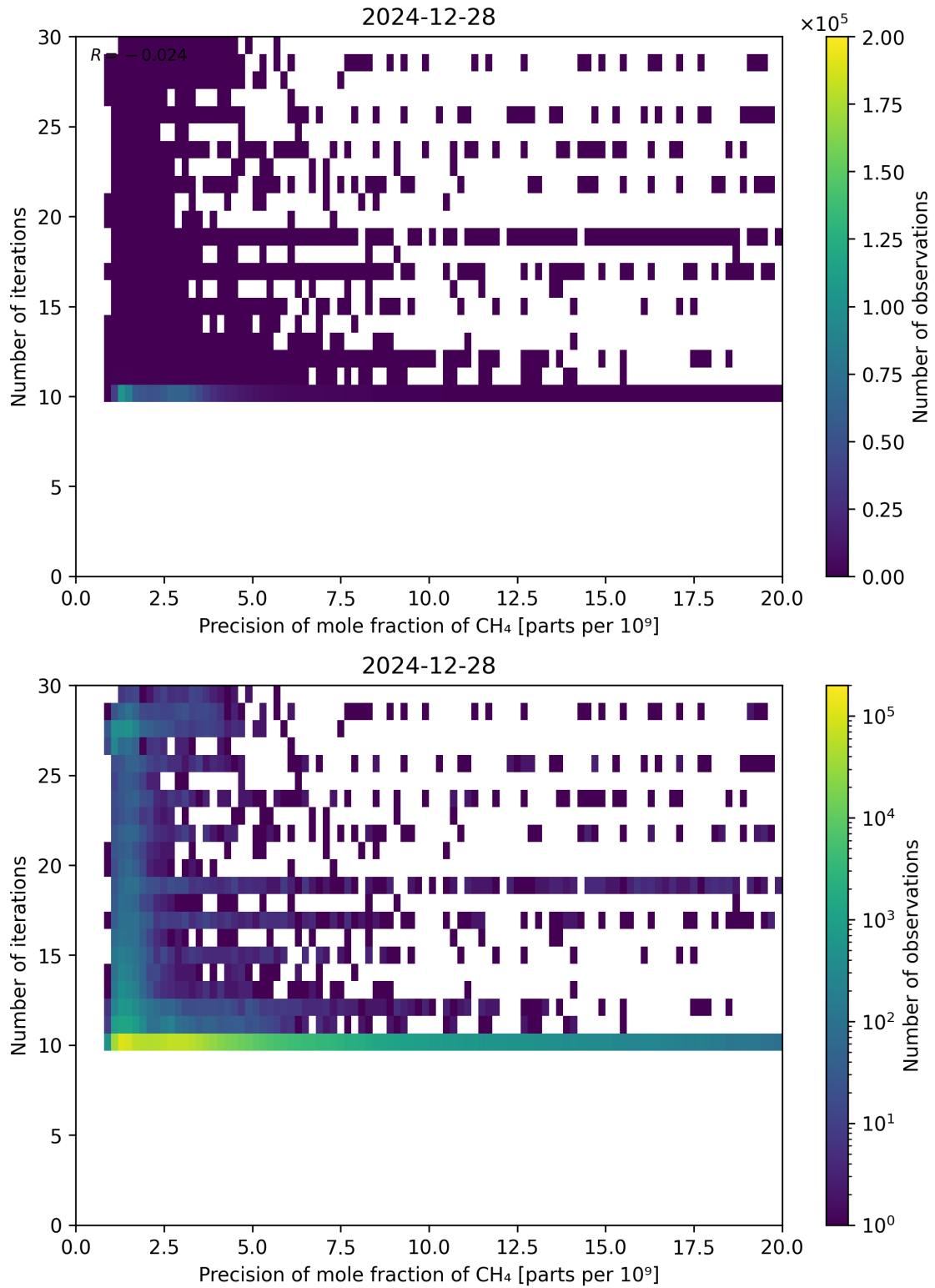
Figure 83: Scatter density plot of “Precision of mole fraction of CH 4 ” against “Number of iterations” for 2024-12-27 to 2024-12-29.
