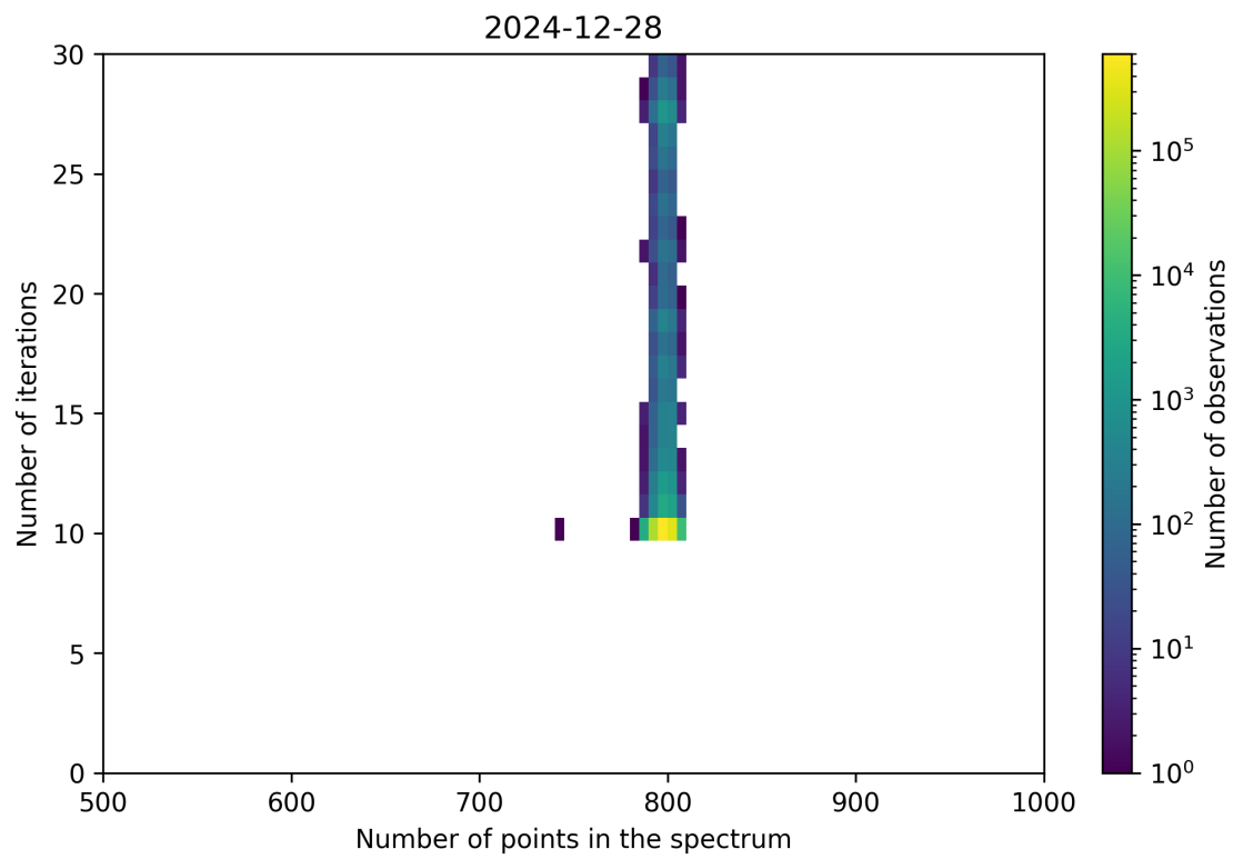
Figure 92: Scatter density plot of “Number of points in the spectrum” against “Number of iterations” for 2024-12-27 to 2024-12-29.
