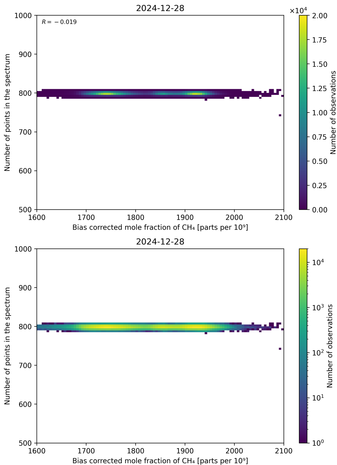
Figure 68: Scatter density plot of “Bias corrected mole fraction of CH 4 ” against “Number of points in the spectrum” for 2024-12-27 to 2024-12-29.
