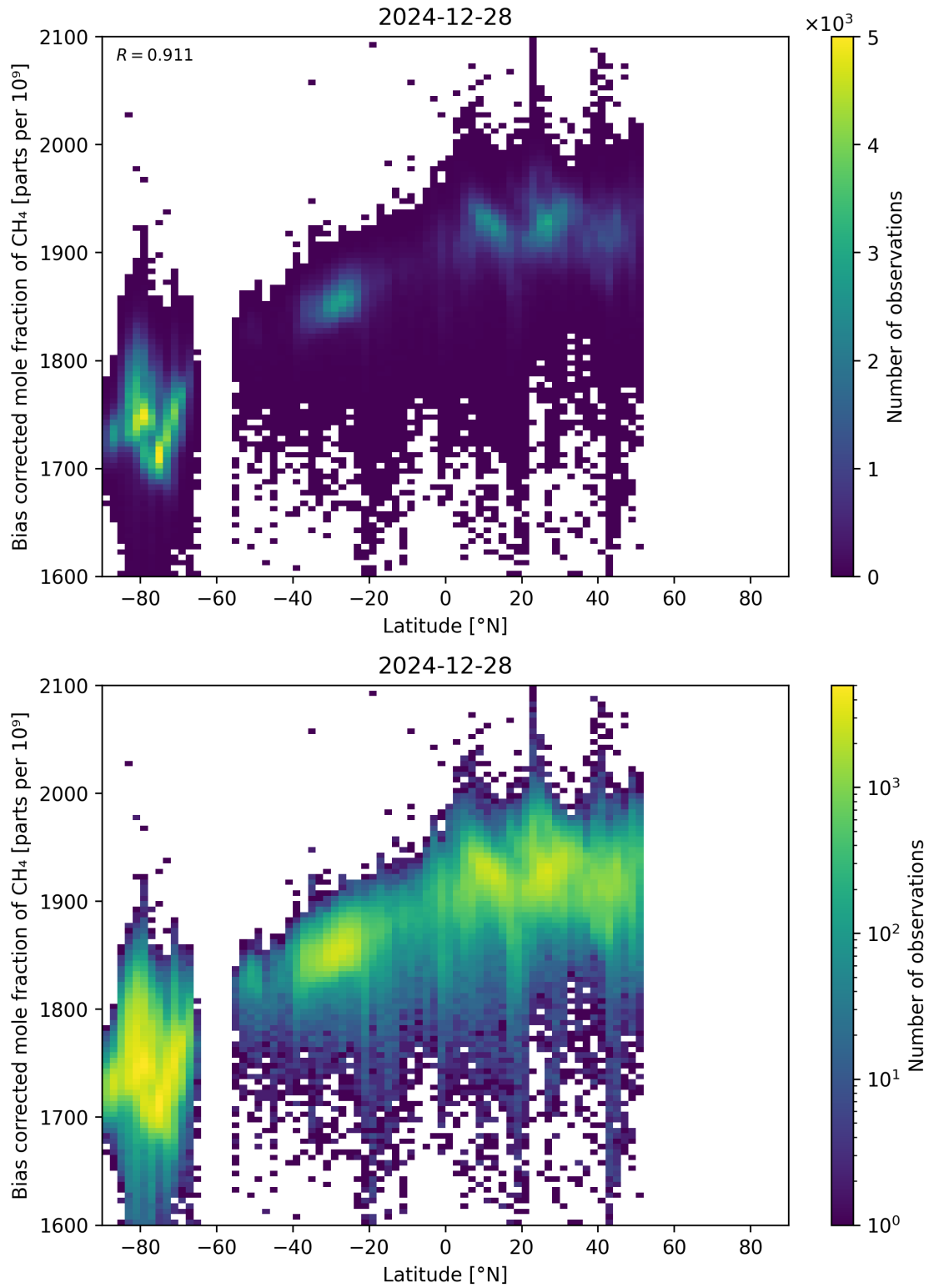
Figure 58: Scatter density plot of “Latitude” against “Bias corrected mole fraction of \text{CH}_4 ” for 2024-12-27 to 2024-12-29.
