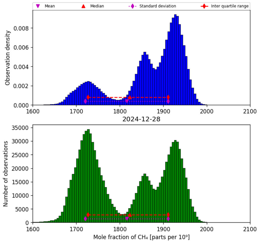
Figure 23: Histogram of “Mole fraction of CH 4 ” for 2024-12-27 to 2024-12-29
