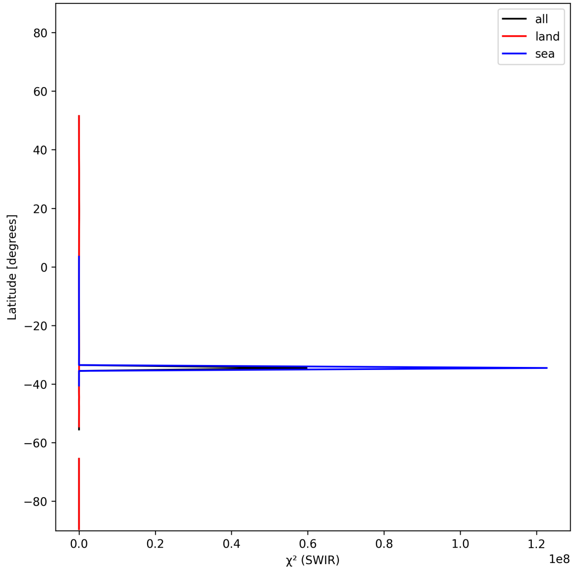
Figure 17: Zonal average of “ \chi^2 (SWIR)” for 2024-12-27 to 2024-12-29.
