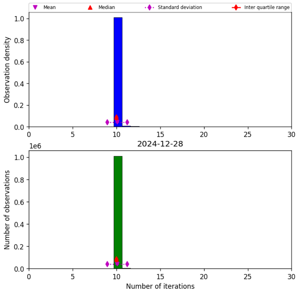
Figure 31: Histogram of “Number of iterations” for 2024-12-27 to 2024-12-29
