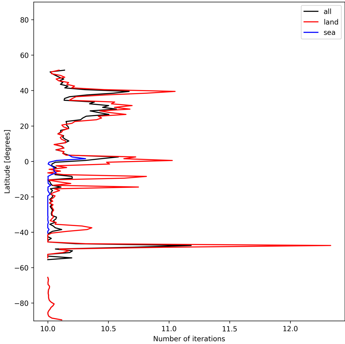
Figure 20: Zonal average of “Number of iterations” for 2024-12-27 to 2024-12-29.
