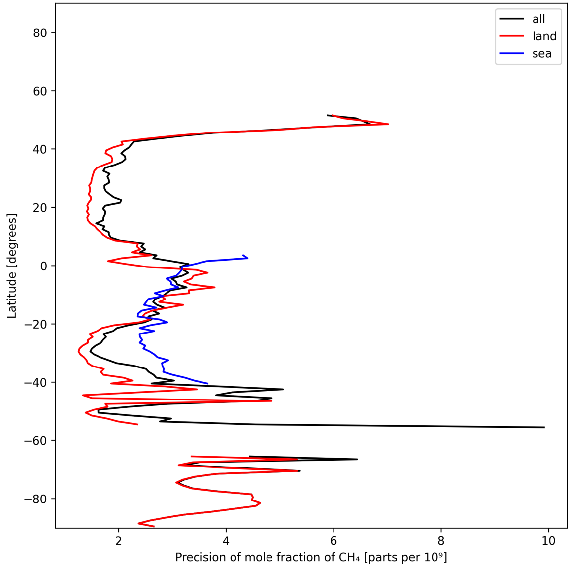
Figure 13: Zonal average of “Precision of mole fraction of CH 4 ” for 2024-12-27 to 2024-12-29.
