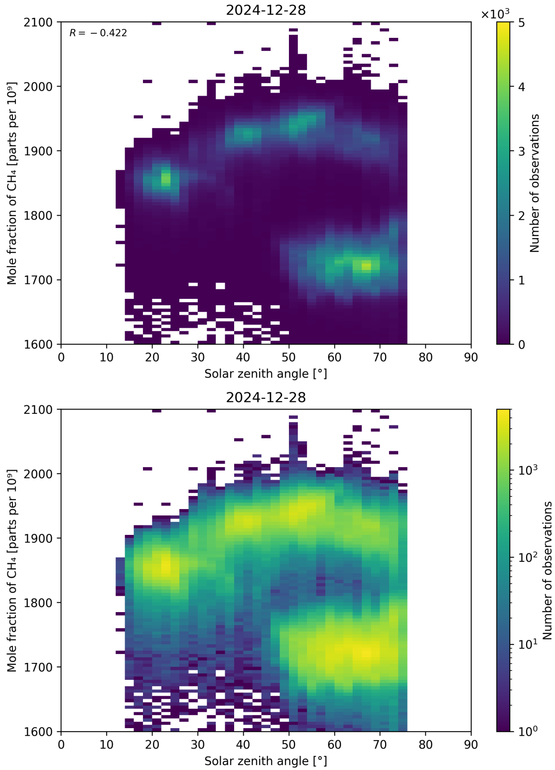
Figure 99: Scatter density plot of “Solar zenith angle” against “Mole fraction of \text{CH}_4 ” for 2024-12-27 to 2024-12-29.
