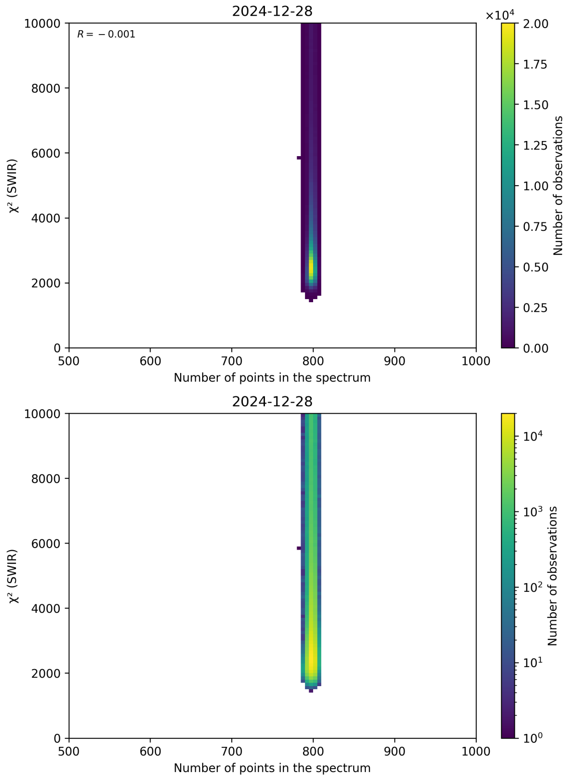
Figure 89: Scatter density plot of “Number of points in the spectrum” against “ \chi^2 (SWIR)” for 2024-12-27 to 2024-12-29.
