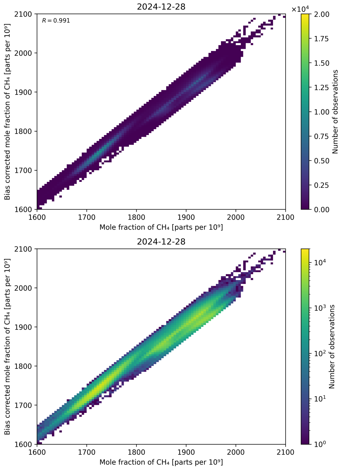
Figure 74: Scatter density plot of “Mole fraction of CH 4 ” against “Bias corrected mole fraction of CH 4 ” for 2024-12-27 to 2024-12-29.
