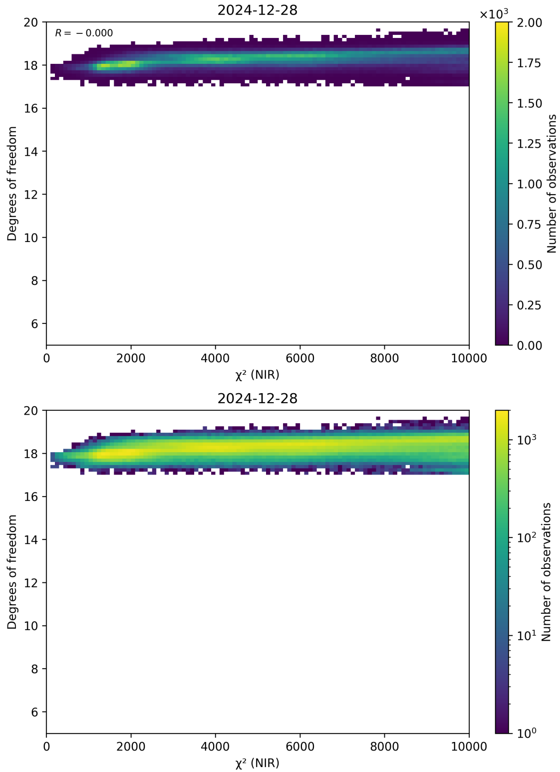
Figure 44: Scatter density plot of “ \chi^2 (NIR)” against “Degrees of freedom” for 2024-12-27 to 2024-12-29.
