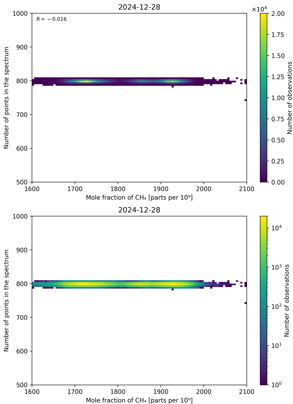
Figure 77: Scatter density plot of “Mole fraction of CH 4 ” against “Number of points in the spectrum” for 2024-12-27 to 2024-12-29.
