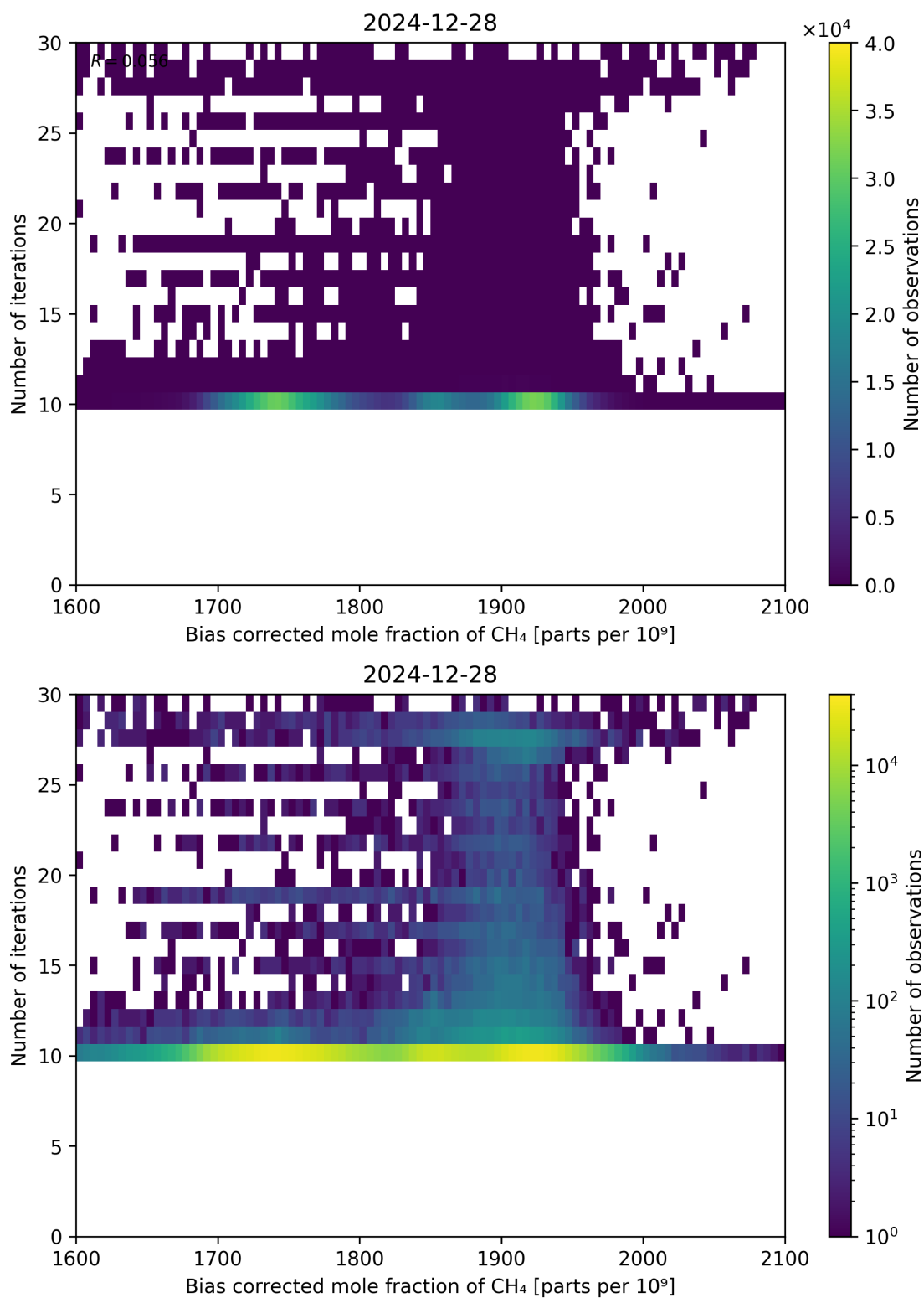
Figure 67: Scatter density plot of “Bias corrected mole fraction of \text{CH}_4 ” against “Number of iterations” for 2024-12-27 to 2024-12-29.
