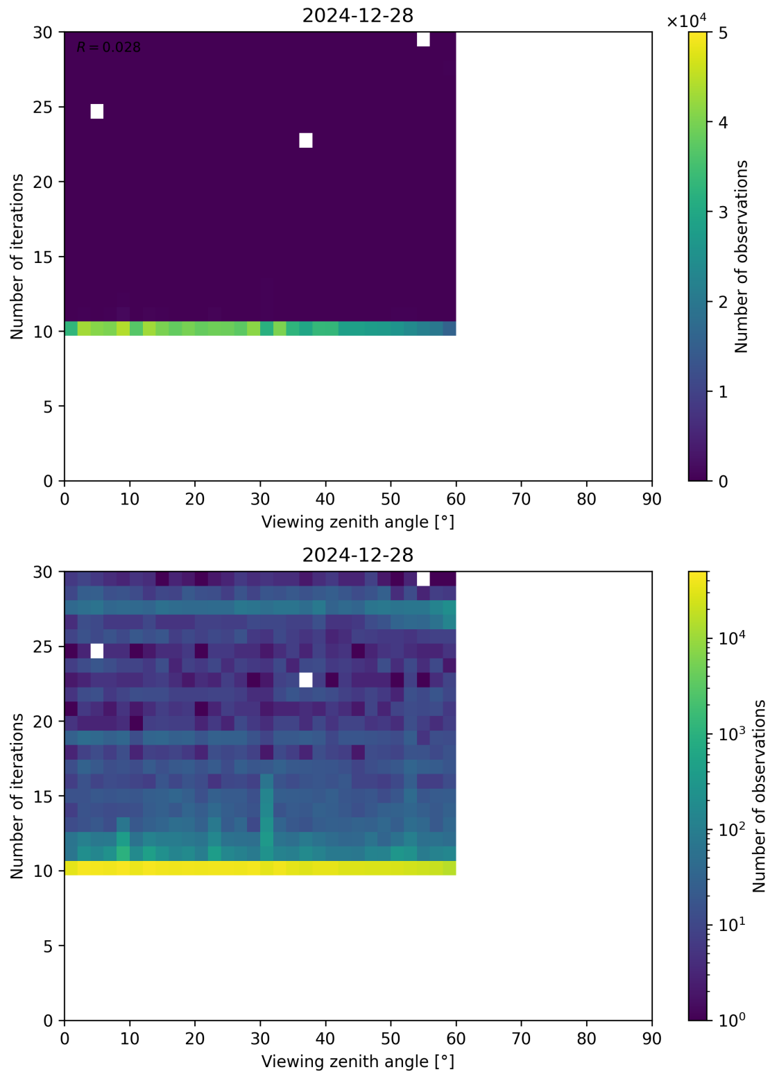
Figure 113: Scatter density plot of “Viewing zenith angle” against “Number of iterations” for 2024-12-27 to 2024-12-29.
