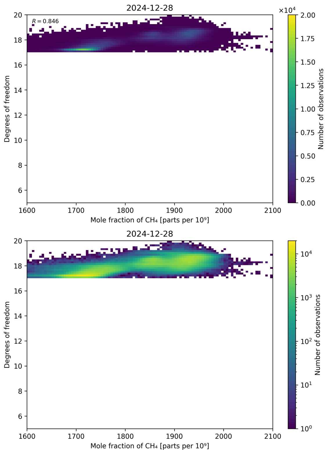
Figure 72: Scatter density plot of “Mole fraction of CH 4 ” against “Degrees of freedom” for 2024-12-27 to 2024-12-29.
