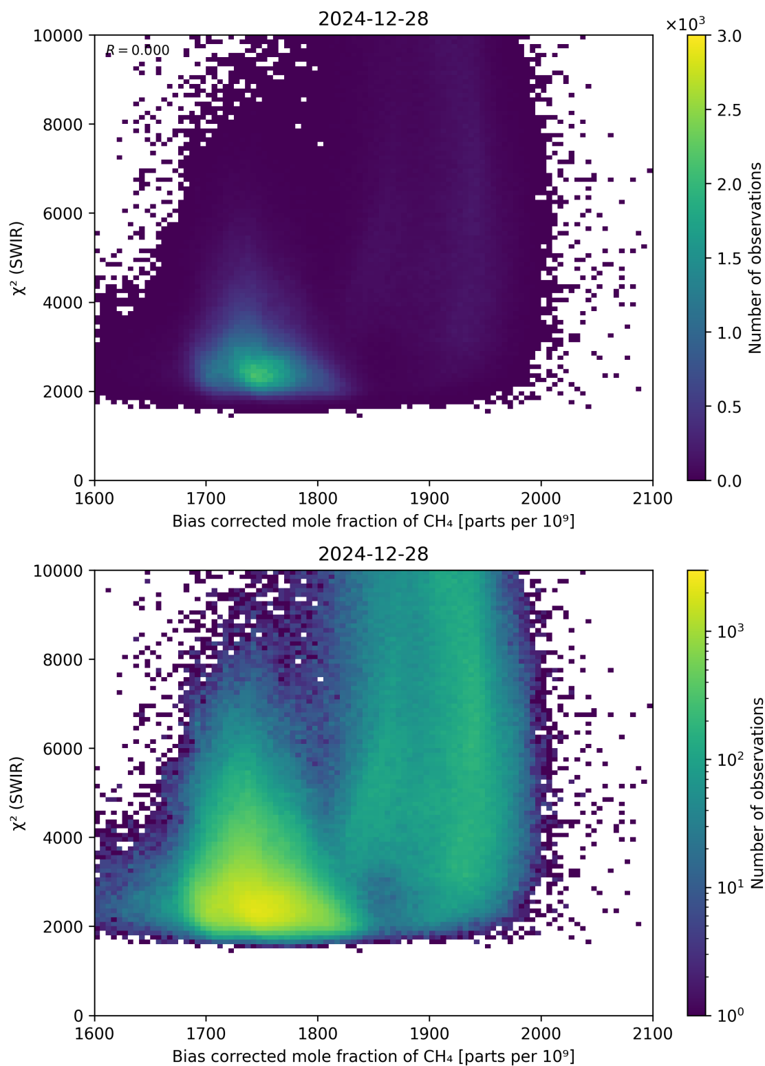
Figure 64: Scatter density plot of “Bias corrected mole fraction of CH 4 ” against “ \chi^2 (SWIR)” for 2024-12-27 to 2024-12-29.
