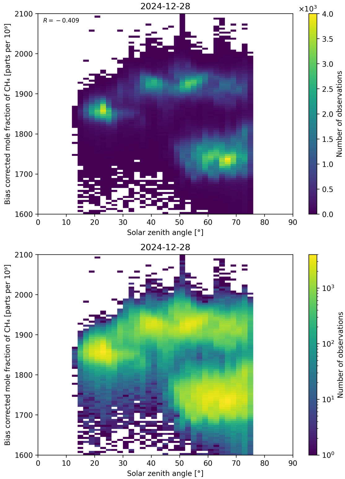
Figure 100: Scatter density plot of “Solar zenith angle” against “Bias corrected mole fraction of CH 4 ” for 2024-12-27 to 2024-12-29.
