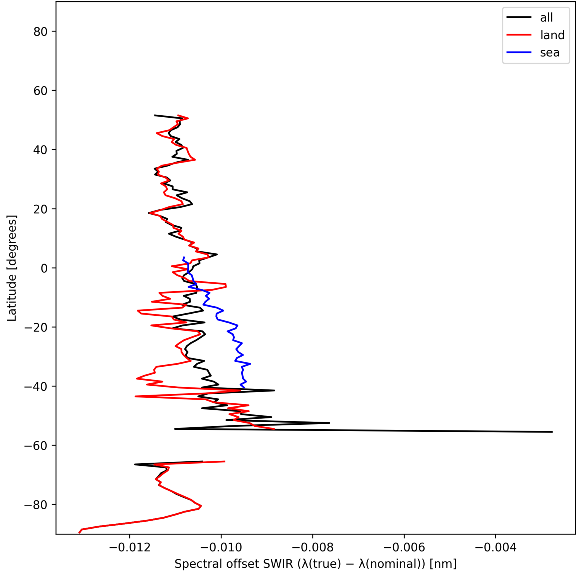
Figure 16: Zonal average of “Spectral offset SWIR ( \lambda_{\text{true}} - \lambda_{\text{nominal}} )” for 2024-12-27 to 2024-12-29.
