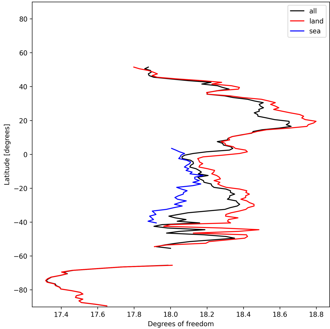
Figure 19: Zonal average of “Degrees of freedom” for 2024-12-27 to 2024-12-29.
