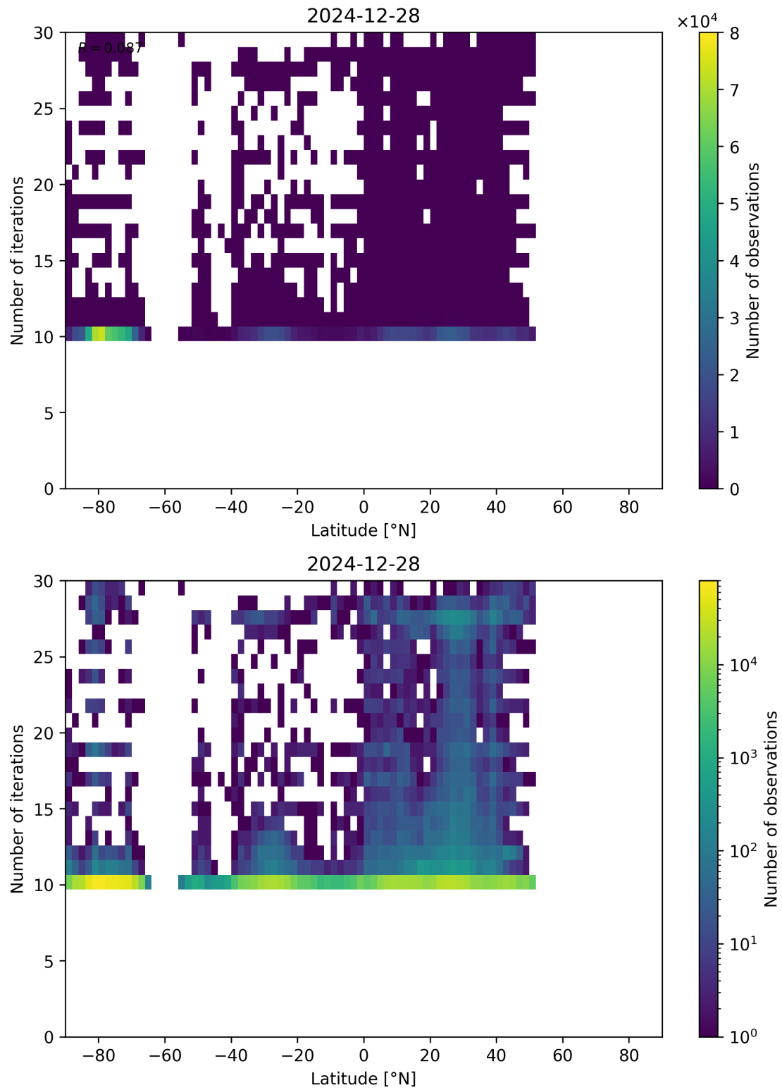
Figure 60: Scatter density plot of “Latitude” against “Number of iterations” for 2024-12-27 to 2024-12-29.
