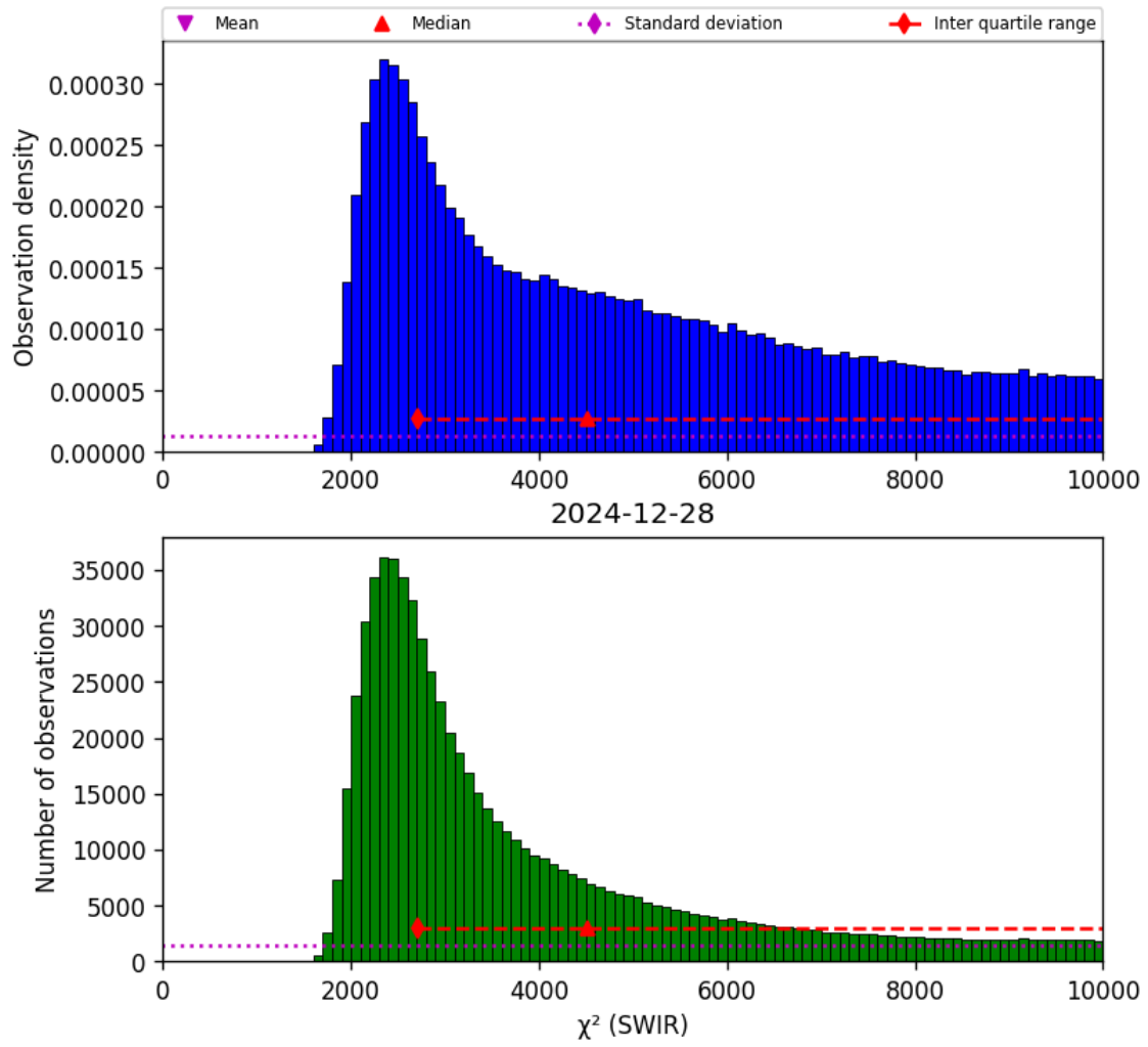
Figure 28: Histogram of “ \chi^2 (SWIR)” for 2024-12-27 to 2024-12-29
