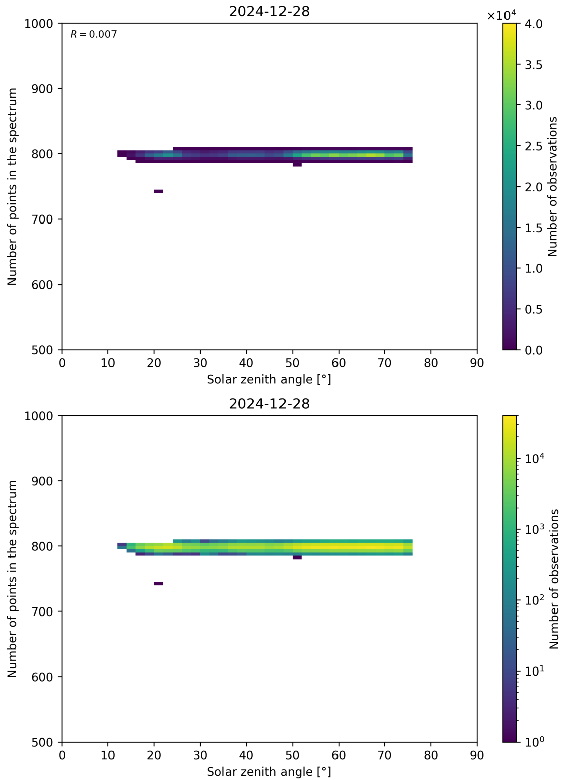
Figure 103: Scatter density plot of “Solar zenith angle” against “Number of points in the spectrum” for 2024-12-27 to 2024-12-29.
