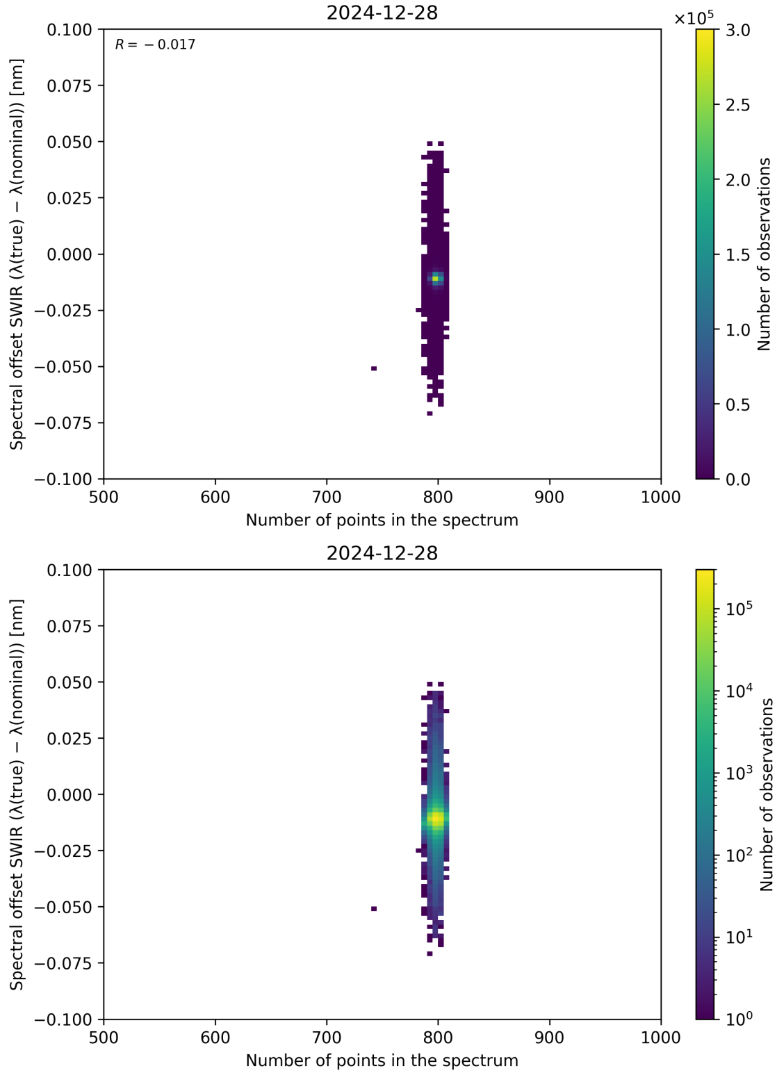
Figure 93: Scatter density plot of “Number of points in the spectrum” against “Spectral offset SWIR ( \lambda_{\text{true}} - \lambda_{\text{nominal}} )” for 2024-12-27 to 2024-12-29.
