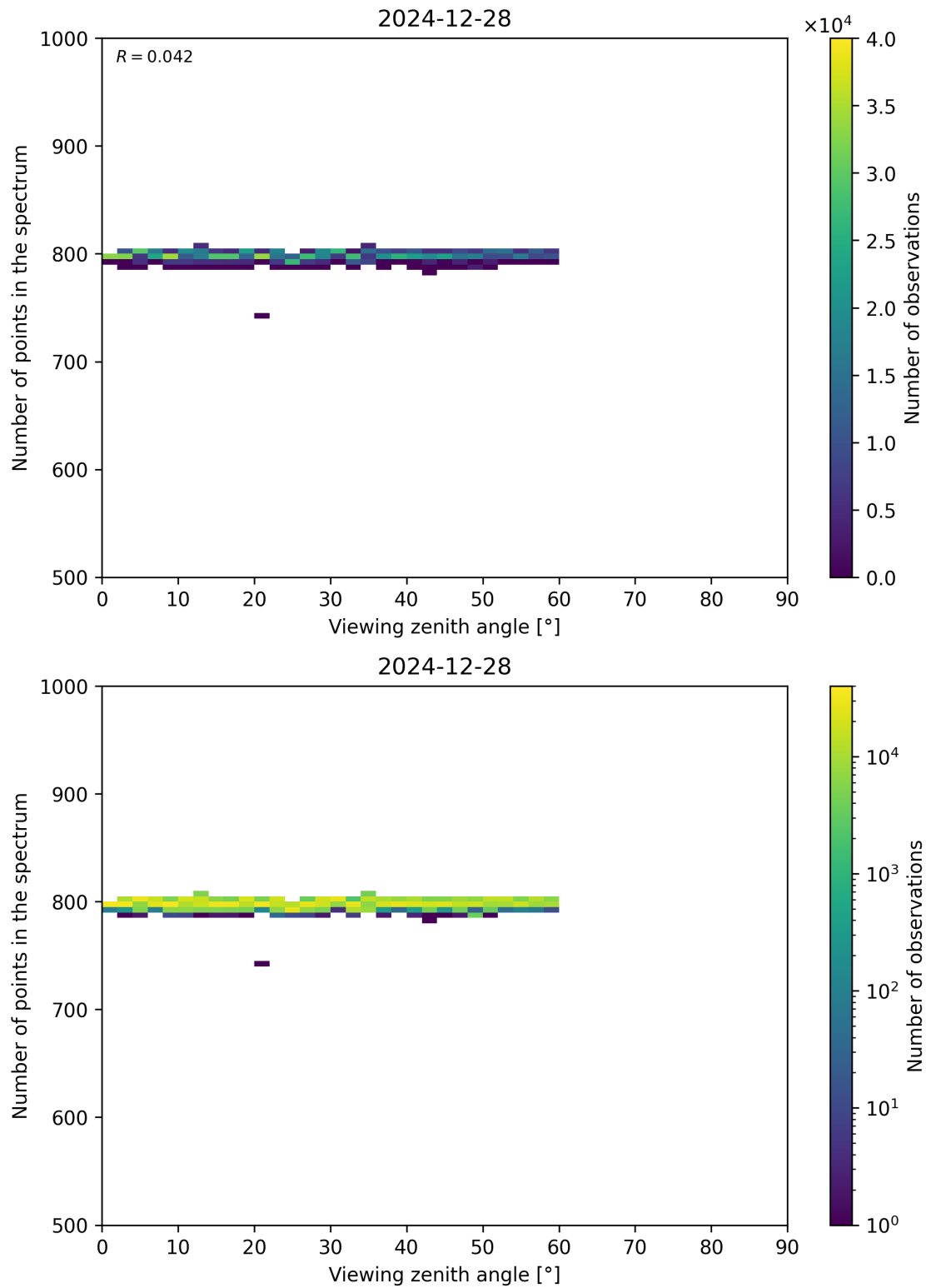
Figure 114: Scatter density plot of “Viewing zenith angle” against “Number of points in the spectrum” for 2024-12-27 to 2024-12-29.
