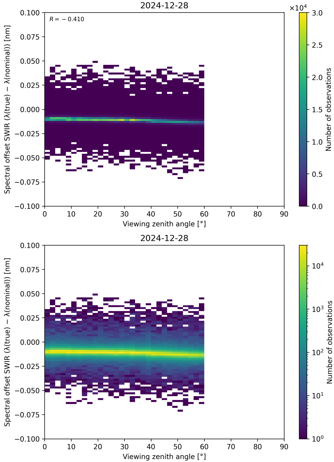
Figure 116: Scatter density plot of “Viewing zenith angle” against “Spectral offset SWIR ( \lambda_{\text{true}} - \lambda_{\text{nominal}} )” for 2024-12-27 to 2024-12-29.
