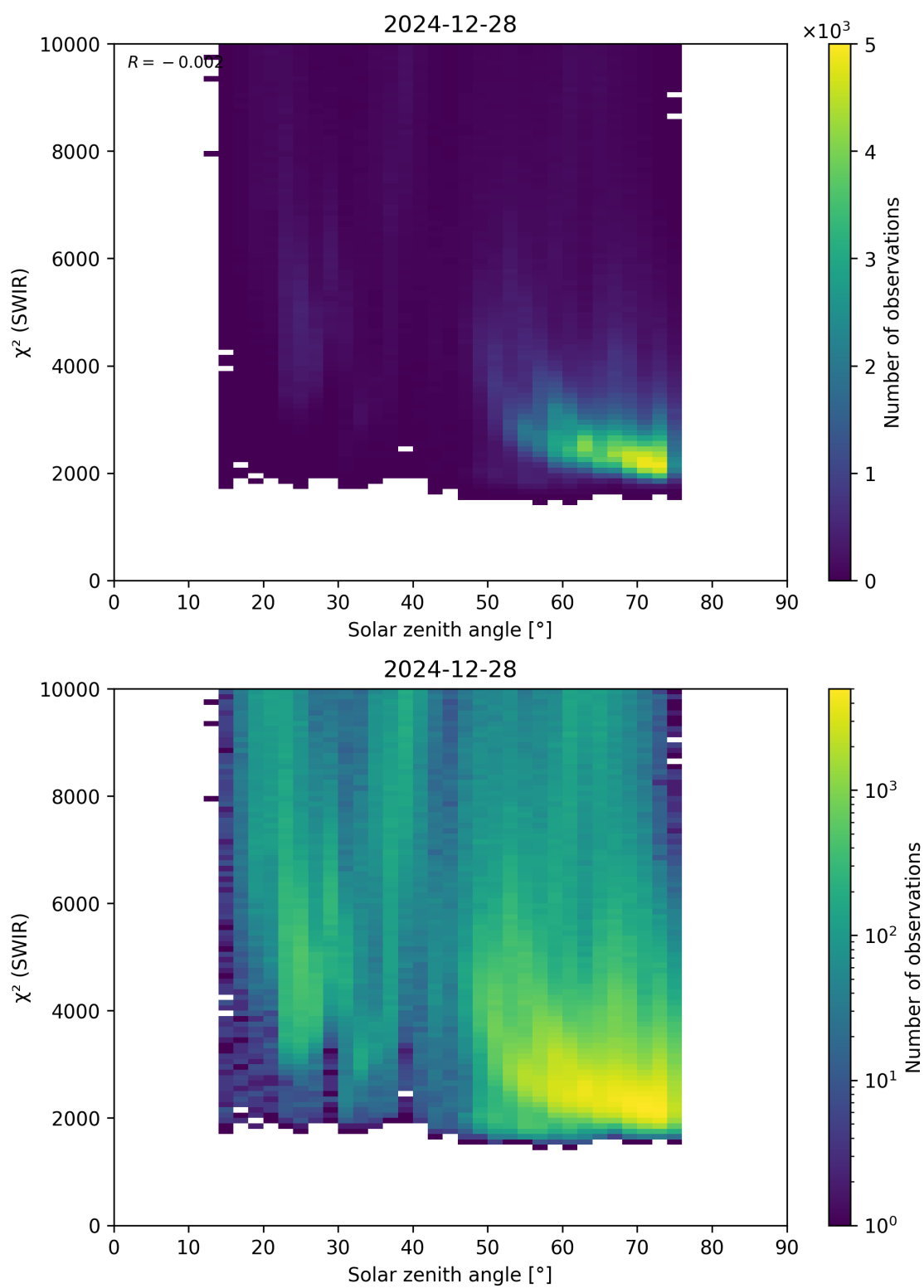
Figure 95: Scatter density plot of “Solar zenith angle” against “ \chi^2 (SWIR)” for 2024-12-27 to 2024-12-29.
