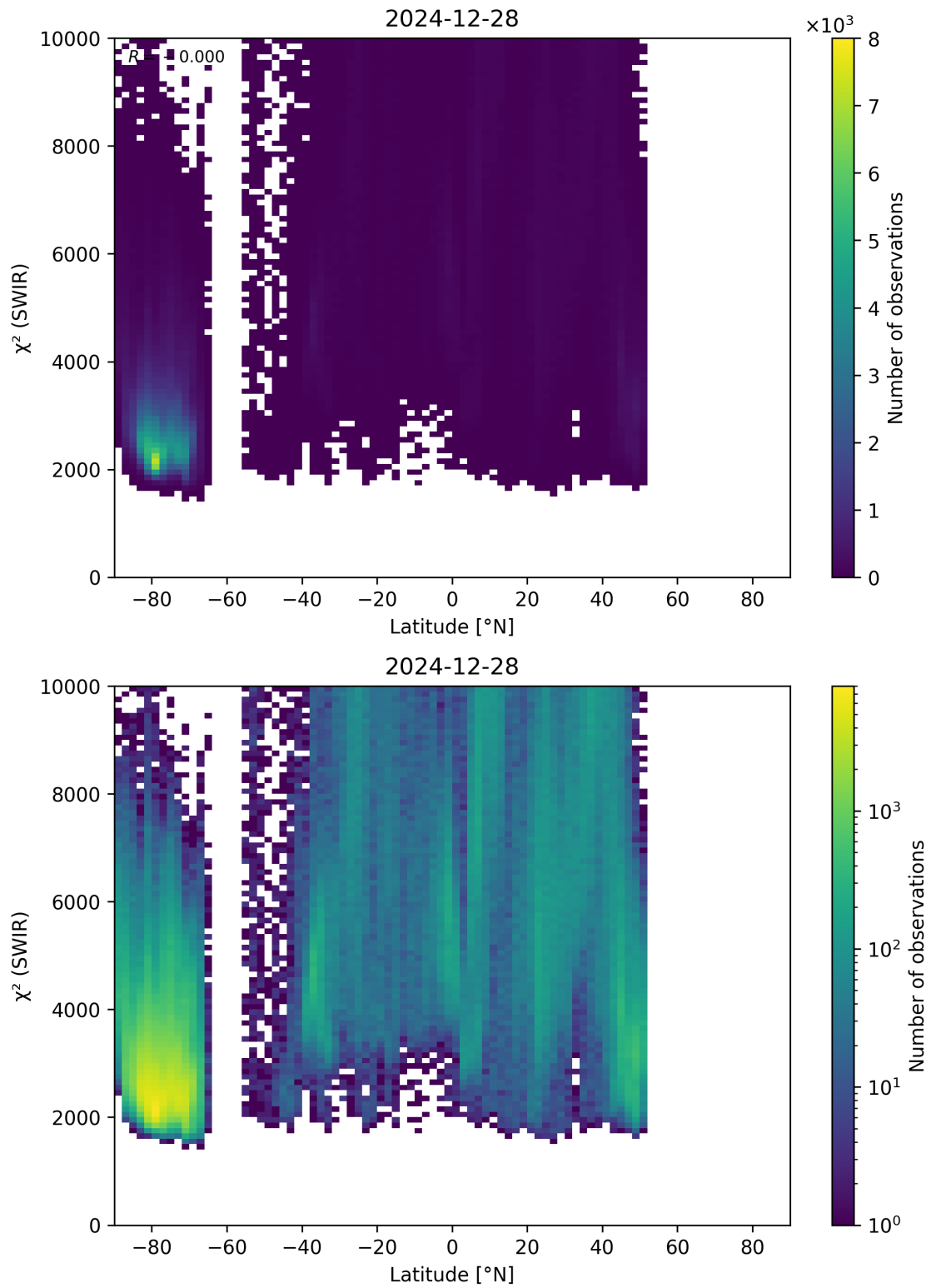
Figure 54: Scatter density plot of “Latitude” against “ \chi^2 (SWIR)” for 2024-12-27 to 2024-12-29.
