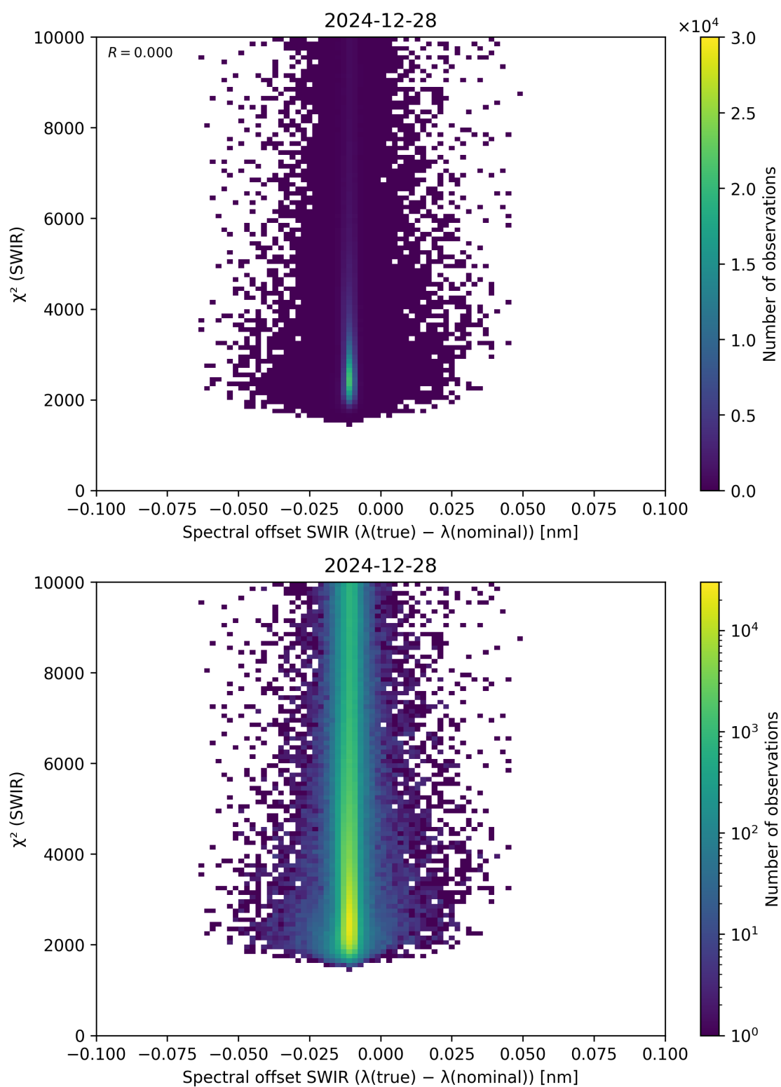
Figure 118: Scatter density plot of “Spectral offset SWIR ( \lambda_{\text{true}} - \lambda_{\text{nominal}} )” against “ \chi^2 (SWIR)” for 2024-12-27 to 2024-12-29.
