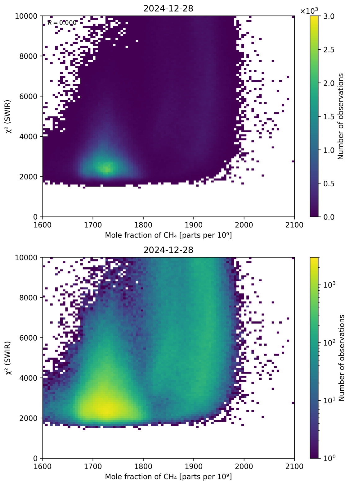
Figure 71: Scatter density plot of “Mole fraction of \text{CH}_4 ” against “ \chi^2 (SWIR)” for 2024-12-27 to 2024-12-29.
