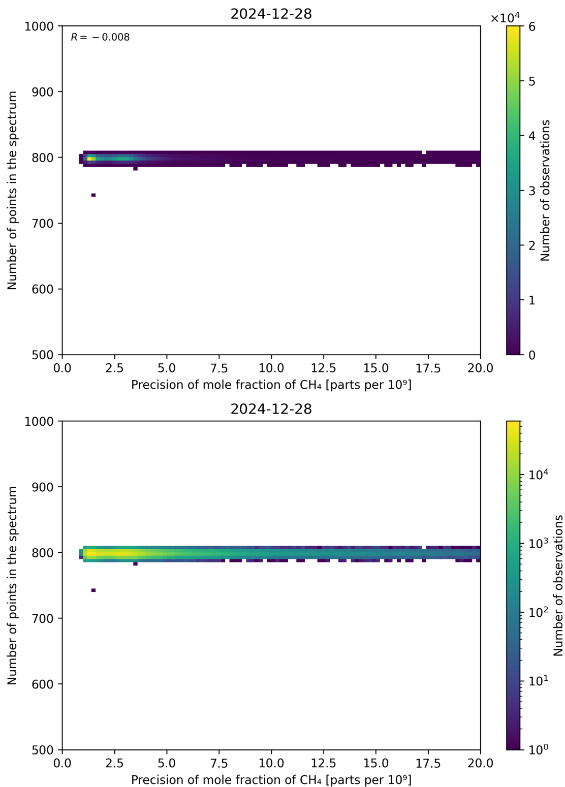
Figure 84: Scatter density plot of “Precision of mole fraction of CH 4 ” against “Number of points in the spectrum” for 2024-12-27 to 2024-12-29.
