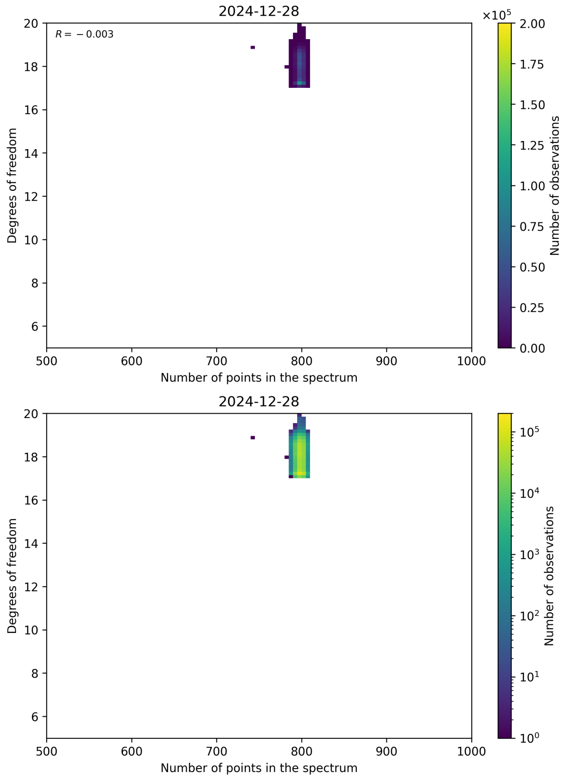
Figure 90: Scatter density plot of “Number of points in the spectrum” against “Degrees of freedom” for 2024-12-27 to 2024-12-29.
