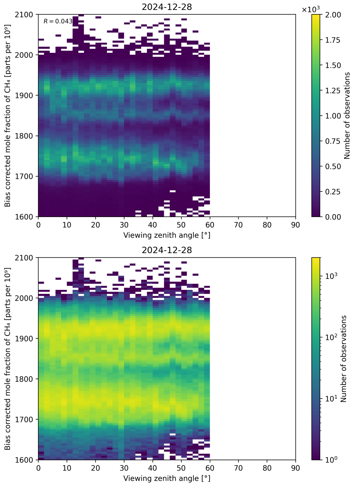
Figure 111: Scatter density plot of “Viewing zenith angle” against “Bias corrected mole fraction of CH 4 ” for 2024-12-27 to 2024-12-29.
