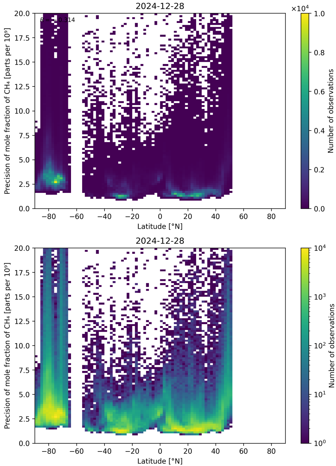
Figure 59: Scatter density plot of “Latitude” against “Precision of mole fraction of CH 4 ” for 2024-12-27 to 2024-12-29.
