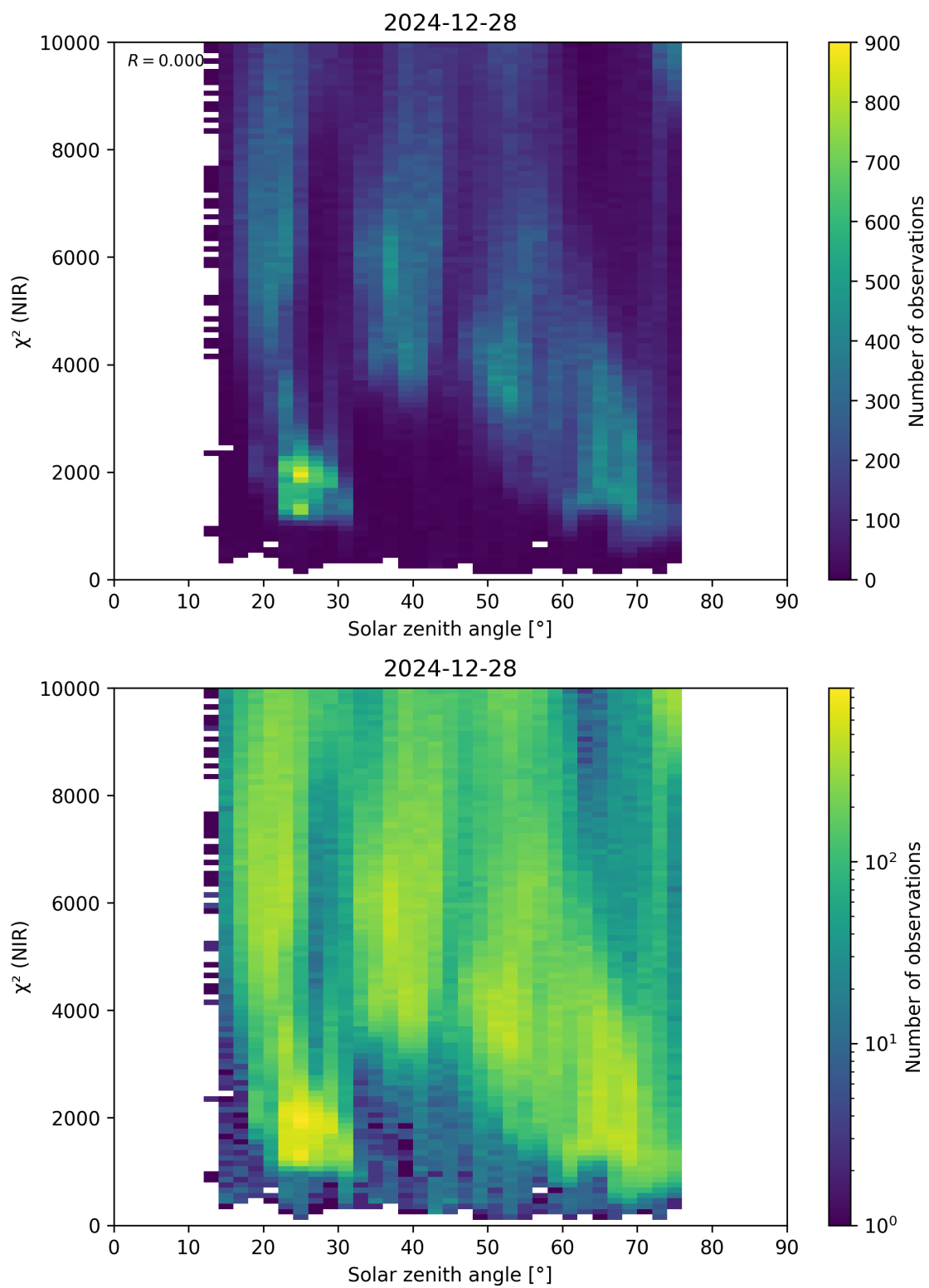
Figure 94: Scatter density plot of “Solar zenith angle” against “ \chi^2 (NIR)” for 2024-12-27 to 2024-12-29.
