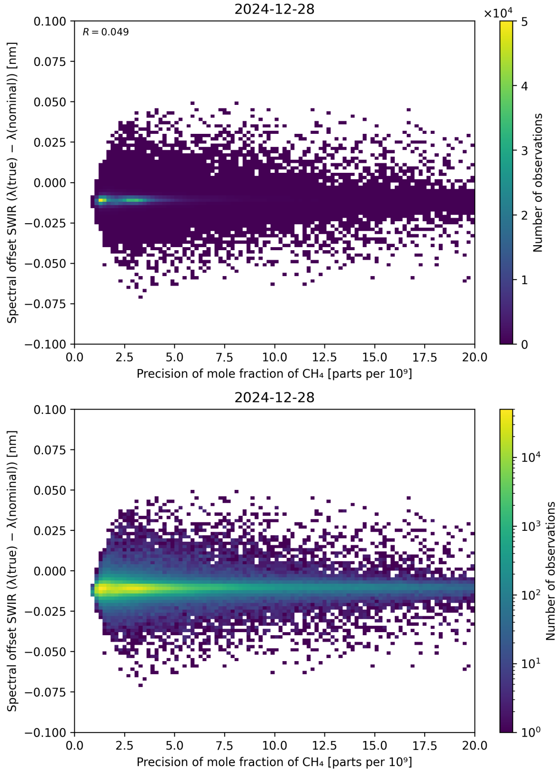
Figure 85: Scatter density plot of “Precision of mole fraction of CH 4 ” against “Spectral offset SWIR ( \lambda_{\text{true}} - \lambda_{\text{nominal}} )” for 2024-12-27 to 2024-12-29.
