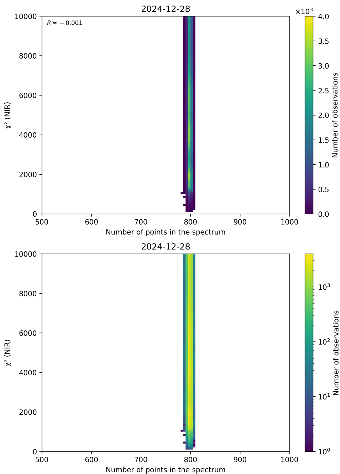
Figure 88: Scatter density plot of “Number of points in the spectrum” against “ \chi^2 (NIR)” for 2024-12-27 to 2024-12-29.
