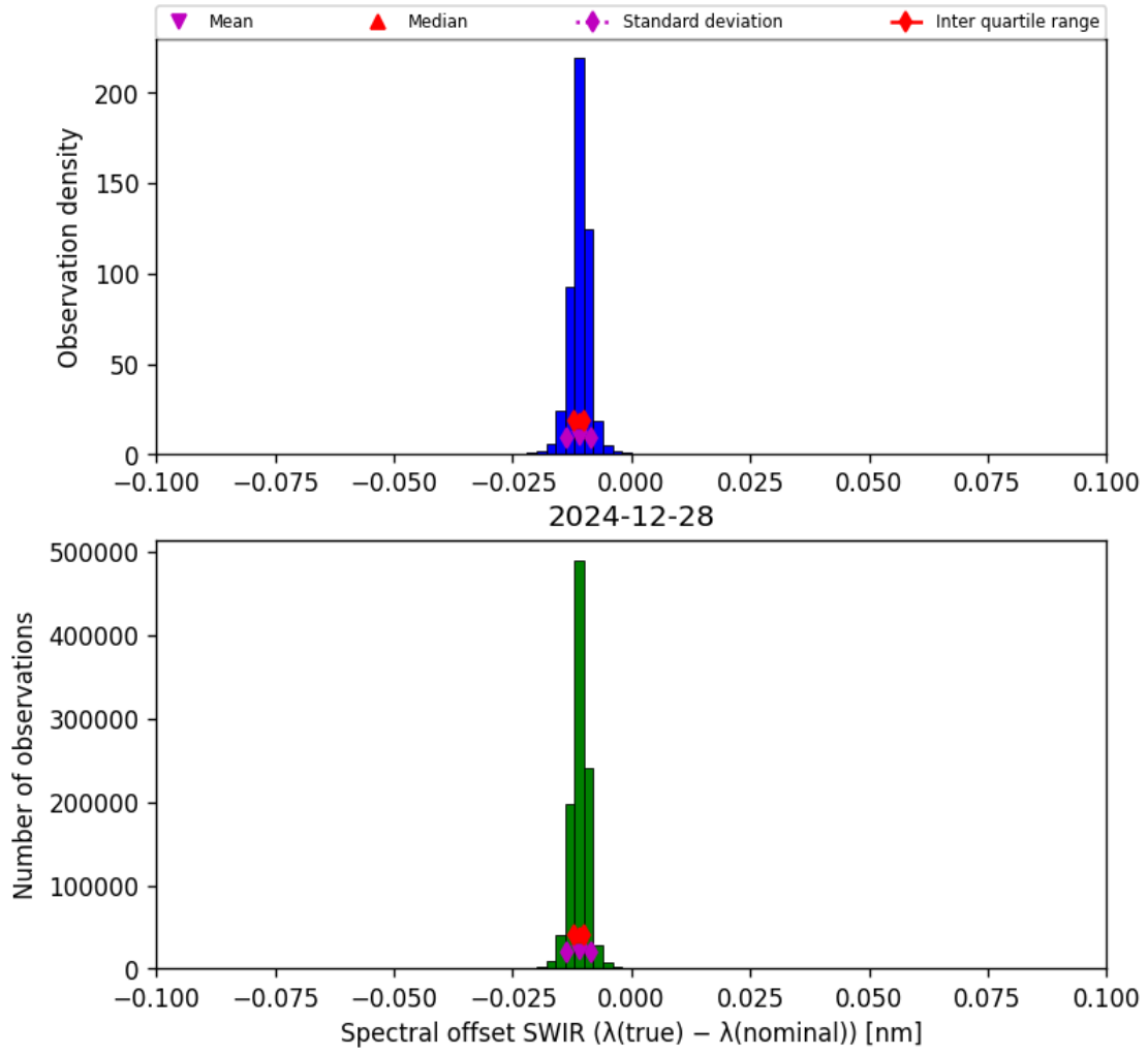
Figure 27: Histogram of “Spectral offset SWIR ( \lambda_{\text{true}} - \lambda_{\text{nominal}} )” for 2024-12-27 to 2024-12-29
