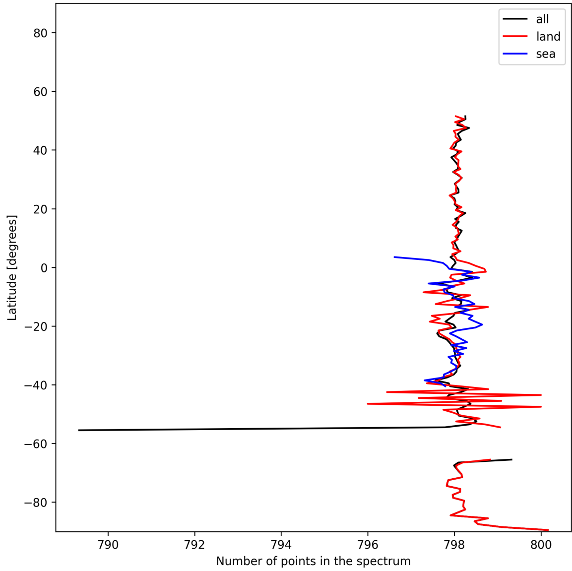
Figure 15: Zonal average of “Number of points in the spectrum” for 2024-12-27 to 2024-12-29.
