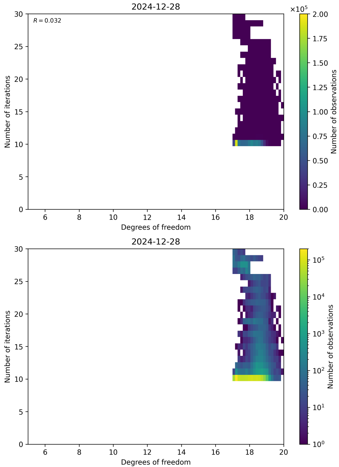
Figure 52: Scatter density plot of “Degrees of freedom” against “Number of iterations” for 2024-12-27 to 2024-12-29.
