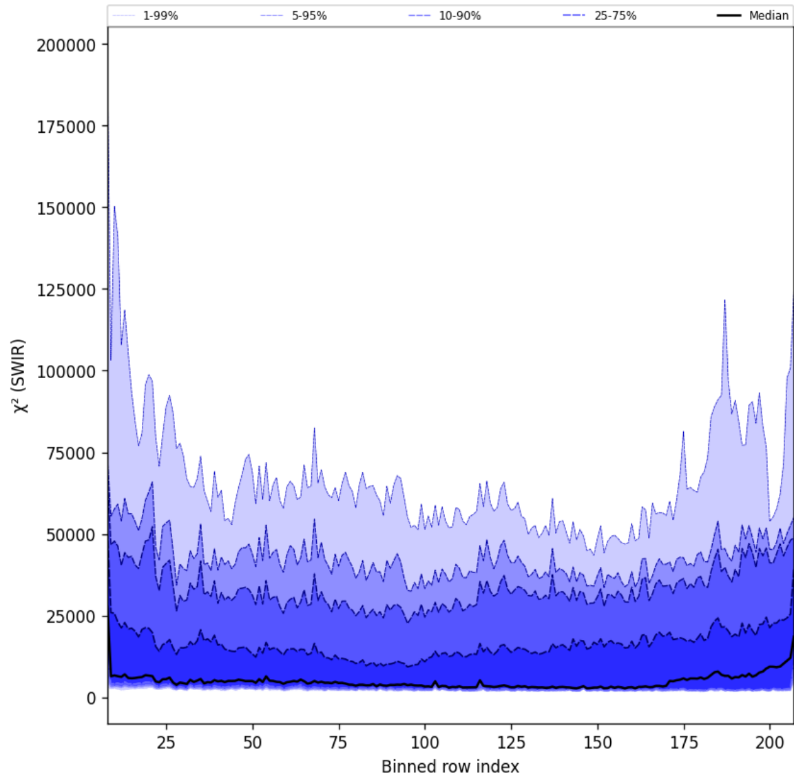
Figure 39: Along track statistics of “ \chi^2 (SWIR)” for 2024-12-27 to 2024-12-29
