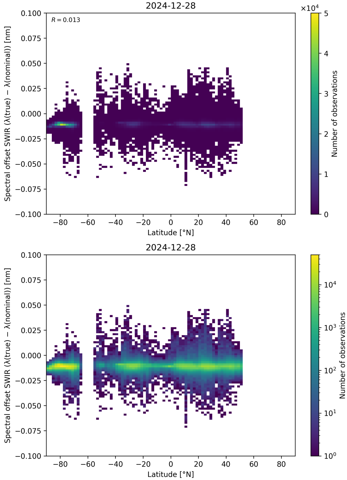
Figure 62: Scatter density plot of “Latitude” against “Spectral offset SWIR ( \lambda_{\text{true}} - \lambda_{\text{nominal}} )” for 2024-12-27 to 2024-12-29.
