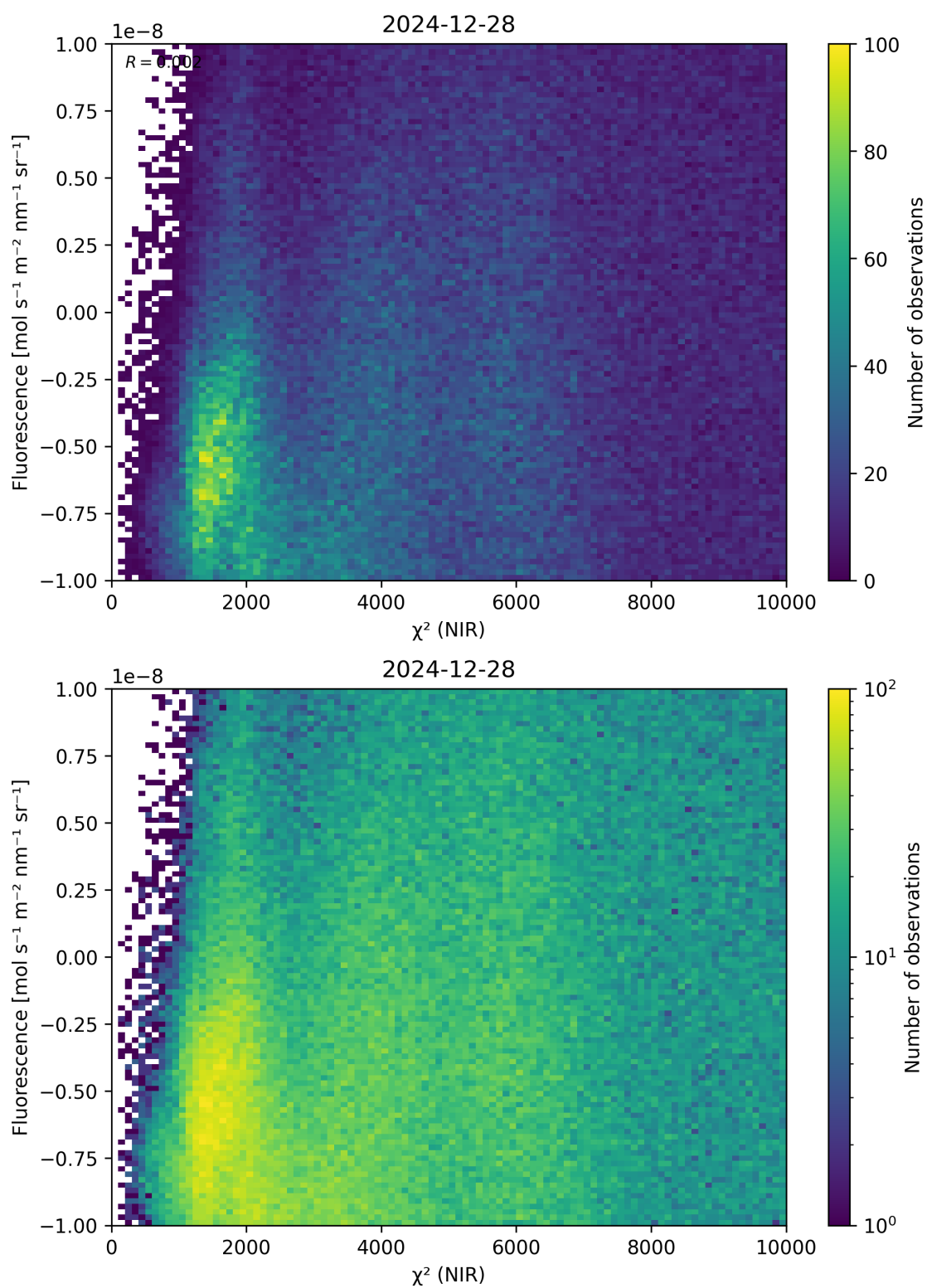
Figure 45: Scatter density plot of “ \chi^2 (NIR)” against “Fluorescence” for 2024-12-27 to 2024-12-29.
