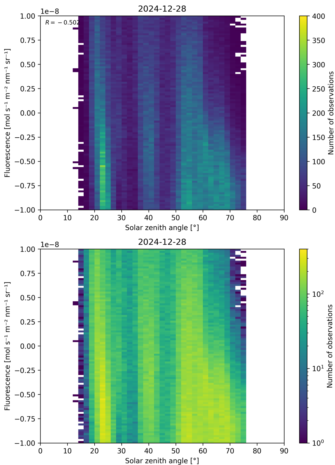
Figure 97: Scatter density plot of “Solar zenith angle” against “Fluorescence” for 2024-12-27 to 2024-12-29.
