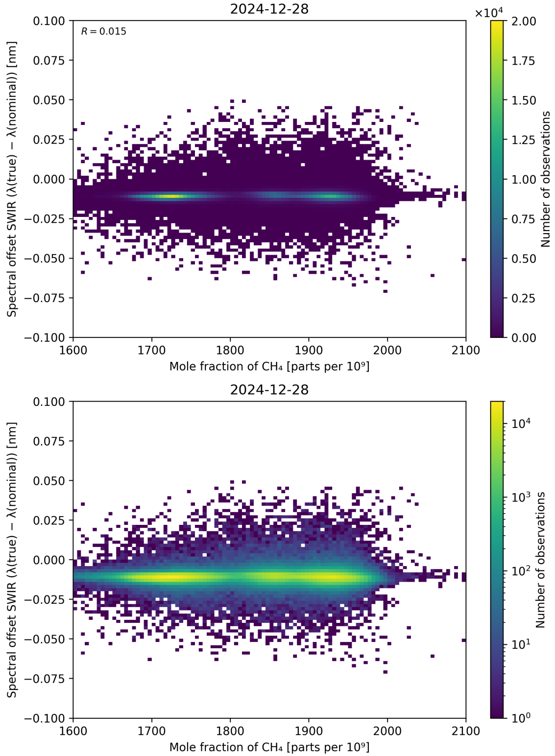
Figure 86: Scatter density plot of “Mole fraction of \text{CH}_4 ” against “Spectral offset SWIR ( \lambda_{\text{true}} - \lambda_{\text{nominal}} )” for 2024-12-27 to 2024-12-29.
