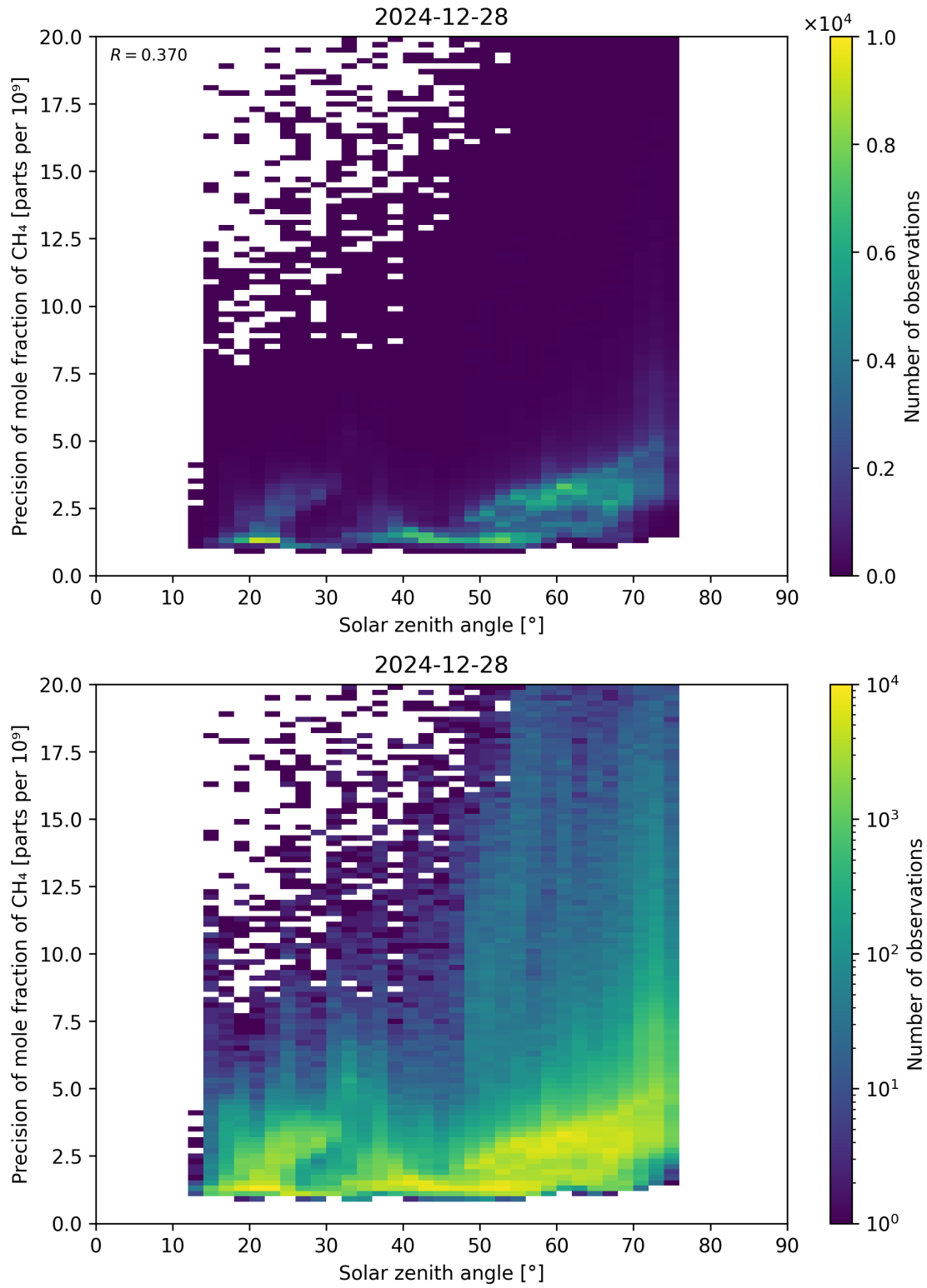
Figure 101: Scatter density plot of “Solar zenith angle” against “Precision of mole fraction of \text{CH}_4 ” for 2024-12-27 to 2024-12-29.
