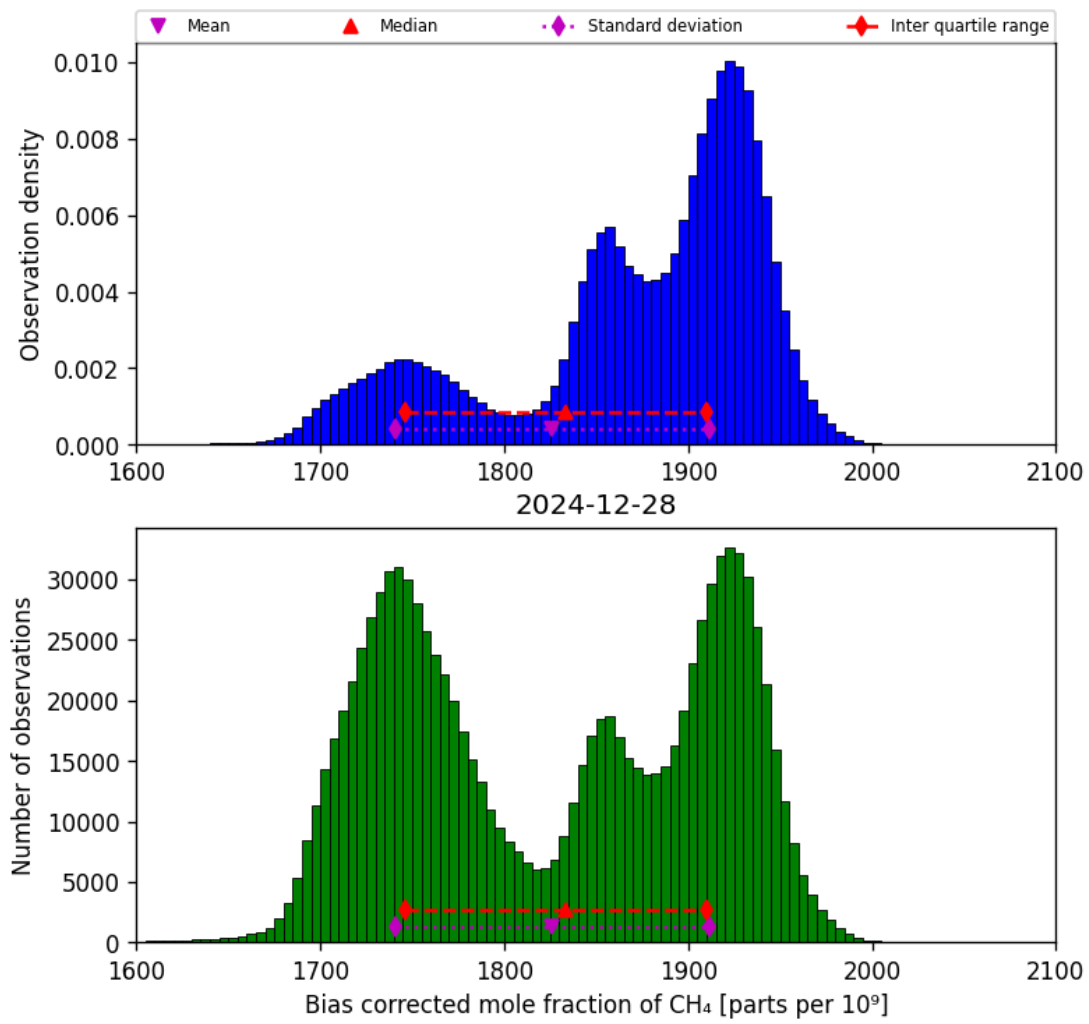
Figure 25: Histogram of “Bias corrected mole fraction of CH 4 ” for 2024-12-27 to 2024-12-29
