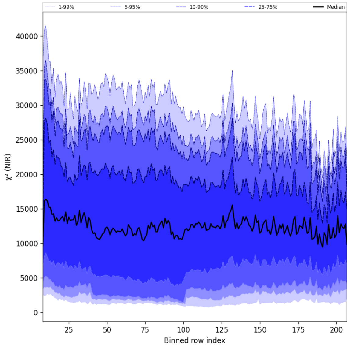
Figure 40: Along track statistics of “ \chi^2 (NIR)” for 2024-12-27 to 2024-12-29
