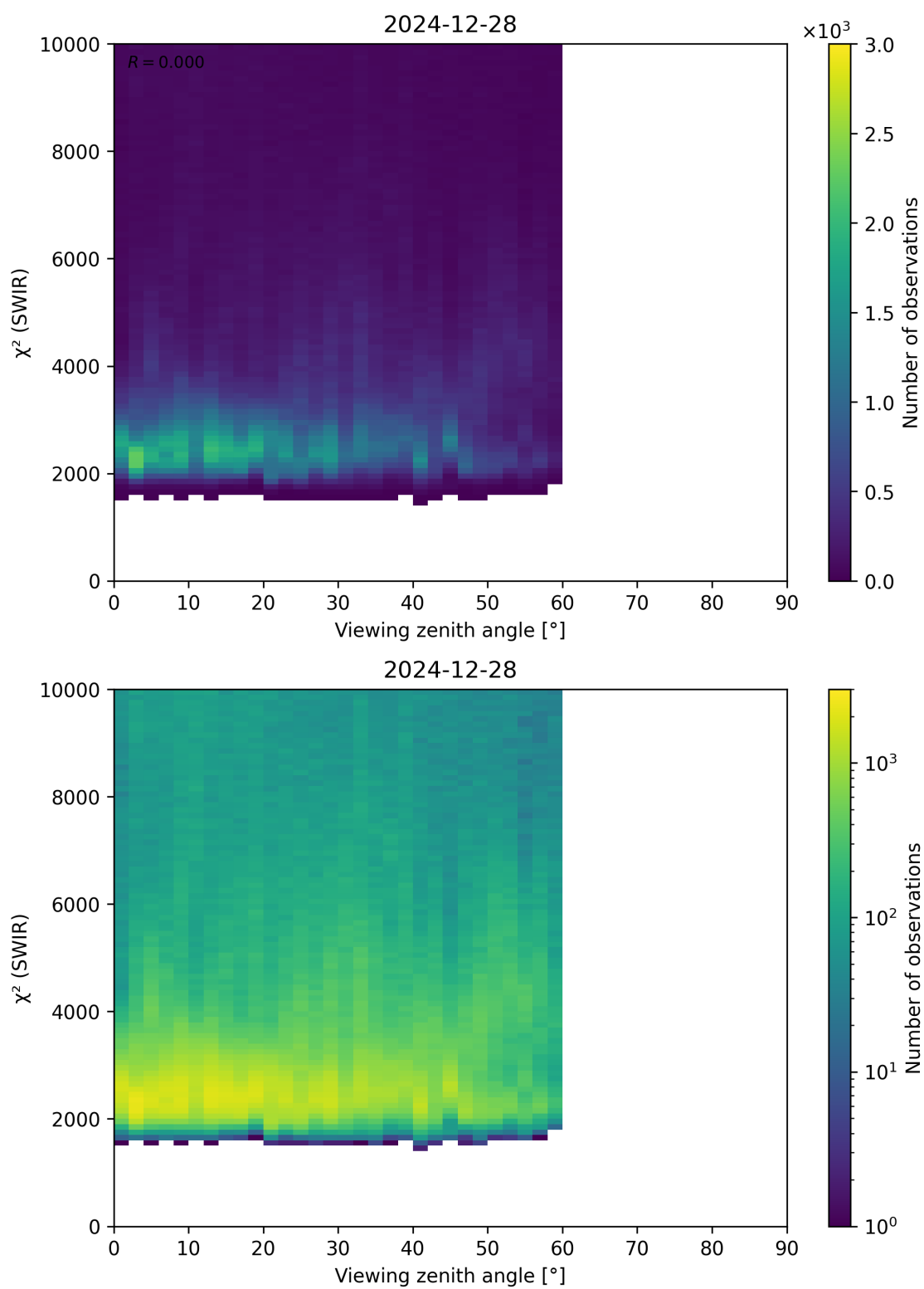
Figure 106: Scatter density plot of “Viewing zenith angle” against “ \chi^2 (SWIR)” for 2024-12-27 to 2024-12-29.
