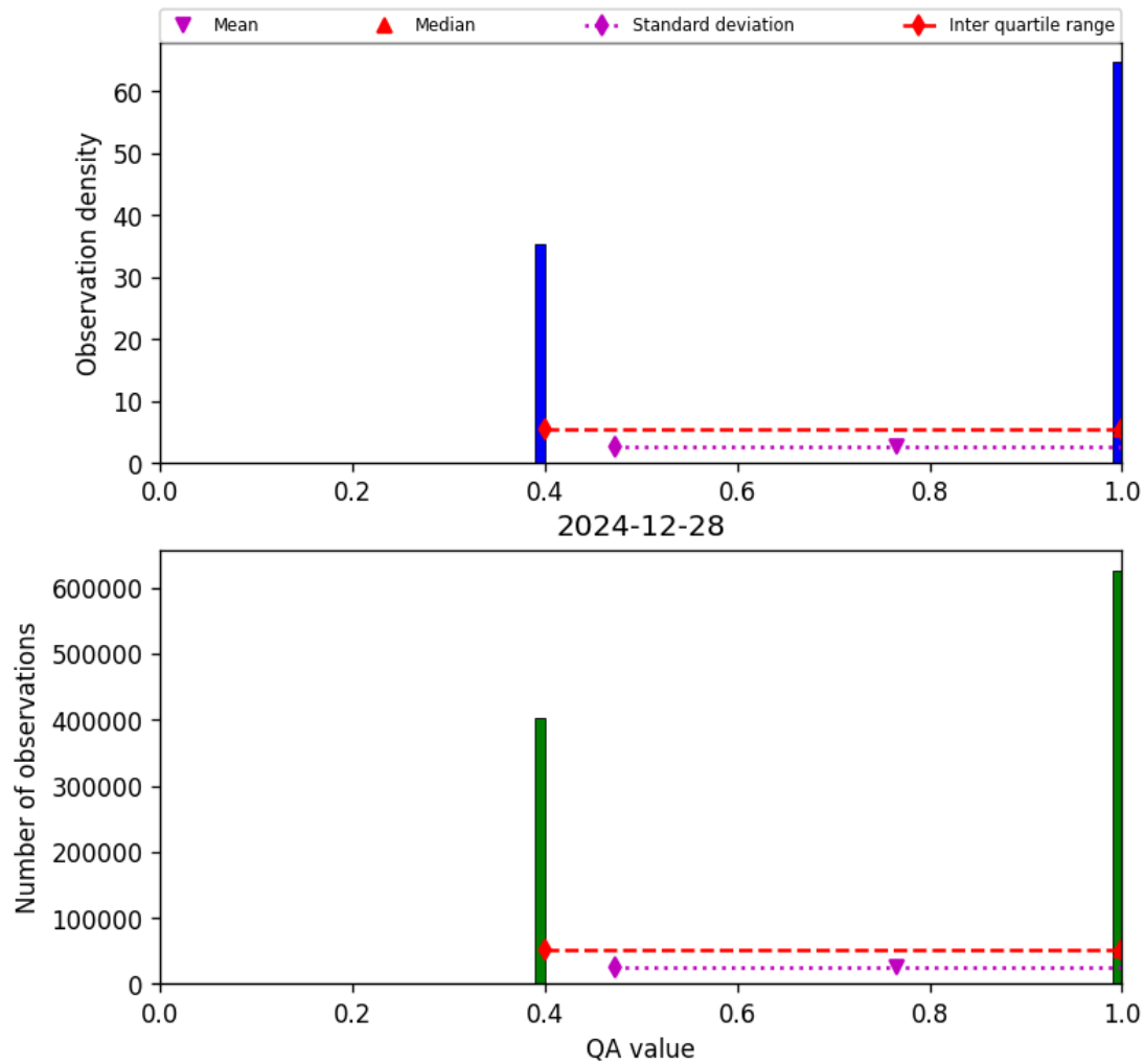
Figure 22: Histogram of “QA value” for 2024-12-27 to 2024-12-29
