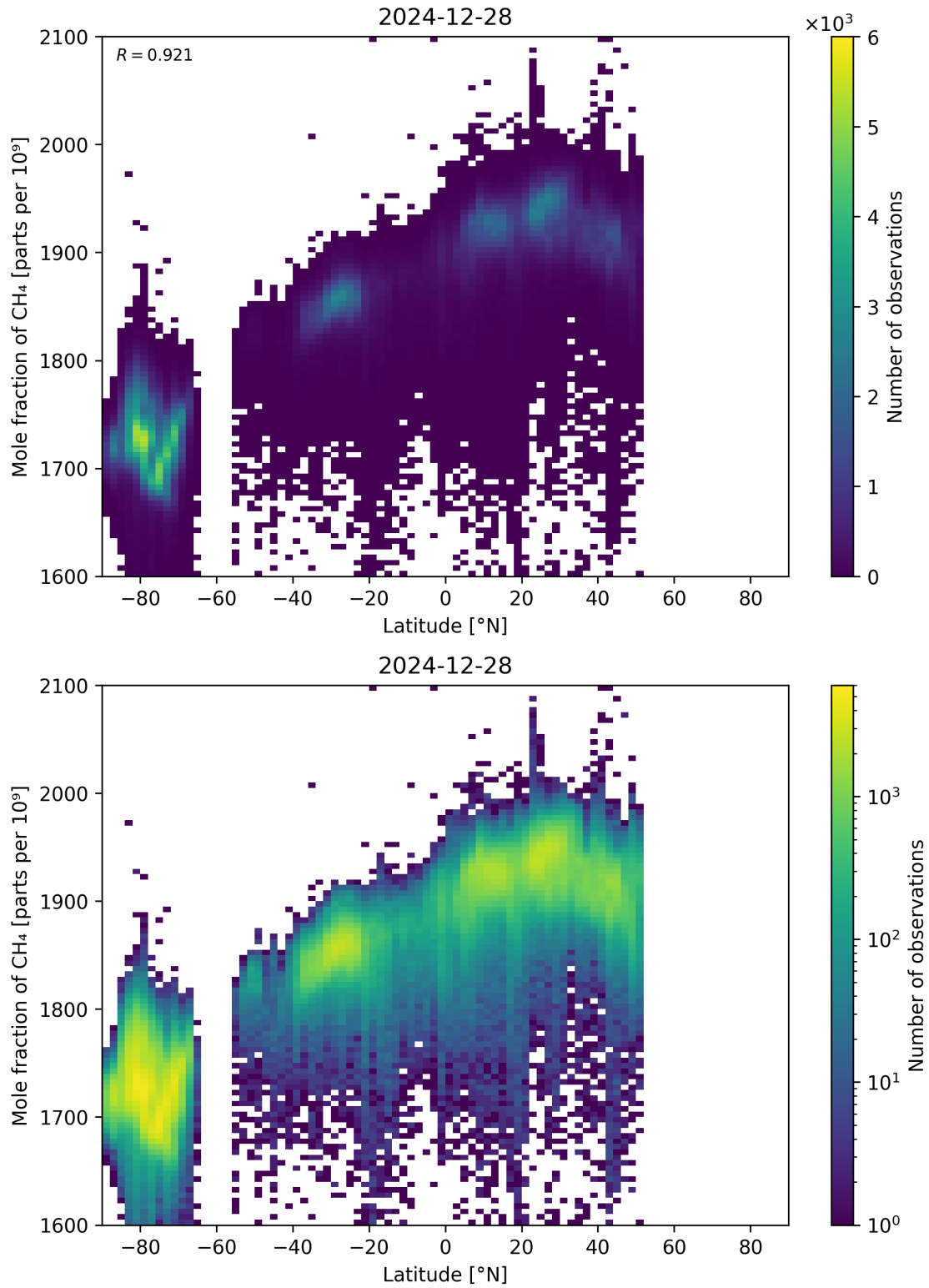
Figure 57: Scatter density plot of “Latitude” against “Mole fraction of CH 4 ” for 2024-12-27 to 2024-12-29.
