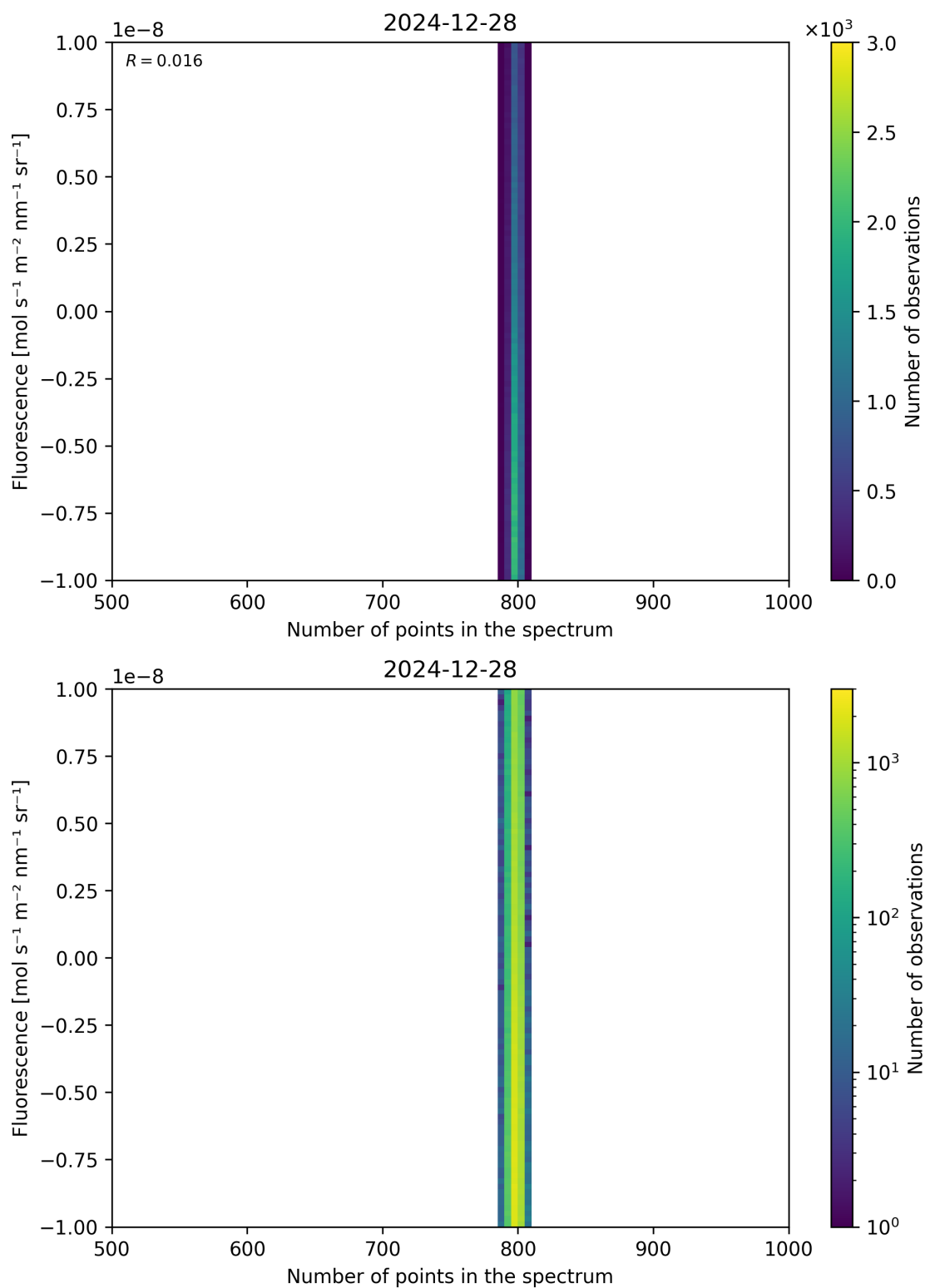
Figure 91: Scatter density plot of “Number of points in the spectrum” against “Fluorescence” for 2024-12-27 to 2024-12-29.
