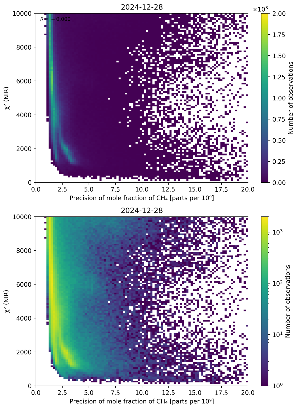
Figure 78: Scatter density plot of “Precision of mole fraction of CH 4 ” against “ \chi^2 (NIR)” for 2024-12-27 to 2024-12-29.
