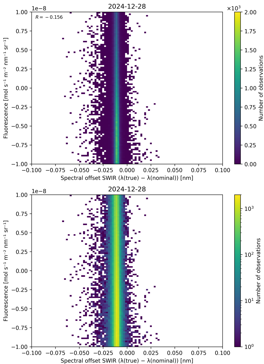
Figure 120: Scatter density plot of “Spectral offset SWIR ( \lambda_{\text{true}} - \lambda_{\text{nominal}} )” against “Fluorescence” for 2024-12-27 to 2024-12-29.
