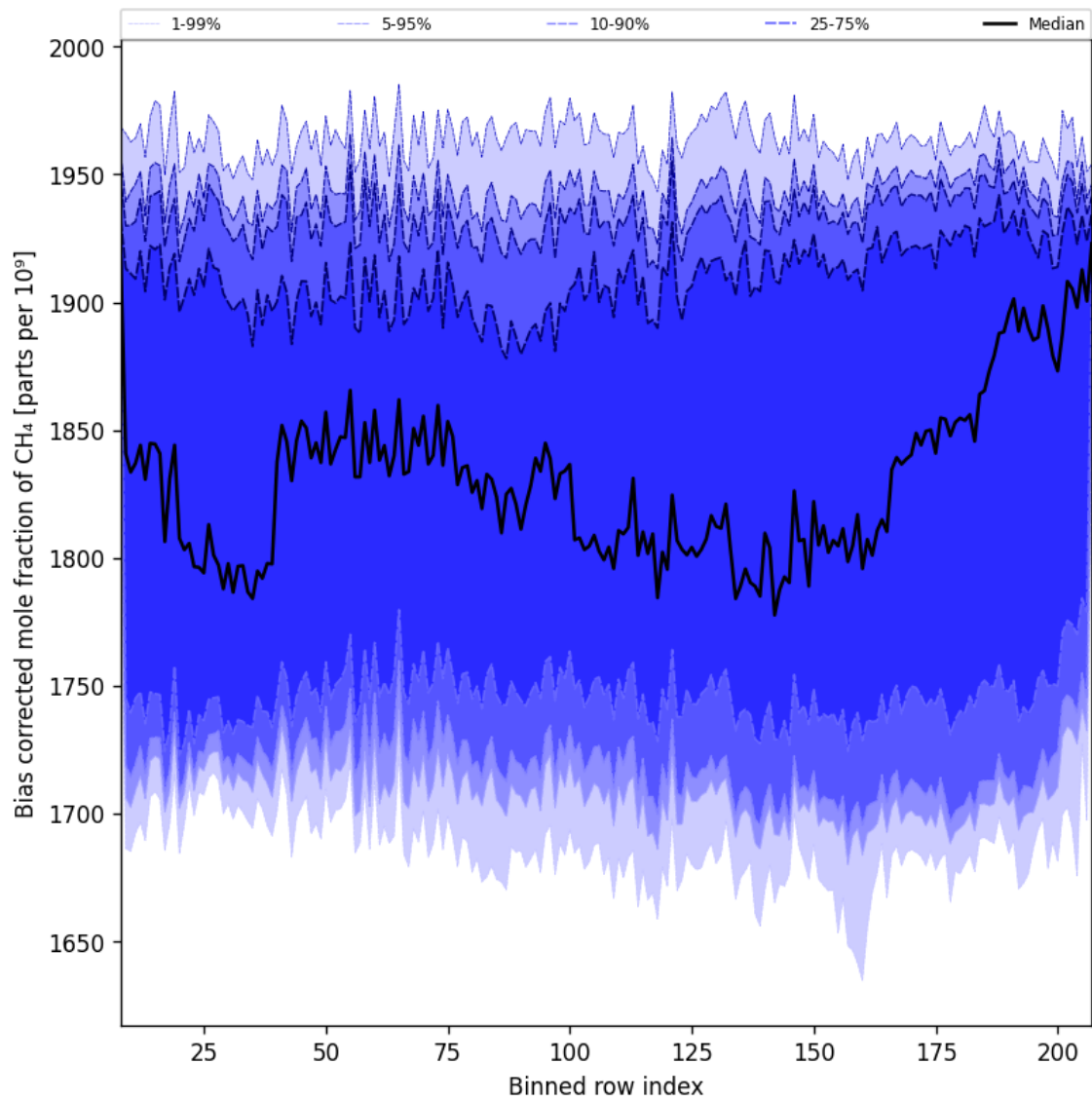
Figure 36: Along track statistics of “Bias corrected mole fraction of CH 4 ” for 2024-12-27 to 2024-12-29
