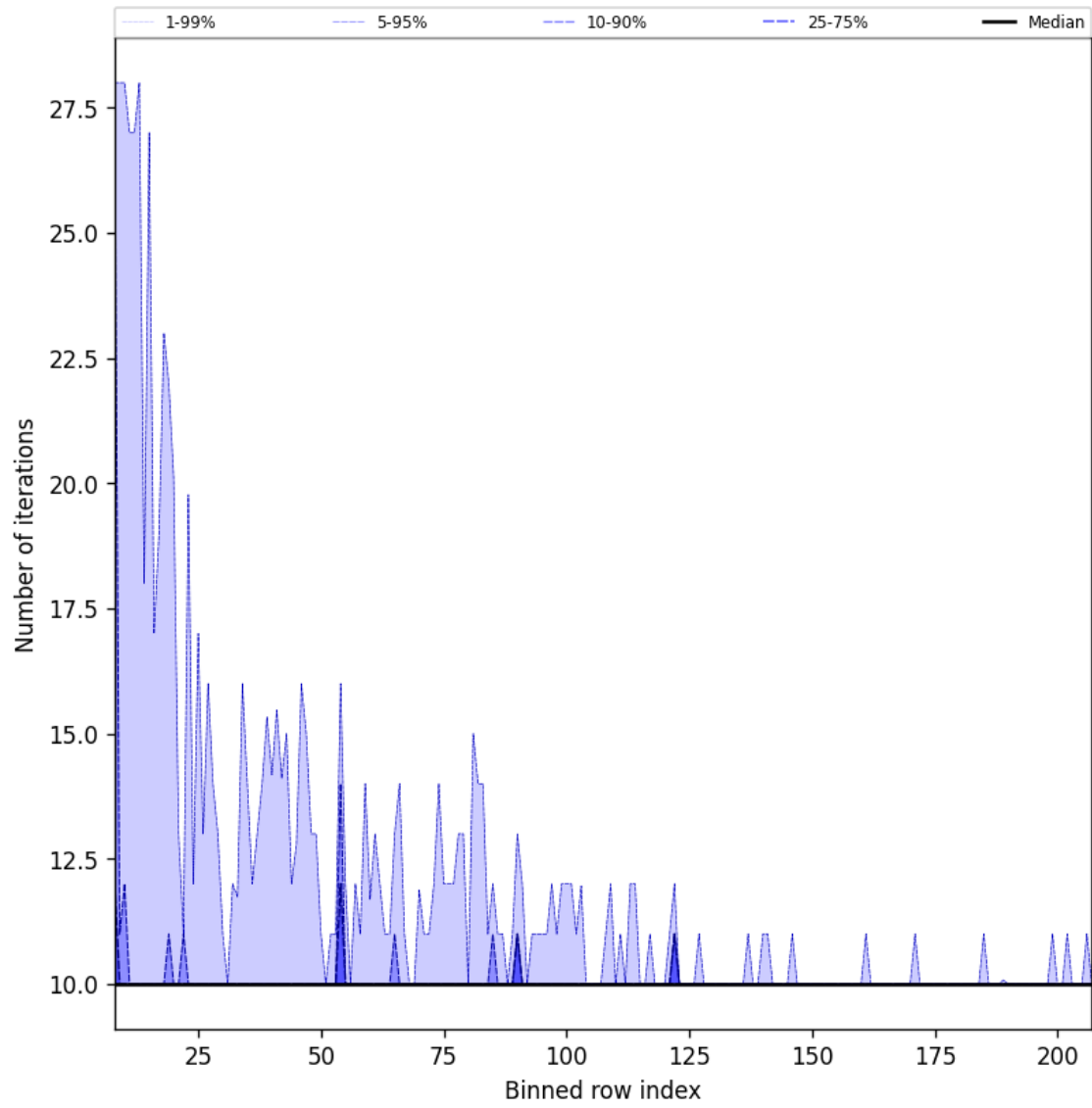
Figure 42: Along track statistics of “Number of iterations” for 2024-12-27 to 2024-12-29
