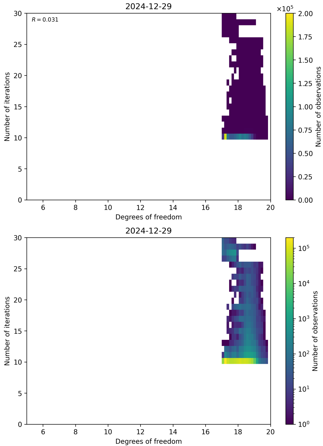
Figure 52: Scatter density plot of “Degrees of freedom” against “Number of iterations” for 2024-12-28 to 2024-12-30.
