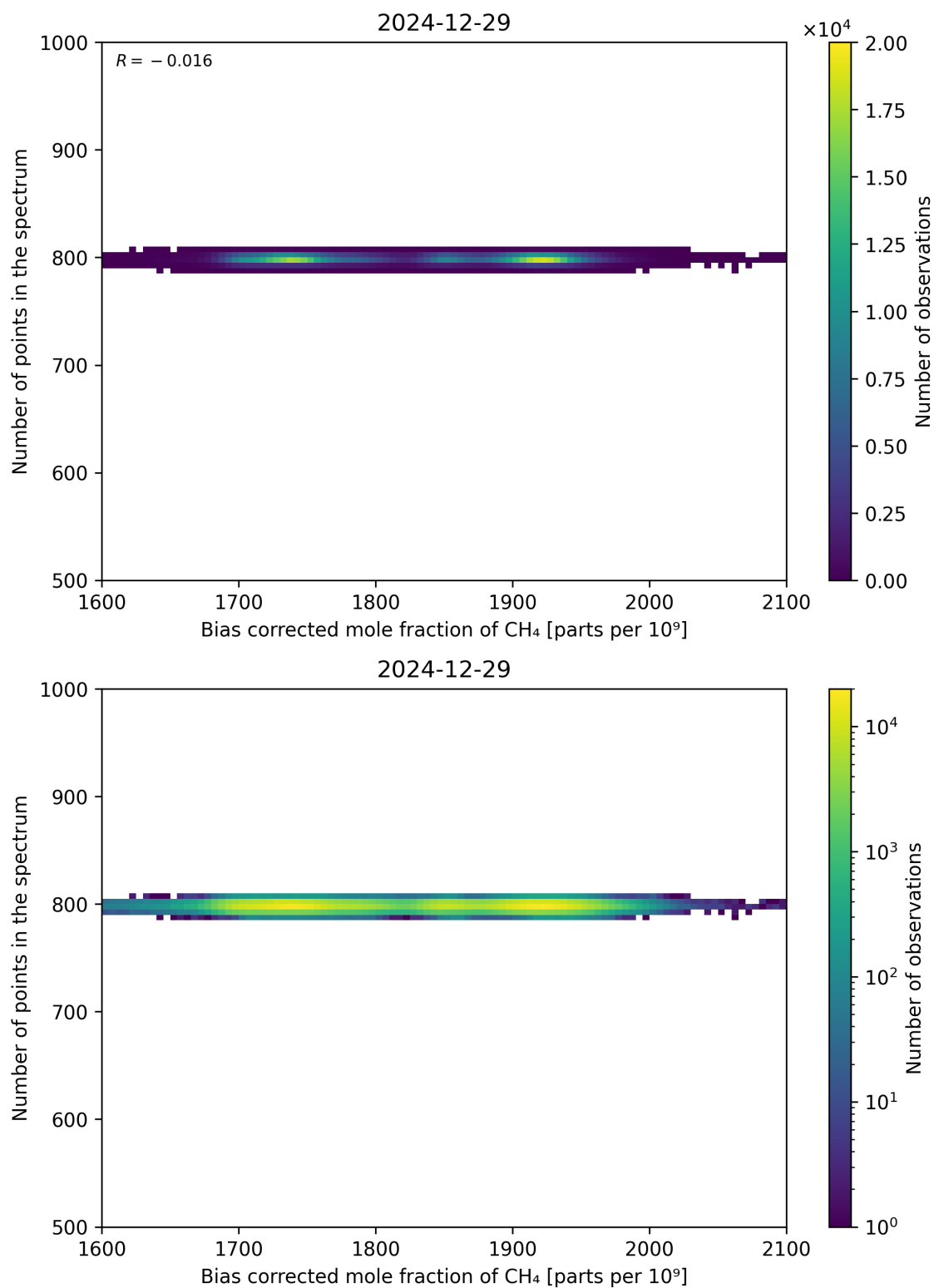
Figure 68: Scatter density plot of “Bias corrected mole fraction of CH 4 ” against “Number of points in the spectrum” for 2024-12-28 to 2024-12-30.
