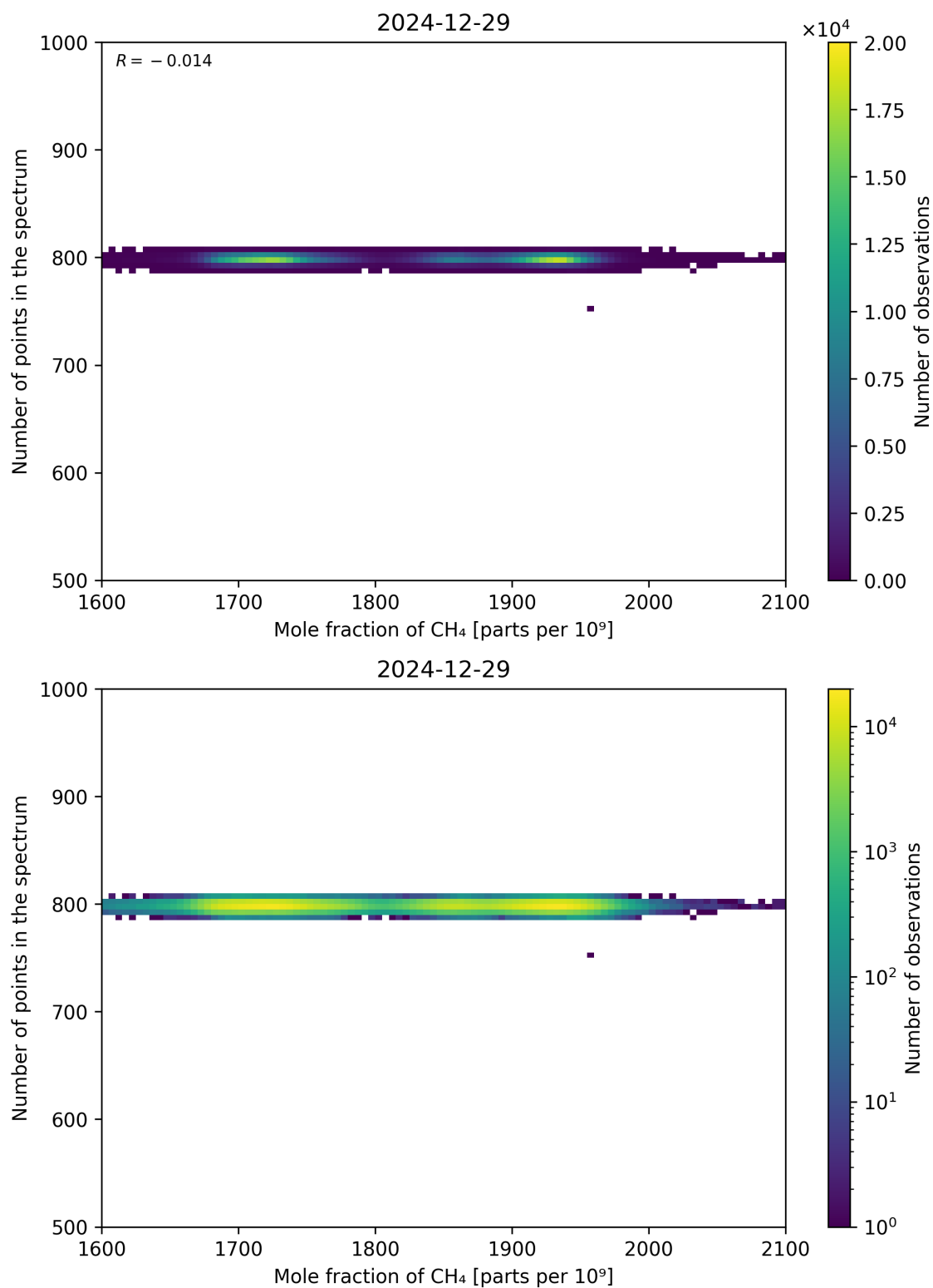
Figure 77: Scatter density plot of “Mole fraction of CH 4 ” against “Number of points in the spectrum” for 2024-12-28 to 2024-12-30.
