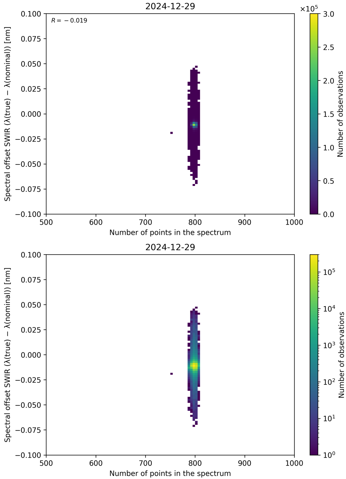
Figure 93: Scatter density plot of “Number of points in the spectrum” against “Spectral offset SWIR ( \lambda_{\text{true}} - \lambda_{\text{nominal}} )” for 2024-12-28 to 2024-12-30.
