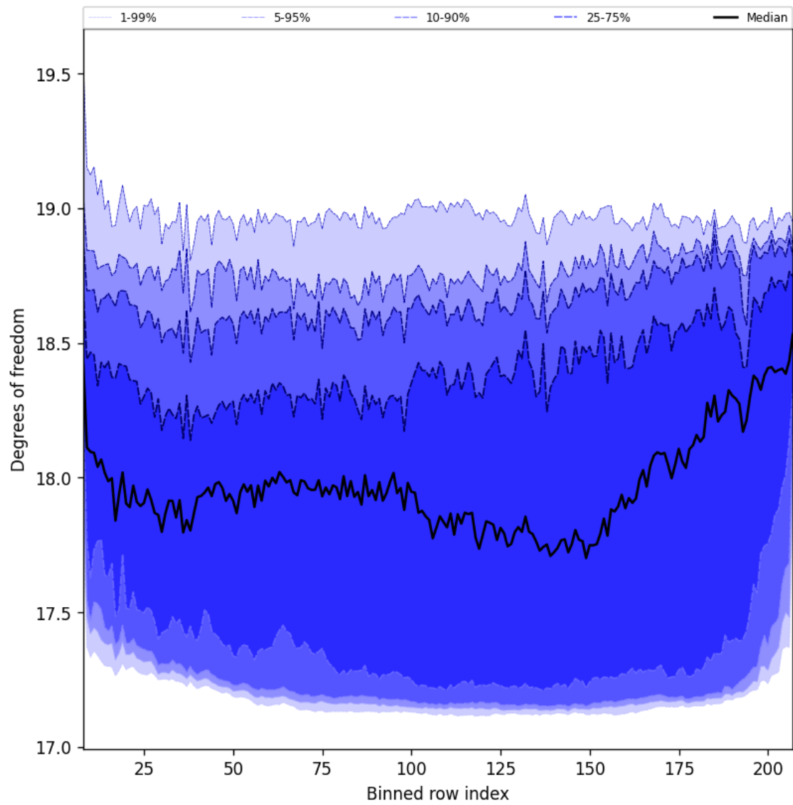
Figure 41: Along track statistics of “Degrees of freedom” for 2024-12-28 to 2024-12-30
