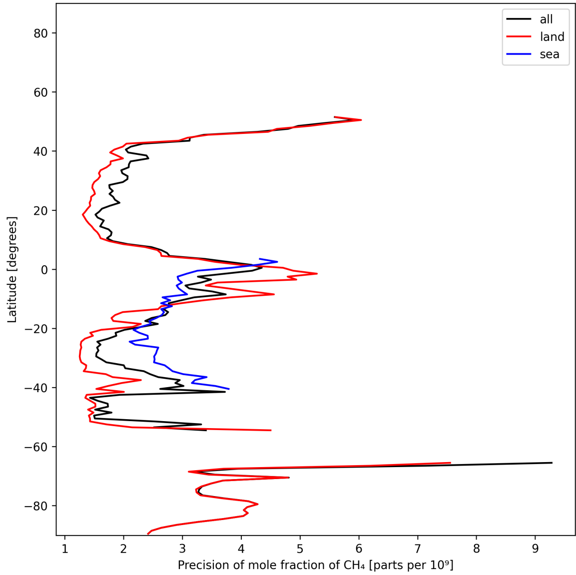
Figure 13: Zonal average of “Precision of mole fraction of CH 4 ” for 2024-12-28 to 2024-12-30.
