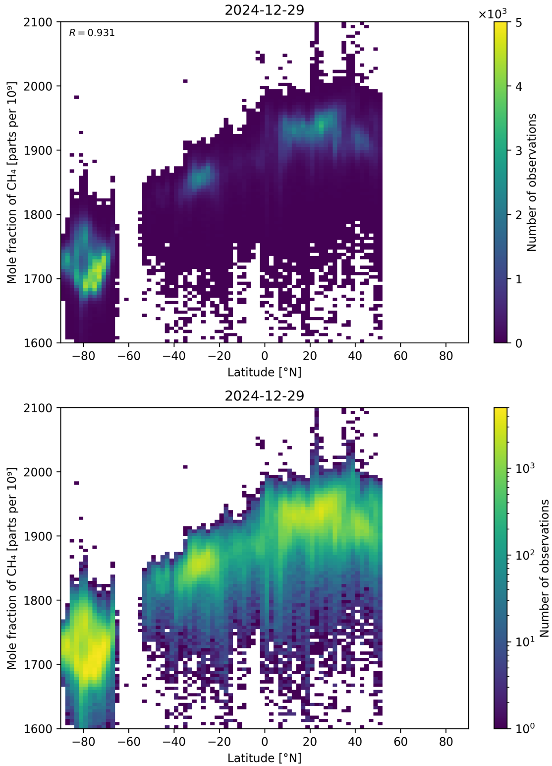
Figure 57: Scatter density plot of “Latitude” against “Mole fraction of CH 4 ” for 2024-12-28 to 2024-12-30.
