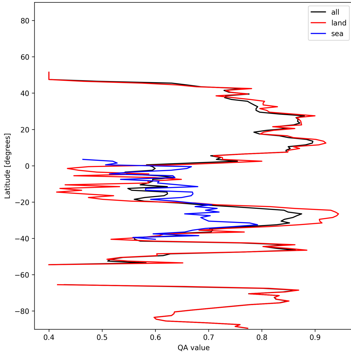
Figure 11: Zonal average of “QA value” for 2024-12-28 to 2024-12-30.
