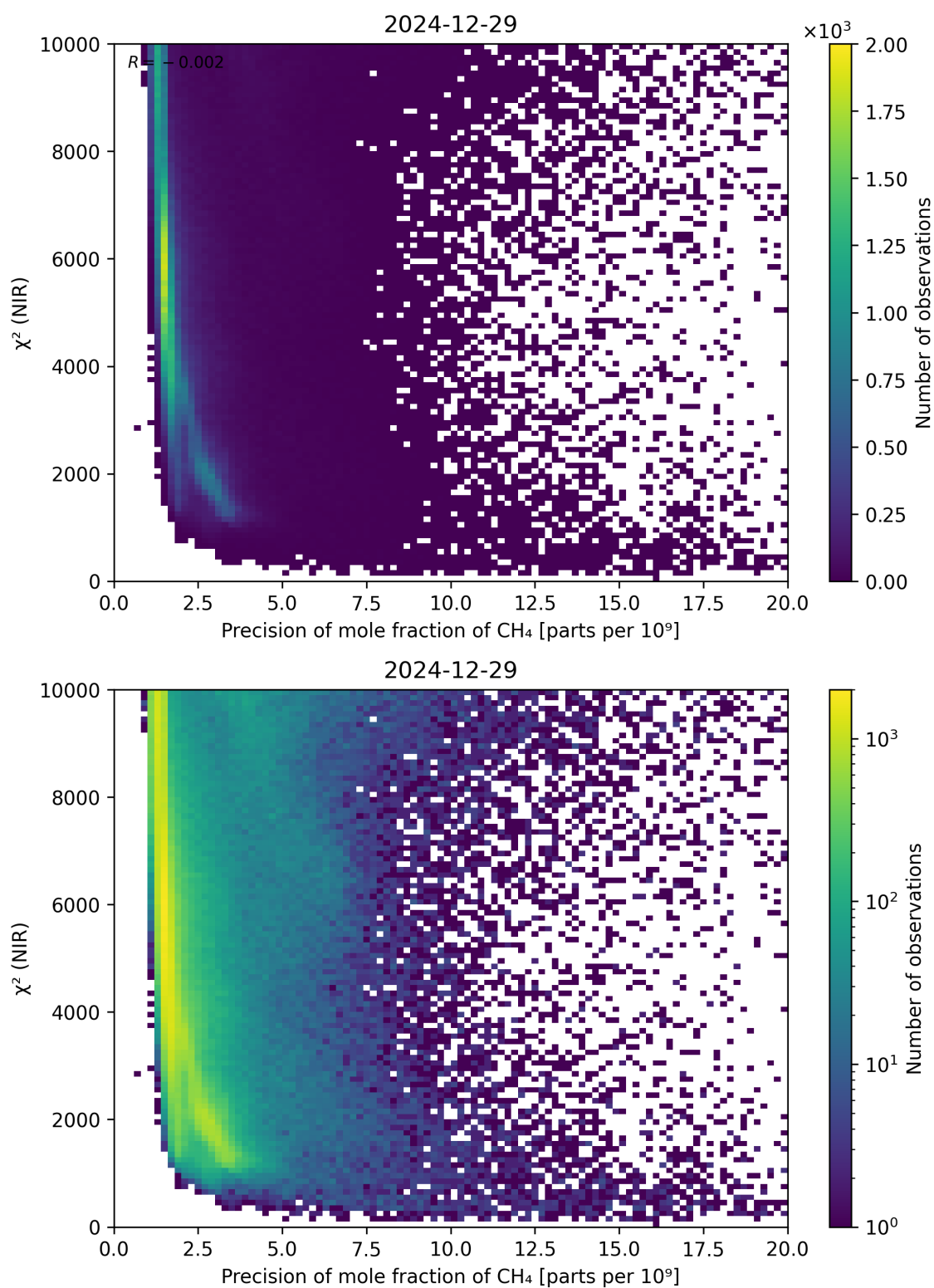
Figure 78: Scatter density plot of “Precision of mole fraction of CH 4 ” against “ \chi^2 (NIR)” for 2024-12-28 to 2024-12-30.
