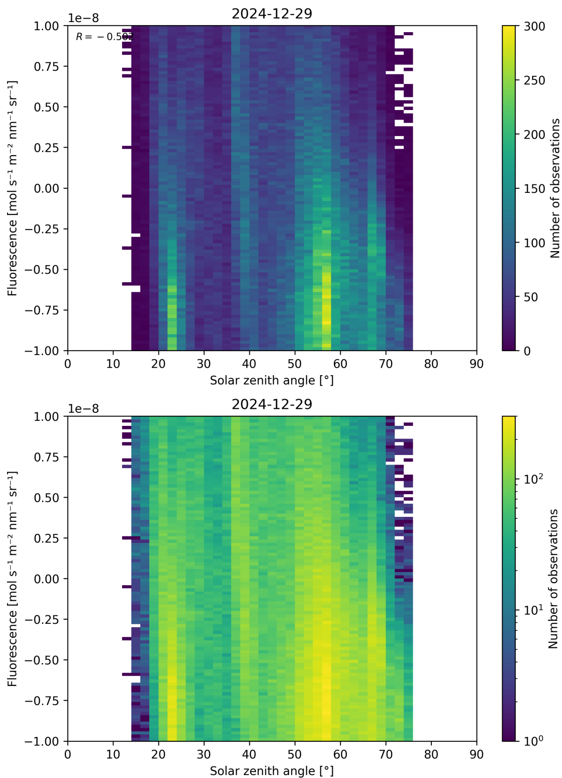
Figure 97: Scatter density plot of “Solar zenith angle” against “Fluorescence” for 2024-12-28 to 2024-12-30.
