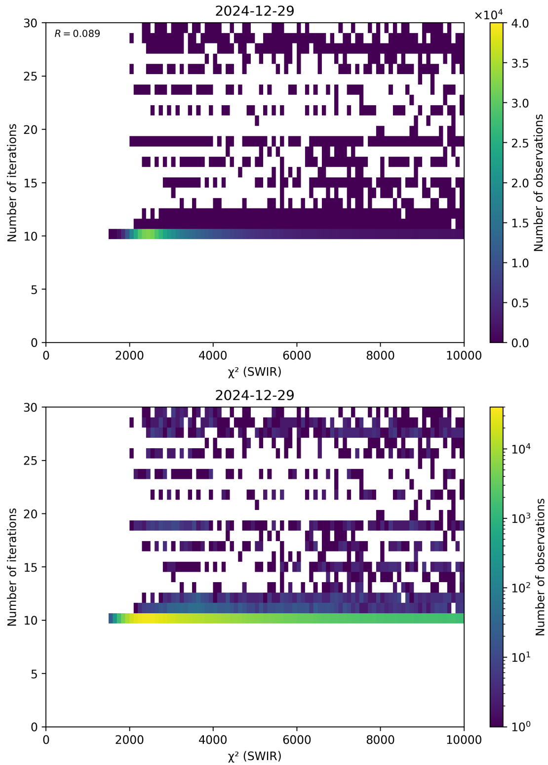
Figure 50: Scatter density plot of “ \chi^2 (SWIR)” against “Number of iterations” for 2024-12-28 to 2024-12-30.
