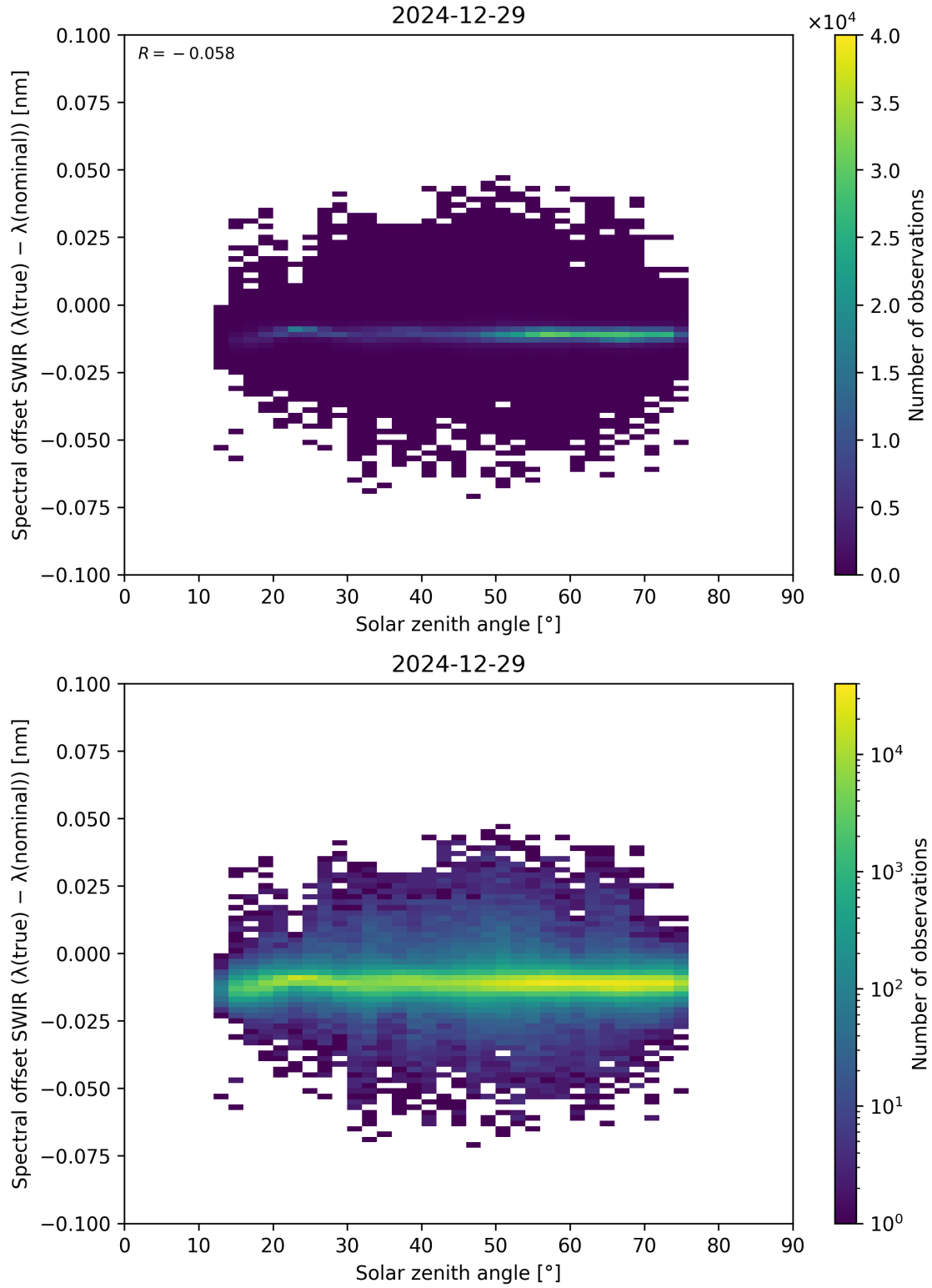
Figure 104: Scatter density plot of “Solar zenith angle” against “Spectral offset SWIR ( \lambda_{\text{true}} - \lambda_{\text{nominal}} )” for 2024-12-28 to 2024-12-30.
