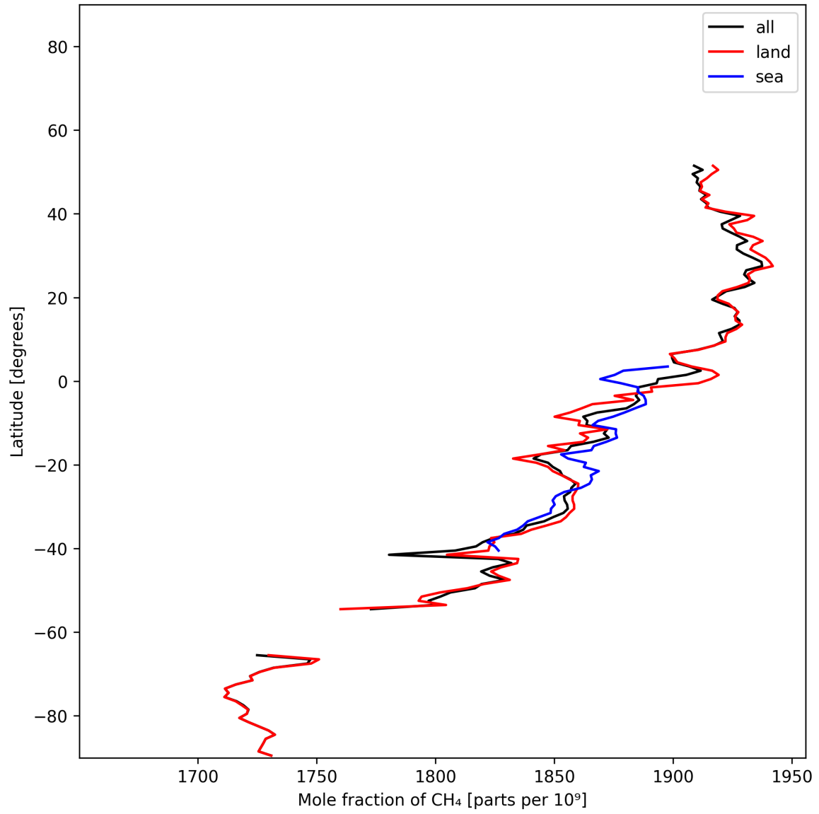
Figure 12: Zonal average of “Mole fraction of CH 4 ” for 2024-12-28 to 2024-12-30.
