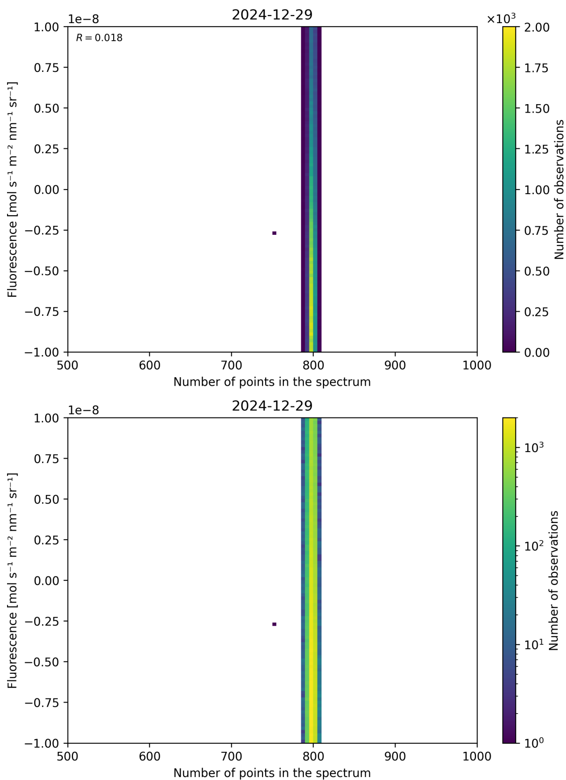
Figure 91: Scatter density plot of “Number of points in the spectrum” against “Fluorescence” for 2024-12-28 to 2024-12-30.
