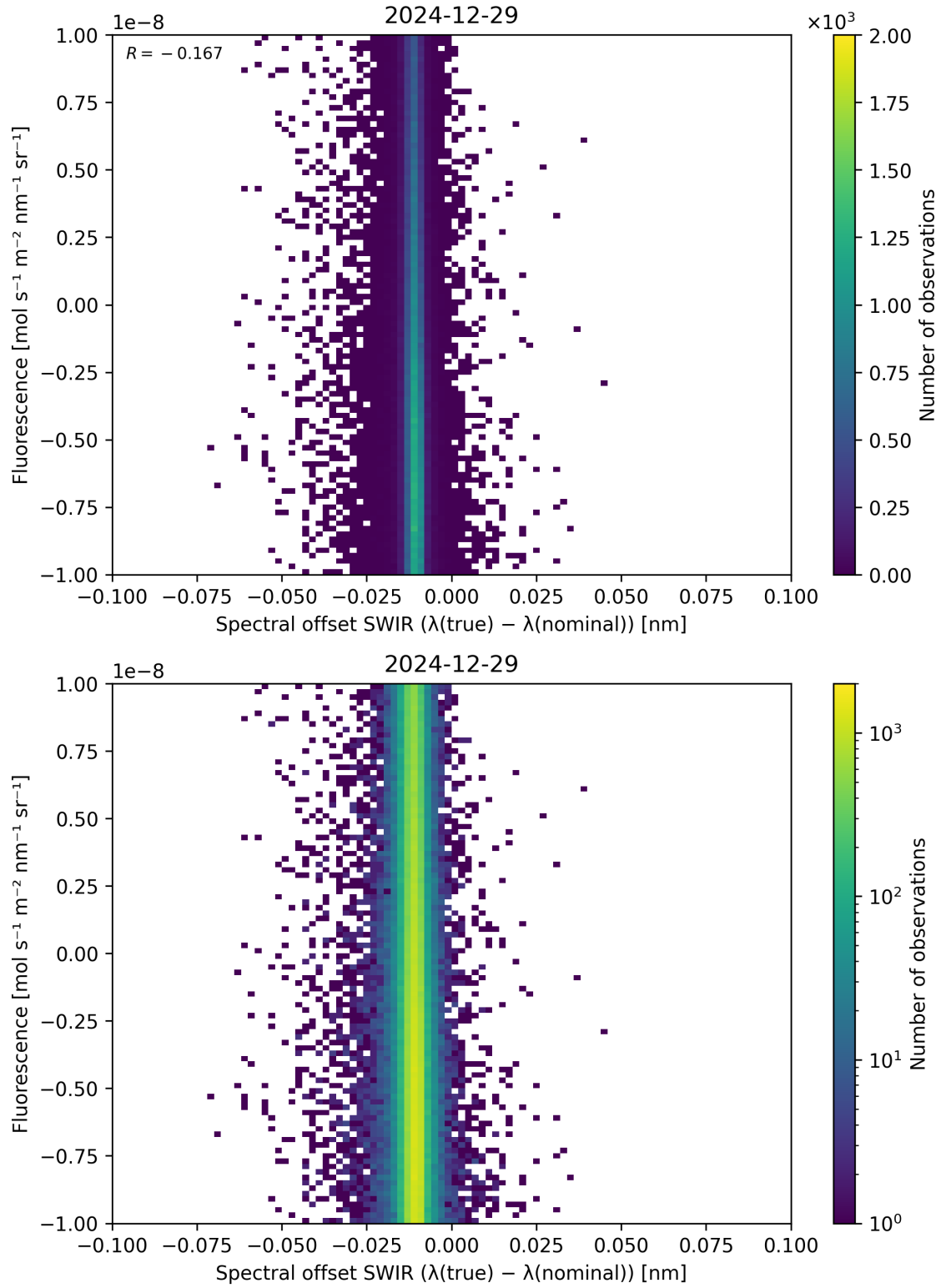
Figure 120: Scatter density plot of “Spectral offset SWIR ( \lambda_{\text{true}} - \lambda_{\text{nominal}} )” against “Fluorescence” for 2024-12-28 to 2024-12-30.
