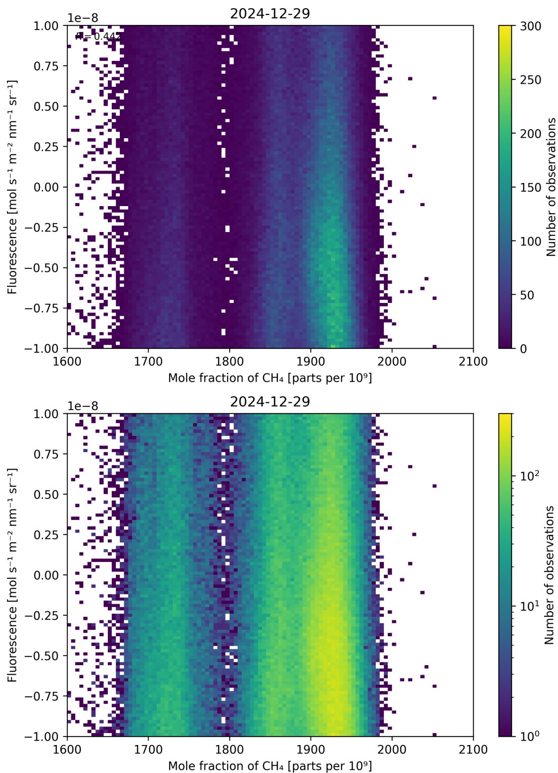
Figure 73: Scatter density plot of “Mole fraction of \text{CH}_4 ” against “Fluorescence” for 2024-12-28 to 2024-12-30.
