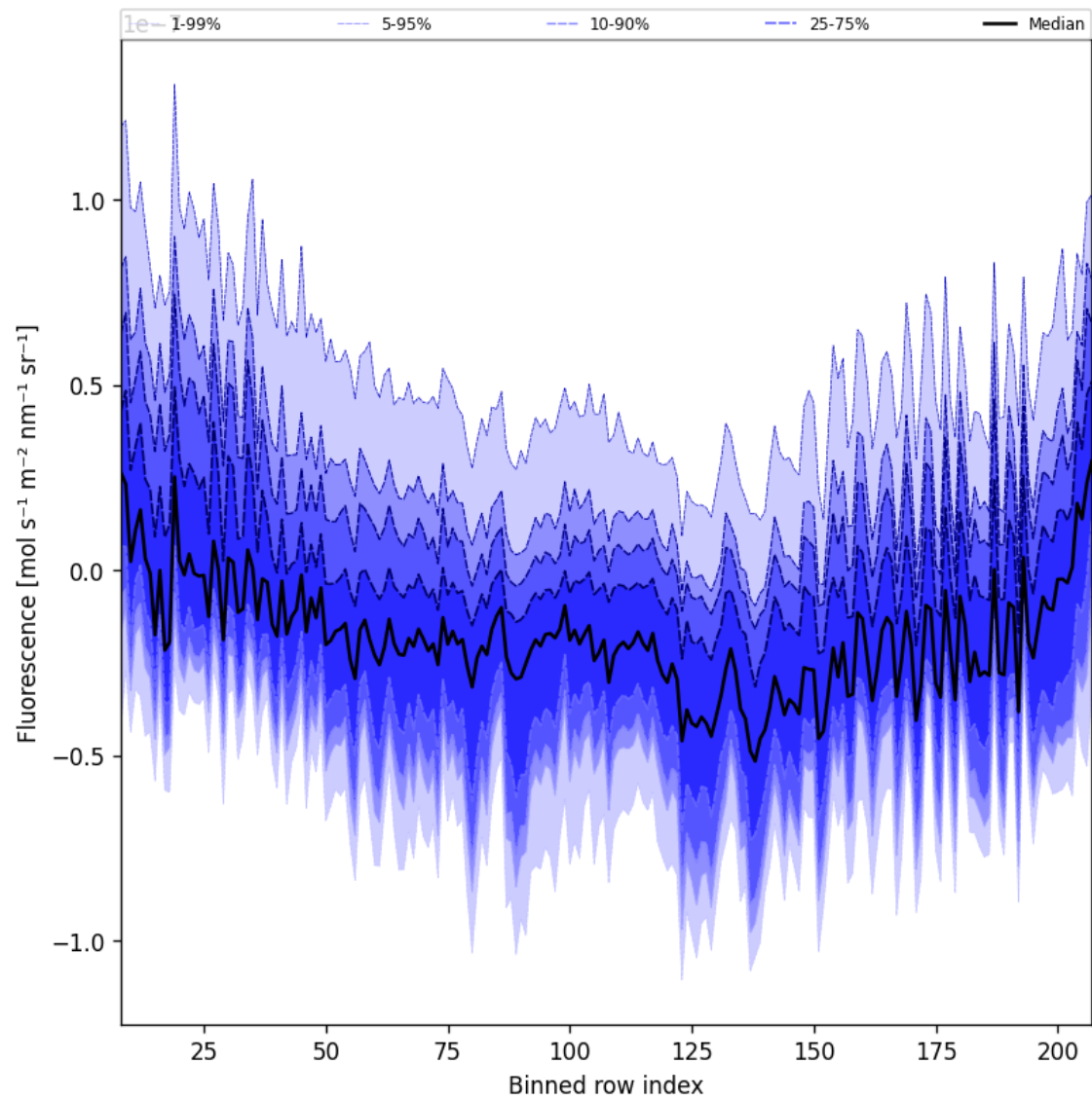
Figure 43: Along track statistics of “Fluorescence” for 2024-12-28 to 2024-12-30
