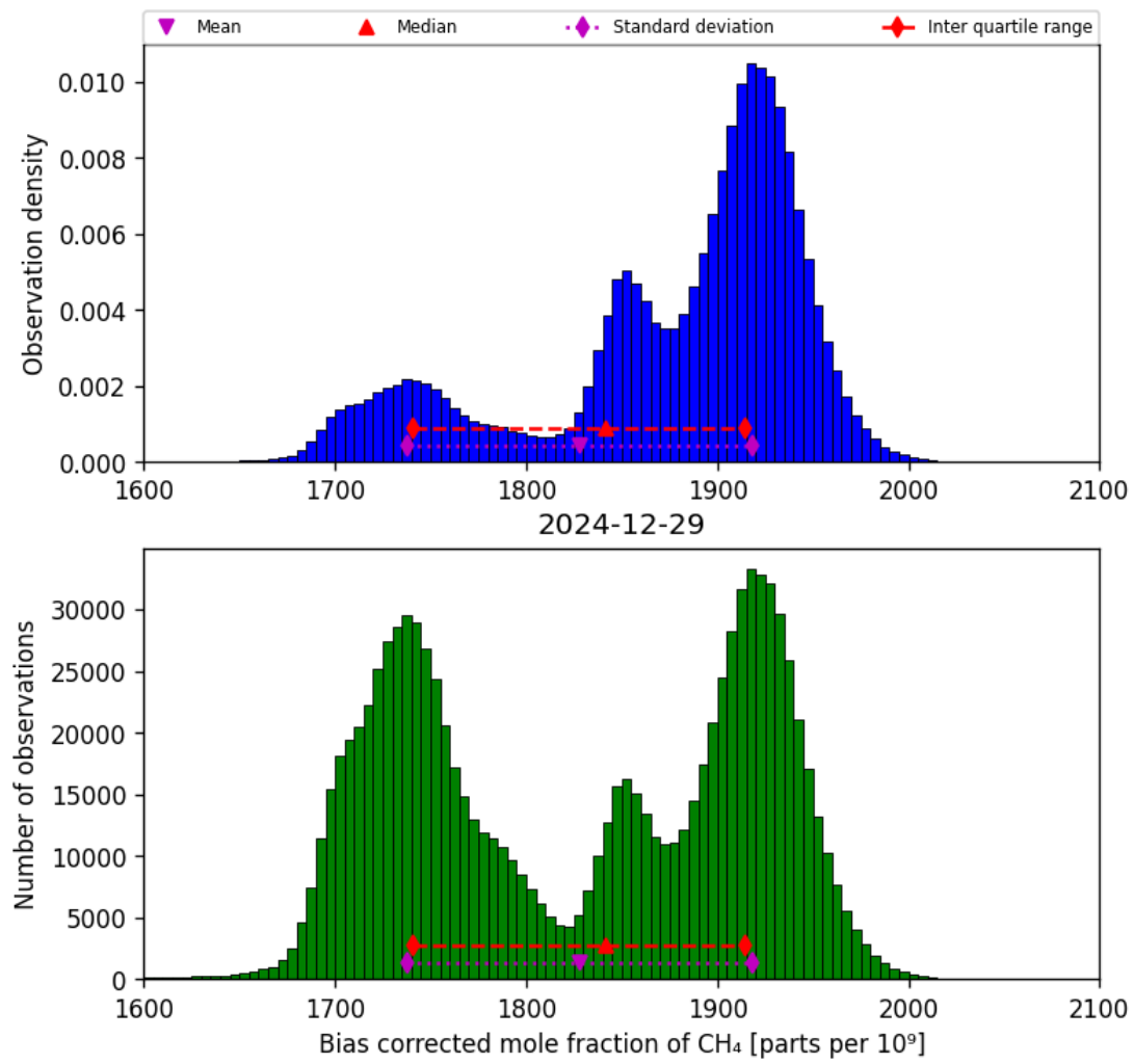
Figure 25: Histogram of “Bias corrected mole fraction of CH 4 ” for 2024-12-28 to 2024-12-30
