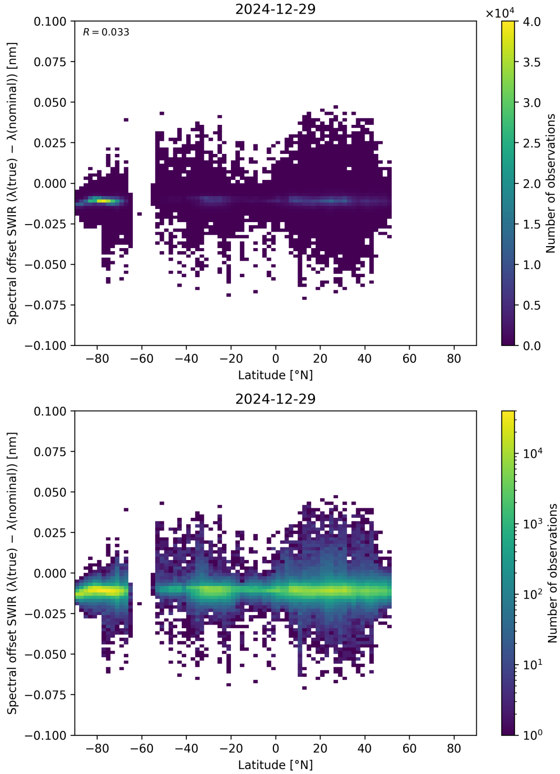
Figure 62: Scatter density plot of “Latitude” against “Spectral offset SWIR ( \lambda_{\text{true}} - \lambda_{\text{nominal}} )” for 2024-12-28 to 2024-12-30.
