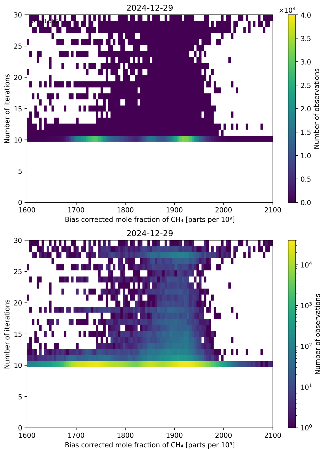
Figure 67: Scatter density plot of “Bias corrected mole fraction of \text{CH}_4 ” against “Number of iterations” for 2024-12-28 to 2024-12-30.
