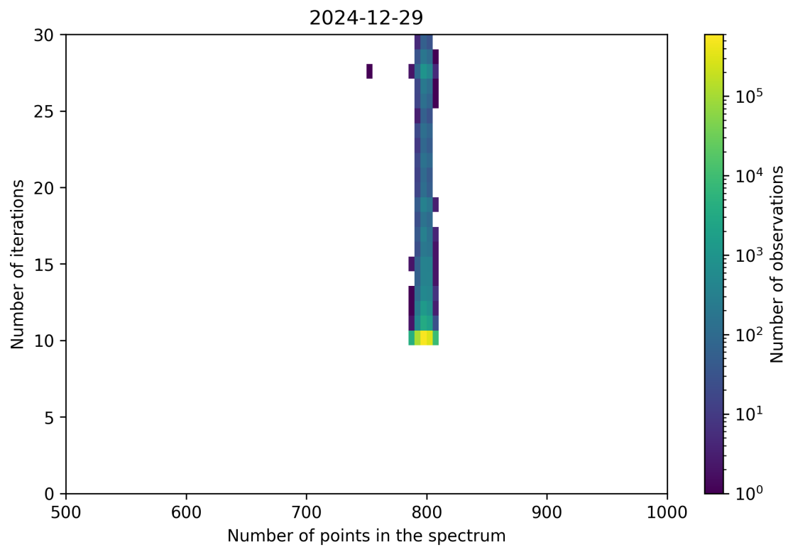
Figure 92: Scatter density plot of “Number of points in the spectrum” against “Number of iterations” for 2024-12-28 to 2024-12-30.
