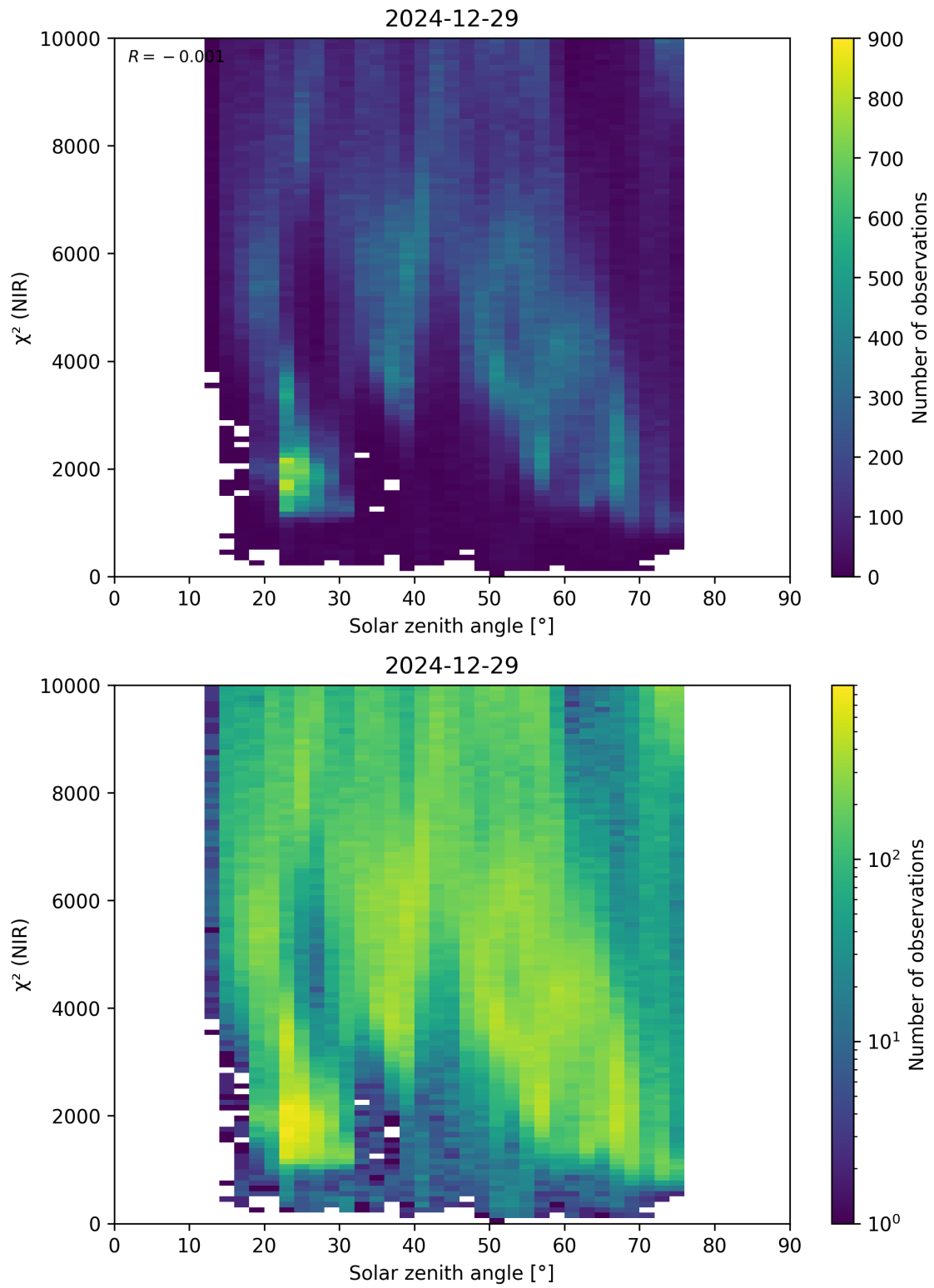
Figure 94: Scatter density plot of “Solar zenith angle” against “ \chi^2 (NIR)” for 2024-12-28 to 2024-12-30.
