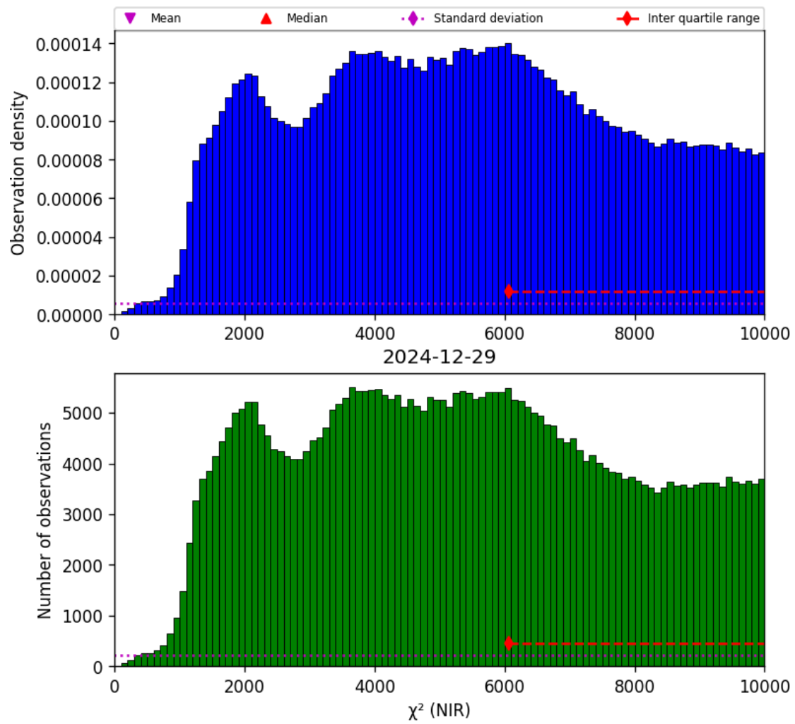
Figure 29: Histogram of “ \chi^2 (NIR)” for 2024-12-28 to 2024-12-30
