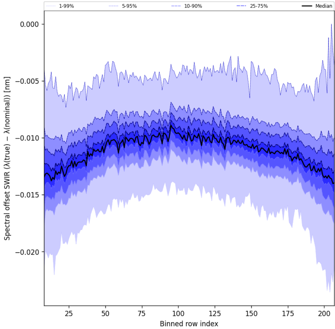
Figure 38: Along track statistics of “Spectral offset SWIR ( \lambda_{\text{true}} - \lambda_{\text{nominal}} )” for 2024-12-28 to 2024-12-30
