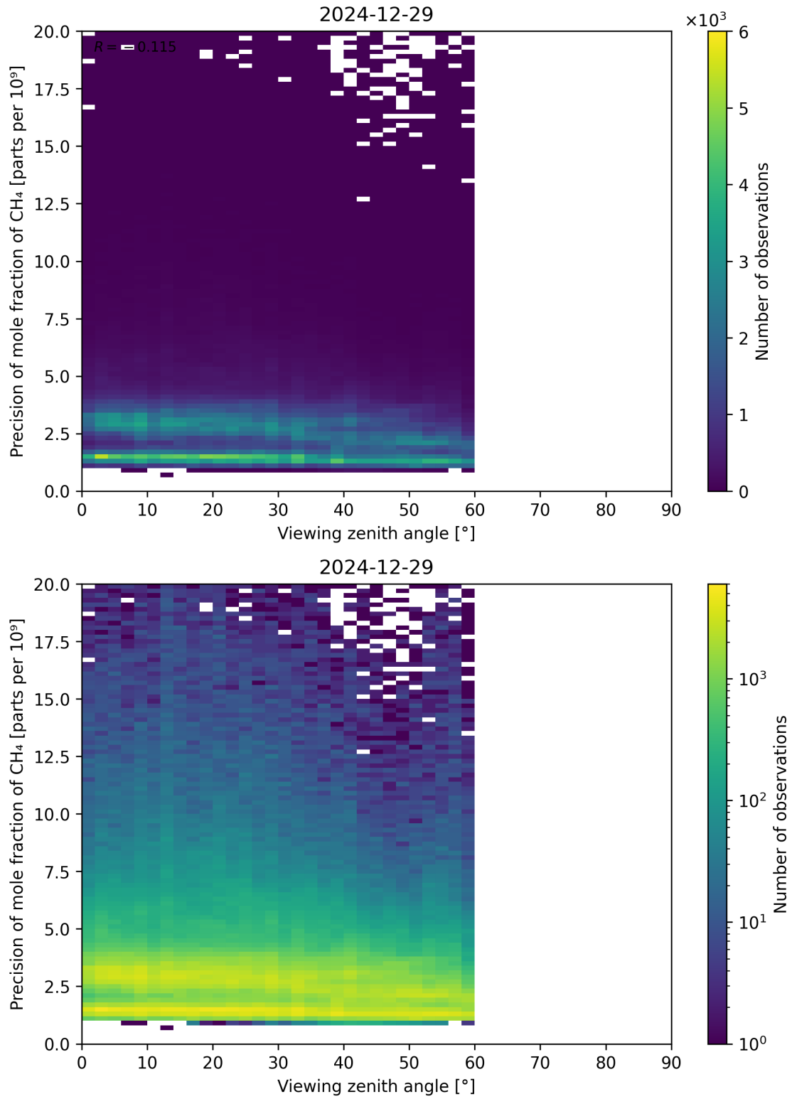
Figure 112: Scatter density plot of “Viewing zenith angle” against “Precision of mole fraction of CH 4 ” for 2024-12-28 to 2024-12-30.
