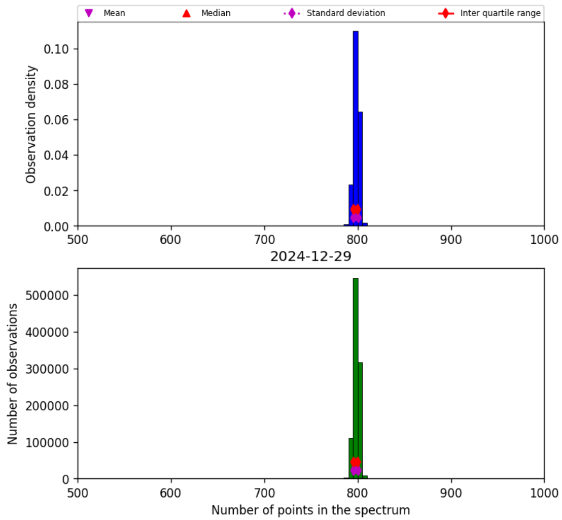
Figure 26: Histogram of “Number of points in the spectrum” for 2024-12-28 to 2024-12-30
