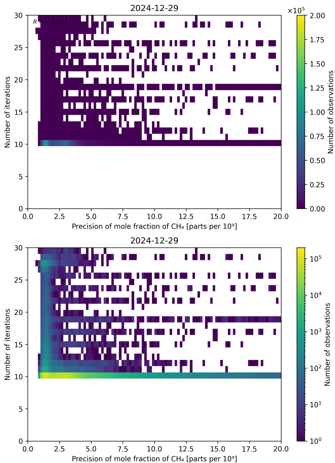
Figure 83: Scatter density plot of “Precision of mole fraction of CH 4 ” against “Number of iterations” for 2024-12-28 to 2024-12-30.
