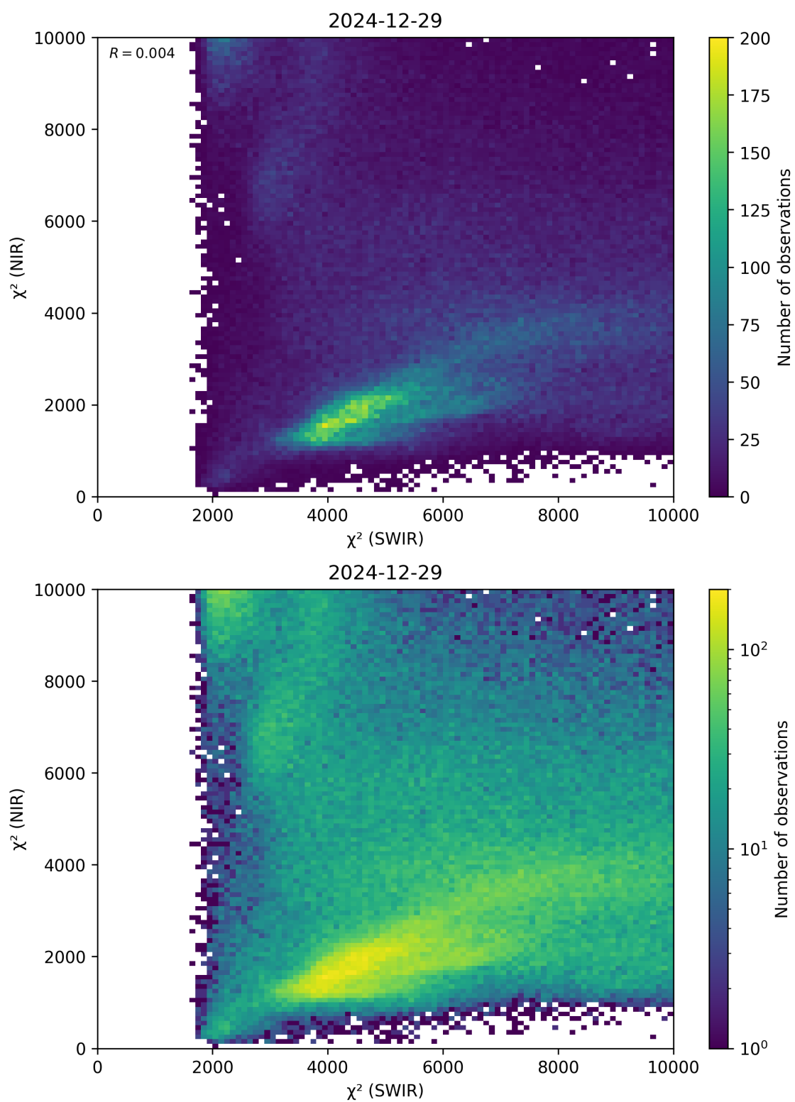
Figure 47: Scatter density plot of “ \chi^2 (SWIR)” against “ \chi^2 (NIR)” for 2024-12-28 to 2024-12-30.
