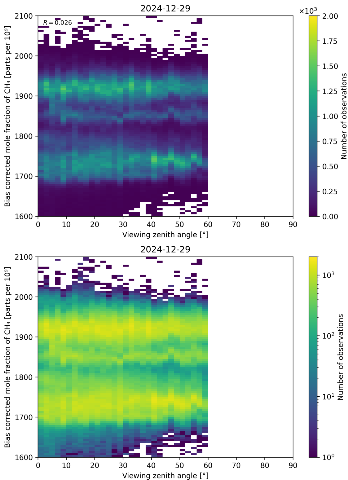
Figure 111: Scatter density plot of “Viewing zenith angle” against “Bias corrected mole fraction of CH 4 ” for 2024-12-28 to 2024-12-30.
