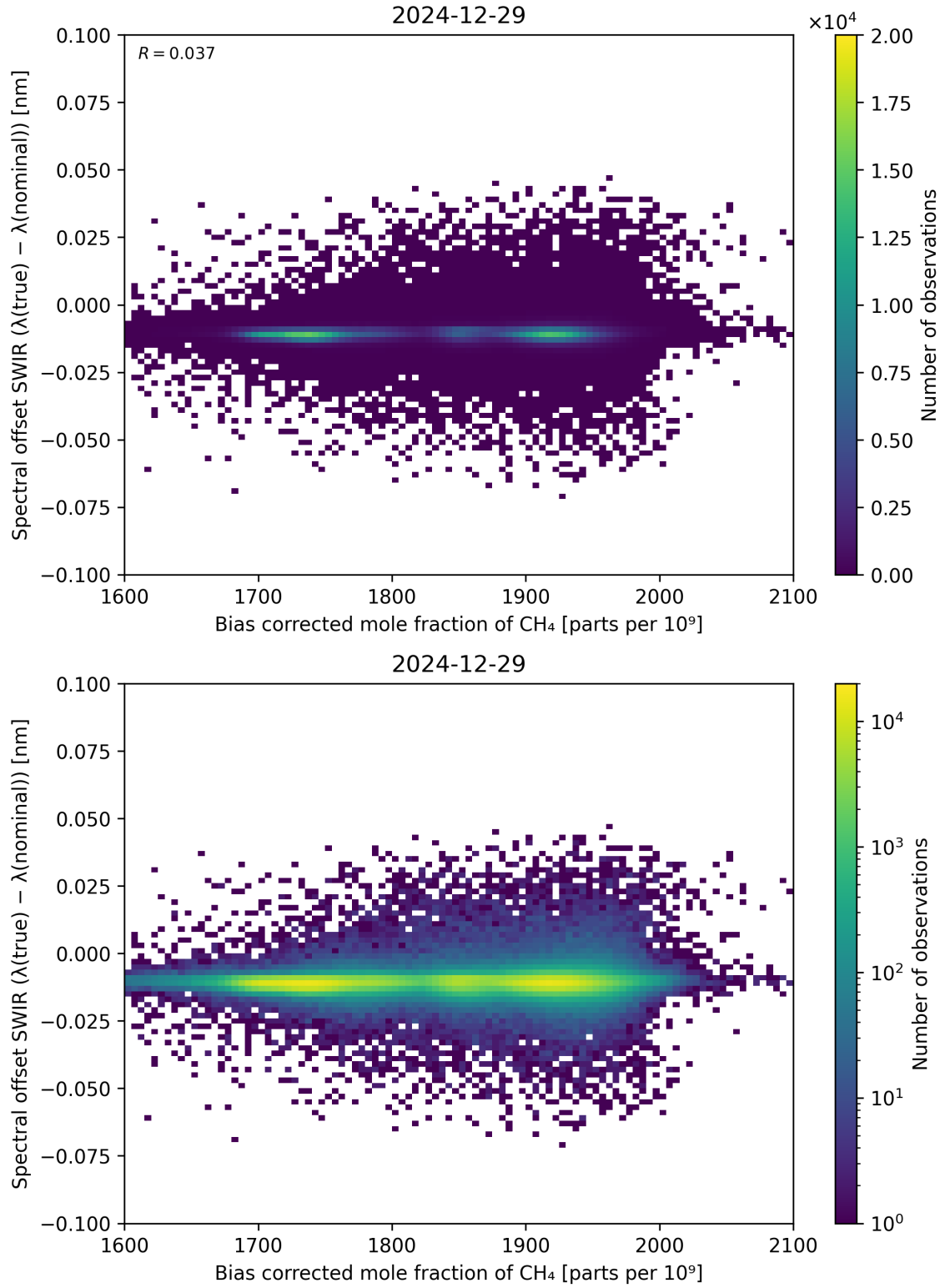
Figure 69: Scatter density plot of “Bias corrected mole fraction of \text{CH}_4 ” against “Spectral offset SWIR ( \lambda_{\text{true}} - \lambda_{\text{nominal}} )” for 2024-12-28 to 2024-12-30.
