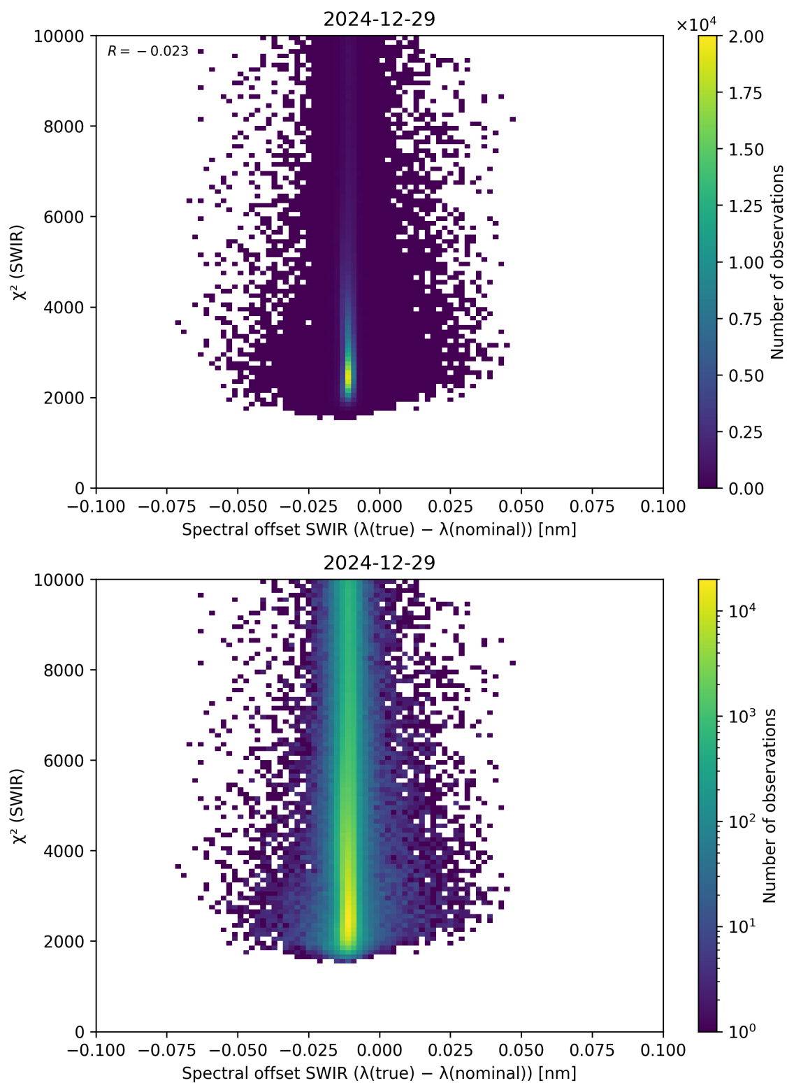
Figure 118: Scatter density plot of “Spectral offset SWIR ( \lambda_{\text{true}} - \lambda_{\text{nominal}} )” against “ \chi^2 (SWIR)” for 2024-12-28 to 2024-12-30.
