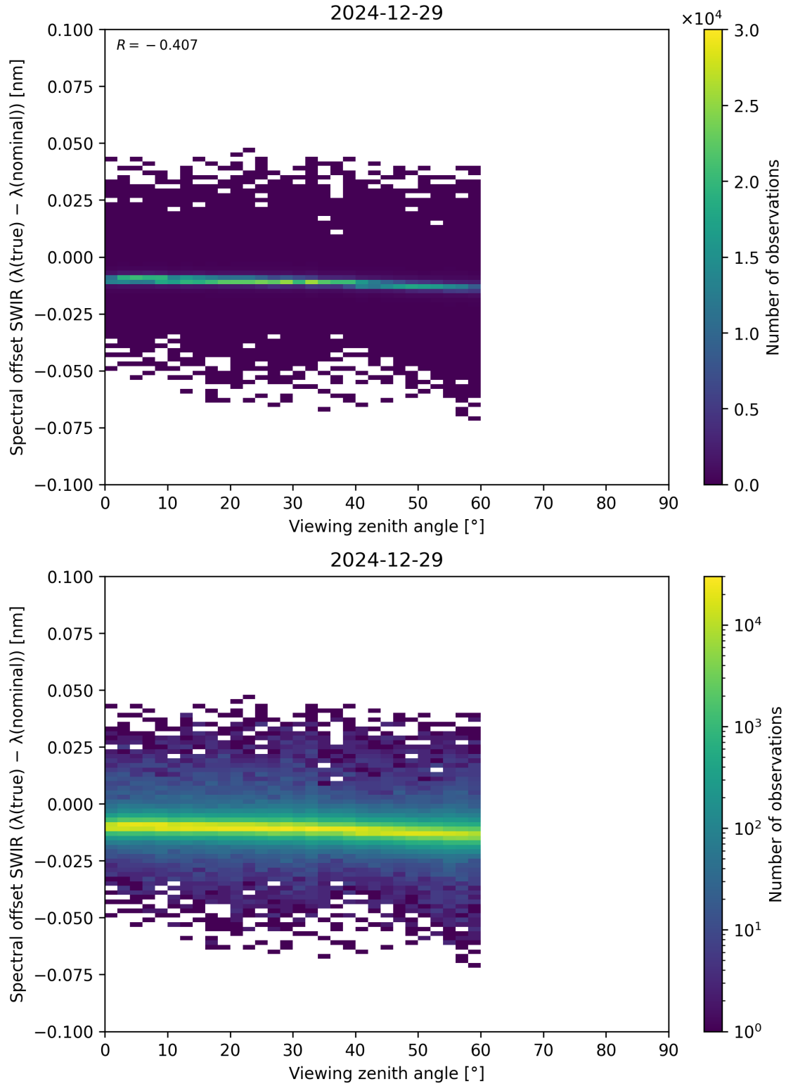
Figure 116: Scatter density plot of “Viewing zenith angle” against “Spectral offset SWIR ( \lambda_{\text{true}} - \lambda_{\text{nominal}} )” for 2024-12-28 to 2024-12-30.
