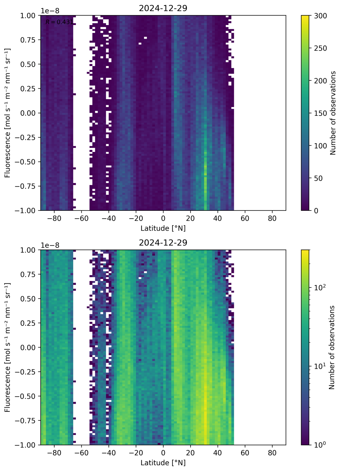
Figure 56: Scatter density plot of “Latitude” against “Fluorescence” for 2024-12-28 to 2024-12-30.
