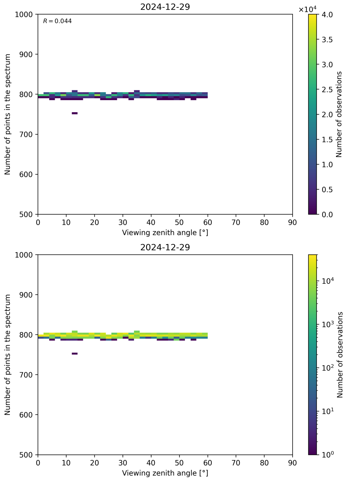
Figure 114: Scatter density plot of “Viewing zenith angle” against “Number of points in the spectrum” for 2024-12-28 to 2024-12-30.
