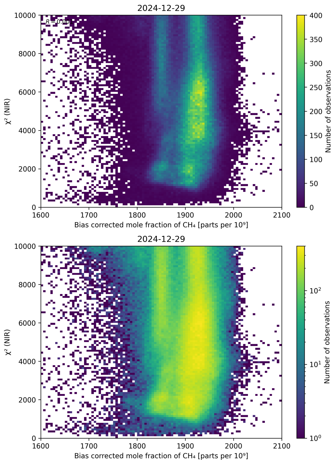
Figure 63: Scatter density plot of “Bias corrected mole fraction of \text{CH}_4 ” against “ \chi^2 (NIR)” for 2024-12-28 to 2024-12-30.
