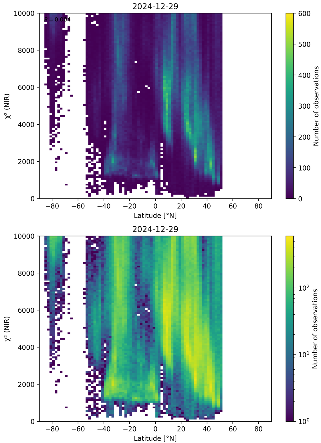
Figure 53: Scatter density plot of “Latitude” against “ \chi^2 (NIR)” for 2024-12-28 to 2024-12-30.
