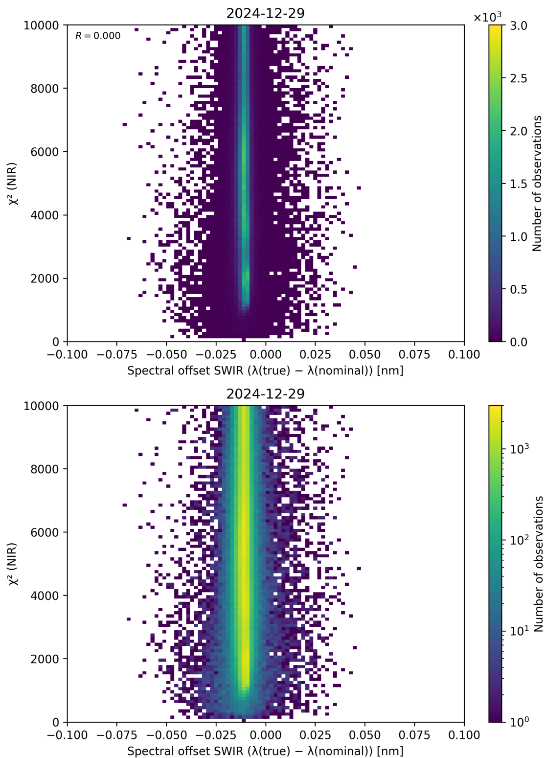
Figure 117: Scatter density plot of “Spectral offset SWIR ( \lambda_{\text{true}} - \lambda_{\text{nominal}} )” against “ \chi^2 (NIR)” for 2024-12-28 to 2024-12-30.
