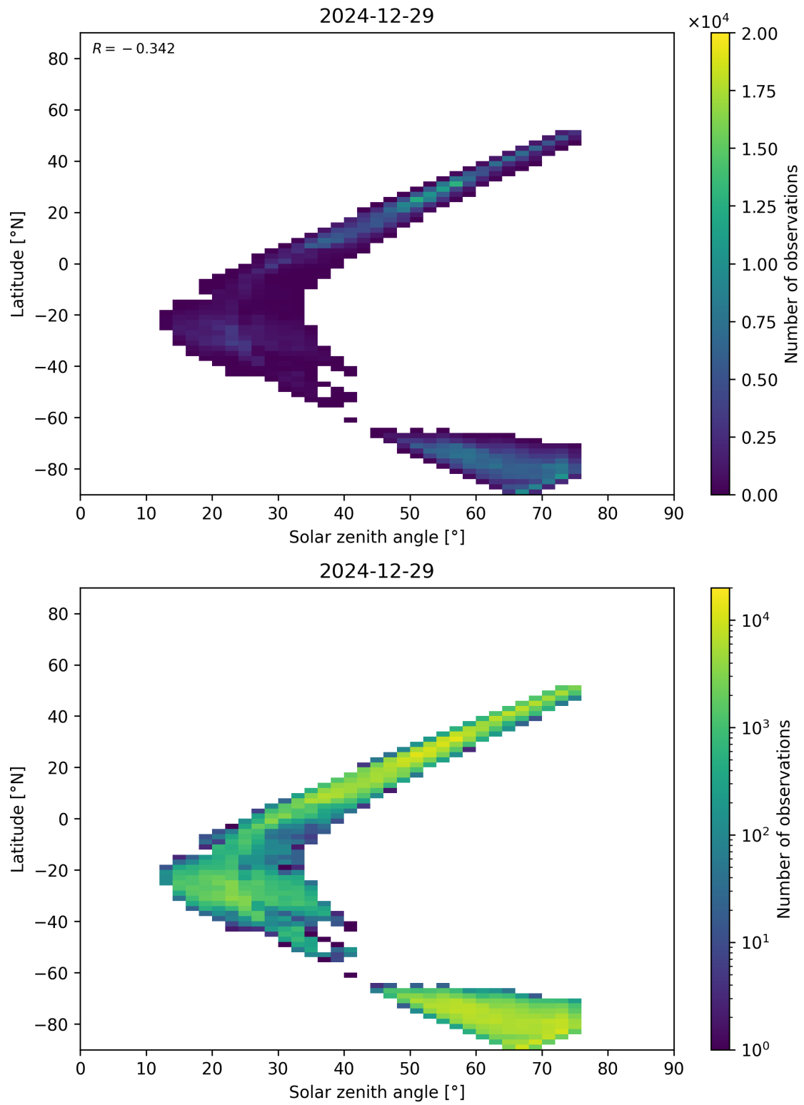
Figure 98: Scatter density plot of “Solar zenith angle” against “Latitude” for 2024-12-28 to 2024-12-30.
