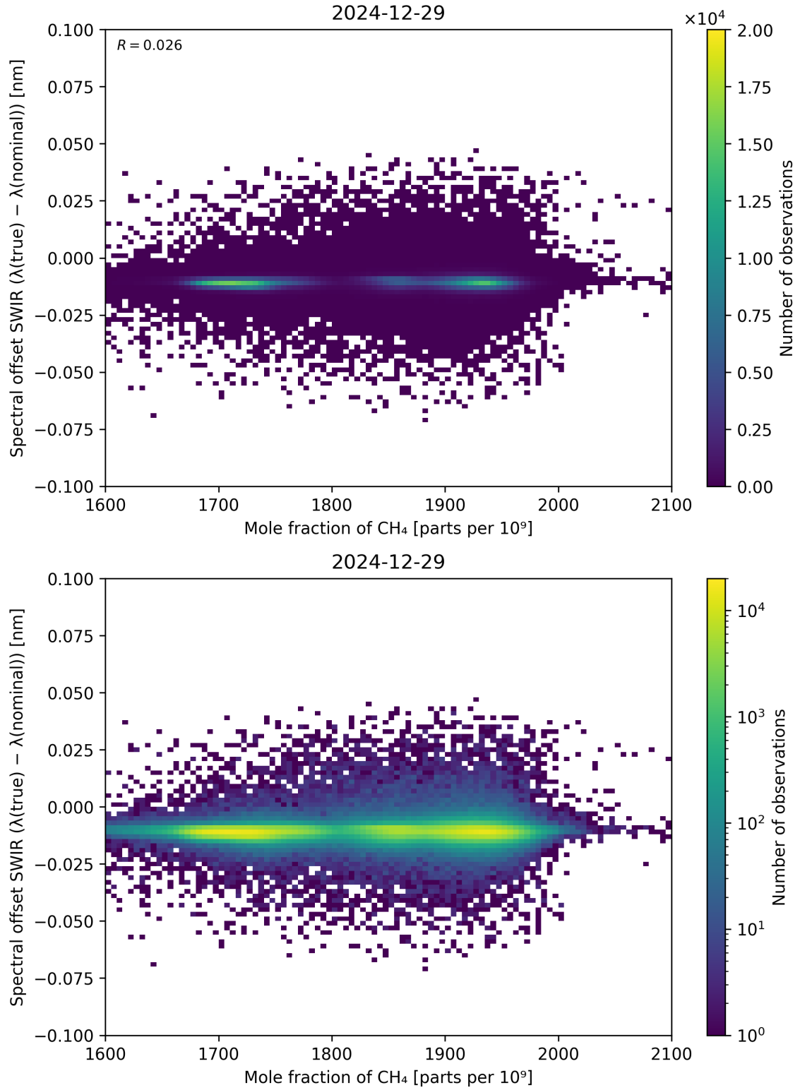
Figure 86: Scatter density plot of “Mole fraction of \text{CH}_4 ” against “Spectral offset SWIR ( \lambda_{\text{true}} - \lambda_{\text{nominal}} )” for 2024-12-28 to 2024-12-30.
