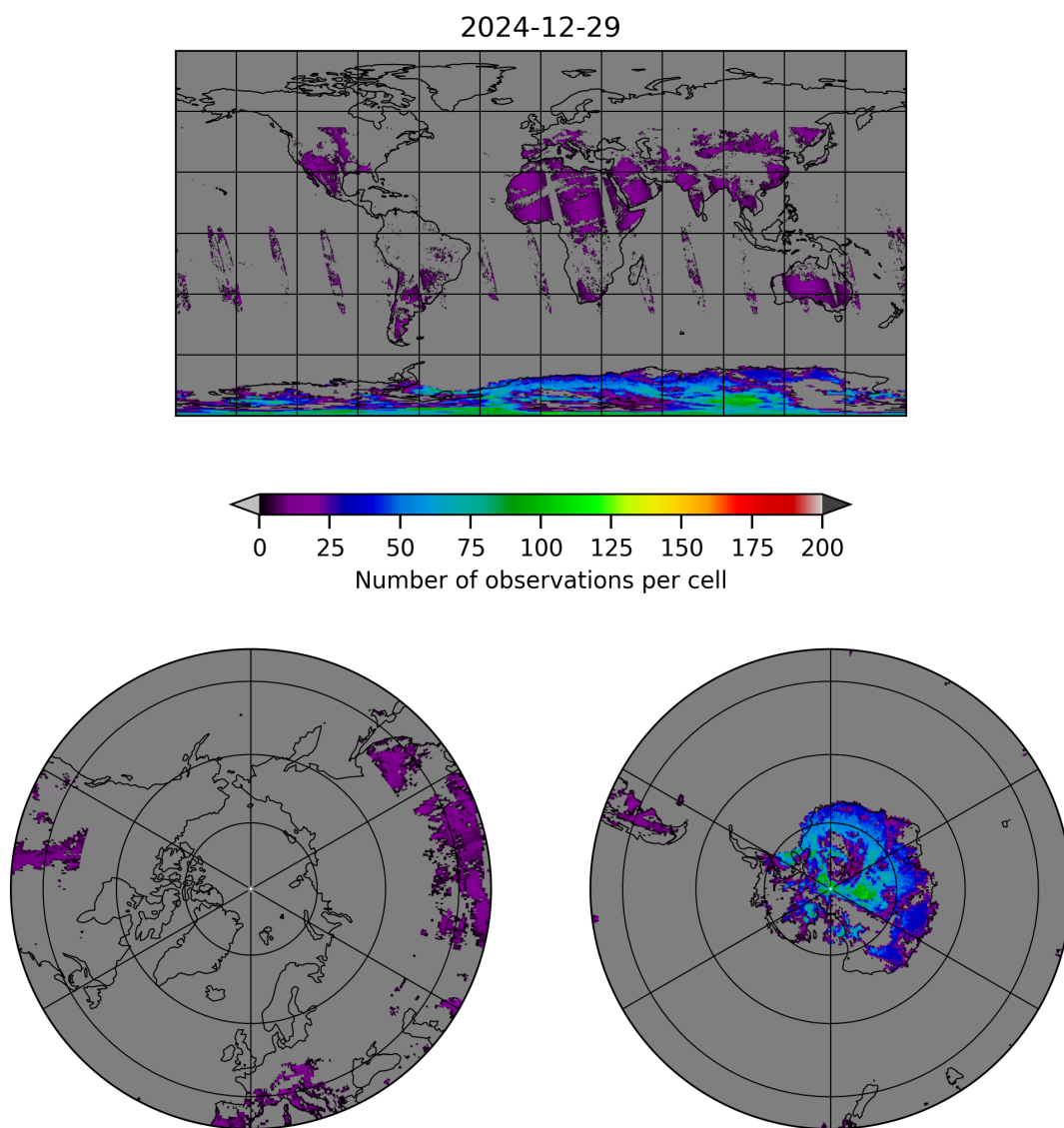
Figure 10: Map of the number of observations for 2024-12-28 to 2024-12-30
