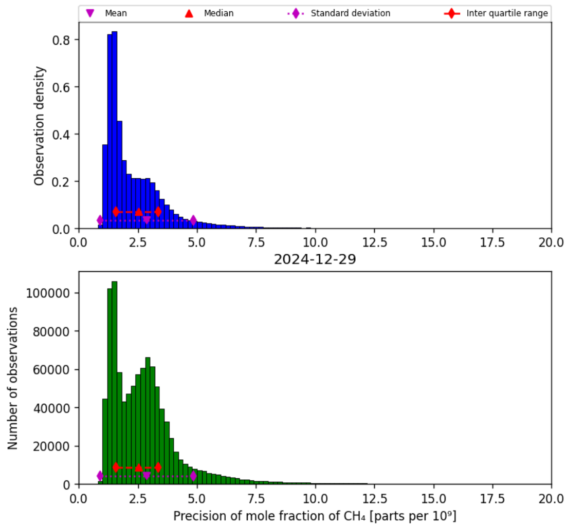
Figure 24: Histogram of “Precision of mole fraction of CH 4 ” for 2024-12-28 to 2024-12-30
