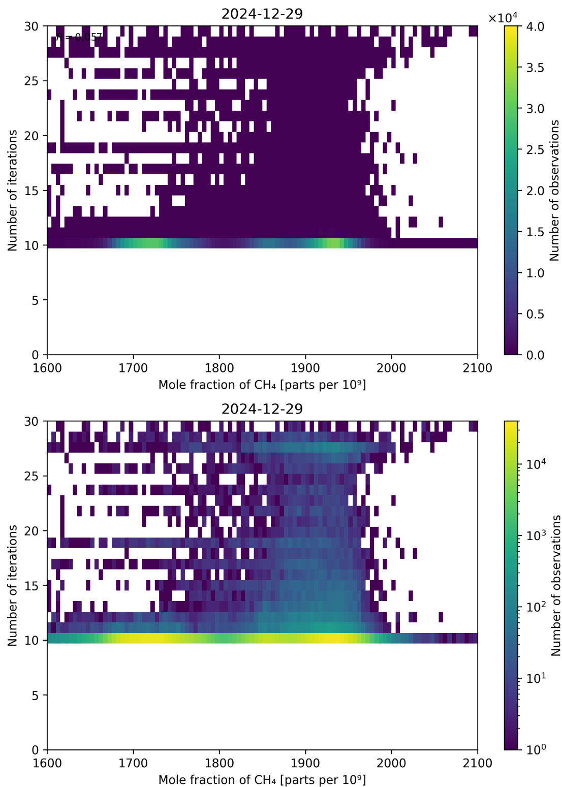
Figure 76: Scatter density plot of “Mole fraction of CH 4 ” against “Number of iterations” for 2024-12-28 to 2024-12-30.
