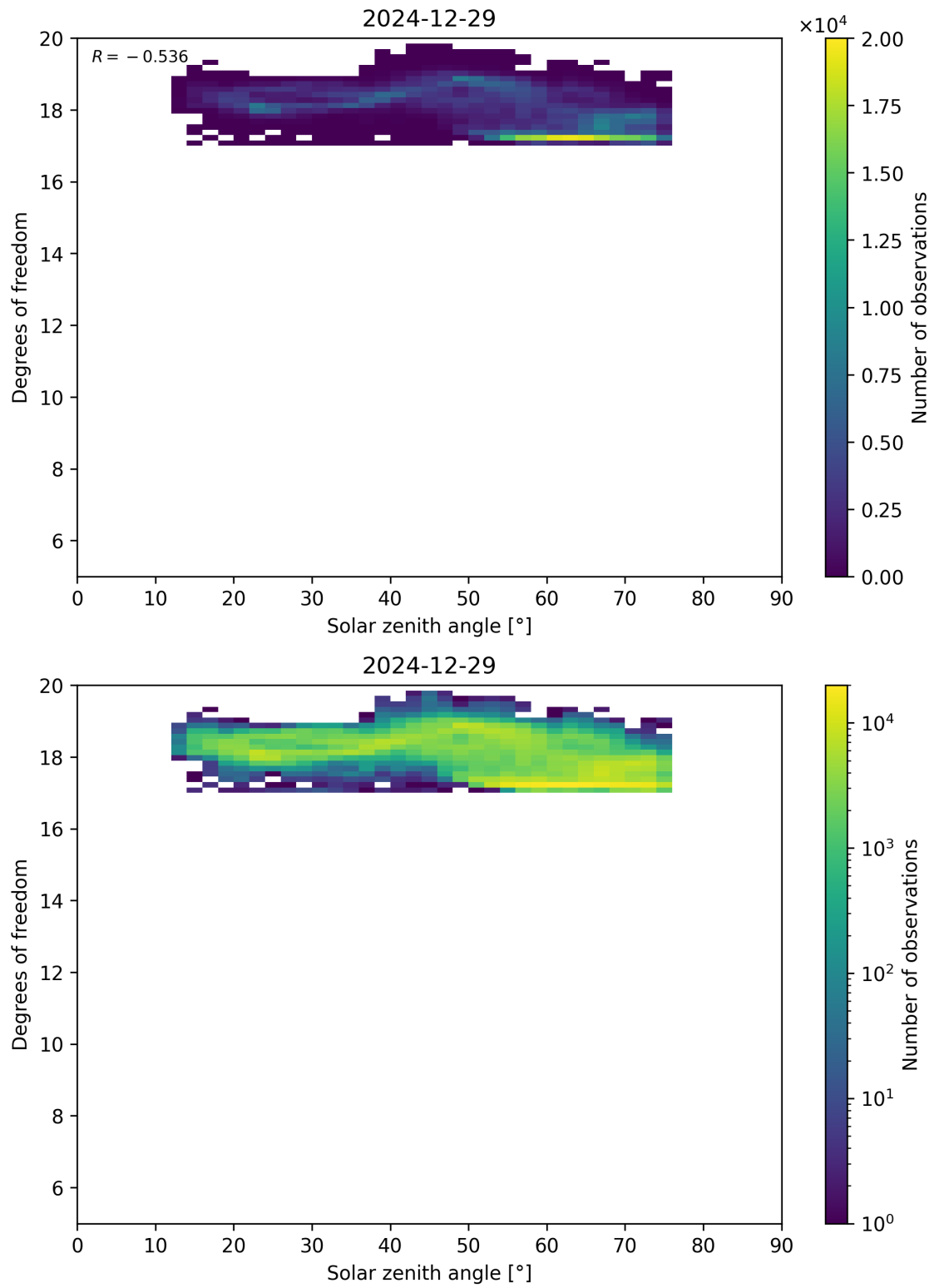
Figure 96: Scatter density plot of “Solar zenith angle” against “Degrees of freedom” for 2024-12-28 to 2024-12-30.
