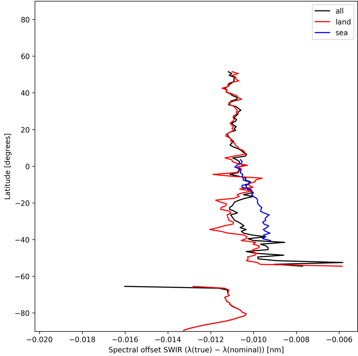
Figure 16: Zonal average of “Spectral offset SWIR ( \lambda_{\text{true}} - \lambda_{\text{nominal}} )” for 2024-12-28 to 2024-12-30.
