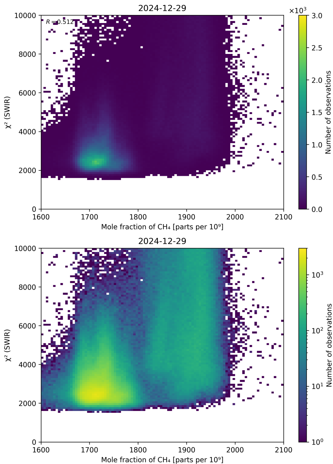
Figure 71: Scatter density plot of “Mole fraction of \text{CH}_4 ” against “ \chi^2 (SWIR)” for 2024-12-28 to 2024-12-30.
