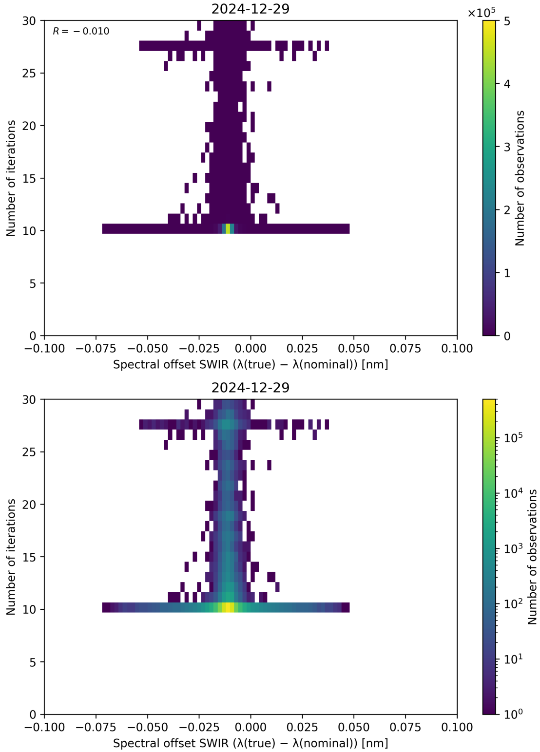
Figure 121: Scatter density plot of “Spectral offset SWIR ( \lambda_{\text{true}} - \lambda_{\text{nominal}} )” against “Number of iterations” for 2024-12-28 to 2024-12-30.
