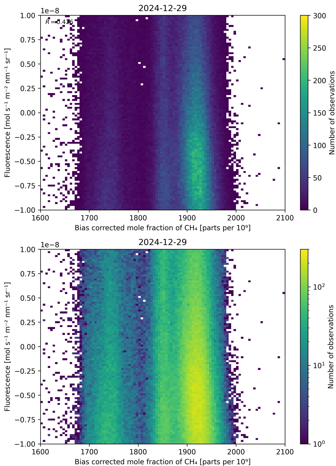
Figure 66: Scatter density plot of “Bias corrected mole fraction of \text{CH}_4 ” against “Fluorescence” for 2024-12-28 to 2024-12-30.
