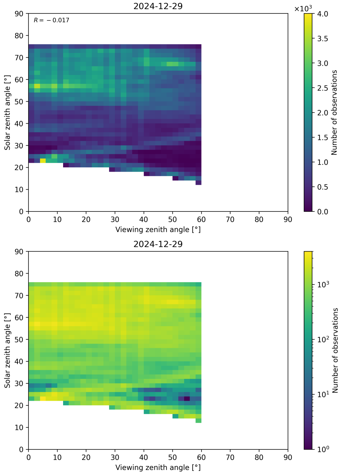
Figure 115: Scatter density plot of “Viewing zenith angle” against “Solar zenith angle” for 2024-12-28 to 2024-12-30.
