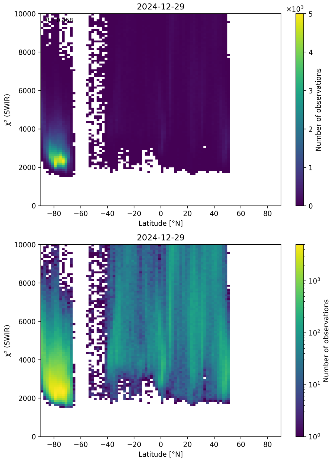
Figure 54: Scatter density plot of “Latitude” against “ \chi^2 (SWIR)” for 2024-12-28 to 2024-12-30.
