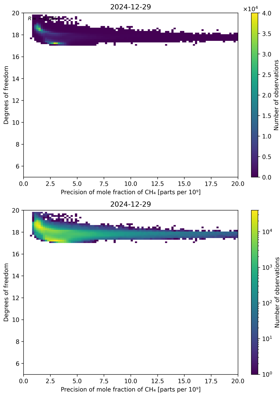
Figure 80: Scatter density plot of “Precision of mole fraction of CH 4 ” against “Degrees of freedom” for 2024-12-28 to 2024-12-30.
