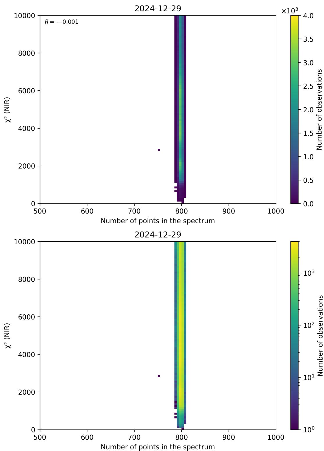
Figure 88: Scatter density plot of “Number of points in the spectrum” against “ \chi^2 (NIR)” for 2024-12-28 to 2024-12-30.
