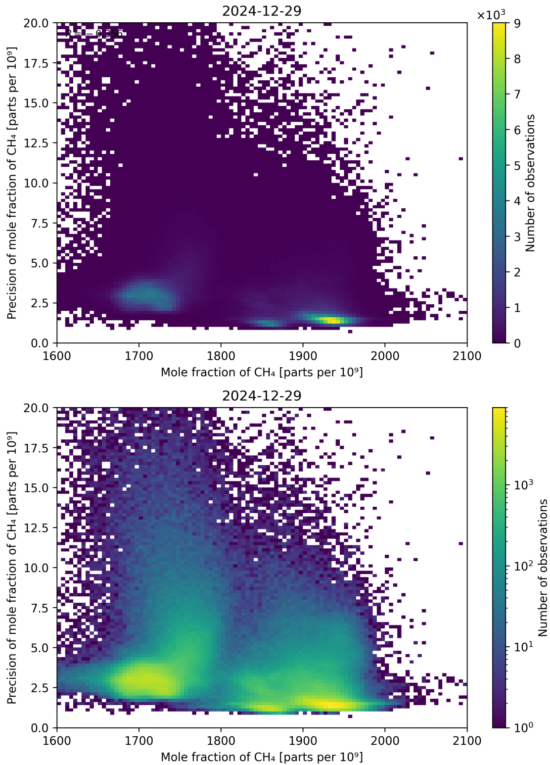
Figure 75: Scatter density plot of “Mole fraction of CH 4 ” against “Precision of mole fraction of CH 4 ” for 2024-12-28 to 2024-12-30.
