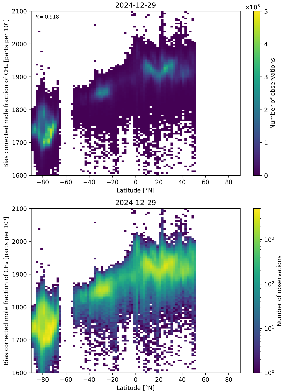
Figure 58: Scatter density plot of “Latitude” against “Bias corrected mole fraction of \text{CH}_4 ” for 2024-12-28 to 2024-12-30.
