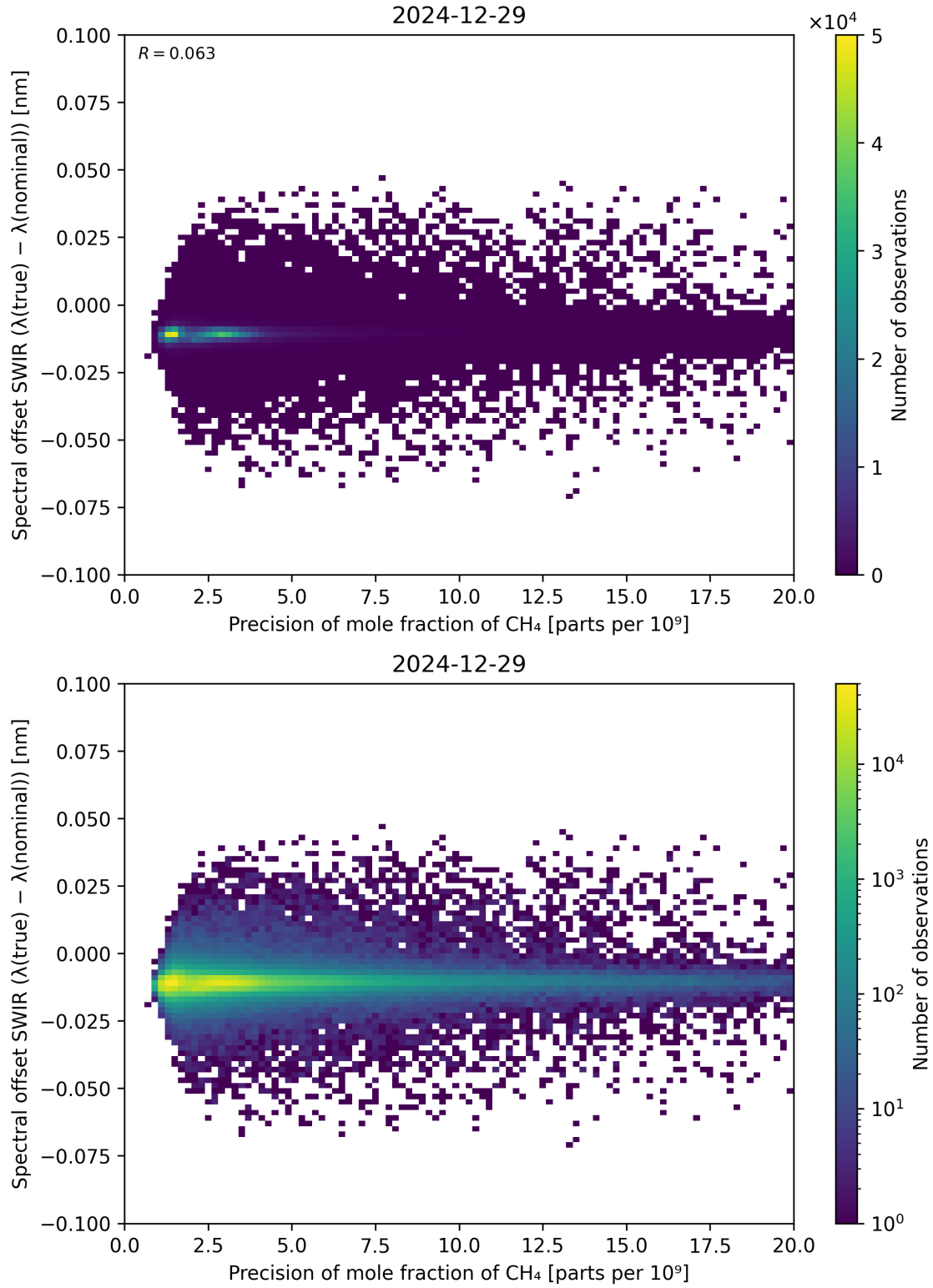
Figure 85: Scatter density plot of “Precision of mole fraction of \text{CH}_4 ” against “Spectral offset SWIR ( \lambda_{\text{true}} - \lambda_{\text{nominal}} )” for 2024-12-28 to 2024-12-30.
