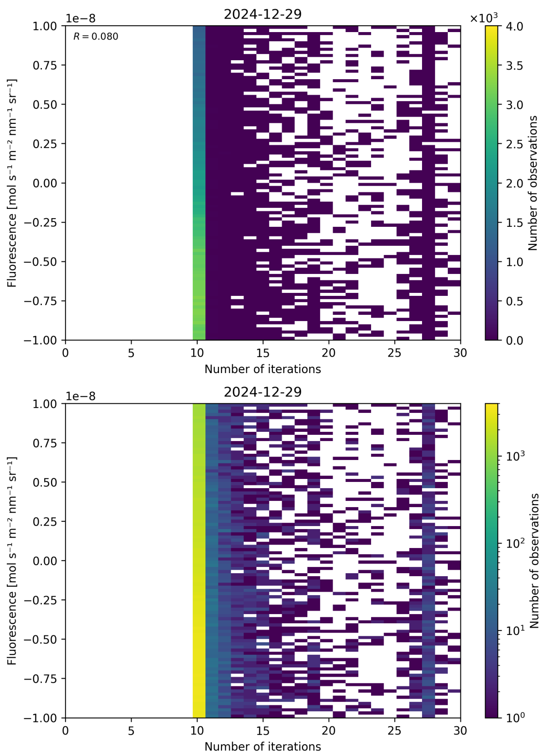
Figure 87: Scatter density plot of “Number of iterations” against “Fluorescence” for 2024-12-28 to 2024-12-30.
