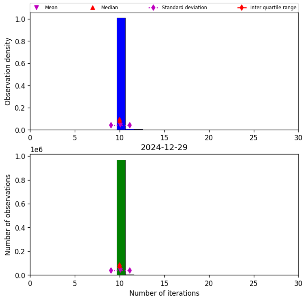
Figure 31: Histogram of “Number of iterations” for 2024-12-28 to 2024-12-30
