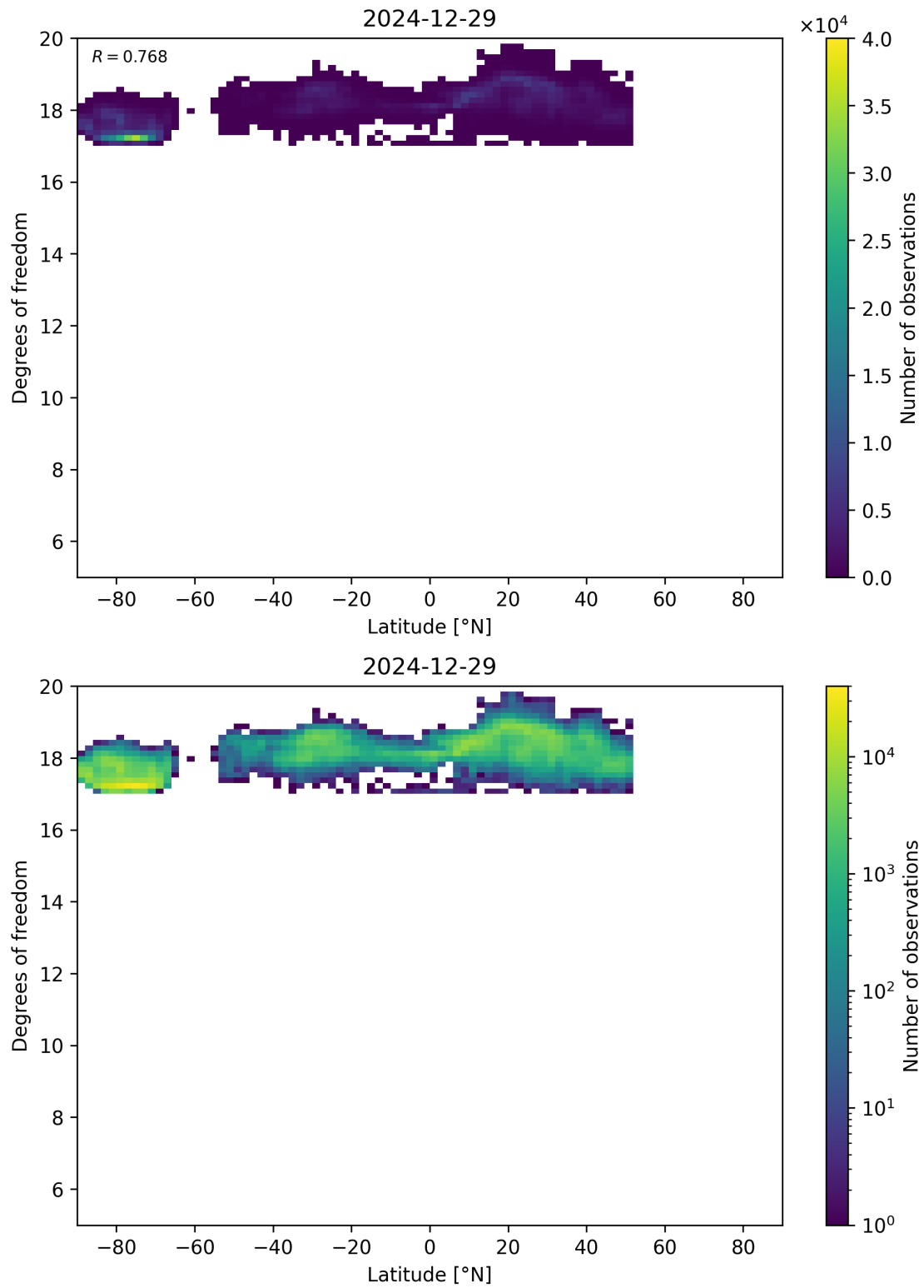
Figure 55: Scatter density plot of “Latitude” against “Degrees of freedom” for 2024-12-28 to 2024-12-30.
