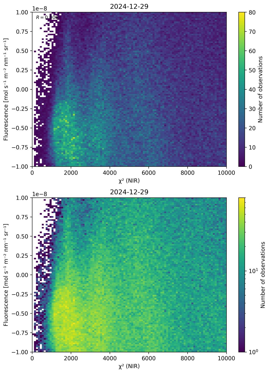
Figure 45: Scatter density plot of “ \chi^2 (NIR)” against “Fluorescence” for 2024-12-28 to 2024-12-30.
