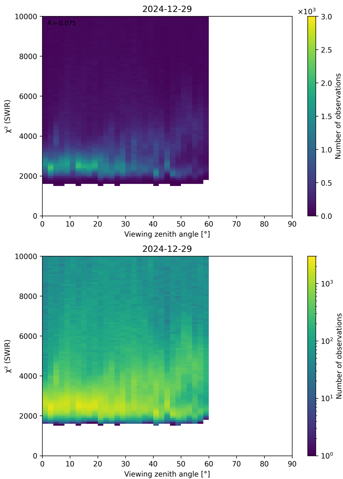
Figure 106: Scatter density plot of “Viewing zenith angle” against “ \chi^2 (SWIR)” for 2024-12-28 to 2024-12-30.
