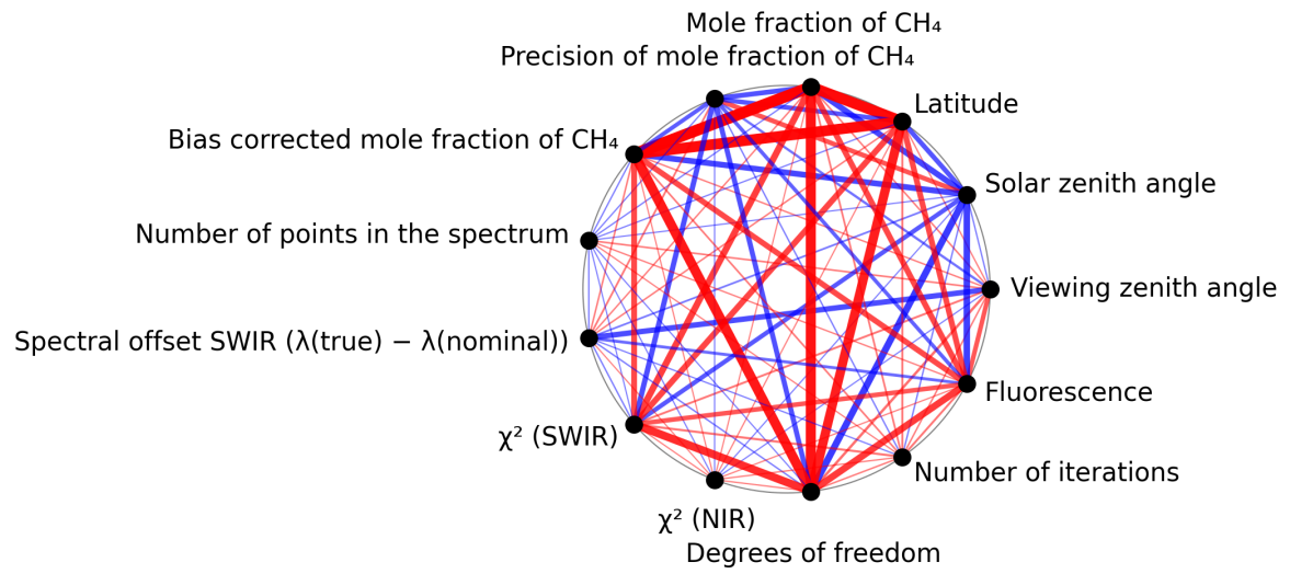
Figure 1: Map of correlation graph for 2024-12-28 to 2024-12-30.
