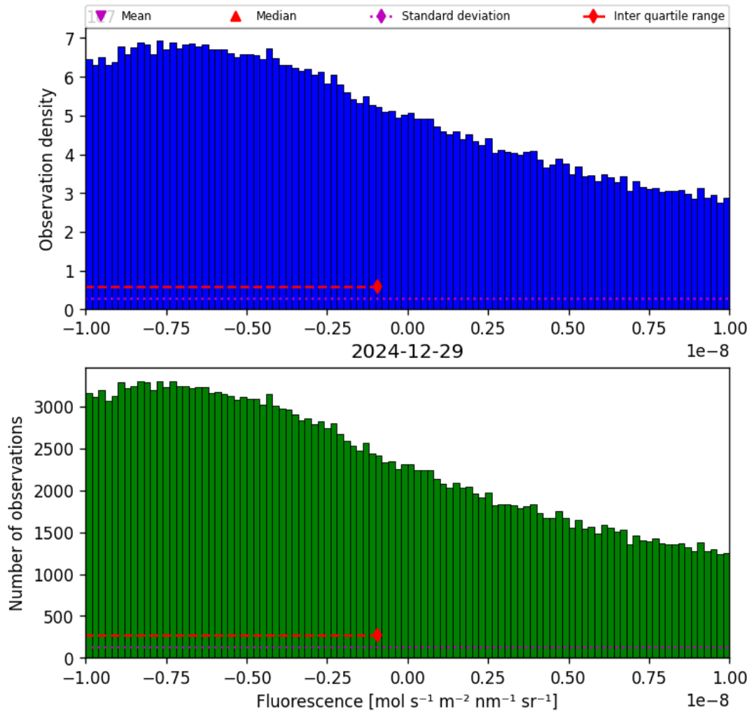
Figure 32: Histogram of “Fluorescence” for 2024-12-28 to 2024-12-30
