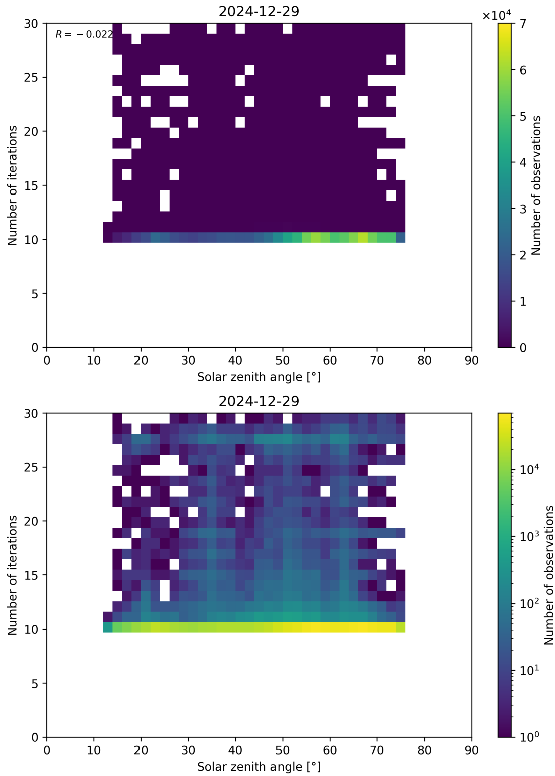
Figure 102: Scatter density plot of “Solar zenith angle” against “Number of iterations” for 2024-12-28 to 2024-12-30.
