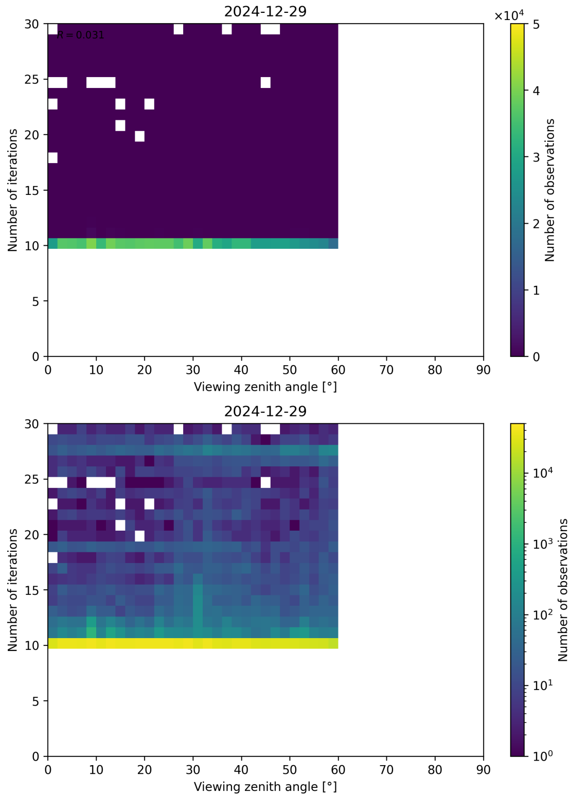
Figure 113: Scatter density plot of “Viewing zenith angle” against “Number of iterations” for 2024-12-28 to 2024-12-30.
