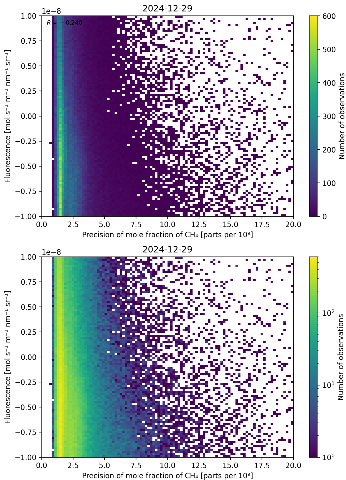
Figure 81: Scatter density plot of “Precision of mole fraction of \text{CH}_4 ” against “Fluorescence” for 2024-12-28 to 2024-12-30.
