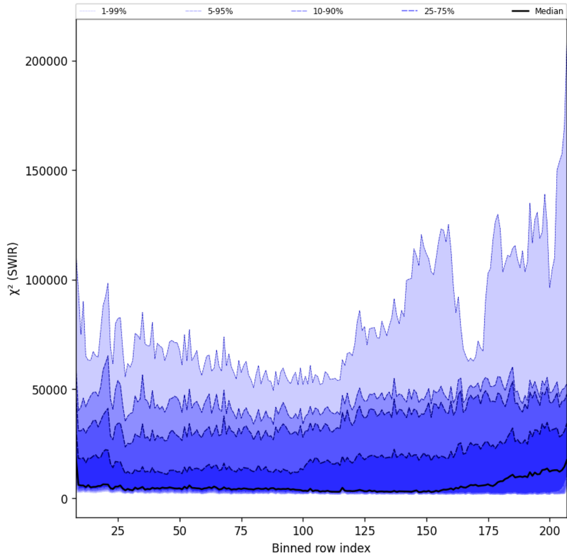
Figure 39: Along track statistics of " \chi^2 (SWIR)" for 2024-12-28 to 2024-12-30
