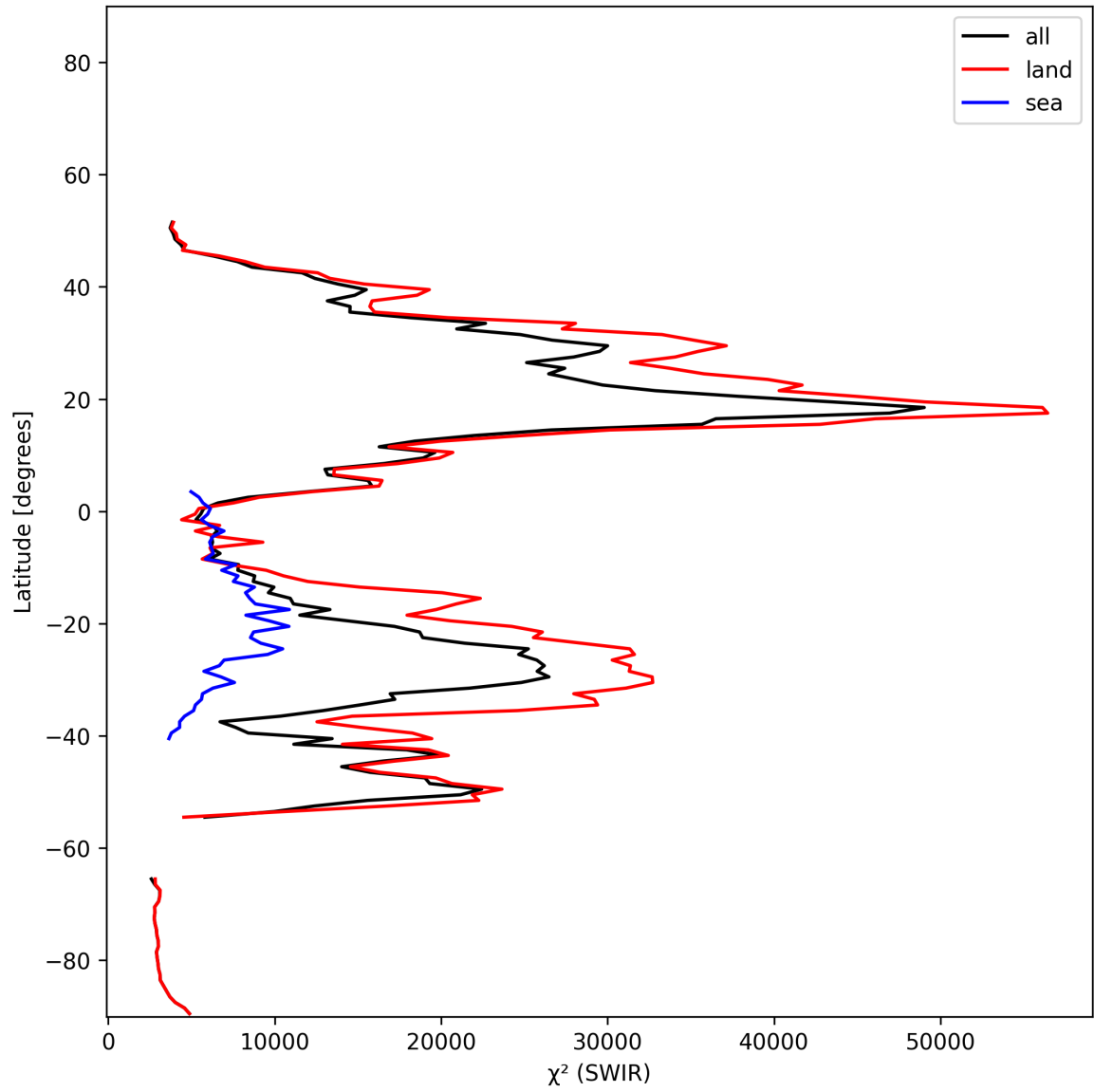
Figure 17: Zonal average of “ \chi^2 (SWIR)” for 2024-12-28 to 2024-12-30.
