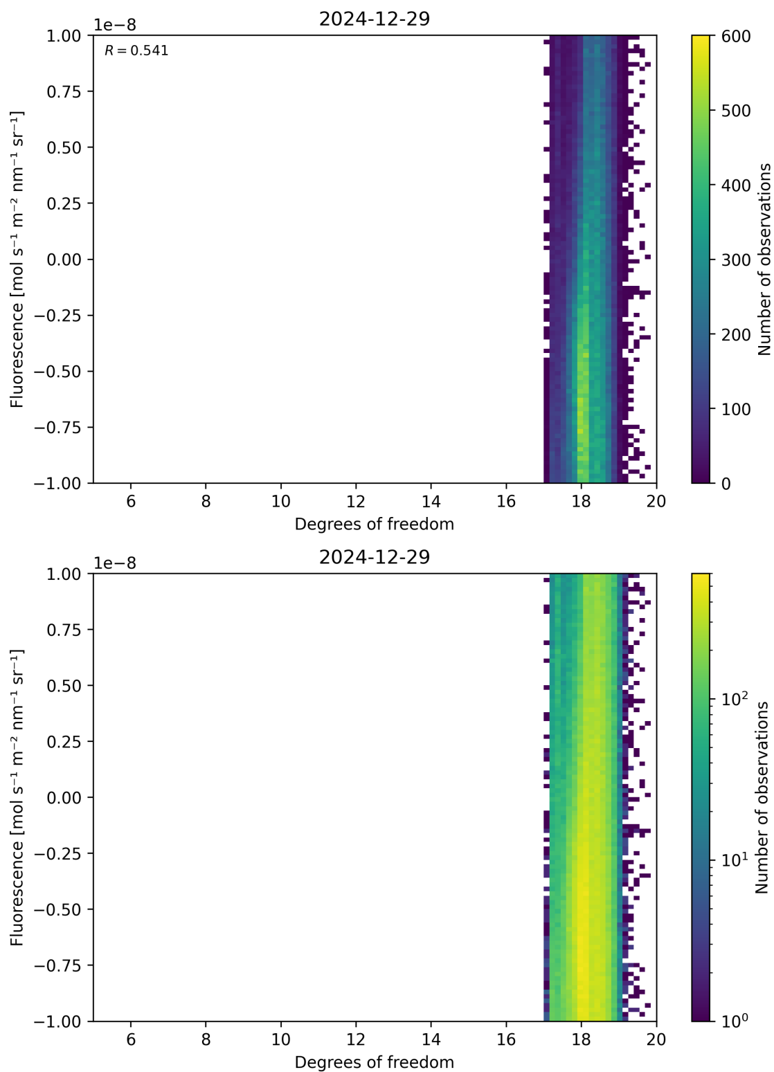
Figure 51: Scatter density plot of “Degrees of freedom” against “Fluorescence” for 2024-12-28 to 2024-12-30.
