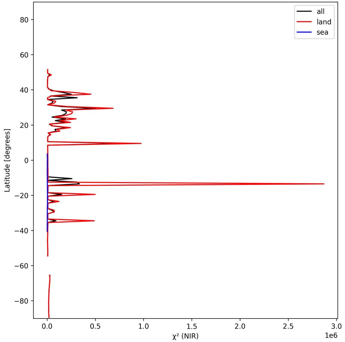
Figure 18: Zonal average of “ \chi^2 (NIR)” for 2024-12-28 to 2024-12-30.
