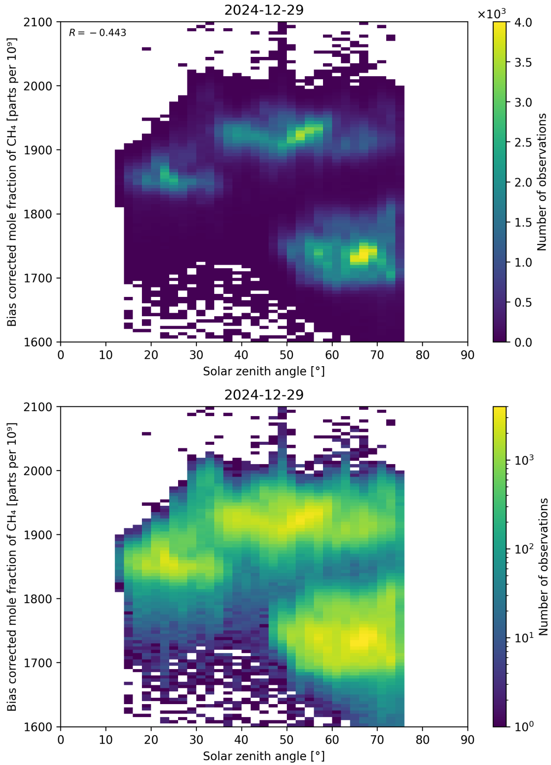
Figure 100: Scatter density plot of “Solar zenith angle” against “Bias corrected mole fraction of CH 4 ” for 2024-12-28 to 2024-12-30.
