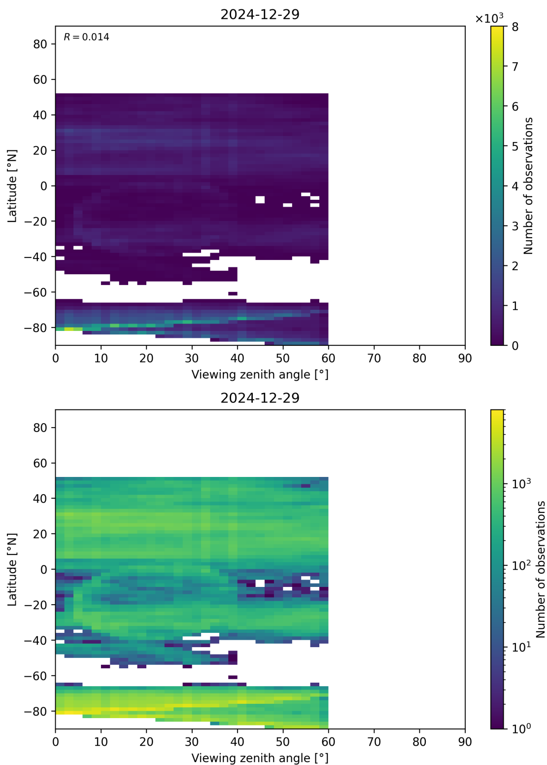
Figure 109: Scatter density plot of “Viewing zenith angle” against “Latitude” for 2024-12-28 to 2024-12-30.
