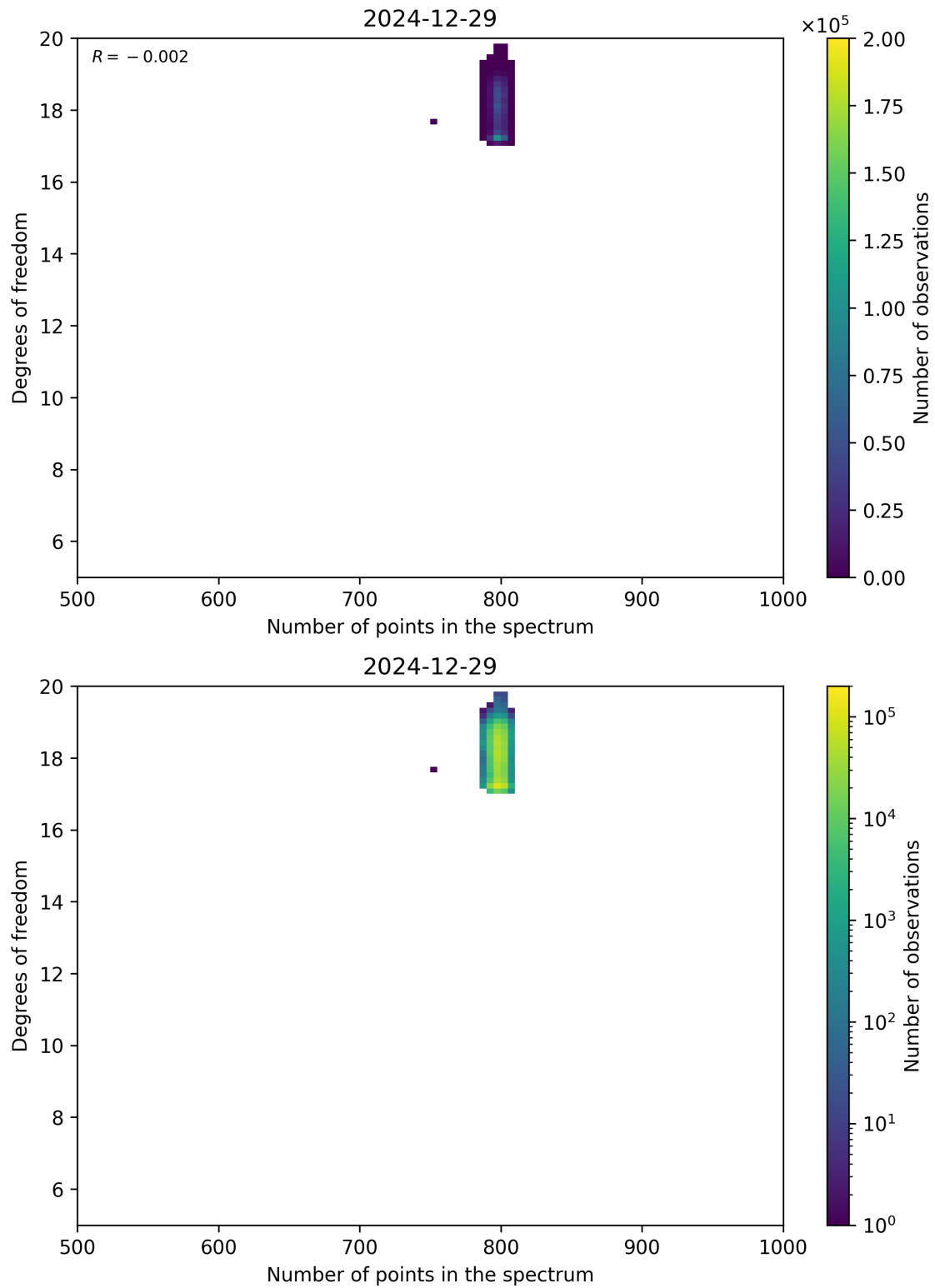
Figure 90: Scatter density plot of “Number of points in the spectrum” against “Degrees of freedom” for 2024-12-28 to 2024-12-30.
