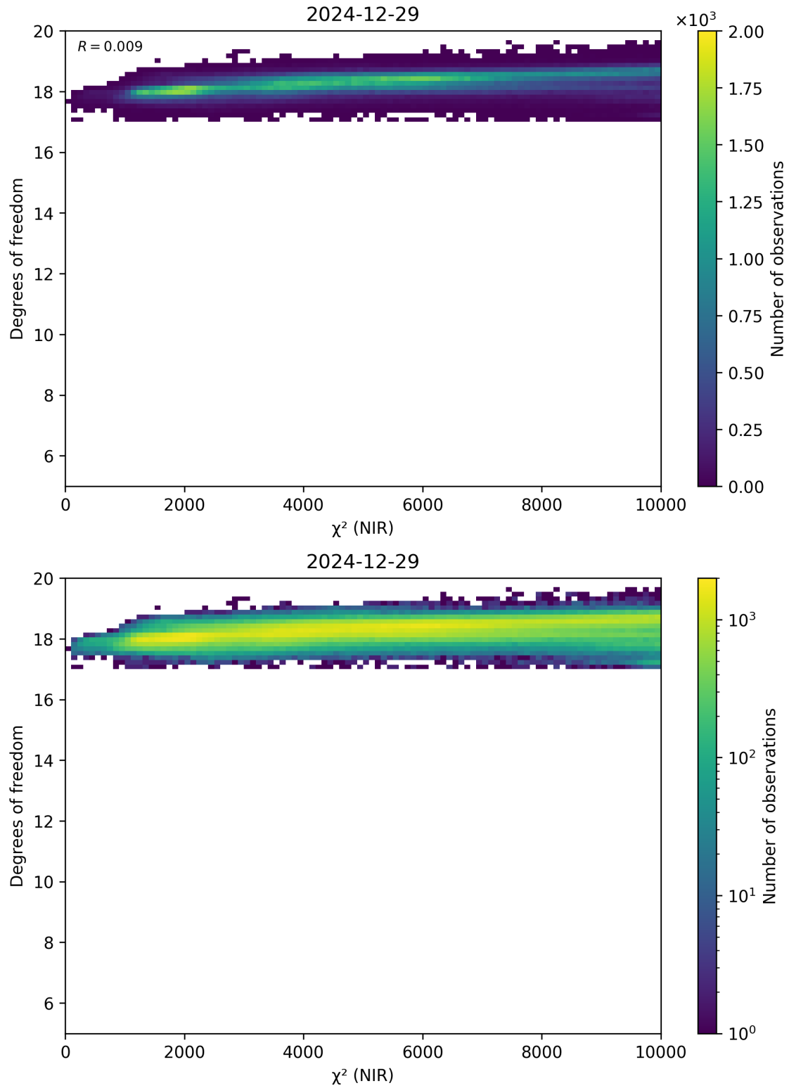
Figure 44: Scatter density plot of “ \chi^2 (NIR)” against “Degrees of freedom” for 2024-12-28 to 2024-12-30.
