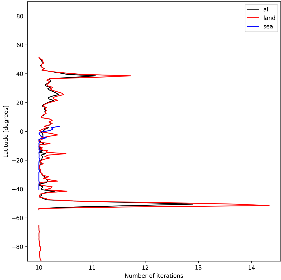
Figure 20: Zonal average of “Number of iterations” for 2024-12-28 to 2024-12-30.
