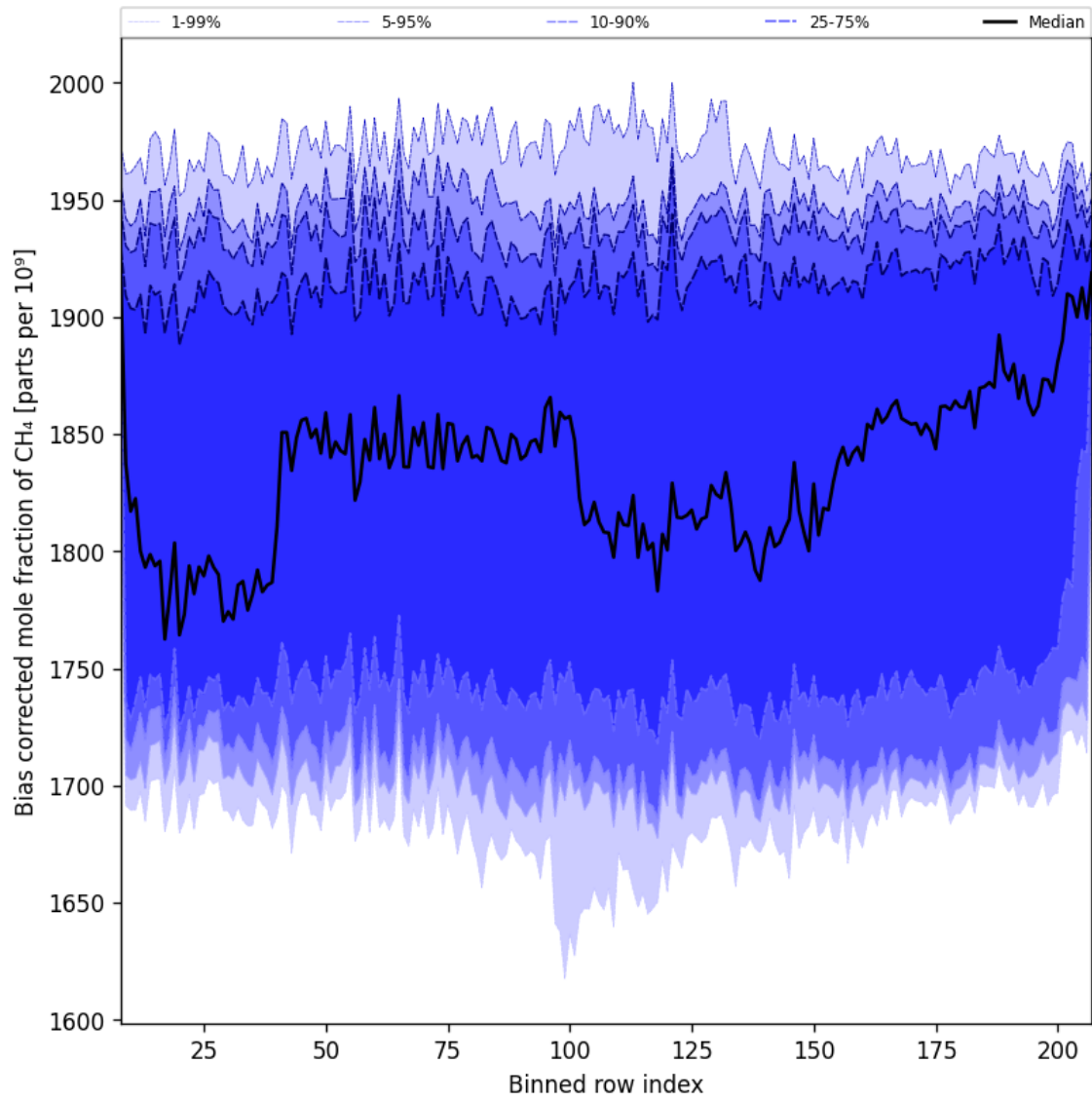
Figure 36: Along track statistics of “Bias corrected mole fraction of CH 4 ” for 2024-12-28 to 2024-12-30
