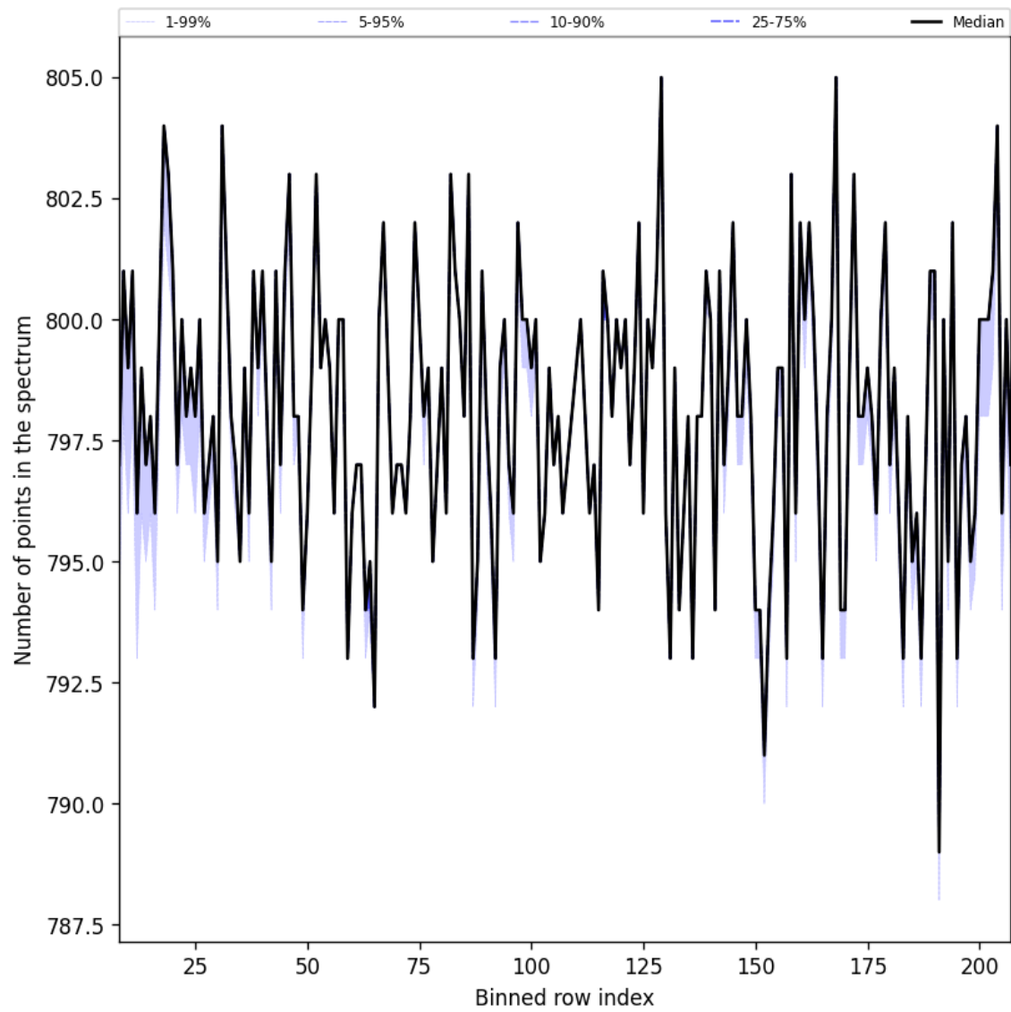
Figure 37: Along track statistics of “Number of points in the spectrum” for 2024-12-28 to 2024-12-30
