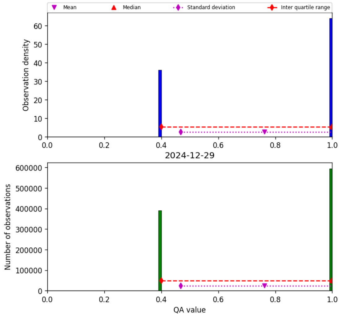
Figure 22: Histogram of “QA value” for 2024-12-28 to 2024-12-30
