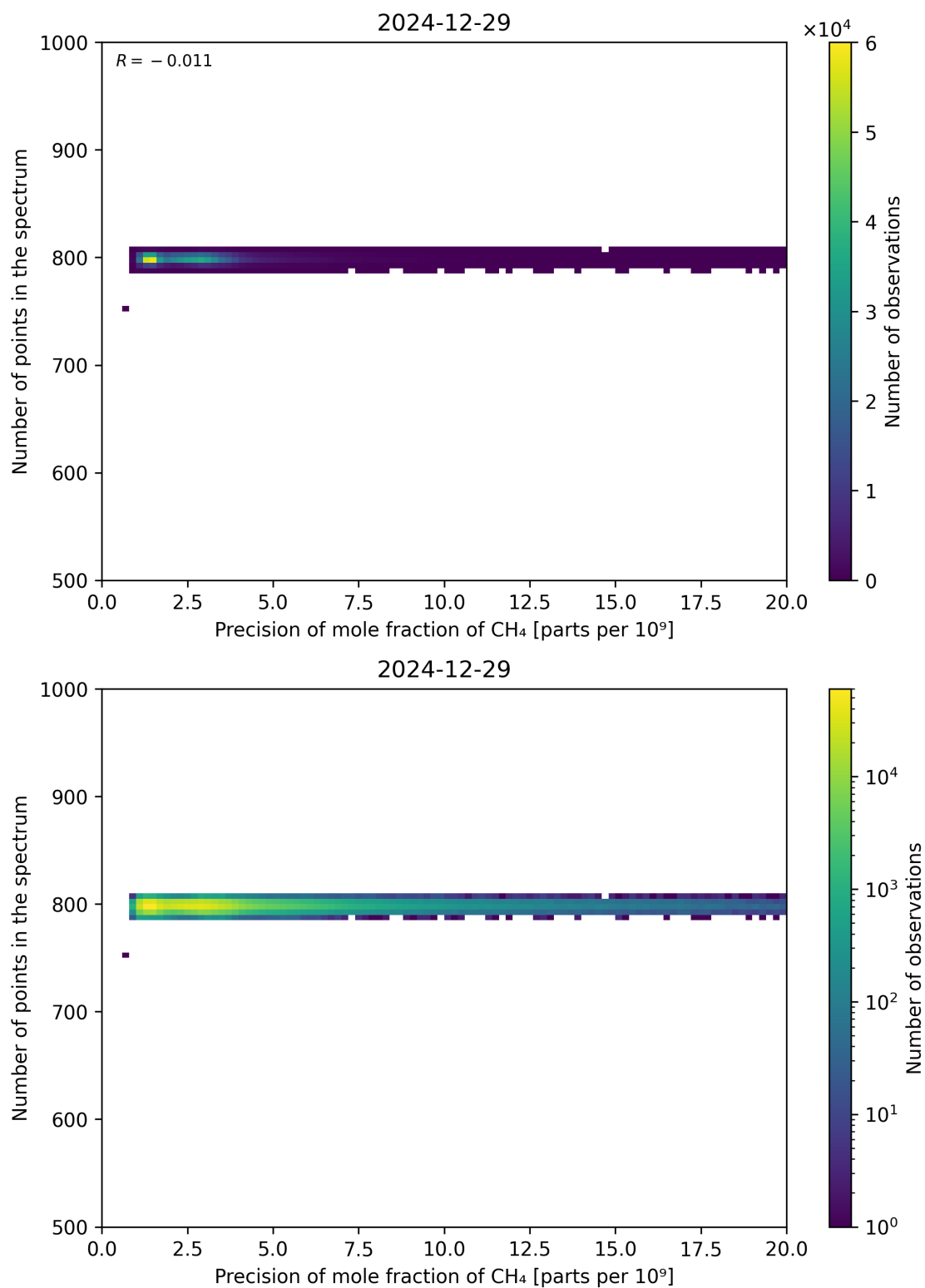
Figure 84: Scatter density plot of “Precision of mole fraction of CH 4 ” against “Number of points in the spectrum” for 2024-12-28 to 2024-12-30.
