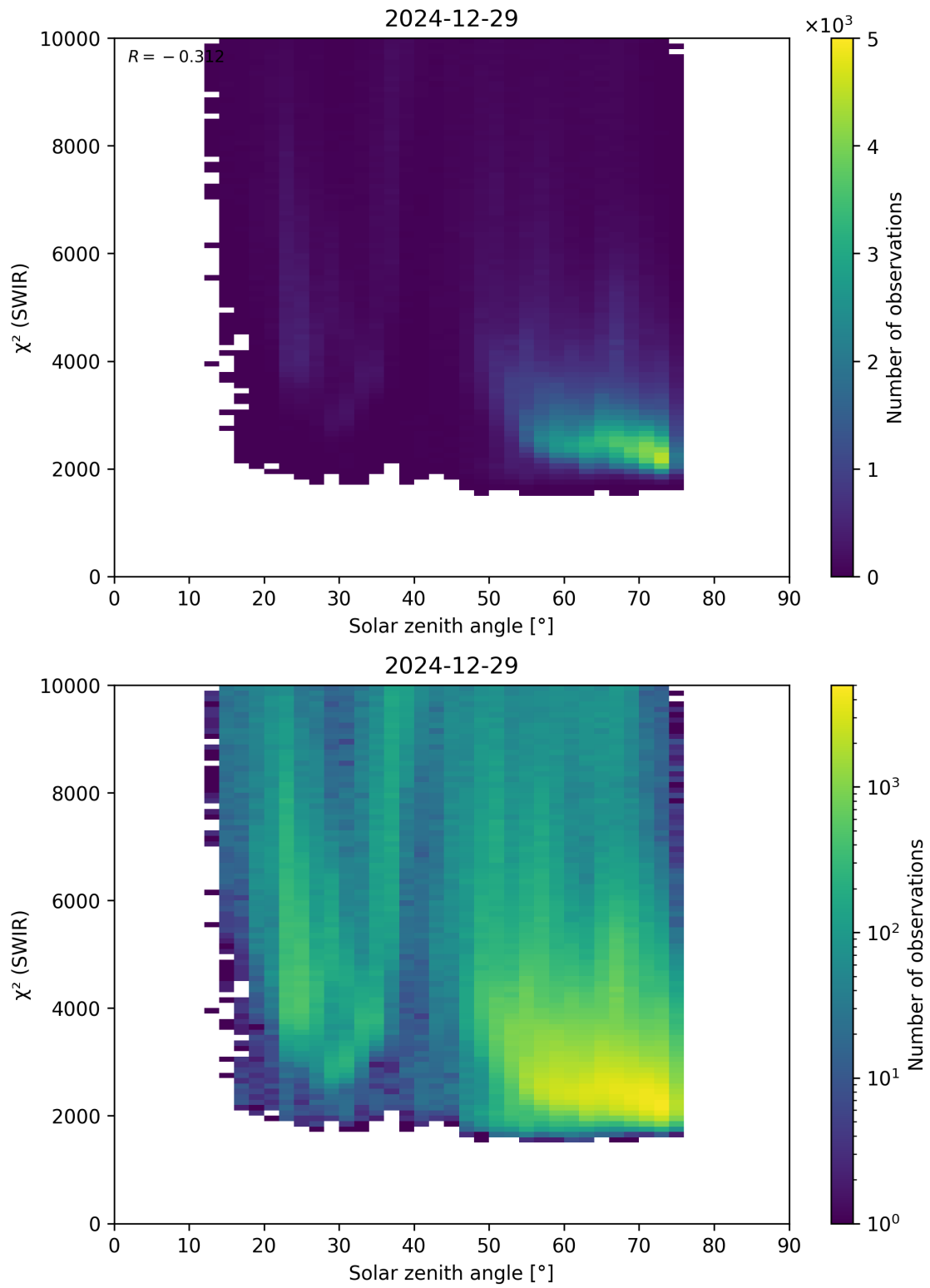
Figure 95: Scatter density plot of “Solar zenith angle” against “ \chi^2 (SWIR)” for 2024-12-28 to 2024-12-30.
