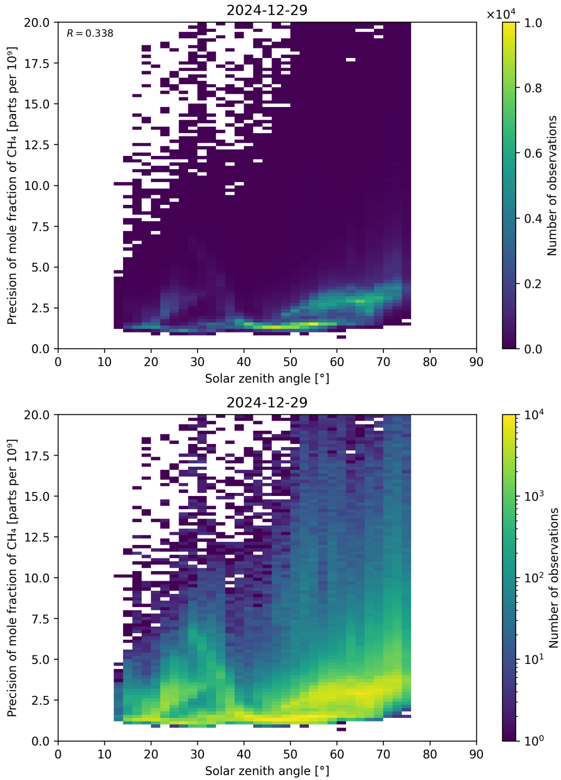
Figure 101: Scatter density plot of “Solar zenith angle” against “Precision of mole fraction of \text{CH}_4 ” for 2024-12-28 to 2024-12-30.
