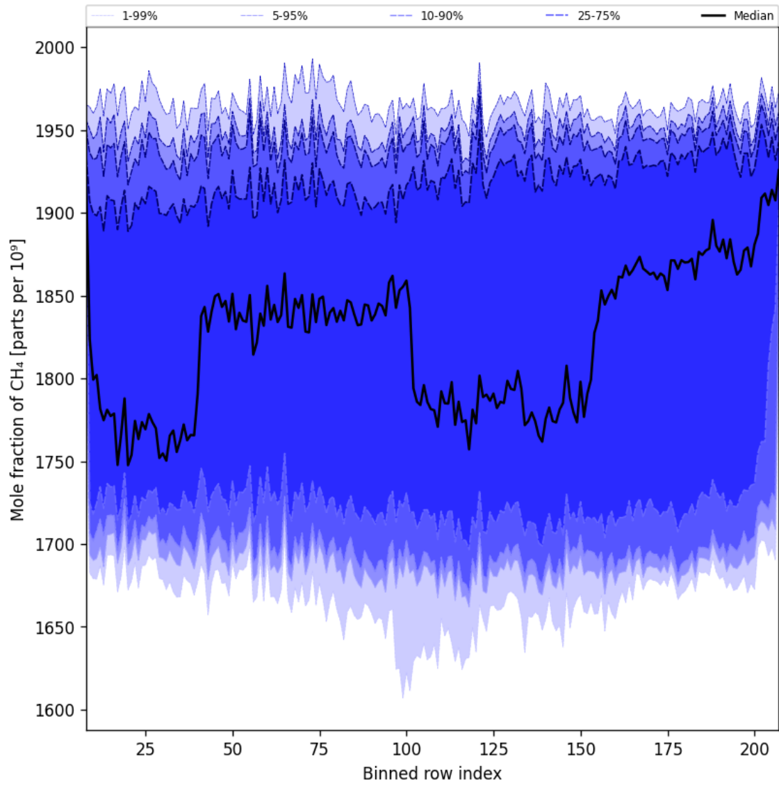
Figure 34: Along track statistics of “Mole fraction of CH 4 ” for 2024-12-28 to 2024-12-30
