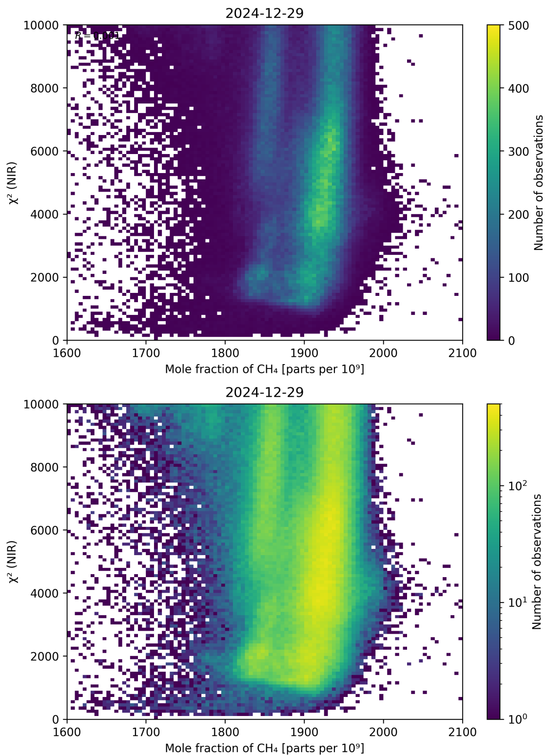
Figure 70: Scatter density plot of “Mole fraction of \text{CH}_4 ” against “ \chi^2 (NIR)” for 2024-12-28 to 2024-12-30.
