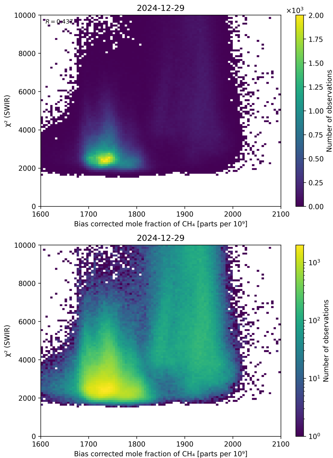
Figure 64: Scatter density plot of “Bias corrected mole fraction of \text{CH}_4 ” against “ \chi^2 (SWIR)” for 2024-12-28 to 2024-12-30.
