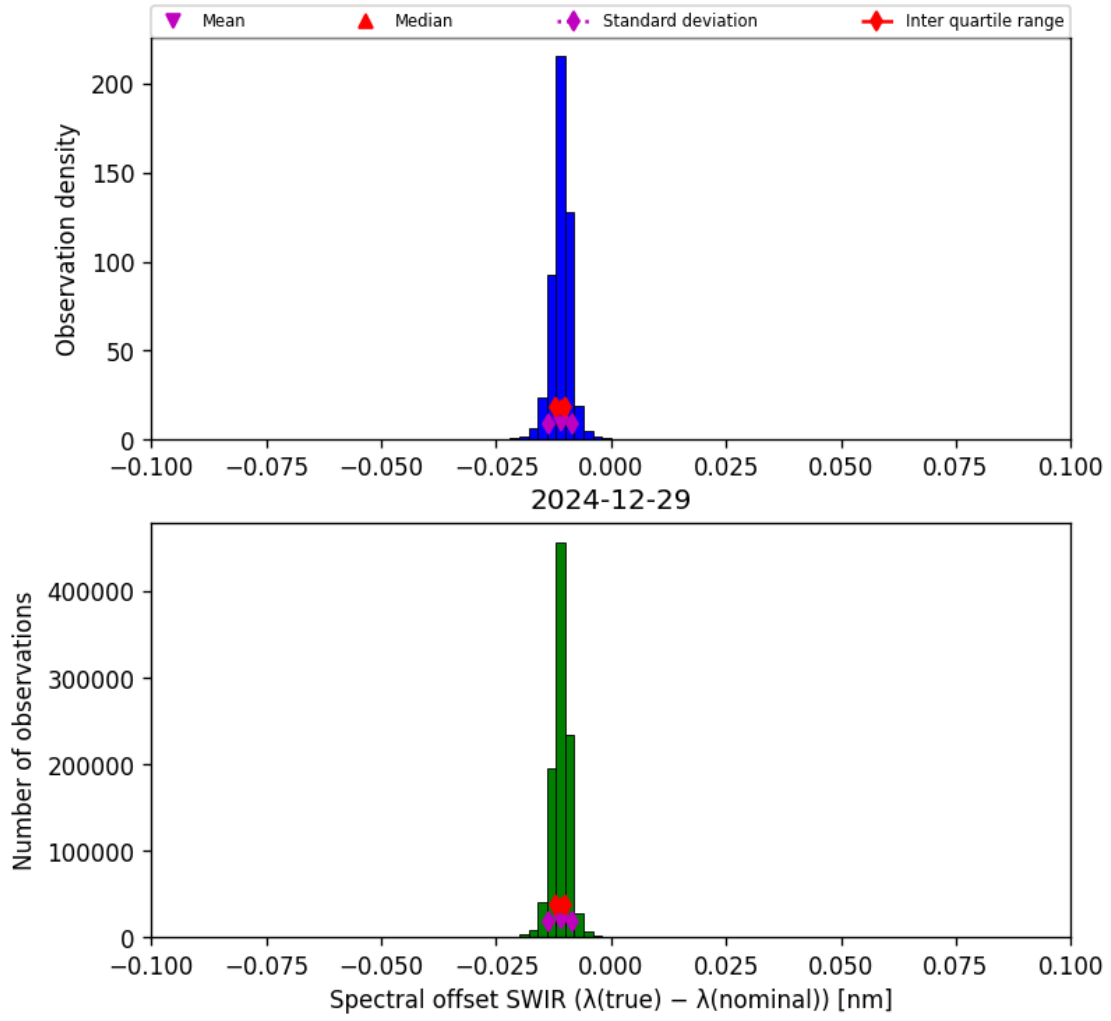
Figure 27: Histogram of “Spectral offset SWIR ( \lambda_{\text{true}} - \lambda_{\text{nominal}} )” for 2024-12-28 to 2024-12-30
