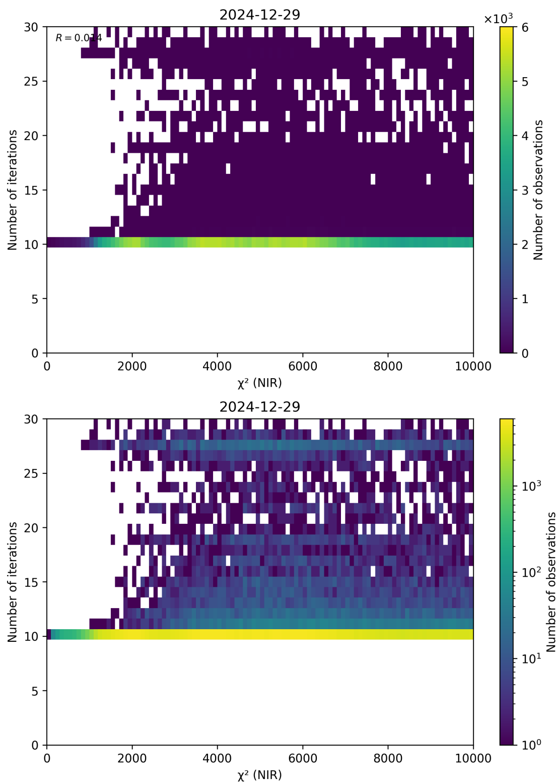
Figure 46: Scatter density plot of “ \chi^2 (NIR)” against “Number of iterations” for 2024-12-28 to 2024-12-30.
