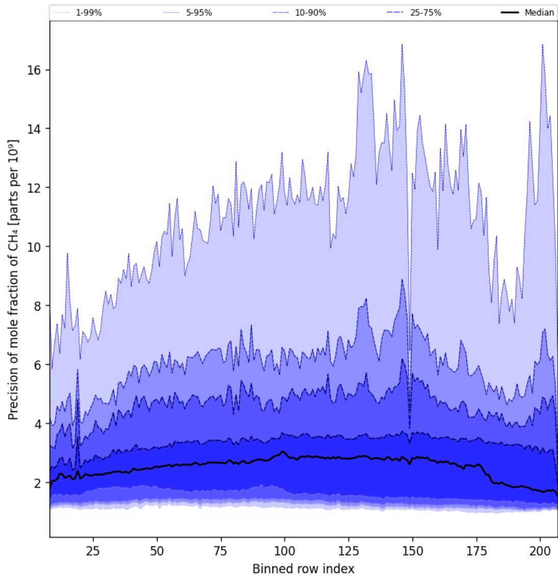
Figure 35: Along track statistics of “Precision of mole fraction of CH 4 ” for 2024-12-28 to 2024-12-30
