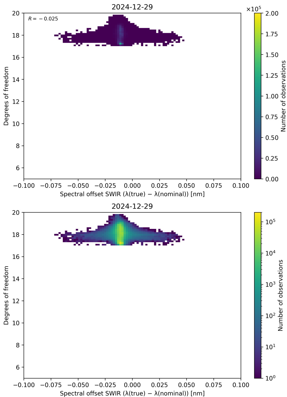
Figure 119: Scatter density plot of “Spectral offset SWIR ( \lambda_{\text{true}} - \lambda_{\text{nominal}} )” against “Degrees of freedom” for 2024-12-28 to 2024-12-30.
