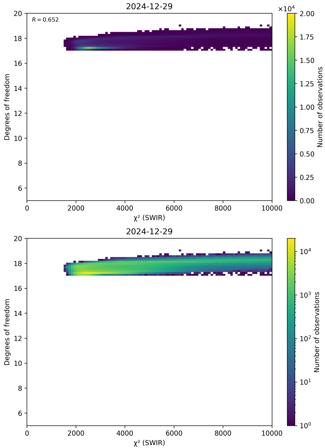
Figure 48: Scatter density plot of “ \chi^2 (SWIR)” against “Degrees of freedom” for 2024-12-28 to 2024-12-30.
