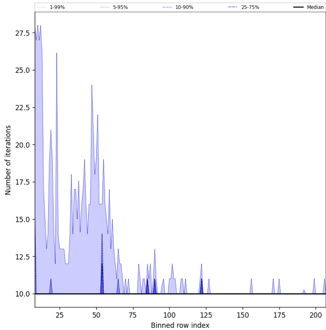
Figure 42: Along track statistics of “Number of iterations” for 2024-12-28 to 2024-12-30
