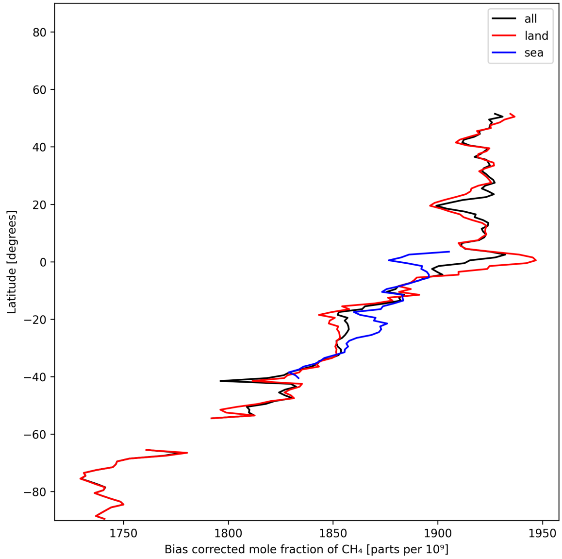
Figure 14: Zonal average of “Bias corrected mole fraction of CH 4 ” for 2024-12-28 to 2024-12-30.
