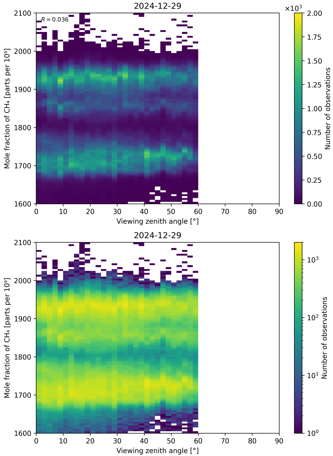
Figure 110: Scatter density plot of “Viewing zenith angle” against “Mole fraction of CH 4 ” for 2024-12-28 to 2024-12-30.
