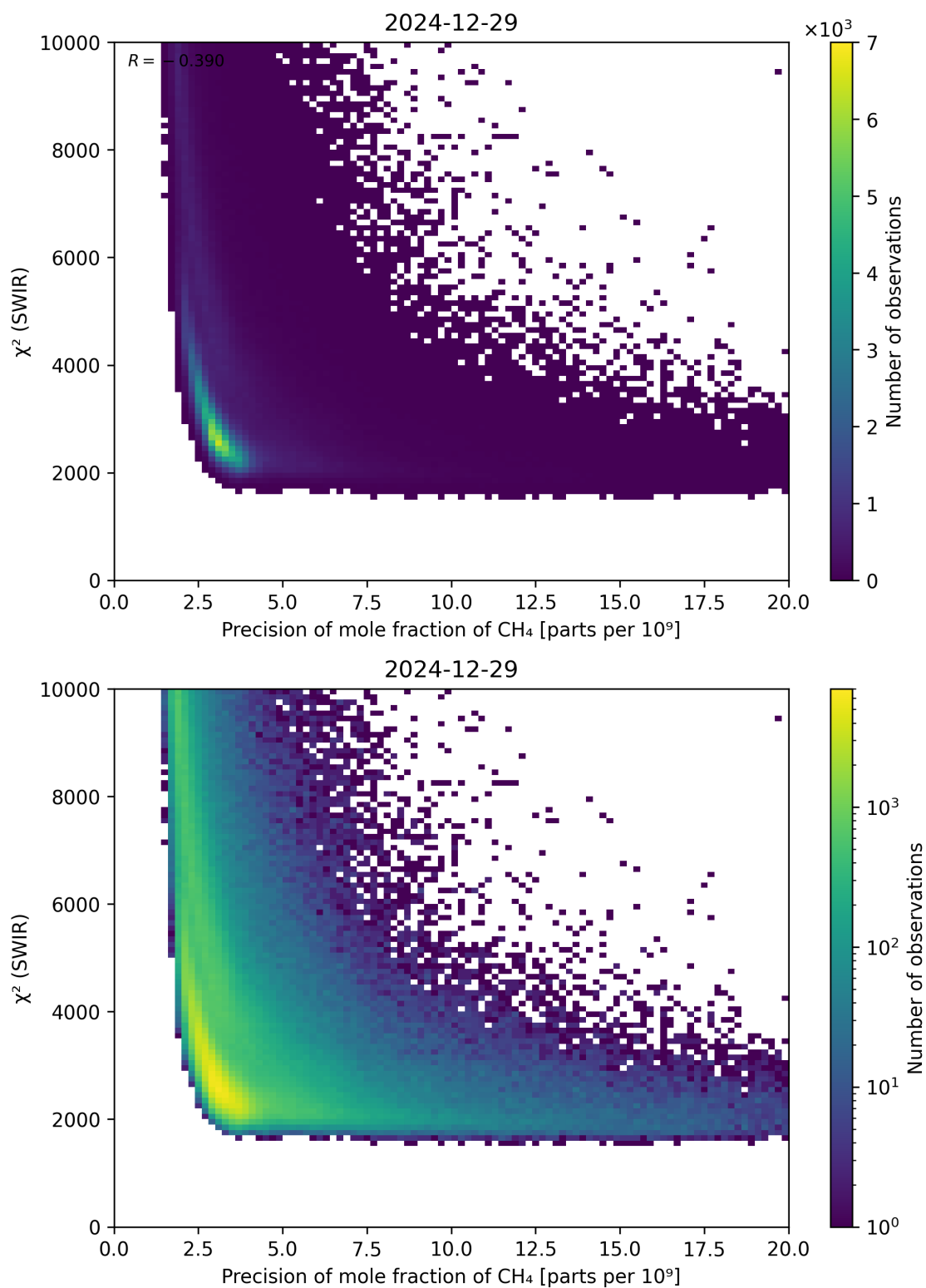
Figure 79: Scatter density plot of “Precision of mole fraction of \text{CH}_4 ” against “ \chi^2 (SWIR)” for 2024-12-28 to 2024-12-30.
