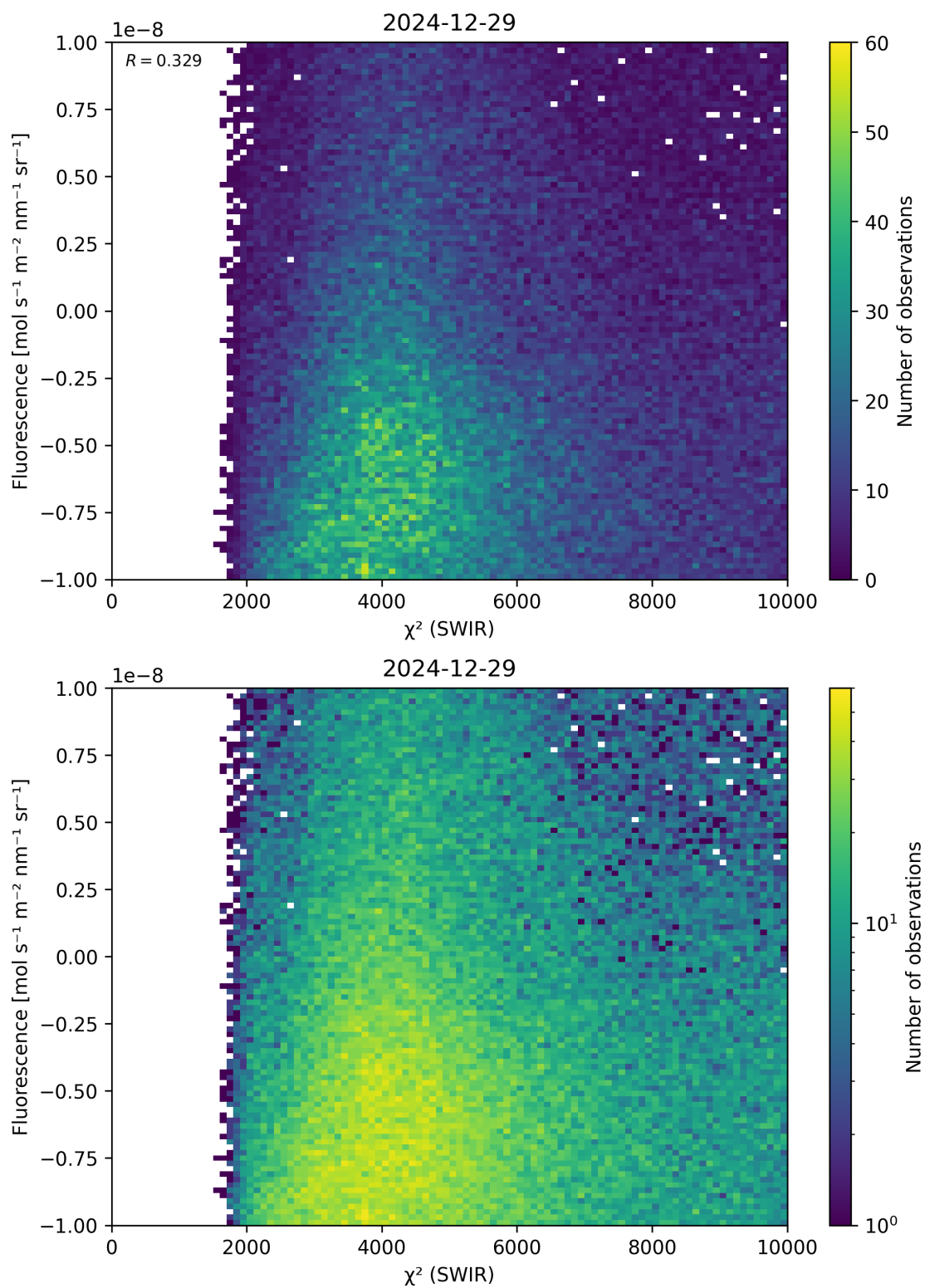
Figure 49: Scatter density plot of “ \chi^2 (SWIR)” against “Fluorescence” for 2024-12-28 to 2024-12-30.
