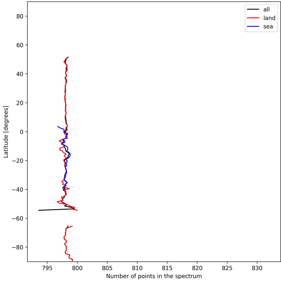
Figure 15: Zonal average of “Number of points in the spectrum” for 2024-12-28 to 2024-12-30.
