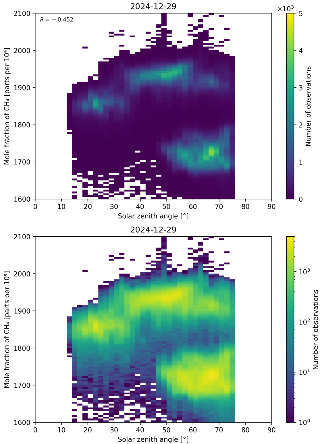
Figure 99: Scatter density plot of “Solar zenith angle” against “Mole fraction of \text{CH}_4 ” for 2024-12-28 to 2024-12-30.
