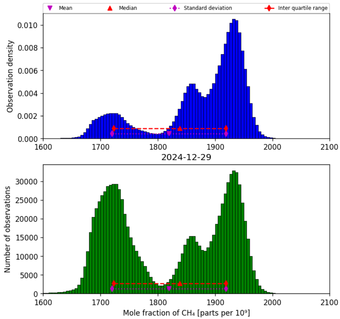
Figure 23: Histogram of “Mole fraction of CH 4 ” for 2024-12-28 to 2024-12-30
