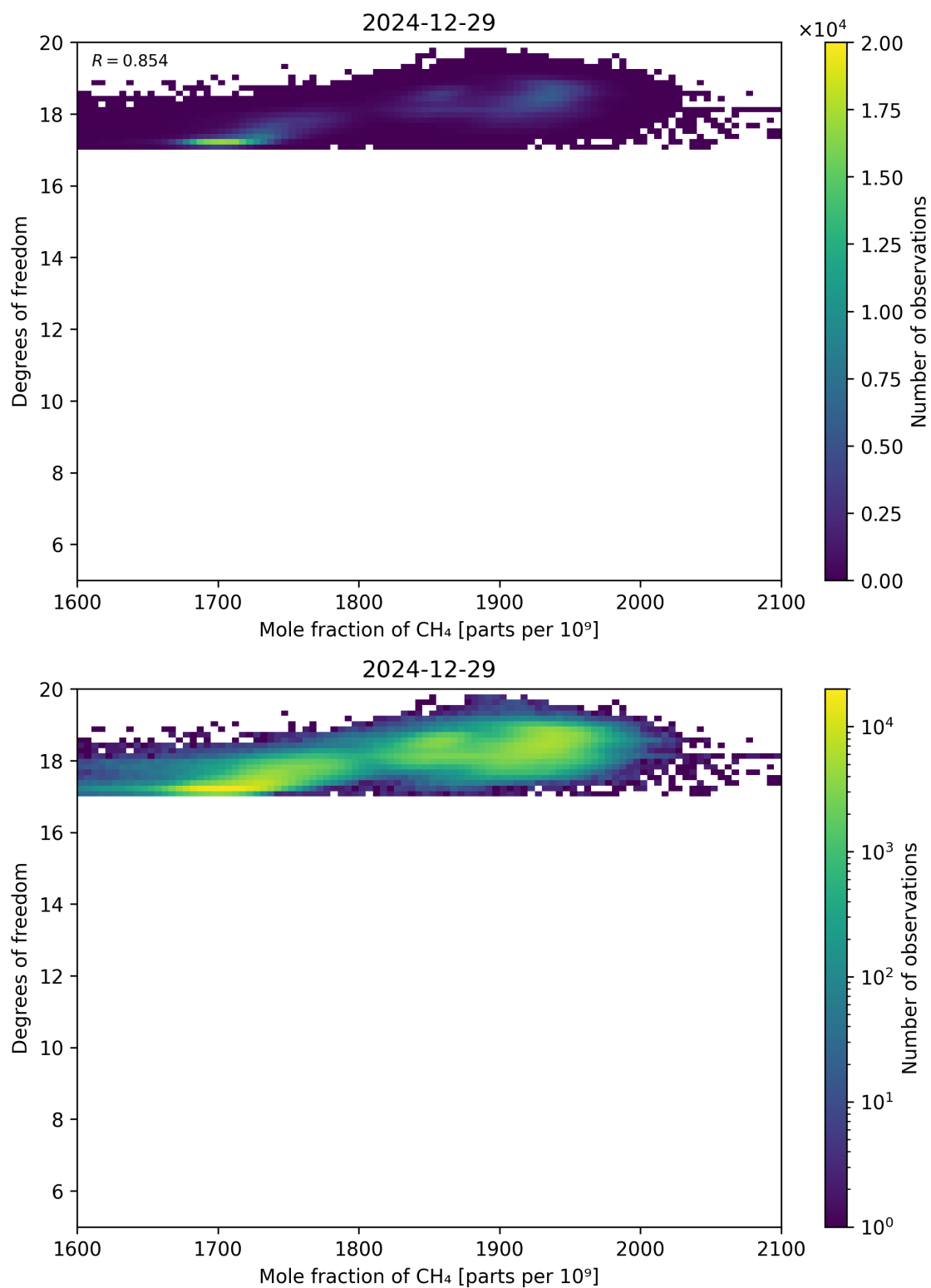
Figure 72: Scatter density plot of “Mole fraction of CH 4 ” against “Degrees of freedom” for 2024-12-28 to 2024-12-30.
