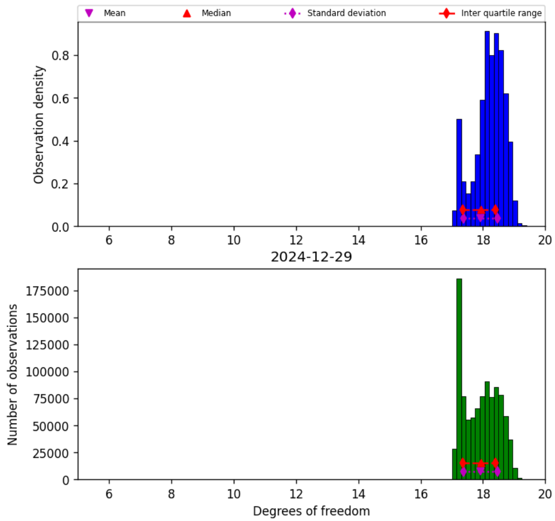
Figure 30: Histogram of “Degrees of freedom” for 2024-12-28 to 2024-12-30
