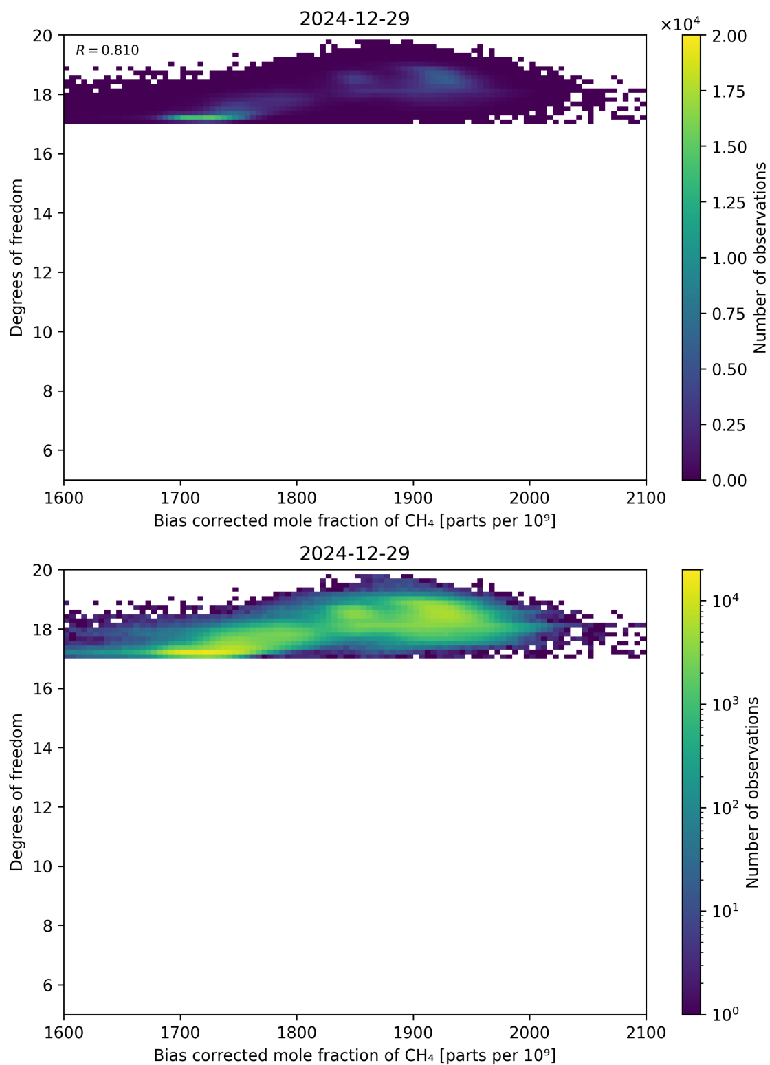
Figure 65: Scatter density plot of “Bias corrected mole fraction of CH 4 ” against “Degrees of freedom” for 2024-12-28 to 2024-12-30.
