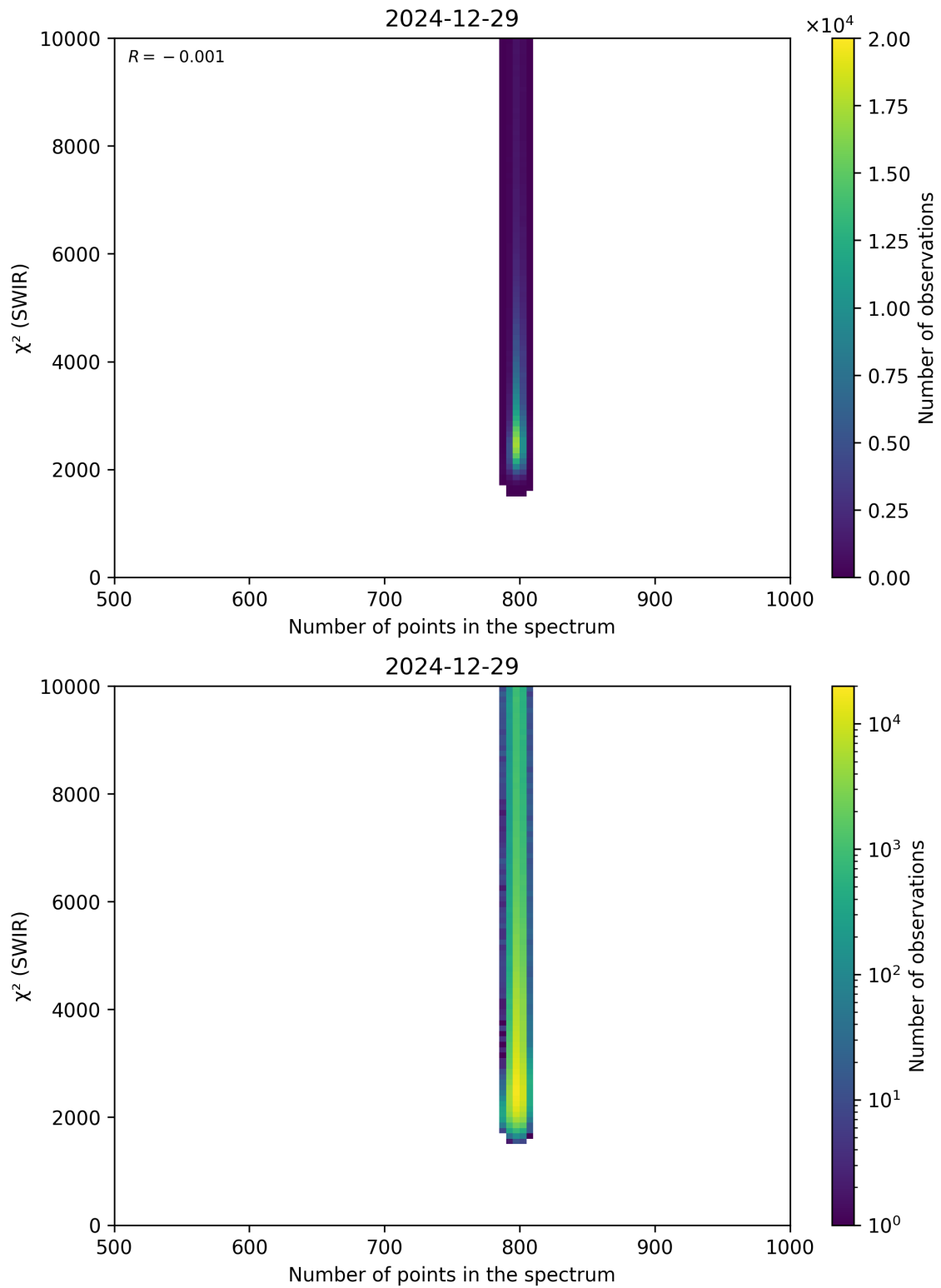
Figure 89: Scatter density plot of “Number of points in the spectrum” against “ \chi^2 (SWIR)” for 2024-12-28 to 2024-12-30.
