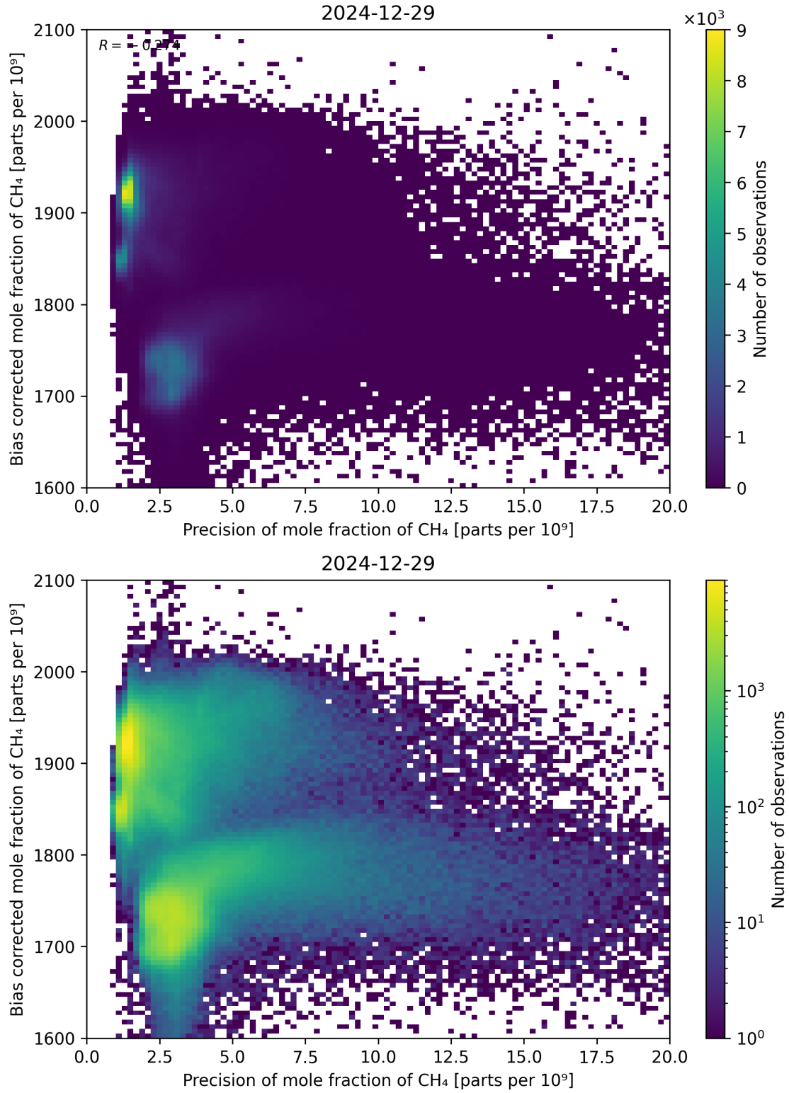
Figure 82: Scatter density plot of “Precision of mole fraction of CH 4 ” against “Bias corrected mole fraction of CH 4 ” for 2024-12-28 to 2024-12-30.
