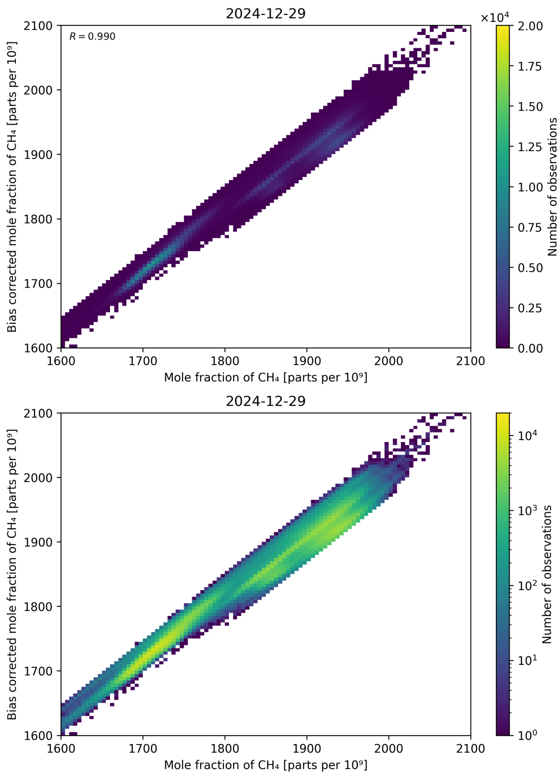
Figure 74: Scatter density plot of “Mole fraction of CH 4 ” against “Bias corrected mole fraction of CH 4 ” for 2024-12-28 to 2024-12-30.
