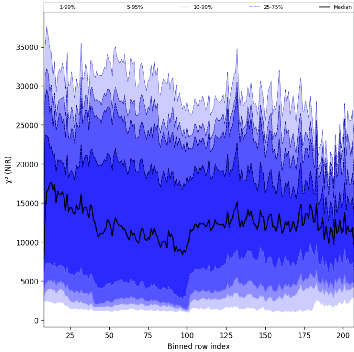
Figure 40: Along track statistics of “ \chi^2 (NIR)” for 2024-12-28 to 2024-12-30
