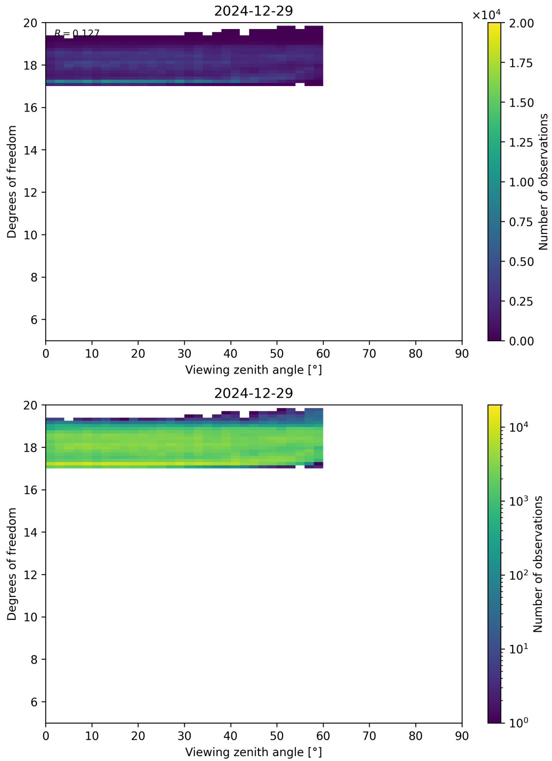
Figure 107: Scatter density plot of “Viewing zenith angle” against “Degrees of freedom” for 2024-12-28 to 2024-12-30.
