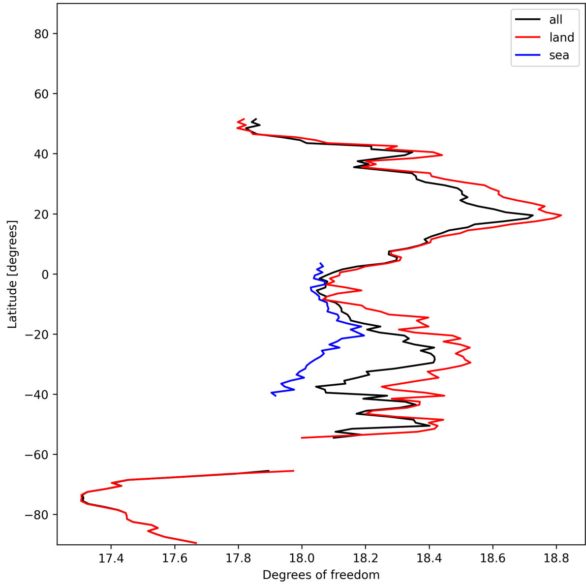
Figure 19: Zonal average of “Degrees of freedom” for 2024-12-28 to 2024-12-30.
