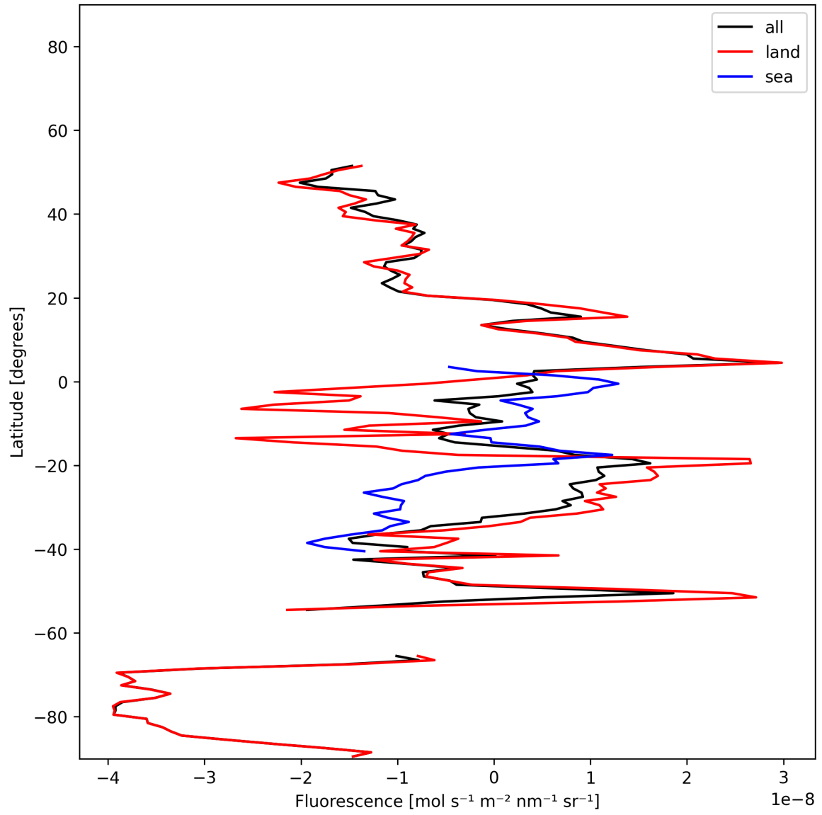
Figure 21: Zonal average of “Fluorescence” for 2024-12-28 to 2024-12-30.
