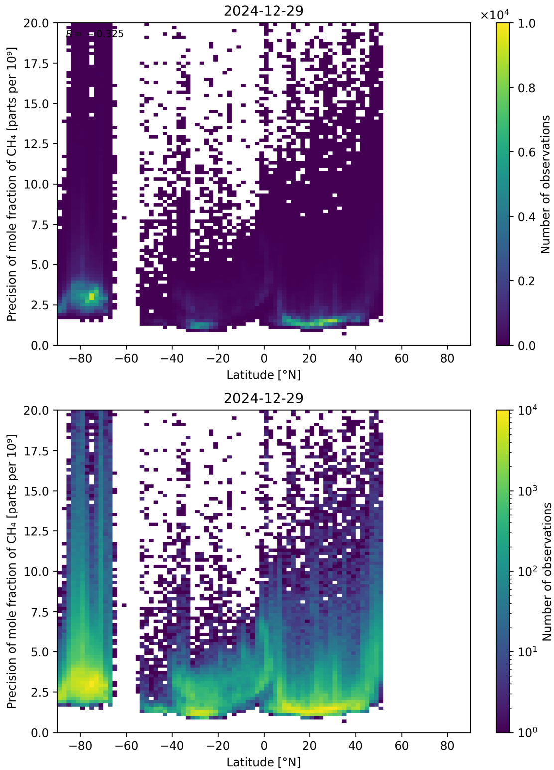
Figure 59: Scatter density plot of “Latitude” against “Precision of mole fraction of CH 4 ” for 2024-12-28 to 2024-12-30.
