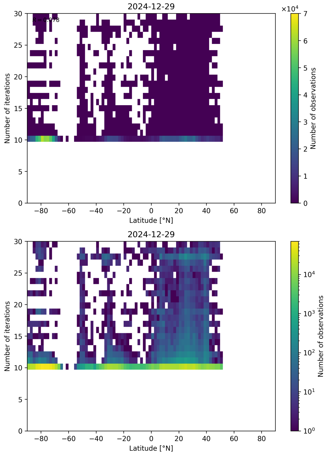
Figure 60: Scatter density plot of “Latitude” against “Number of iterations” for 2024-12-28 to 2024-12-30.
