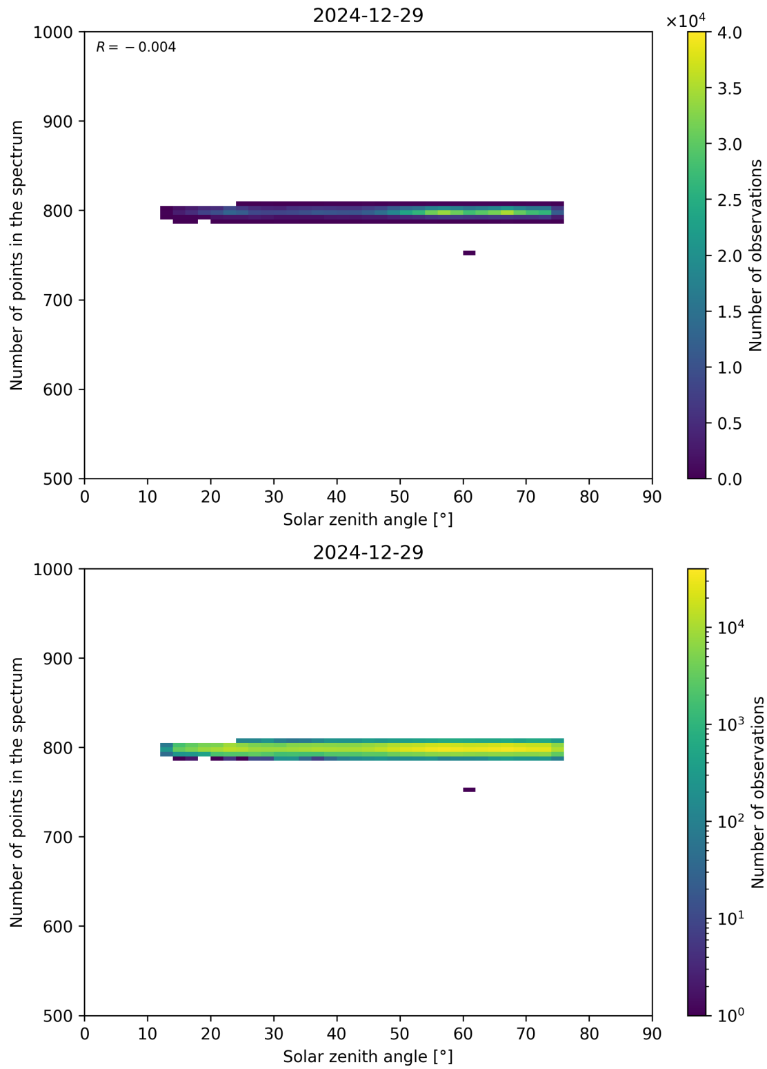
Figure 103: Scatter density plot of “Solar zenith angle” against “Number of points in the spectrum” for 2024-12-28 to 2024-12-30.
