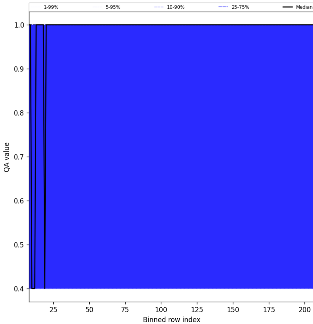
Figure 33: Along track statistics of “QA value” for 2024-12-28 to 2024-12-30
