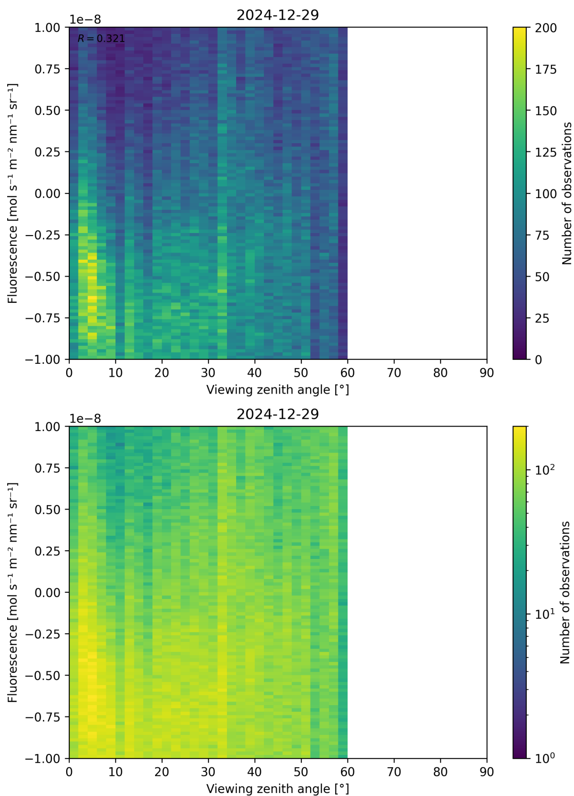
Figure 108: Scatter density plot of “Viewing zenith angle” against “Fluorescence” for 2024-12-28 to 2024-12-30.
