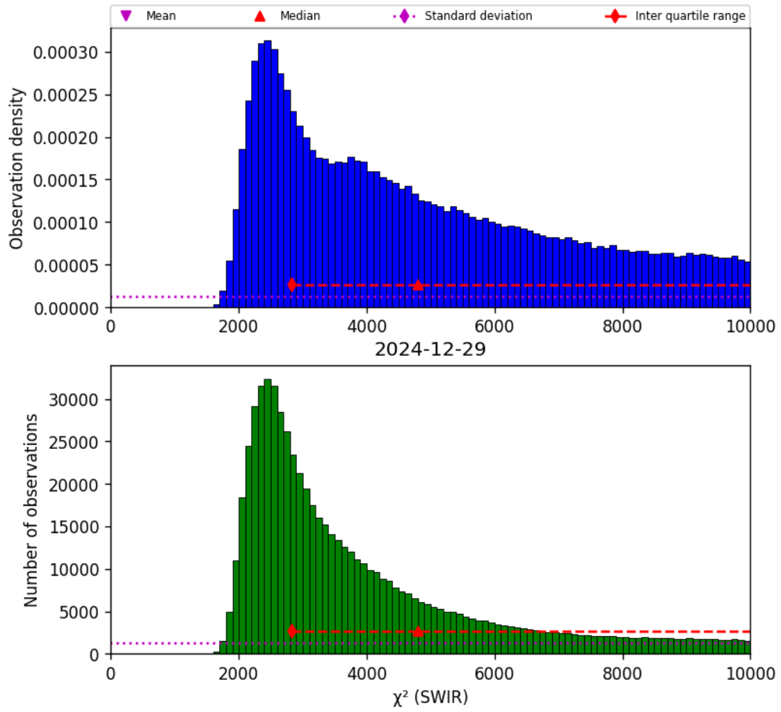
Figure 28: Histogram of “ \chi^2 (SWIR)” for 2024-12-28 to 2024-12-30
