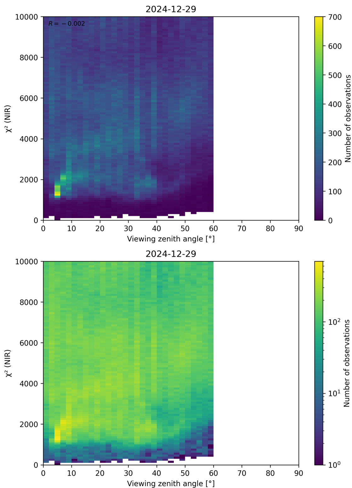
Figure 105: Scatter density plot of “Viewing zenith angle” against “ \chi^2 (NIR)” for 2024-12-28 to 2024-12-30.
