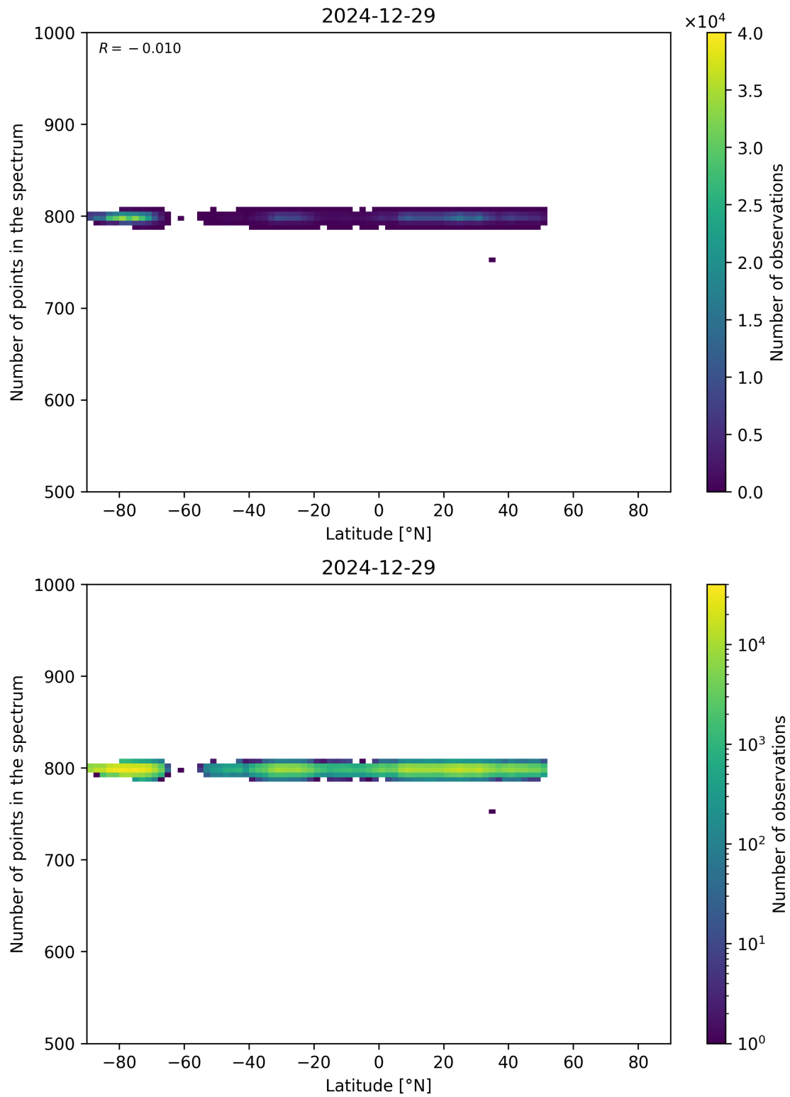
Figure 61: Scatter density plot of “Latitude” against “Number of points in the spectrum” for 2024-12-28 to 2024-12-30.
