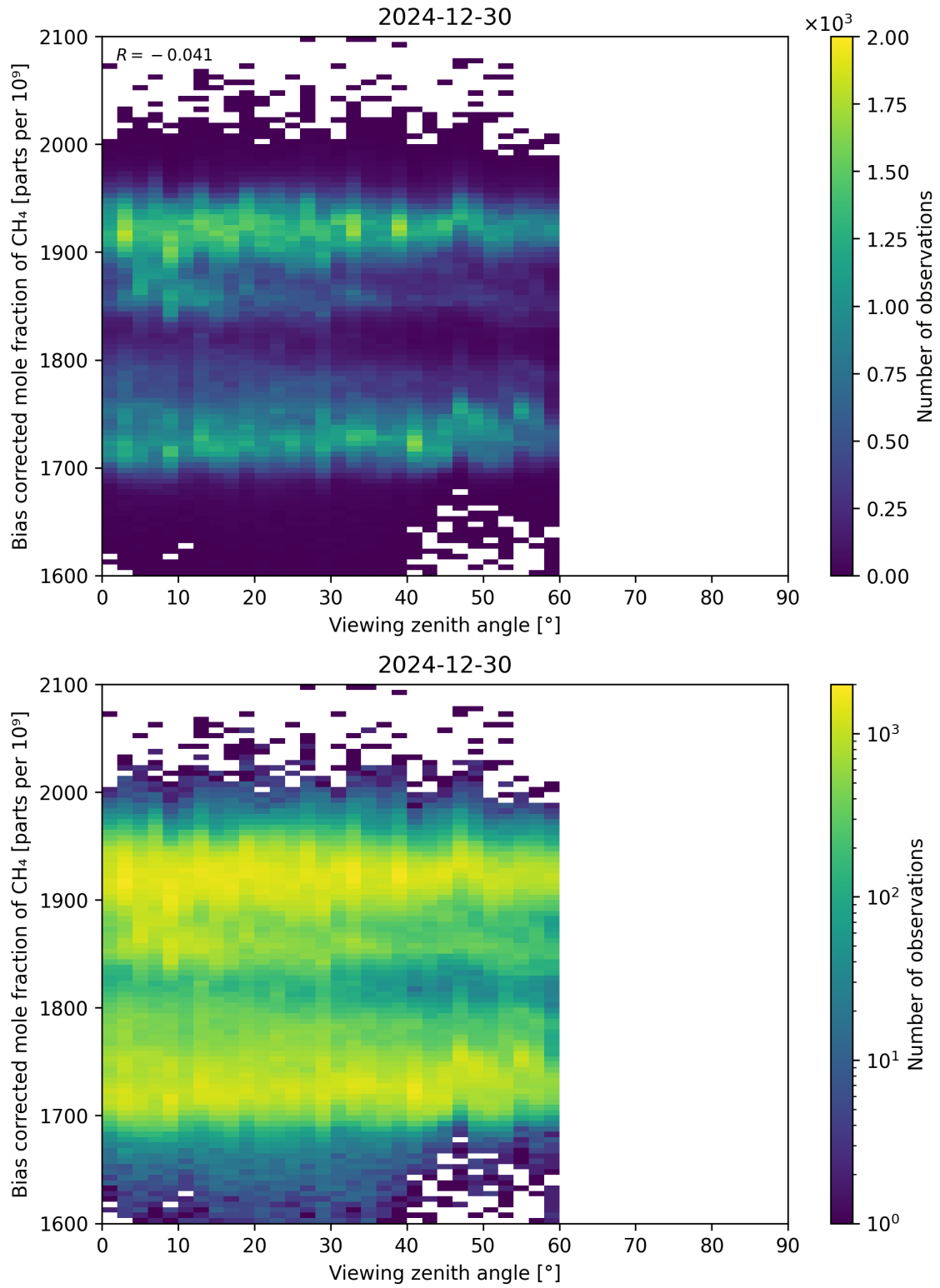
Figure 111: Scatter density plot of “Viewing zenith angle” against “Bias corrected mole fraction of CH 4 ” for 2024-12-29 to 2024-12-31.
