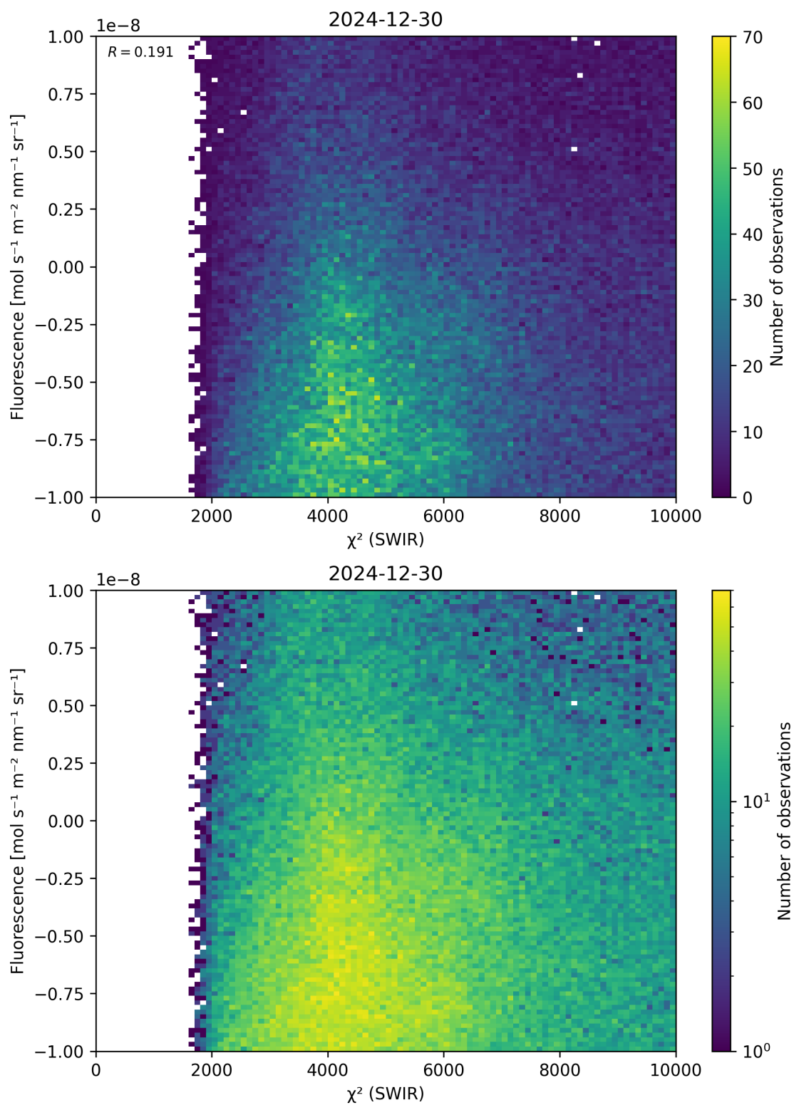
Figure 49: Scatter density plot of “ \chi^2 (SWIR)” against “Fluorescence” for 2024-12-29 to 2024-12-31.
