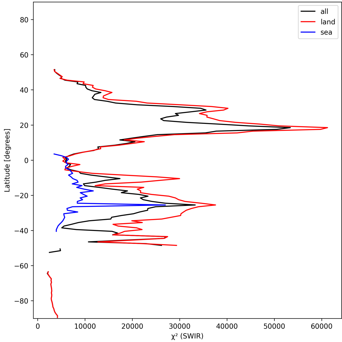
Figure 17: Zonal average of “ \chi^2 (SWIR)” for 2024-12-29 to 2024-12-31.
