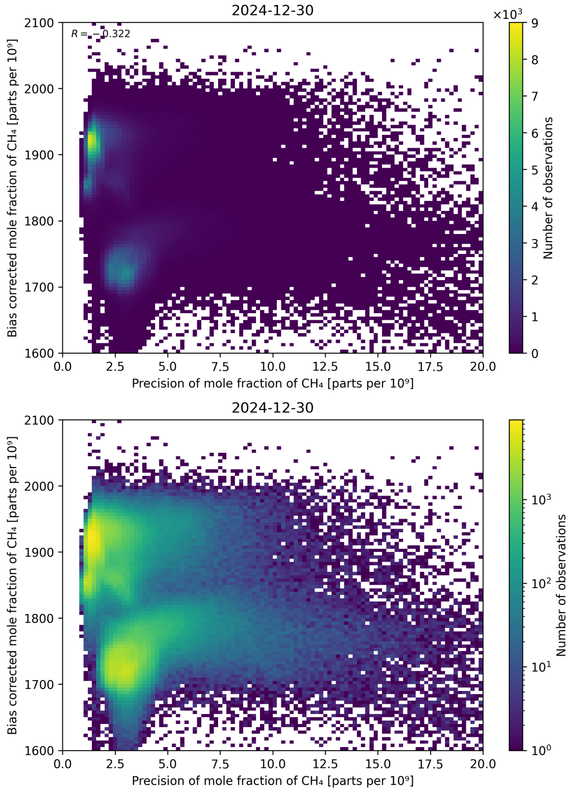
Figure 82: Scatter density plot of “Precision of mole fraction of CH 4 ” against “Bias corrected mole fraction of CH 4 ” for 2024-12-29 to 2024-12-31.
