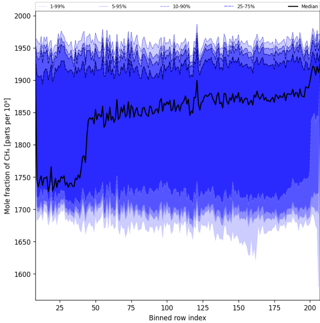
Figure 34: Along track statistics of “Mole fraction of CH 4 ” for 2024-12-29 to 2024-12-31
