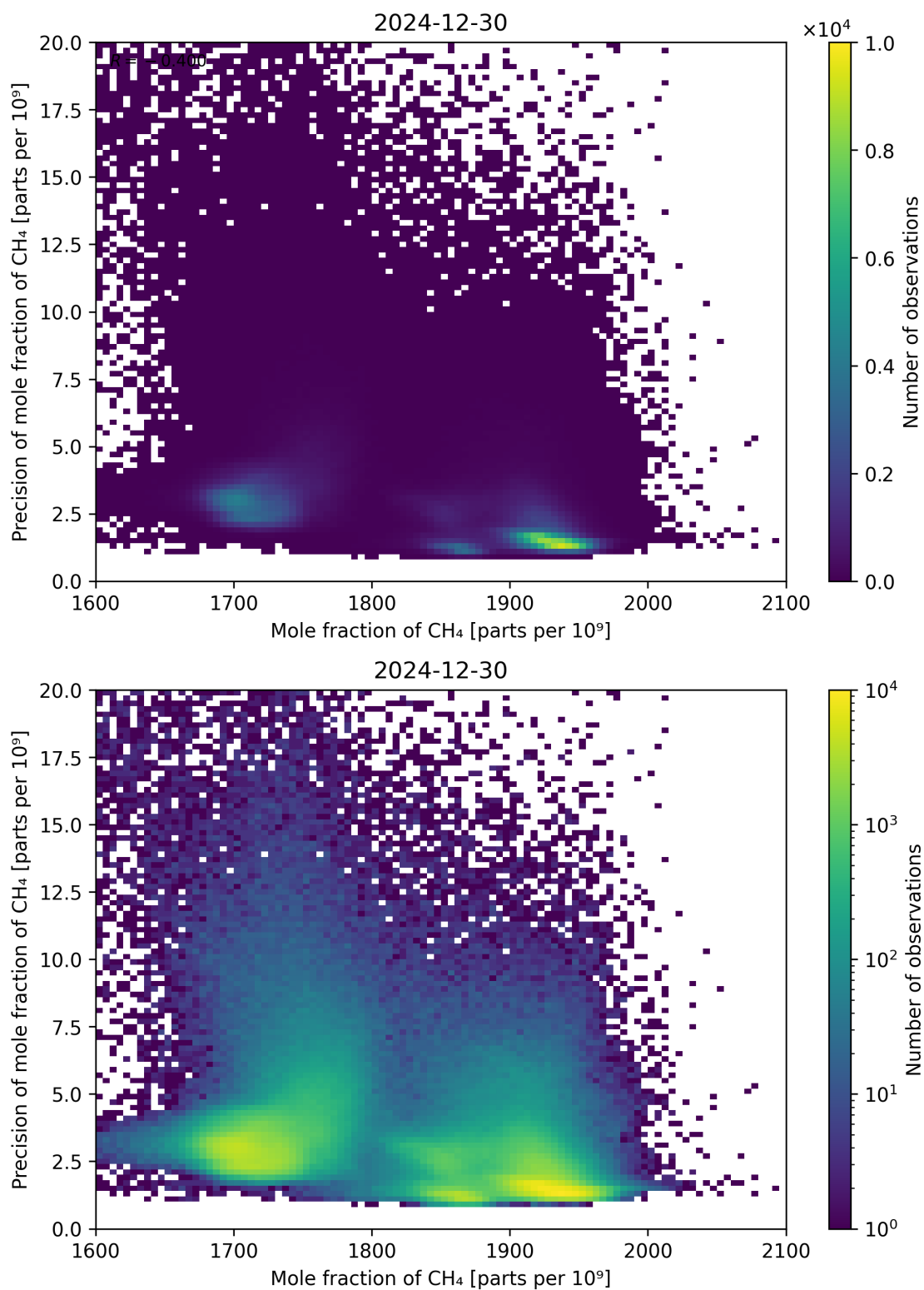
Figure 75: Scatter density plot of “Mole fraction of CH 4 ” against “Precision of mole fraction of CH 4 ” for 2024-12-29 to 2024-12-31.
