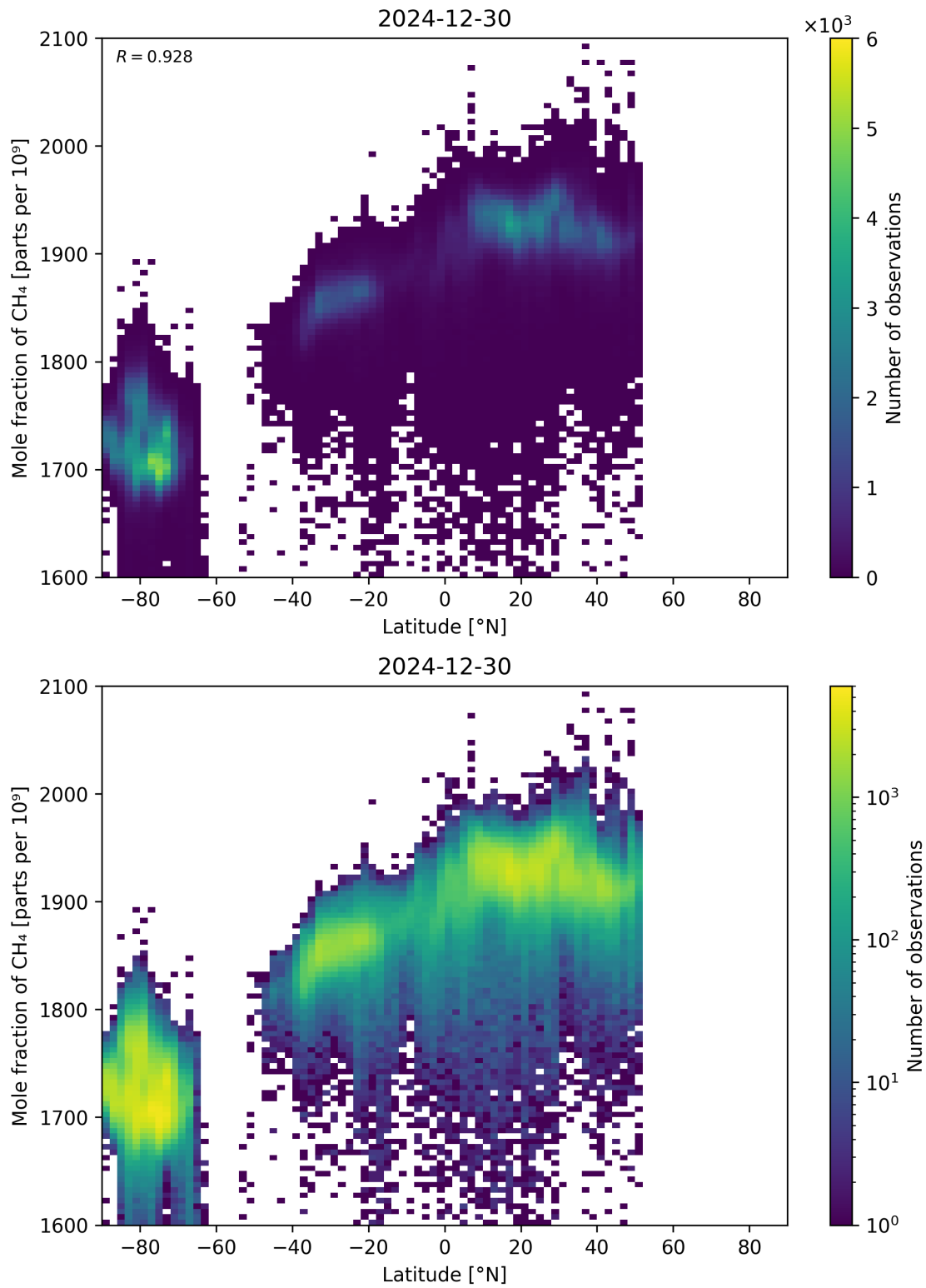
Figure 57: Scatter density plot of “Latitude” against “Mole fraction of CH 4 ” for 2024-12-29 to 2024-12-31.
