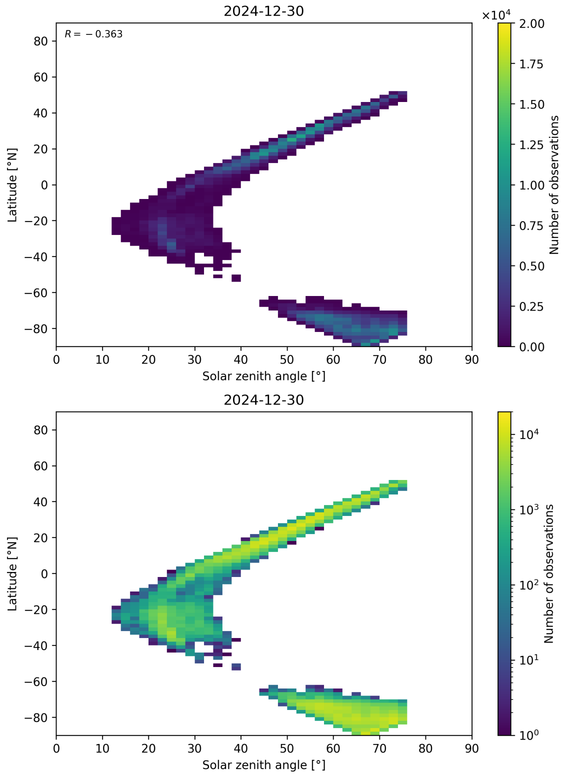
Figure 98: Scatter density plot of “Solar zenith angle” against “Latitude” for 2024-12-29 to 2024-12-31.
