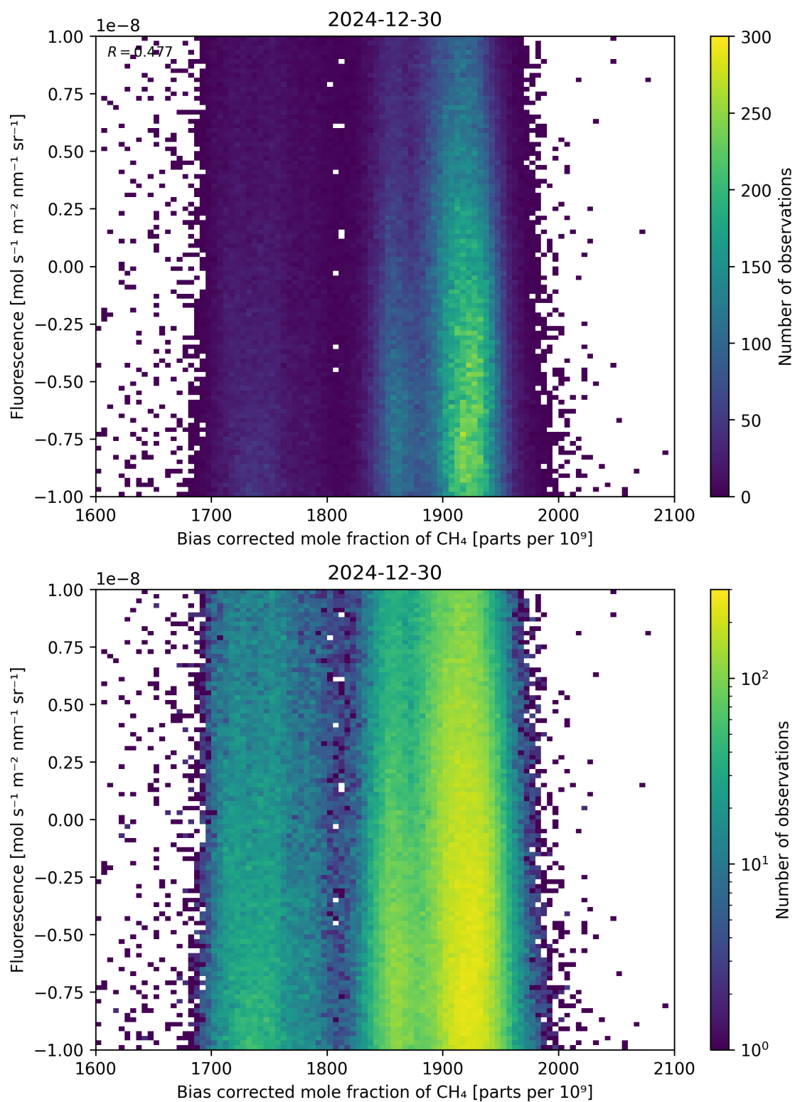
Figure 66: Scatter density plot of “Bias corrected mole fraction of \text{CH}_4 ” against “Fluorescence” for 2024-12-29 to 2024-12-31.
