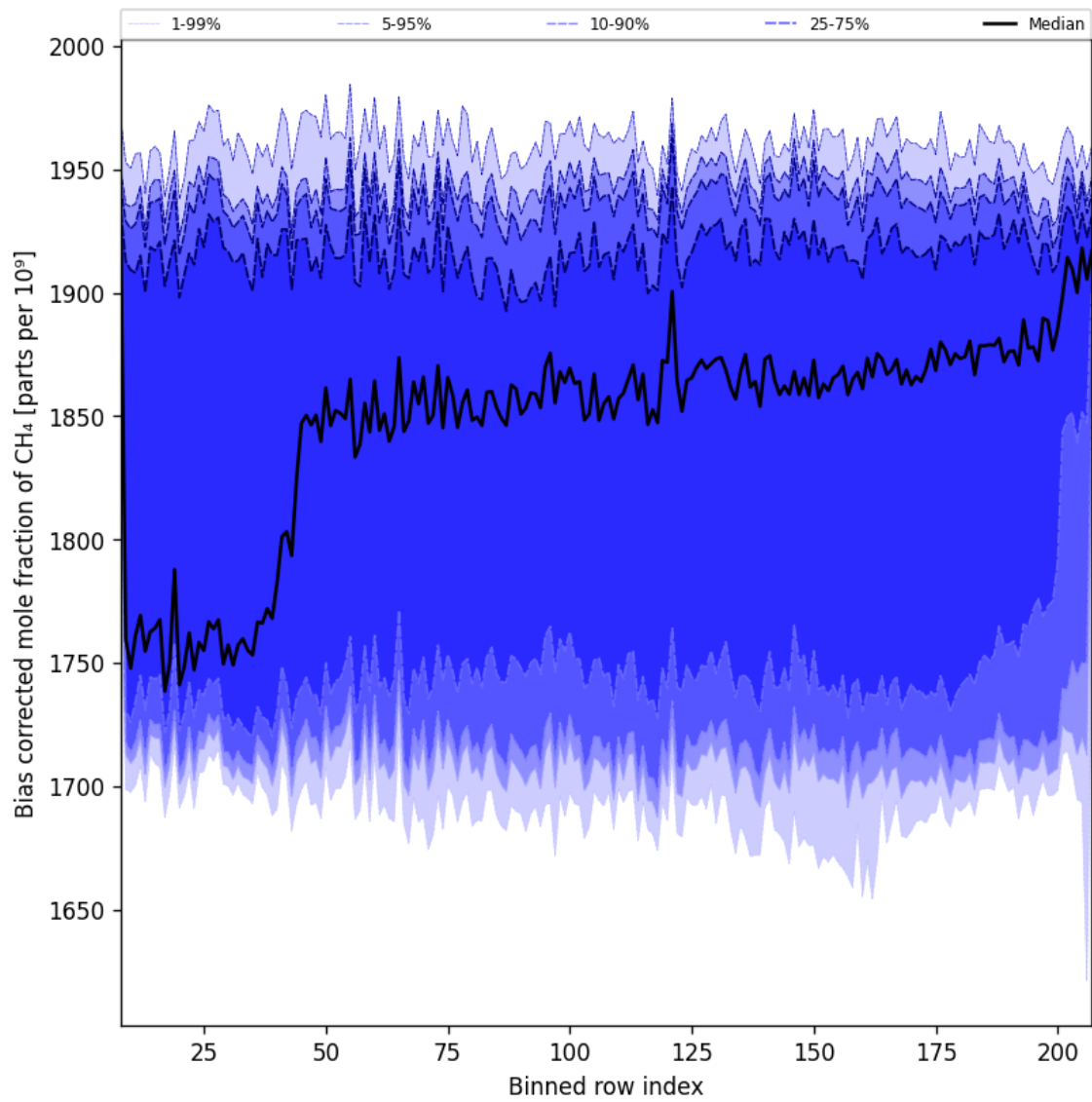
Figure 36: Along track statistics of “Bias corrected mole fraction of CH 4 ” for 2024-12-29 to 2024-12-31
