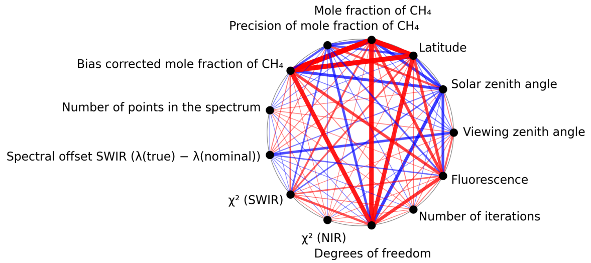
Figure 1: Map of correlation graph for 2024-12-29 to 2024-12-31.
