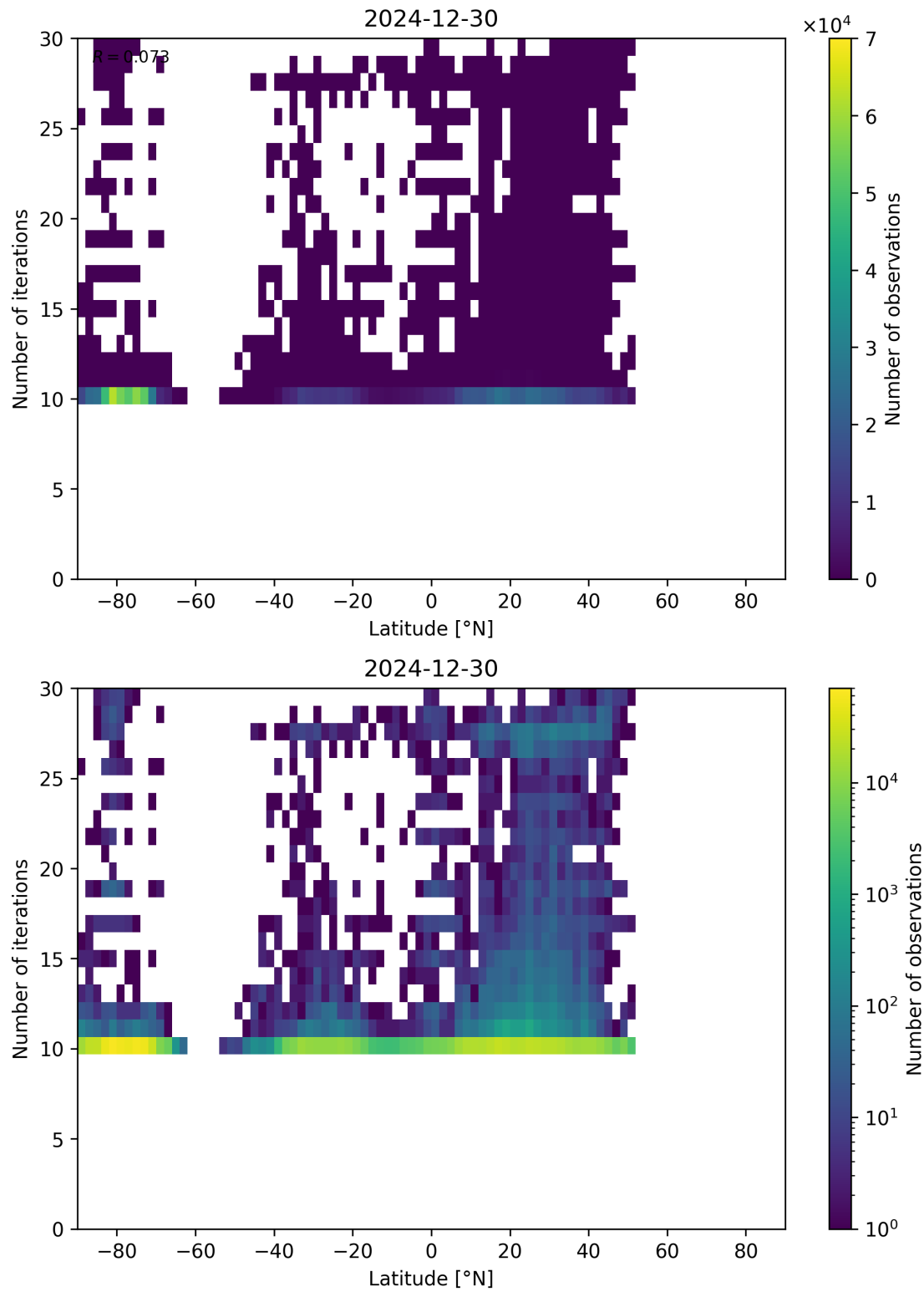
Figure 60: Scatter density plot of “Latitude” against “Number of iterations” for 2024-12-29 to 2024-12-31.
