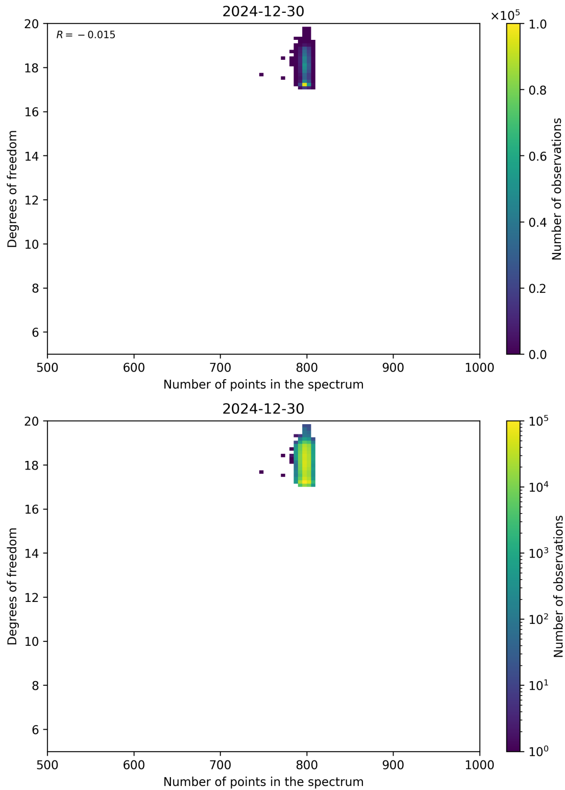
Figure 90: Scatter density plot of “Number of points in the spectrum” against “Degrees of freedom” for 2024-12-29 to 2024-12-31.
