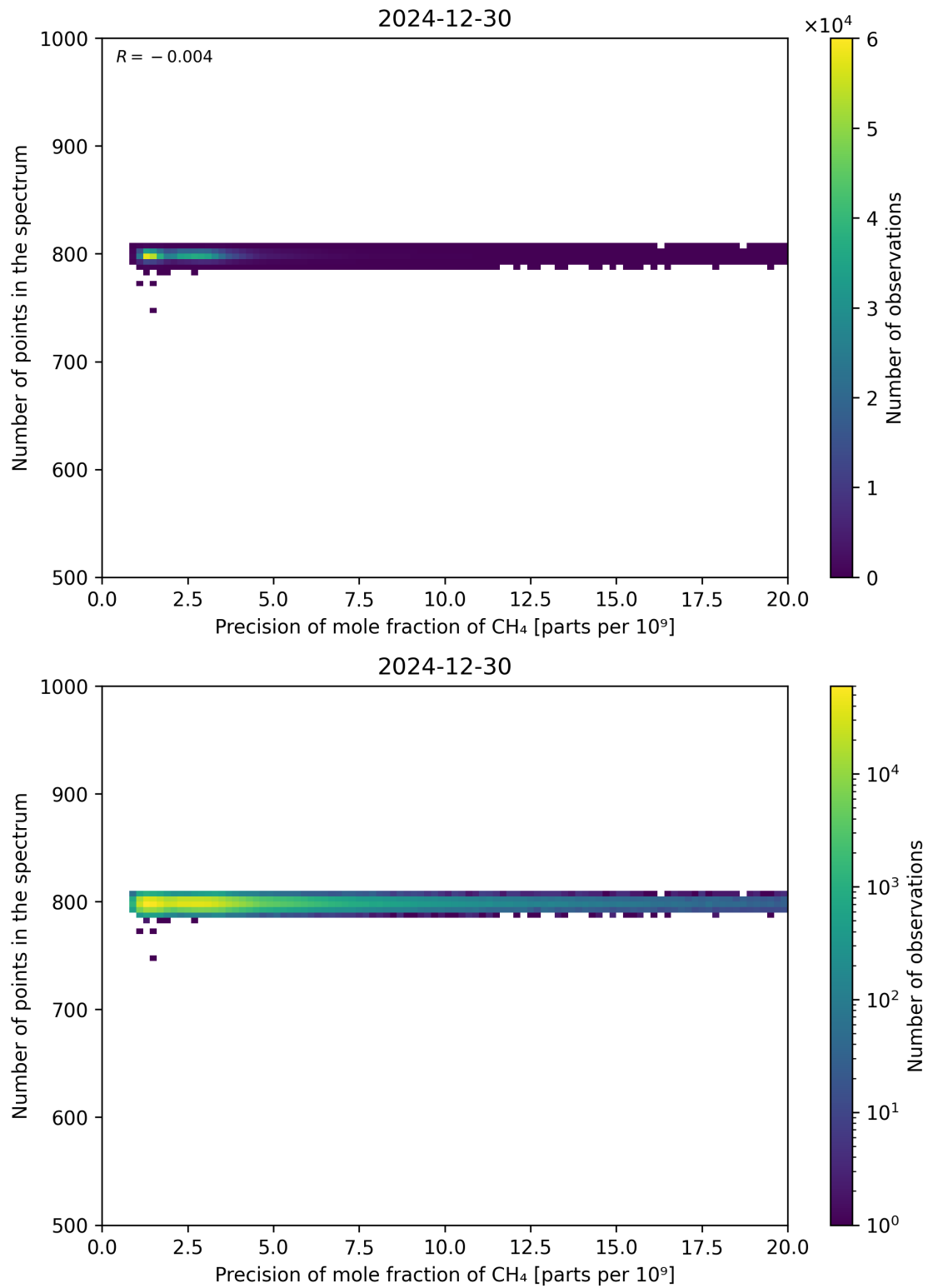
Figure 84: Scatter density plot of “Precision of mole fraction of CH 4 ” against “Number of points in the spectrum” for 2024-12-29 to 2024-12-31.
