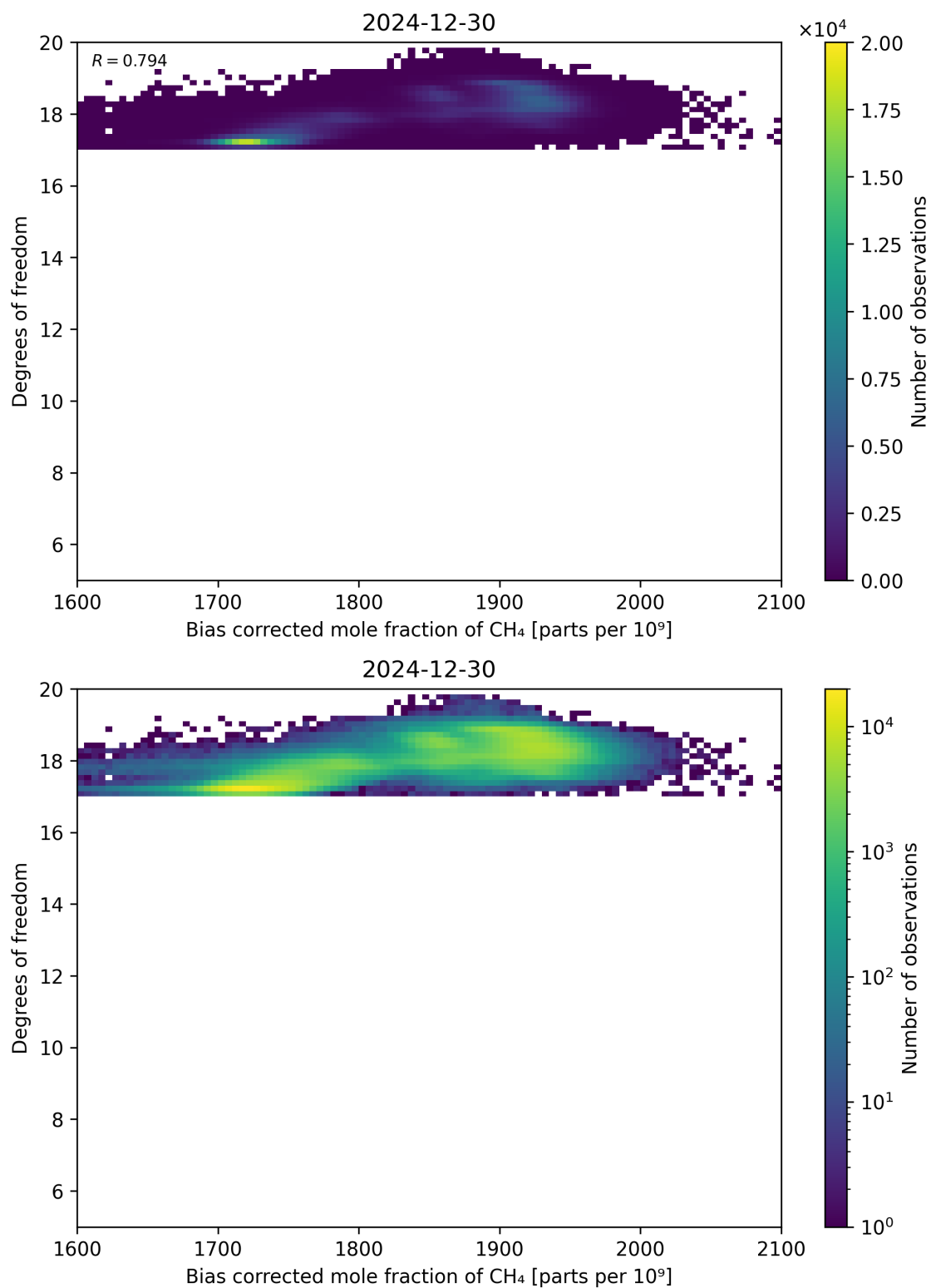
Figure 65: Scatter density plot of “Bias corrected mole fraction of CH 4 ” against “Degrees of freedom” for 2024-12-29 to 2024-12-31.
