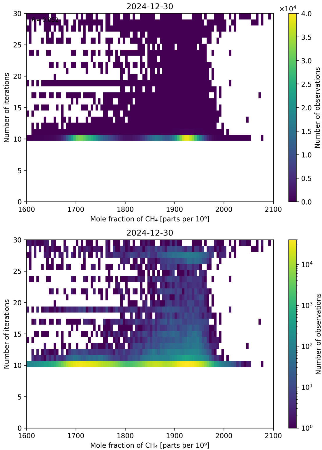
Figure 76: Scatter density plot of “Mole fraction of CH 4 ” against “Number of iterations” for 2024-12-29 to 2024-12-31.
