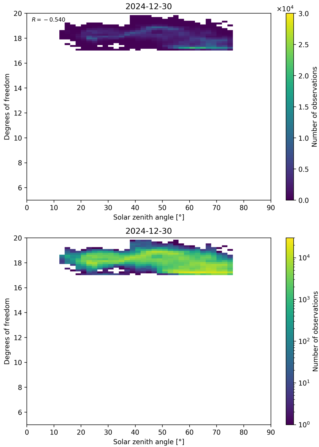
Figure 96: Scatter density plot of “Solar zenith angle” against “Degrees of freedom” for 2024-12-29 to 2024-12-31.
