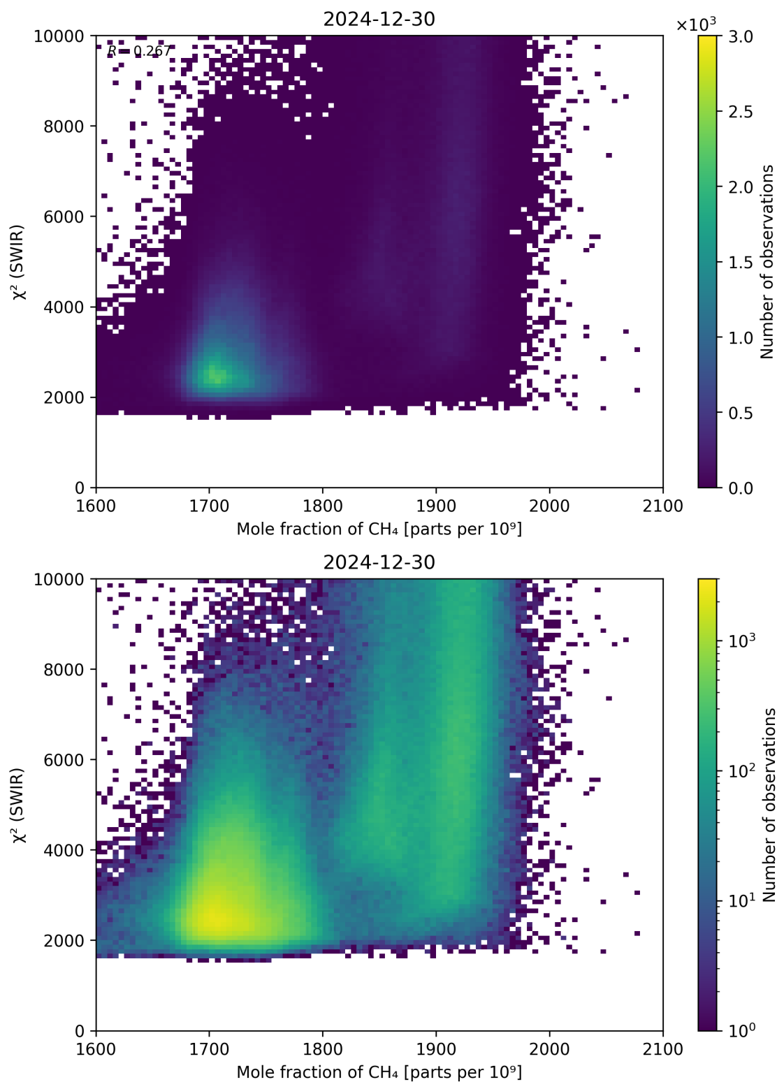
Figure 71: Scatter density plot of “Mole fraction of \text{CH}_4 ” against “ \chi^2 (SWIR)” for 2024-12-29 to 2024-12-31.
