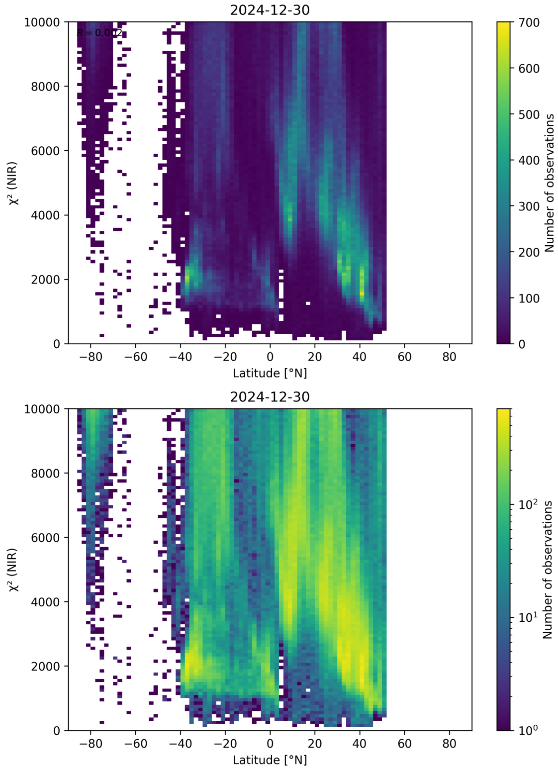
Figure 53: Scatter density plot of “Latitude” against “ \chi^2 (NIR)” for 2024-12-29 to 2024-12-31.
