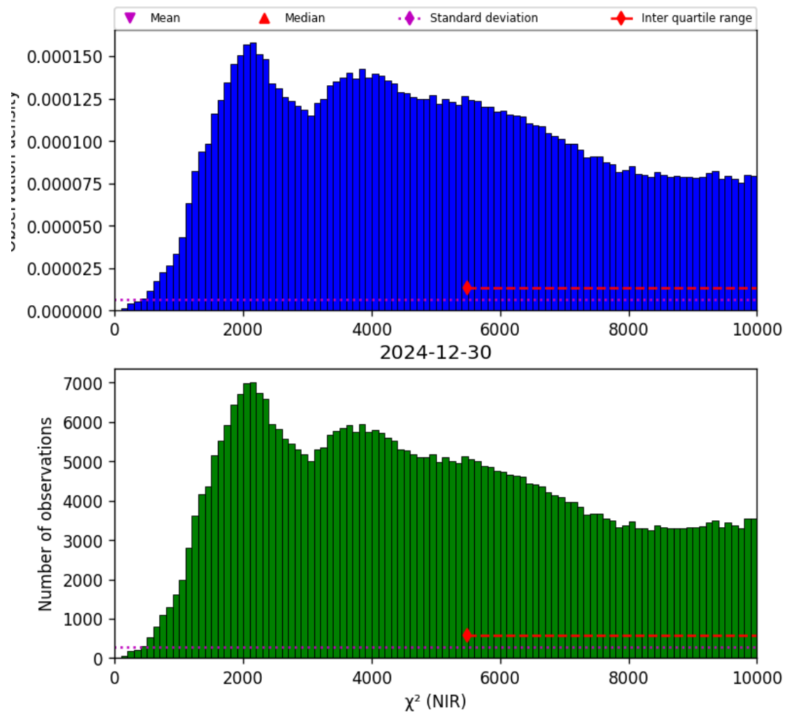
Figure 29: Histogram of “ \chi^2 (NIR)” for 2024-12-29 to 2024-12-31
