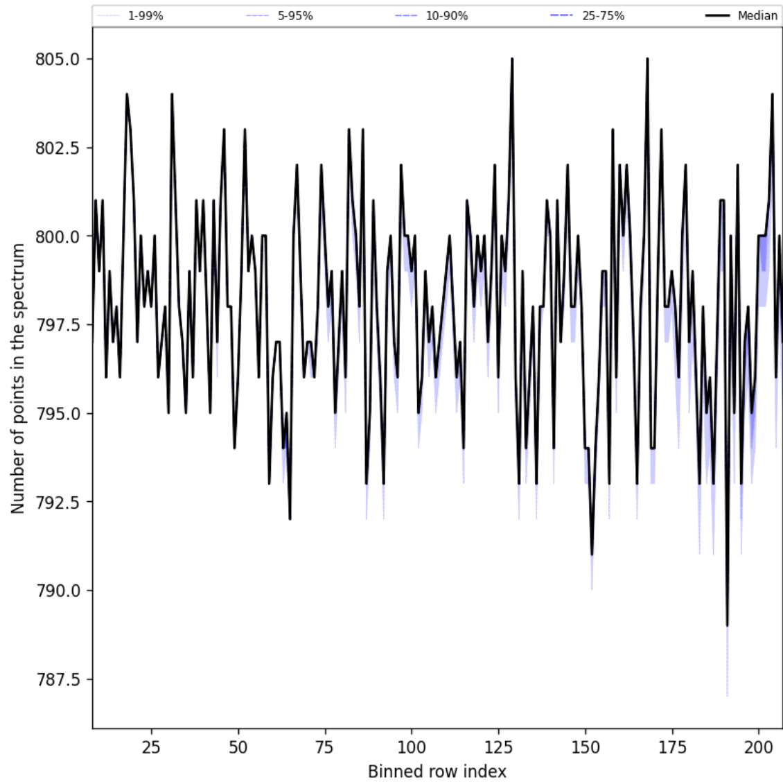
Figure 37: Along track statistics of “Number of points in the spectrum” for 2024-12-29 to 2024-12-31
