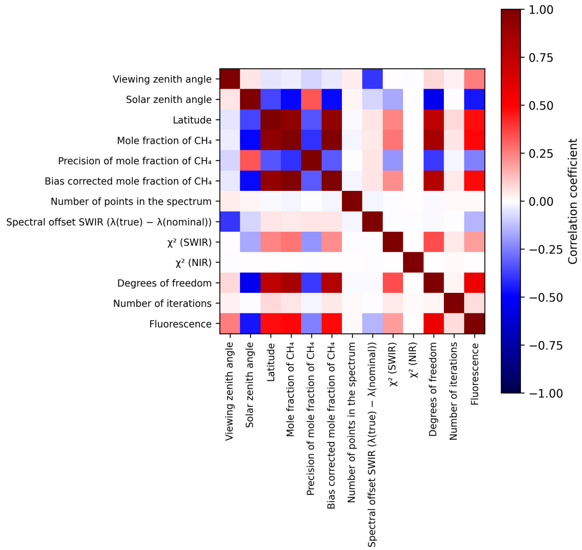
Figure 2: Map of correlation matrix for 2024-12-29 to 2024-12-31.
