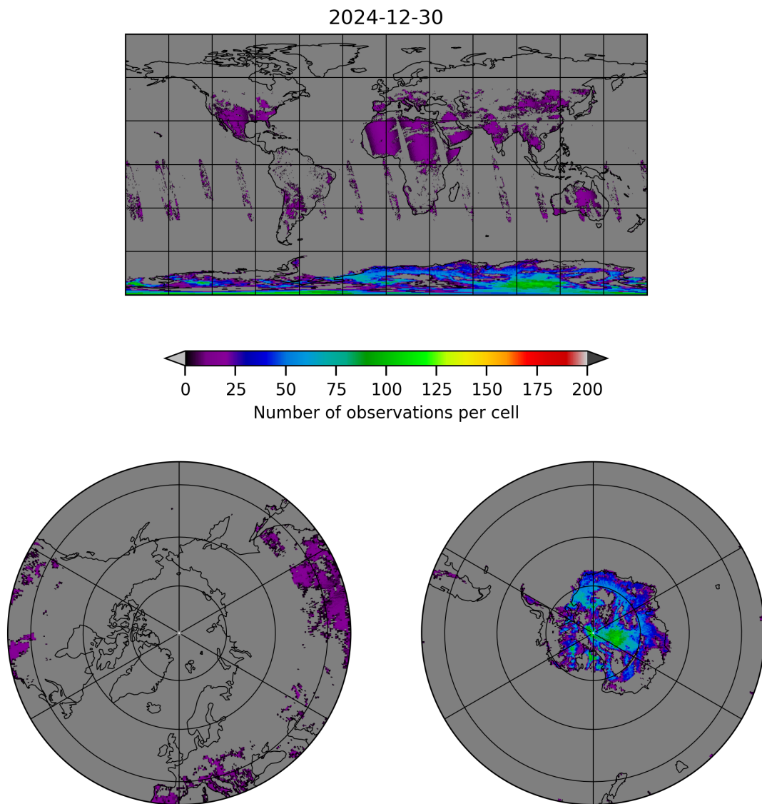
Figure 10: Map of the number of observations for 2024-12-29 to 2024-12-31
