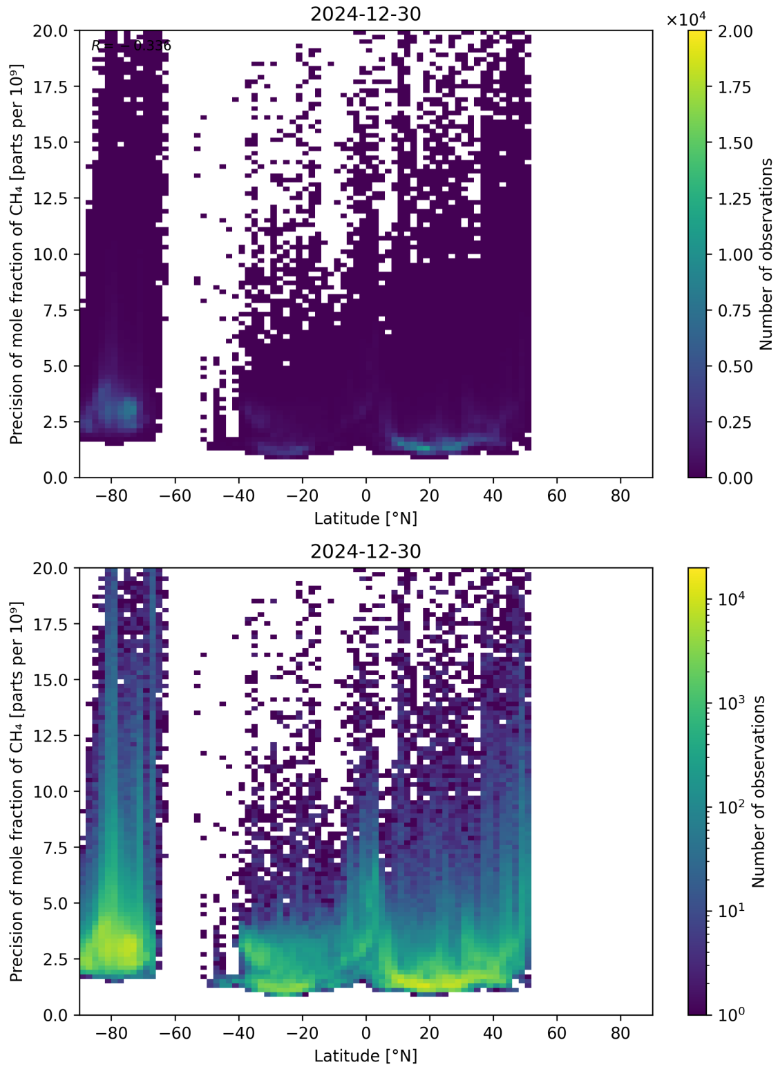
Figure 59: Scatter density plot of “Latitude” against “Precision of mole fraction of CH 4 ” for 2024-12-29 to 2024-12-31.
