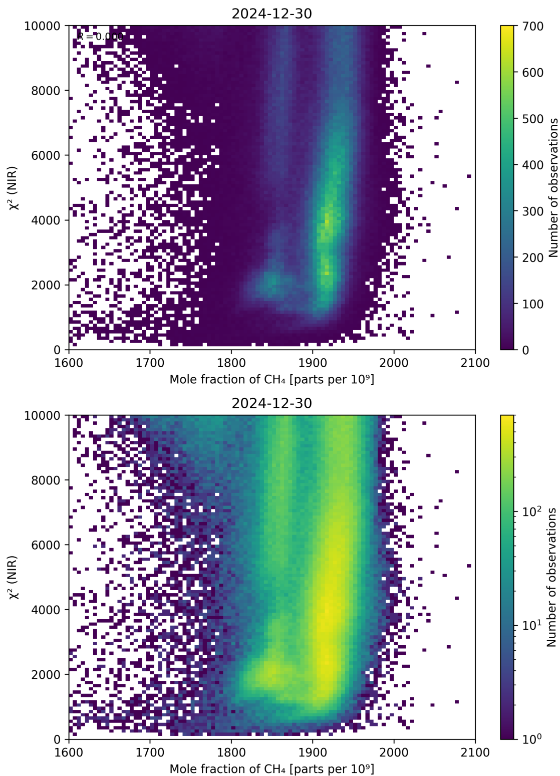
Figure 70: Scatter density plot of “Mole fraction of CH 4 ” against “ \chi^2 (NIR)” for 2024-12-29 to 2024-12-31.
