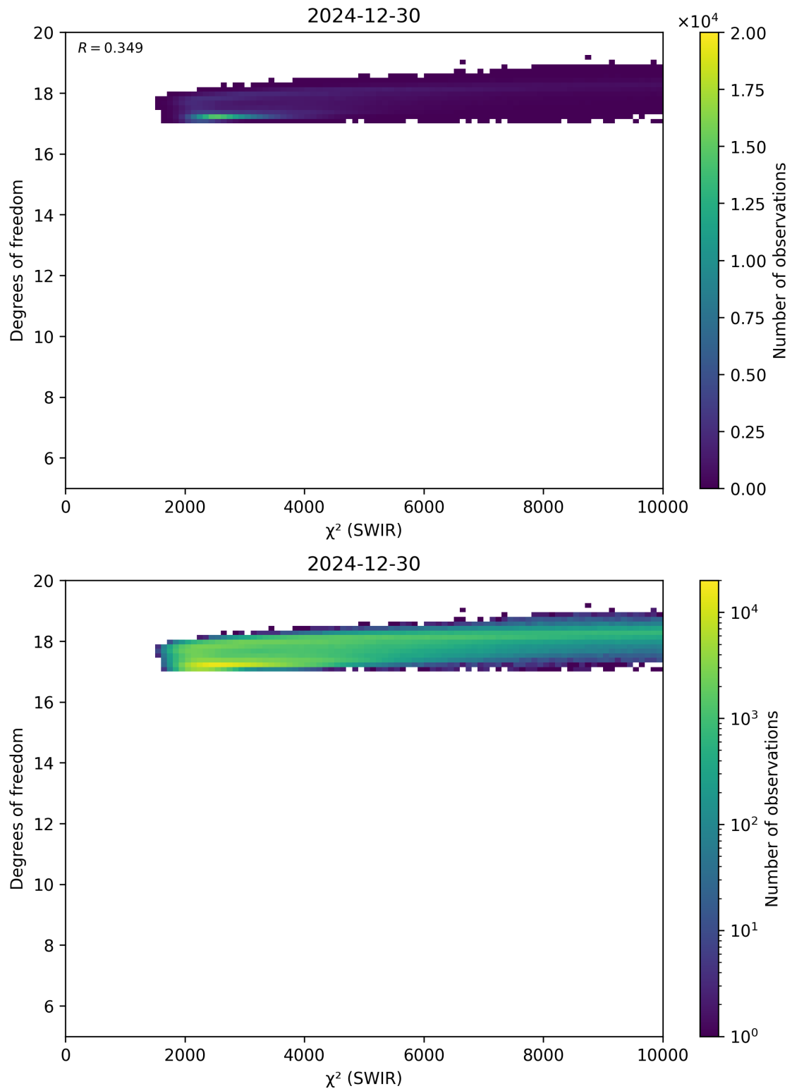
Figure 48: Scatter density plot of “ \chi^2 (SWIR)” against “Degrees of freedom” for 2024-12-29 to 2024-12-31.
