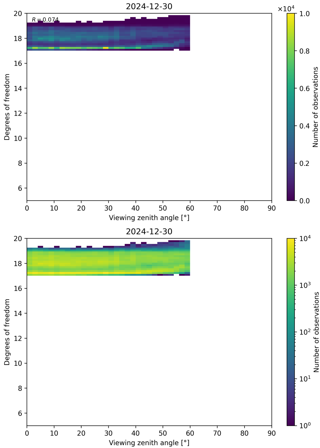
Figure 107: Scatter density plot of “Viewing zenith angle” against “Degrees of freedom” for 2024-12-29 to 2024-12-31.
