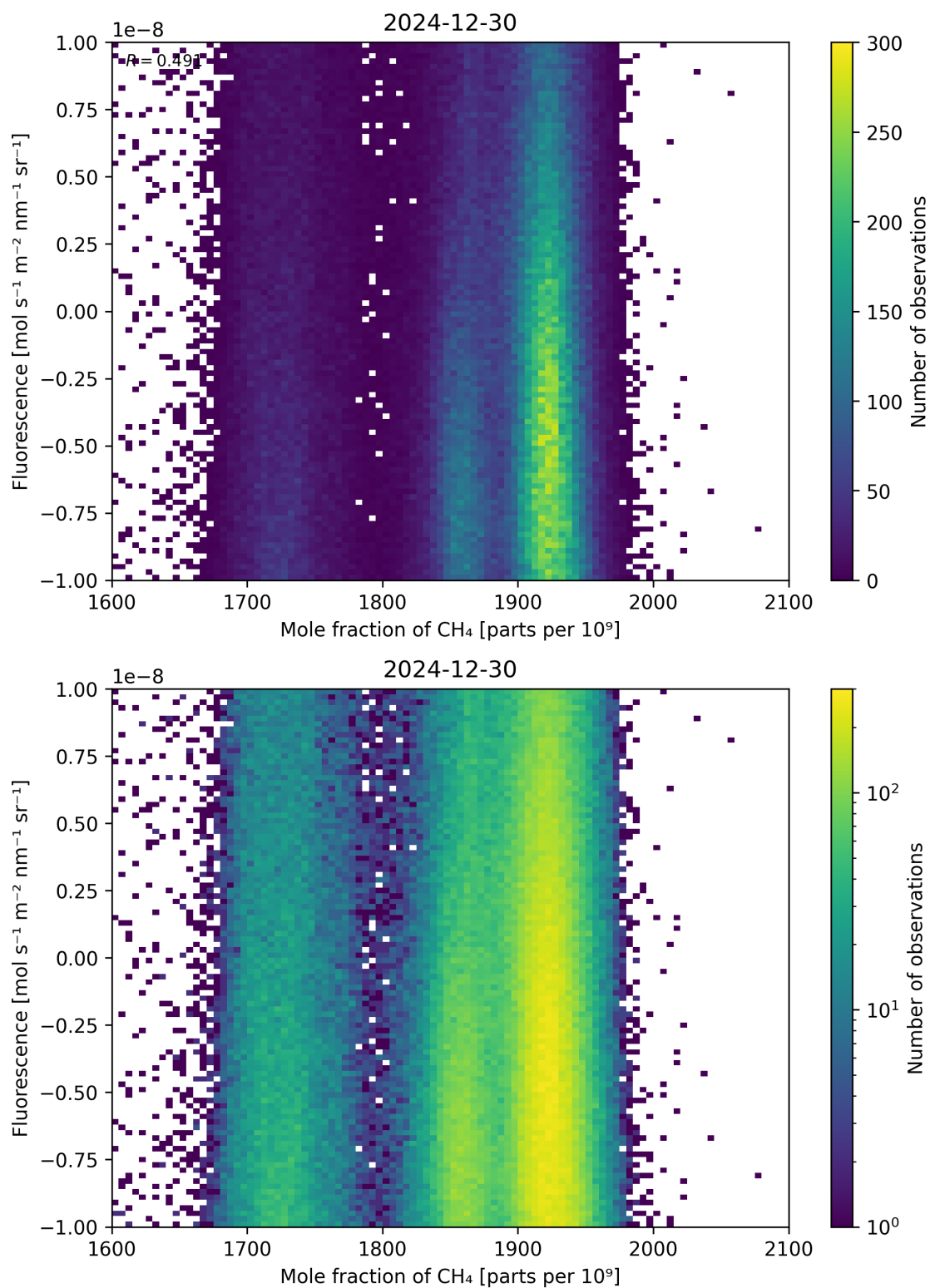
Figure 73: Scatter density plot of “Mole fraction of \text{CH}_4 ” against “Fluorescence” for 2024-12-29 to 2024-12-31.
