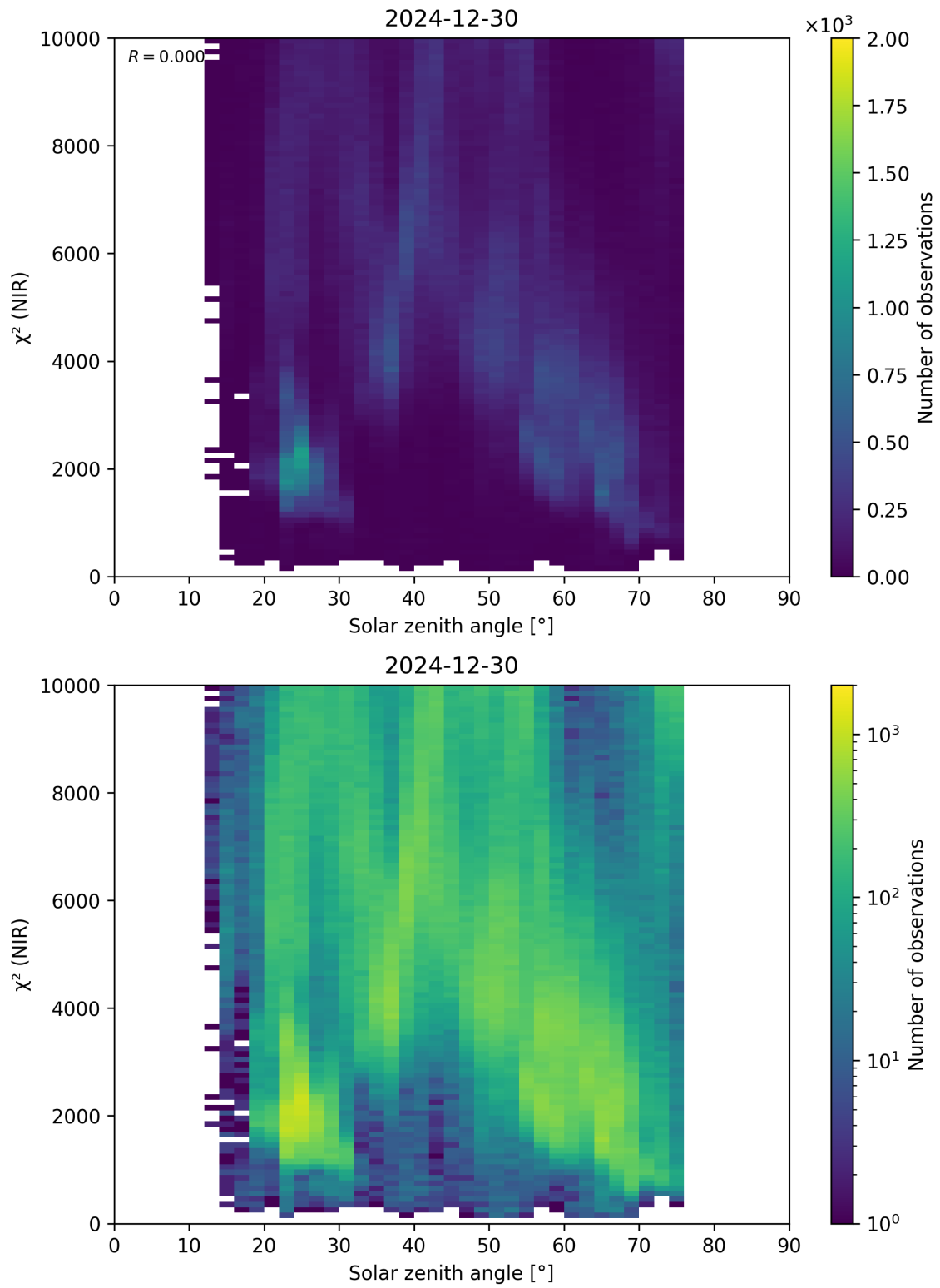
Figure 94: Scatter density plot of “Solar zenith angle” against “ \chi^2 (NIR)” for 2024-12-29 to 2024-12-31.
