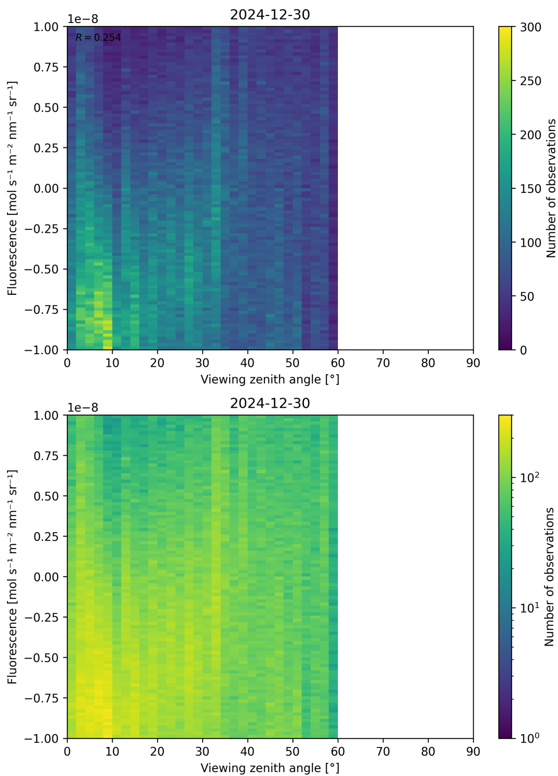
Figure 108: Scatter density plot of “Viewing zenith angle” against “Fluorescence” for 2024-12-29 to 2024-12-31.
