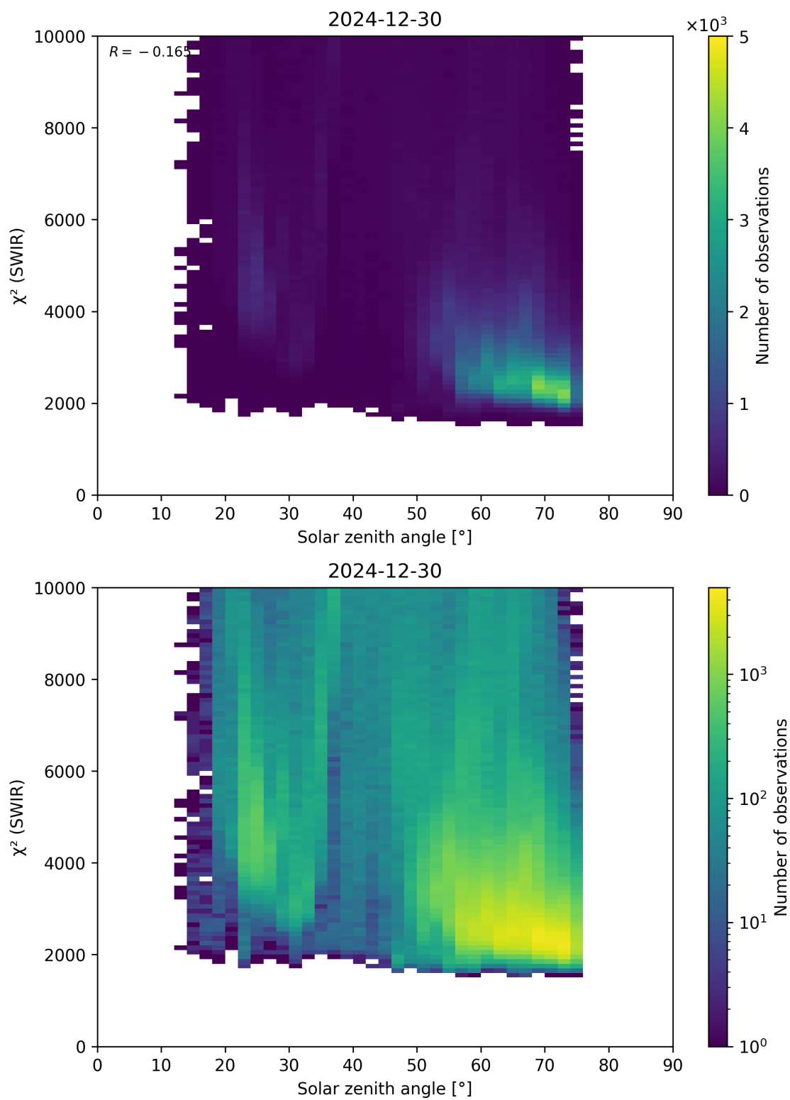
Figure 95: Scatter density plot of “Solar zenith angle” against “ \chi^2 (SWIR)” for 2024-12-29 to 2024-12-31.
