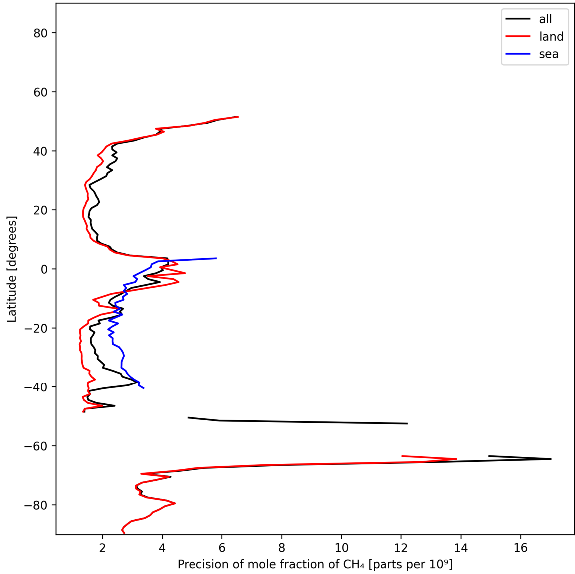
Figure 13: Zonal average of “Precision of mole fraction of CH 4 ” for 2024-12-29 to 2024-12-31.
