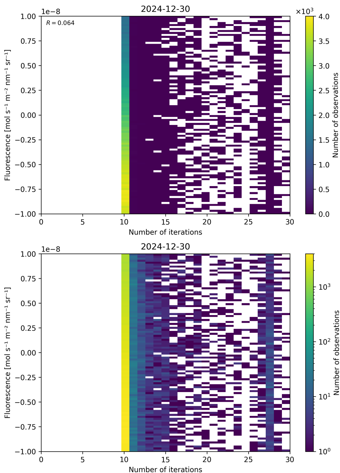
Figure 87: Scatter density plot of “Number of iterations” against “Fluorescence” for 2024-12-29 to 2024-12-31.
