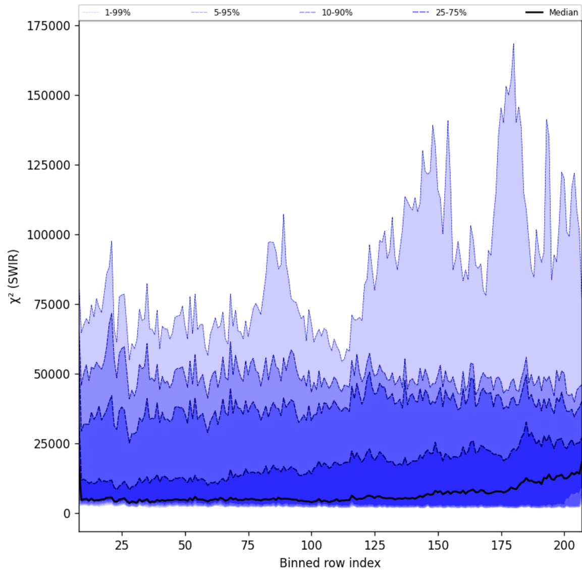
Figure 39: Along track statistics of “ \chi^2 (SWIR)” for 2024-12-29 to 2024-12-31
