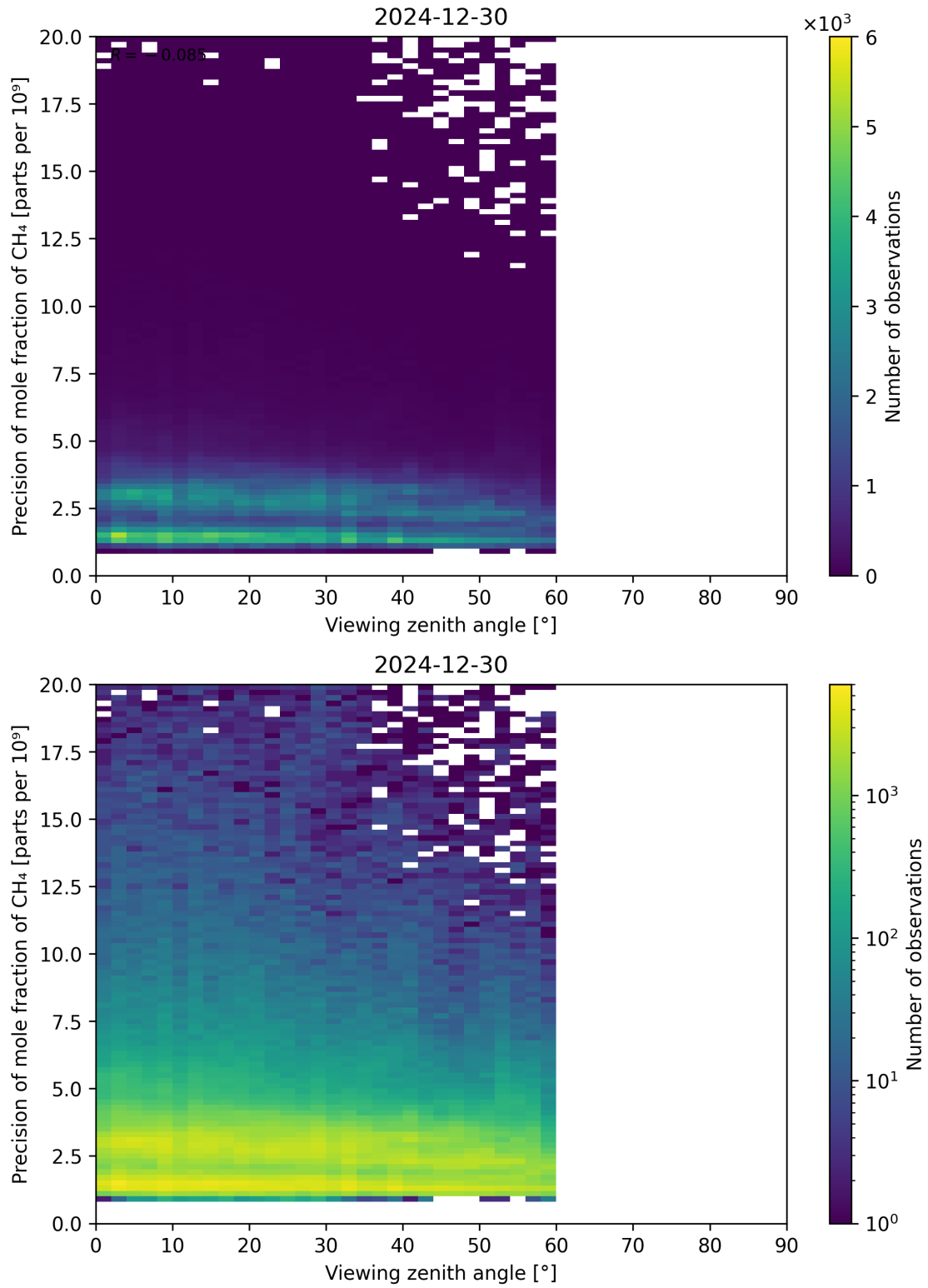
Figure 112: Scatter density plot of “Viewing zenith angle” against “Precision of mole fraction of CH 4 ” for 2024-12-29 to 2024-12-31.
