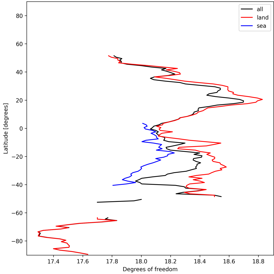
Figure 19: Zonal average of “Degrees of freedom” for 2024-12-29 to 2024-12-31.
