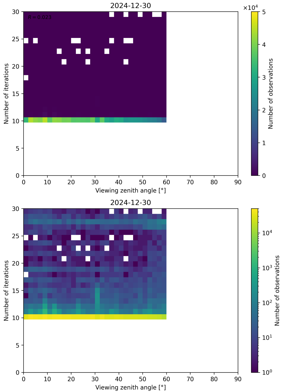
Figure 113: Scatter density plot of “Viewing zenith angle” against “Number of iterations” for 2024-12-29 to 2024-12-31.
