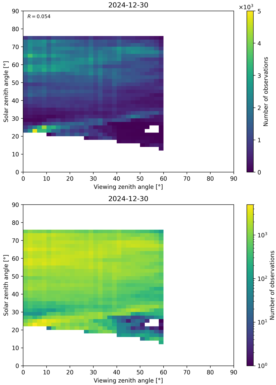
Figure 115: Scatter density plot of “Viewing zenith angle” against “Solar zenith angle” for 2024-12-29 to 2024-12-31.
