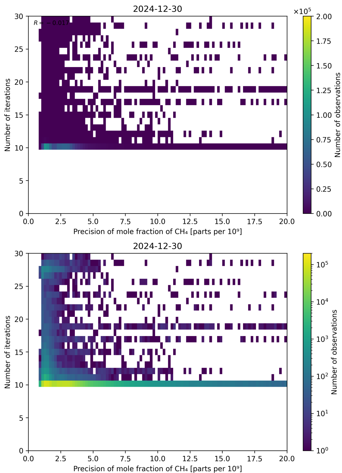
Figure 83: Scatter density plot of “Precision of mole fraction of CH 4 ” against “Number of iterations” for 2024-12-29 to 2024-12-31.
