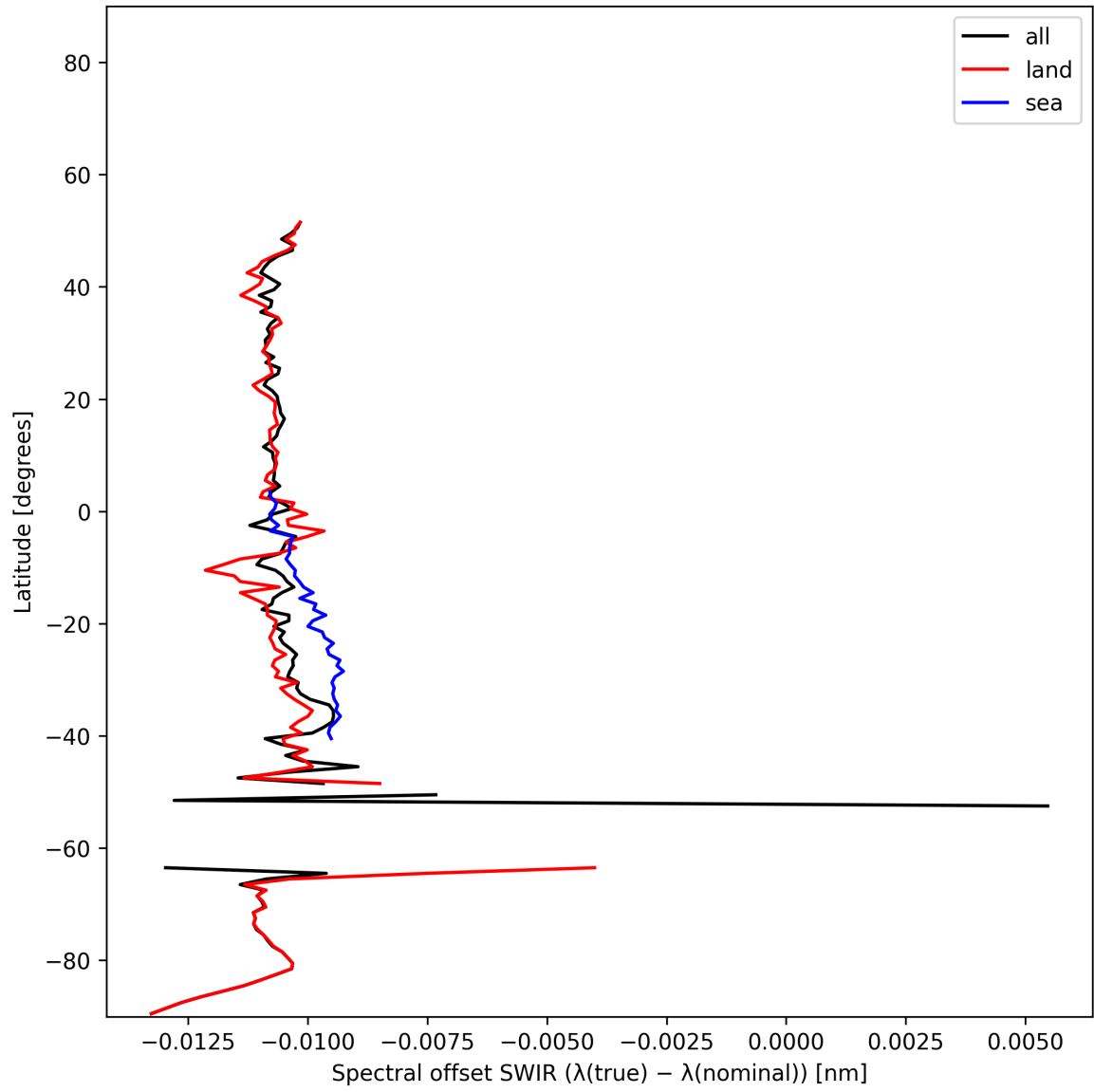
Figure 16: Zonal average of “Spectral offset SWIR ( \lambda_{\text{true}} - \lambda_{\text{nominal}} )” for 2024-12-29 to 2024-12-31.
