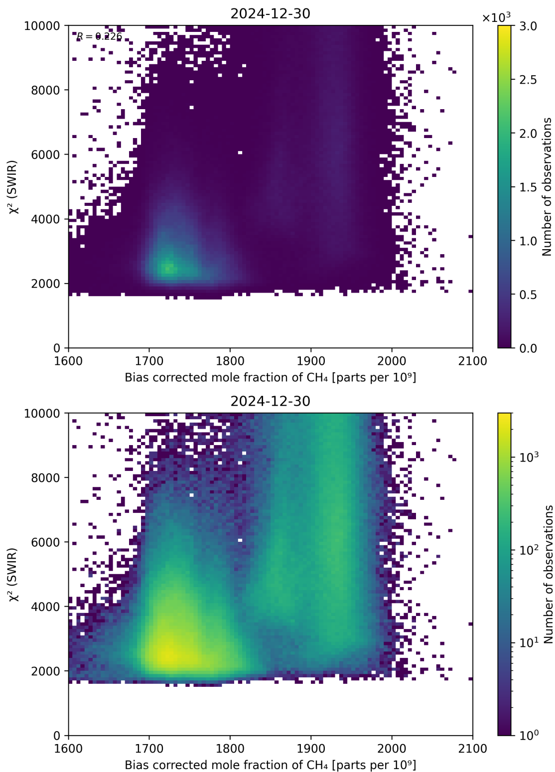
Figure 64: Scatter density plot of “Bias corrected mole fraction of \text{CH}_4 ” against “ \chi^2 (SWIR)” for 2024-12-29 to 2024-12-31.
