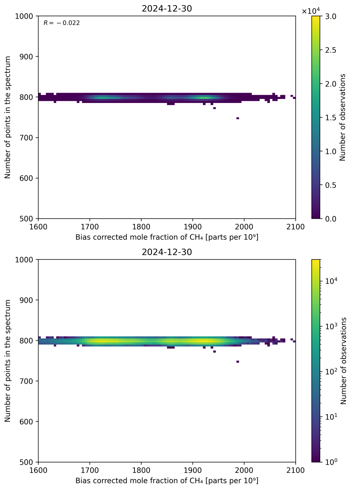
Figure 68: Scatter density plot of “Bias corrected mole fraction of CH 4 ” against “Number of points in the spectrum” for 2024-12-29 to 2024-12-31.
