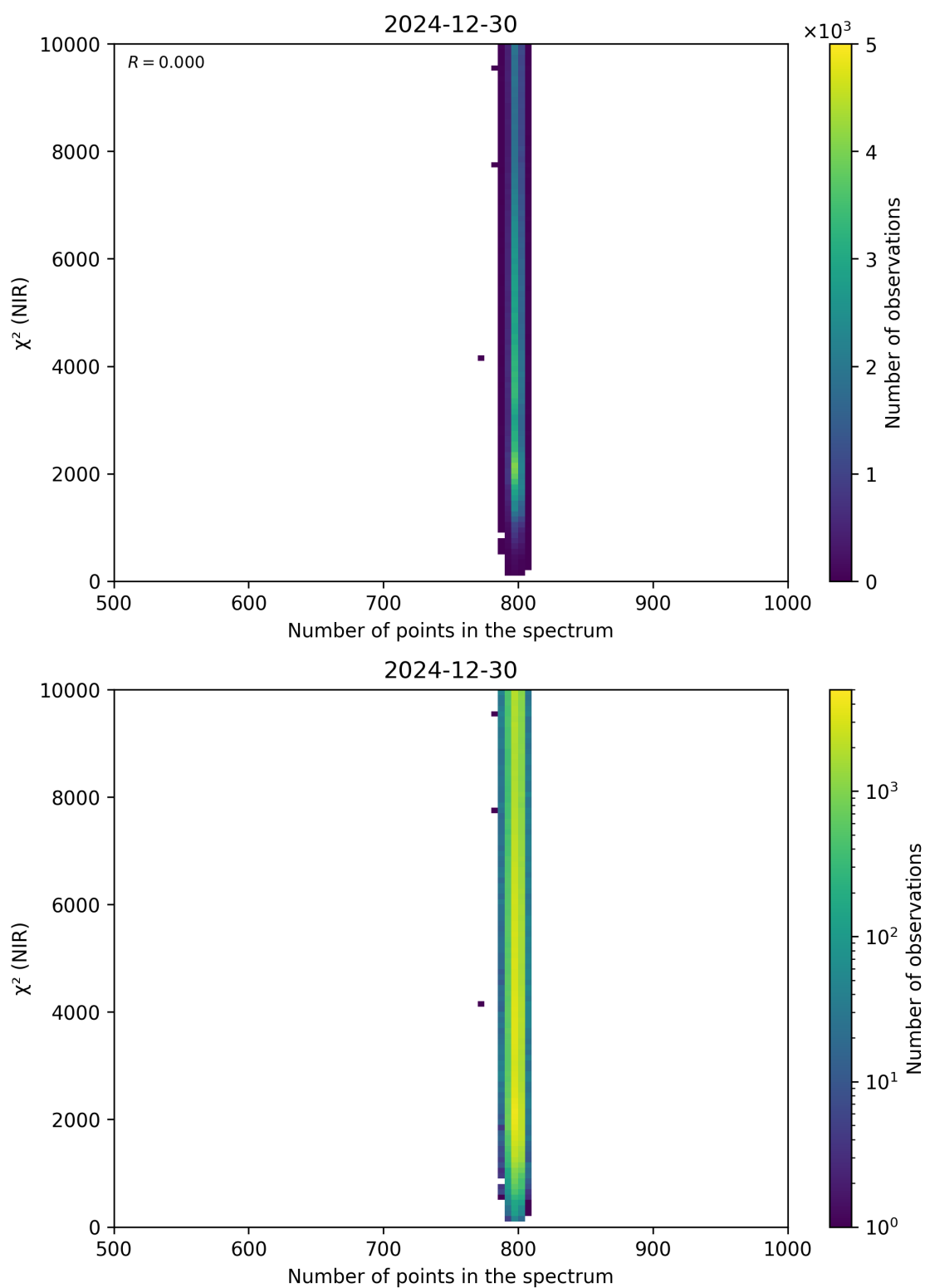
Figure 88: Scatter density plot of “Number of points in the spectrum” against “ \chi^2 (NIR)” for 2024-12-29 to 2024-12-31.
