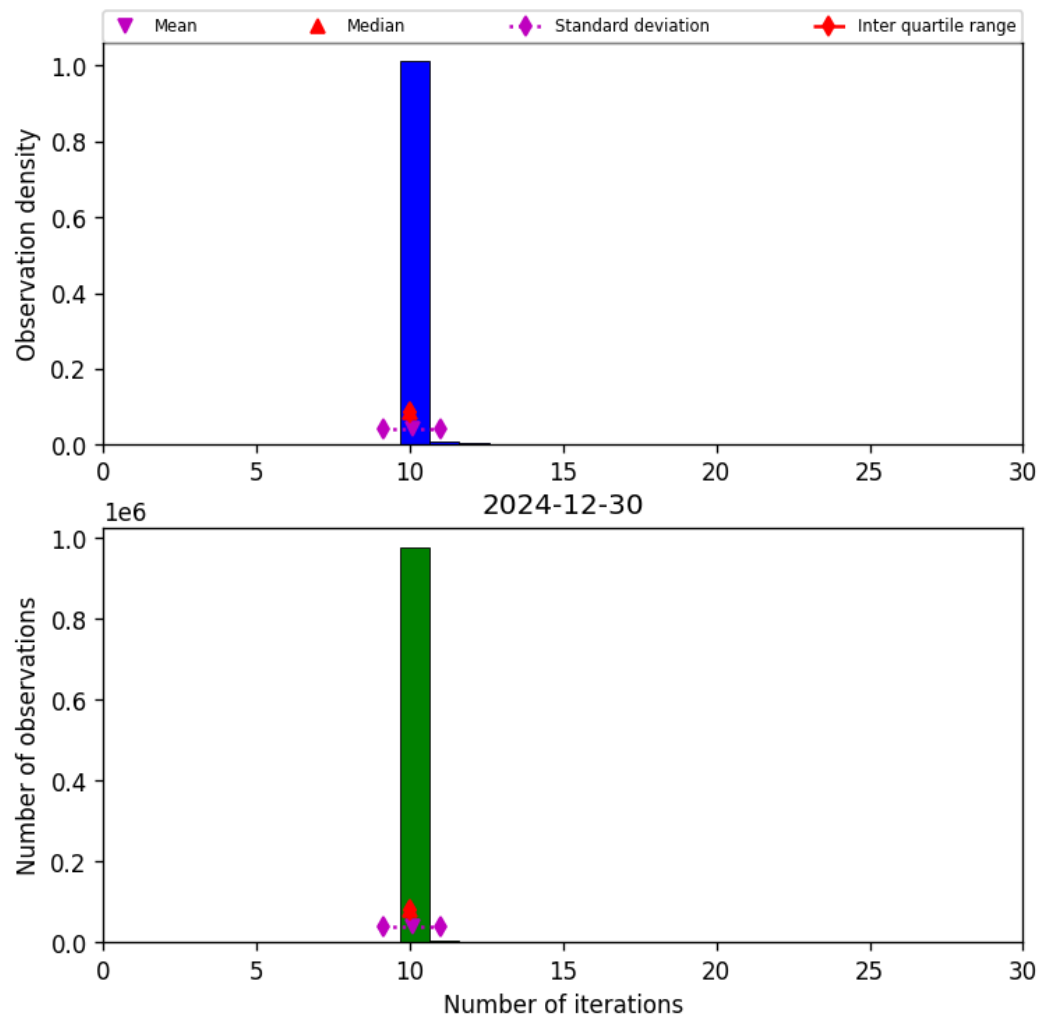
Figure 31: Histogram of “Number of iterations” for 2024-12-29 to 2024-12-31
