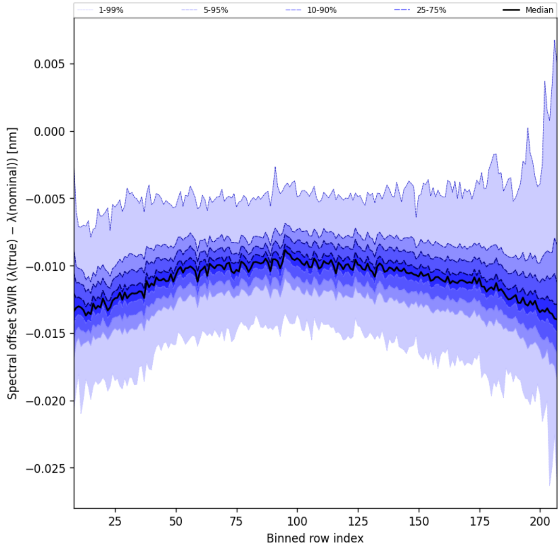
Figure 38: Along track statistics of “Spectral offset SWIR ( \lambda_{\text{true}} - \lambda_{\text{nominal}} )” for 2024-12-29 to 2024-12-31
