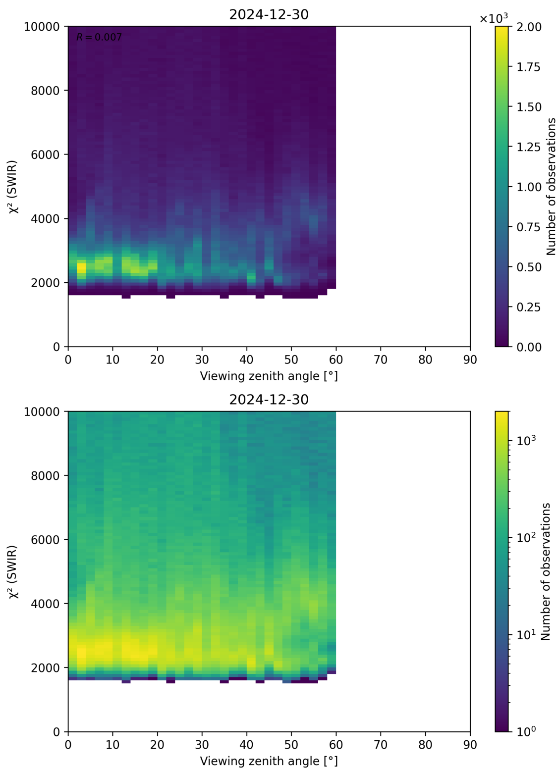
Figure 106: Scatter density plot of “Viewing zenith angle” against “ \chi^2 (SWIR)” for 2024-12-29 to 2024-12-31.
