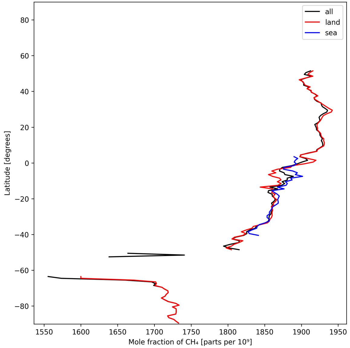
Figure 12: Zonal average of “Mole fraction of CH 4 ” for 2024-12-29 to 2024-12-31.
