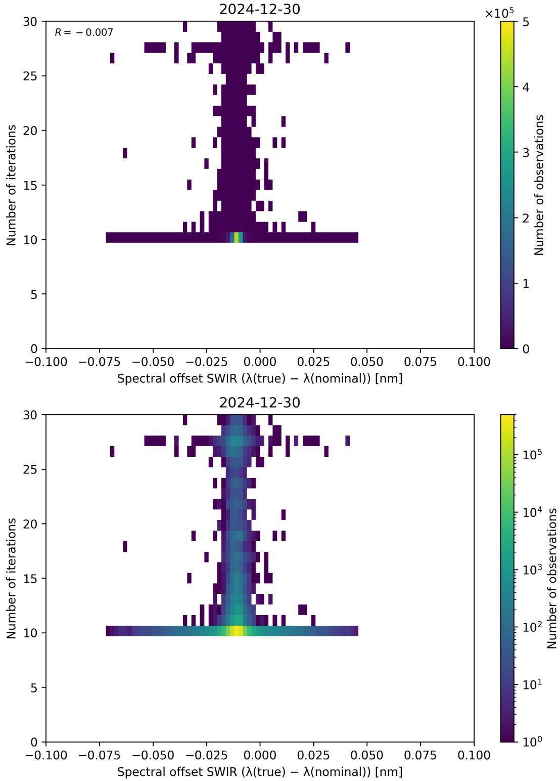
Figure 121: Scatter density plot of “Spectral offset SWIR ( \lambda_{\text{true}} - \lambda_{\text{nominal}} )” against “Number of iterations” for 2024-12-29 to 2024-12-31.
