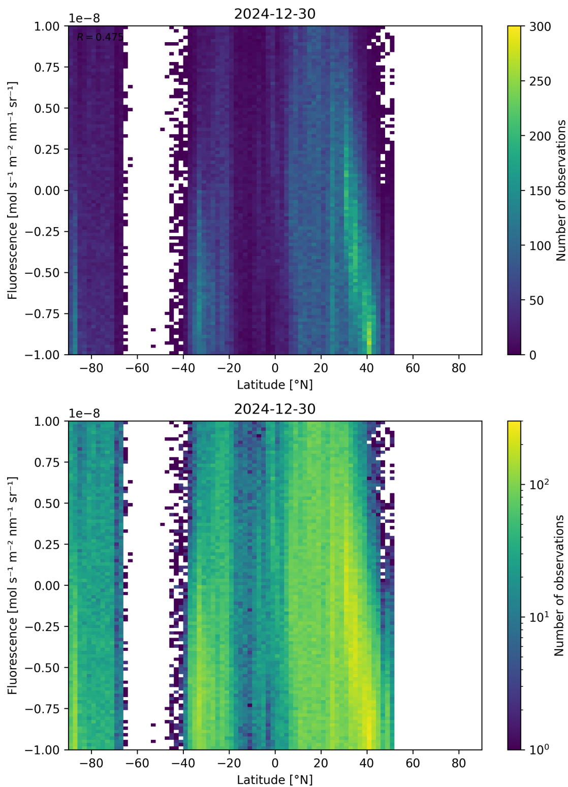
Figure 56: Scatter density plot of “Latitude” against “Fluorescence” for 2024-12-29 to 2024-12-31.
