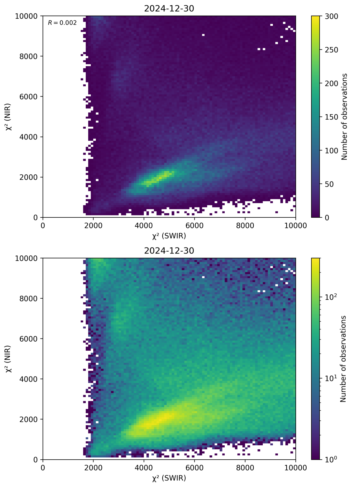
Figure 47: Scatter density plot of “ \chi^2 (SWIR)” against “ \chi^2 (NIR)” for 2024-12-29 to 2024-12-31.
