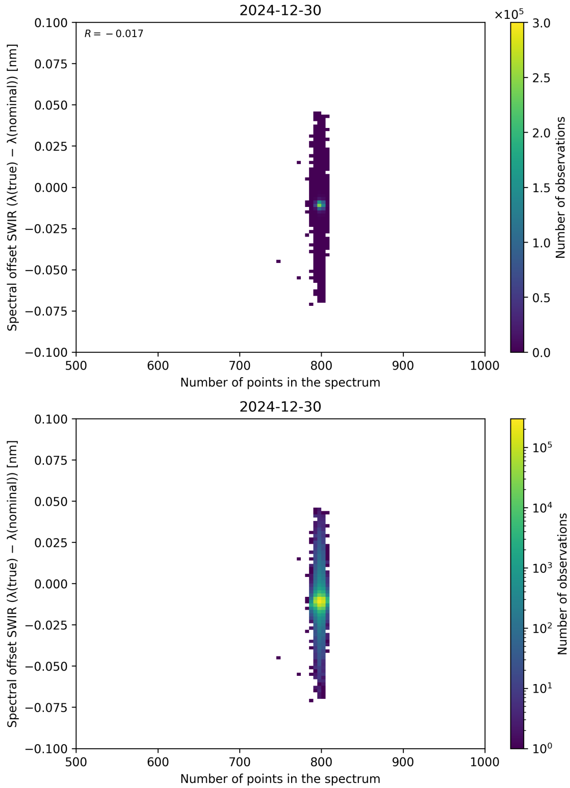
Figure 93: Scatter density plot of “Number of points in the spectrum” against “Spectral offset SWIR ( \lambda_{\text{true}} - \lambda_{\text{nominal}} )” for 2024-12-29 to 2024-12-31.
