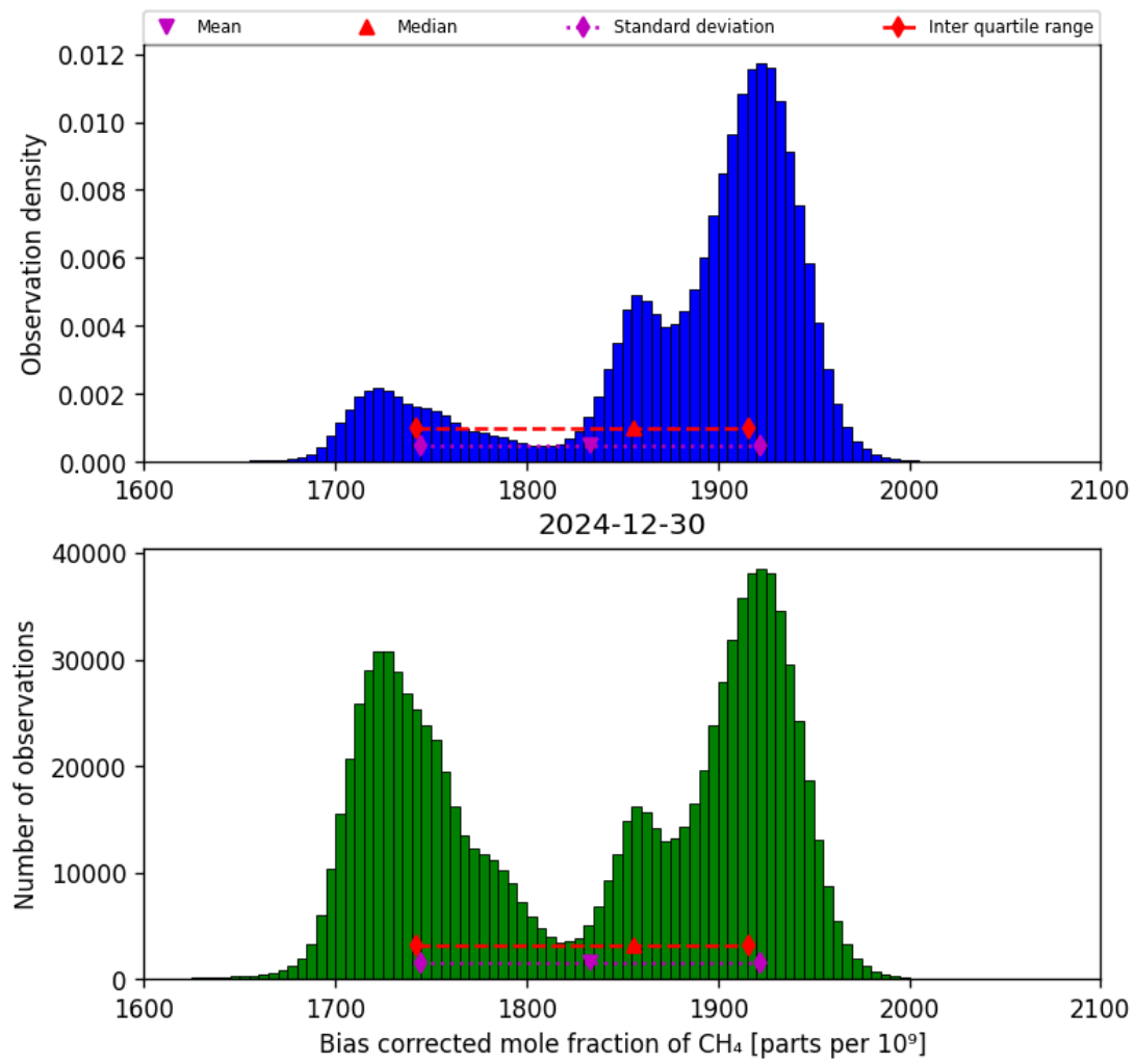
Figure 25: Histogram of “Bias corrected mole fraction of CH 4 ” for 2024-12-29 to 2024-12-31
