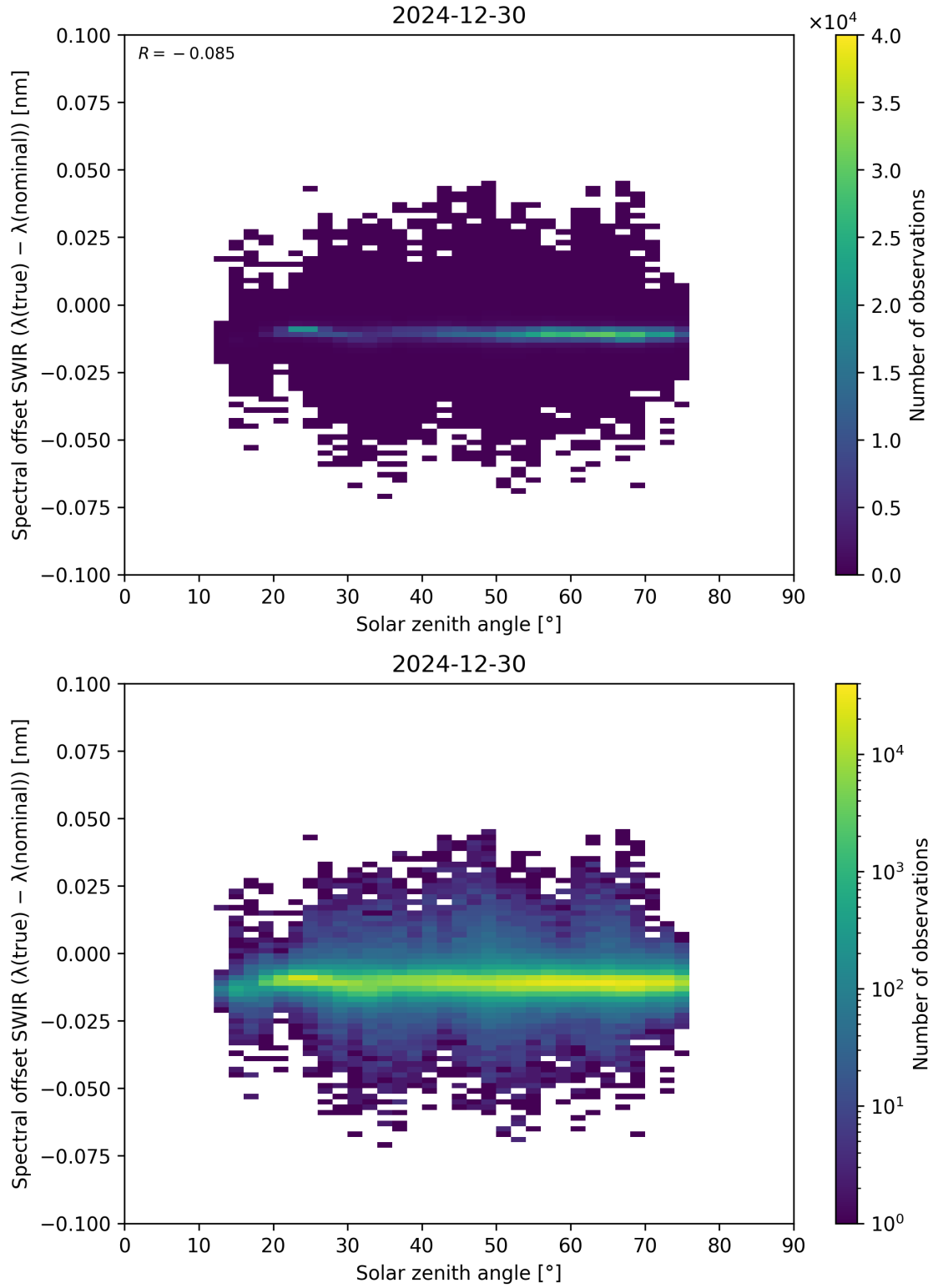
Figure 104: Scatter density plot of “Solar zenith angle” against “Spectral offset SWIR ( \lambda_{\text{true}} - \lambda_{\text{nominal}} )” for 2024-12-29 to 2024-12-31.
