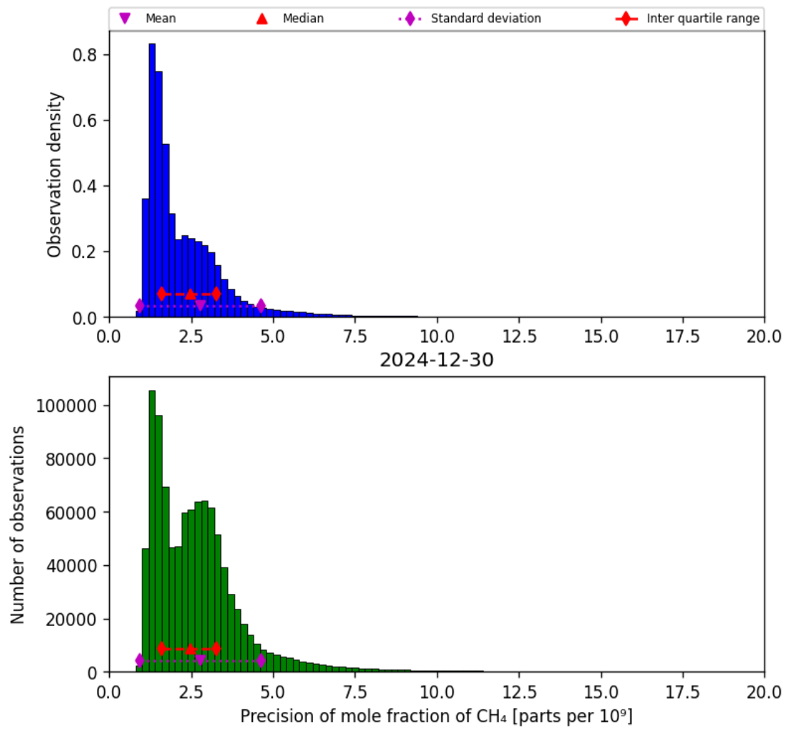
Figure 24: Histogram of “Precision of mole fraction of CH 4 ” for 2024-12-29 to 2024-12-31
