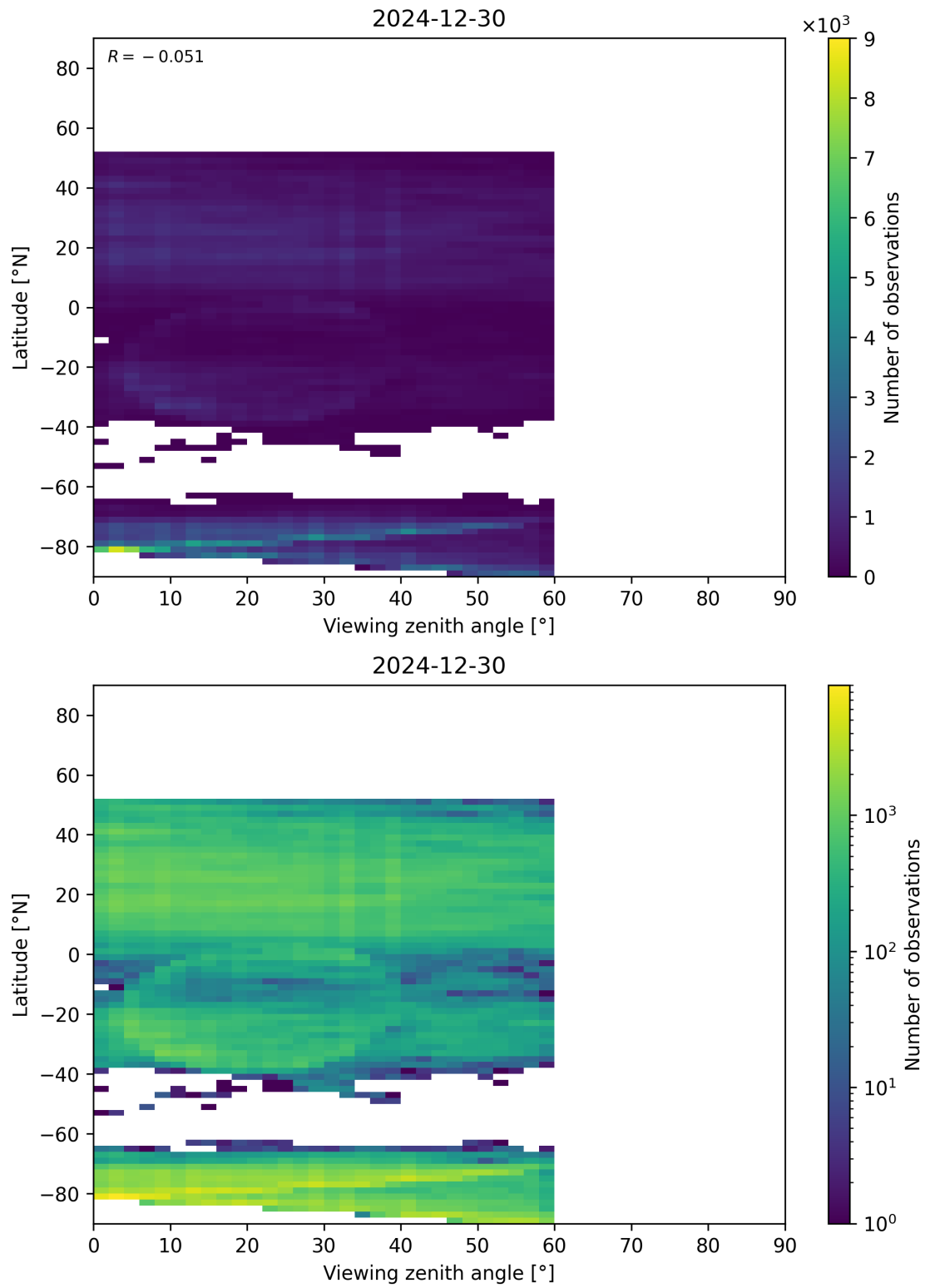
Figure 109: Scatter density plot of “Viewing zenith angle” against “Latitude” for 2024-12-29 to 2024-12-31.
