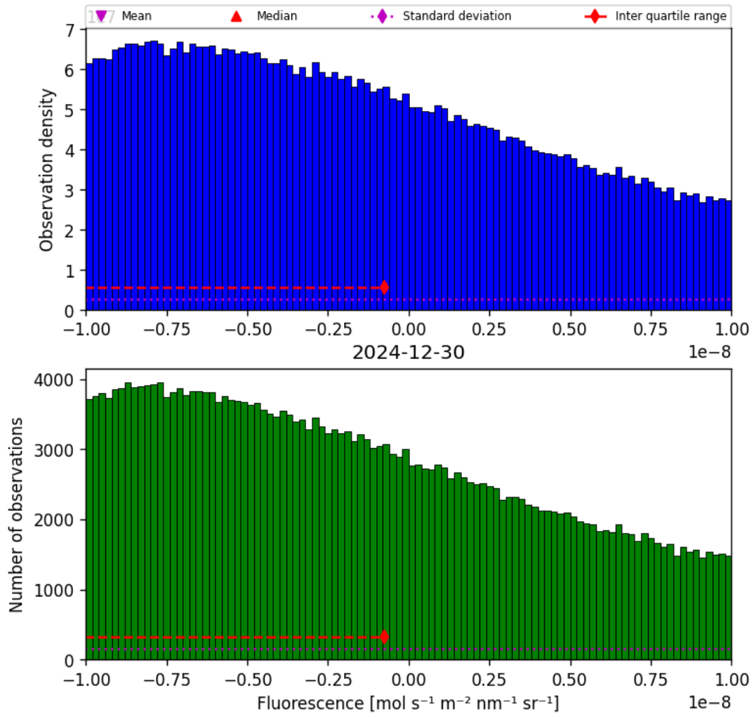
Figure 32: Histogram of “Fluorescence” for 2024-12-29 to 2024-12-31
