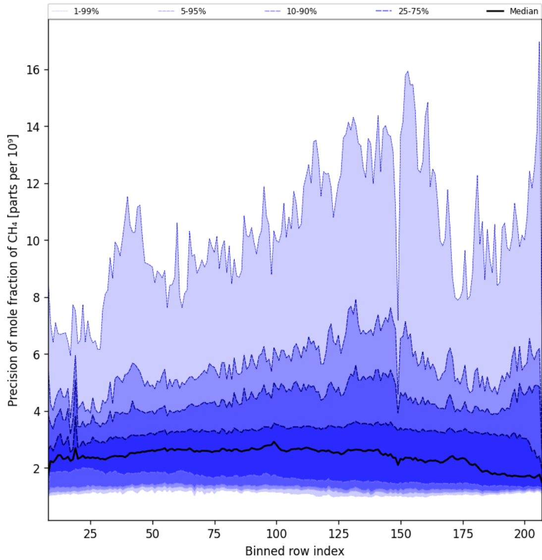
Figure 35: Along track statistics of “Precision of mole fraction of CH 4 ” for 2024-12-29 to 2024-12-31
