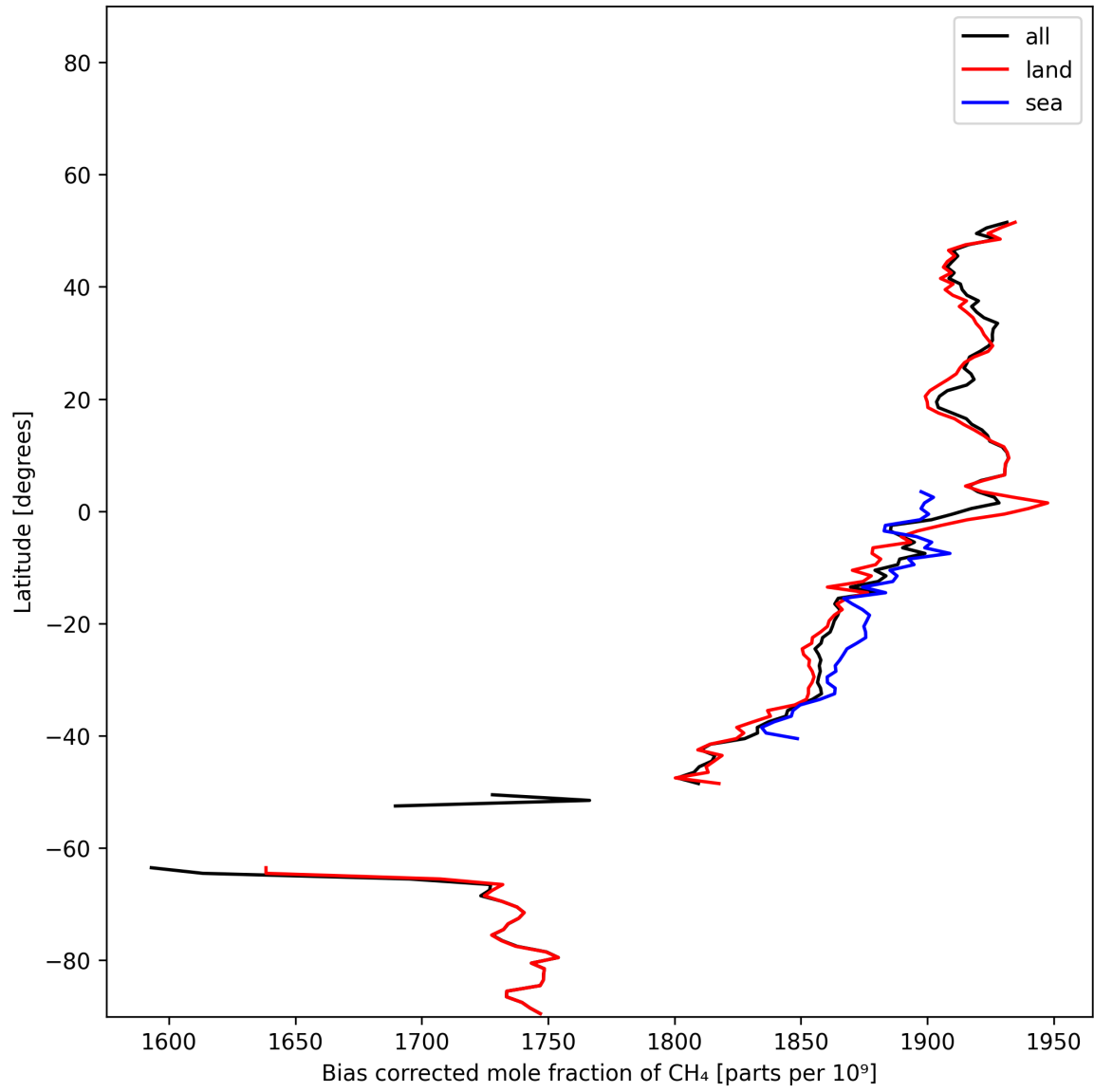
Figure 14: Zonal average of “Bias corrected mole fraction of CH 4 ” for 2024-12-29 to 2024-12-31.
