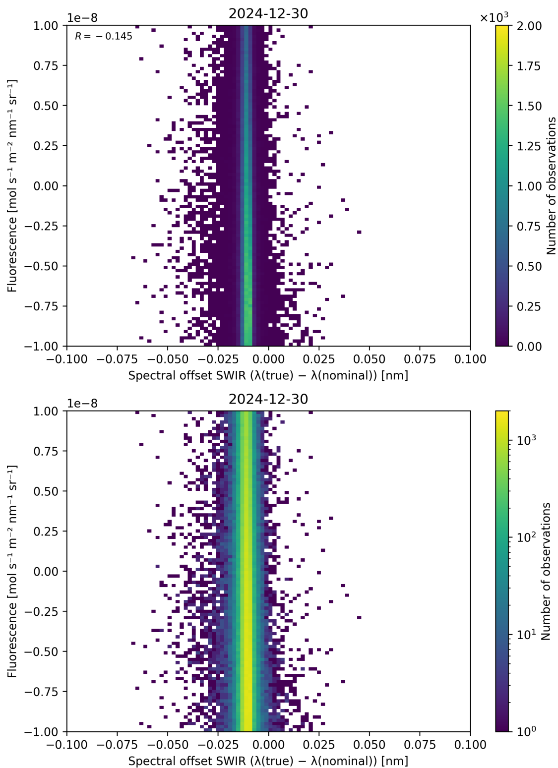
Figure 120: Scatter density plot of “Spectral offset SWIR ( \lambda_{\text{true}} - \lambda_{\text{nominal}} )” against “Fluorescence” for 2024-12-29 to 2024-12-31.
