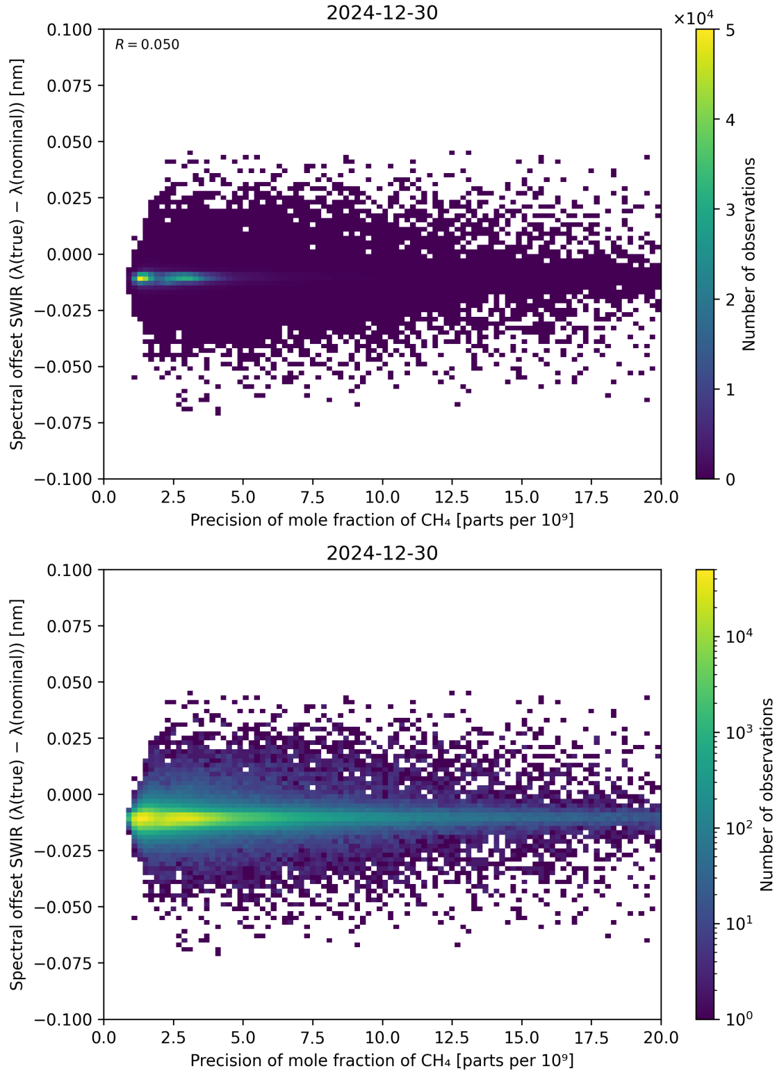
Figure 85: Scatter density plot of “Precision of mole fraction of CH 4 ” against “Spectral offset SWIR ( \lambda_{\text{true}} - \lambda_{\text{nominal}} )” for 2024-12-29 to 2024-12-31.
