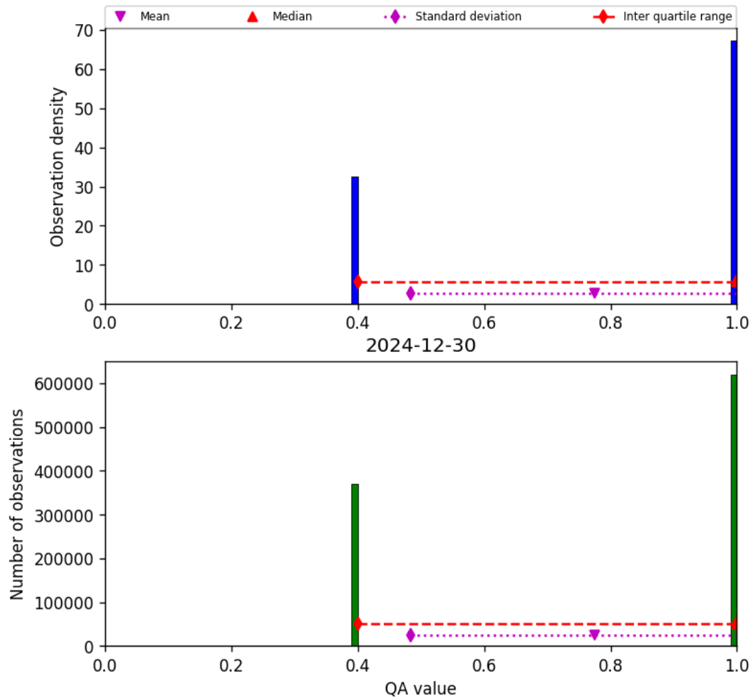
Figure 22: Histogram of “QA value” for 2024-12-29 to 2024-12-31
