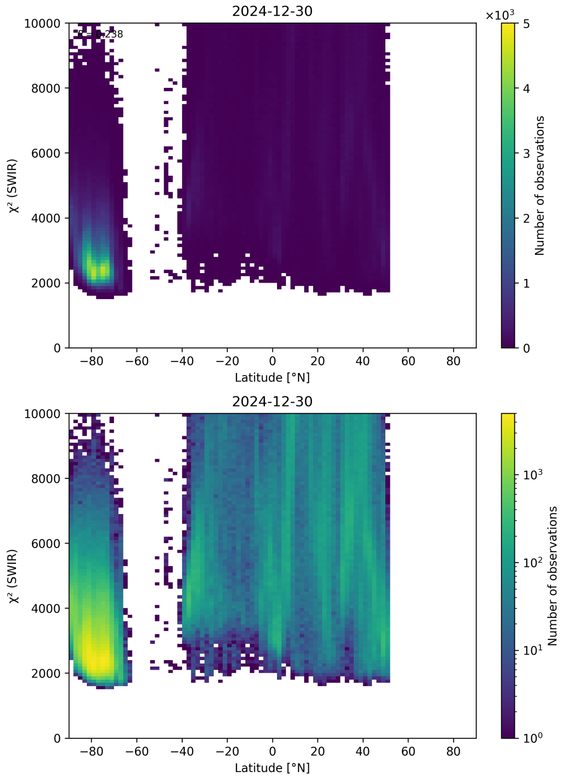
Figure 54: Scatter density plot of “Latitude” against “ \chi^2 (SWIR)” for 2024-12-29 to 2024-12-31.
