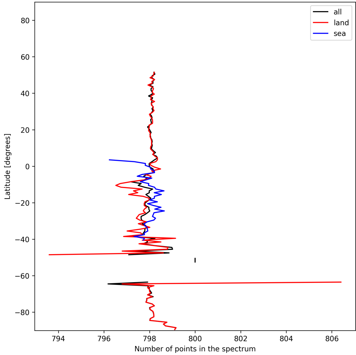
Figure 15: Zonal average of “Number of points in the spectrum” for 2024-12-29 to 2024-12-31.
