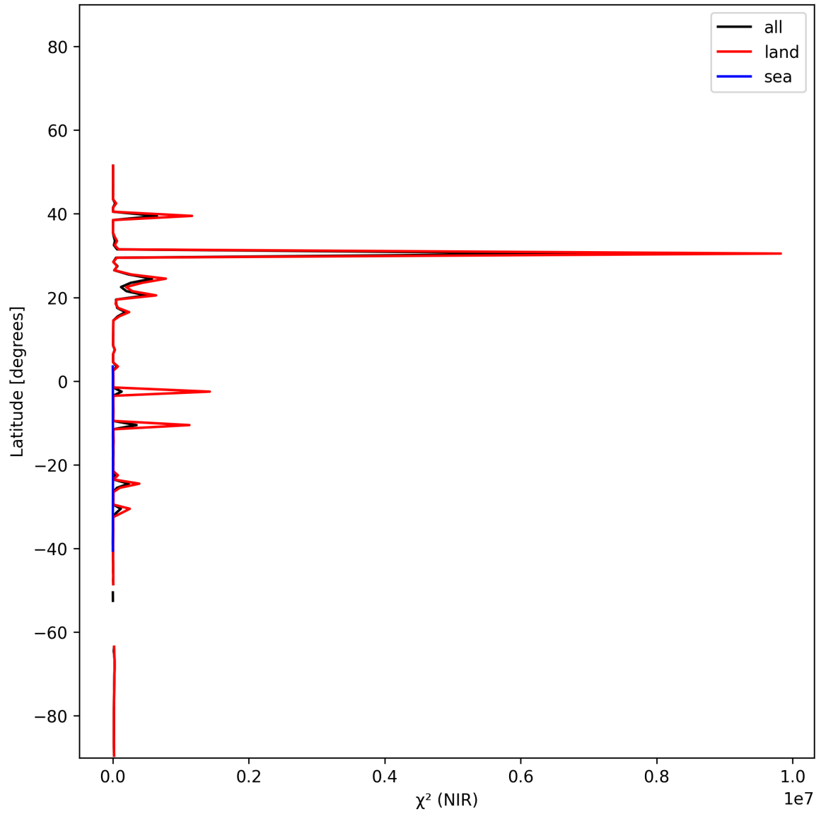
Figure 18: Zonal average of “ \chi^2 (NIR)” for 2024-12-29 to 2024-12-31.
