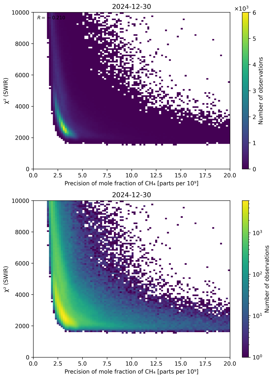
Figure 79: Scatter density plot of “Precision of mole fraction of \text{CH}_4 ” against “ \chi^2 (SWIR)” for 2024-12-29 to 2024-12-31.
