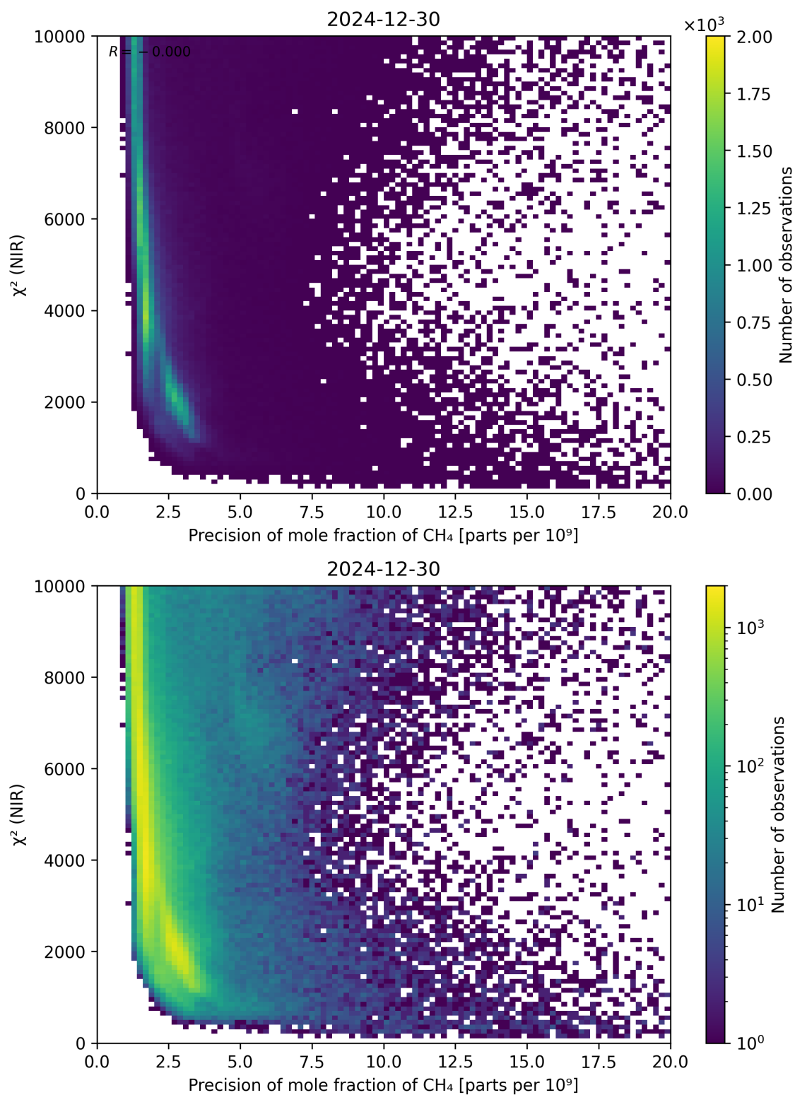
Figure 78: Scatter density plot of “Precision of mole fraction of CH 4 ” against “ \chi^2 (NIR)” for 2024-12-29 to 2024-12-31.
