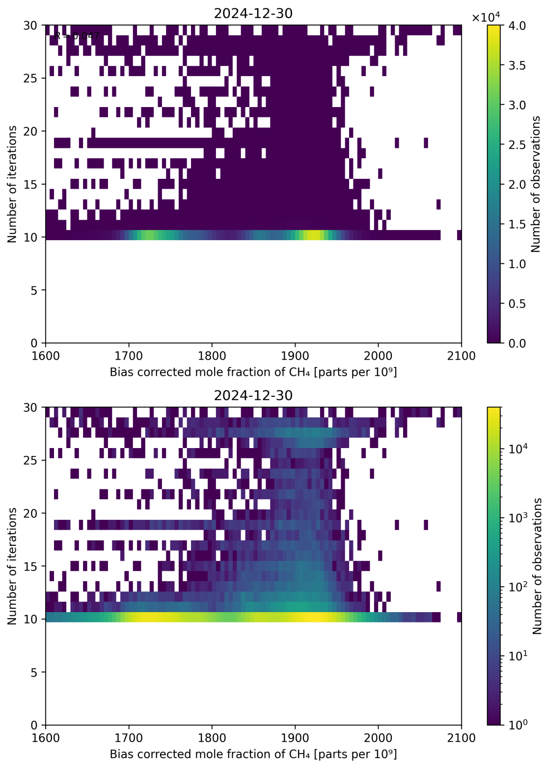
Figure 67: Scatter density plot of “Bias corrected mole fraction of CH 4 ” against “Number of iterations” for 2024-12-29 to 2024-12-31.
