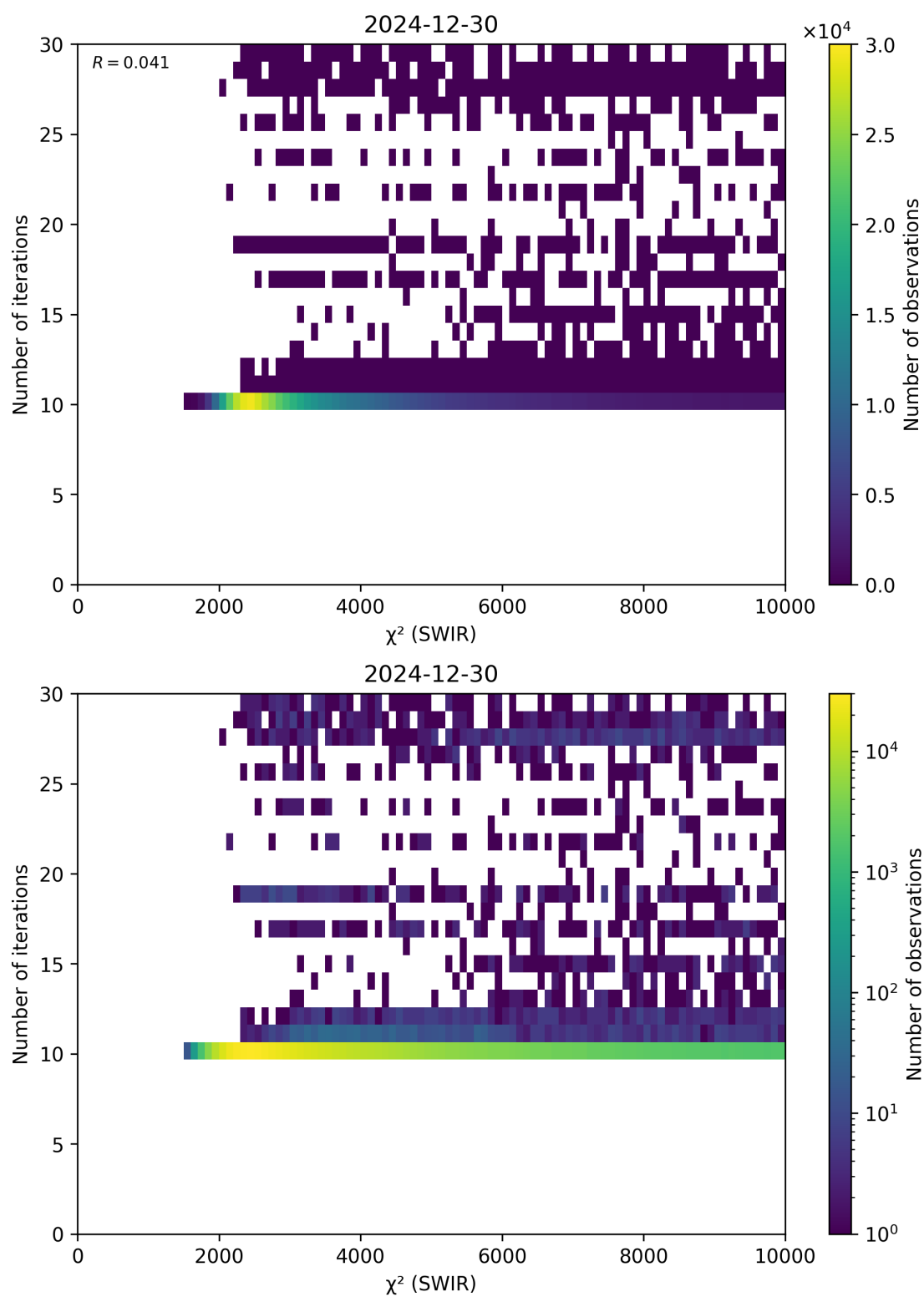
Figure 50: Scatter density plot of “ \chi^2 (SWIR)” against “Number of iterations” for 2024-12-29 to 2024-12-31.
