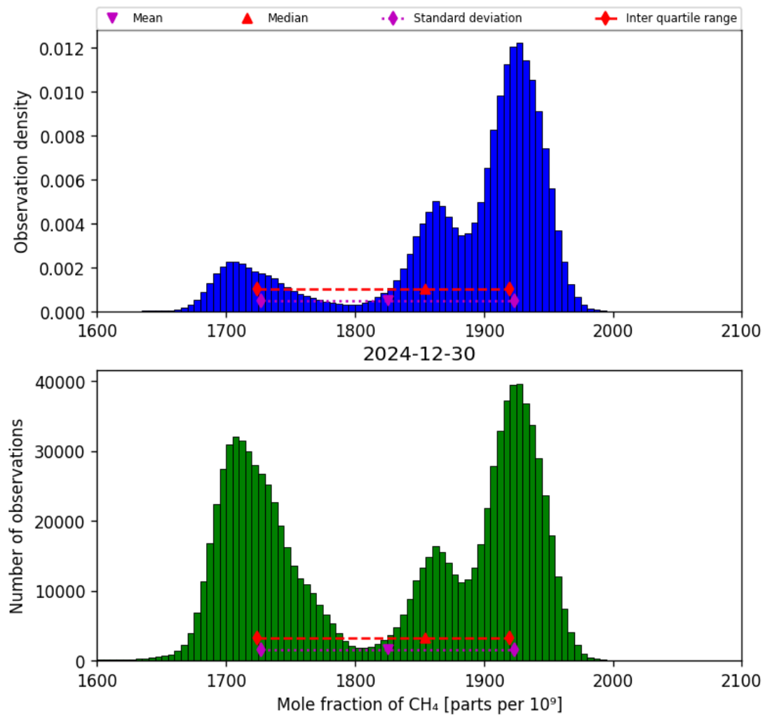
Figure 23: Histogram of “Mole fraction of CH 4 ” for 2024-12-29 to 2024-12-31
