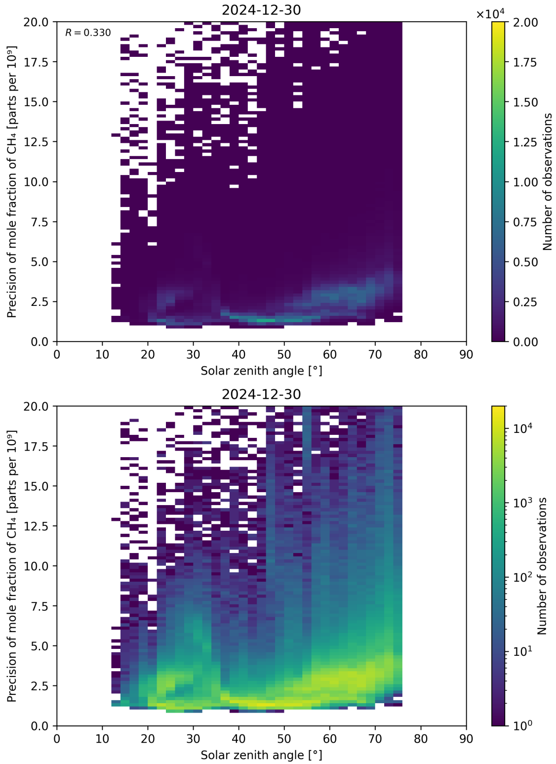
Figure 101: Scatter density plot of “Solar zenith angle” against “Precision of mole fraction of CH 4 ” for 2024-12-29 to 2024-12-31.
