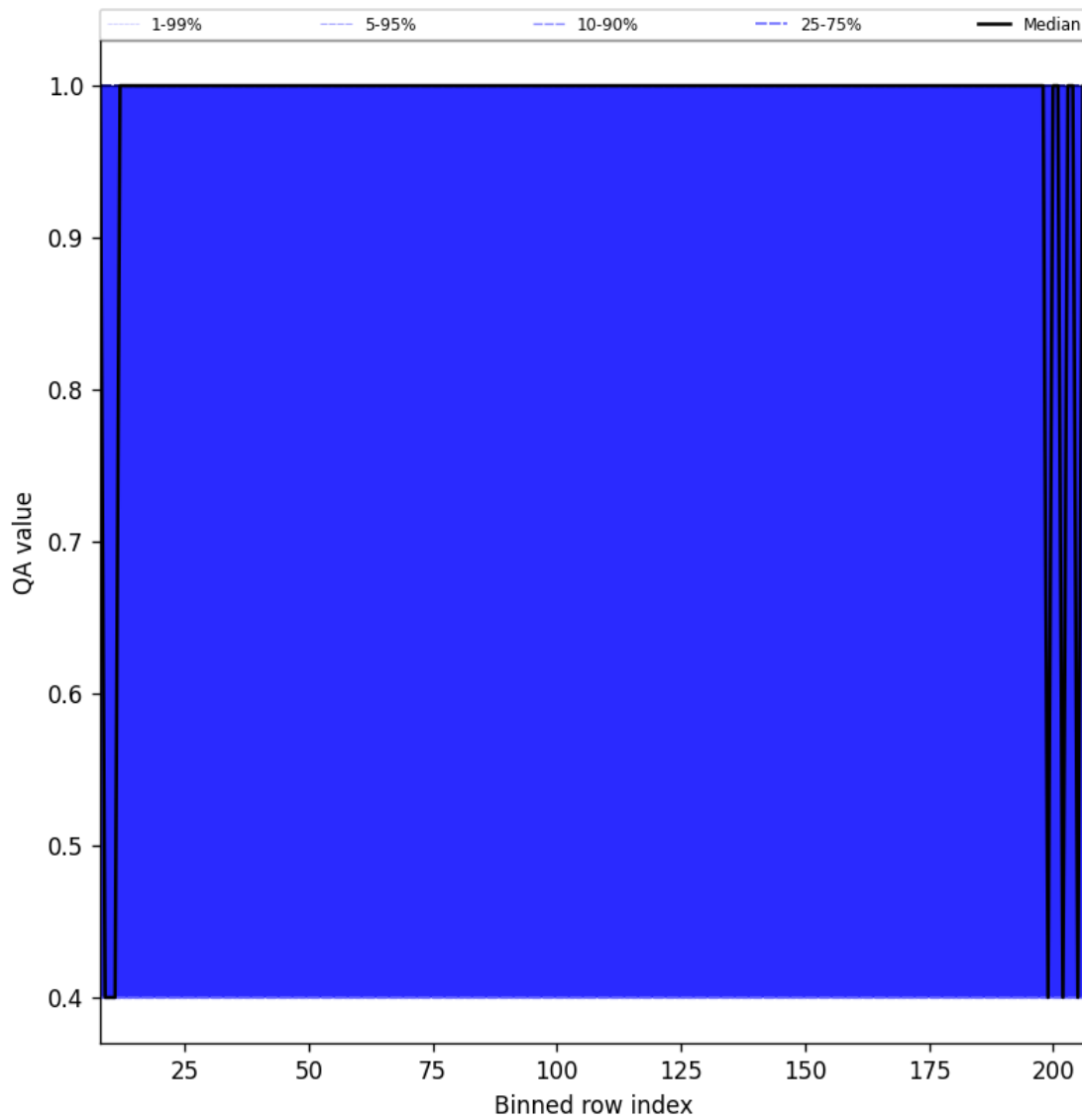
Figure 33: Along track statistics of “QA value” for 2024-12-29 to 2024-12-31
