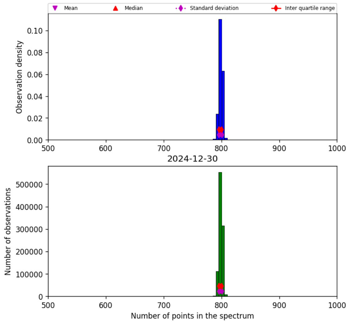
Figure 26: Histogram of “Number of points in the spectrum” for 2024-12-29 to 2024-12-31
