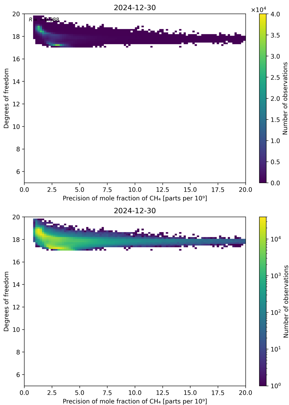
Figure 80: Scatter density plot of “Precision of mole fraction of CH 4 ” against “Degrees of freedom” for 2024-12-29 to 2024-12-31.
