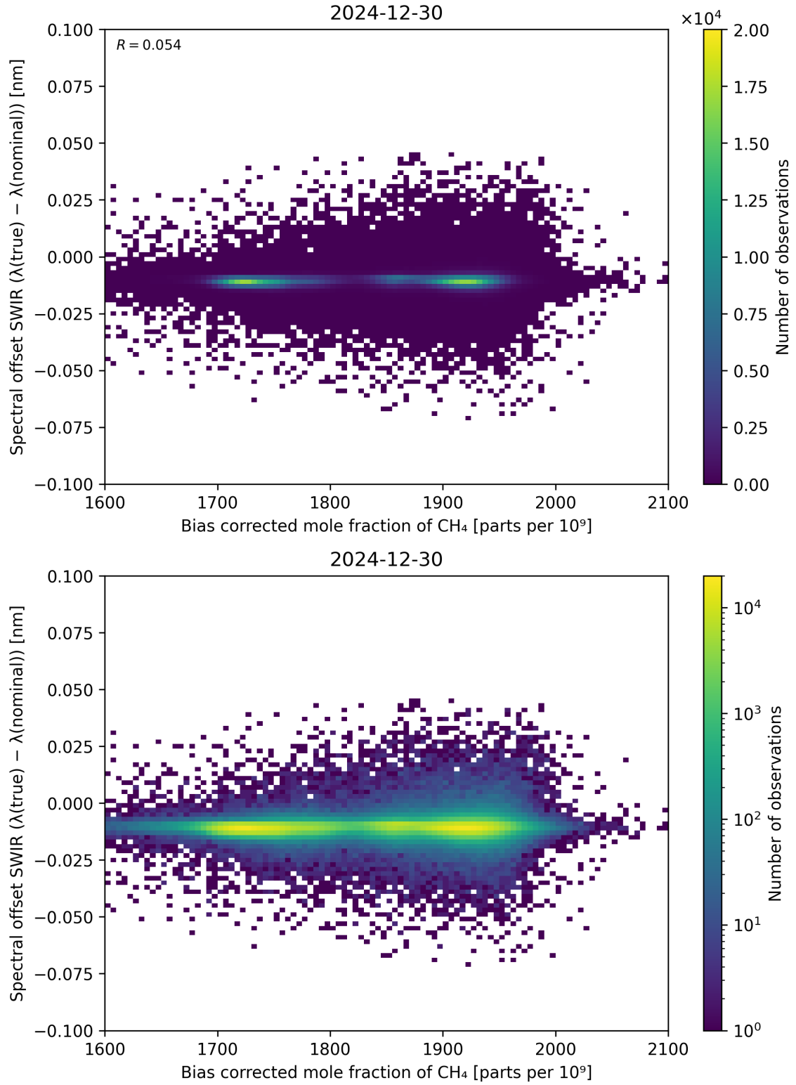
Figure 69: Scatter density plot of “Bias corrected mole fraction of \text{CH}_4 ” against “Spectral offset SWIR ( \lambda_{\text{true}} - \lambda_{\text{nominal}} )” for 2024-12-29 to 2024-12-31.
