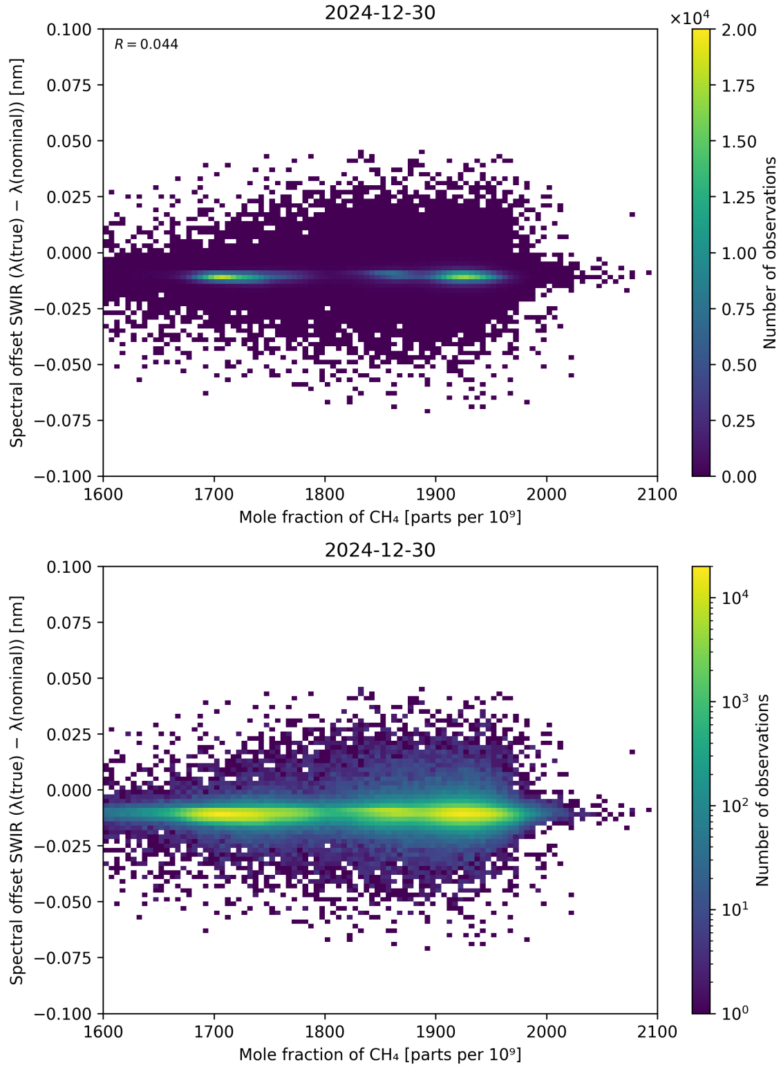
Figure 86: Scatter density plot of “Mole fraction of \text{CH}_4 ” against “Spectral offset SWIR ( \lambda_{\text{true}} - \lambda_{\text{nominal}} )” for 2024-12-29 to 2024-12-31.
