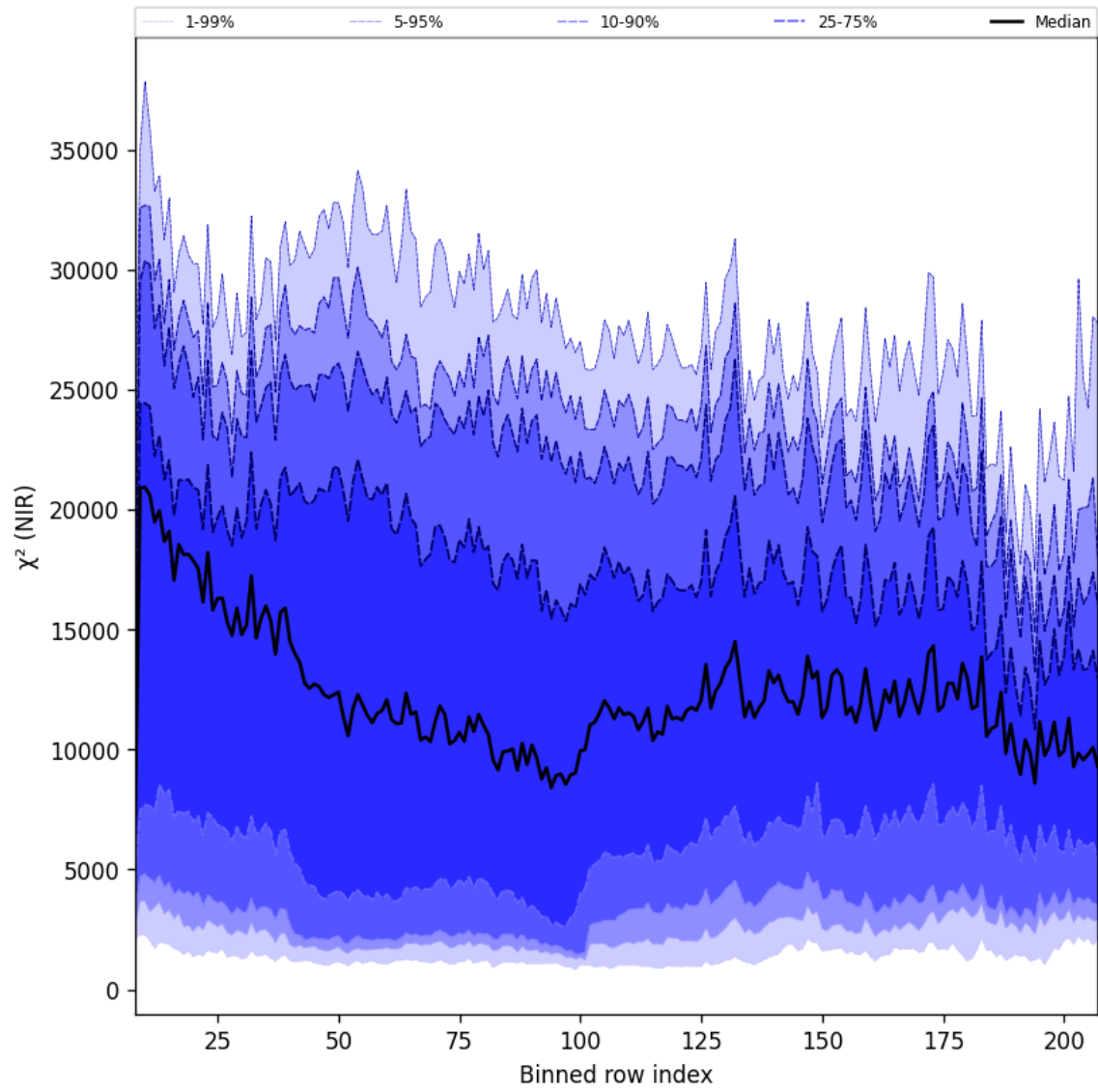
Figure 40: Along track statistics of “ \chi^2 (NIR)” for 2024-12-29 to 2024-12-31
