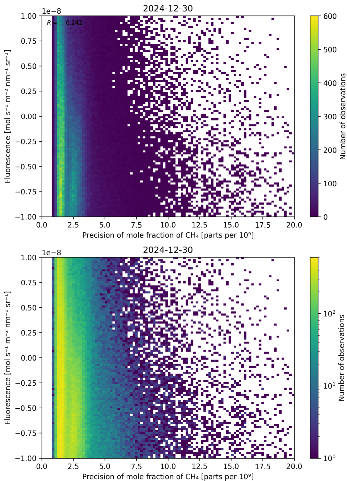
Figure 81: Scatter density plot of “Precision of mole fraction of \text{CH}_4 ” against “Fluorescence” for 2024-12-29 to 2024-12-31.
