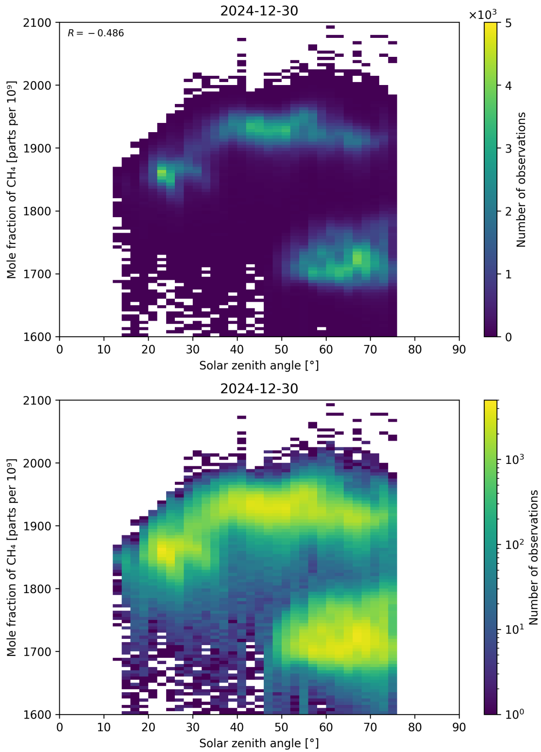
Figure 99: Scatter density plot of “Solar zenith angle” against “Mole fraction of \text{CH}_4 ” for 2024-12-29 to 2024-12-31.
