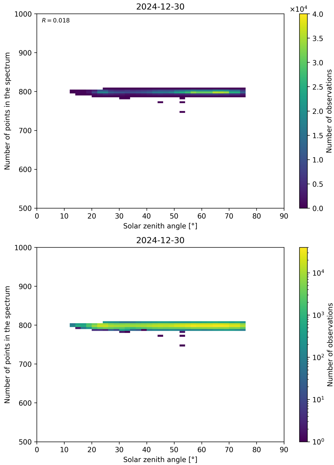
Figure 103: Scatter density plot of “Solar zenith angle” against “Number of points in the spectrum” for 2024-12-29 to 2024-12-31.
