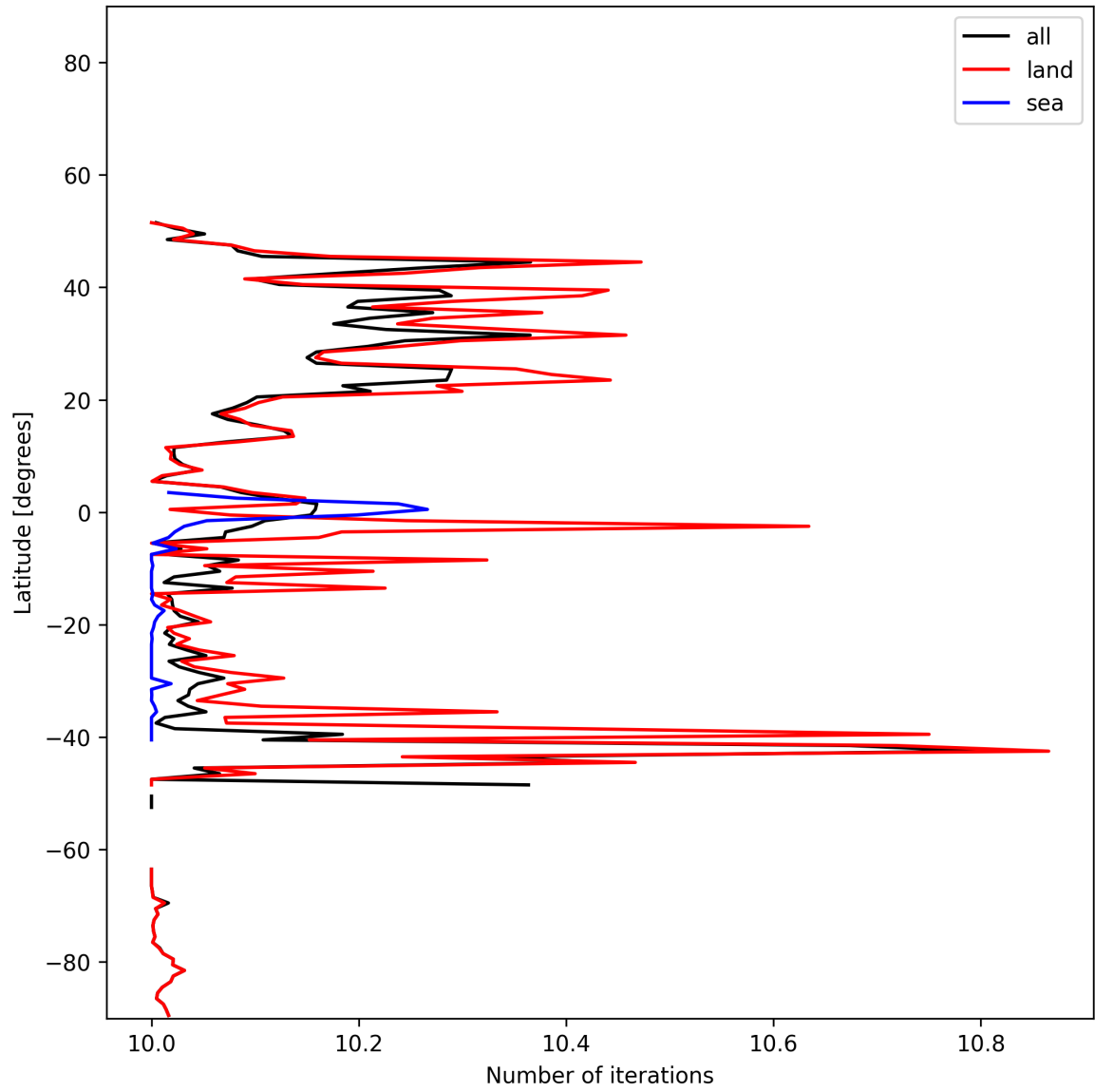
Figure 20: Zonal average of “Number of iterations” for 2024-12-29 to 2024-12-31.
