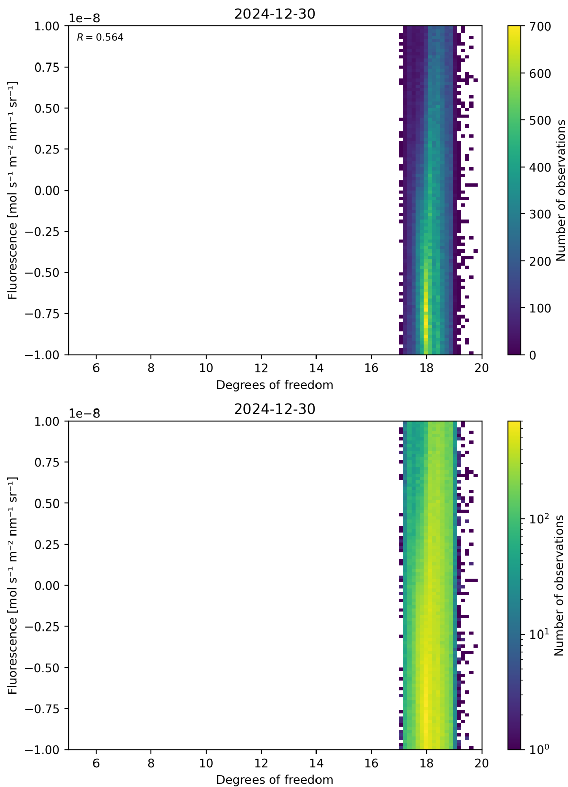
Figure 51: Scatter density plot of “Degrees of freedom” against “Fluorescence” for 2024-12-29 to 2024-12-31.
