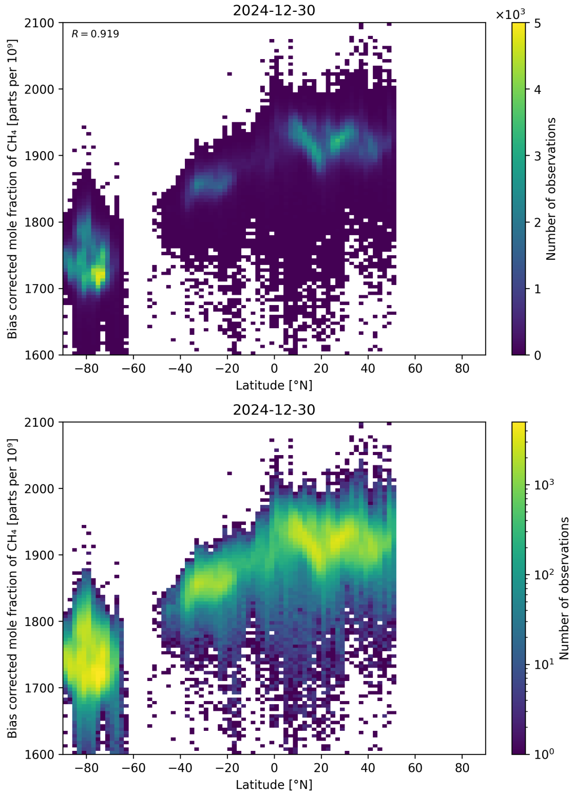
Figure 58: Scatter density plot of “Latitude” against “Bias corrected mole fraction of \text{CH}_4 ” for 2024-12-29 to 2024-12-31.
