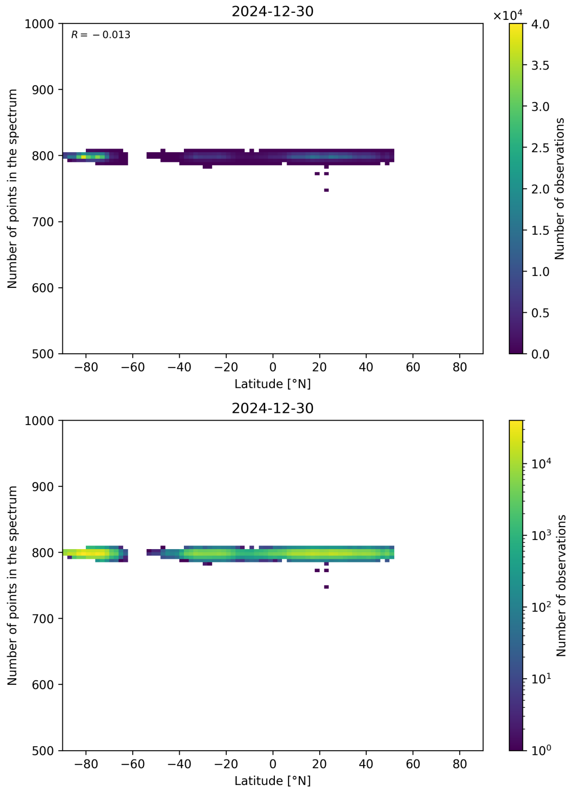
Figure 61: Scatter density plot of “Latitude” against “Number of points in the spectrum” for 2024-12-29 to 2024-12-31.
