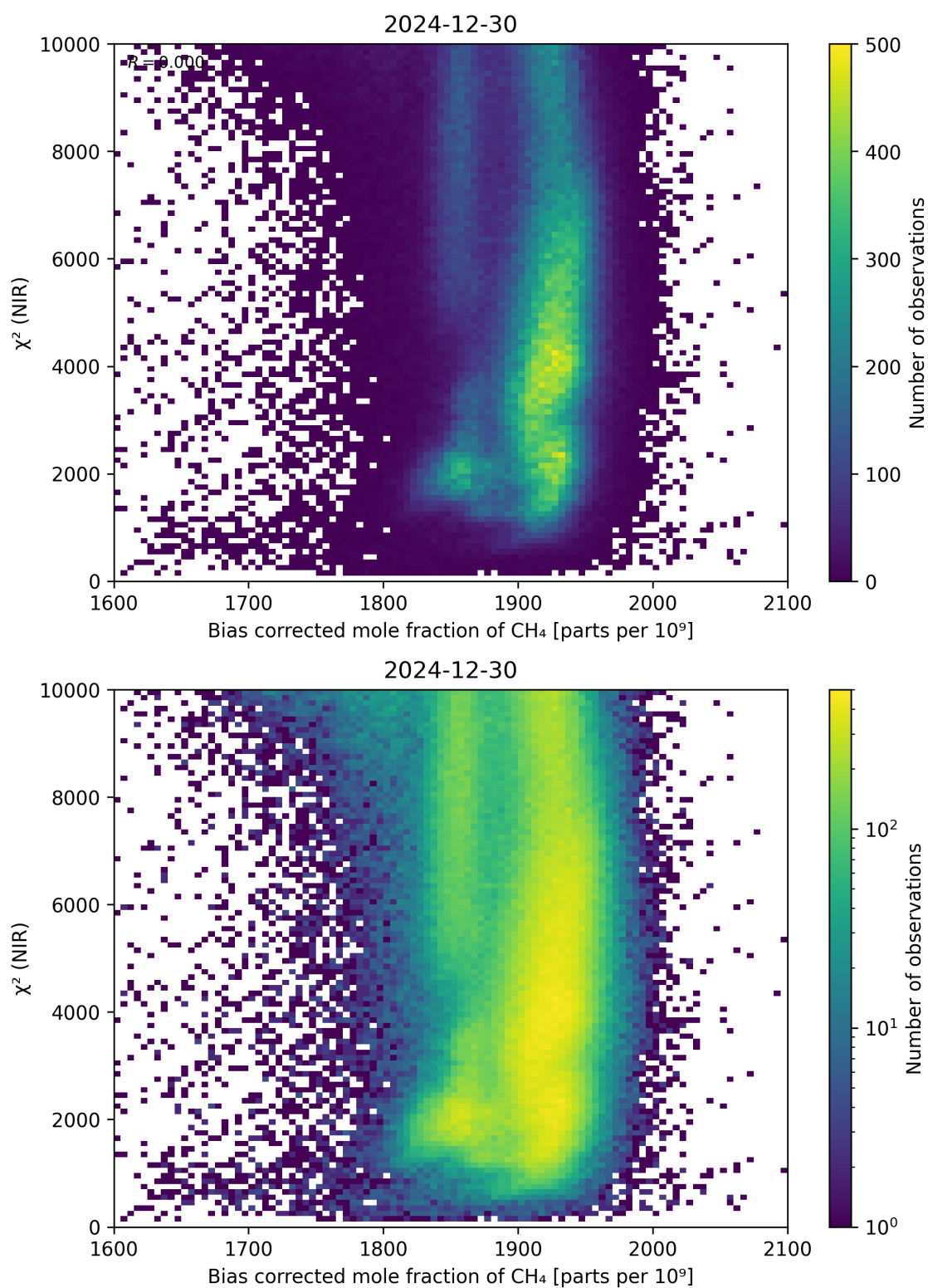
Figure 63: Scatter density plot of “Bias corrected mole fraction of \text{CH}_4 ” against “ \chi^2 (NIR)” for 2024-12-29 to 2024-12-31.
