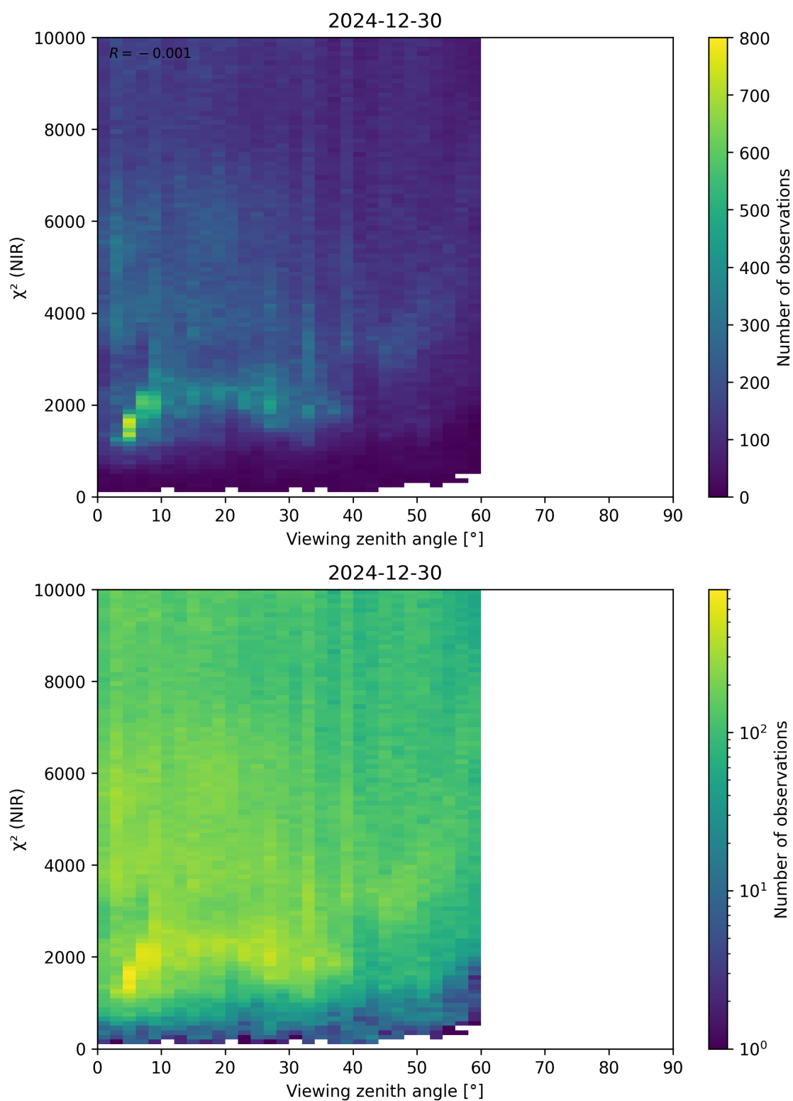
Figure 105: Scatter density plot of “Viewing zenith angle” against “ \chi^2 (NIR)” for 2024-12-29 to 2024-12-31.
