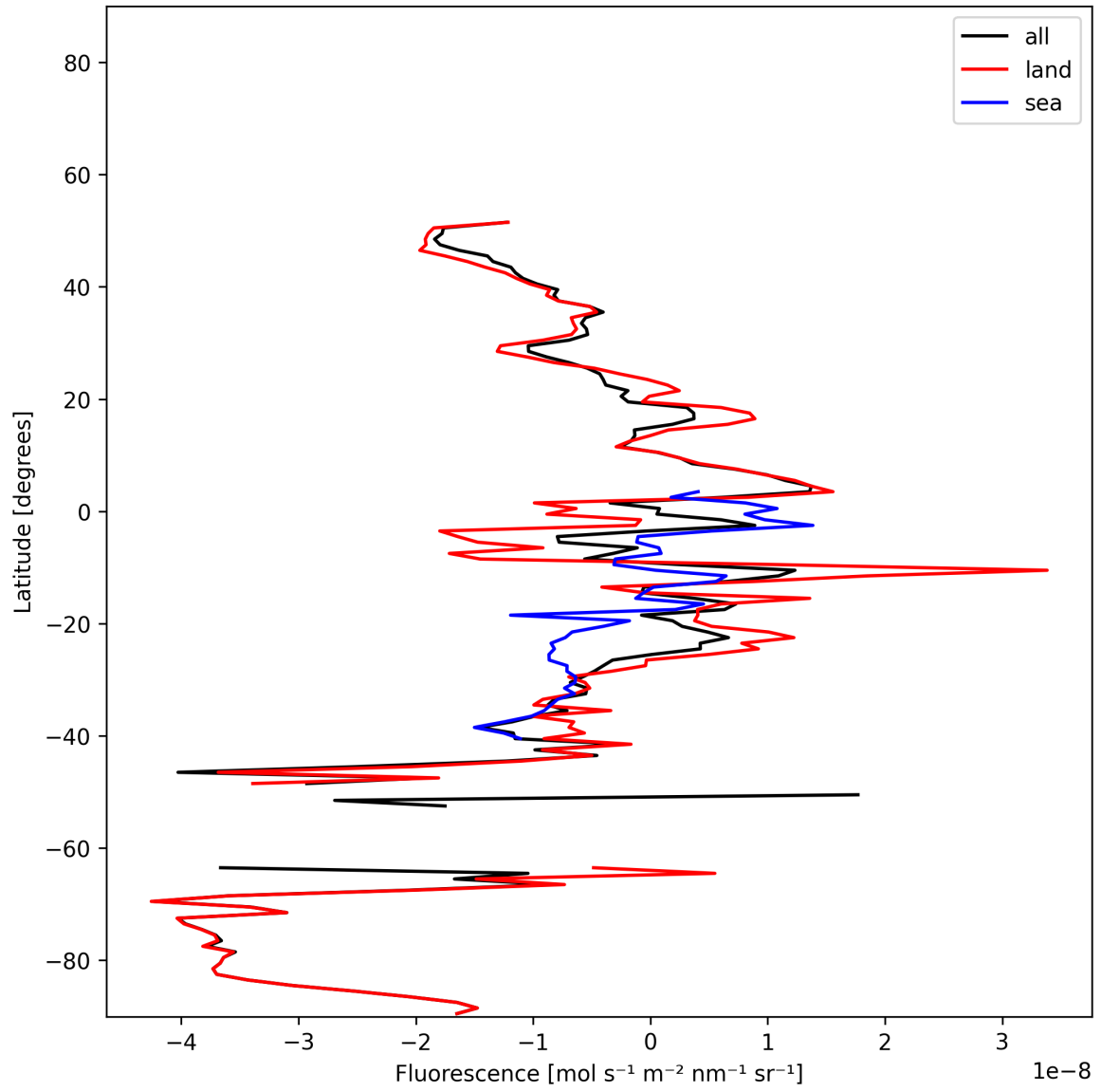
Figure 21: Zonal average of “Fluorescence” for 2024-12-29 to 2024-12-31.
