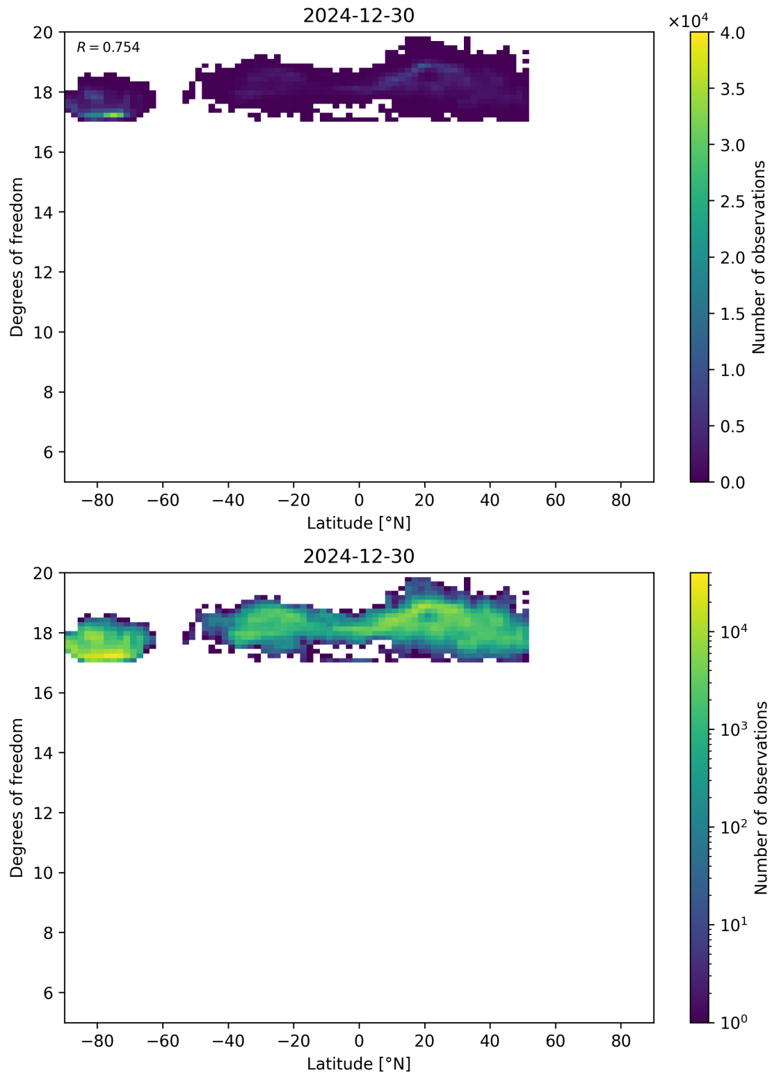
Figure 55: Scatter density plot of “Latitude” against “Degrees of freedom” for 2024-12-29 to 2024-12-31.
