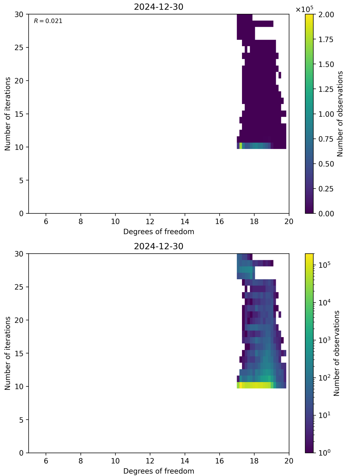
Figure 52: Scatter density plot of “Degrees of freedom” against “Number of iterations” for 2024-12-29 to 2024-12-31.
