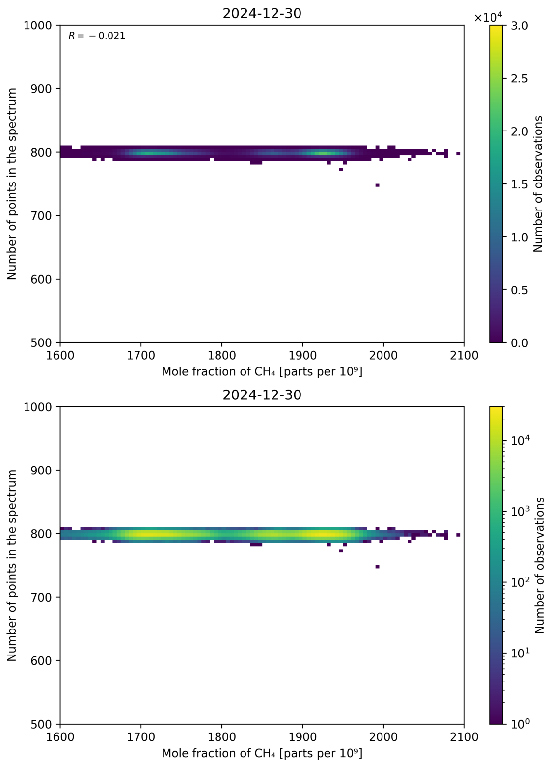
Figure 77: Scatter density plot of “Mole fraction of CH 4 ” against “Number of points in the spectrum” for 2024-12-29 to 2024-12-31.
