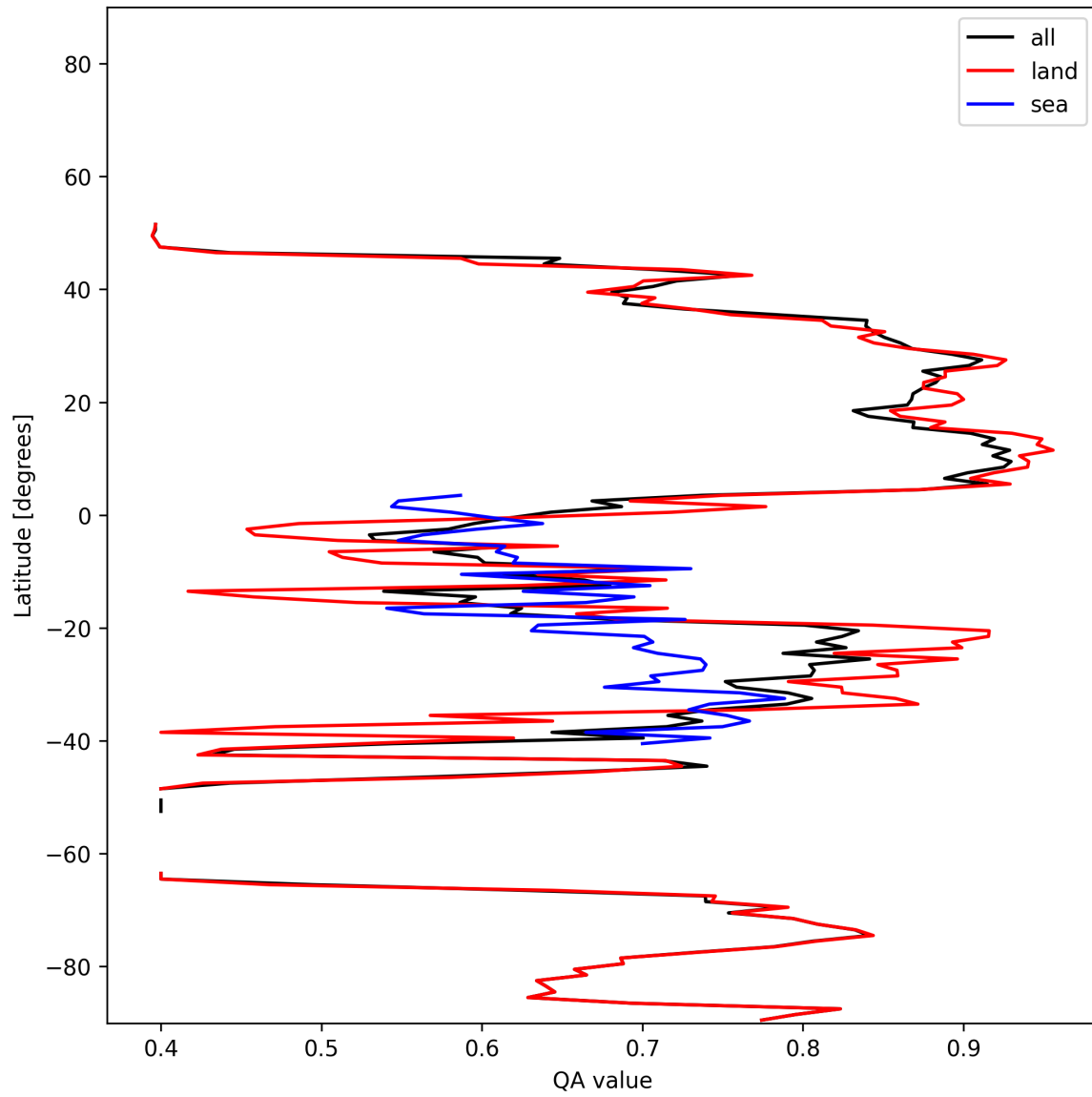
Figure 11: Zonal average of “QA value” for 2024-12-29 to 2024-12-31.
