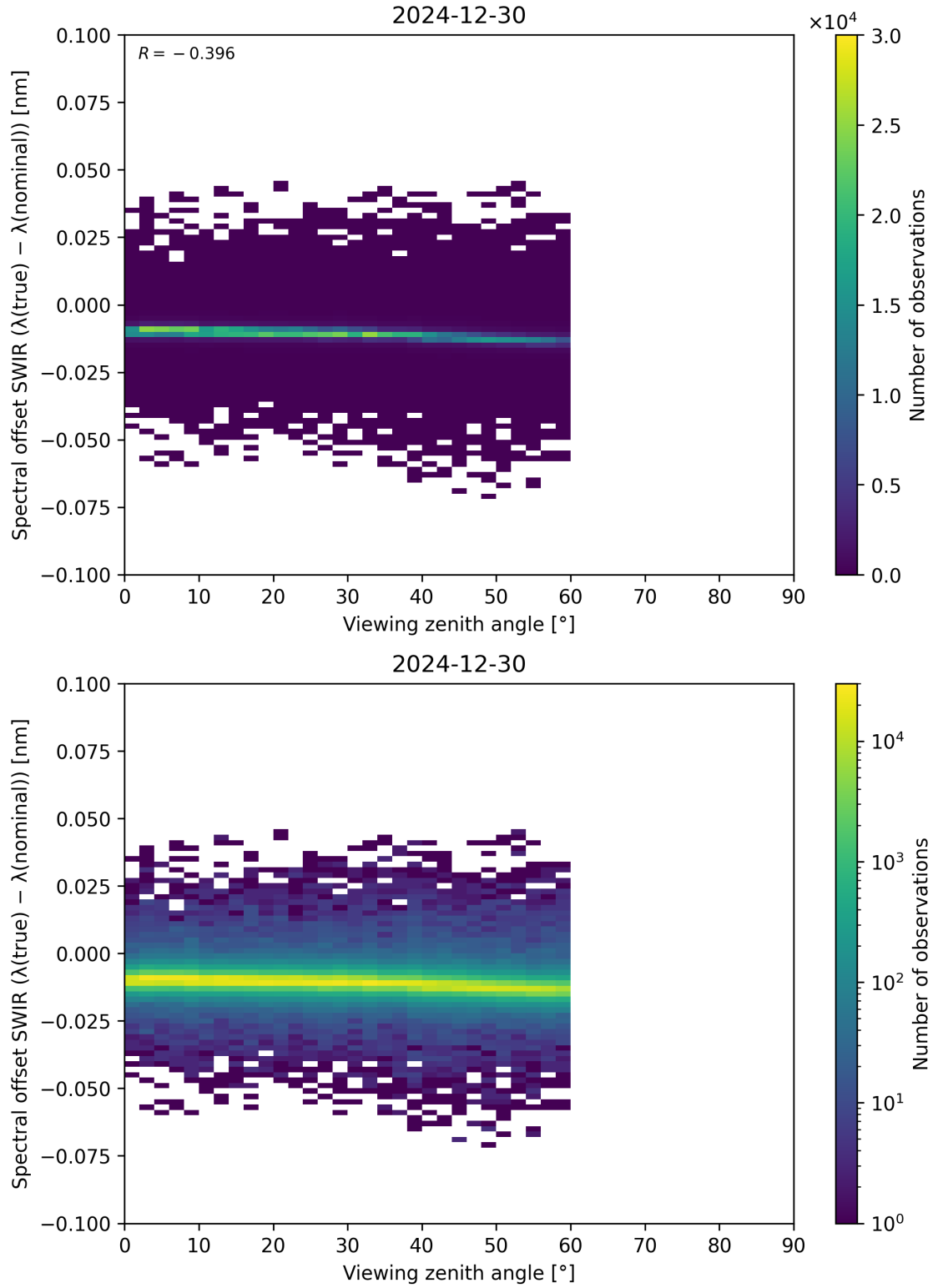
Figure 116: Scatter density plot of “Viewing zenith angle” against “Spectral offset SWIR ( \lambda_{\text{true}} - \lambda_{\text{nominal}} )” for 2024-12-29 to 2024-12-31.
