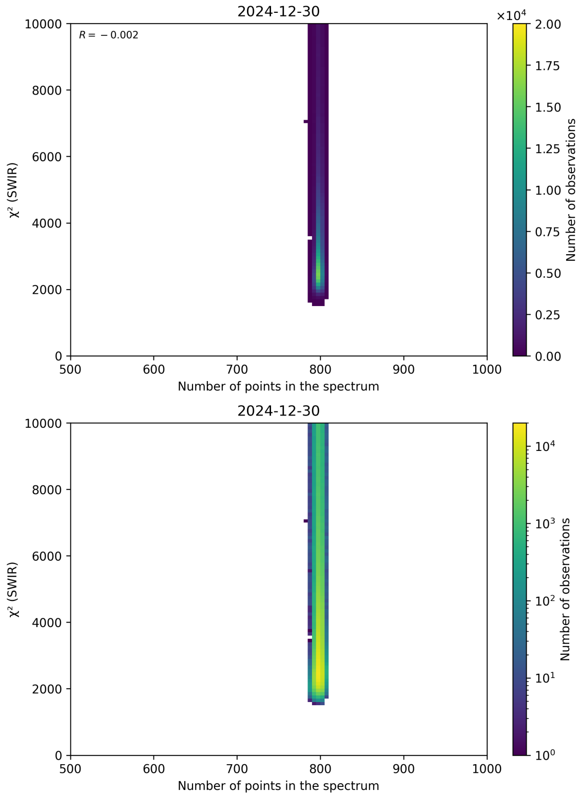
Figure 89: Scatter density plot of “Number of points in the spectrum” against “ \chi^2 (SWIR)” for 2024-12-29 to 2024-12-31.
