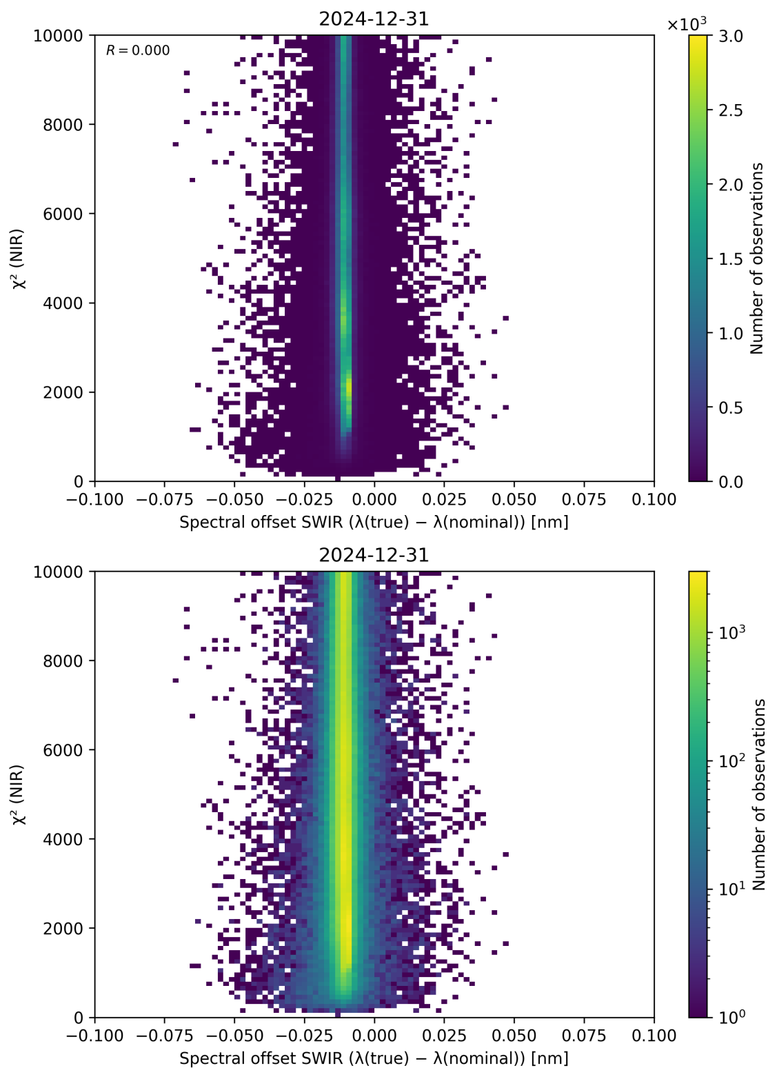
Figure 117: Scatter density plot of “Spectral offset SWIR ( \lambda_{\text{true}} - \lambda_{\text{nominal}} )” against “ \chi^2 (NIR)” for 2024-12-30 to 2025-01-01.
