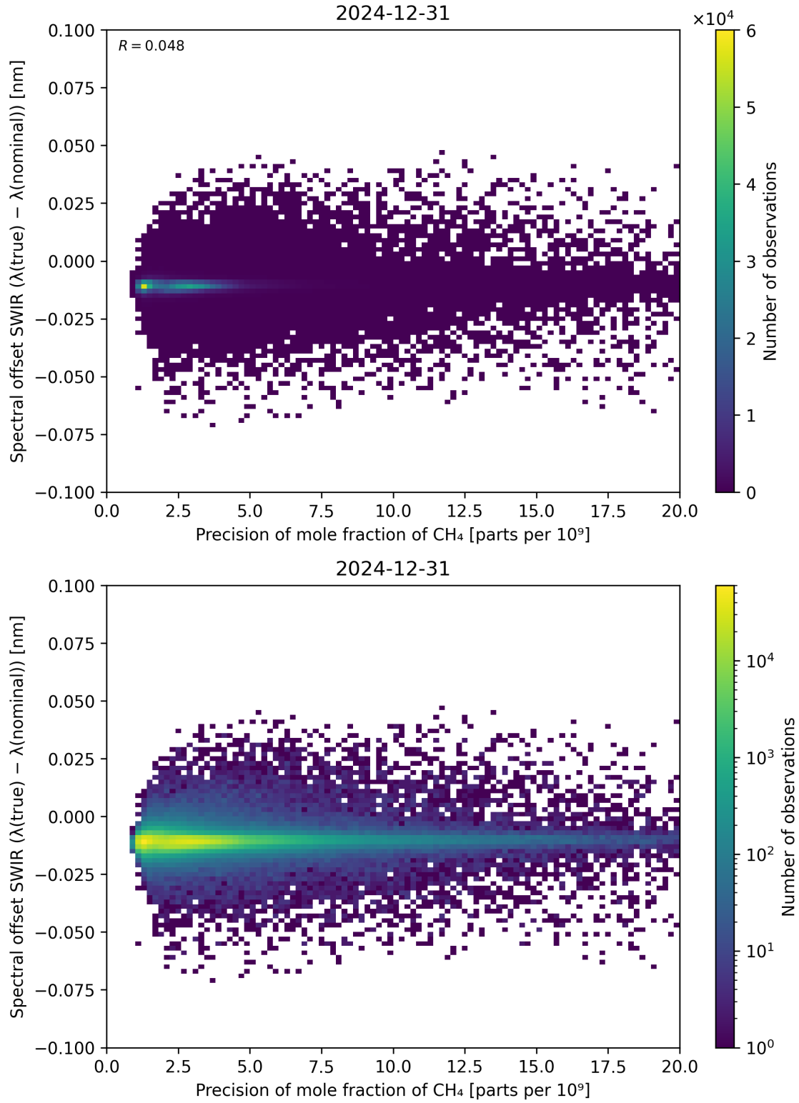
Figure 85: Scatter density plot of “Precision of mole fraction of \text{CH}_4 ” against “Spectral offset SWIR ( \lambda_{\text{true}} - \lambda_{\text{nominal}} )” for 2024-12-30 to 2025-01-01.
