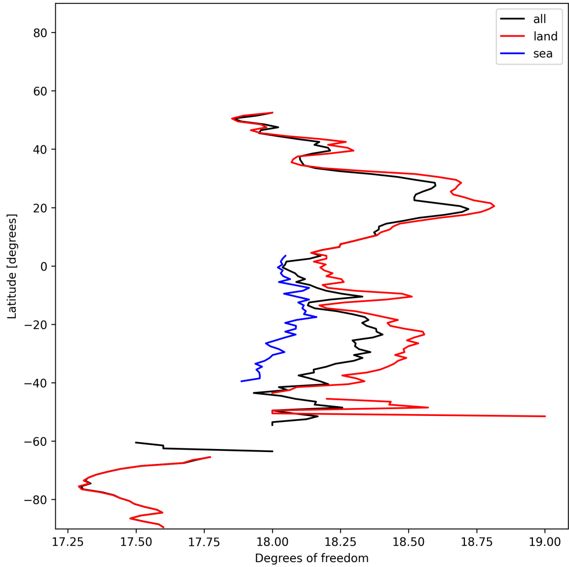
Figure 19: Zonal average of “Degrees of freedom” for 2024-12-30 to 2025-01-01.
