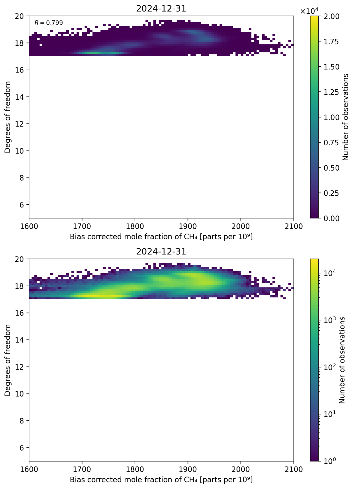
Figure 65: Scatter density plot of “Bias corrected mole fraction of CH 4 ” against “Degrees of freedom” for 2024-12-30 to 2025-01-01.
