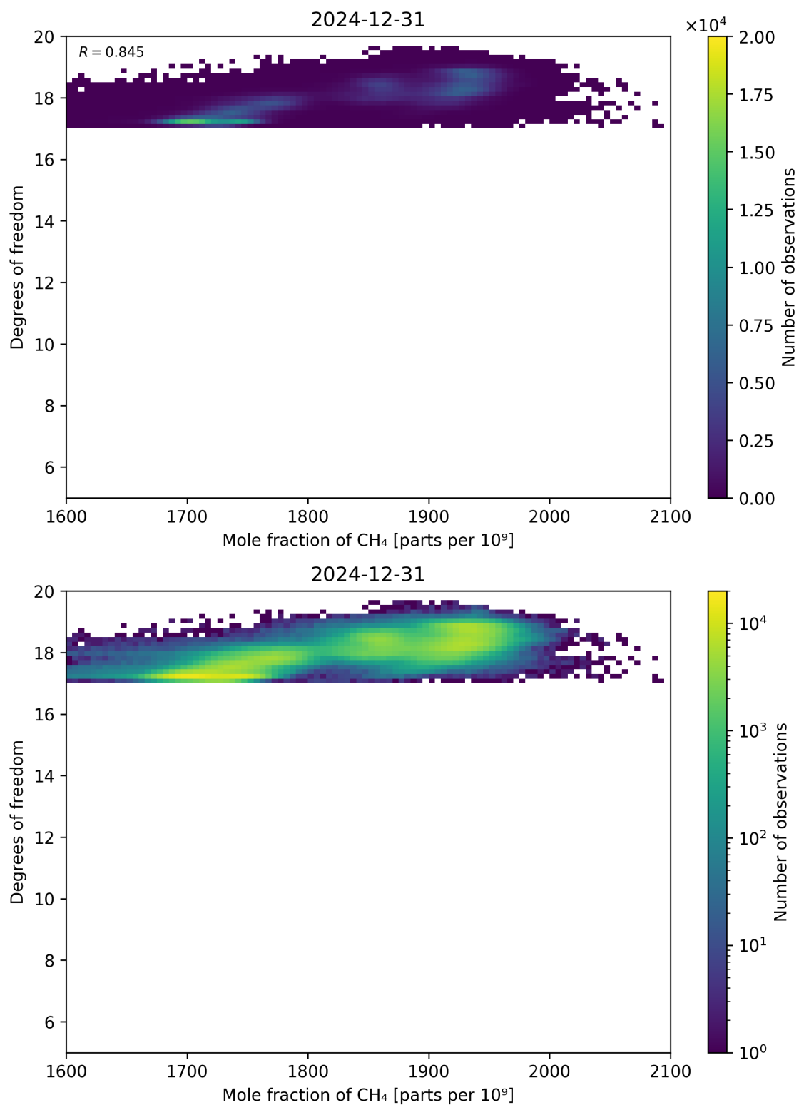
Figure 72: Scatter density plot of “Mole fraction of CH 4 ” against “Degrees of freedom” for 2024-12-30 to 2025-01-01.
