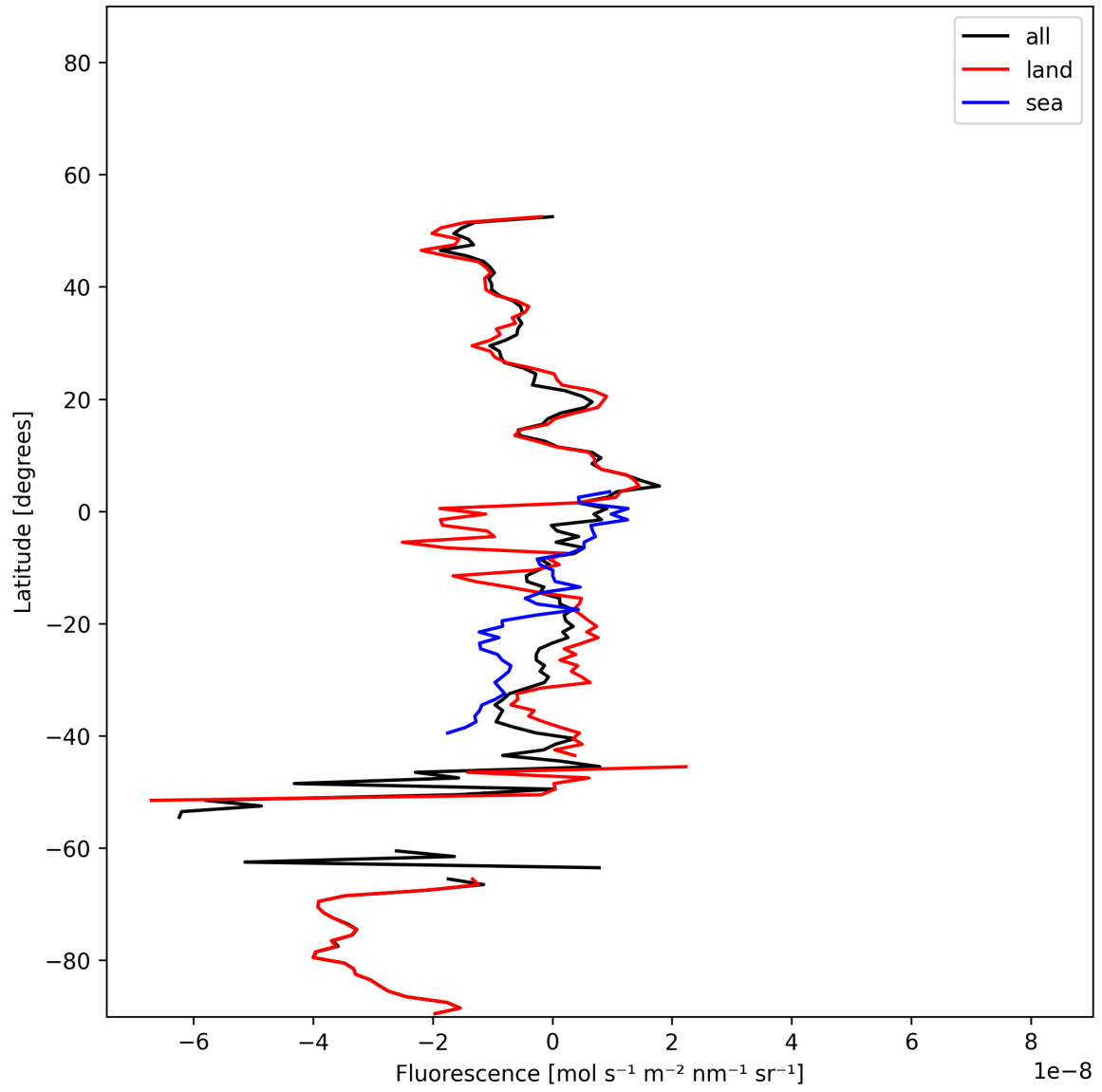
Figure 21: Zonal average of “Fluorescence” for 2024-12-30 to 2025-01-01.
