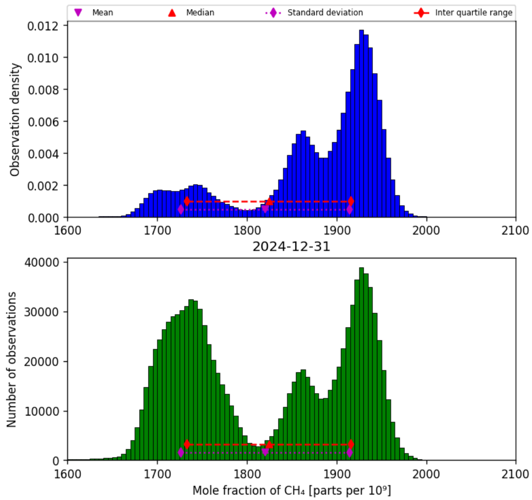
Figure 23: Histogram of “Mole fraction of CH 4 ” for 2024-12-30 to 2025-01-01
