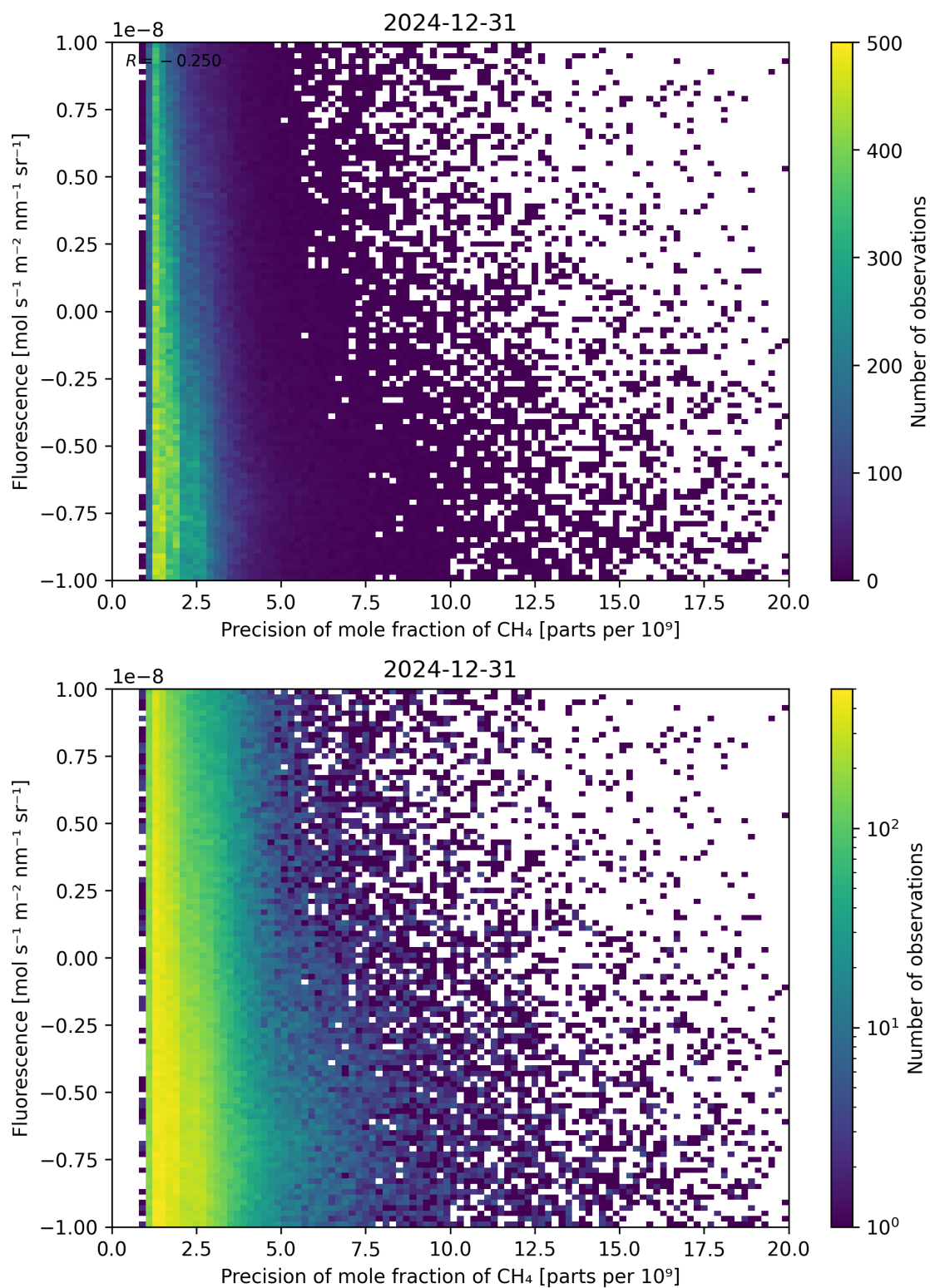
Figure 81: Scatter density plot of “Precision of mole fraction of CH 4 ” against “Fluorescence” for 2024-12-30 to 2025-01-01.
