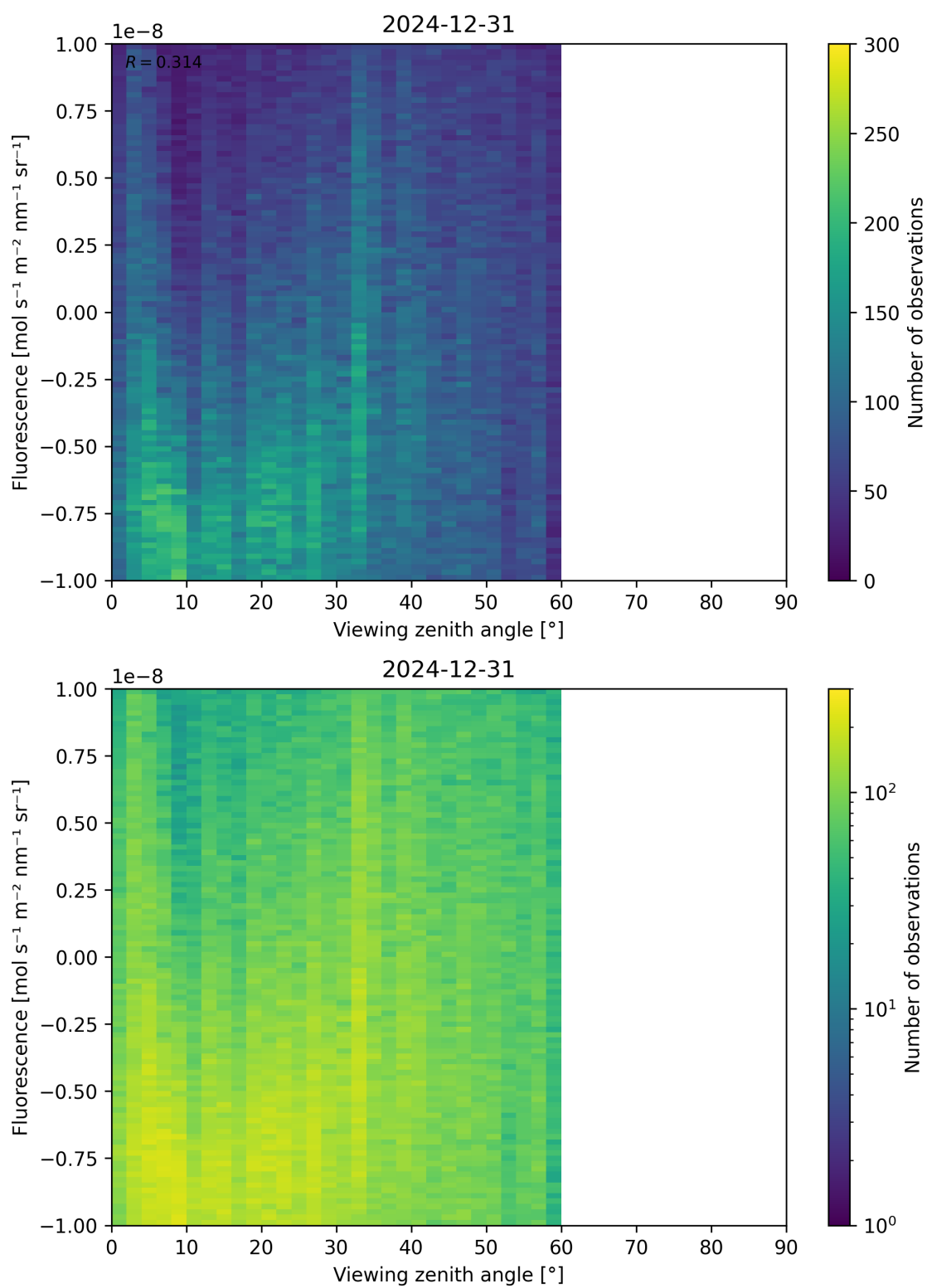
Figure 108: Scatter density plot of “Viewing zenith angle” against “Fluorescence” for 2024-12-30 to 2025-01-01.
