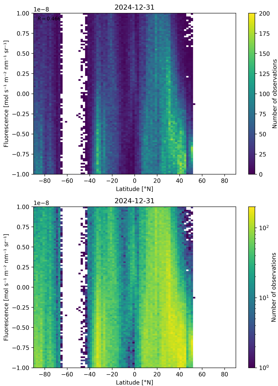
Figure 56: Scatter density plot of “Latitude” against “Fluorescence” for 2024-12-30 to 2025-01-01.
