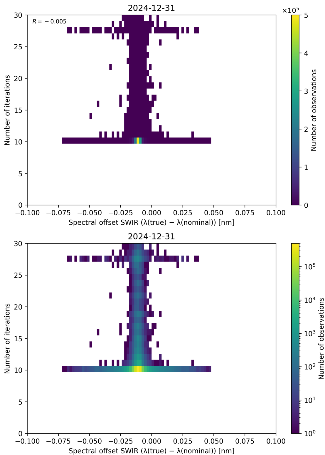
Figure 121: Scatter density plot of “Spectral offset SWIR ( \lambda_{\text{true}} - \lambda_{\text{nominal}} )” against “Number of iterations” for 2024-12-30 to 2025-01-01.
