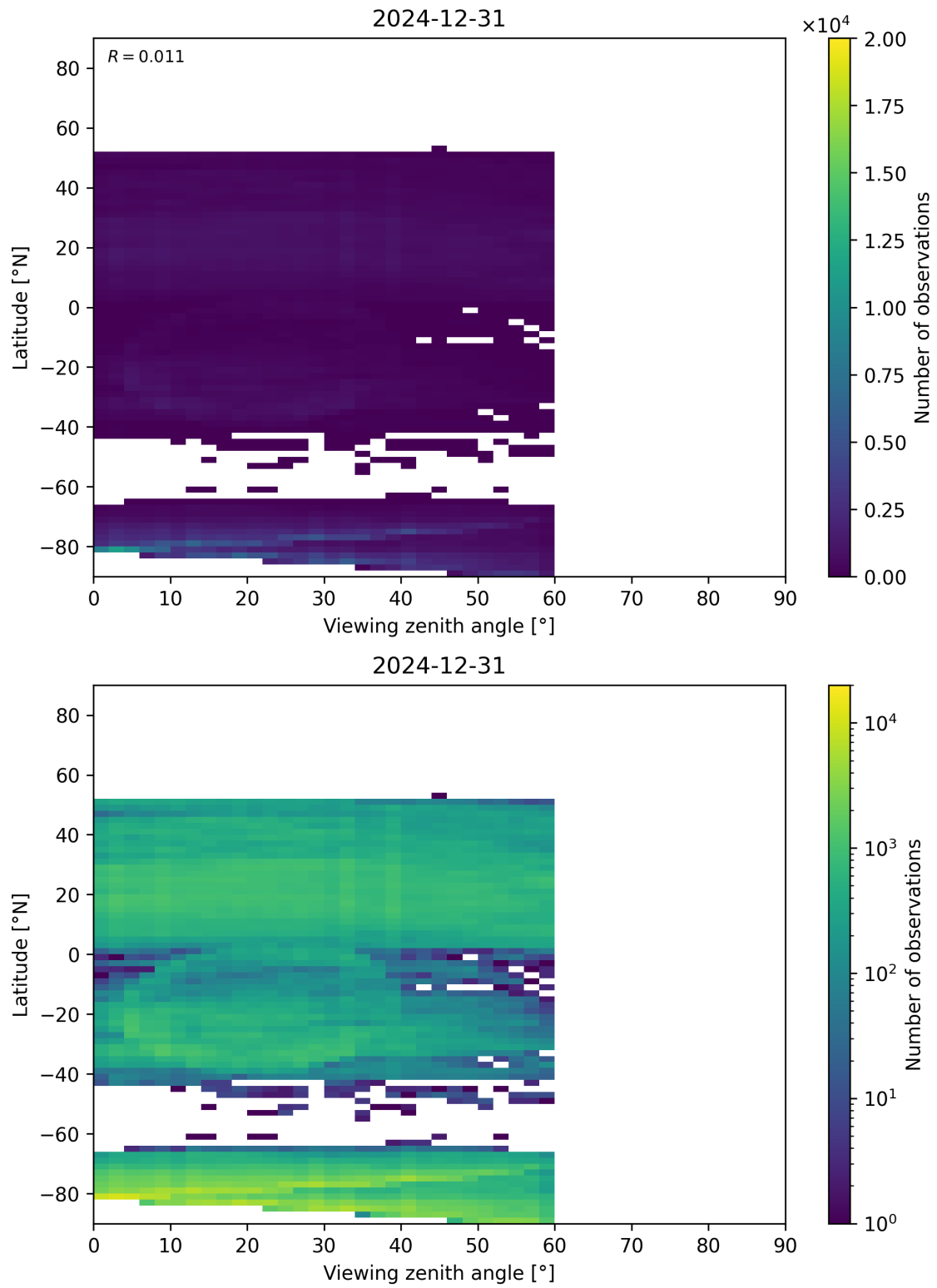
Figure 109: Scatter density plot of “Viewing zenith angle” against “Latitude” for 2024-12-30 to 2025-01-01.
