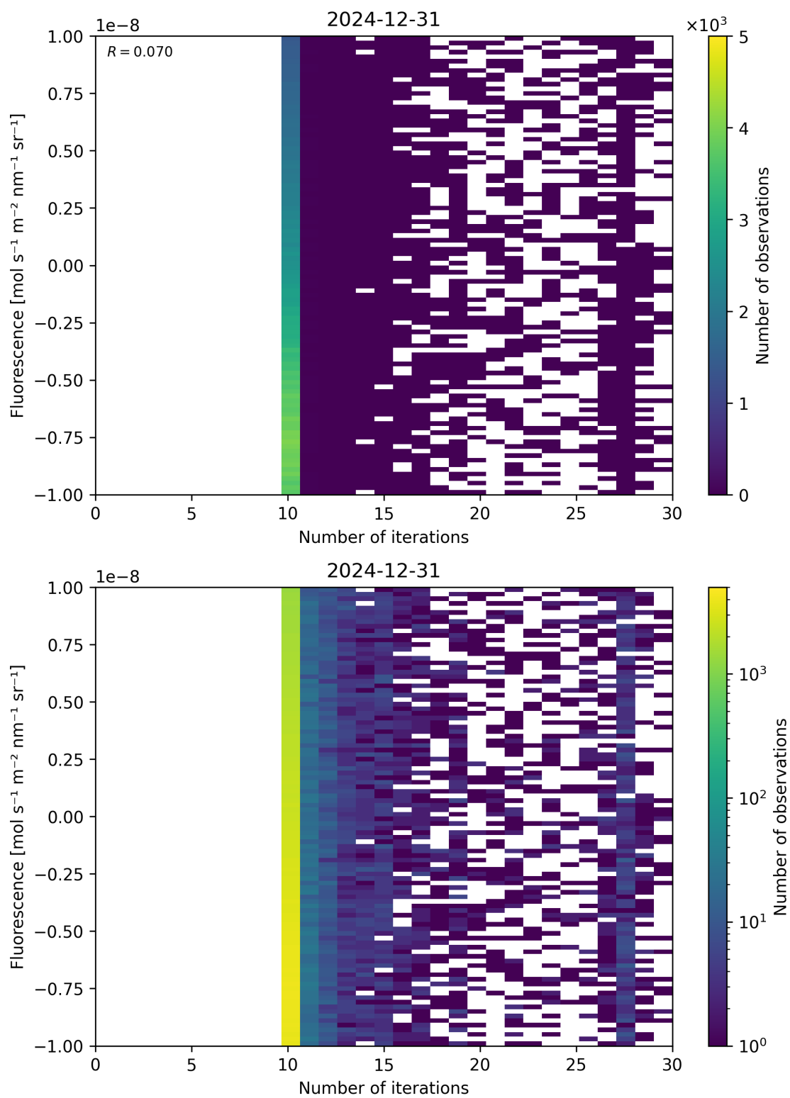
Figure 87: Scatter density plot of “Number of iterations” against “Fluorescence” for 2024-12-30 to 2025-01-01.
