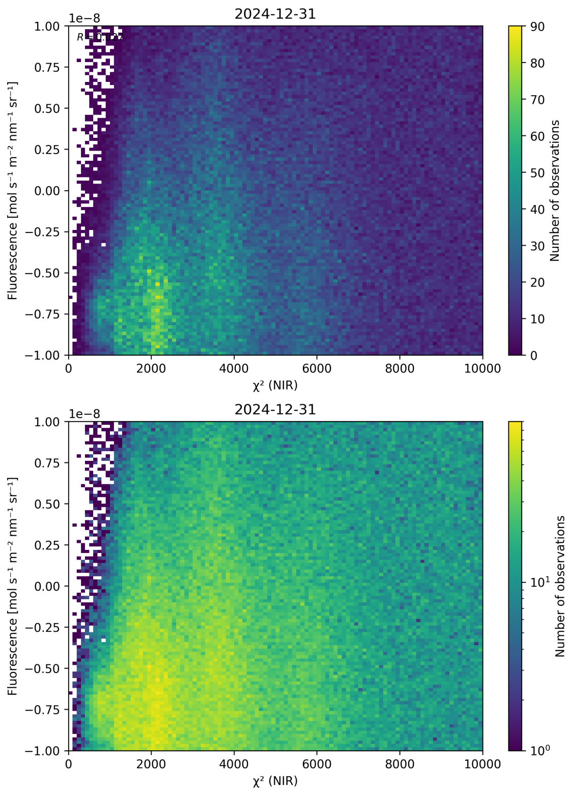
Figure 45: Scatter density plot of “ \chi^2 (NIR)” against “Fluorescence” for 2024-12-30 to 2025-01-01.
