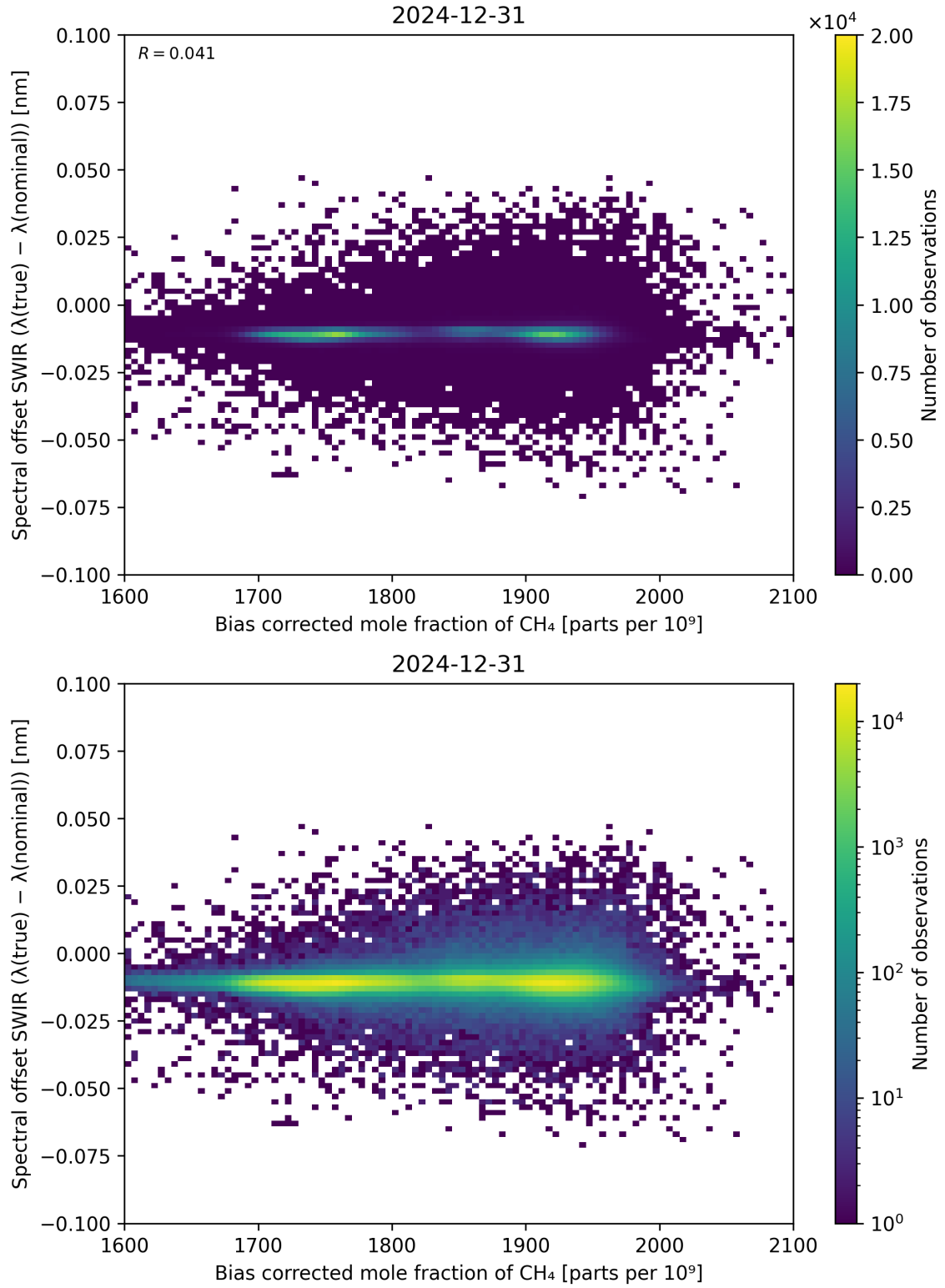
Figure 69: Scatter density plot of “Bias corrected mole fraction of \text{CH}_4 ” against “Spectral offset SWIR ( \lambda_{\text{true}} - \lambda_{\text{nominal}} )” for 2024-12-30 to 2025-01-01.
