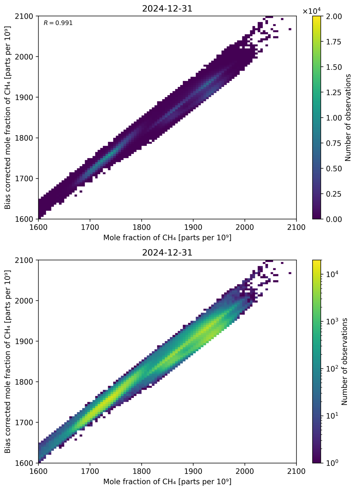
Figure 74: Scatter density plot of “Mole fraction of CH 4 ” against “Bias corrected mole fraction of CH 4 ” for 2024-12-30 to 2025-01-01.
