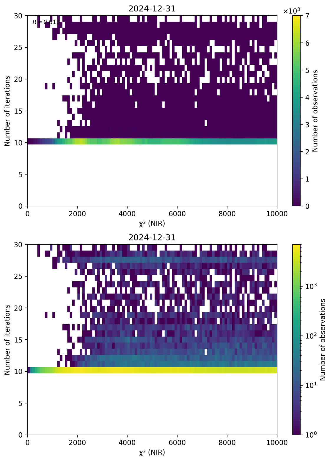
Figure 46: Scatter density plot of “ \chi^2 (NIR)” against “Number of iterations” for 2024-12-30 to 2025-01-01.
