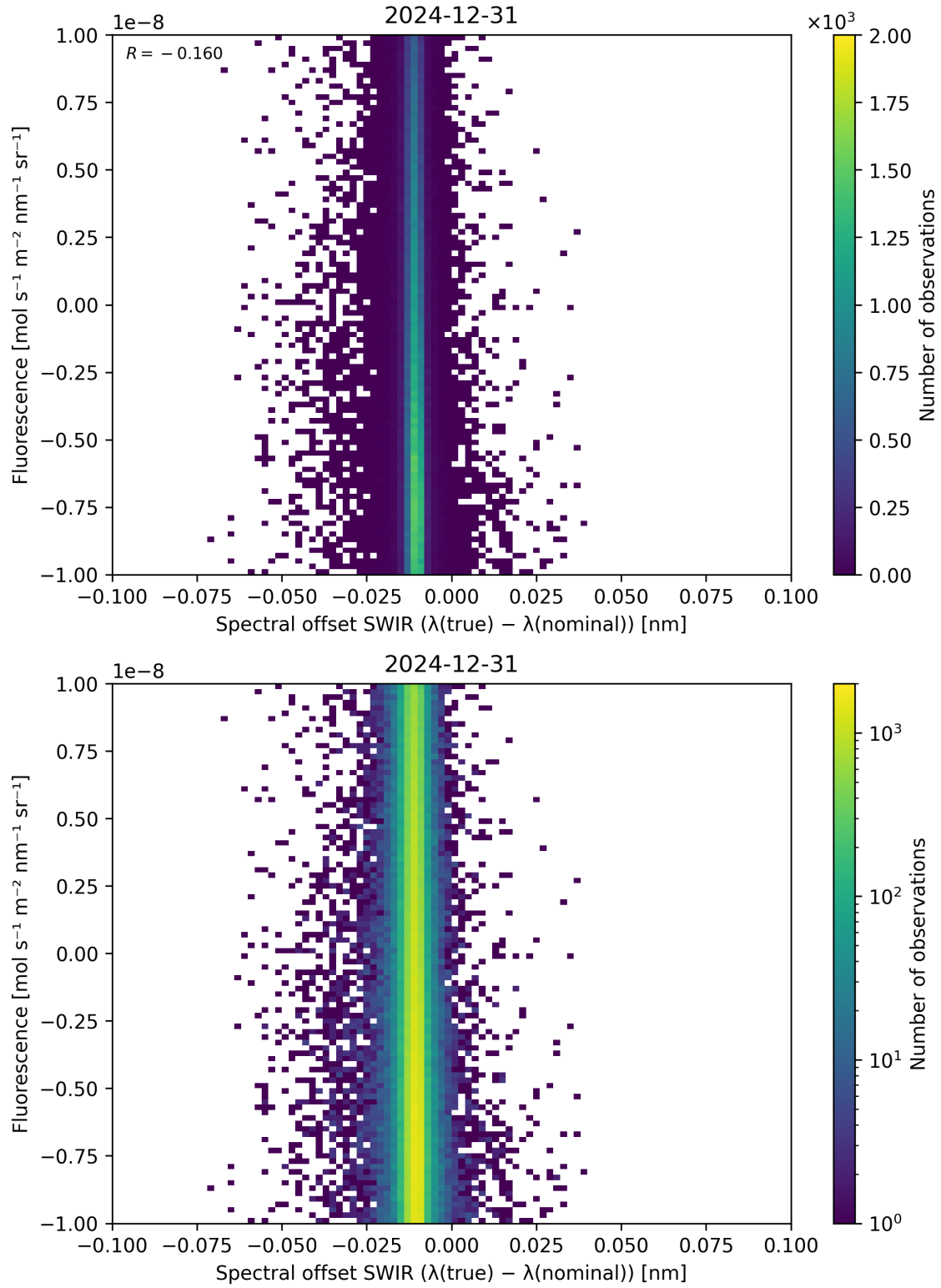
Figure 120: Scatter density plot of “Spectral offset SWIR ( \lambda_{\text{true}} - \lambda_{\text{nominal}} )” against “Fluorescence” for 2024-12-30 to 2025-01-01.
