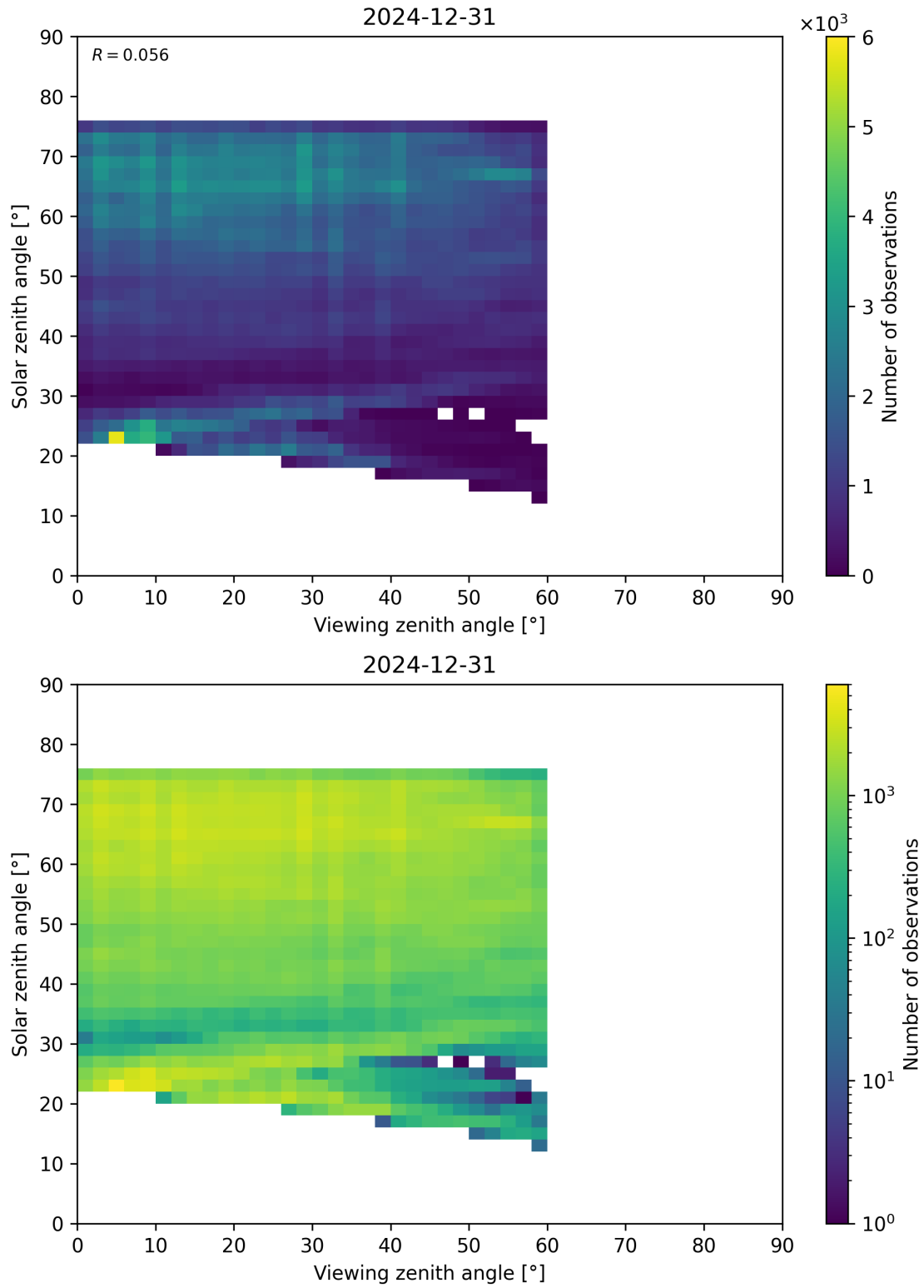
Figure 115: Scatter density plot of “Viewing zenith angle” against “Solar zenith angle” for 2024-12-30 to 2025-01-01.
