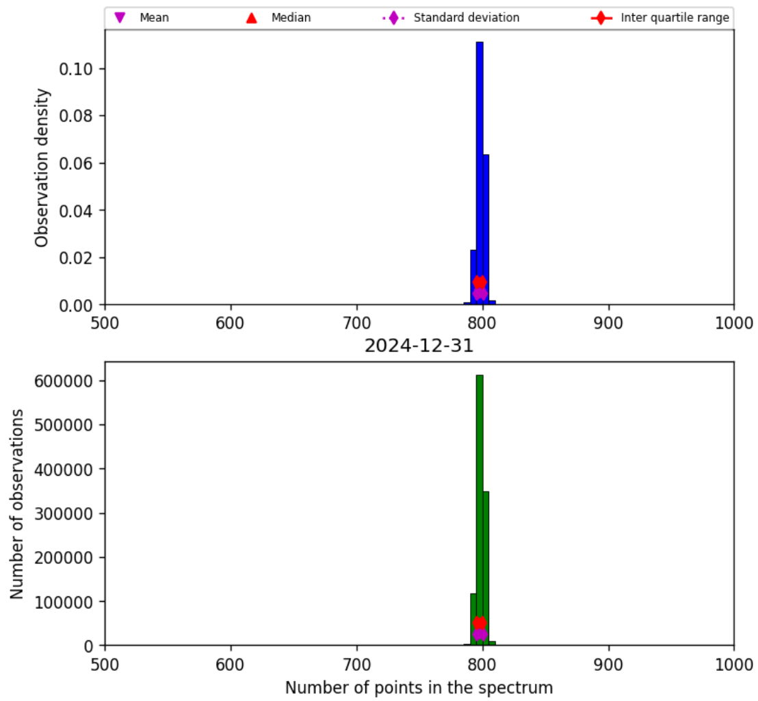
Figure 26: Histogram of “Number of points in the spectrum” for 2024-12-30 to 2025-01-01
