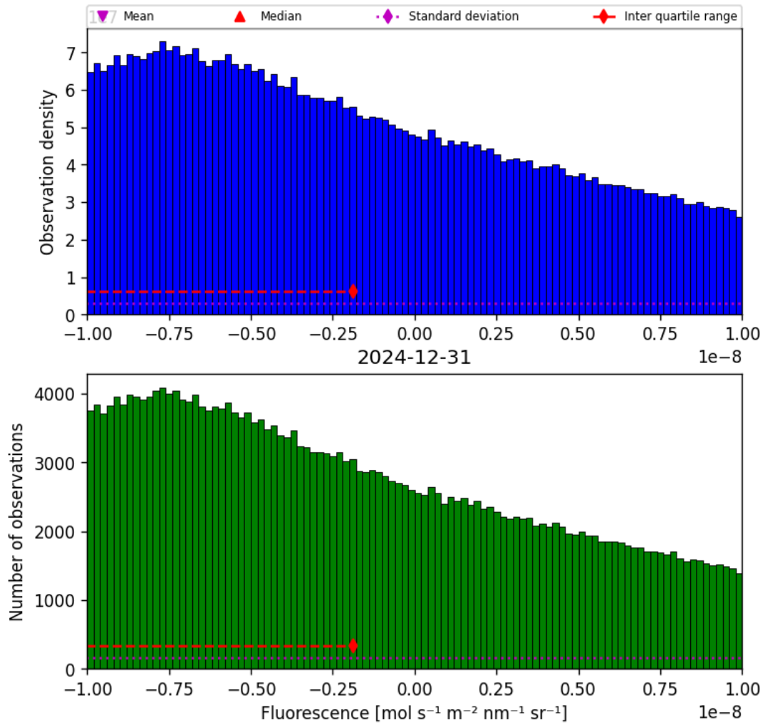
Figure 32: Histogram of “Fluorescence” for 2024-12-30 to 2025-01-01
