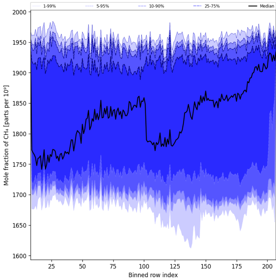
Figure 34: Along track statistics of “Mole fraction of CH 4 ” for 2024-12-30 to 2025-01-01
