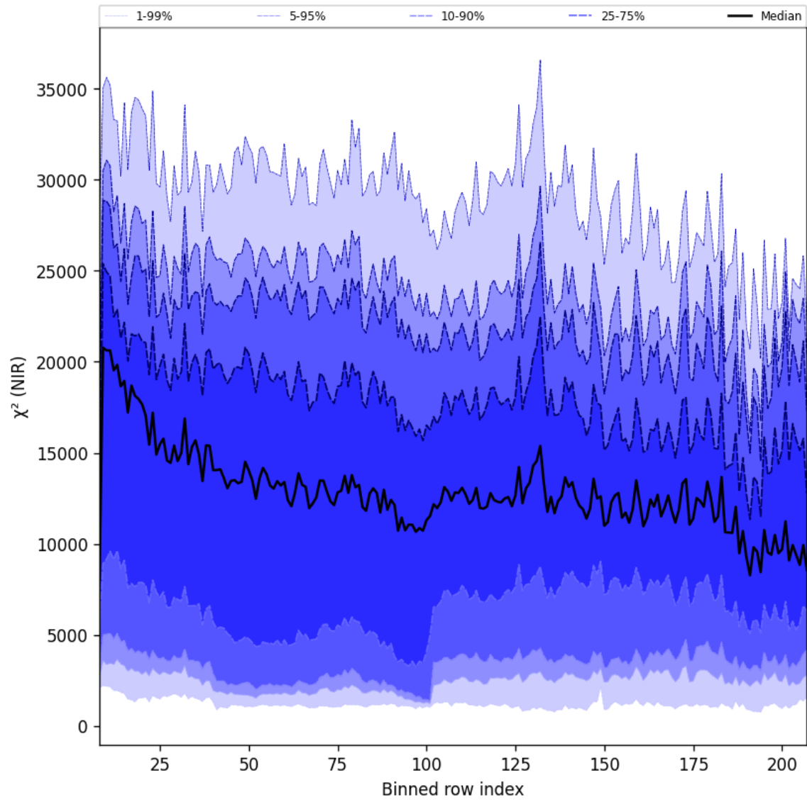
Figure 40: Along track statistics of " \chi^2 (NIR)" for 2024-12-30 to 2025-01-01
