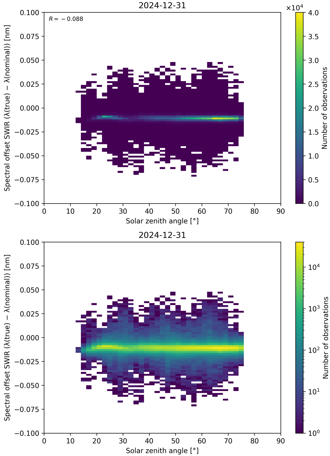
Figure 104: Scatter density plot of “Solar zenith angle” against “Spectral offset SWIR ( \lambda_{\text{true}} - \lambda_{\text{nominal}} )” for 2024-12-30 to 2025-01-01.
