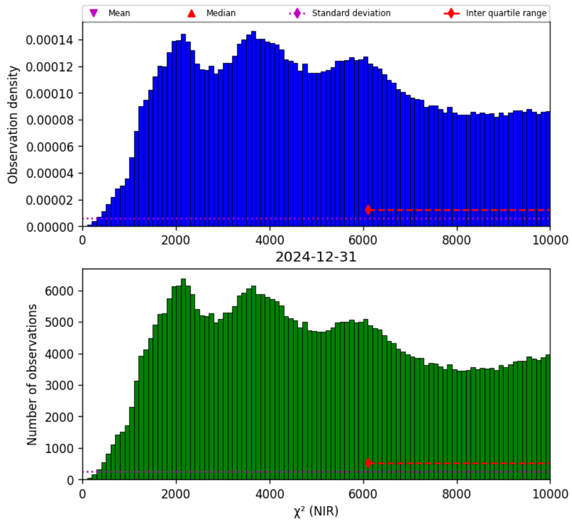
Figure 29: Histogram of “ \chi^2 (NIR)” for 2024-12-30 to 2025-01-01
