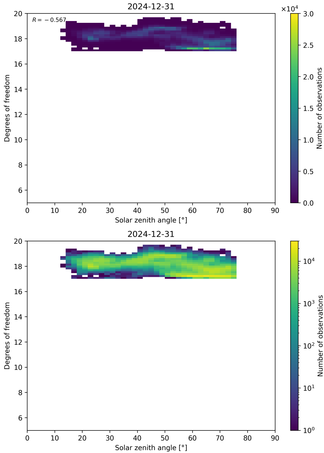
Figure 96: Scatter density plot of “Solar zenith angle” against “Degrees of freedom” for 2024-12-30 to 2025-01-01.
