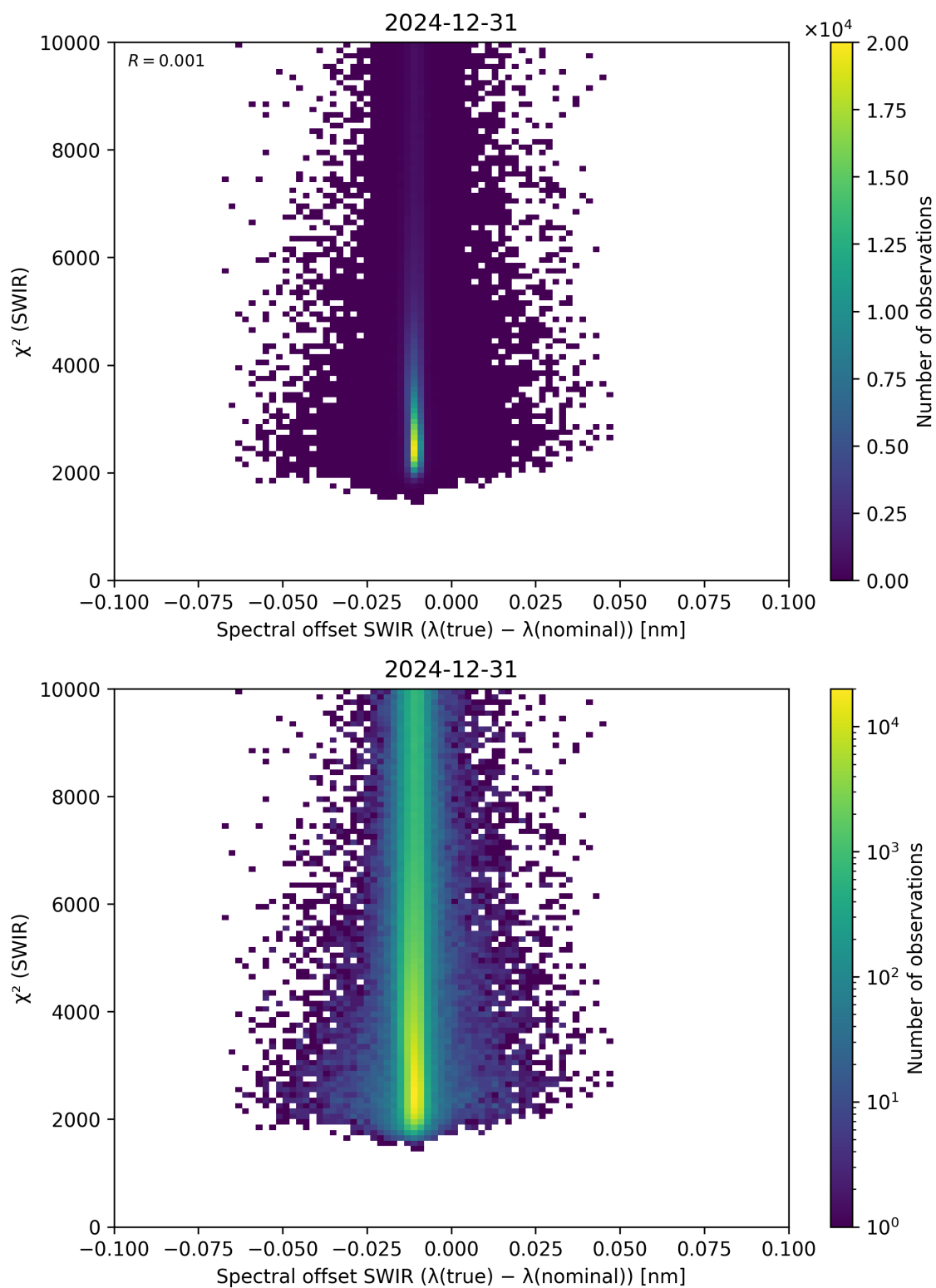
Figure 118: Scatter density plot of “Spectral offset SWIR ( \lambda_{\text{true}} - \lambda_{\text{nominal}} )” against “ \chi^2 (SWIR)” for 2024-12-30 to 2025-01-01.
