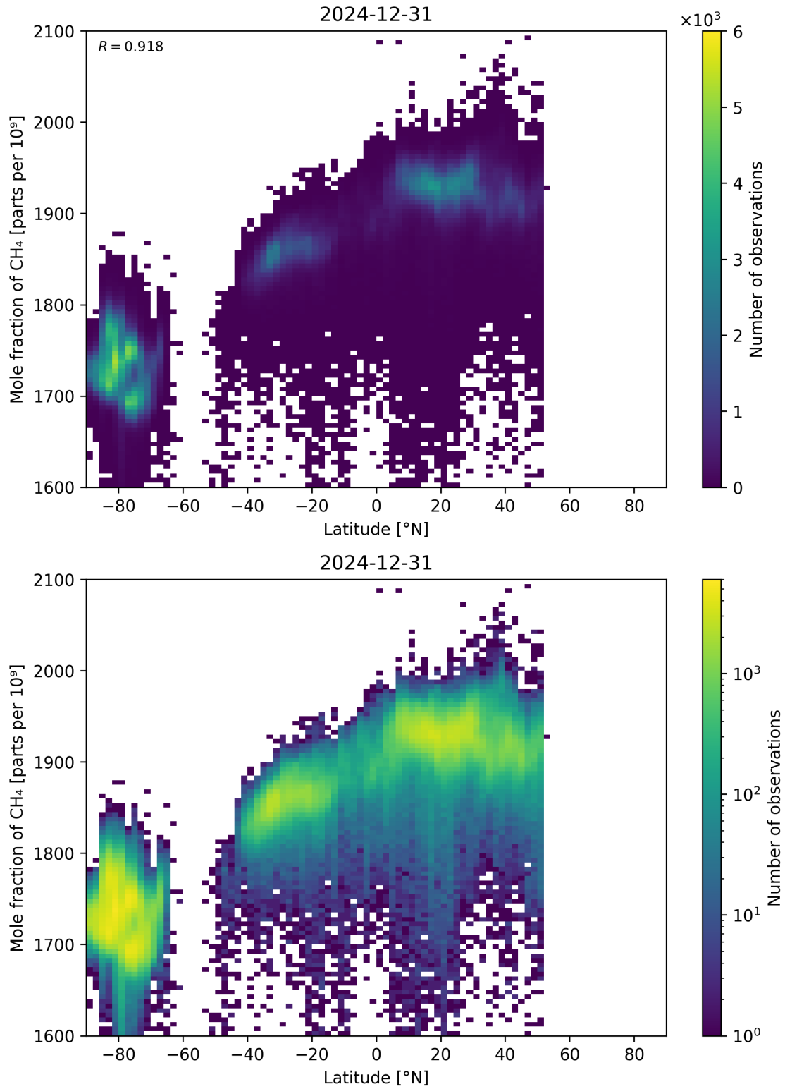
Figure 57: Scatter density plot of “Latitude” against “Mole fraction of CH 4 ” for 2024-12-30 to 2025-01-01.
