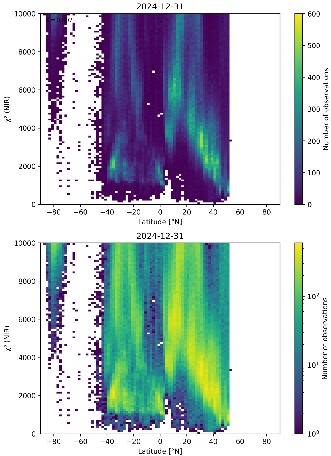
Figure 53: Scatter density plot of “Latitude” against “ \chi^2 (NIR)” for 2024-12-30 to 2025-01-01.
