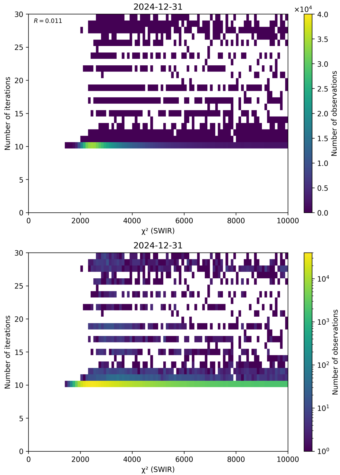
Figure 50: Scatter density plot of " \chi^2 (SWIR)" against "Number of iterations" for 2024-12-30 to 2025-01-01.
