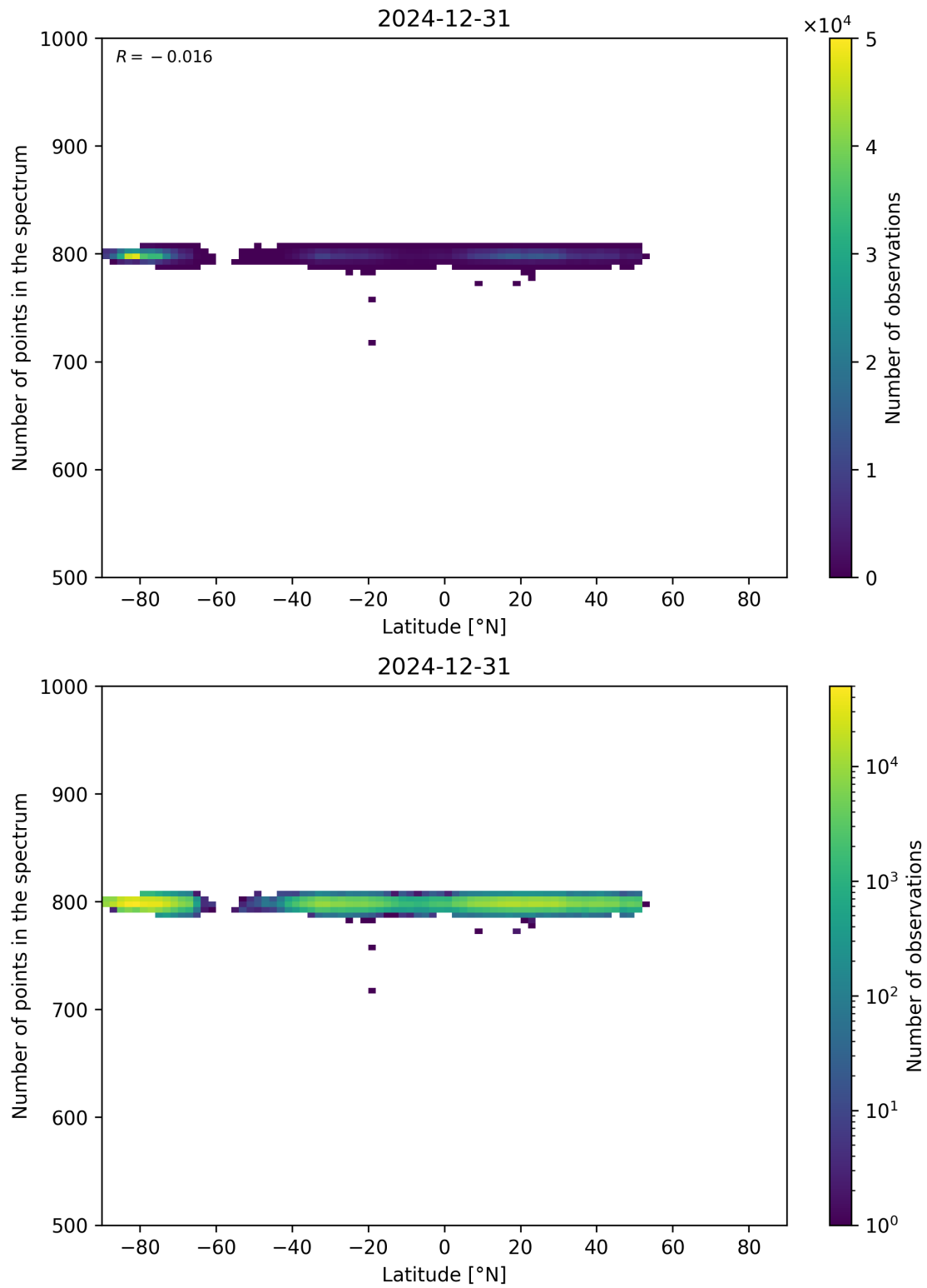
Figure 61: Scatter density plot of “Latitude” against “Number of points in the spectrum” for 2024-12-30 to 2025-01-01.
