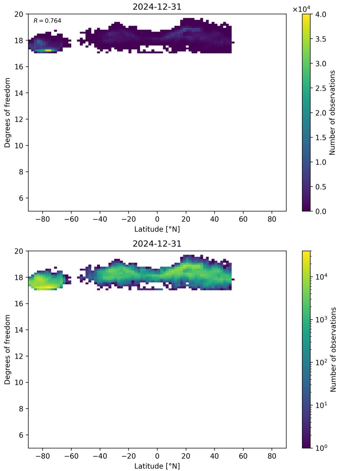
Figure 55: Scatter density plot of “Latitude” against “Degrees of freedom” for 2024-12-30 to 2025-01-01.
