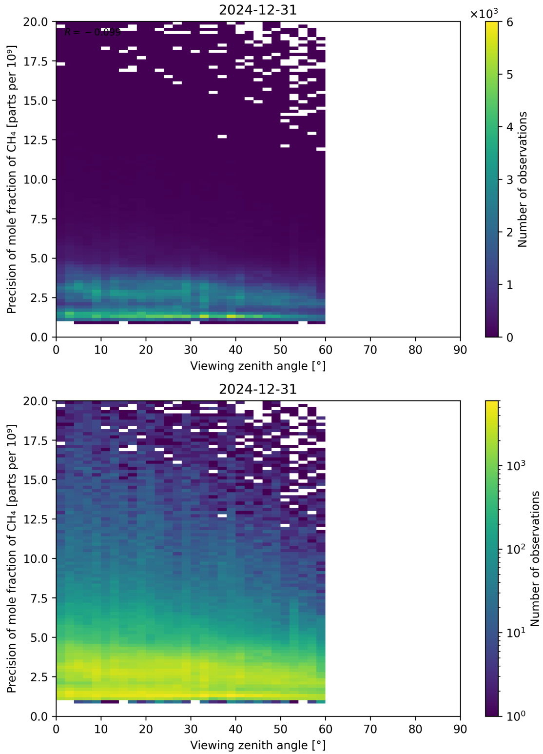
Figure 112: Scatter density plot of “Viewing zenith angle” against “Precision of mole fraction of CH 4 ” for 2024-12-30 to 2025-01-01.
