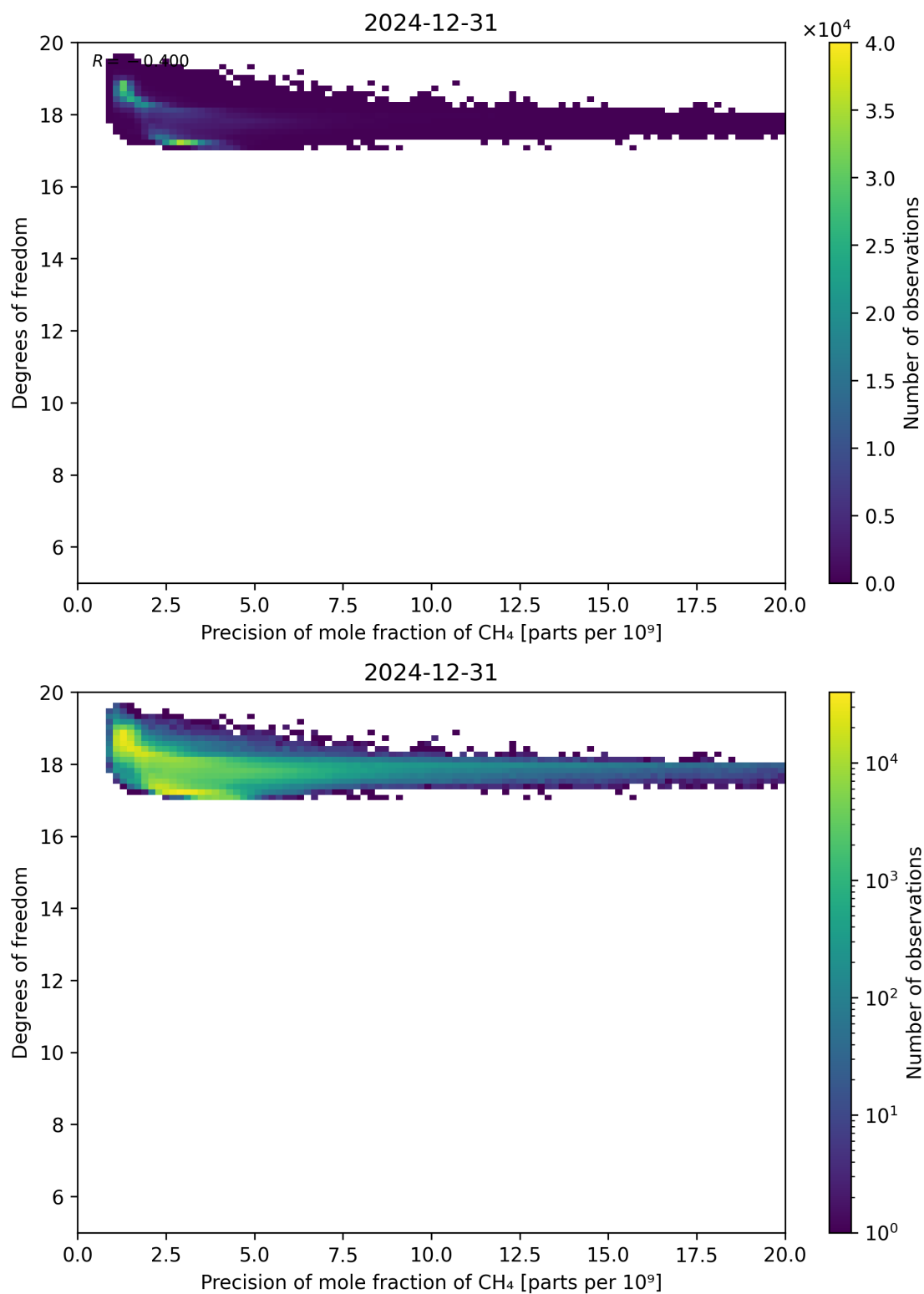
Figure 80: Scatter density plot of “Precision of mole fraction of CH 4 ” against “Degrees of freedom” for 2024-12-30 to 2025-01-01.
