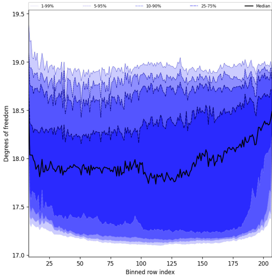
Figure 41: Along track statistics of “Degrees of freedom” for 2024-12-30 to 2025-01-01
