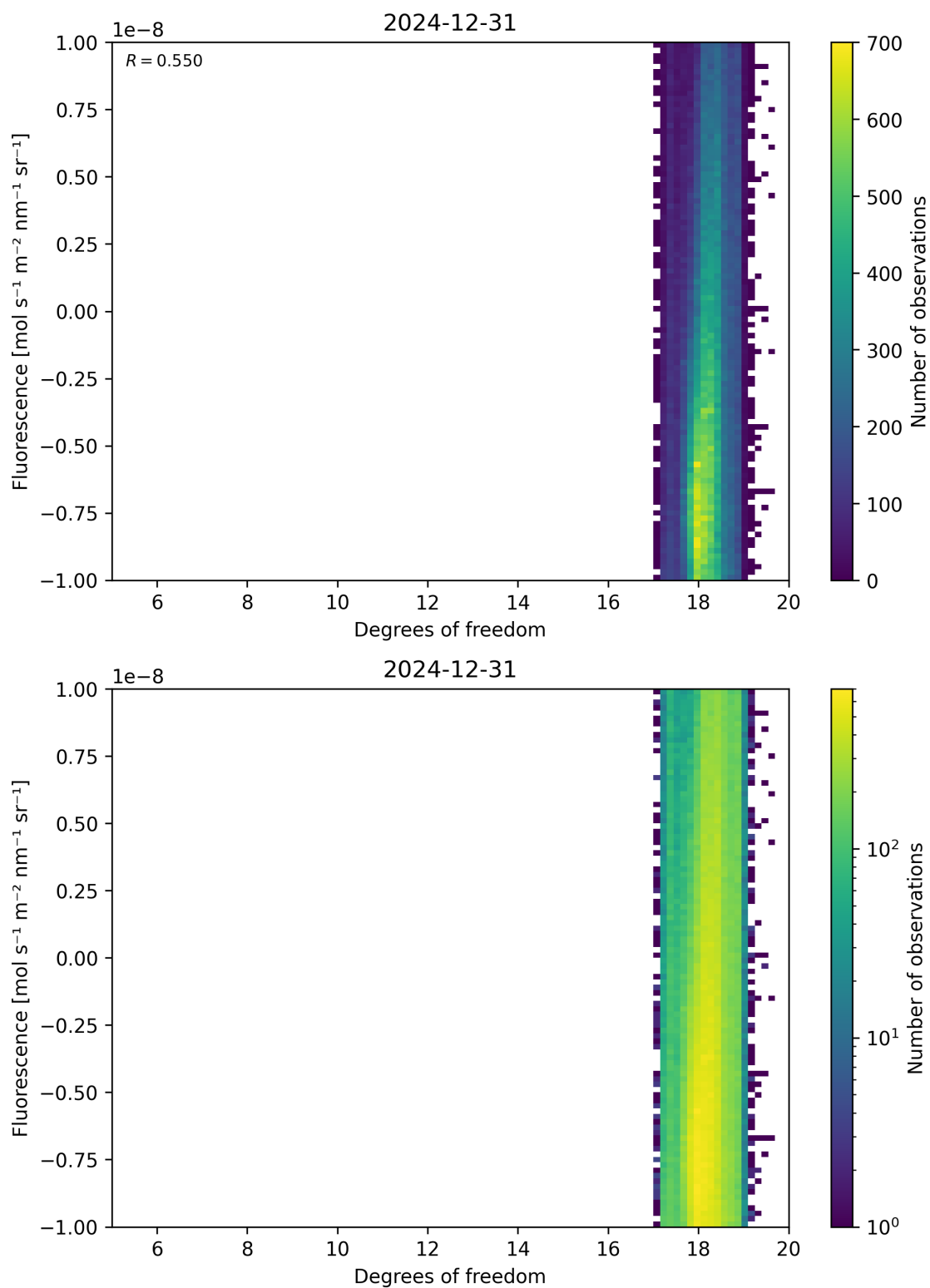
Figure 51: Scatter density plot of “Degrees of freedom” against “Fluorescence” for 2024-12-30 to 2025-01-01.
