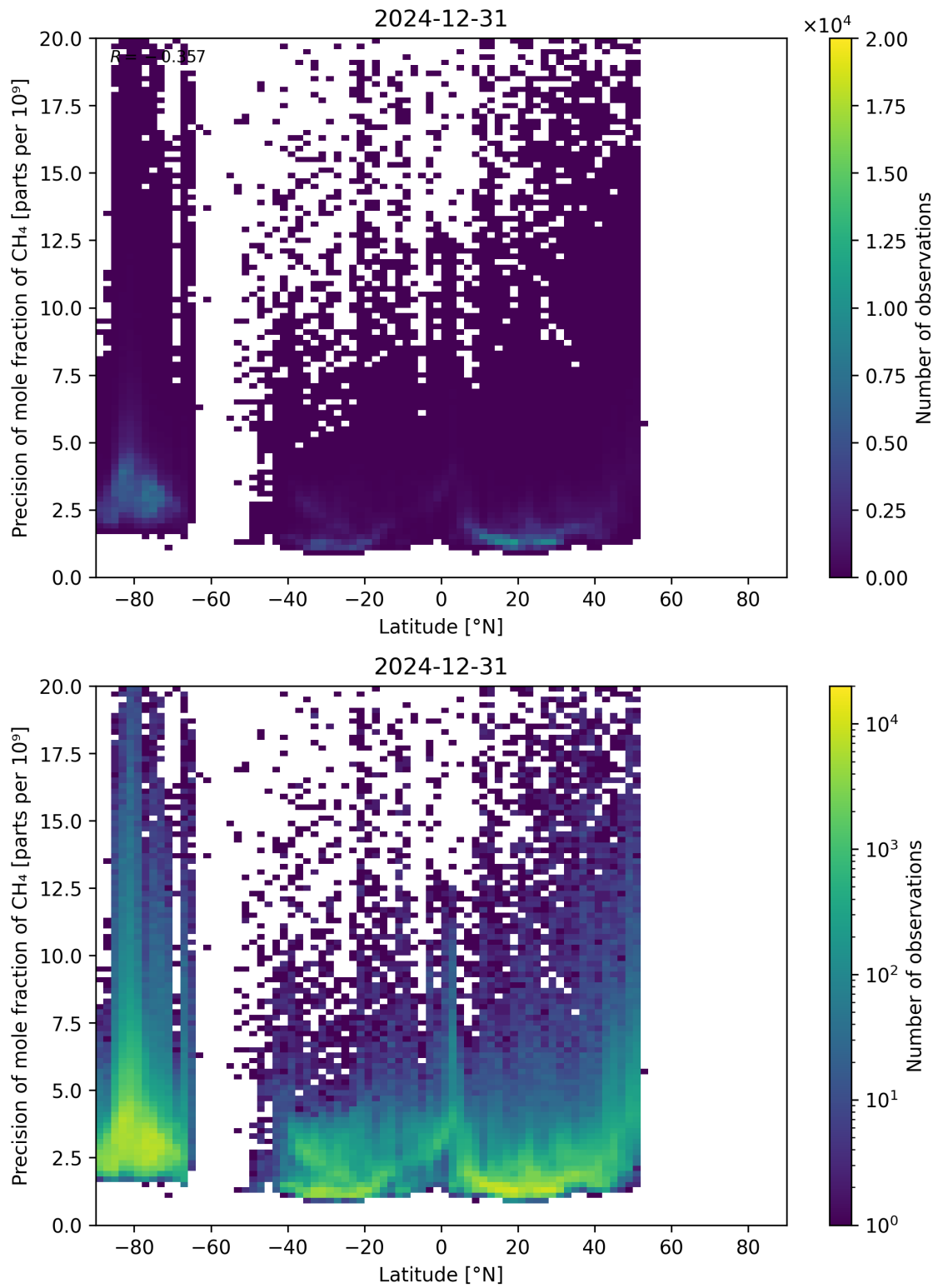
Figure 59: Scatter density plot of “Latitude” against “Precision of mole fraction of CH 4 ” for 2024-12-30 to 2025-01-01.
