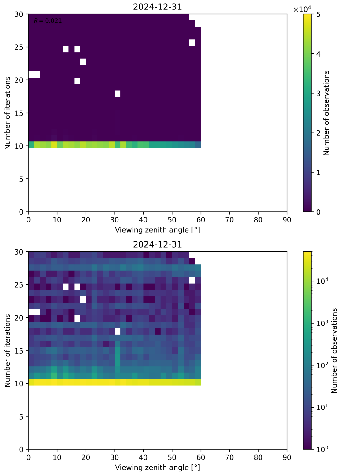
Figure 113: Scatter density plot of “Viewing zenith angle” against “Number of iterations” for 2024-12-30 to 2025-01-01.
