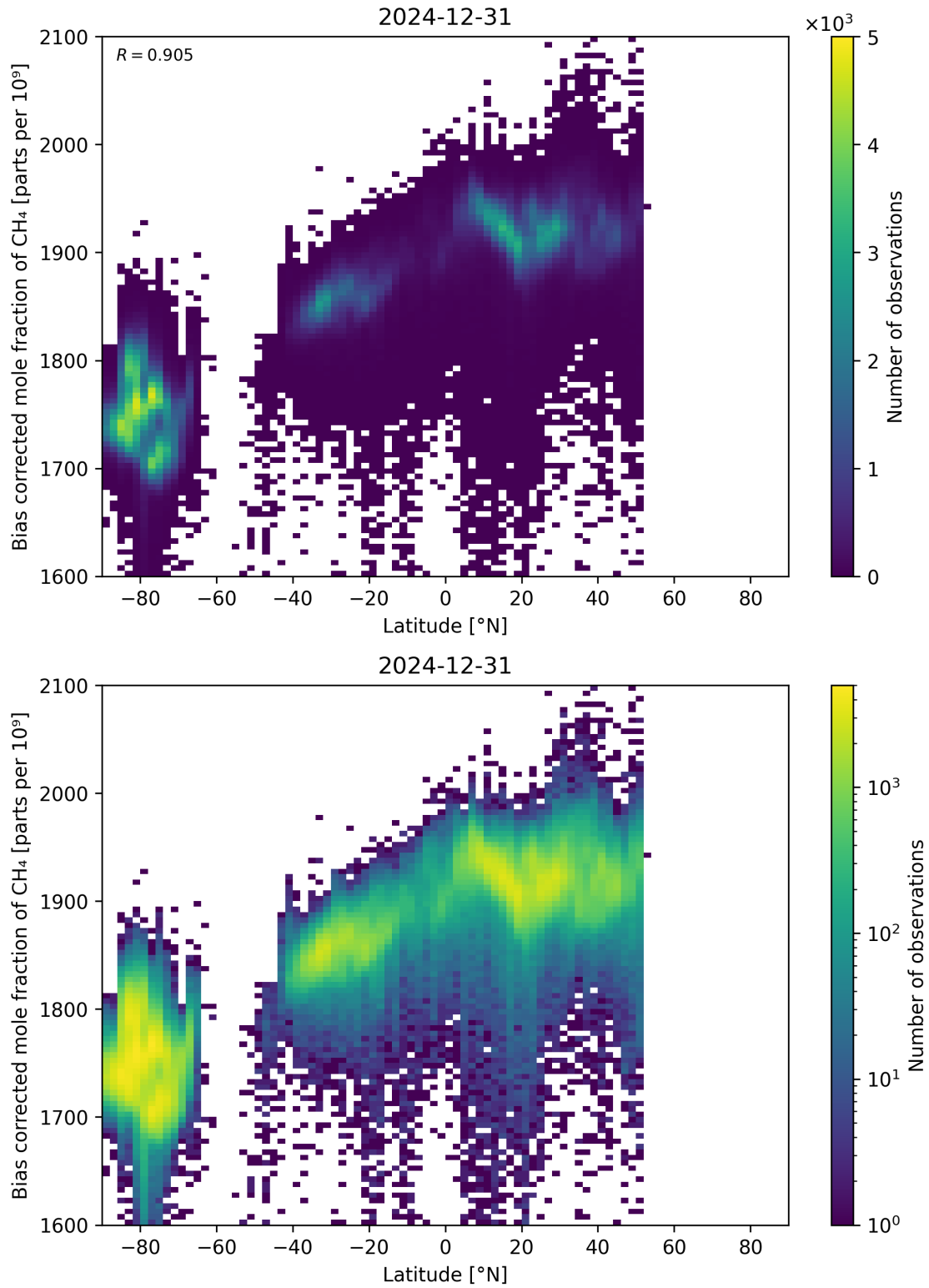
Figure 58: Scatter density plot of “Latitude” against “Bias corrected mole fraction of CH 4 ” for 2024-12-30 to 2025-01-01.
