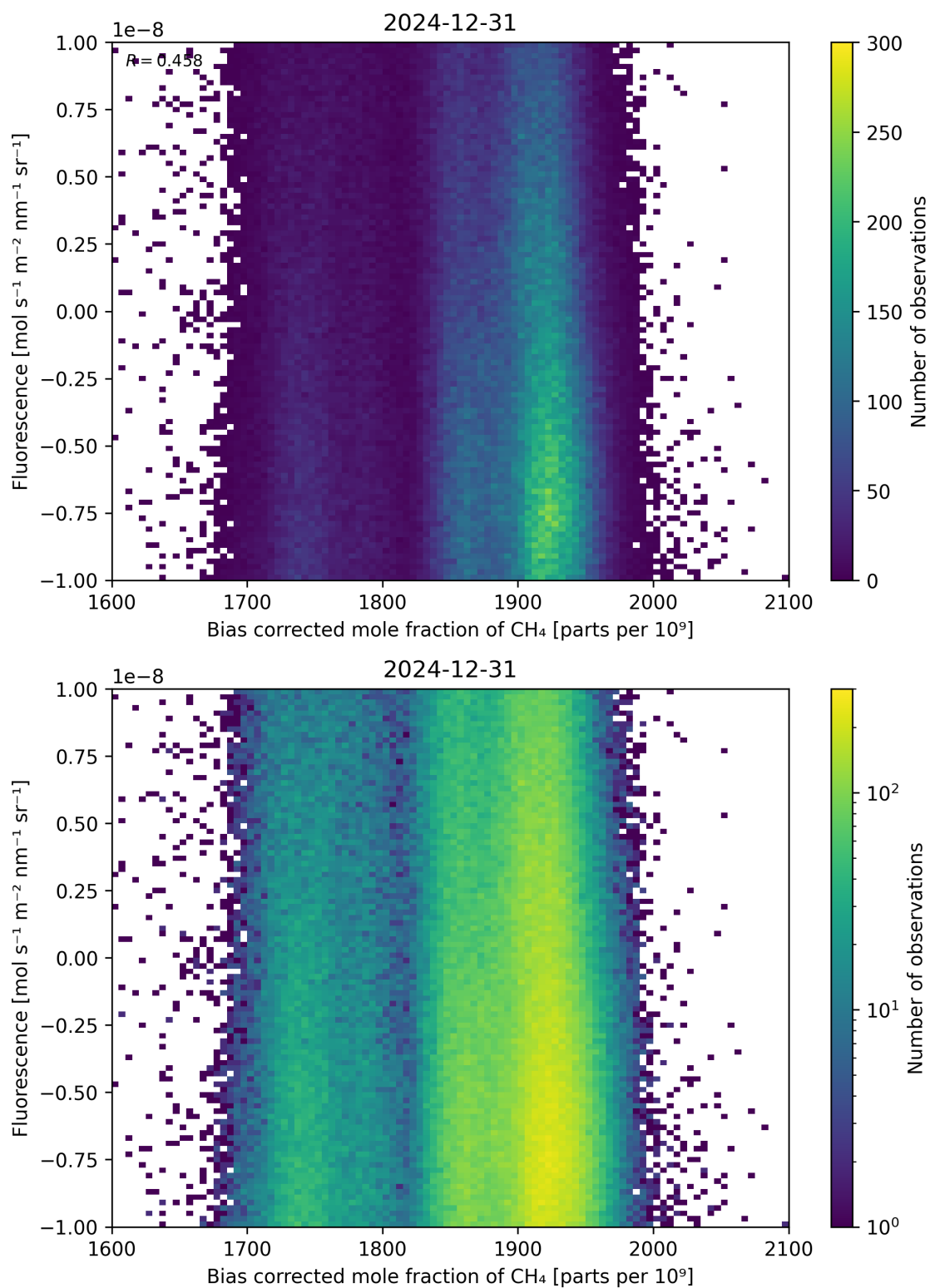
Figure 66: Scatter density plot of “Bias corrected mole fraction of \text{CH}_4 ” against “Fluorescence” for 2024-12-30 to 2025-01-01.
