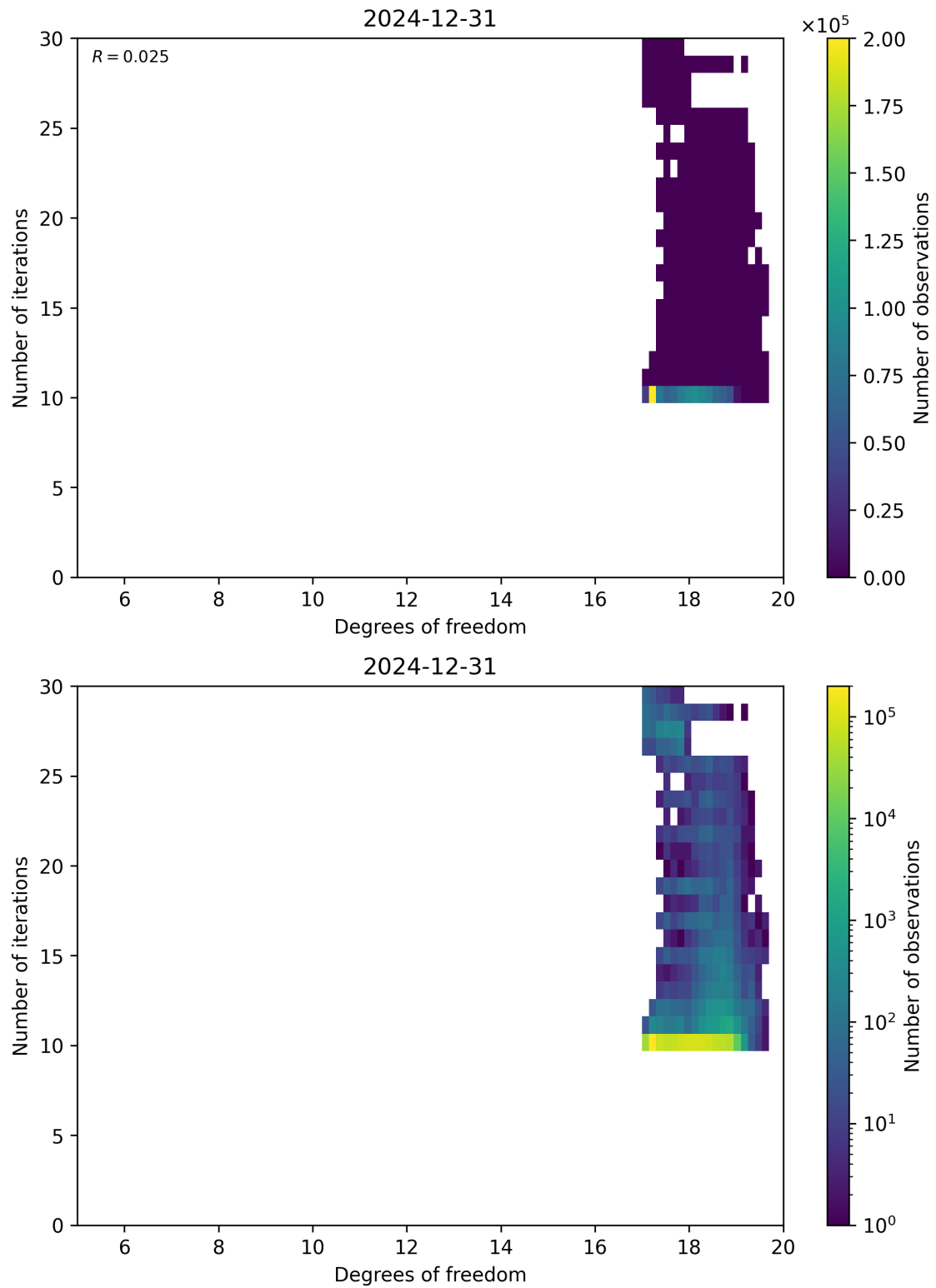
Figure 52: Scatter density plot of “Degrees of freedom” against “Number of iterations” for 2024-12-30 to 2025-01-01.
