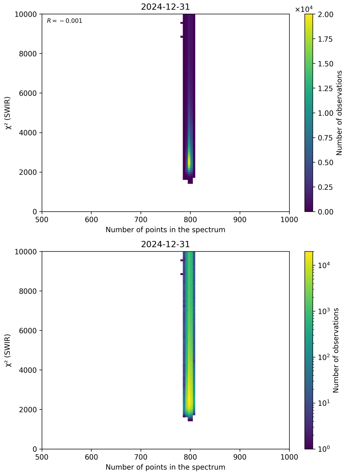
Figure 89: Scatter density plot of “Number of points in the spectrum” against “ \chi^2 (SWIR)” for 2024-12-30 to 2025-01-01.
