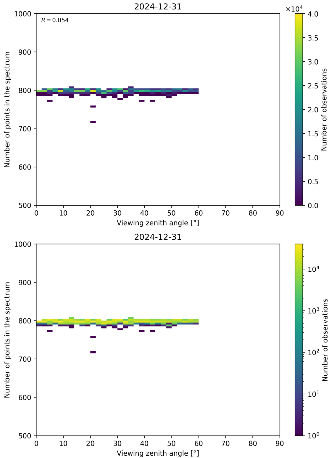
Figure 114: Scatter density plot of “Viewing zenith angle” against “Number of points in the spectrum” for 2024-12-30 to 2025-01-01.
