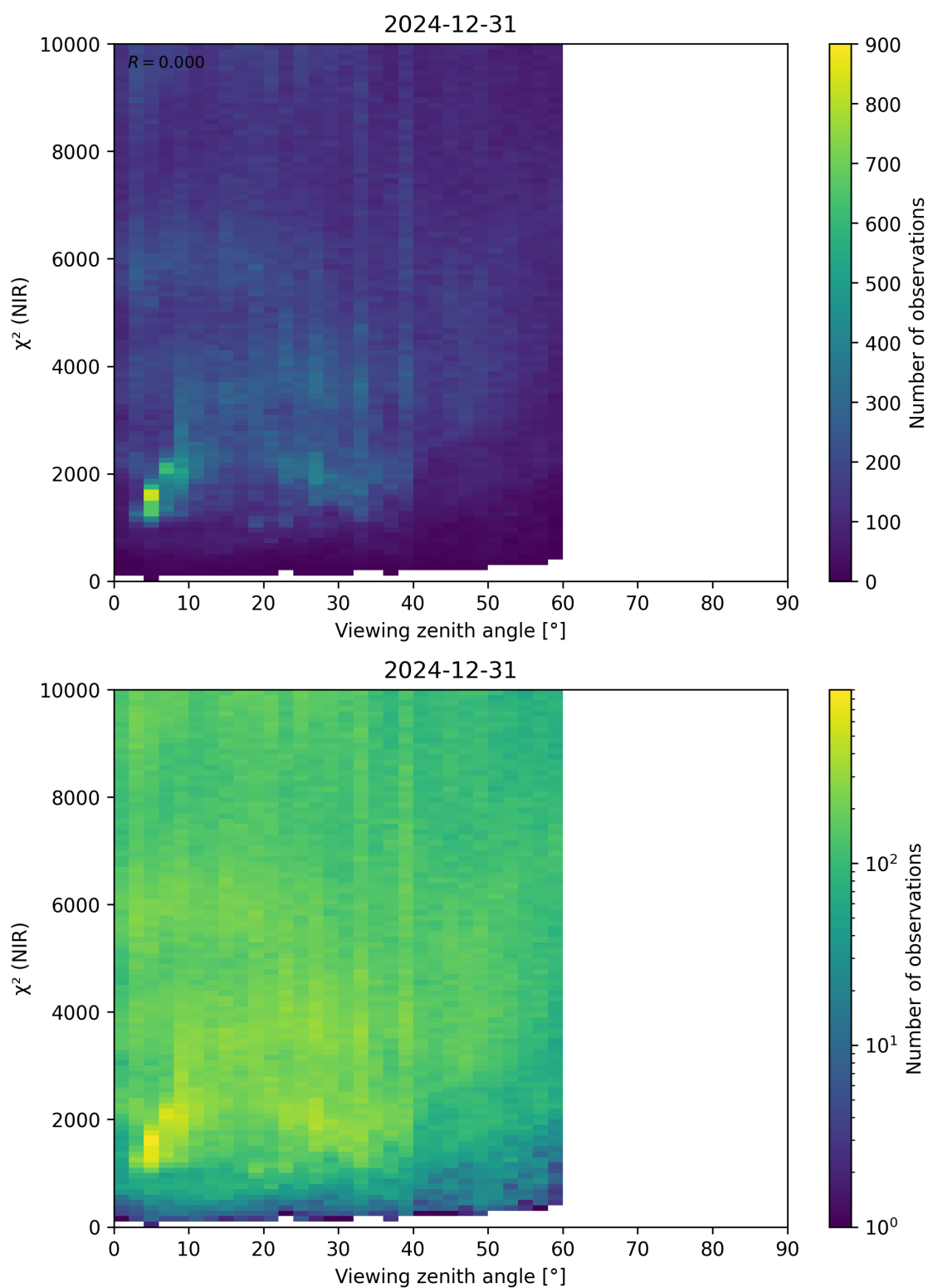
Figure 105: Scatter density plot of “Viewing zenith angle” against “ \chi^2 (NIR)” for 2024-12-30 to 2025-01-01.
