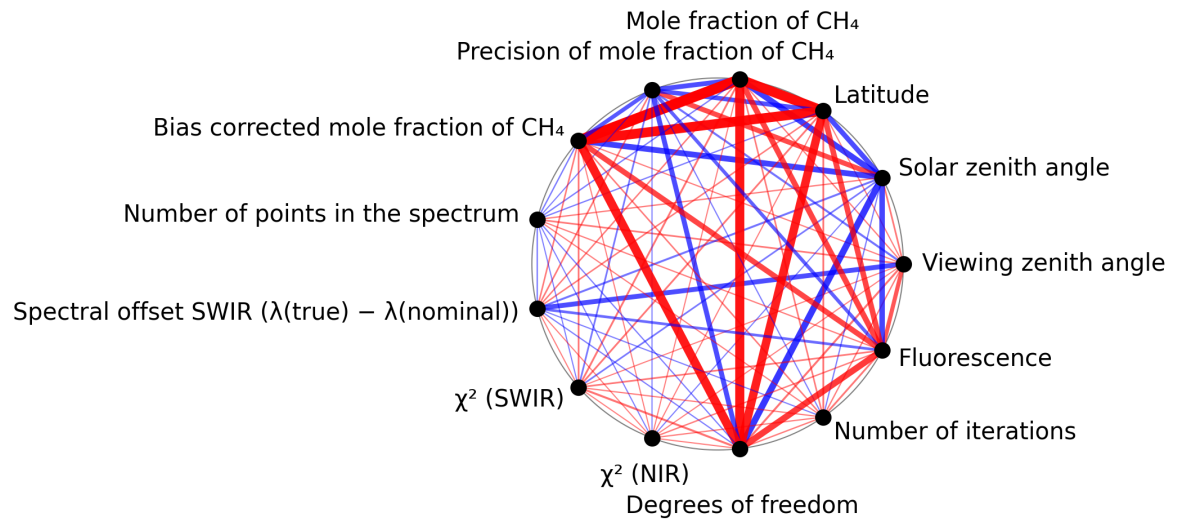
Figure 1: Map of correlation graph for 2024-12-30 to 2025-01-01.
