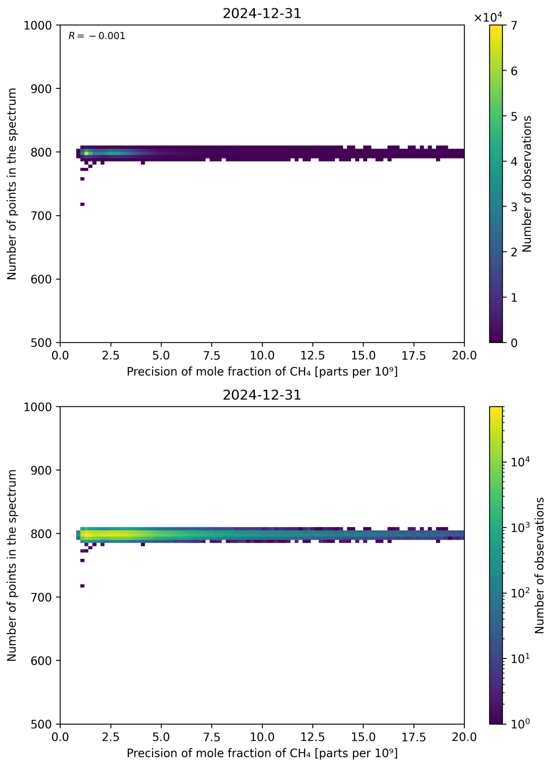
Figure 84: Scatter density plot of “Precision of mole fraction of CH 4 ” against “Number of points in the spectrum” for 2024-12-30 to 2025-01-01.
