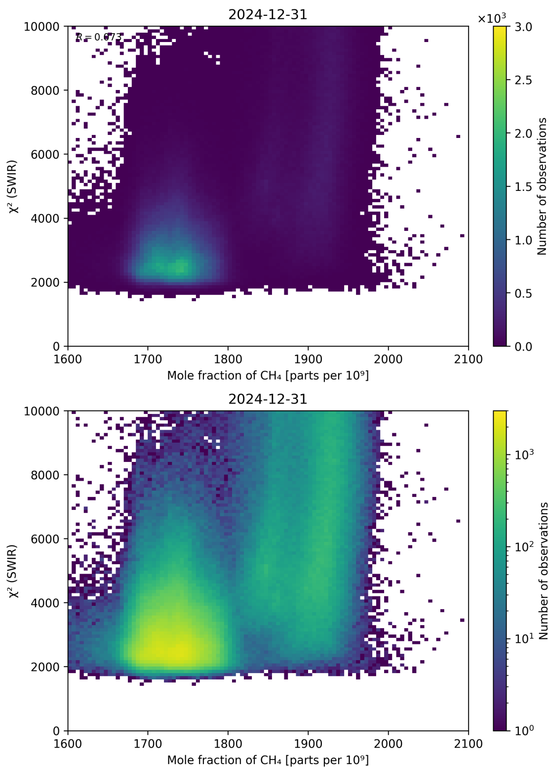
Figure 71: Scatter density plot of “Mole fraction of \text{CH}_4 ” against “ \chi^2 (SWIR)” for 2024-12-30 to 2025-01-01.
