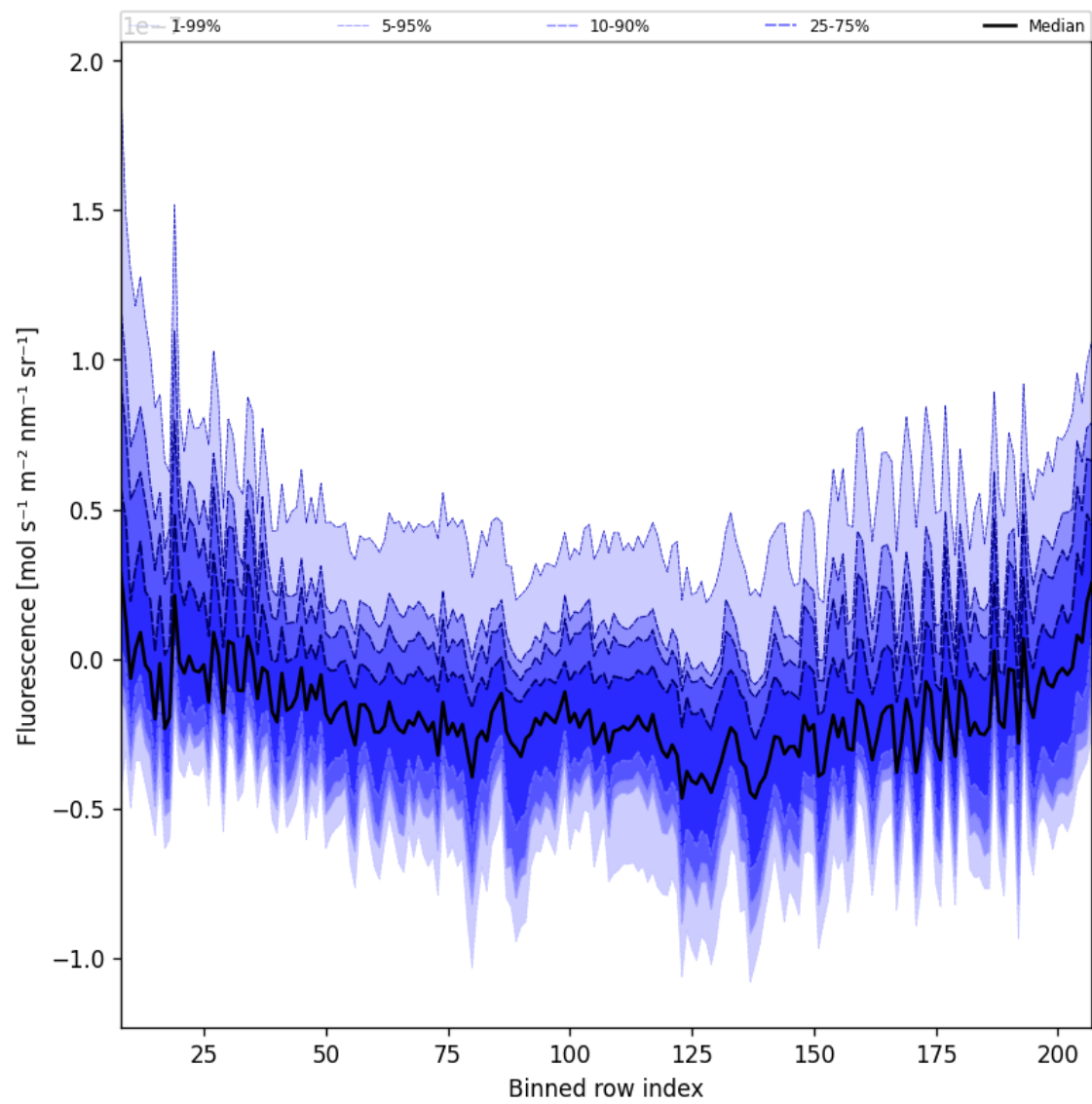
Figure 43: Along track statistics of “Fluorescence” for 2024-12-30 to 2025-01-01
