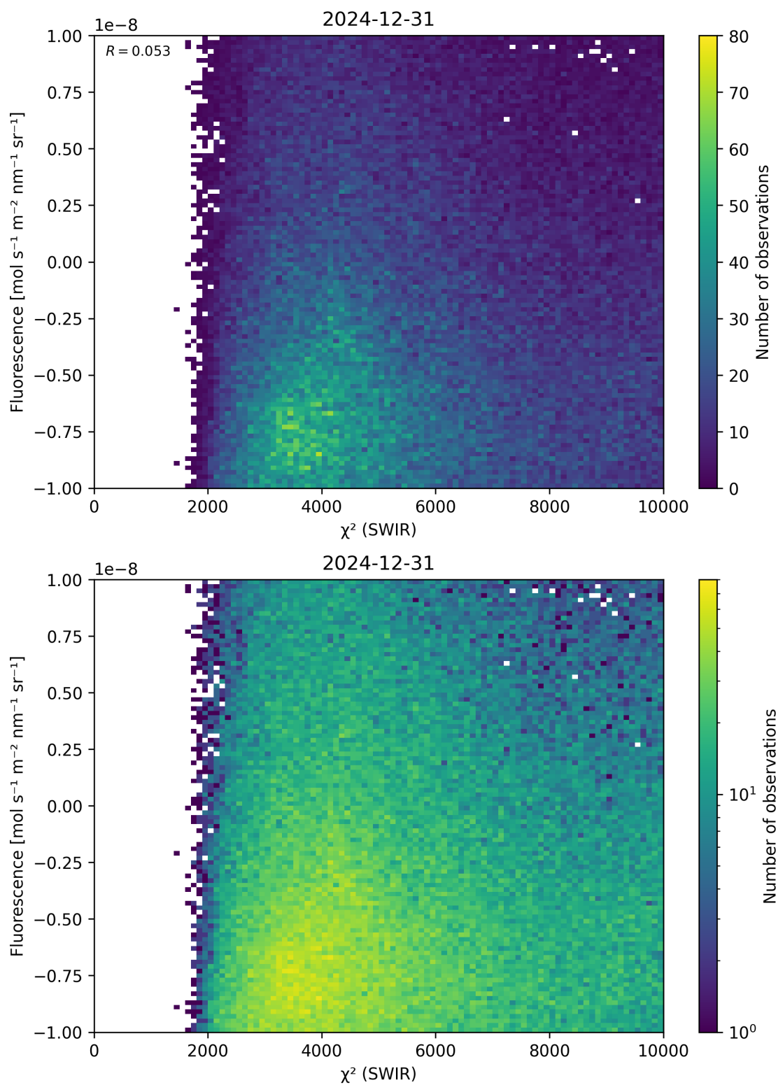
Figure 49: Scatter density plot of “ \chi^2 (SWIR)” against “Fluorescence” for 2024-12-30 to 2025-01-01.
