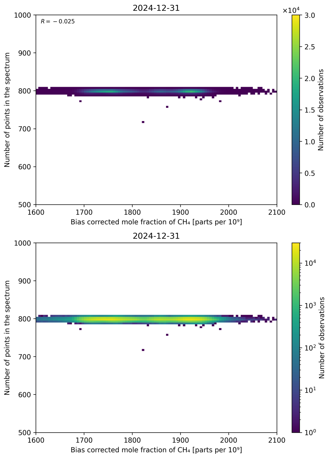
Figure 68: Scatter density plot of “Bias corrected mole fraction of CH 4 ” against “Number of points in the spectrum” for 2024-12-30 to 2025-01-01.
