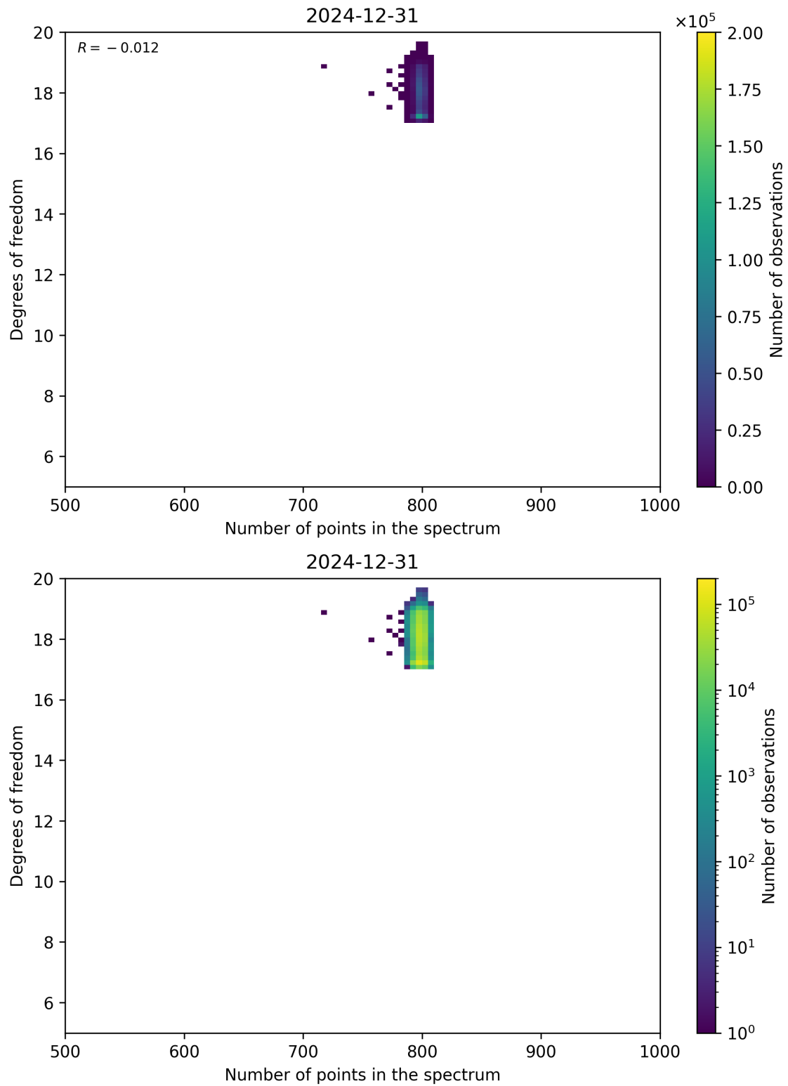
Figure 90: Scatter density plot of “Number of points in the spectrum” against “Degrees of freedom” for 2024-12-30 to 2025-01-01.
