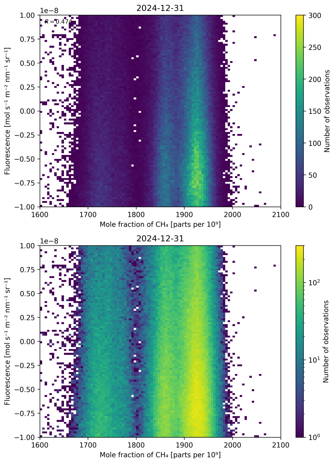
Figure 73: Scatter density plot of “Mole fraction of CH 4 ” against “Fluorescence” for 2024-12-30 to 2025-01-01.
