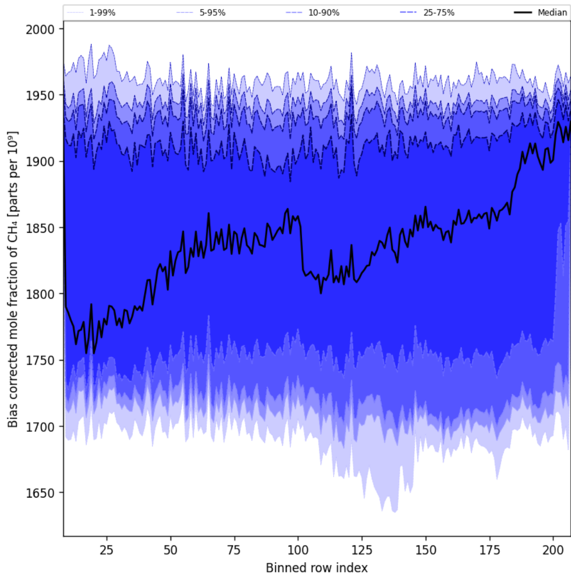
Figure 36: Along track statistics of “Bias corrected mole fraction of CH 4 ” for 2024-12-30 to 2025-01-01
