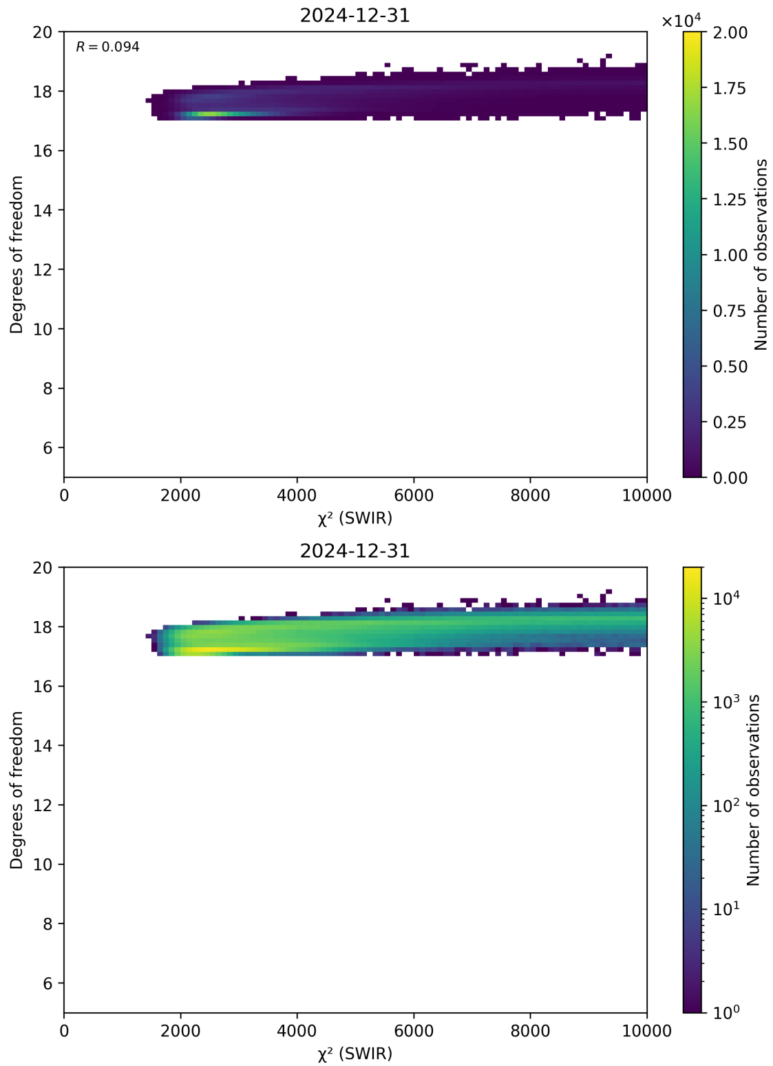
Figure 48: Scatter density plot of “ \chi^2 (SWIR)” against “Degrees of freedom” for 2024-12-30 to 2025-01-01.
