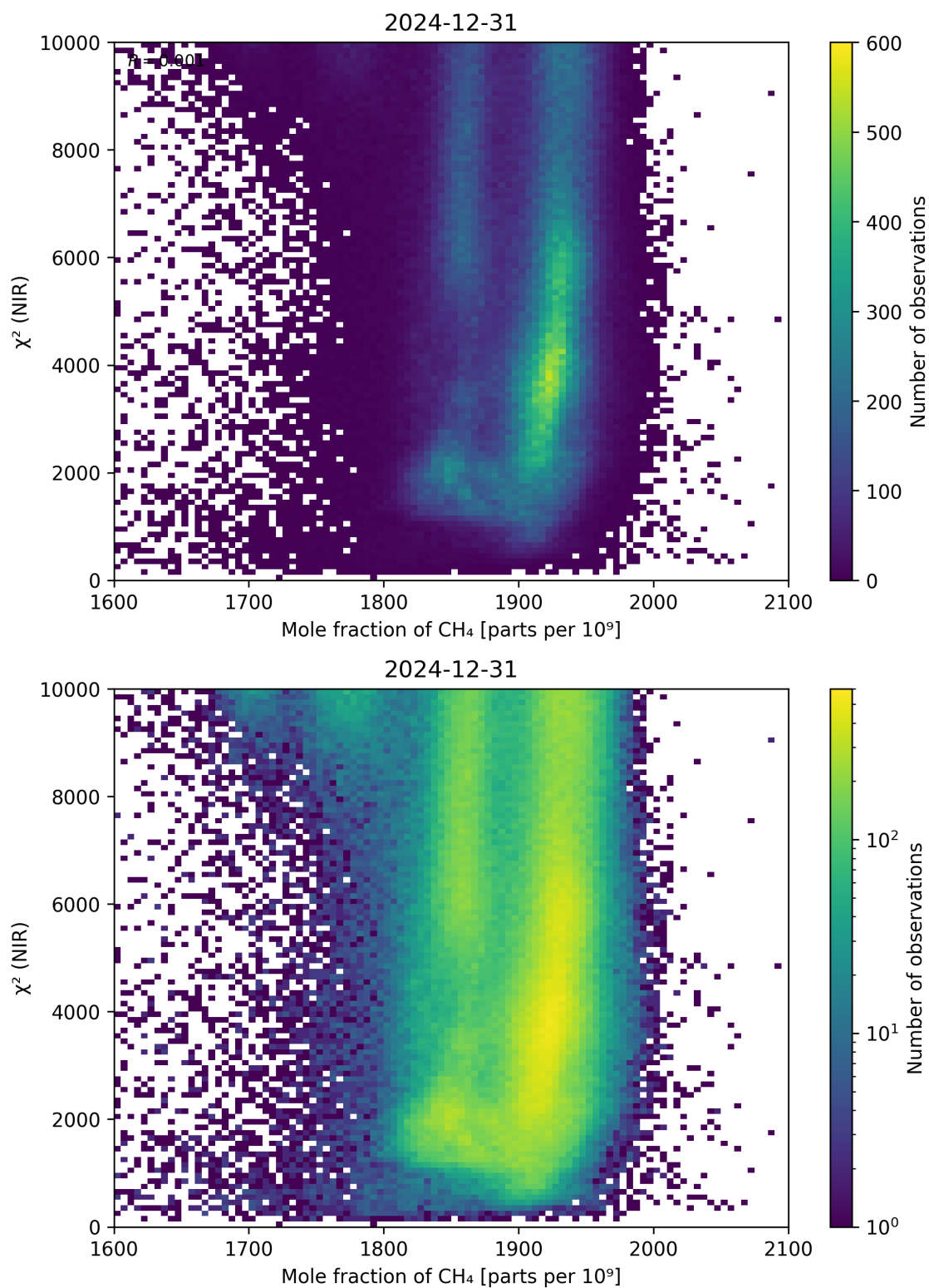
Figure 70: Scatter density plot of “Mole fraction of \text{CH}_4 ” against “ \chi^2 (NIR)” for 2024-12-30 to 2025-01-01.
