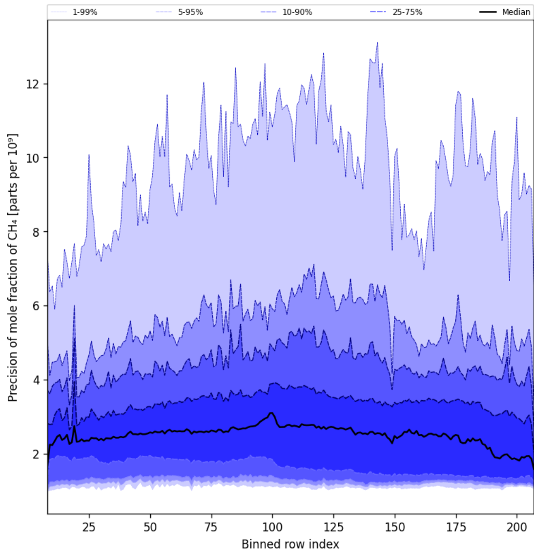
Figure 35: Along track statistics of “Precision of mole fraction of CH 4 ” for 2024-12-30 to 2025-01-01
