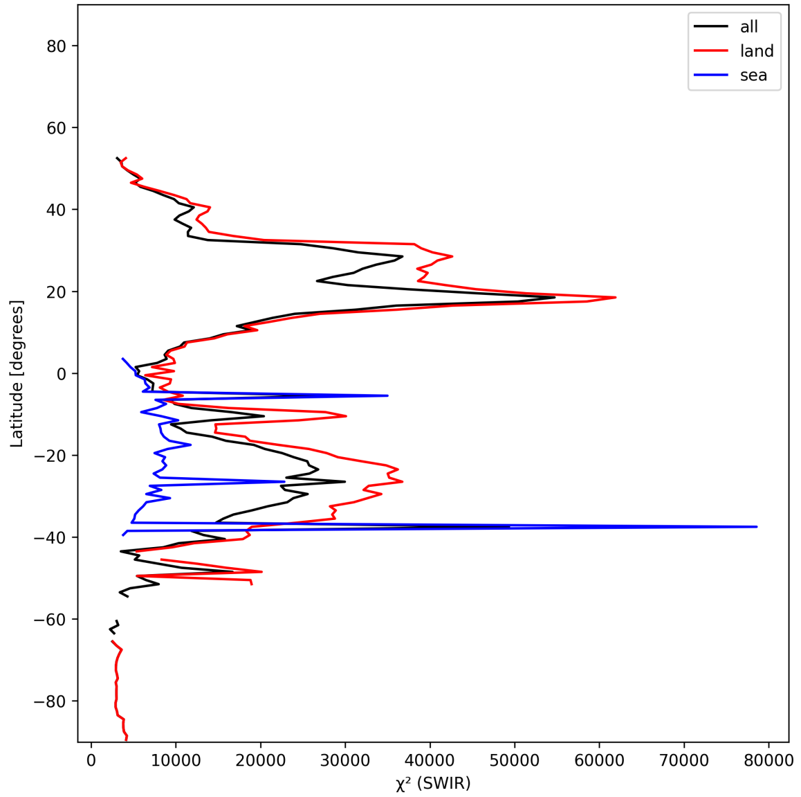
Figure 17: Zonal average of “ \chi^2 (SWIR)” for 2024-12-30 to 2025-01-01.
