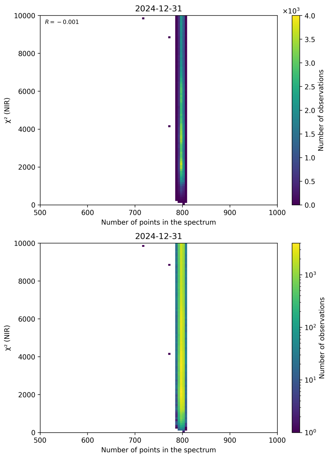
Figure 88: Scatter density plot of “Number of points in the spectrum” against “ \chi^2 (NIR)” for 2024-12-30 to 2025-01-01.
