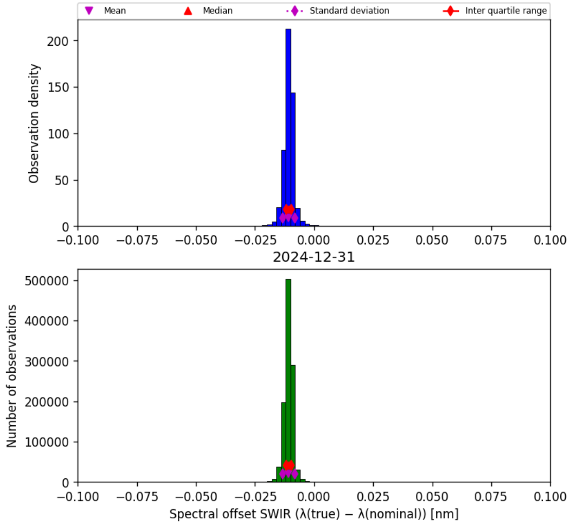
Figure 27: Histogram of “Spectral offset SWIR ( \lambda_{\text{true}} - \lambda_{\text{nominal}} )” for 2024-12-30 to 2025-01-01
