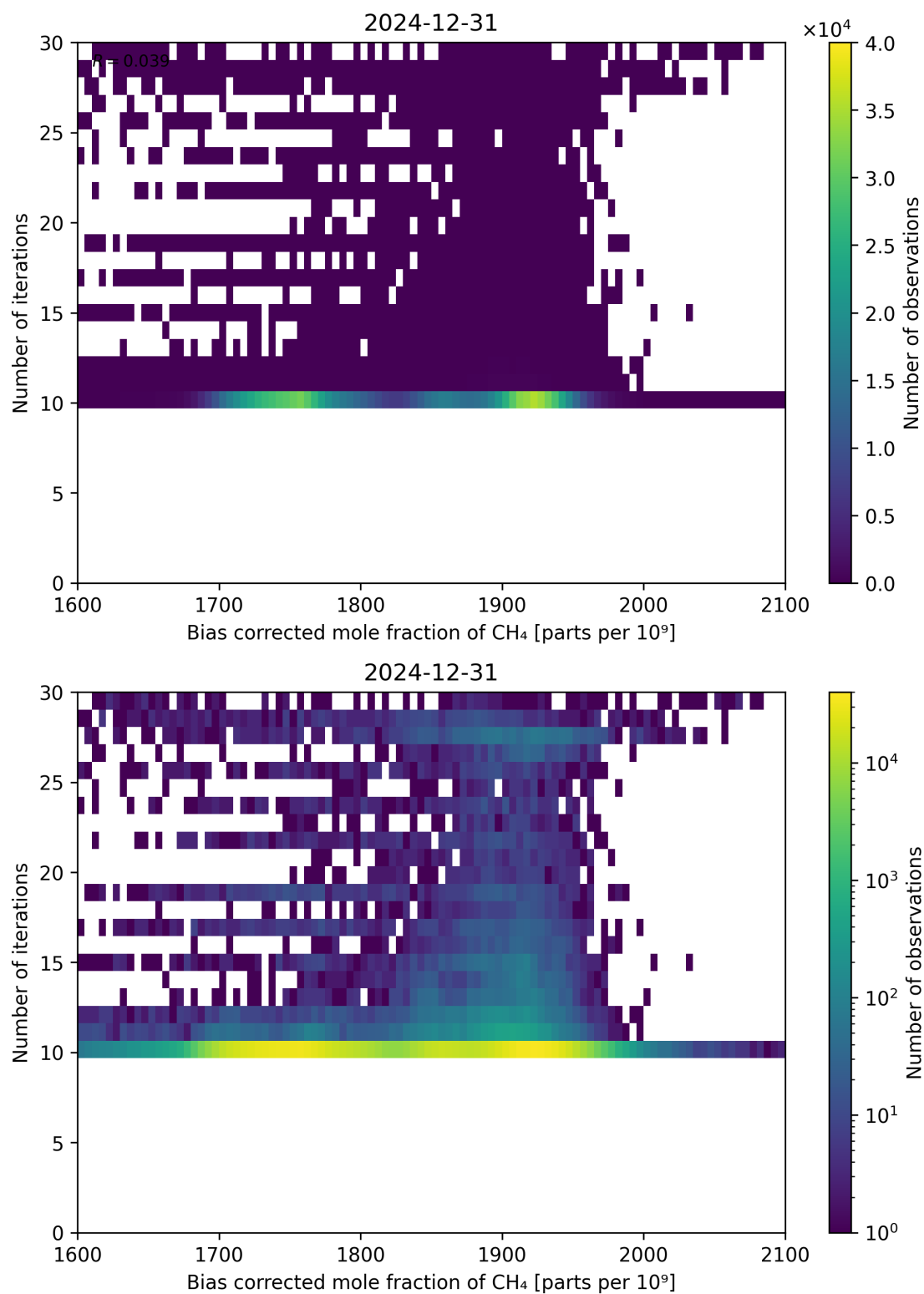
Figure 67: Scatter density plot of “Bias corrected mole fraction of CH 4 ” against “Number of iterations” for 2024-12-30 to 2025-01-01.
