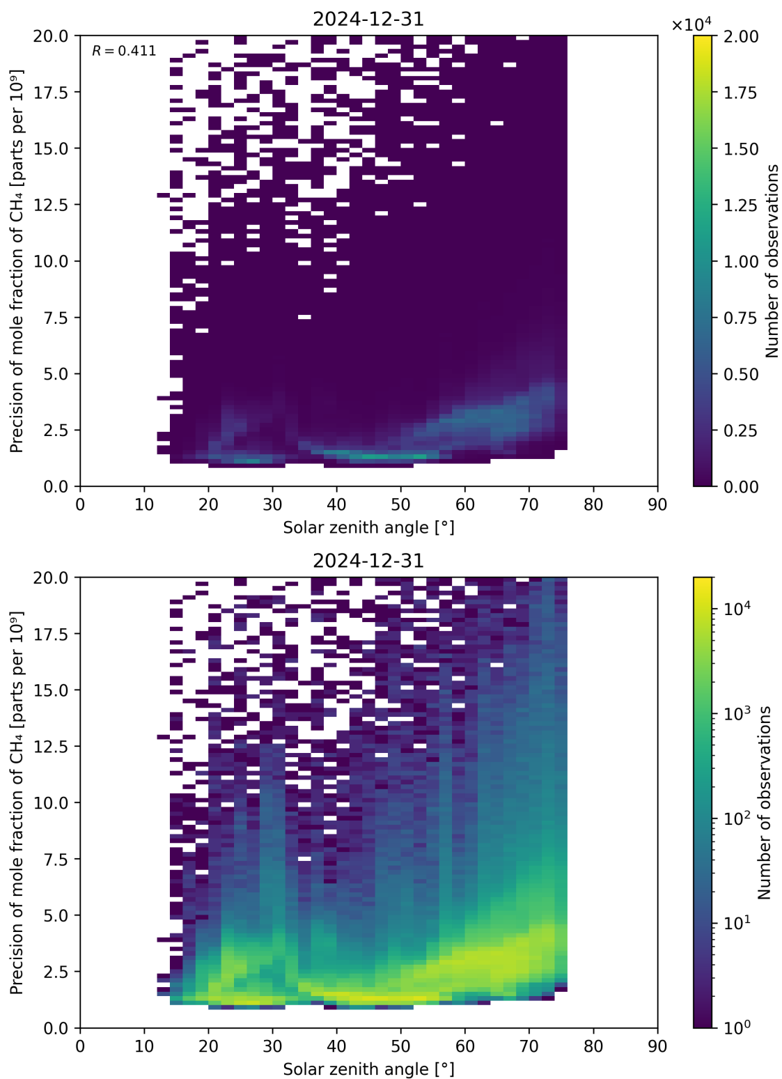
Figure 101: Scatter density plot of “Solar zenith angle” against “Precision of mole fraction of \text{CH}_4 ” for 2024-12-30 to 2025-01-01.
