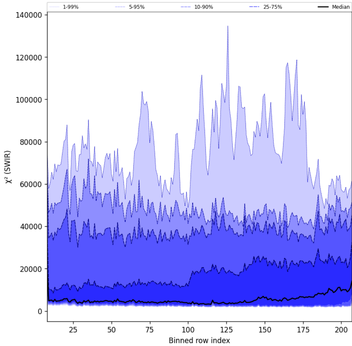
Figure 39: Along track statistics of “ \chi^2 (SWIR)” for 2024-12-30 to 2025-01-01
