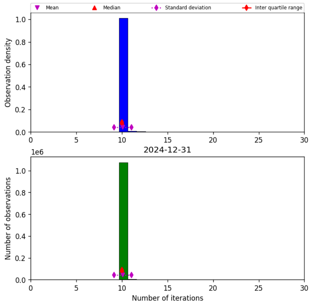
Figure 31: Histogram of “Number of iterations” for 2024-12-30 to 2025-01-01
