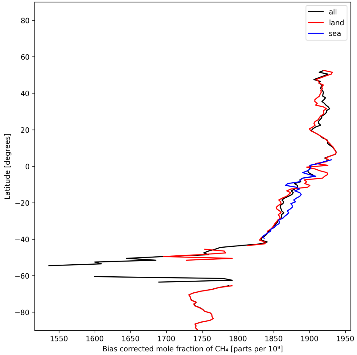
Figure 14: Zonal average of “Bias corrected mole fraction of CH 4 ” for 2024-12-30 to 2025-01-01.
