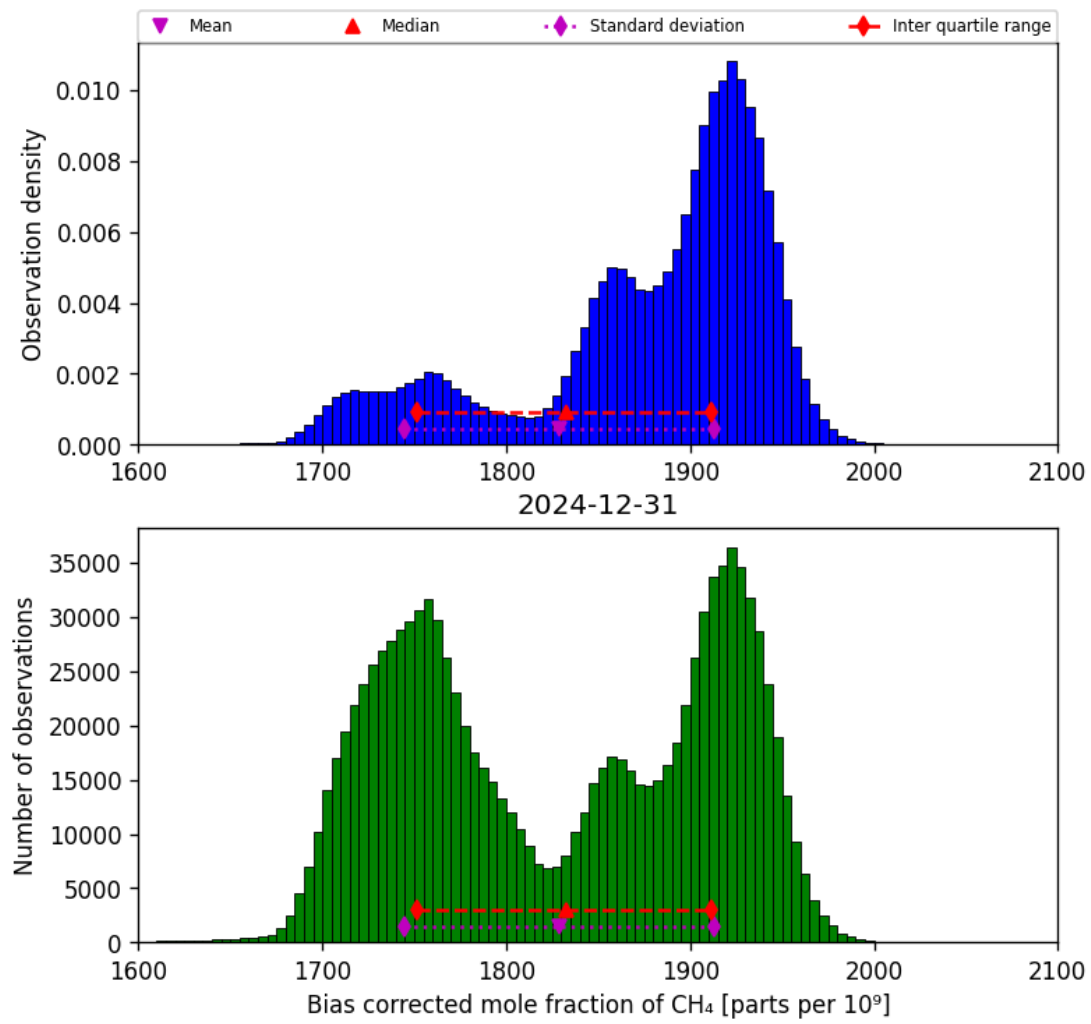
Figure 25: Histogram of “Bias corrected mole fraction of CH 4 ” for 2024-12-30 to 2025-01-01
