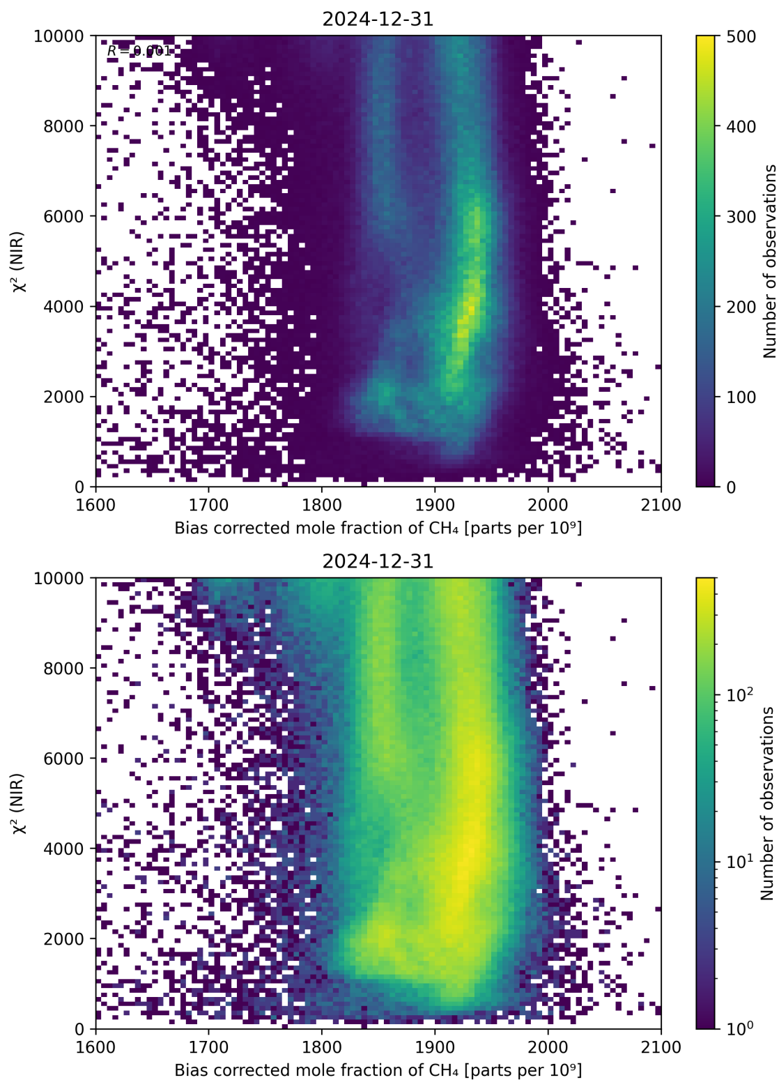
Figure 63: Scatter density plot of “Bias corrected mole fraction of \text{CH}_4 ” against “ \chi^2 (NIR)” for 2024-12-30 to 2025-01-01.
