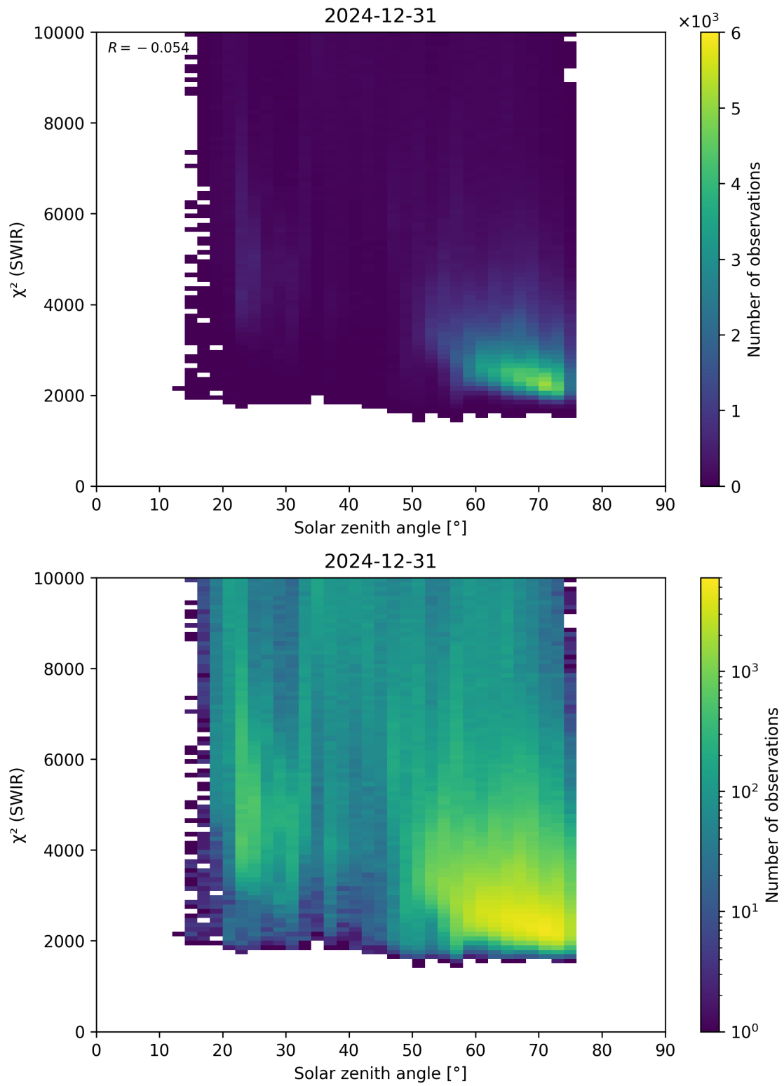
Figure 95: Scatter density plot of “Solar zenith angle” against “ \chi^2 (SWIR)” for 2024-12-30 to 2025-01-01.
