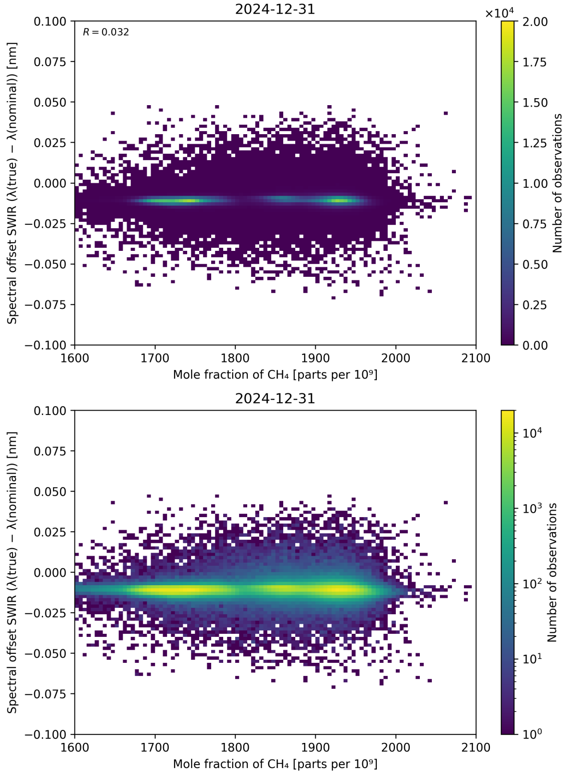
Figure 86: Scatter density plot of “Mole fraction of CH 4 ” against “Spectral offset SWIR ( \lambda_{\text{true}} - \lambda_{\text{nominal}} )” for 2024-12-30 to 2025-01-01.
