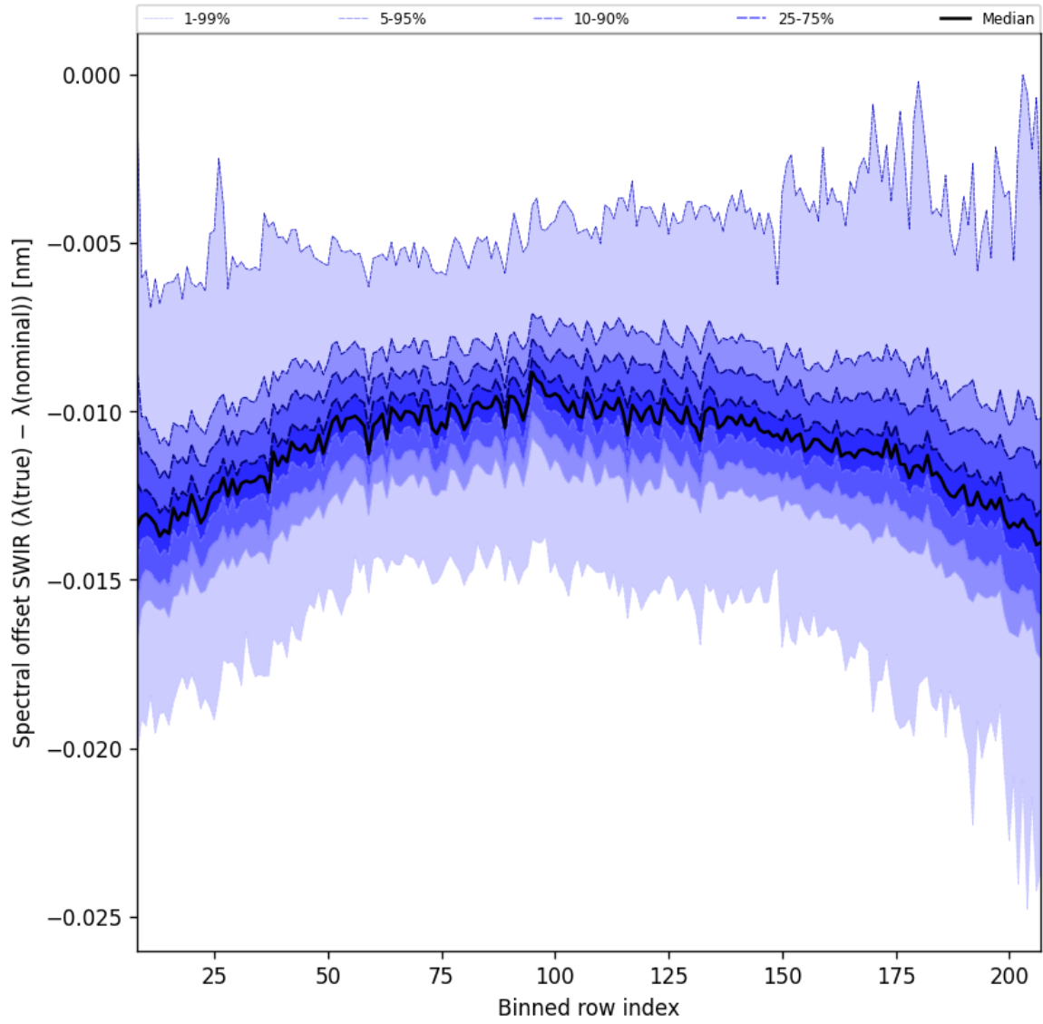
Figure 38: Along track statistics of “Spectral offset SWIR ( \lambda_{\text{true}} - \lambda_{\text{nominal}} )” for 2024-12-30 to 2025-01-01
