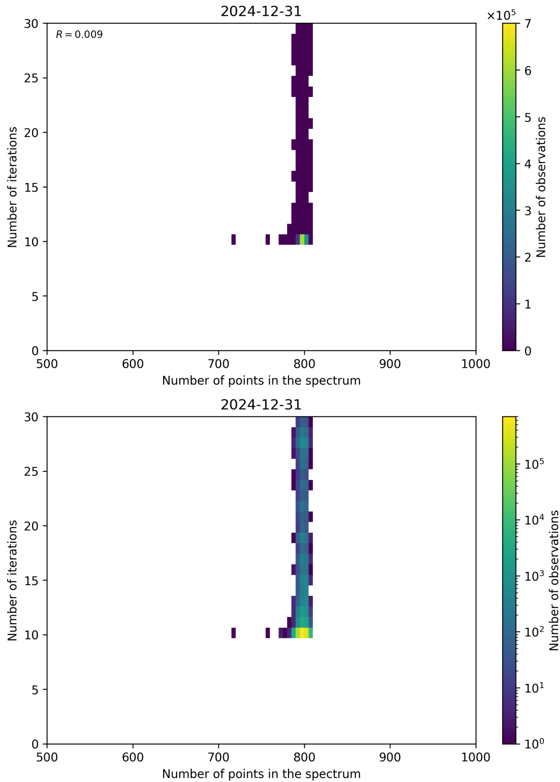
Figure 92: Scatter density plot of “Number of points in the spectrum” against “Number of iterations” for 2024-12-30 to 2025-01-01.
