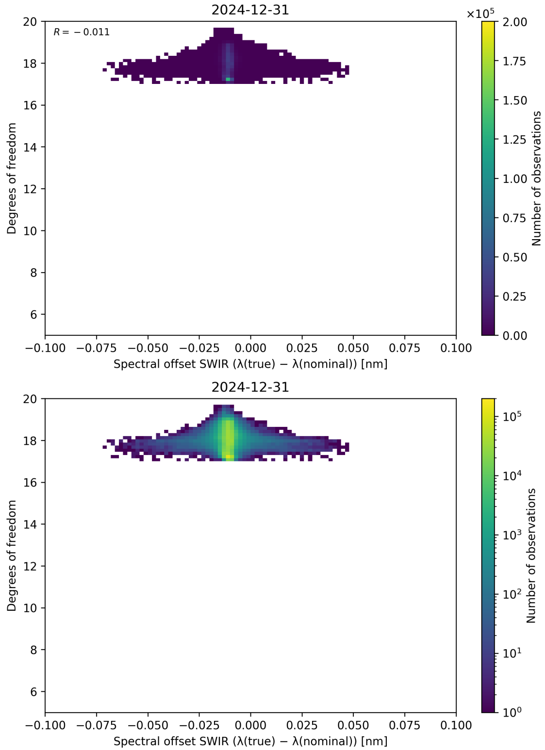
Figure 119: Scatter density plot of “Spectral offset SWIR ( \lambda_{\text{true}} - \lambda_{\text{nominal}} )” against “Degrees of freedom” for 2024-12-30 to 2025-01-01.
