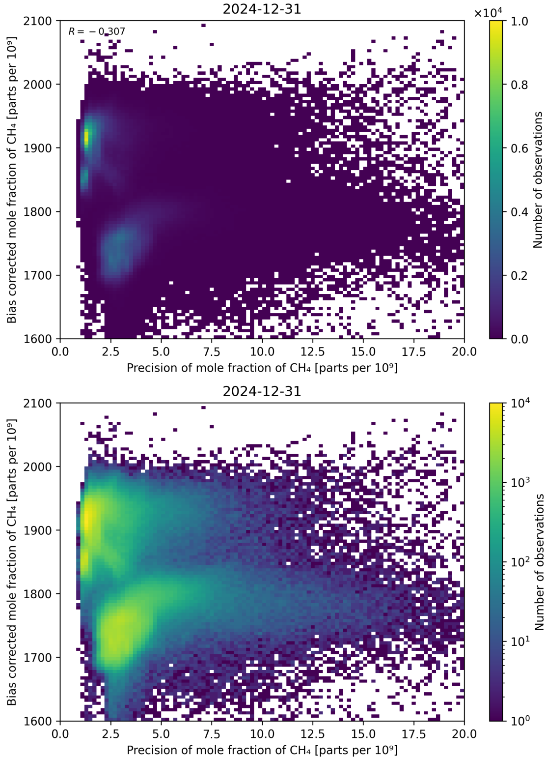
Figure 82: Scatter density plot of “Precision of mole fraction of CH 4 ” against “Bias corrected mole fraction of CH 4 ” for 2024-12-30 to 2025-01-01.
