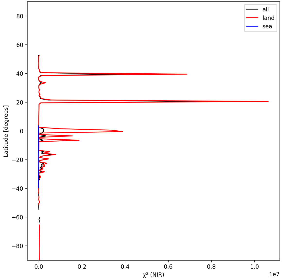
Figure 18: Zonal average of “ \chi^2 (NIR)” for 2024-12-30 to 2025-01-01.
