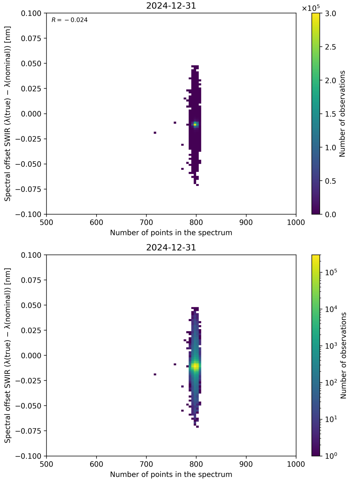
Figure 93: Scatter density plot of “Number of points in the spectrum” against “Spectral offset SWIR ( \lambda_{\text{true}} - \lambda_{\text{nominal}} )” for 2024-12-30 to 2025-01-01.
