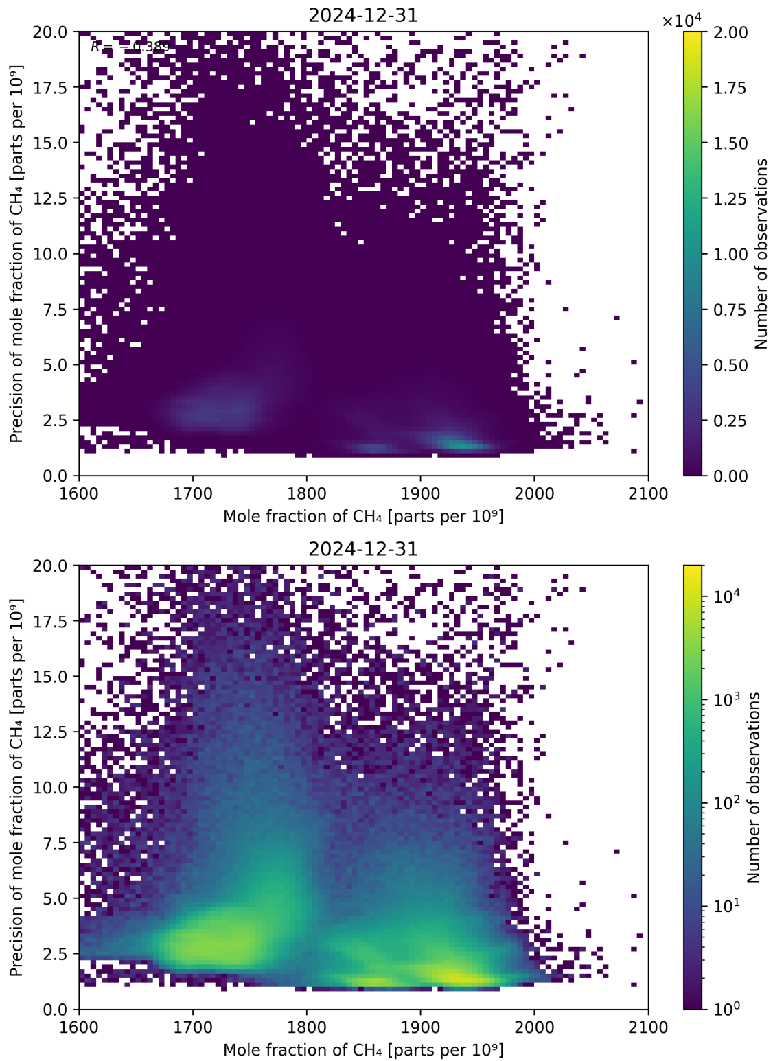
Figure 75: Scatter density plot of “Mole fraction of CH 4 ” against “Precision of mole fraction of CH 4 ” for 2024-12-30 to 2025-01-01.
