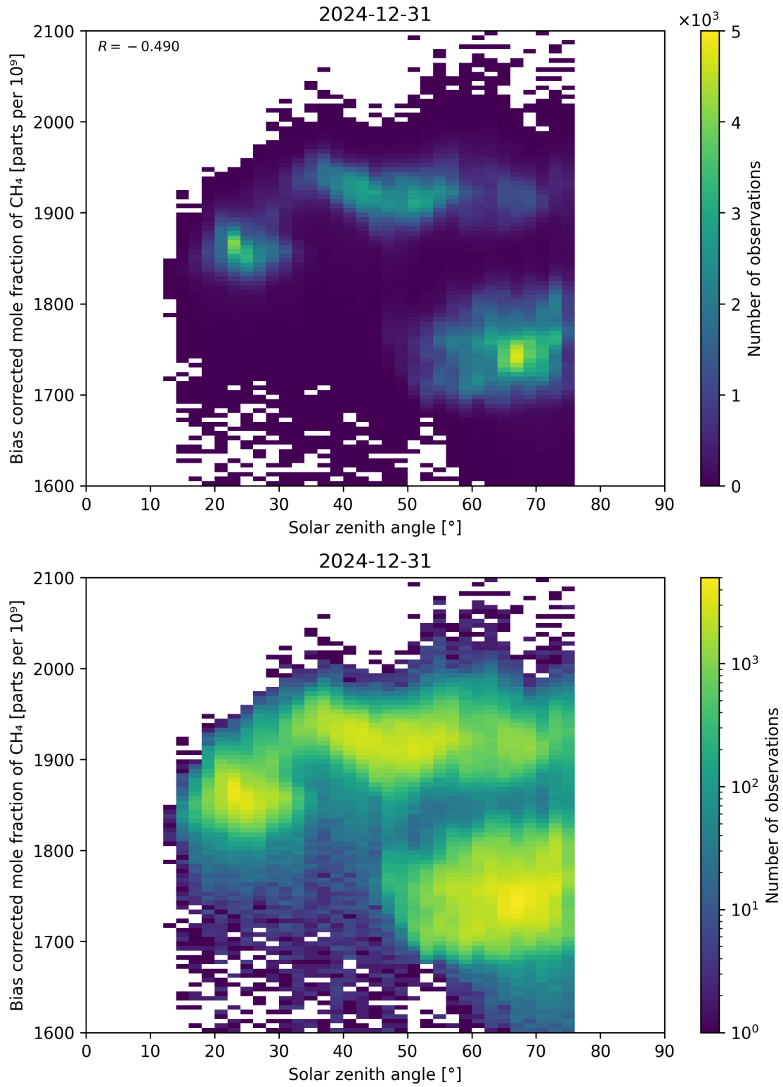
Figure 100: Scatter density plot of “Solar zenith angle” against “Bias corrected mole fraction of CH 4 ” for 2024-12-30 to 2025-01-01.
