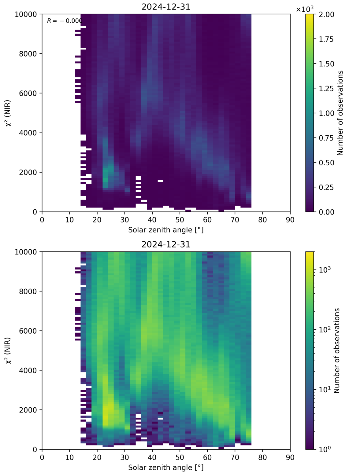
Figure 94: Scatter density plot of “Solar zenith angle” against “ \chi^2 (NIR)” for 2024-12-30 to 2025-01-01.
