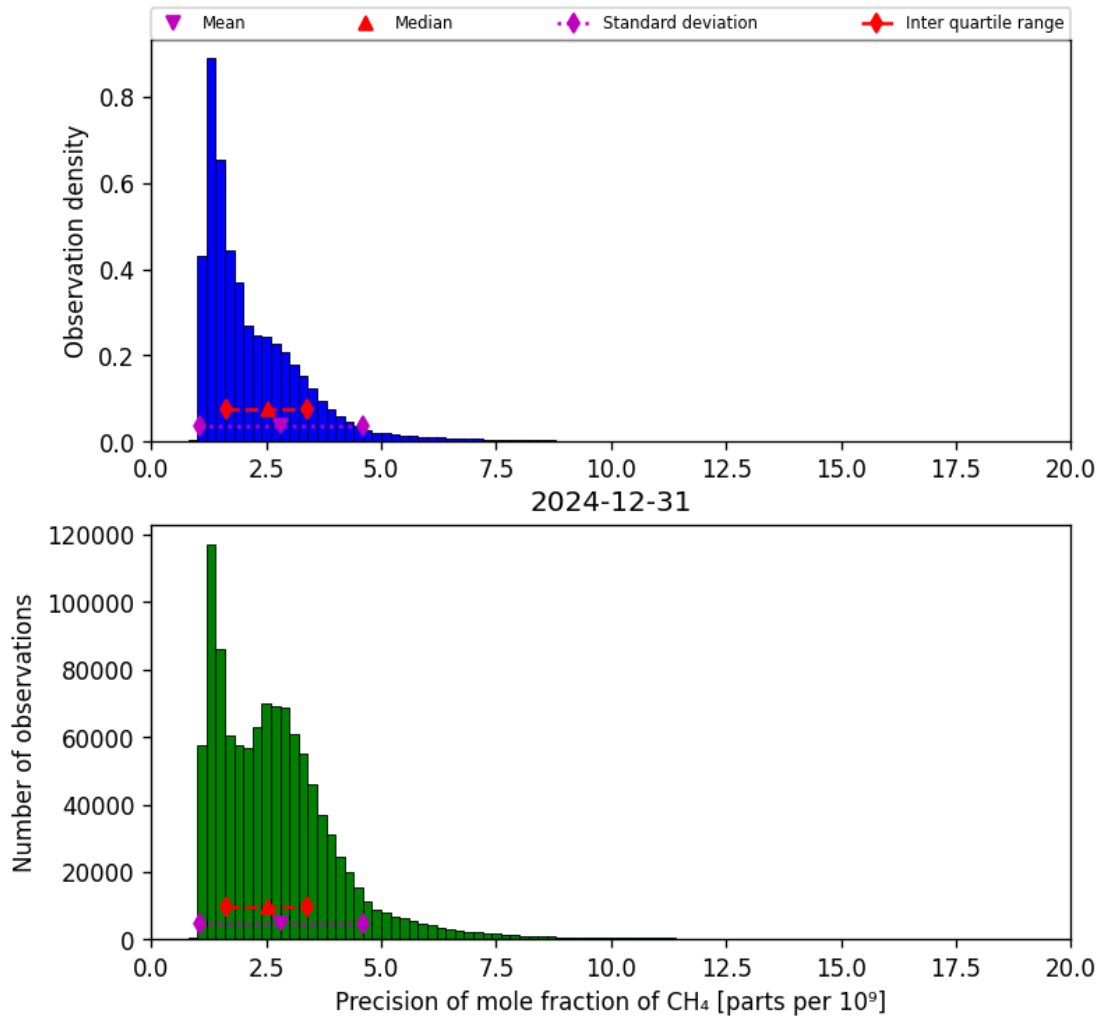
Figure 24: Histogram of “Precision of mole fraction of CH 4 ” for 2024-12-30 to 2025-01-01
