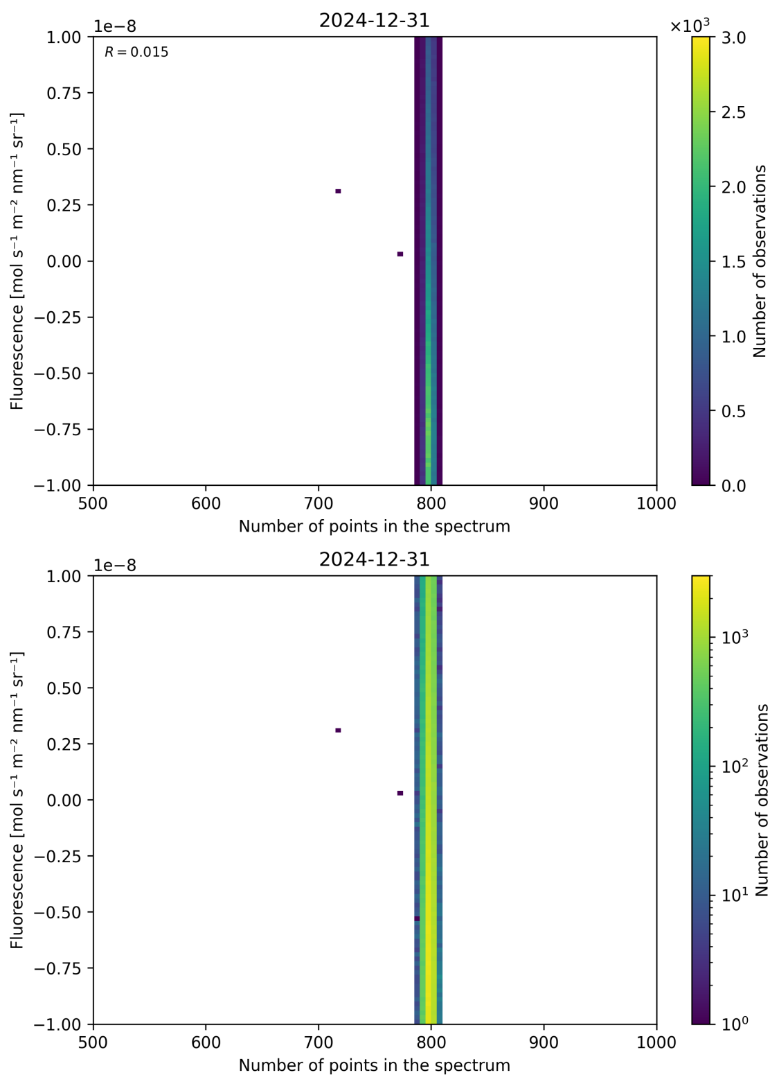
Figure 91: Scatter density plot of “Number of points in the spectrum” against “Fluorescence” for 2024-12-30 to 2025-01-01.
