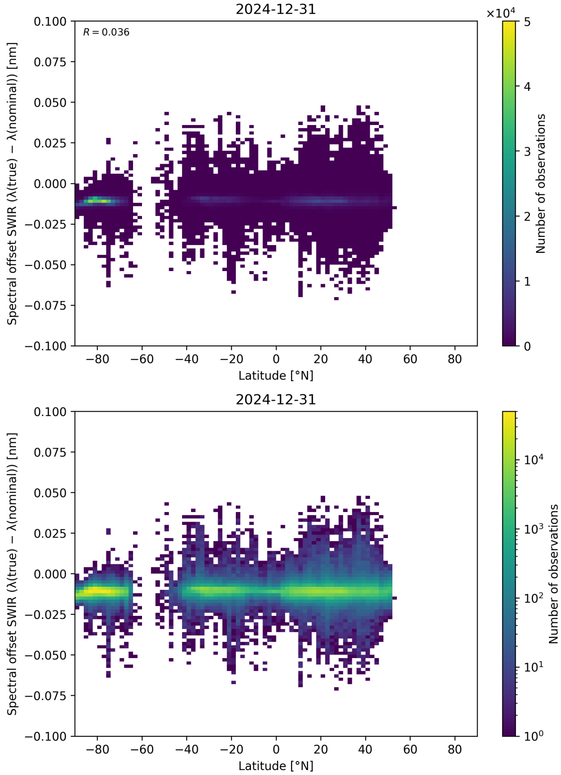
Figure 62: Scatter density plot of “Latitude” against “Spectral offset SWIR ( \lambda_{\text{true}} - \lambda_{\text{nominal}} )” for 2024-12-30 to 2025-01-01.
