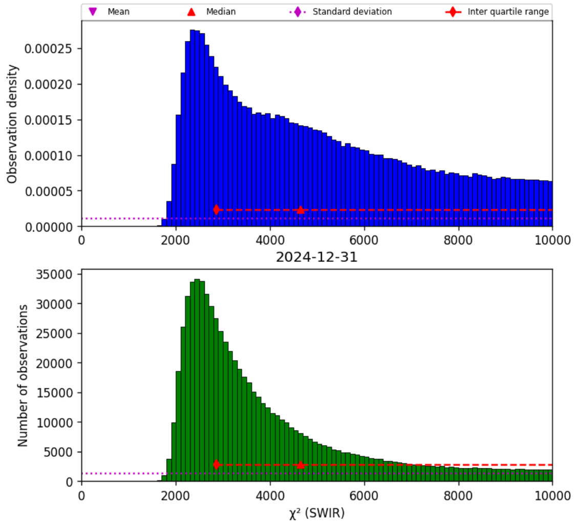
Figure 28: Histogram of “ \chi^2 (SWIR)” for 2024-12-30 to 2025-01-01
