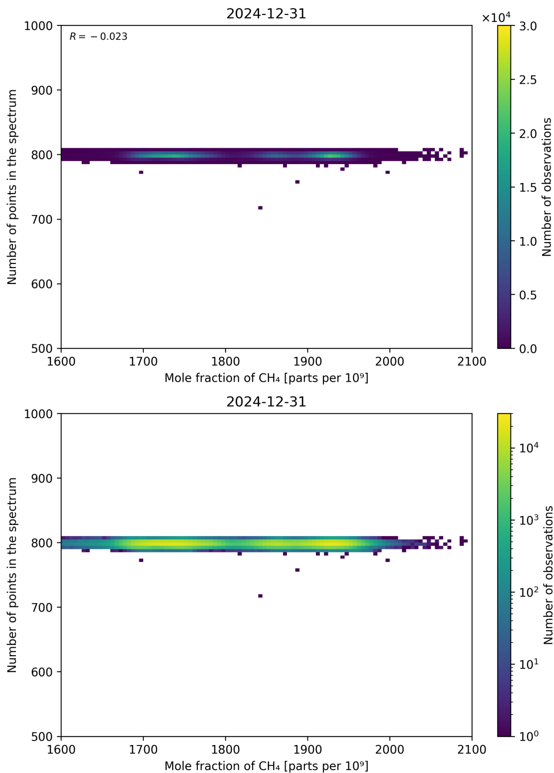
Figure 77: Scatter density plot of “Mole fraction of CH 4 ” against “Number of points in the spectrum” for 2024-12-30 to 2025-01-01.
