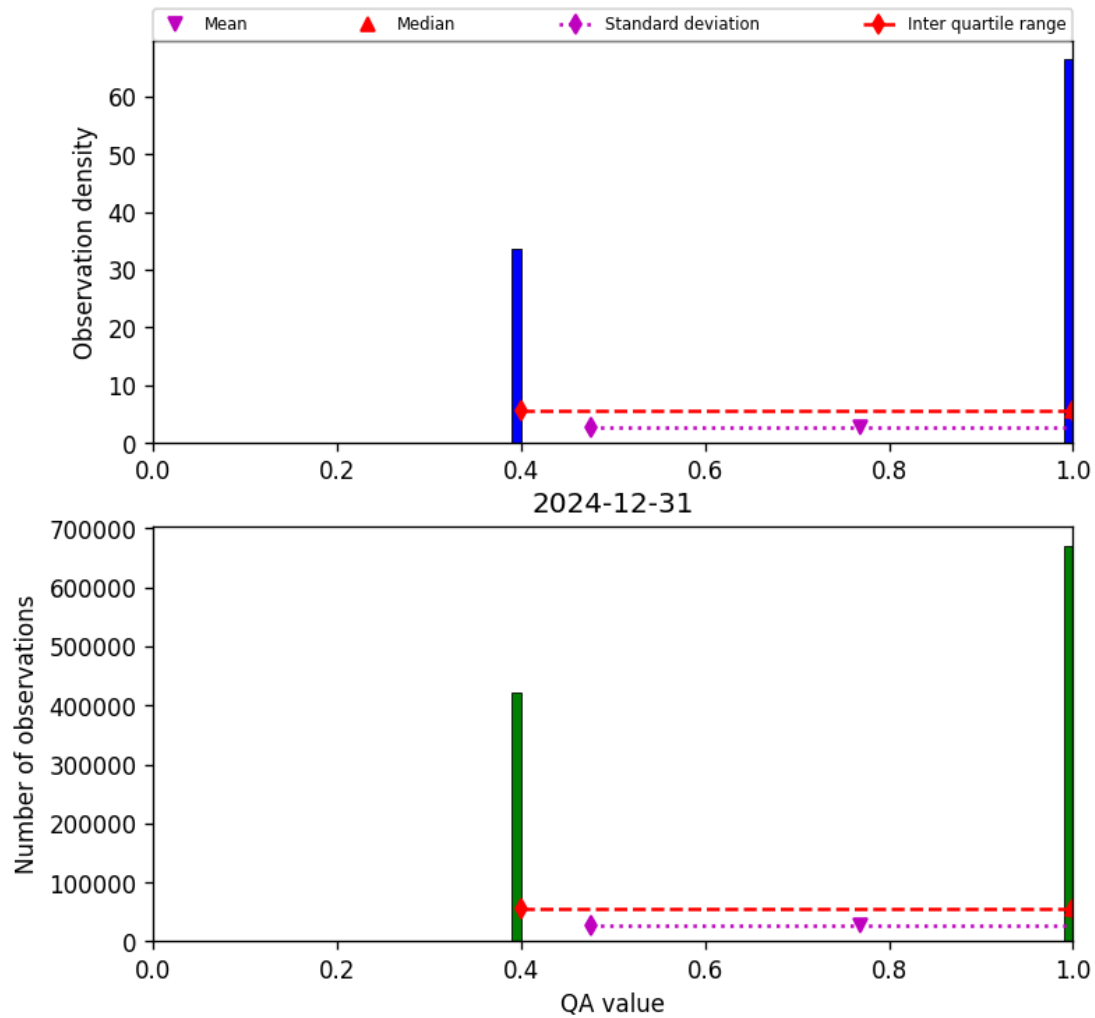
Figure 22: Histogram of “QA value” for 2024-12-30 to 2025-01-01
