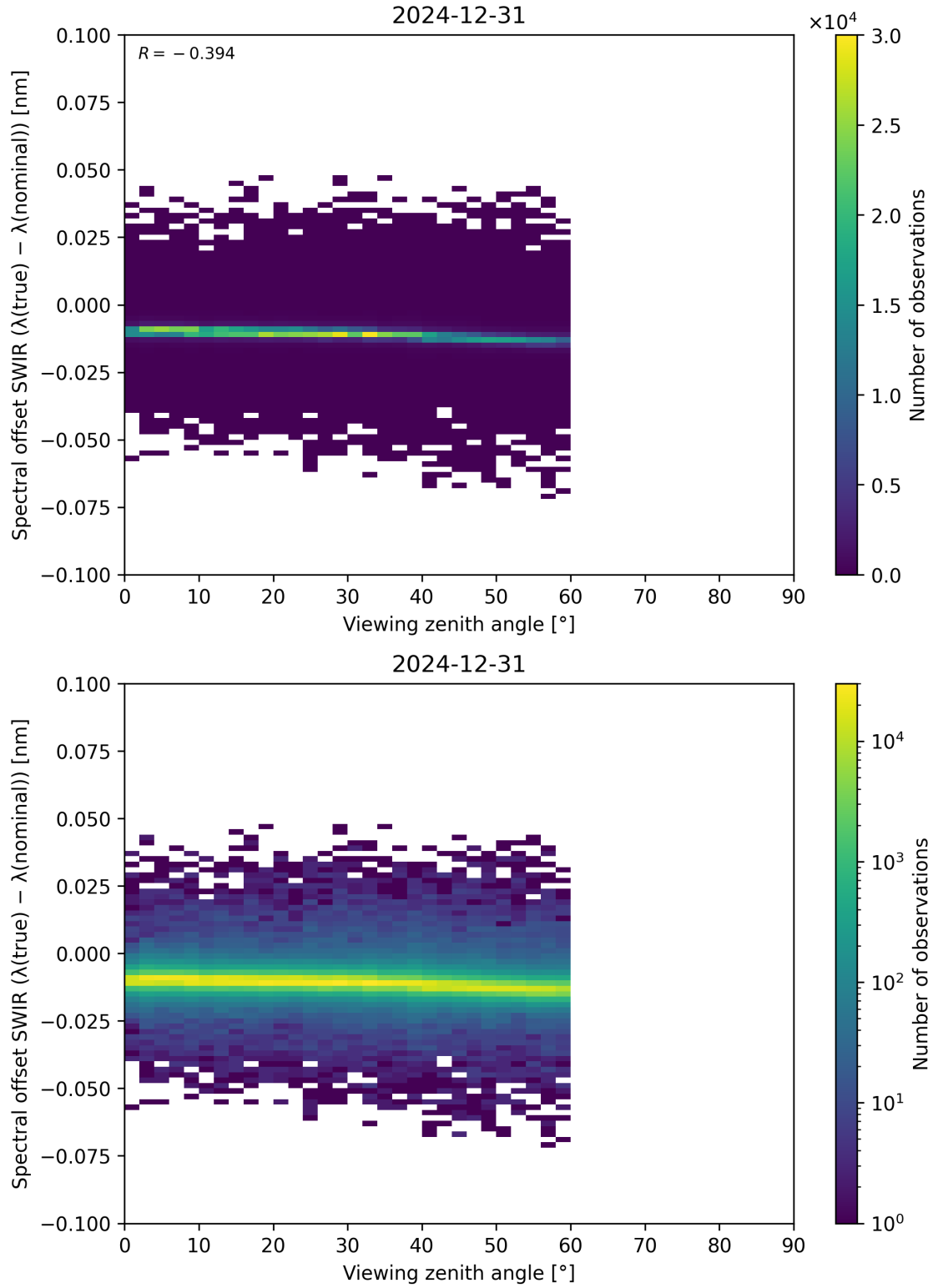
Figure 116: Scatter density plot of “Viewing zenith angle” against “Spectral offset SWIR ( \lambda_{\text{true}} - \lambda_{\text{nominal}} )” for 2024-12-30 to 2025-01-01.
