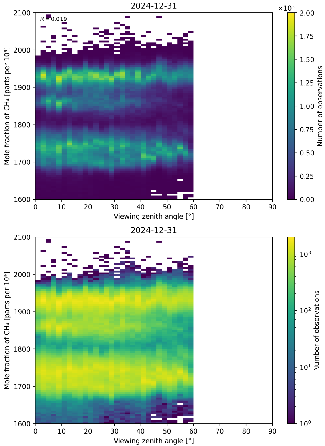
Figure 110: Scatter density plot of “Viewing zenith angle” against “Mole fraction of CH 4 ” for 2024-12-30 to 2025-01-01.
