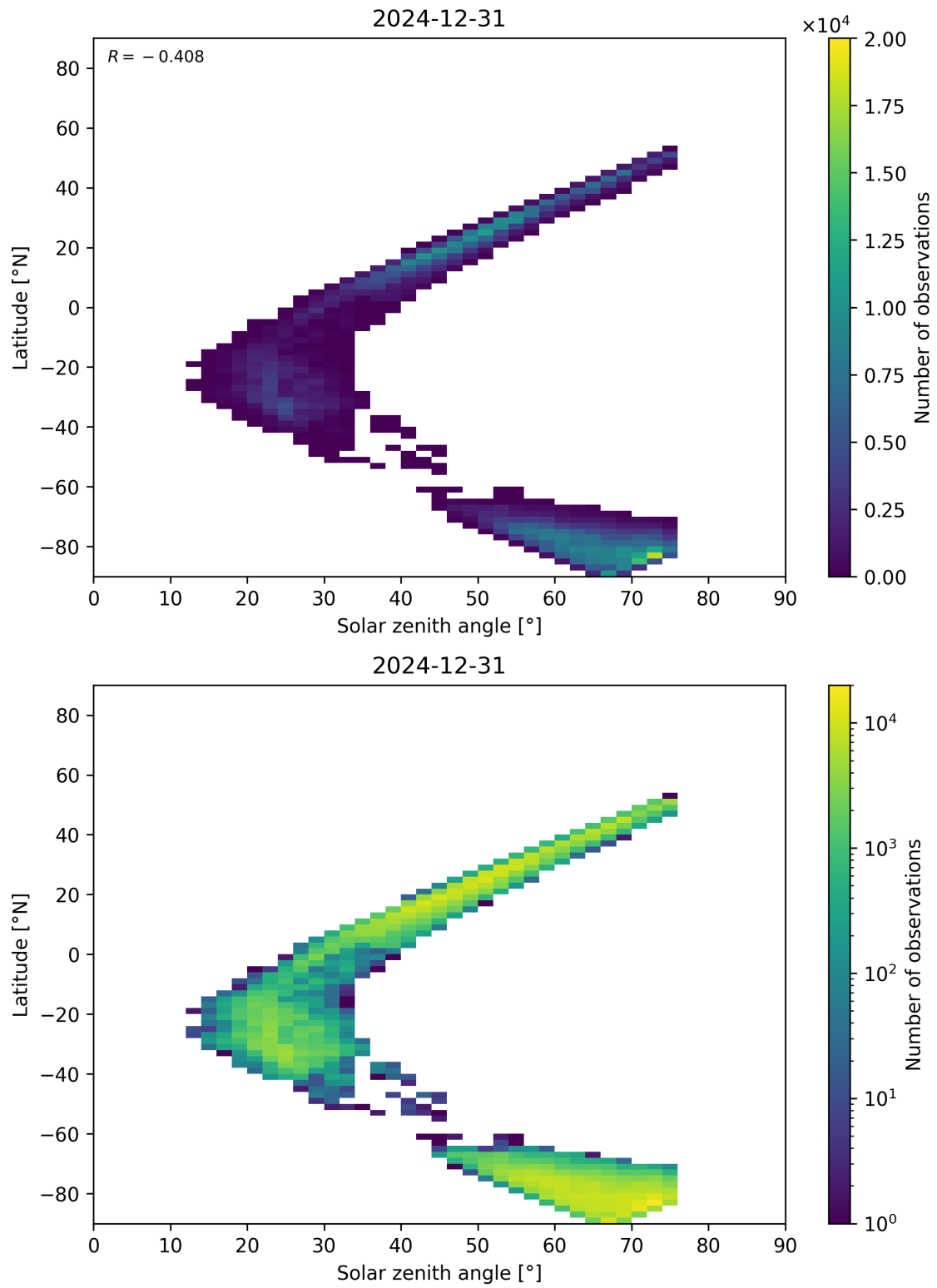
Figure 98: Scatter density plot of “Solar zenith angle” against “Latitude” for 2024-12-30 to 2025-01-01.
