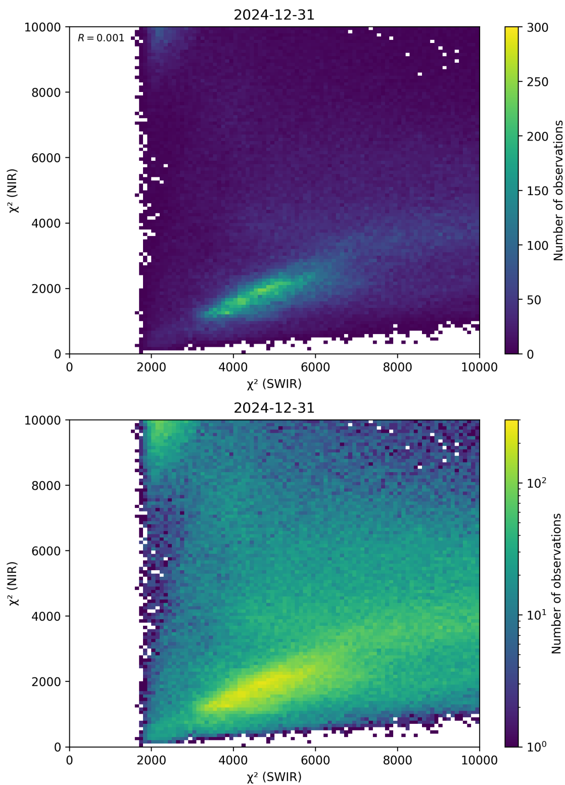
Figure 47: Scatter density plot of “ \chi^2 (SWIR)” against “ \chi^2 (NIR)” for 2024-12-30 to 2025-01-01.
