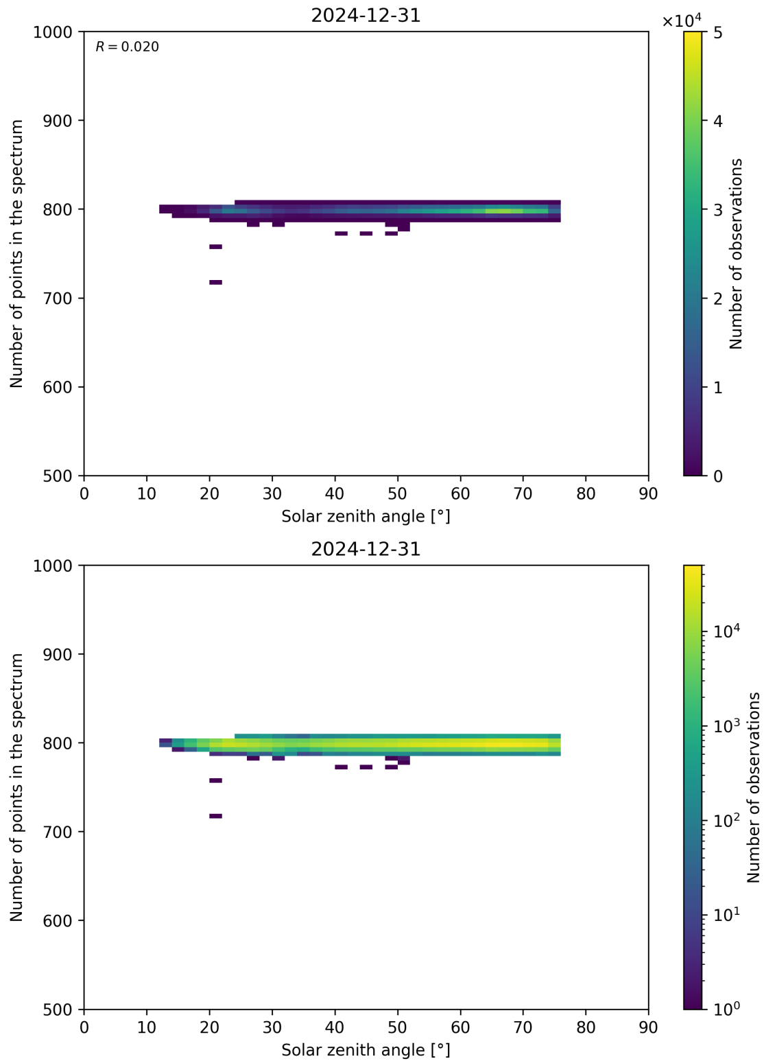
Figure 103: Scatter density plot of “Solar zenith angle” against “Number of points in the spectrum” for 2024-12-30 to 2025-01-01.
