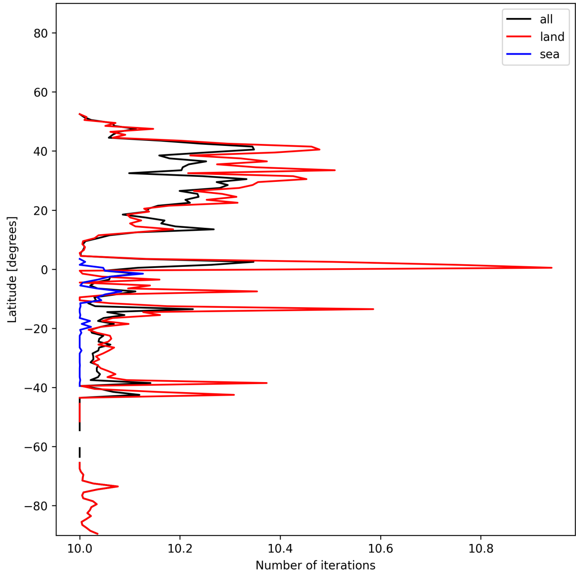
Figure 20: Zonal average of “Number of iterations” for 2024-12-30 to 2025-01-01.
