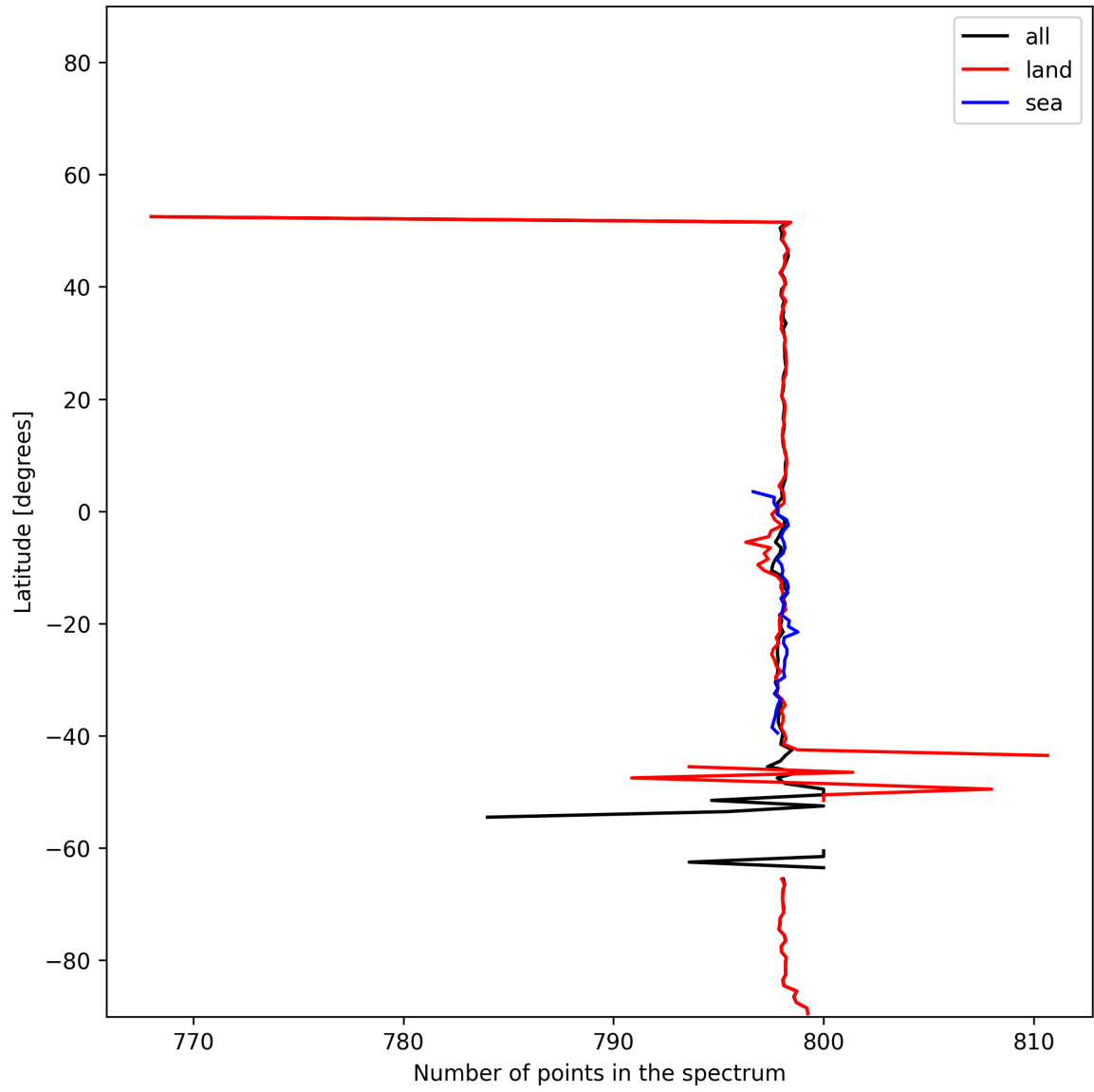
Figure 15: Zonal average of “Number of points in the spectrum” for 2024-12-30 to 2025-01-01.
