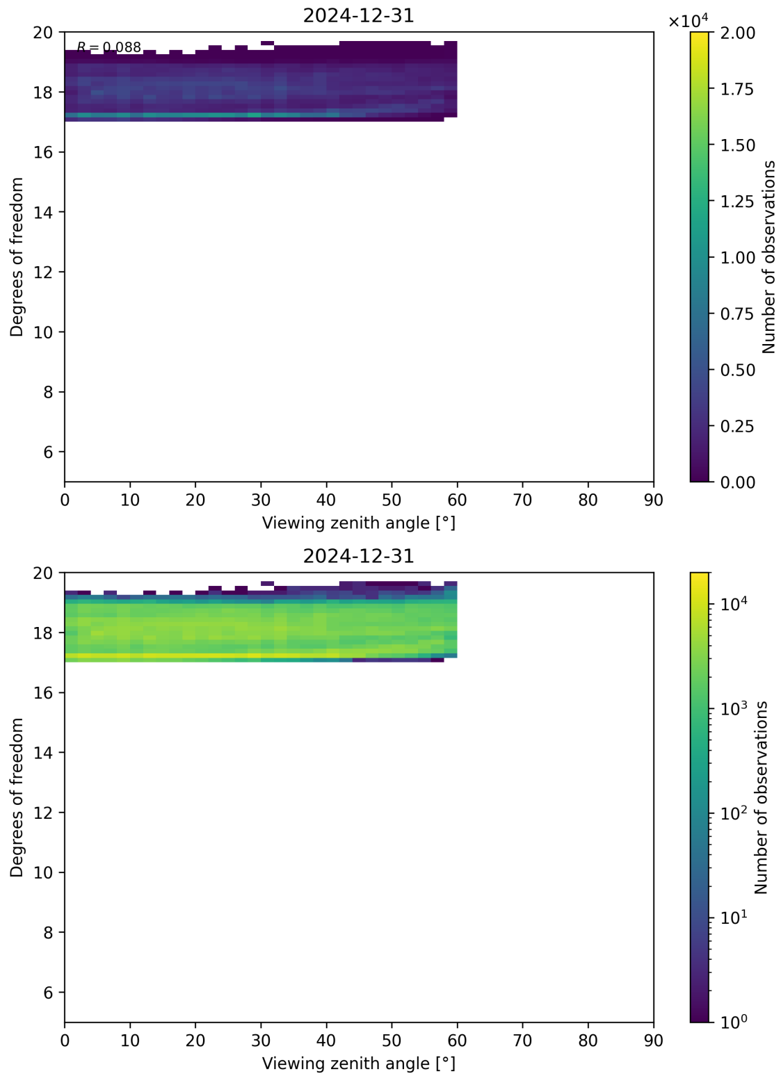
Figure 107: Scatter density plot of “Viewing zenith angle” against “Degrees of freedom” for 2024-12-30 to 2025-01-01.
