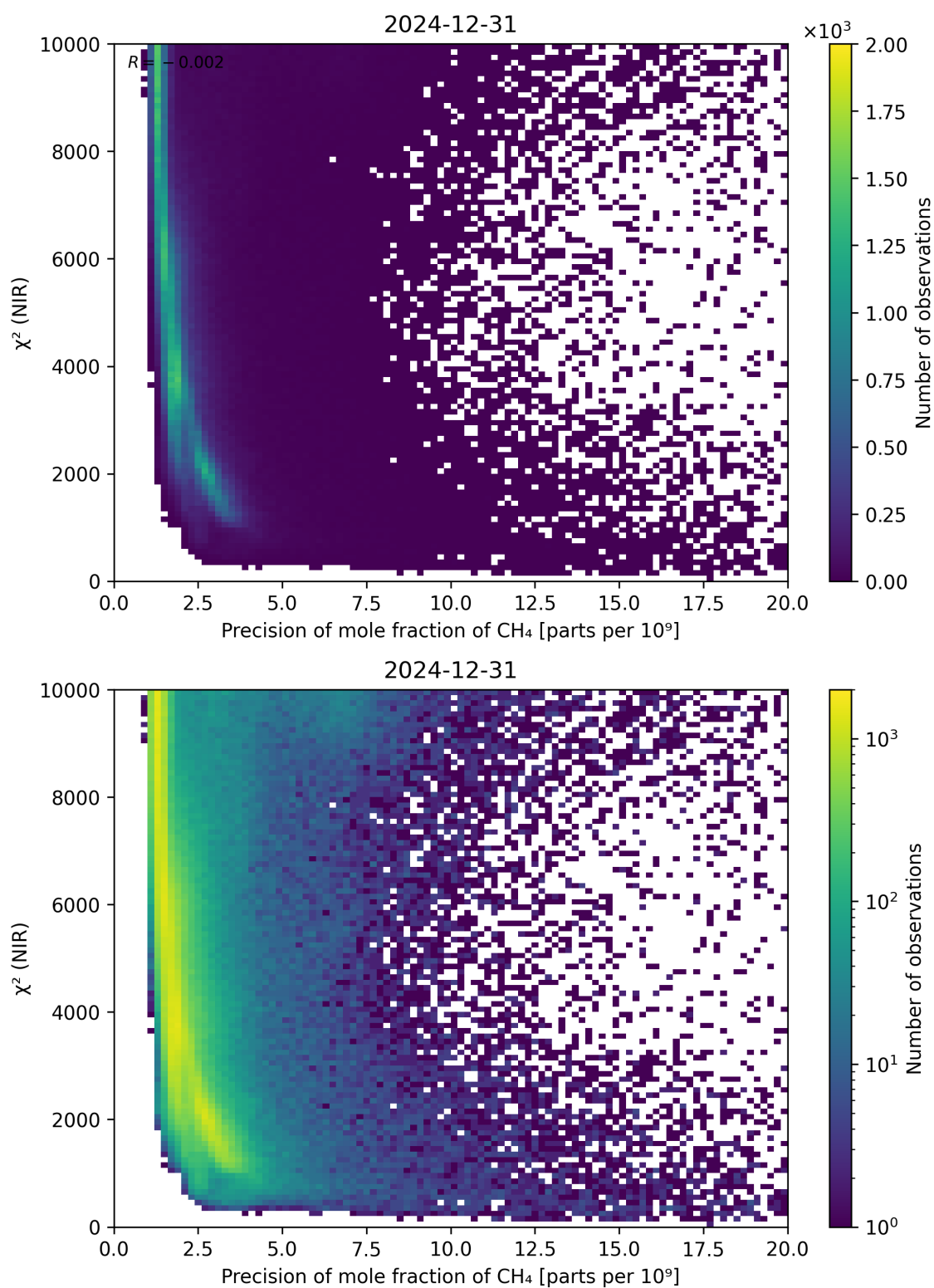
Figure 78: Scatter density plot of “Precision of mole fraction of \text{CH}_4 ” against “ \chi^2 (NIR)” for 2024-12-30 to 2025-01-01.
