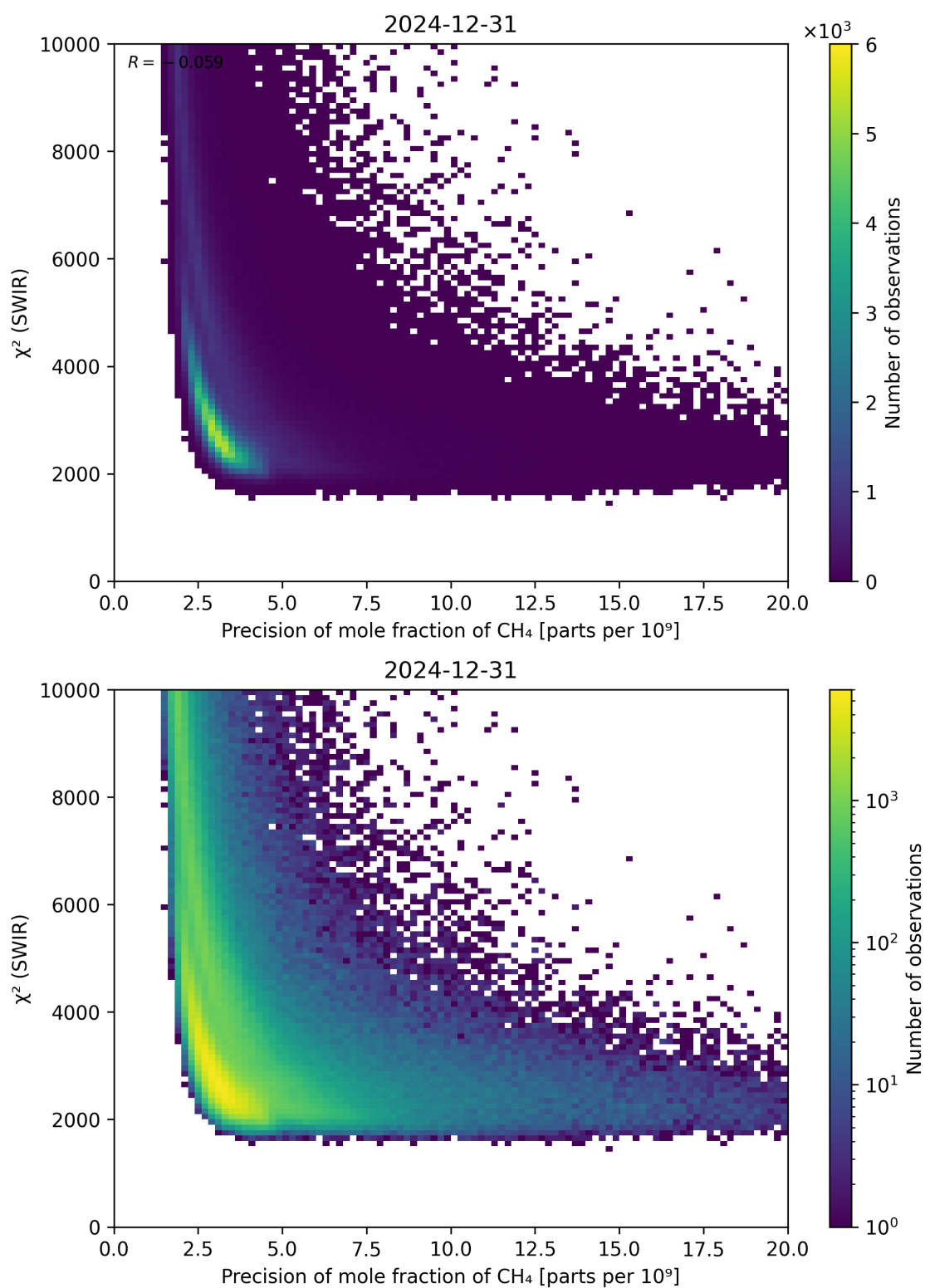
Figure 79: Scatter density plot of “Precision of mole fraction of CH 4 ” against “ \chi^2 (SWIR)” for 2024-12-30 to 2025-01-01.
