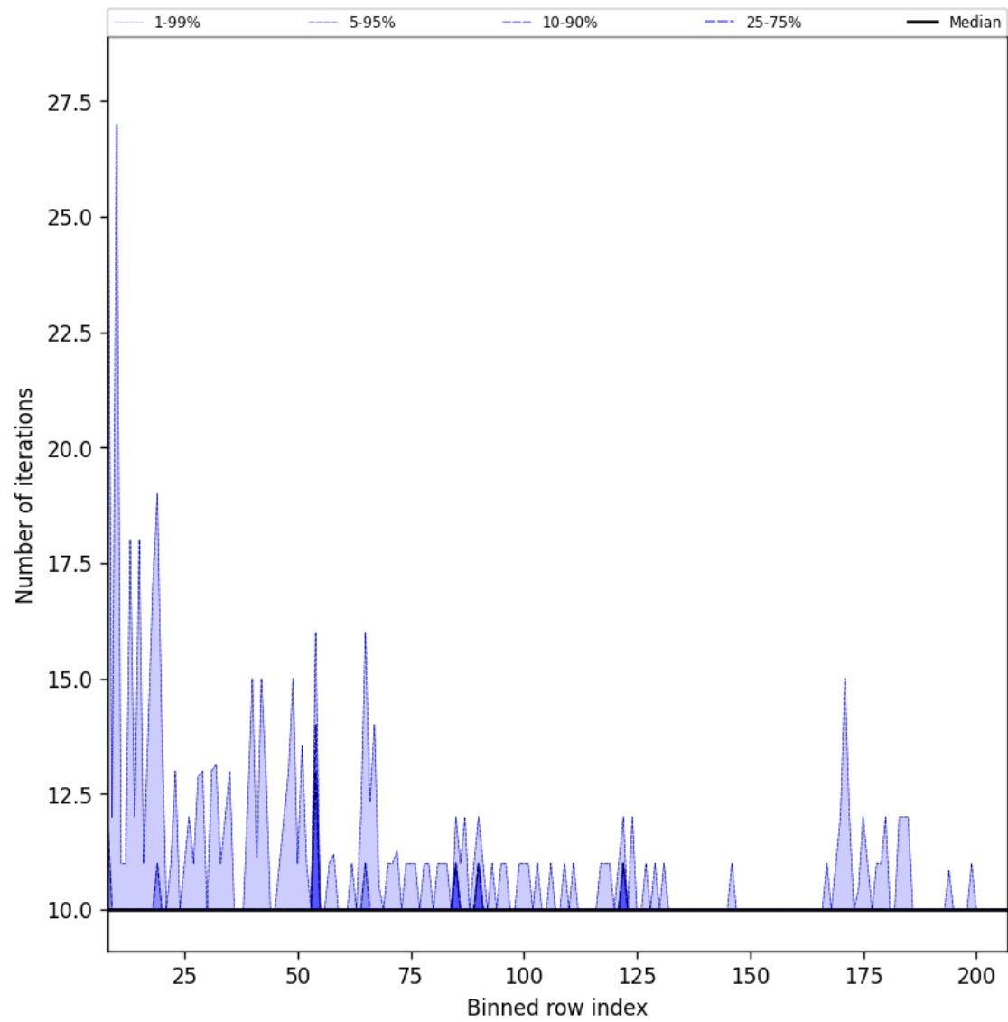
Figure 42: Along track statistics of “Number of iterations” for 2024-12-30 to 2025-01-01
