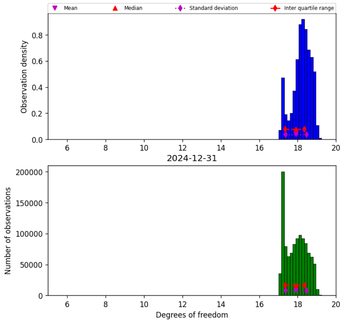
Figure 30: Histogram of “Degrees of freedom” for 2024-12-30 to 2025-01-01
