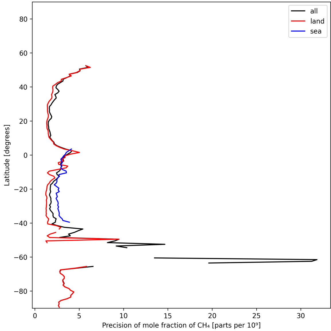
Figure 13: Zonal average of “Precision of mole fraction of CH 4 ” for 2024-12-30 to 2025-01-01.
