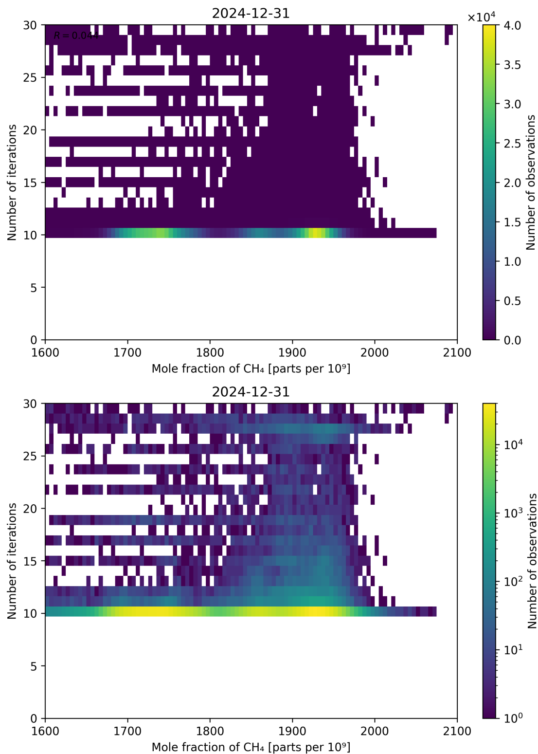
Figure 76: Scatter density plot of “Mole fraction of CH 4 ” against “Number of iterations” for 2024-12-30 to 2025-01-01.
