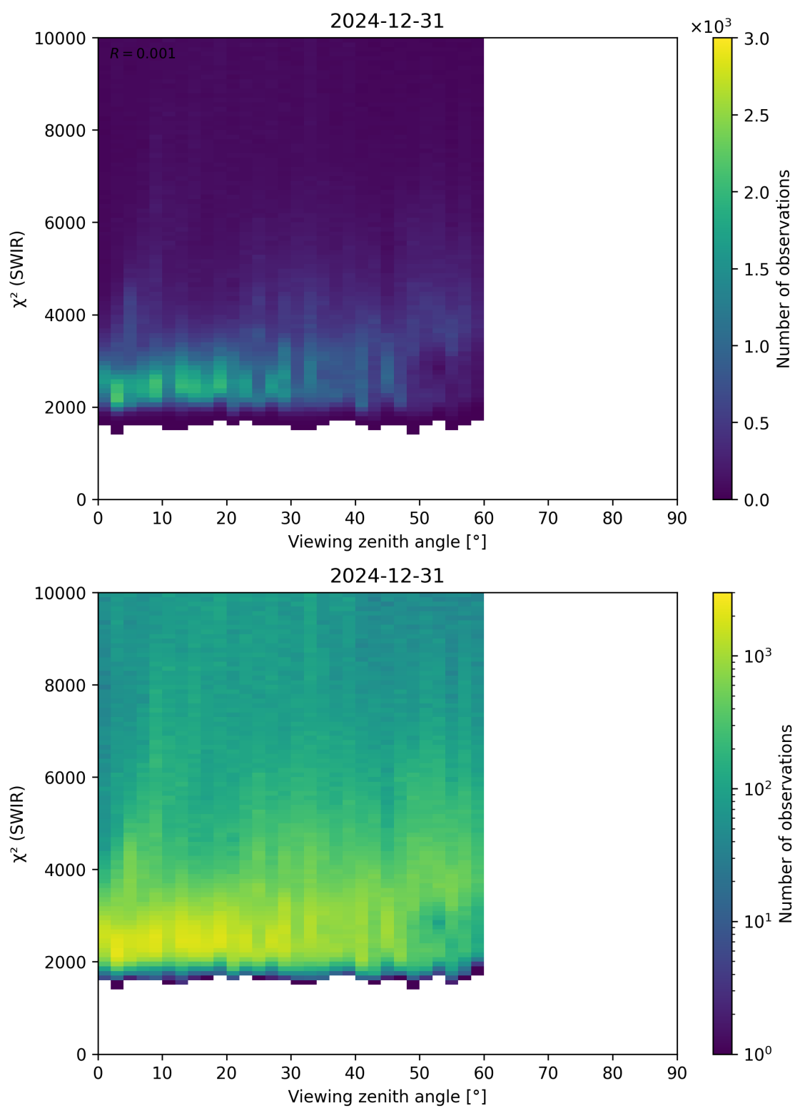
Figure 106: Scatter density plot of “Viewing zenith angle” against “ \chi^2 (SWIR)” for 2024-12-30 to 2025-01-01.
