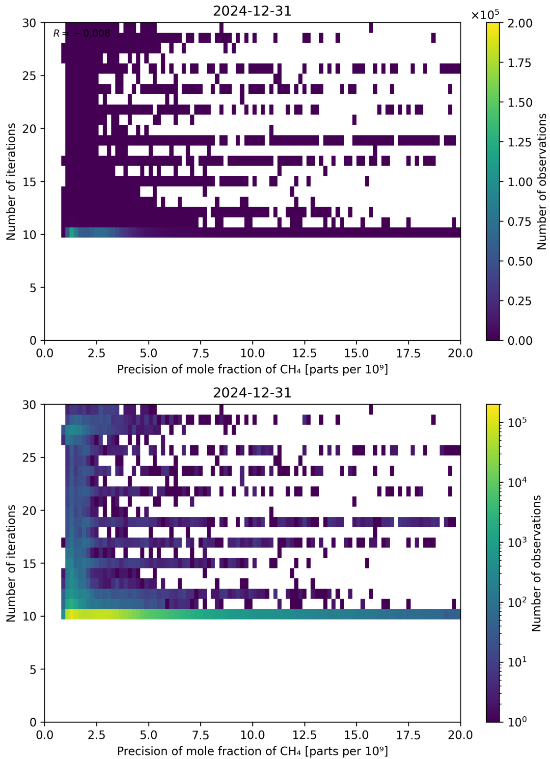
Figure 83: Scatter density plot of “Precision of mole fraction of CH 4 ” against “Number of iterations” for 2024-12-30 to 2025-01-01.
