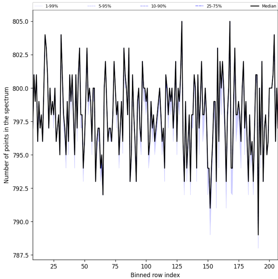
Figure 37: Along track statistics of “Number of points in the spectrum” for 2024-12-30 to 2025-01-01
