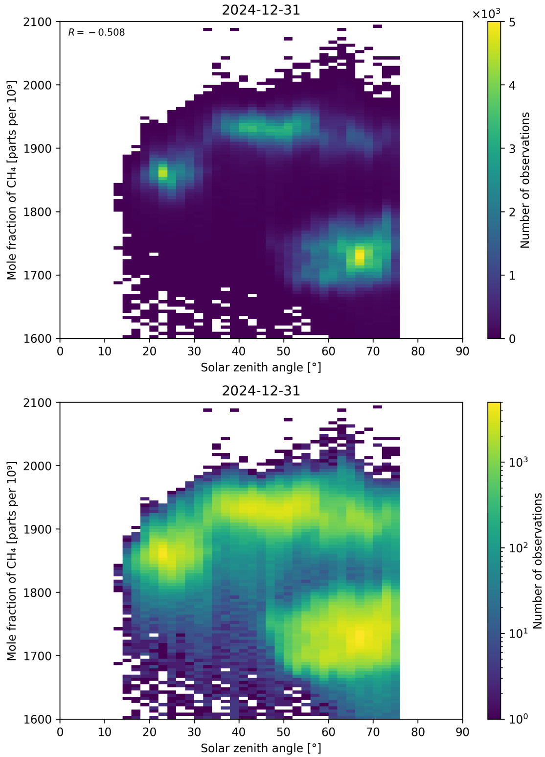
Figure 99: Scatter density plot of “Solar zenith angle” against “Mole fraction of CH 4 ” for 2024-12-30 to 2025-01-01.
