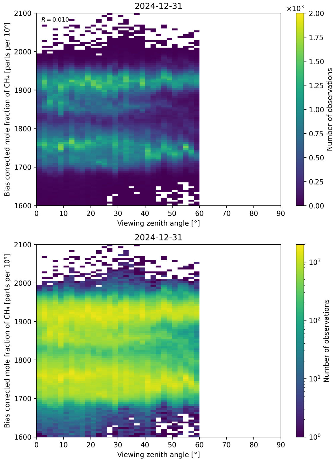
Figure 111: Scatter density plot of “Viewing zenith angle” against “Bias corrected mole fraction of CH 4 ” for 2024-12-30 to 2025-01-01.
