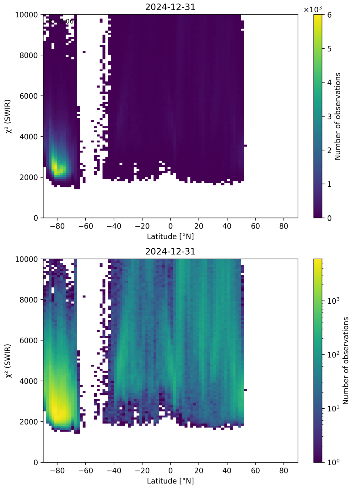
Figure 54: Scatter density plot of “Latitude” against “ \chi^2 (SWIR)” for 2024-12-30 to 2025-01-01.
