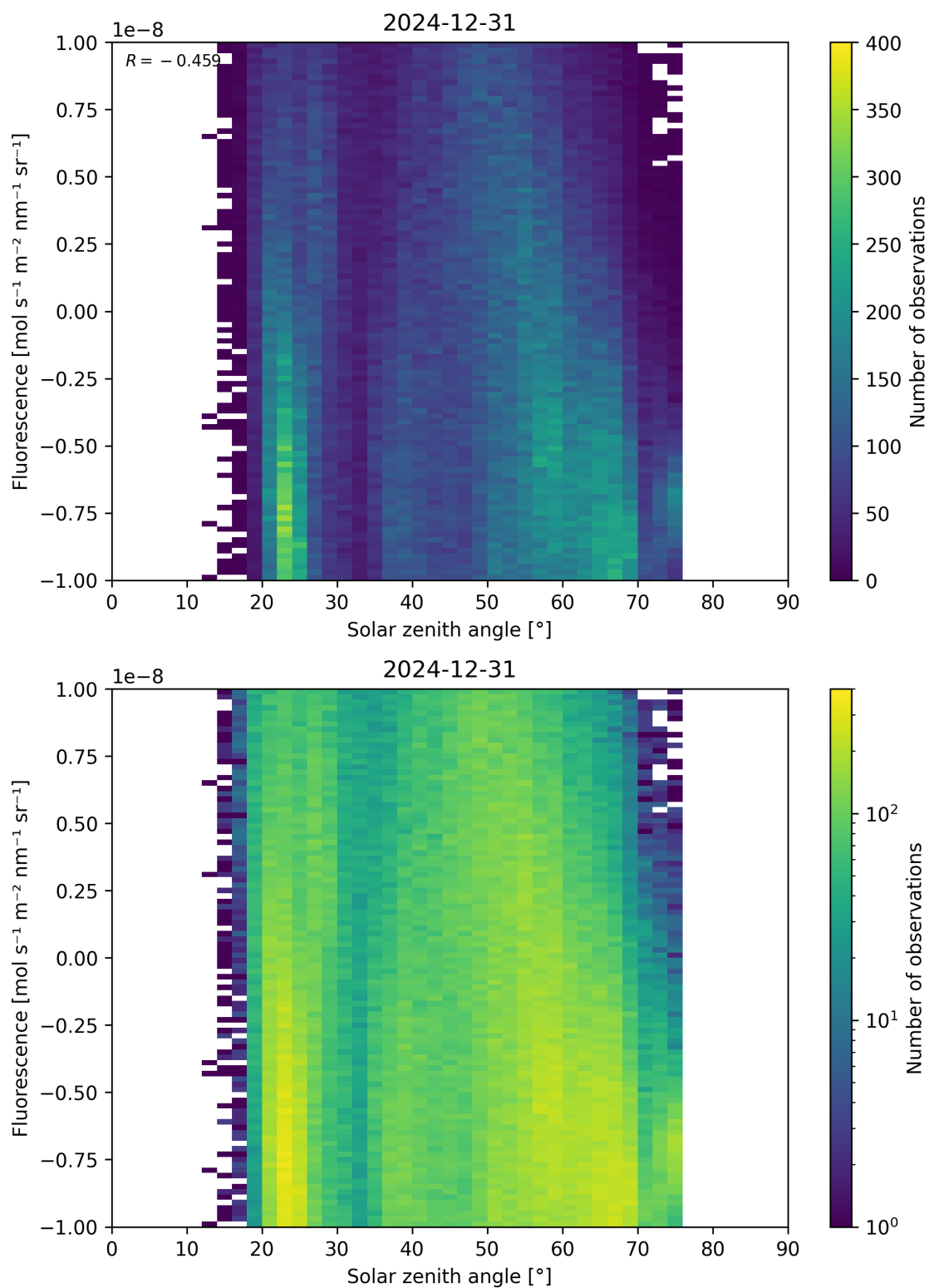
Figure 97: Scatter density plot of “Solar zenith angle” against “Fluorescence” for 2024-12-30 to 2025-01-01.
