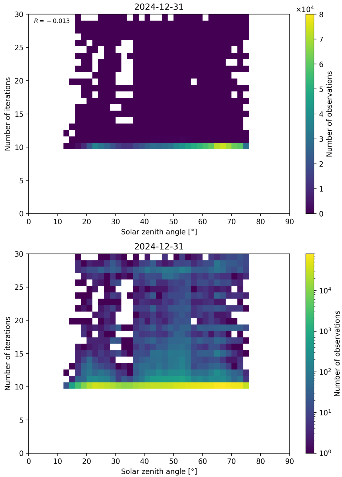
Figure 102: Scatter density plot of “Solar zenith angle” against “Number of iterations” for 2024-12-30 to 2025-01-01.
