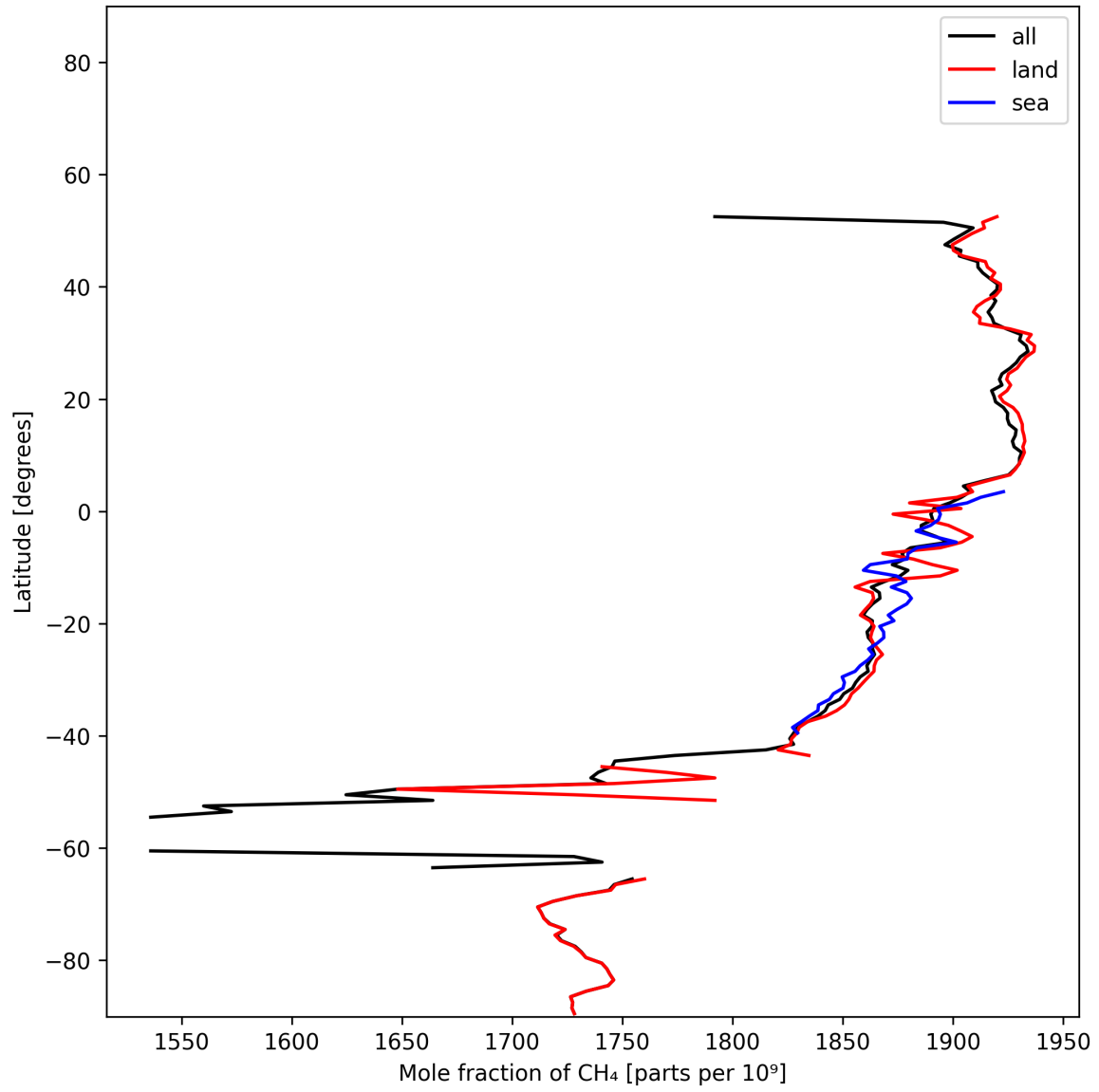
Figure 12: Zonal average of “Mole fraction of CH 4 ” for 2024-12-30 to 2025-01-01.
