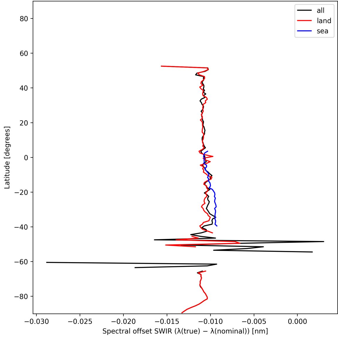
Figure 16: Zonal average of “Spectral offset SWIR ( \lambda_{\text{true}} - \lambda_{\text{nominal}} )” for 2024-12-30 to 2025-01-01.
