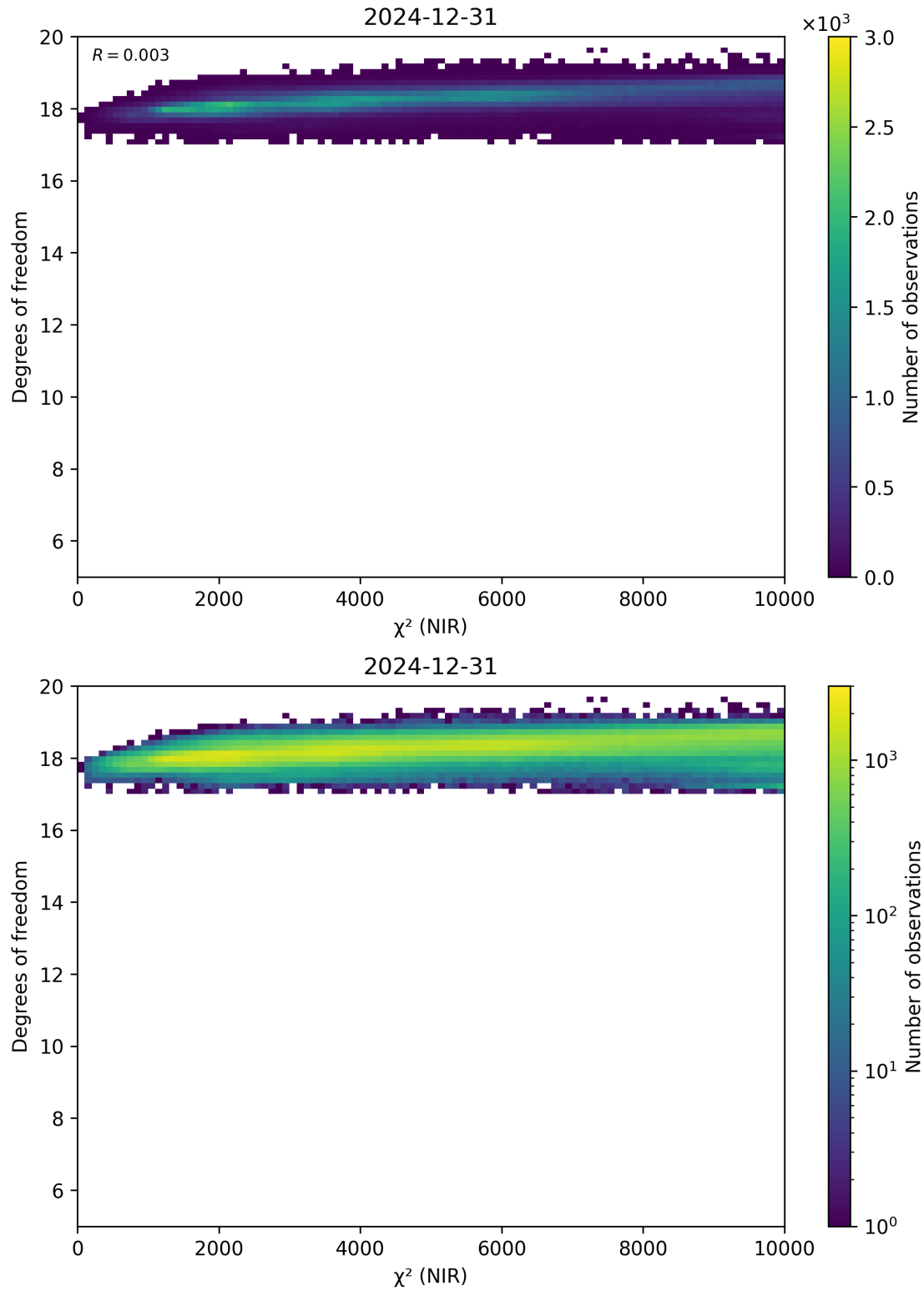
Figure 44: Scatter density plot of “ \chi^2 (NIR)” against “Degrees of freedom” for 2024-12-30 to 2025-01-01.
