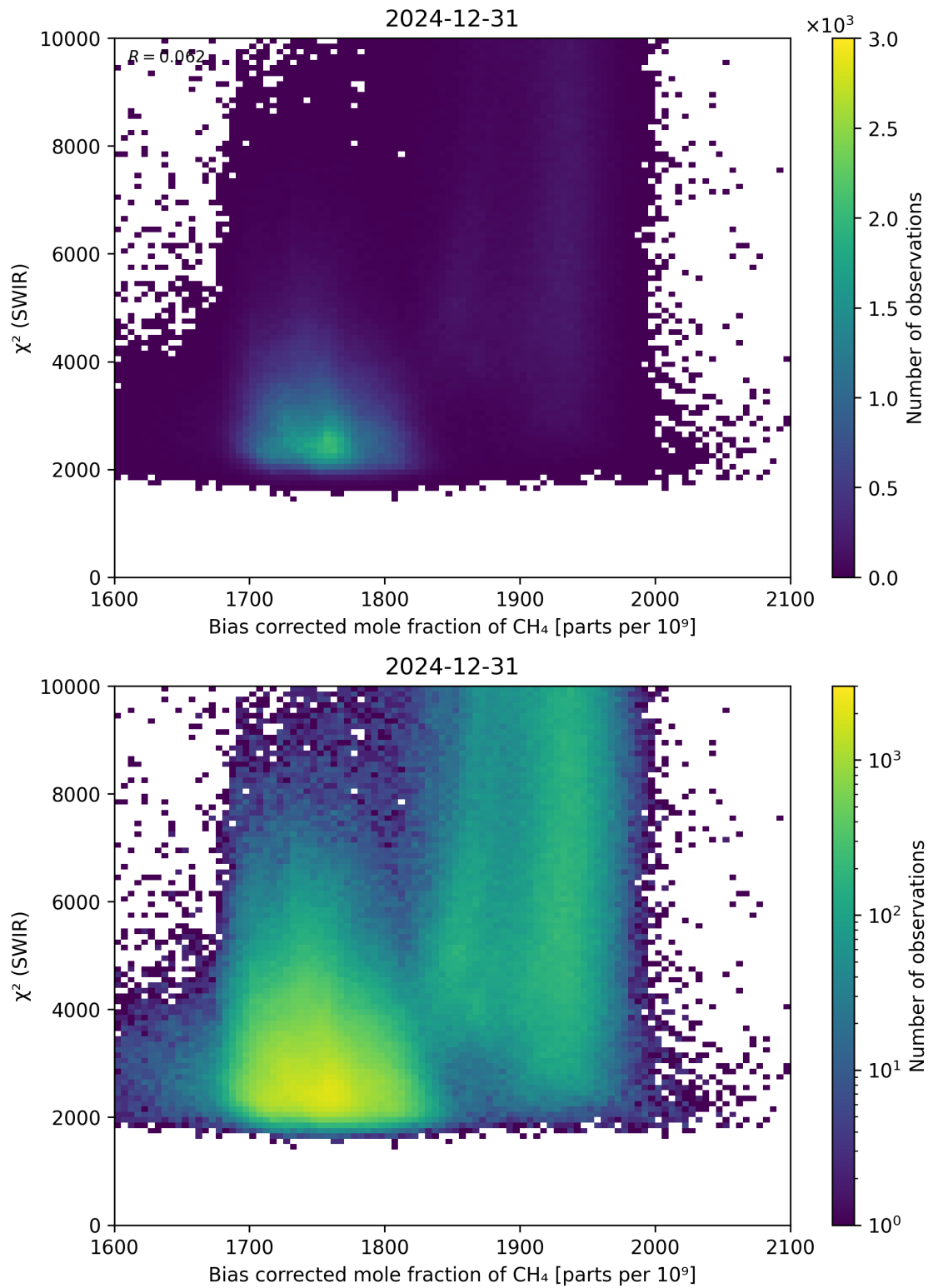
Figure 64: Scatter density plot of “Bias corrected mole fraction of \text{CH}_4 ” against “ \chi^2 (SWIR)” for 2024-12-30 to 2025-01-01.
