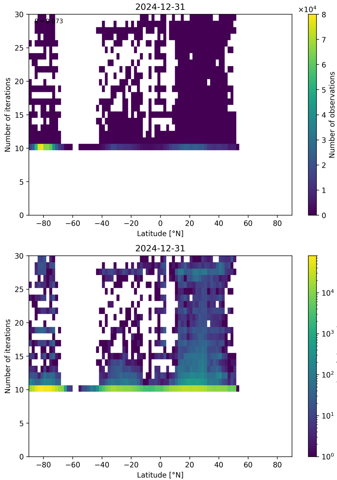
Figure 60: Scatter density plot of “Latitude” against “Number of iterations” for 2024-12-30 to 2025-01-01.
