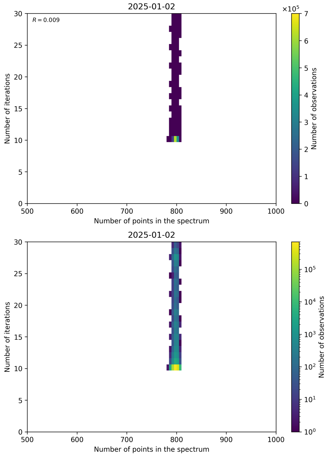
Figure 92: Scatter density plot of “Number of points in the spectrum” against “Number of iterations” for 2025-01-01 to 2025-01-03.
