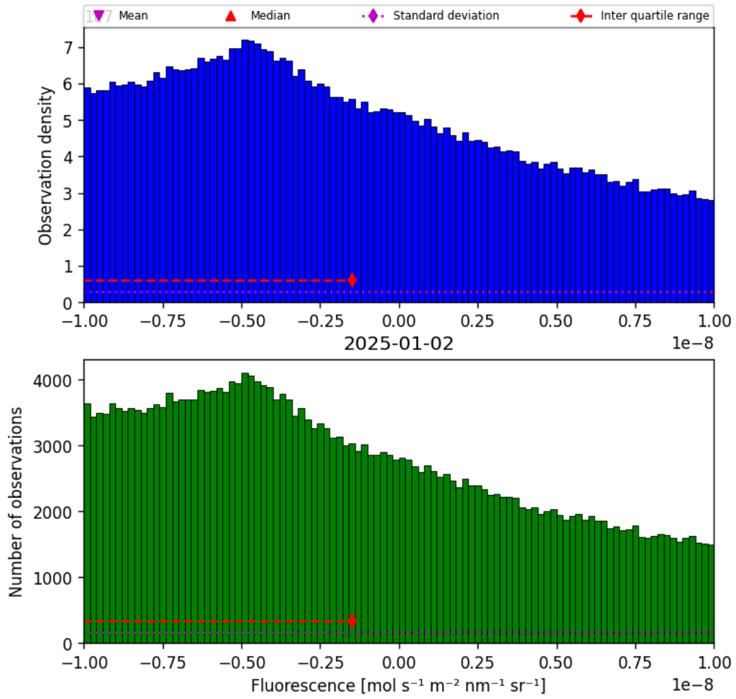
Figure 32: Histogram of “Fluorescence” for 2025-01-01 to 2025-01-03
