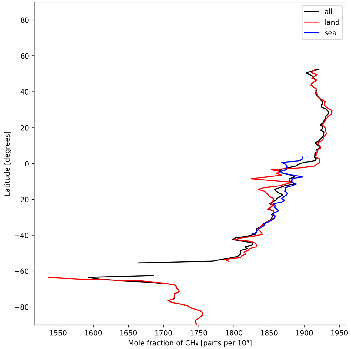
Figure 12: Zonal average of “Mole fraction of CH 4 ” for 2025-01-01 to 2025-01-03.
