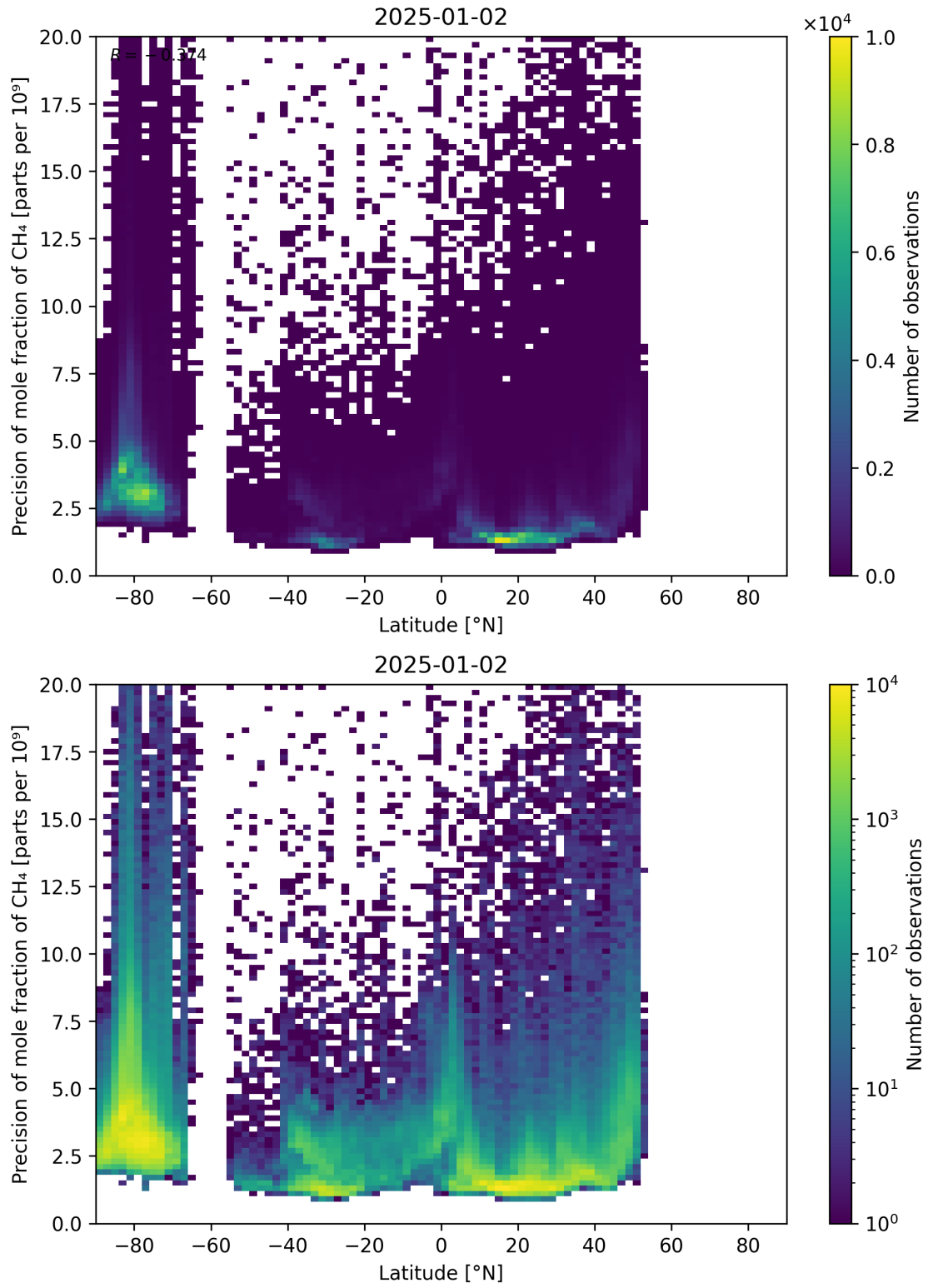
Figure 59: Scatter density plot of “Latitude” against “Precision of mole fraction of CH 4 ” for 2025-01-01 to 2025-01-03.
