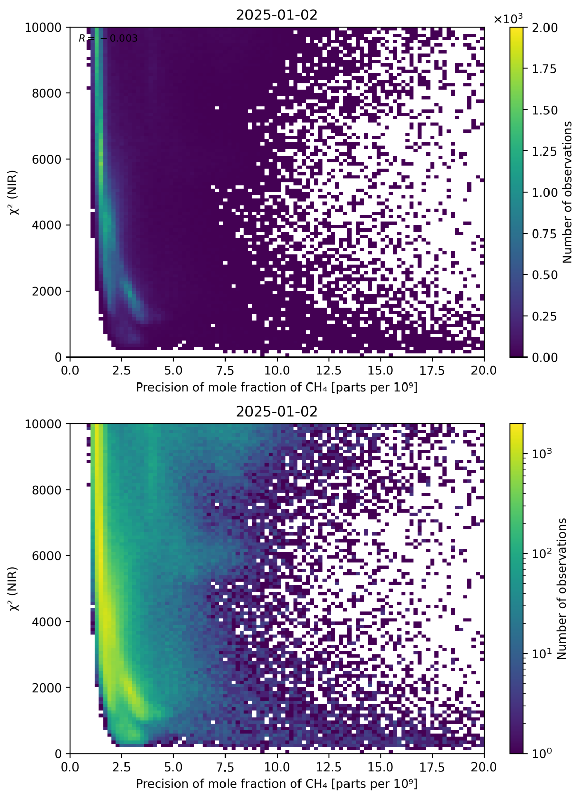
Figure 78: Scatter density plot of “Precision of mole fraction of CH 4 ” against “ \chi^2 (NIR)” for 2025-01-01 to 2025-01-03.
