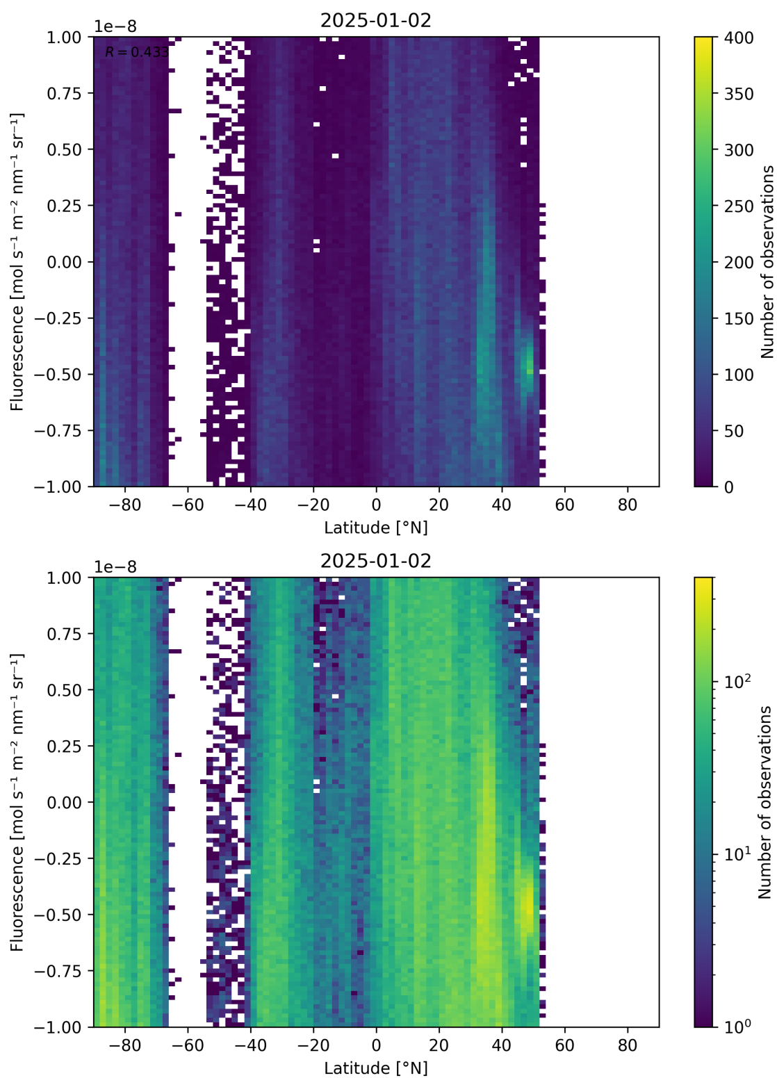
Figure 56: Scatter density plot of “Latitude” against “Fluorescence” for 2025-01-01 to 2025-01-03.
