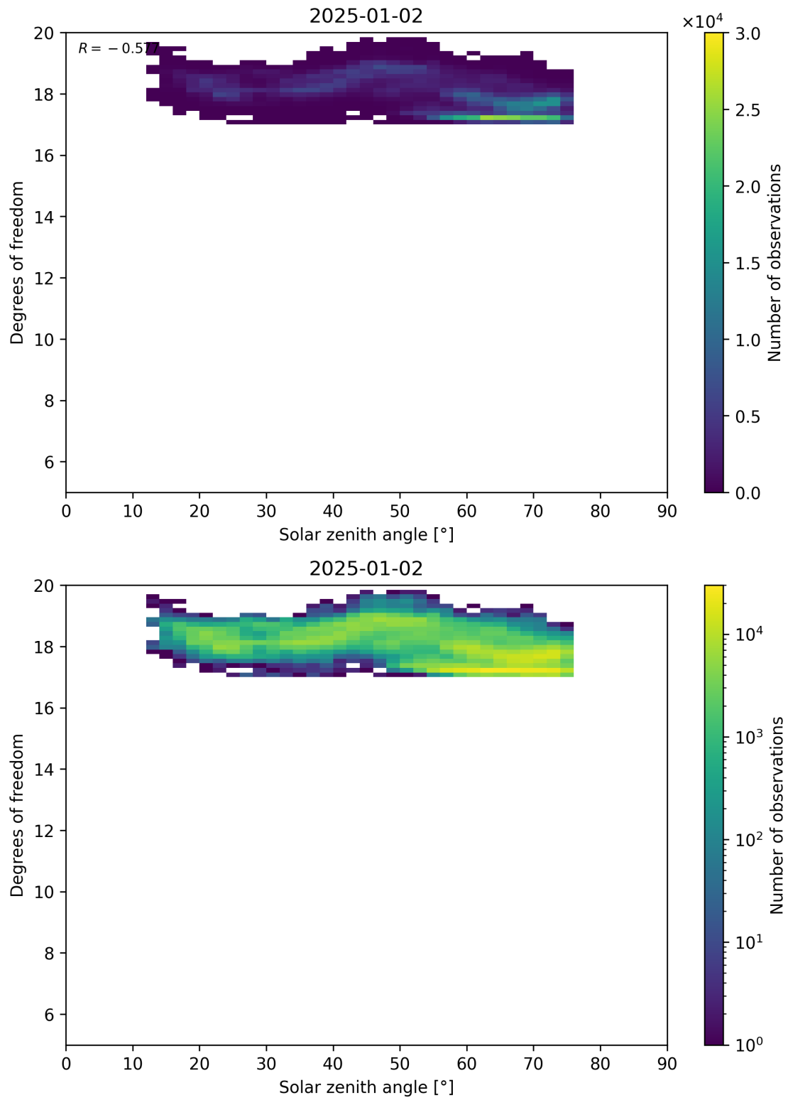
Figure 96: Scatter density plot of “Solar zenith angle” against “Degrees of freedom” for 2025-01-01 to 2025-01-03.
