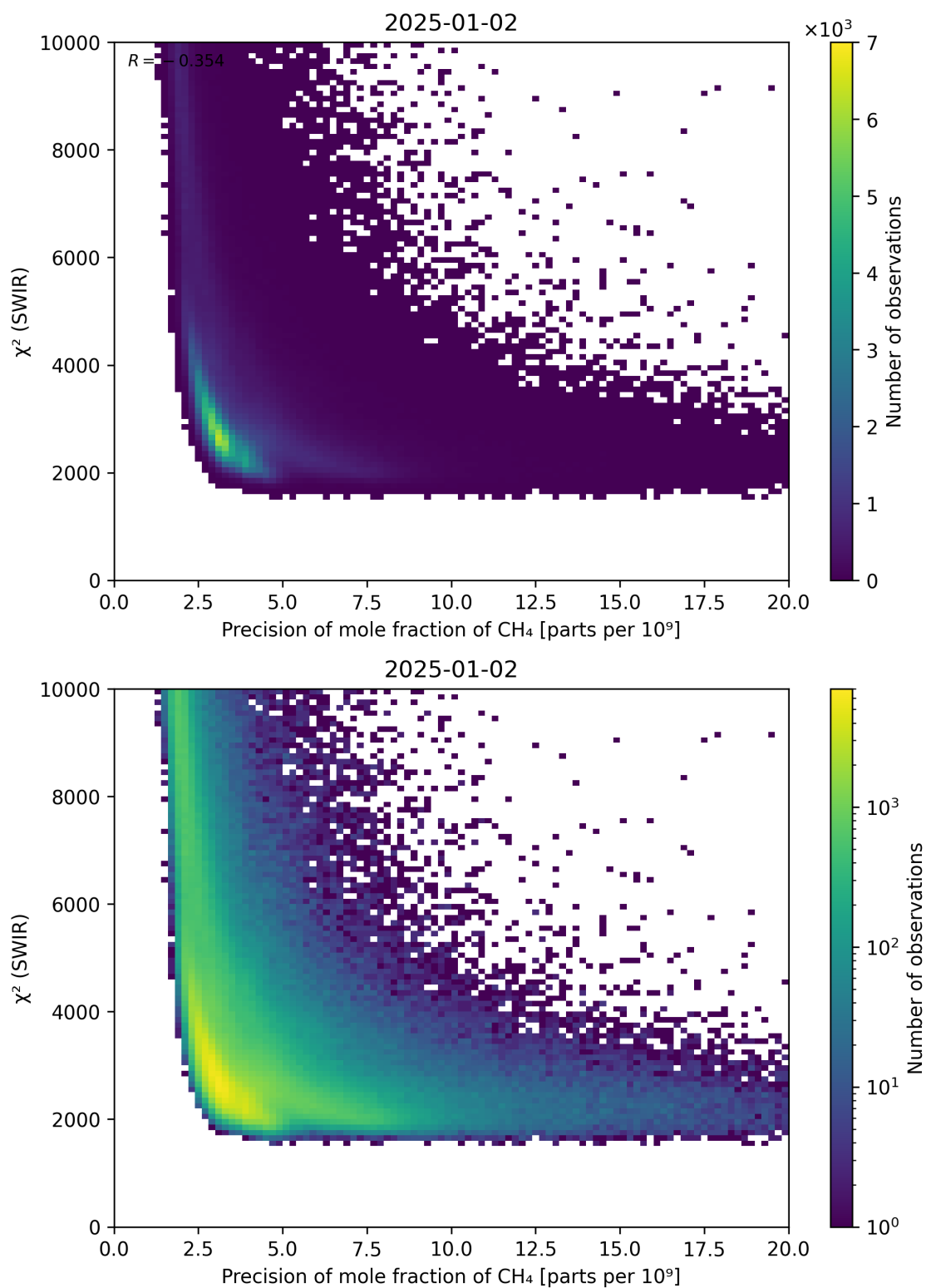
Figure 79: Scatter density plot of “Precision of mole fraction of \text{CH}_4 ” against “ \chi^2 (SWIR)” for 2025-01-01 to 2025-01-03.
