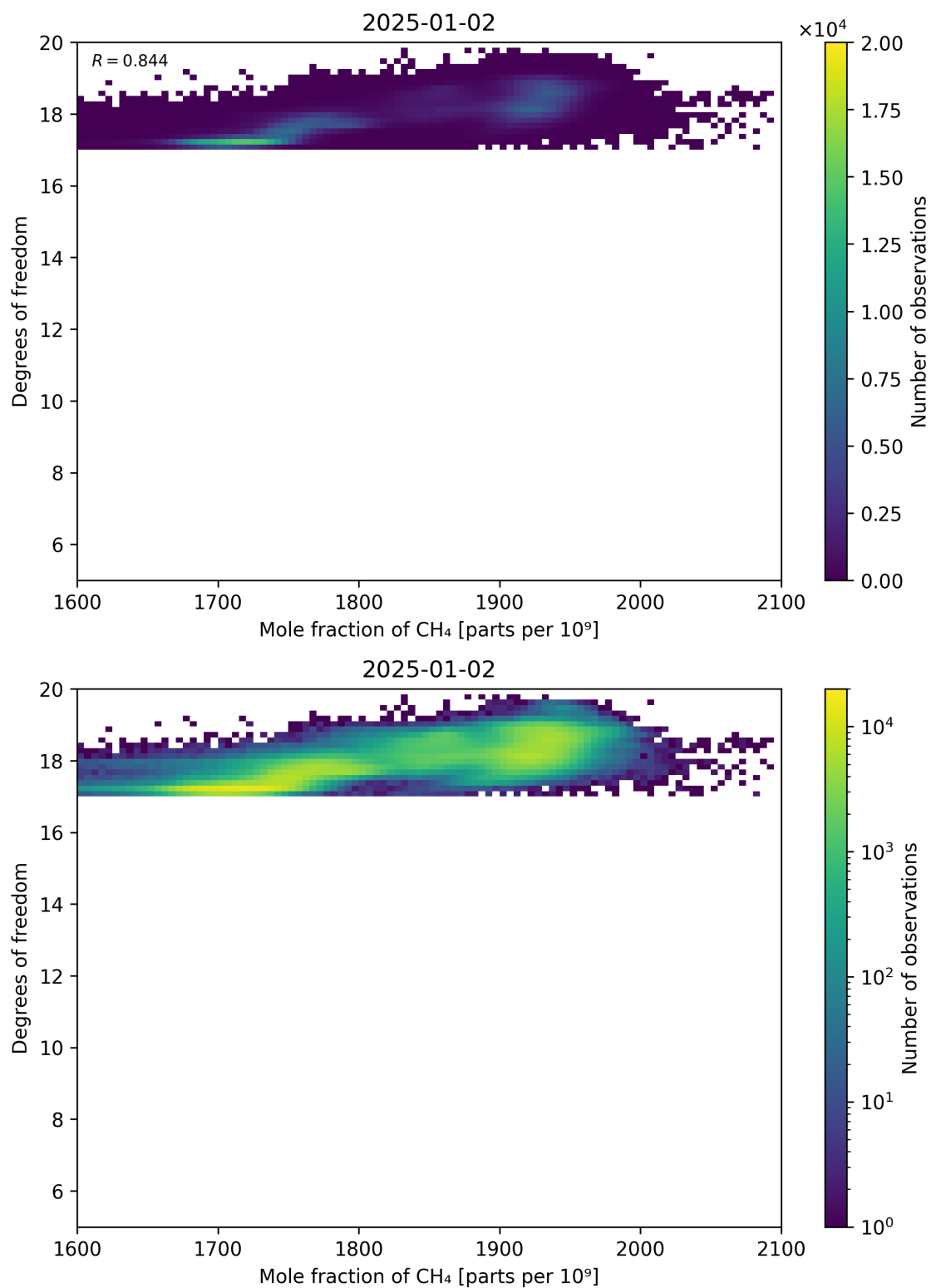
Figure 72: Scatter density plot of “Mole fraction of CH 4 ” against “Degrees of freedom” for 2025-01-01 to 2025-01-03.
