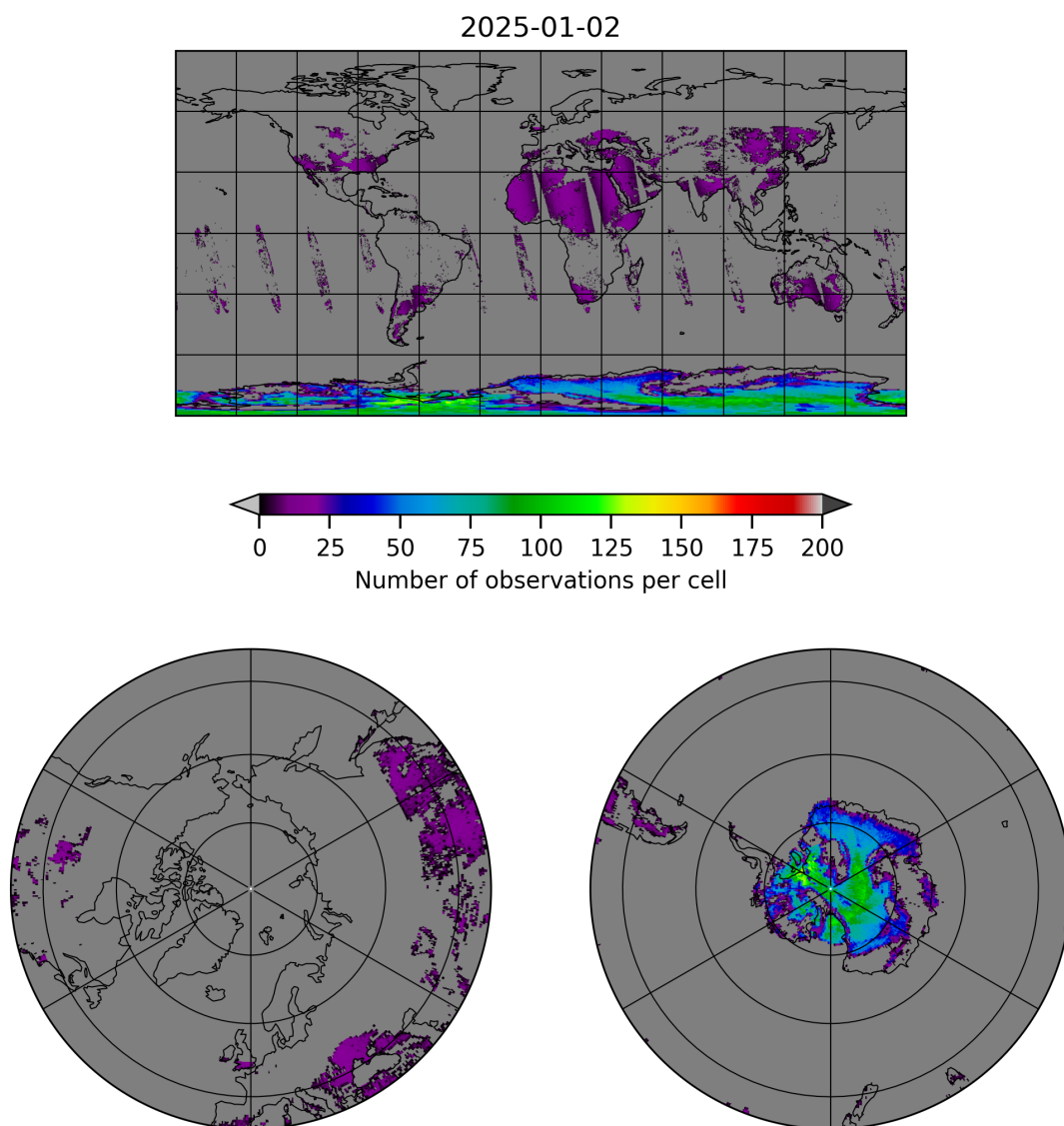
Figure 10: Map of the number of observations for 2025-01-01 to 2025-01-03
