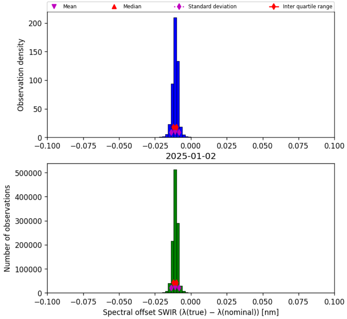
Figure 27: Histogram of “Spectral offset SWIR ( \lambda_{\text{true}} - \lambda_{\text{nominal}} )” for 2025-01-01 to 2025-01-03
