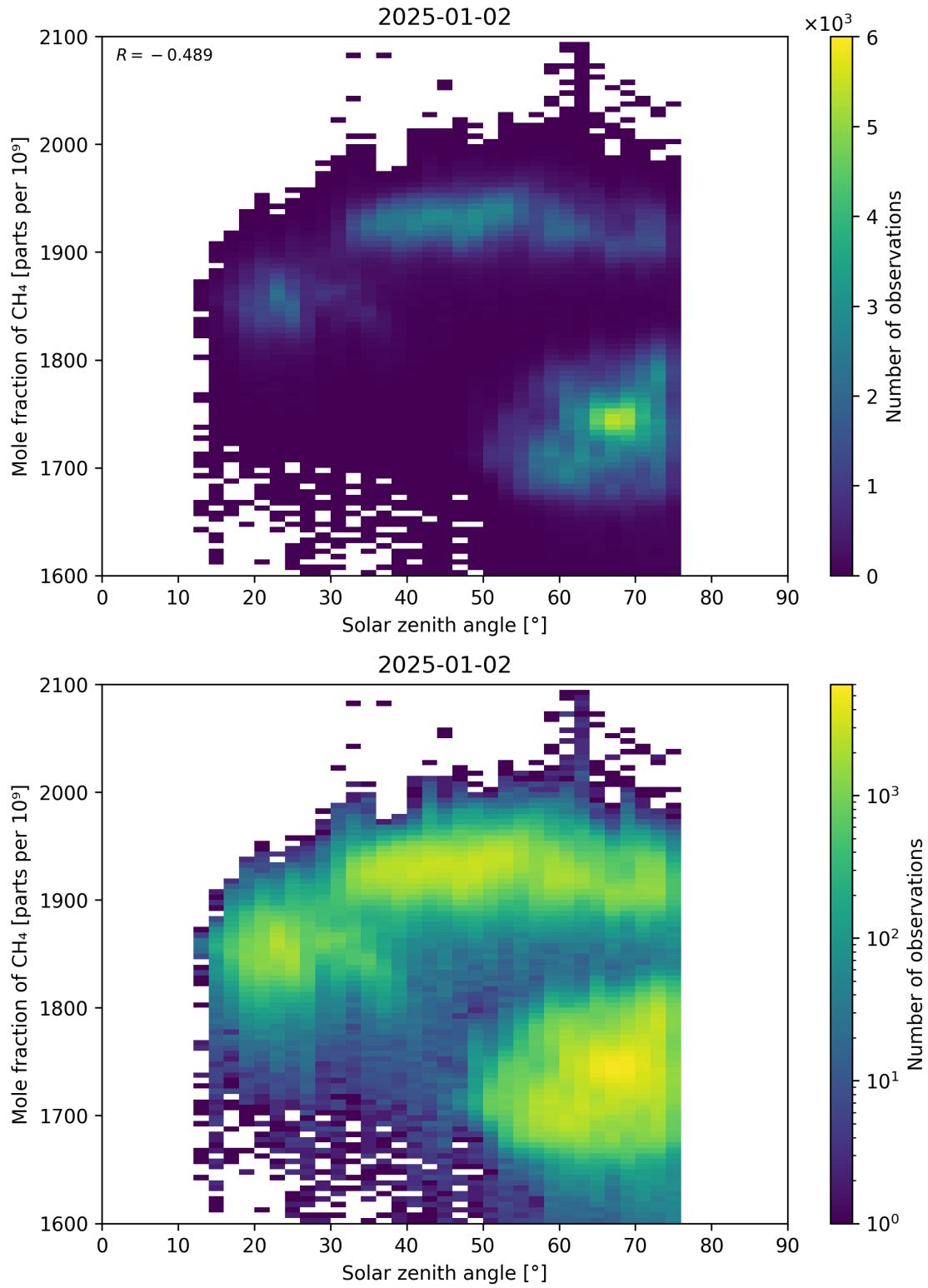
Figure 99: Scatter density plot of “Solar zenith angle” against “Mole fraction of CH 4 ” for 2025-01-01 to 2025-01-03.
