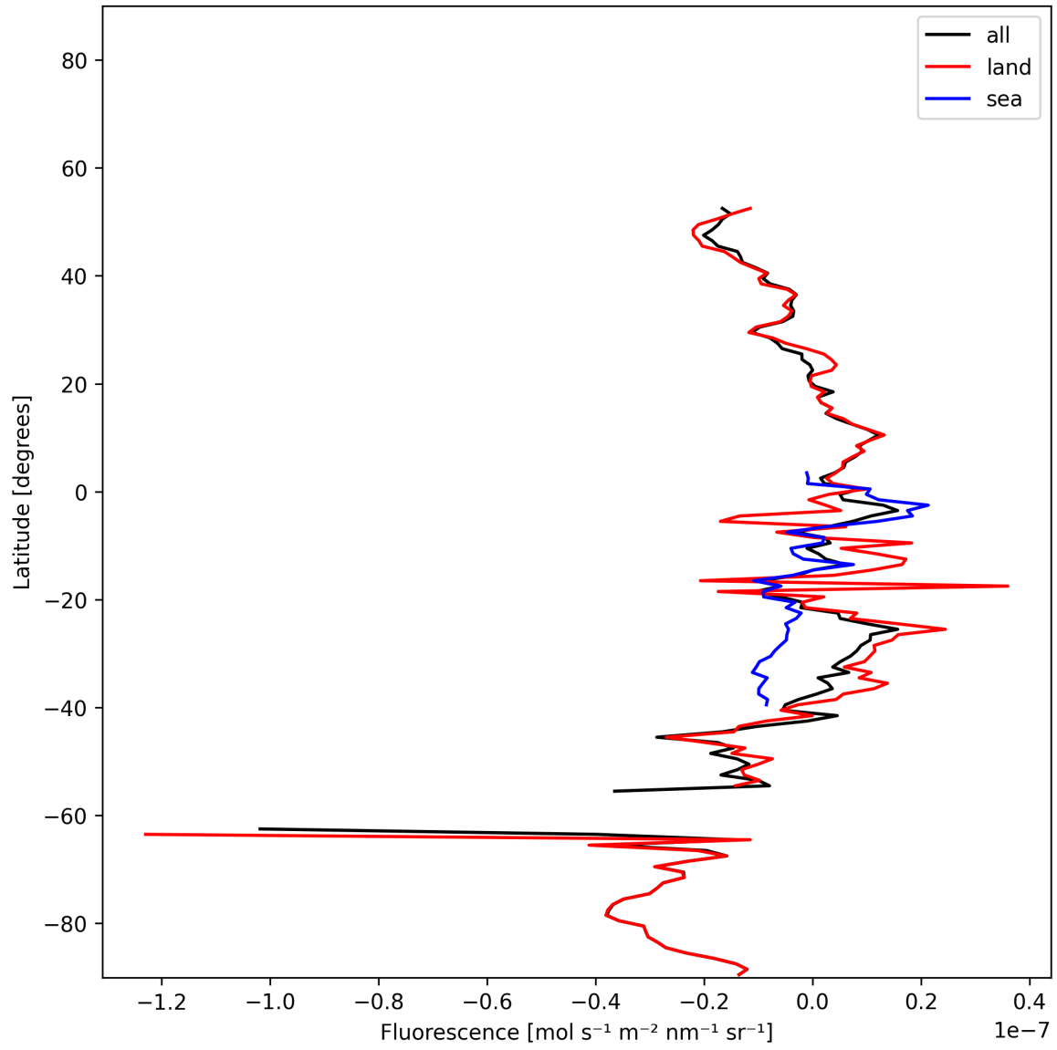
Figure 21: Zonal average of “Fluorescence” for 2025-01-01 to 2025-01-03.
