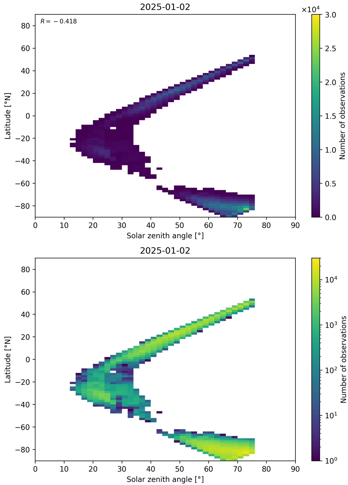
Figure 98: Scatter density plot of “Solar zenith angle” against “Latitude” for 2025-01-01 to 2025-01-03.
