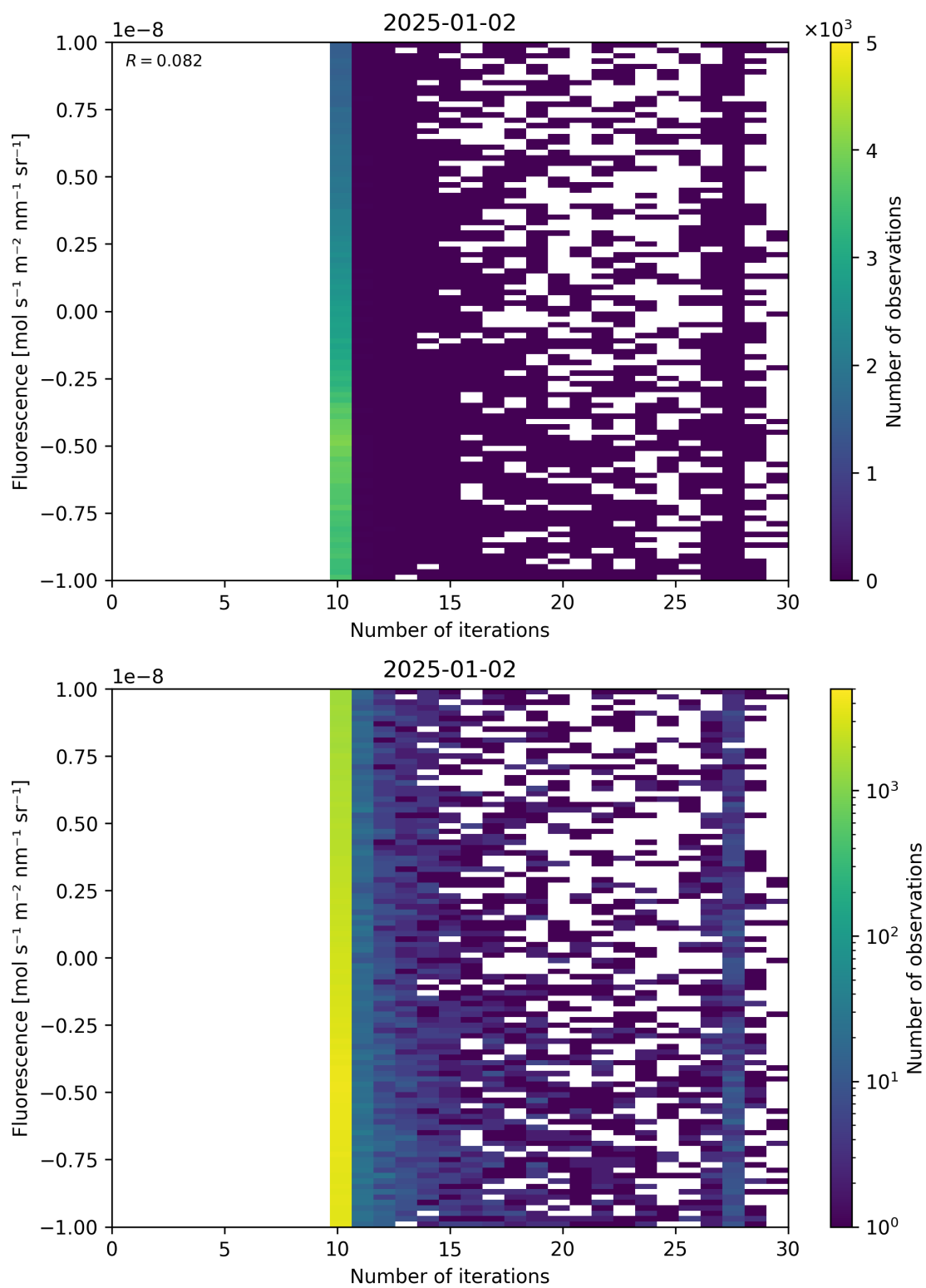
Figure 87: Scatter density plot of “Number of iterations” against “Fluorescence” for 2025-01-01 to 2025-01-03.
