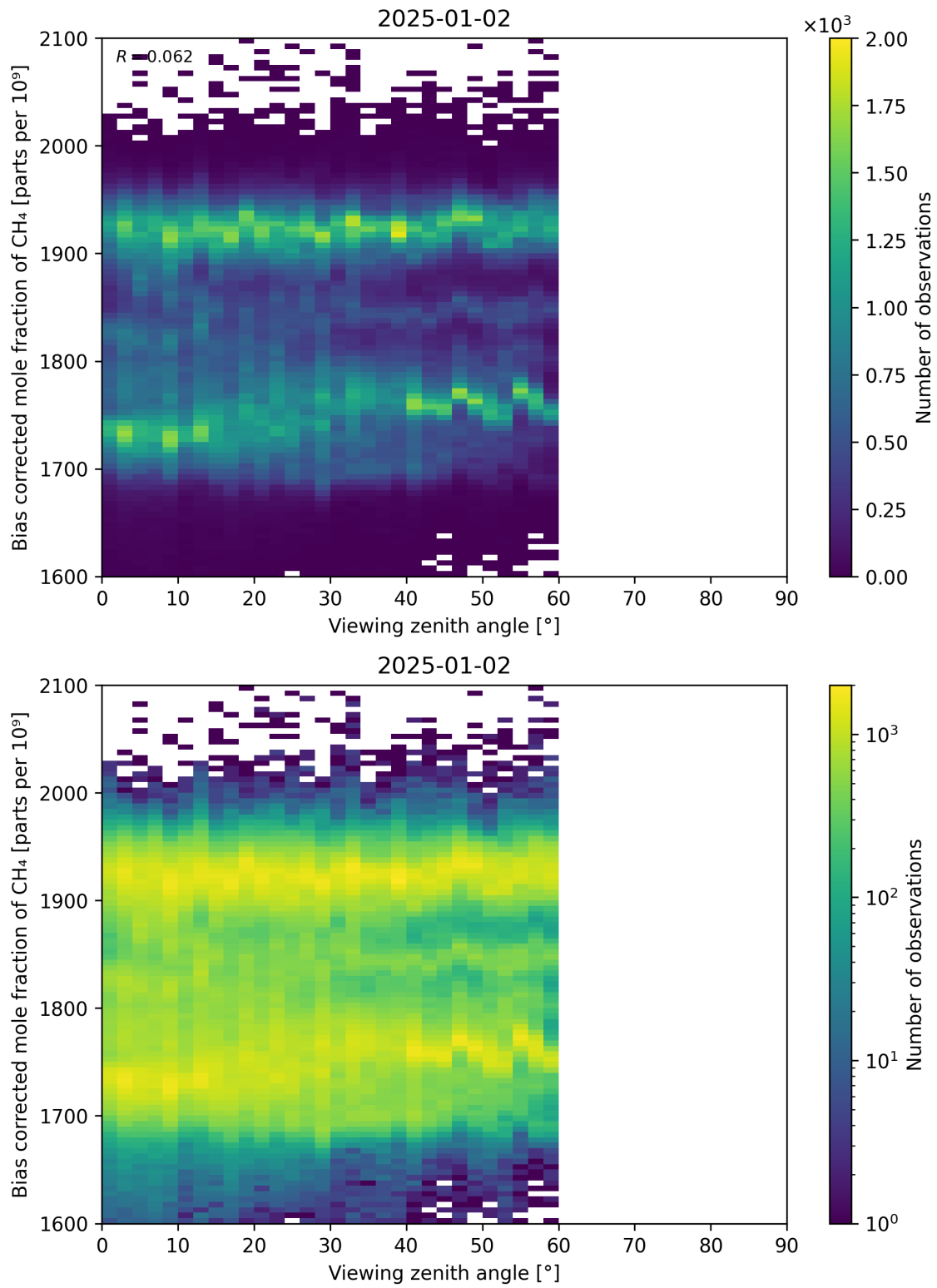
Figure 111: Scatter density plot of “Viewing zenith angle” against “Bias corrected mole fraction of CH 4 ” for 2025-01-01 to 2025-01-03.
