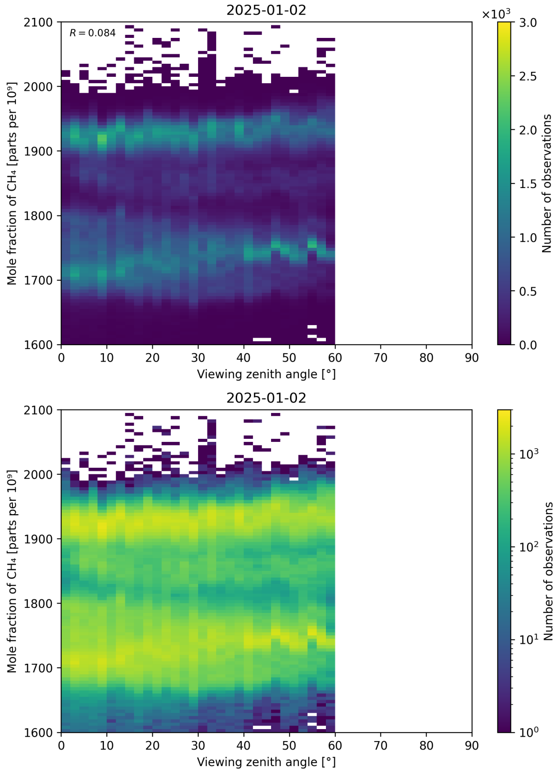
Figure 110: Scatter density plot of “Viewing zenith angle” against “Mole fraction of \text{CH}_4 ” for 2025-01-01 to 2025-01-03.
