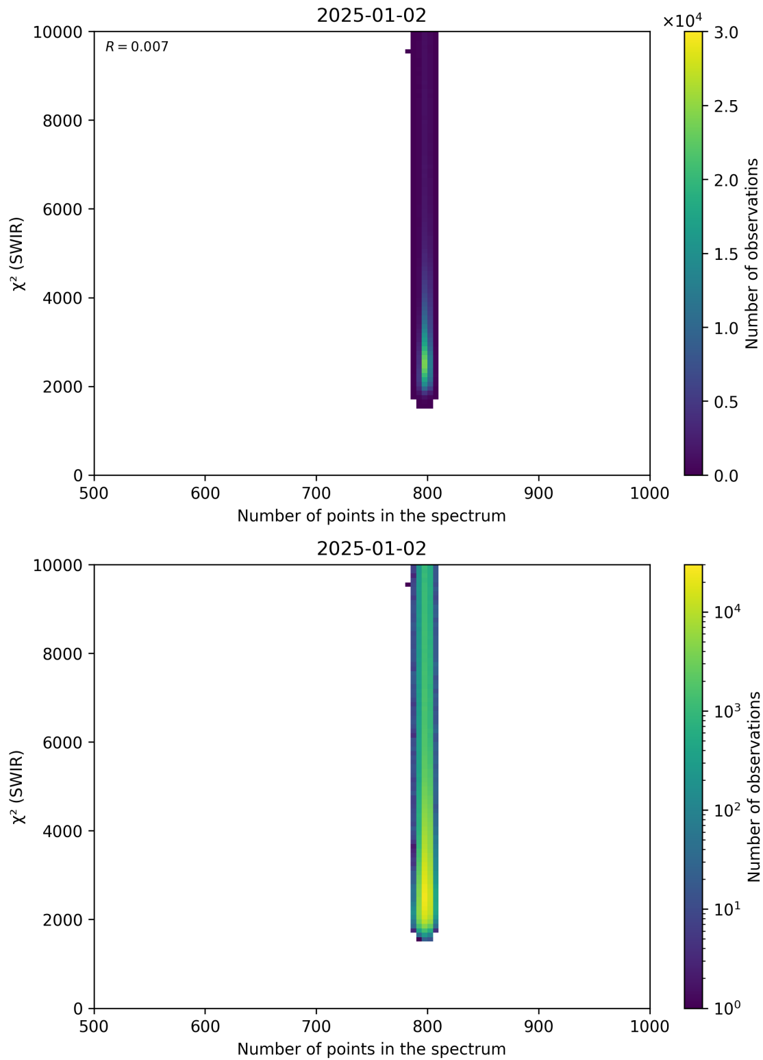
Figure 89: Scatter density plot of “Number of points in the spectrum” against “ \chi^2 (SWIR)” for 2025-01-01 to 2025-01-03.
