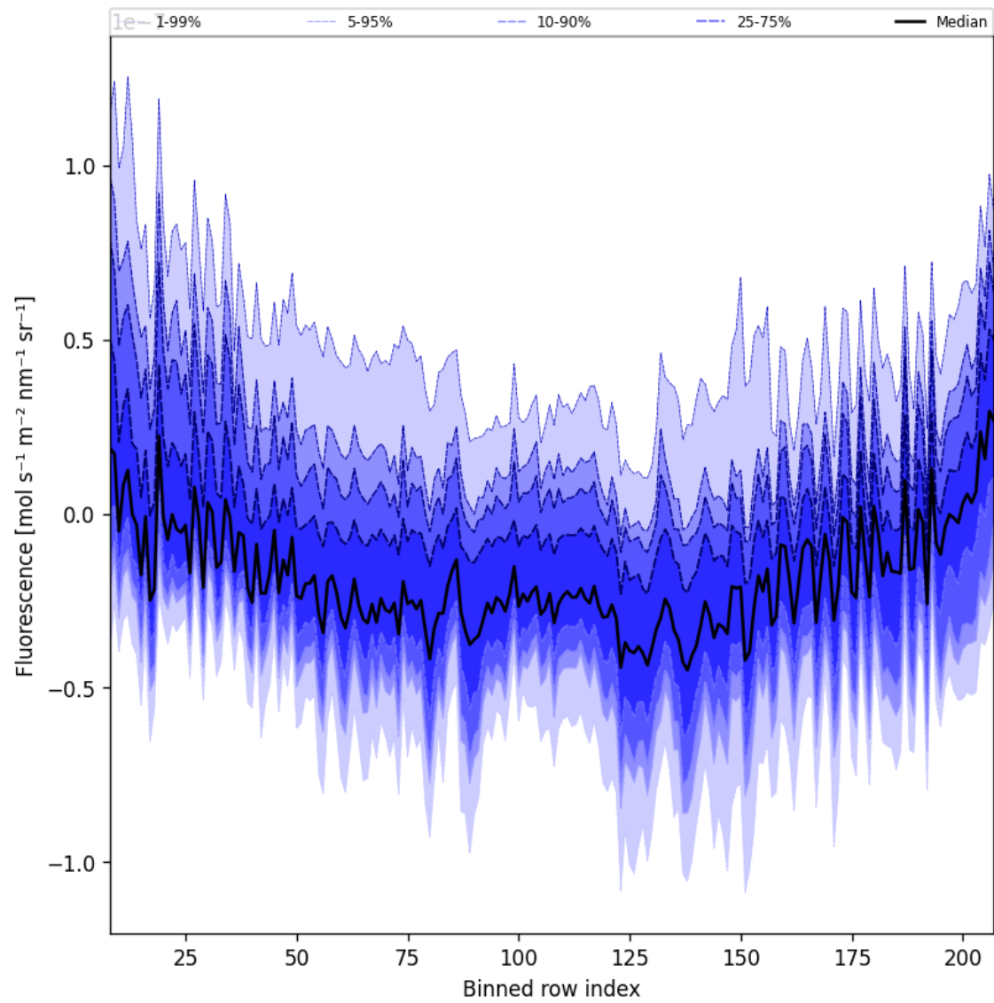
Figure 43: Along track statistics of “Fluorescence” for 2025-01-01 to 2025-01-03
