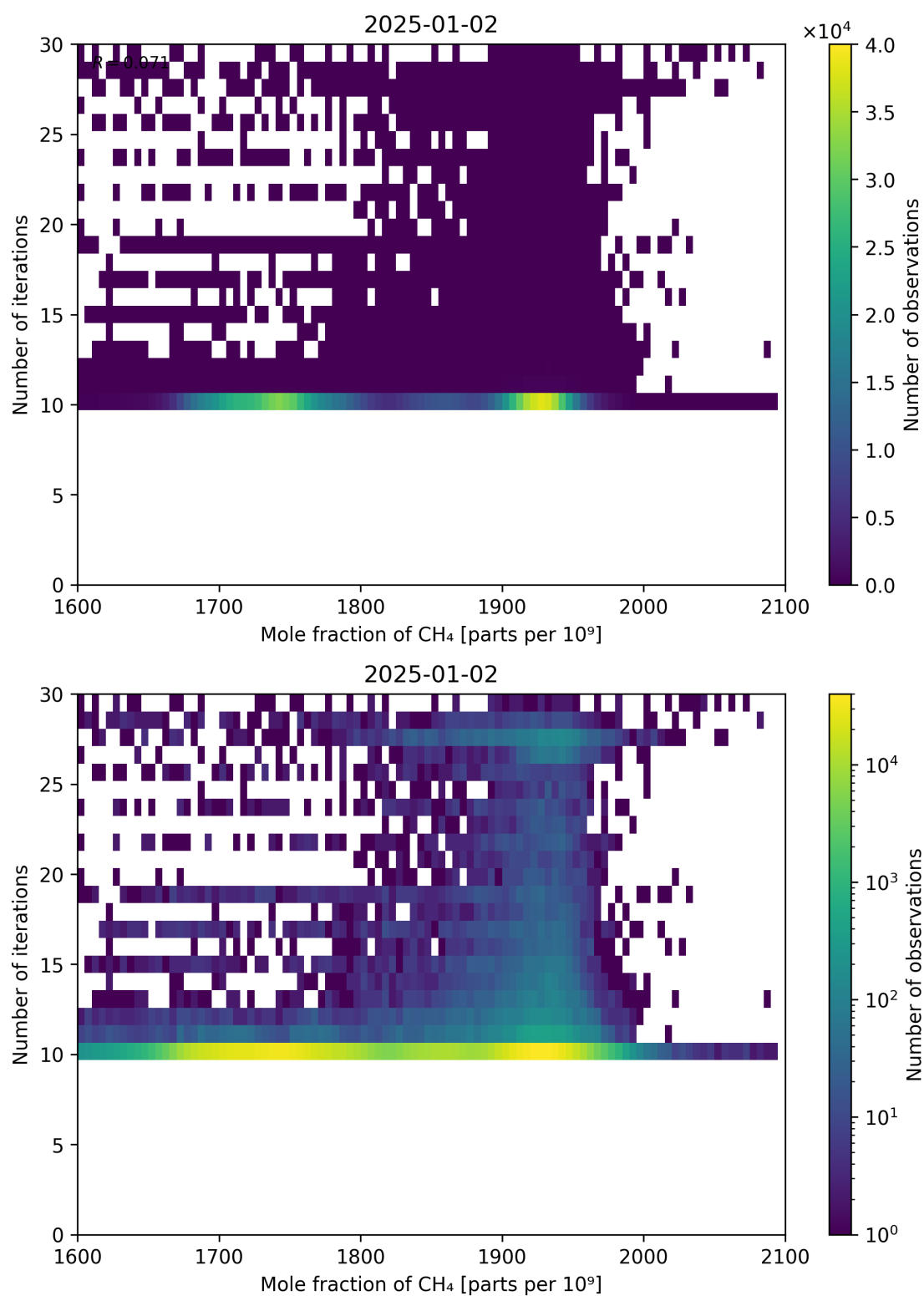
Figure 76: Scatter density plot of “Mole fraction of CH 4 ” against “Number of iterations” for 2025-01-01 to 2025-01-03.
