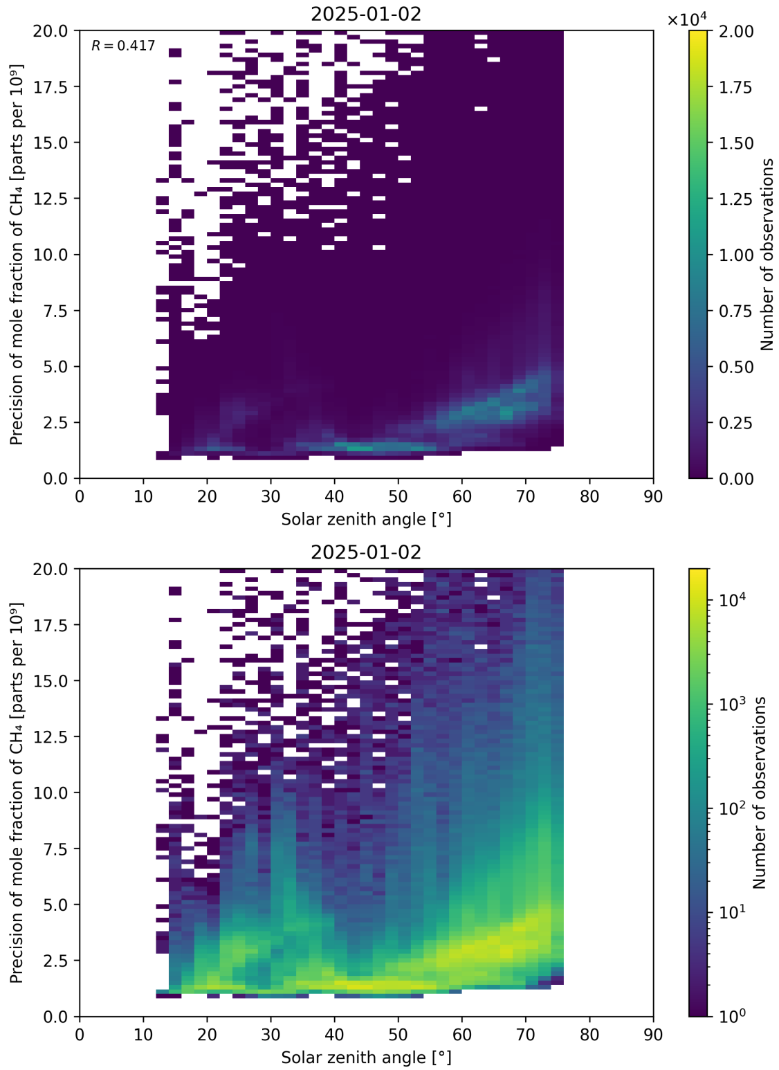
Figure 101: Scatter density plot of “Solar zenith angle” against “Precision of mole fraction of \text{CH}_4 ” for 2025-01-01 to 2025-01-03.
