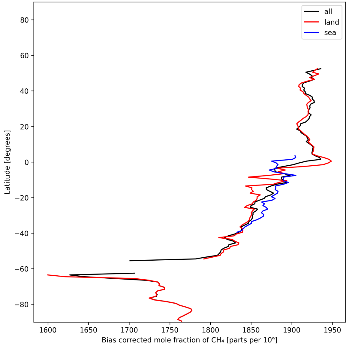
Figure 14: Zonal average of “Bias corrected mole fraction of CH 4 ” for 2025-01-01 to 2025-01-03.
