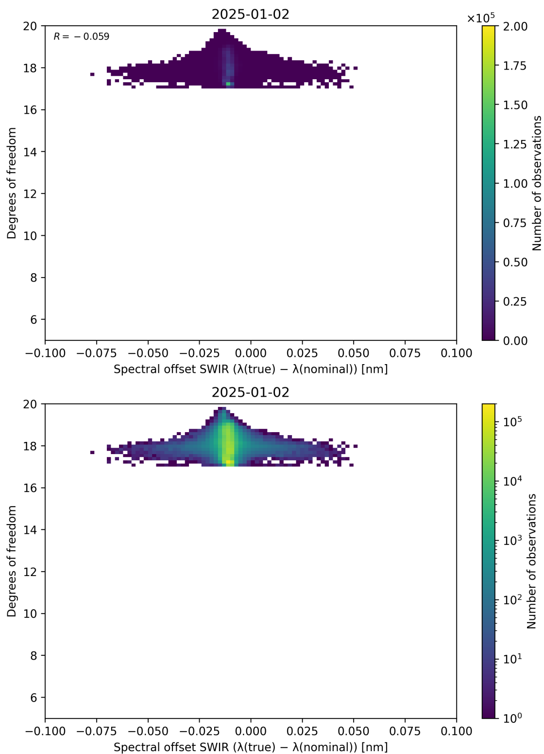
Figure 119: Scatter density plot of “Spectral offset SWIR ( \lambda_{\text{true}} - \lambda_{\text{nominal}} )” against “Degrees of freedom” for 2025-01-01 to 2025-01-03.
