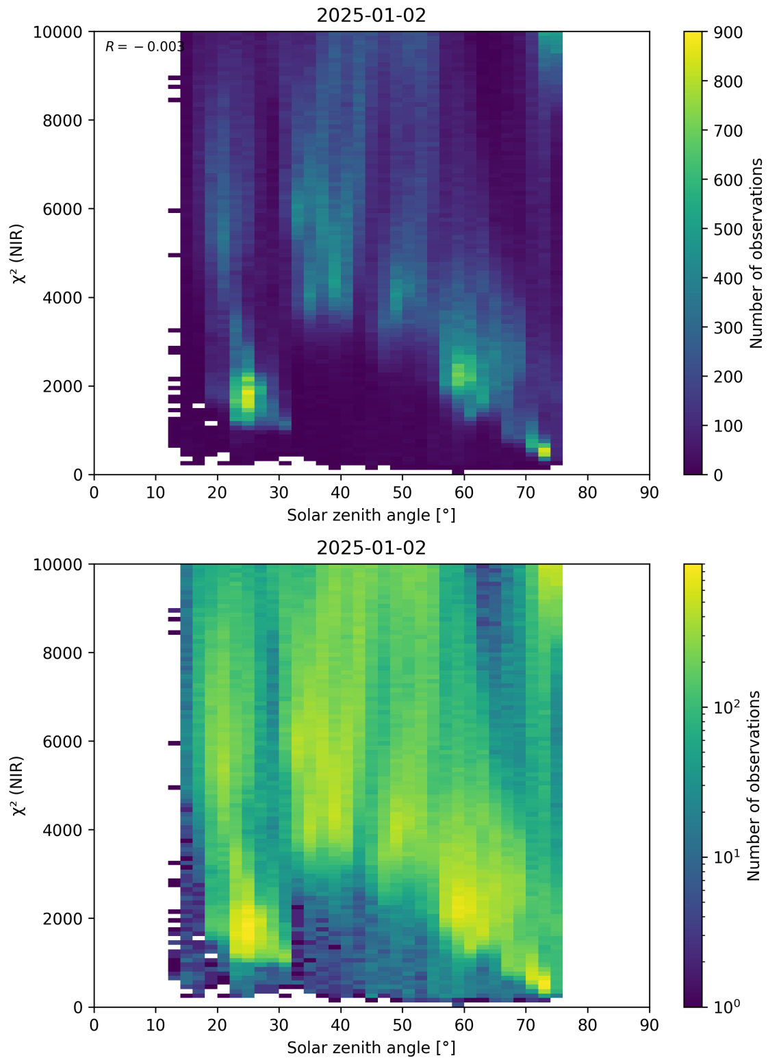
Figure 94: Scatter density plot of “Solar zenith angle” against “ \chi^2 (NIR)” for 2025-01-01 to 2025-01-03.
