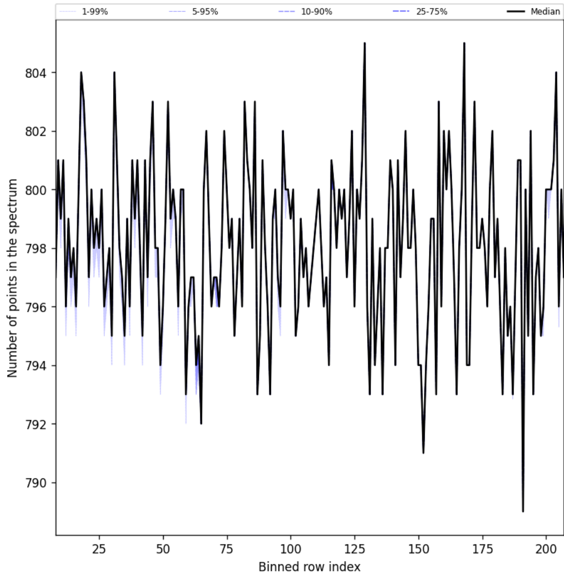
Figure 37: Along track statistics of “Number of points in the spectrum” for 2025-01-01 to 2025-01-03
