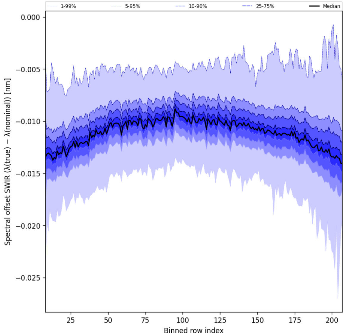
Figure 38: Along track statistics of “Spectral offset SWIR ( \lambda_{\text{true}} - \lambda_{\text{nominal}} )” for 2025-01-01 to 2025-01-03
