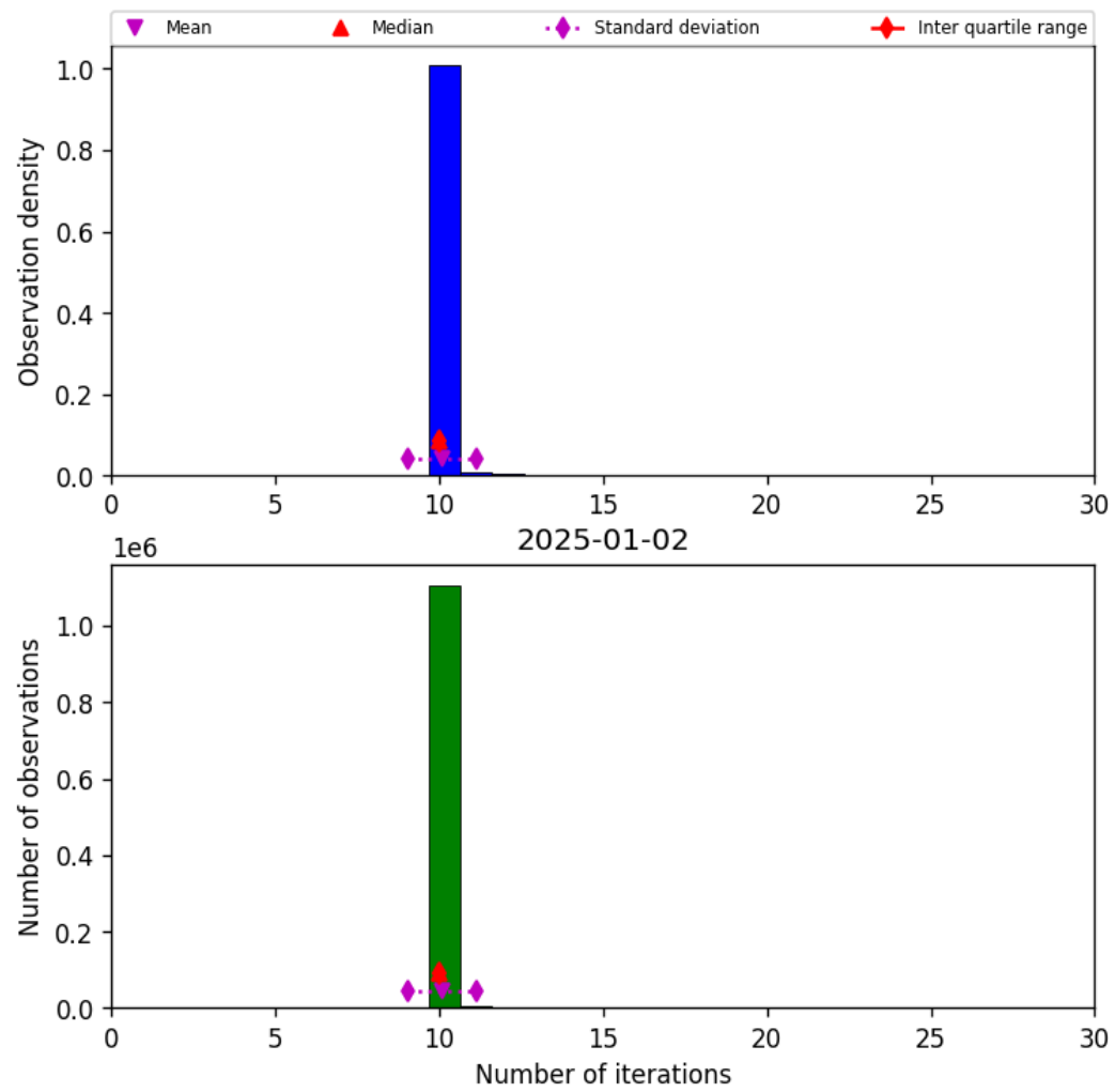
Figure 31: Histogram of “Number of iterations” for 2025-01-01 to 2025-01-03
