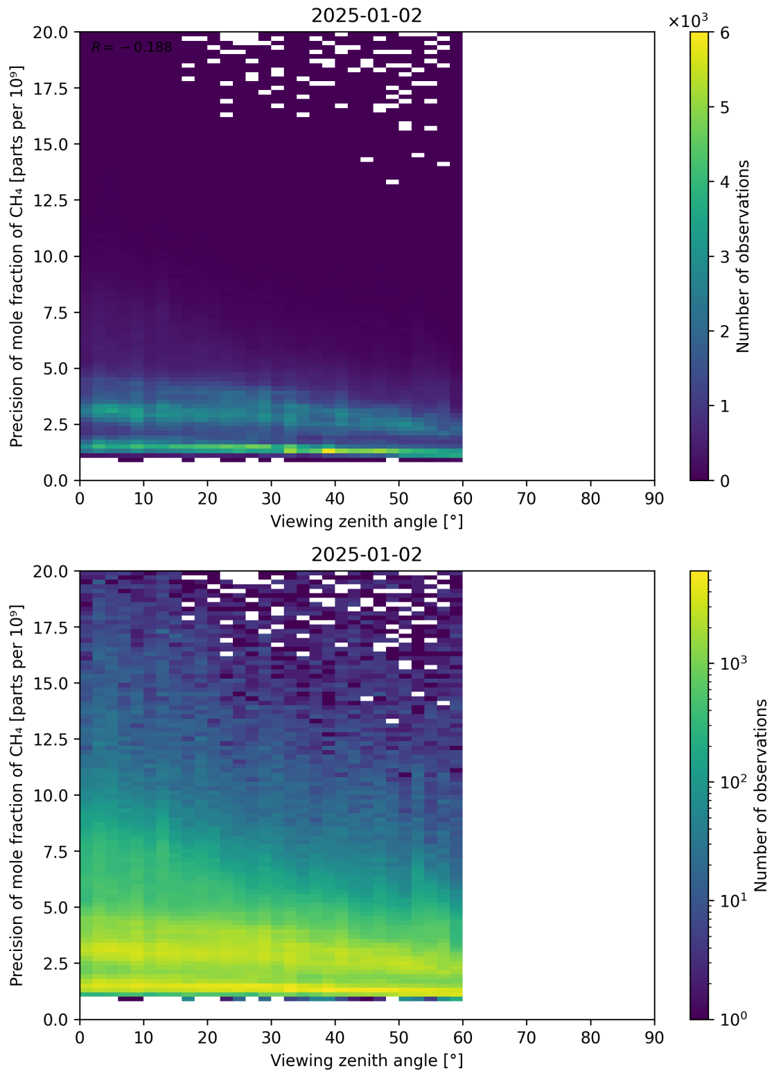
Figure 112: Scatter density plot of “Viewing zenith angle” against “Precision of mole fraction of CH 4 ” for 2025-01-01 to 2025-01-03.
