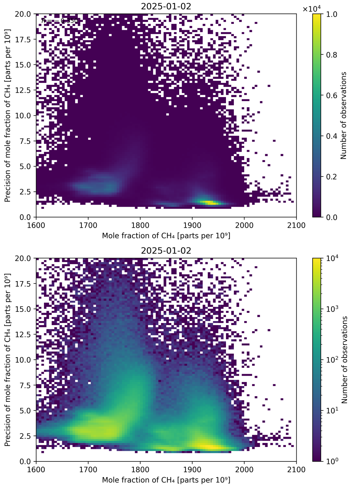
Figure 75: Scatter density plot of “Mole fraction of CH 4 ” against “Precision of mole fraction of CH 4 ” for 2025-01-01 to 2025-01-03.
