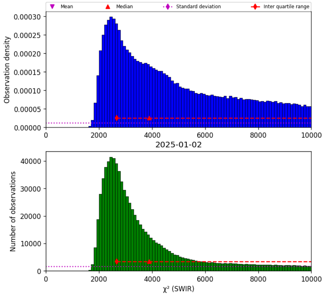
Figure 28: Histogram of “ \chi^2 (SWIR)” for 2025-01-01 to 2025-01-03
