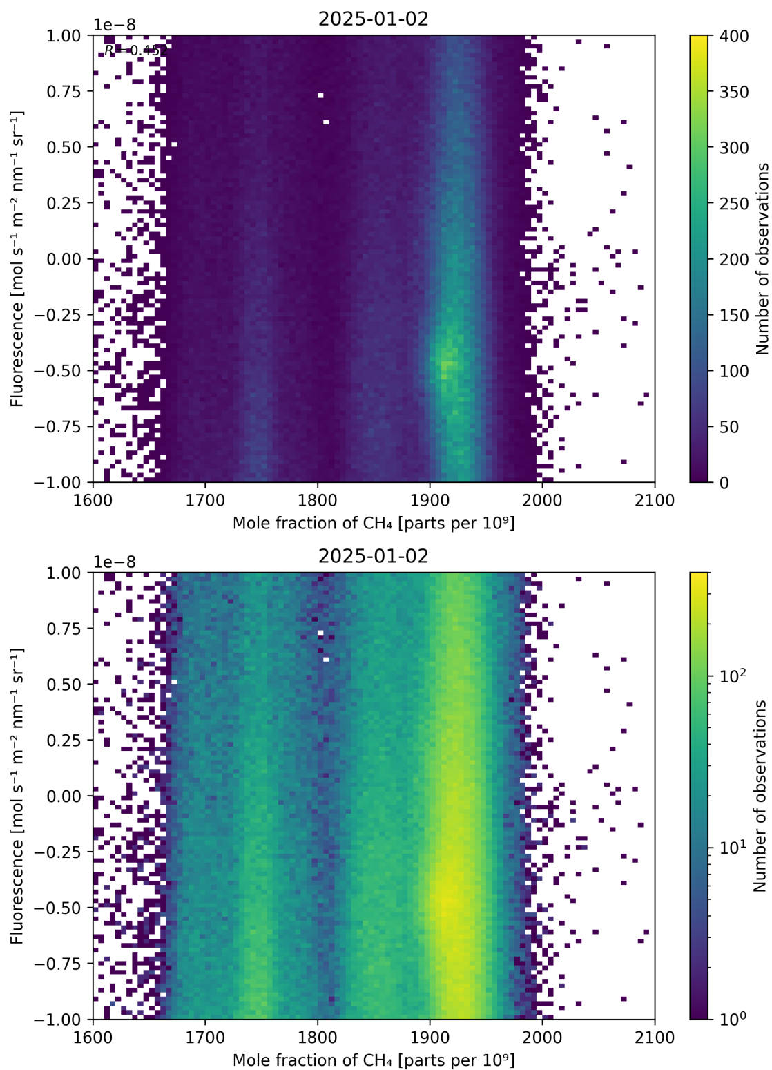
Figure 73: Scatter density plot of “Mole fraction of \text{CH}_4 ” against “Fluorescence” for 2025-01-01 to 2025-01-03.
