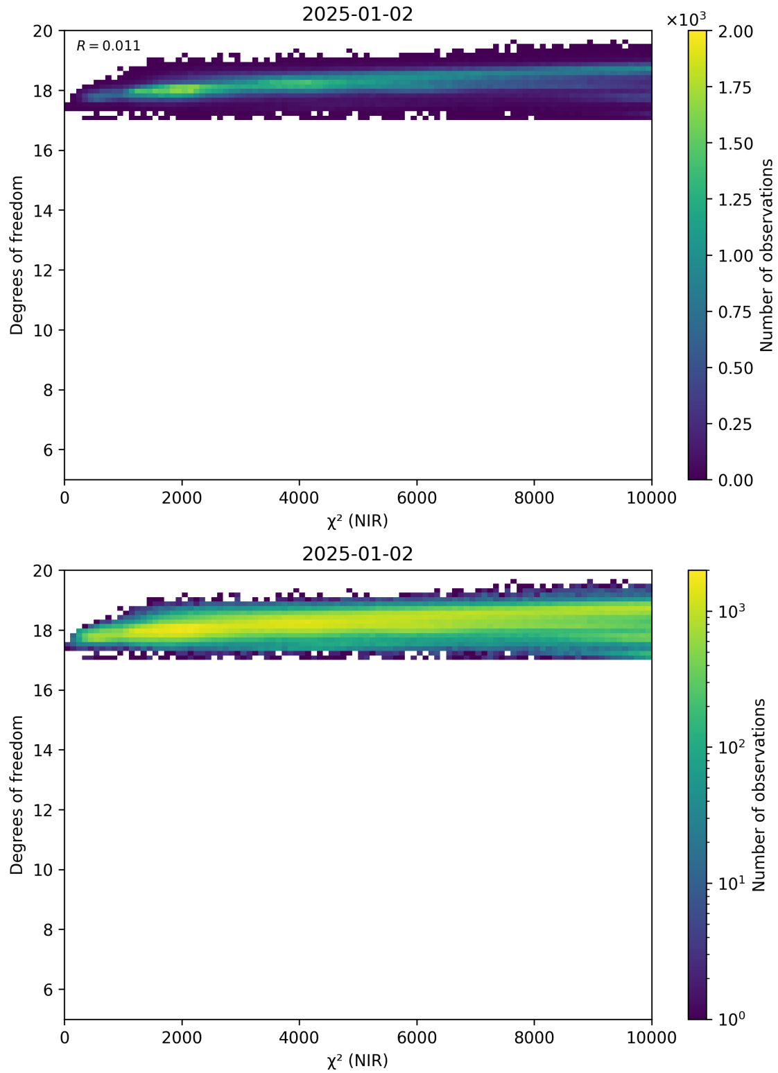
Figure 44: Scatter density plot of “ \chi^2 (NIR)” against “Degrees of freedom” for 2025-01-01 to 2025-01-03.
