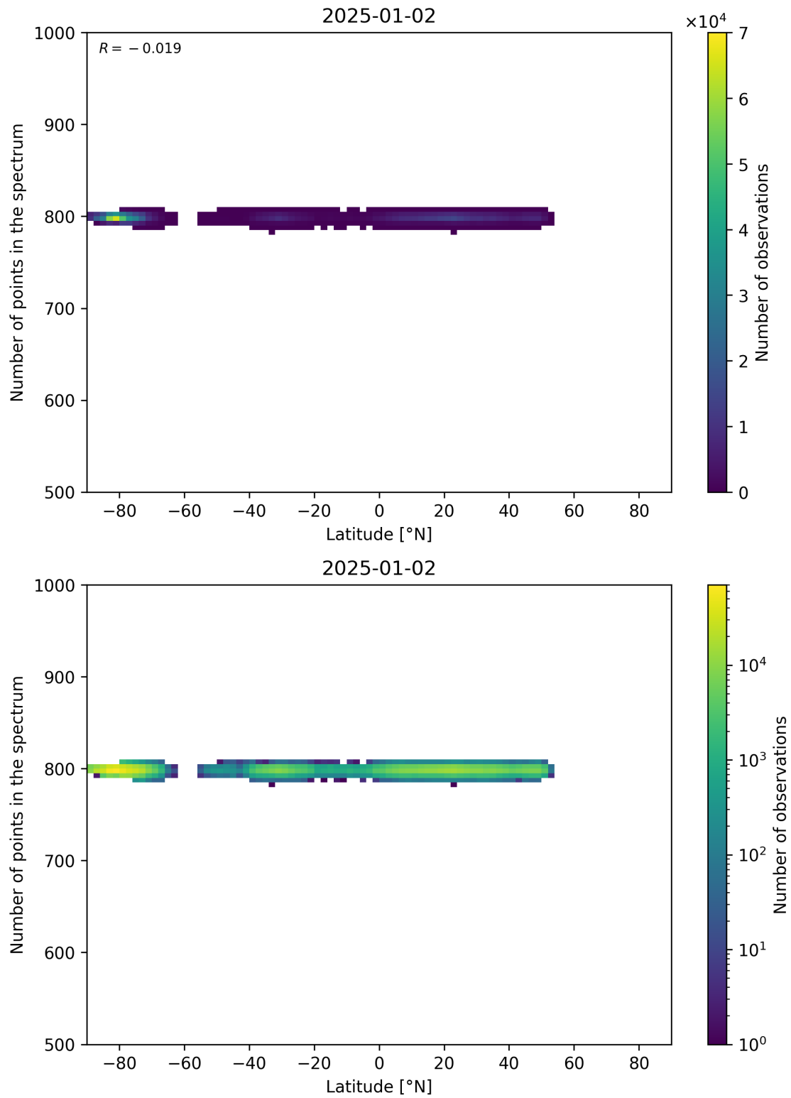
Figure 61: Scatter density plot of “Latitude” against “Number of points in the spectrum” for 2025-01-01 to 2025-01-03.
