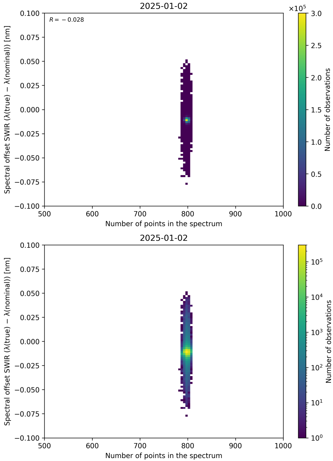
Figure 93: Scatter density plot of “Number of points in the spectrum” against “Spectral offset SWIR ( \lambda_{\text{true}} - \lambda_{\text{nominal}} )” for 2025-01-01 to 2025-01-03.
