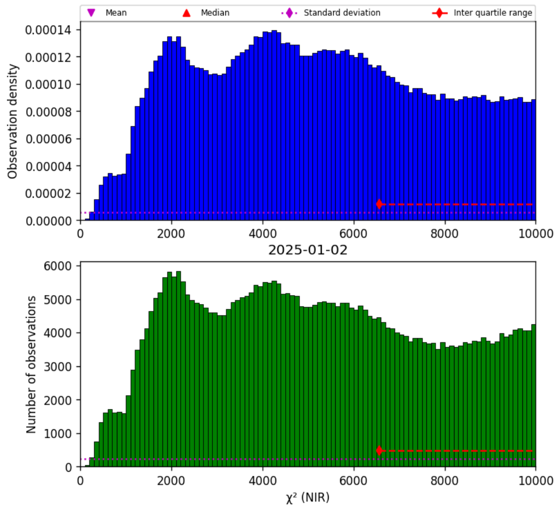
Figure 29: Histogram of " \chi^2 (NIR)" for 2025-01-01 to 2025-01-03
