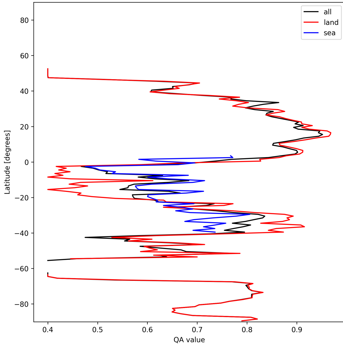
Figure 11: Zonal average of “QA value” for 2025-01-01 to 2025-01-03.
