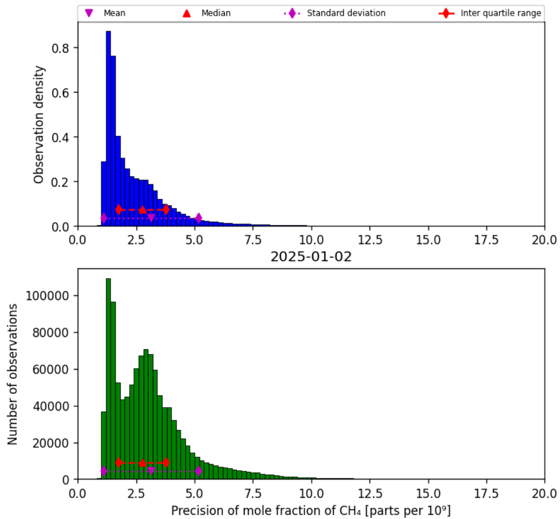
Figure 24: Histogram of “Precision of mole fraction of CH 4 ” for 2025-01-01 to 2025-01-03
