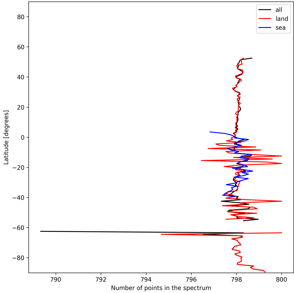
Figure 15: Zonal average of “Number of points in the spectrum” for 2025-01-01 to 2025-01-03.
