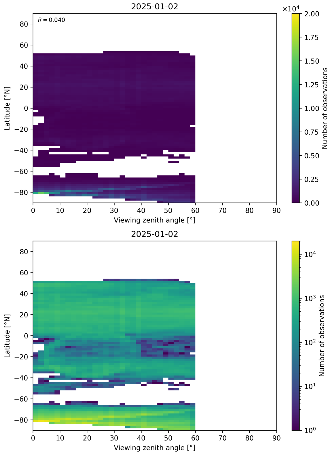
Figure 109: Scatter density plot of “Viewing zenith angle” against “Latitude” for 2025-01-01 to 2025-01-03.
