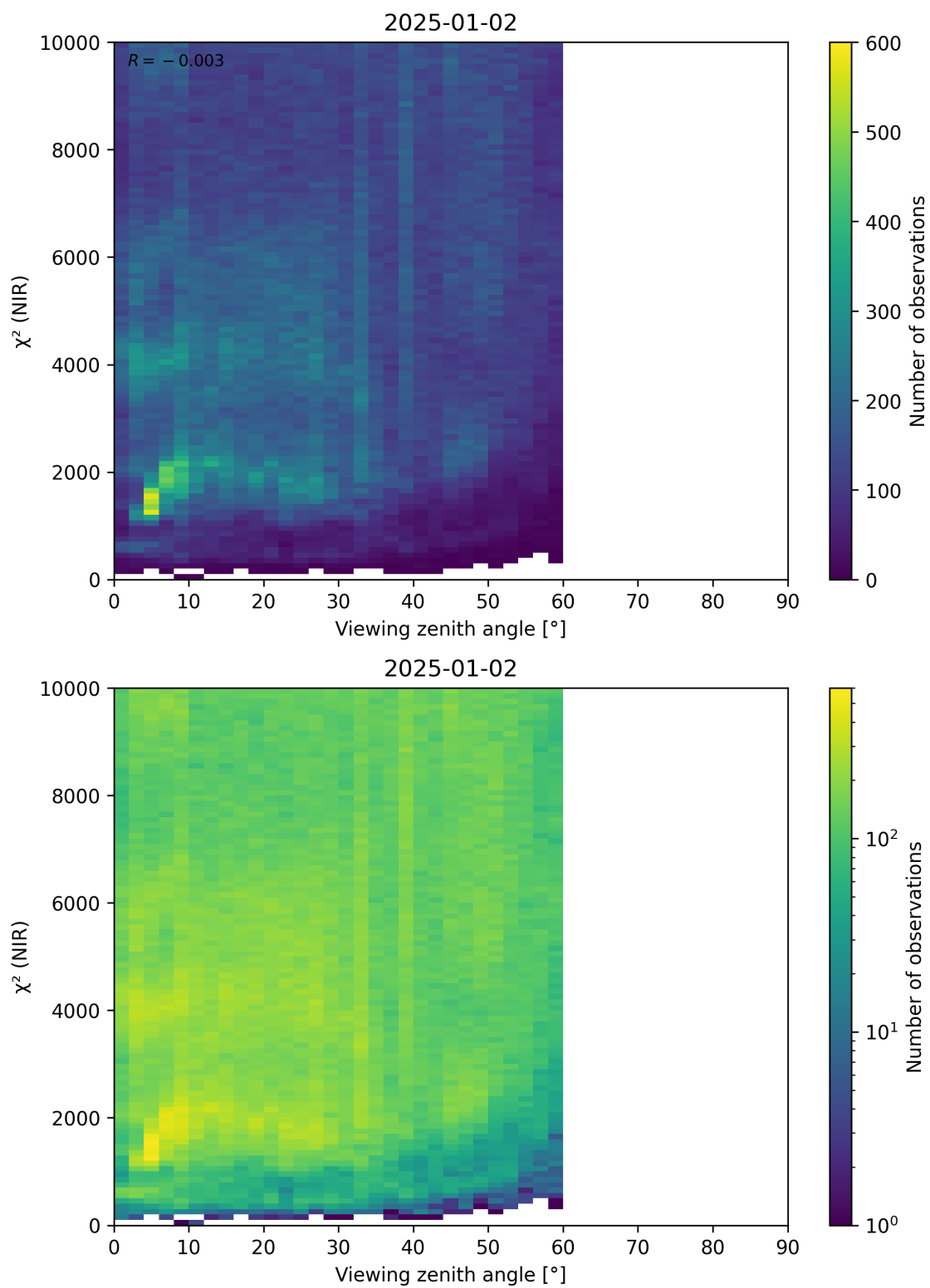
Figure 105: Scatter density plot of “Viewing zenith angle” against “ \chi^2 (NIR)” for 2025-01-01 to 2025-01-03.
