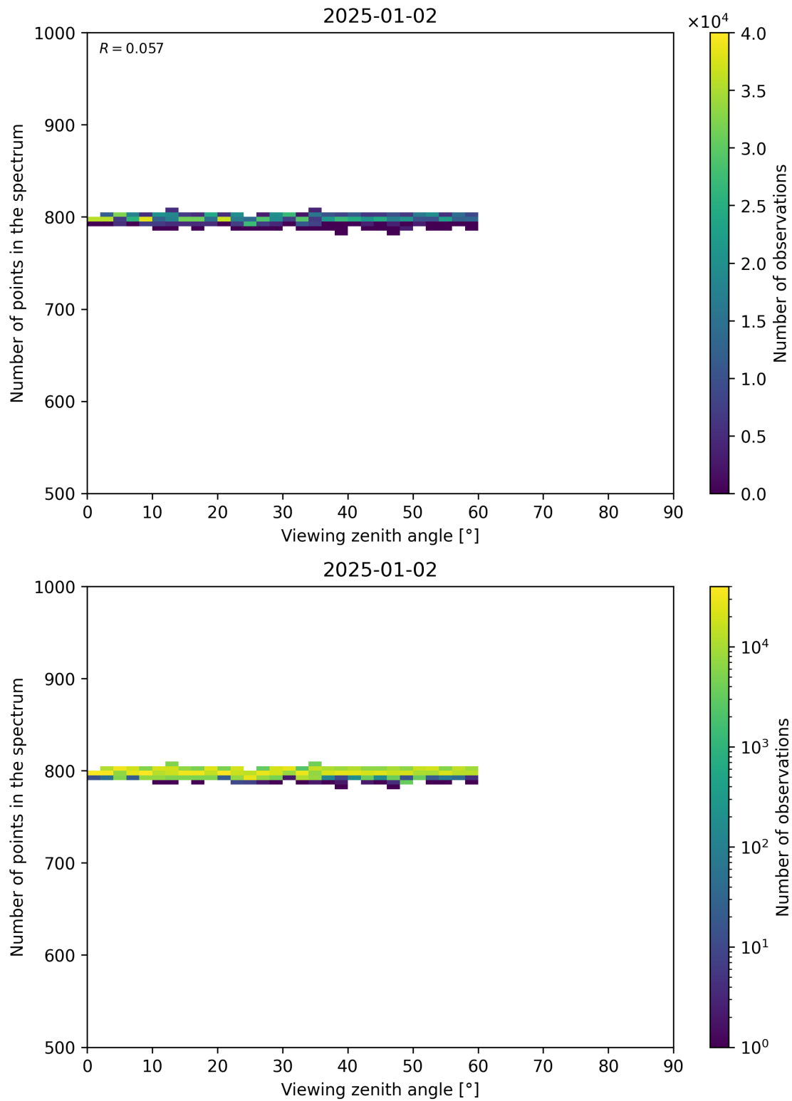
Figure 114: Scatter density plot of “Viewing zenith angle” against “Number of points in the spectrum” for 2025-01-01 to 2025-01-03.
