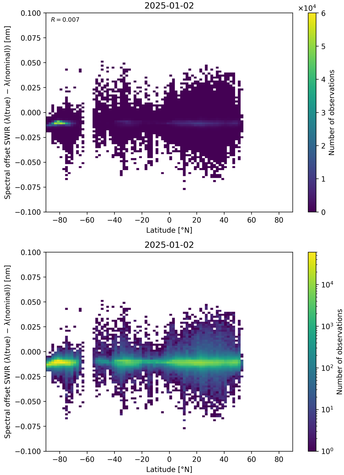
Figure 62: Scatter density plot of “Latitude” against “Spectral offset SWIR ( \lambda_{\text{true}} - \lambda_{\text{nominal}} )” for 2025-01-01 to 2025-01-03.
