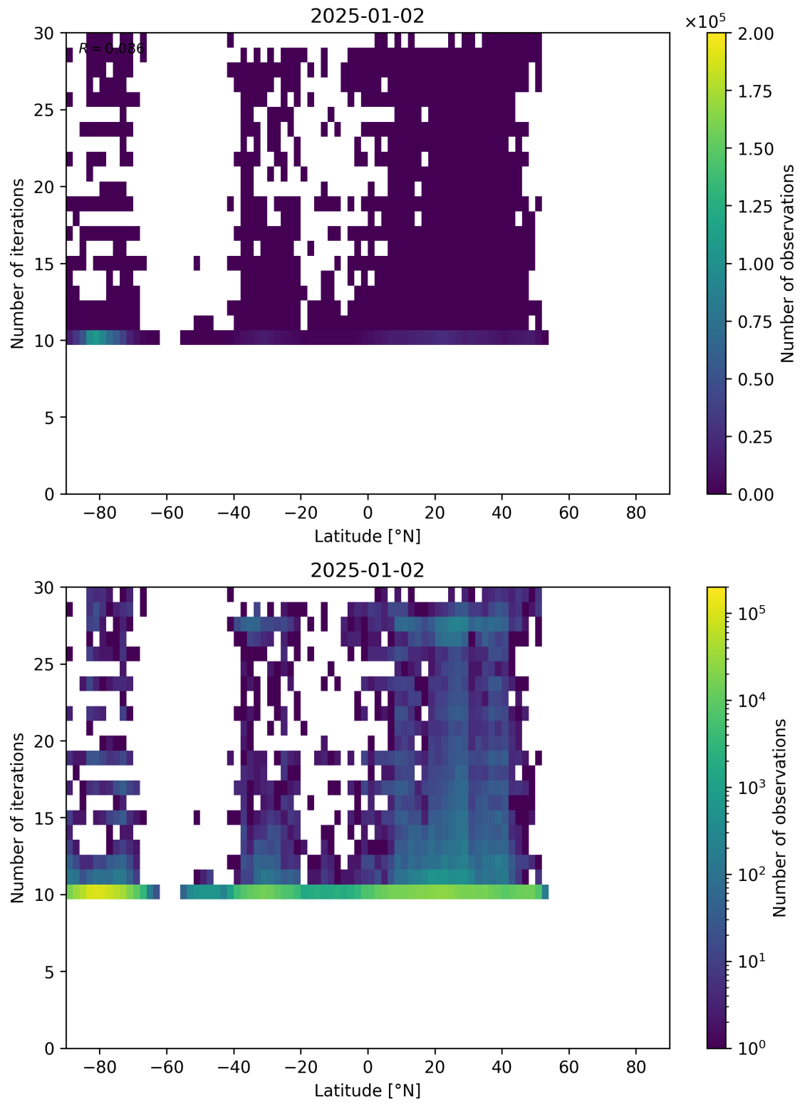
Figure 60: Scatter density plot of “Latitude” against “Number of iterations” for 2025-01-01 to 2025-01-03.
