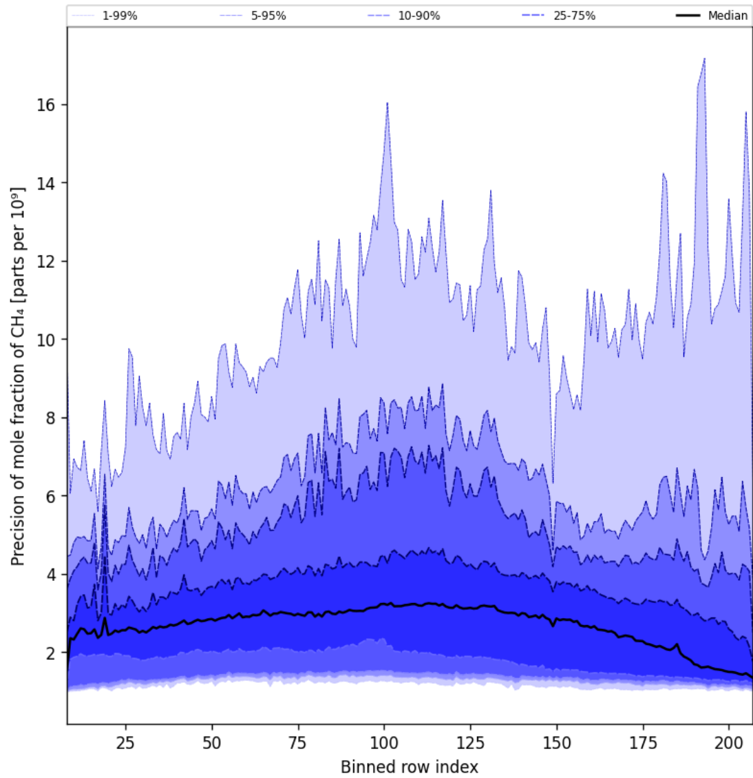
Figure 35: Along track statistics of “Precision of mole fraction of CH 4 ” for 2025-01-01 to 2025-01-03
