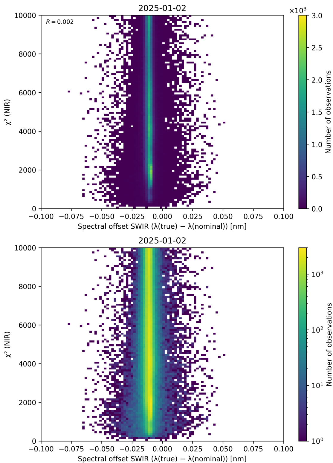
Figure 117: Scatter density plot of “Spectral offset SWIR ( \lambda_{\text{true}} - \lambda_{\text{nominal}} )” against “ \chi^2 (NIR)” for 2025-01-01 to 2025-01-03.
