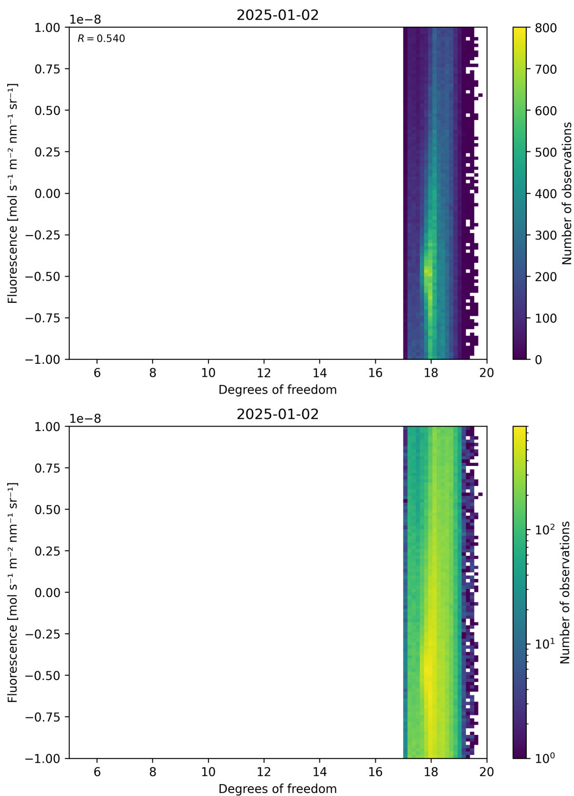
Figure 51: Scatter density plot of “Degrees of freedom” against “Fluorescence” for 2025-01-01 to 2025-01-03.
