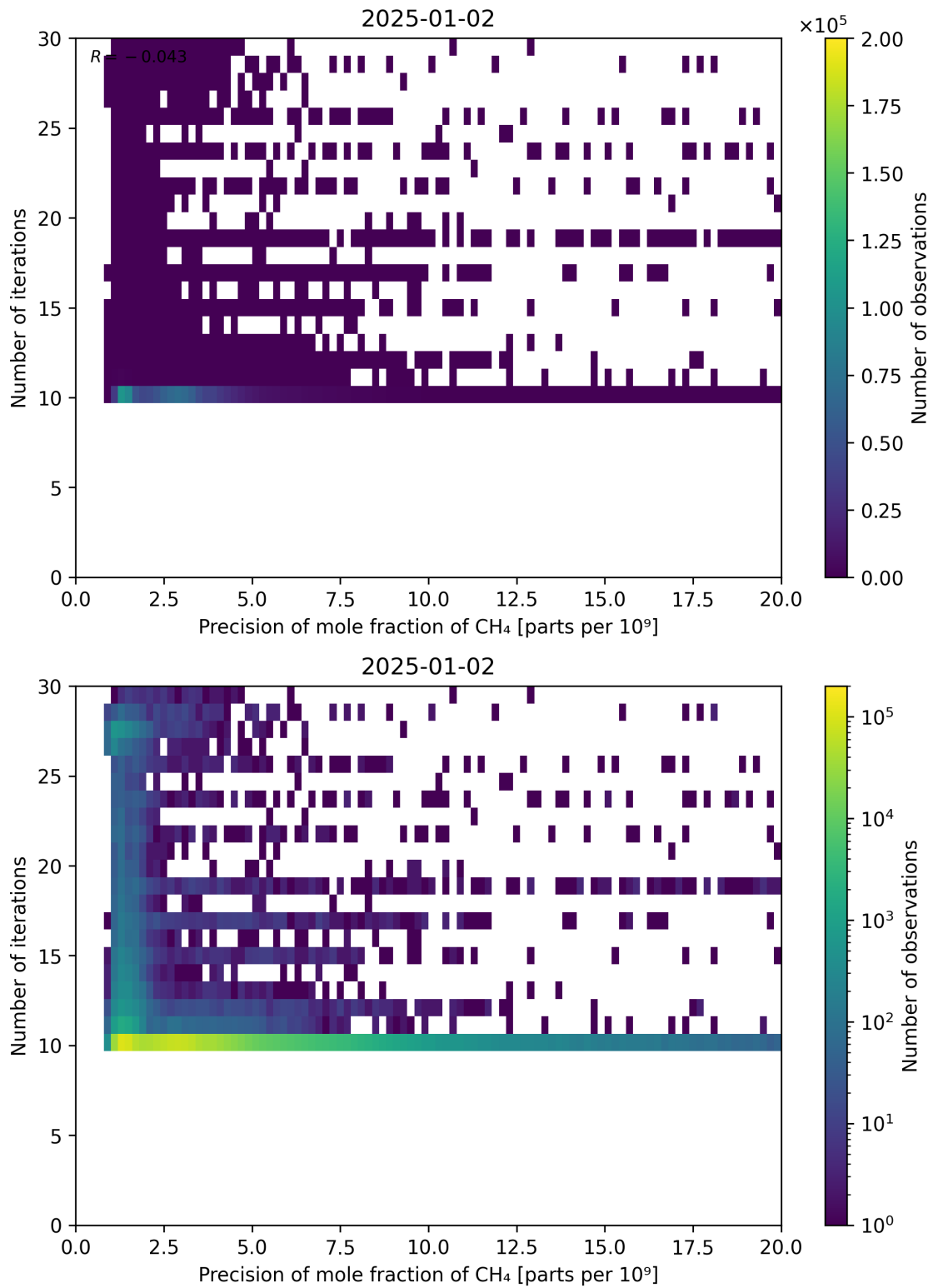
Figure 83: Scatter density plot of “Precision of mole fraction of CH 4 ” against “Number of iterations” for 2025-01-01 to 2025-01-03.
