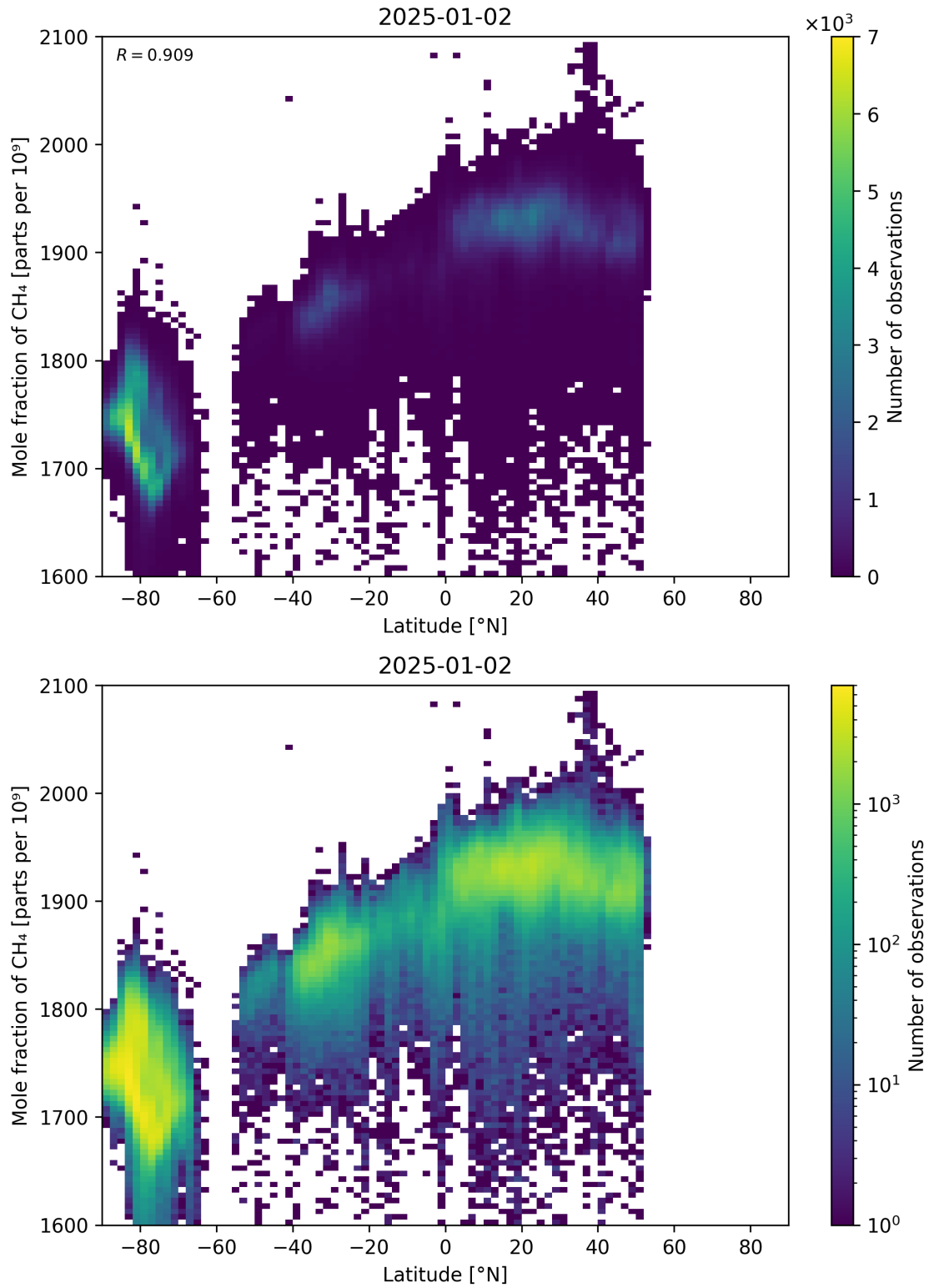
Figure 57: Scatter density plot of “Latitude” against “Mole fraction of \text{CH}_4 ” for 2025-01-01 to 2025-01-03.
