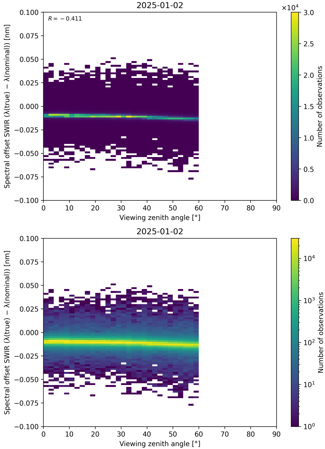
Figure 116: Scatter density plot of “Viewing zenith angle” against “Spectral offset SWIR ( \lambda_{\text{true}} - \lambda_{\text{nominal}} )” for 2025-01-01 to 2025-01-03.
