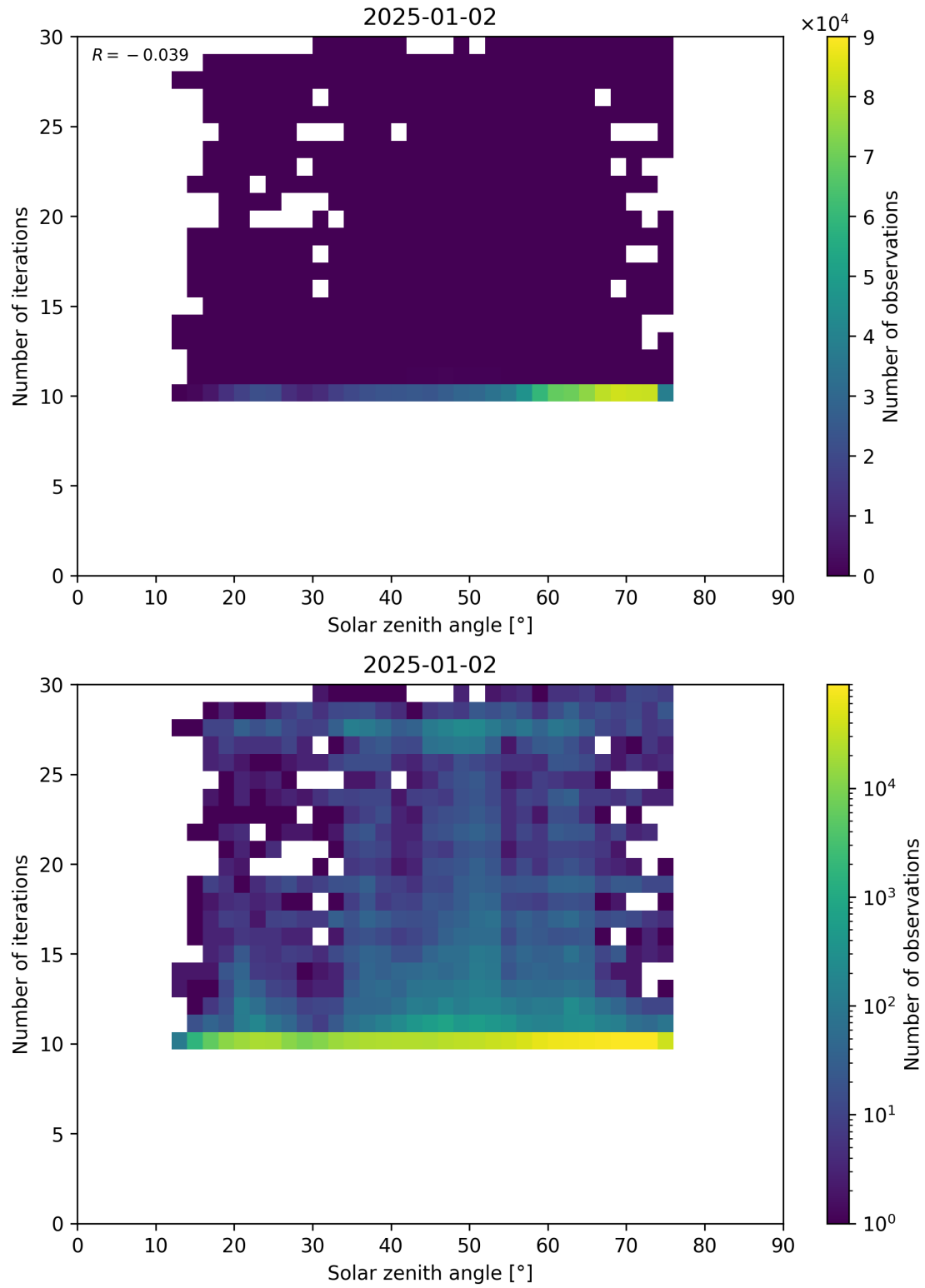
Figure 102: Scatter density plot of “Solar zenith angle” against “Number of iterations” for 2025-01-01 to 2025-01-03.
