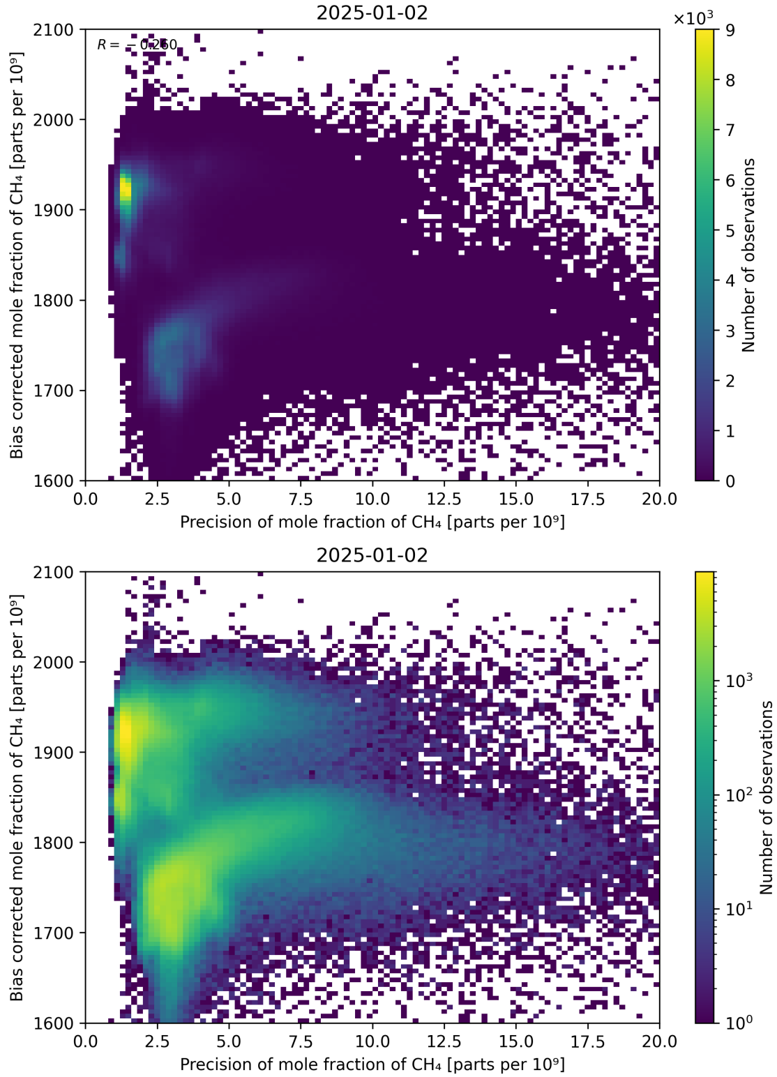
Figure 82: Scatter density plot of “Precision of mole fraction of CH 4 ” against “Bias corrected mole fraction of CH 4 ” for 2025-01-01 to 2025-01-03.
