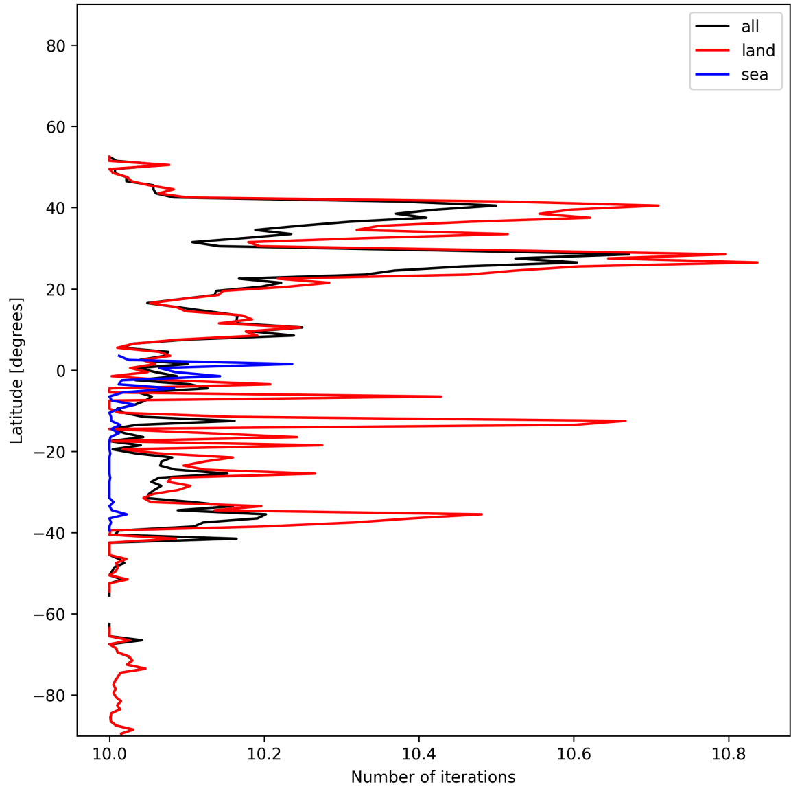
Figure 20: Zonal average of “Number of iterations” for 2025-01-01 to 2025-01-03.
