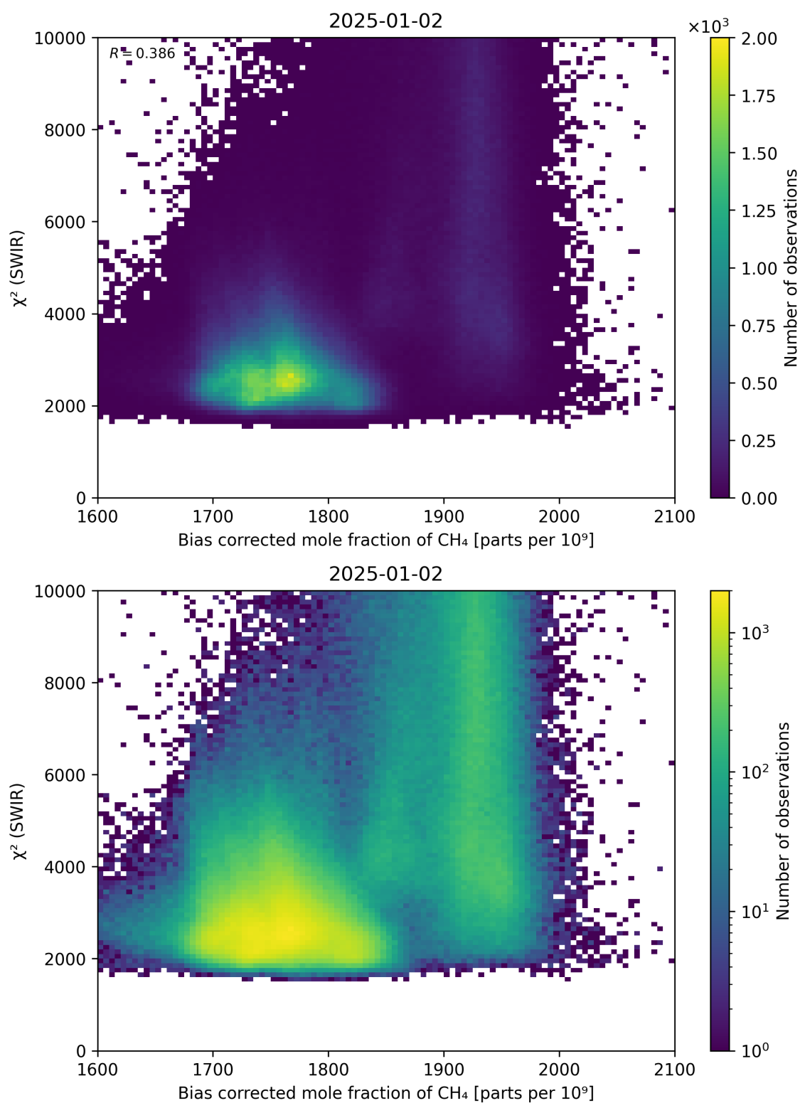
Figure 64: Scatter density plot of “Bias corrected mole fraction of \text{CH}_4 ” against “ \chi^2 (SWIR)” for 2025-01-01 to 2025-01-03.
