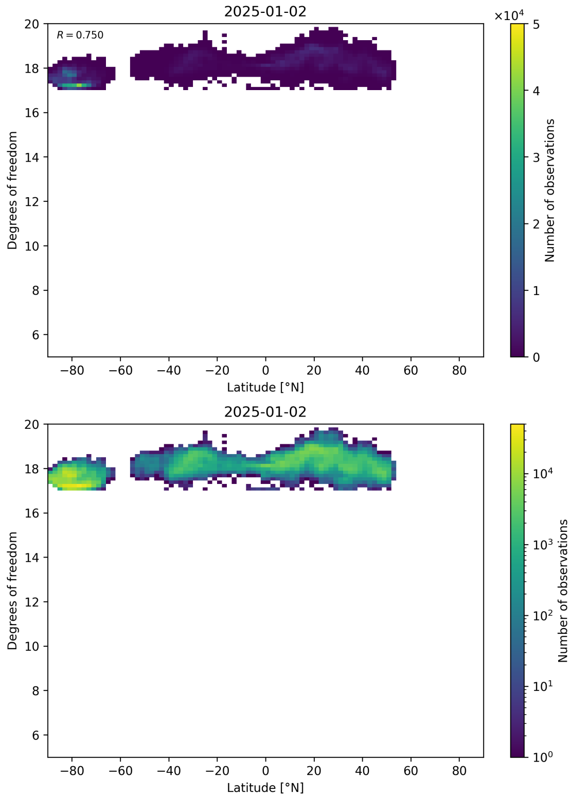
Figure 55: Scatter density plot of “Latitude” against “Degrees of freedom” for 2025-01-01 to 2025-01-03.
