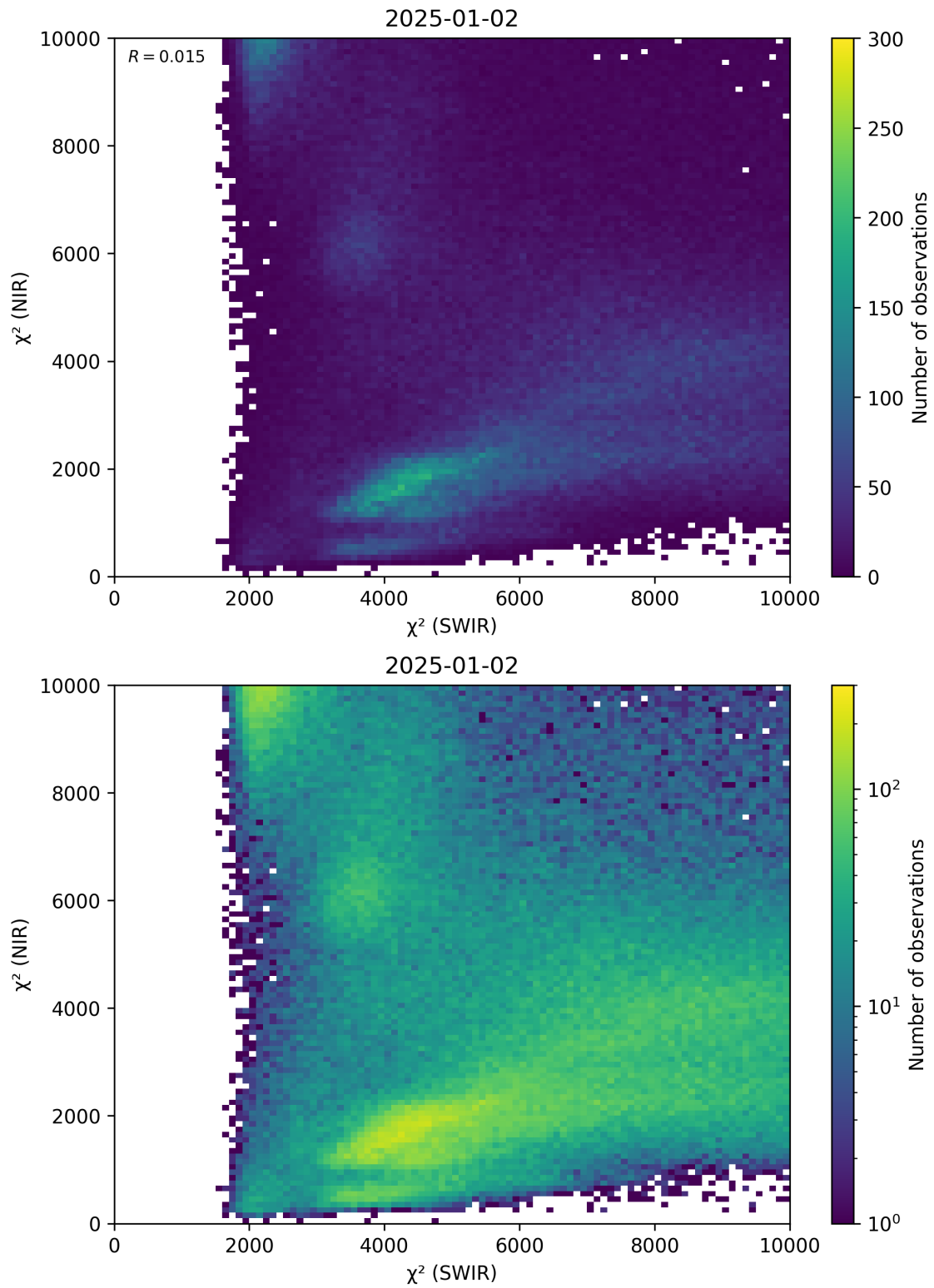
Figure 47: Scatter density plot of “ \chi^2 (SWIR)” against “ \chi^2 (NIR)” for 2025-01-01 to 2025-01-03.
