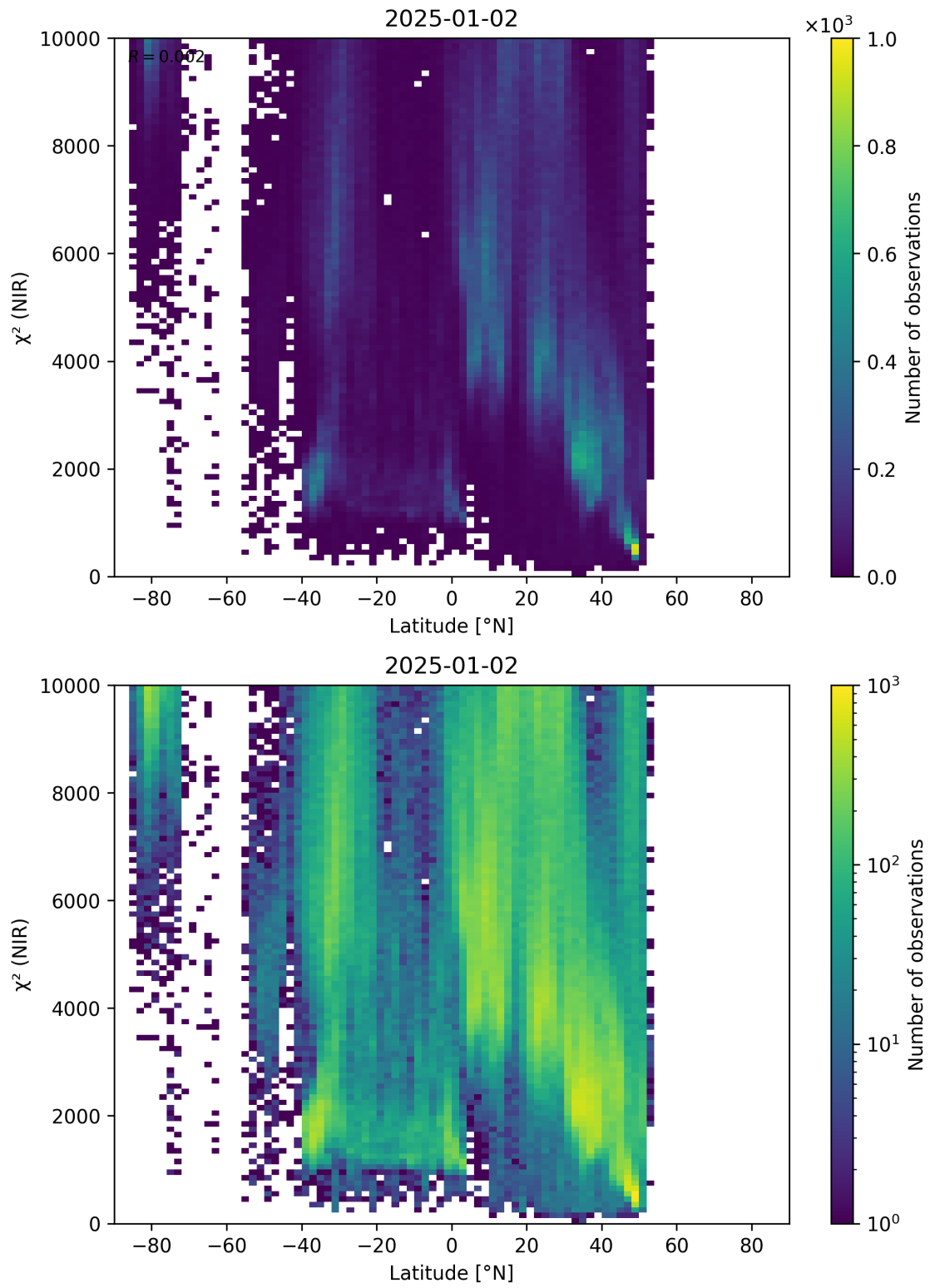
Figure 53: Scatter density plot of “Latitude” against “ \chi^2 (NIR)” for 2025-01-01 to 2025-01-03.
