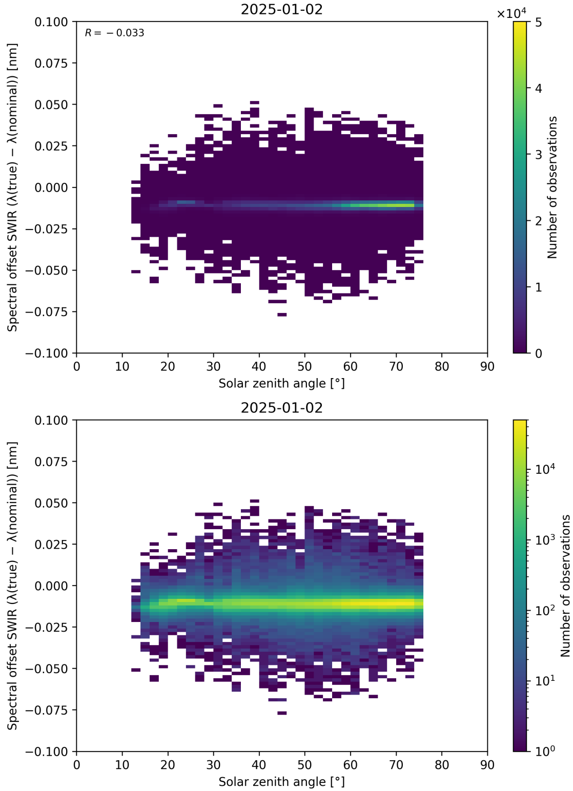
Figure 104: Scatter density plot of “Solar zenith angle” against “Spectral offset SWIR ( \lambda_{\text{true}} - \lambda_{\text{nominal}} )” for 2025-01-01 to 2025-01-03.
