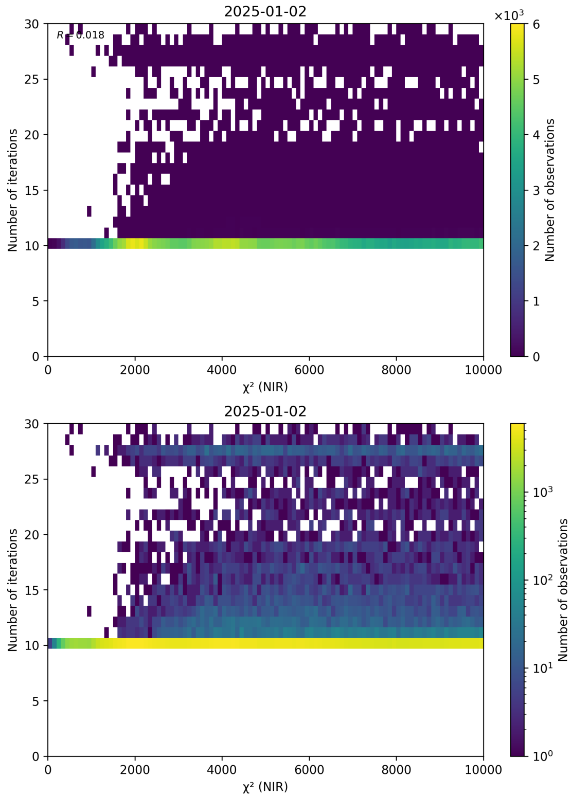
Figure 46: Scatter density plot of “ \chi^2 (NIR)” against “Number of iterations” for 2025-01-01 to 2025-01-03.
