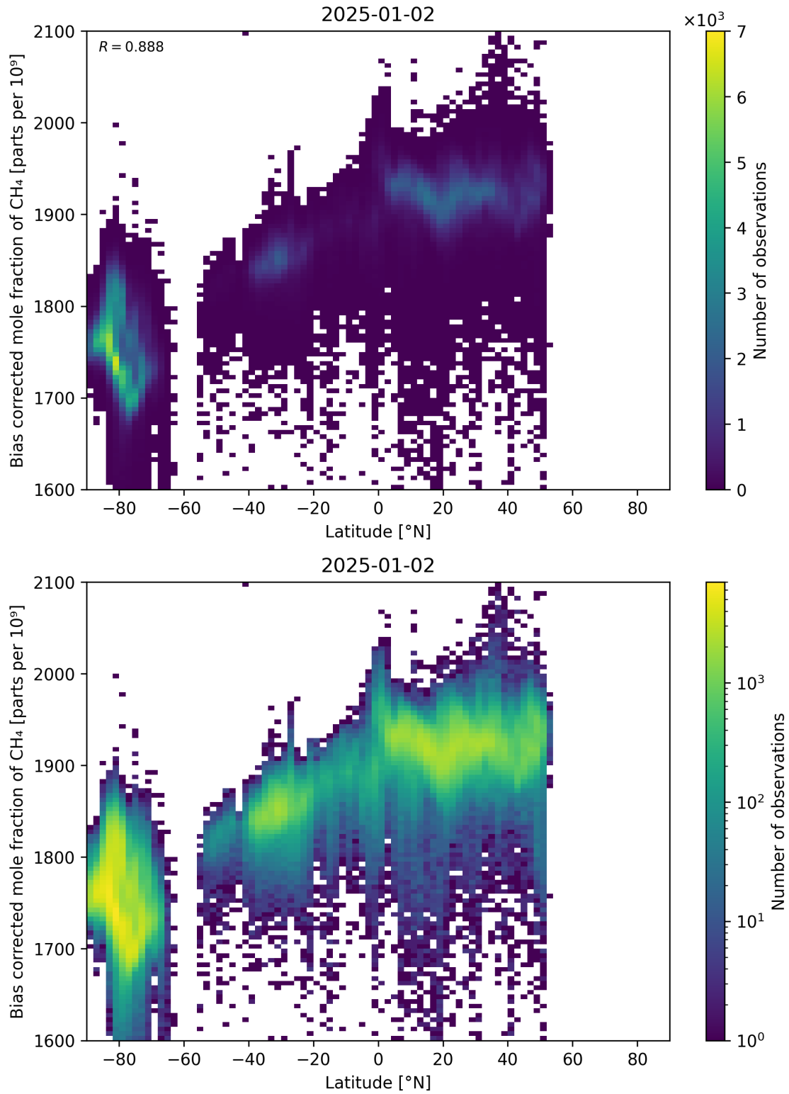
Figure 58: Scatter density plot of “Latitude” against “Bias corrected mole fraction of CH 4 ” for 2025-01-01 to 2025-01-03.
