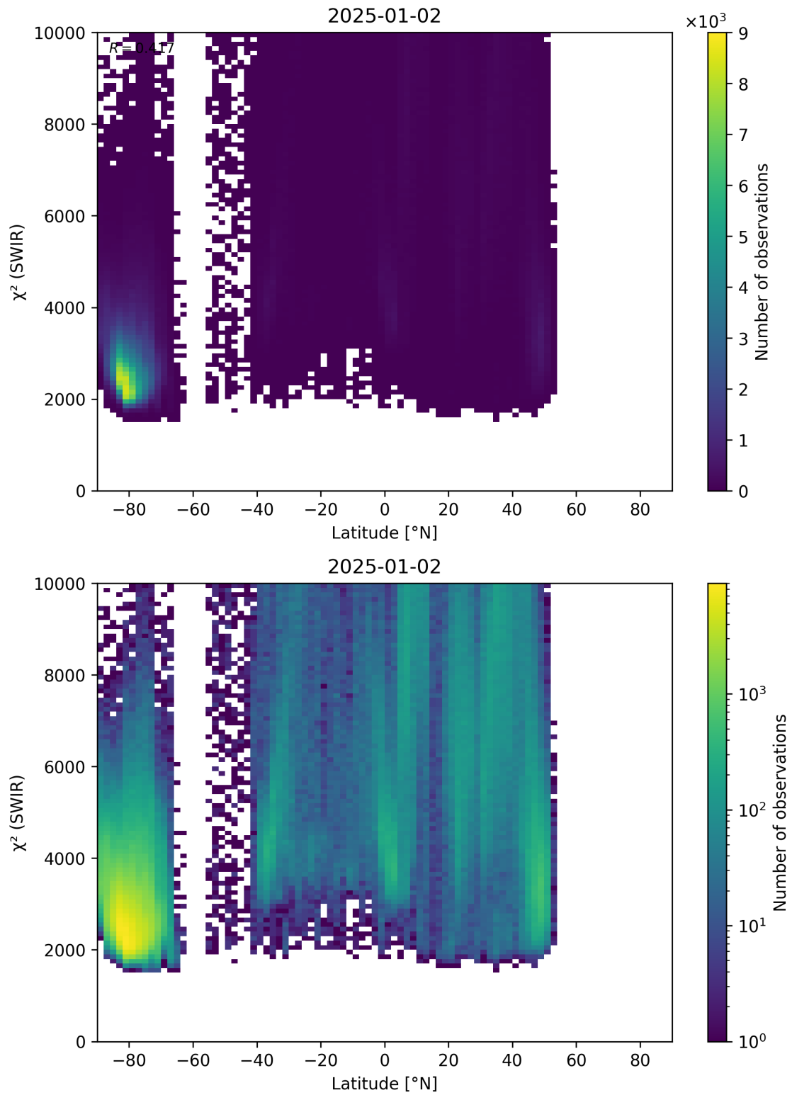
Figure 54: Scatter density plot of “Latitude” against “ \chi^2 (SWIR)” for 2025-01-01 to 2025-01-03.
