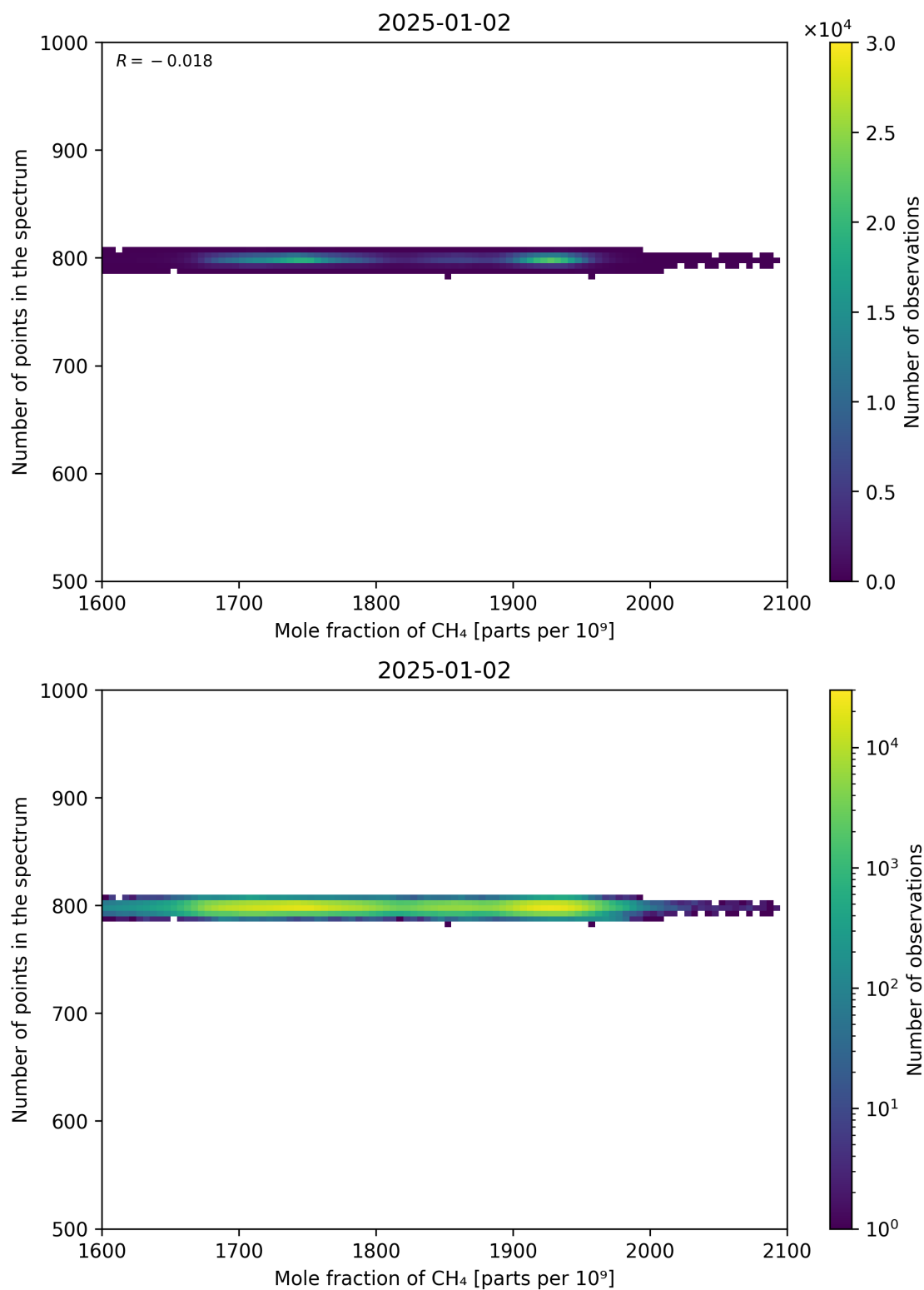
Figure 77: Scatter density plot of “Mole fraction of CH 4 ” against “Number of points in the spectrum” for 2025-01-01 to 2025-01-03.
