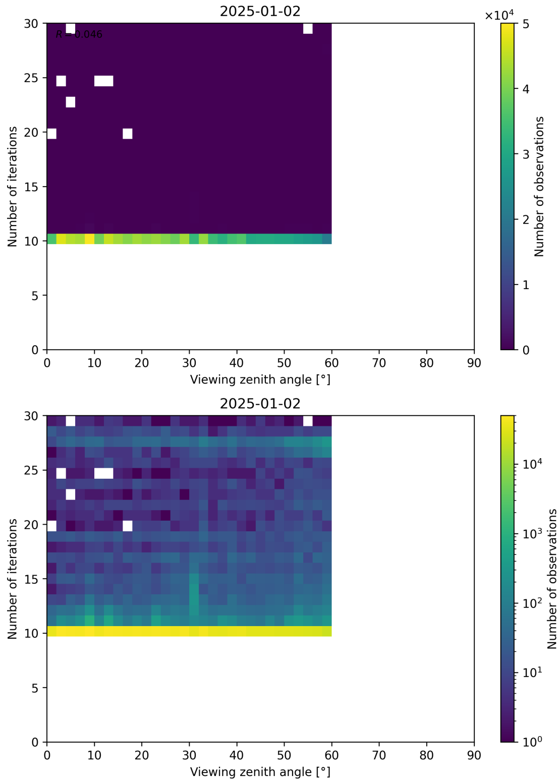
Figure 113: Scatter density plot of “Viewing zenith angle” against “Number of iterations” for 2025-01-01 to 2025-01-03.
