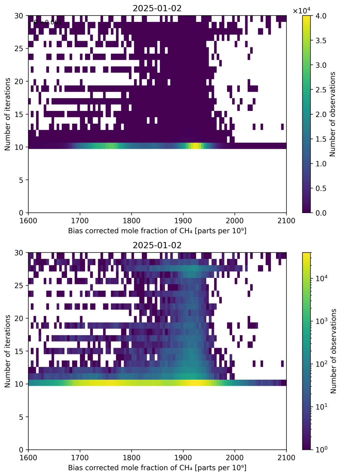
Figure 67: Scatter density plot of “Bias corrected mole fraction of CH 4 ” against “Number of iterations” for 2025-01-01 to 2025-01-03.
