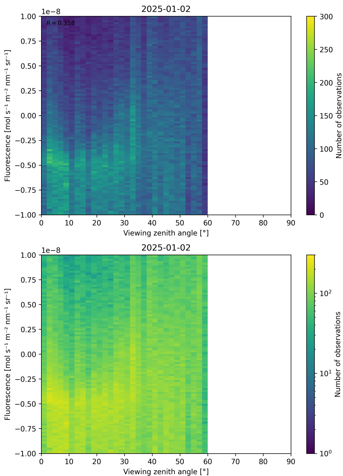
Figure 108: Scatter density plot of “Viewing zenith angle” against “Fluorescence” for 2025-01-01 to 2025-01-03.
