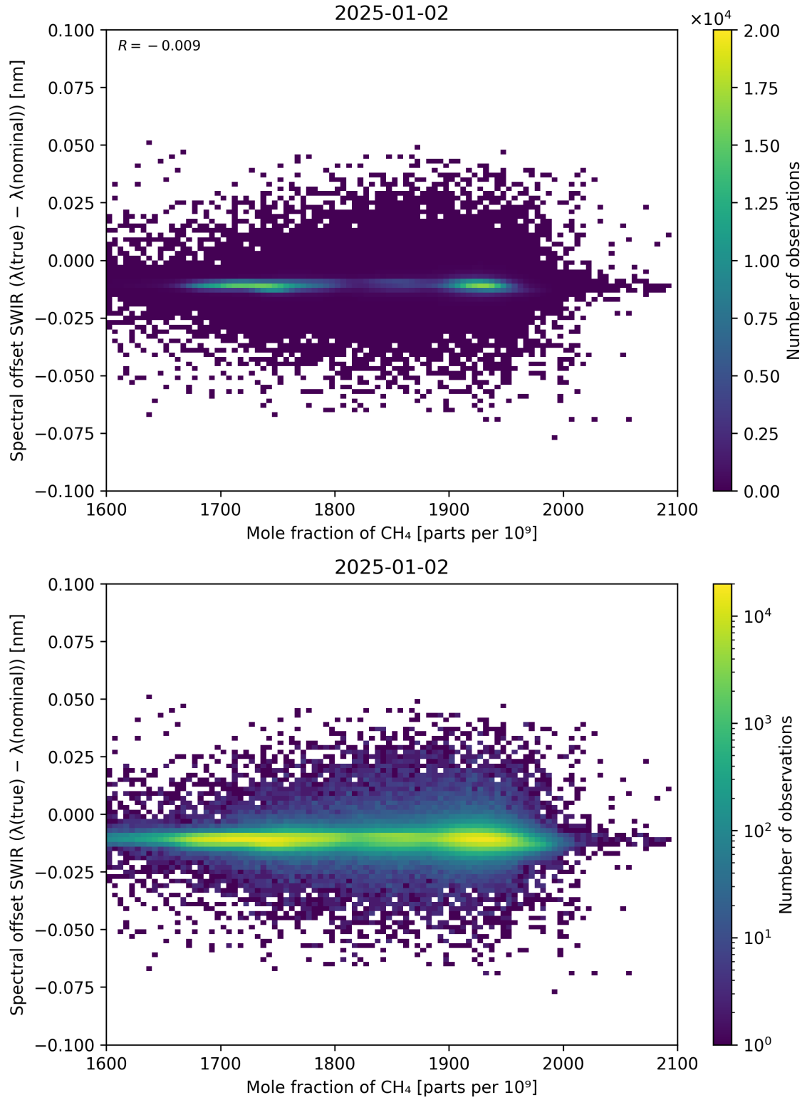
Figure 86: Scatter density plot of “Mole fraction of \text{CH}_4 ” against “Spectral offset SWIR ( \lambda_{\text{true}} - \lambda_{\text{nominal}} )” for 2025-01-01 to 2025-01-03.
