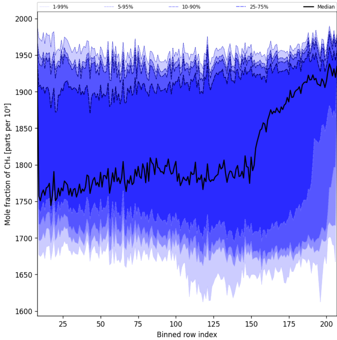
Figure 34: Along track statistics of “Mole fraction of CH 4 ” for 2025-01-01 to 2025-01-03
