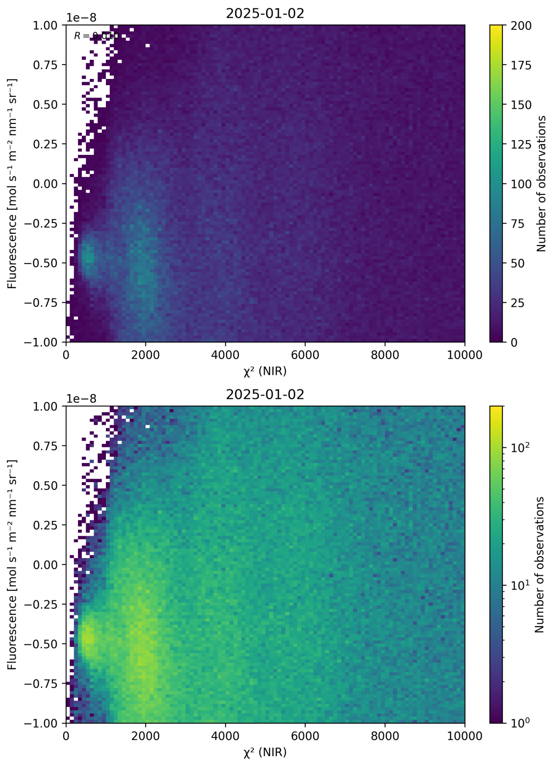
Figure 45: Scatter density plot of “ \chi^2 (NIR)” against “Fluorescence” for 2025-01-01 to 2025-01-03.
