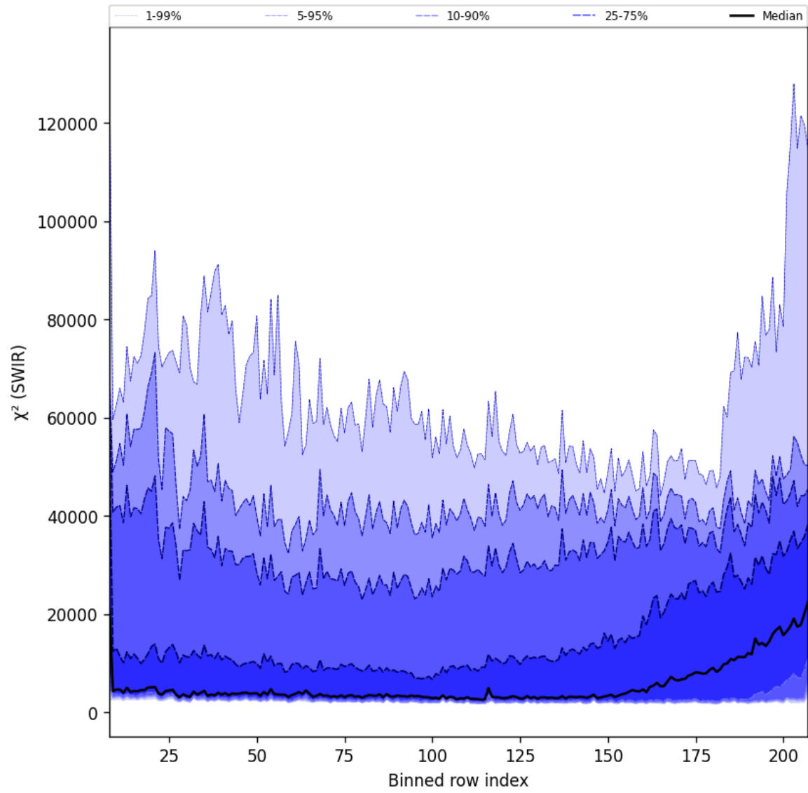
Figure 39: Along track statistics of “ \chi^2 (SWIR)” for 2025-01-01 to 2025-01-03
