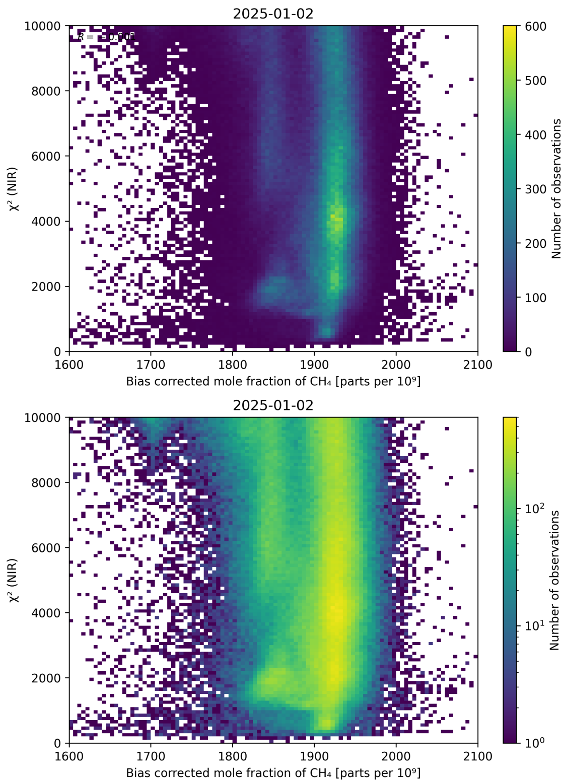
Figure 63: Scatter density plot of “Bias corrected mole fraction of \text{CH}_4 ” against “ \chi^2 (NIR)” for 2025-01-01 to 2025-01-03.
