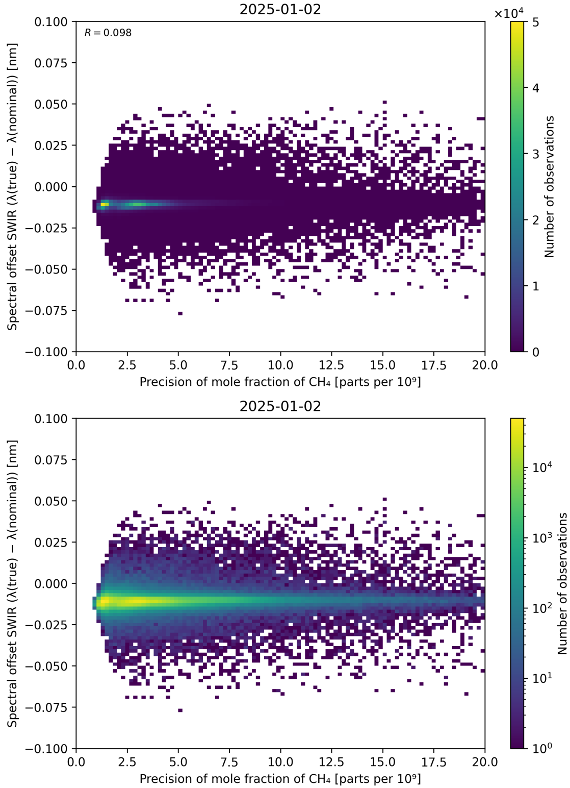
Figure 85: Scatter density plot of “Precision of mole fraction of \text{CH}_4 ” against “Spectral offset SWIR ( \lambda_{\text{true}} - \lambda_{\text{nominal}} )” for 2025-01-01 to 2025-01-03.
