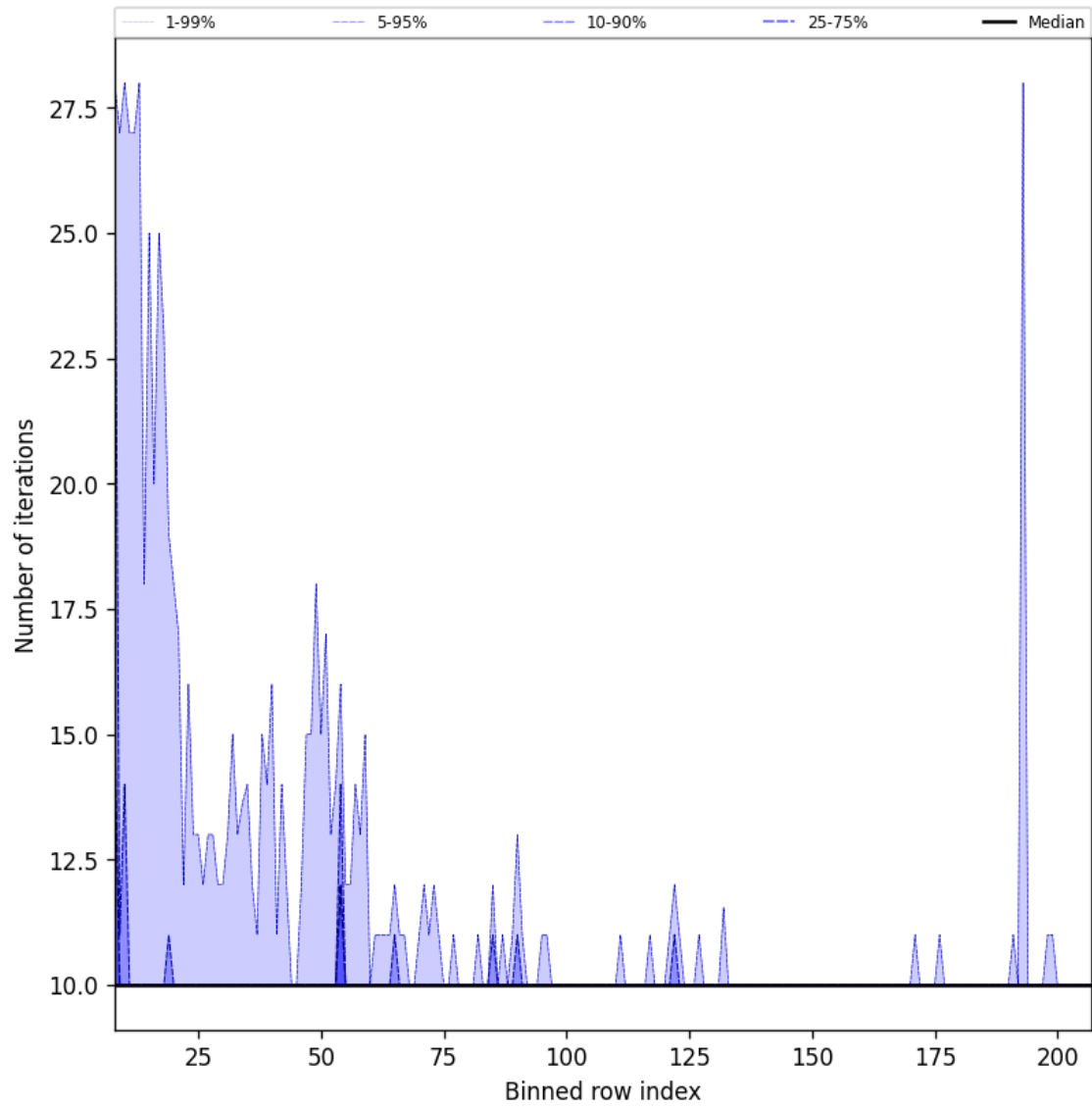
Figure 42: Along track statistics of “Number of iterations” for 2025-01-01 to 2025-01-03
