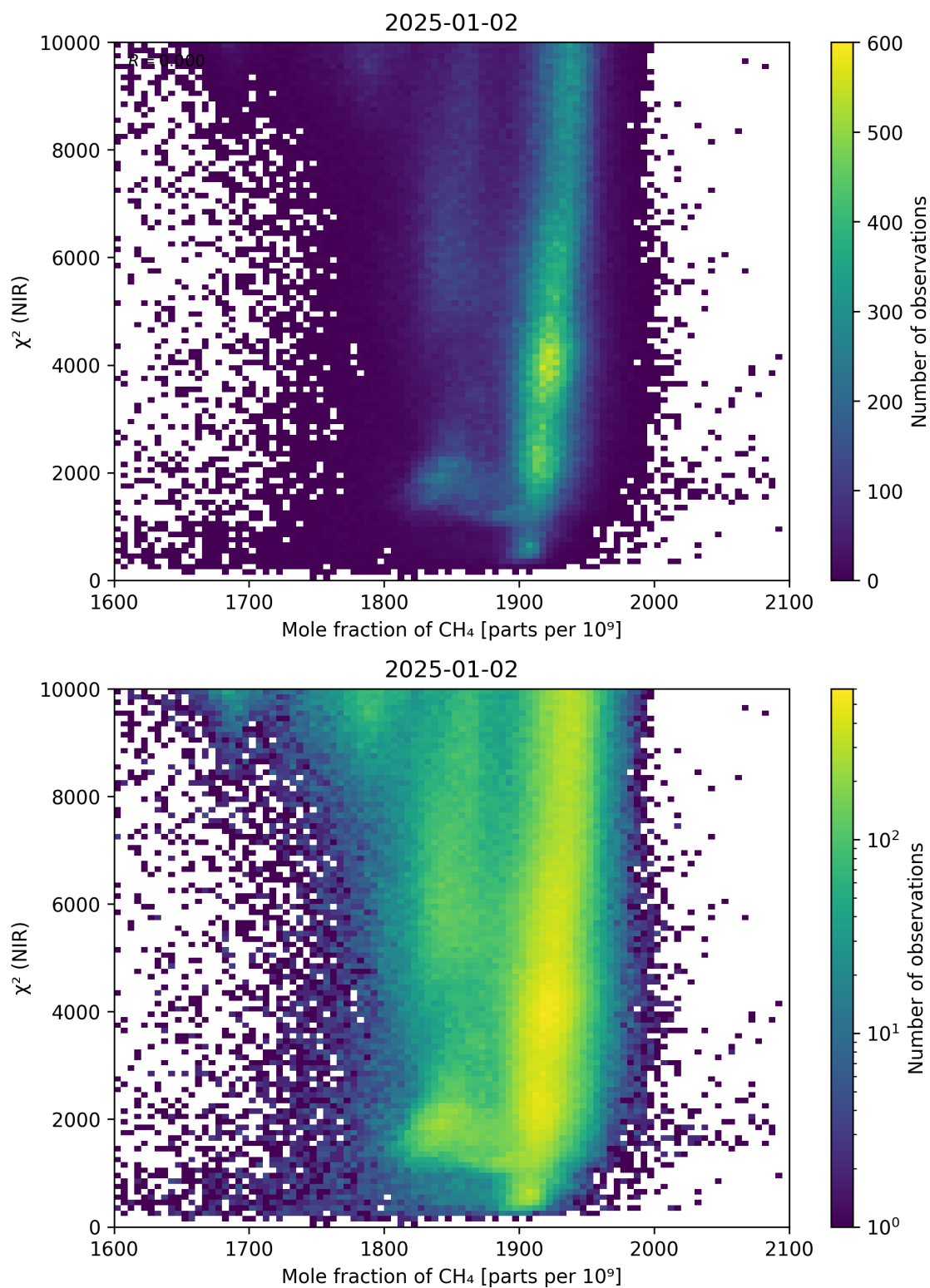
Figure 70: Scatter density plot of “Mole fraction of \text{CH}_4 ” against “ \chi^2 (NIR)” for 2025-01-01 to 2025-01-03.
