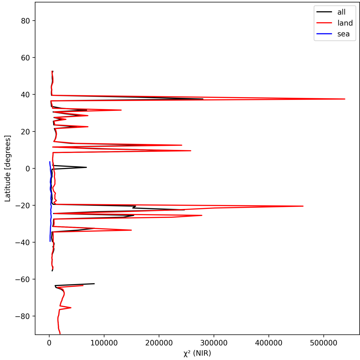
Figure 18: Zonal average of “ \chi^2 (NIR)” for 2025-01-01 to 2025-01-03.
