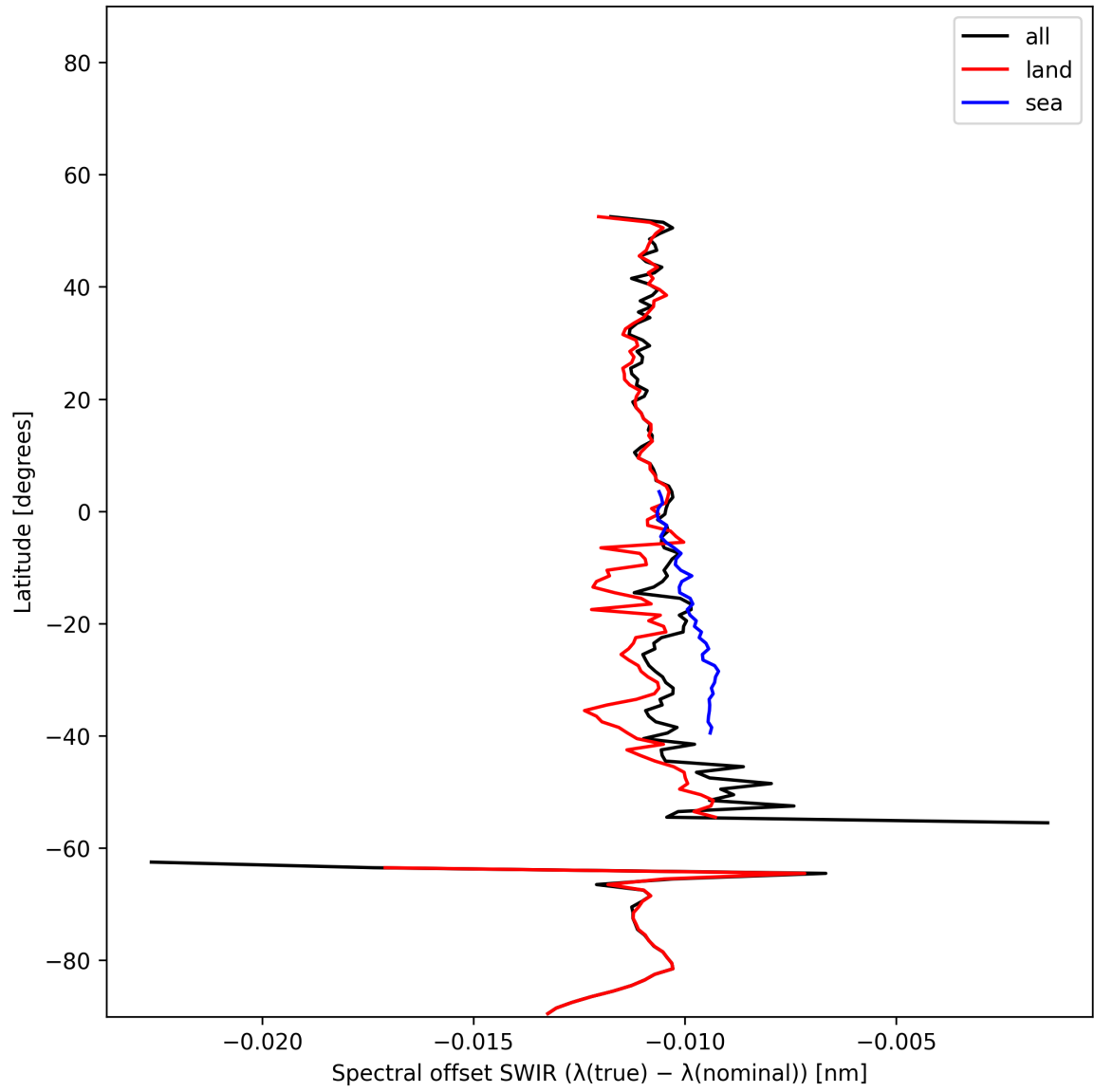
Figure 16: Zonal average of “Spectral offset SWIR ( \lambda_{\text{true}} - \lambda_{\text{nominal}} )” for 2025-01-01 to 2025-01-03.
