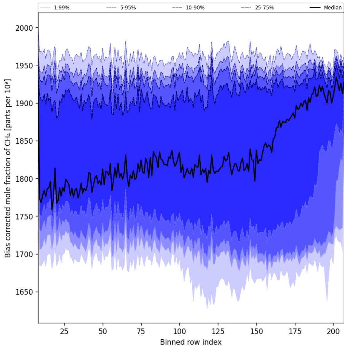
Figure 36: Along track statistics of “Bias corrected mole fraction of CH 4 ” for 2025-01-01 to 2025-01-03
