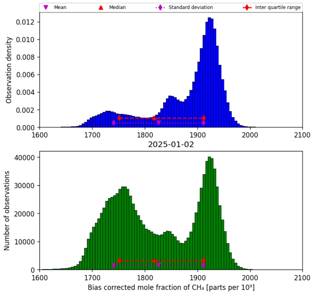
Figure 25: Histogram of “Bias corrected mole fraction of CH 4 ” for 2025-01-01 to 2025-01-03
