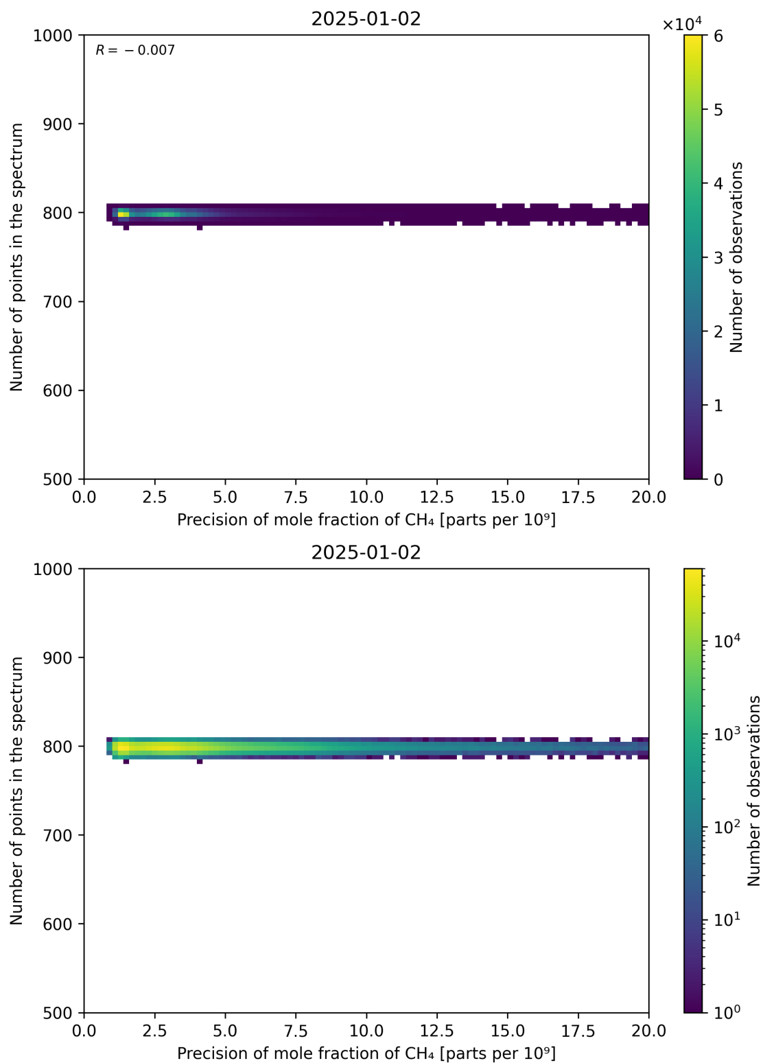
Figure 84: Scatter density plot of “Precision of mole fraction of CH 4 ” against “Number of points in the spectrum” for 2025-01-01 to 2025-01-03.
