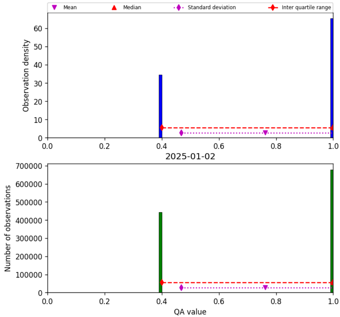
Figure 22: Histogram of “QA value” for 2025-01-01 to 2025-01-03
