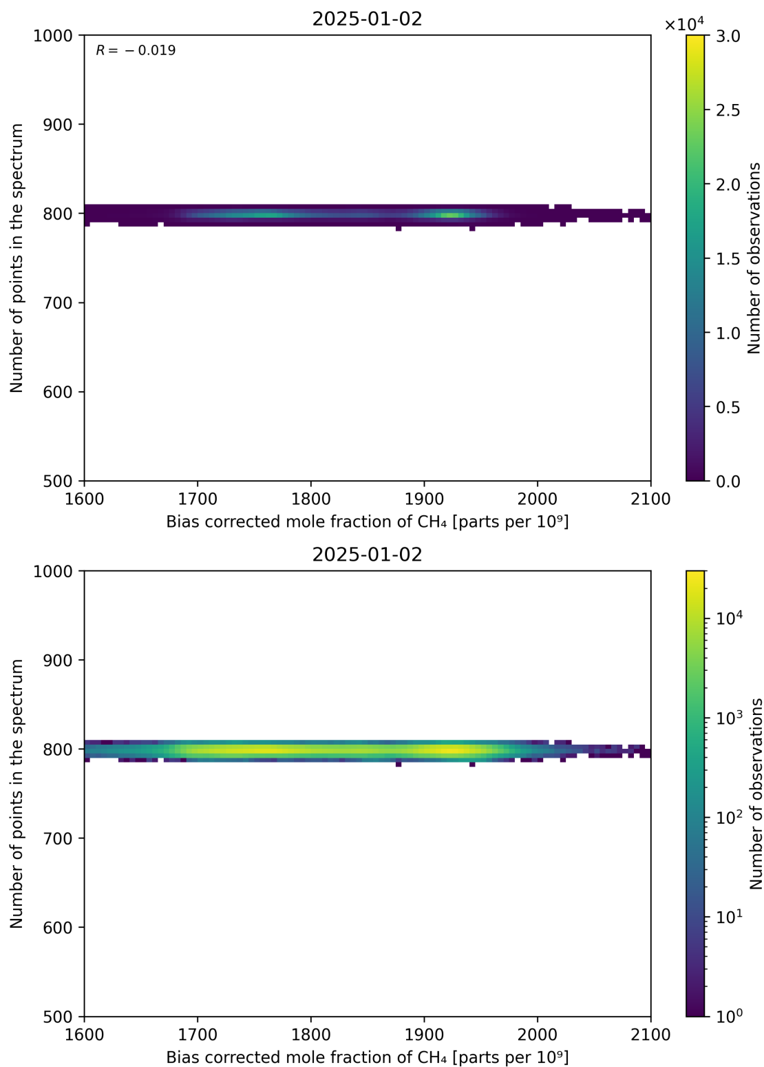
Figure 68: Scatter density plot of “Bias corrected mole fraction of CH 4 ” against “Number of points in the spectrum” for 2025-01-01 to 2025-01-03.
