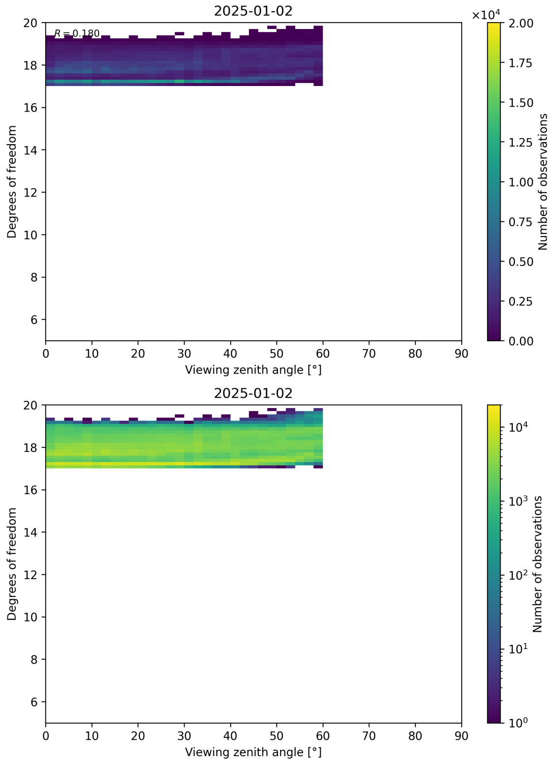
Figure 107: Scatter density plot of “Viewing zenith angle” against “Degrees of freedom” for 2025-01-01 to 2025-01-03.
