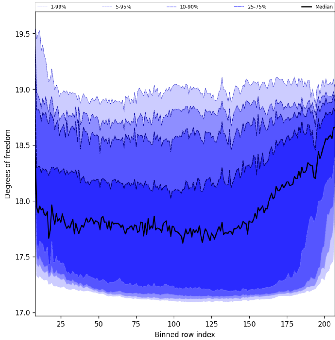
Figure 41: Along track statistics of “Degrees of freedom” for 2025-01-01 to 2025-01-03
