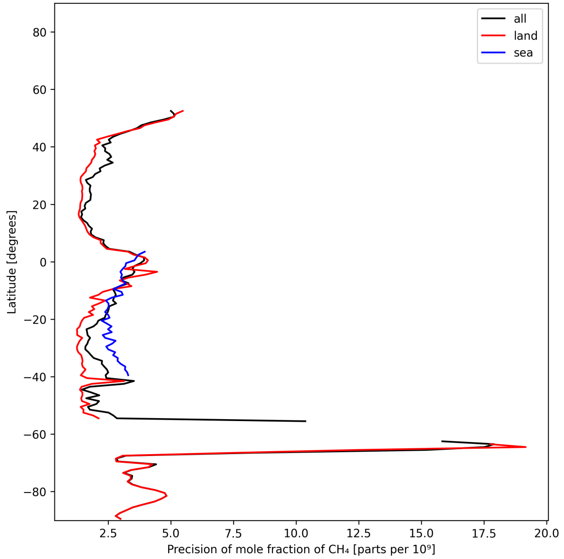
Figure 13: Zonal average of “Precision of mole fraction of CH 4 ” for 2025-01-01 to 2025-01-03.
