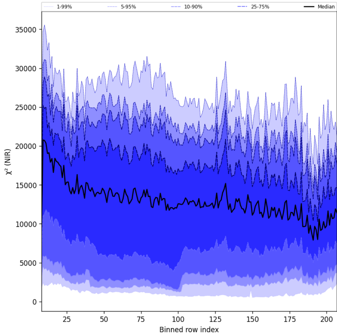
Figure 40: Along track statistics of “ \chi^2 (NIR)” for 2025-01-01 to 2025-01-03
