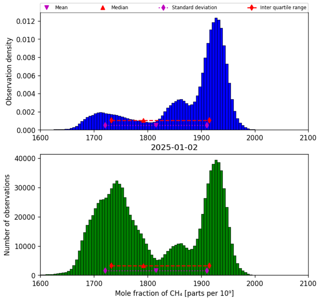
Figure 23: Histogram of “Mole fraction of CH 4 ” for 2025-01-01 to 2025-01-03
