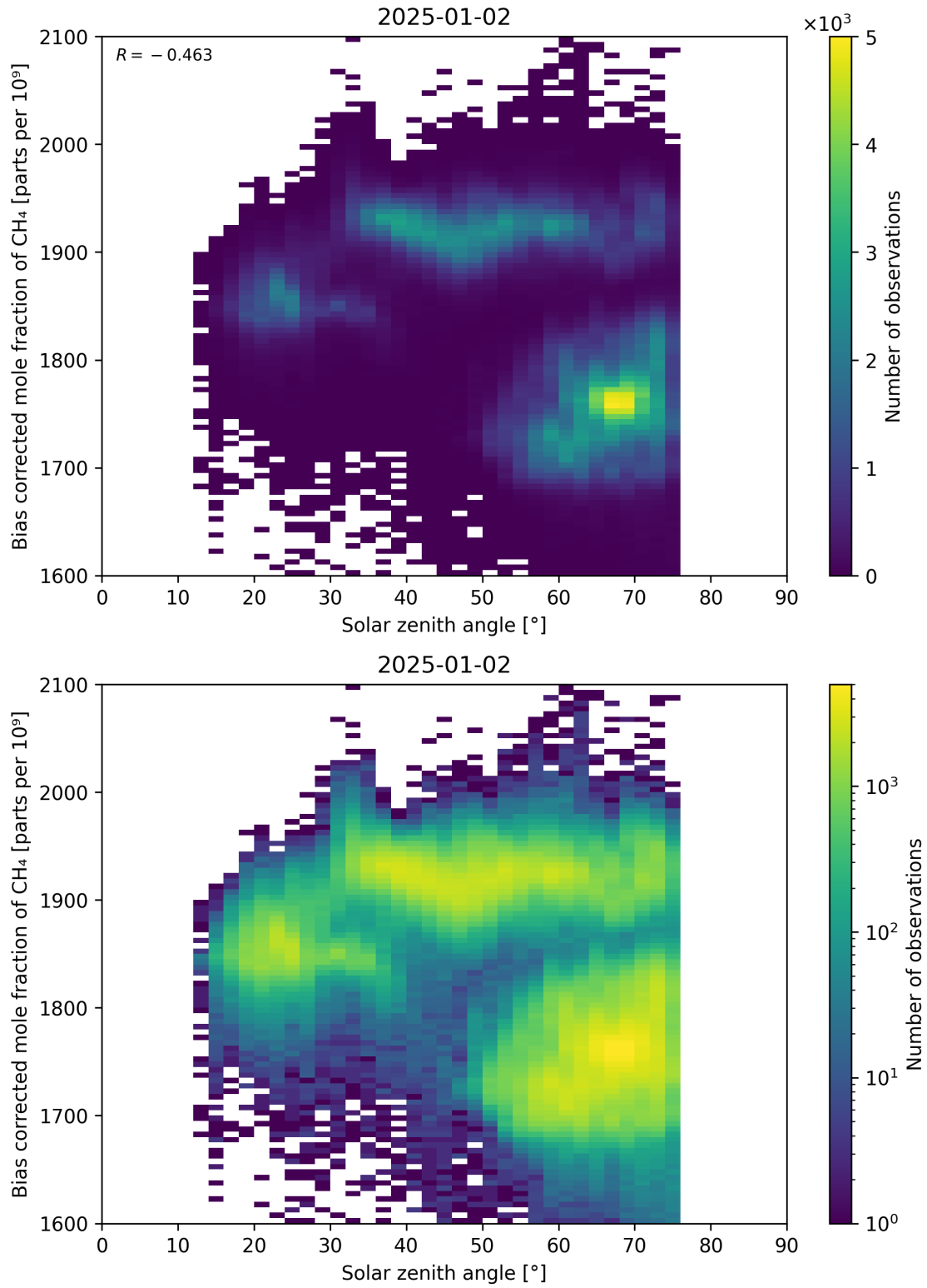
Figure 100: Scatter density plot of “Solar zenith angle” against “Bias corrected mole fraction of \text{CH}_4 ” for 2025-01-01 to 2025-01-03.
