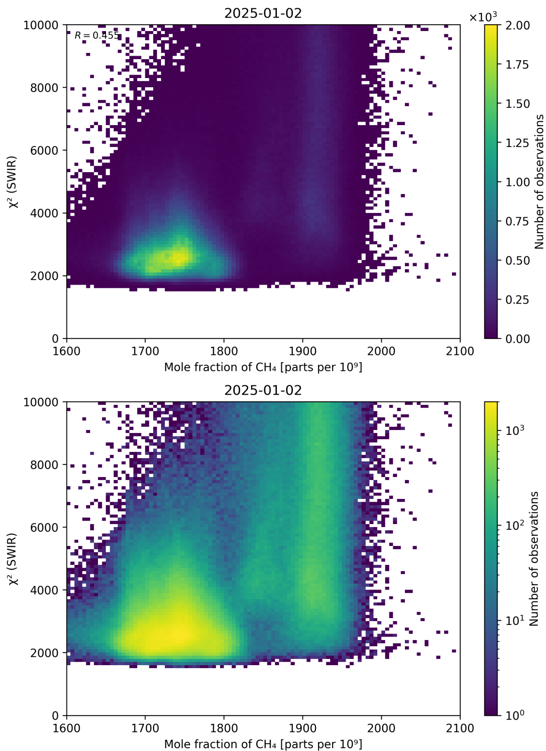
Figure 71: Scatter density plot of “Mole fraction of \text{CH}_4 ” against “ \chi^2 (SWIR)” for 2025-01-01 to 2025-01-03.
