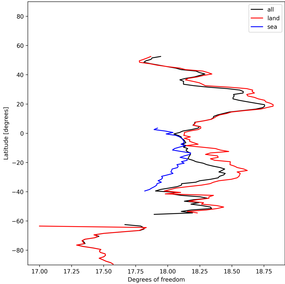
Figure 19: Zonal average of “Degrees of freedom” for 2025-01-01 to 2025-01-03.
