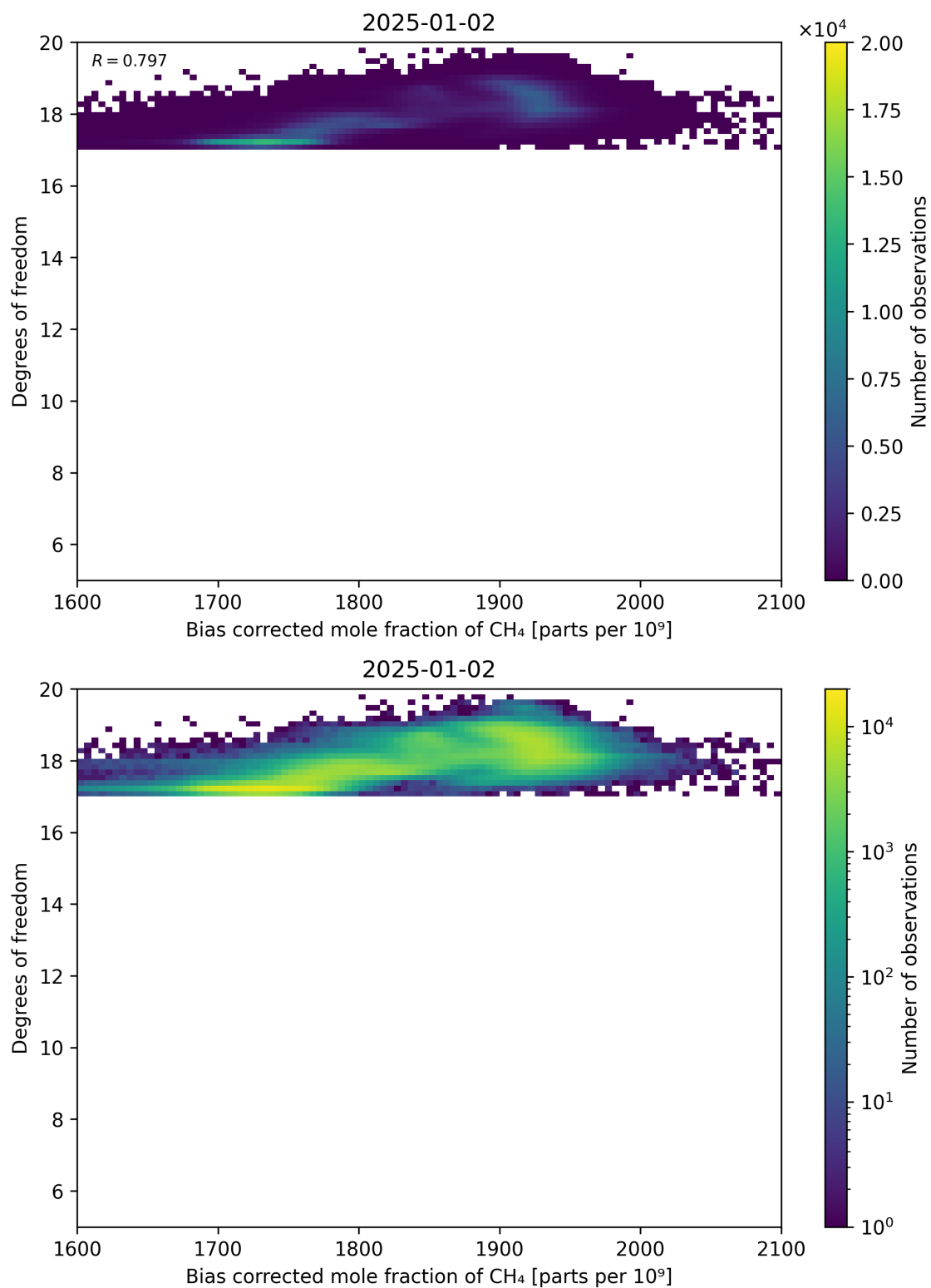
Figure 65: Scatter density plot of “Bias corrected mole fraction of CH 4 ” against “Degrees of freedom” for 2025-01-01 to 2025-01-03.
