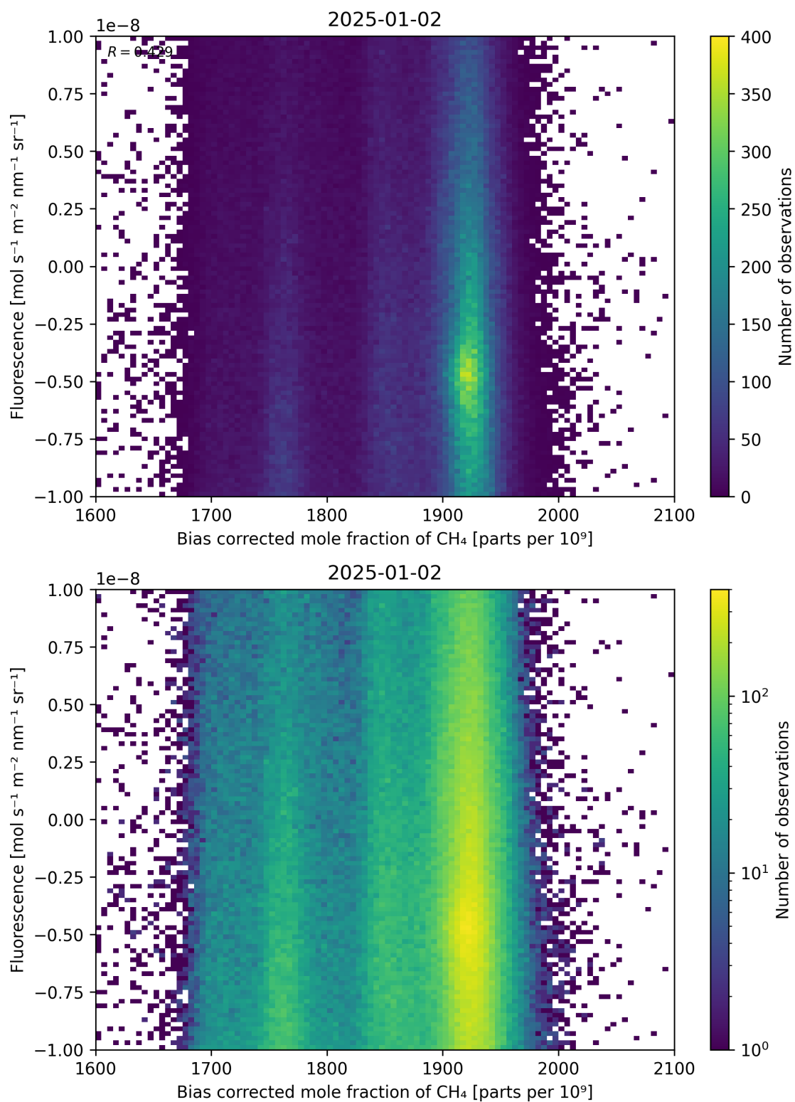
Figure 66: Scatter density plot of “Bias corrected mole fraction of \text{CH}_4 ” against “Fluorescence” for 2025-01-01 to 2025-01-03.
