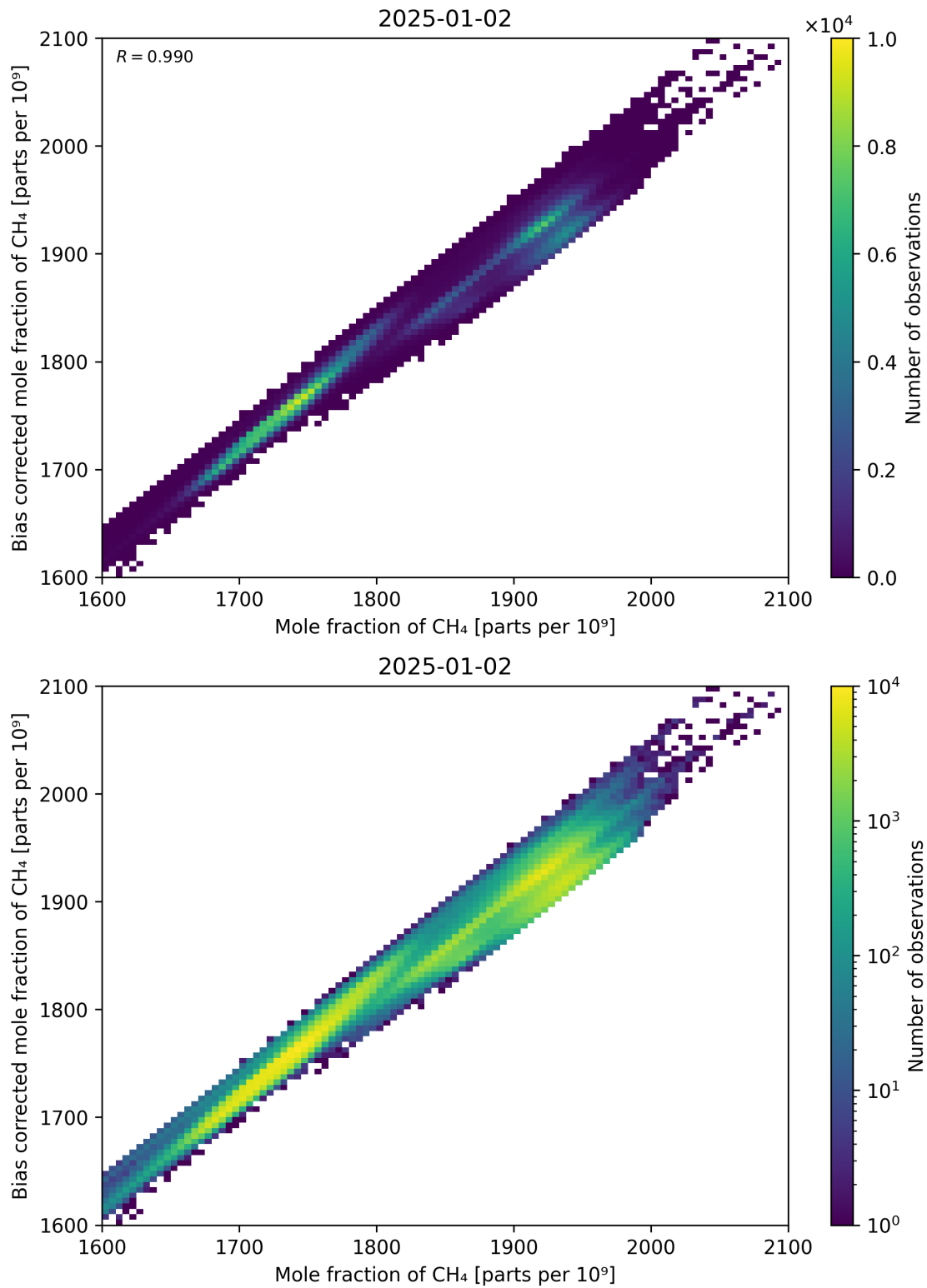
Figure 74: Scatter density plot of “Mole fraction of CH 4 ” against “Bias corrected mole fraction of CH 4 ” for 2025-01-01 to 2025-01-03.
