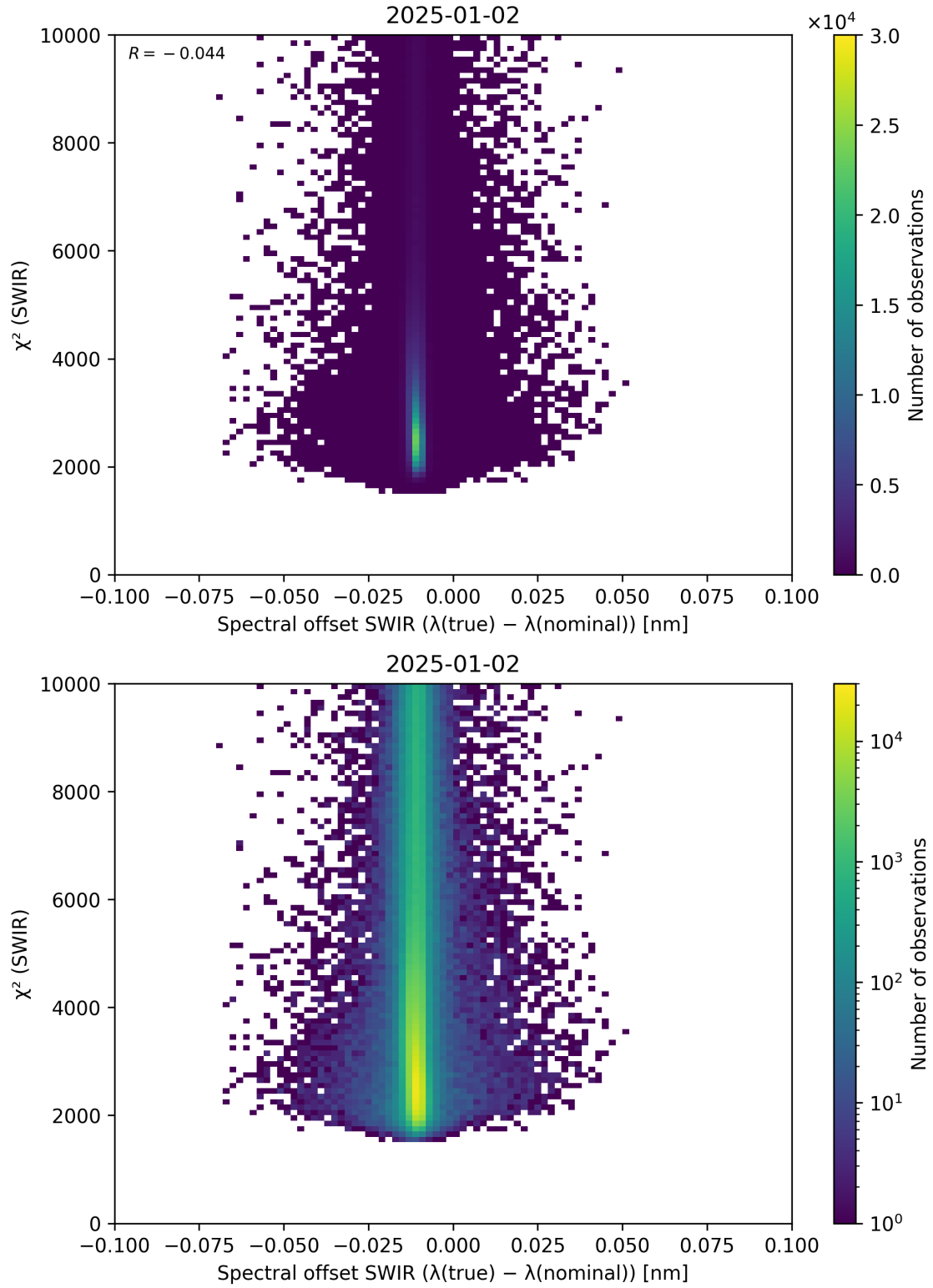
Figure 118: Scatter density plot of “Spectral offset SWIR ( \lambda_{\text{true}} - \lambda_{\text{nominal}} )” against “ \chi^2 (SWIR)” for 2025-01-01 to 2025-01-03.
