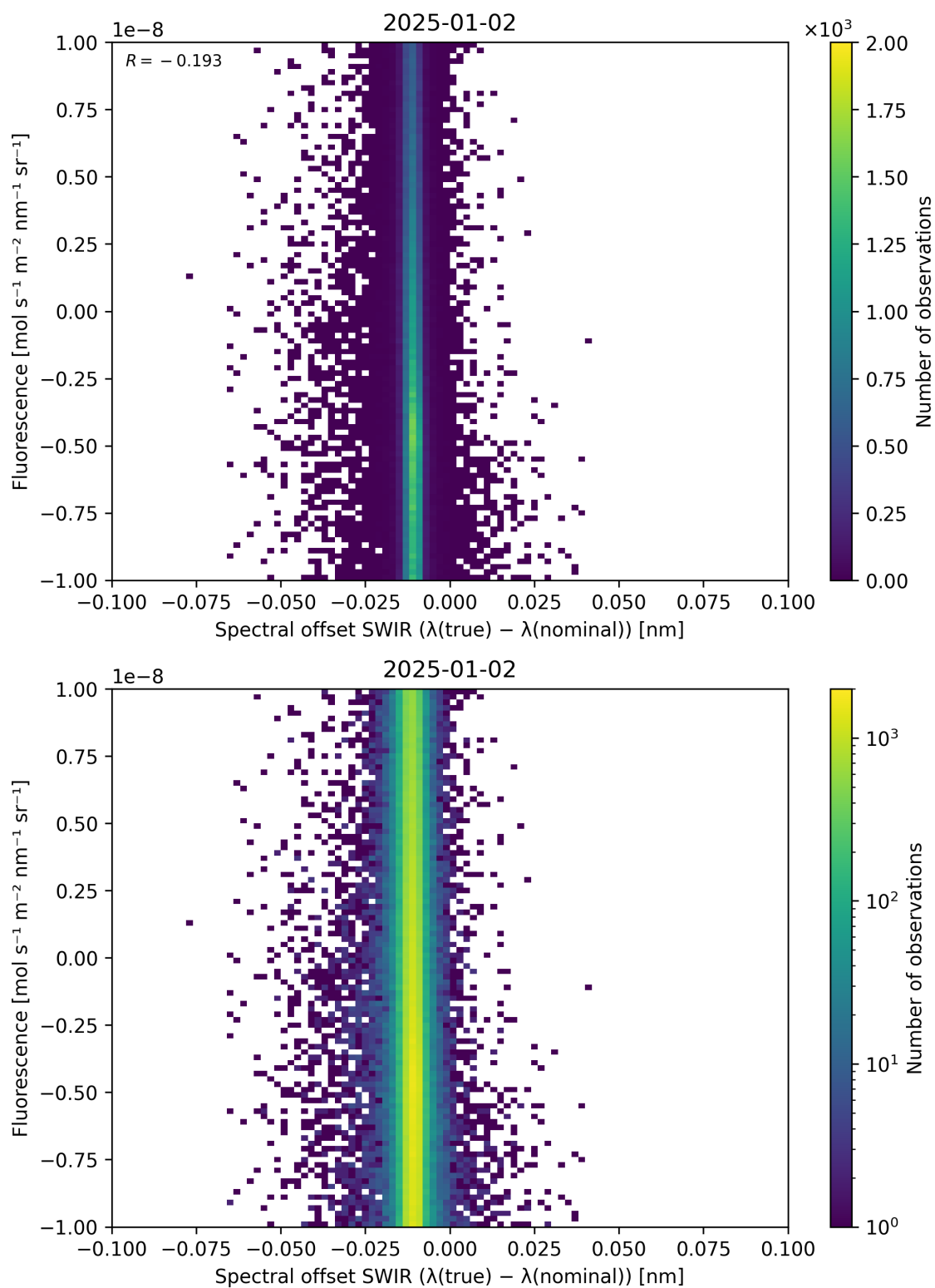
Figure 120: Scatter density plot of “Spectral offset SWIR ( \lambda_{\text{true}} - \lambda_{\text{nominal}} )” against “Fluorescence” for 2025-01-01 to 2025-01-03.
