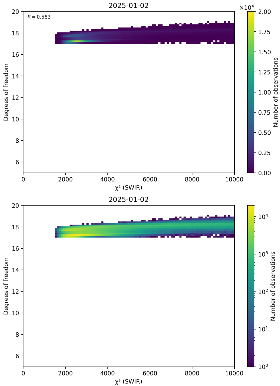
Figure 48: Scatter density plot of “ \chi^2 (SWIR)” against “Degrees of freedom” for 2025-01-01 to 2025-01-03.
