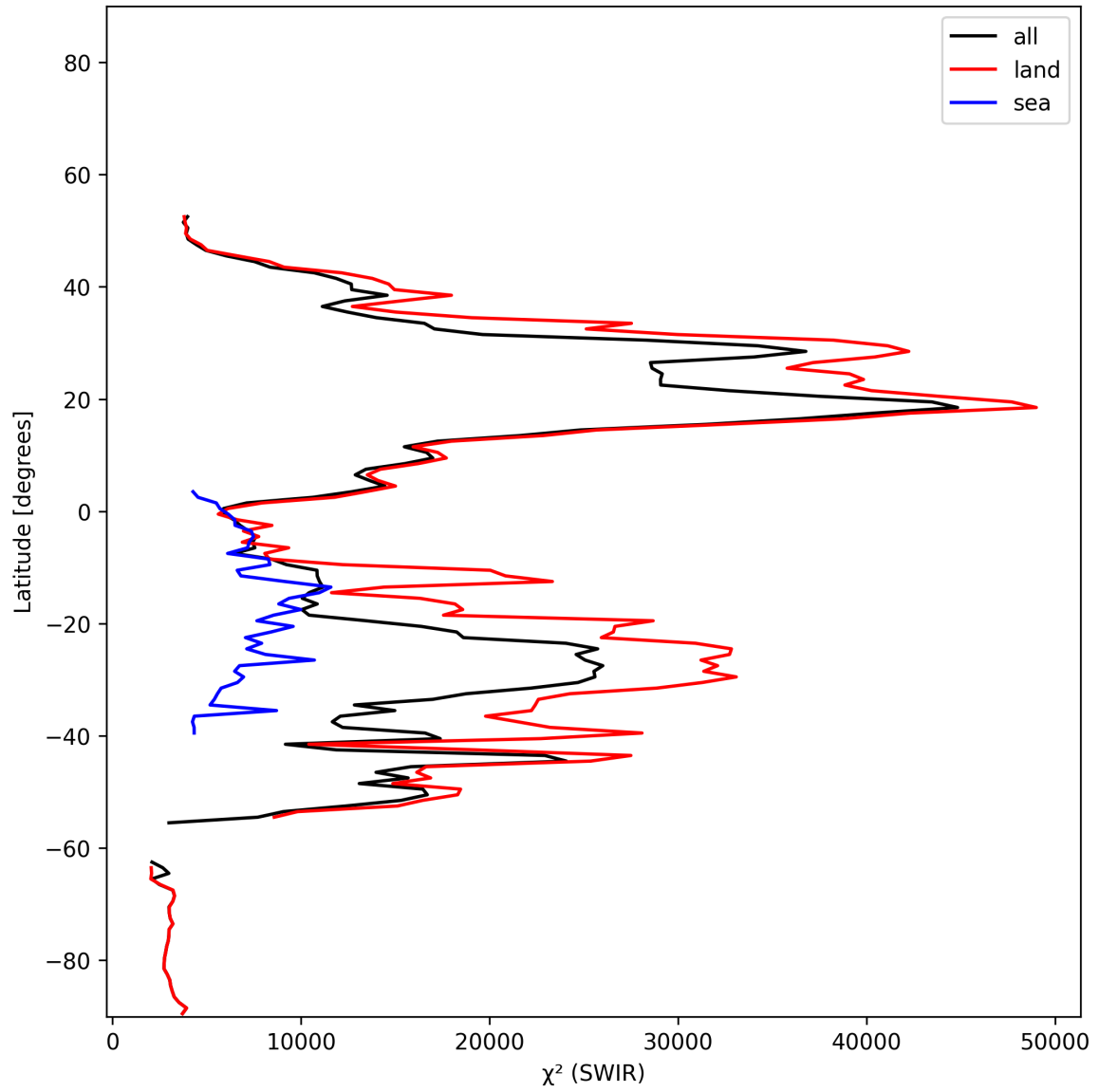
Figure 17: Zonal average of “ \chi^2 (SWIR)” for 2025-01-01 to 2025-01-03.
