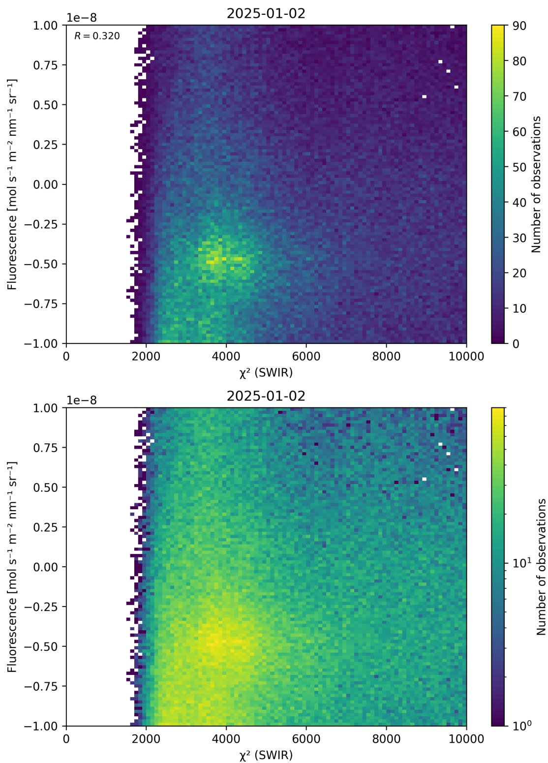
Figure 49: Scatter density plot of “ \chi^2 (SWIR)” against “Fluorescence” for 2025-01-01 to 2025-01-03.
