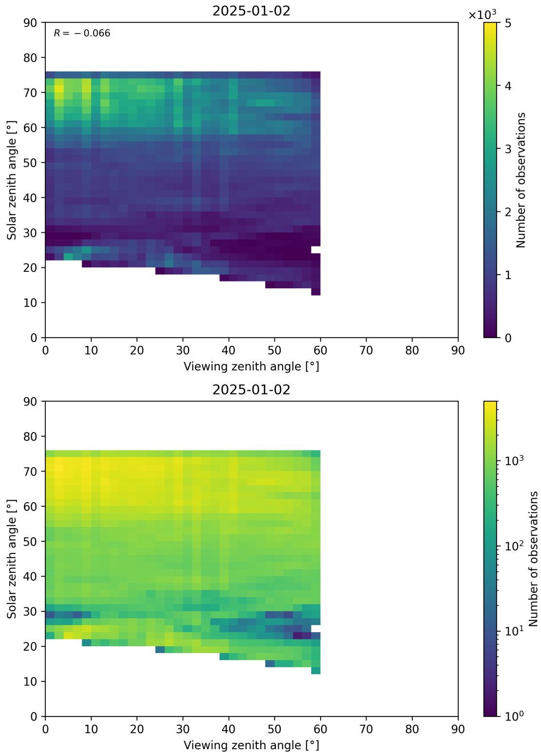
Figure 115: Scatter density plot of “Viewing zenith angle” against “Solar zenith angle” for 2025-01-01 to 2025-01-03.
