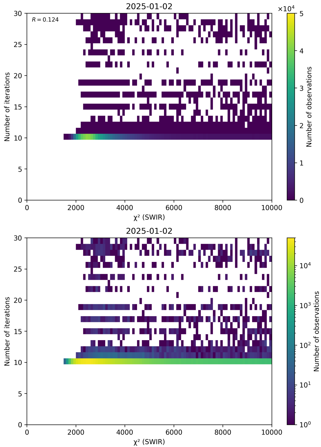
Figure 50: Scatter density plot of “ \chi^2 (SWIR)” against “Number of iterations” for 2025-01-01 to 2025-01-03.
