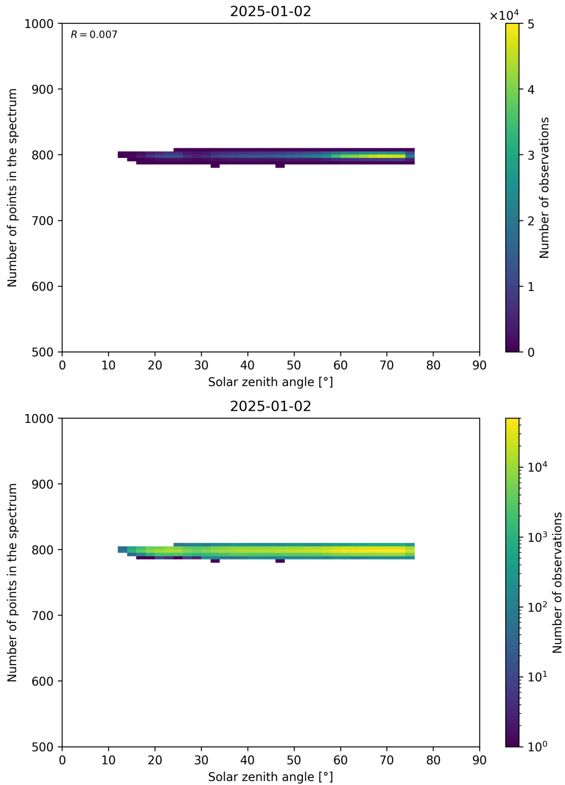
Figure 103: Scatter density plot of “Solar zenith angle” against “Number of points in the spectrum” for 2025-01-01 to 2025-01-03.
