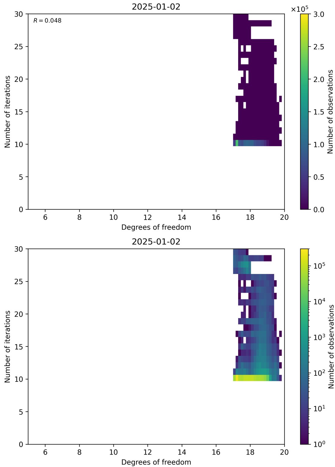
Figure 52: Scatter density plot of “Degrees of freedom” against “Number of iterations” for 2025-01-01 to 2025-01-03.
