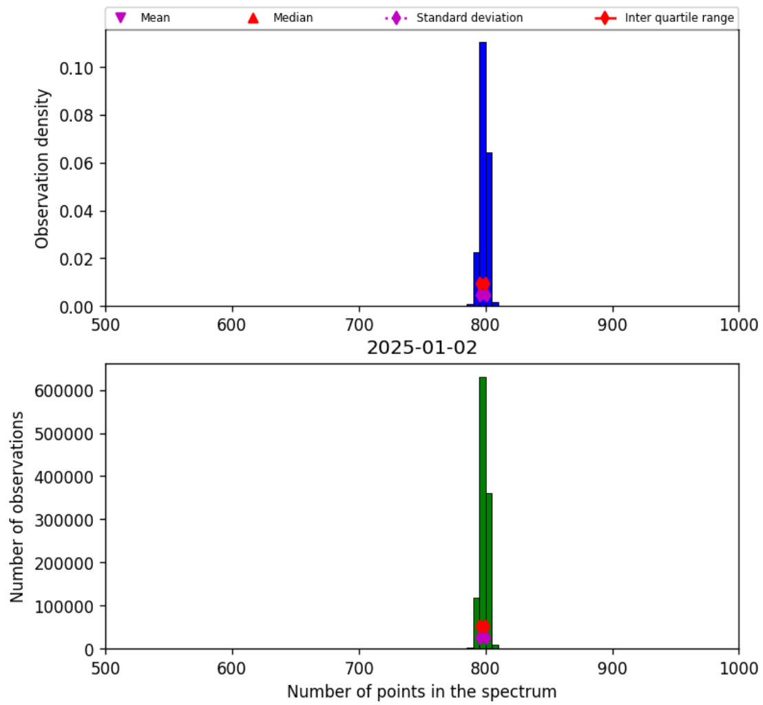
Figure 26: Histogram of “Number of points in the spectrum” for 2025-01-01 to 2025-01-03
