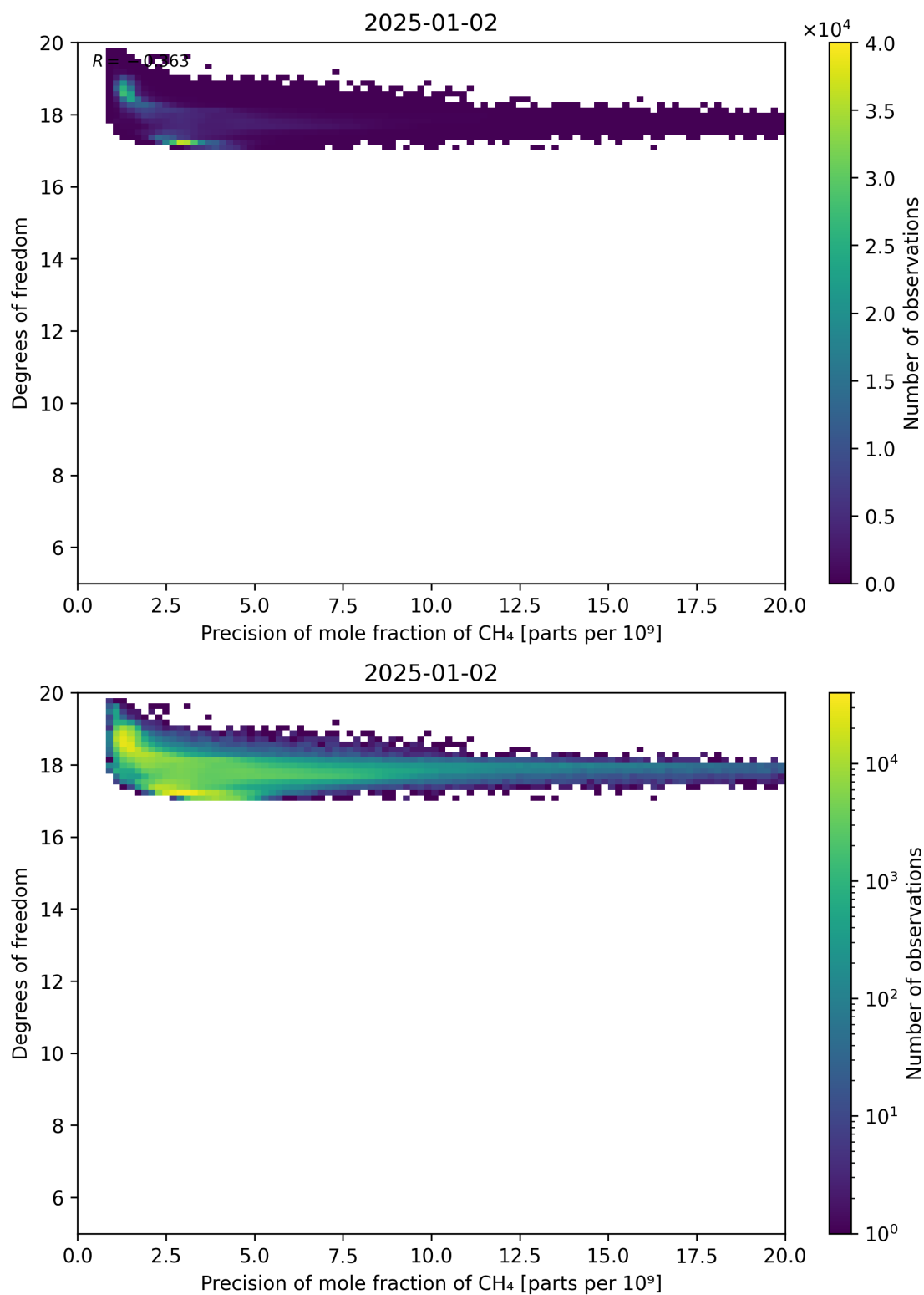
Figure 80: Scatter density plot of “Precision of mole fraction of CH 4 ” against “Degrees of freedom” for 2025-01-01 to 2025-01-03.
