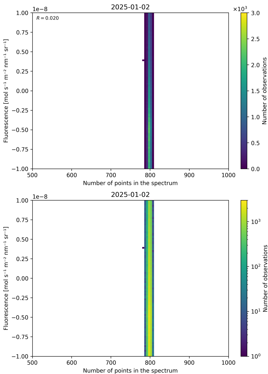
Figure 91: Scatter density plot of “Number of points in the spectrum” against “Fluorescence” for 2025-01-01 to 2025-01-03.
