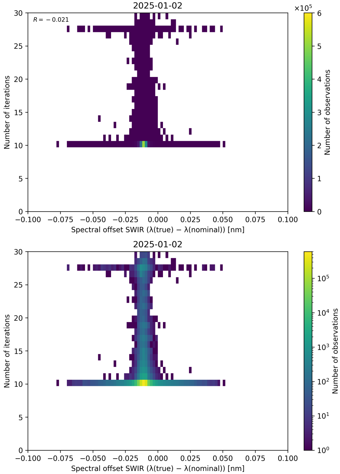
Figure 121: Scatter density plot of “Spectral offset SWIR ( \lambda_{\text{true}} - \lambda_{\text{nominal}} )” against “Number of iterations” for 2025-01-01 to 2025-01-03.
