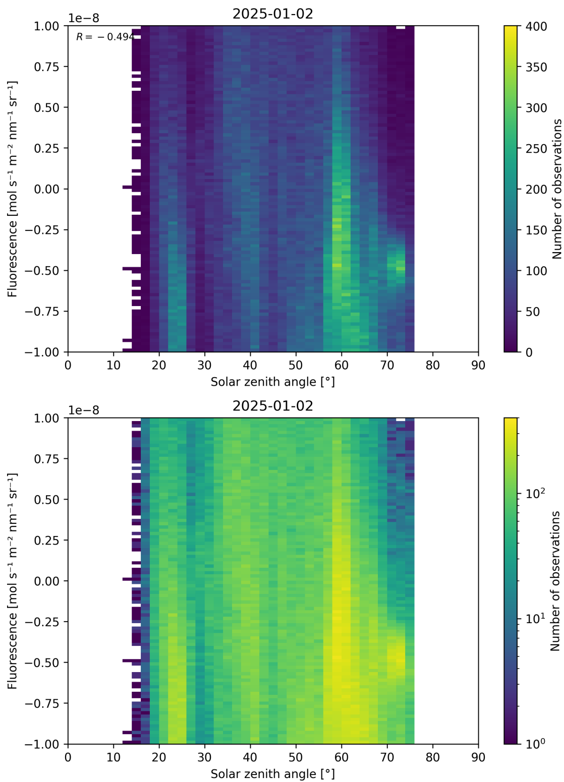
Figure 97: Scatter density plot of “Solar zenith angle” against “Fluorescence” for 2025-01-01 to 2025-01-03.
