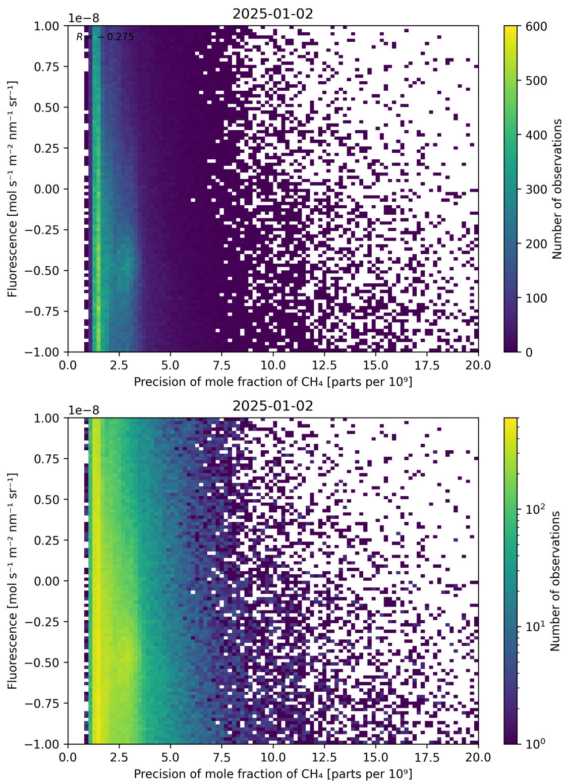
Figure 81: Scatter density plot of “Precision of mole fraction of \text{CH}_4 ” against “Fluorescence” for 2025-01-01 to 2025-01-03.
