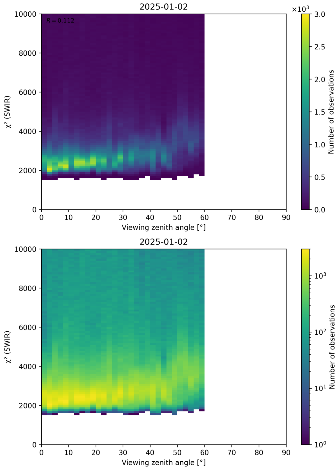
Figure 106: Scatter density plot of “Viewing zenith angle” against “ \chi^2 (SWIR)” for 2025-01-01 to 2025-01-03.
