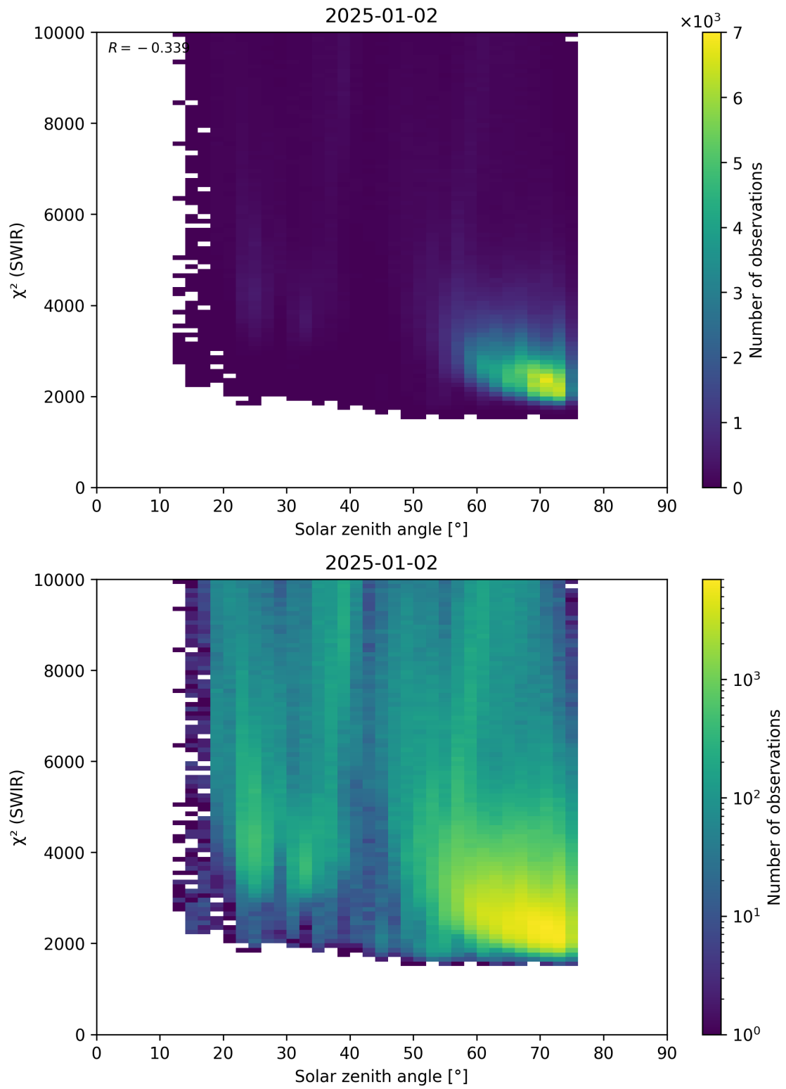
Figure 95: Scatter density plot of “Solar zenith angle” against “ \chi^2 (SWIR)” for 2025-01-01 to 2025-01-03.
