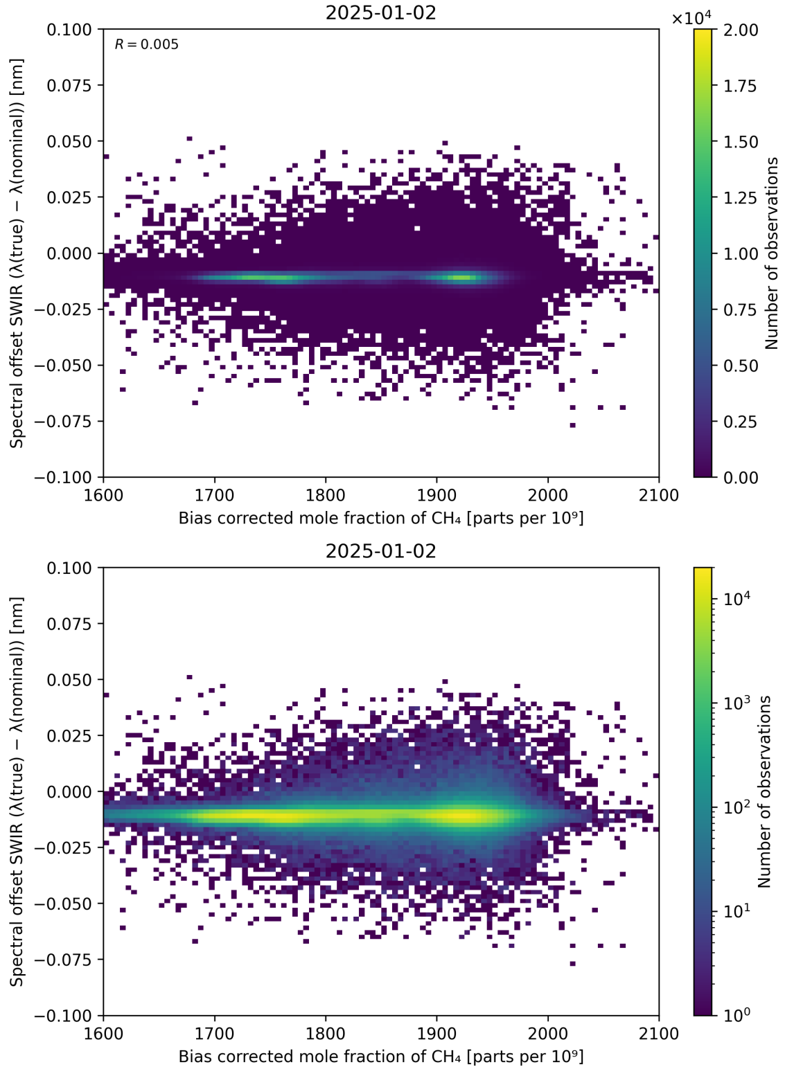
Figure 69: Scatter density plot of “Bias corrected mole fraction of \text{CH}_4 ” against “Spectral offset SWIR ( \lambda_{\text{true}} - \lambda_{\text{nominal}} )” for 2025-01-01 to 2025-01-03.
