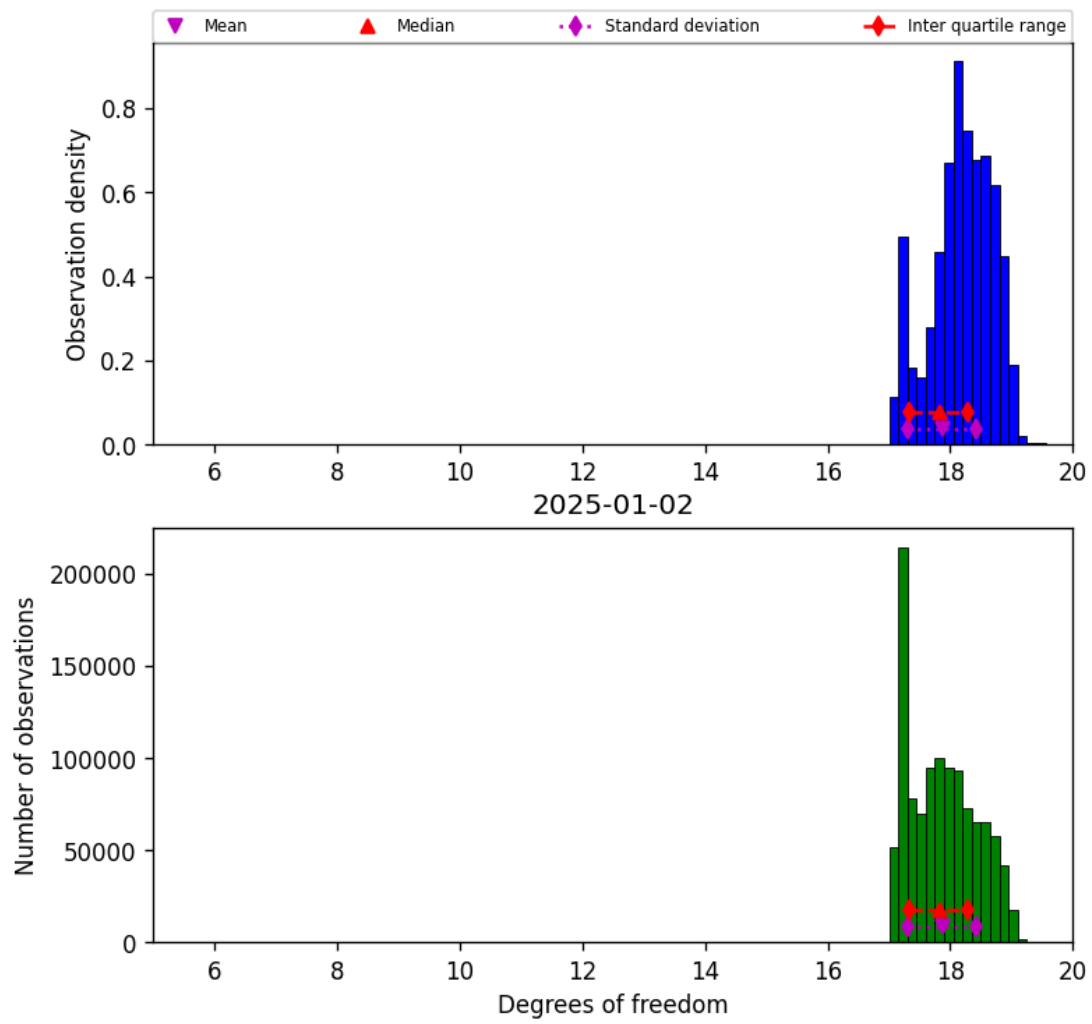
Figure 30: Histogram of “Degrees of freedom” for 2025-01-01 to 2025-01-03
