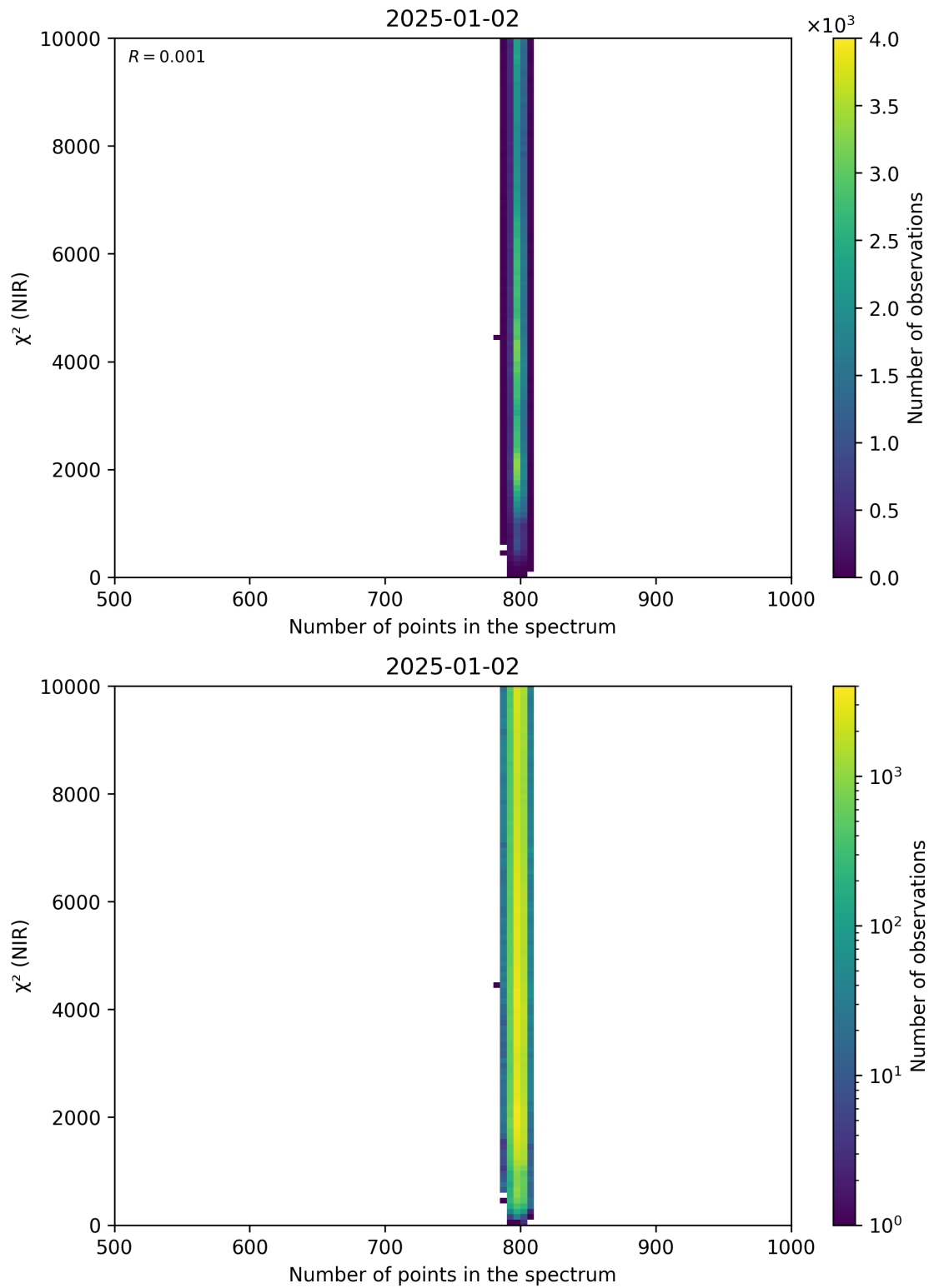
Figure 88: Scatter density plot of “Number of points in the spectrum” against “ \chi^2 (NIR)” for 2025-01-01 to 2025-01-03.
