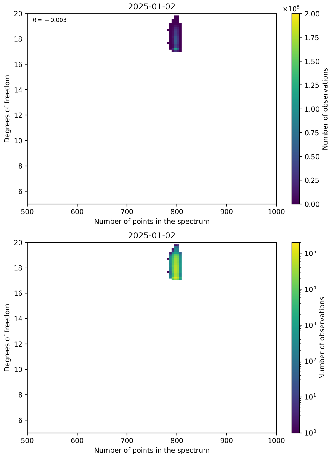
Figure 90: Scatter density plot of “Number of points in the spectrum” against “Degrees of freedom” for 2025-01-01 to 2025-01-03.
