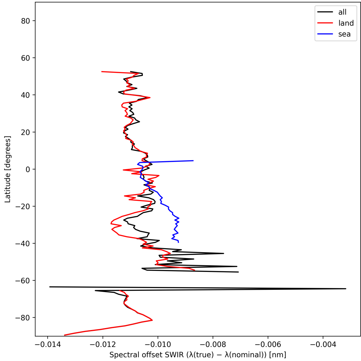
Figure 16: Zonal average of “Spectral offset SWIR ( \lambda_{\text{true}} - \lambda_{\text{nominal}} )” for 2025-01-02 to 2025-01-04.
