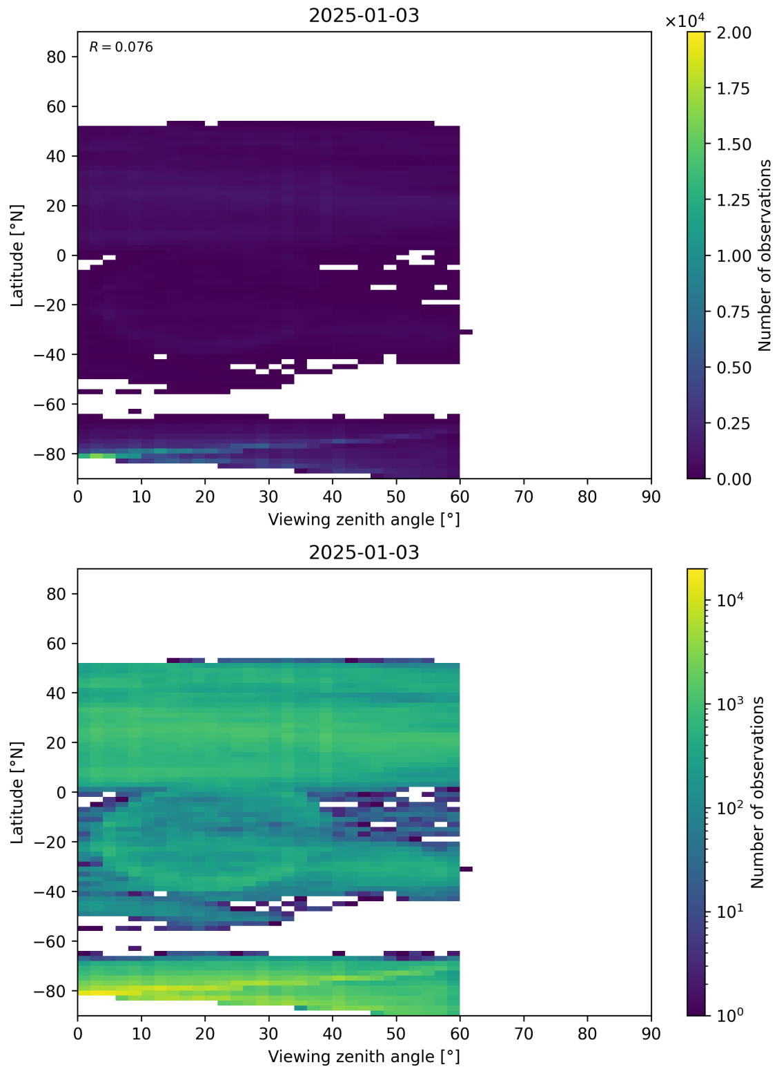
Figure 109: Scatter density plot of “Viewing zenith angle” against “Latitude” for 2025-01-02 to 2025-01-04.
