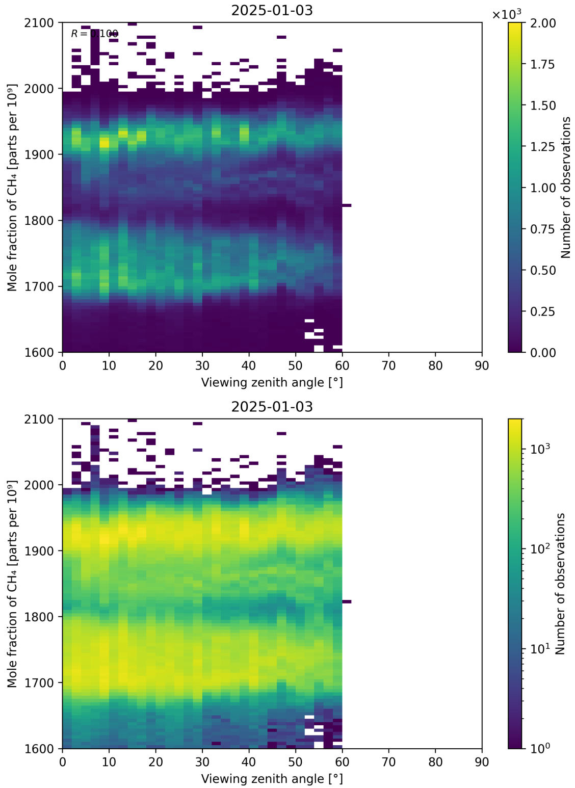
Figure 110: Scatter density plot of “Viewing zenith angle” against “Mole fraction of CH 4 ” for 2025-01-02 to 2025-01-04.
