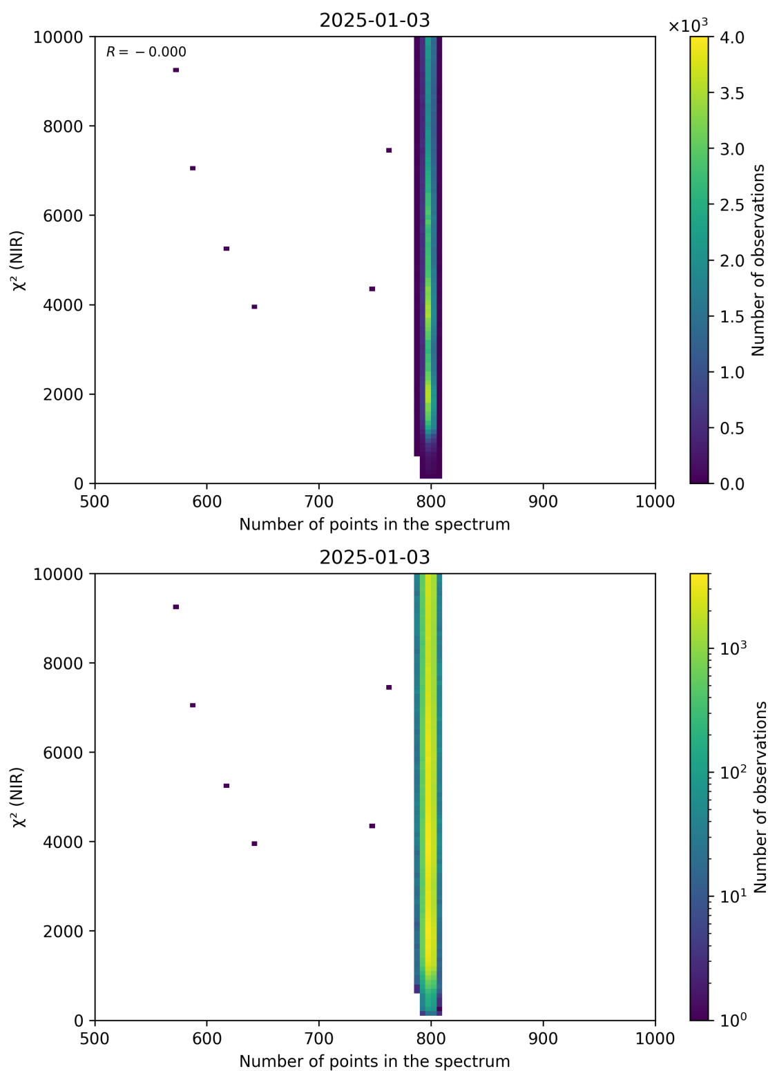
Figure 88: Scatter density plot of “Number of points in the spectrum” against “ \chi^2 (NIR)” for 2025-01-02 to 2025-01-04.
