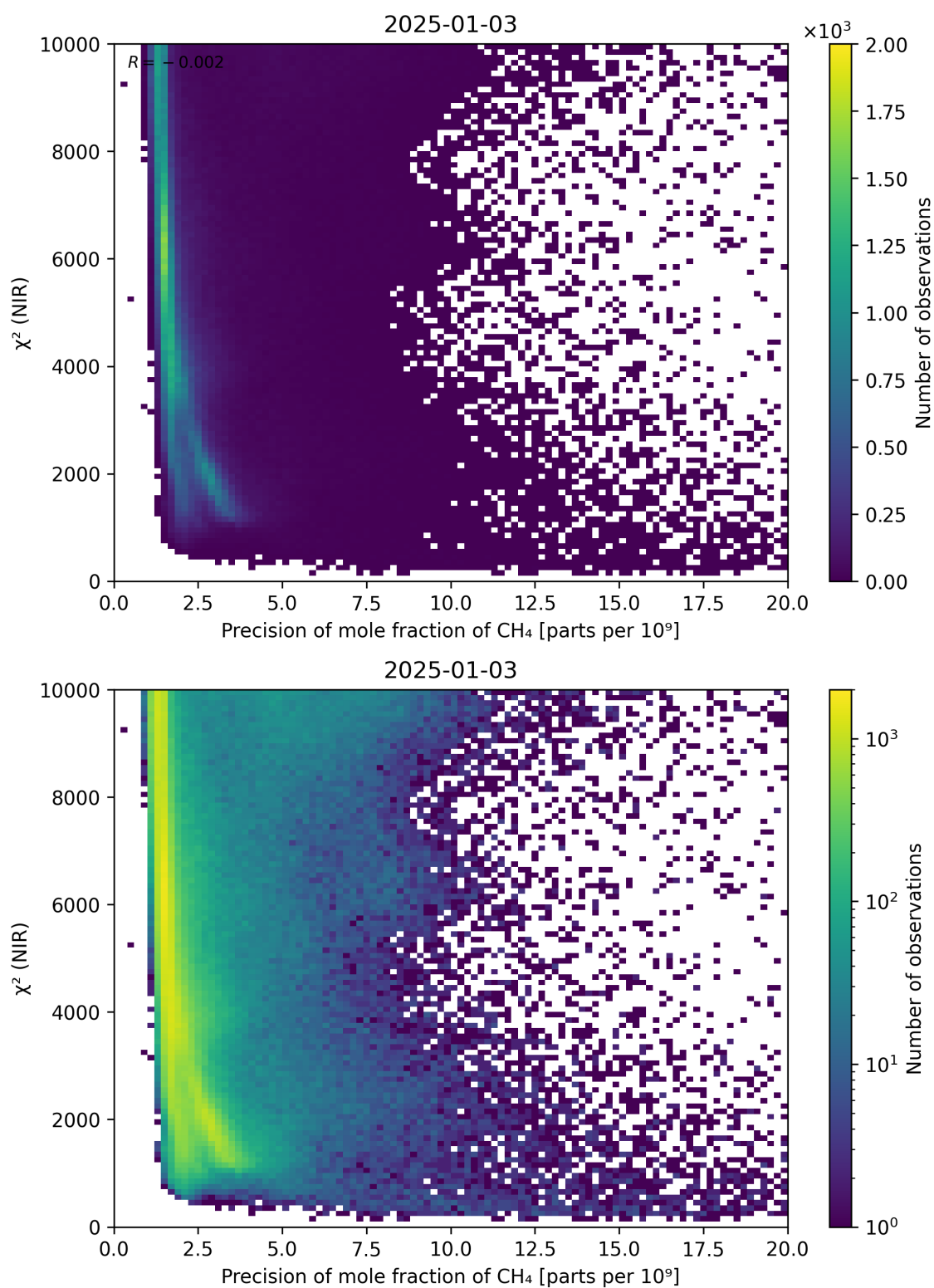
Figure 78: Scatter density plot of “Precision of mole fraction of CH 4 ” against “ \chi^2 (NIR)” for 2025-01-02 to 2025-01-04.
