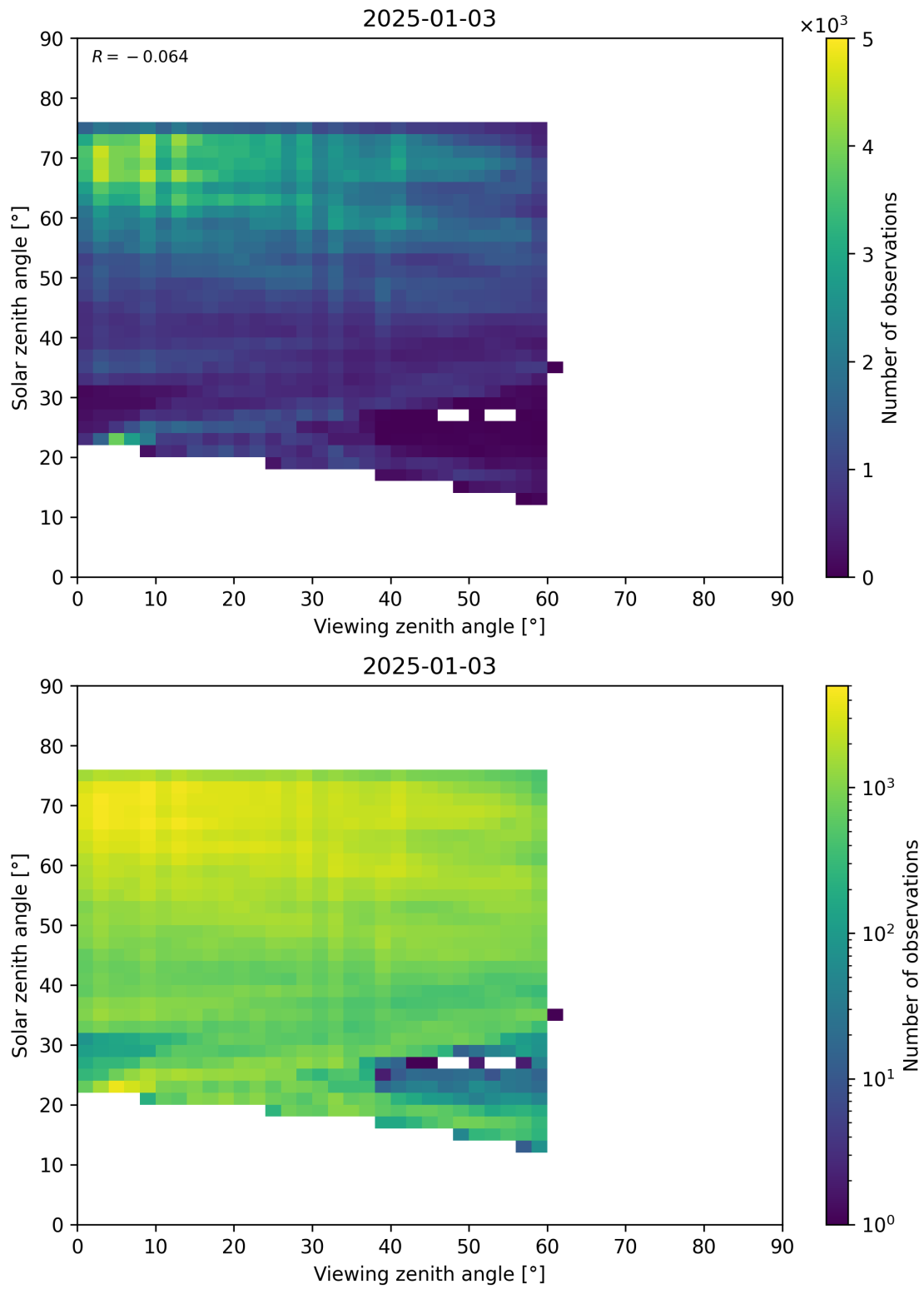
Figure 115: Scatter density plot of “Viewing zenith angle” against “Solar zenith angle” for 2025-01-02 to 2025-01-04.
