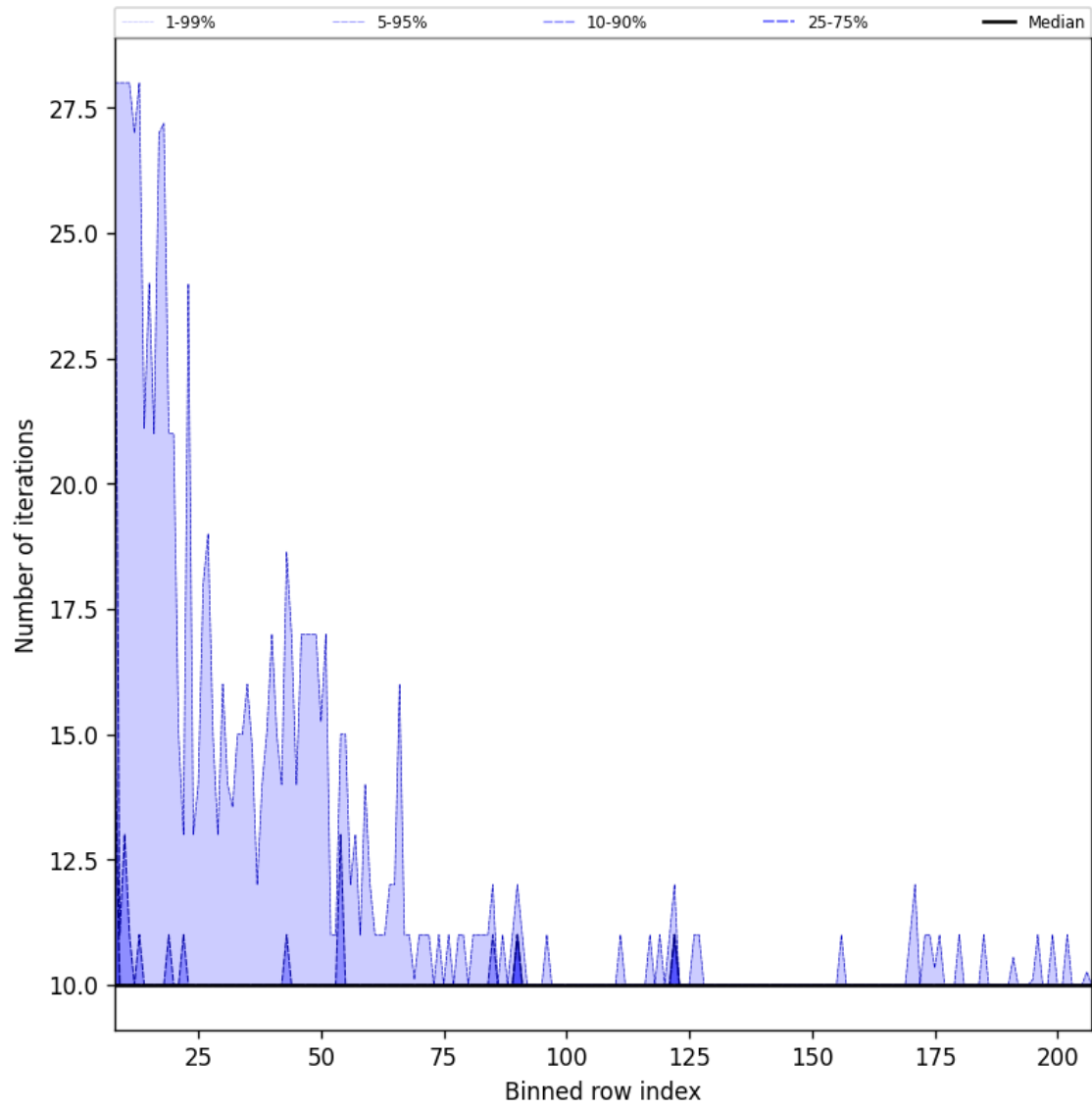
Figure 42: Along track statistics of “Number of iterations” for 2025-01-02 to 2025-01-04
