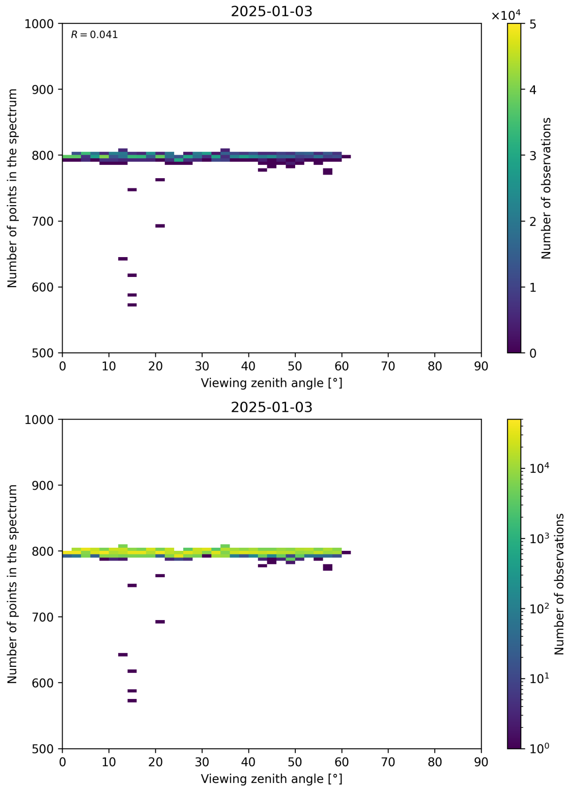
Figure 114: Scatter density plot of “Viewing zenith angle” against “Number of points in the spectrum” for 2025-01-02 to 2025-01-04.
