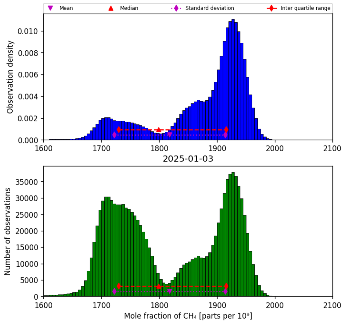
Figure 23: Histogram of “Mole fraction of CH 4 ” for 2025-01-02 to 2025-01-04
