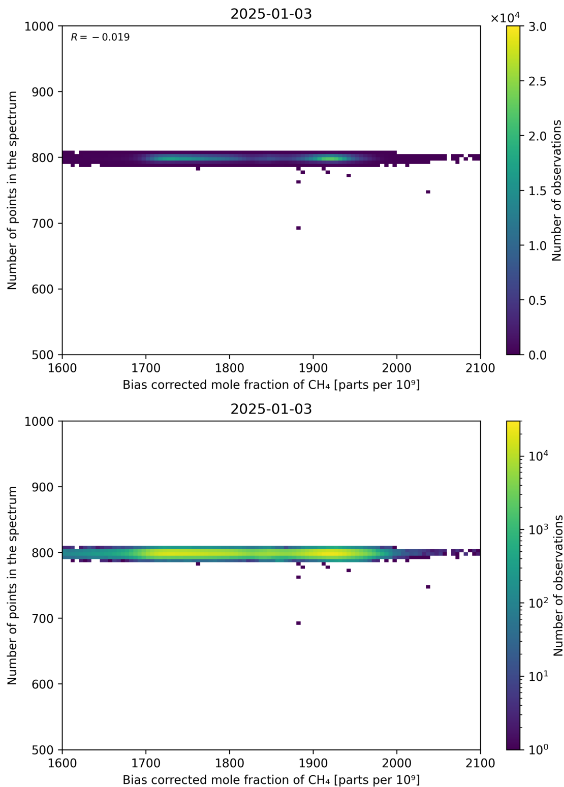
Figure 68: Scatter density plot of “Bias corrected mole fraction of CH 4 ” against “Number of points in the spectrum” for 2025-01-02 to 2025-01-04.
