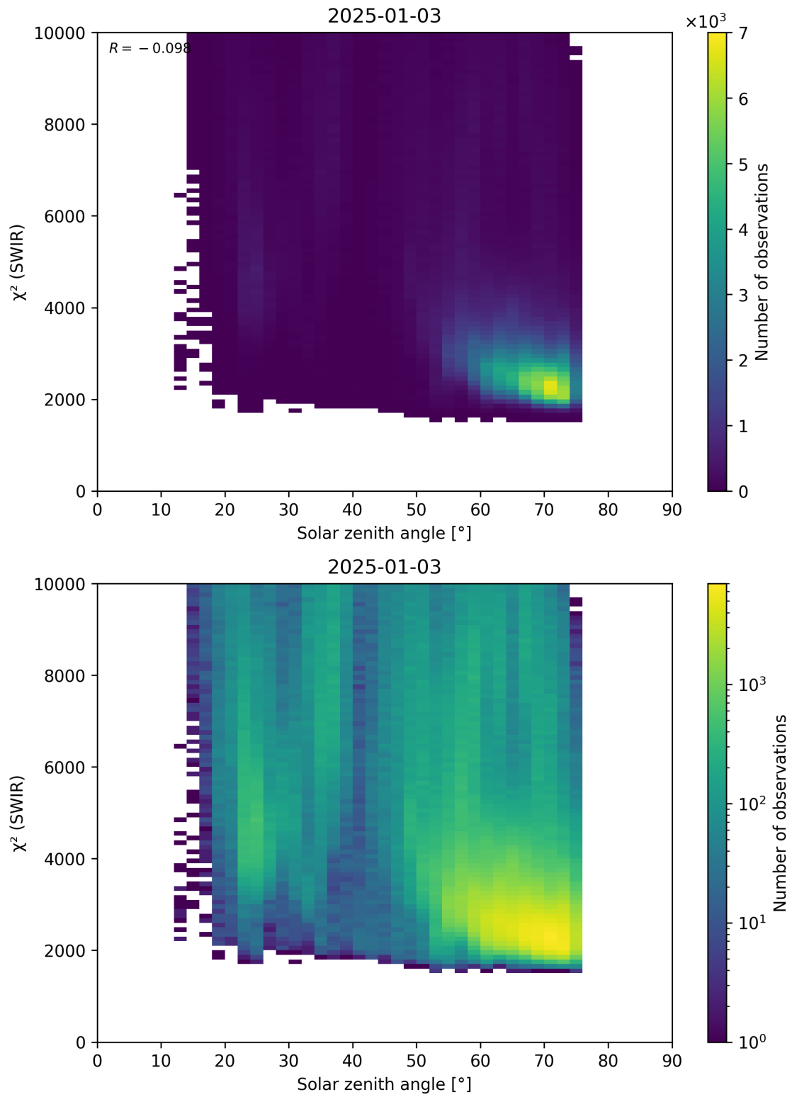
Figure 95: Scatter density plot of “Solar zenith angle” against “ \chi^2 (SWIR)” for 2025-01-02 to 2025-01-04.
