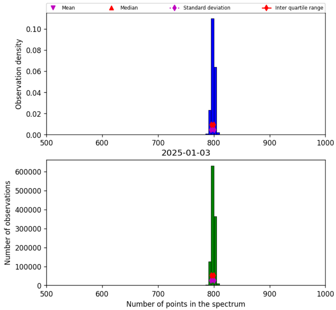
Figure 26: Histogram of “Number of points in the spectrum” for 2025-01-02 to 2025-01-04
