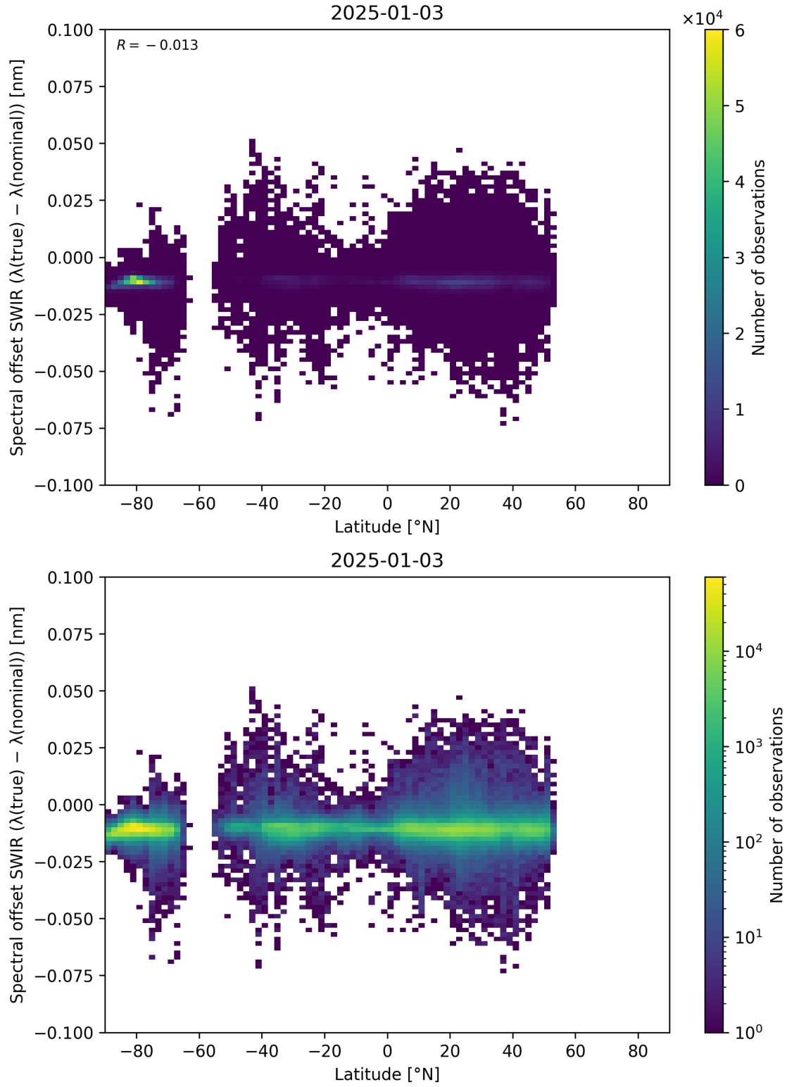
Figure 62: Scatter density plot of “Latitude” against “Spectral offset SWIR ( \lambda_{\text{true}} - \lambda_{\text{nominal}} )” for 2025-01-02 to 2025-01-04.
