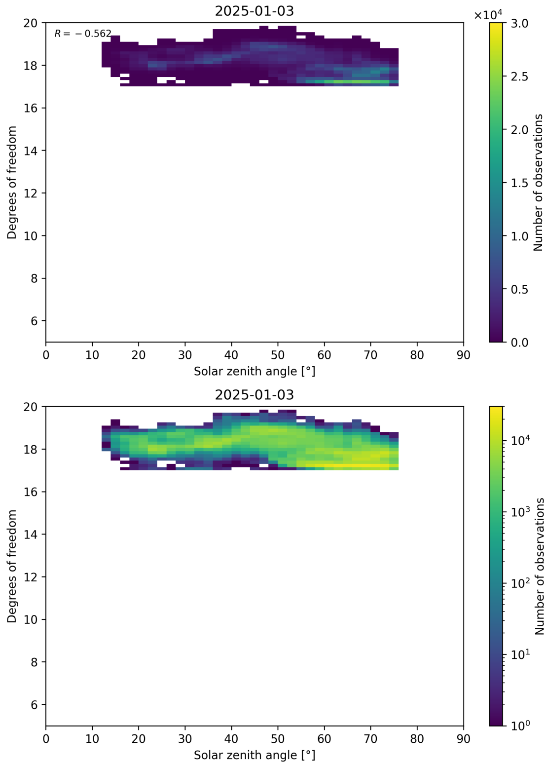
Figure 96: Scatter density plot of “Solar zenith angle” against “Degrees of freedom” for 2025-01-02 to 2025-01-04.
