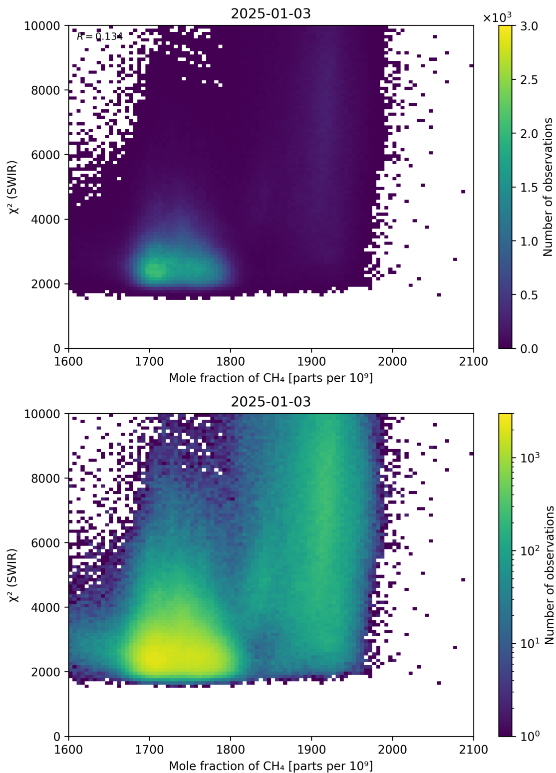
Figure 71: Scatter density plot of “Mole fraction of \text{CH}_4 ” against “ \chi^2 (SWIR)” for 2025-01-02 to 2025-01-04.
