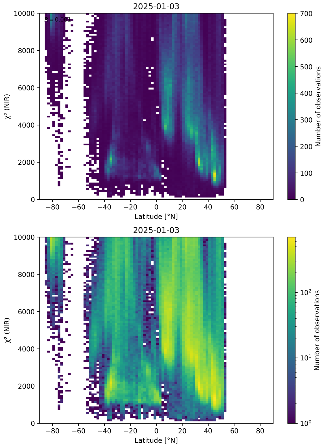
Figure 53: Scatter density plot of “Latitude” against “ \chi^2 (NIR)” for 2025-01-02 to 2025-01-04.
