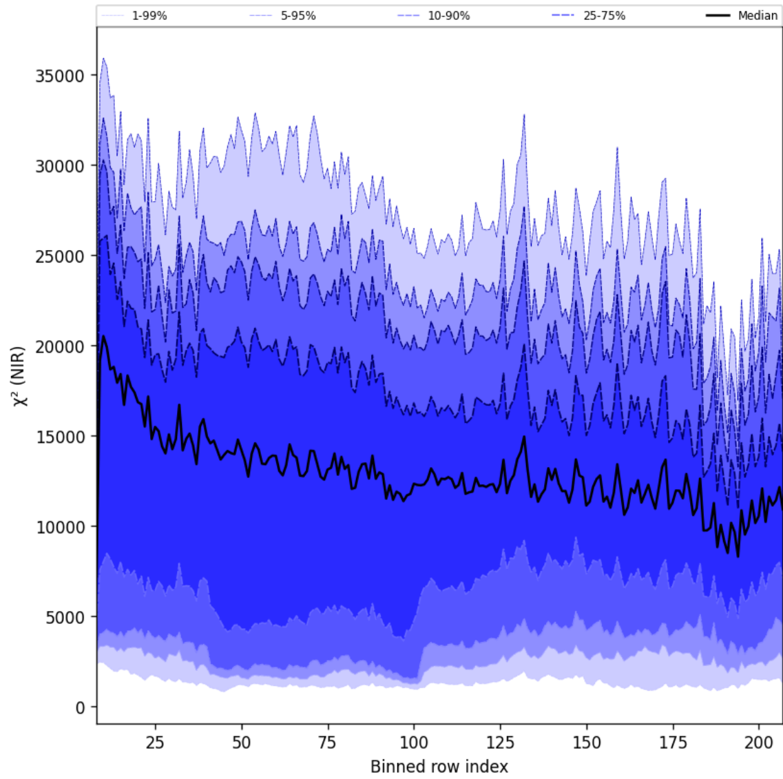
Figure 40: Along track statistics of “ \chi^2 (NIR)” for 2025-01-02 to 2025-01-04
