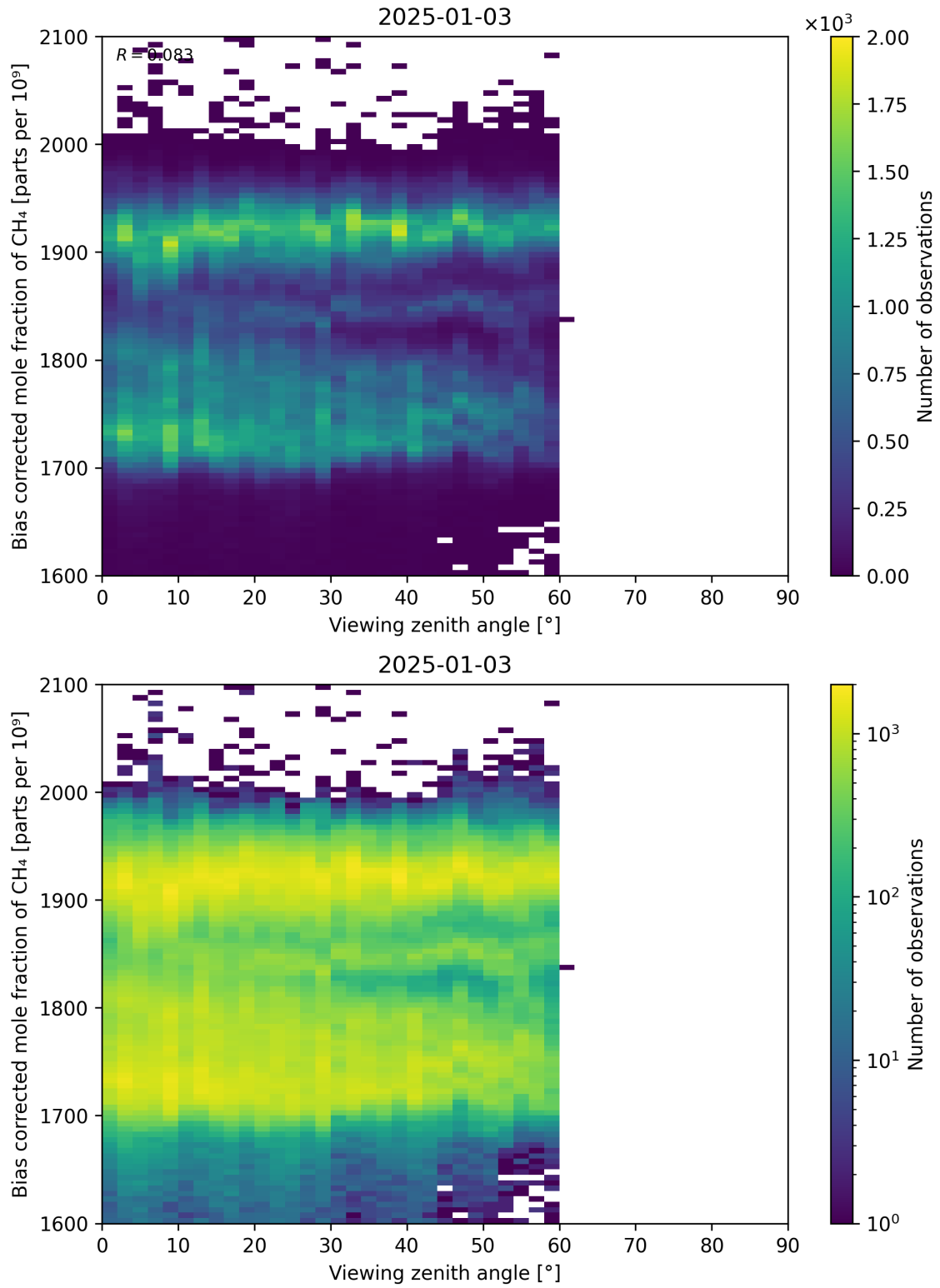
Figure 111: Scatter density plot of “Viewing zenith angle” against “Bias corrected mole fraction of CH 4 ” for 2025-01-02 to 2025-01-04.
