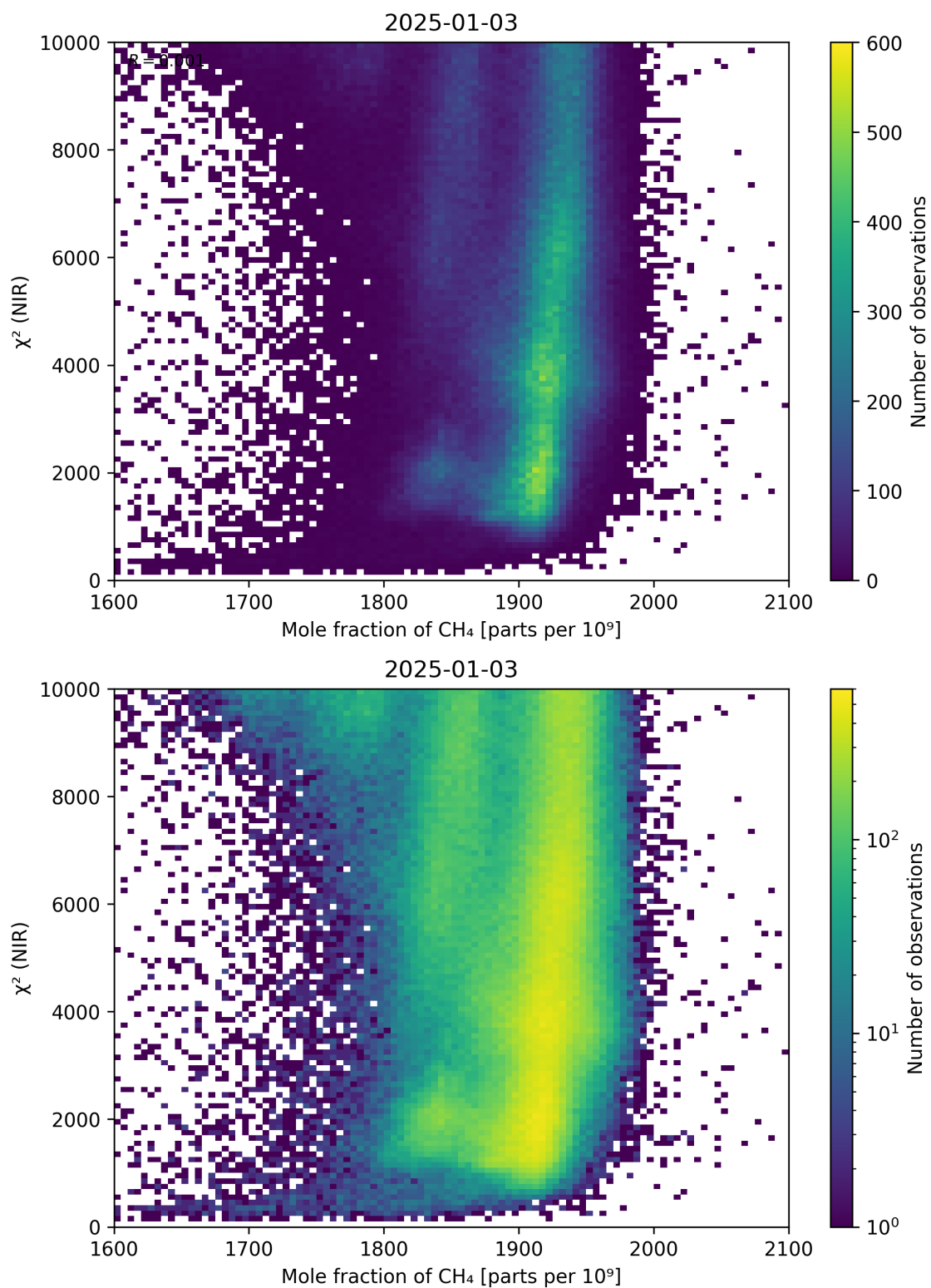
Figure 70: Scatter density plot of “Mole fraction of CH 4 ” against “ \chi^2 (NIR)” for 2025-01-02 to 2025-01-04.
