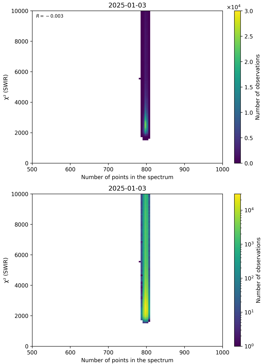
Figure 89: Scatter density plot of “Number of points in the spectrum” against “ \chi^2 (SWIR)” for 2025-01-02 to 2025-01-04.
