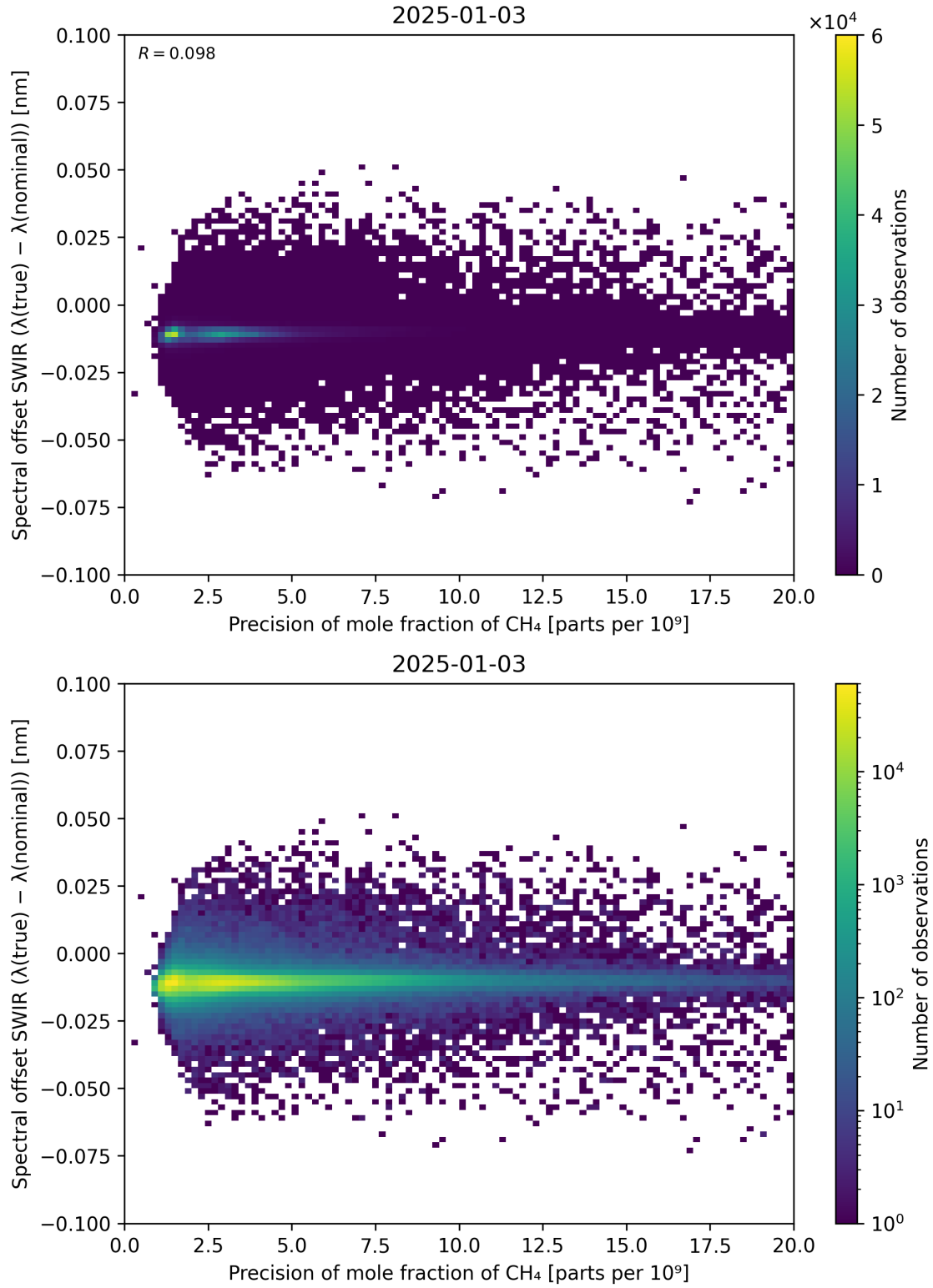
Figure 85: Scatter density plot of “Precision of mole fraction of CH 4 ” against “Spectral offset SWIR ( \lambda_{\text{true}} - \lambda_{\text{nominal}} )” for 2025-01-02 to 2025-01-04.
