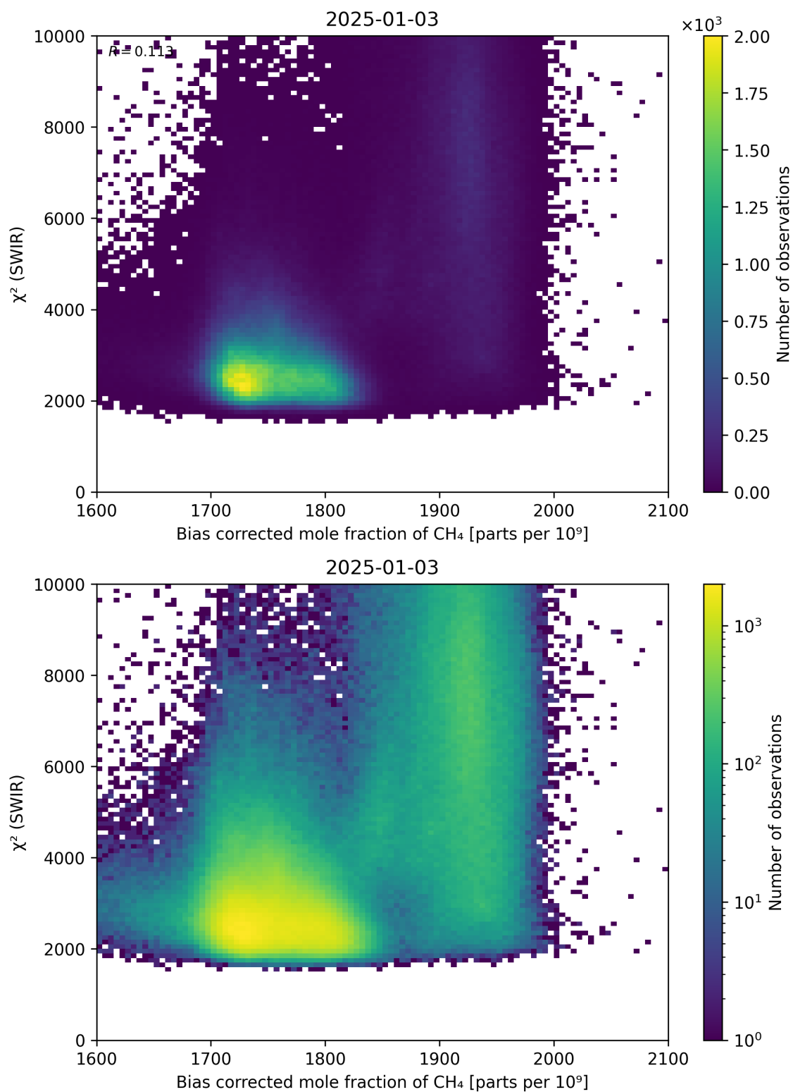
Figure 64: Scatter density plot of “Bias corrected mole fraction of CH 4 ” against “ \chi^2 (SWIR)” for 2025-01-02 to 2025-01-04.
