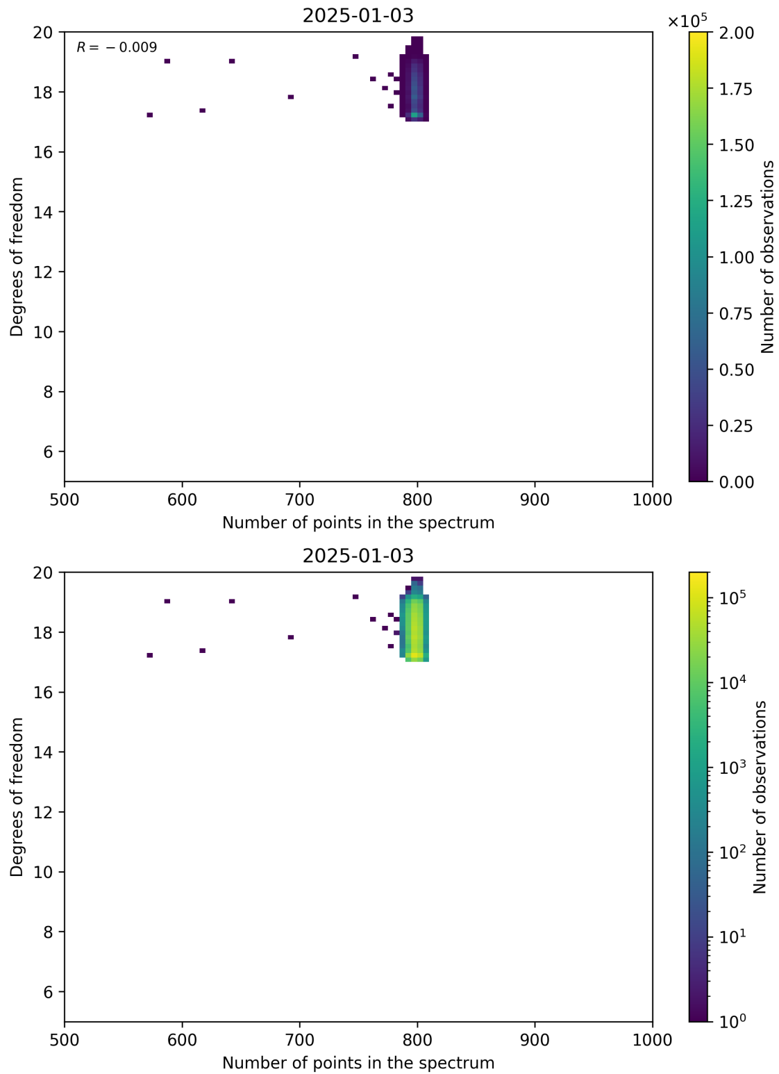
Figure 90: Scatter density plot of “Number of points in the spectrum” against “Degrees of freedom” for 2025-01-02 to 2025-01-04.
