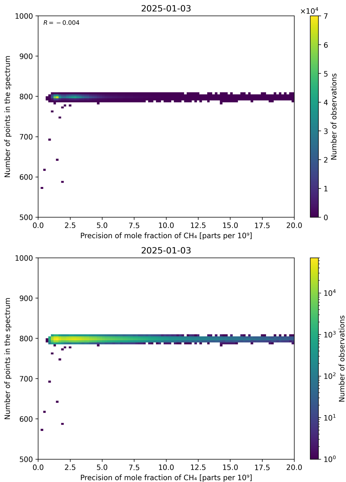
Figure 84: Scatter density plot of “Precision of mole fraction of CH 4 ” against “Number of points in the spectrum” for 2025-01-02 to 2025-01-04.
