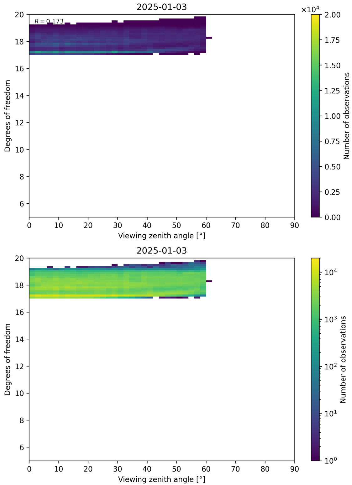
Figure 107: Scatter density plot of “Viewing zenith angle” against “Degrees of freedom” for 2025-01-02 to 2025-01-04.
