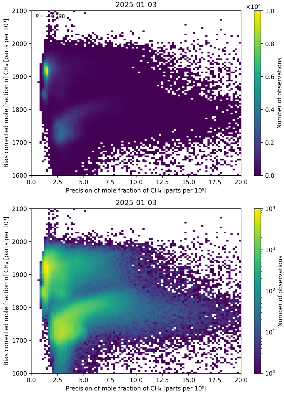
Figure 82: Scatter density plot of “Precision of mole fraction of CH 4 ” against “Bias corrected mole fraction of CH 4 ” for 2025-01-02 to 2025-01-04.
