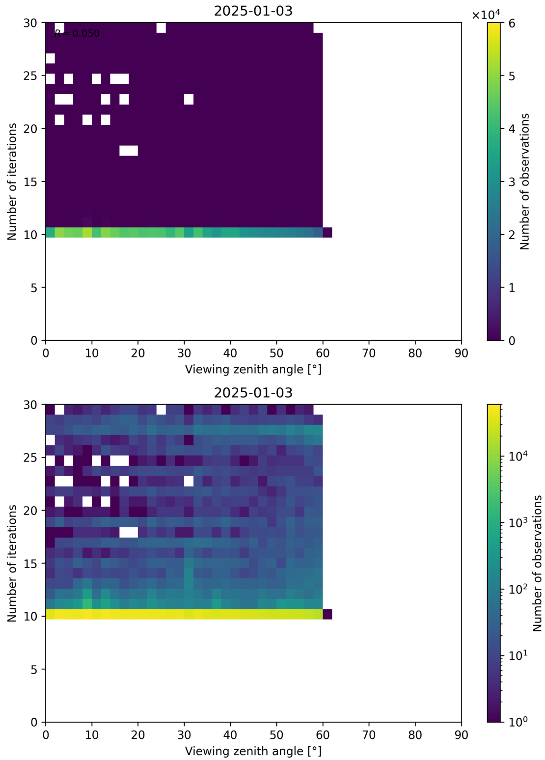
Figure 113: Scatter density plot of “Viewing zenith angle” against “Number of iterations” for 2025-01-02 to 2025-01-04.
