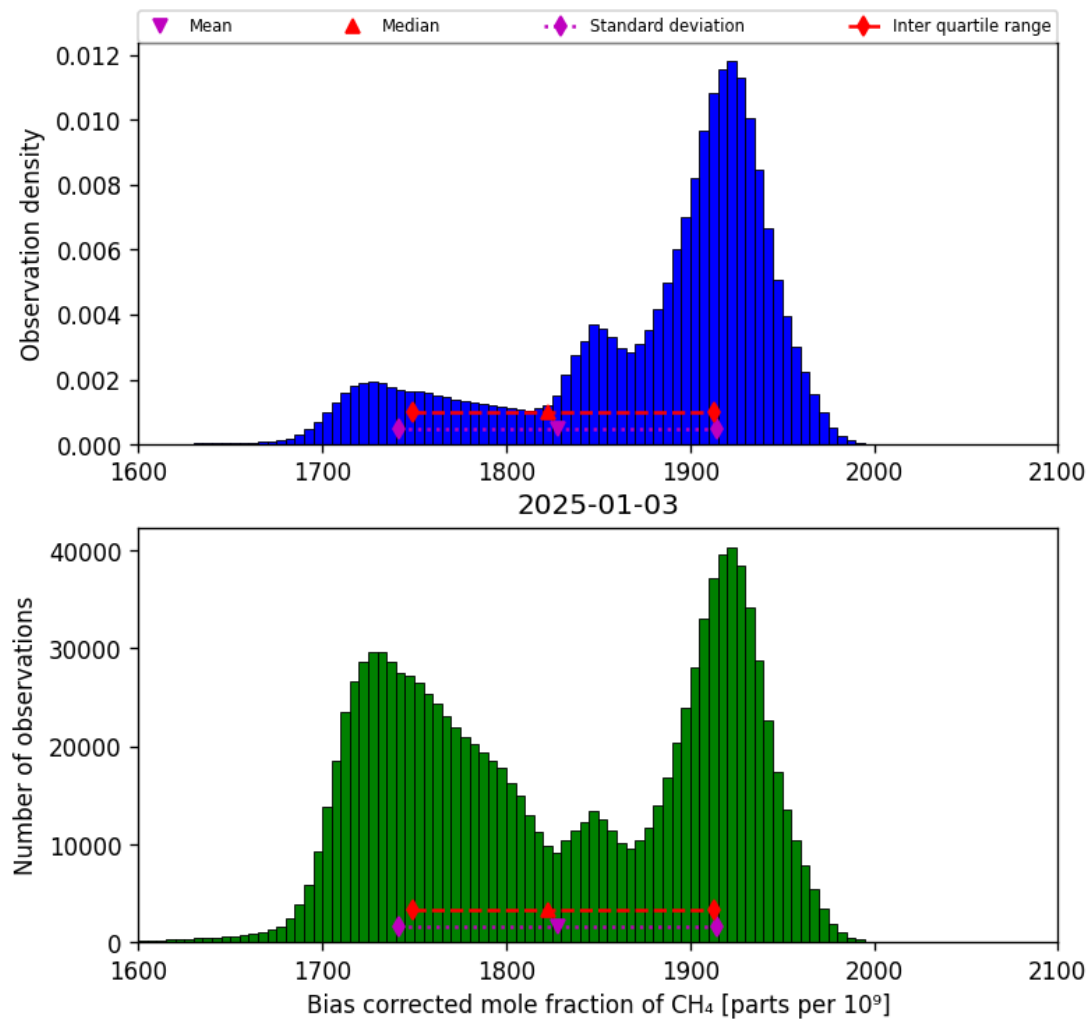
Figure 25: Histogram of “Bias corrected mole fraction of CH 4 ” for 2025-01-02 to 2025-01-04
