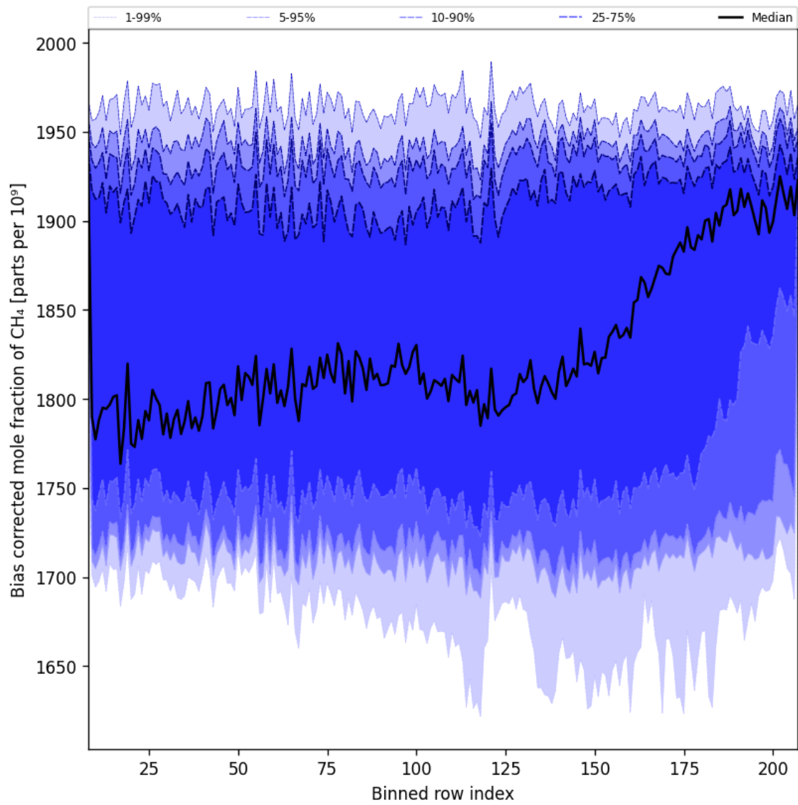
Figure 36: Along track statistics of “Bias corrected mole fraction of CH 4 ” for 2025-01-02 to 2025-01-04
