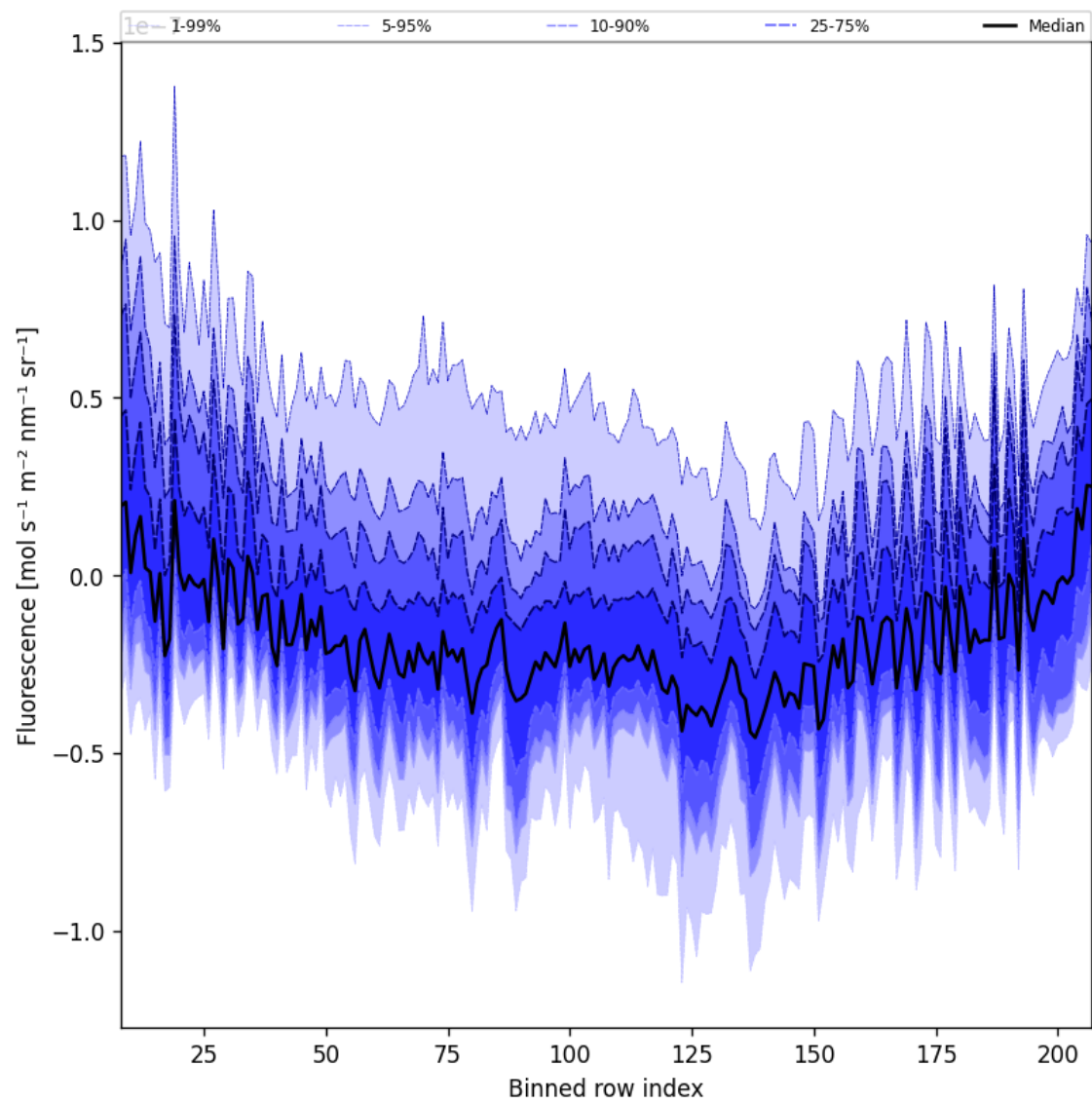
Figure 43: Along track statistics of “Fluorescence” for 2025-01-02 to 2025-01-04
