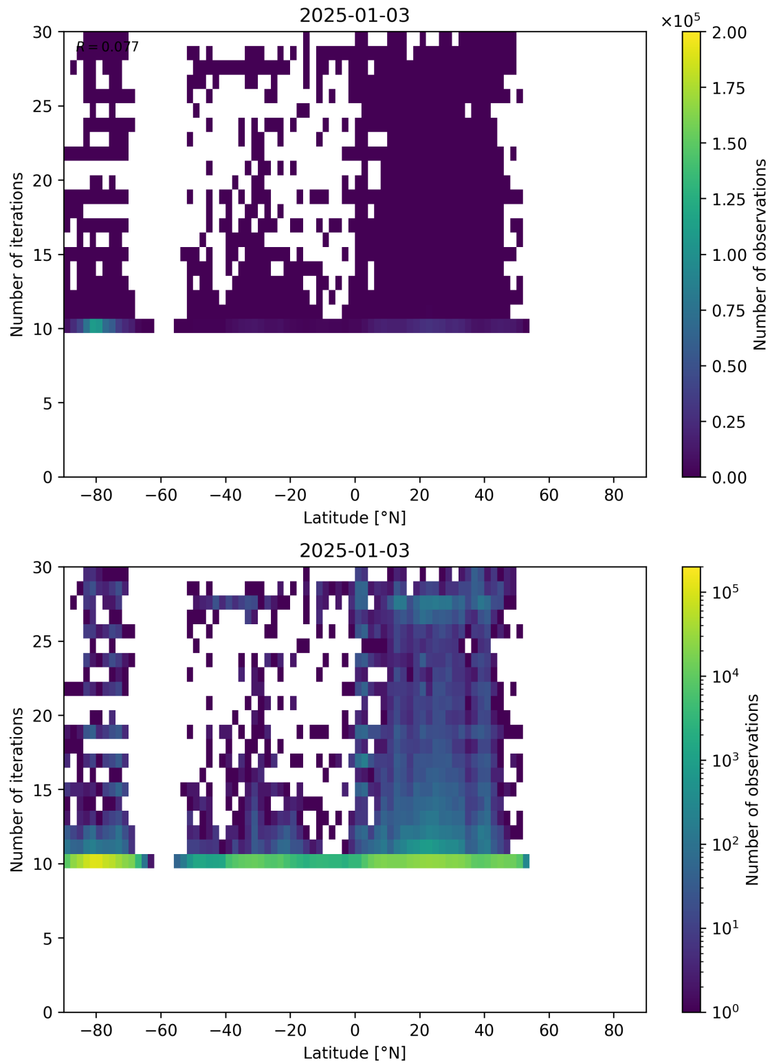
Figure 60: Scatter density plot of “Latitude” against “Number of iterations” for 2025-01-02 to 2025-01-04.
