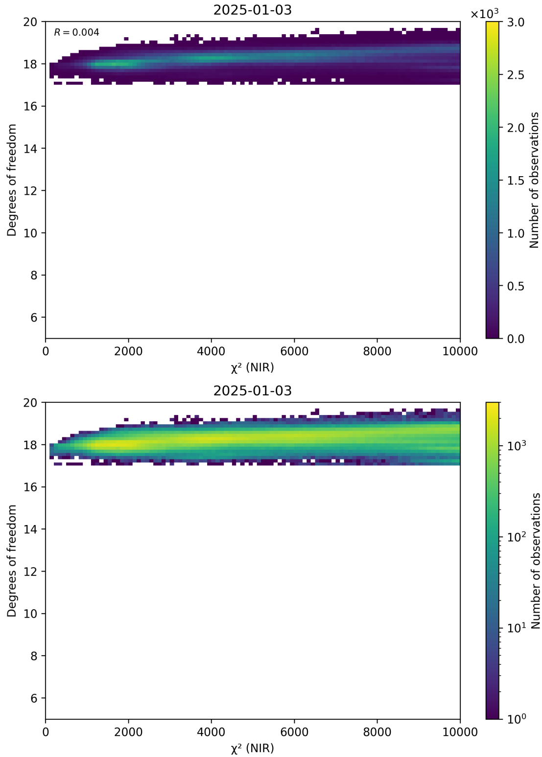
Figure 44: Scatter density plot of “ \chi^2 (NIR)” against “Degrees of freedom” for 2025-01-02 to 2025-01-04.
