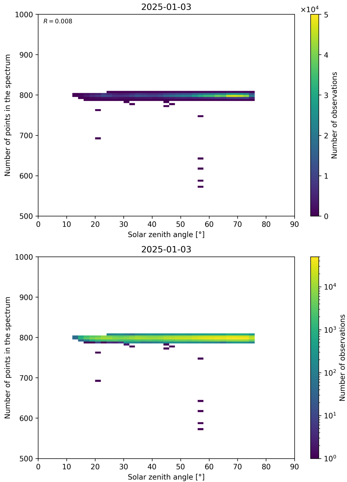
Figure 103: Scatter density plot of “Solar zenith angle” against “Number of points in the spectrum” for 2025-01-02 to 2025-01-04.
