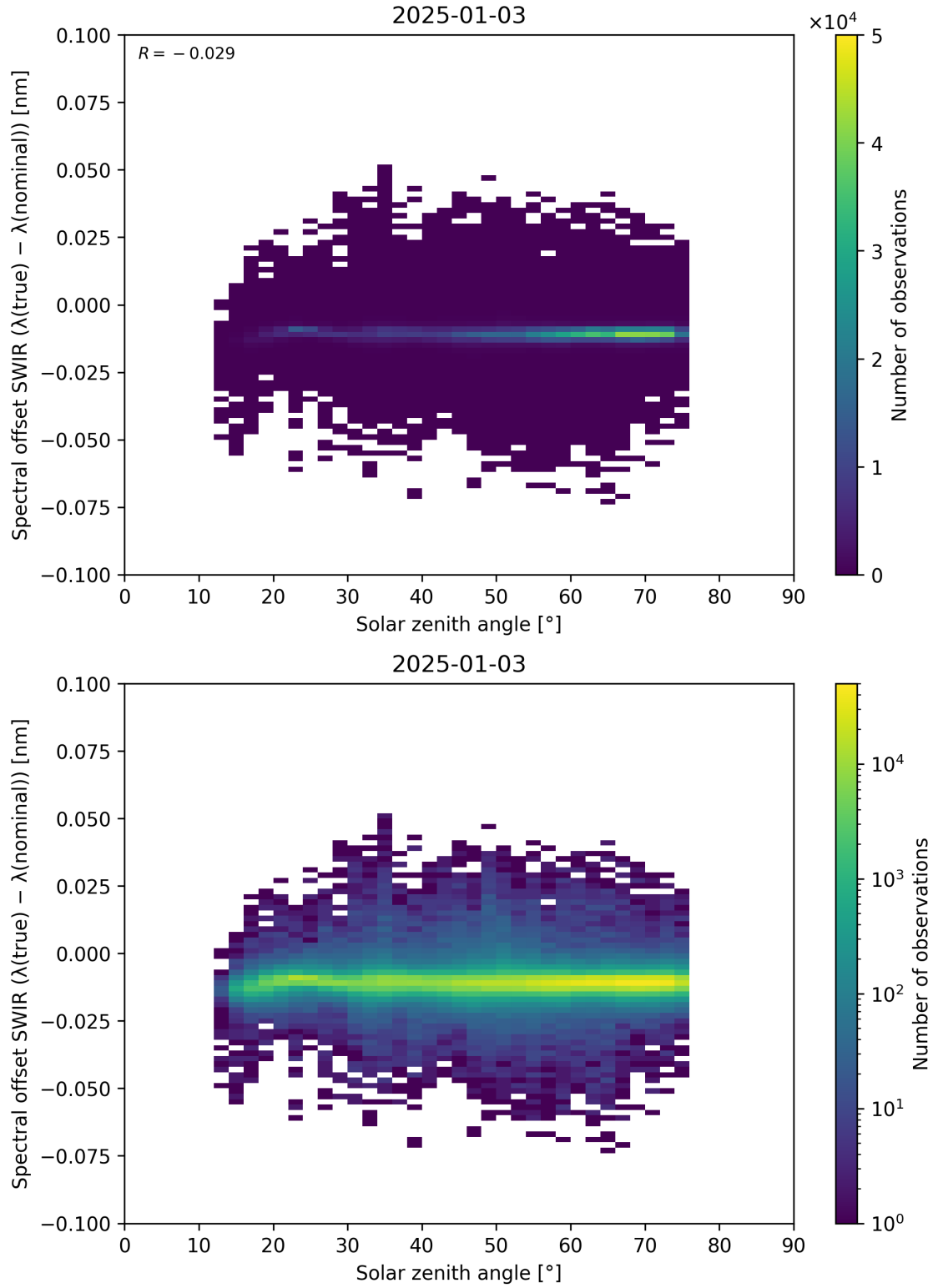
Figure 104: Scatter density plot of “Solar zenith angle” against “Spectral offset SWIR ( \lambda_{\text{true}} - \lambda_{\text{nominal}} )” for 2025-01-02 to 2025-01-04.
