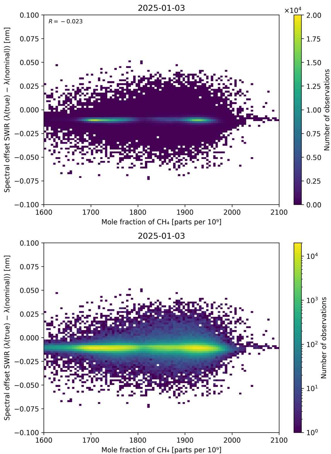
Figure 86: Scatter density plot of “Mole fraction of \text{CH}_4 ” against “Spectral offset SWIR ( \lambda_{\text{true}} - \lambda_{\text{nominal}} )” for 2025-01-02 to 2025-01-04.
