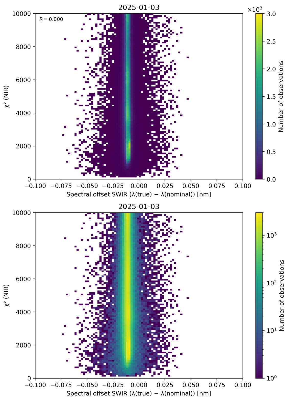
Figure 117: Scatter density plot of “Spectral offset SWIR ( \lambda_{\text{true}} - \lambda_{\text{nominal}} )” against “ \chi^2 (NIR)” for 2025-01-02 to 2025-01-04.
