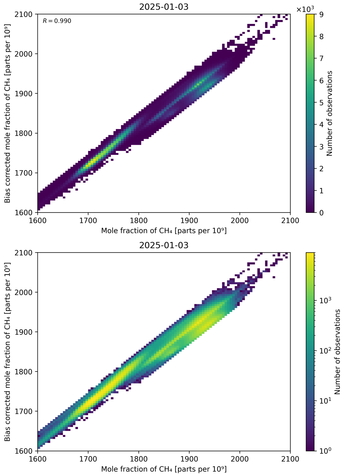
Figure 74: Scatter density plot of “Mole fraction of CH 4 ” against “Bias corrected mole fraction of CH 4 ” for 2025-01-02 to 2025-01-04.
