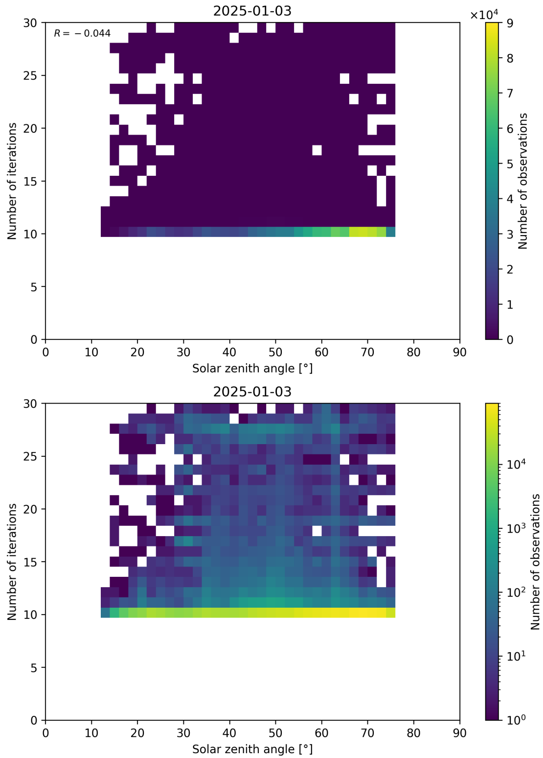
Figure 102: Scatter density plot of “Solar zenith angle” against “Number of iterations” for 2025-01-02 to 2025-01-04.
