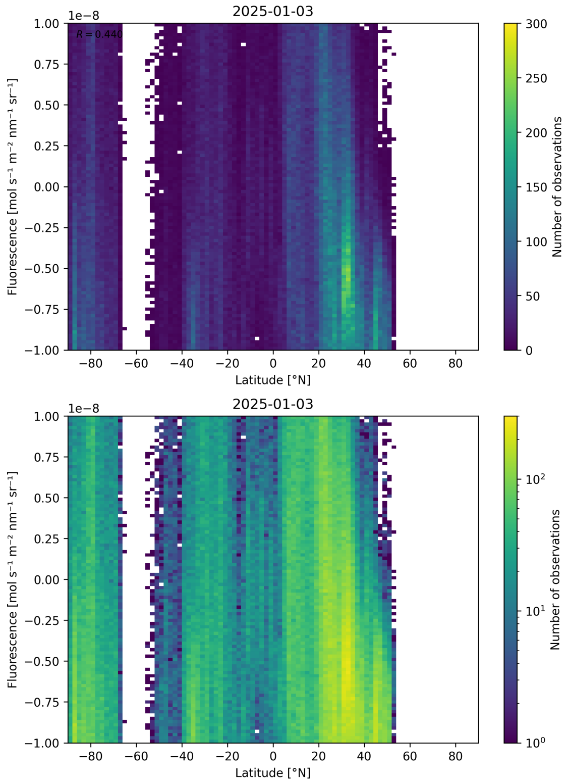
Figure 56: Scatter density plot of “Latitude” against “Fluorescence” for 2025-01-02 to 2025-01-04.
