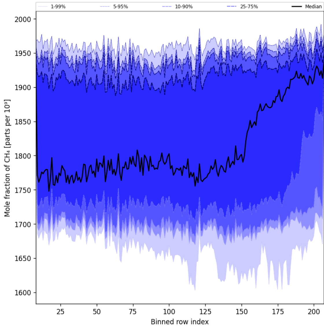
Figure 34: Along track statistics of “Mole fraction of CH 4 ” for 2025-01-02 to 2025-01-04
