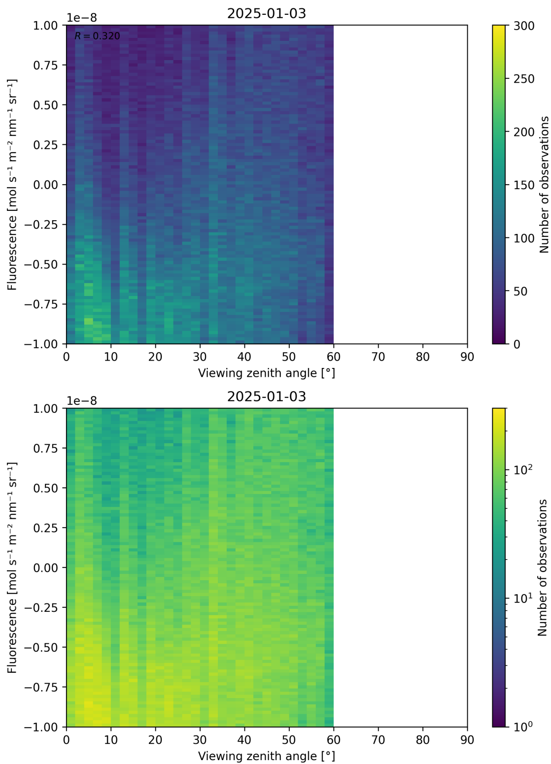
Figure 108: Scatter density plot of “Viewing zenith angle” against “Fluorescence” for 2025-01-02 to 2025-01-04.
