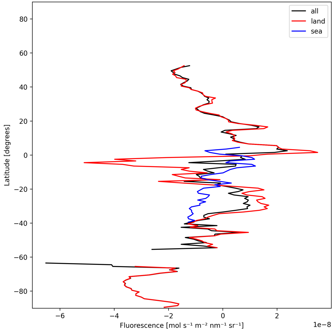
Figure 21: Zonal average of “Fluorescence” for 2025-01-02 to 2025-01-04.
