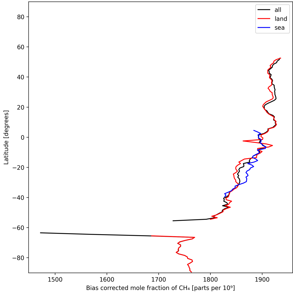
Figure 14: Zonal average of “Bias corrected mole fraction of CH 4 ” for 2025-01-02 to 2025-01-04.
