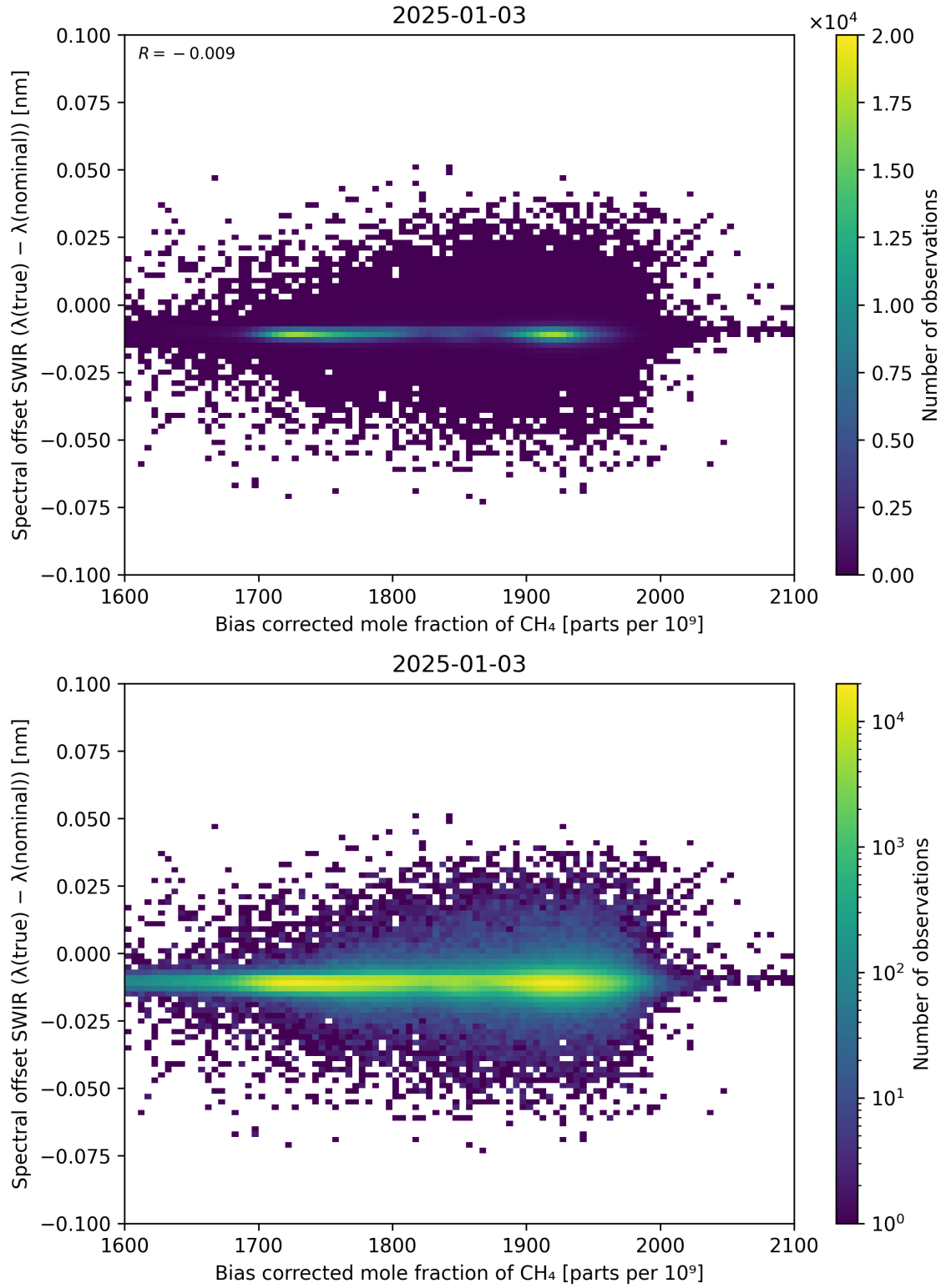
Figure 69: Scatter density plot of “Bias corrected mole fraction of \text{CH}_4 ” against “Spectral offset SWIR ( \lambda_{\text{true}} - \lambda_{\text{nominal}} )” for 2025-01-02 to 2025-01-04.
