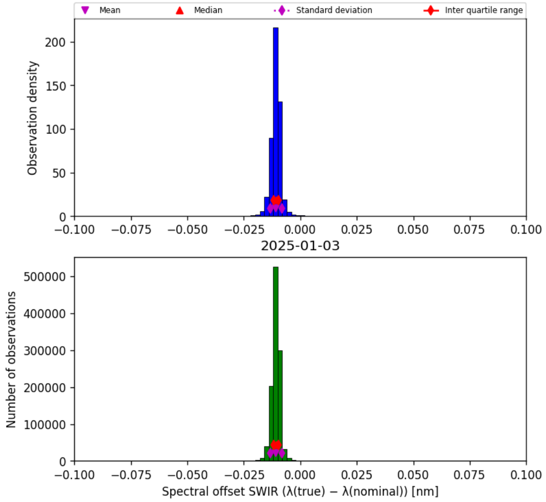
Figure 27: Histogram of “Spectral offset SWIR ( \lambda_{\text{true}} - \lambda_{\text{nominal}} )” for 2025-01-02 to 2025-01-04
