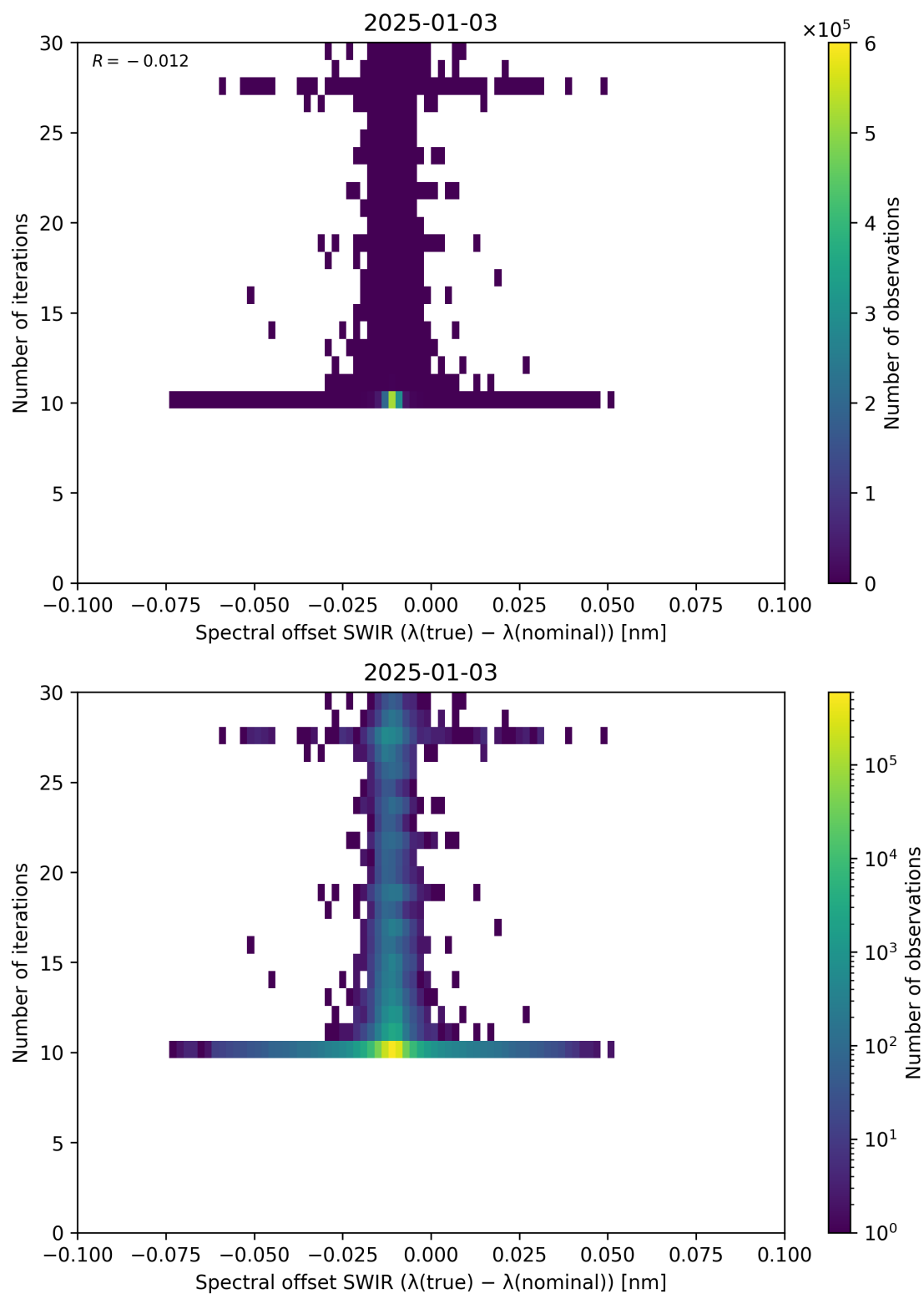
Figure 121: Scatter density plot of “Spectral offset SWIR ( \lambda_{\text{true}} - \lambda_{\text{nominal}} )” against “Number of iterations” for 2025-01-02 to 2025-01-04.
