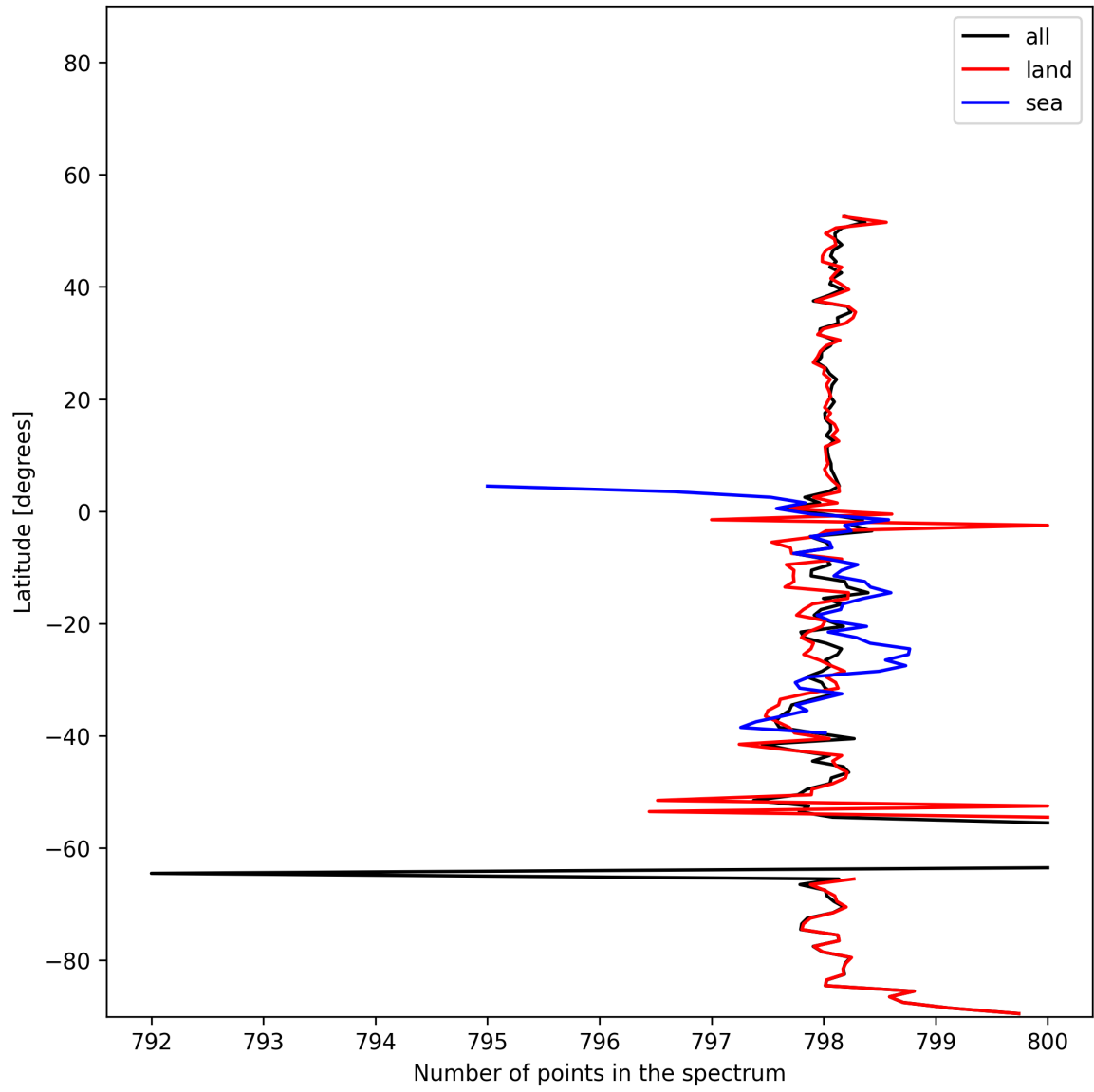
Figure 15: Zonal average of “Number of points in the spectrum” for 2025-01-02 to 2025-01-04.
