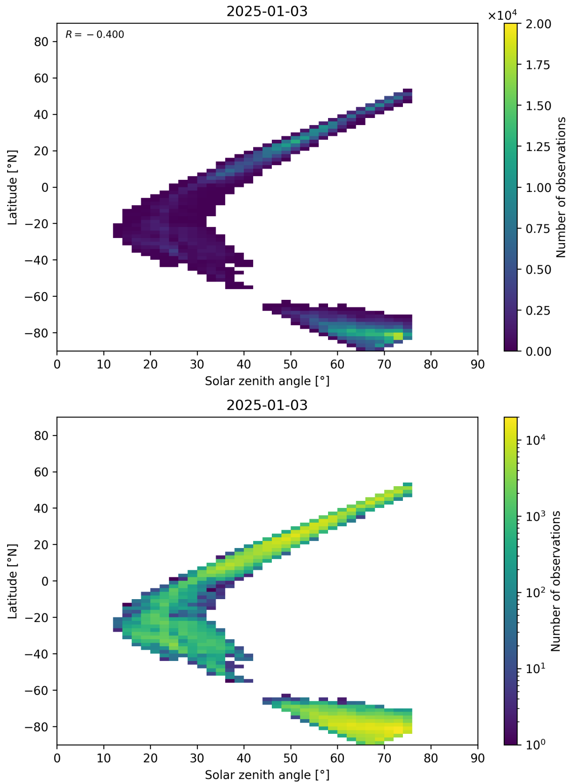
Figure 98: Scatter density plot of “Solar zenith angle” against “Latitude” for 2025-01-02 to 2025-01-04.
