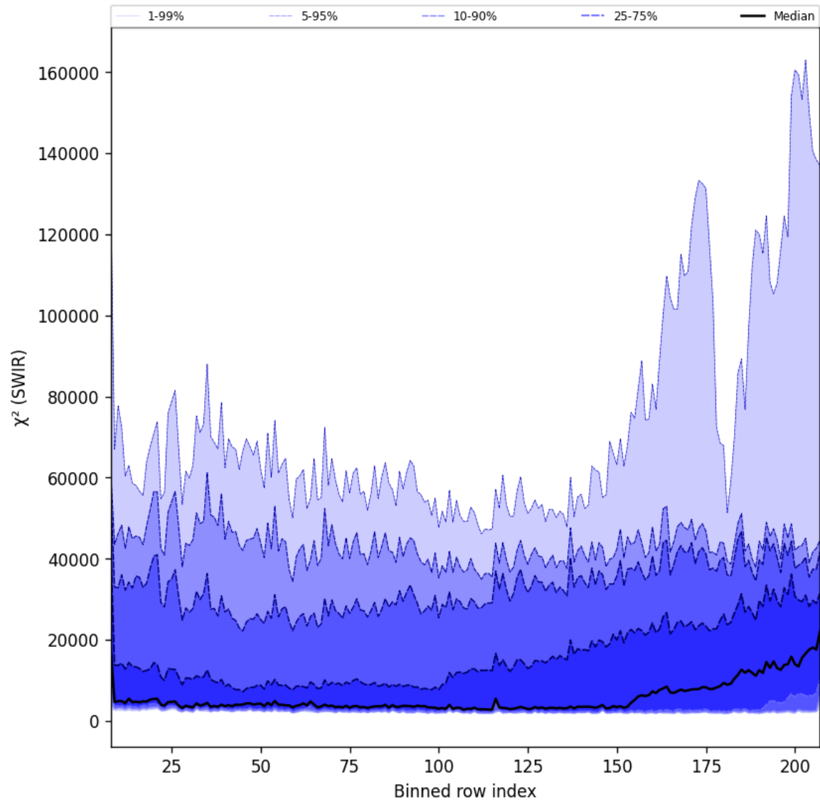
Figure 39: Along track statistics of “ \chi^2 (SWIR)” for 2025-01-02 to 2025-01-04
