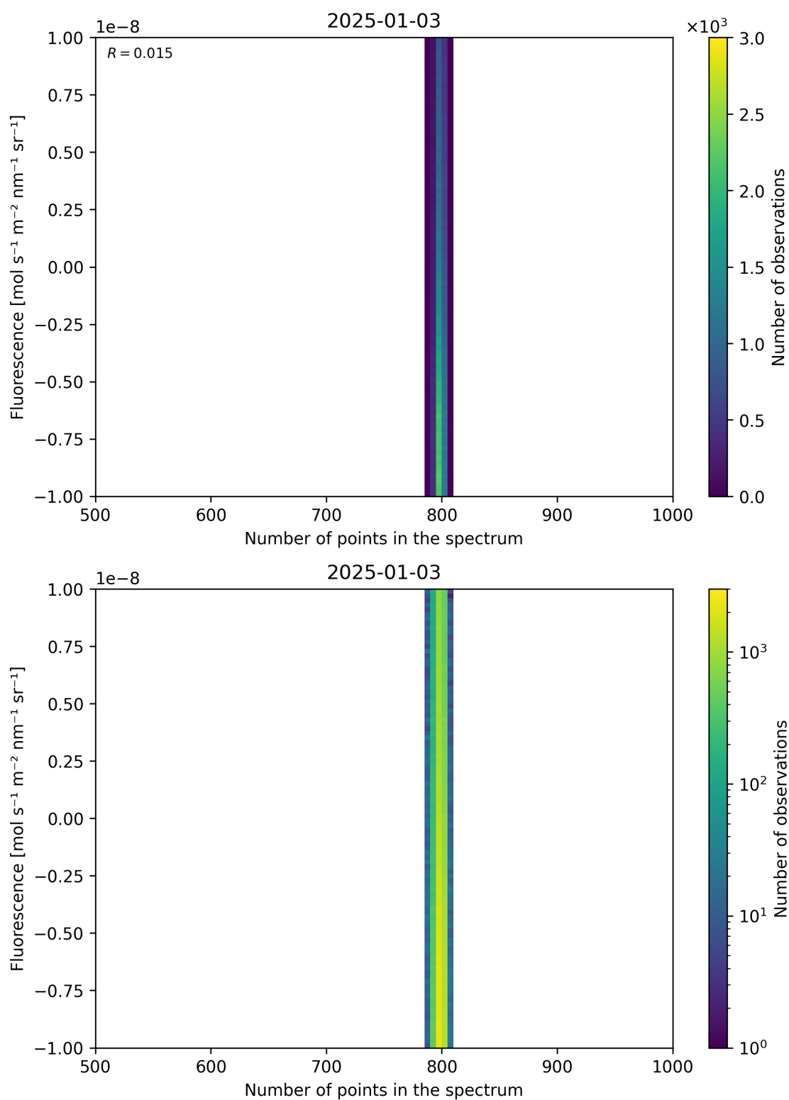
Figure 91: Scatter density plot of “Number of points in the spectrum” against “Fluorescence” for 2025-01-02 to 2025-01-04.
