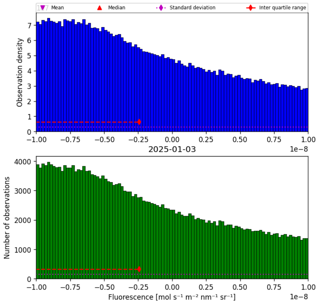
Figure 32: Histogram of “Fluorescence” for 2025-01-02 to 2025-01-04
