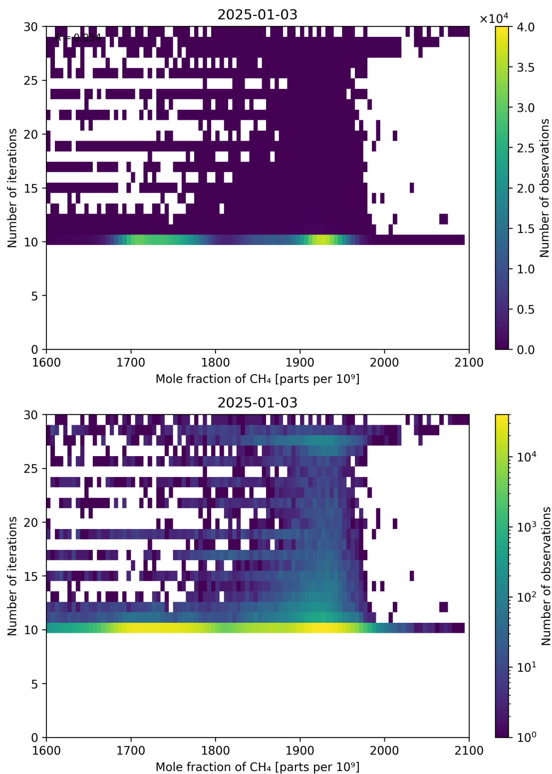
Figure 76: Scatter density plot of “Mole fraction of CH 4 ” against “Number of iterations” for 2025-01-02 to 2025-01-04.
