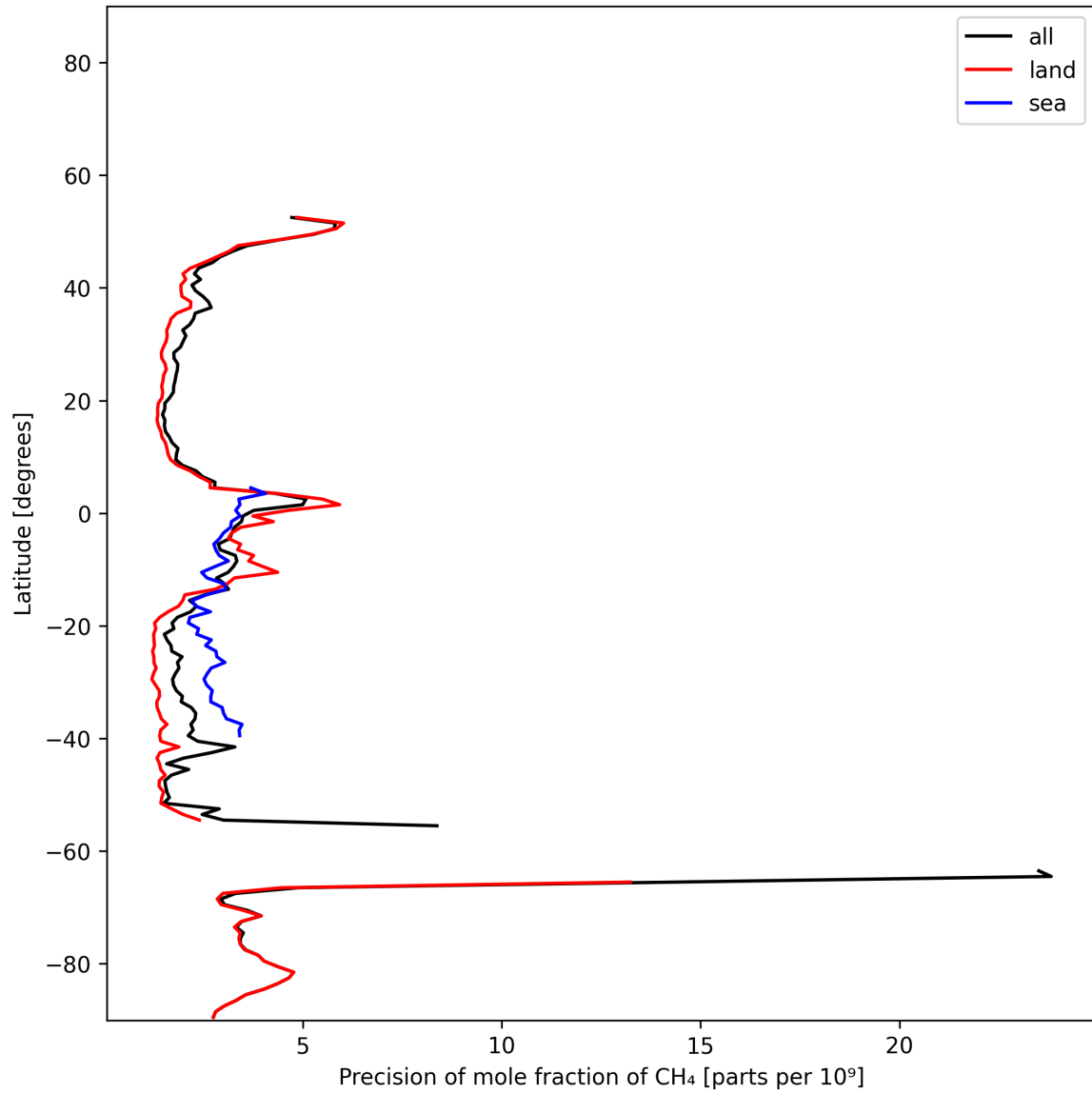
Figure 13: Zonal average of “Precision of mole fraction of CH 4 ” for 2025-01-02 to 2025-01-04.
