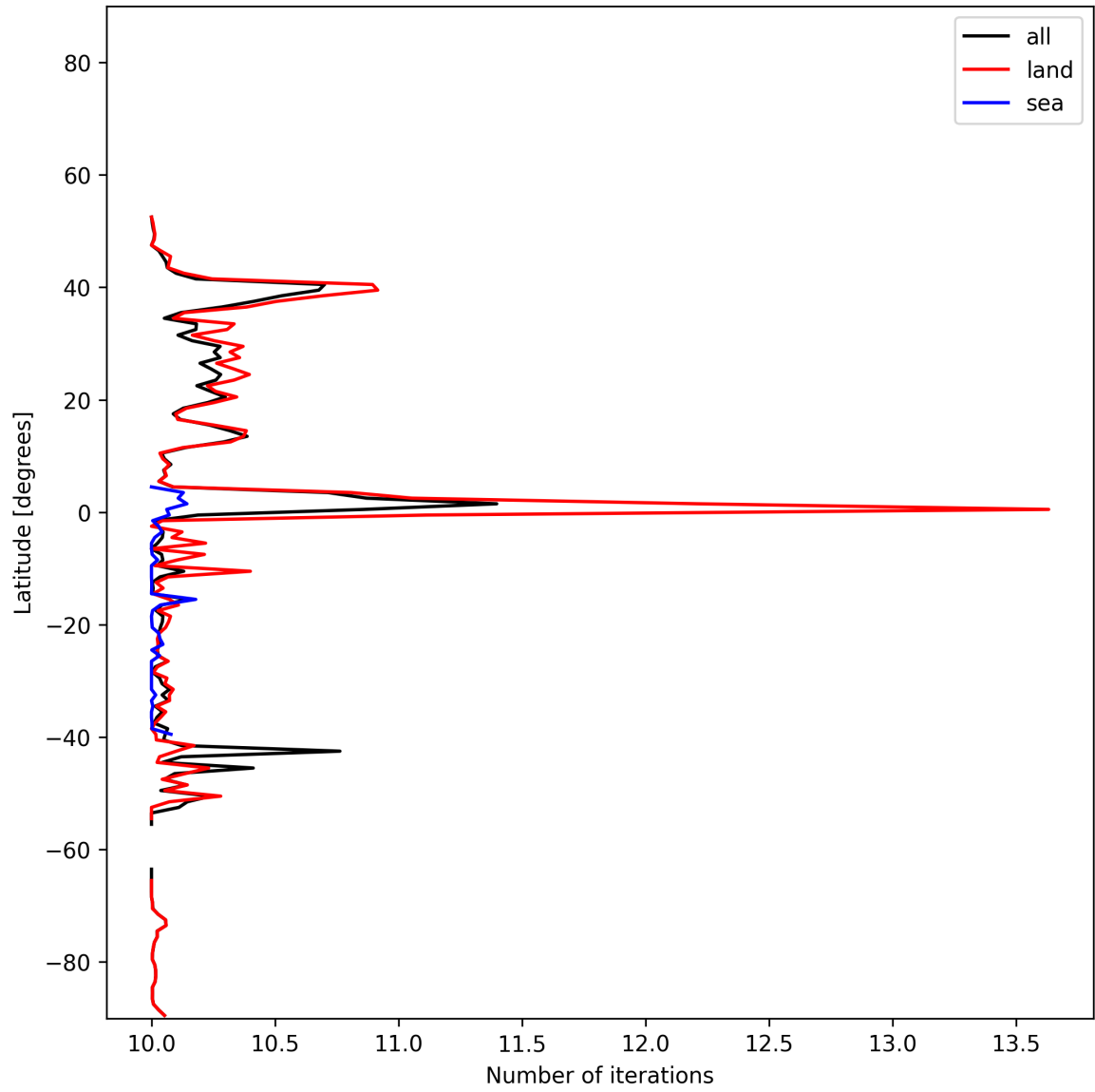
Figure 20: Zonal average of “Number of iterations” for 2025-01-02 to 2025-01-04.
