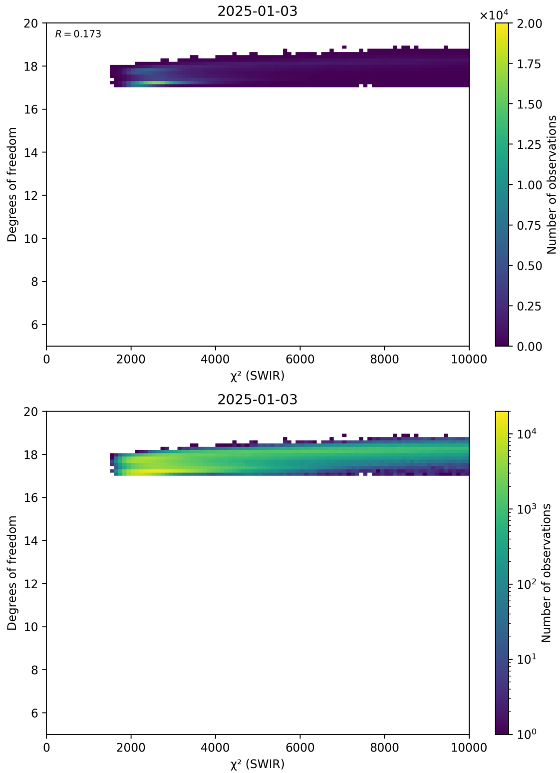
Figure 48: Scatter density plot of “ \chi^2 (SWIR)” against “Degrees of freedom” for 2025-01-02 to 2025-01-04.
