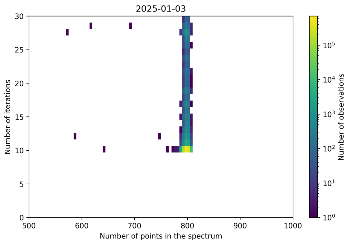
Figure 92: Scatter density plot of “Number of points in the spectrum” against “Number of iterations” for 2025-01-02 to 2025-01-04.
