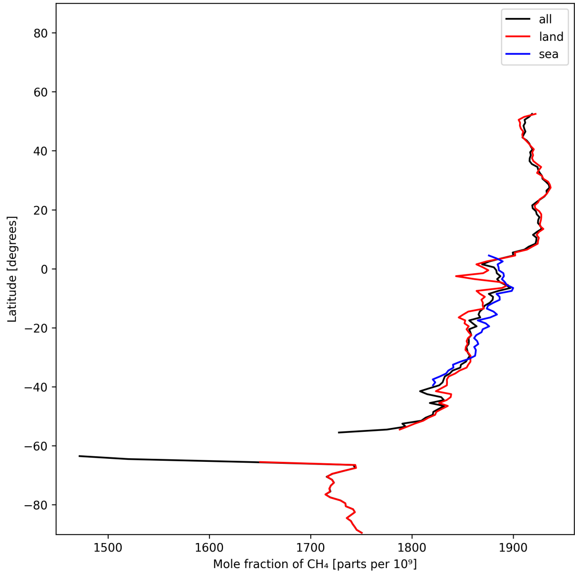
Figure 12: Zonal average of “Mole fraction of CH 4 ” for 2025-01-02 to 2025-01-04.
