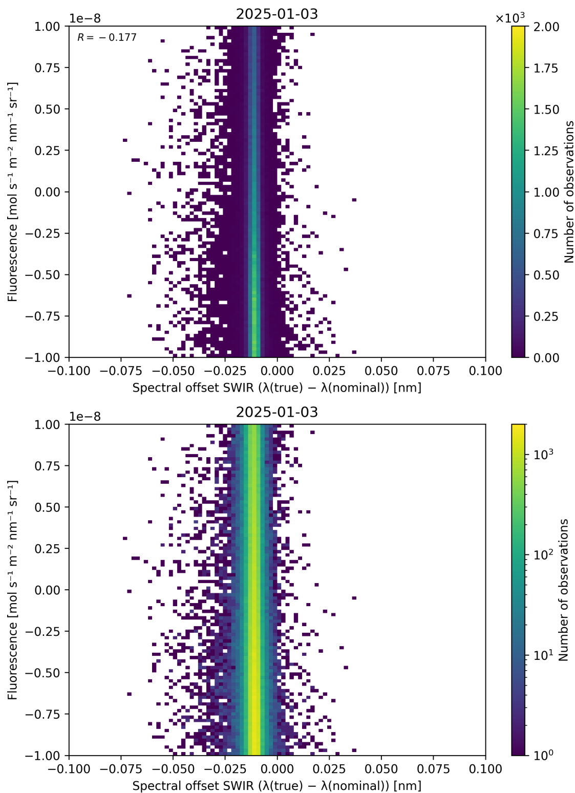
Figure 120: Scatter density plot of “Spectral offset SWIR ( \lambda_{\text{true}} - \lambda_{\text{nominal}} )” against “Fluorescence” for 2025-01-02 to 2025-01-04.
