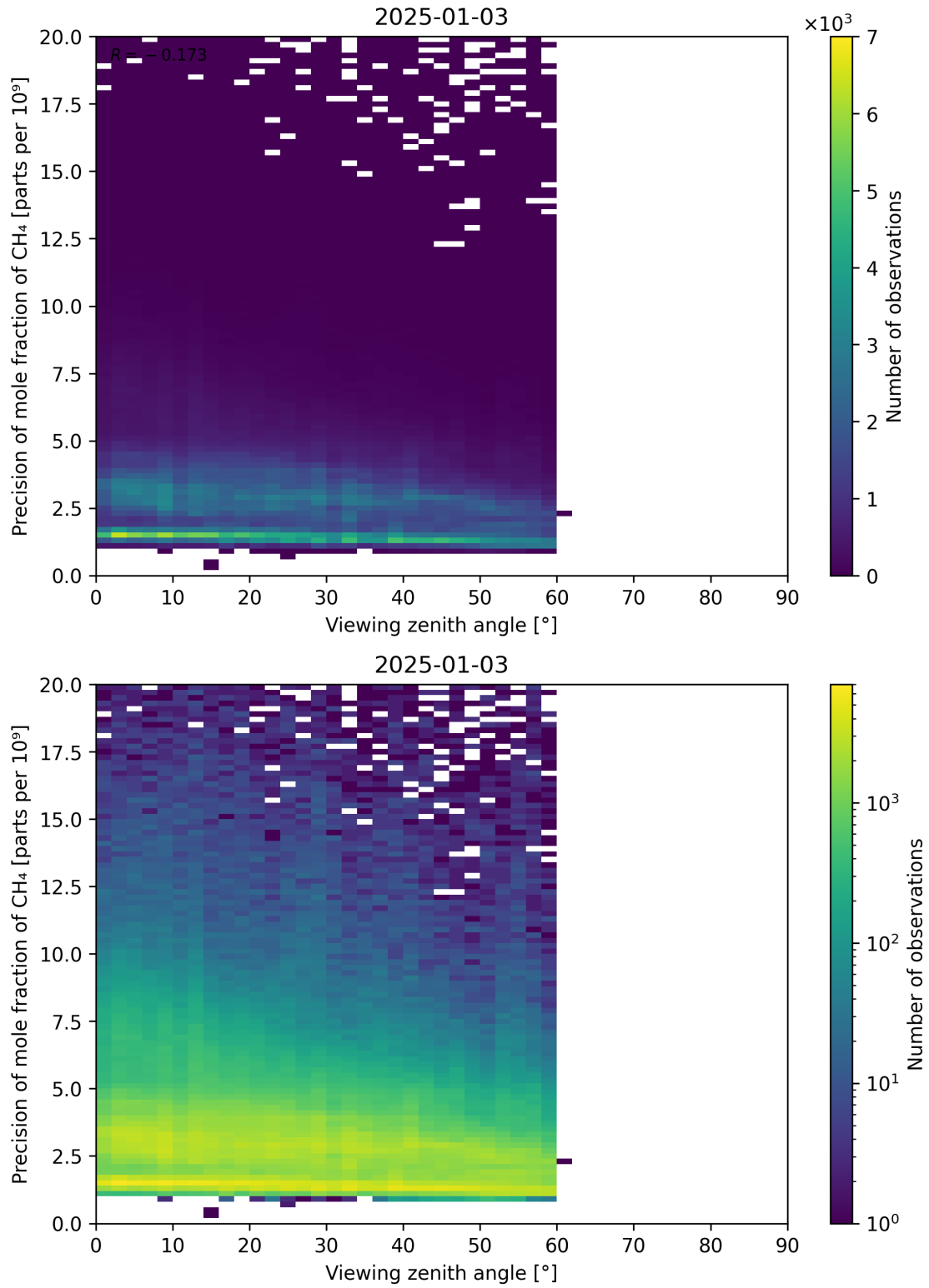
Figure 112: Scatter density plot of “Viewing zenith angle” against “Precision of mole fraction of CH 4 ” for 2025-01-02 to 2025-01-04.
