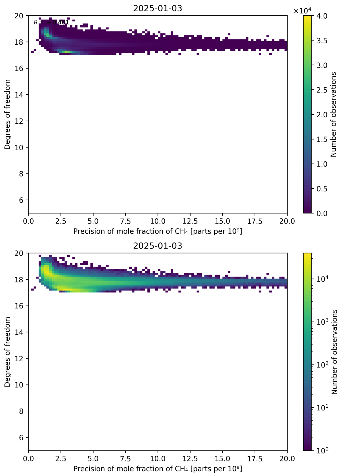
Figure 80: Scatter density plot of “Precision of mole fraction of CH 4 ” against “Degrees of freedom” for 2025-01-02 to 2025-01-04.
