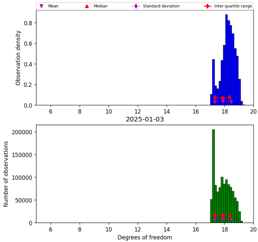
Figure 30: Histogram of “Degrees of freedom” for 2025-01-02 to 2025-01-04
