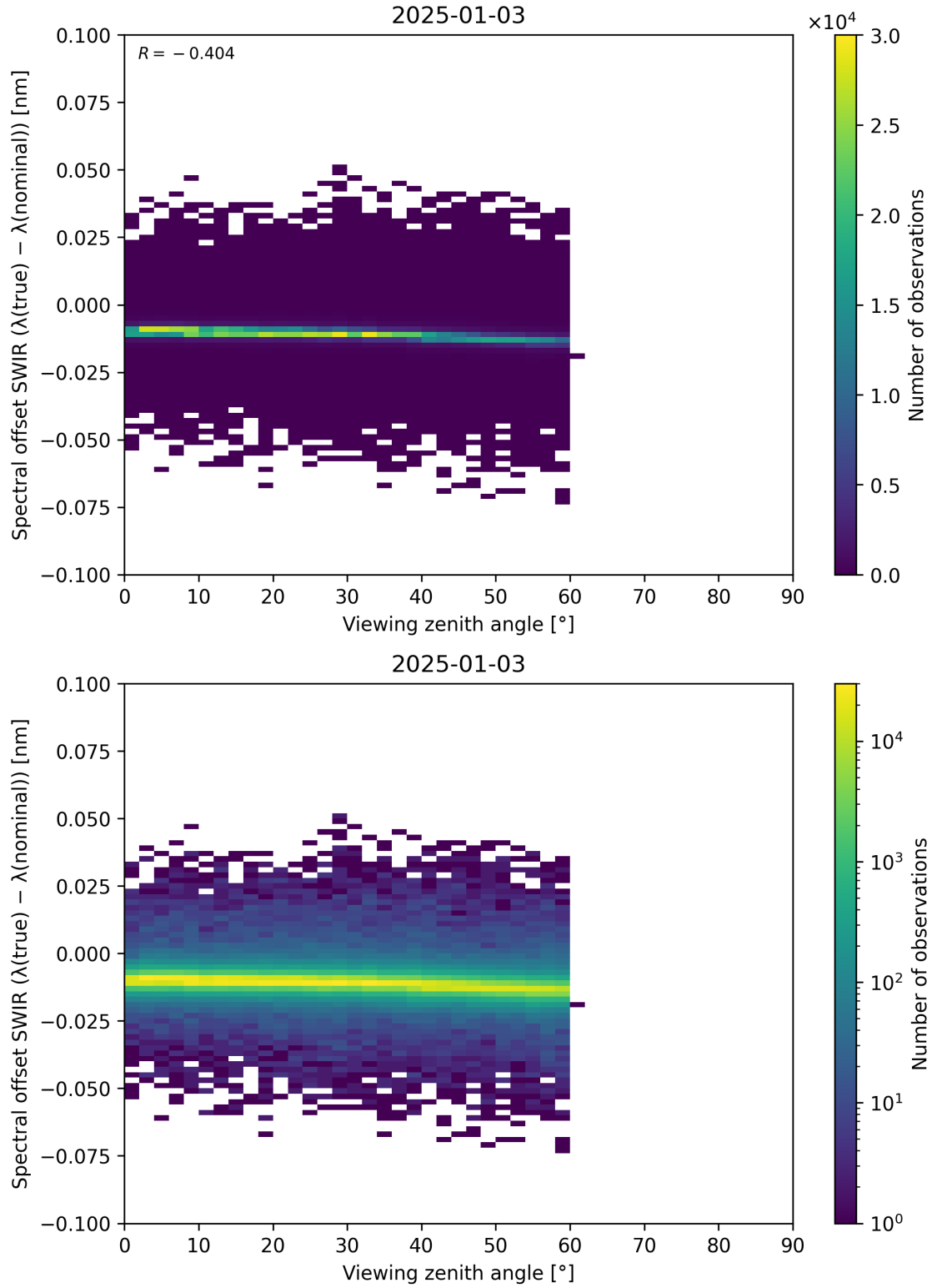
Figure 116: Scatter density plot of “Viewing zenith angle” against “Spectral offset SWIR ( \lambda_{\text{true}} - \lambda_{\text{nominal}} )” for 2025-01-02 to 2025-01-04.
