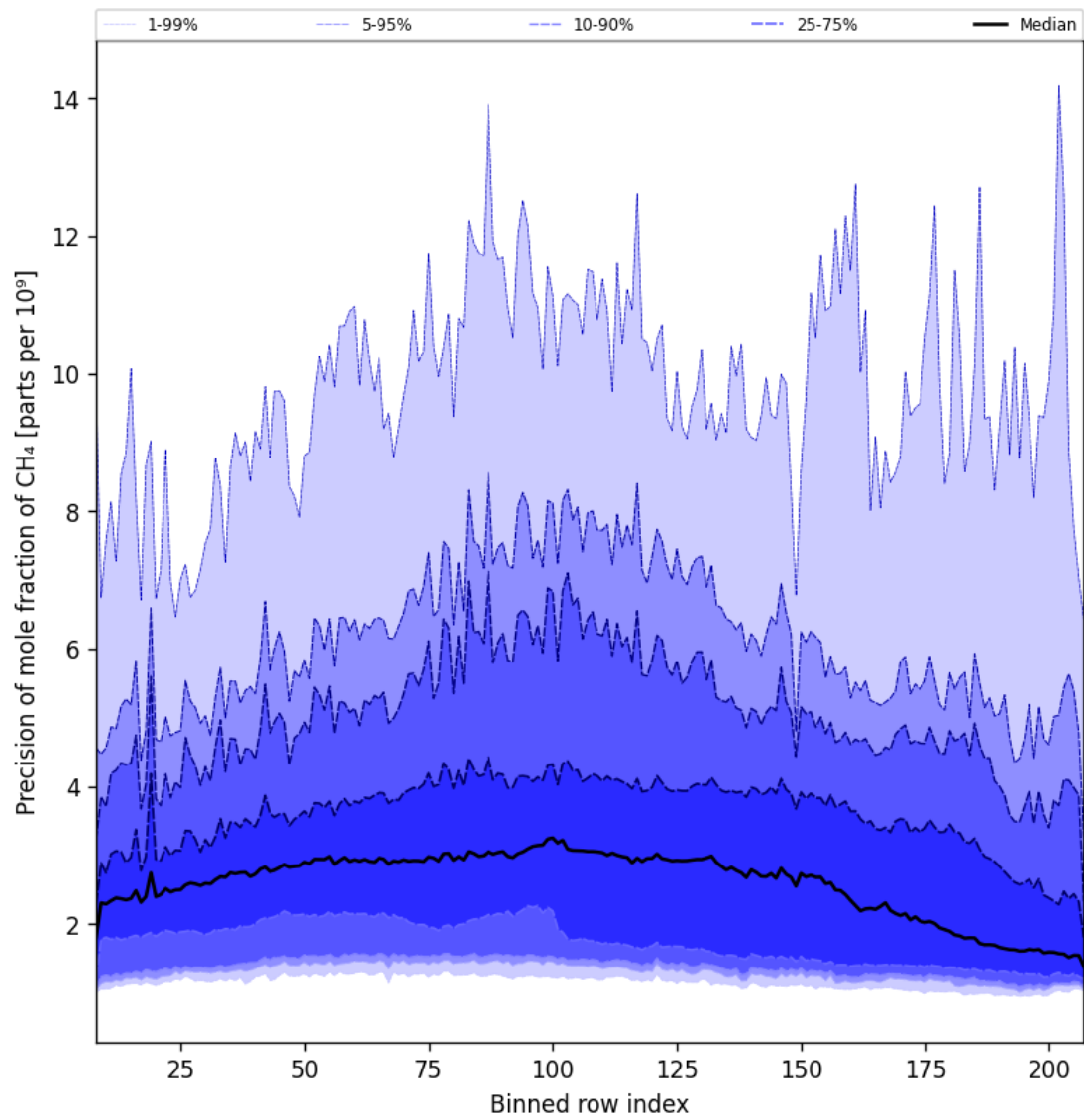
Figure 35: Along track statistics of “Precision of mole fraction of CH 4 ” for 2025-01-02 to 2025-01-04
