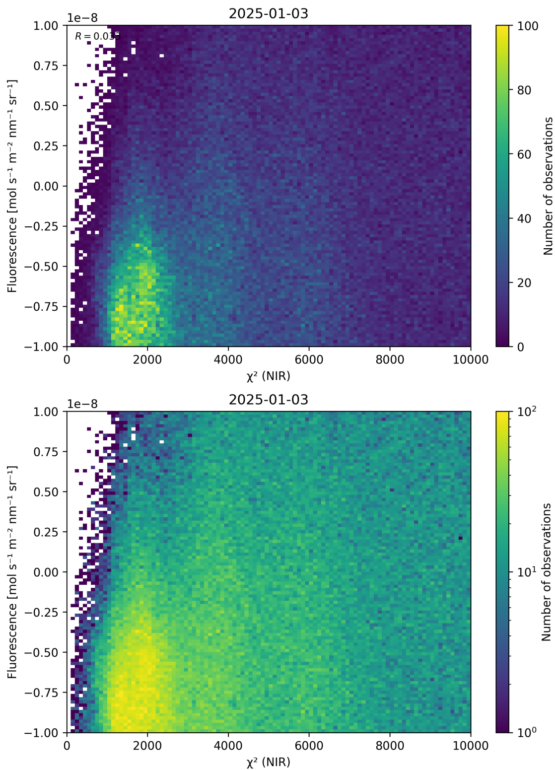
Figure 45: Scatter density plot of “ \chi^2 (NIR)” against “Fluorescence” for 2025-01-02 to 2025-01-04.
