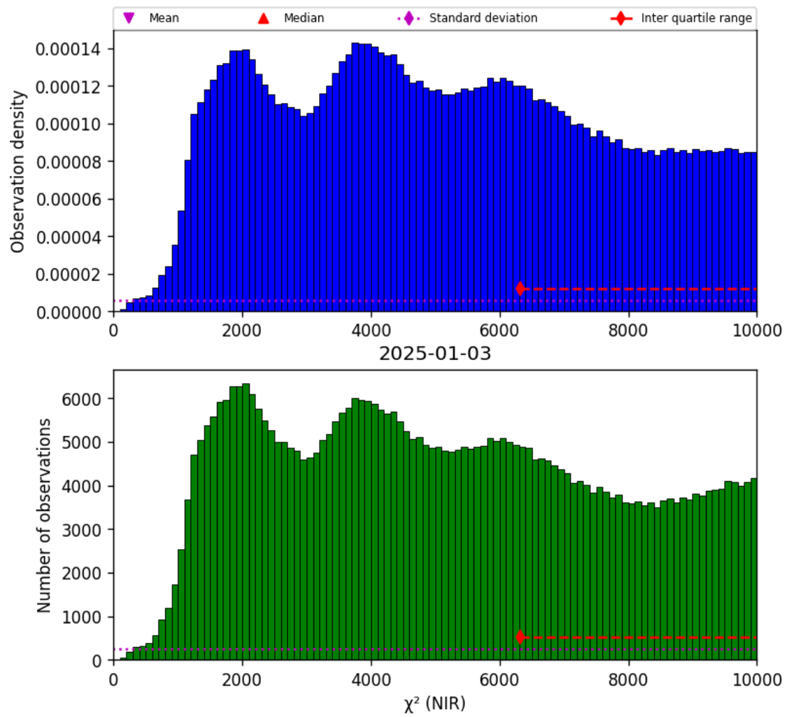
Figure 29: Histogram of “ \chi^2 (NIR)” for 2025-01-02 to 2025-01-04
