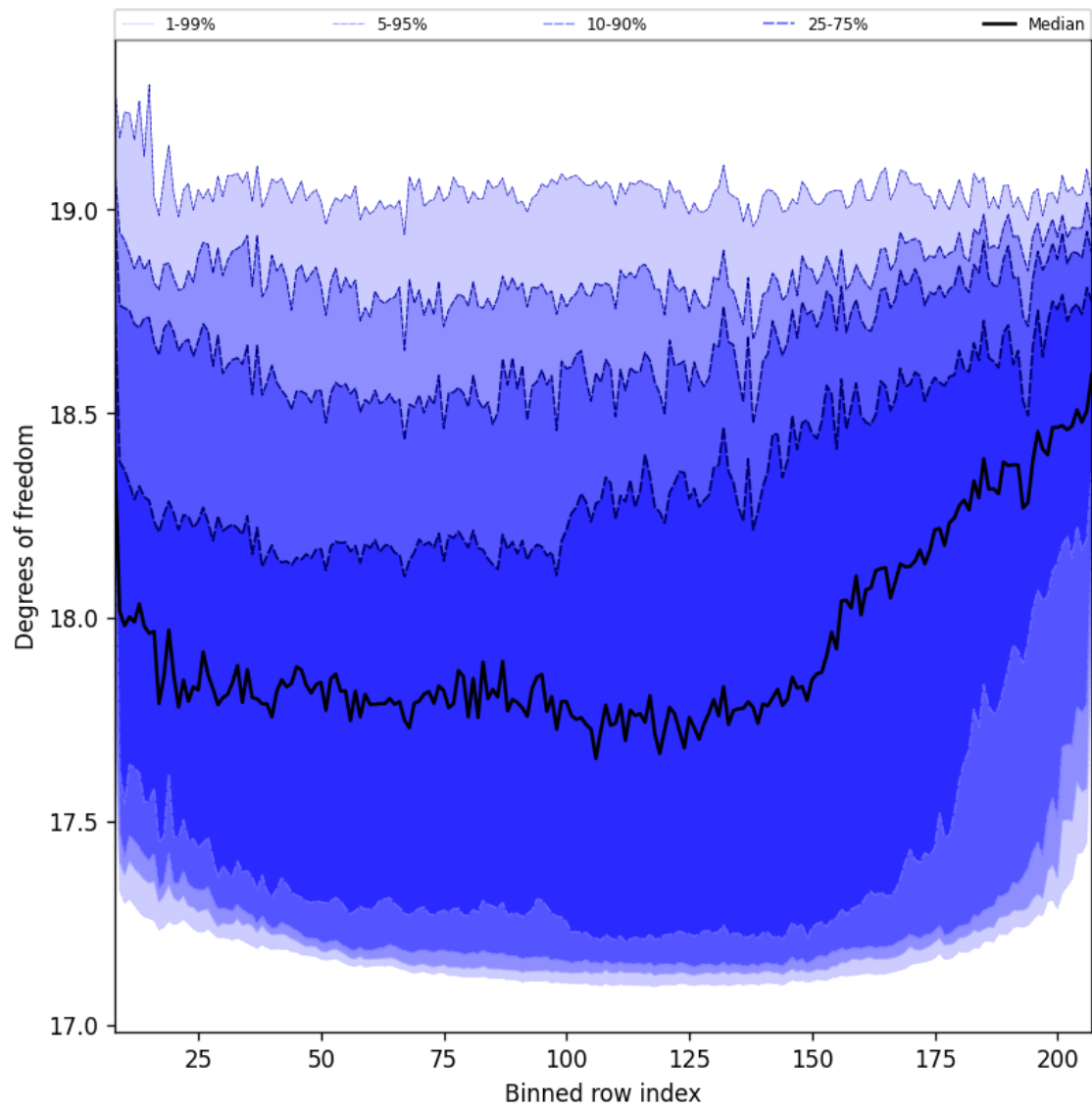
Figure 41: Along track statistics of “Degrees of freedom” for 2025-01-02 to 2025-01-04
