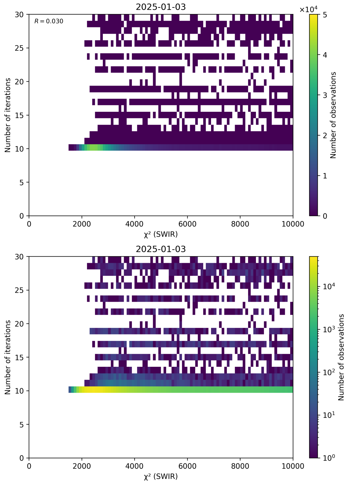
Figure 50: Scatter density plot of “ \chi^2 (SWIR)” against “Number of iterations” for 2025-01-02 to 2025-01-04.
