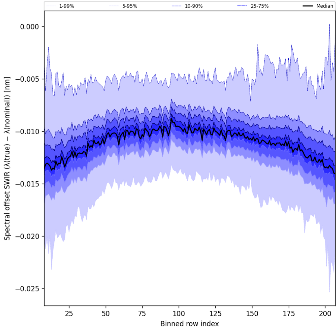
Figure 38: Along track statistics of “Spectral offset SWIR ( \lambda_{\text{true}} - \lambda_{\text{nominal}} )” for 2025-01-02 to 2025-01-04
