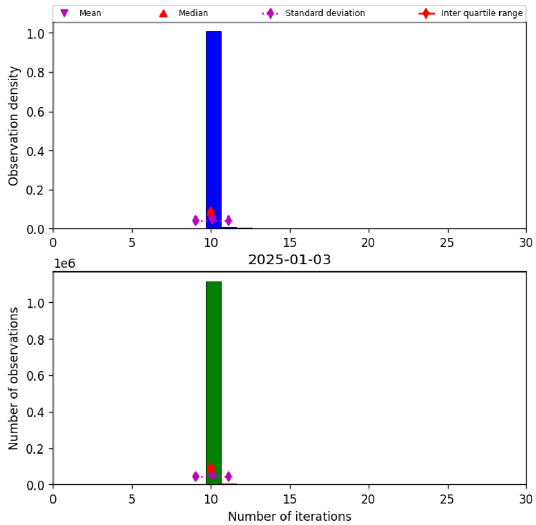
Figure 31: Histogram of “Number of iterations” for 2025-01-02 to 2025-01-04
