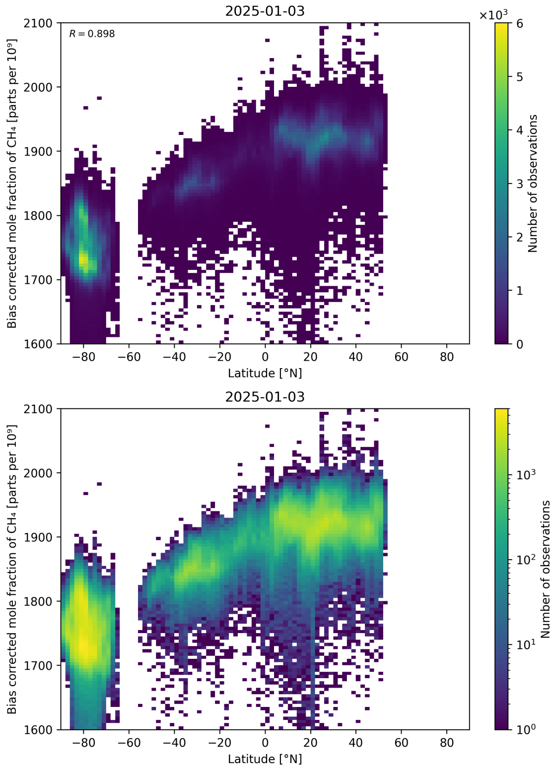
Figure 58: Scatter density plot of “Latitude” against “Bias corrected mole fraction of CH 4 ” for 2025-01-02 to 2025-01-04.
