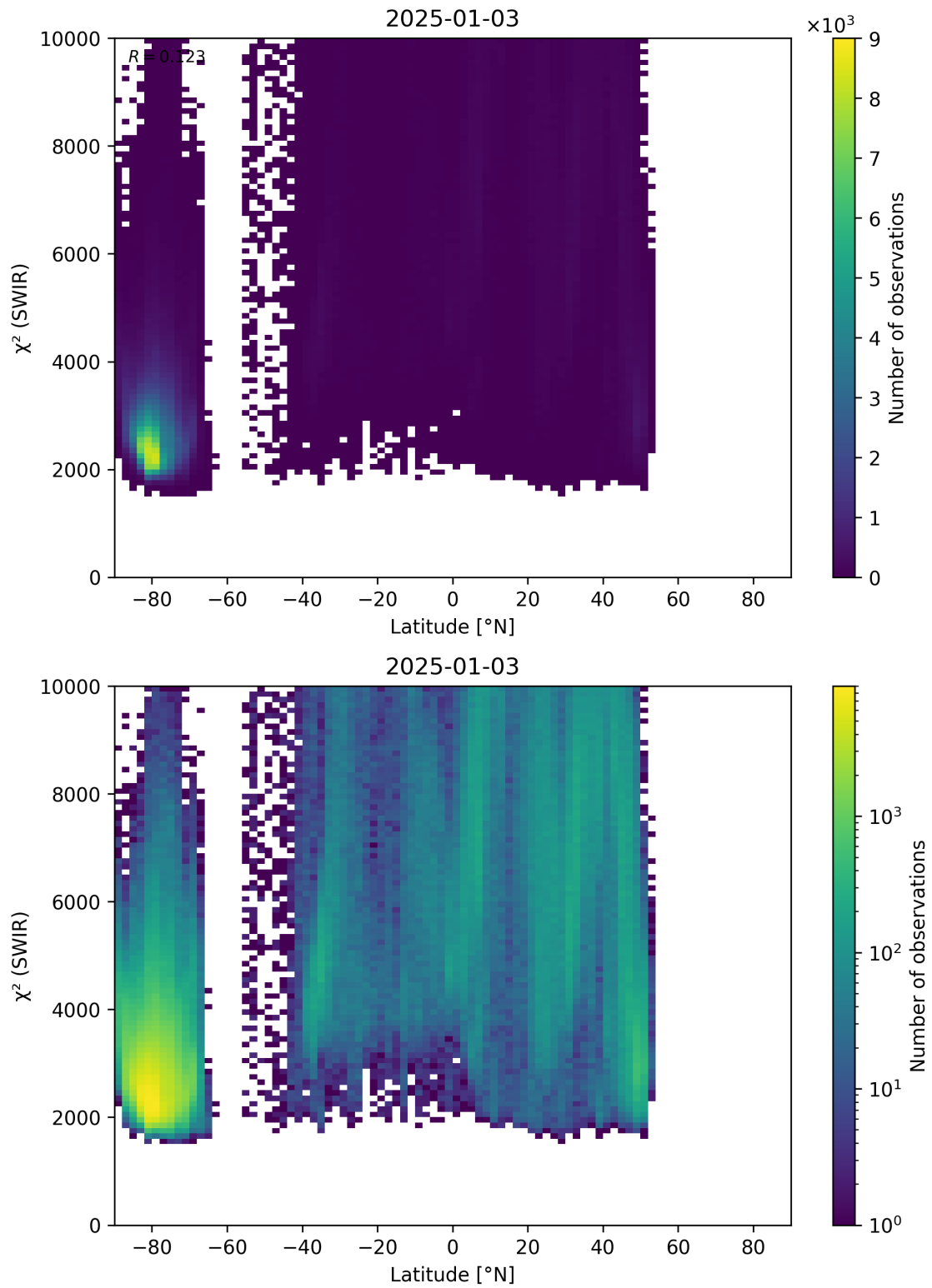
Figure 54: Scatter density plot of “Latitude” against “ \chi^2 (SWIR)” for 2025-01-02 to 2025-01-04.
