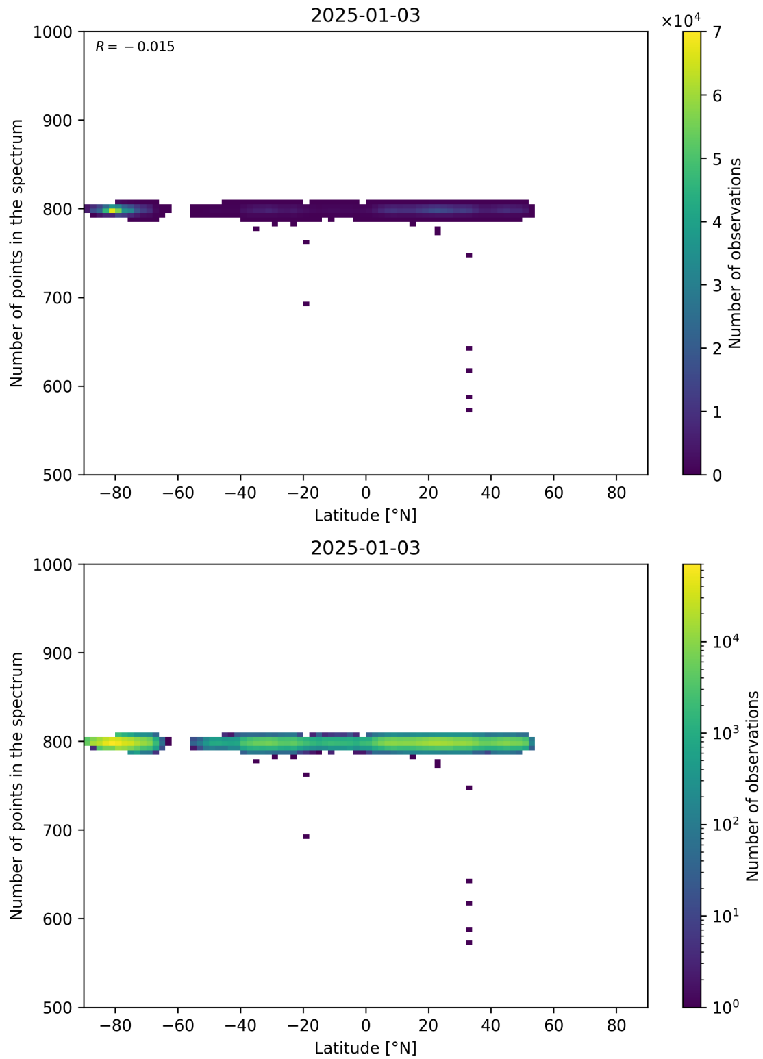
Figure 61: Scatter density plot of “Latitude” against “Number of points in the spectrum” for 2025-01-02 to 2025-01-04.
