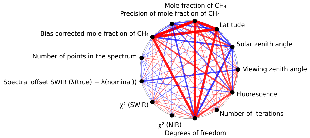
Figure 1: Map of correlation graph for 2025-01-02 to 2025-01-04.
