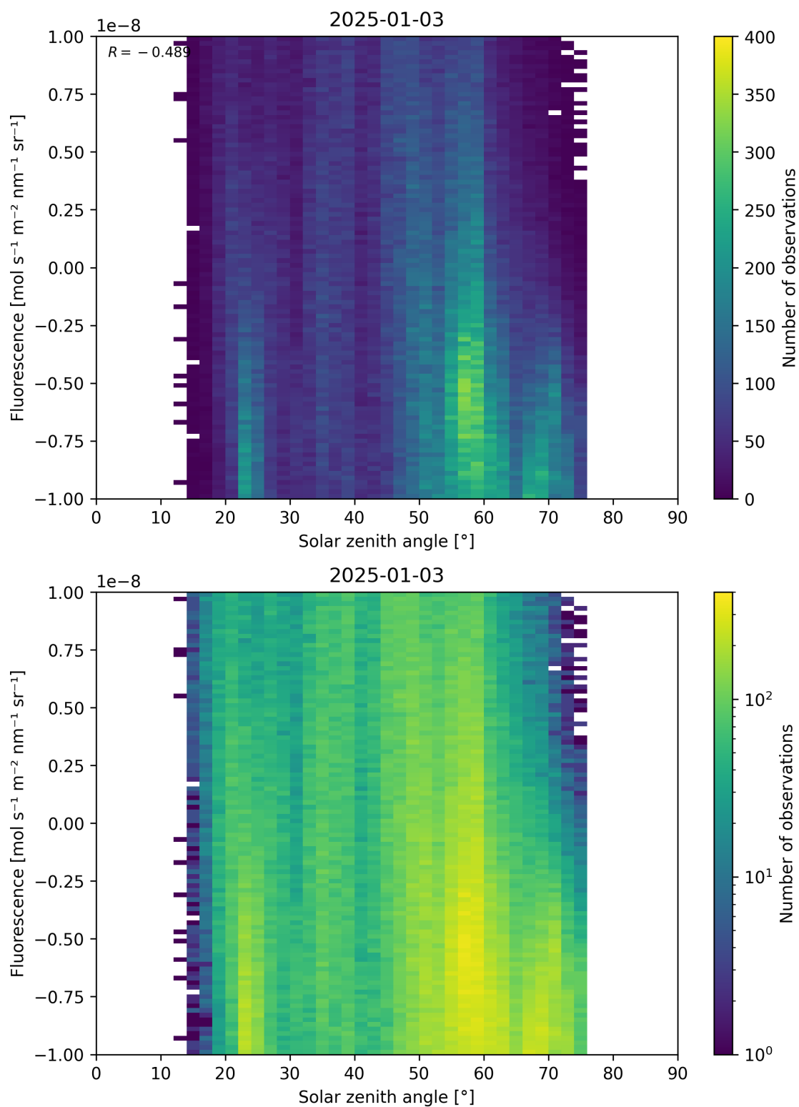
Figure 97: Scatter density plot of “Solar zenith angle” against “Fluorescence” for 2025-01-02 to 2025-01-04.
