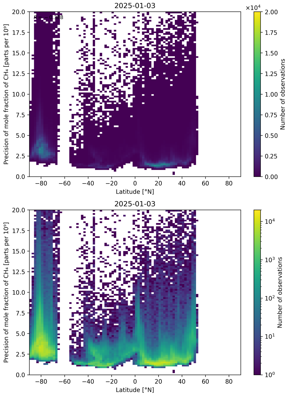
Figure 59: Scatter density plot of “Latitude” against “Precision of mole fraction of CH 4 ” for 2025-01-02 to 2025-01-04.
