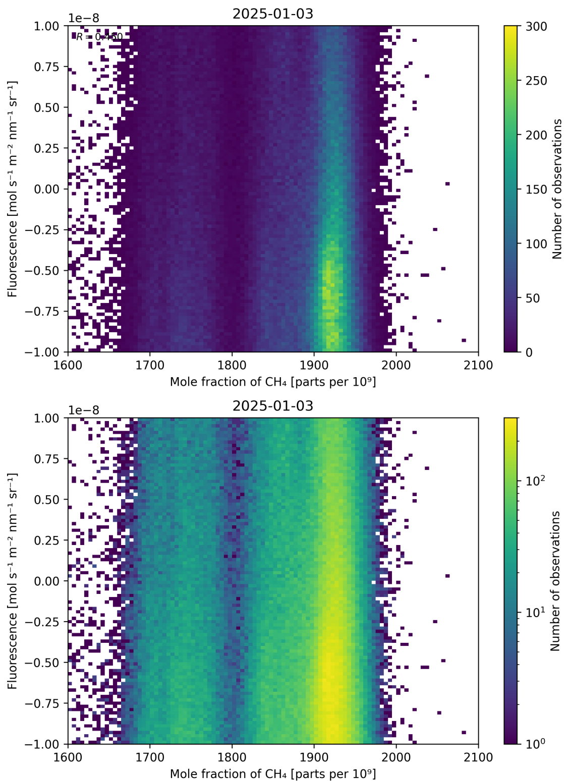
Figure 73: Scatter density plot of “Mole fraction of \text{CH}_4 ” against “Fluorescence” for 2025-01-02 to 2025-01-04.
