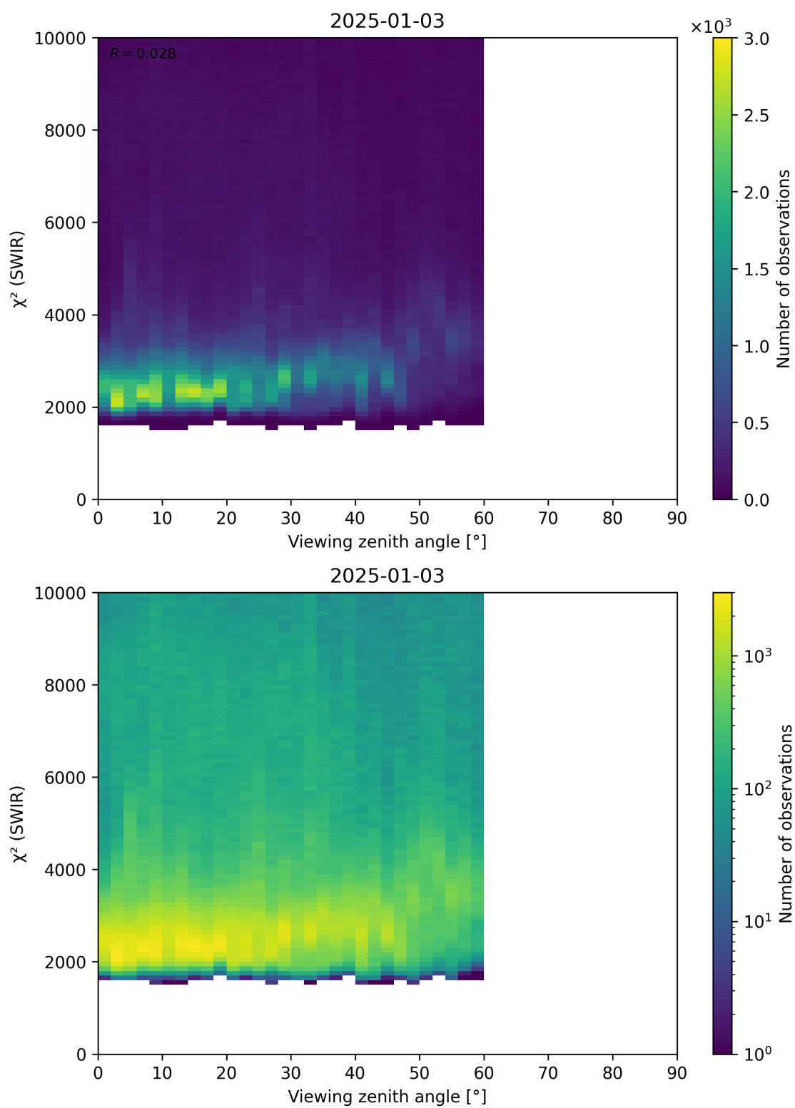
Figure 106: Scatter density plot of “Viewing zenith angle” against “ \chi^2 (SWIR)” for 2025-01-02 to 2025-01-04.
