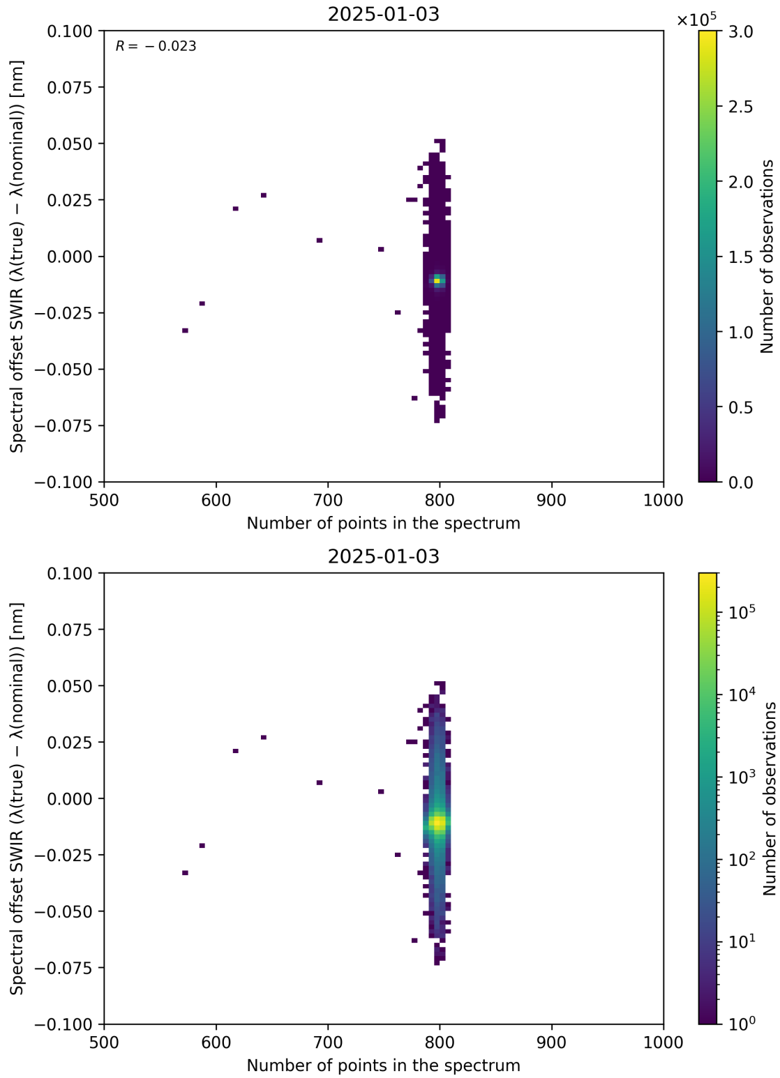
Figure 93: Scatter density plot of “Number of points in the spectrum” against “Spectral offset SWIR ( \lambda_{\text{true}} - \lambda_{\text{nominal}} )” for 2025-01-02 to 2025-01-04.
