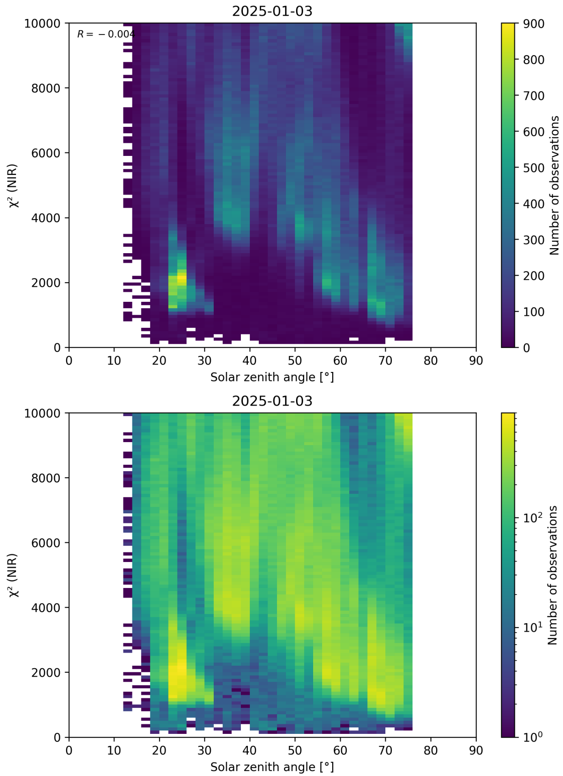
Figure 94: Scatter density plot of “Solar zenith angle” against “ \chi^2 (NIR)” for 2025-01-02 to 2025-01-04.
