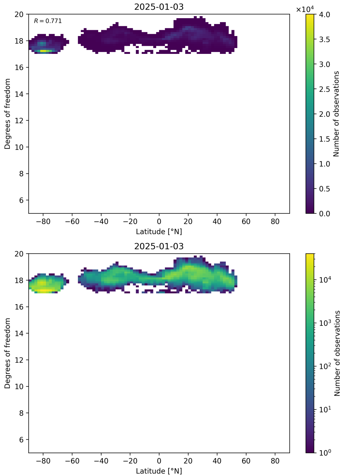
Figure 55: Scatter density plot of “Latitude” against “Degrees of freedom” for 2025-01-02 to 2025-01-04.
