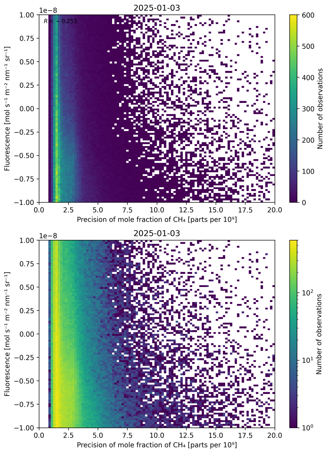
Figure 81: Scatter density plot of “Precision of mole fraction of \text{CH}_4 ” against “Fluorescence” for 2025-01-02 to 2025-01-04.
