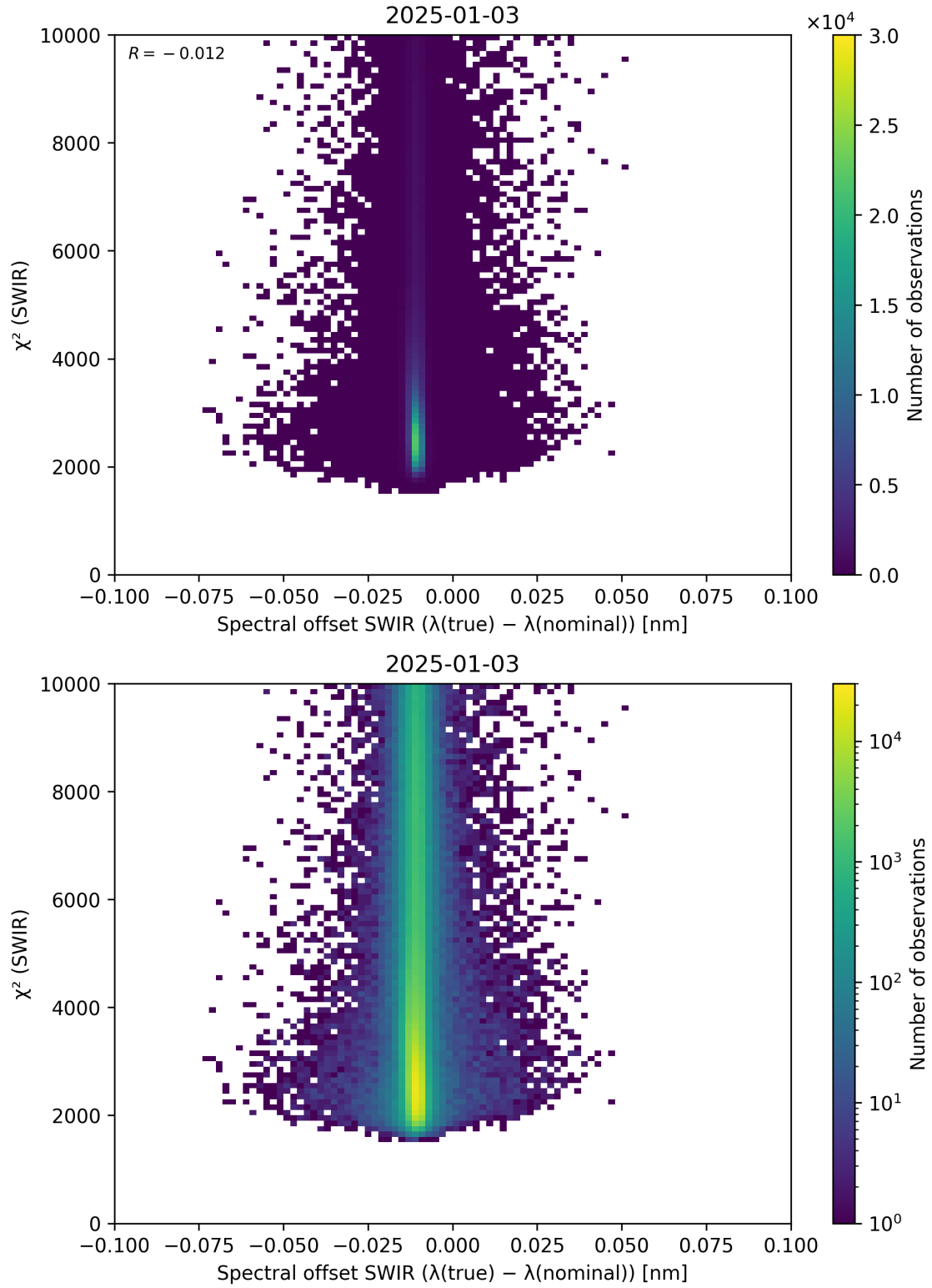
Figure 118: Scatter density plot of “Spectral offset SWIR ( \lambda_{\text{true}} - \lambda_{\text{nominal}} )” against “ \chi^2 (SWIR)” for 2025-01-02 to 2025-01-04.
