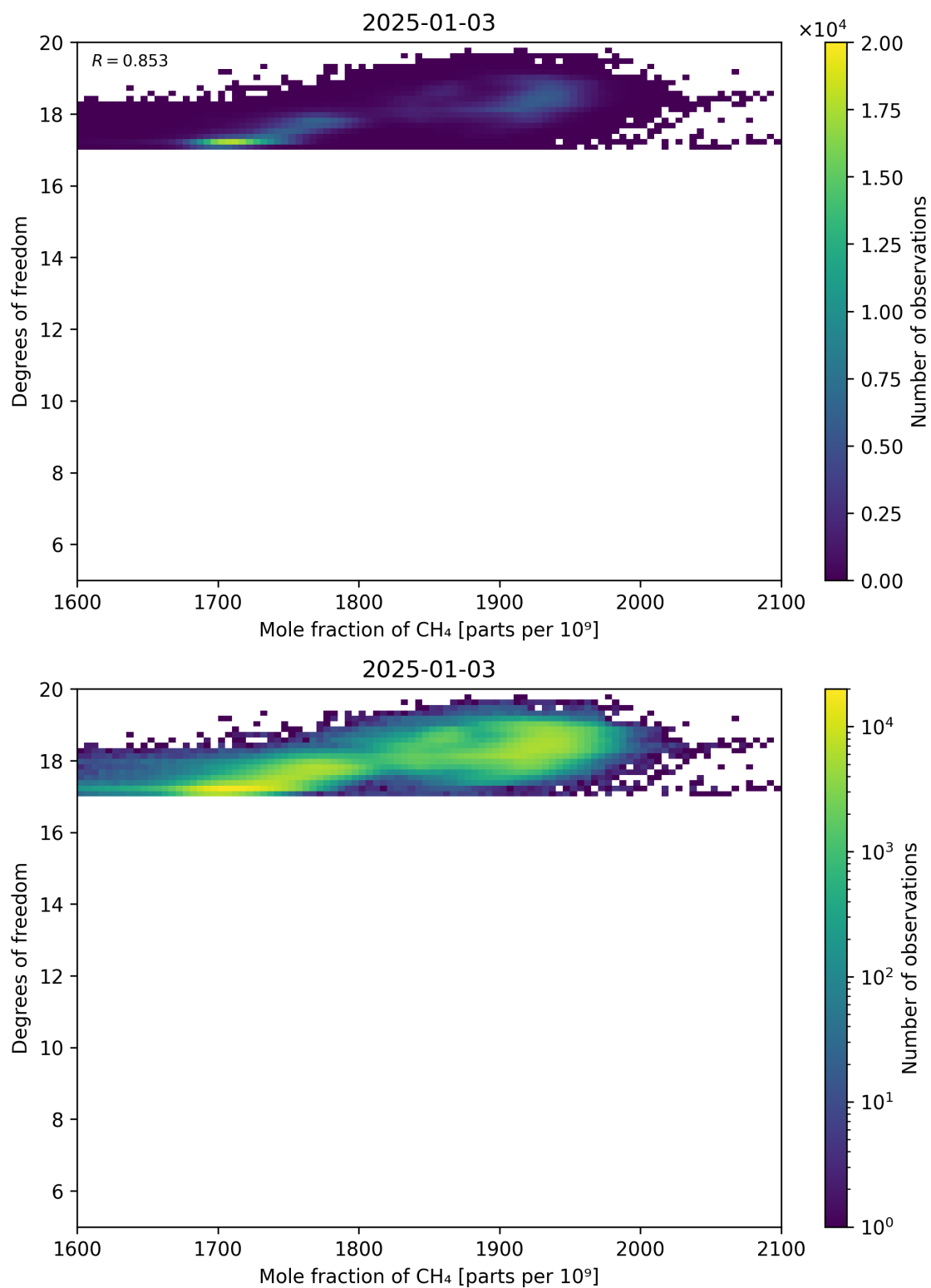
Figure 72: Scatter density plot of “Mole fraction of CH 4 ” against “Degrees of freedom” for 2025-01-02 to 2025-01-04.
