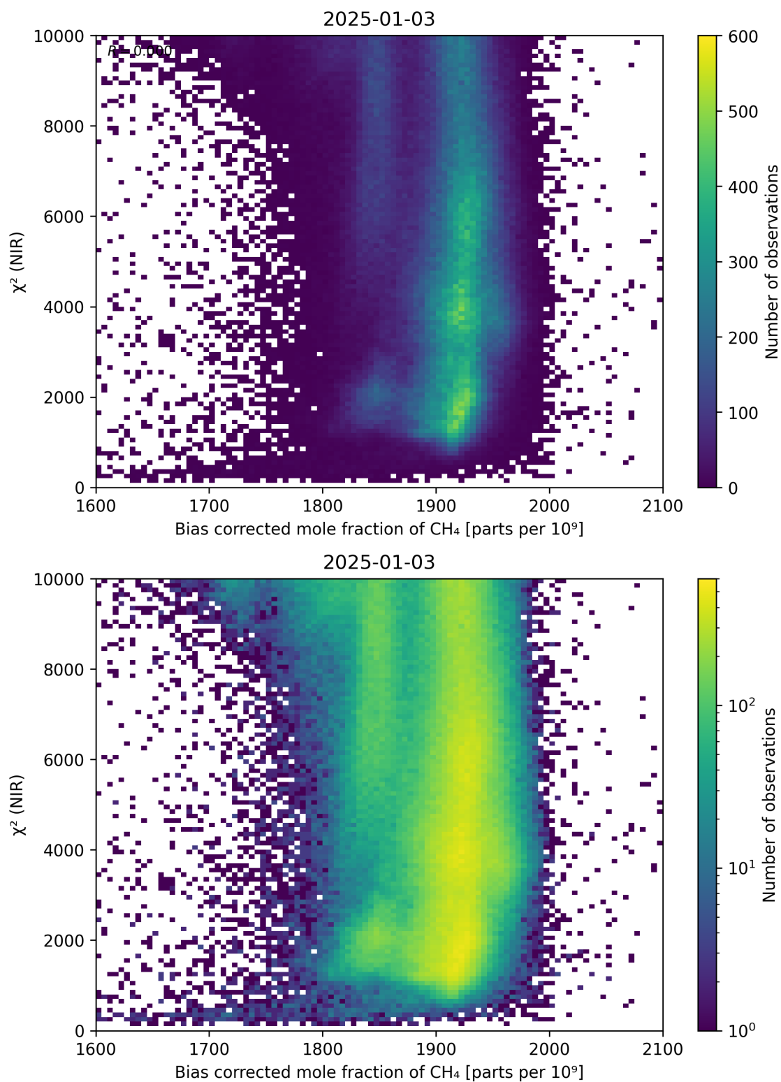
Figure 63: Scatter density plot of “Bias corrected mole fraction of CH 4 ” against “ \chi^2 (NIR)” for 2025-01-02 to 2025-01-04.
