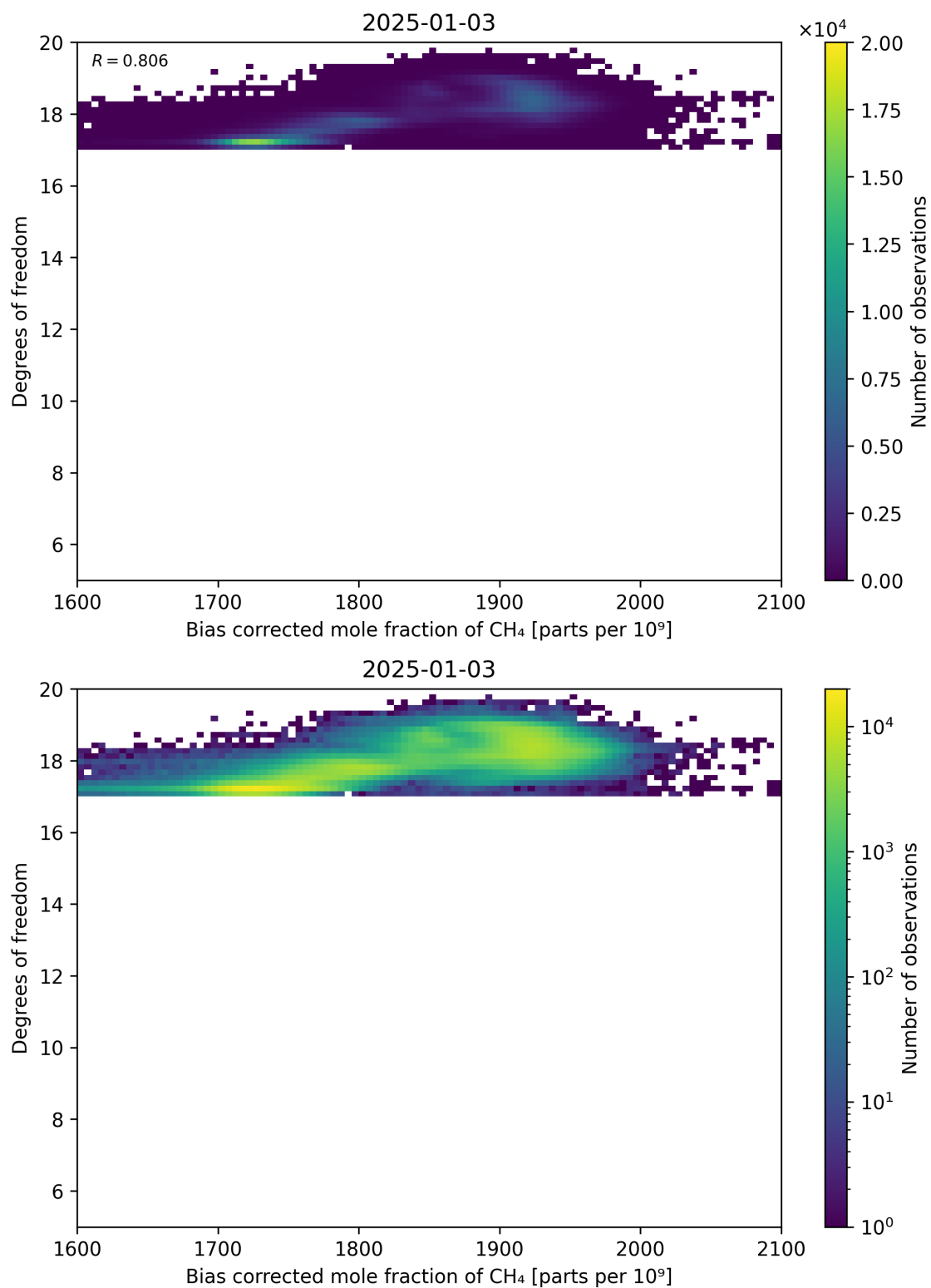
Figure 65: Scatter density plot of “Bias corrected mole fraction of CH 4 ” against “Degrees of freedom” for 2025-01-02 to 2025-01-04.
