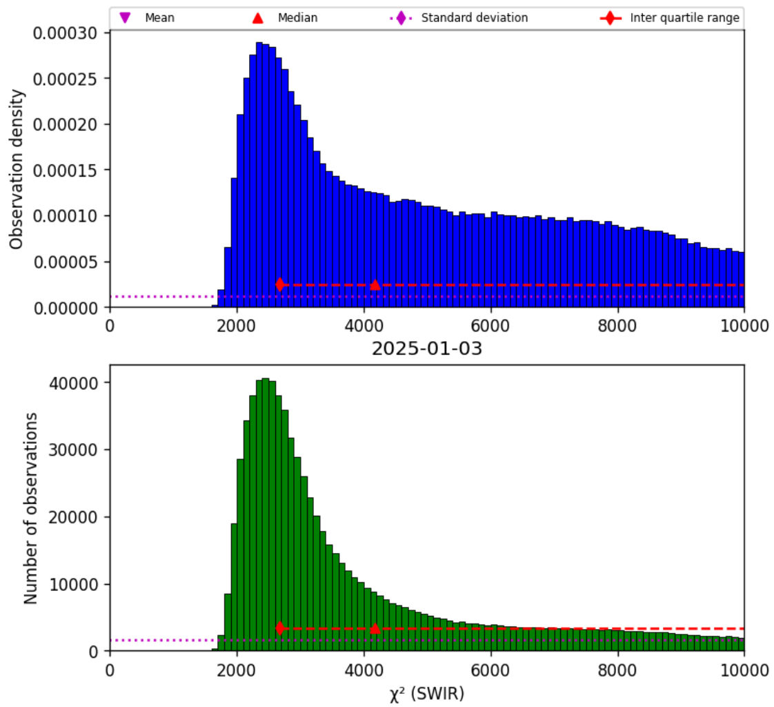
Figure 28: Histogram of “ \chi^2 (SWIR)” for 2025-01-02 to 2025-01-04
