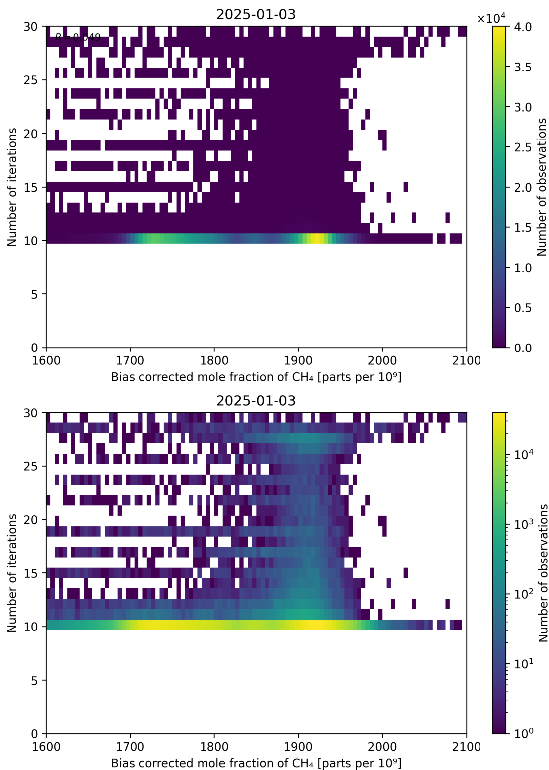
Figure 67: Scatter density plot of “Bias corrected mole fraction of \text{CH}_4 ” against “Number of iterations” for 2025-01-02 to 2025-01-04.
