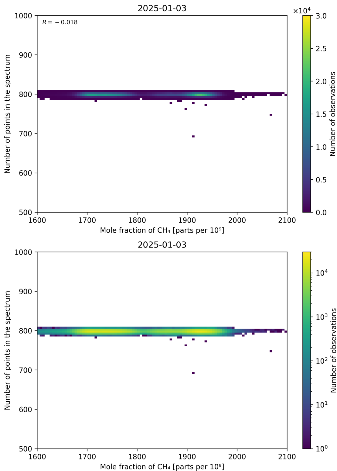
Figure 77: Scatter density plot of “Mole fraction of CH 4 ” against “Number of points in the spectrum” for 2025-01-02 to 2025-01-04.
