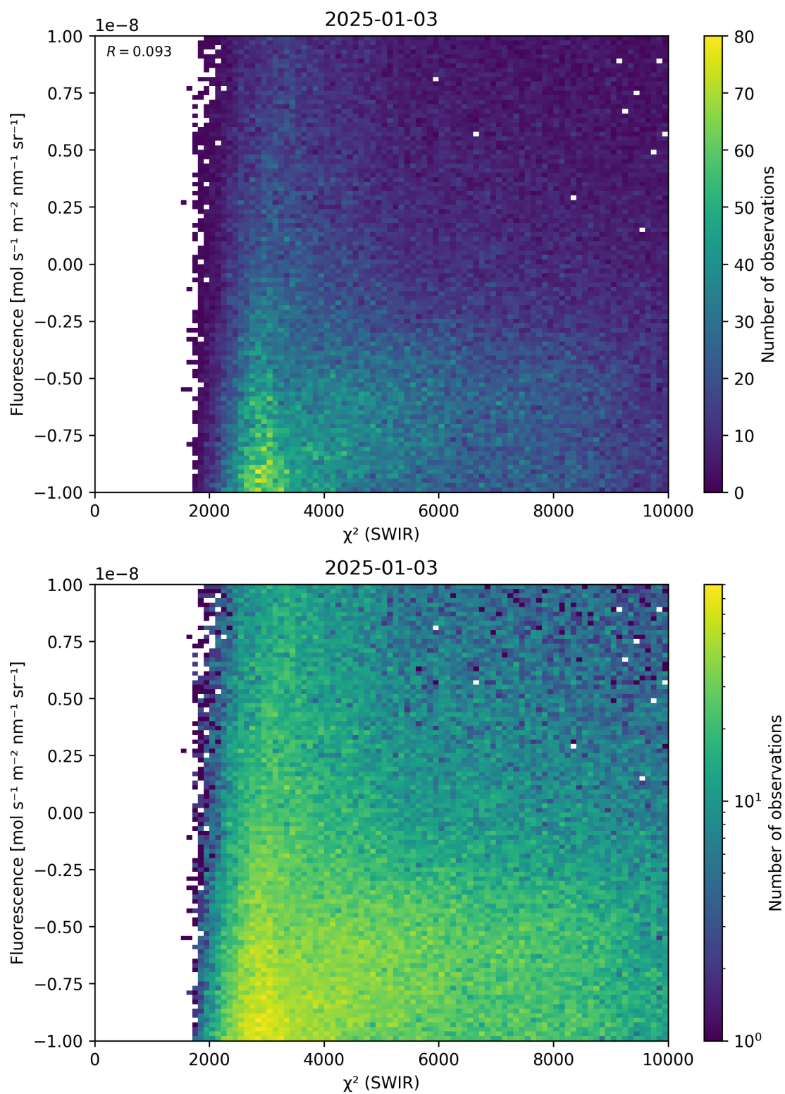
Figure 49: Scatter density plot of “ \chi^2 (SWIR)” against “Fluorescence” for 2025-01-02 to 2025-01-04.
