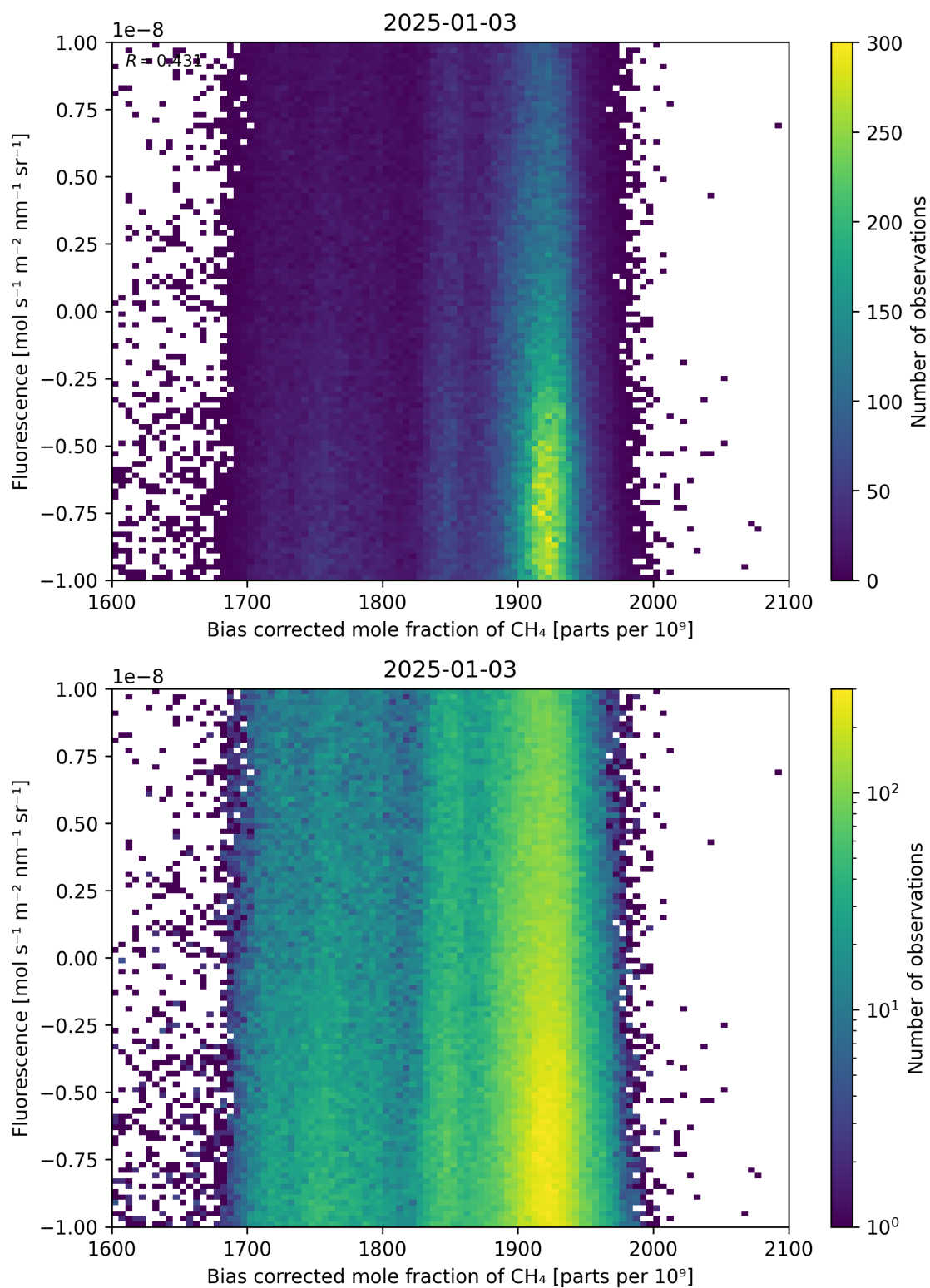
Figure 66: Scatter density plot of “Bias corrected mole fraction of \text{CH}_4 ” against “Fluorescence” for 2025-01-02 to 2025-01-04.
