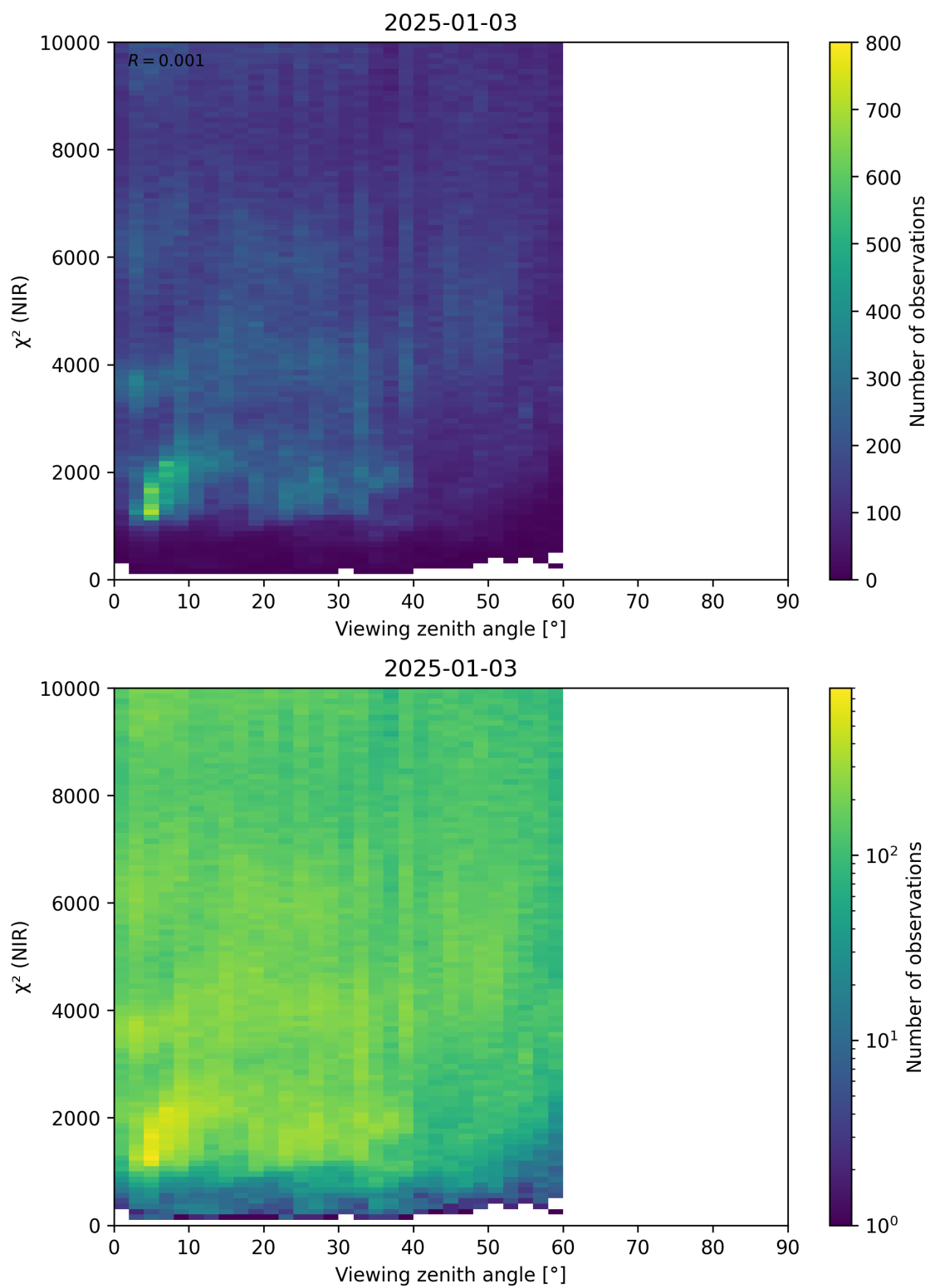
Figure 105: Scatter density plot of “Viewing zenith angle” against “ \chi^2 (NIR)” for 2025-01-02 to 2025-01-04.
