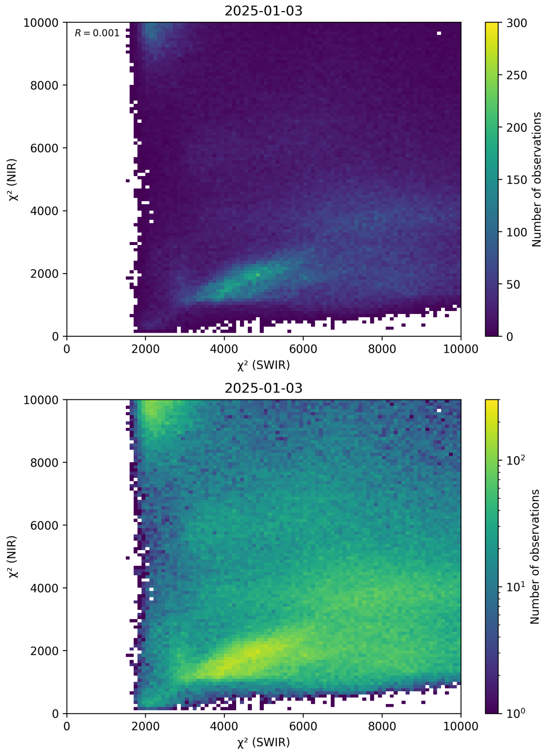
Figure 47: Scatter density plot of “ \chi^2 (SWIR)” against “ \chi^2 (NIR)” for 2025-01-02 to 2025-01-04.
