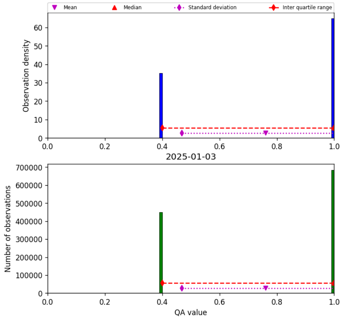
Figure 22: Histogram of “QA value” for 2025-01-02 to 2025-01-04
