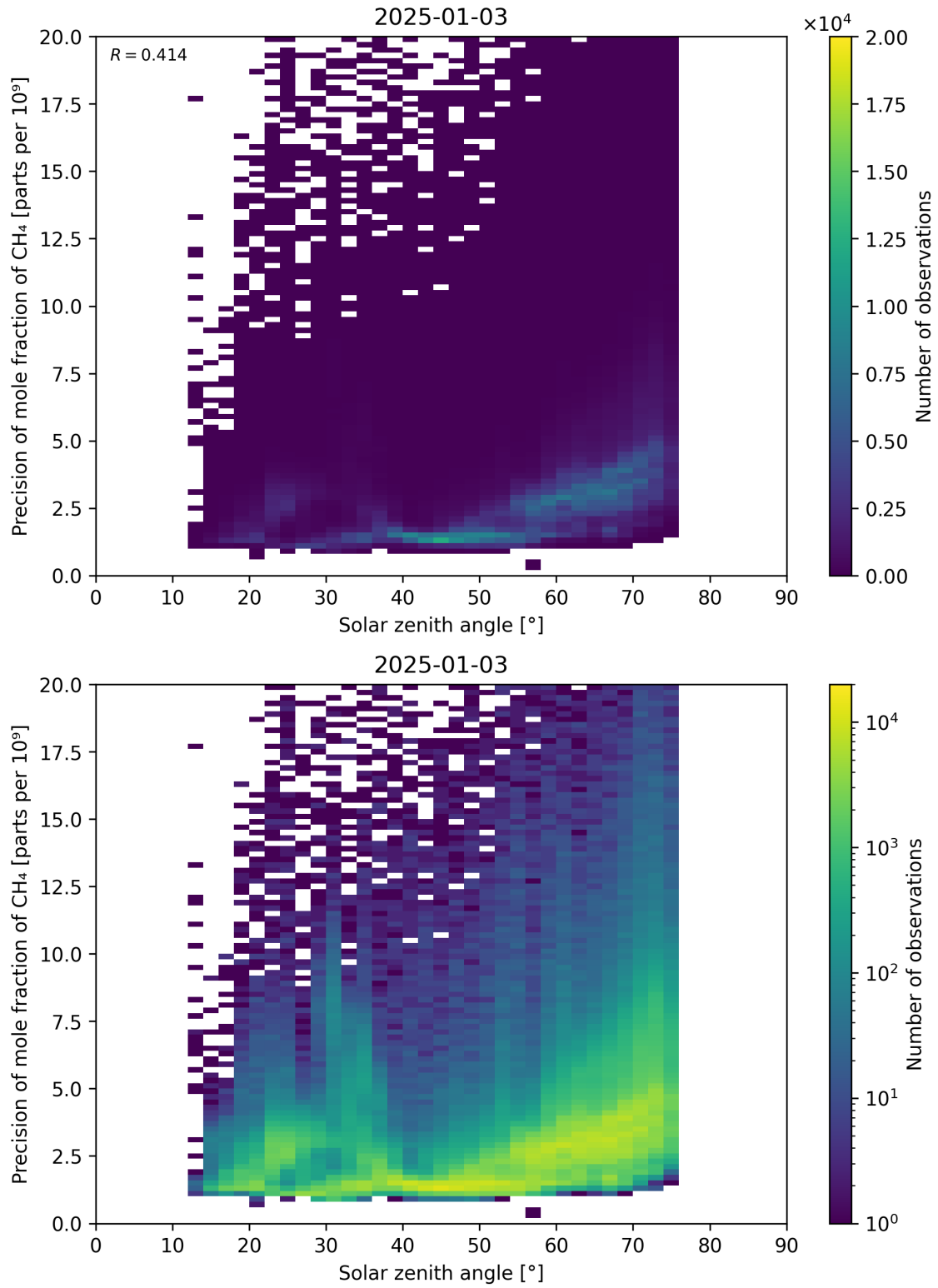
Figure 101: Scatter density plot of “Solar zenith angle” against “Precision of mole fraction of CH 4 ” for 2025-01-02 to 2025-01-04.
