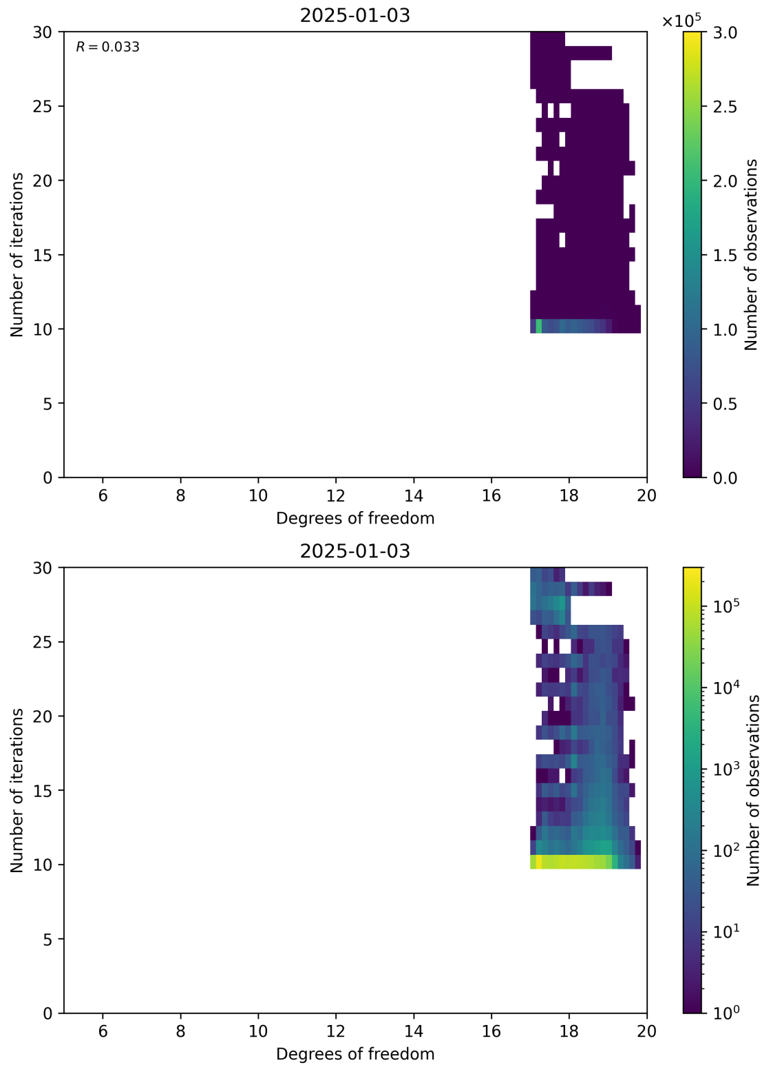
Figure 52: Scatter density plot of “Degrees of freedom” against “Number of iterations” for 2025-01-02 to 2025-01-04.
