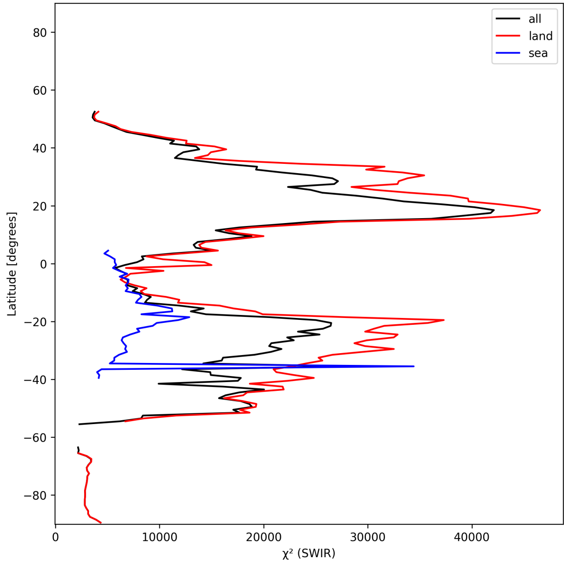
Figure 17: Zonal average of “ \chi^2 (SWIR)” for 2025-01-02 to 2025-01-04.
