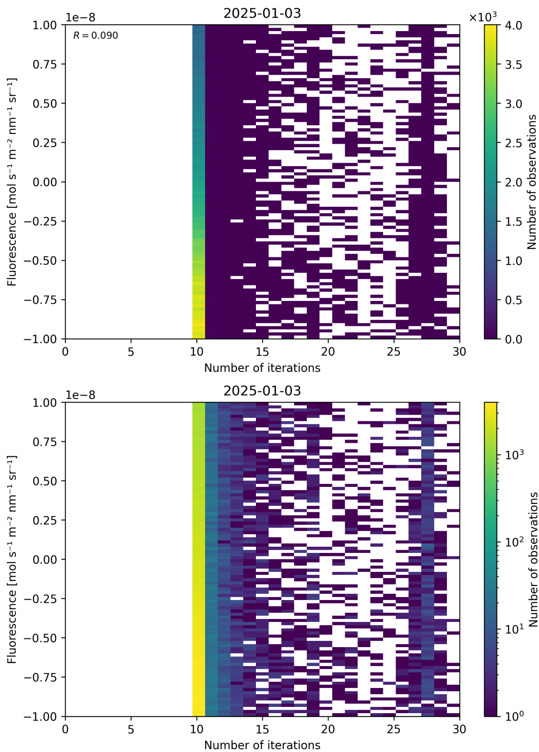
Figure 87: Scatter density plot of “Number of iterations” against “Fluorescence” for 2025-01-02 to 2025-01-04.
