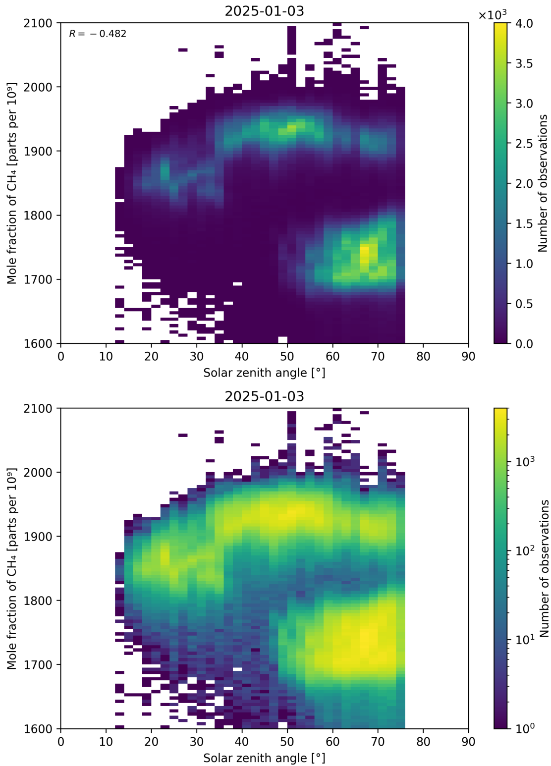
Figure 99: Scatter density plot of “Solar zenith angle” against “Mole fraction of CH 4 ” for 2025-01-02 to 2025-01-04.
