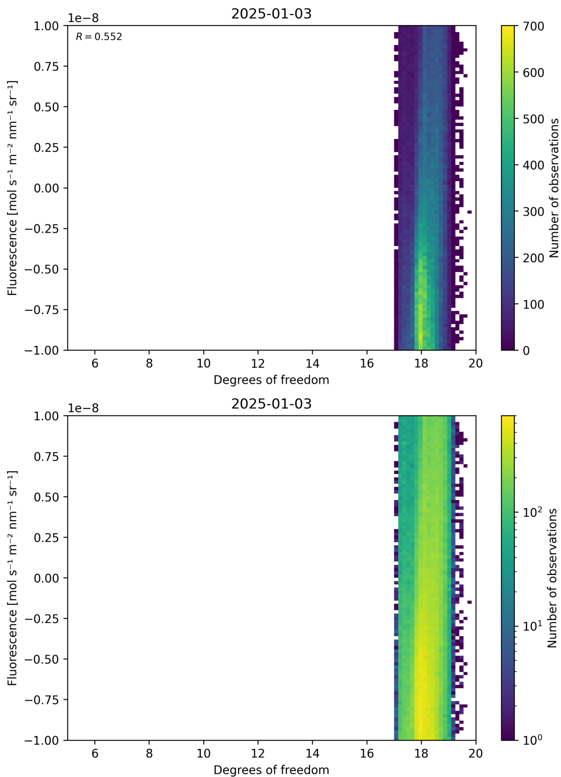
Figure 51: Scatter density plot of “Degrees of freedom” against “Fluorescence” for 2025-01-02 to 2025-01-04.
