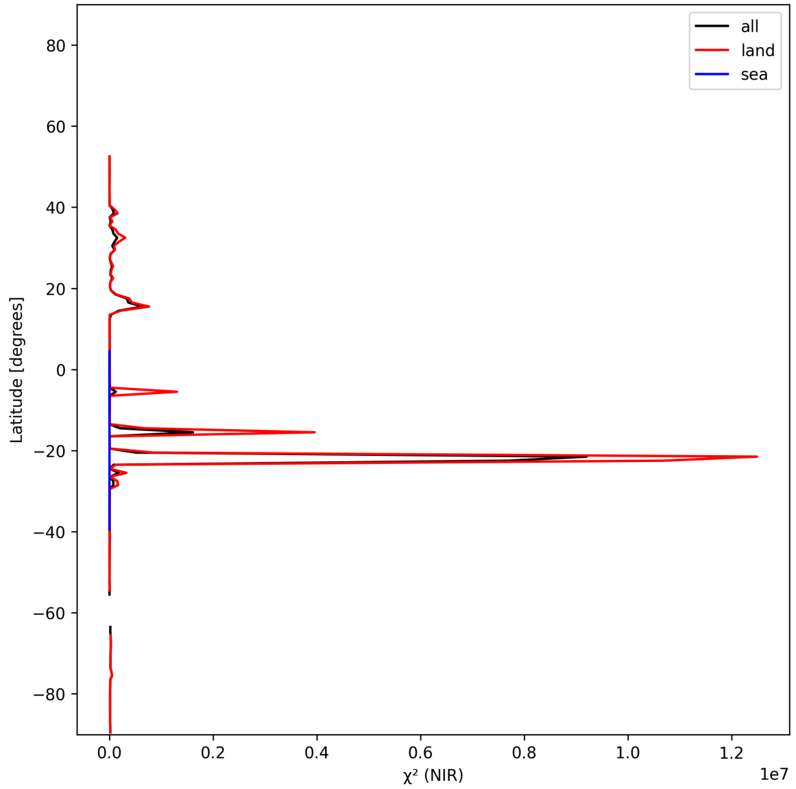
Figure 18: Zonal average of “ \chi^2 (NIR)” for 2025-01-02 to 2025-01-04.
