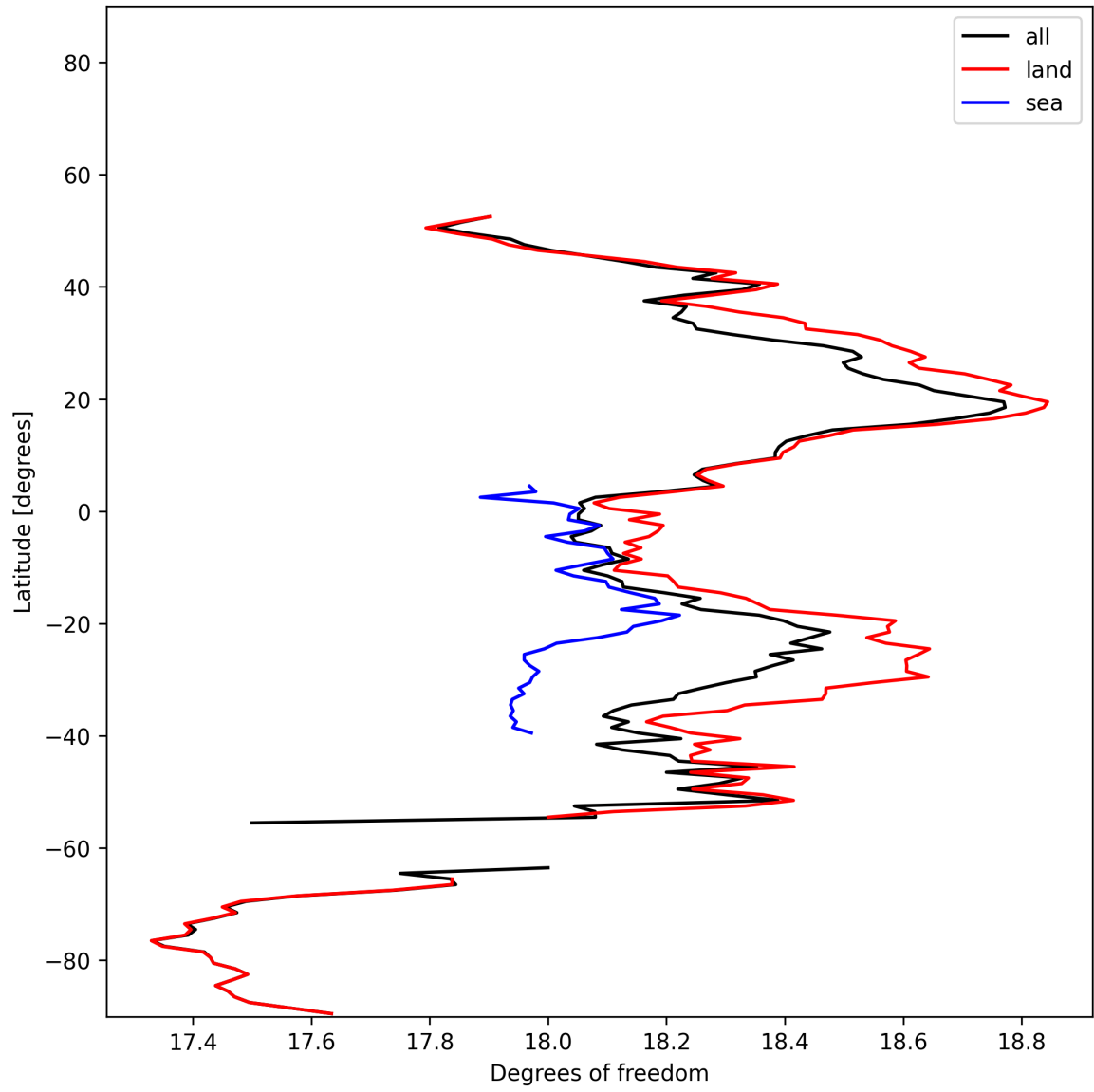
Figure 19: Zonal average of “Degrees of freedom” for 2025-01-02 to 2025-01-04.
