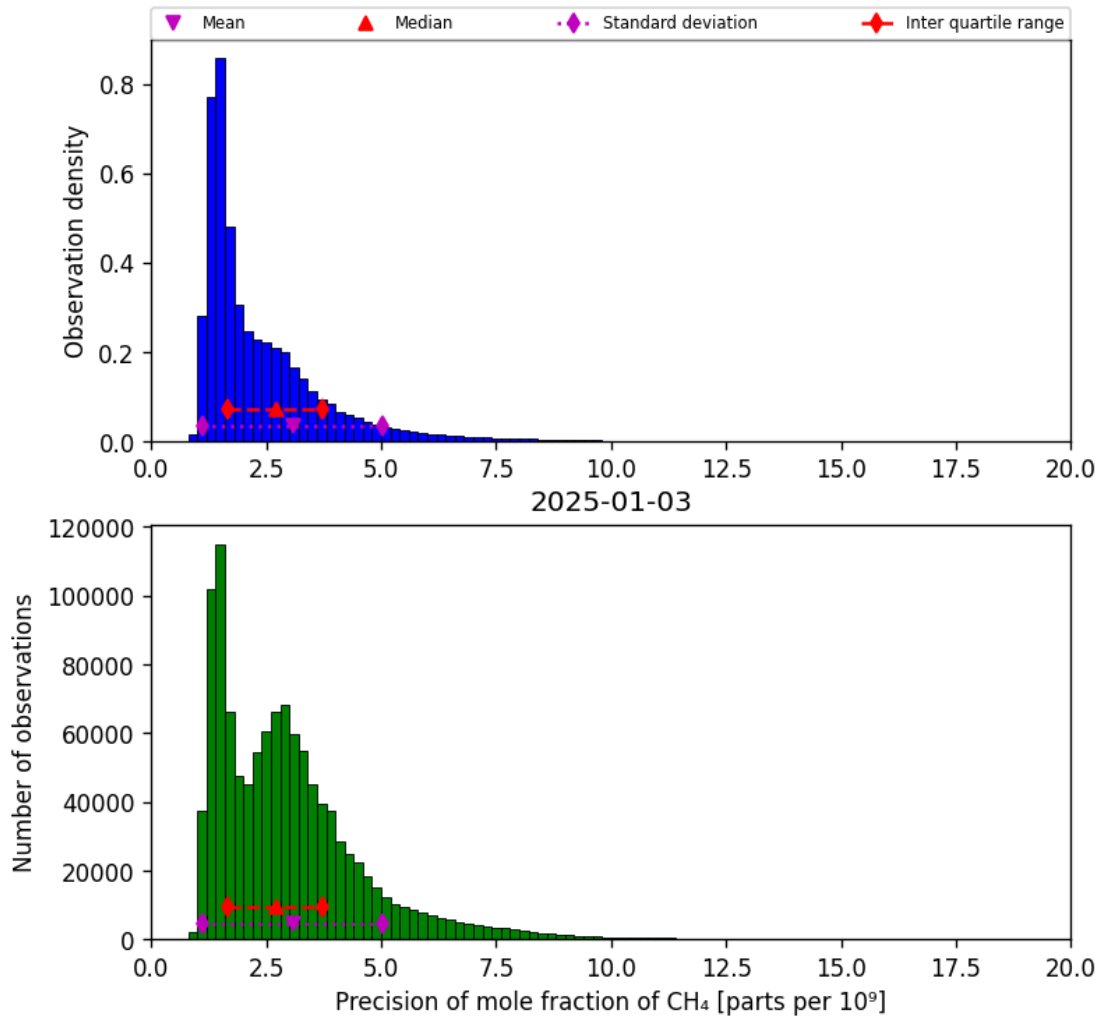
Figure 24: Histogram of “Precision of mole fraction of CH 4 ” for 2025-01-02 to 2025-01-04
