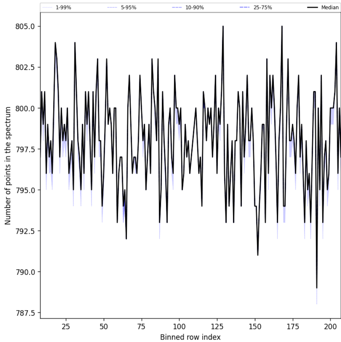
Figure 37: Along track statistics of “Number of points in the spectrum” for 2025-01-02 to 2025-01-04
