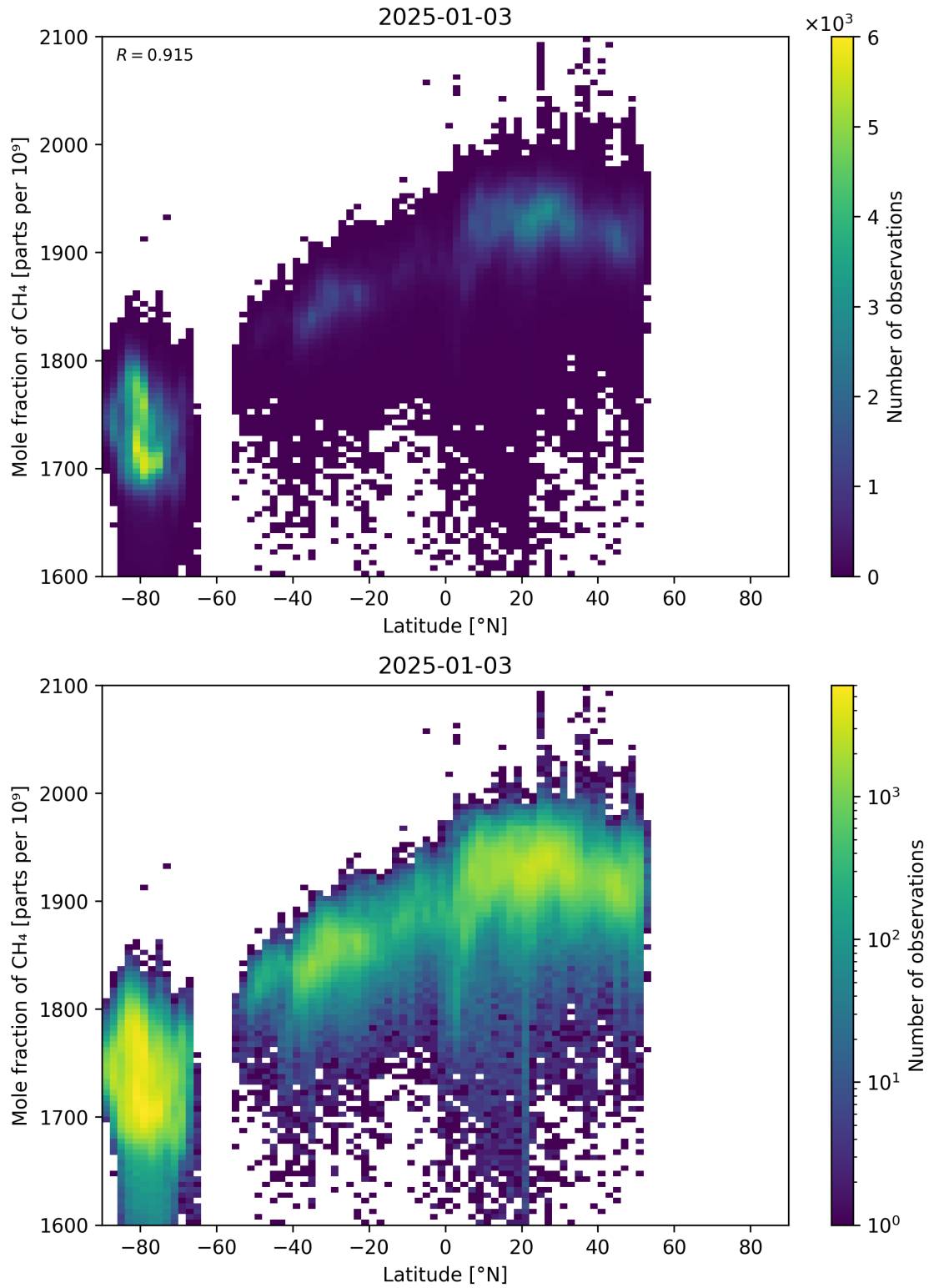
Figure 57: Scatter density plot of “Latitude” against “Mole fraction of CH 4 ” for 2025-01-02 to 2025-01-04.
