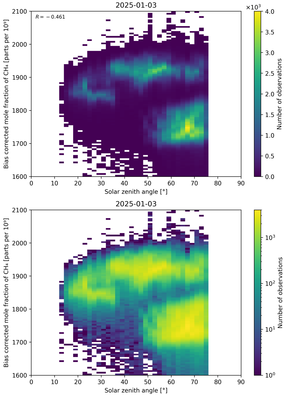
Figure 100: Scatter density plot of “Solar zenith angle” against “Bias corrected mole fraction of CH 4 ” for 2025-01-02 to 2025-01-04.
