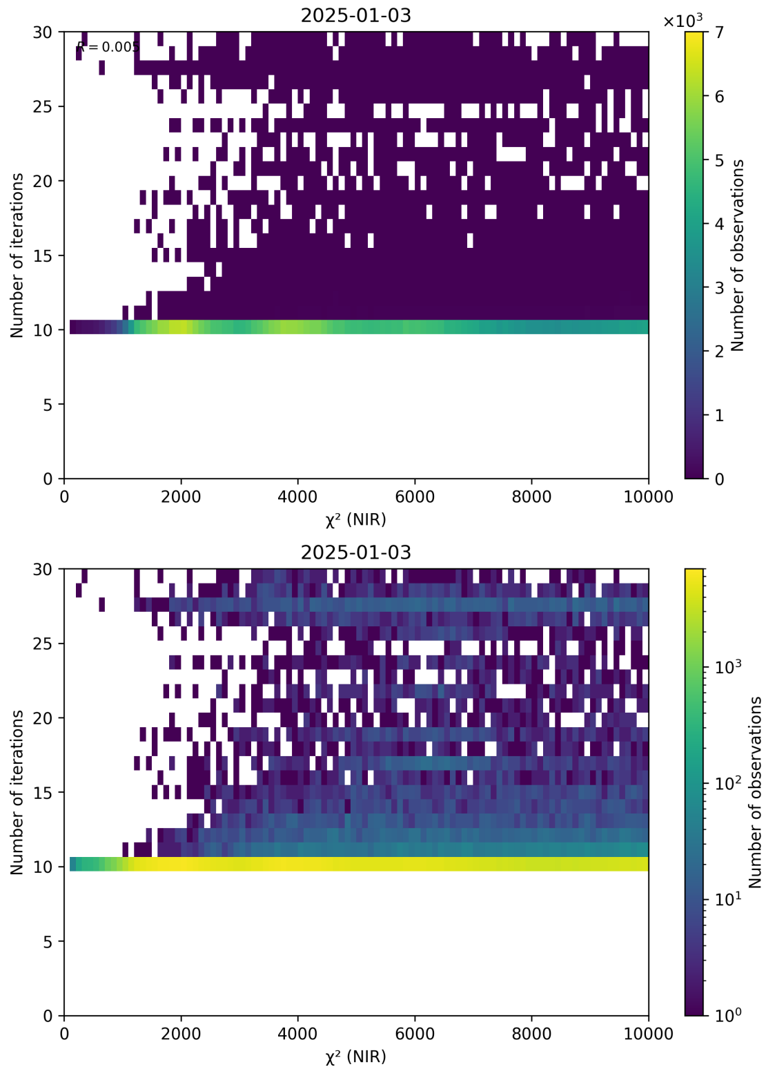
Figure 46: Scatter density plot of “ \chi^2 (NIR)” against “Number of iterations” for 2025-01-02 to 2025-01-04.
