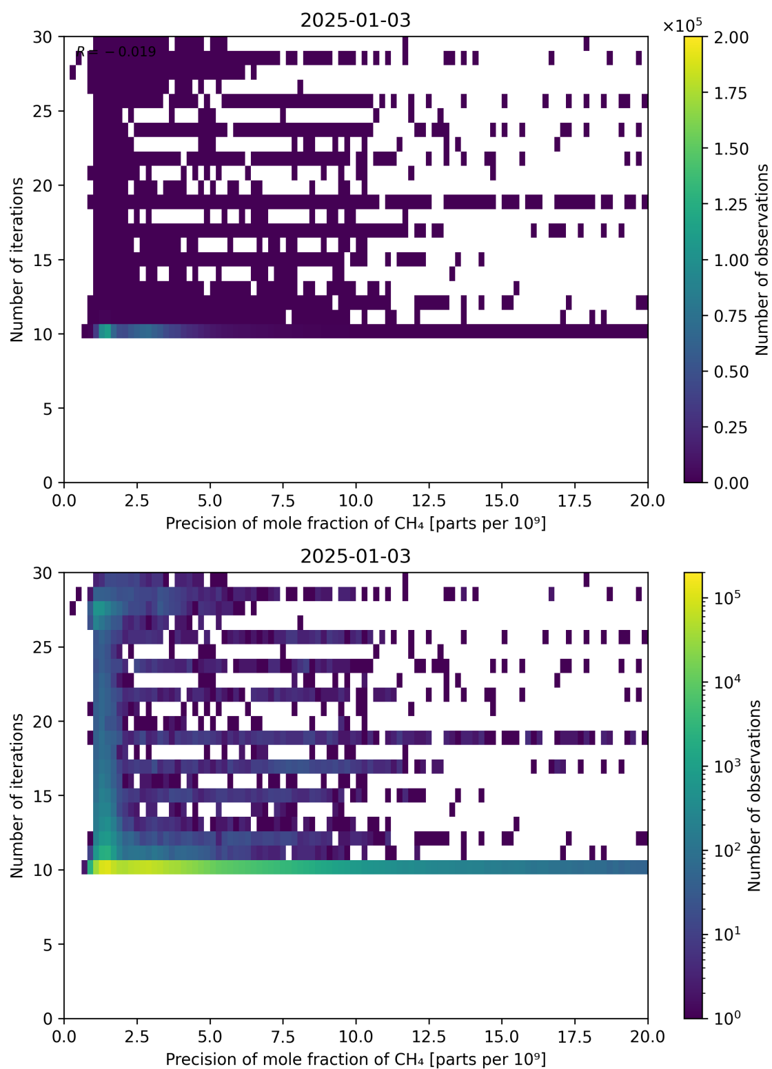
Figure 83: Scatter density plot of “Precision of mole fraction of CH 4 ” against “Number of iterations” for 2025-01-02 to 2025-01-04.
