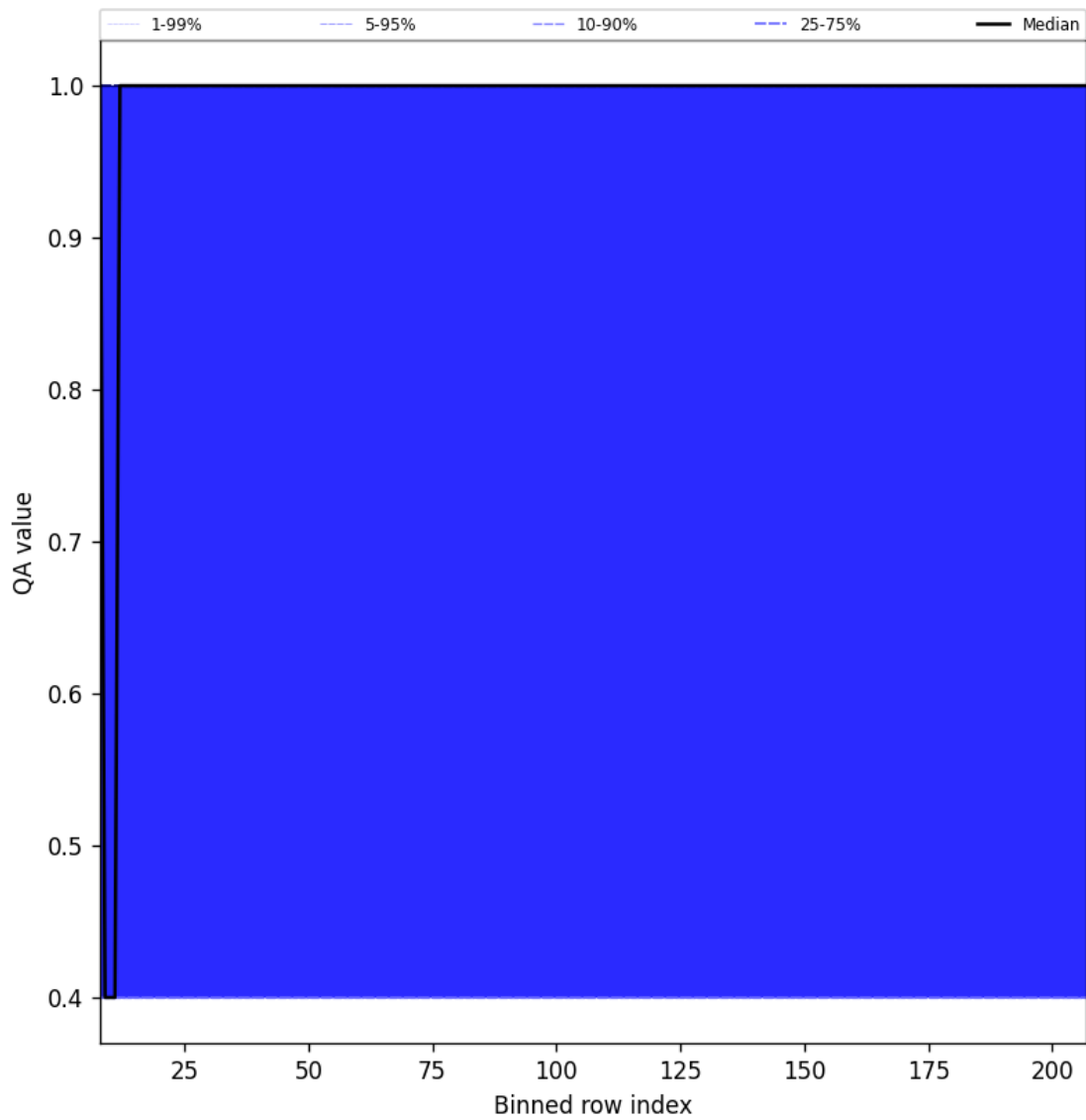
Figure 33: Along track statistics of “QA value” for 2025-01-02 to 2025-01-04
