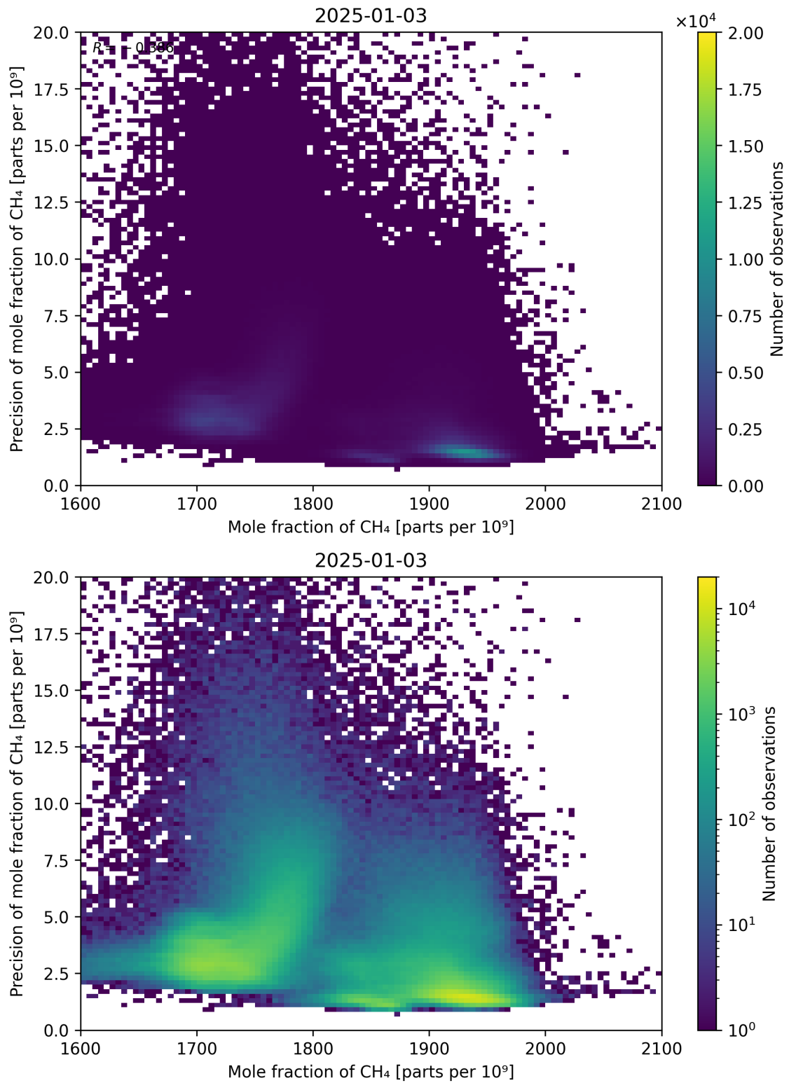
Figure 75: Scatter density plot of “Mole fraction of CH 4 ” against “Precision of mole fraction of CH 4 ” for 2025-01-02 to 2025-01-04.
