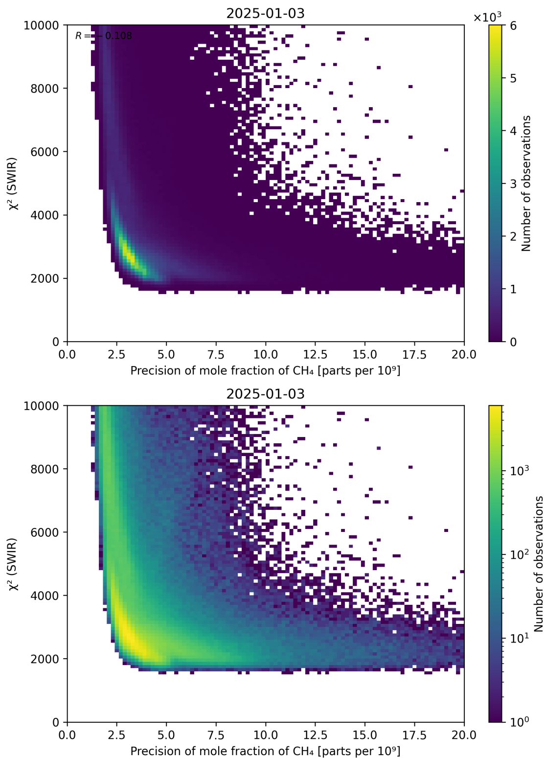
Figure 79: Scatter density plot of “Precision of mole fraction of \text{CH}_4 ” against “ \chi^2 (SWIR)” for 2025-01-02 to 2025-01-04.
