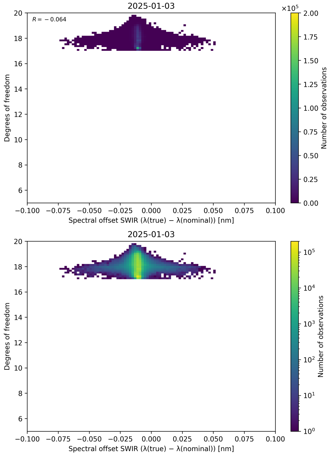
Figure 119: Scatter density plot of “Spectral offset SWIR ( \lambda_{\text{true}} - \lambda_{\text{nominal}} )” against “Degrees of freedom” for 2025-01-02 to 2025-01-04.
