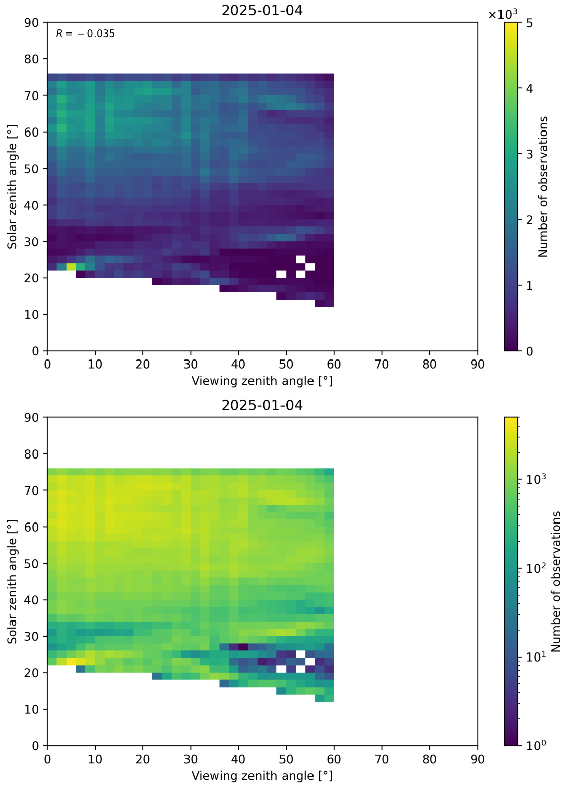
Figure 115: Scatter density plot of “Viewing zenith angle” against “Solar zenith angle” for 2025-01-03 to 2025-01-05.
