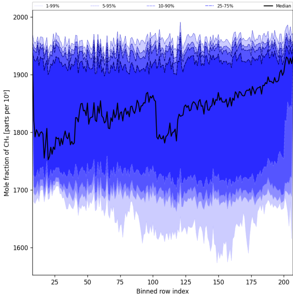
Figure 34: Along track statistics of “Mole fraction of CH 4 ” for 2025-01-03 to 2025-01-05
