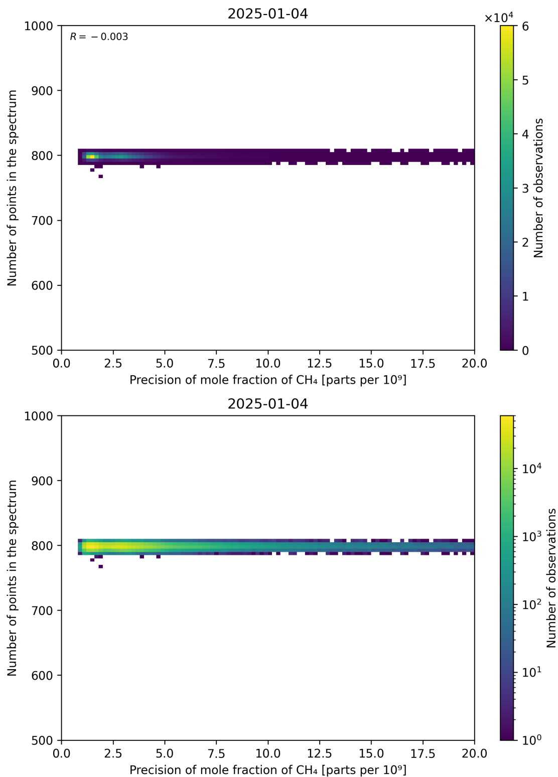
Figure 84: Scatter density plot of “Precision of mole fraction of CH 4 ” against “Number of points in the spectrum” for 2025-01-03 to 2025-01-05.
