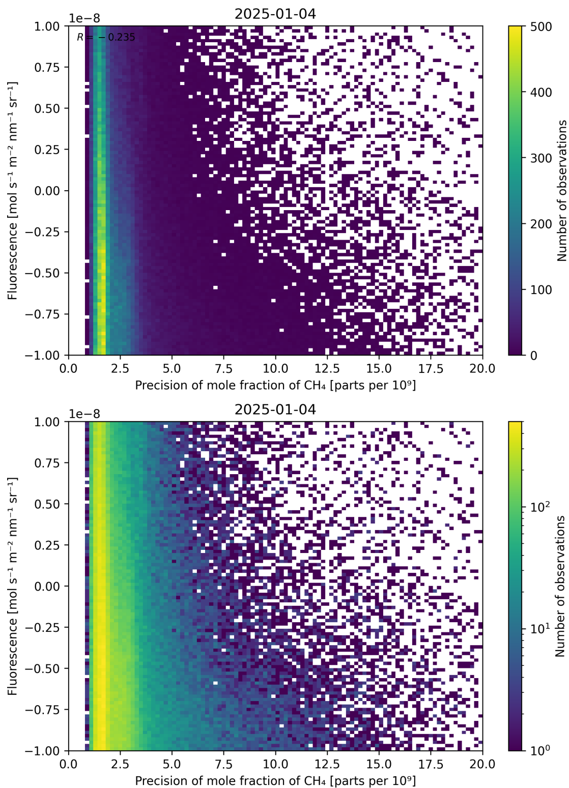
Figure 81: Scatter density plot of “Precision of mole fraction of \text{CH}_4 ” against “Fluorescence” for 2025-01-03 to 2025-01-05.
