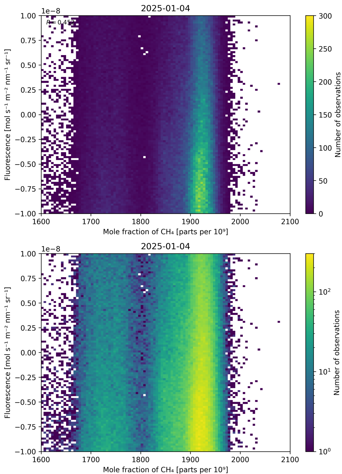
Figure 73: Scatter density plot of “Mole fraction of \text{CH}_4 ” against “Fluorescence” for 2025-01-03 to 2025-01-05.
