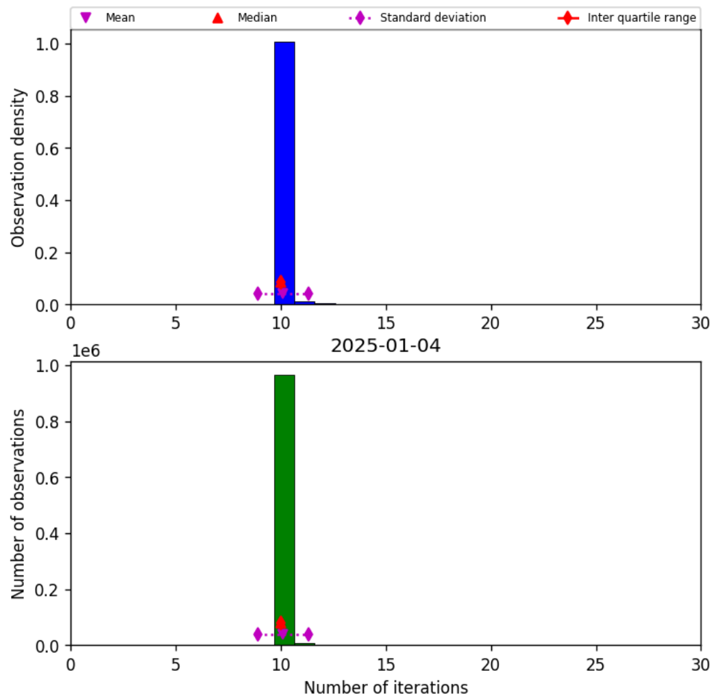
Figure 31: Histogram of “Number of iterations” for 2025-01-03 to 2025-01-05
