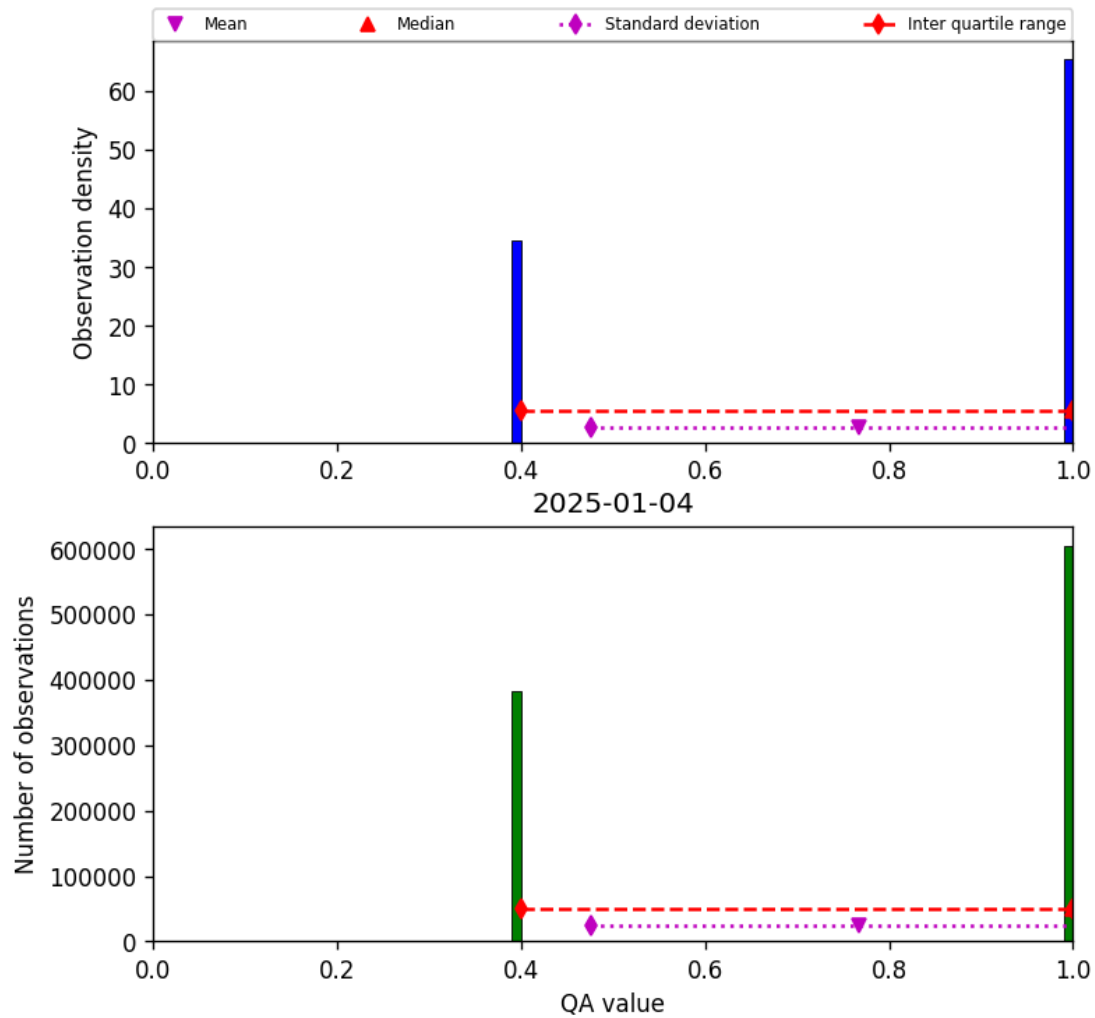
Figure 22: Histogram of “QA value” for 2025-01-03 to 2025-01-05
