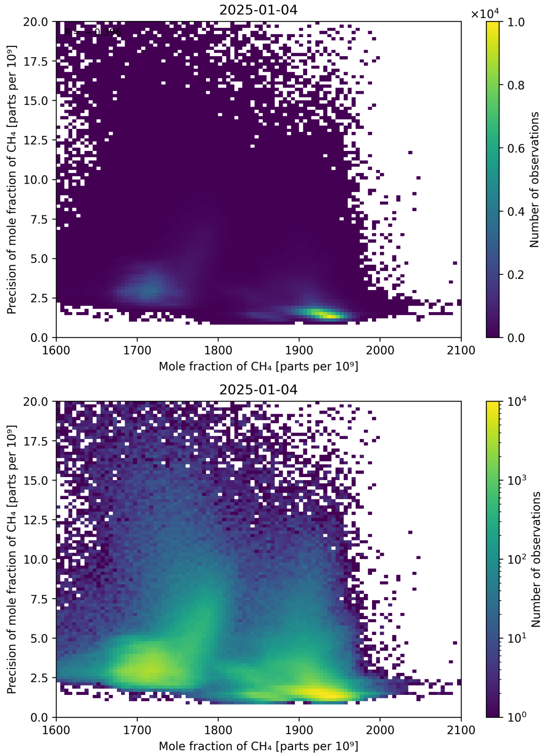
Figure 75: Scatter density plot of “Mole fraction of CH 4 ” against “Precision of mole fraction of CH 4 ” for 2025-01-03 to 2025-01-05.
