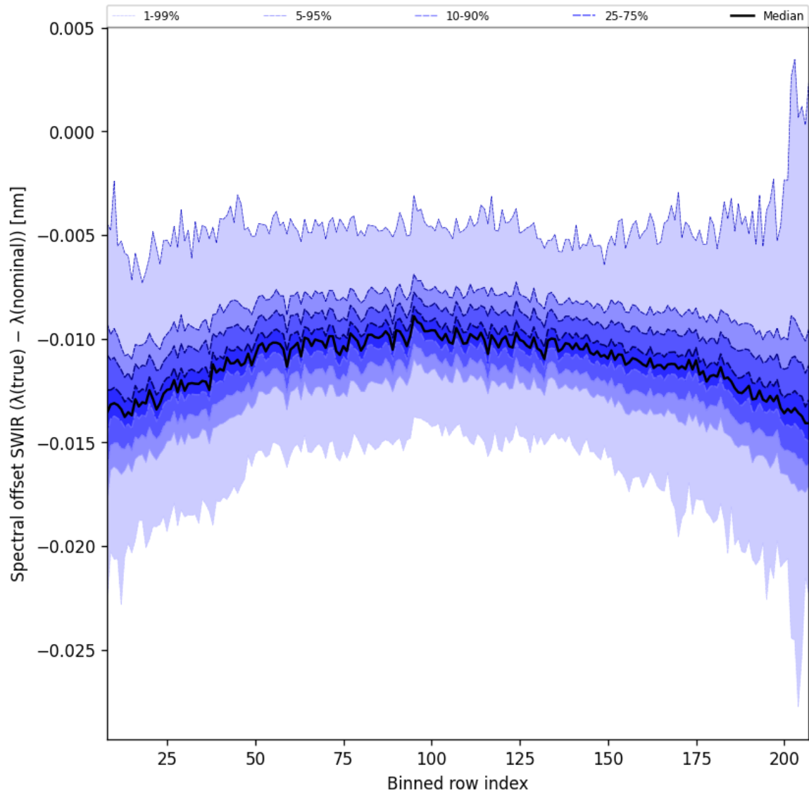
Figure 38: Along track statistics of “Spectral offset SWIR ( \lambda_{\text{true}} - \lambda_{\text{nominal}} )” for 2025-01-03 to 2025-01-05
