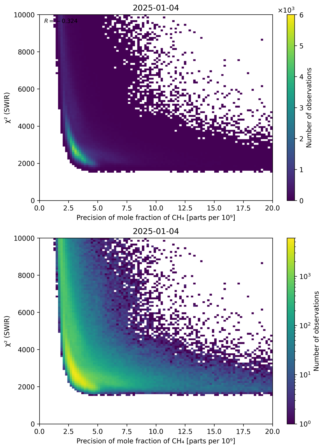
Figure 79: Scatter density plot of “Precision of mole fraction of CH 4 ” against “ \chi^2 (SWIR)” for 2025-01-03 to 2025-01-05.
