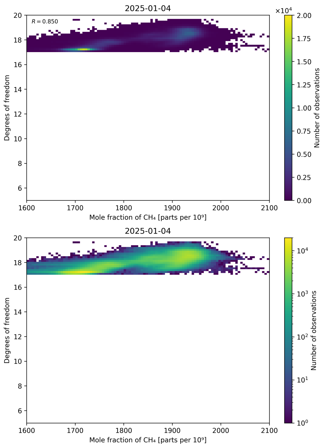
Figure 72: Scatter density plot of “Mole fraction of CH 4 ” against “Degrees of freedom” for 2025-01-03 to 2025-01-05.
