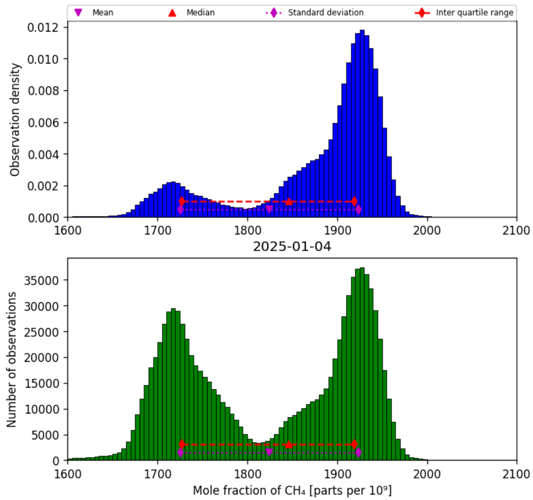
Figure 23: Histogram of “Mole fraction of CH 4 ” for 2025-01-03 to 2025-01-05
