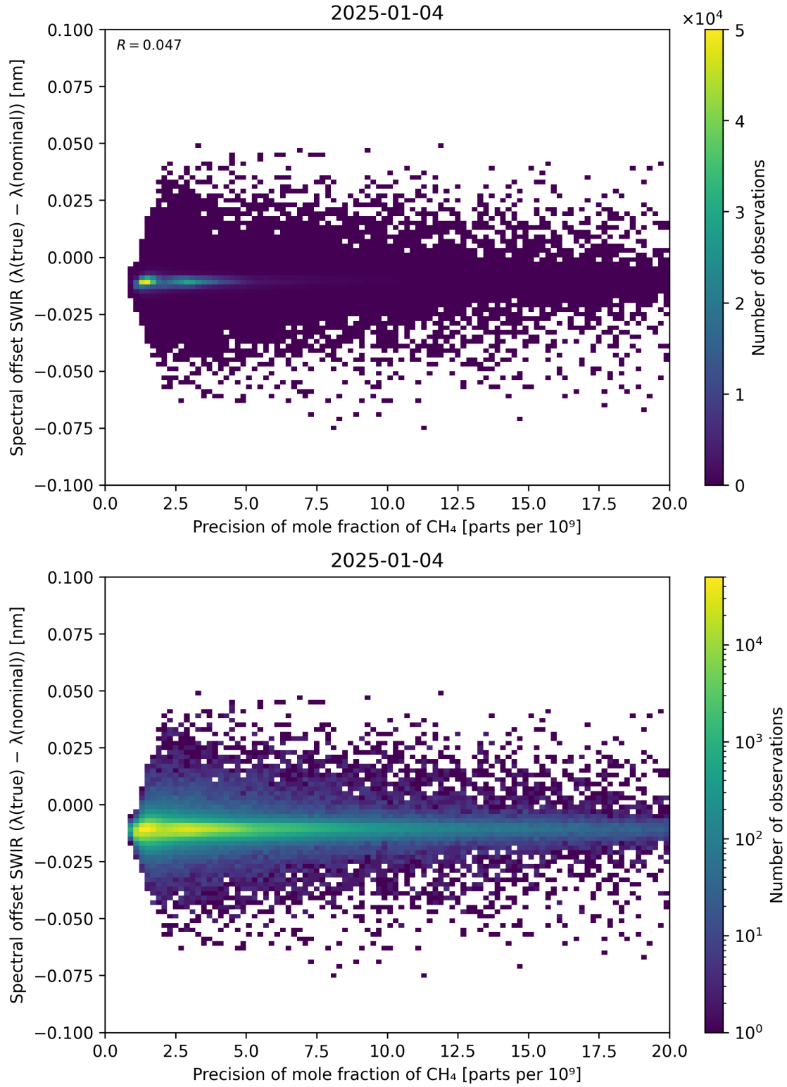
Figure 85: Scatter density plot of “Precision of mole fraction of CH 4 ” against “Spectral offset SWIR ( \lambda_{\text{true}} - \lambda_{\text{nominal}} )” for 2025-01-03 to 2025-01-05.
