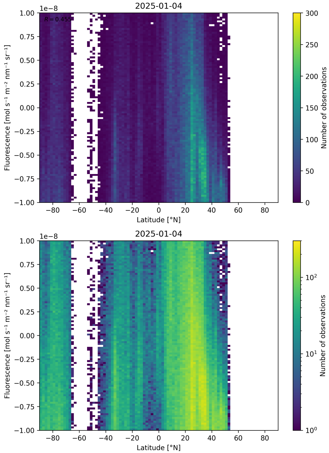
Figure 56: Scatter density plot of “Latitude” against “Fluorescence” for 2025-01-03 to 2025-01-05.
