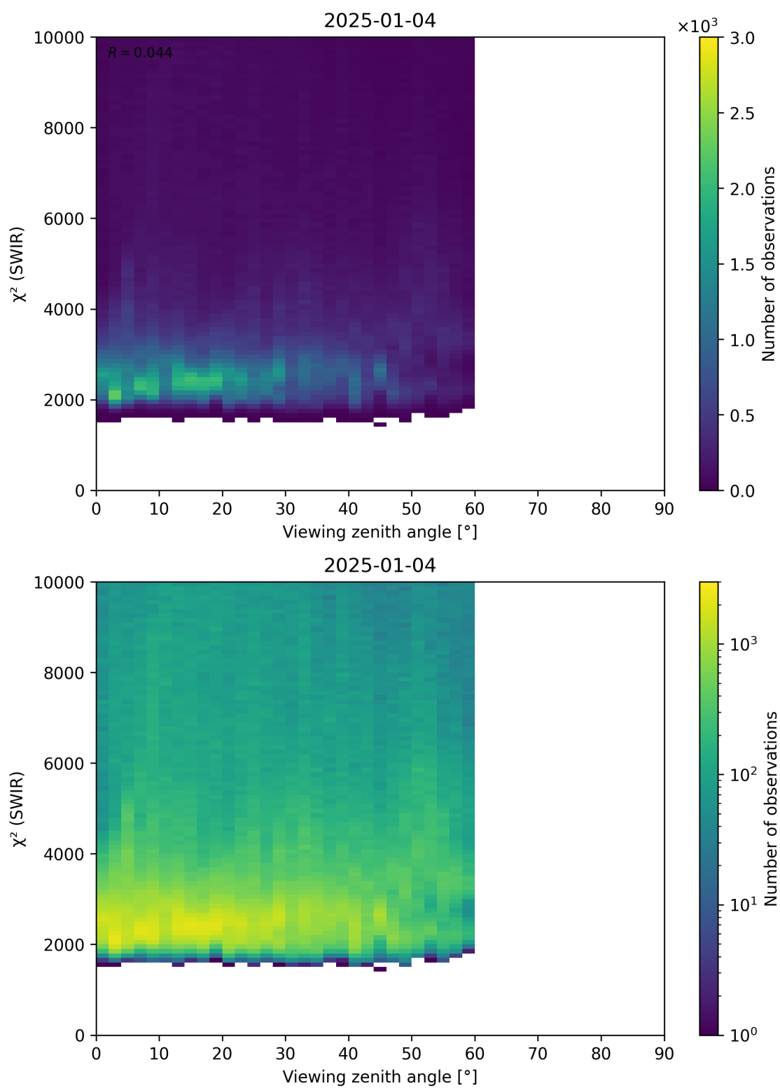
Figure 106: Scatter density plot of “Viewing zenith angle” against “ \chi^2 (SWIR)” for 2025-01-03 to 2025-01-05.
