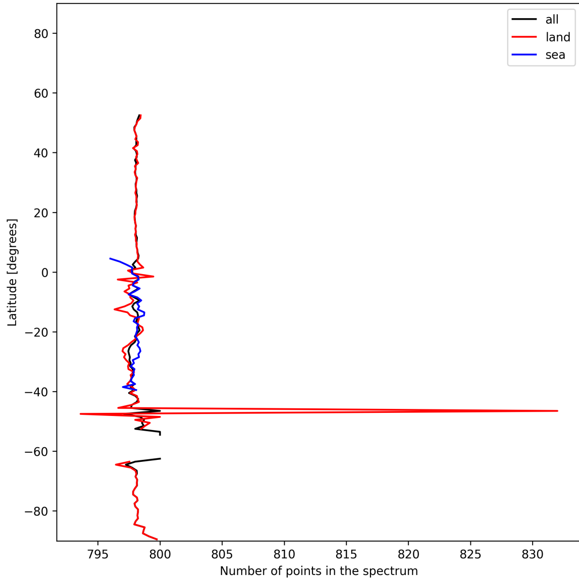
Figure 15: Zonal average of “Number of points in the spectrum” for 2025-01-03 to 2025-01-05.
