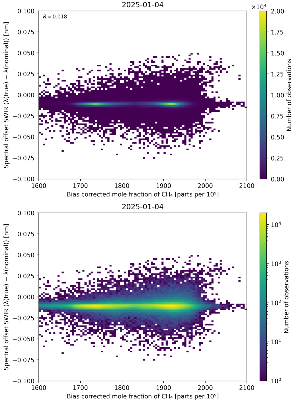
Figure 69: Scatter density plot of “Bias corrected mole fraction of \text{CH}_4 ” against “Spectral offset SWIR ( \lambda_{\text{true}} - \lambda_{\text{nominal}} )” for 2025-01-03 to 2025-01-05.
