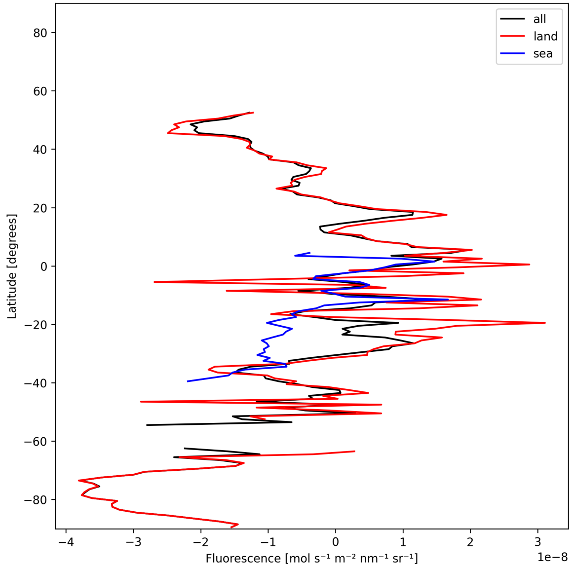
Figure 21: Zonal average of “Fluorescence” for 2025-01-03 to 2025-01-05.
