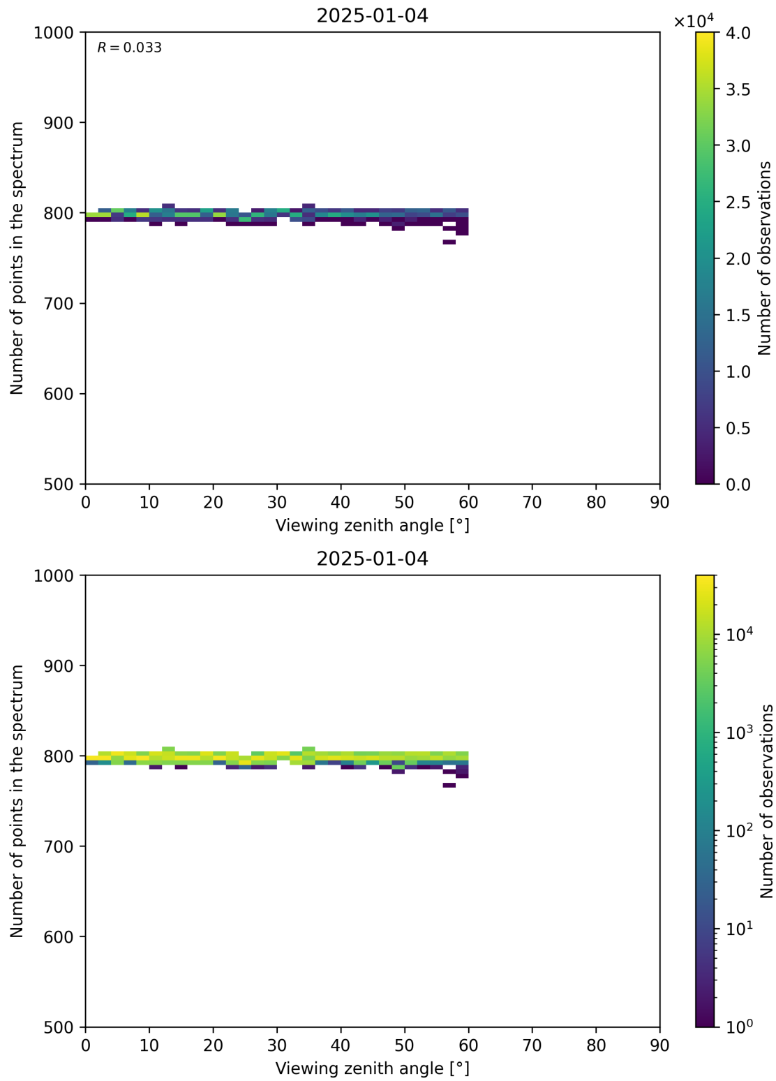
Figure 114: Scatter density plot of “Viewing zenith angle” against “Number of points in the spectrum” for 2025-01-03 to 2025-01-05.
