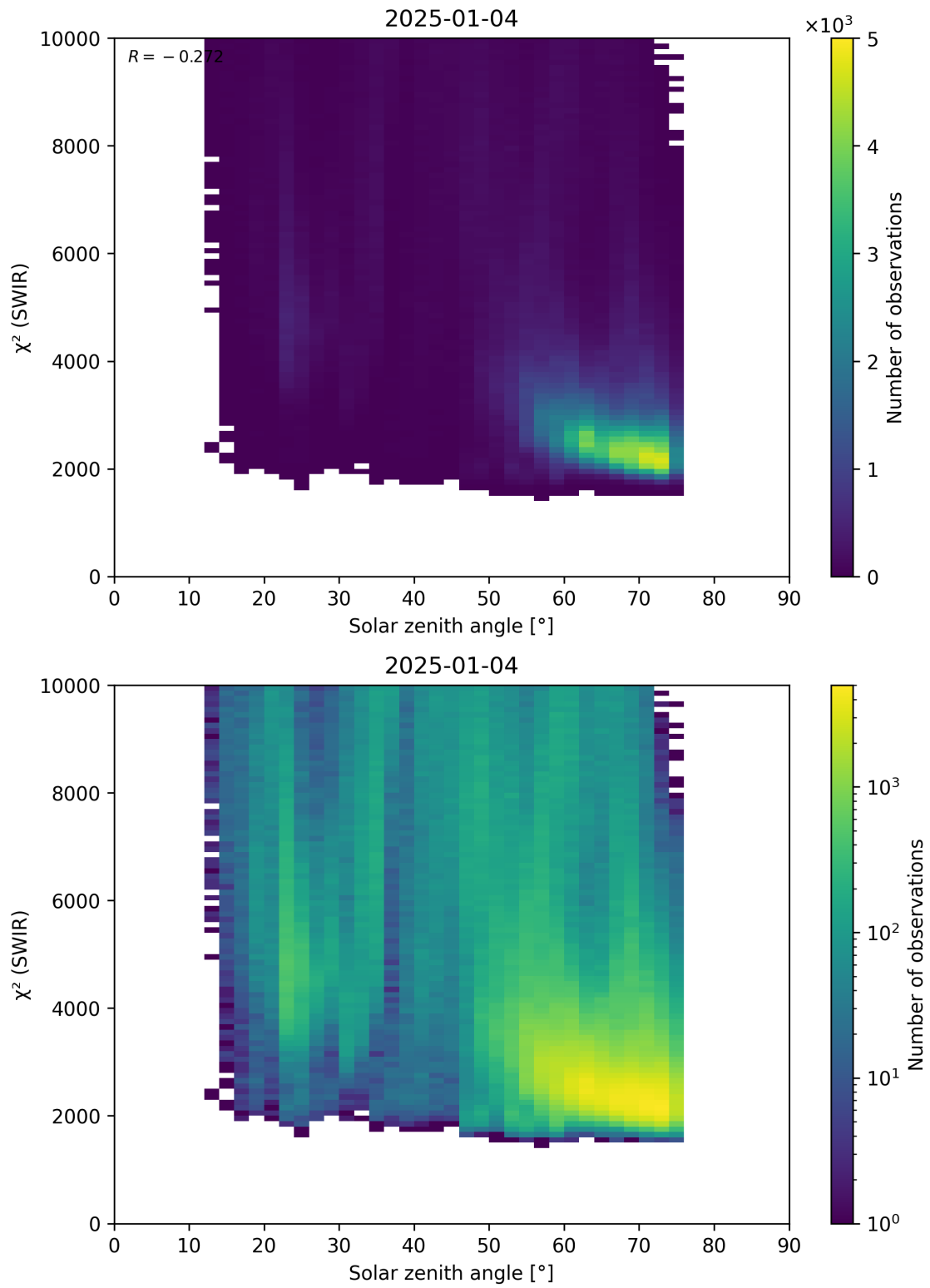
Figure 95: Scatter density plot of “Solar zenith angle” against “ \chi^2 (SWIR)” for 2025-01-03 to 2025-01-05.
