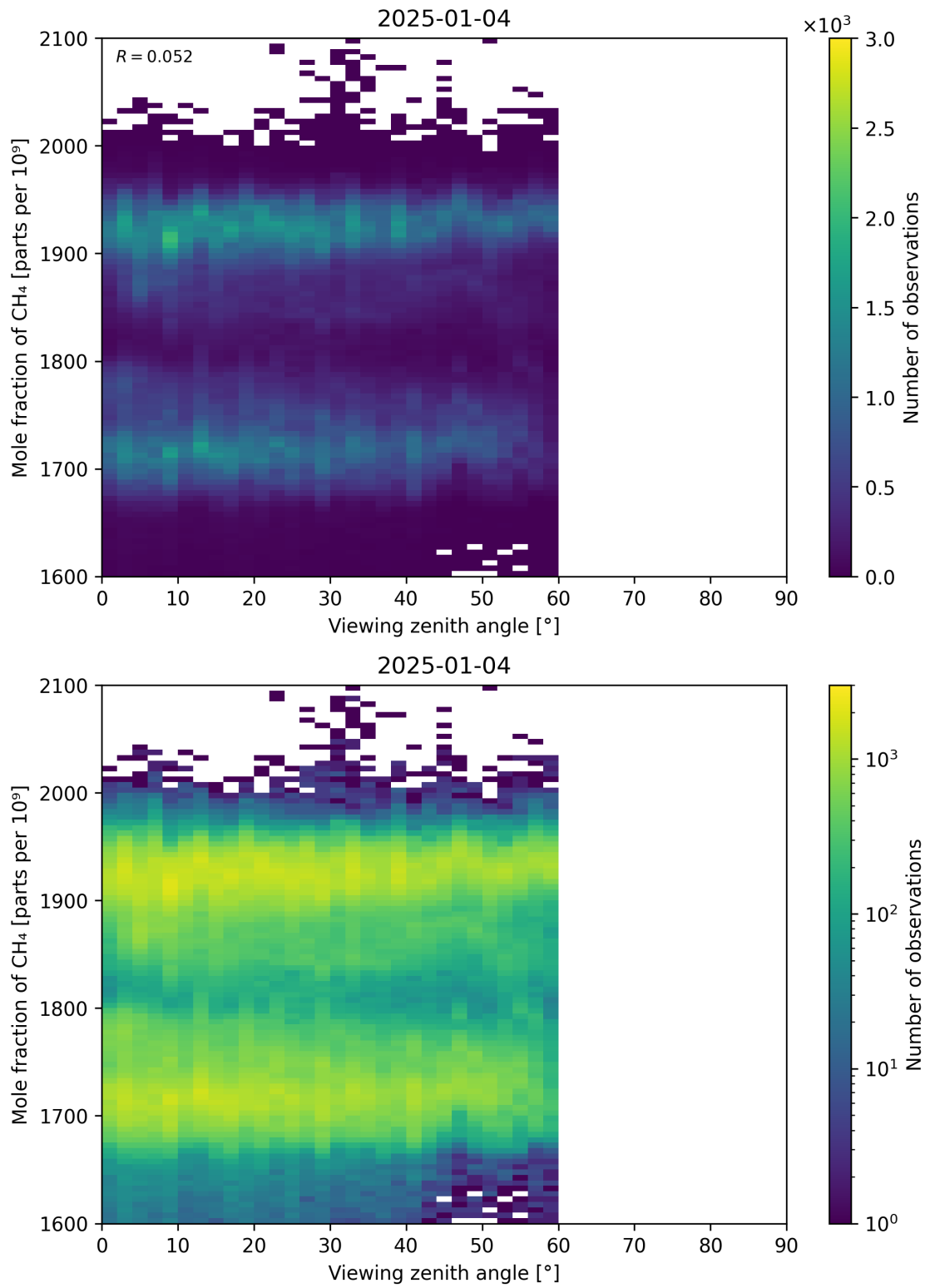
Figure 110: Scatter density plot of “Viewing zenith angle” against “Mole fraction of CH 4 ” for 2025-01-03 to 2025-01-05.
