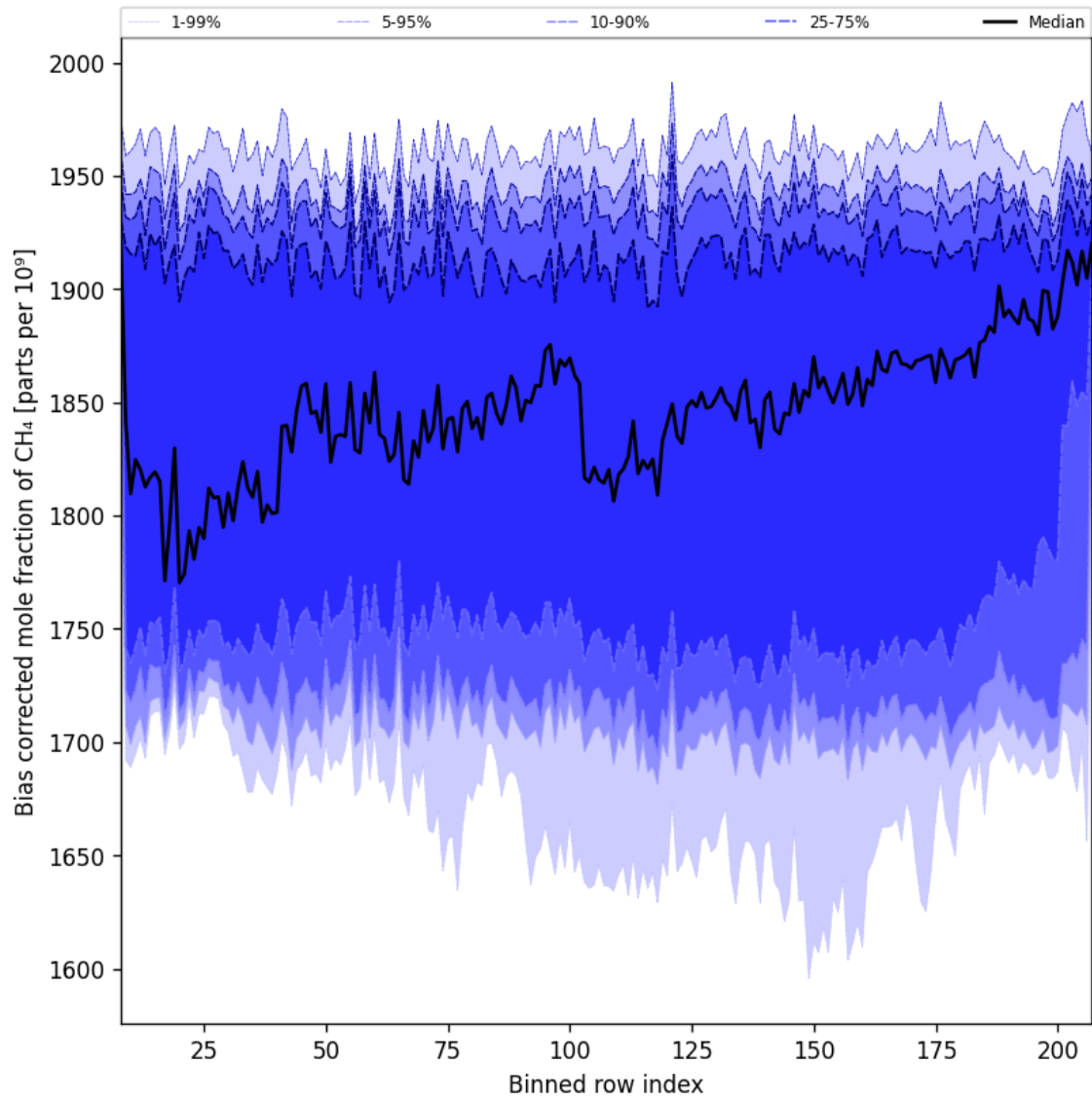
Figure 36: Along track statistics of “Bias corrected mole fraction of CH 4 ” for 2025-01-03 to 2025-01-05
