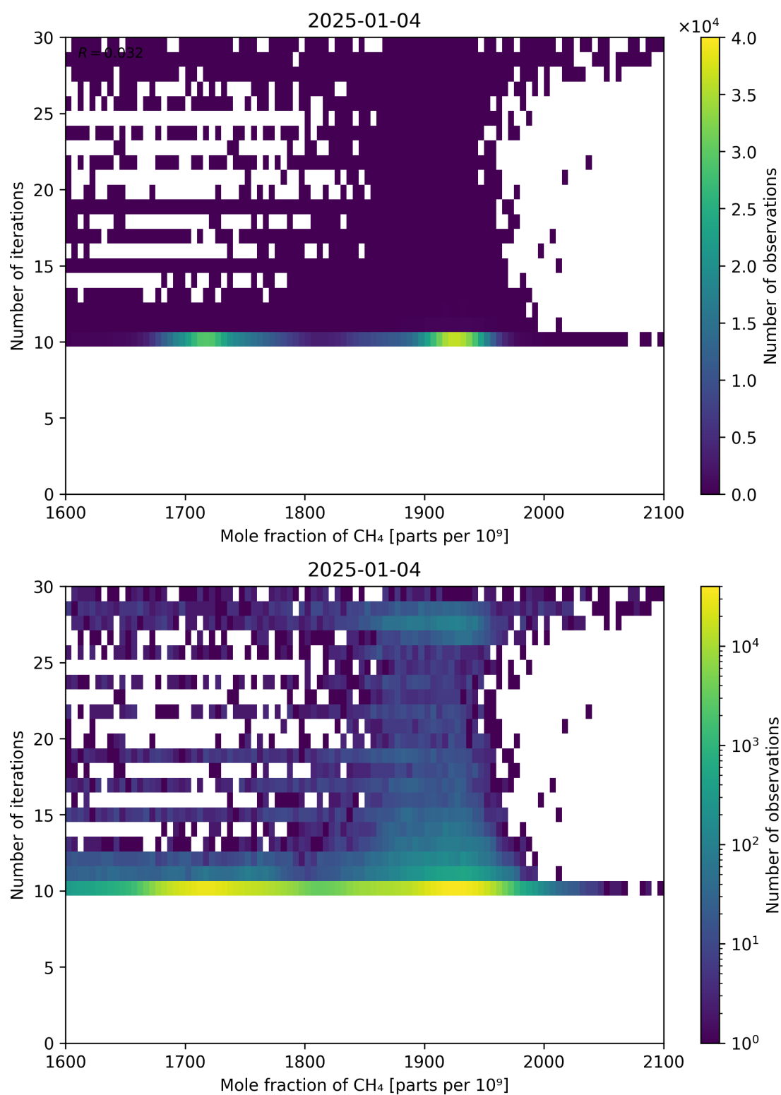
Figure 76: Scatter density plot of “Mole fraction of CH 4 ” against “Number of iterations” for 2025-01-03 to 2025-01-05.
