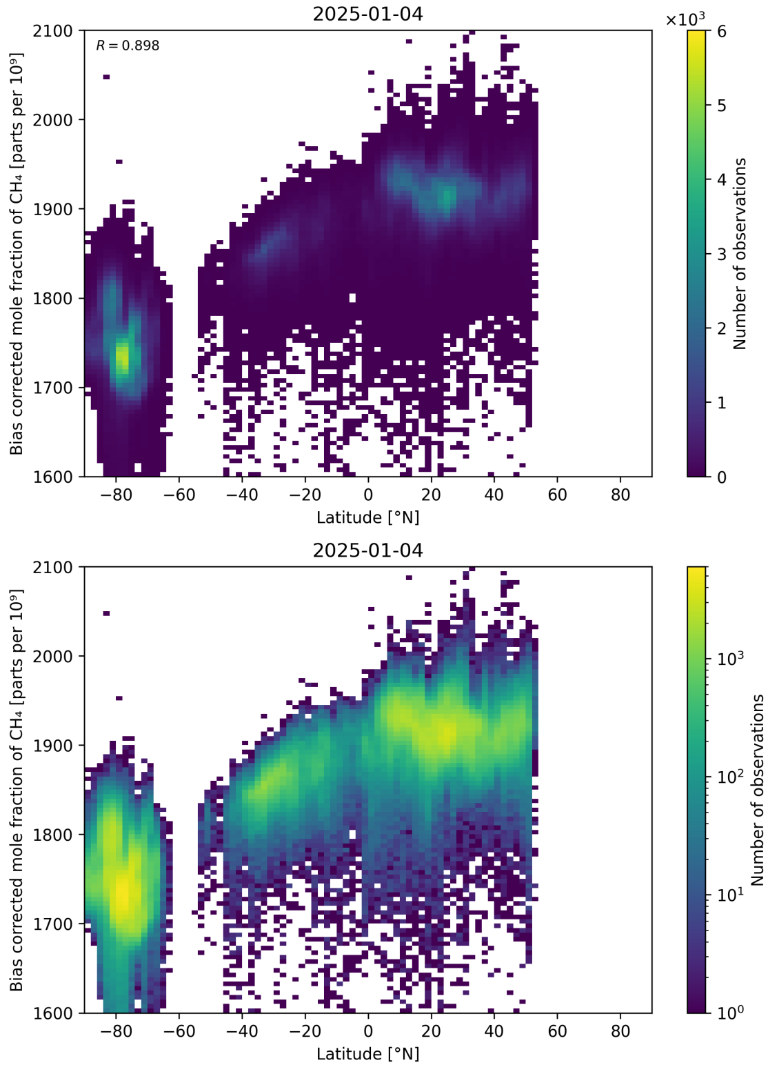
Figure 58: Scatter density plot of “Latitude” against “Bias corrected mole fraction of CH 4 ” for 2025-01-03 to 2025-01-05.
