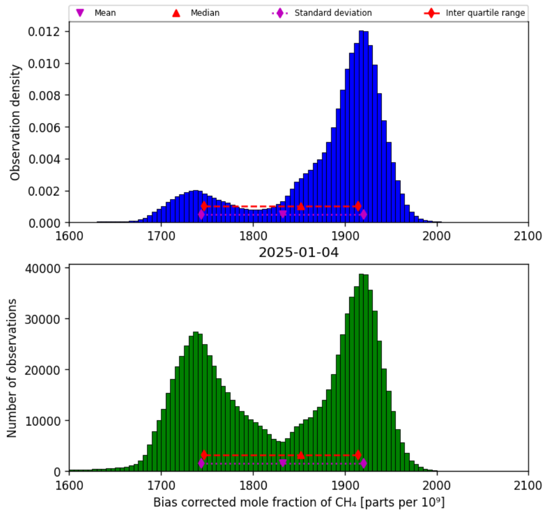
Figure 25: Histogram of “Bias corrected mole fraction of CH 4 ” for 2025-01-03 to 2025-01-05
