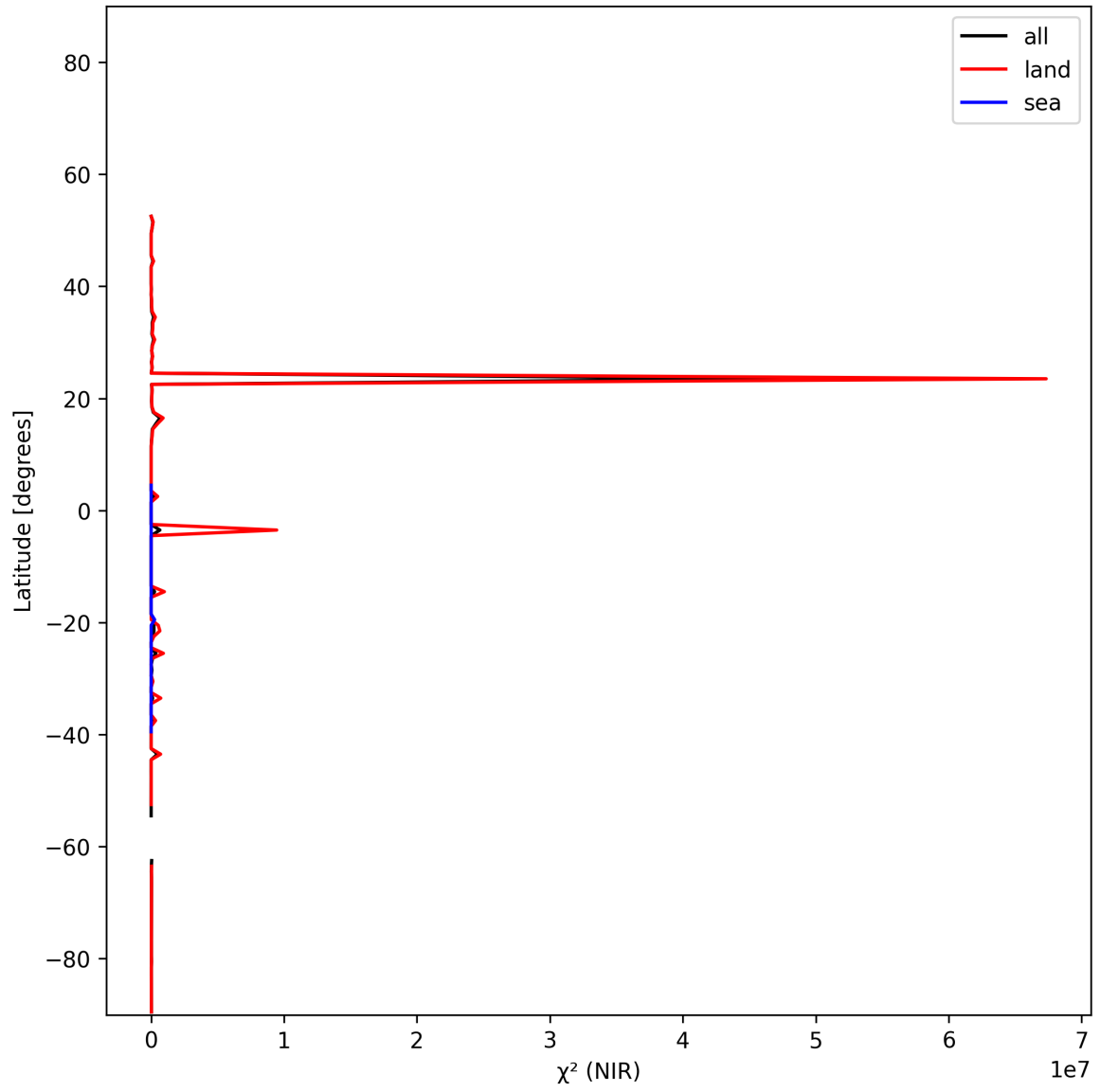
Figure 18: Zonal average of “ \chi^2 (NIR)” for 2025-01-03 to 2025-01-05.
