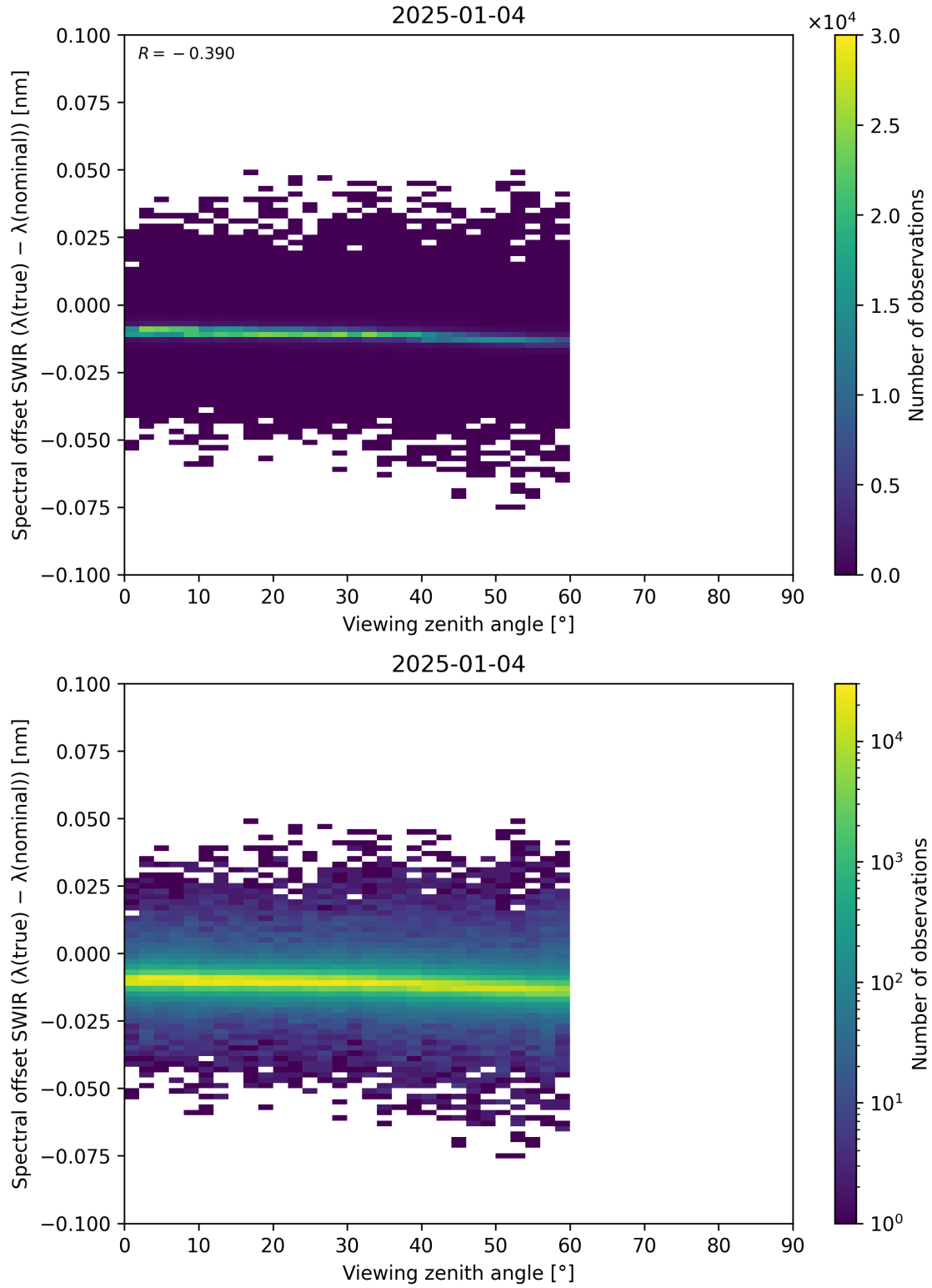
Figure 116: Scatter density plot of “Viewing zenith angle” against “Spectral offset SWIR ( \lambda_{\text{true}} - \lambda_{\text{nominal}} )” for 2025-01-03 to 2025-01-05.
