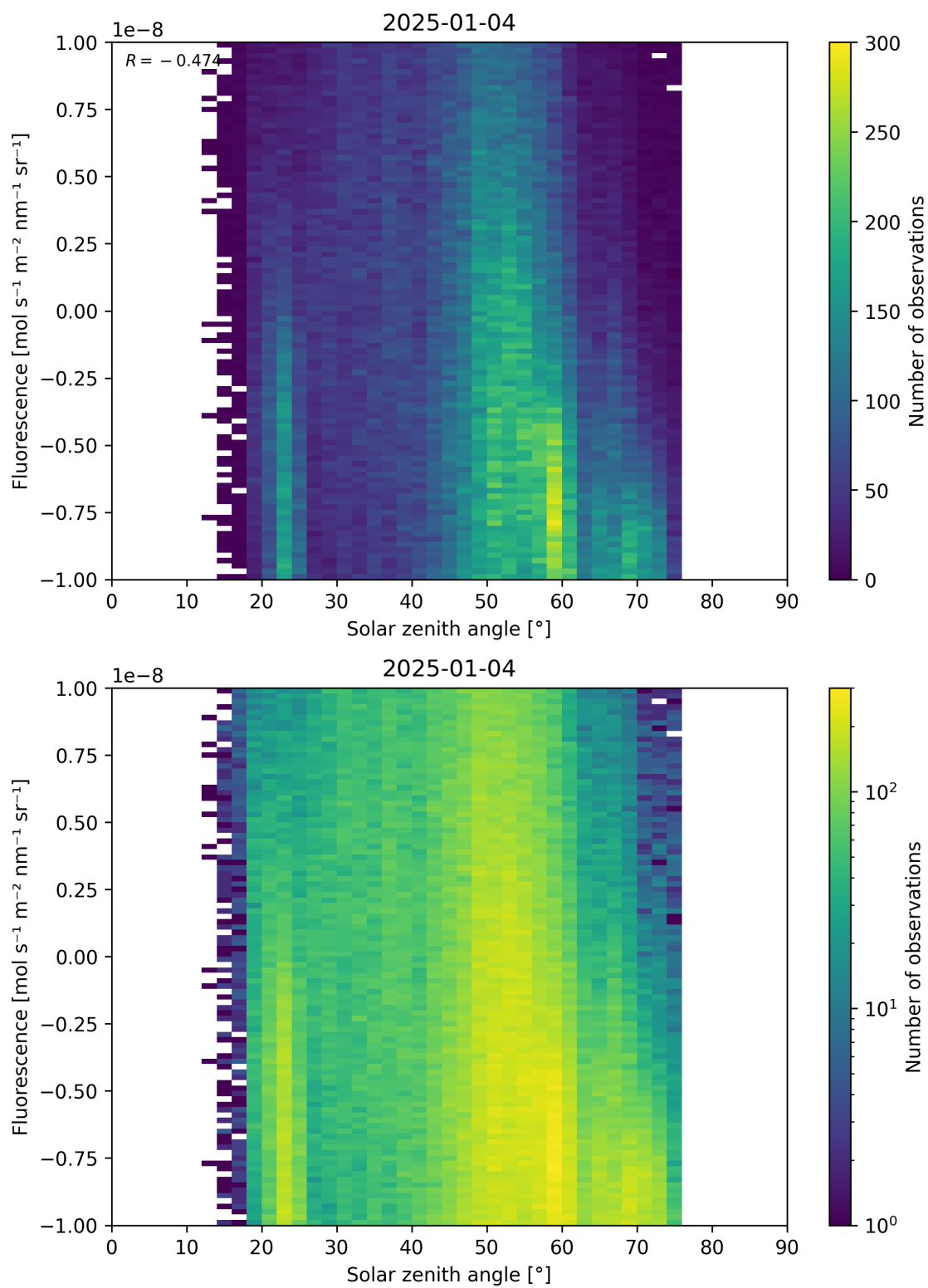
Figure 97: Scatter density plot of “Solar zenith angle” against “Fluorescence” for 2025-01-03 to 2025-01-05.
