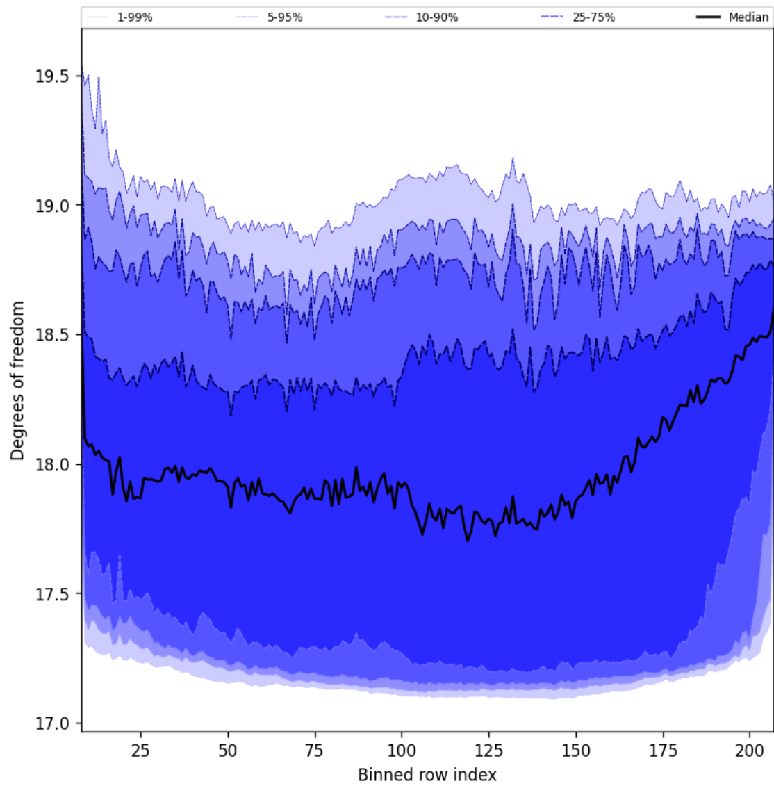
Figure 41: Along track statistics of “Degrees of freedom” for 2025-01-03 to 2025-01-05
