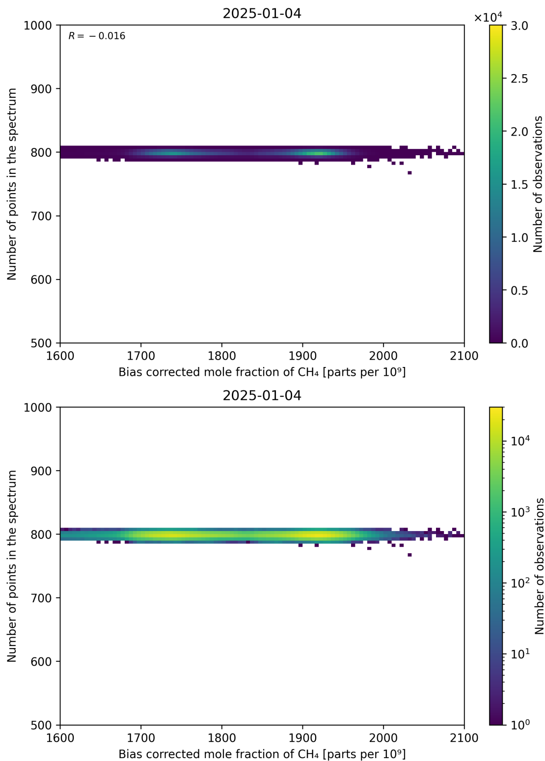
Figure 68: Scatter density plot of “Bias corrected mole fraction of CH 4 ” against “Number of points in the spectrum” for 2025-01-03 to 2025-01-05.
