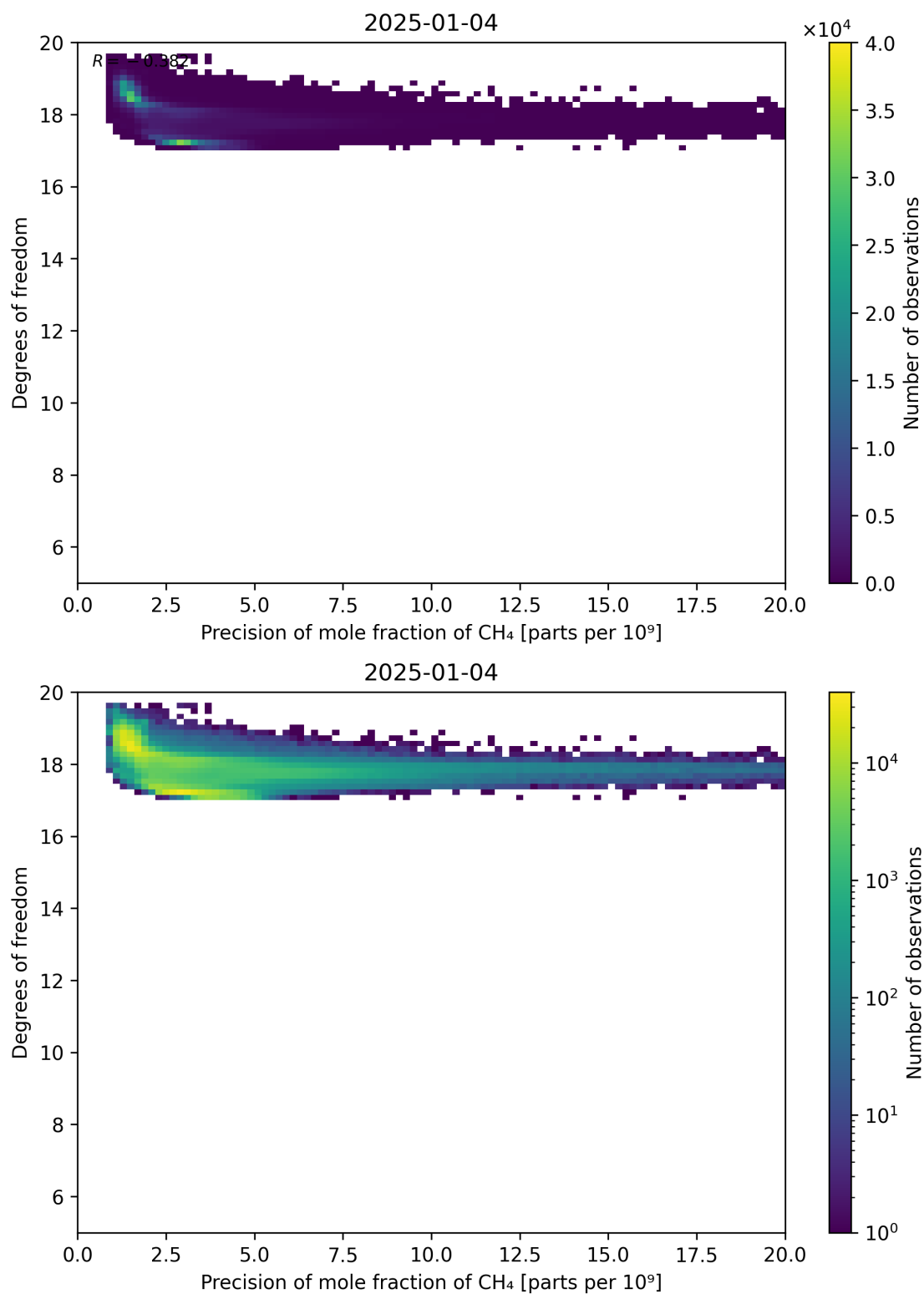
Figure 80: Scatter density plot of “Precision of mole fraction of CH 4 ” against “Degrees of freedom” for 2025-01-03 to 2025-01-05.
