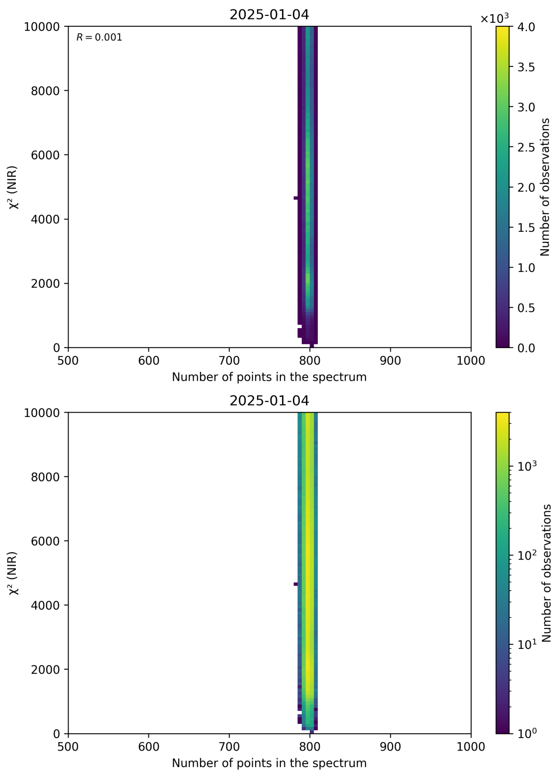
Figure 88: Scatter density plot of “Number of points in the spectrum” against “ \chi^2 (NIR)” for 2025-01-03 to 2025-01-05.
