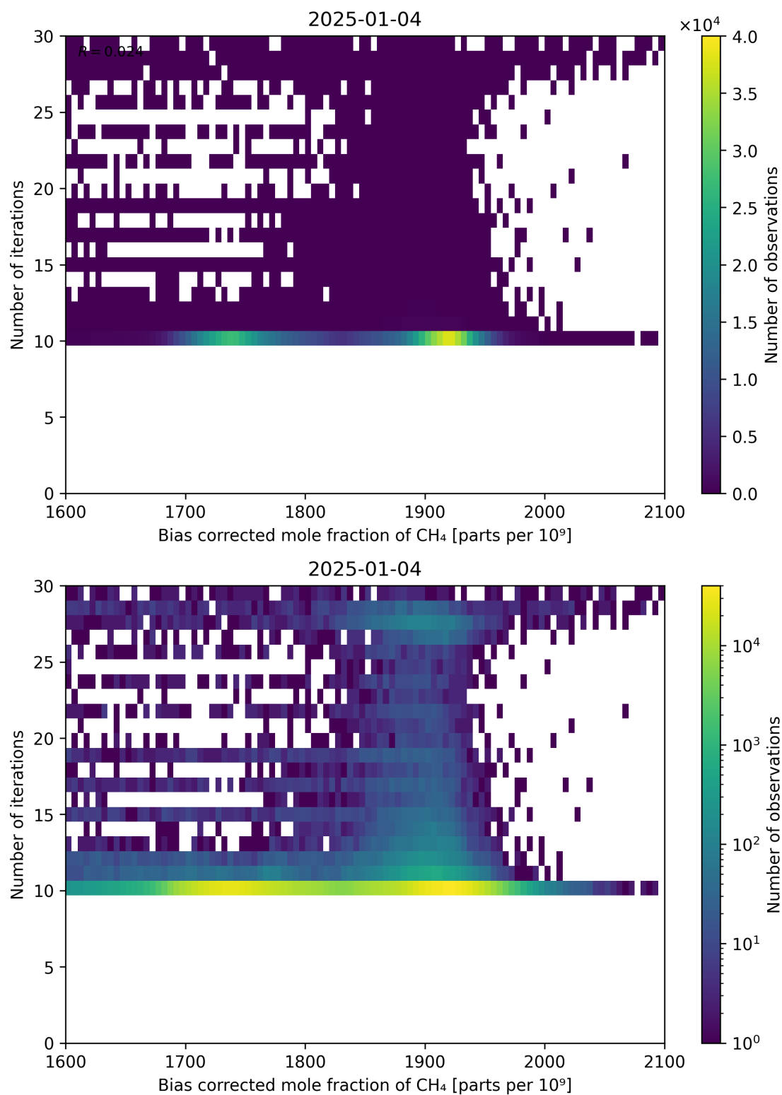
Figure 67: Scatter density plot of “Bias corrected mole fraction of CH 4 ” against “Number of iterations” for 2025-01-03 to 2025-01-05.
