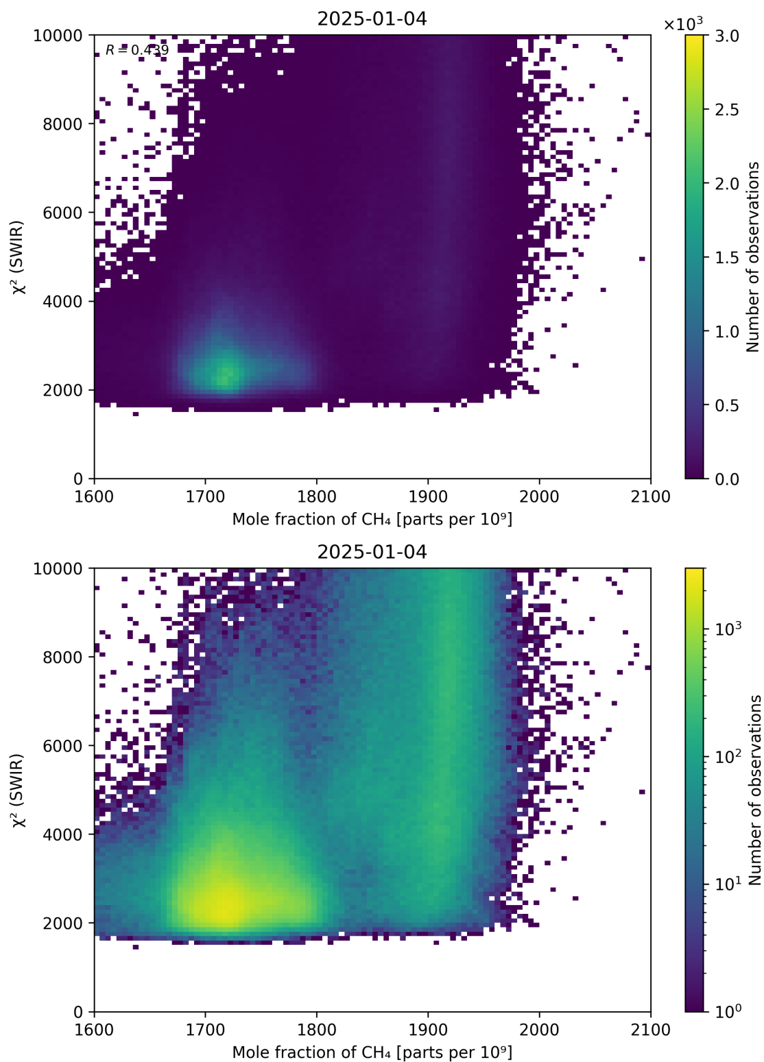
Figure 71: Scatter density plot of “Mole fraction of \text{CH}_4 ” against “ \chi^2 (SWIR)” for 2025-01-03 to 2025-01-05.
