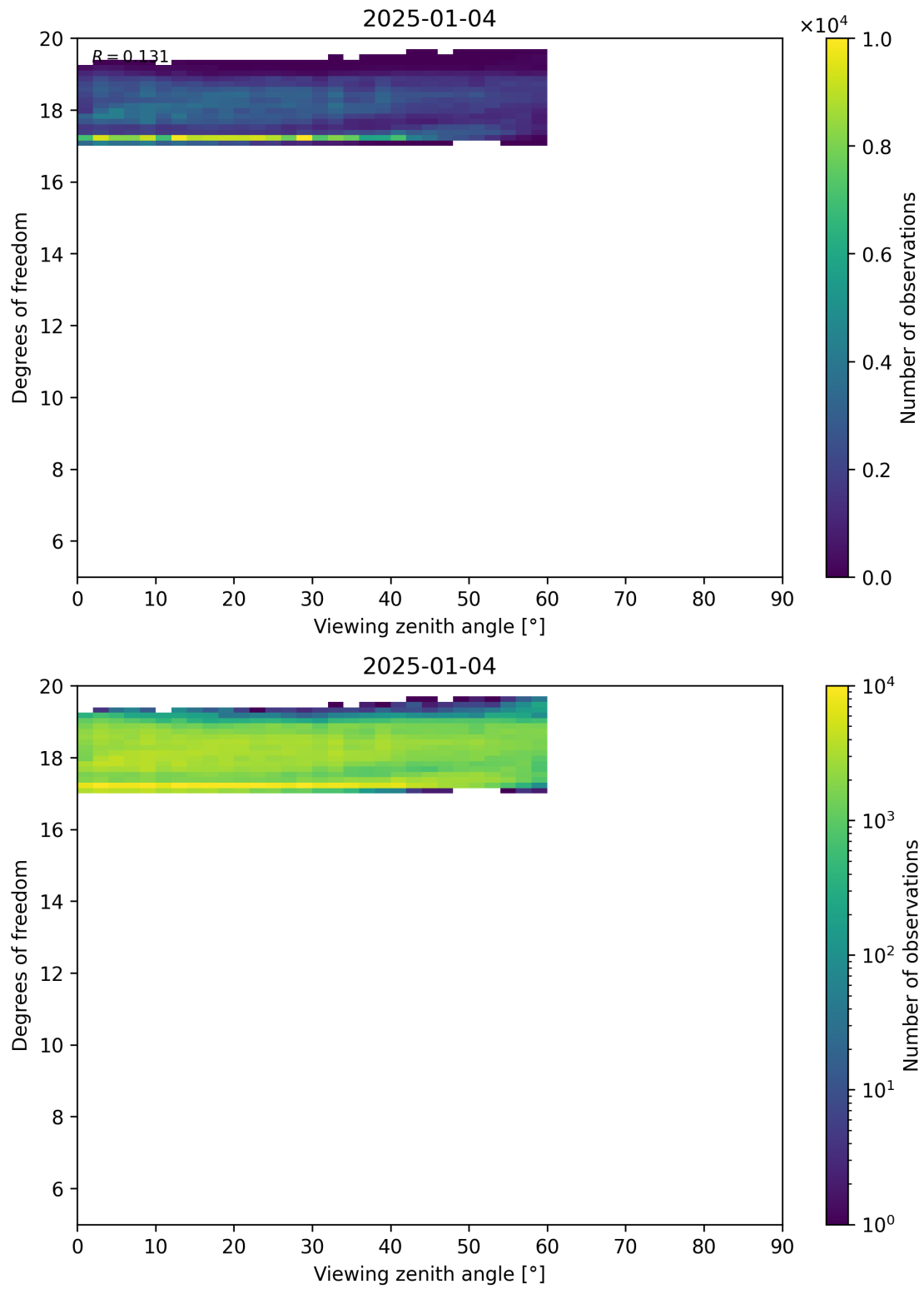
Figure 107: Scatter density plot of “Viewing zenith angle” against “Degrees of freedom” for 2025-01-03 to 2025-01-05.
