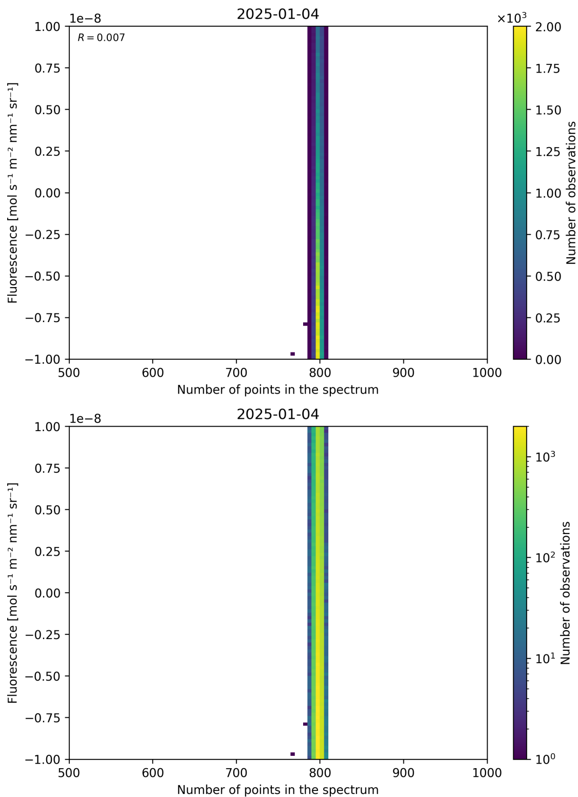
Figure 91: Scatter density plot of “Number of points in the spectrum” against “Fluorescence” for 2025-01-03 to 2025-01-05.
