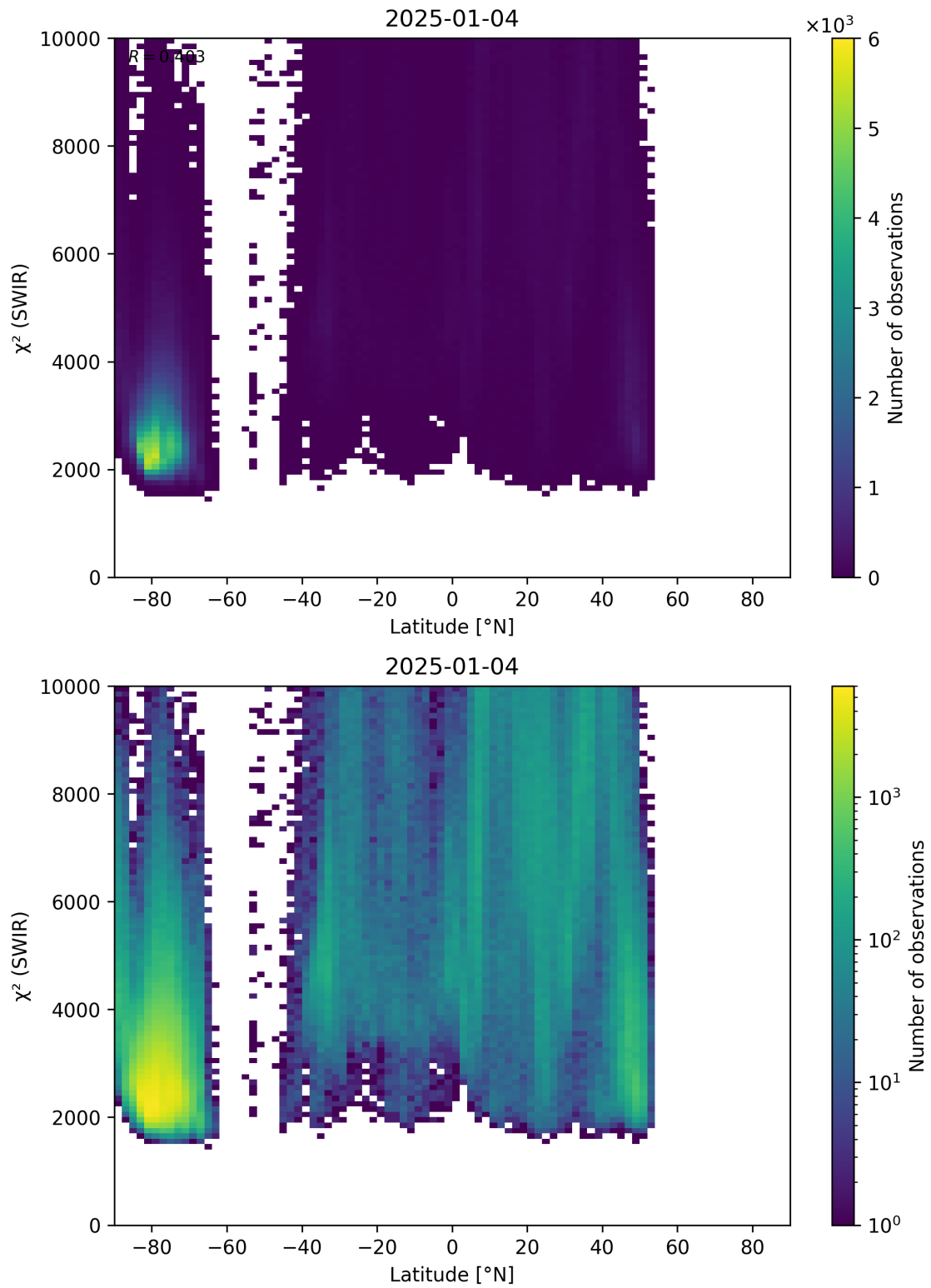
Figure 54: Scatter density plot of “Latitude” against “ \chi^2 (SWIR)” for 2025-01-03 to 2025-01-05.
