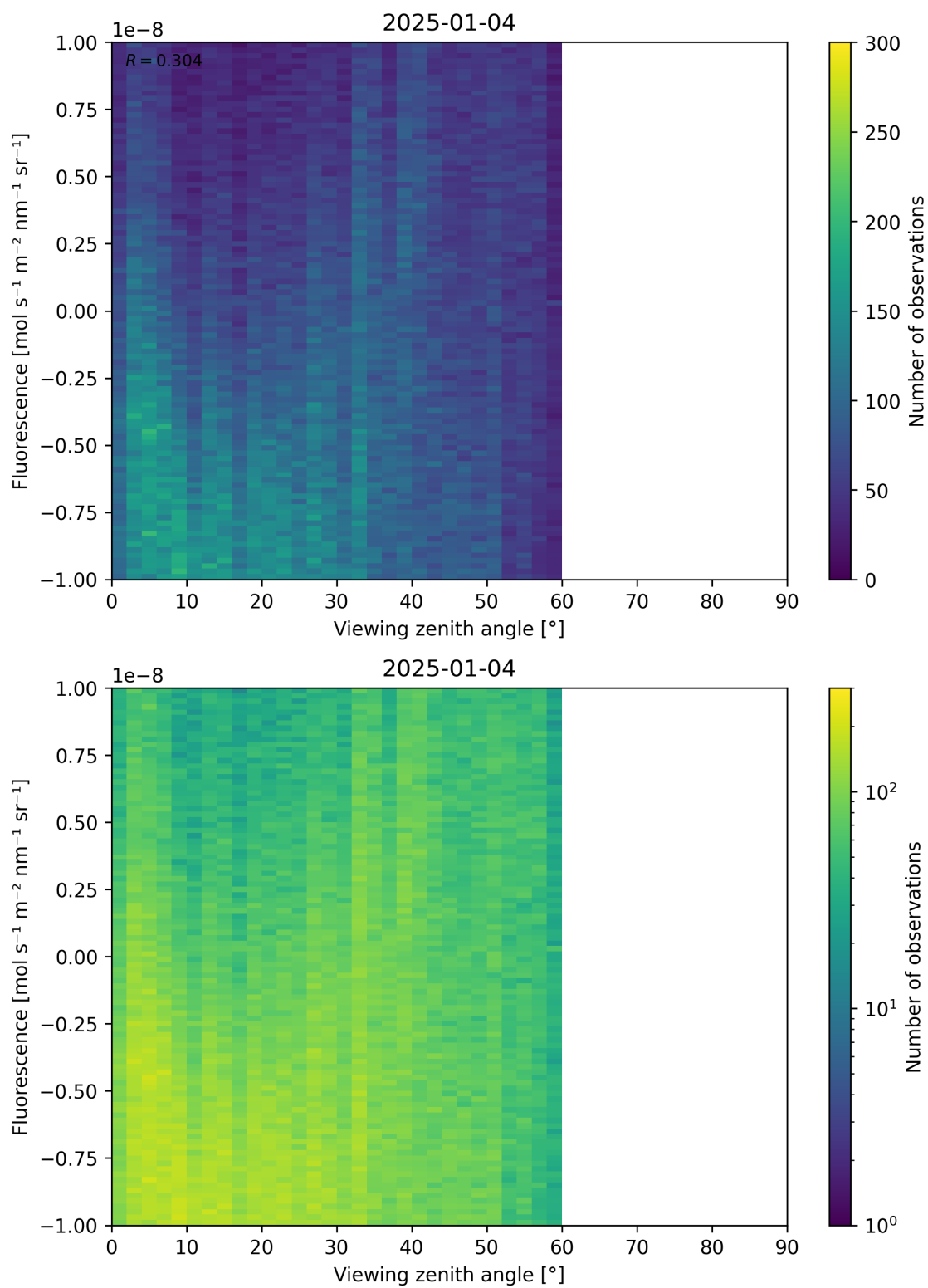
Figure 108: Scatter density plot of “Viewing zenith angle” against “Fluorescence” for 2025-01-03 to 2025-01-05.
