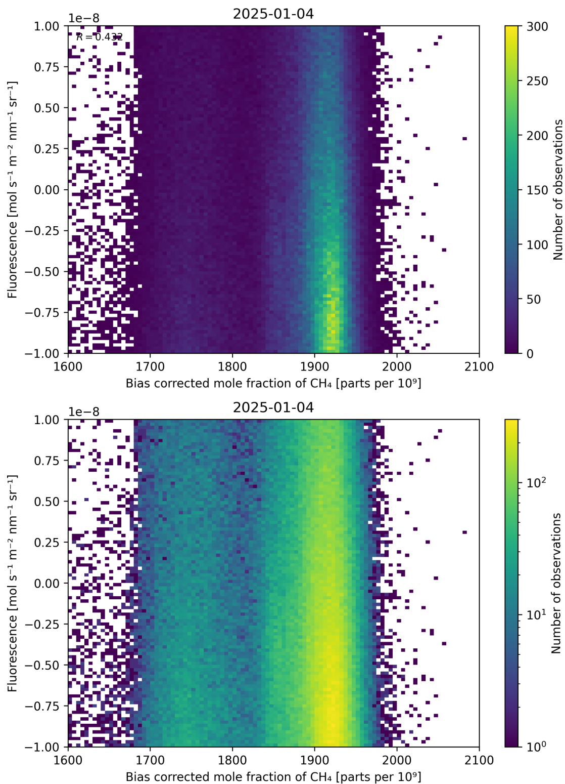
Figure 66: Scatter density plot of “Bias corrected mole fraction of \text{CH}_4 ” against “Fluorescence” for 2025-01-03 to 2025-01-05.
