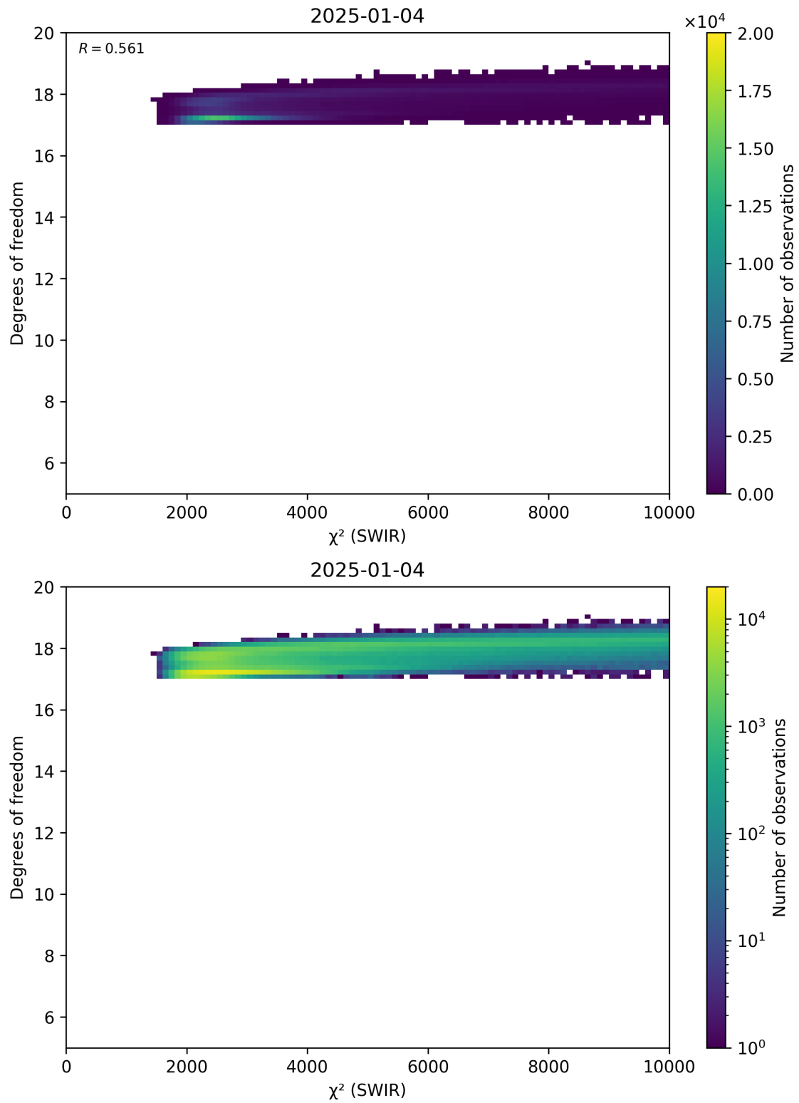
Figure 48: Scatter density plot of “ \chi^2 (SWIR)” against “Degrees of freedom” for 2025-01-03 to 2025-01-05.
