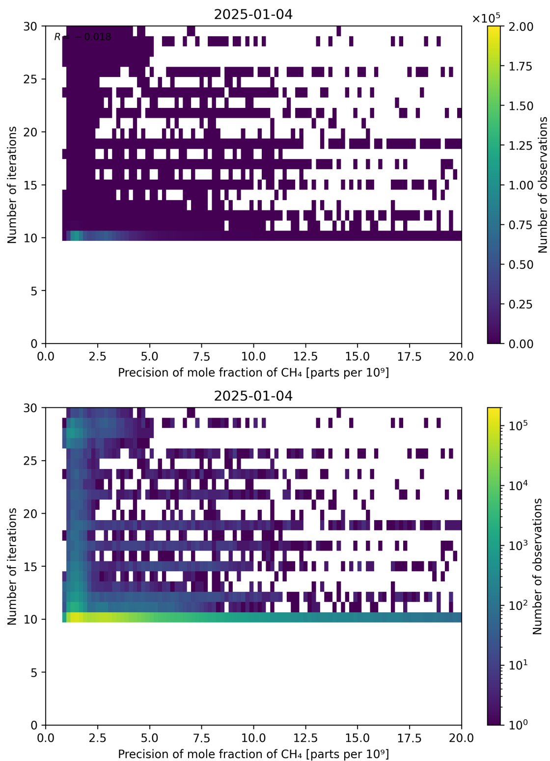
Figure 83: Scatter density plot of “Precision of mole fraction of CH 4 ” against “Number of iterations” for 2025-01-03 to 2025-01-05.
