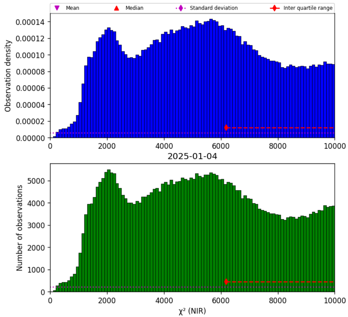
Figure 29: Histogram of " \chi^2 (NIR)" for 2025-01-03 to 2025-01-05
