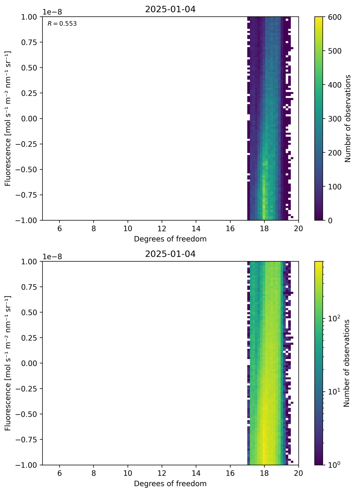
Figure 51: Scatter density plot of “Degrees of freedom” against “Fluorescence” for 2025-01-03 to 2025-01-05.
