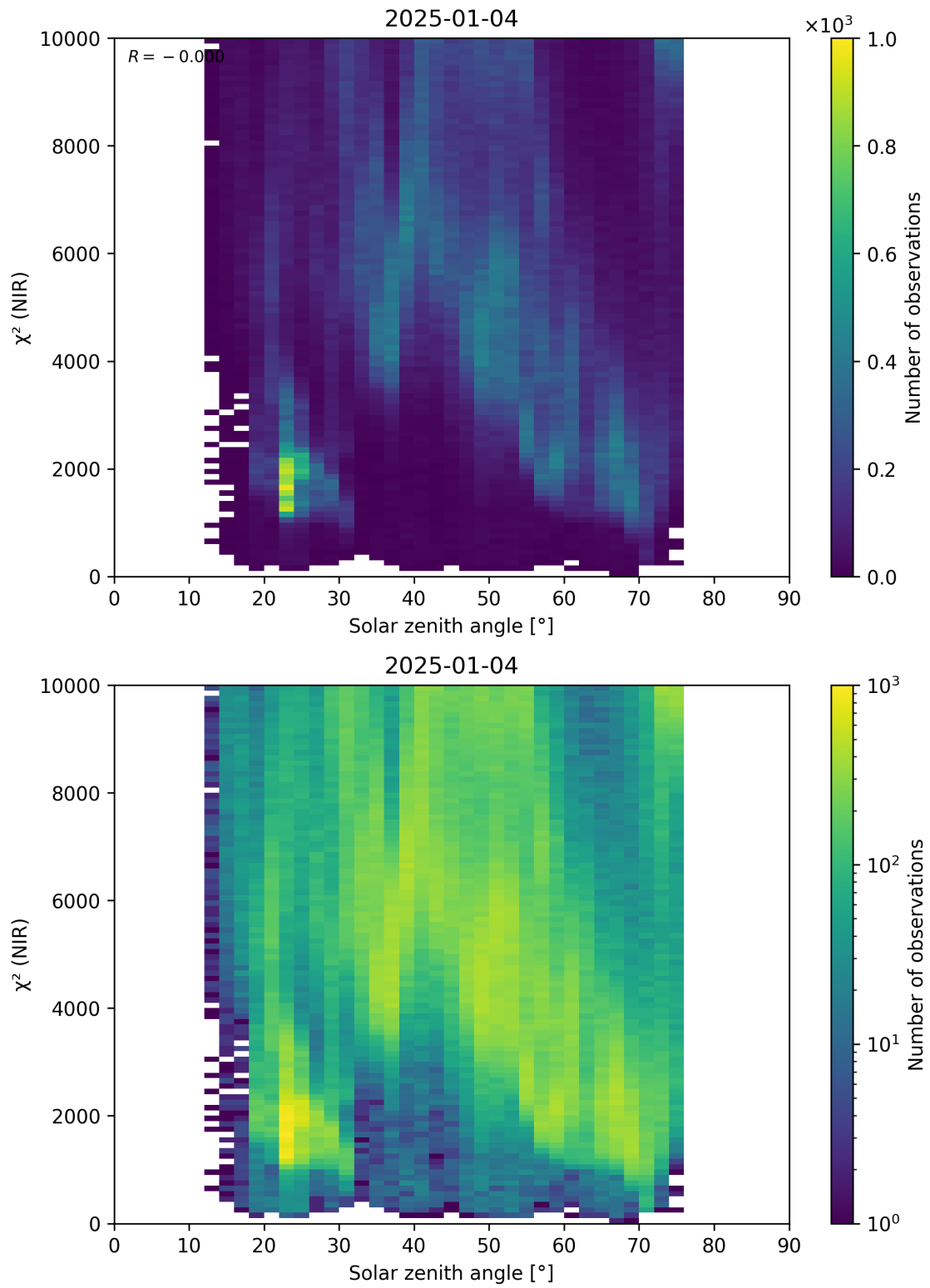
Figure 94: Scatter density plot of “Solar zenith angle” against “ \chi^2 (NIR)” for 2025-01-03 to 2025-01-05.
