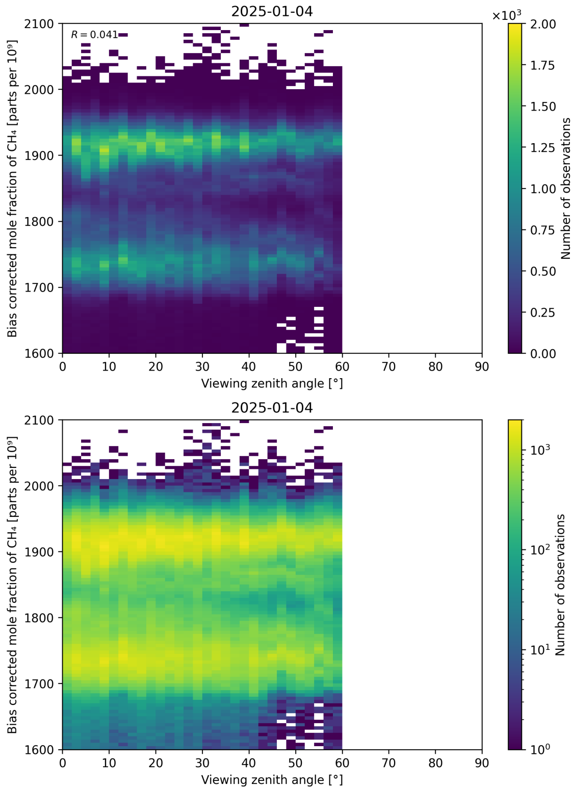
Figure 111: Scatter density plot of “Viewing zenith angle” against “Bias corrected mole fraction of CH 4 ” for 2025-01-03 to 2025-01-05.
