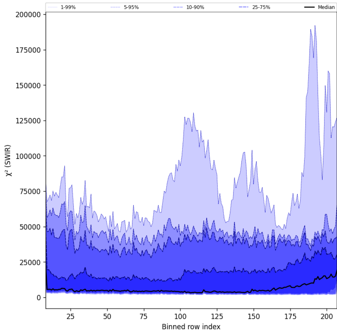
Figure 39: Along track statistics of “ \chi^2 (SWIR)” for 2025-01-03 to 2025-01-05
