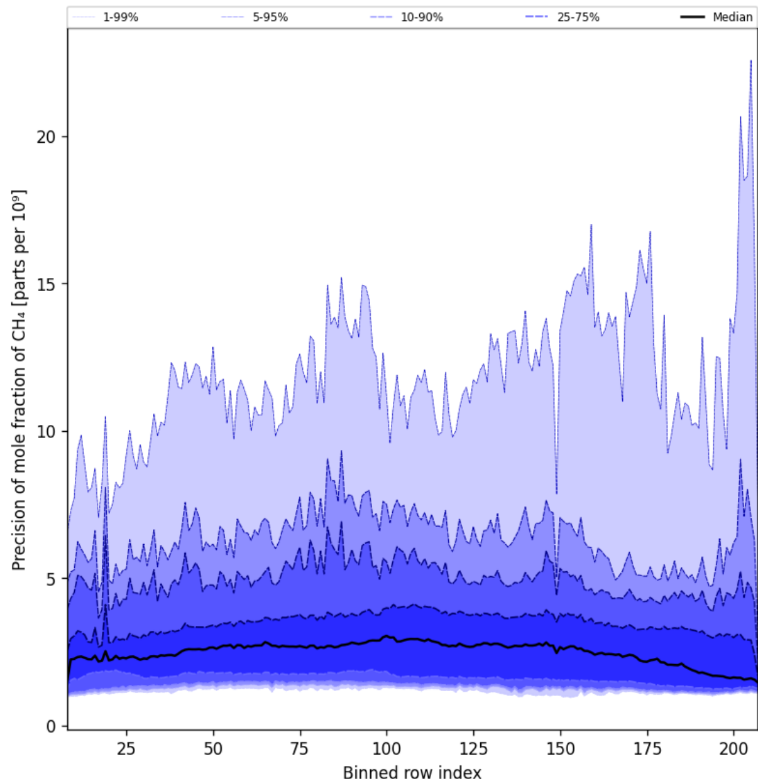
Figure 35: Along track statistics of “Precision of mole fraction of CH 4 ” for 2025-01-03 to 2025-01-05
