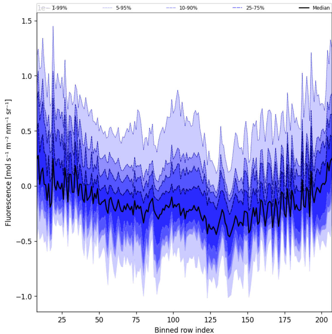
Figure 43: Along track statistics of “Fluorescence” for 2025-01-03 to 2025-01-05
