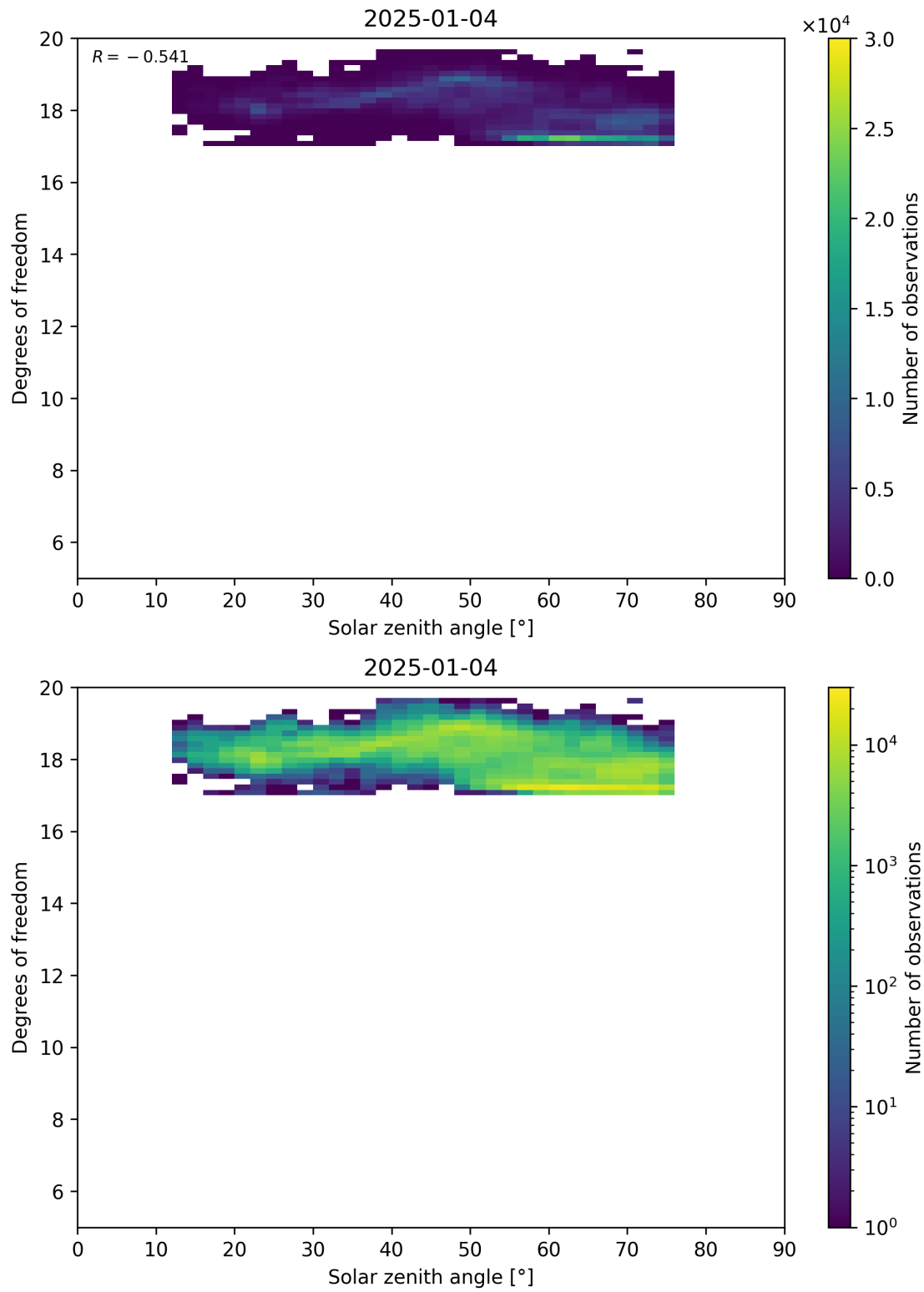
Figure 96: Scatter density plot of “Solar zenith angle” against “Degrees of freedom” for 2025-01-03 to 2025-01-05.
