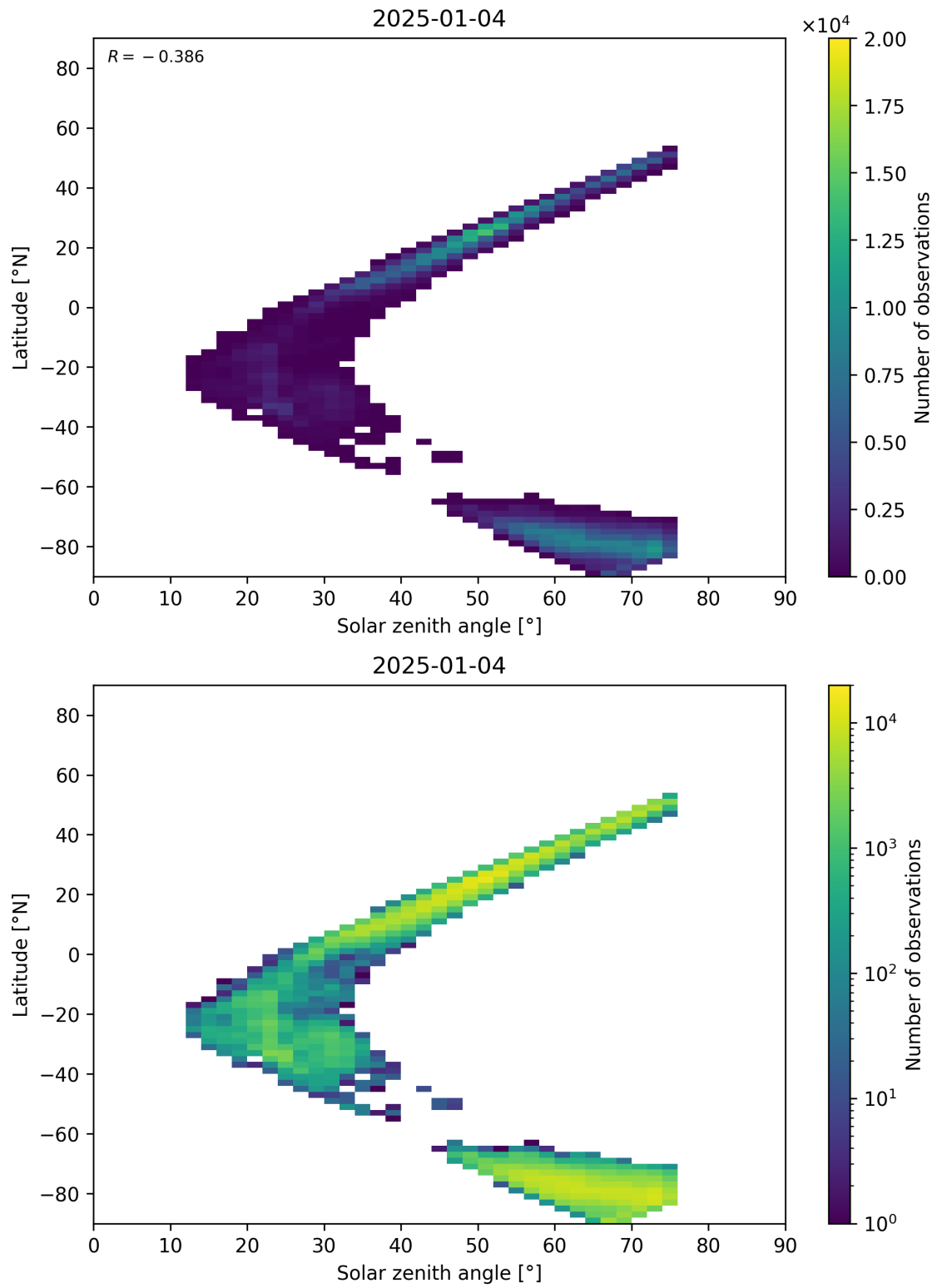
Figure 98: Scatter density plot of “Solar zenith angle” against “Latitude” for 2025-01-03 to 2025-01-05.
