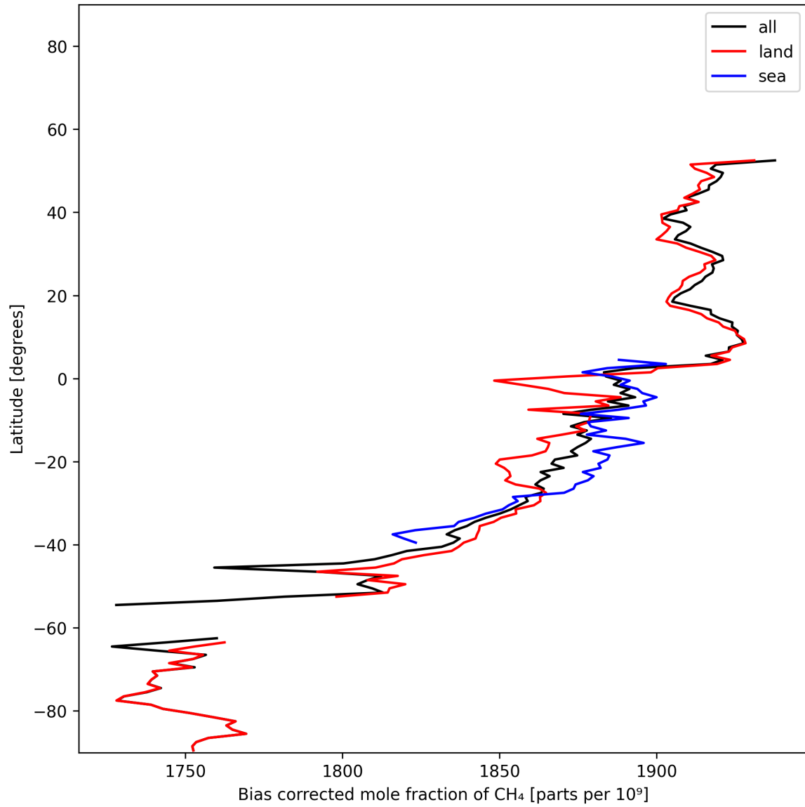
Figure 14: Zonal average of “Bias corrected mole fraction of CH 4 ” for 2025-01-03 to 2025-01-05.
