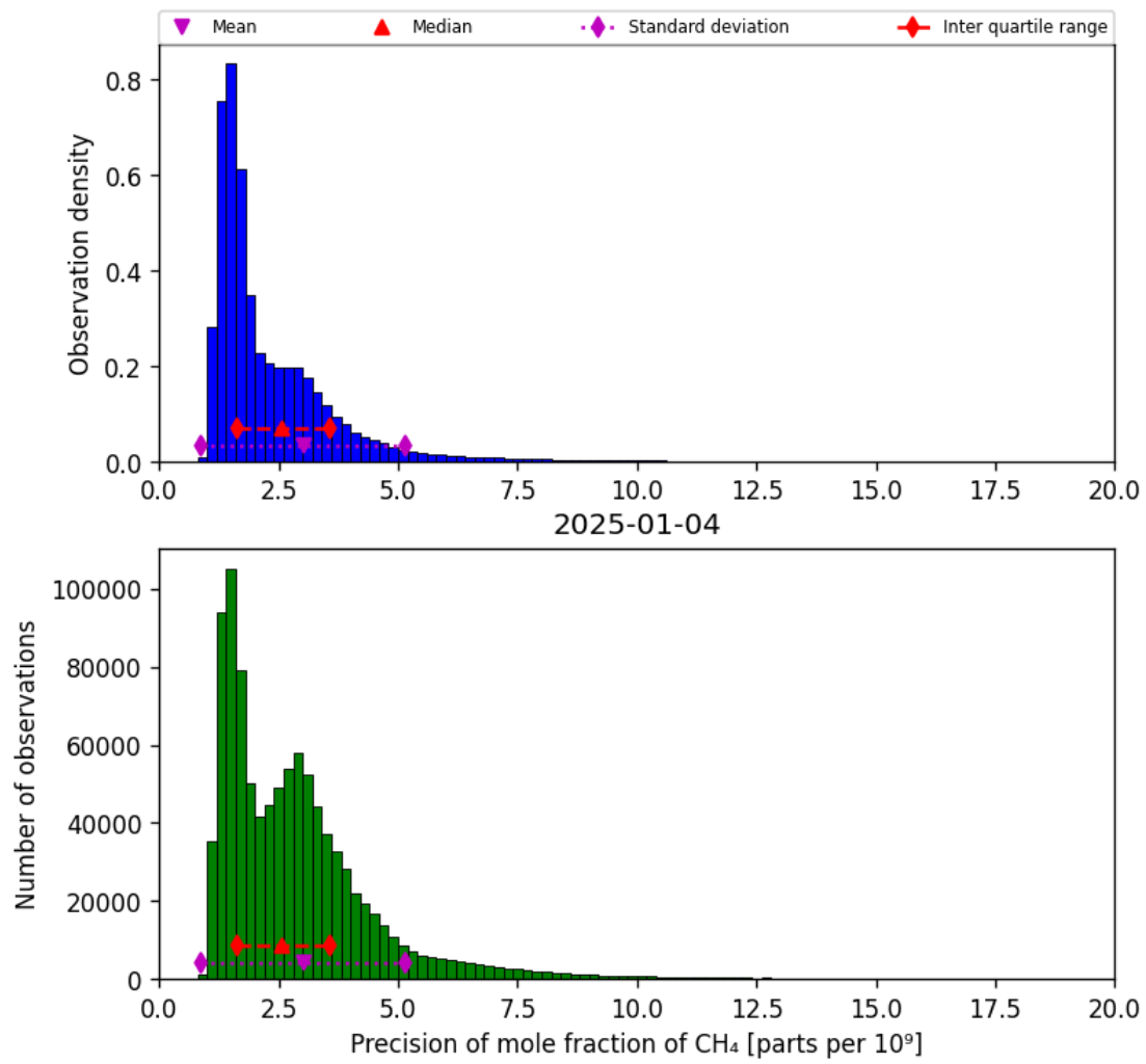
Figure 24: Histogram of “Precision of mole fraction of CH 4 ” for 2025-01-03 to 2025-01-05
