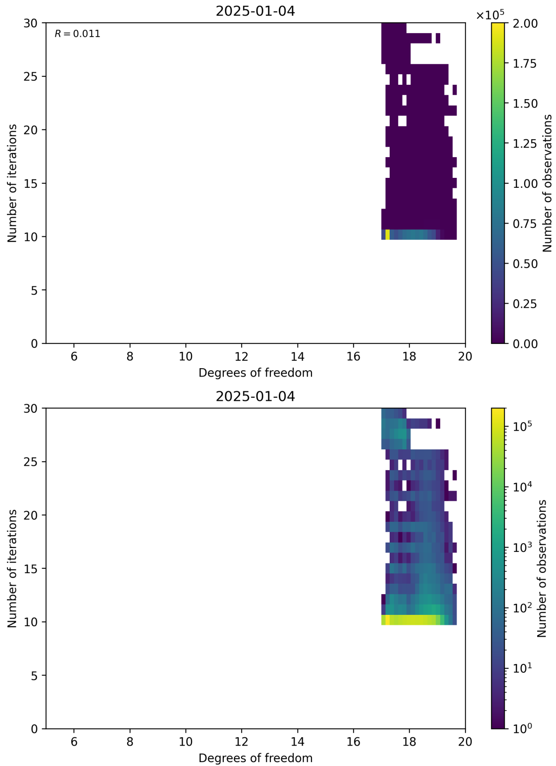
Figure 52: Scatter density plot of “Degrees of freedom” against “Number of iterations” for 2025-01-03 to 2025-01-05.
