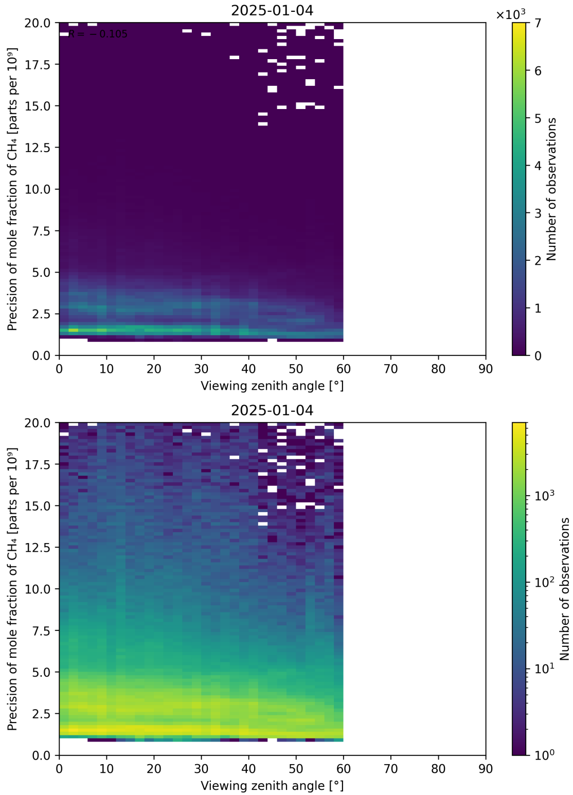
Figure 112: Scatter density plot of “Viewing zenith angle” against “Precision of mole fraction of CH 4 ” for 2025-01-03 to 2025-01-05.
