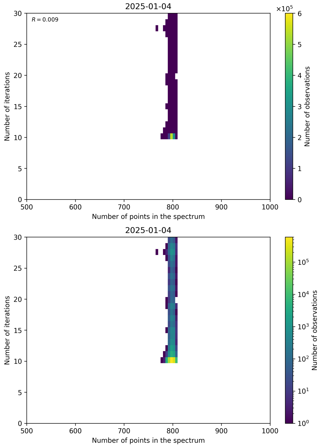
Figure 92: Scatter density plot of “Number of points in the spectrum” against “Number of iterations” for 2025-01-03 to 2025-01-05.
