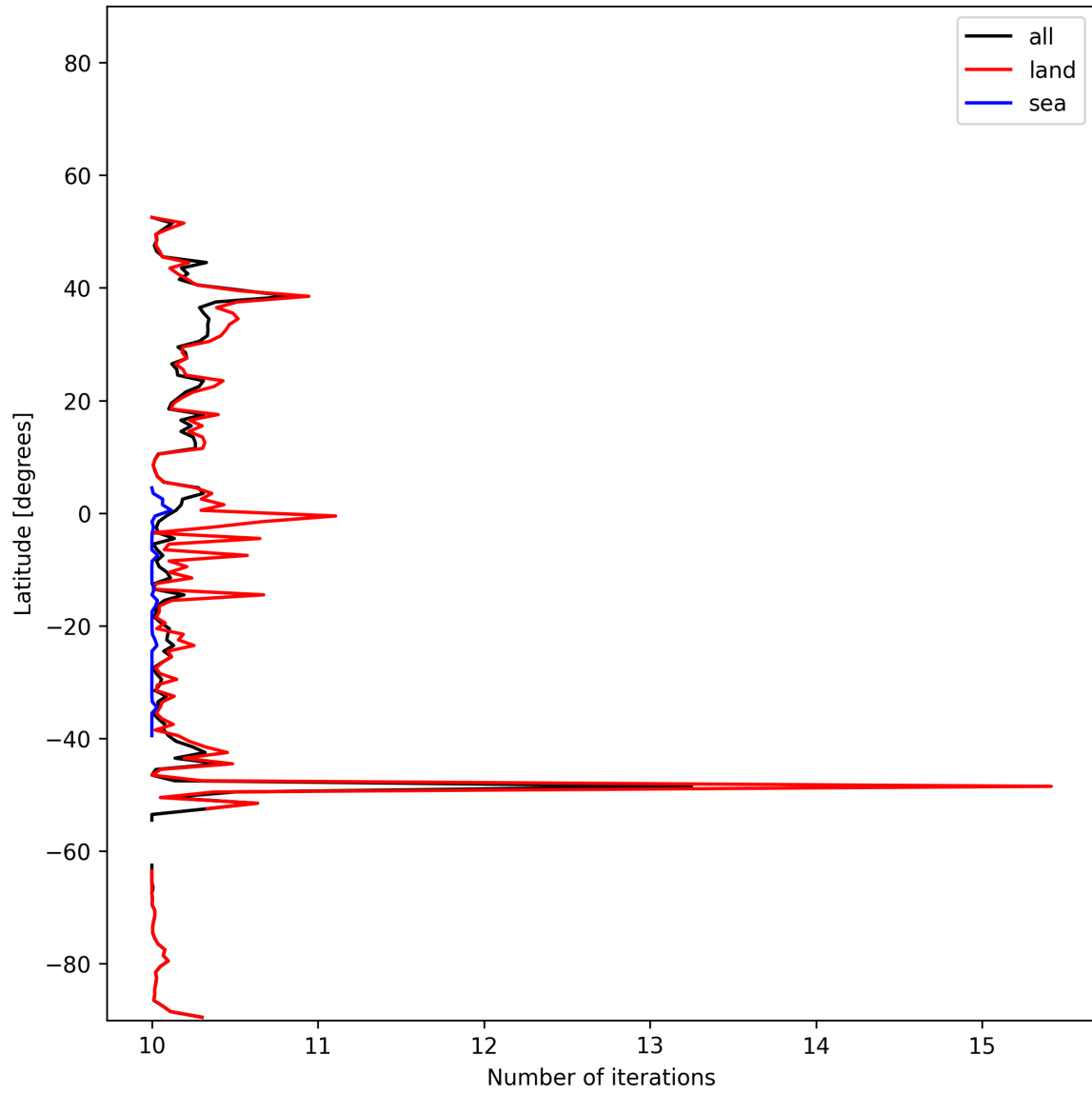
Figure 20: Zonal average of “Number of iterations” for 2025-01-03 to 2025-01-05.
