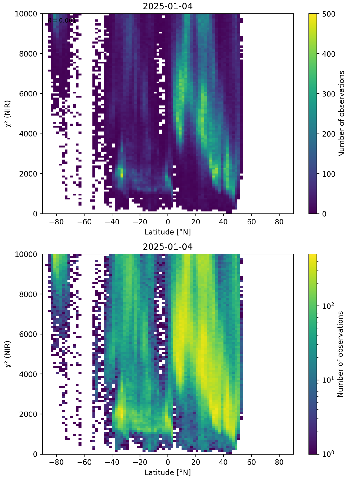
Figure 53: Scatter density plot of “Latitude” against “ \chi^2 (NIR)” for 2025-01-03 to 2025-01-05.
