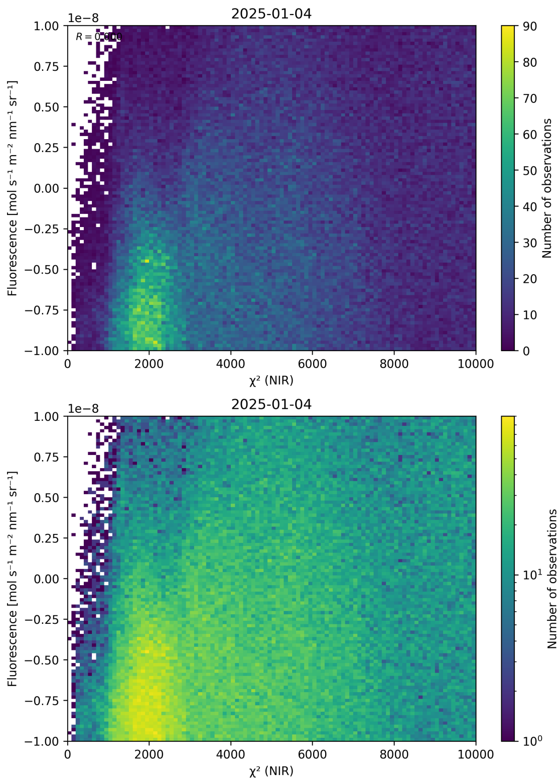
Figure 45: Scatter density plot of “ \chi^2 (NIR)” against “Fluorescence” for 2025-01-03 to 2025-01-05.
