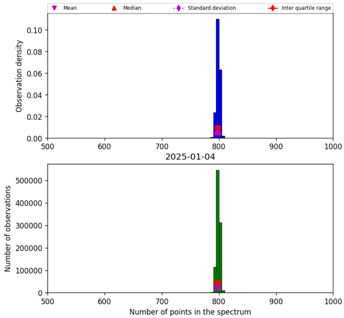
Figure 26: Histogram of “Number of points in the spectrum” for 2025-01-03 to 2025-01-05
