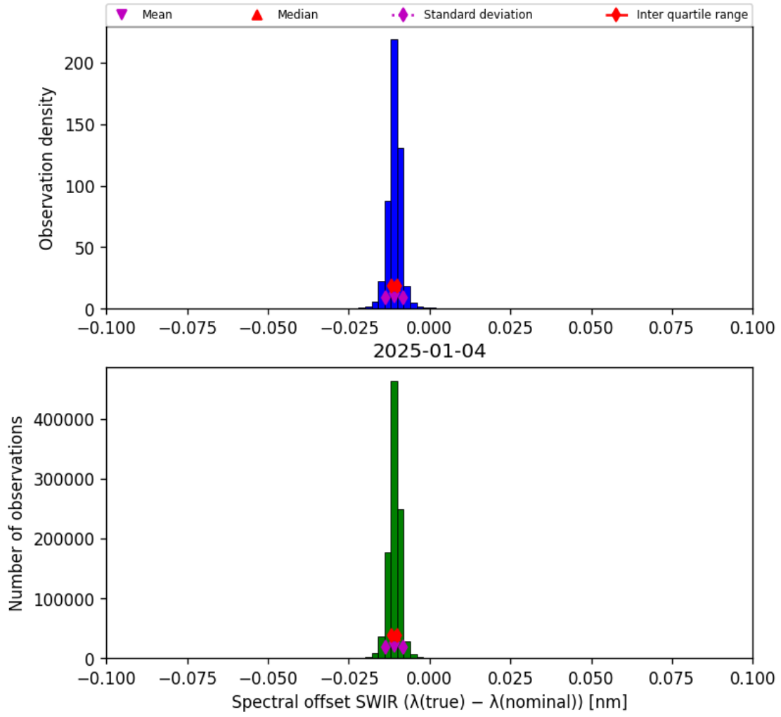
Figure 27: Histogram of “Spectral offset SWIR ( \lambda_{\text{true}} - \lambda_{\text{nominal}} )” for 2025-01-03 to 2025-01-05
