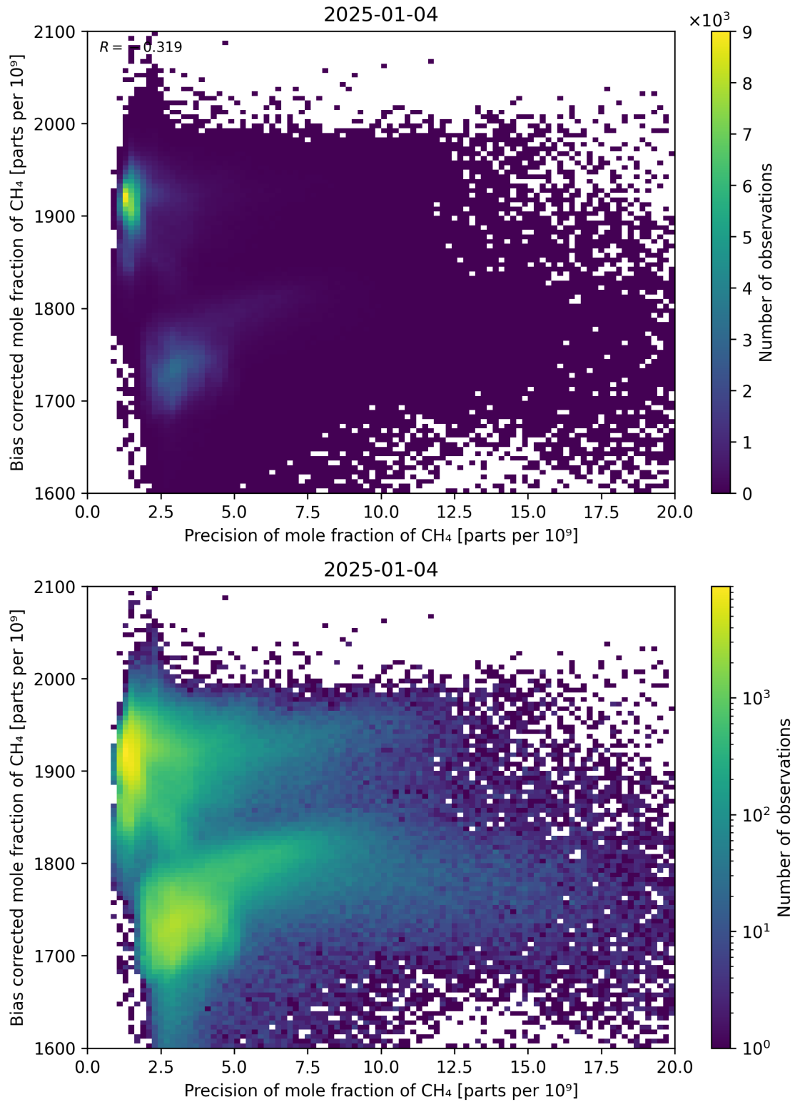
Figure 82: Scatter density plot of “Precision of mole fraction of \text{CH}_4 ” against “Bias corrected mole fraction of \text{CH}_4 ” for 2025-01-03 to 2025-01-05.
