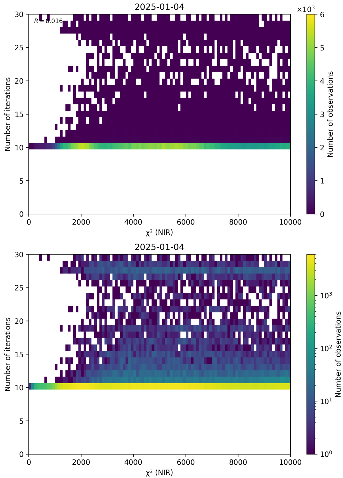
Figure 46: Scatter density plot of “ \chi^2 (NIR)” against “Number of iterations” for 2025-01-03 to 2025-01-05.
