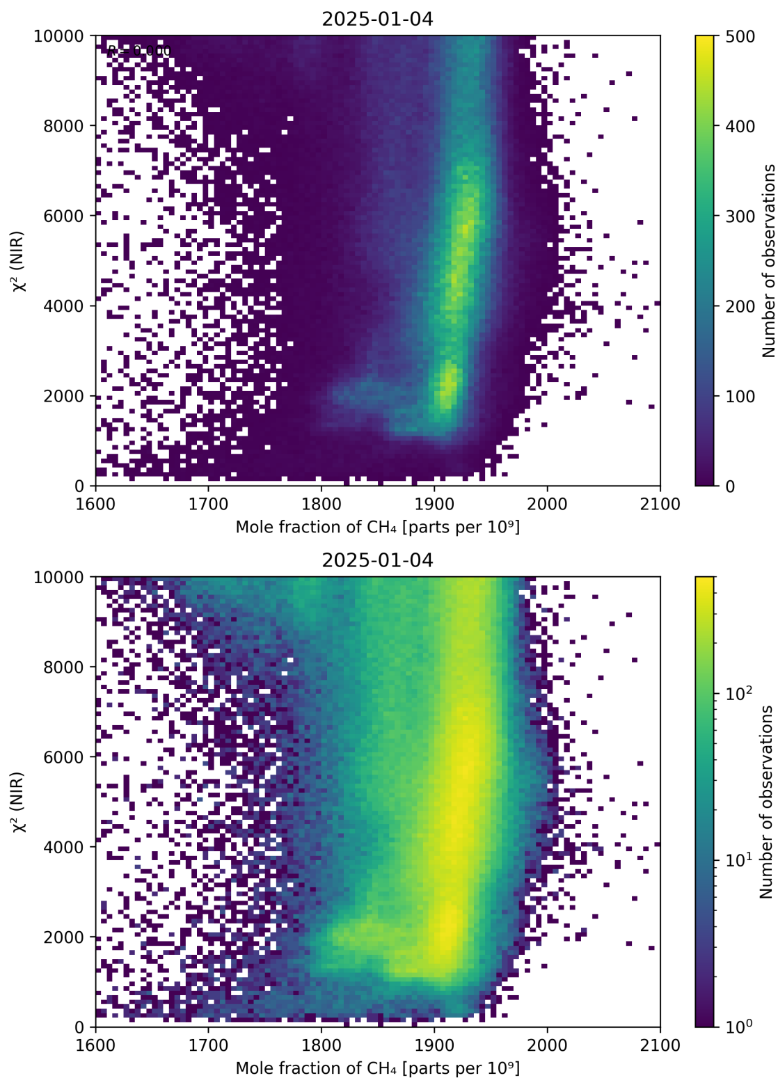
Figure 70: Scatter density plot of “Mole fraction of CH 4 ” against “ \chi^2 (NIR)” for 2025-01-03 to 2025-01-05.
