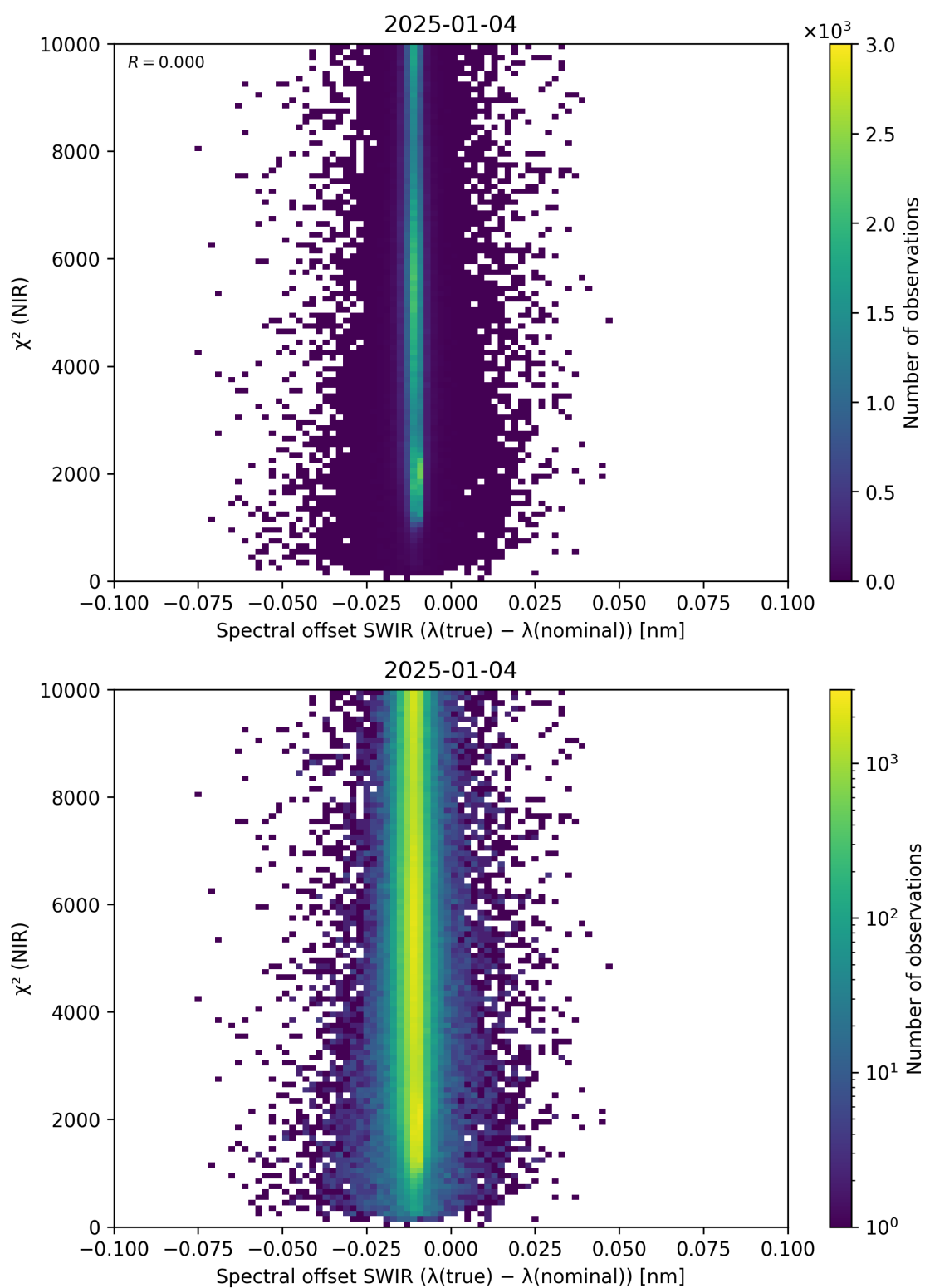
Figure 117: Scatter density plot of “Spectral offset SWIR ( \lambda_{\text{true}} - \lambda_{\text{nominal}} )” against “ \chi^2 (NIR)” for 2025-01-03 to 2025-01-05.
