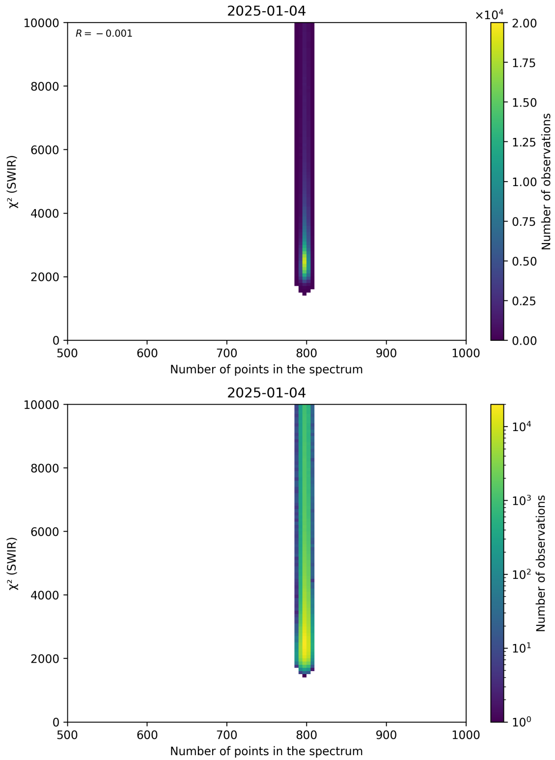
Figure 89: Scatter density plot of “Number of points in the spectrum” against “ \chi^2 (SWIR)” for 2025-01-03 to 2025-01-05.
