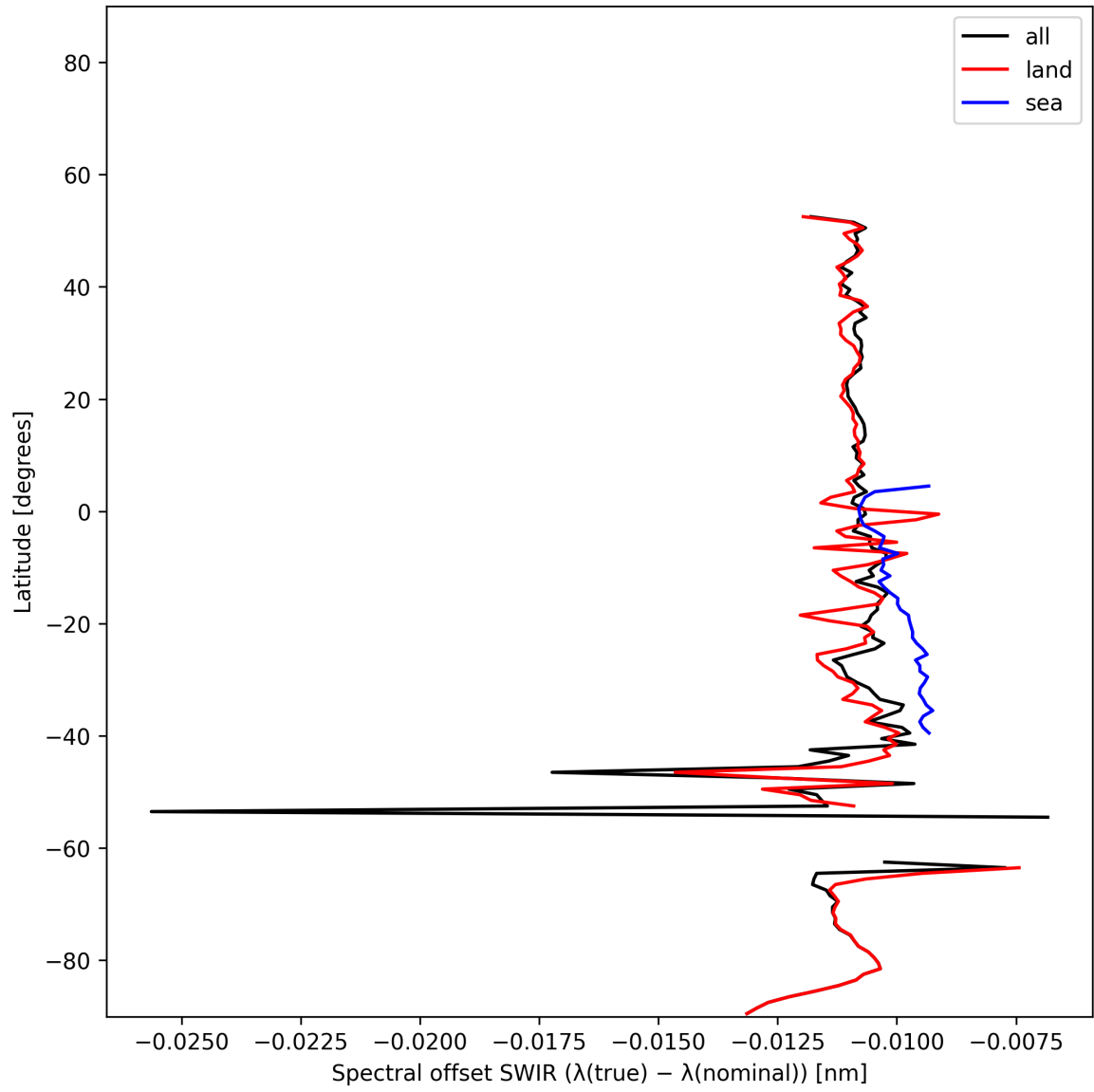
Figure 16: Zonal average of “Spectral offset SWIR ( \lambda_{\text{true}} - \lambda_{\text{nominal}} )” for 2025-01-03 to 2025-01-05.
