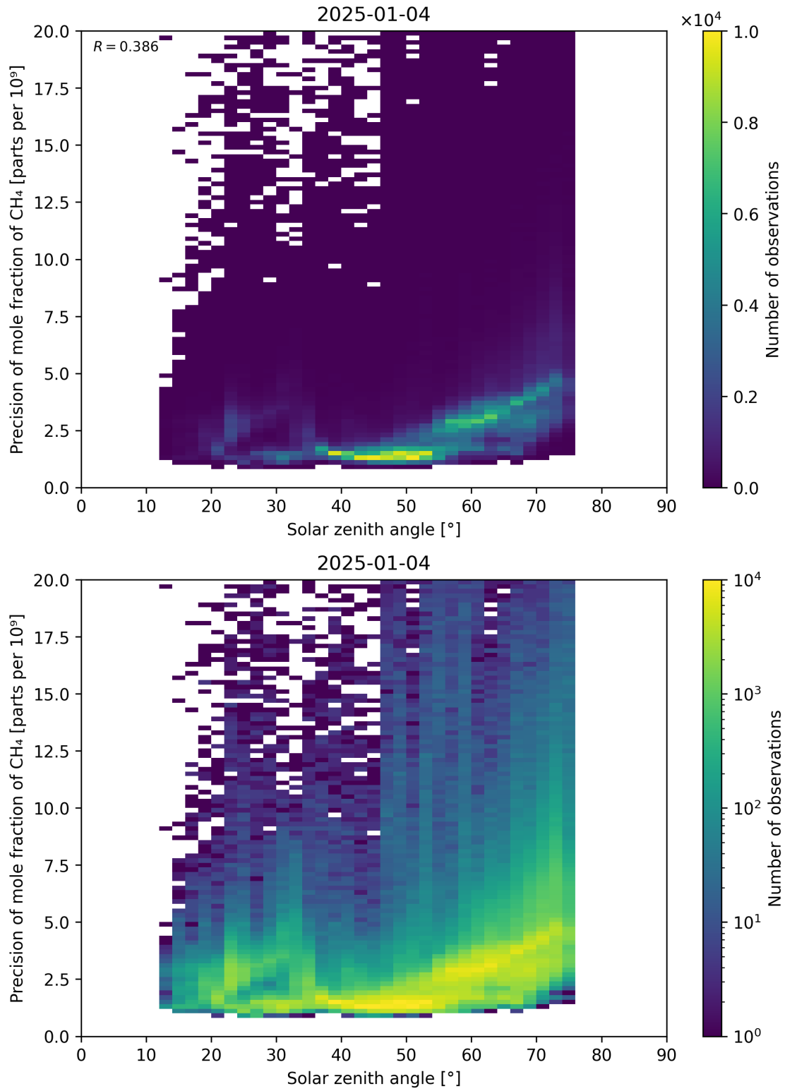
Figure 101: Scatter density plot of “Solar zenith angle” against “Precision of mole fraction of CH 4 ” for 2025-01-03 to 2025-01-05.
