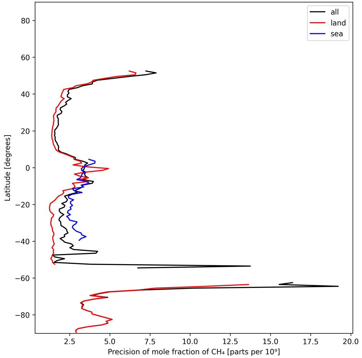
Figure 13: Zonal average of “Precision of mole fraction of CH 4 ” for 2025-01-03 to 2025-01-05.
