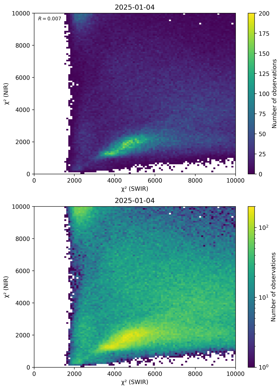
Figure 47: Scatter density plot of “ \chi^2 (SWIR)” against “ \chi^2 (NIR)” for 2025-01-03 to 2025-01-05.
