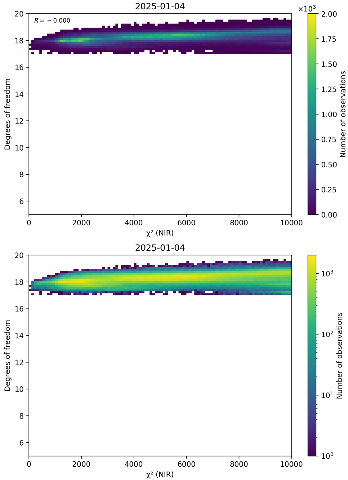
Figure 44: Scatter density plot of “ \chi^2 (NIR)” against “Degrees of freedom” for 2025-01-03 to 2025-01-05.
