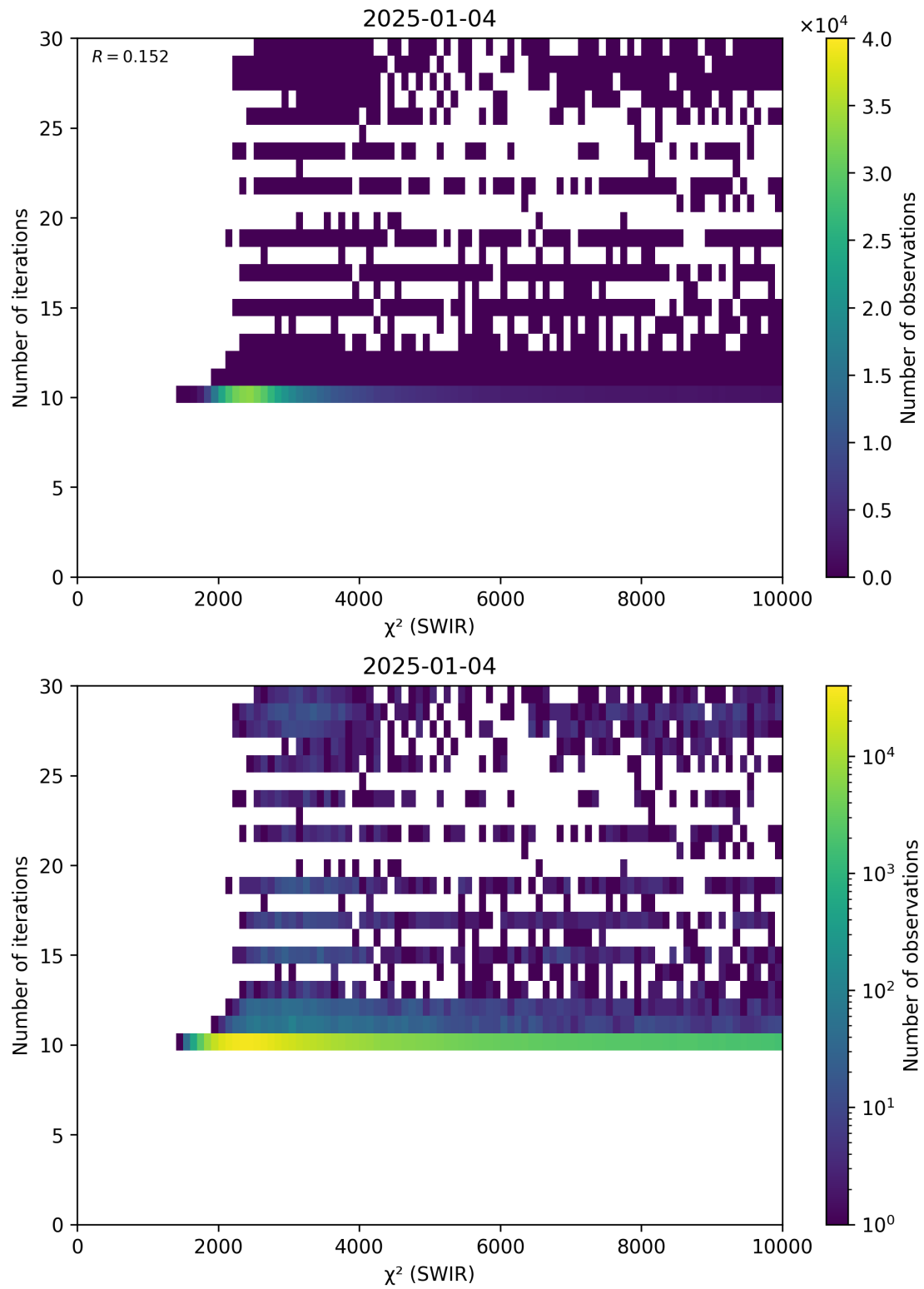
Figure 50: Scatter density plot of “ \chi^2 (SWIR)” against “Number of iterations” for 2025-01-03 to 2025-01-05.
