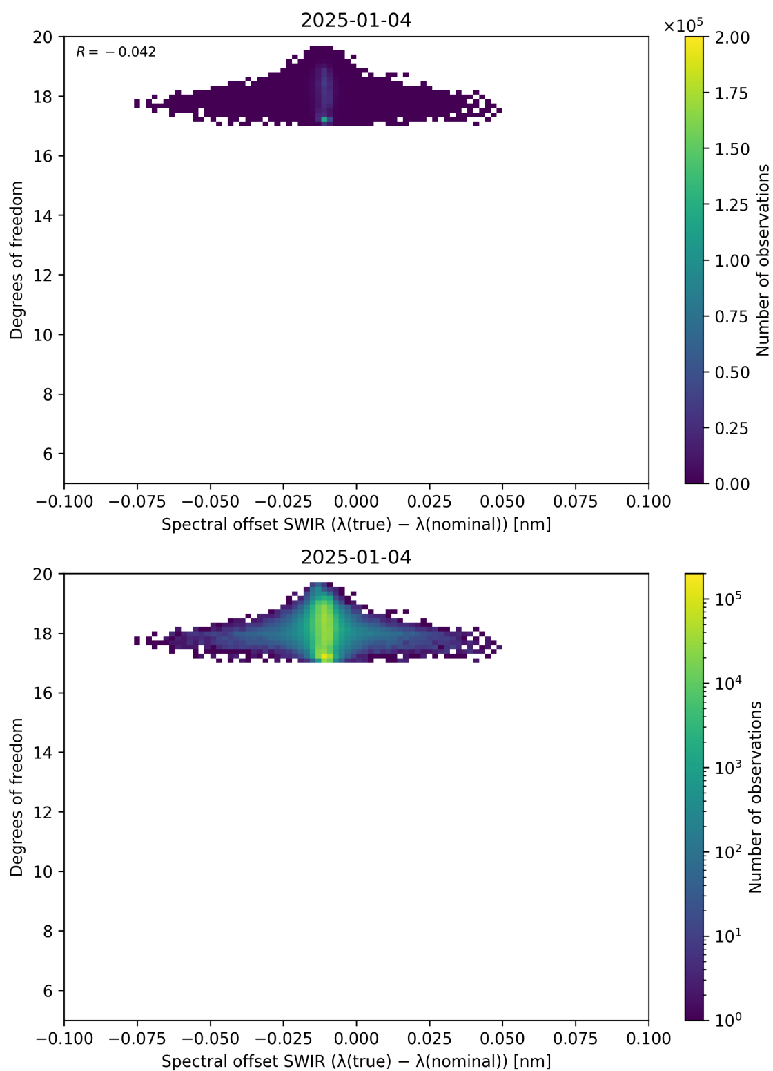
Figure 119: Scatter density plot of “Spectral offset SWIR ( \lambda_{\text{true}} - \lambda_{\text{nominal}} )” against “Degrees of freedom” for 2025-01-03 to 2025-01-05.
