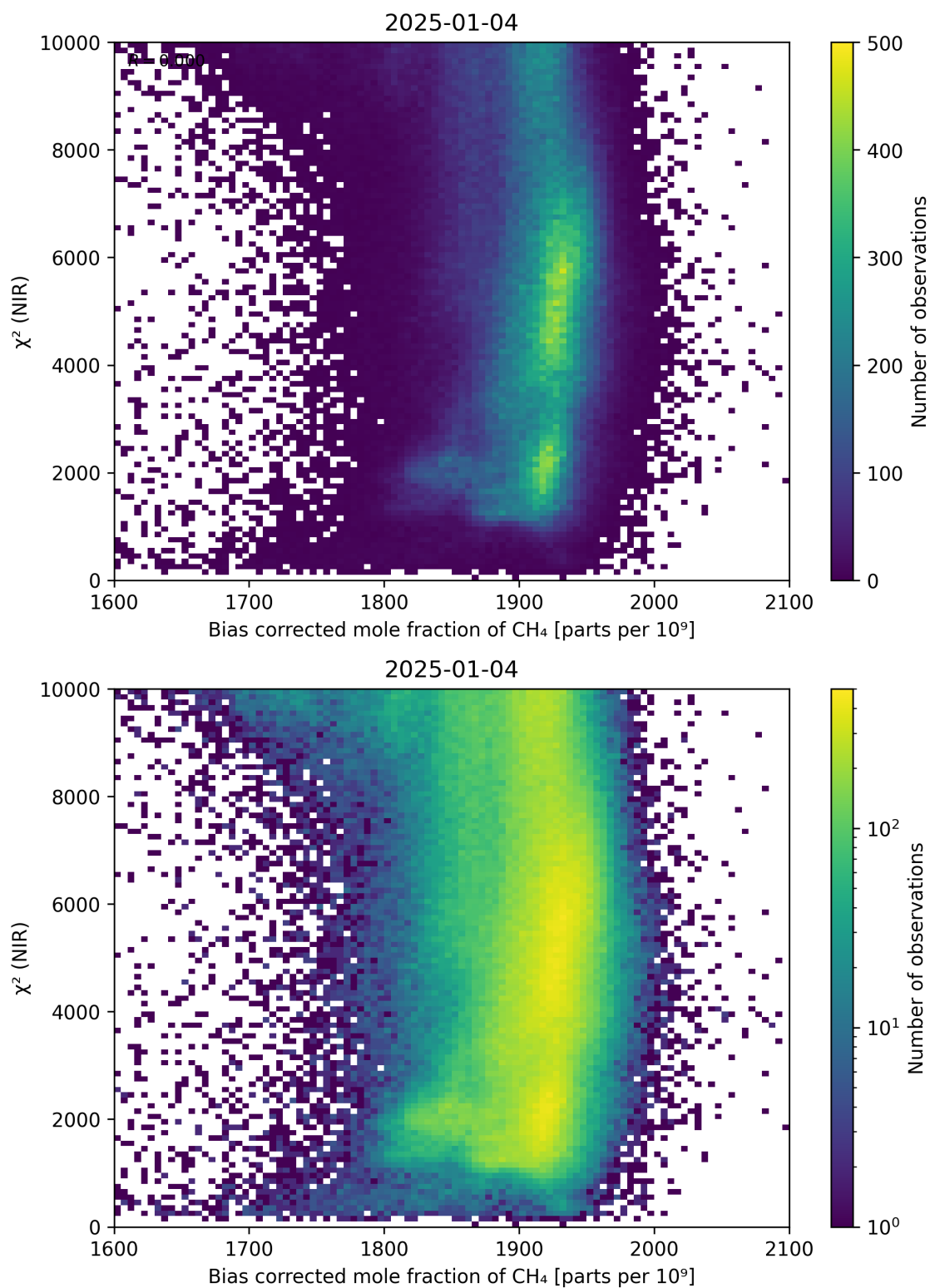
Figure 63: Scatter density plot of “Bias corrected mole fraction of \text{CH}_4 ” against “ \chi^2 (NIR)” for 2025-01-03 to 2025-01-05.
