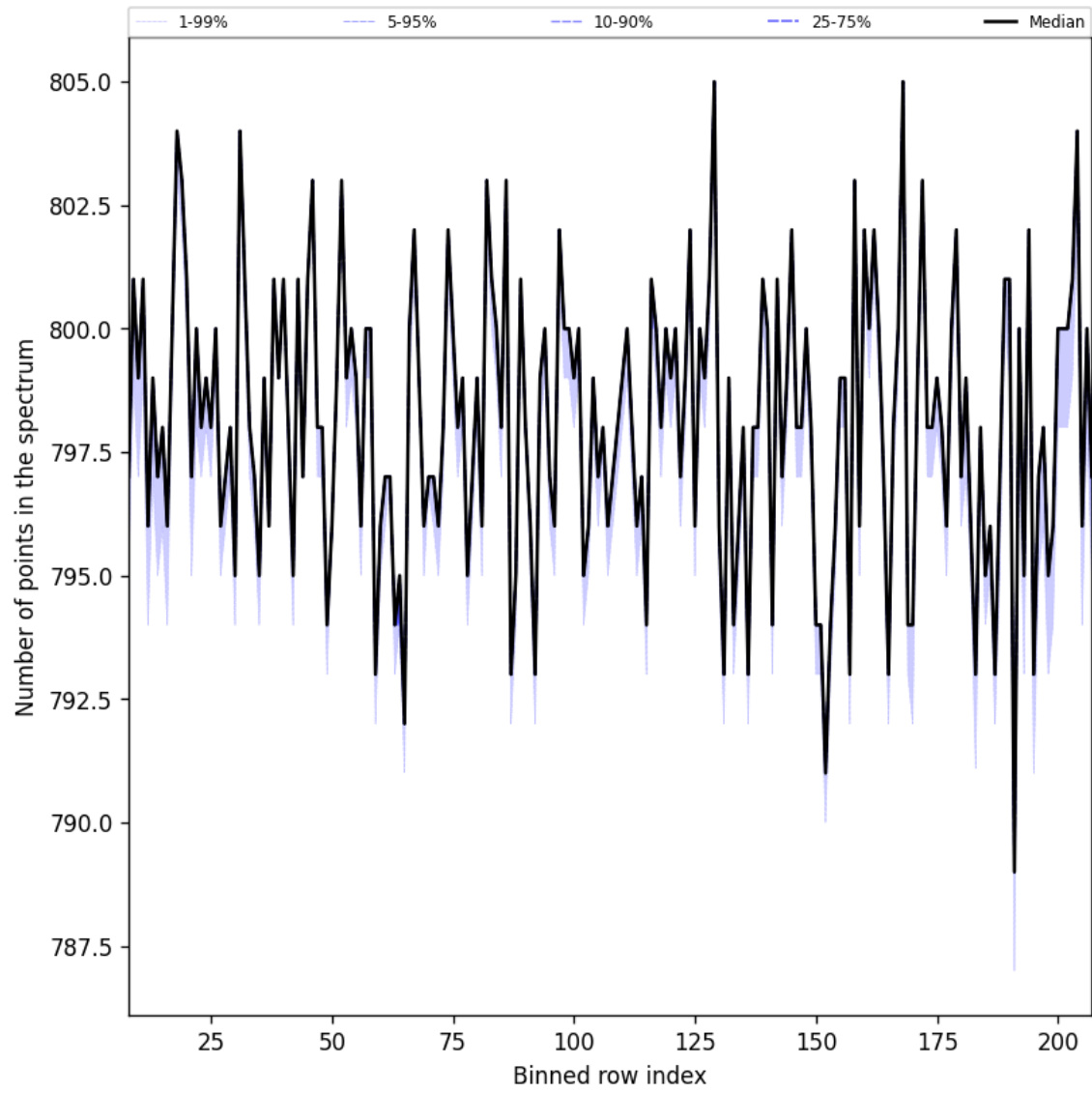
Figure 37: Along track statistics of “Number of points in the spectrum” for 2025-01-03 to 2025-01-05
