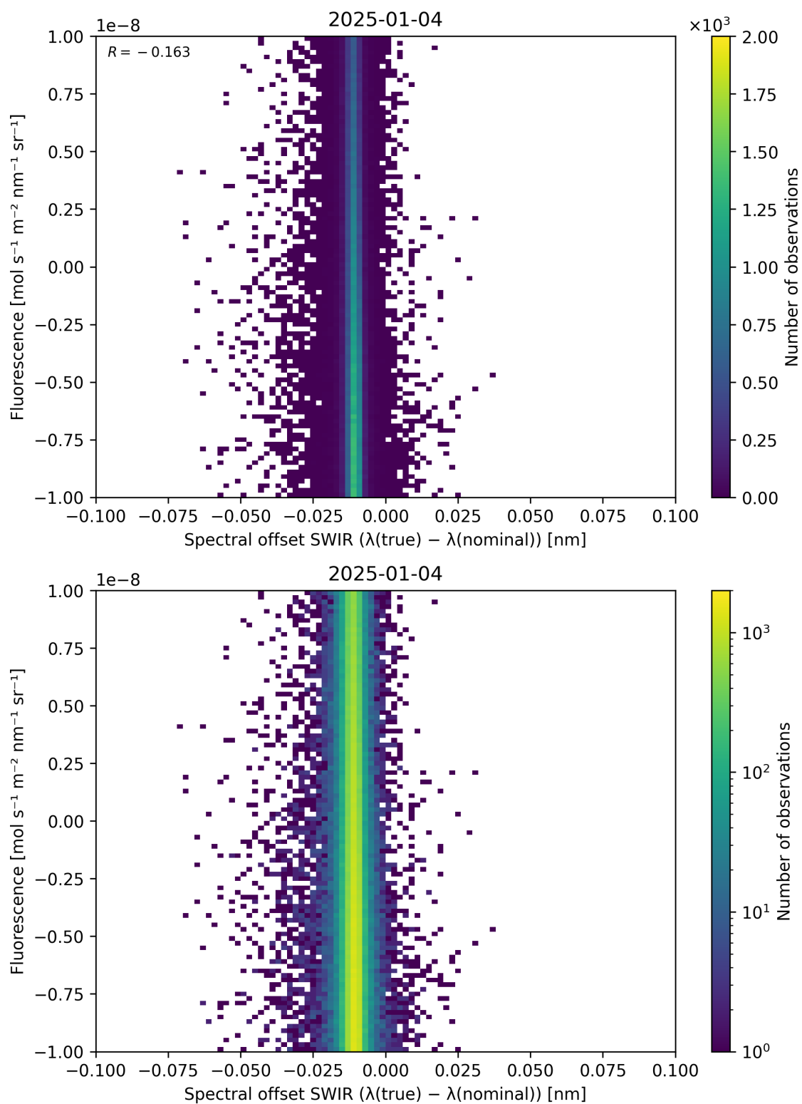
Figure 120: Scatter density plot of “Spectral offset SWIR ( \lambda_{\text{true}} - \lambda_{\text{nominal}} )” against “Fluorescence” for 2025-01-03 to 2025-01-05.
