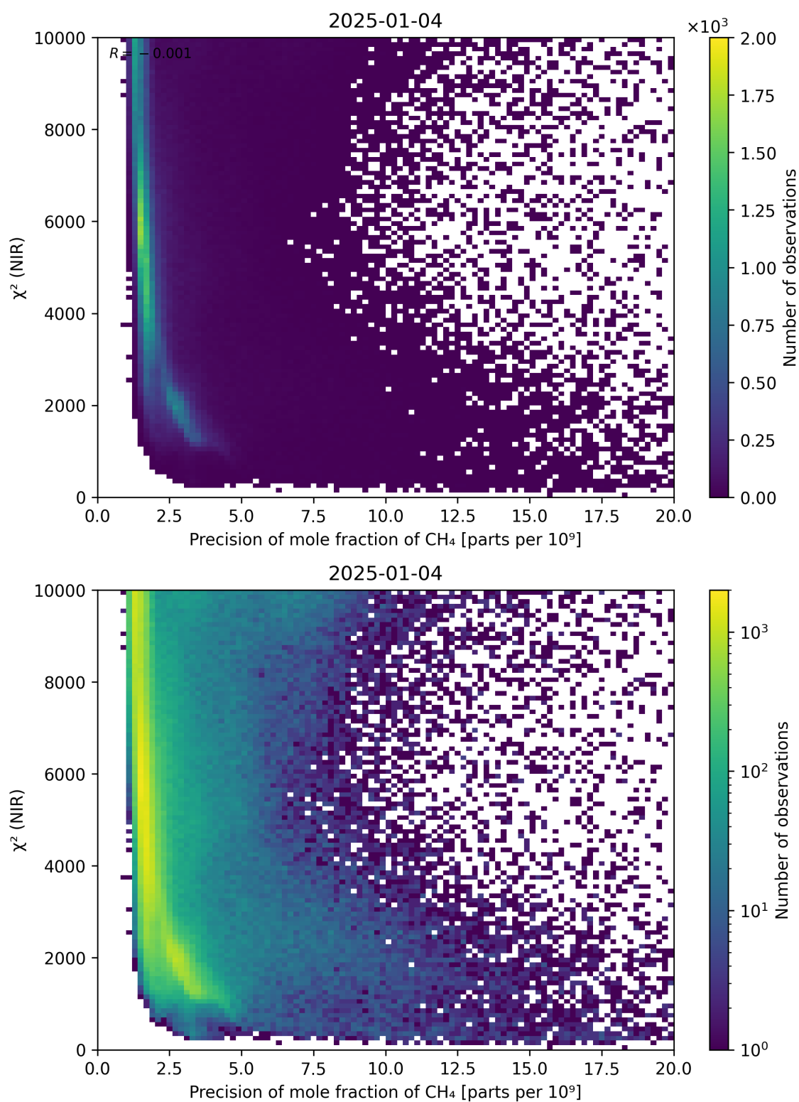
Figure 78: Scatter density plot of “Precision of mole fraction of \text{CH}_4 ” against “ \chi^2 (NIR)” for 2025-01-03 to 2025-01-05.
