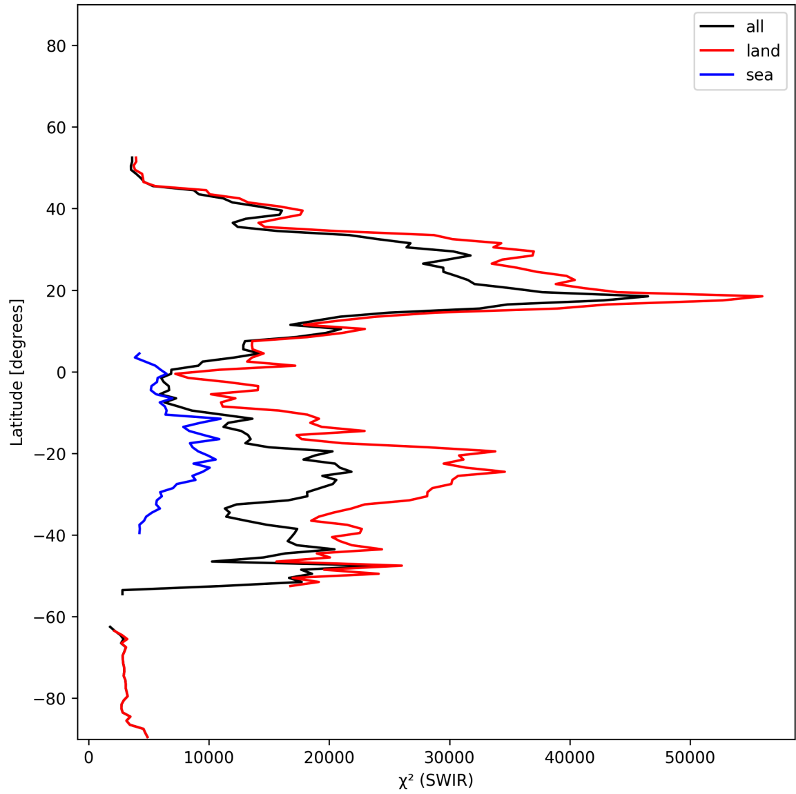
Figure 17: Zonal average of “ \chi^2 (SWIR)” for 2025-01-03 to 2025-01-05.
