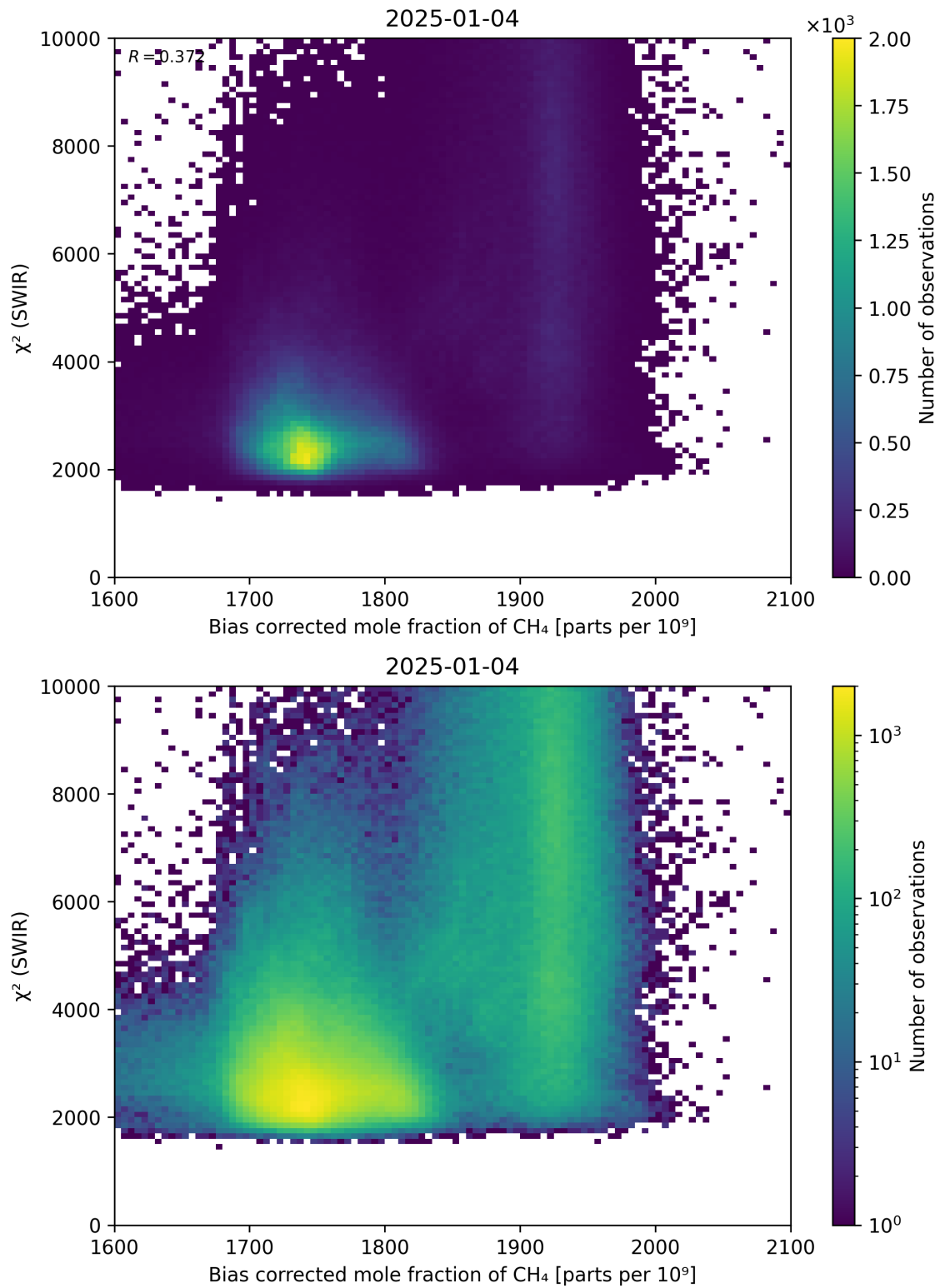
Figure 64: Scatter density plot of “Bias corrected mole fraction of \text{CH}_4 ” against “ \chi^2 (SWIR)” for 2025-01-03 to 2025-01-05.
