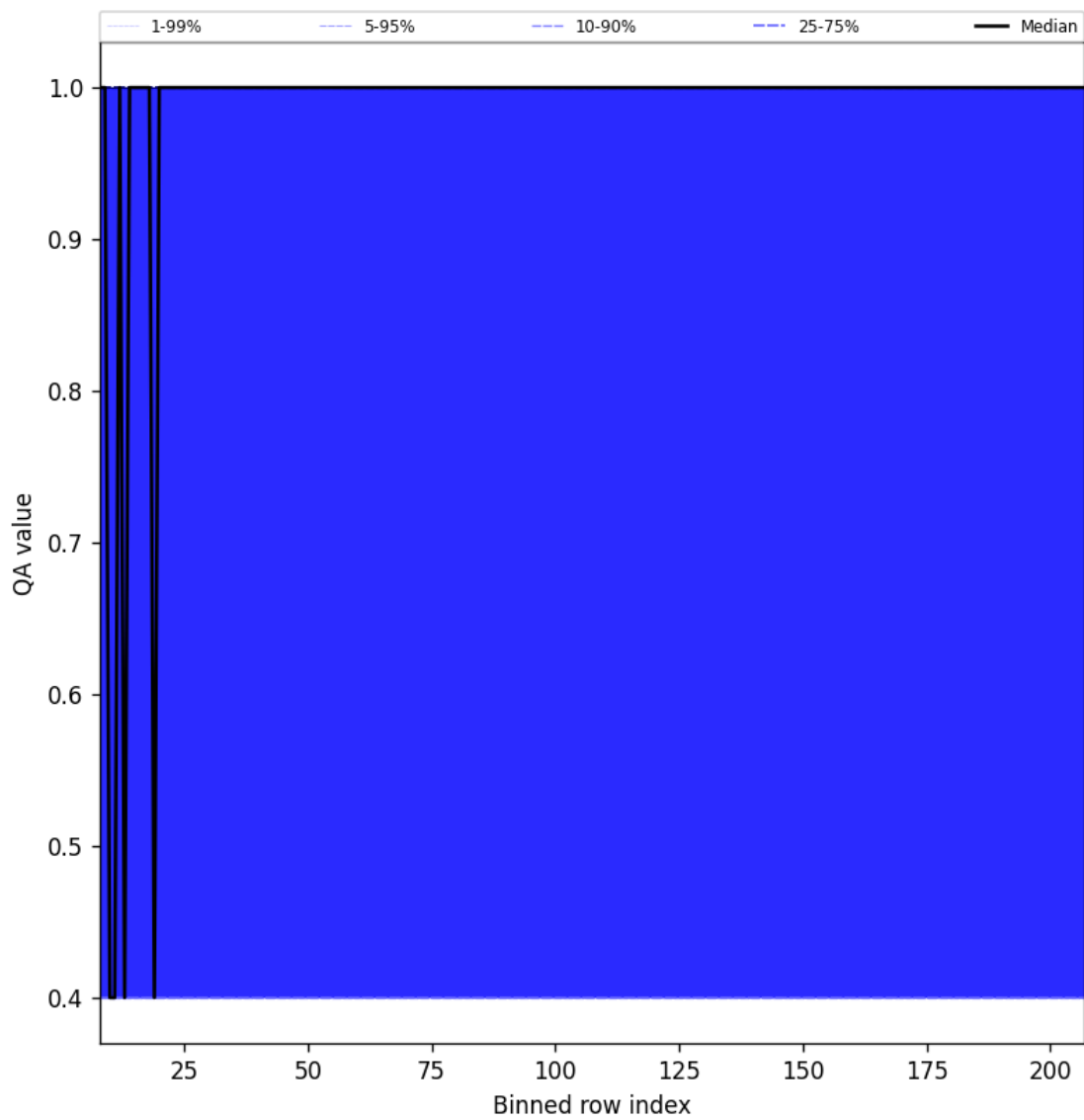
Figure 33: Along track statistics of “QA value” for 2025-01-03 to 2025-01-05
