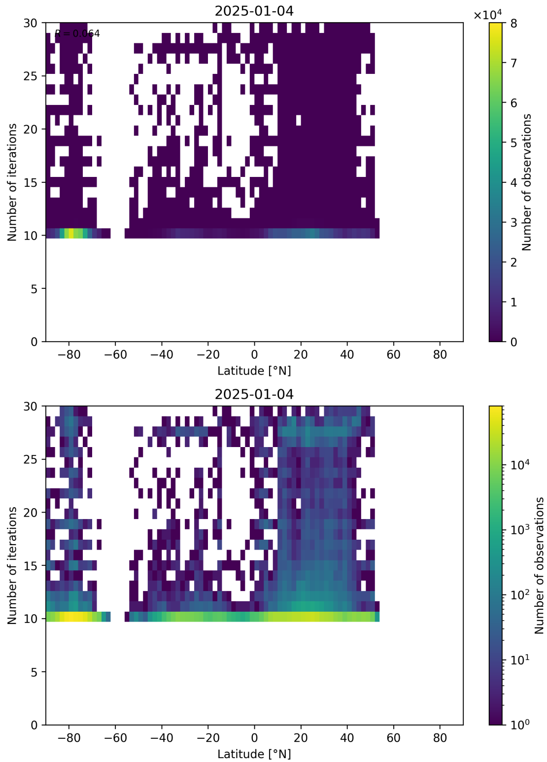
Figure 60: Scatter density plot of “Latitude” against “Number of iterations” for 2025-01-03 to 2025-01-05.
