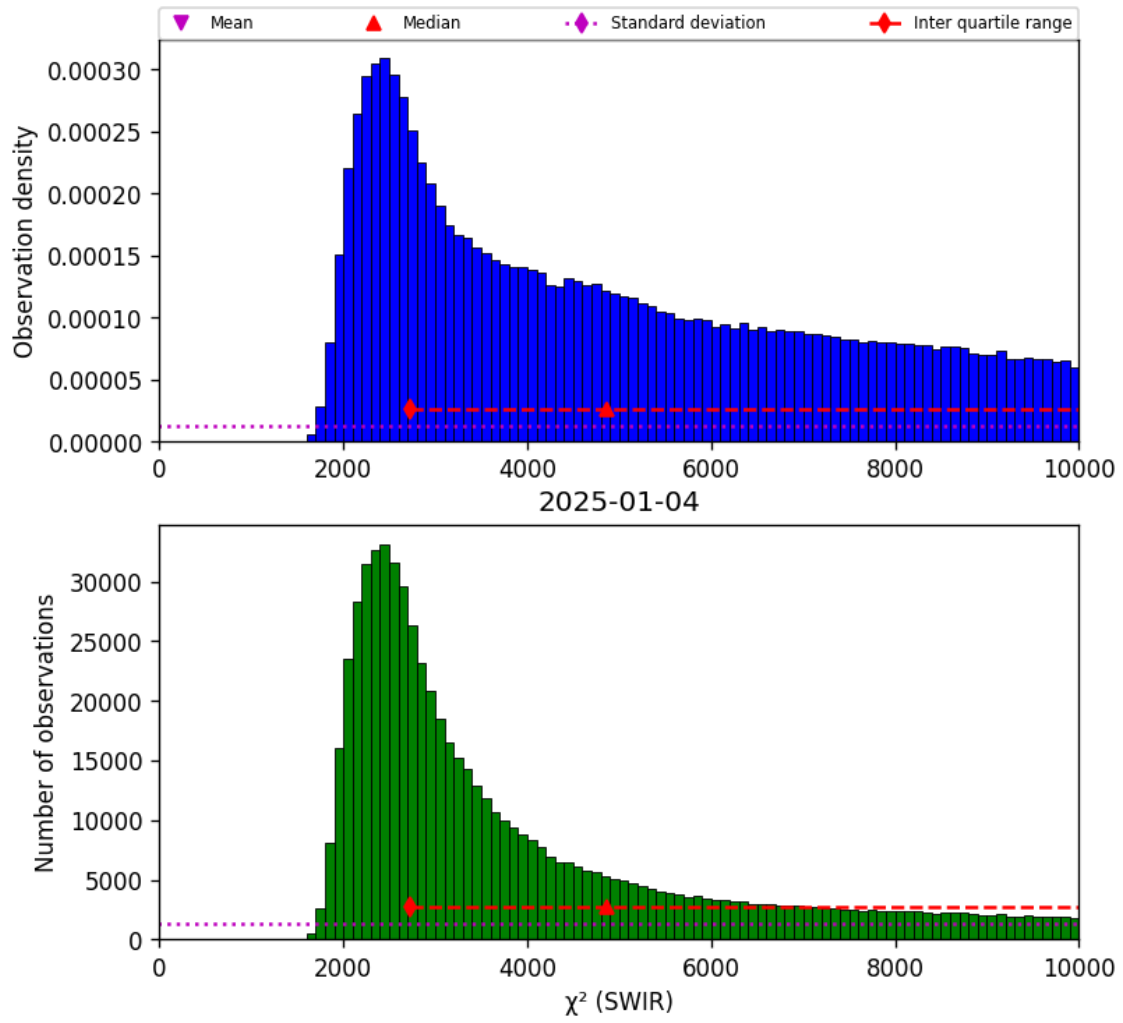
Figure 28: Histogram of " \chi^2 (SWIR)" for 2025-01-03 to 2025-01-05
