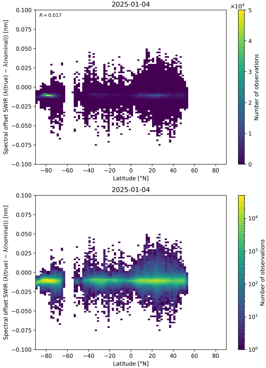
Figure 62: Scatter density plot of “Latitude” against “Spectral offset SWIR ( \lambda_{\text{true}} - \lambda_{\text{nominal}} )” for 2025-01-03 to 2025-01-05.
