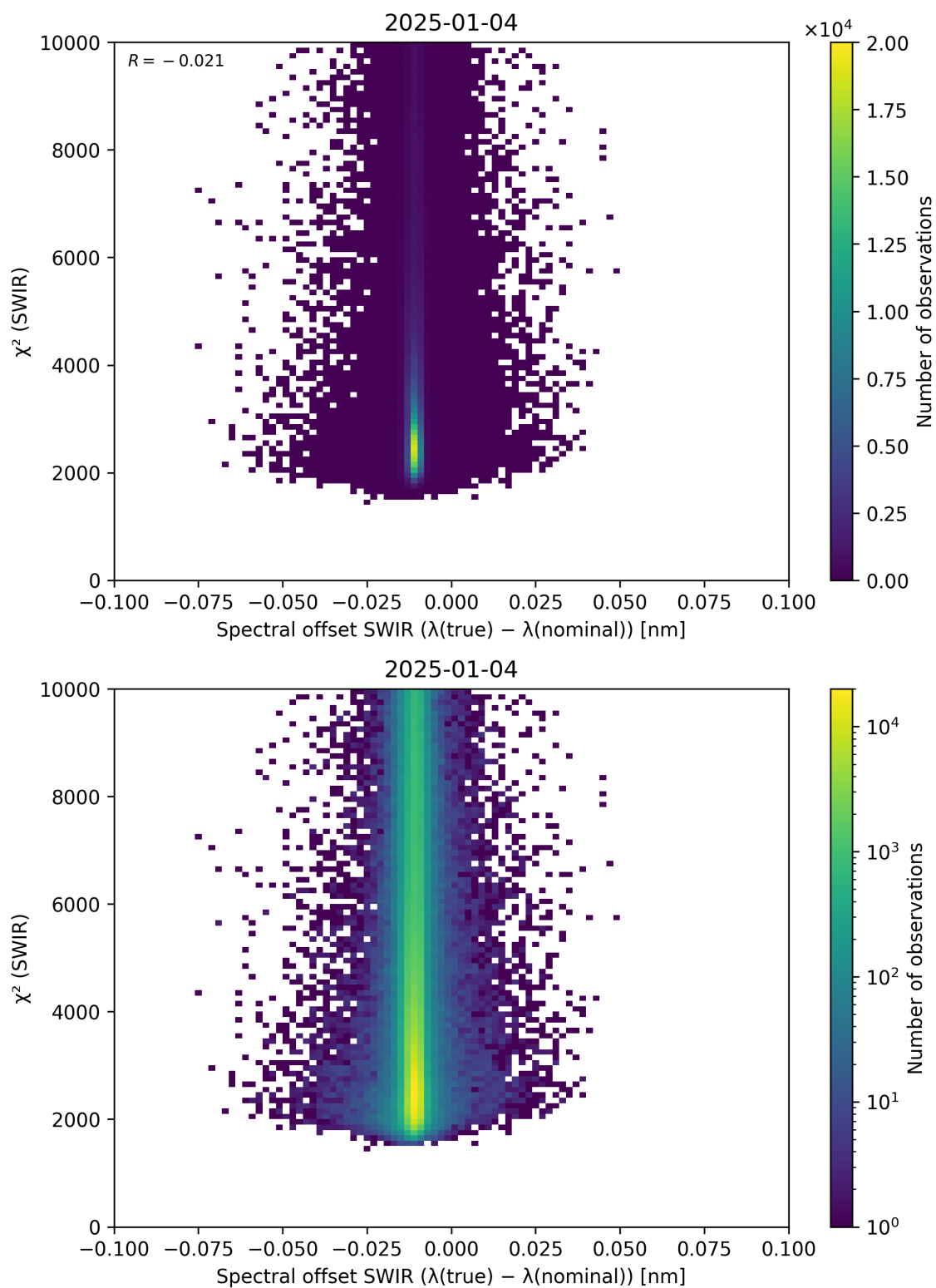
Figure 118: Scatter density plot of “Spectral offset SWIR ( \lambda_{\text{true}} - \lambda_{\text{nominal}} )” against “ \chi^2 (SWIR)” for 2025-01-03 to 2025-01-05.
