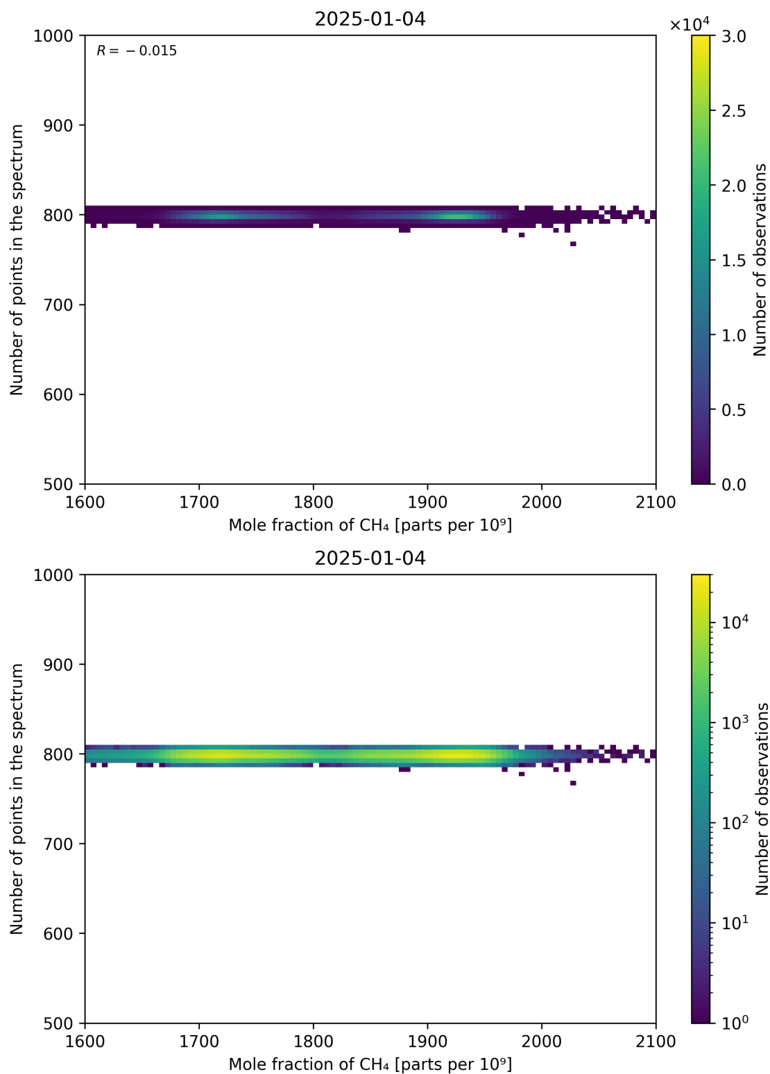
Figure 77: Scatter density plot of “Mole fraction of CH 4 ” against “Number of points in the spectrum” for 2025-01-03 to 2025-01-05.
