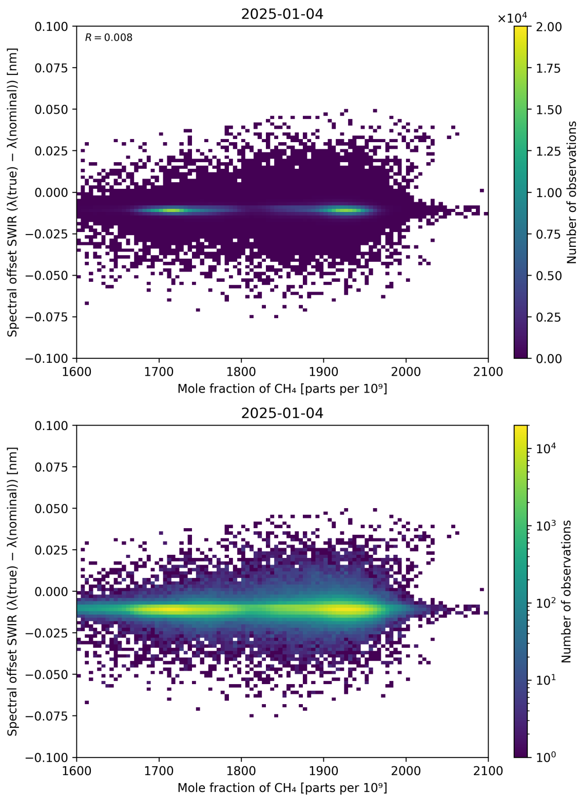
Figure 86: Scatter density plot of “Mole fraction of \text{CH}_4 ” against “Spectral offset SWIR ( \lambda_{\text{true}} - \lambda_{\text{nominal}} )” for 2025-01-03 to 2025-01-05.
