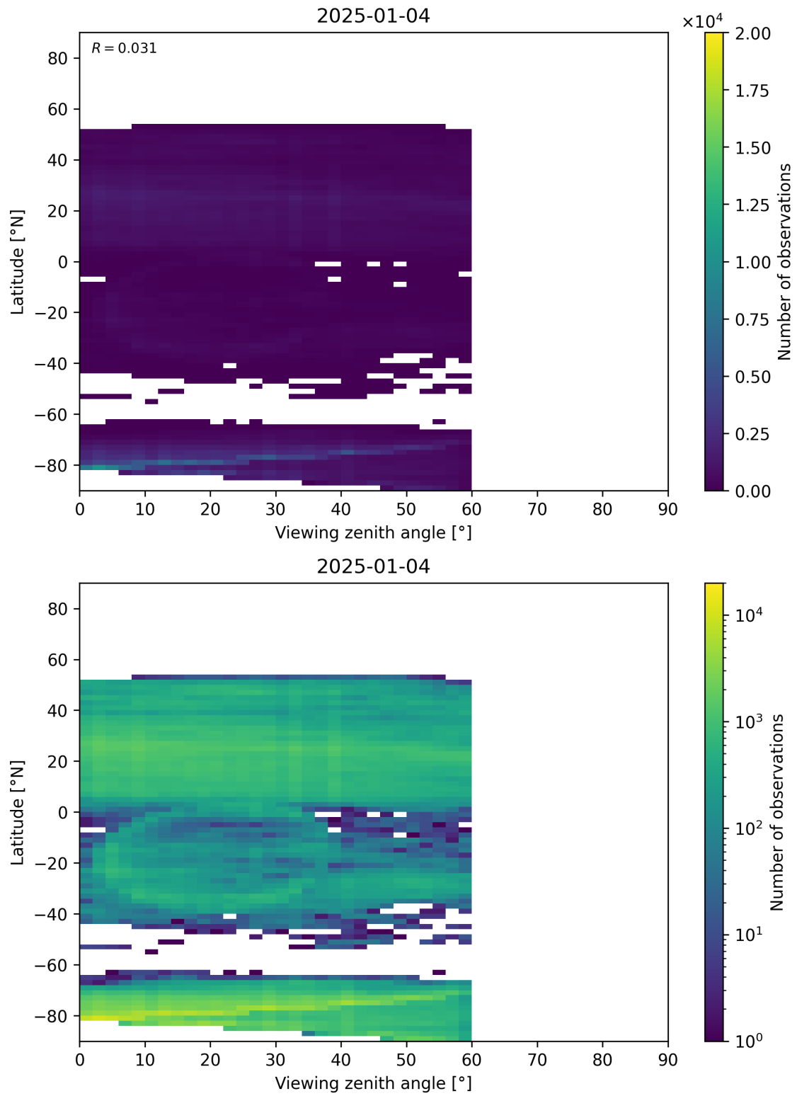
Figure 109: Scatter density plot of “Viewing zenith angle” against “Latitude” for 2025-01-03 to 2025-01-05.
