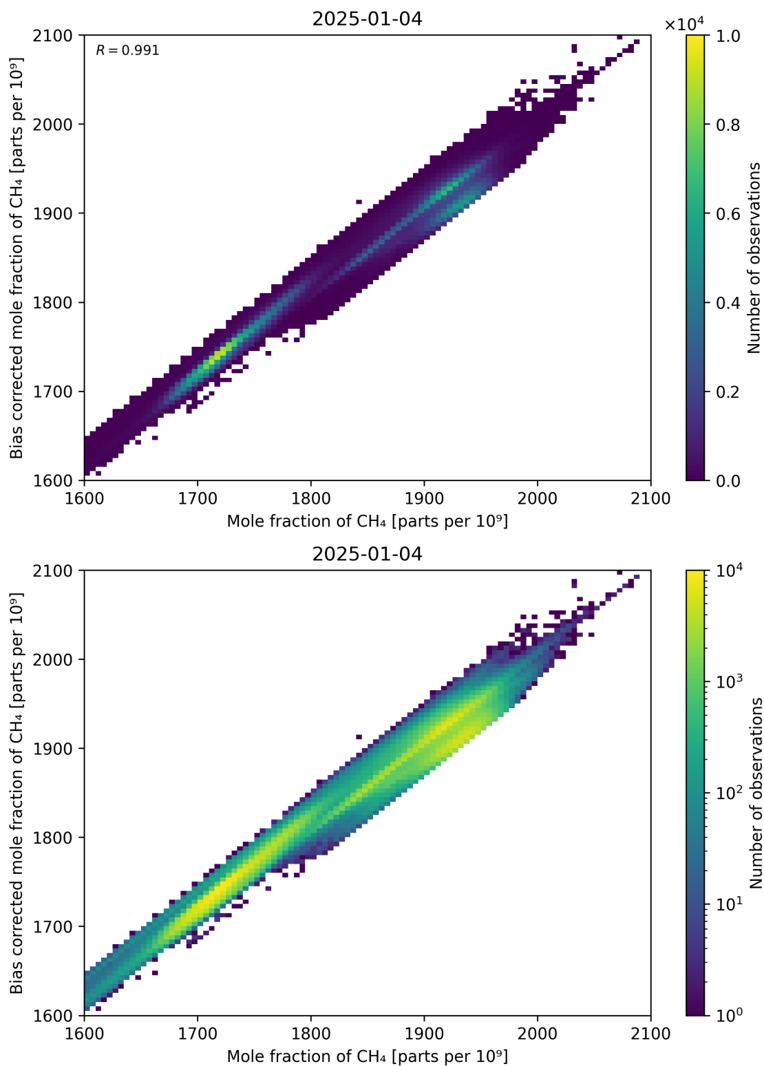
Figure 74: Scatter density plot of “Mole fraction of CH 4 ” against “Bias corrected mole fraction of CH 4 ” for 2025-01-03 to 2025-01-05.
