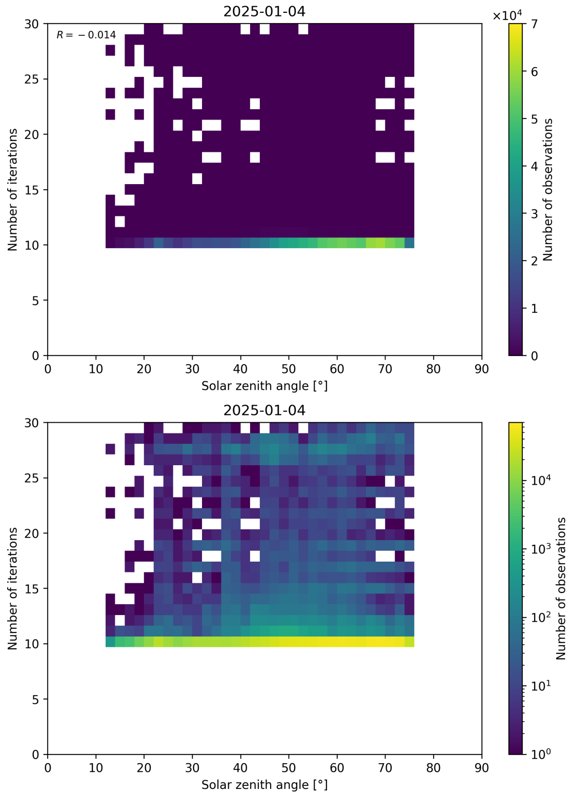
Figure 102: Scatter density plot of “Solar zenith angle” against “Number of iterations” for 2025-01-03 to 2025-01-05.
