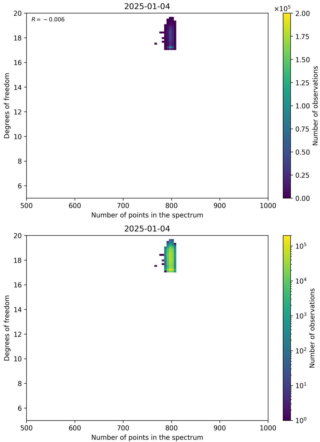
Figure 90: Scatter density plot of “Number of points in the spectrum” against “Degrees of freedom” for 2025-01-03 to 2025-01-05.
