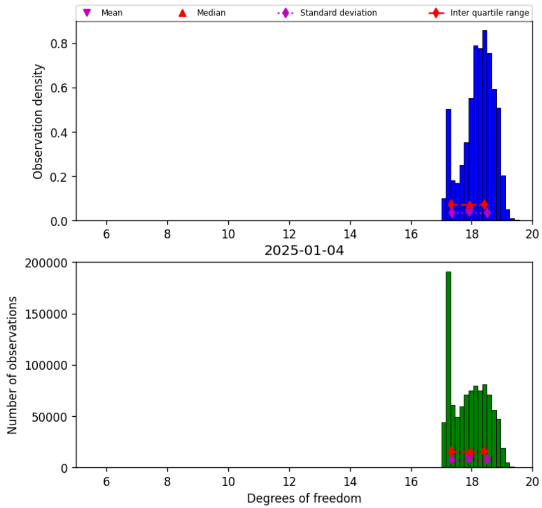
Figure 30: Histogram of “Degrees of freedom” for 2025-01-03 to 2025-01-05
