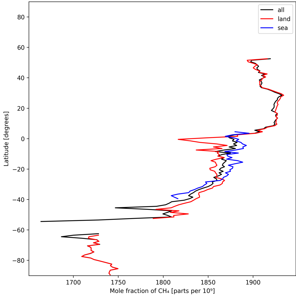
Figure 12: Zonal average of “Mole fraction of CH 4 ” for 2025-01-03 to 2025-01-05.
