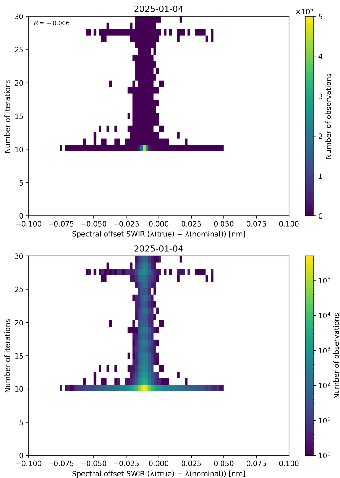
Figure 121: Scatter density plot of “Spectral offset SWIR ( \lambda_{\text{true}} - \lambda_{\text{nominal}} )” against “Number of iterations” for 2025-01-03 to 2025-01-05.
