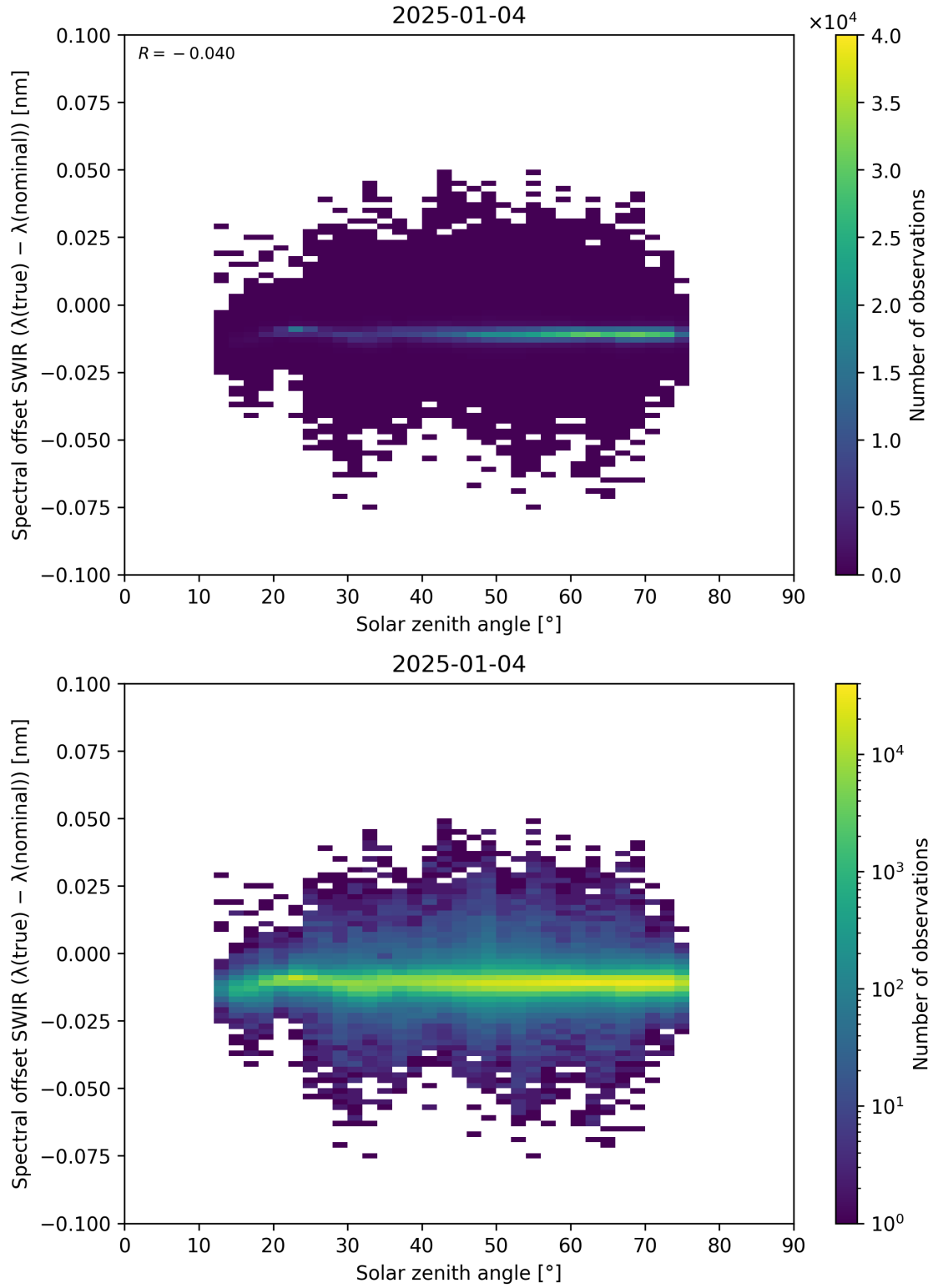
Figure 104: Scatter density plot of “Solar zenith angle” against “Spectral offset SWIR ( \lambda_{\text{true}} - \lambda_{\text{nominal}} )” for 2025-01-03 to 2025-01-05.
