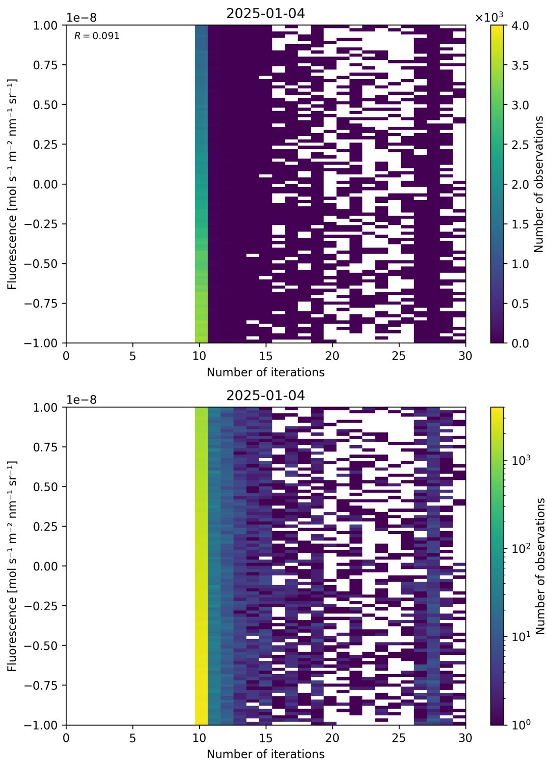
Figure 87: Scatter density plot of "Number of iterations" against "Fluorescence" for 2025-01-03 to 2025-01-05.
