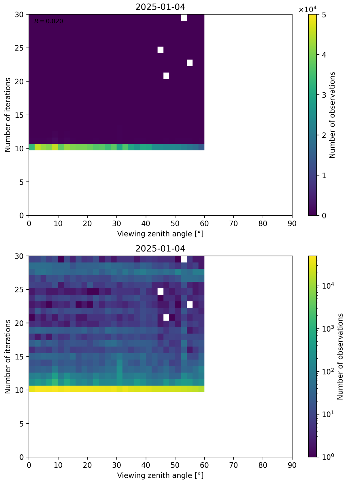
Figure 113: Scatter density plot of “Viewing zenith angle” against “Number of iterations” for 2025-01-03 to 2025-01-05.
