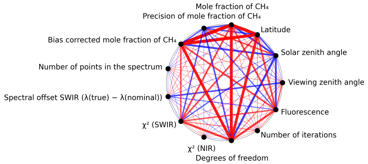
Figure 1: Map of correlation graph for 2025-01-03 to 2025-01-05.
