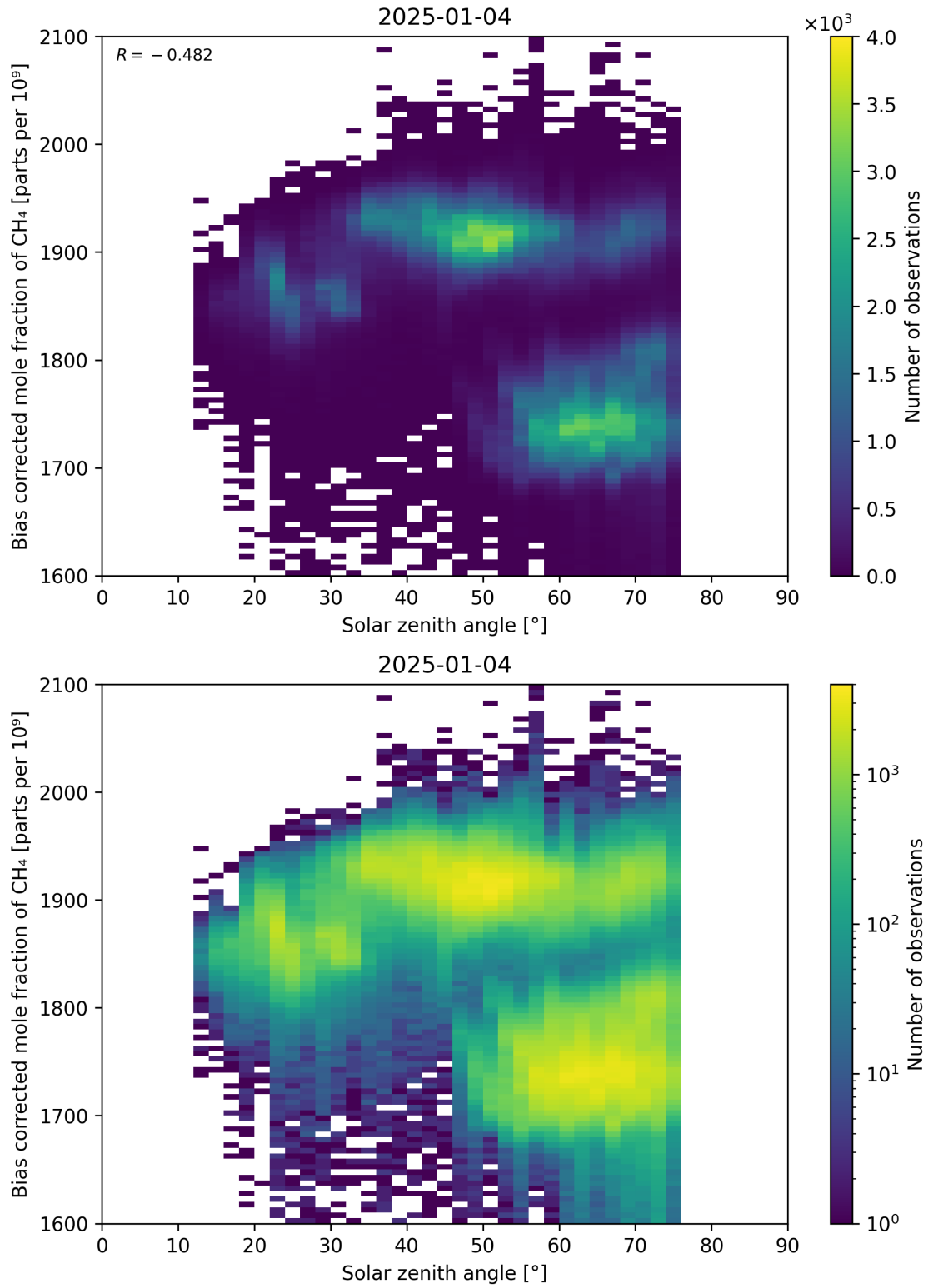
Figure 100: Scatter density plot of “Solar zenith angle” against “Bias corrected mole fraction of CH 4 ” for 2025-01-03 to 2025-01-05.
