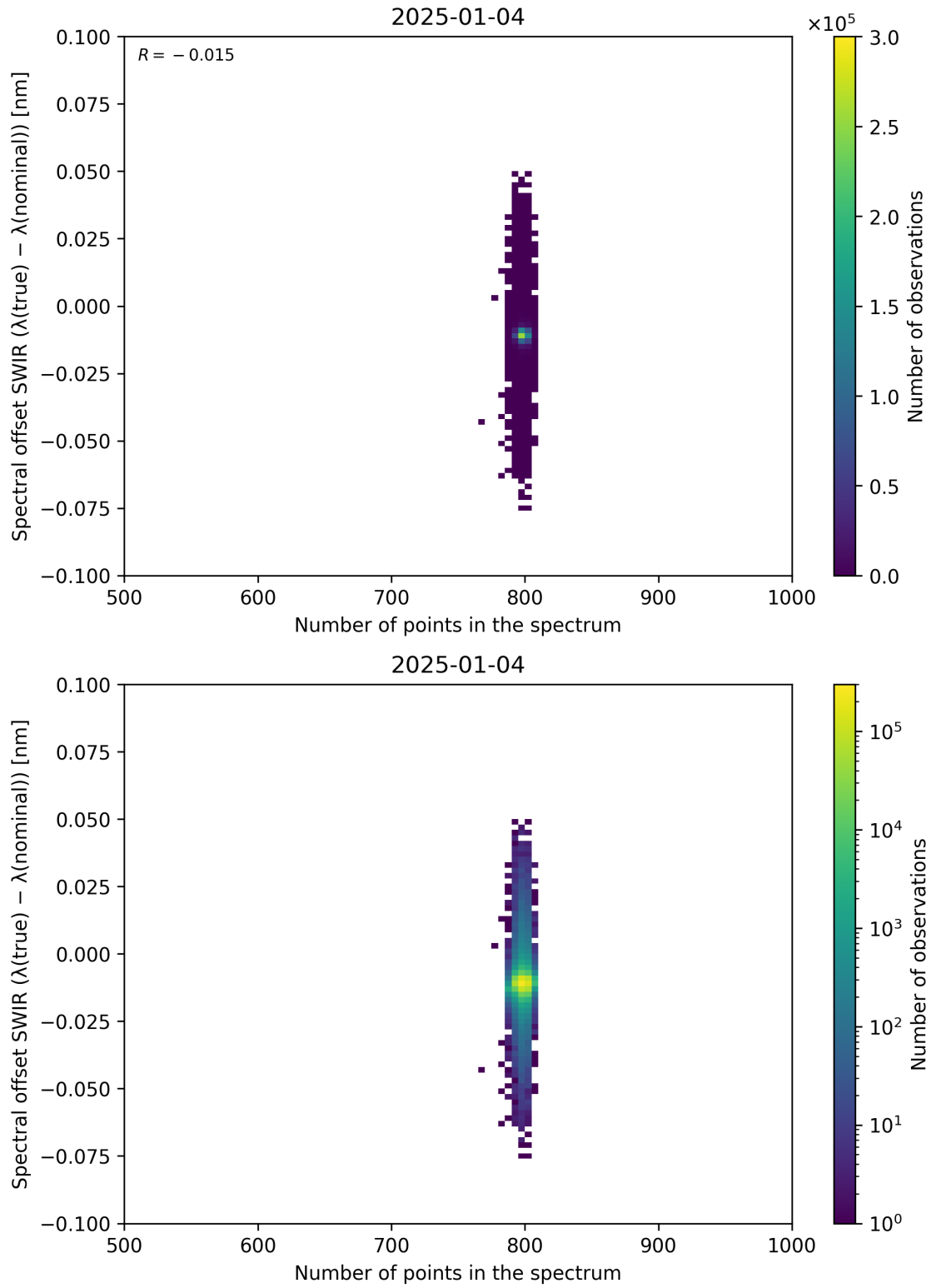
Figure 93: Scatter density plot of “Number of points in the spectrum” against “Spectral offset SWIR ( \lambda_{\text{true}} - \lambda_{\text{nominal}} )” for 2025-01-03 to 2025-01-05.
