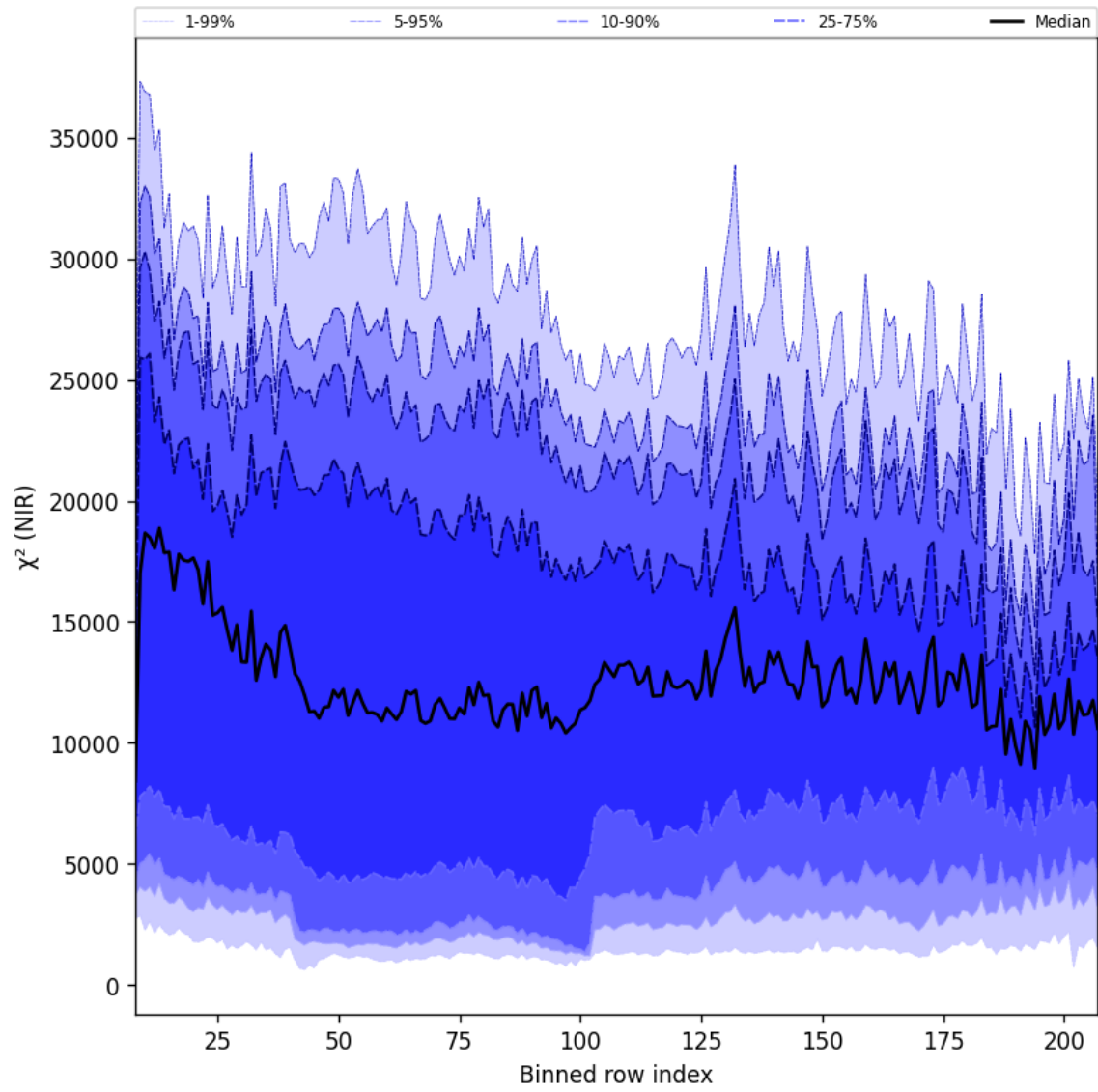
Figure 40: Along track statistics of “ \chi^2 (NIR)” for 2025-01-03 to 2025-01-05
