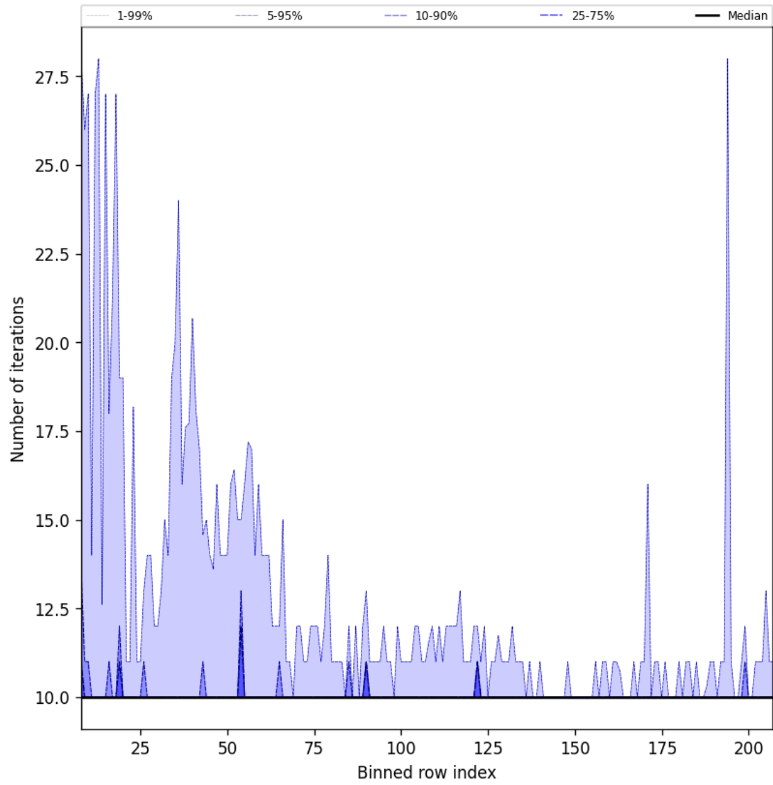
Figure 42: Along track statistics of “Number of iterations” for 2025-01-03 to 2025-01-05
