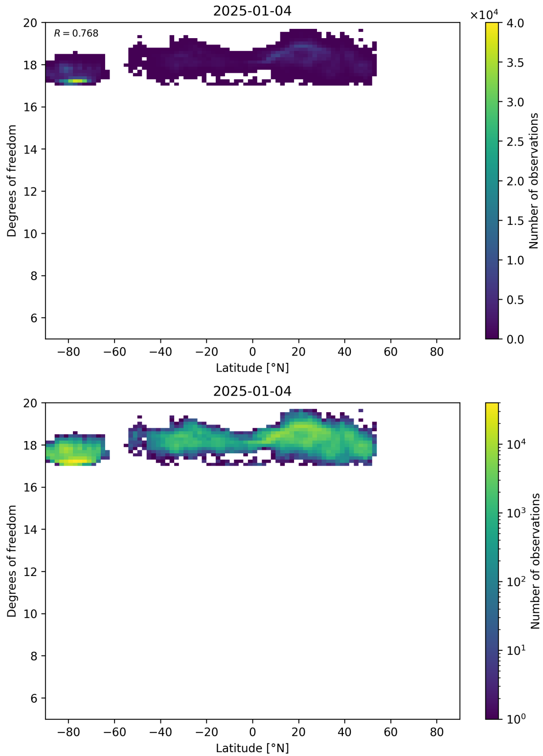
Figure 55: Scatter density plot of “Latitude” against “Degrees of freedom” for 2025-01-03 to 2025-01-05.
