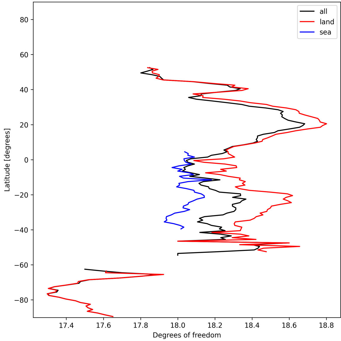
Figure 19: Zonal average of “Degrees of freedom” for 2025-01-03 to 2025-01-05.
