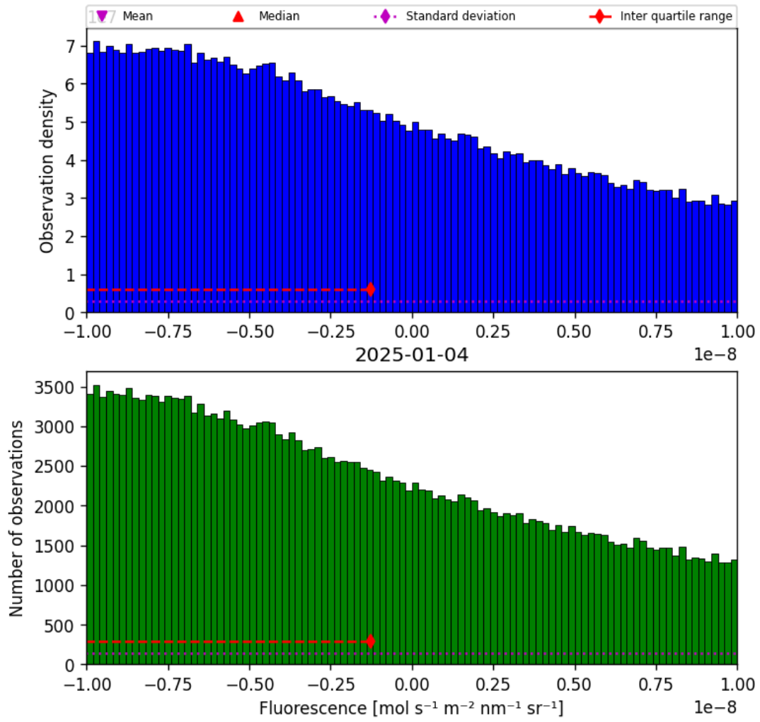
Figure 32: Histogram of “Fluorescence” for 2025-01-03 to 2025-01-05
