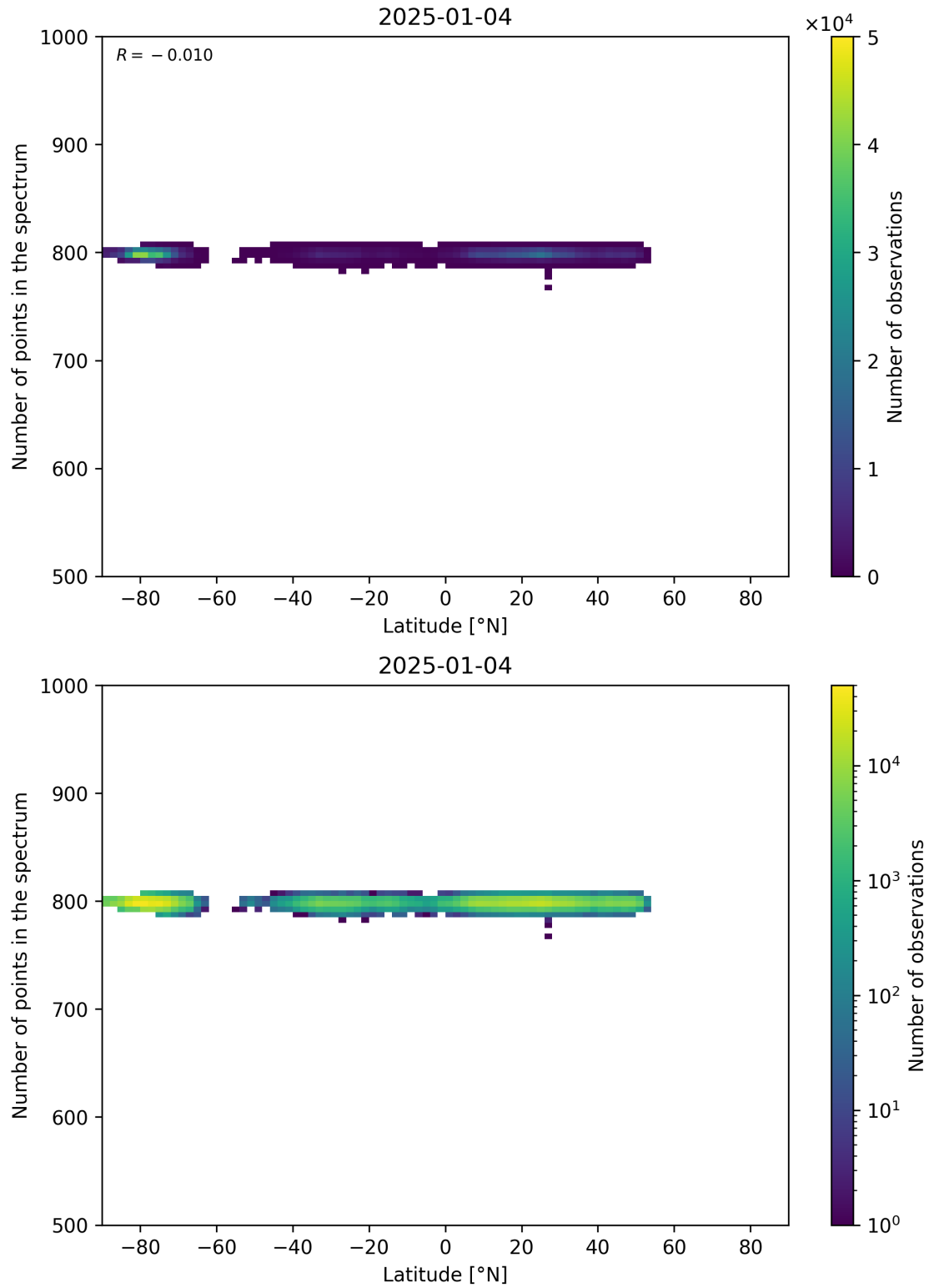
Figure 61: Scatter density plot of “Latitude” against “Number of points in the spectrum” for 2025-01-03 to 2025-01-05.
