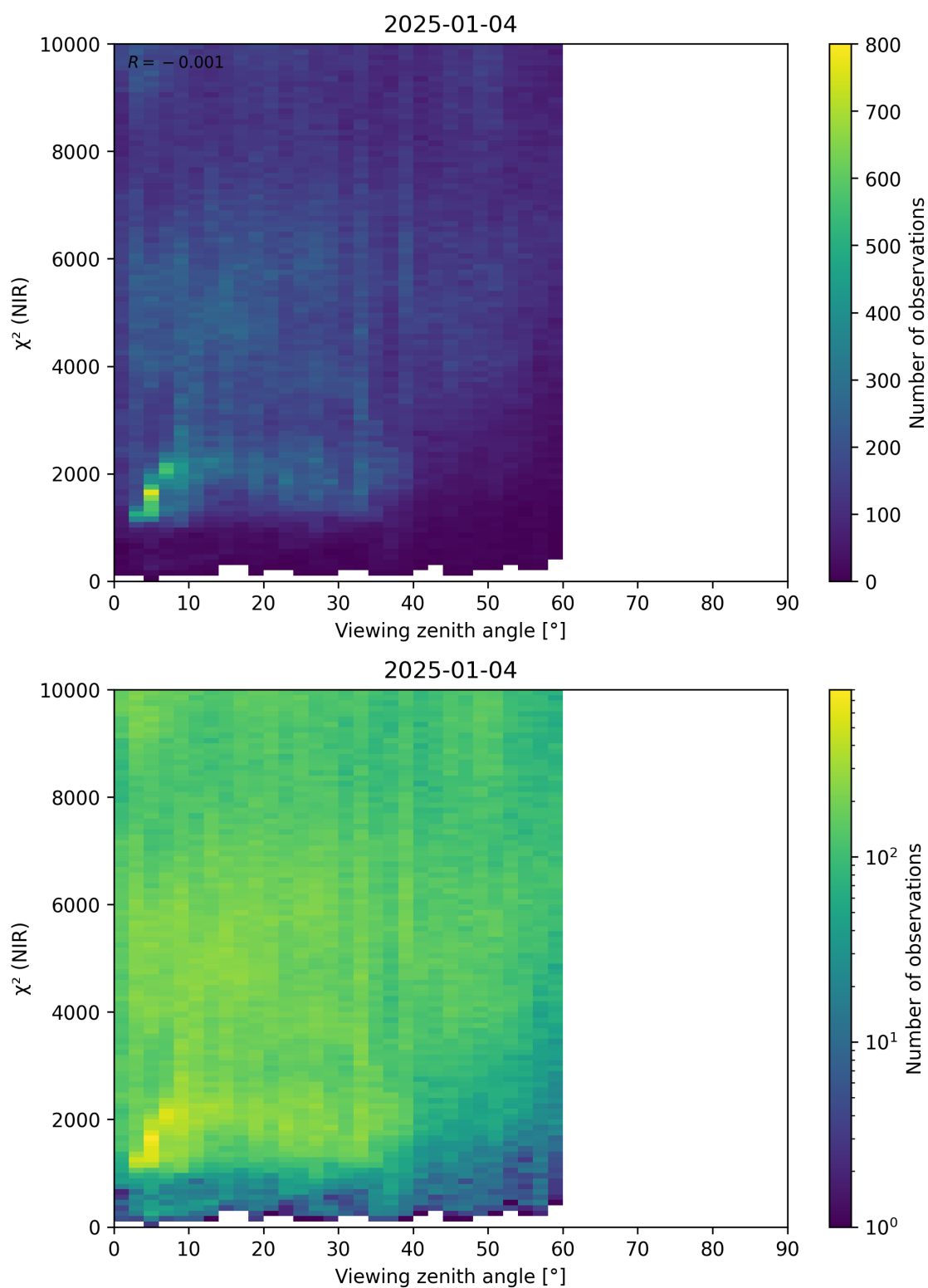
Figure 105: Scatter density plot of “Viewing zenith angle” against “ \chi^2 (NIR)” for 2025-01-03 to 2025-01-05.
