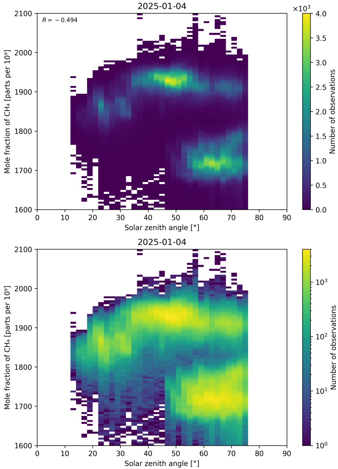
Figure 99: Scatter density plot of “Solar zenith angle” against “Mole fraction of CH 4 ” for 2025-01-03 to 2025-01-05.
