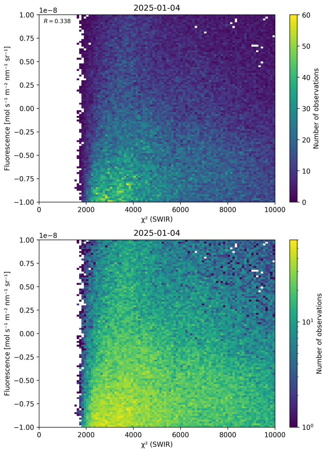
Figure 49: Scatter density plot of “ \chi^2 (SWIR)” against “Fluorescence” for 2025-01-03 to 2025-01-05.
