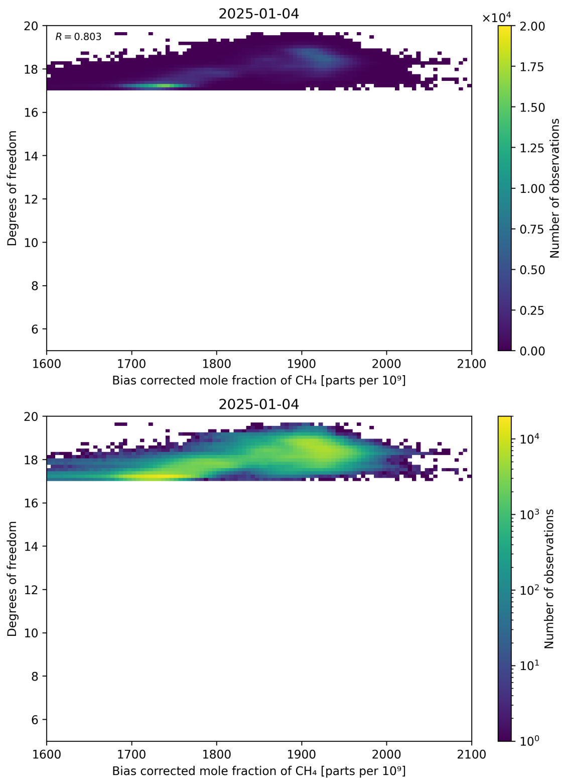
Figure 65: Scatter density plot of “Bias corrected mole fraction of CH 4 ” against “Degrees of freedom” for 2025-01-03 to 2025-01-05.
