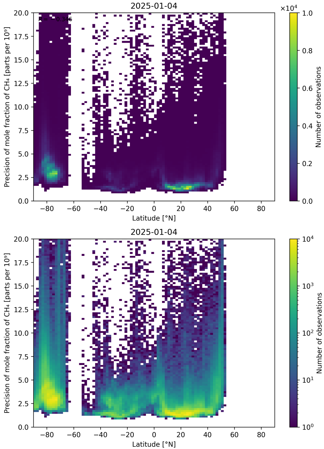
Figure 59: Scatter density plot of “Latitude” against “Precision of mole fraction of CH 4 ” for 2025-01-03 to 2025-01-05.
