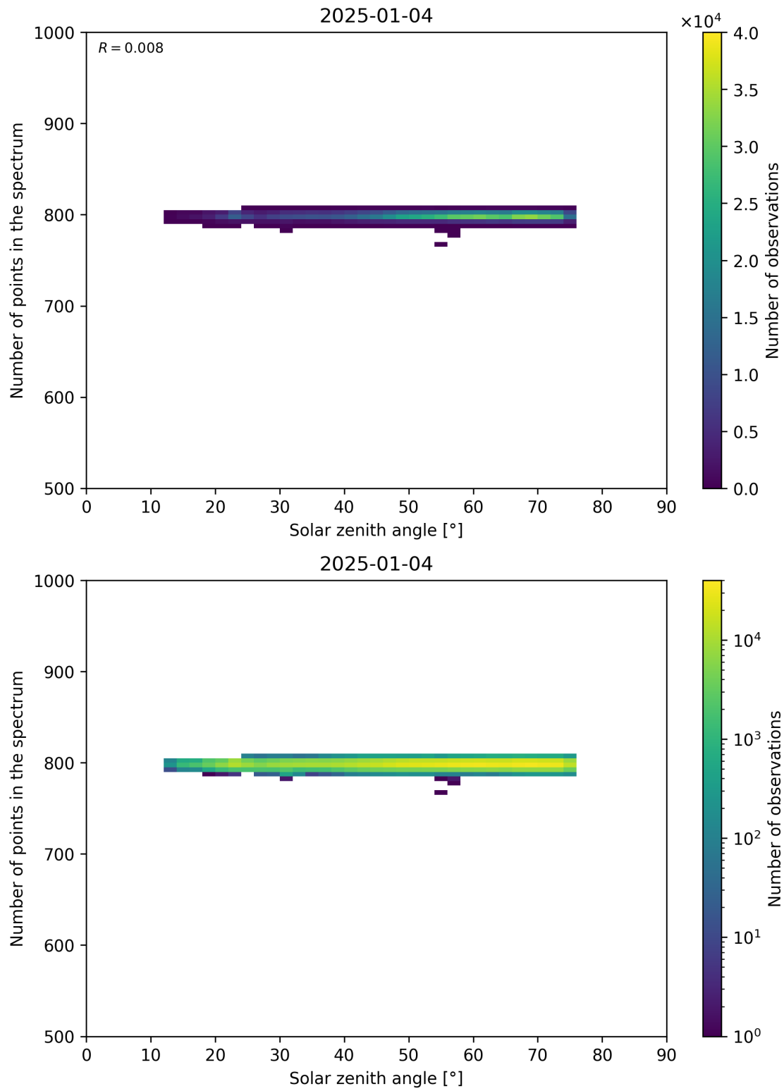
Figure 103: Scatter density plot of “Solar zenith angle” against “Number of points in the spectrum” for 2025-01-03 to 2025-01-05.
