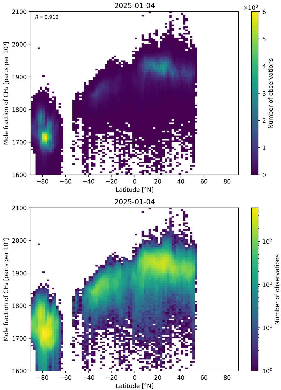
Figure 57: Scatter density plot of “Latitude” against “Mole fraction of CH 4 ” for 2025-01-03 to 2025-01-05.
