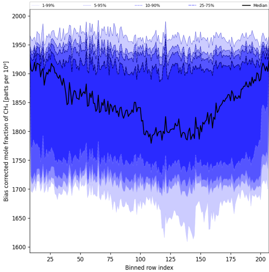
Figure 36: Along track statistics of “Bias corrected mole fraction of CH 4 ” for 2025-01-04 to 2025-01-06
