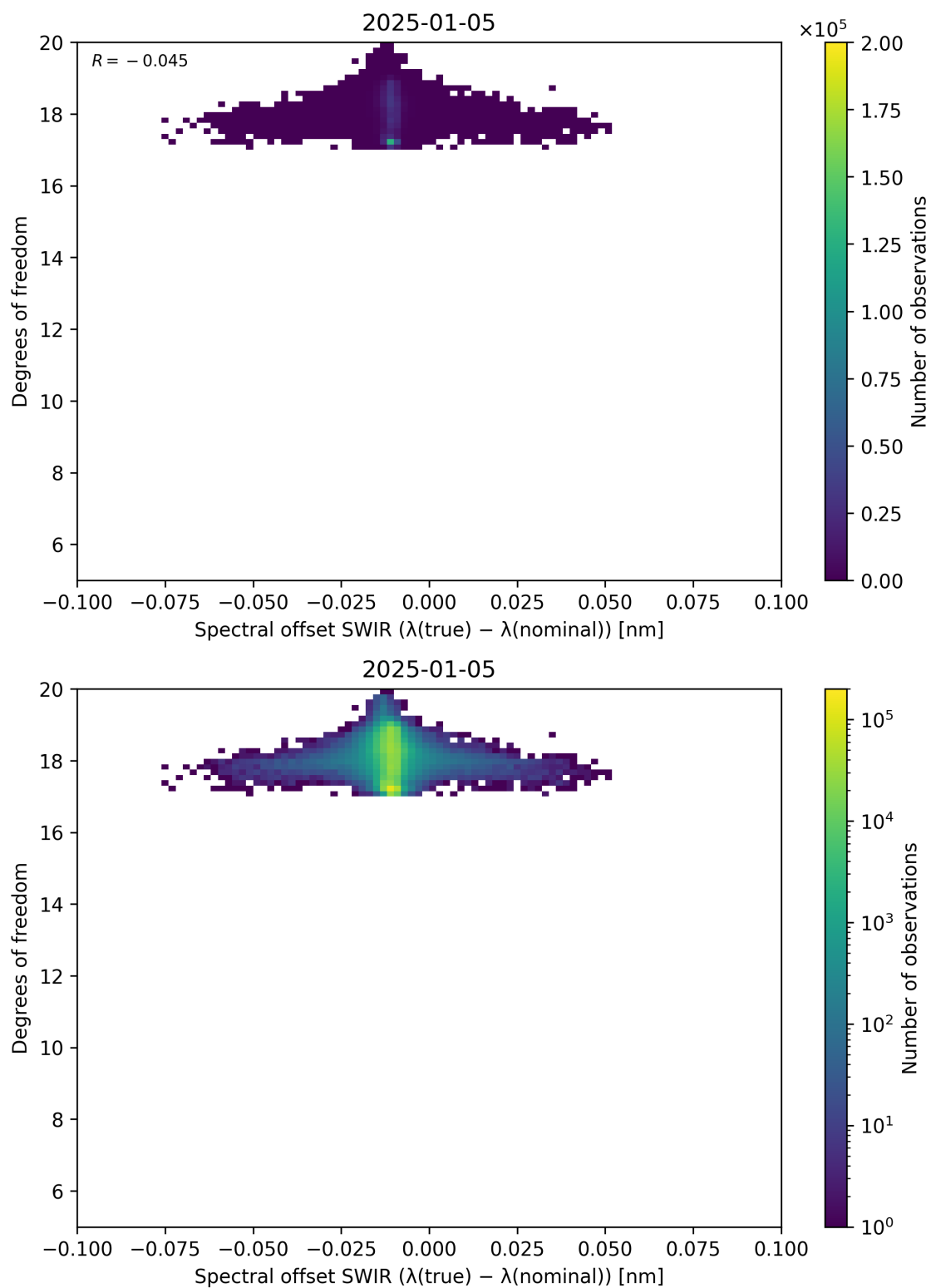
Figure 119: Scatter density plot of “Spectral offset SWIR ( \lambda_{\text{true}} - \lambda_{\text{nominal}} )” against “Degrees of freedom” for 2025-01-04 to 2025-01-06.
