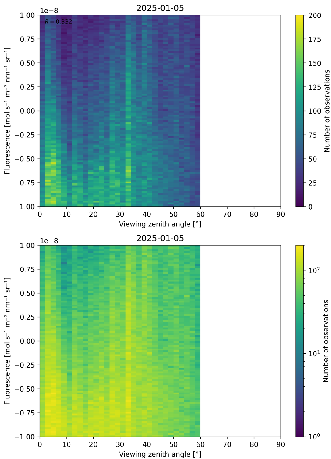
Figure 108: Scatter density plot of “Viewing zenith angle” against “Fluorescence” for 2025-01-04 to 2025-01-06.
