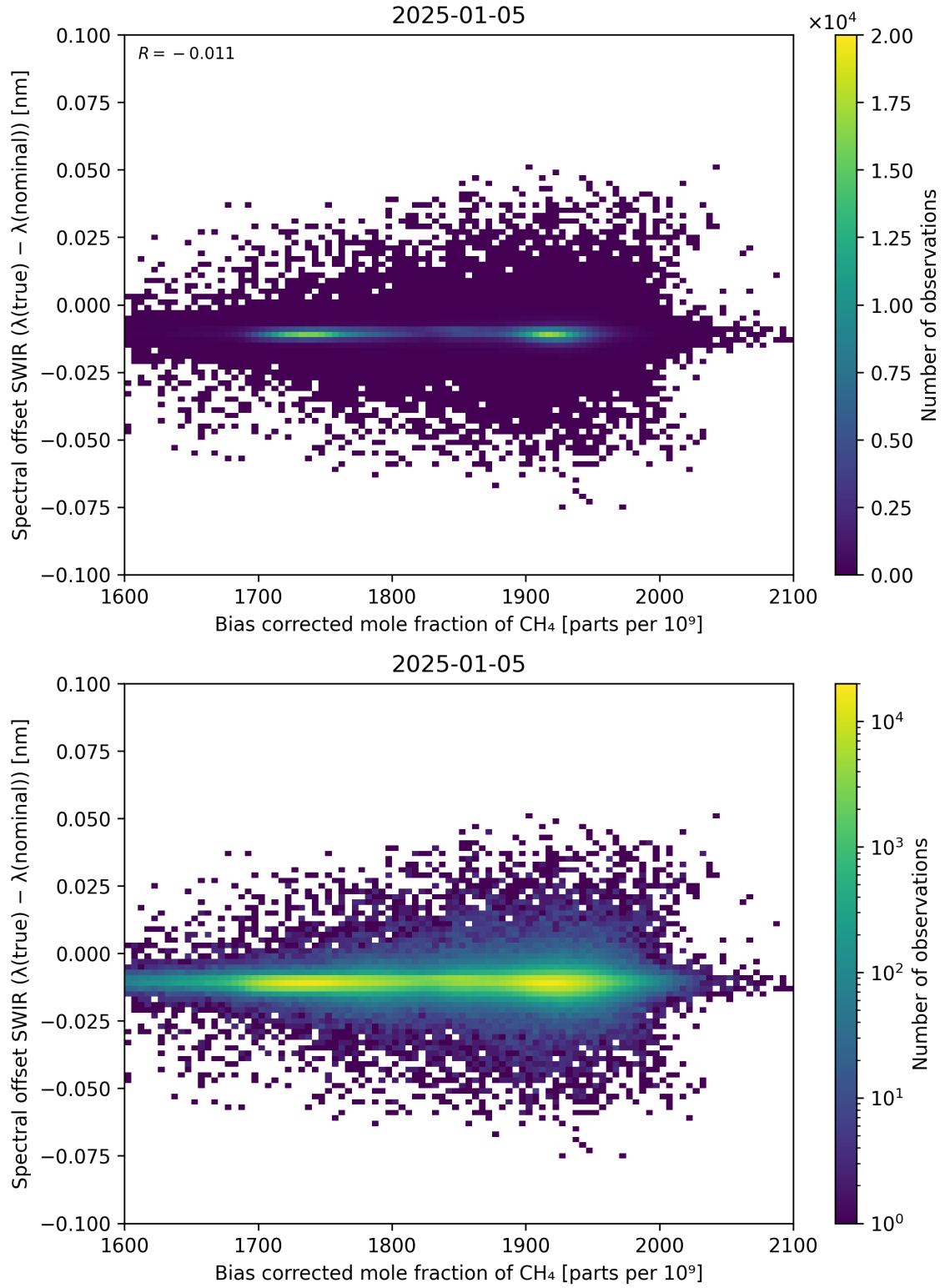
Figure 69: Scatter density plot of “Bias corrected mole fraction of \text{CH}_4 ” against “Spectral offset SWIR ( \lambda_{\text{true}} - \lambda_{\text{nominal}} )” for 2025-01-04 to 2025-01-06.
