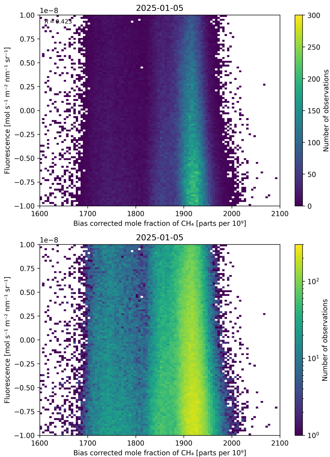
Figure 66: Scatter density plot of “Bias corrected mole fraction of \text{CH}_4 ” against “Fluorescence” for 2025-01-04 to 2025-01-06.
