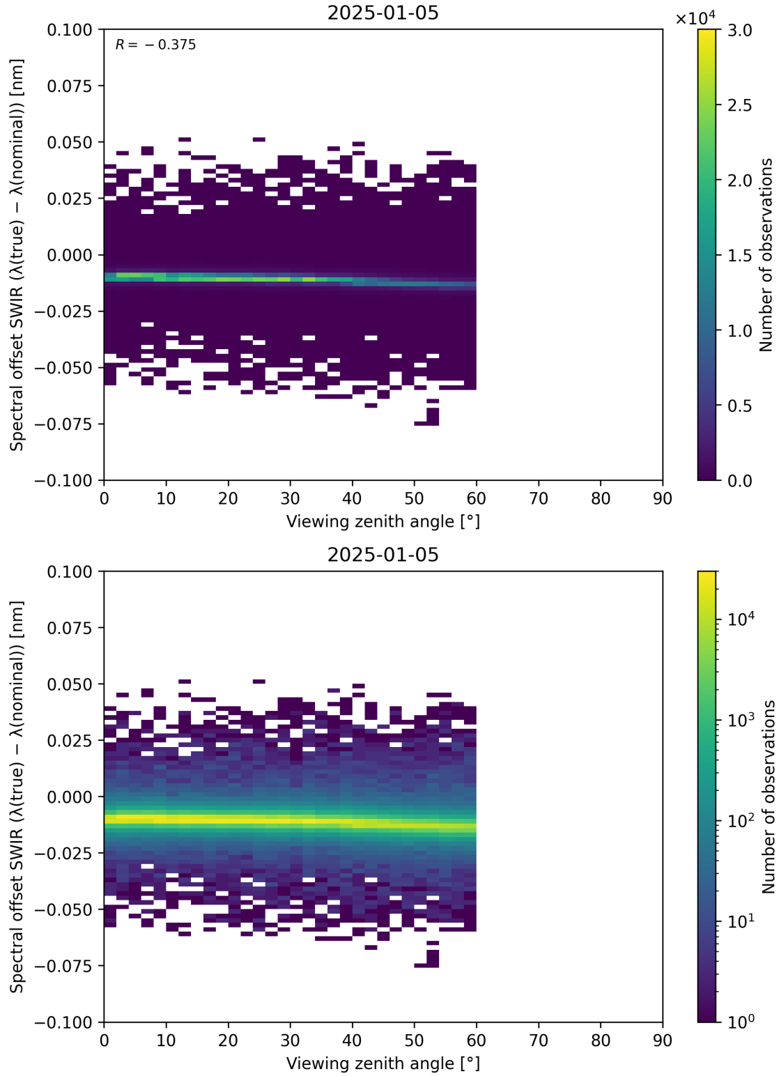
Figure 116: Scatter density plot of “Viewing zenith angle” against “Spectral offset SWIR ( \lambda_{\text{true}} - \lambda_{\text{nominal}} )” for 2025-01-04 to 2025-01-06.
