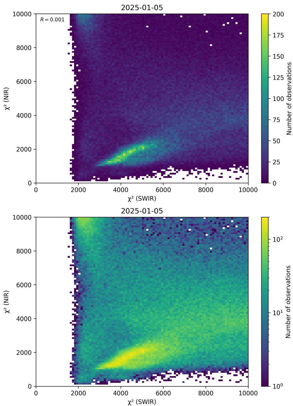
Figure 47: Scatter density plot of “ \chi^2 (SWIR)” against “ \chi^2 (NIR)” for 2025-01-04 to 2025-01-06.
