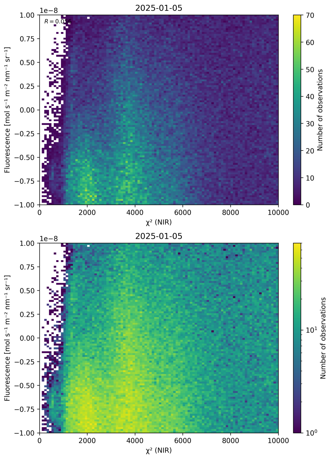
Figure 45: Scatter density plot of “ \chi^2 (NIR)” against “Fluorescence” for 2025-01-04 to 2025-01-06.
