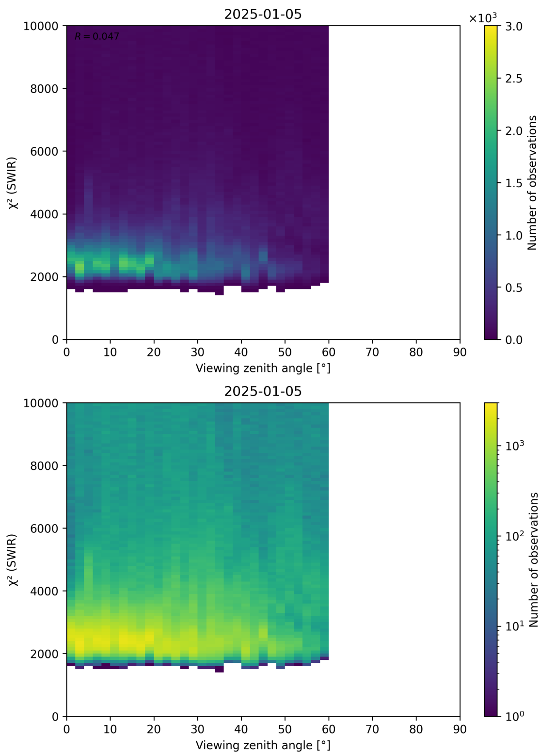
Figure 106: Scatter density plot of “Viewing zenith angle” against “ \chi^2 (SWIR)” for 2025-01-04 to 2025-01-06.
