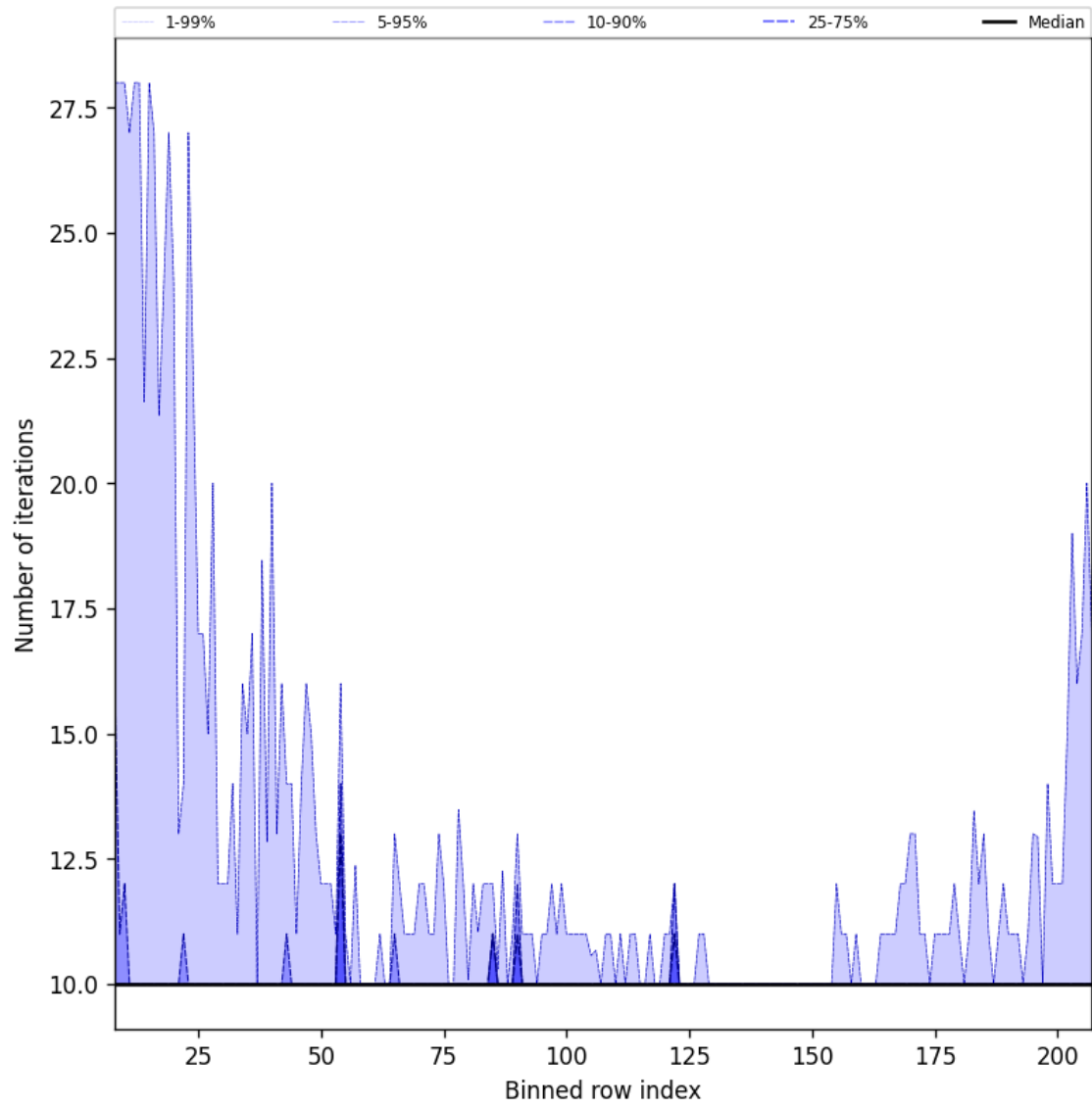
Figure 42: Along track statistics of “Number of iterations” for 2025-01-04 to 2025-01-06
