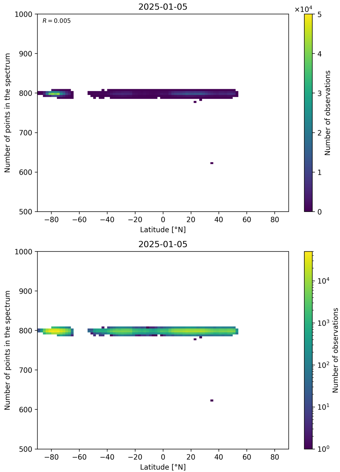
Figure 61: Scatter density plot of “Latitude” against “Number of points in the spectrum” for 2025-01-04 to 2025-01-06.
