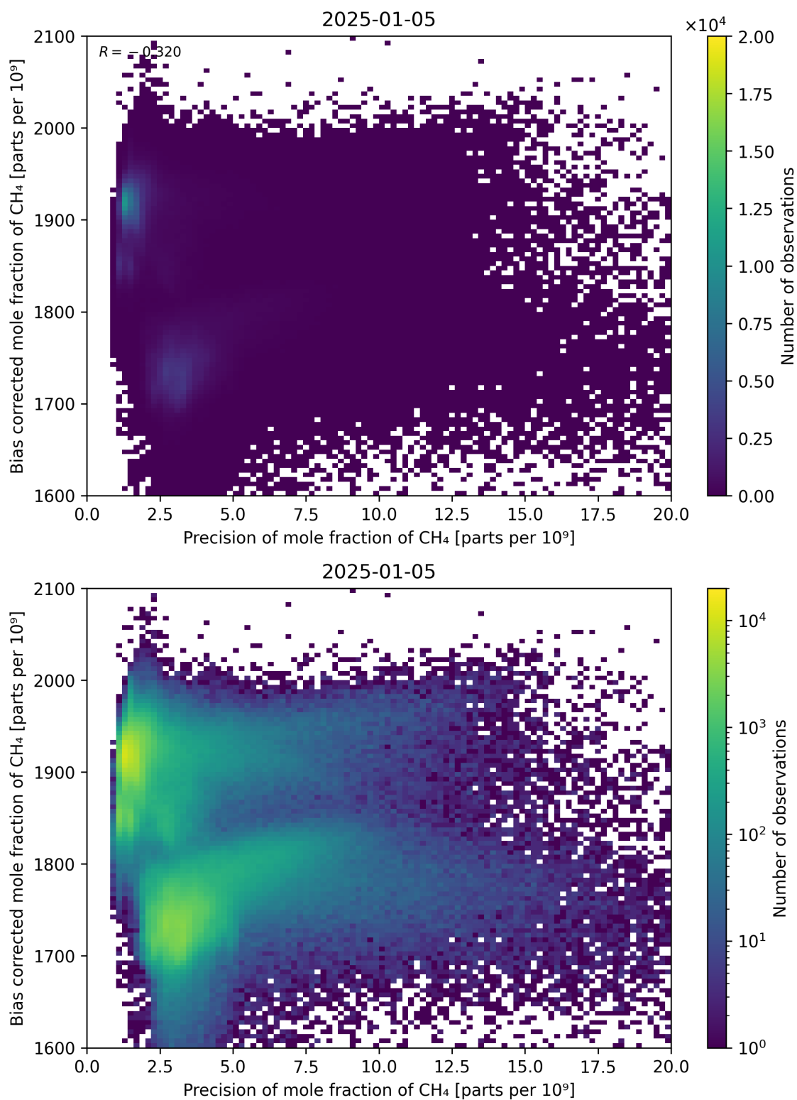
Figure 82: Scatter density plot of “Precision of mole fraction of CH 4 ” against “Bias corrected mole fraction of CH 4 ” for 2025-01-04 to 2025-01-06.
