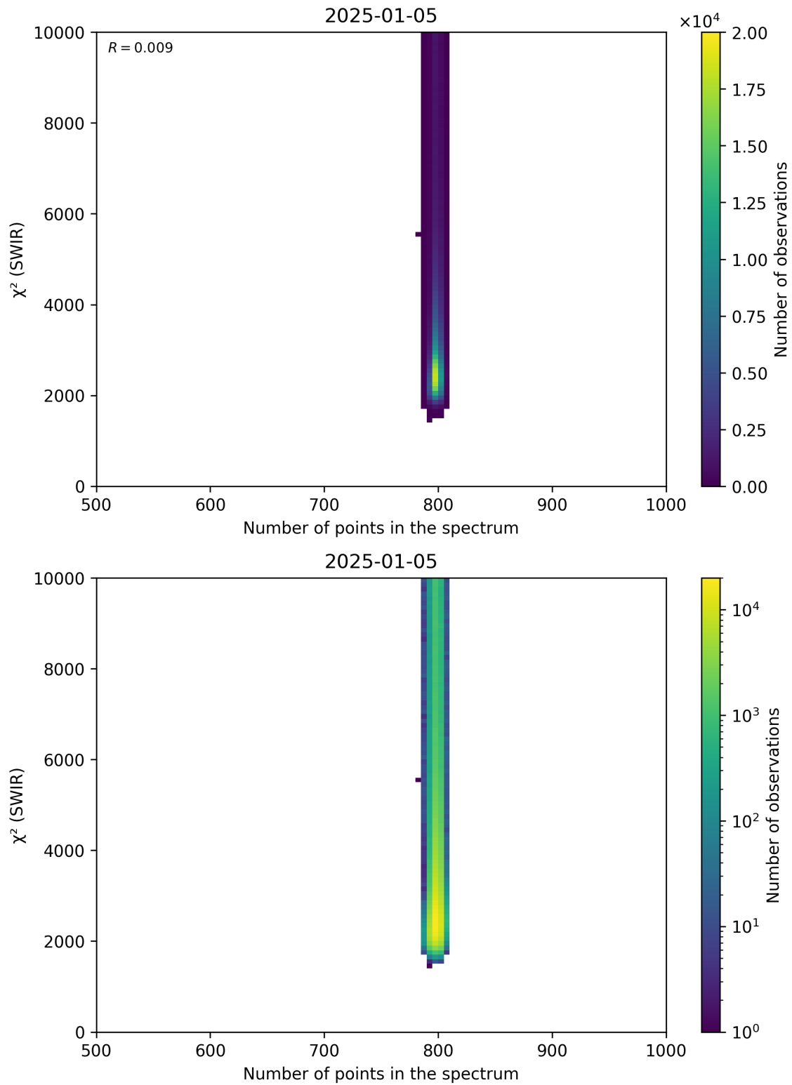
Figure 89: Scatter density plot of “Number of points in the spectrum” against “ \chi^2 (SWIR)” for 2025-01-04 to 2025-01-06.
