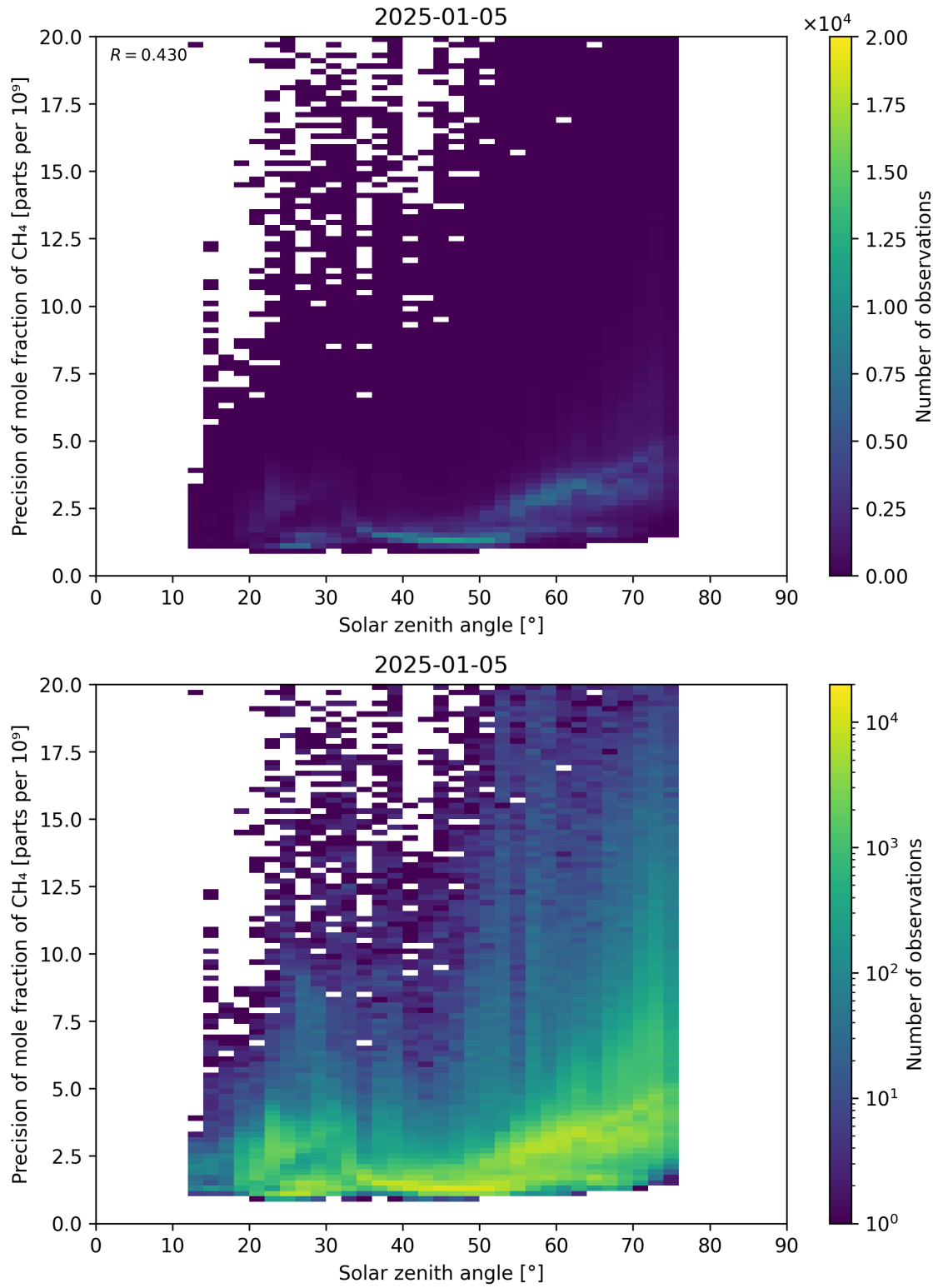
Figure 101: Scatter density plot of “Solar zenith angle” against “Precision of mole fraction of CH 4 ” for 2025-01-04 to 2025-01-06.
