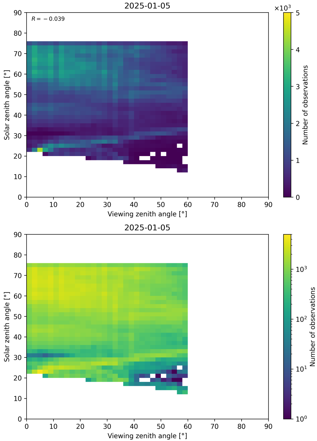
Figure 115: Scatter density plot of “Viewing zenith angle” against “Solar zenith angle” for 2025-01-04 to 2025-01-06.
