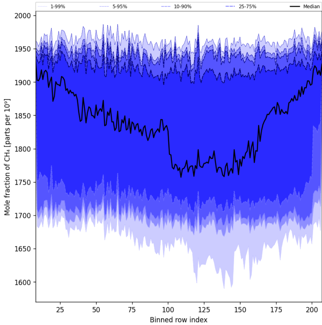
Figure 34: Along track statistics of “Mole fraction of CH 4 ” for 2025-01-04 to 2025-01-06
