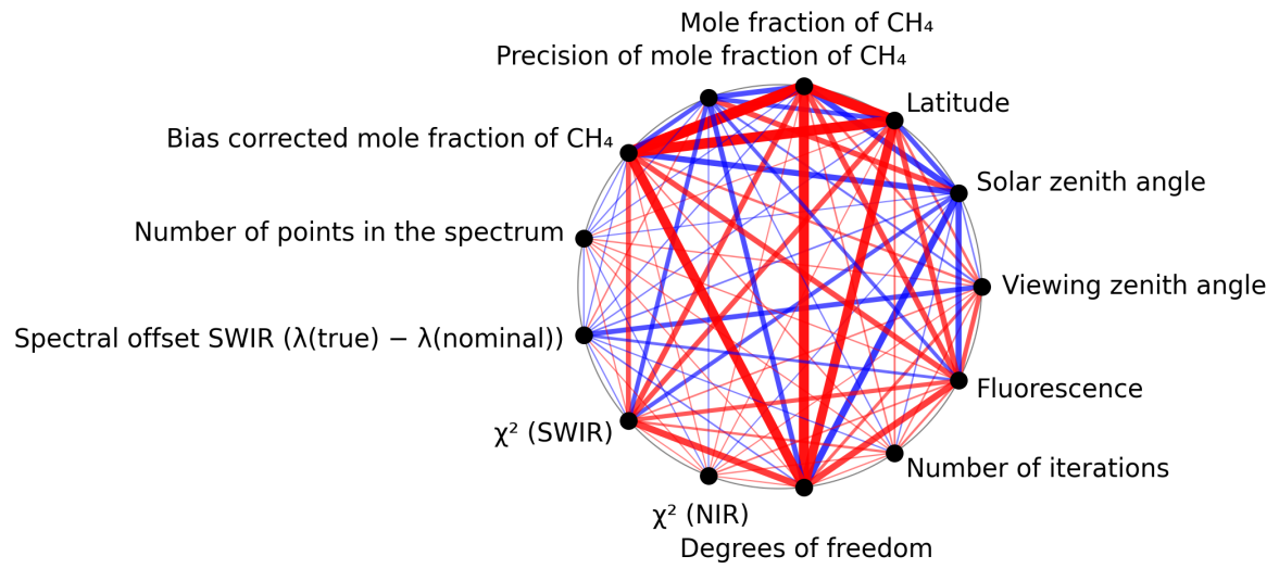
Figure 1: Map of correlation graph for 2025-01-04 to 2025-01-06.
