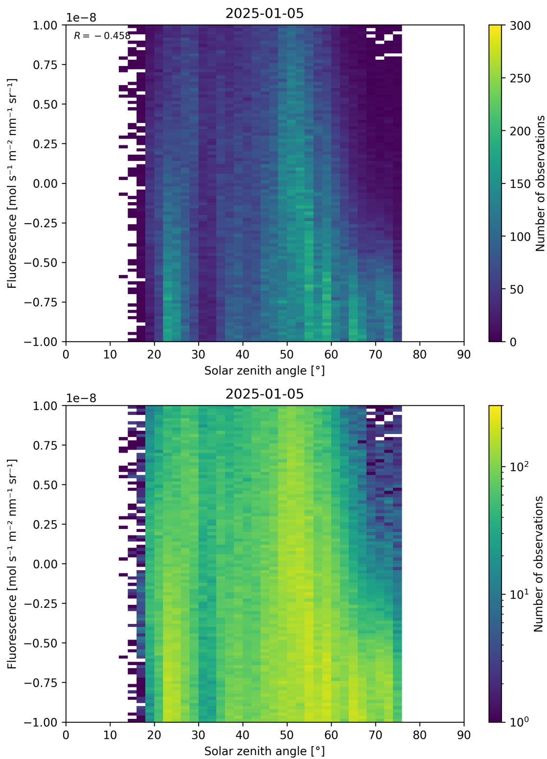
Figure 97: Scatter density plot of “Solar zenith angle” against “Fluorescence” for 2025-01-04 to 2025-01-06.
