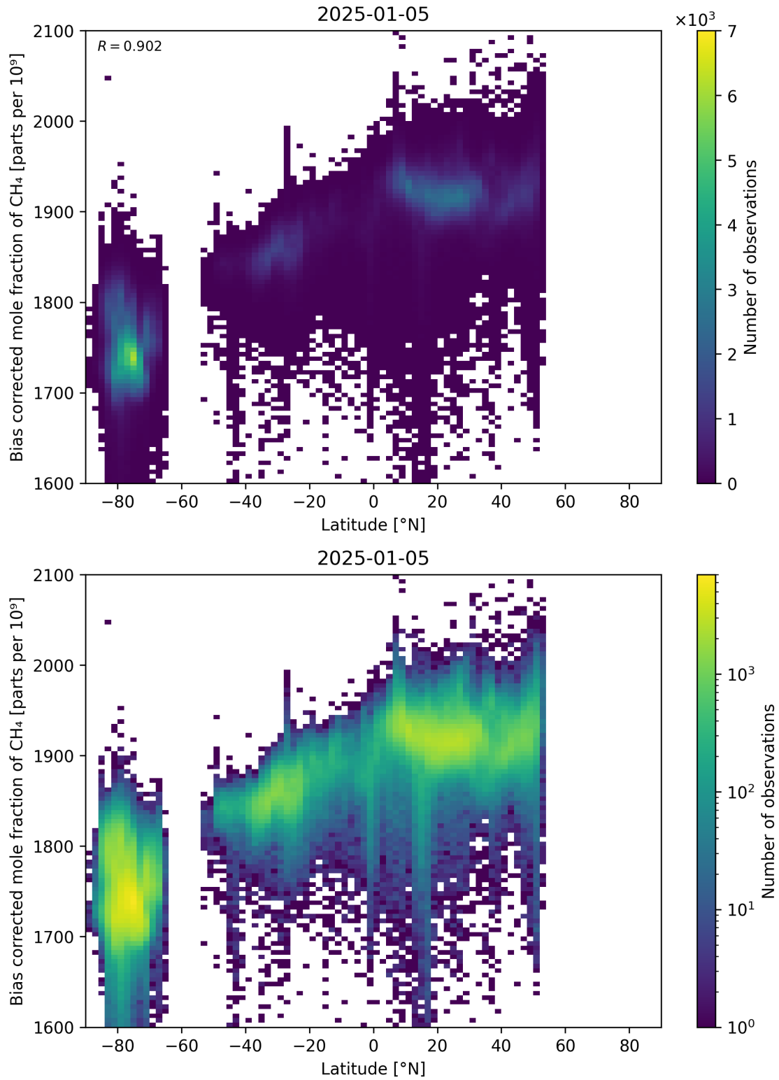
Figure 58: Scatter density plot of “Latitude” against “Bias corrected mole fraction of CH 4 ” for 2025-01-04 to 2025-01-06.
