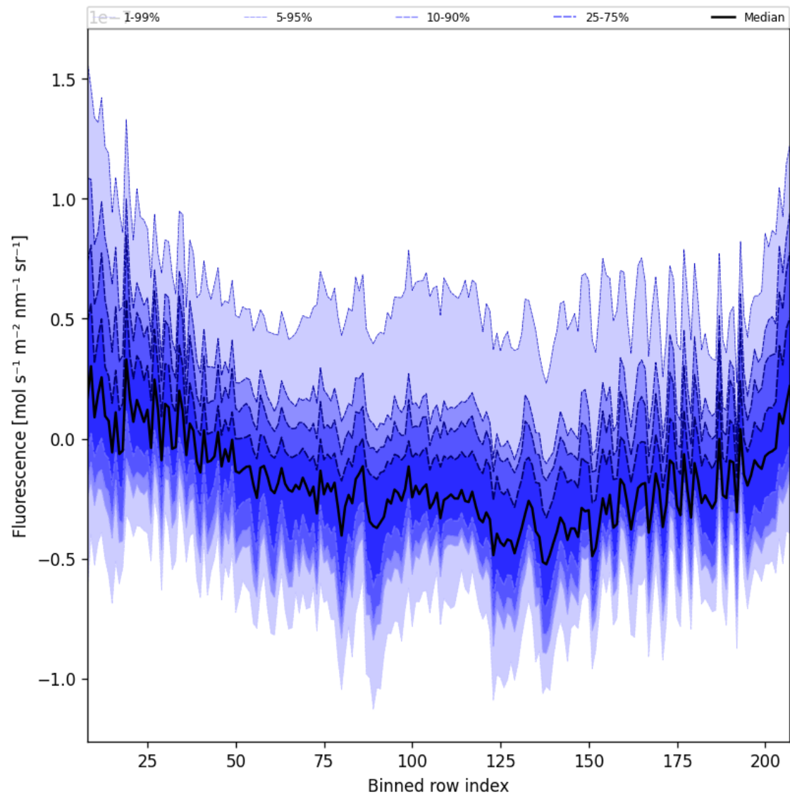
Figure 43: Along track statistics of “Fluorescence” for 2025-01-04 to 2025-01-06
