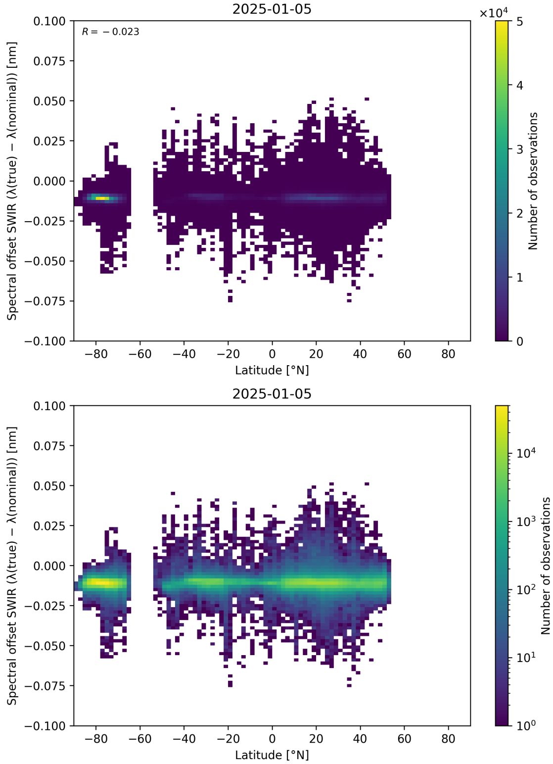
Figure 62: Scatter density plot of “Latitude” against “Spectral offset SWIR ( \lambda_{\text{true}} - \lambda_{\text{nominal}} )” for 2025-01-04 to 2025-01-06.
