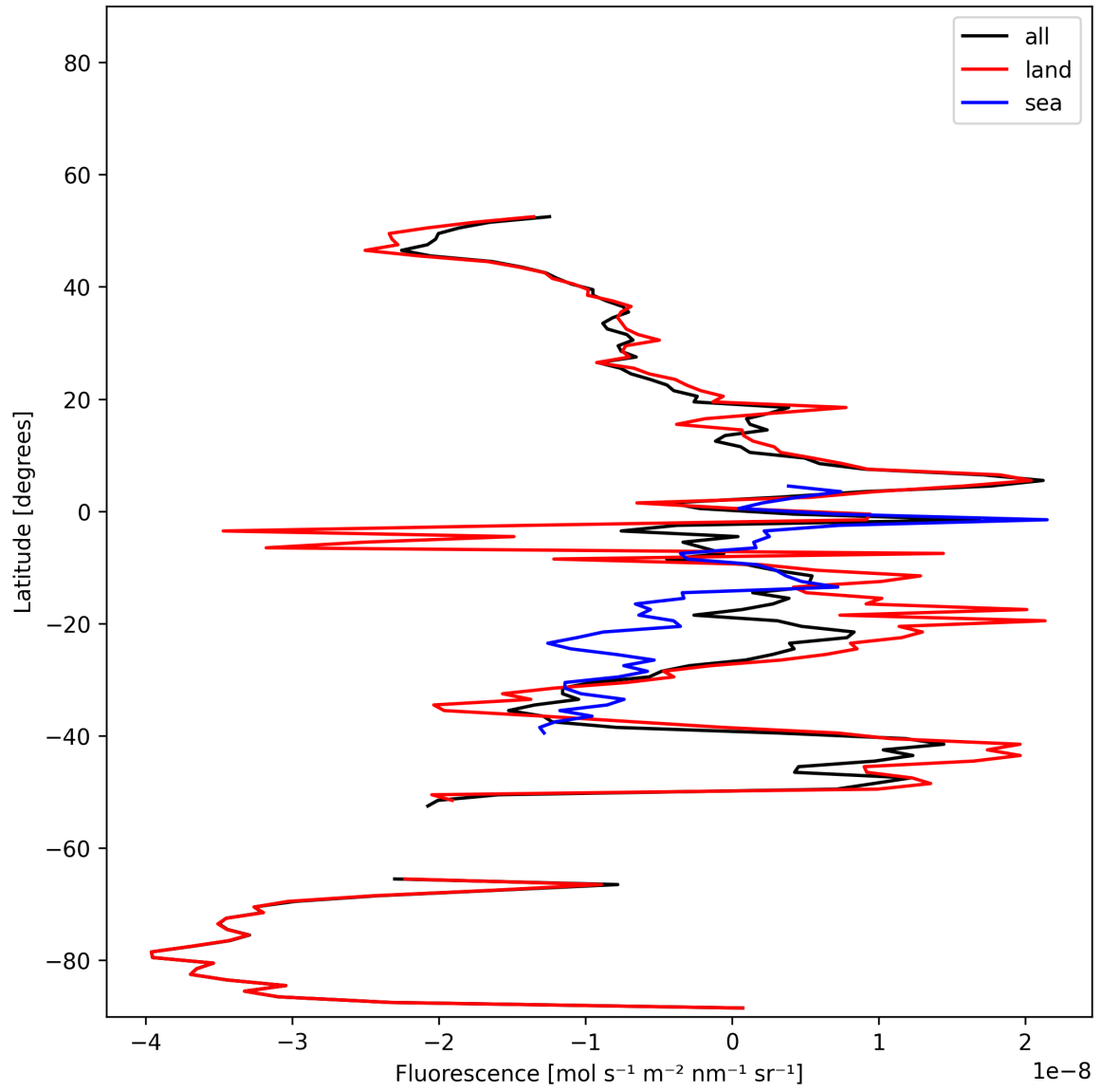
Figure 21: Zonal average of “Fluorescence” for 2025-01-04 to 2025-01-06.
