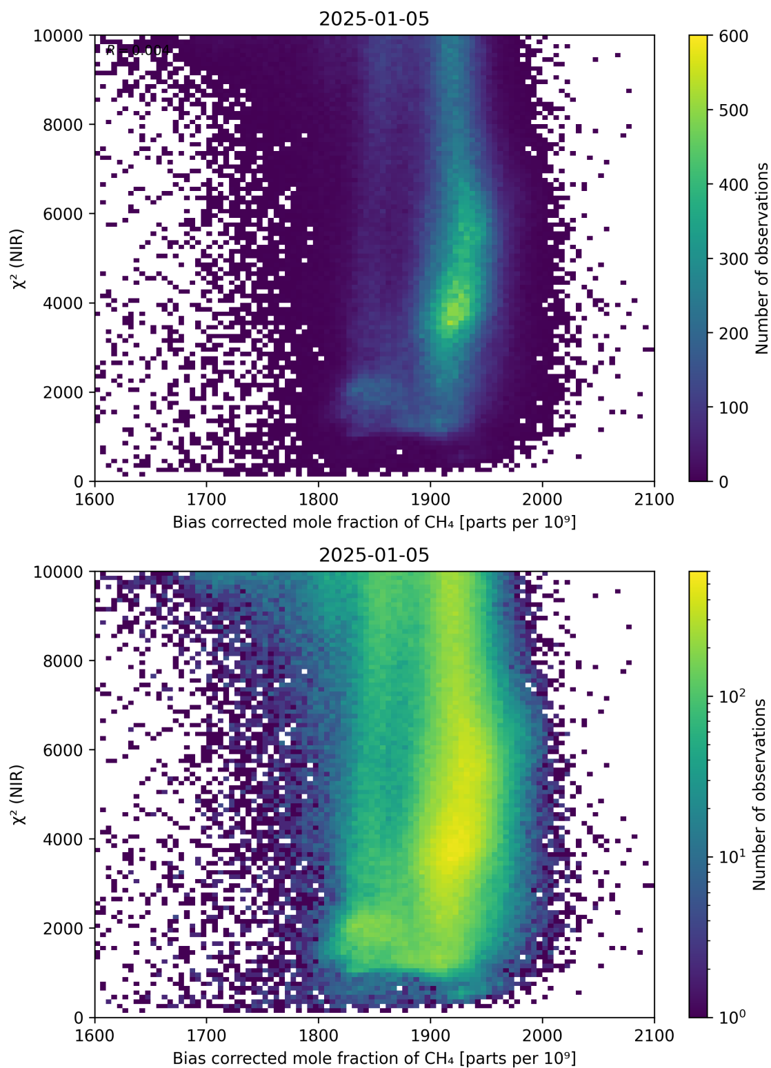
Figure 63: Scatter density plot of “Bias corrected mole fraction of CH 4 ” against “ \chi^2 (NIR)” for 2025-01-04 to 2025-01-06.
