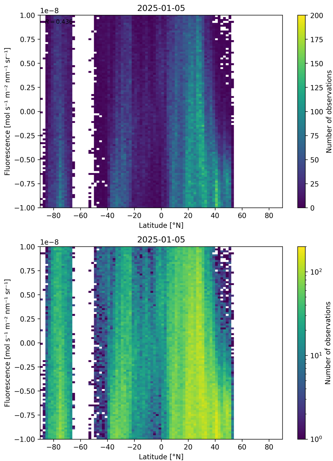
Figure 56: Scatter density plot of “Latitude” against “Fluorescence” for 2025-01-04 to 2025-01-06.
