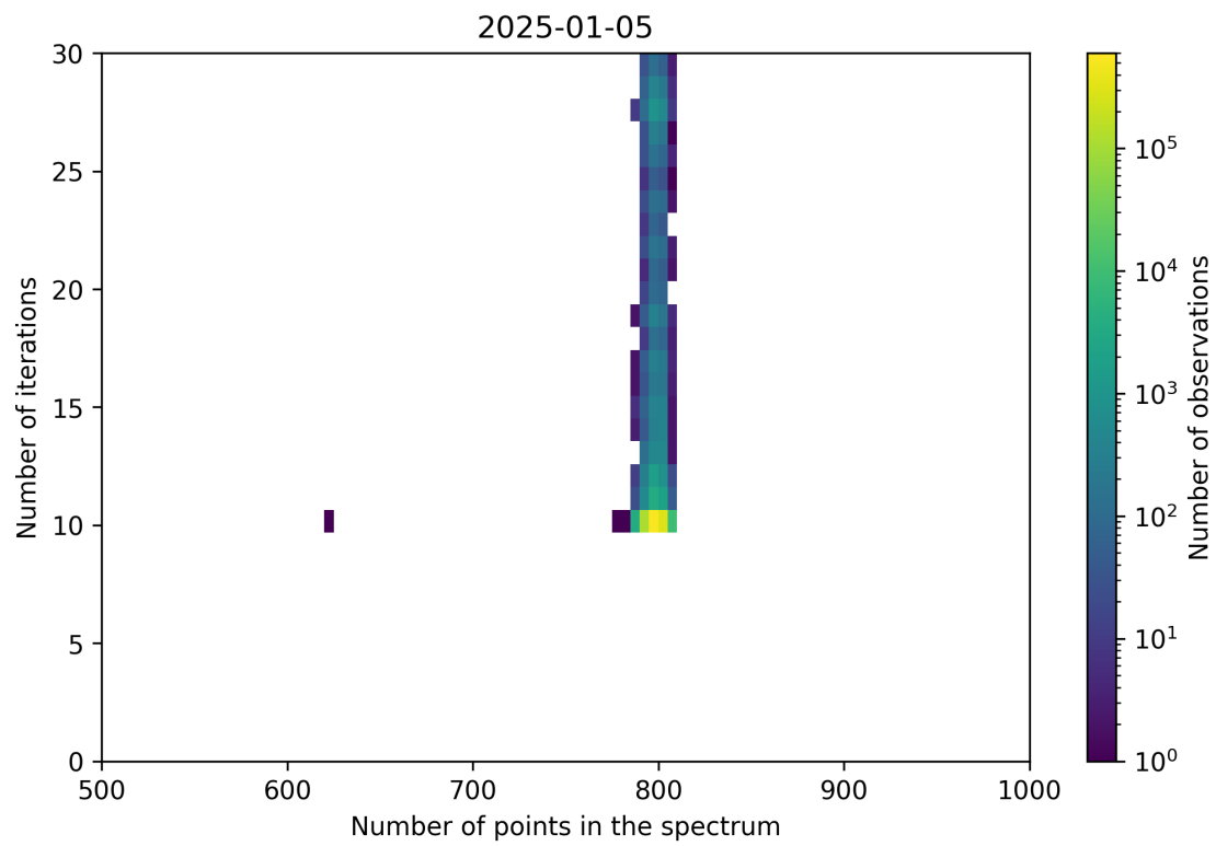
Figure 92: Scatter density plot of “Number of points in the spectrum” against “Number of iterations” for 2025-01-04 to 2025-01-06.
