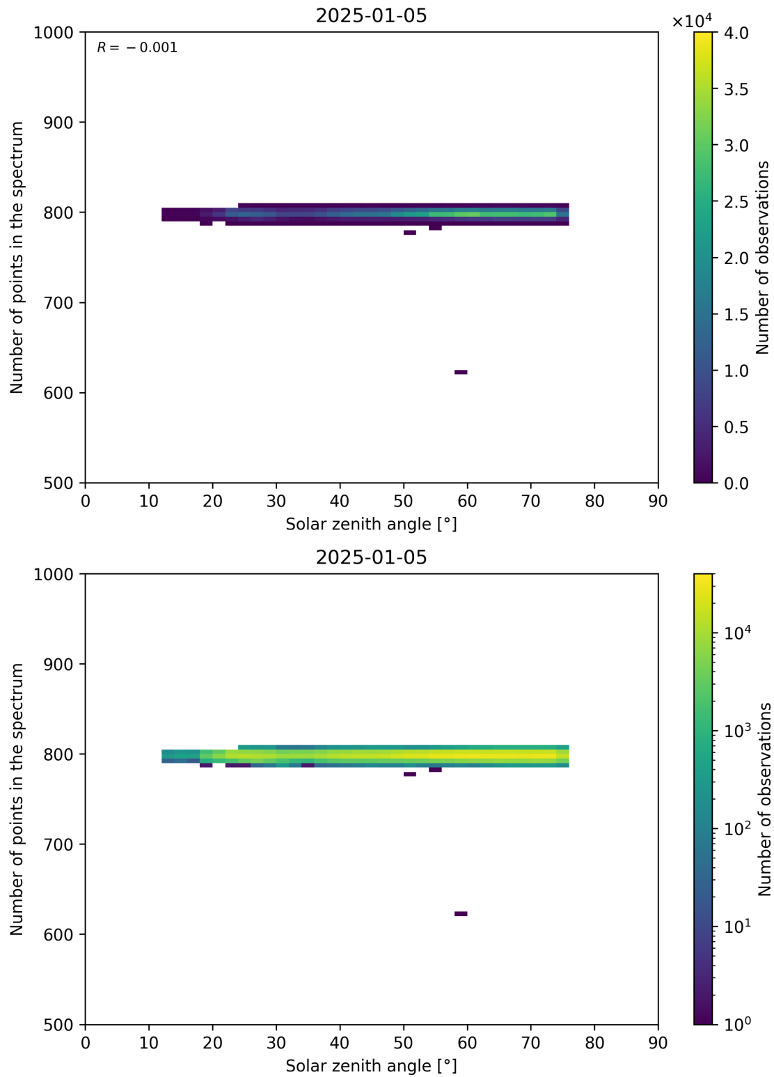
Figure 103: Scatter density plot of “Solar zenith angle” against “Number of points in the spectrum” for 2025-01-04 to 2025-01-06.
