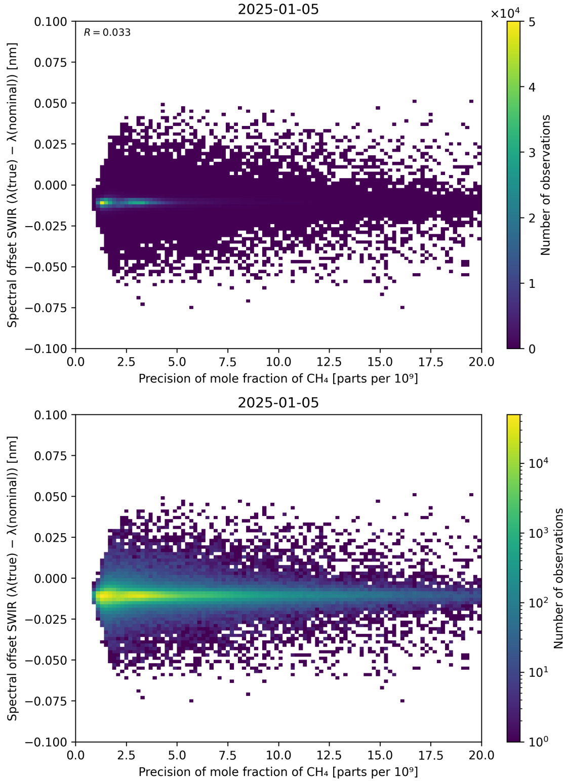
Figure 85: Scatter density plot of “Precision of mole fraction of \text{CH}_4 ” against “Spectral offset SWIR ( \lambda_{\text{true}} - \lambda_{\text{nominal}} )” for 2025-01-04 to 2025-01-06.
