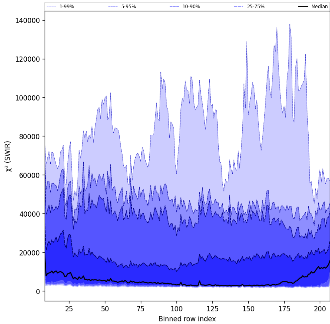
Figure 39: Along track statistics of “ \chi^2 (SWIR)” for 2025-01-04 to 2025-01-06
