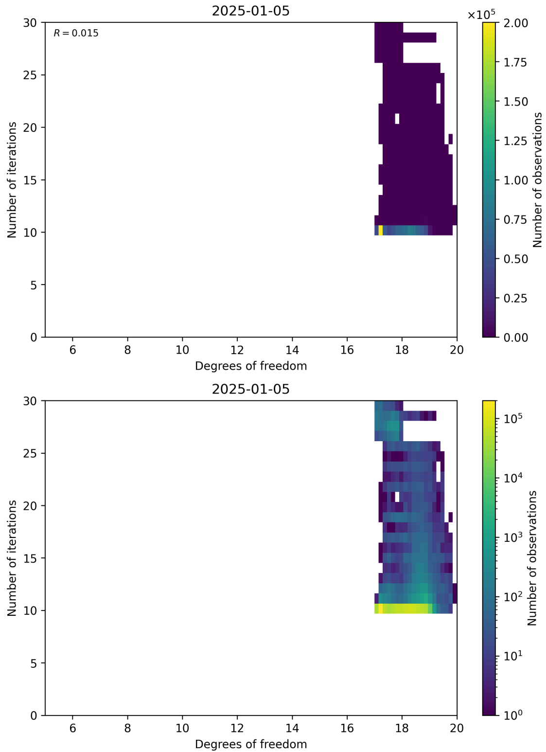
Figure 52: Scatter density plot of “Degrees of freedom” against “Number of iterations” for 2025-01-04 to 2025-01-06.
