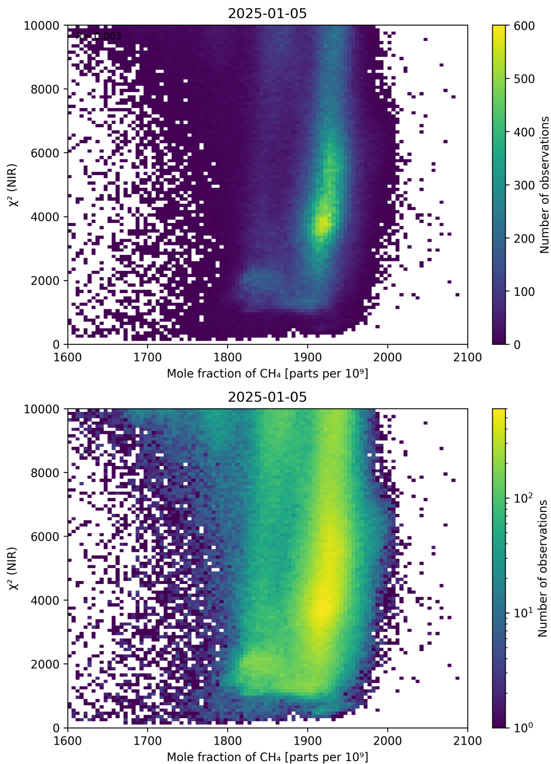
Figure 70: Scatter density plot of “Mole fraction of \text{CH}_4 ” against “ \chi^2 (NIR)” for 2025-01-04 to 2025-01-06.
