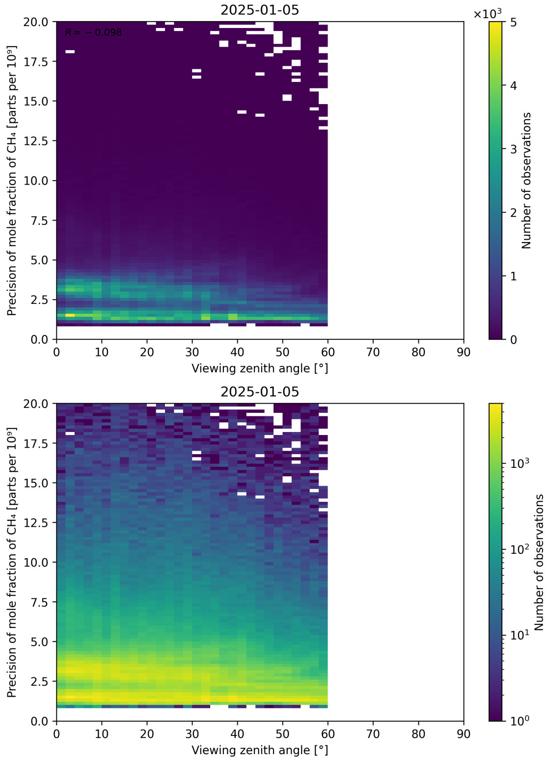
Figure 112: Scatter density plot of “Viewing zenith angle” against “Precision of mole fraction of CH 4 ” for 2025-01-04 to 2025-01-06.
