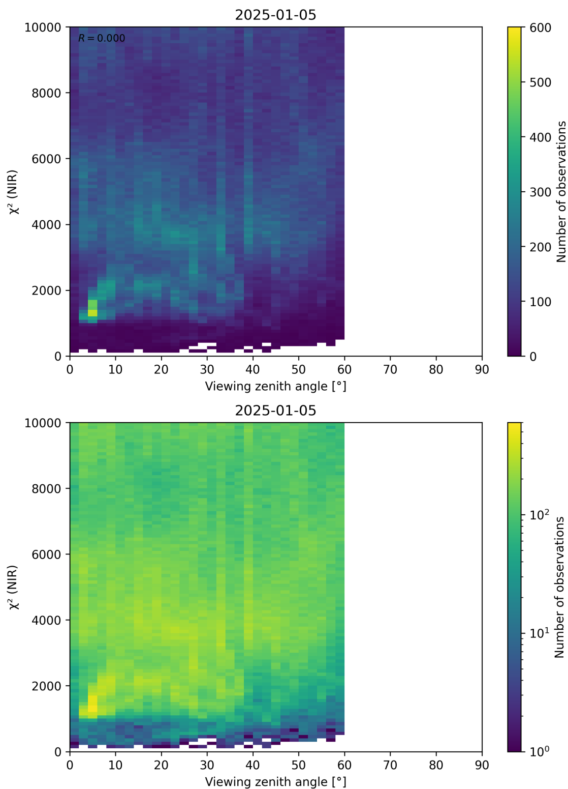
Figure 105: Scatter density plot of “Viewing zenith angle” against “ \chi^2 (NIR)” for 2025-01-04 to 2025-01-06.
