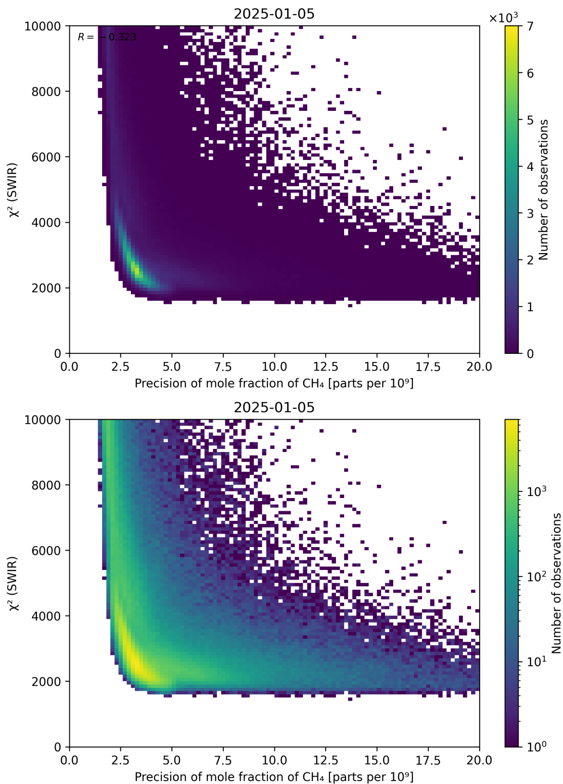
Figure 79: Scatter density plot of “Precision of mole fraction of \text{CH}_4 ” against “ \chi^2 (SWIR)” for 2025-01-04 to 2025-01-06.
