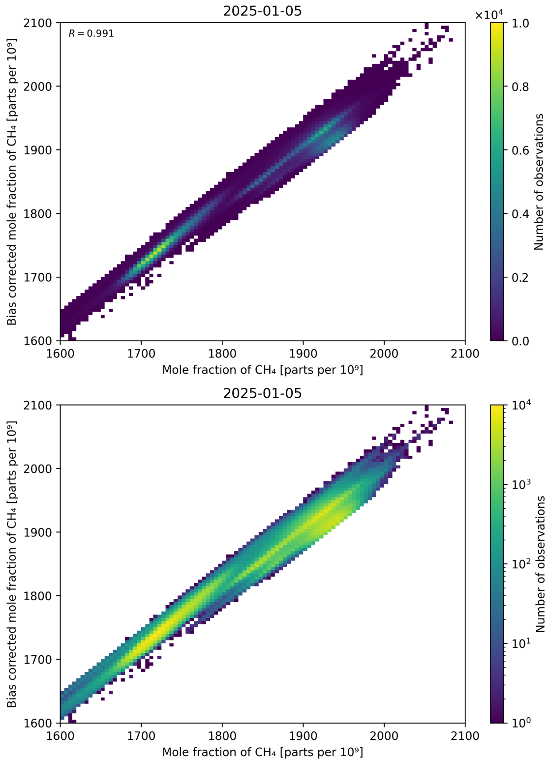
Figure 74: Scatter density plot of “Mole fraction of CH 4 ” against “Bias corrected mole fraction of CH 4 ” for 2025-01-04 to 2025-01-06.
