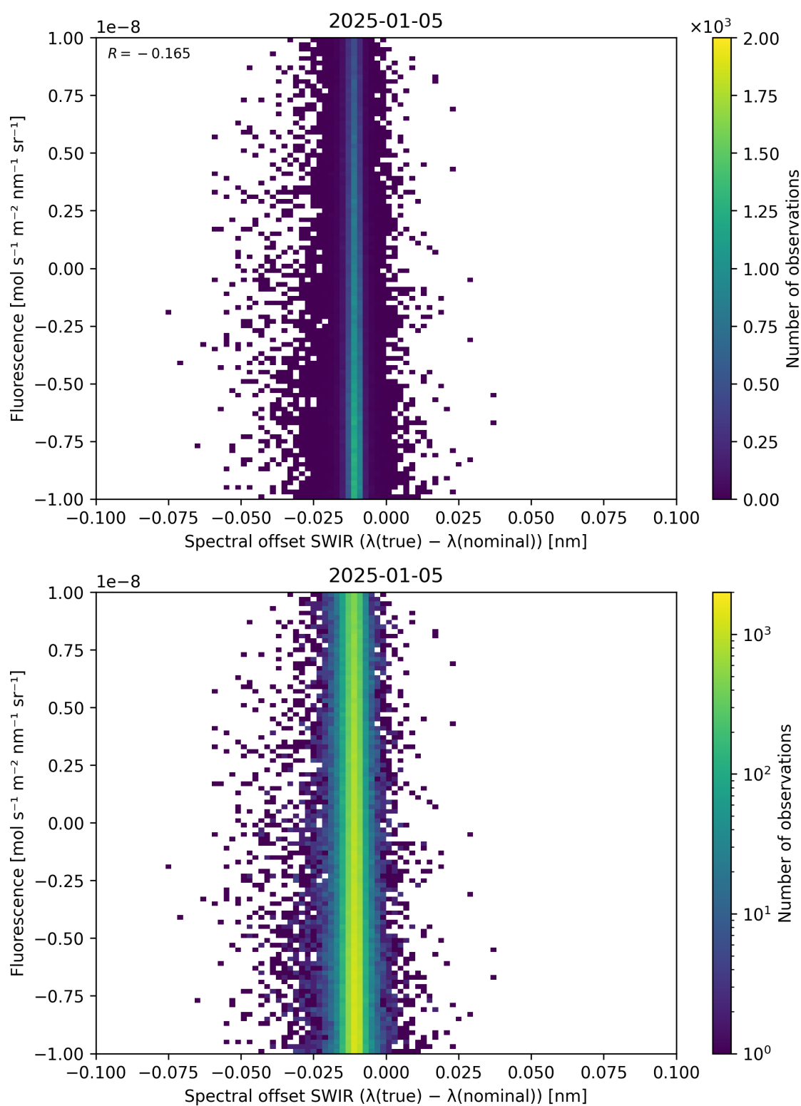
Figure 120: Scatter density plot of “Spectral offset SWIR ( \lambda_{\text{true}} - \lambda_{\text{nominal}} )” against “Fluorescence” for 2025-01-04 to 2025-01-06.
