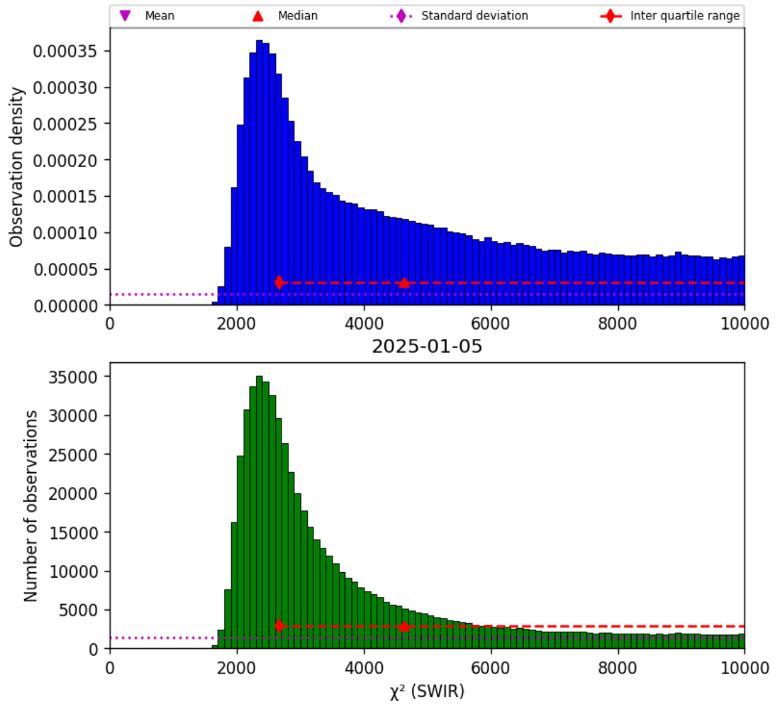
Figure 28: Histogram of " \chi^2 (SWIR)" for 2025-01-04 to 2025-01-06
