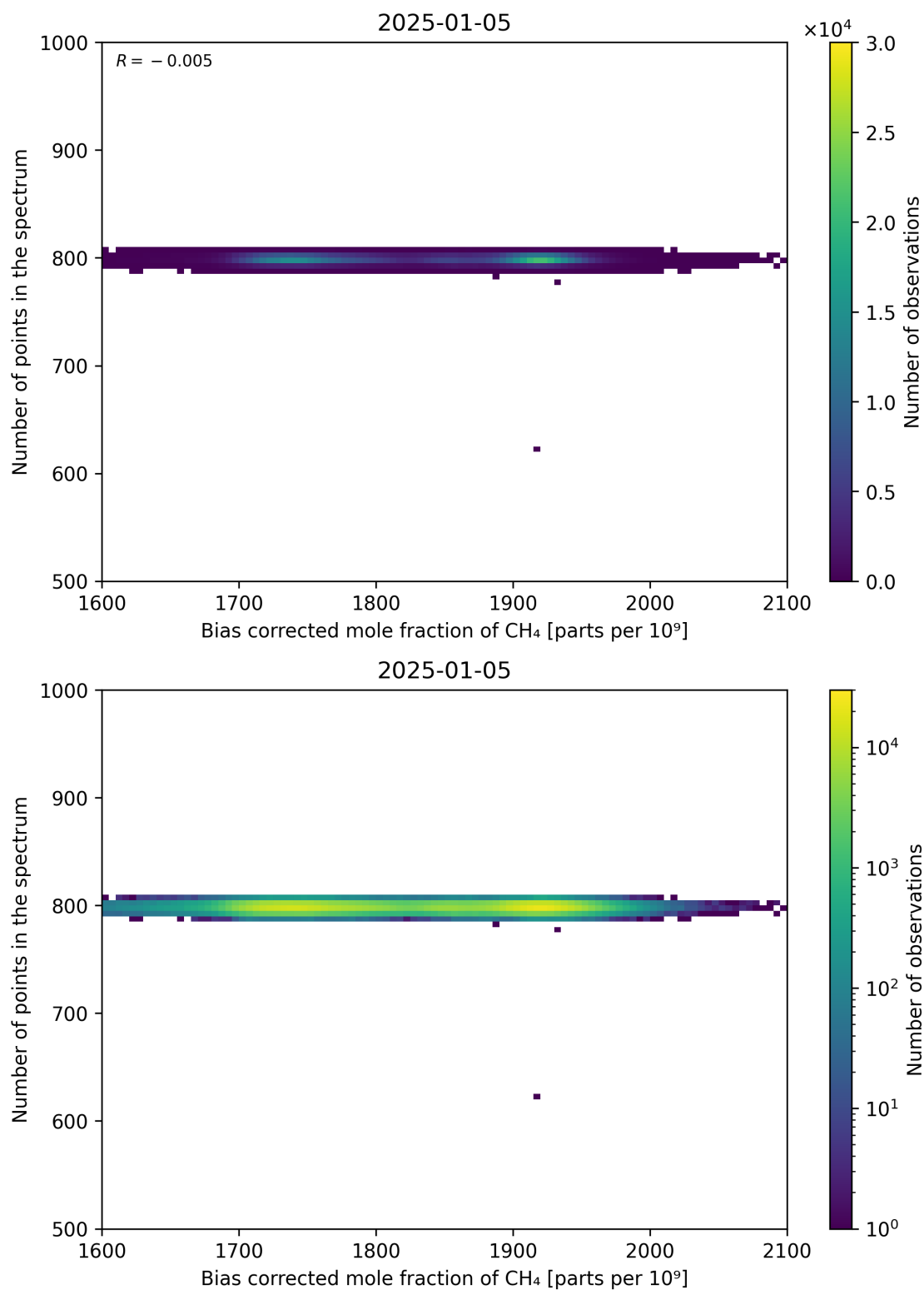
Figure 68: Scatter density plot of “Bias corrected mole fraction of CH 4 ” against “Number of points in the spectrum” for 2025-01-04 to 2025-01-06.
