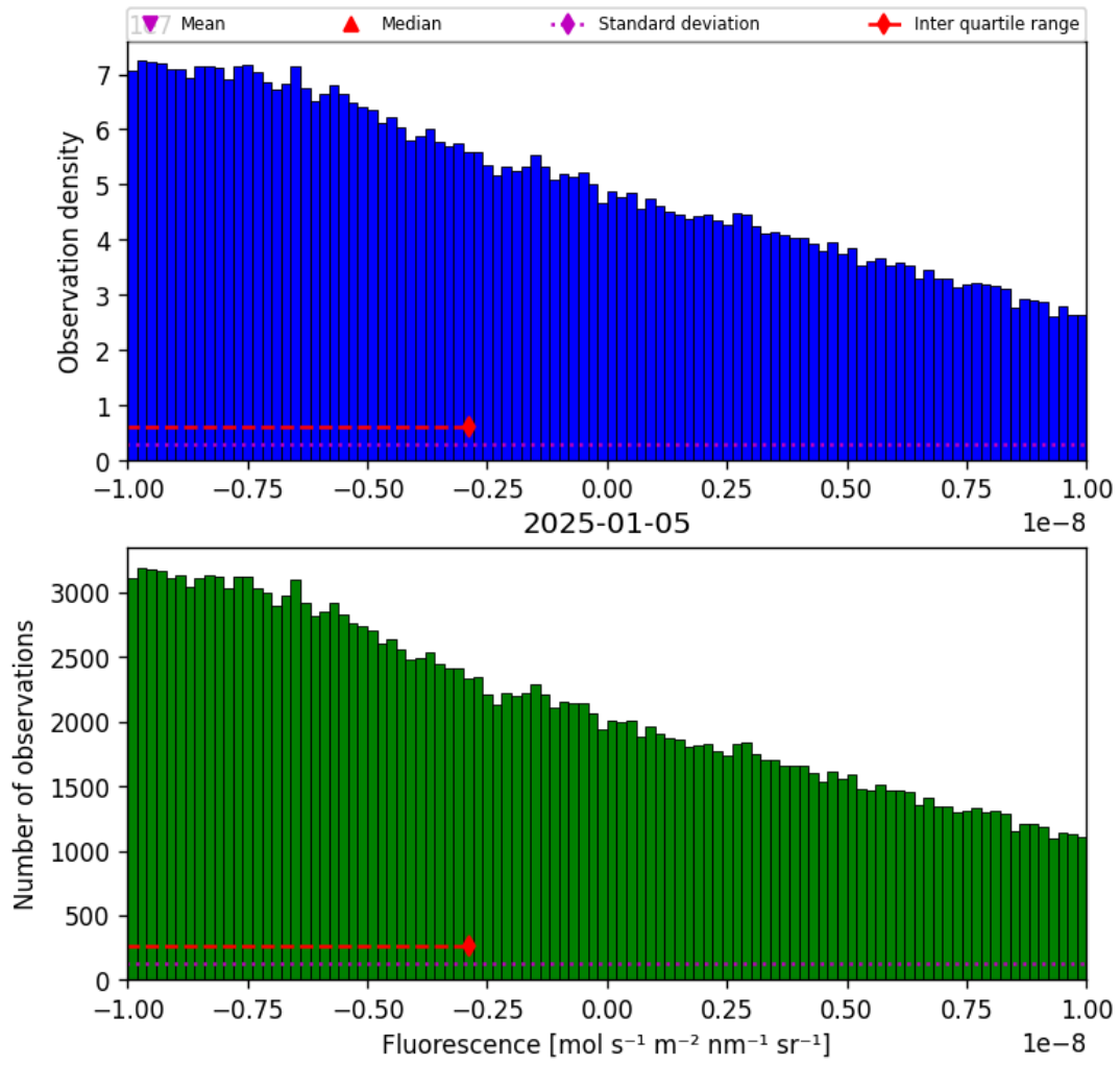
Figure 32: Histogram of “Fluorescence” for 2025-01-04 to 2025-01-06
