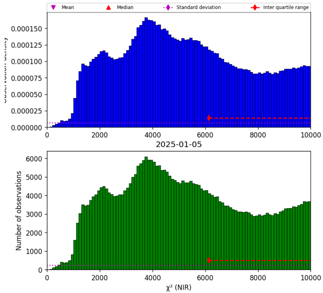
Figure 29: Histogram of “ \chi^2 (NIR)” for 2025-01-04 to 2025-01-06
