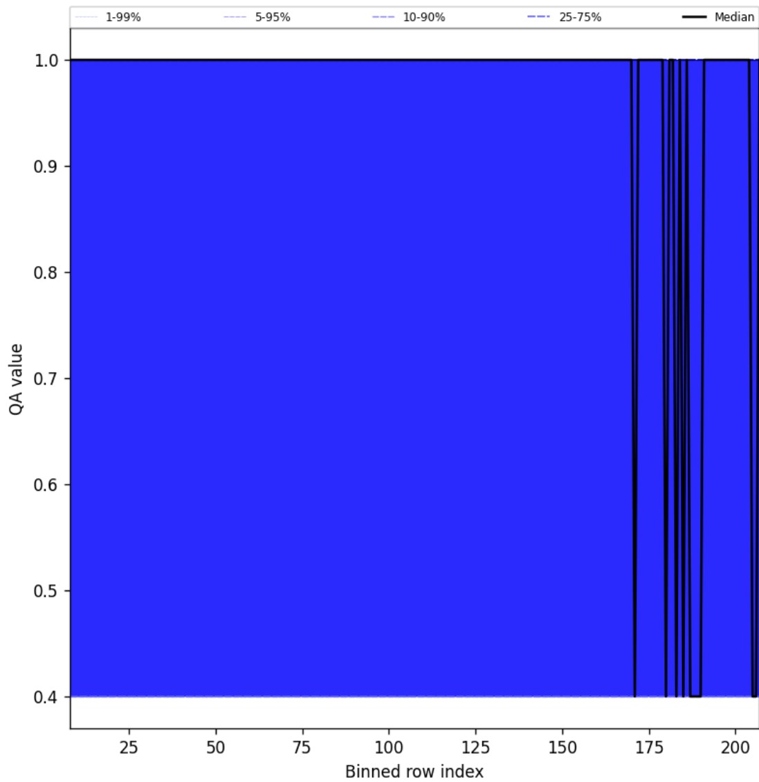
Figure 33: Along track statistics of “QA value” for 2025-01-04 to 2025-01-06
