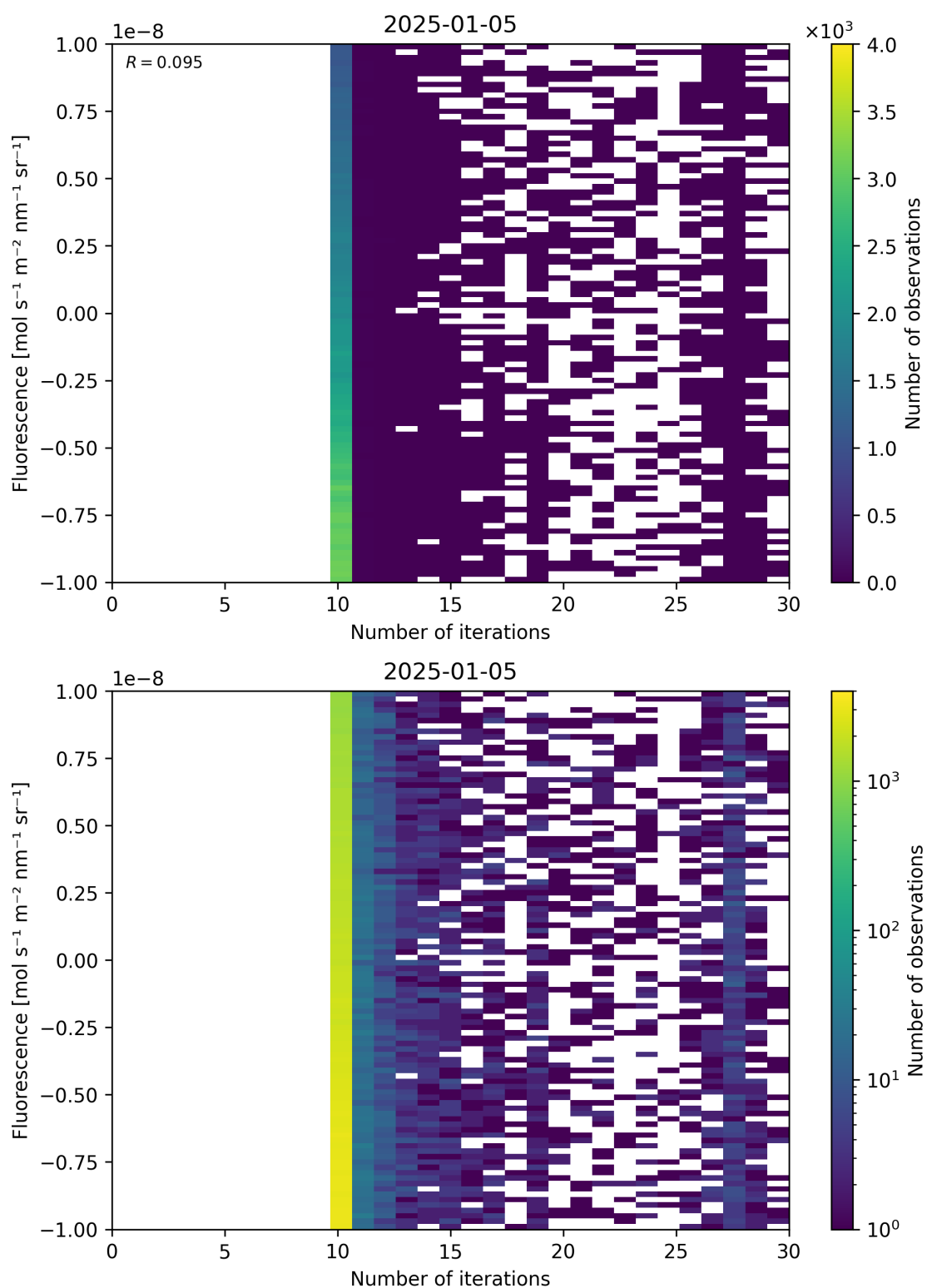
Figure 87: Scatter density plot of “Number of iterations” against “Fluorescence” for 2025-01-04 to 2025-01-06.
