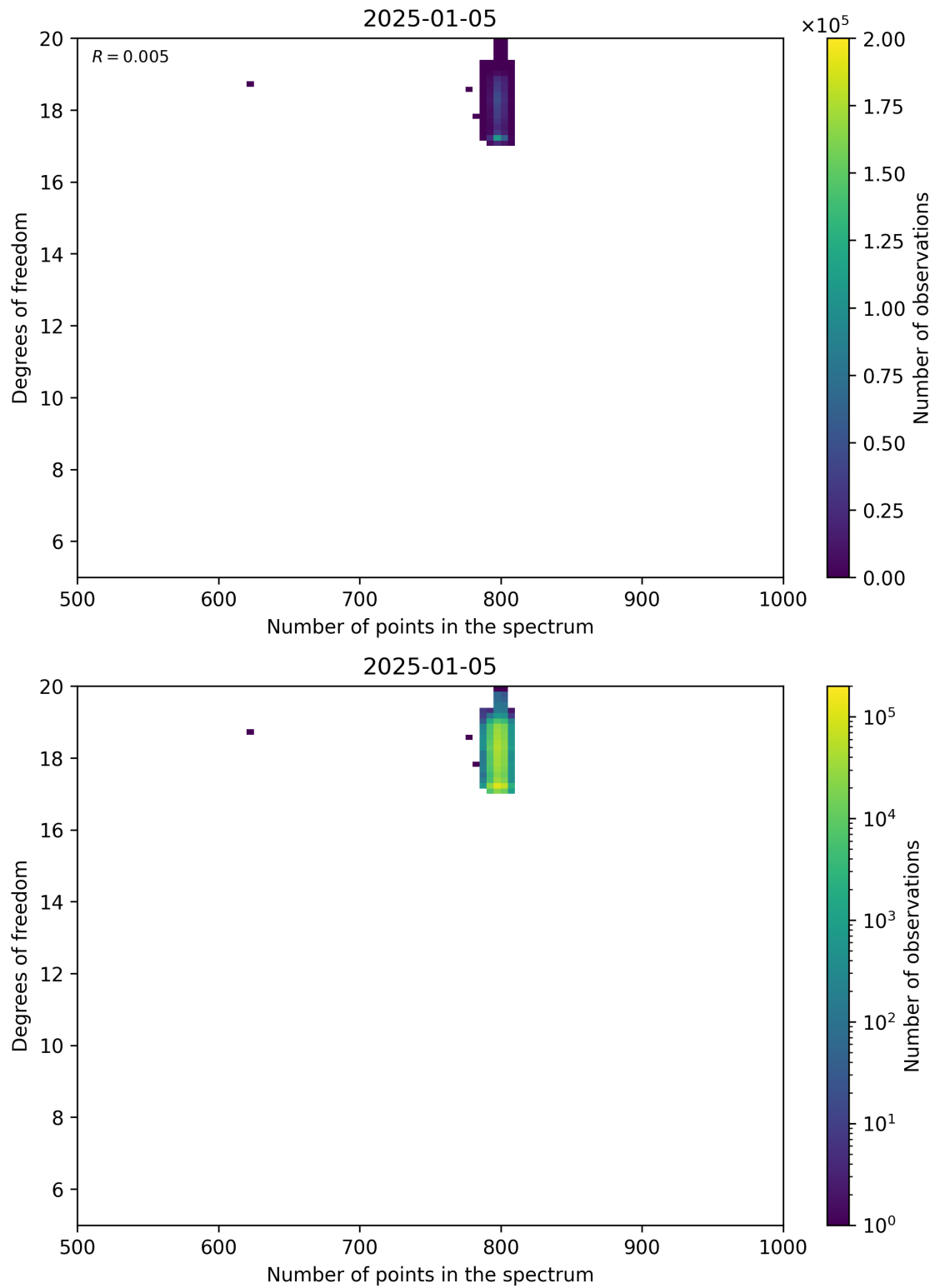
Figure 90: Scatter density plot of “Number of points in the spectrum” against “Degrees of freedom” for 2025-01-04 to 2025-01-06.
