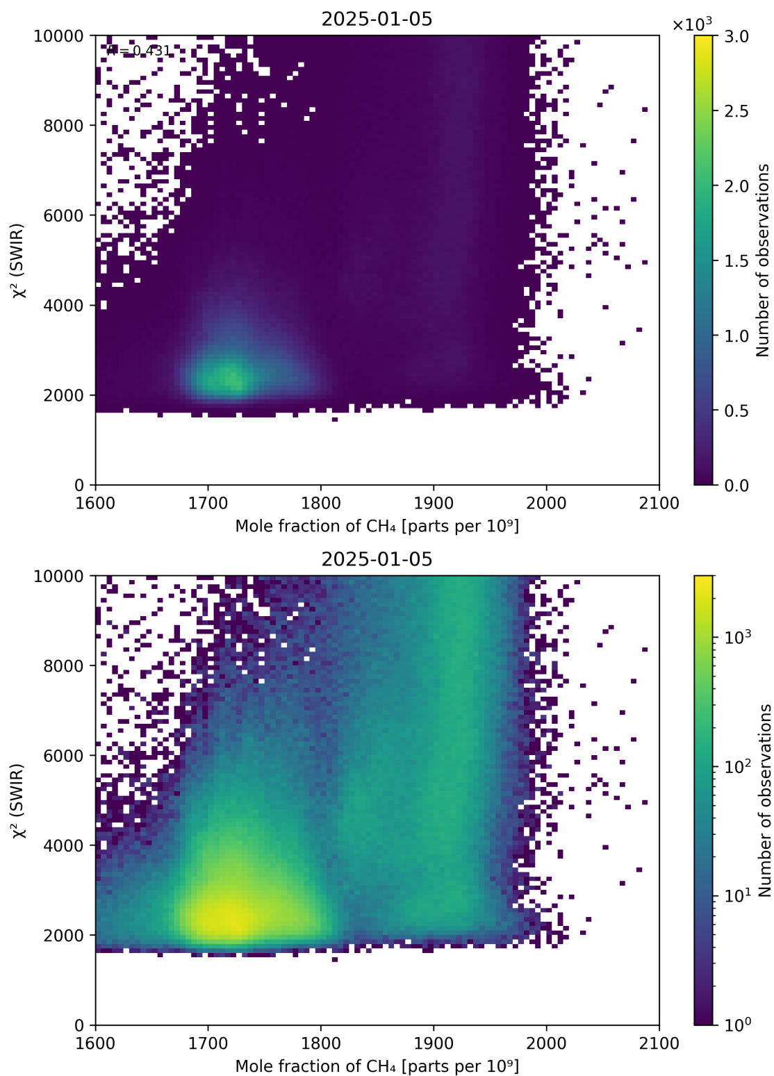
Figure 71: Scatter density plot of “Mole fraction of CH 4 ” against “ \chi^2 (SWIR)” for 2025-01-04 to 2025-01-06.
