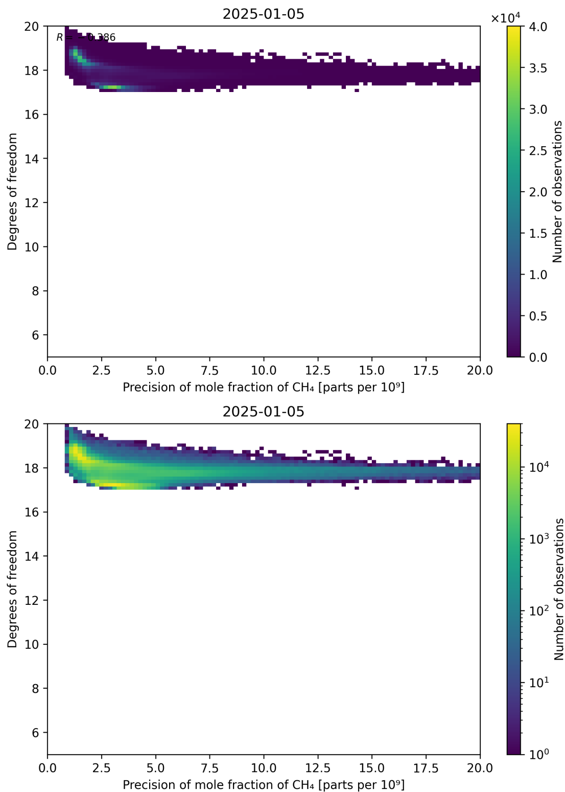
Figure 80: Scatter density plot of “Precision of mole fraction of CH 4 ” against “Degrees of freedom” for 2025-01-04 to 2025-01-06.
