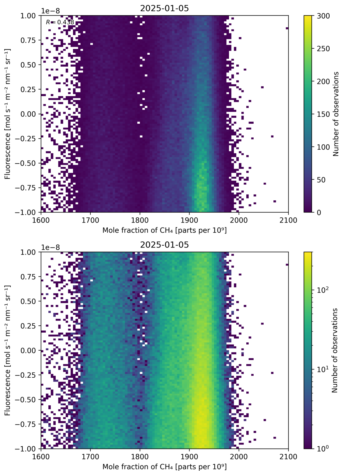
Figure 73: Scatter density plot of “Mole fraction of CH 4 ” against “Fluorescence” for 2025-01-04 to 2025-01-06.
