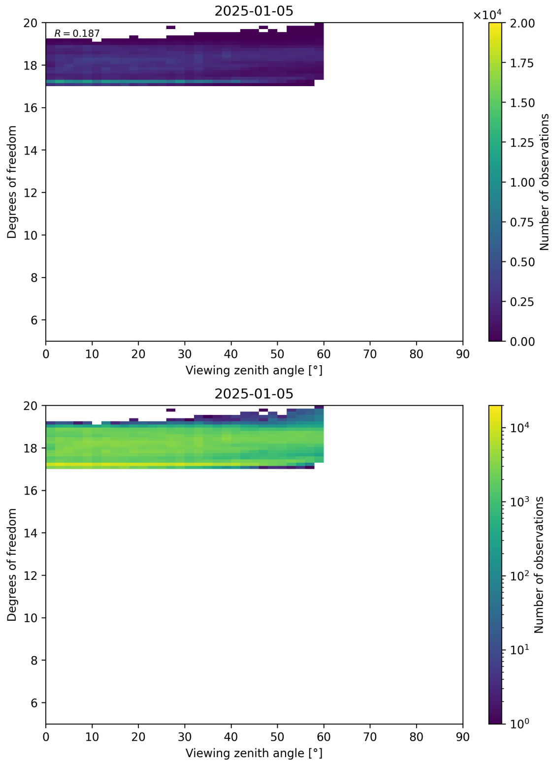
Figure 107: Scatter density plot of “Viewing zenith angle” against “Degrees of freedom” for 2025-01-04 to 2025-01-06.
