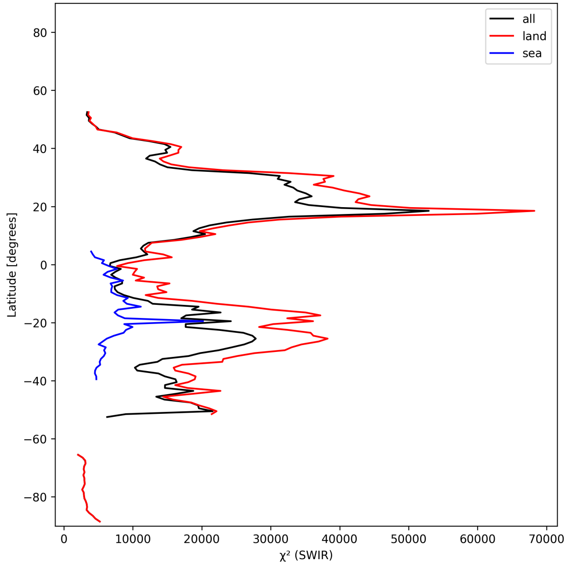
Figure 17: Zonal average of “ \chi^2 (SWIR)” for 2025-01-04 to 2025-01-06.
