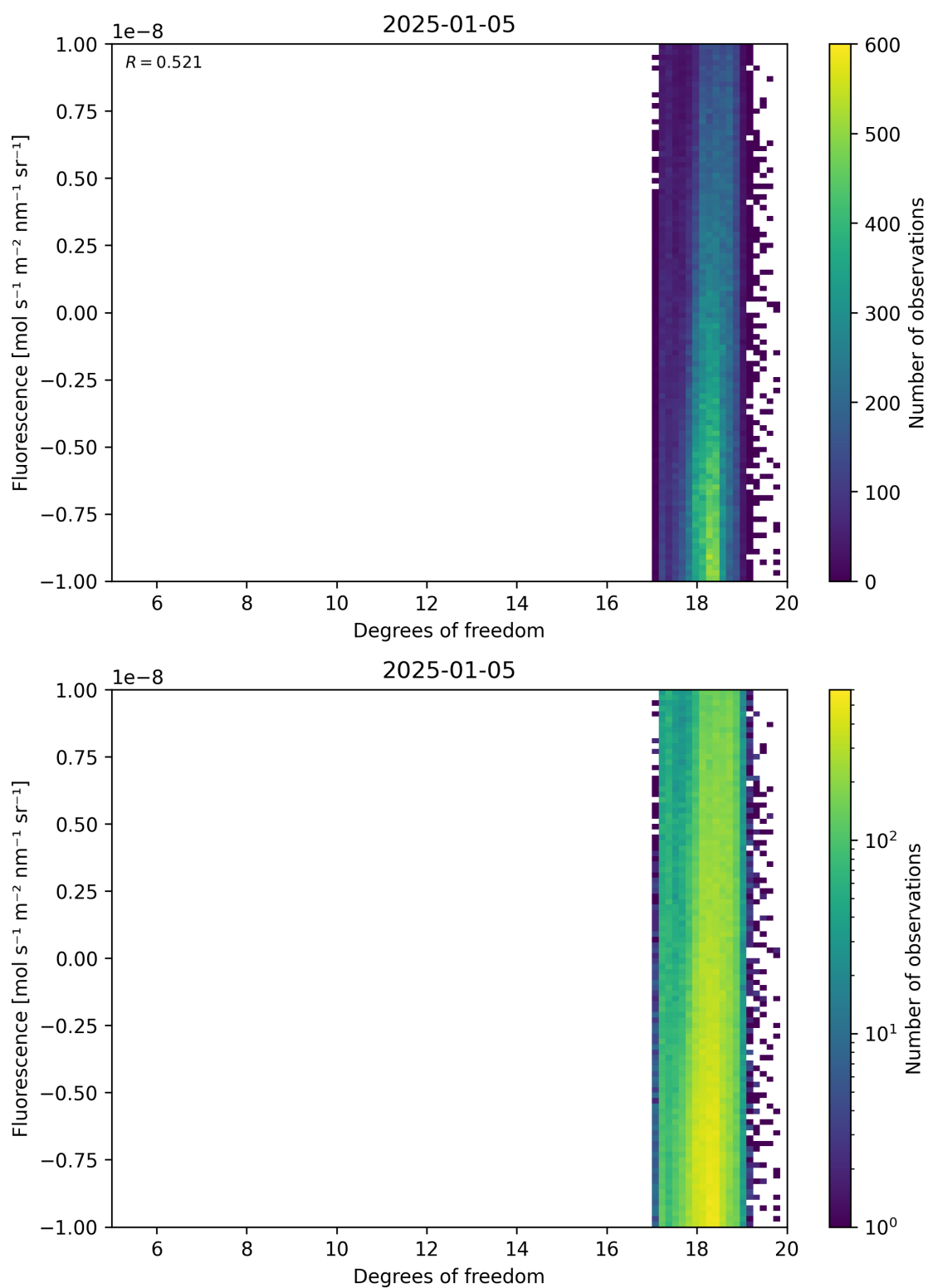
Figure 51: Scatter density plot of “Degrees of freedom” against “Fluorescence” for 2025-01-04 to 2025-01-06.
