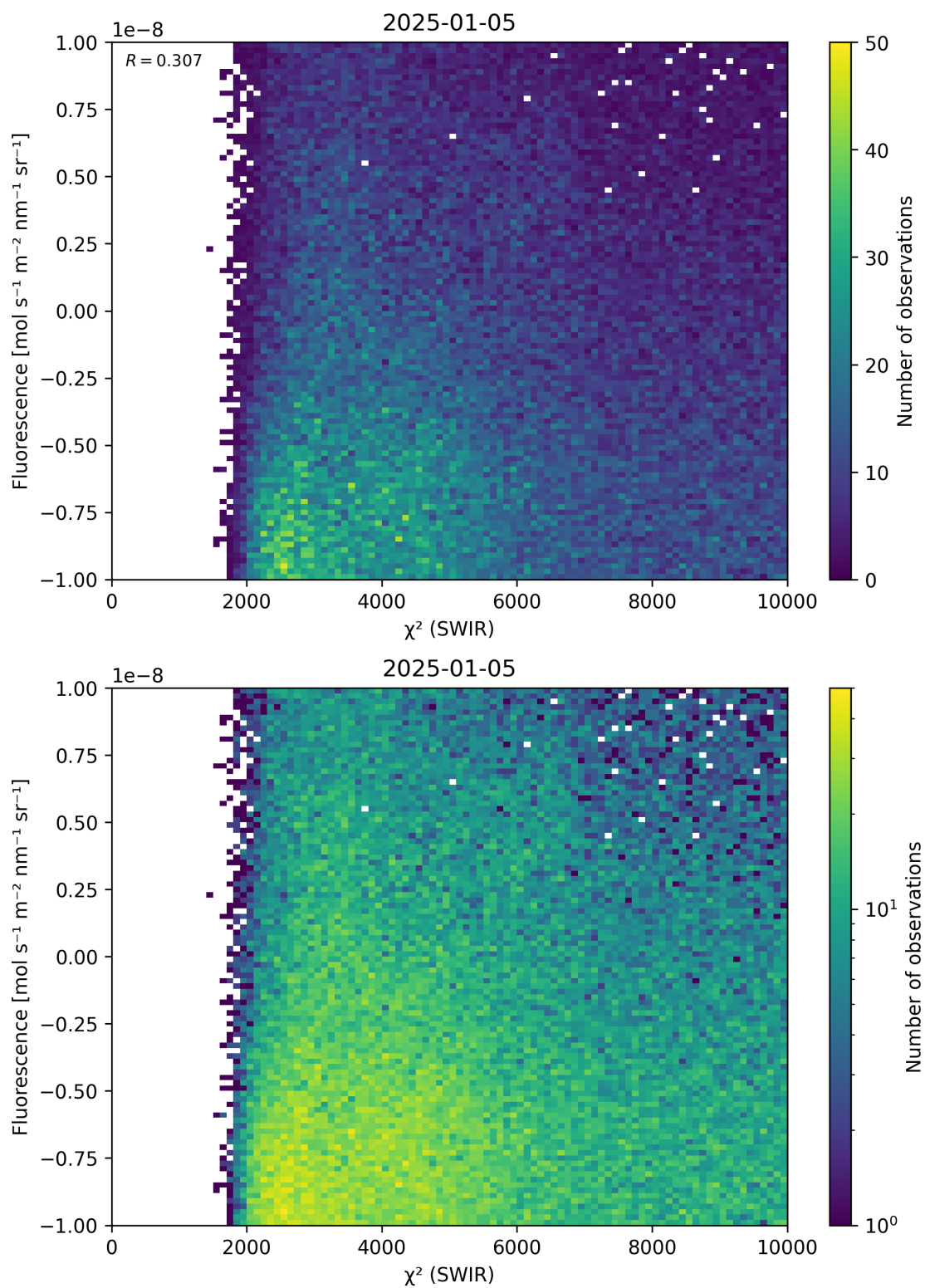
Figure 49: Scatter density plot of “ \chi^2 (SWIR)” against “Fluorescence” for 2025-01-04 to 2025-01-06.
