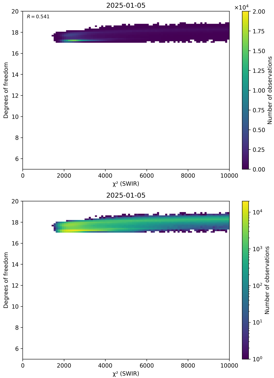
Figure 48: Scatter density plot of “ \chi^2 (SWIR)” against “Degrees of freedom” for 2025-01-04 to 2025-01-06.
