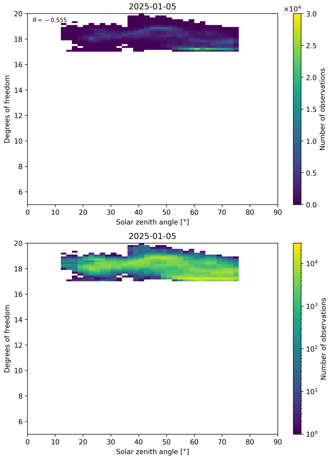
Figure 96: Scatter density plot of “Solar zenith angle” against “Degrees of freedom” for 2025-01-04 to 2025-01-06.
