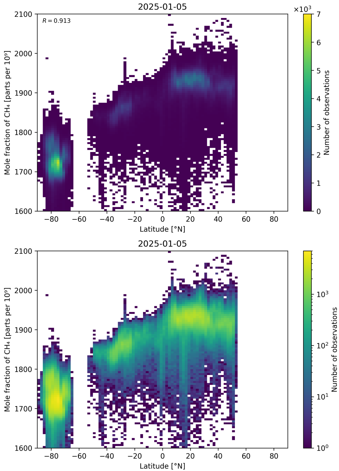
Figure 57: Scatter density plot of “Latitude” against “Mole fraction of CH 4 ” for 2025-01-04 to 2025-01-06.
