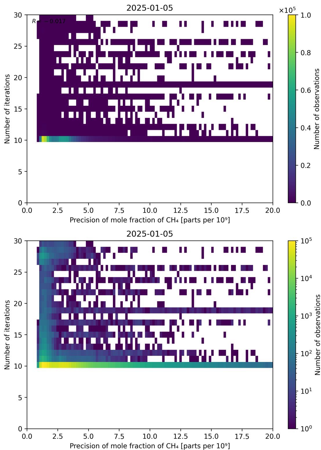
Figure 83: Scatter density plot of “Precision of mole fraction of CH 4 ” against “Number of iterations” for 2025-01-04 to 2025-01-06.
