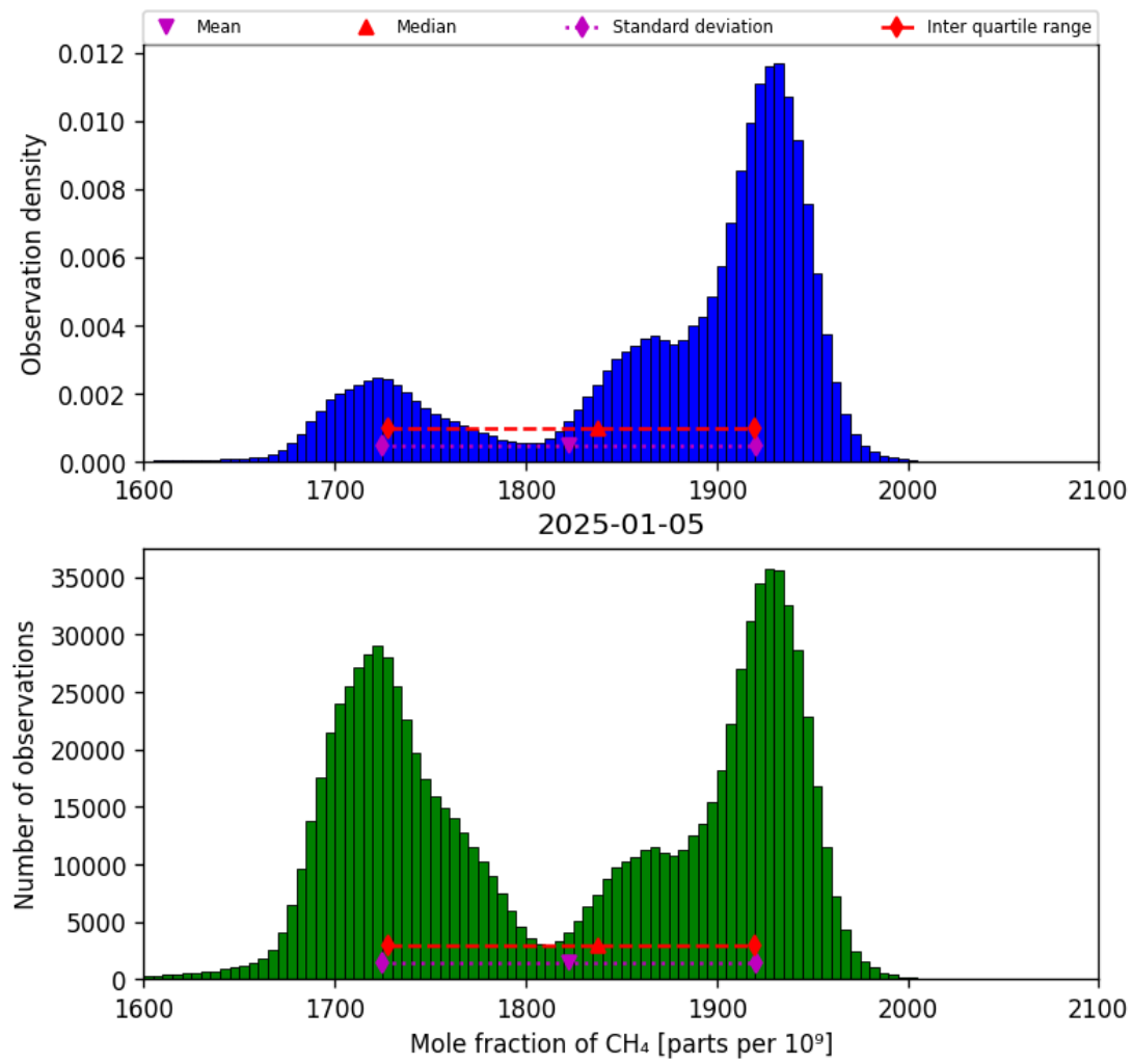
Figure 23: Histogram of “Mole fraction of CH 4 ” for 2025-01-04 to 2025-01-06
