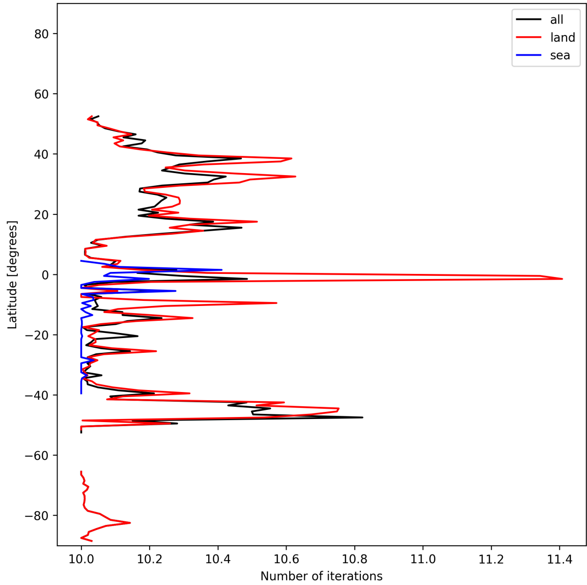
Figure 20: Zonal average of “Number of iterations” for 2025-01-04 to 2025-01-06.
