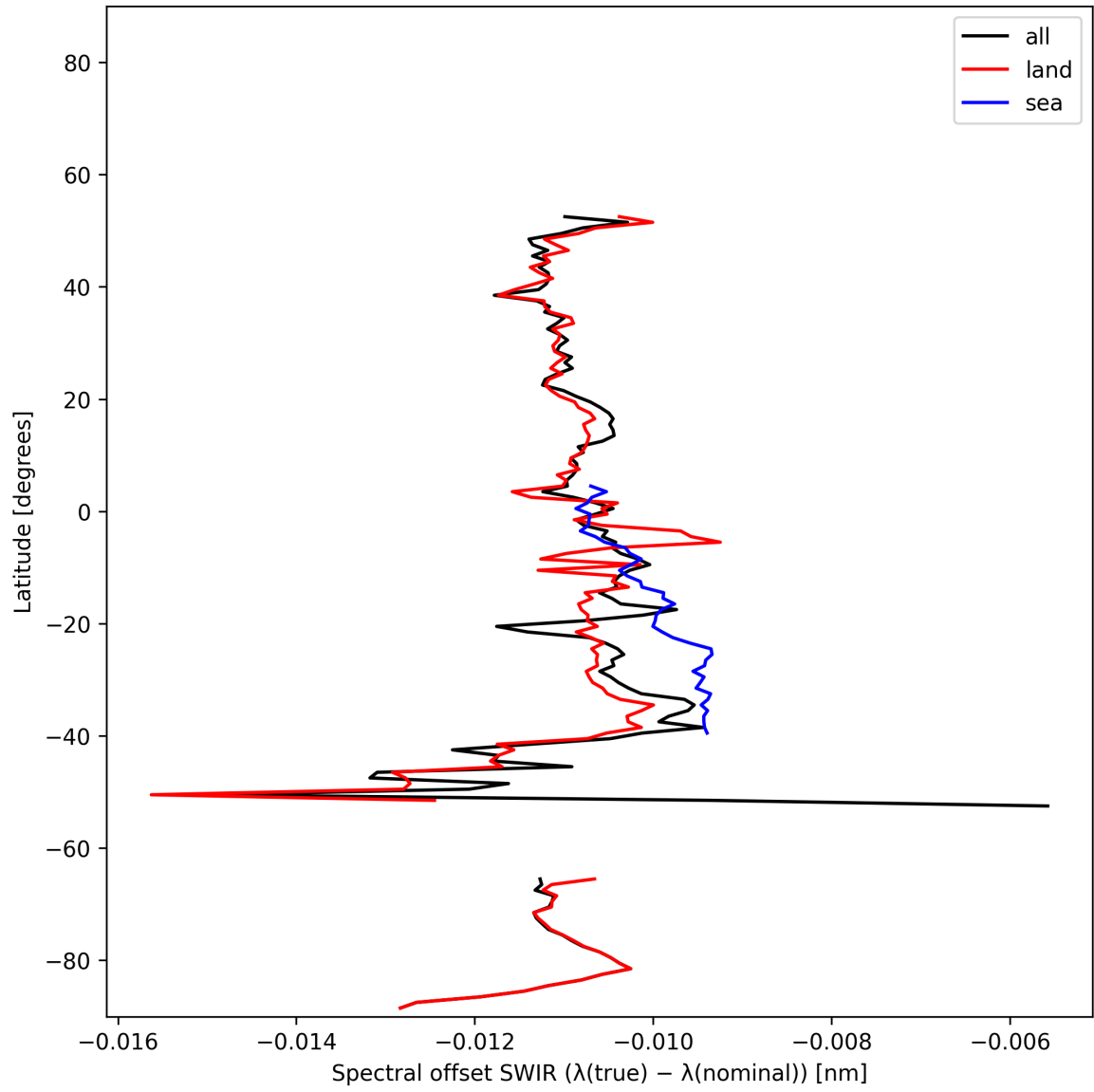
Figure 16: Zonal average of “Spectral offset SWIR ( \lambda_{\text{true}} - \lambda_{\text{nominal}} )” for 2025-01-04 to 2025-01-06.
