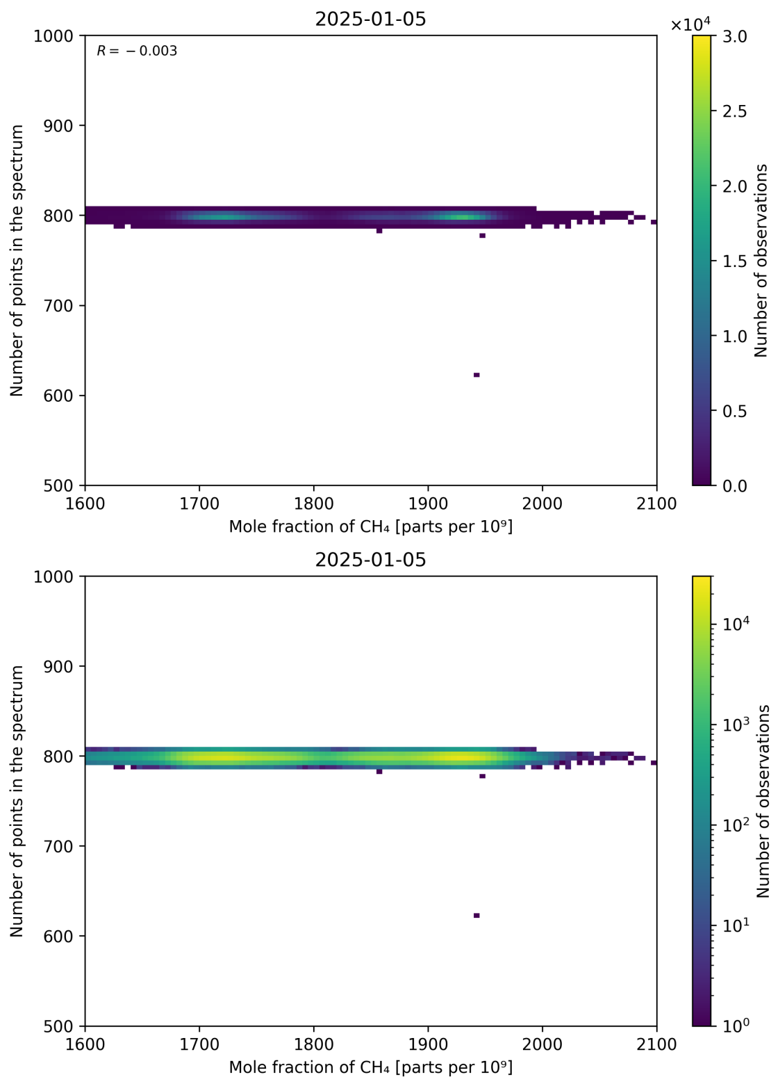
Figure 77: Scatter density plot of “Mole fraction of CH 4 ” against “Number of points in the spectrum” for 2025-01-04 to 2025-01-06.
