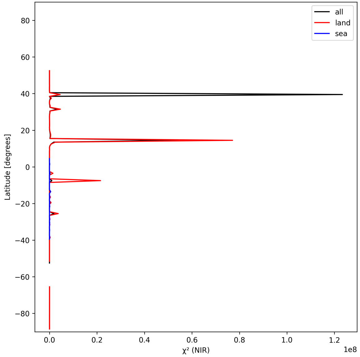
Figure 18: Zonal average of “ \chi^2 (NIR)” for 2025-01-04 to 2025-01-06.
