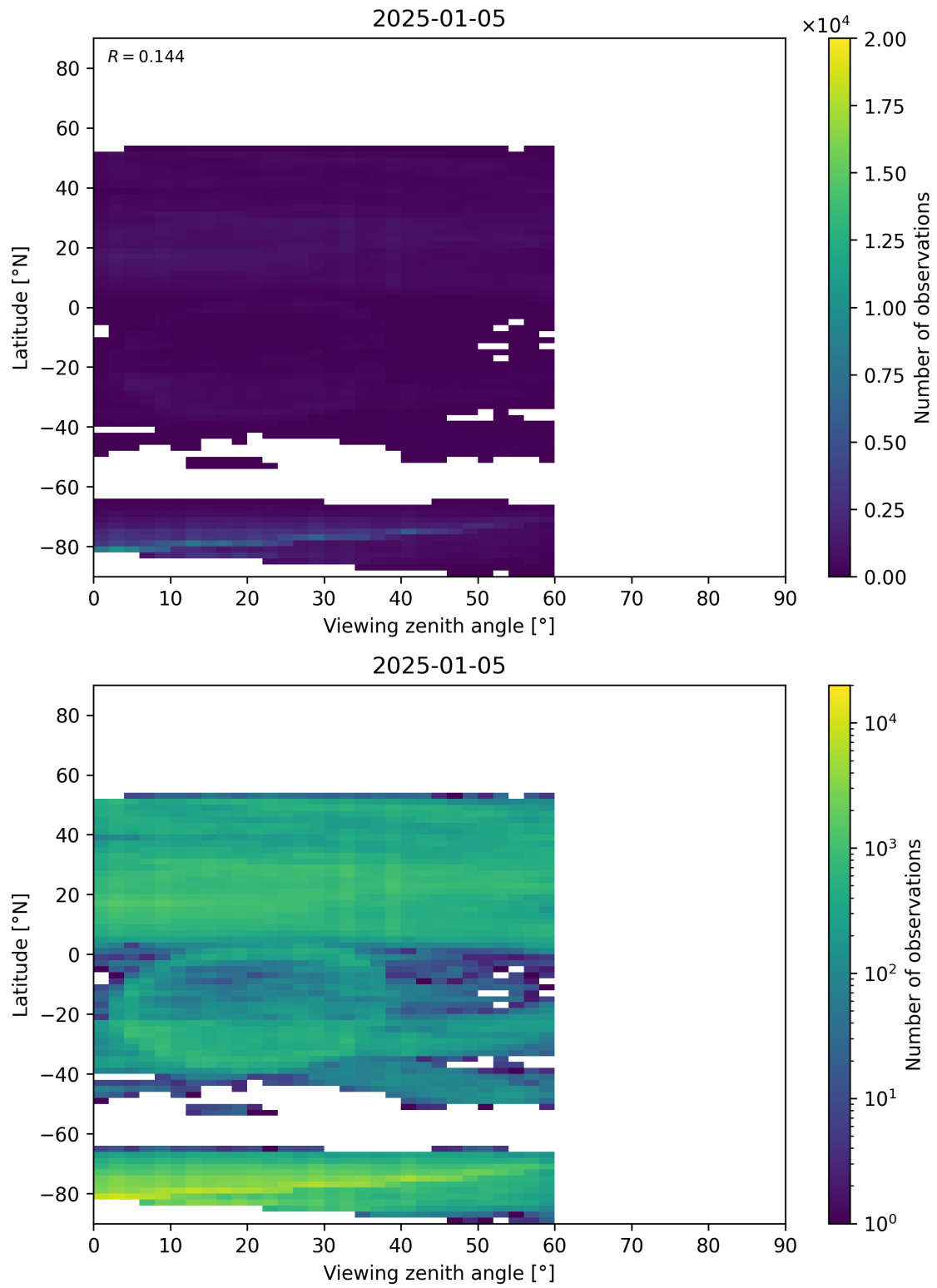
Figure 109: Scatter density plot of “Viewing zenith angle” against “Latitude” for 2025-01-04 to 2025-01-06.
