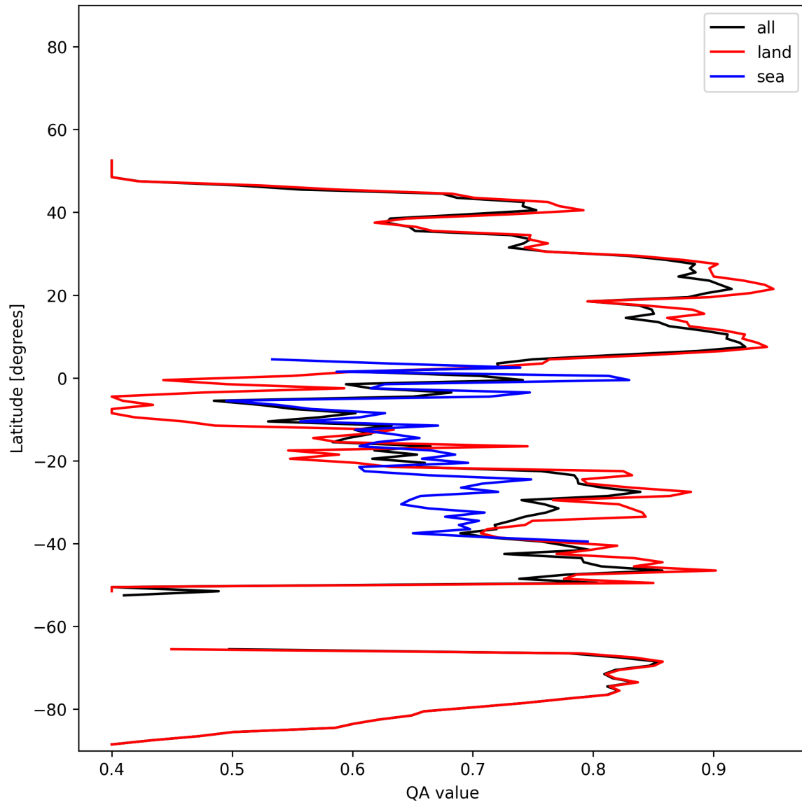
Figure 11: Zonal average of “QA value” for 2025-01-04 to 2025-01-06.
