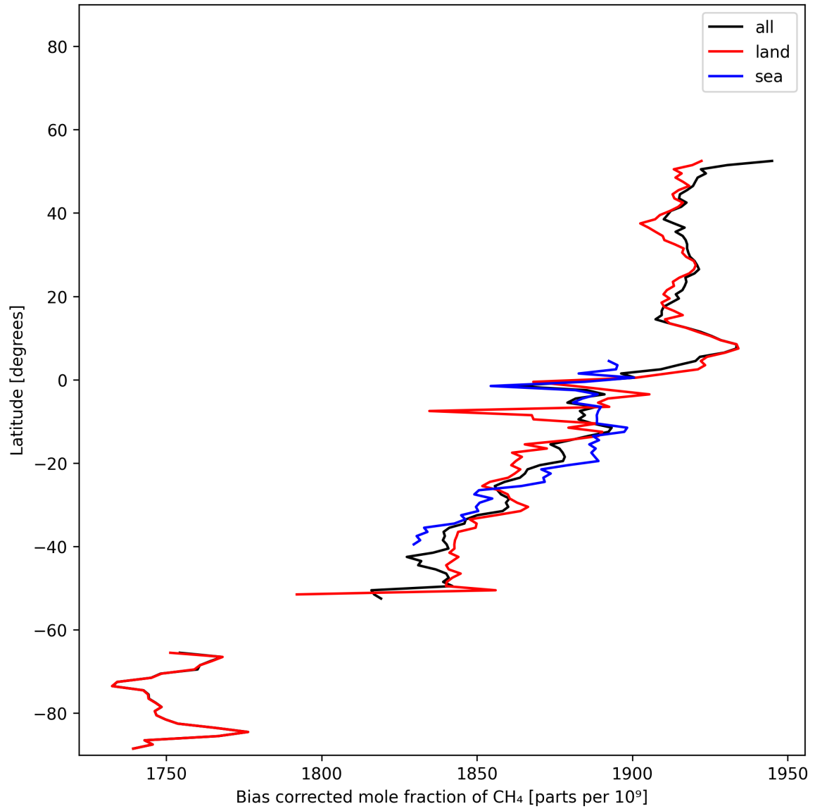
Figure 14: Zonal average of “Bias corrected mole fraction of CH 4 ” for 2025-01-04 to 2025-01-06.
