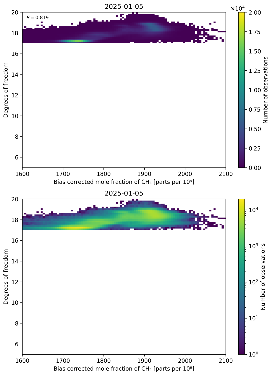
Figure 65: Scatter density plot of “Bias corrected mole fraction of CH 4 ” against “Degrees of freedom” for 2025-01-04 to 2025-01-06.
