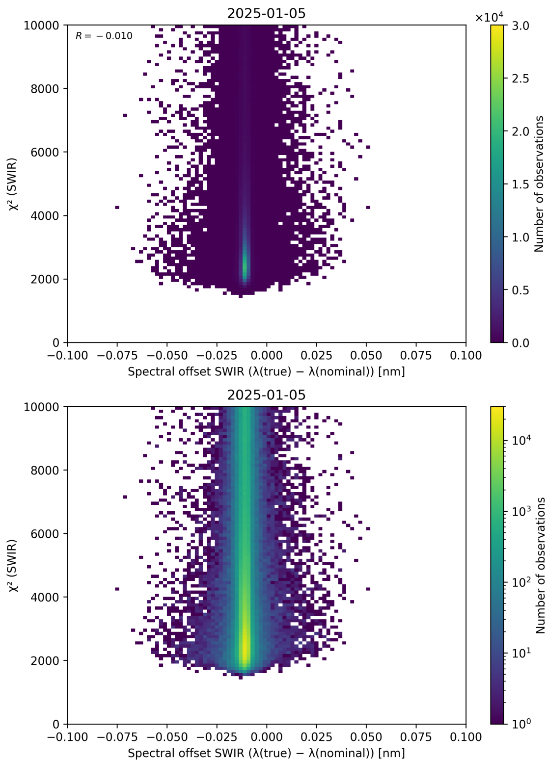
Figure 118: Scatter density plot of “Spectral offset SWIR ( \lambda_{\text{true}} - \lambda_{\text{nominal}} )” against “ \chi^2 (SWIR)” for 2025-01-04 to 2025-01-06.
