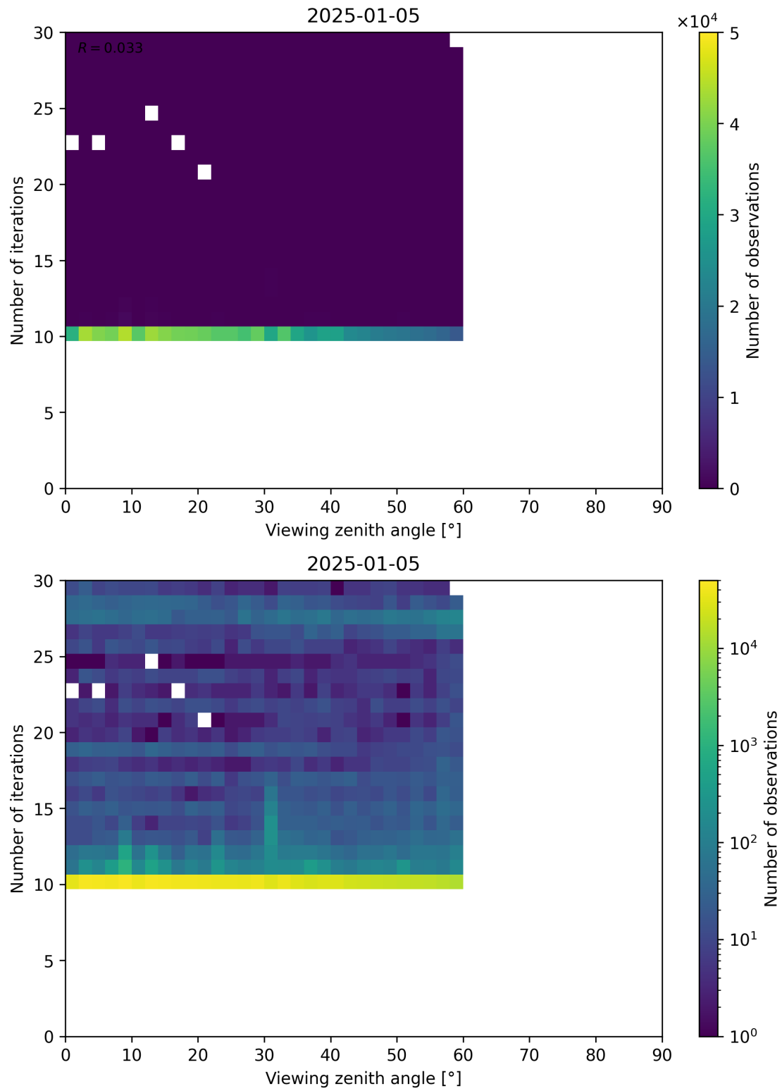
Figure 113: Scatter density plot of “Viewing zenith angle” against “Number of iterations” for 2025-01-04 to 2025-01-06.
