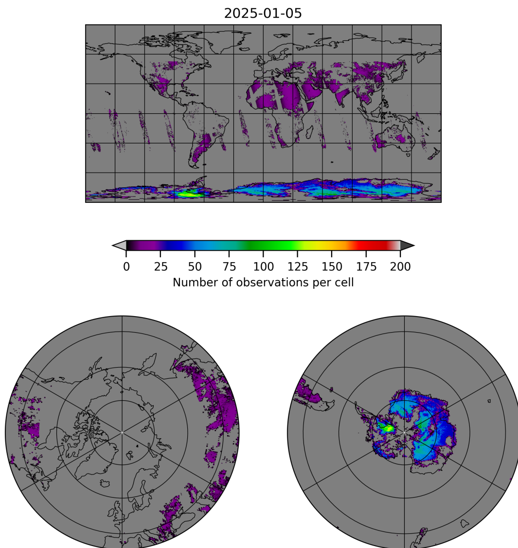
Figure 10: Map of the number of observations for 2025-01-04 to 2025-01-06
