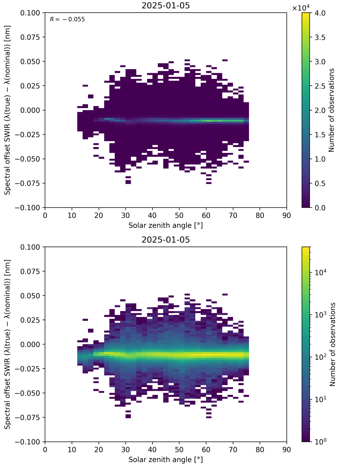
Figure 104: Scatter density plot of “Solar zenith angle” against “Spectral offset SWIR ( \lambda_{\text{true}} - \lambda_{\text{nominal}} )” for 2025-01-04 to 2025-01-06.
