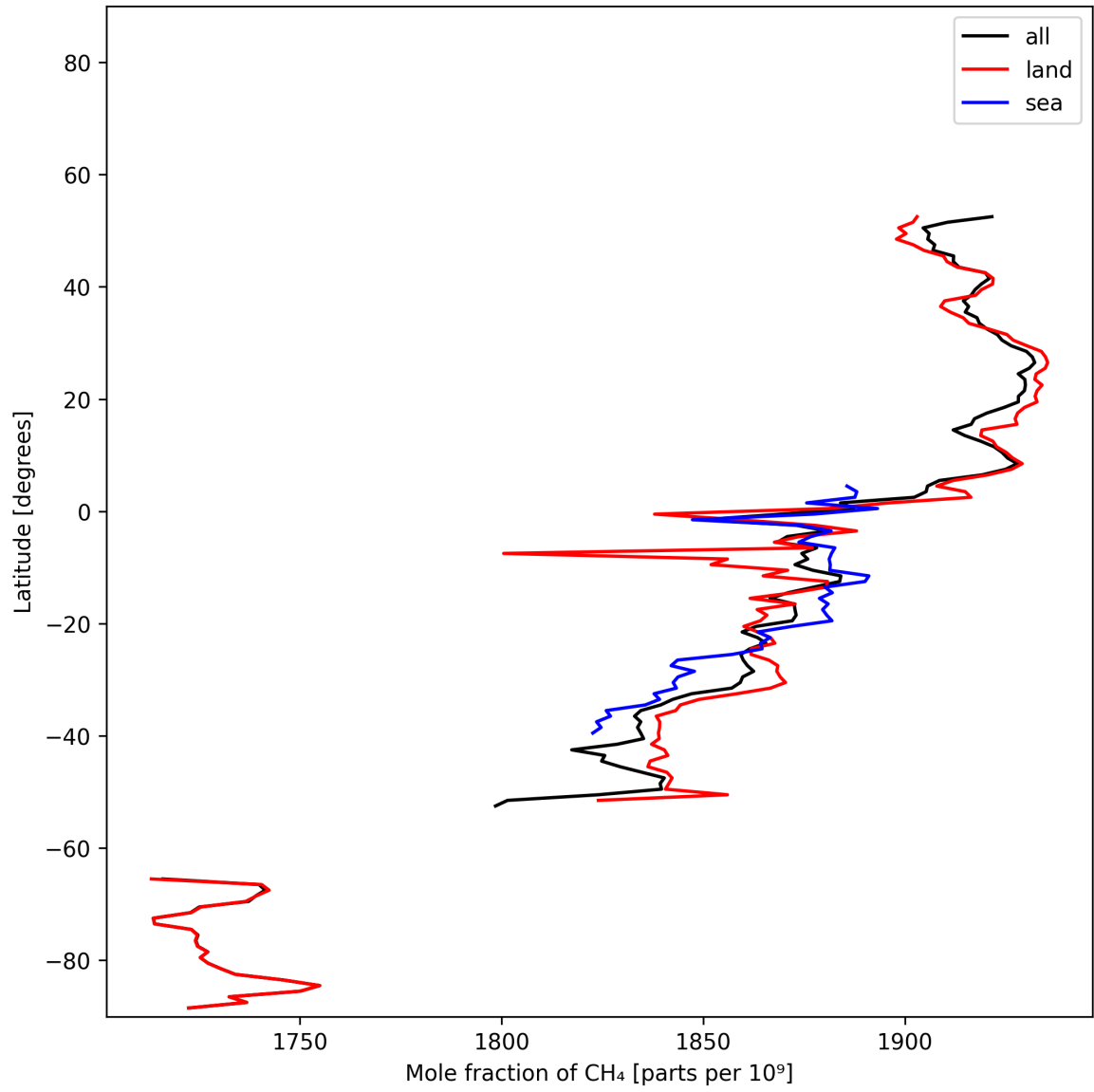
Figure 12: Zonal average of “Mole fraction of CH 4 ” for 2025-01-04 to 2025-01-06.
