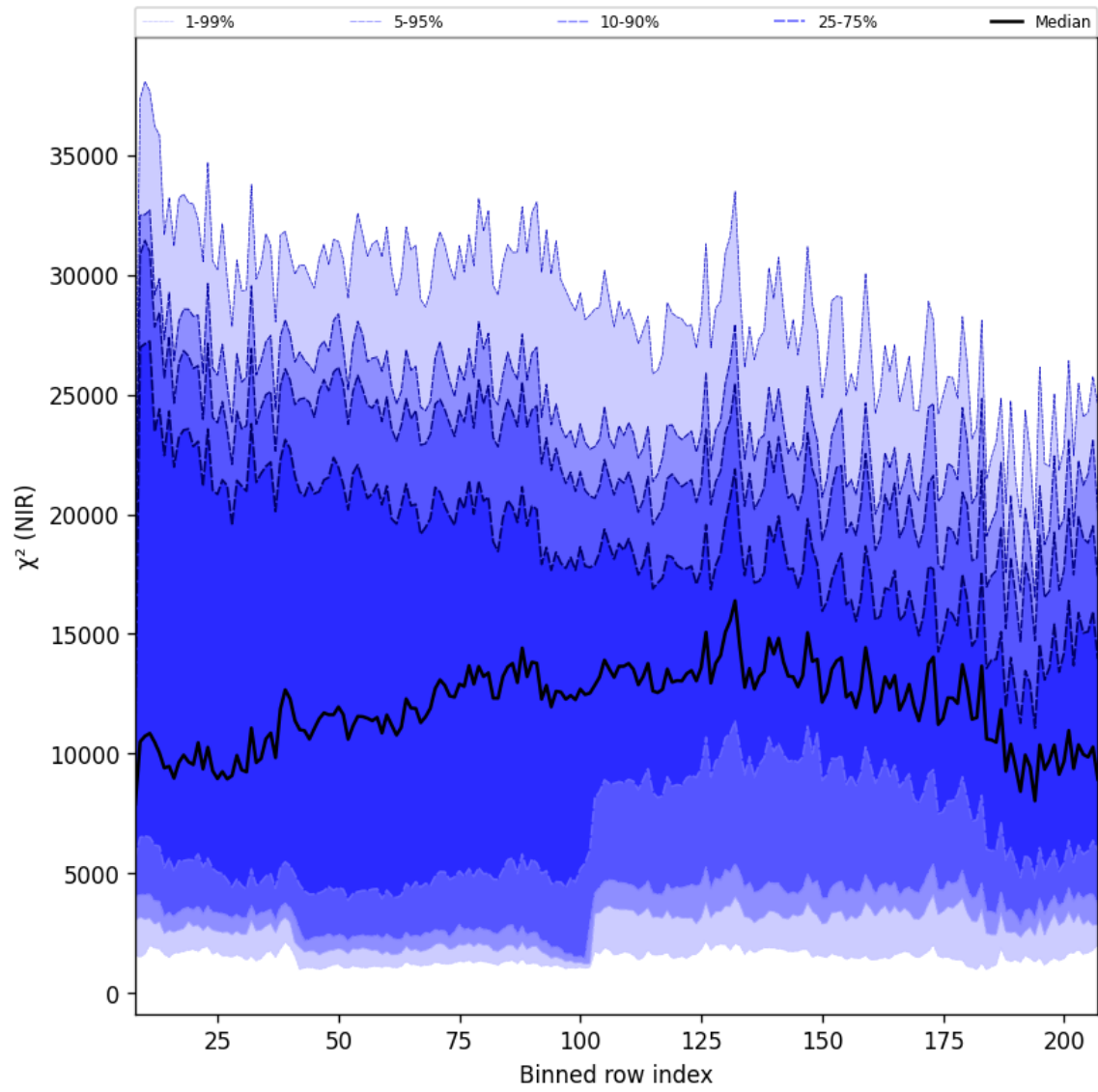
Figure 40: Along track statistics of “ \chi^2 (NIR)” for 2025-01-04 to 2025-01-06
