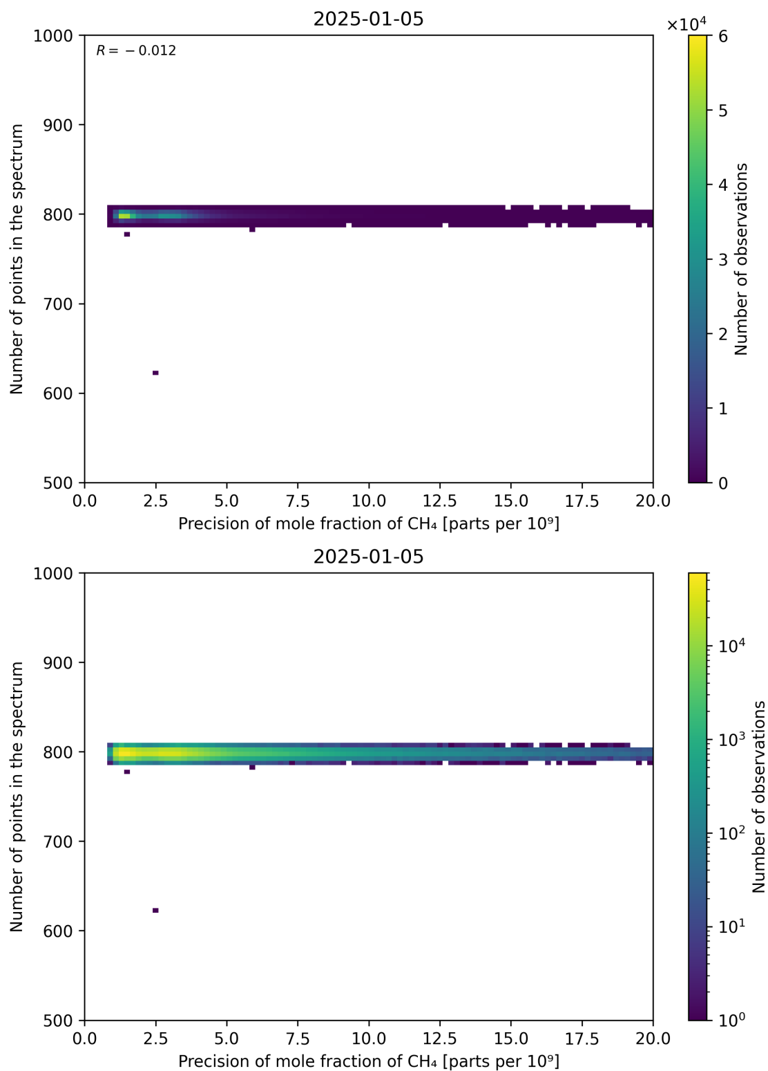
Figure 84: Scatter density plot of “Precision of mole fraction of CH 4 ” against “Number of points in the spectrum” for 2025-01-04 to 2025-01-06.
