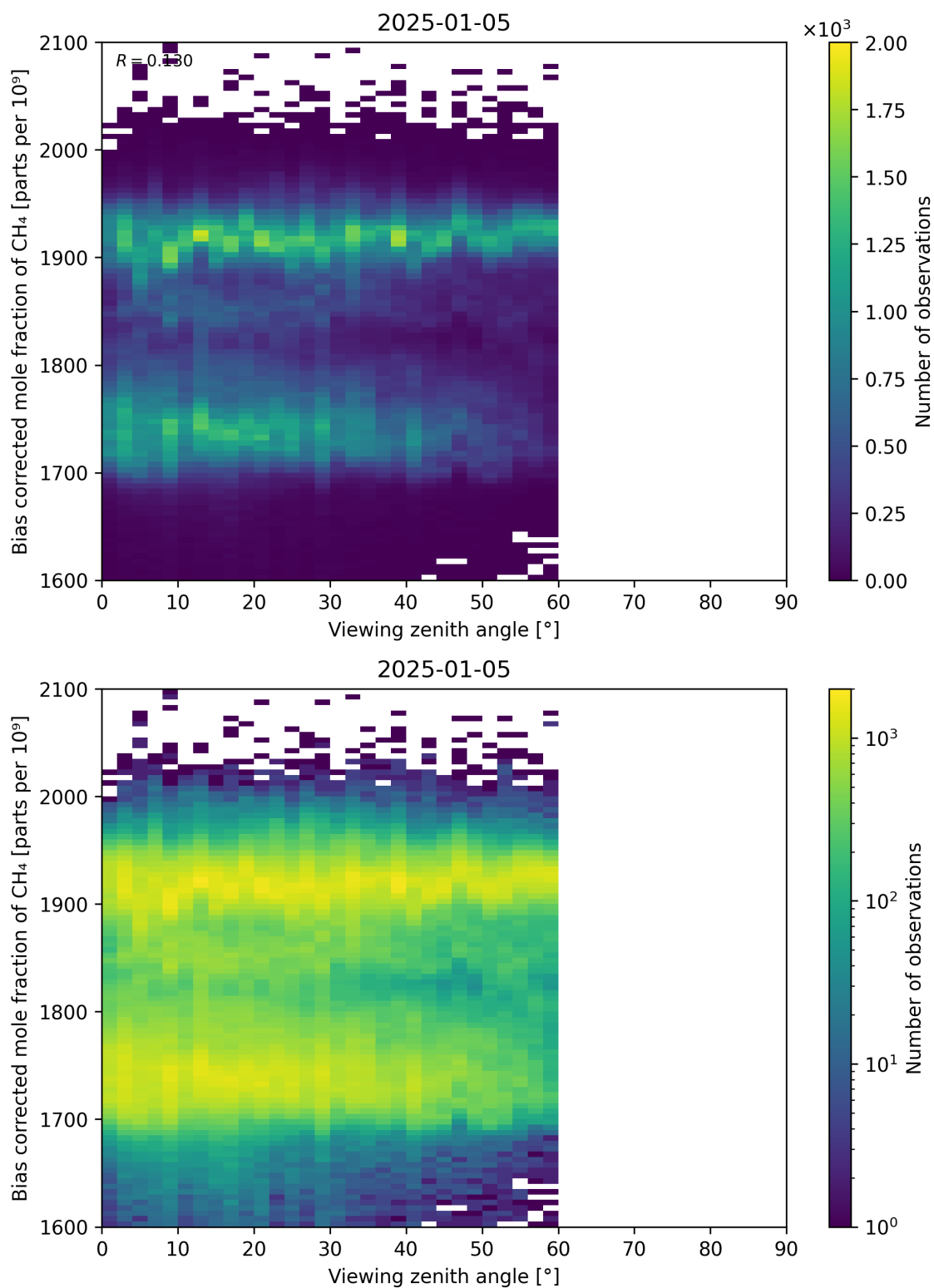
Figure 111: Scatter density plot of “Viewing zenith angle” against “Bias corrected mole fraction of CH 4 ” for 2025-01-04 to 2025-01-06.
