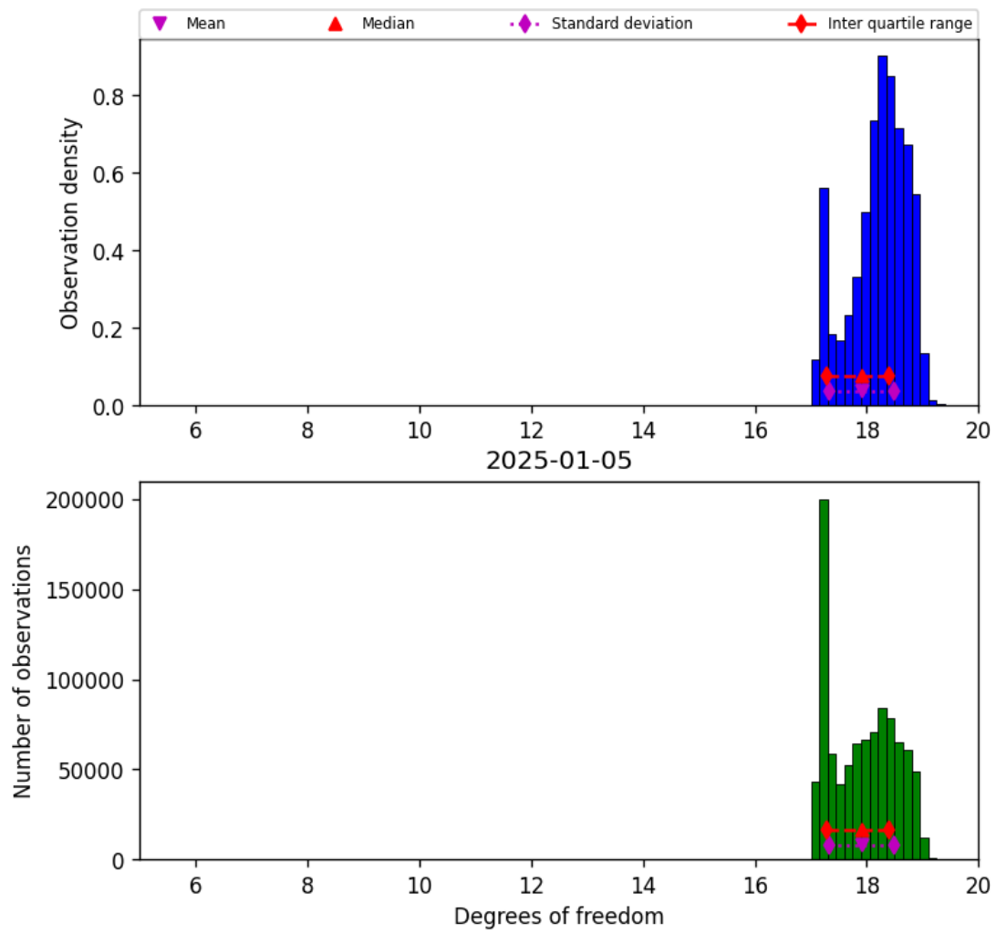
Figure 30: Histogram of “Degrees of freedom” for 2025-01-04 to 2025-01-06
