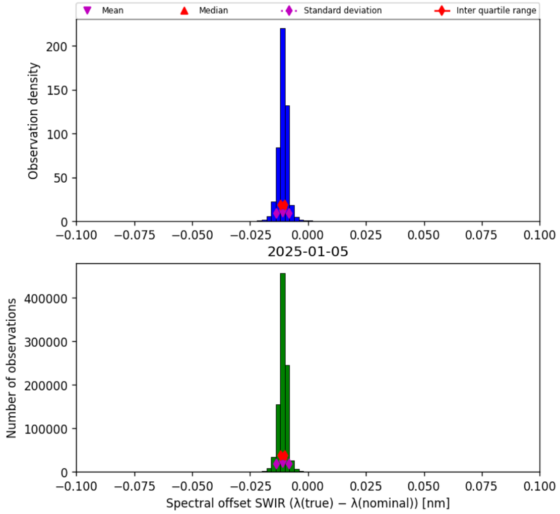
Figure 27: Histogram of “Spectral offset SWIR ( \lambda_{\text{true}} - \lambda_{\text{nominal}} )” for 2025-01-04 to 2025-01-06
