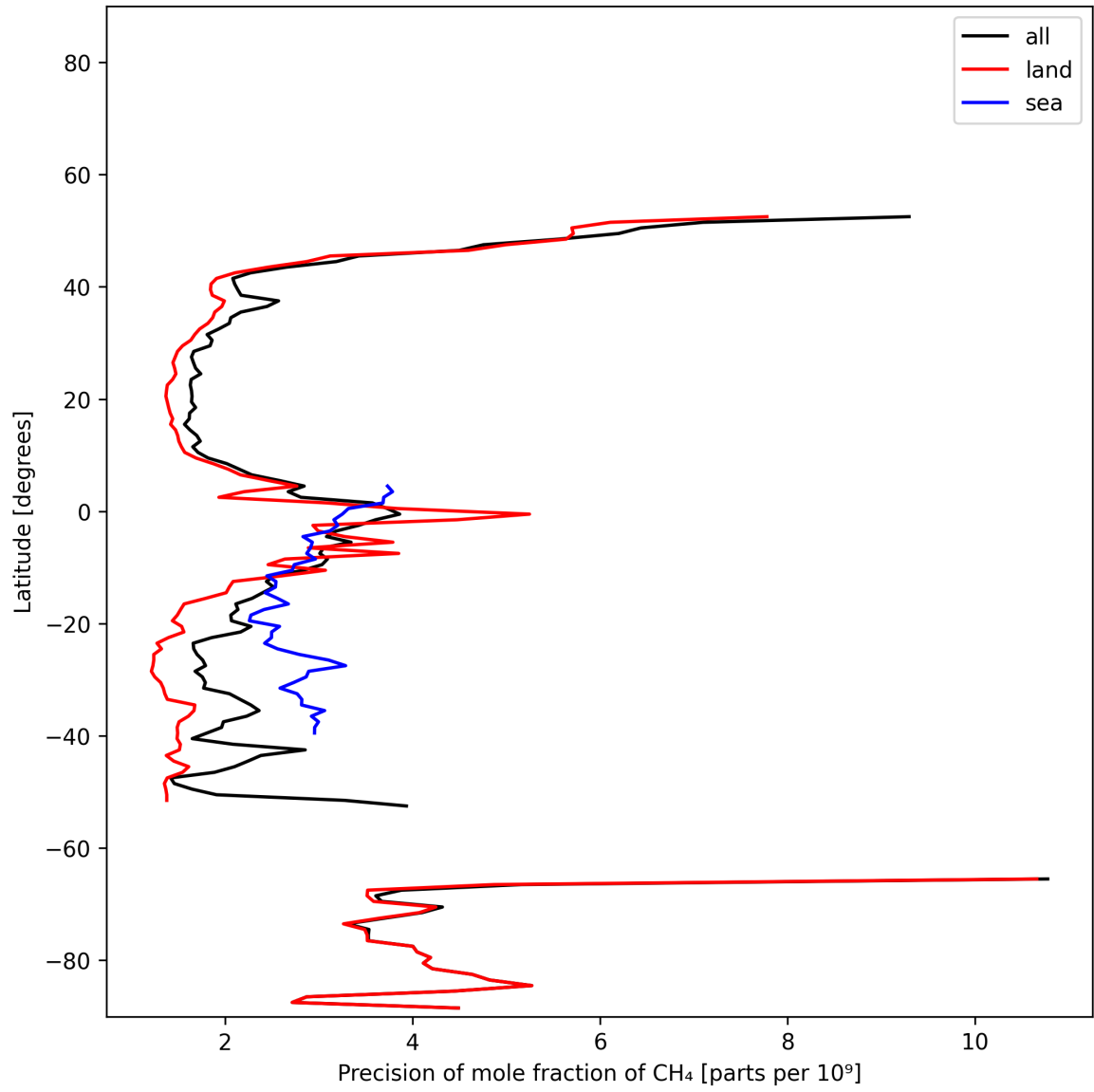
Figure 13: Zonal average of “Precision of mole fraction of CH 4 ” for 2025-01-04 to 2025-01-06.
