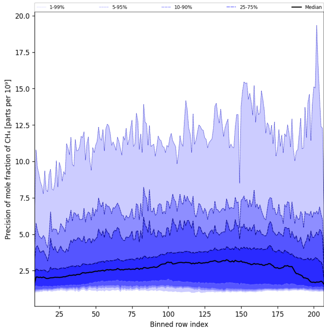
Figure 35: Along track statistics of “Precision of mole fraction of CH 4 ” for 2025-01-04 to 2025-01-06
