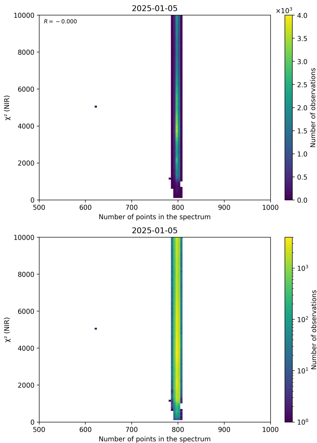
Figure 88: Scatter density plot of “Number of points in the spectrum” against “ \chi^2 (NIR)” for 2025-01-04 to 2025-01-06.
