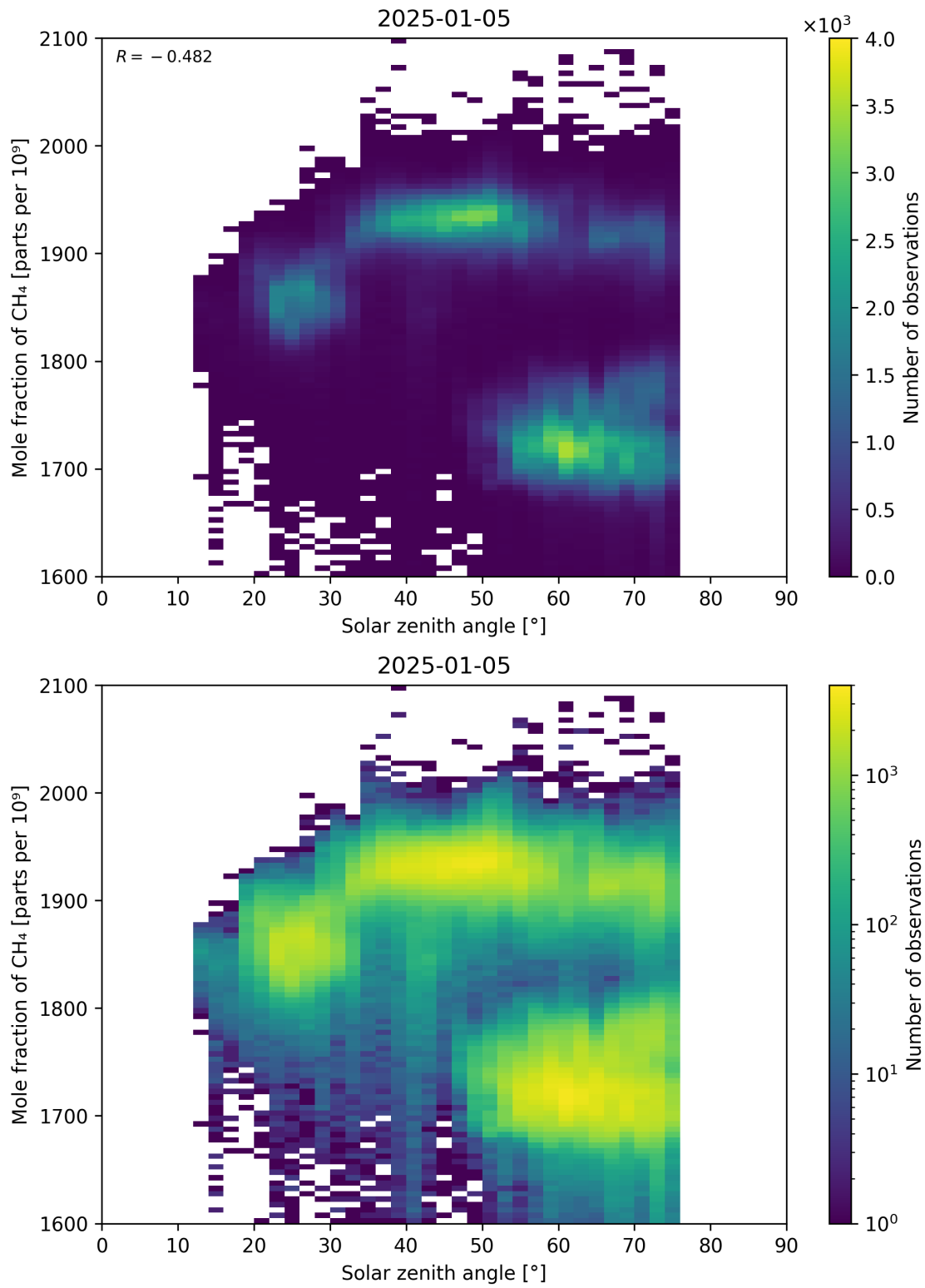
Figure 99: Scatter density plot of “Solar zenith angle” against “Mole fraction of CH 4 ” for 2025-01-04 to 2025-01-06.
