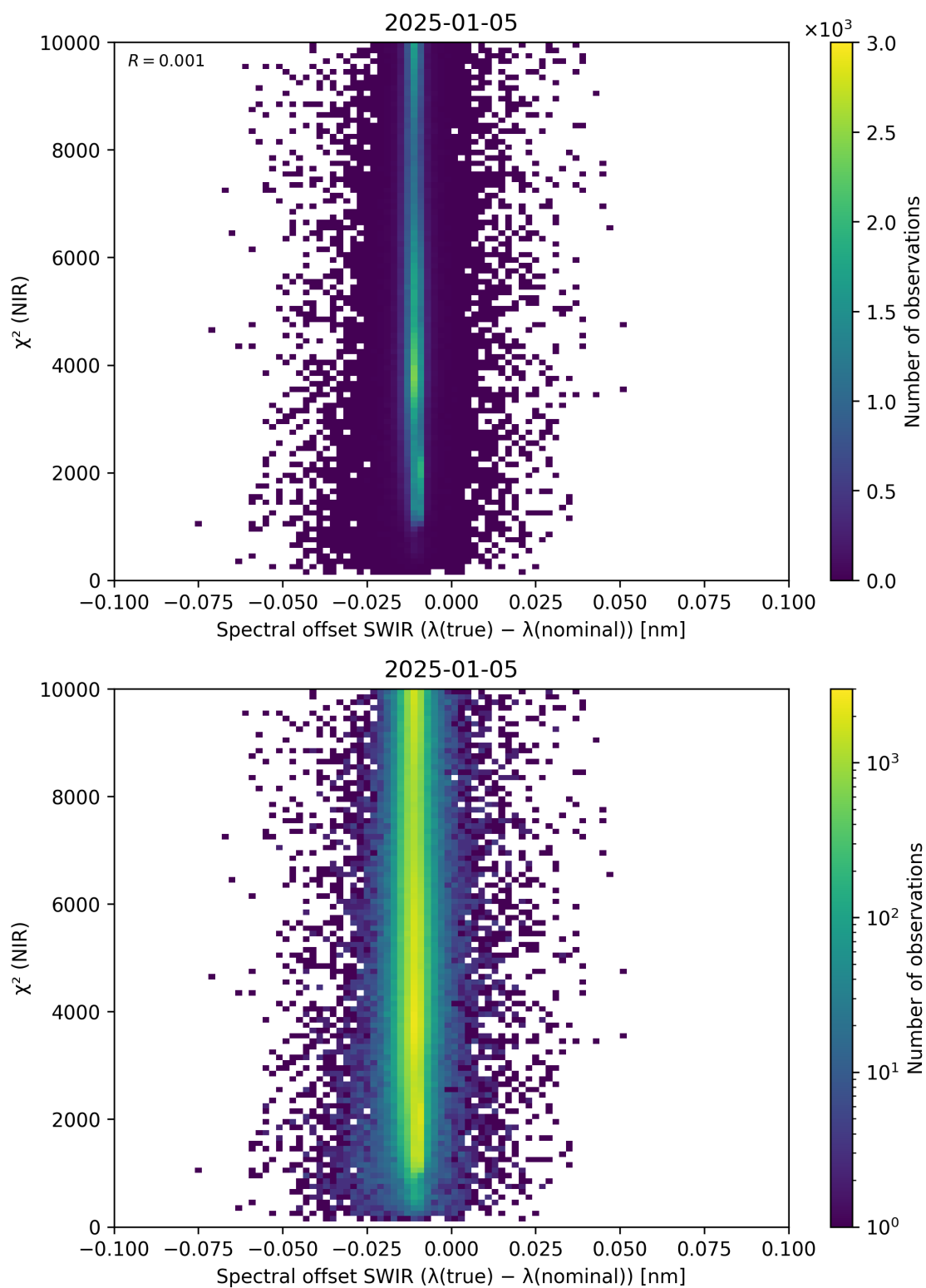
Figure 117: Scatter density plot of “Spectral offset SWIR ( \lambda_{\text{true}} - \lambda_{\text{nominal}} )” against “ \chi^2 (NIR)” for 2025-01-04 to 2025-01-06.
