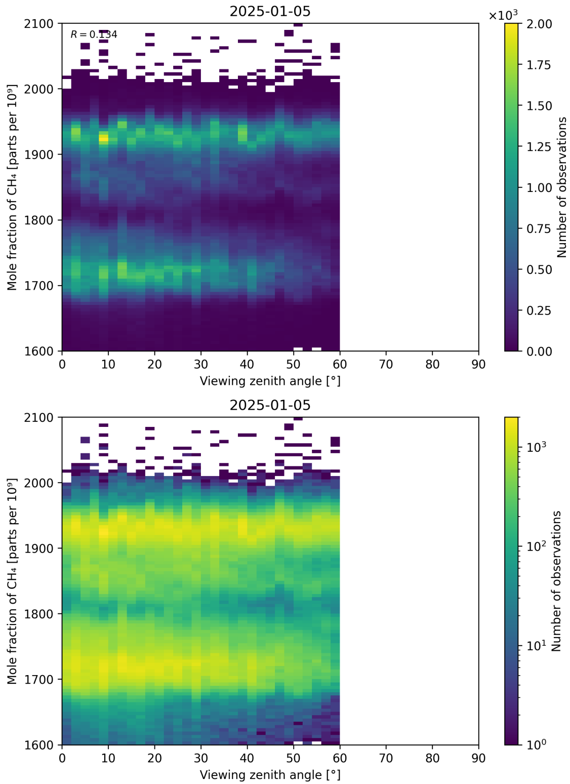
Figure 110: Scatter density plot of “Viewing zenith angle” against “Mole fraction of CH 4 ” for 2025-01-04 to 2025-01-06.
