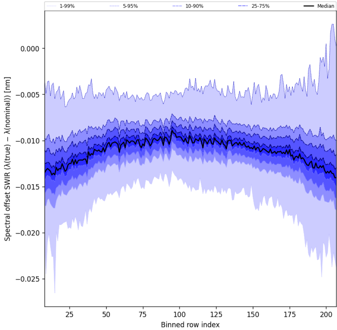
Figure 38: Along track statistics of “Spectral offset SWIR ( \lambda_{\text{true}} - \lambda_{\text{nominal}} )” for 2025-01-04 to 2025-01-06
