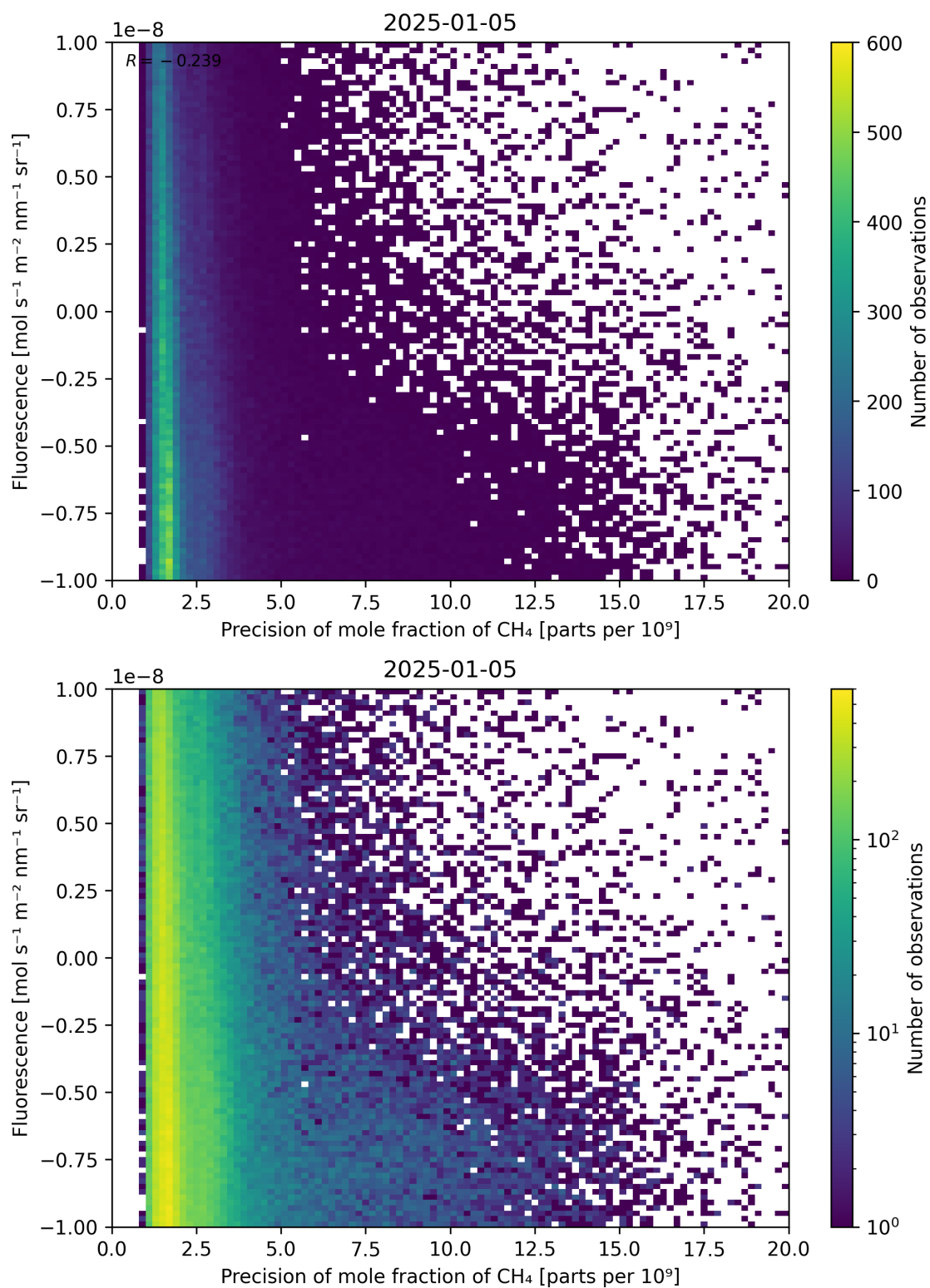
Figure 81: Scatter density plot of “Precision of mole fraction of \text{CH}_4 ” against “Fluorescence” for 2025-01-04 to 2025-01-06.
