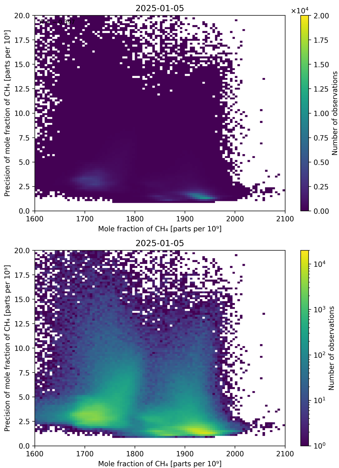
Figure 75: Scatter density plot of “Mole fraction of CH 4 ” against “Precision of mole fraction of CH 4 ” for 2025-01-04 to 2025-01-06.
