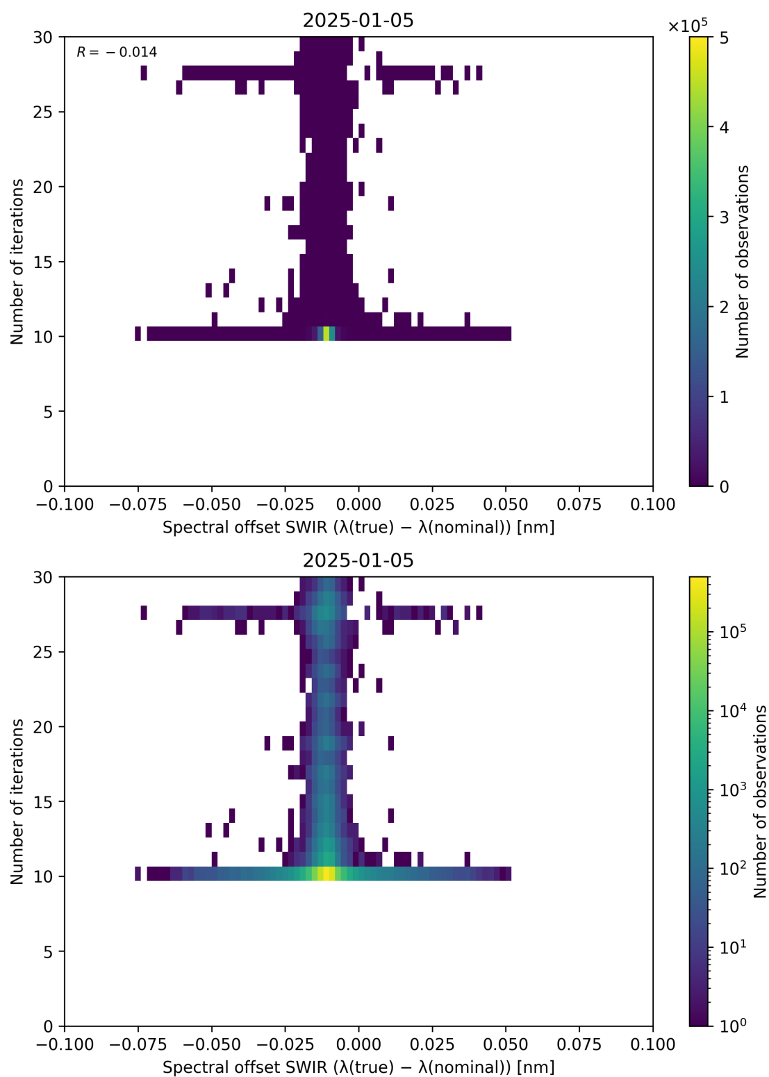
Figure 121: Scatter density plot of “Spectral offset SWIR ( \lambda_{\text{true}} - \lambda_{\text{nominal}} )” against “Number of iterations” for 2025-01-04 to 2025-01-06.
