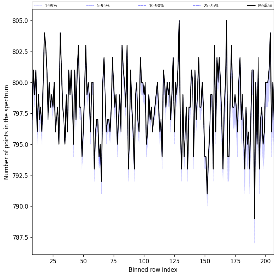
Figure 37: Along track statistics of “Number of points in the spectrum” for 2025-01-04 to 2025-01-06
