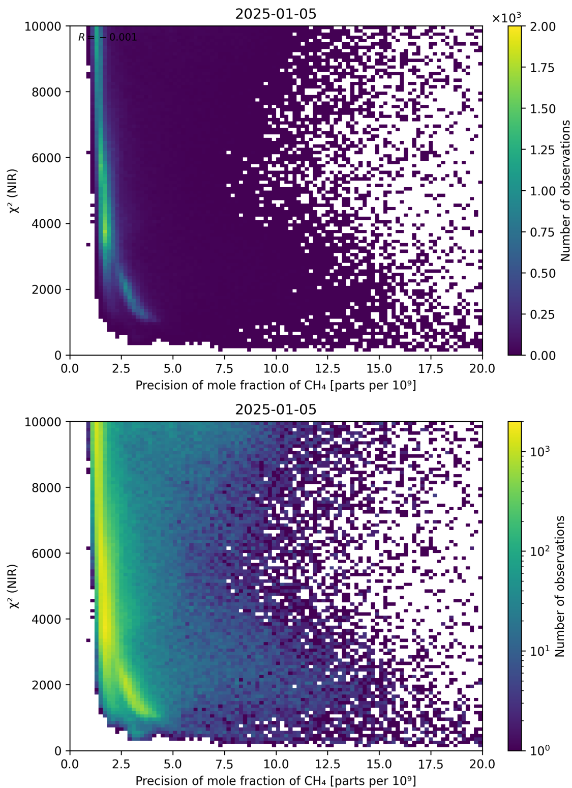
Figure 78: Scatter density plot of “Precision of mole fraction of CH 4 ” against “ \chi^2 (NIR)” for 2025-01-04 to 2025-01-06.
