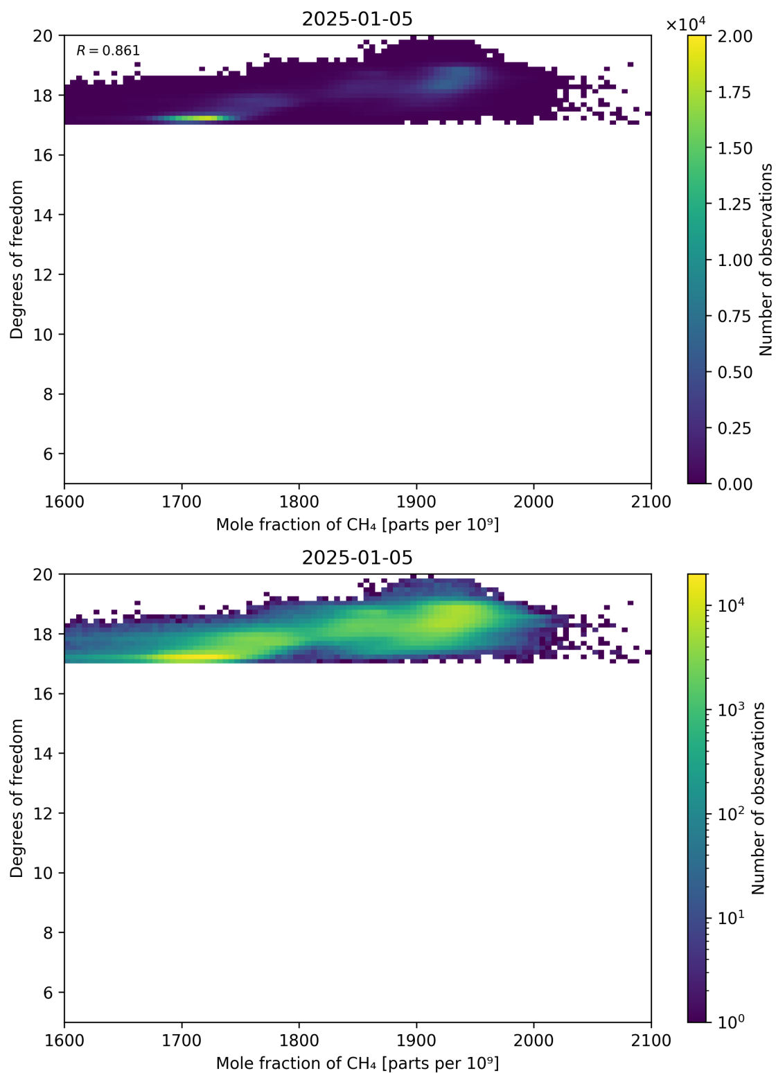
Figure 72: Scatter density plot of “Mole fraction of CH 4 ” against “Degrees of freedom” for 2025-01-04 to 2025-01-06.
