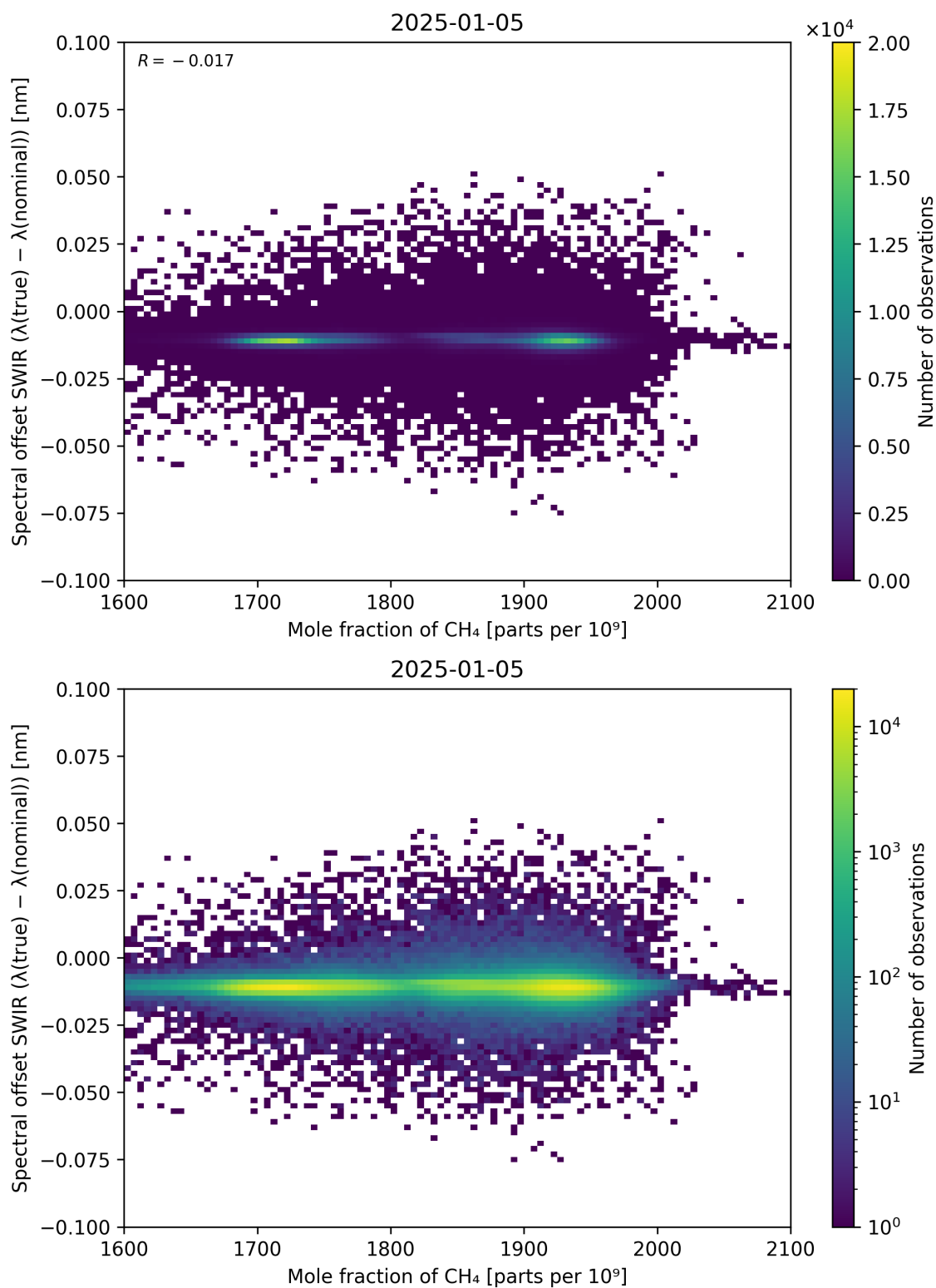
Figure 86: Scatter density plot of “Mole fraction of CH 4 ” against “Spectral offset SWIR ( \lambda_{\text{true}} - \lambda_{\text{nominal}} )” for 2025-01-04 to 2025-01-06.
