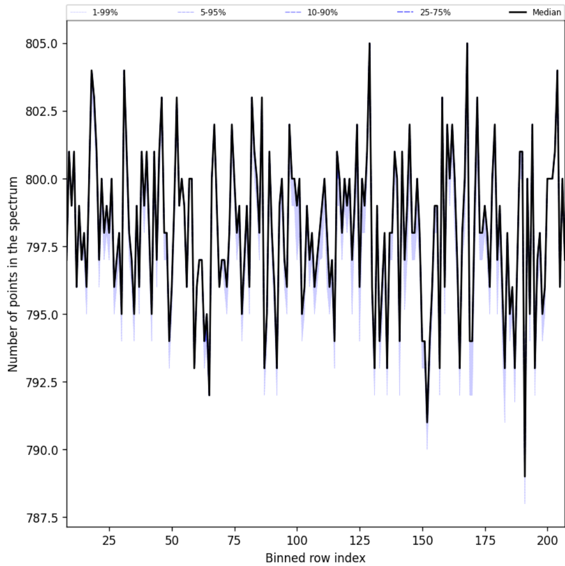
Figure 37: Along track statistics of “Number of points in the spectrum” for 2025-01-05 to 2025-01-07
