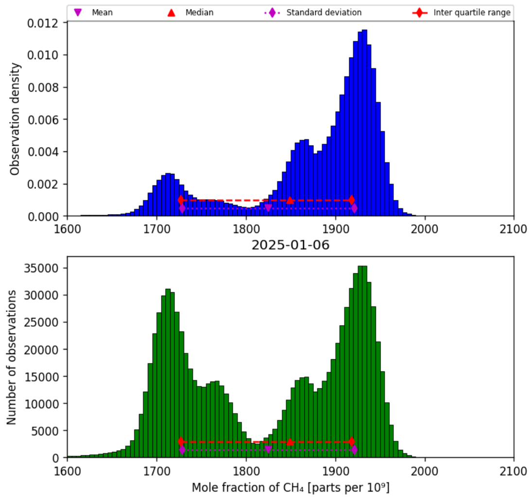
Figure 23: Histogram of “Mole fraction of CH 4 ” for 2025-01-05 to 2025-01-07
