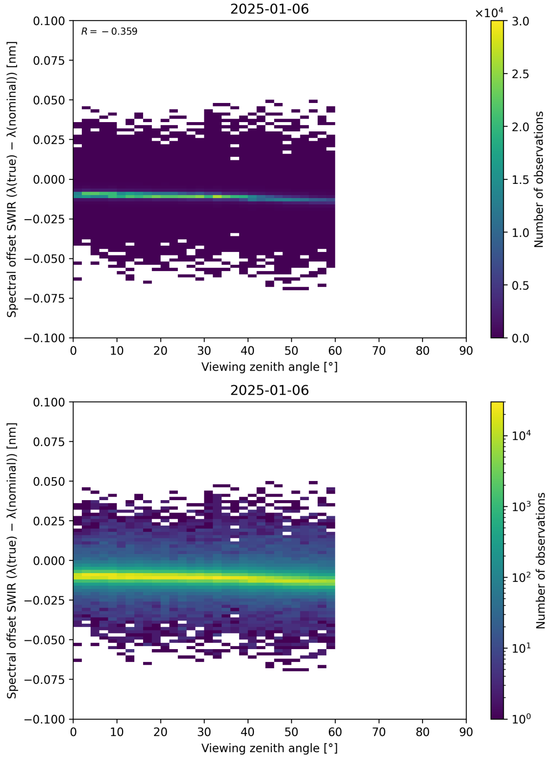
Figure 116: Scatter density plot of “Viewing zenith angle” against “Spectral offset SWIR ( \lambda_{\text{true}} - \lambda_{\text{nominal}} )” for 2025-01-05 to 2025-01-07.
