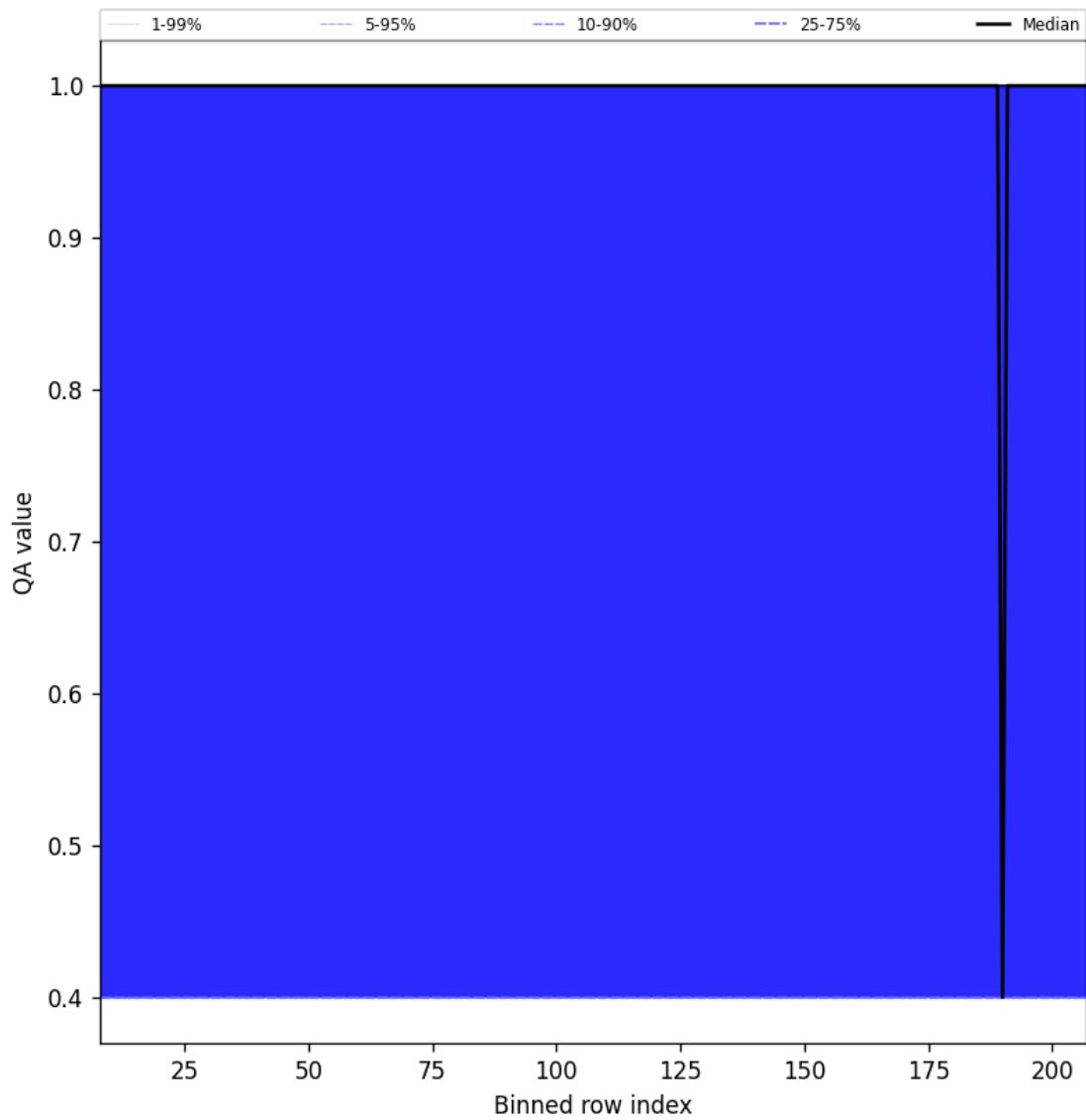
Figure 33: Along track statistics of “QA value” for 2025-01-05 to 2025-01-07
