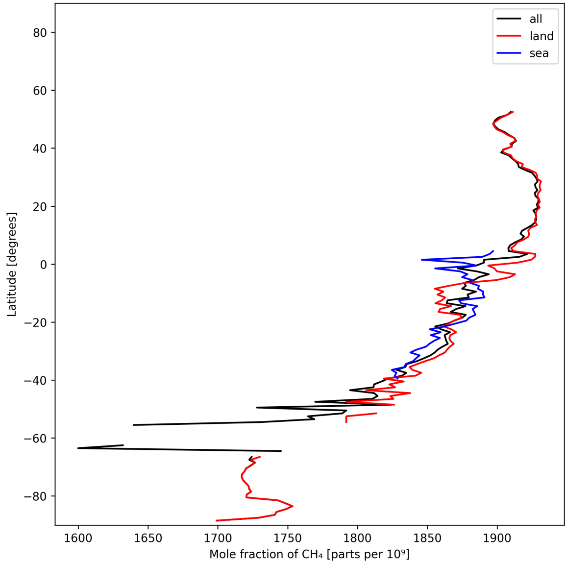
Figure 12: Zonal average of “Mole fraction of CH 4 ” for 2025-01-05 to 2025-01-07.
