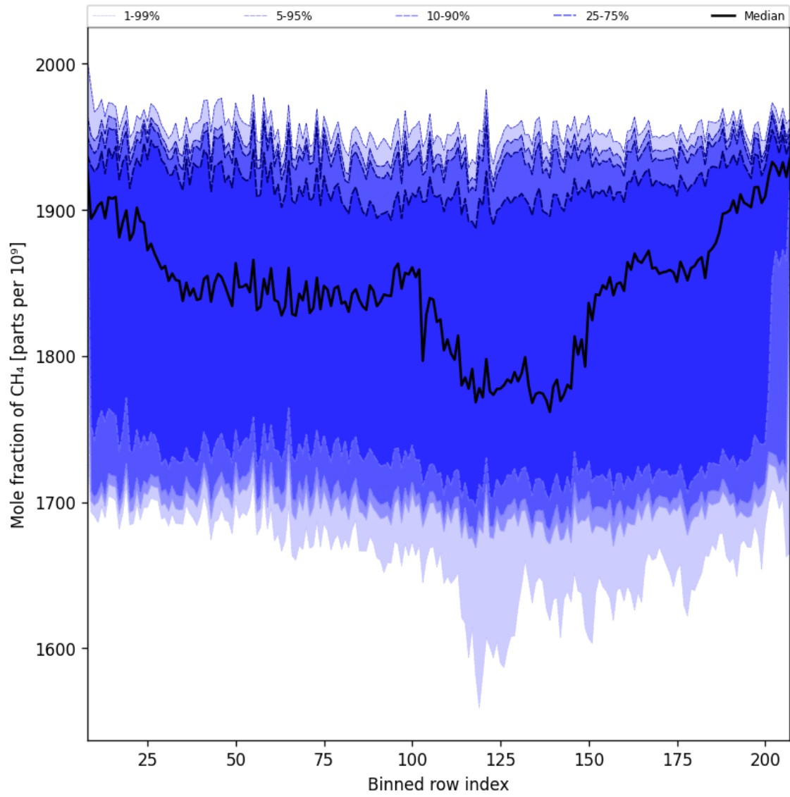
Figure 34: Along track statistics of “Mole fraction of CH 4 ” for 2025-01-05 to 2025-01-07
