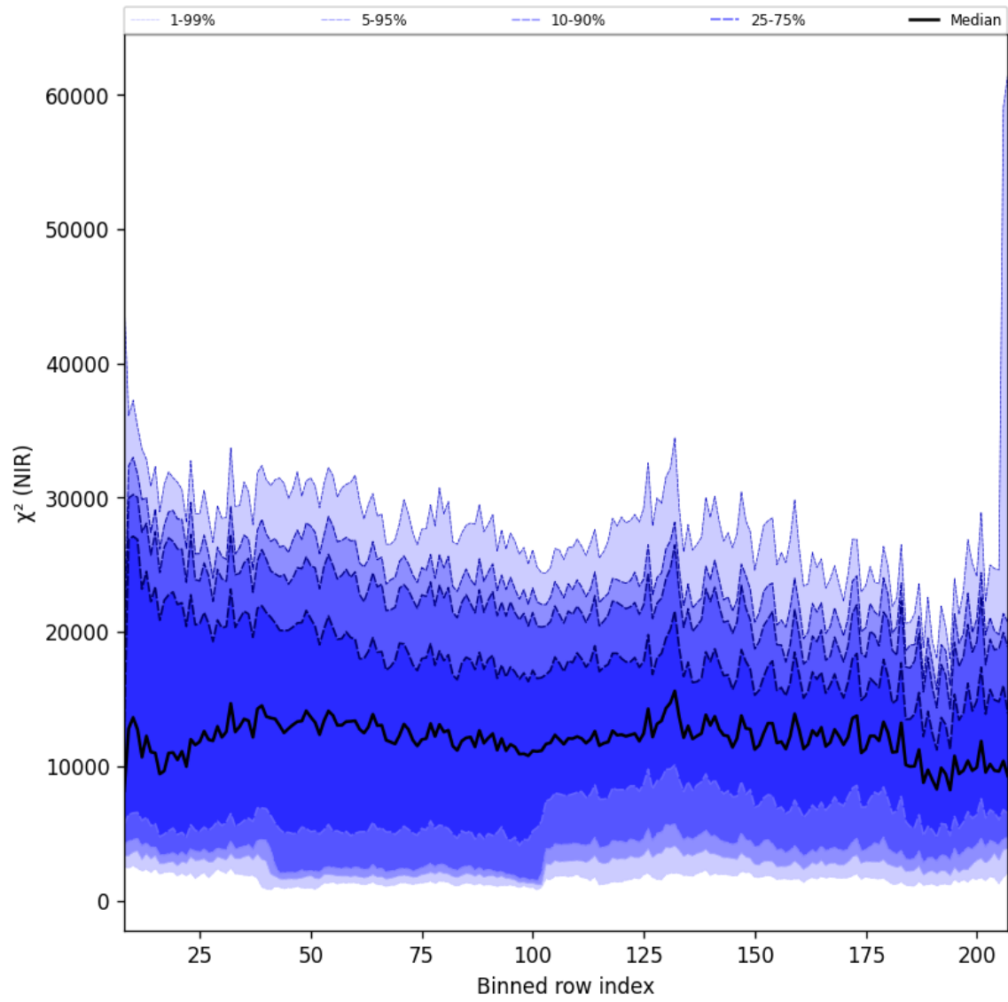
Figure 40: Along track statistics of “ \chi^2 (NIR)” for 2025-01-05 to 2025-01-07
