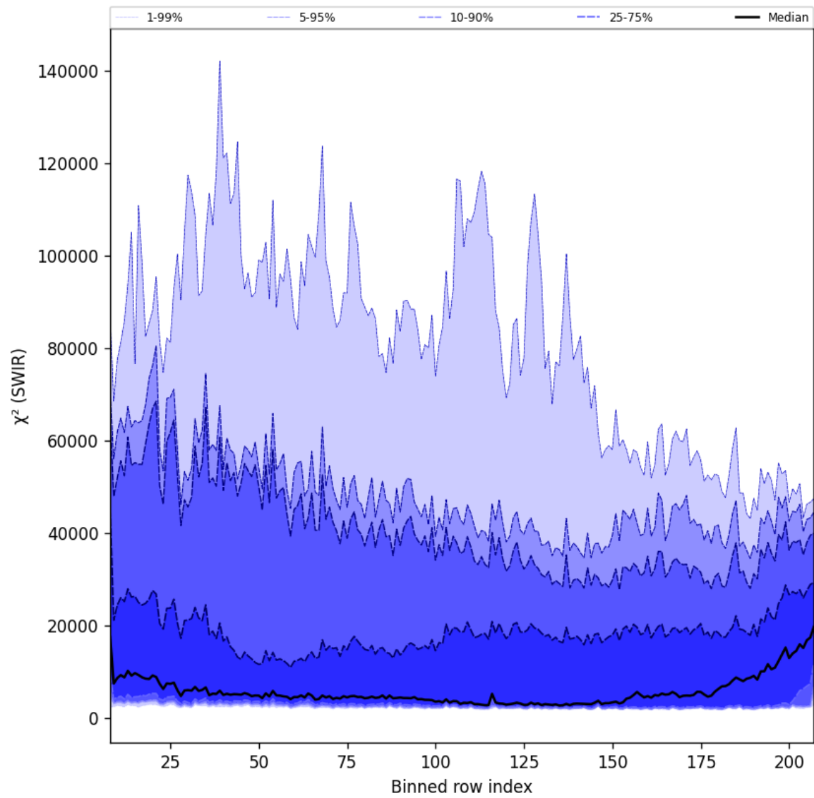
Figure 39: Along track statistics of “ \chi^2 (SWIR)” for 2025-01-05 to 2025-01-07
