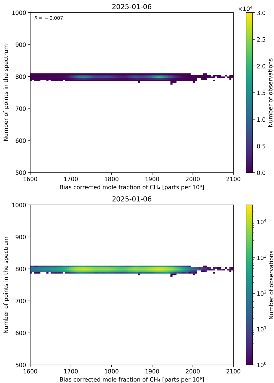
Figure 68: Scatter density plot of “Bias corrected mole fraction of CH 4 ” against “Number of points in the spectrum” for 2025-01-05 to 2025-01-07.
