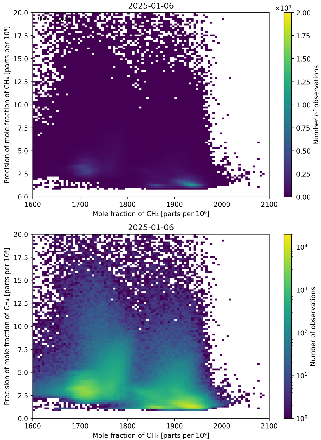
Figure 75: Scatter density plot of “Mole fraction of CH 4 ” against “Precision of mole fraction of CH 4 ” for 2025-01-05 to 2025-01-07.
