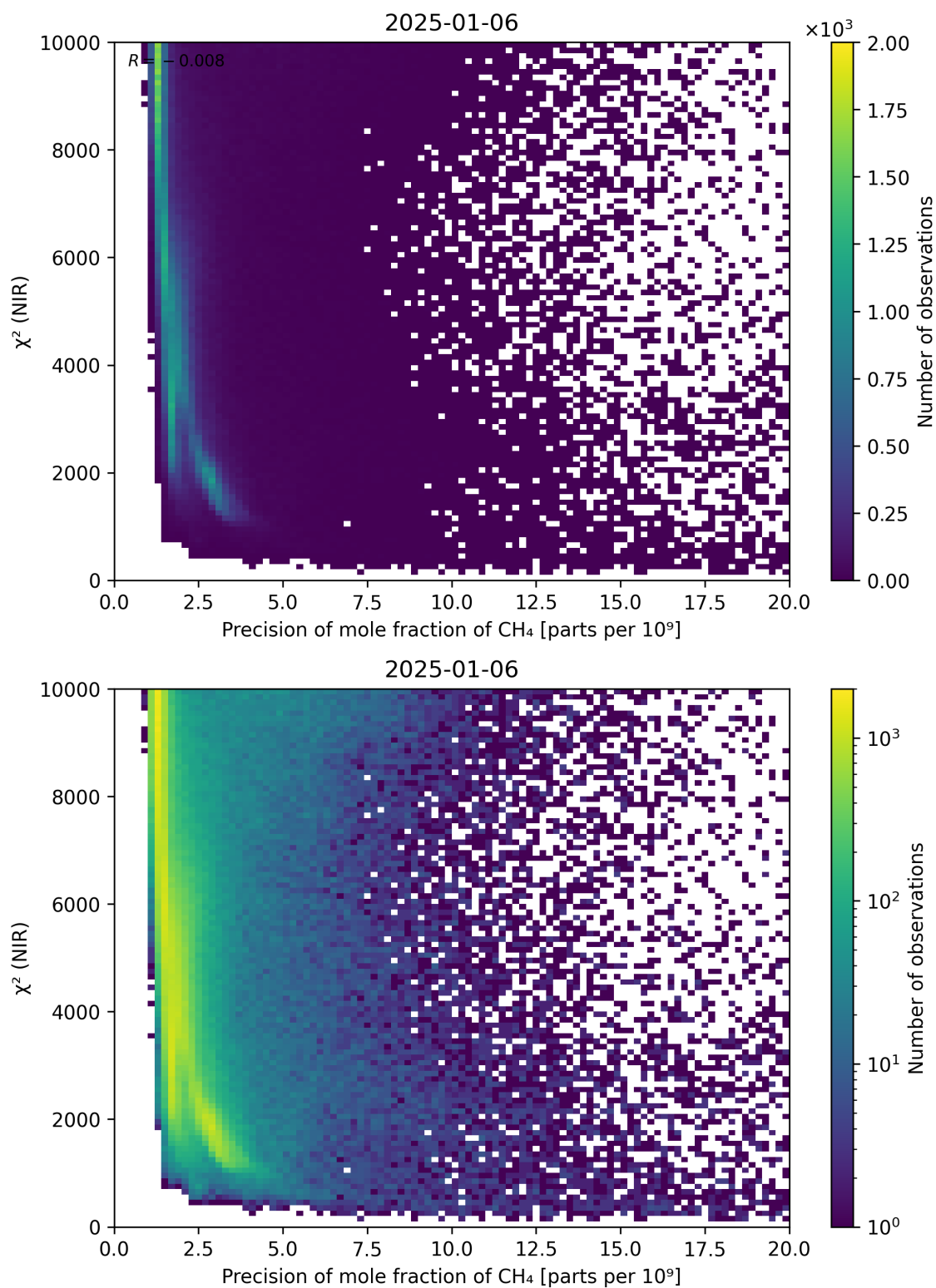
Figure 78: Scatter density plot of “Precision of mole fraction of \text{CH}_4 ” against “ \chi^2 (NIR)” for 2025-01-05 to 2025-01-07.
