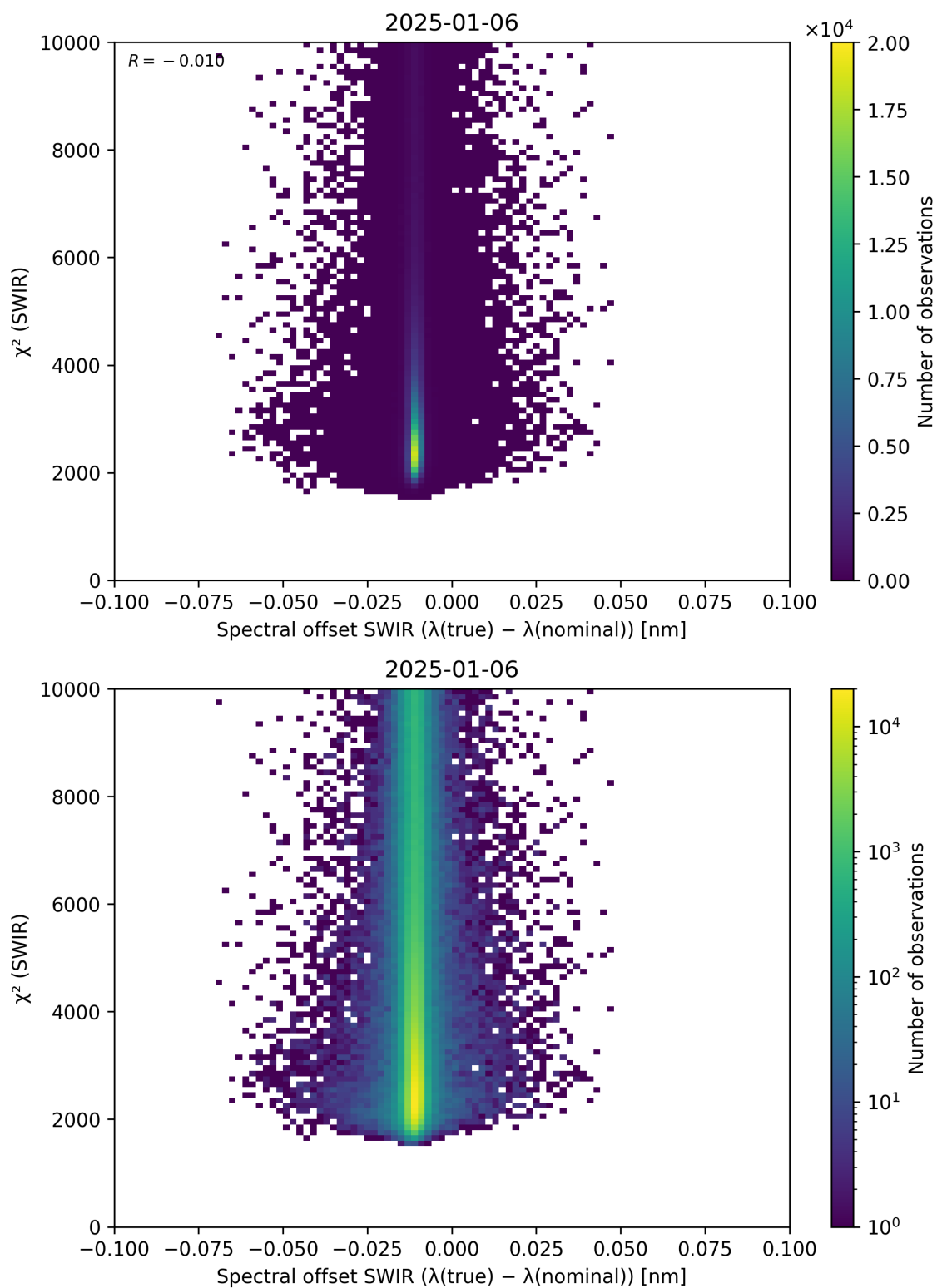
Figure 118: Scatter density plot of “Spectral offset SWIR ( \lambda_{\text{true}} - \lambda_{\text{nominal}} )” against “ \chi^2 (SWIR)” for 2025-01-05 to 2025-01-07.
