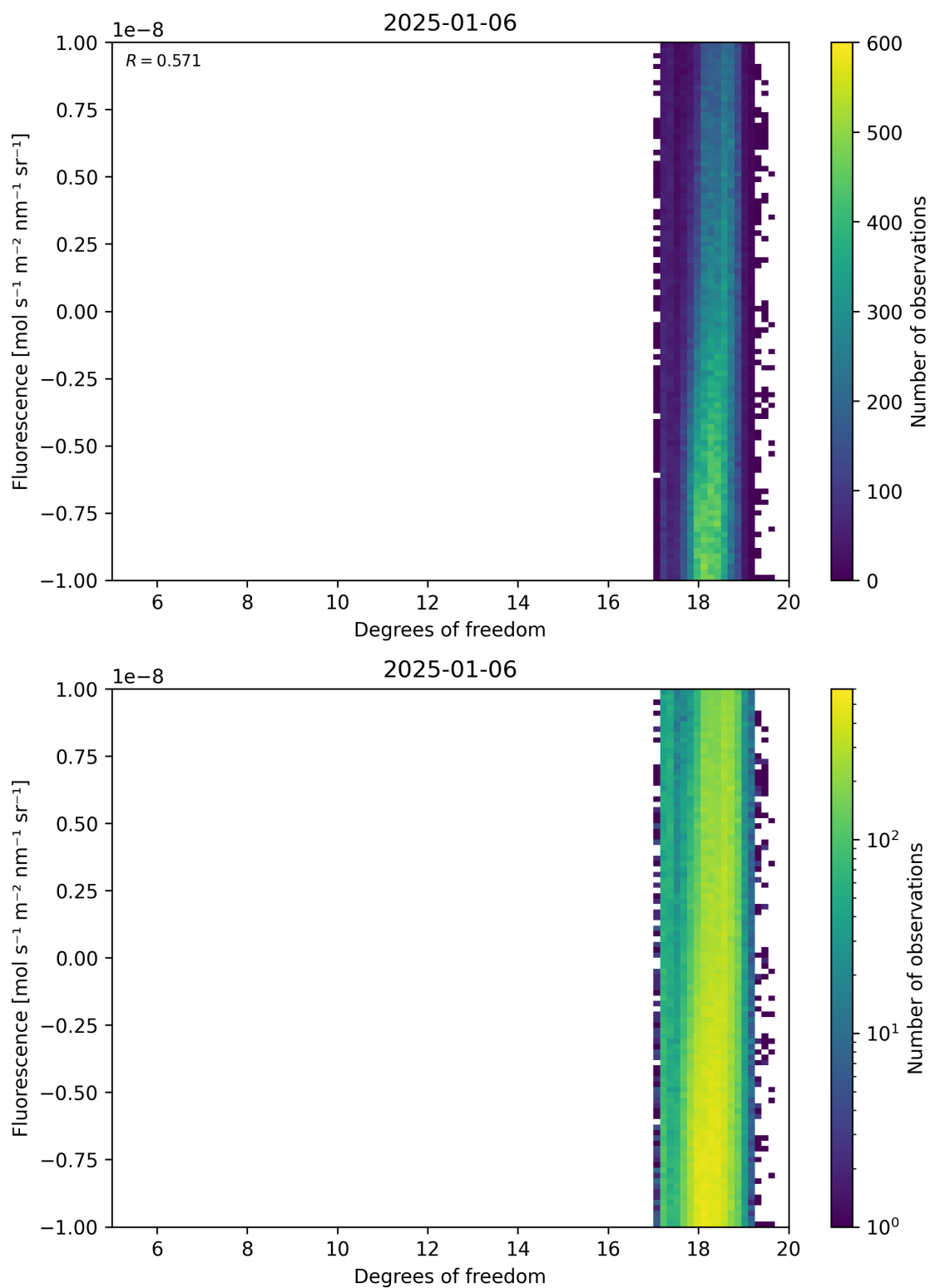
Figure 51: Scatter density plot of “Degrees of freedom” against “Fluorescence” for 2025-01-05 to 2025-01-07.
