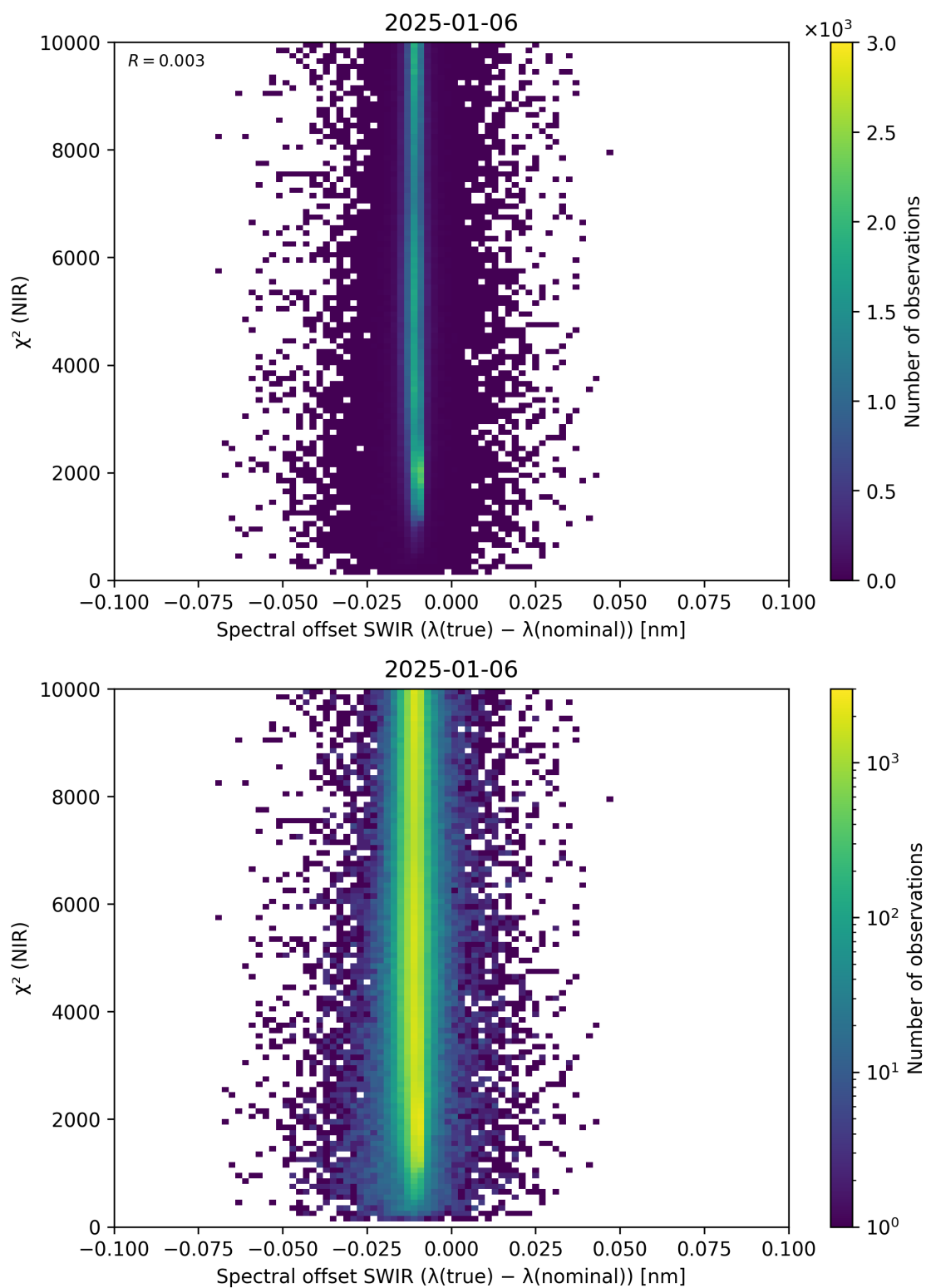
Figure 117: Scatter density plot of “Spectral offset SWIR ( \lambda_{\text{true}} - \lambda_{\text{nominal}} )” against “ \chi^2 (NIR)” for 2025-01-05 to 2025-01-07.
