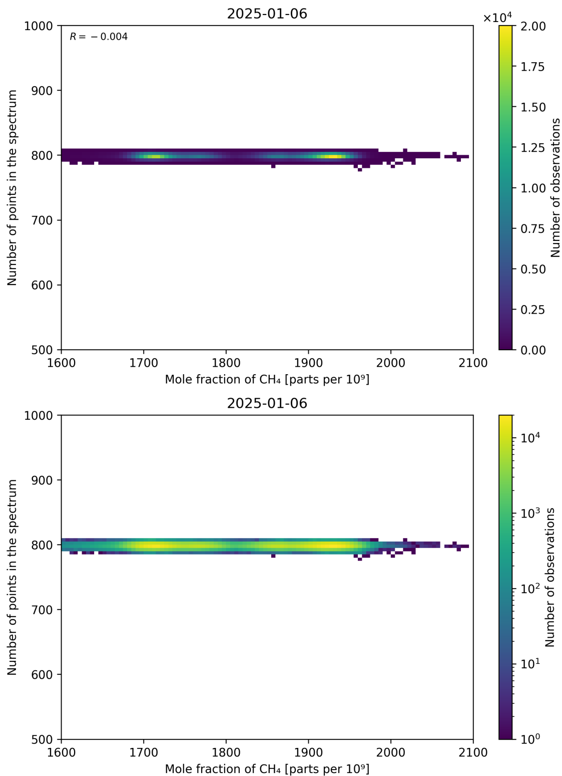
Figure 77: Scatter density plot of “Mole fraction of CH 4 ” against “Number of points in the spectrum” for 2025-01-05 to 2025-01-07.
