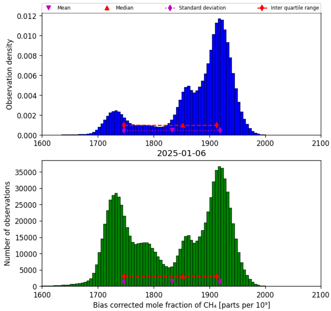
Figure 25: Histogram of “Bias corrected mole fraction of CH 4 ” for 2025-01-05 to 2025-01-07
