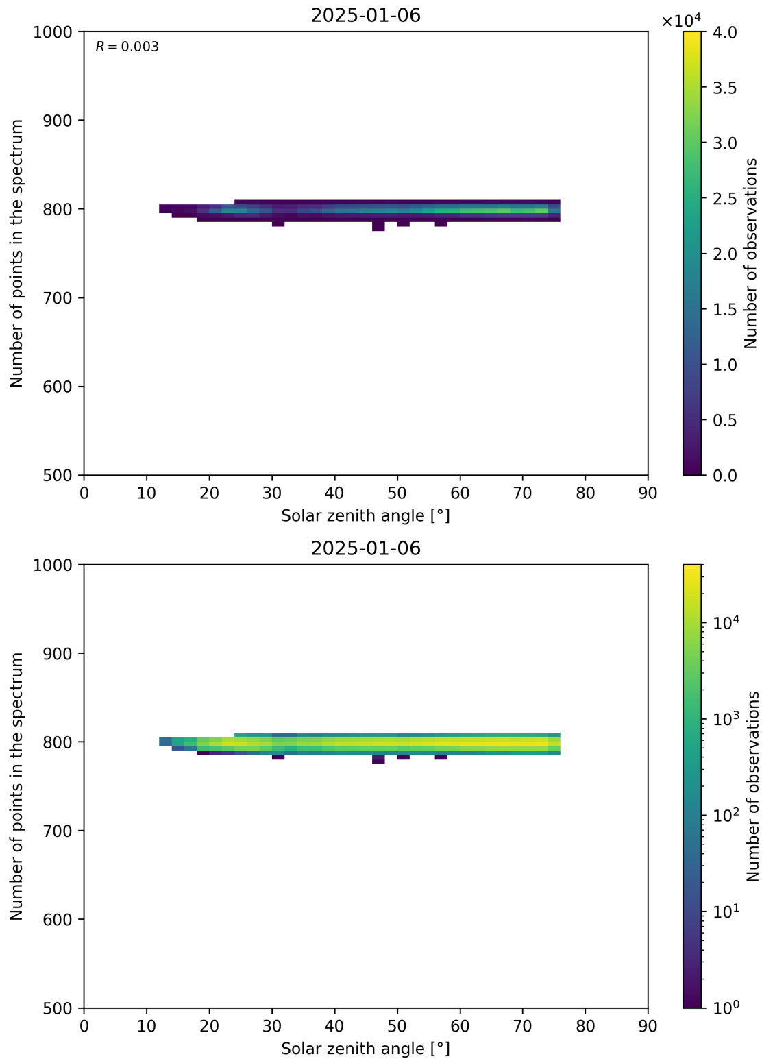
Figure 103: Scatter density plot of “Solar zenith angle” against “Number of points in the spectrum” for 2025-01-05 to 2025-01-07.
