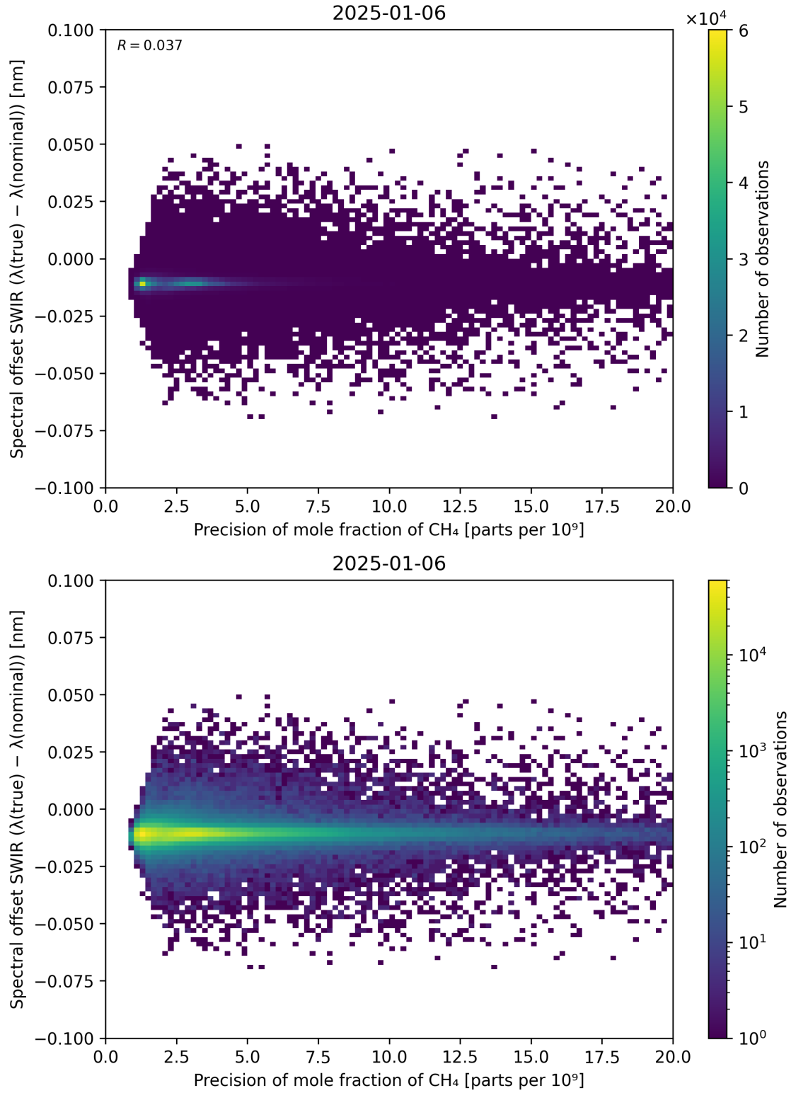
Figure 85: Scatter density plot of “Precision of mole fraction of CH 4 ” against “Spectral offset SWIR ( \lambda_{\text{true}} - \lambda_{\text{nominal}} )” for 2025-01-05 to 2025-01-07.
