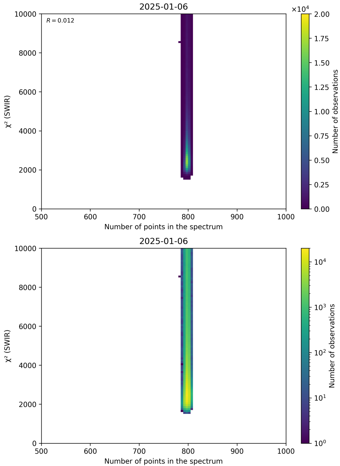
Figure 89: Scatter density plot of “Number of points in the spectrum” against “ \chi^2 (SWIR)” for 2025-01-05 to 2025-01-07.
