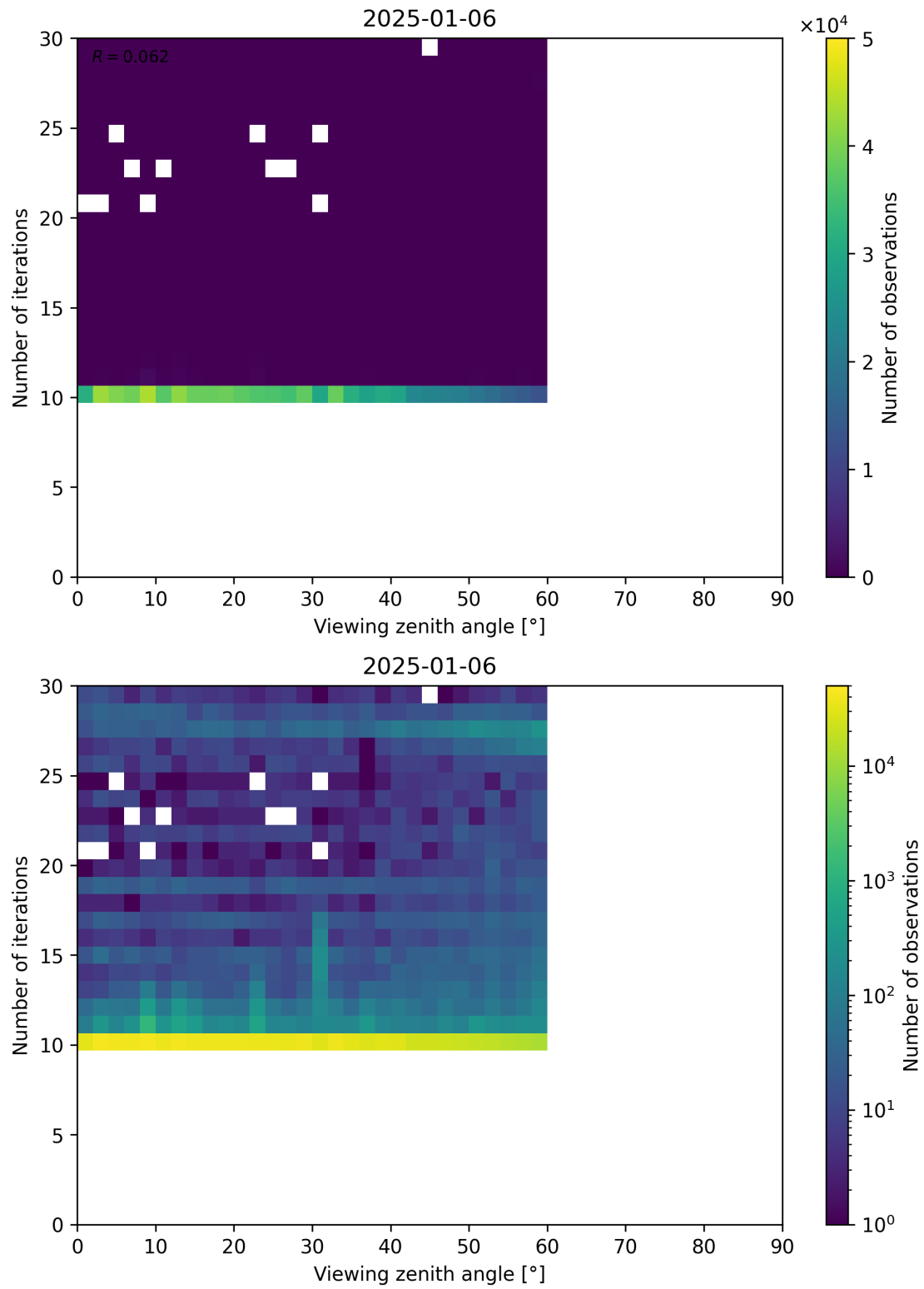
Figure 113: Scatter density plot of “Viewing zenith angle” against “Number of iterations” for 2025-01-05 to 2025-01-07.
