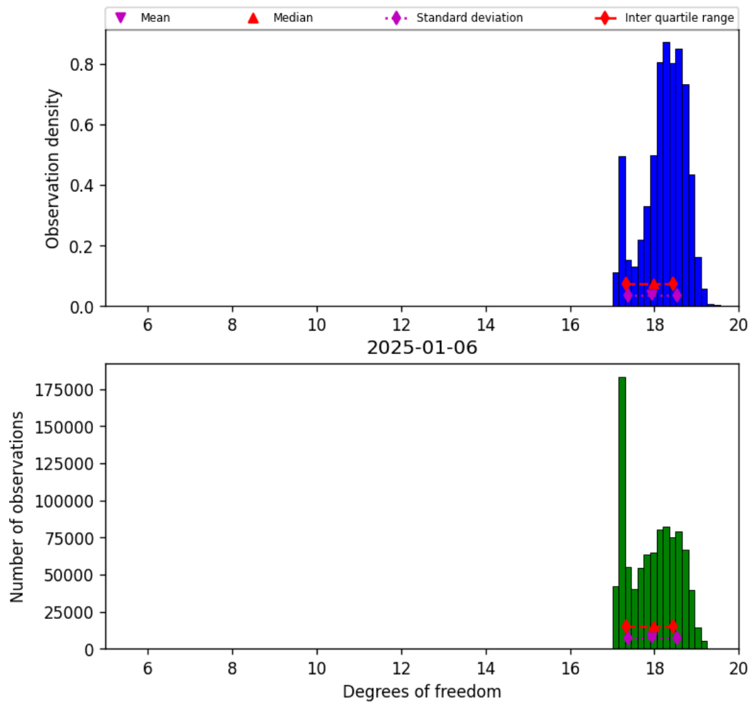
Figure 30: Histogram of “Degrees of freedom” for 2025-01-05 to 2025-01-07
