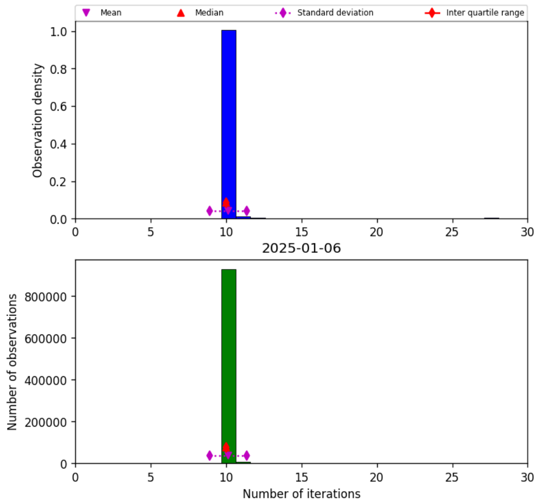
Figure 31: Histogram of “Number of iterations” for 2025-01-05 to 2025-01-07
