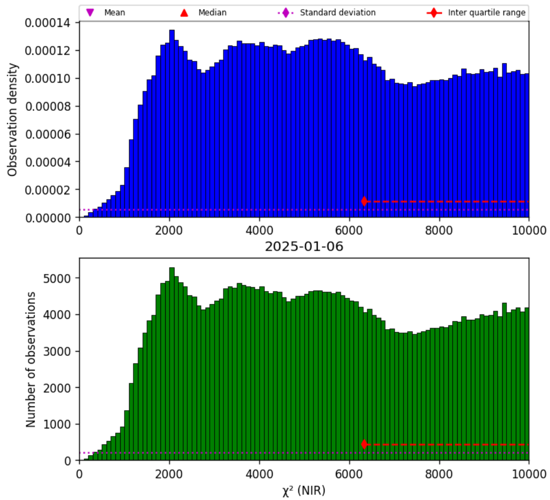
Figure 29: Histogram of “ \chi^2 (NIR)” for 2025-01-05 to 2025-01-07
