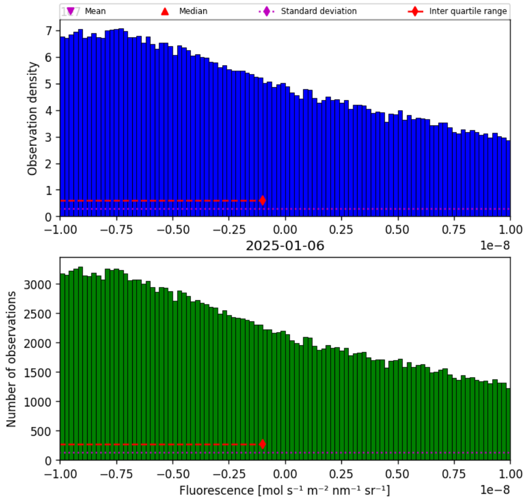
Figure 32: Histogram of “Fluorescence” for 2025-01-05 to 2025-01-07
