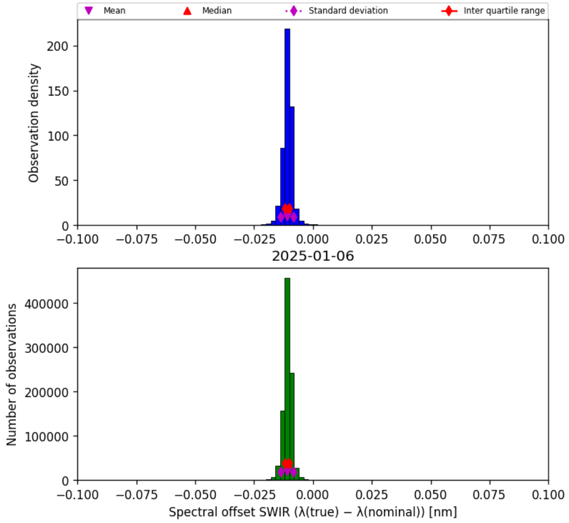
Figure 27: Histogram of “Spectral offset SWIR ( \lambda_{\text{true}} - \lambda_{\text{nominal}} )” for 2025-01-05 to 2025-01-07
