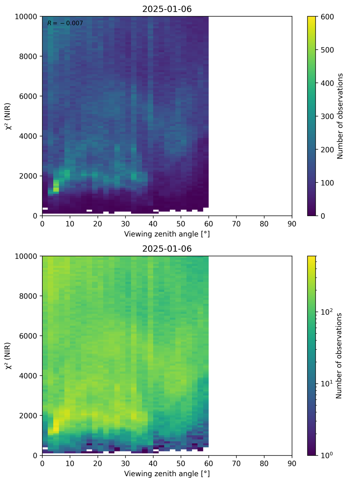
Figure 105: Scatter density plot of “Viewing zenith angle” against “ \chi^2 (NIR)” for 2025-01-05 to 2025-01-07.
