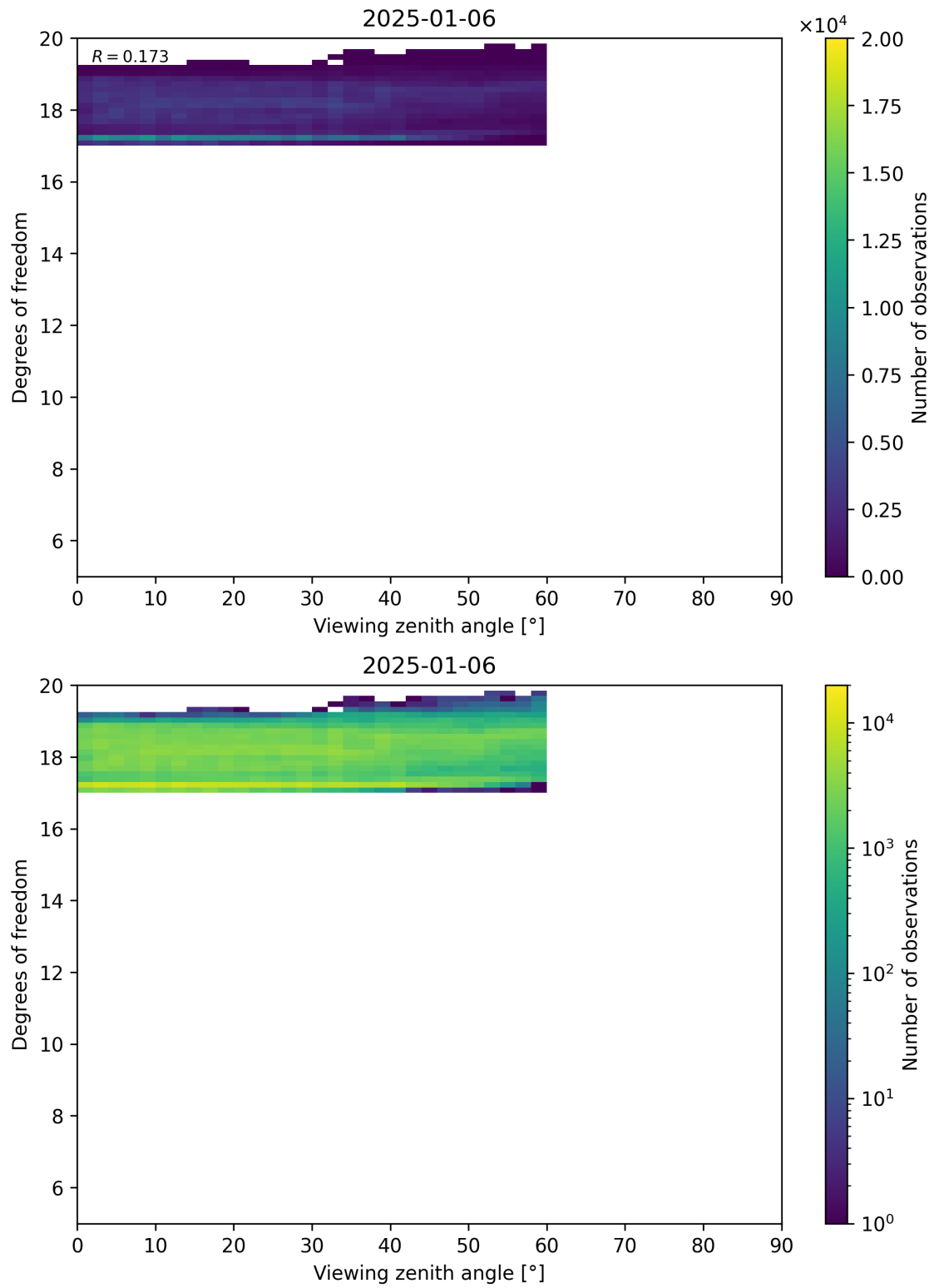
Figure 107: Scatter density plot of “Viewing zenith angle” against “Degrees of freedom” for 2025-01-05 to 2025-01-07.
