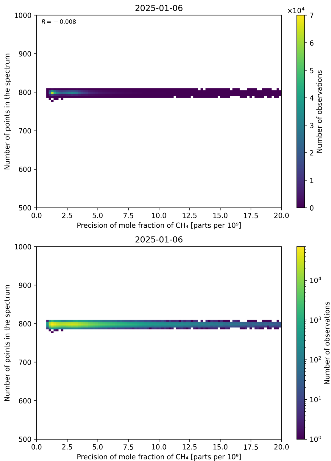
Figure 84: Scatter density plot of “Precision of mole fraction of CH 4 ” against “Number of points in the spectrum” for 2025-01-05 to 2025-01-07.
