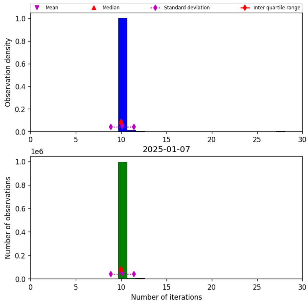
Figure 31: Histogram of “Number of iterations” for 2025-01-07 to 2025-01-08
