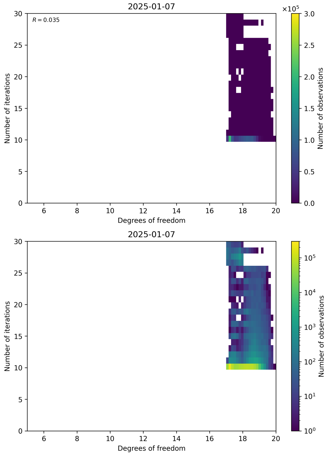
Figure 52: Scatter density plot of “Degrees of freedom” against “Number of iterations” for 2025-01-07 to 2025-01-08.
