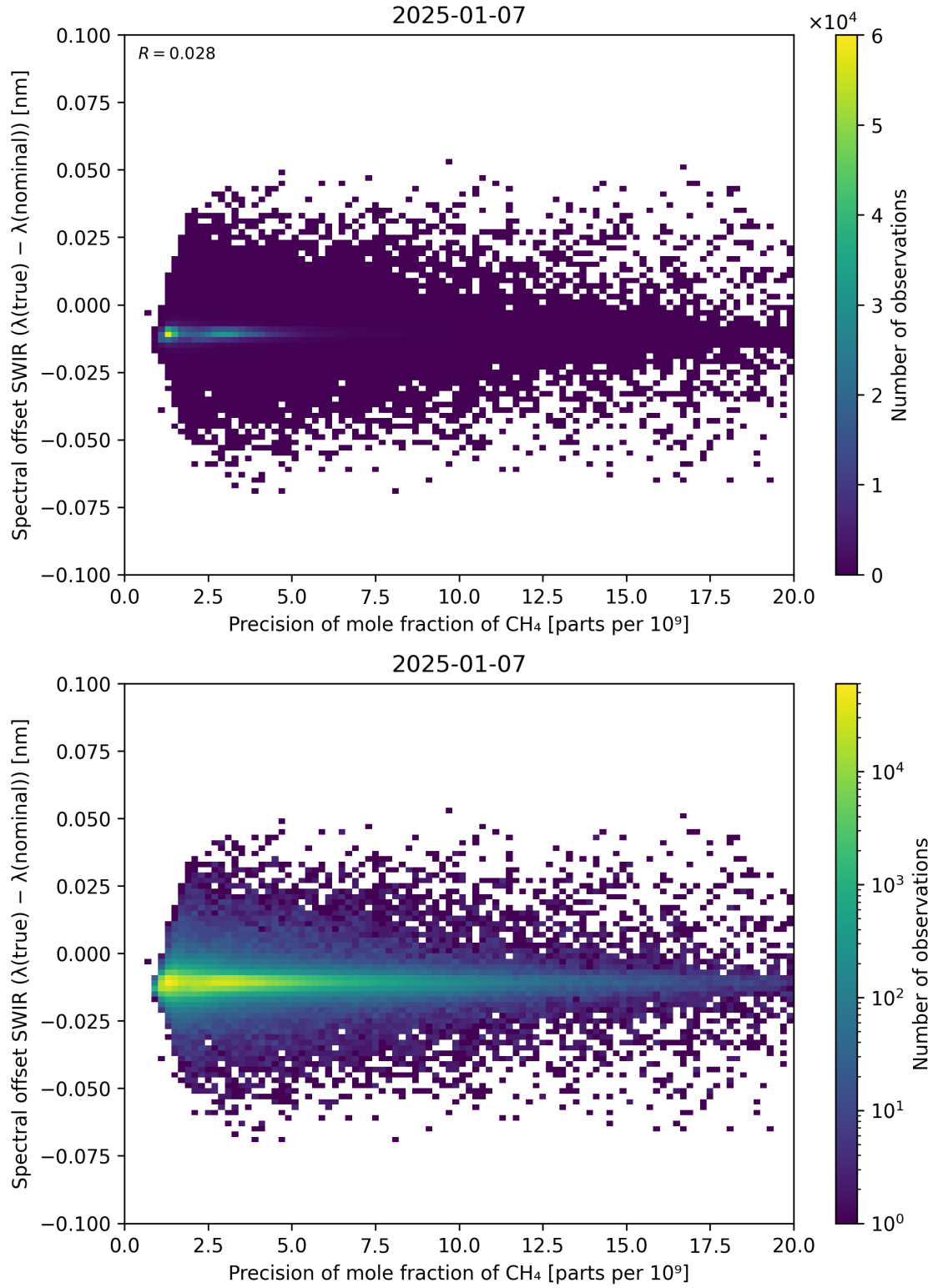
Figure 85: Scatter density plot of “Precision of mole fraction of \text{CH}_4 ” against “Spectral offset SWIR ( \lambda_{\text{true}} - \lambda_{\text{nominal}} )” for 2025-01-07 to 2025-01-08.
