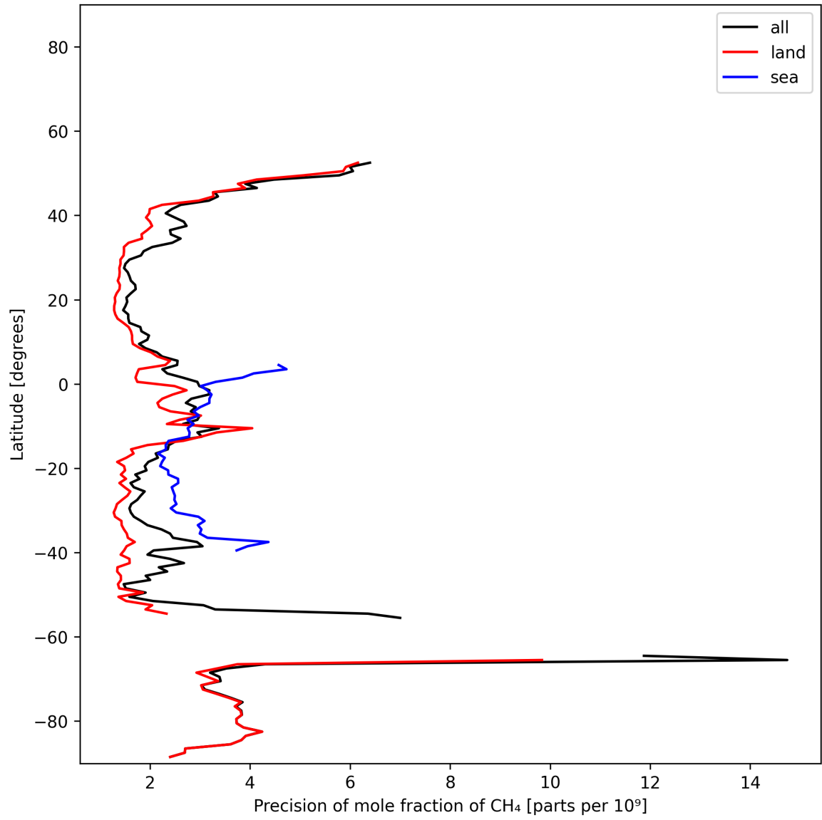
Figure 13: Zonal average of “Precision of mole fraction of CH 4 ” for 2025-01-07 to 2025-01-08.
