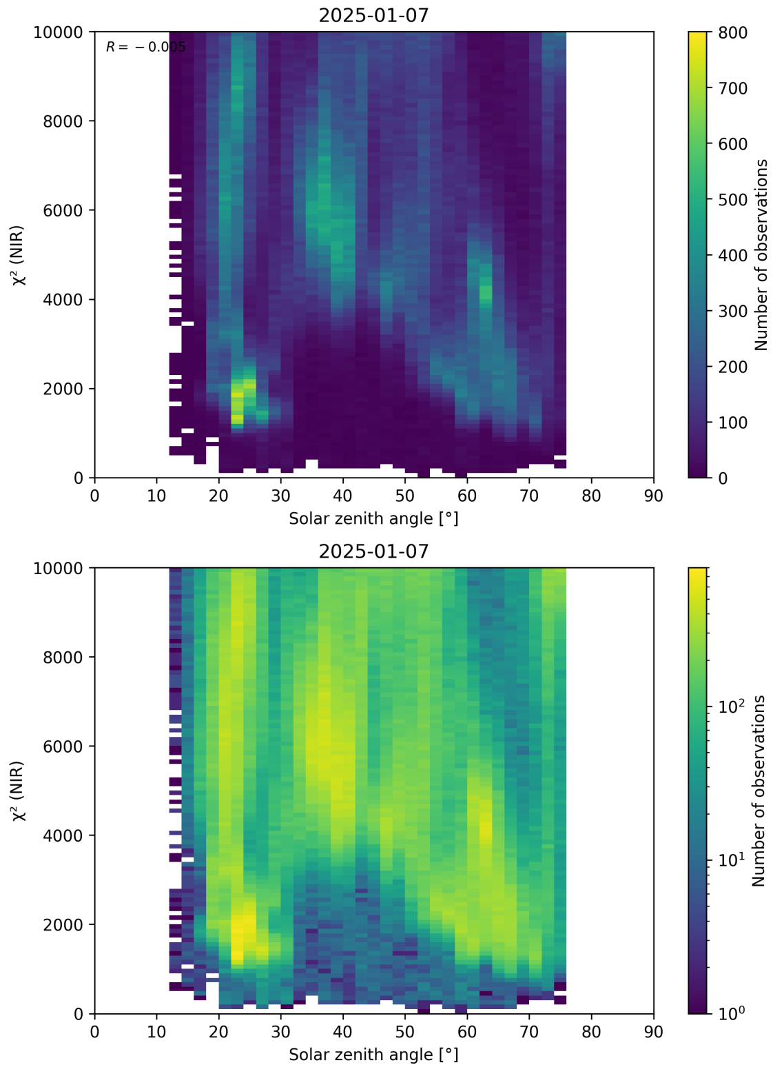
Figure 94: Scatter density plot of “Solar zenith angle” against “ \chi^2 (NIR)” for 2025-01-07 to 2025-01-08.
