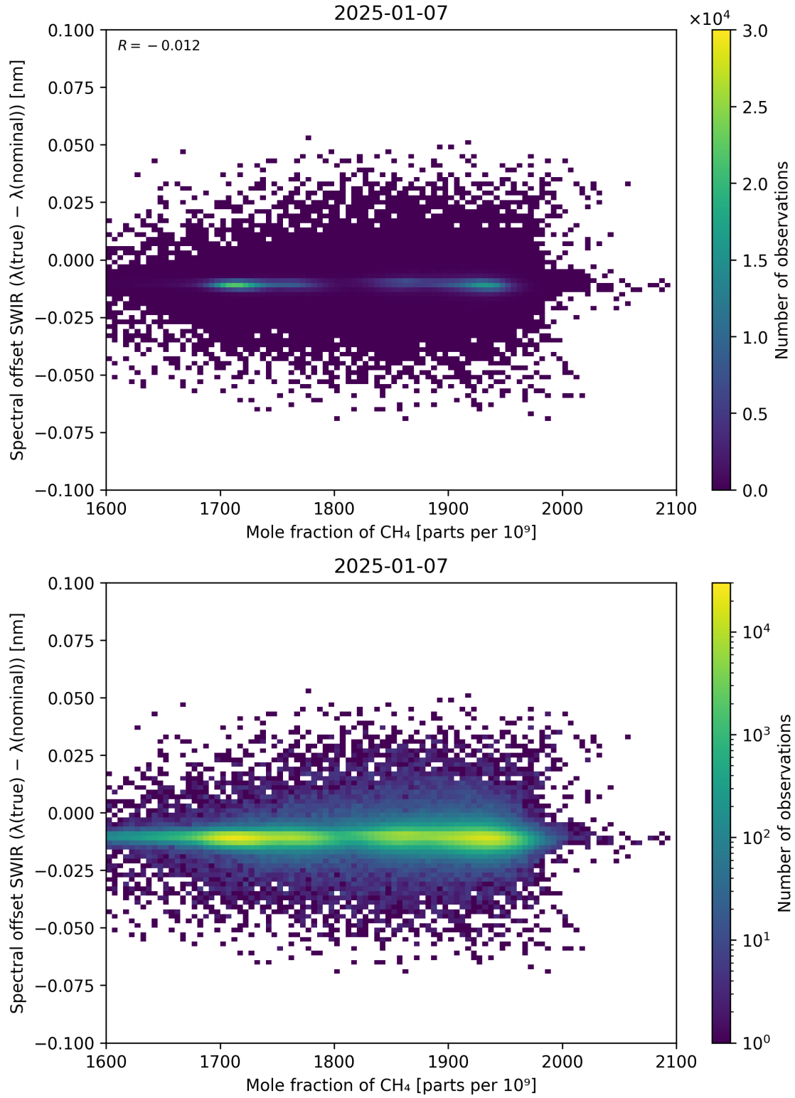
Figure 86: Scatter density plot of “Mole fraction of \text{CH}_4 ” against “Spectral offset SWIR ( \lambda_{\text{true}} - \lambda_{\text{nominal}} )” for 2025-01-07 to 2025-01-08.
