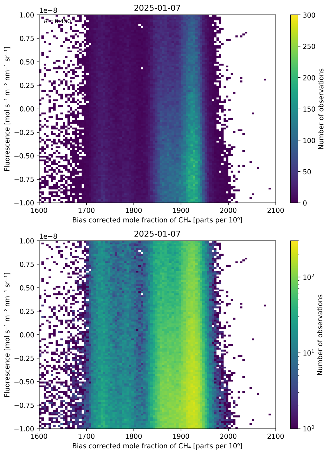
Figure 66: Scatter density plot of “Bias corrected mole fraction of \text{CH}_4 ” against “Fluorescence” for 2025-01-07 to 2025-01-08.
