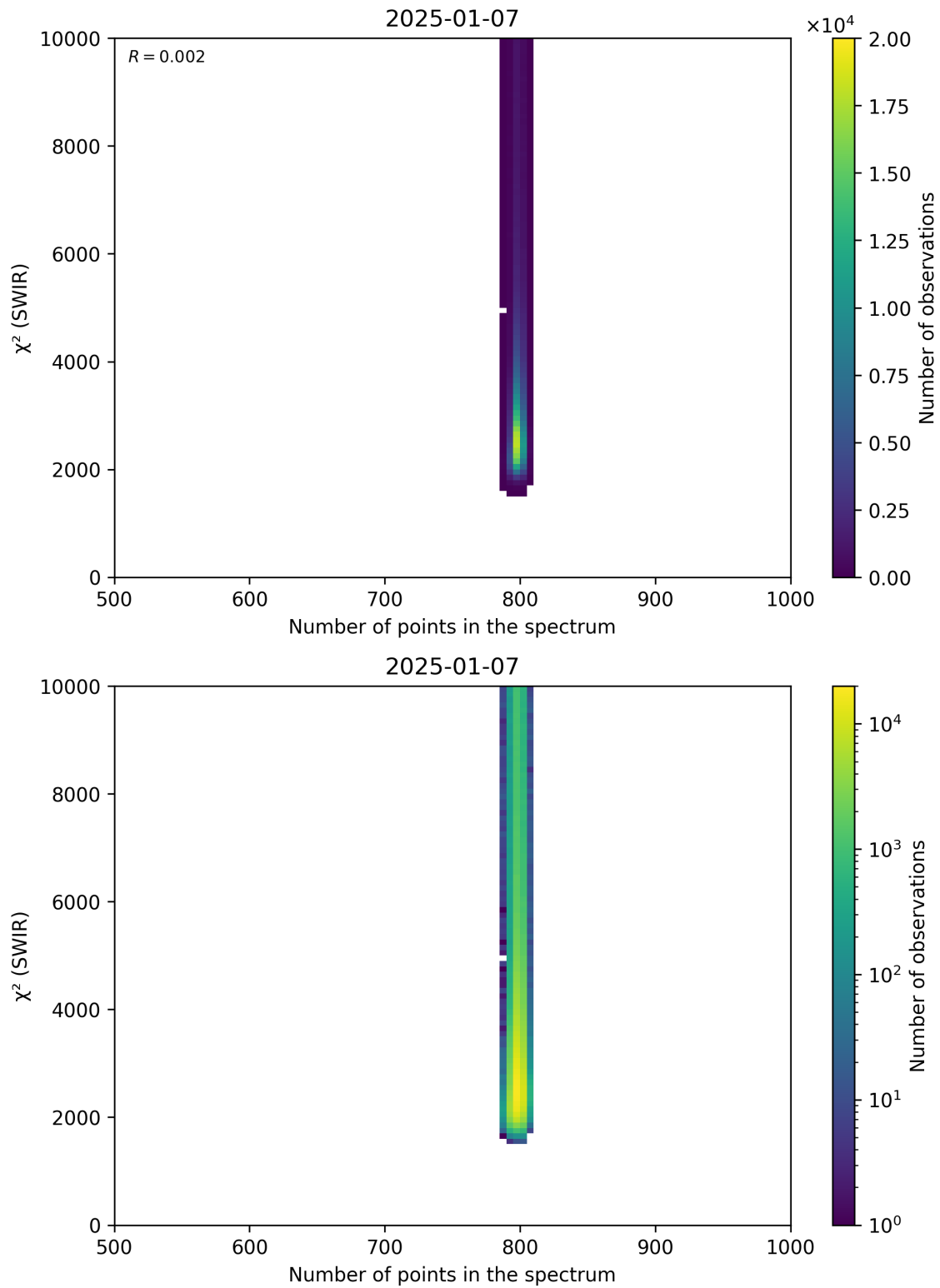
Figure 89: Scatter density plot of “Number of points in the spectrum” against “ \chi^2 (SWIR)” for 2025-01-07 to 2025-01-08.
