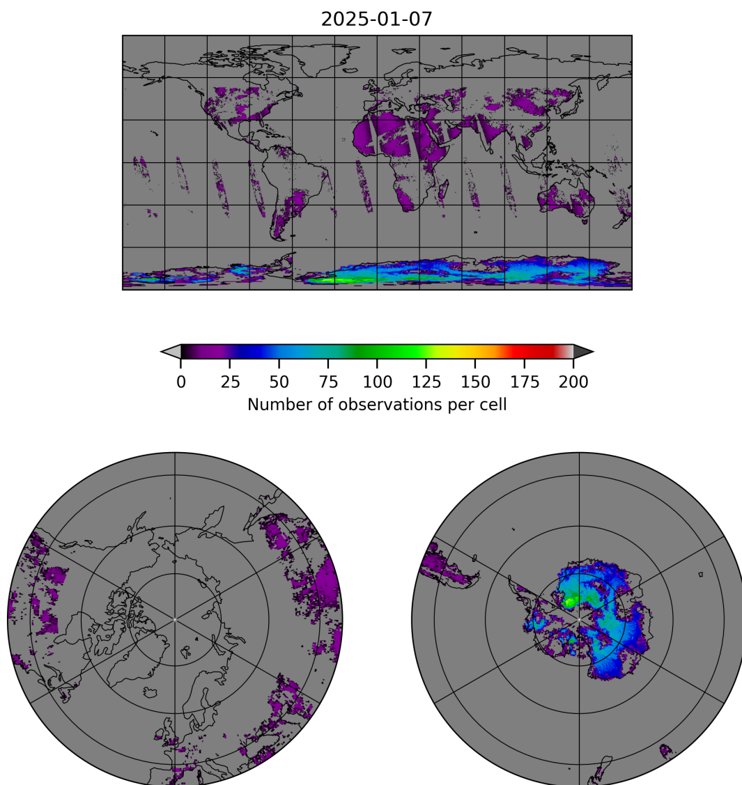
Figure 10: Map of the number of observations for 2025-01-07 to 2025-01-08
