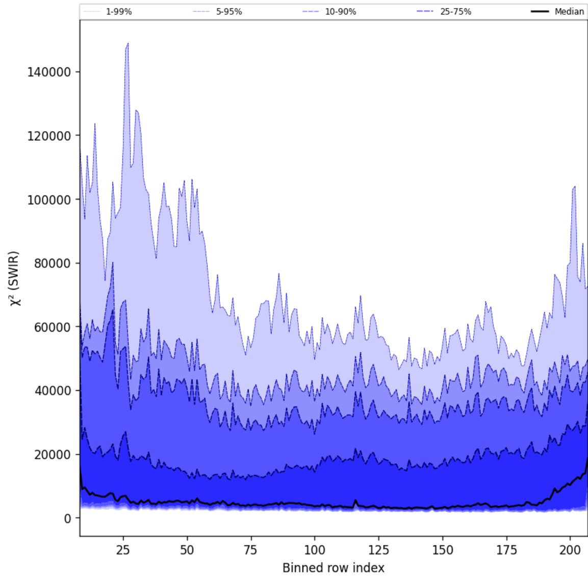
Figure 39: Along track statistics of “ \chi^2 (SWIR)” for 2025-01-07 to 2025-01-08
