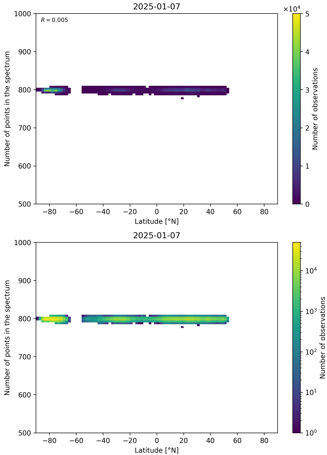
Figure 61: Scatter density plot of “Latitude” against “Number of points in the spectrum” for 2025-01-07 to 2025-01-08.
