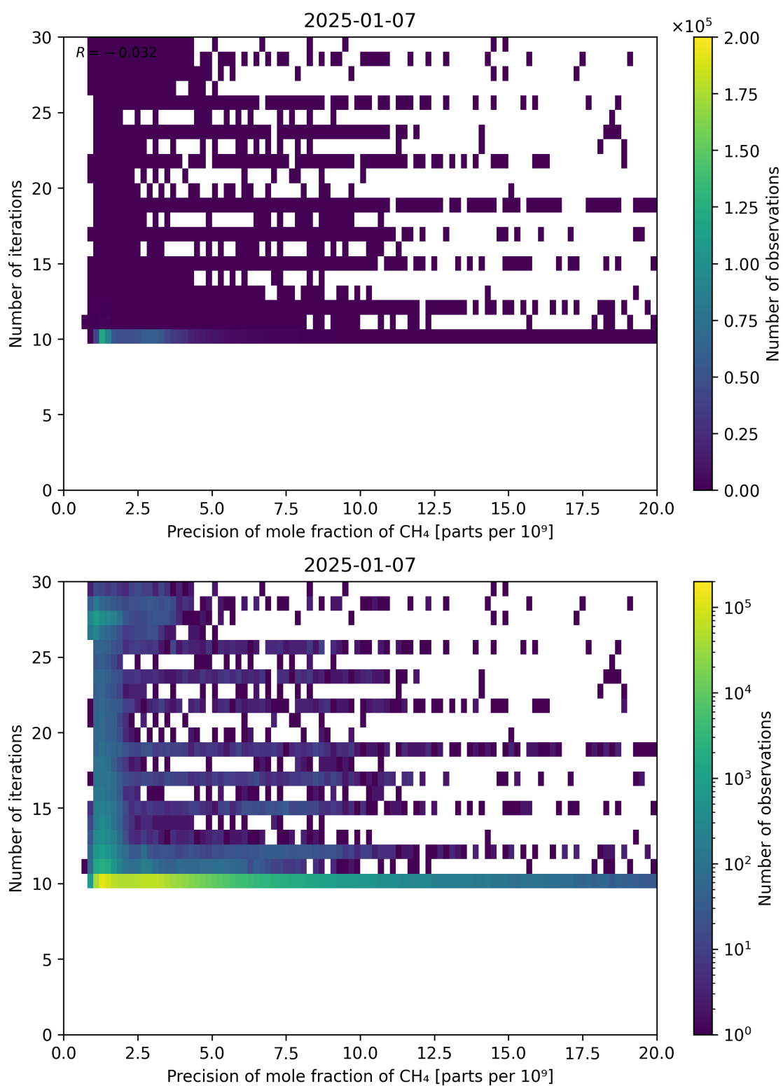
Figure 83: Scatter density plot of “Precision of mole fraction of CH 4 ” against “Number of iterations” for 2025-01-07 to 2025-01-08.
