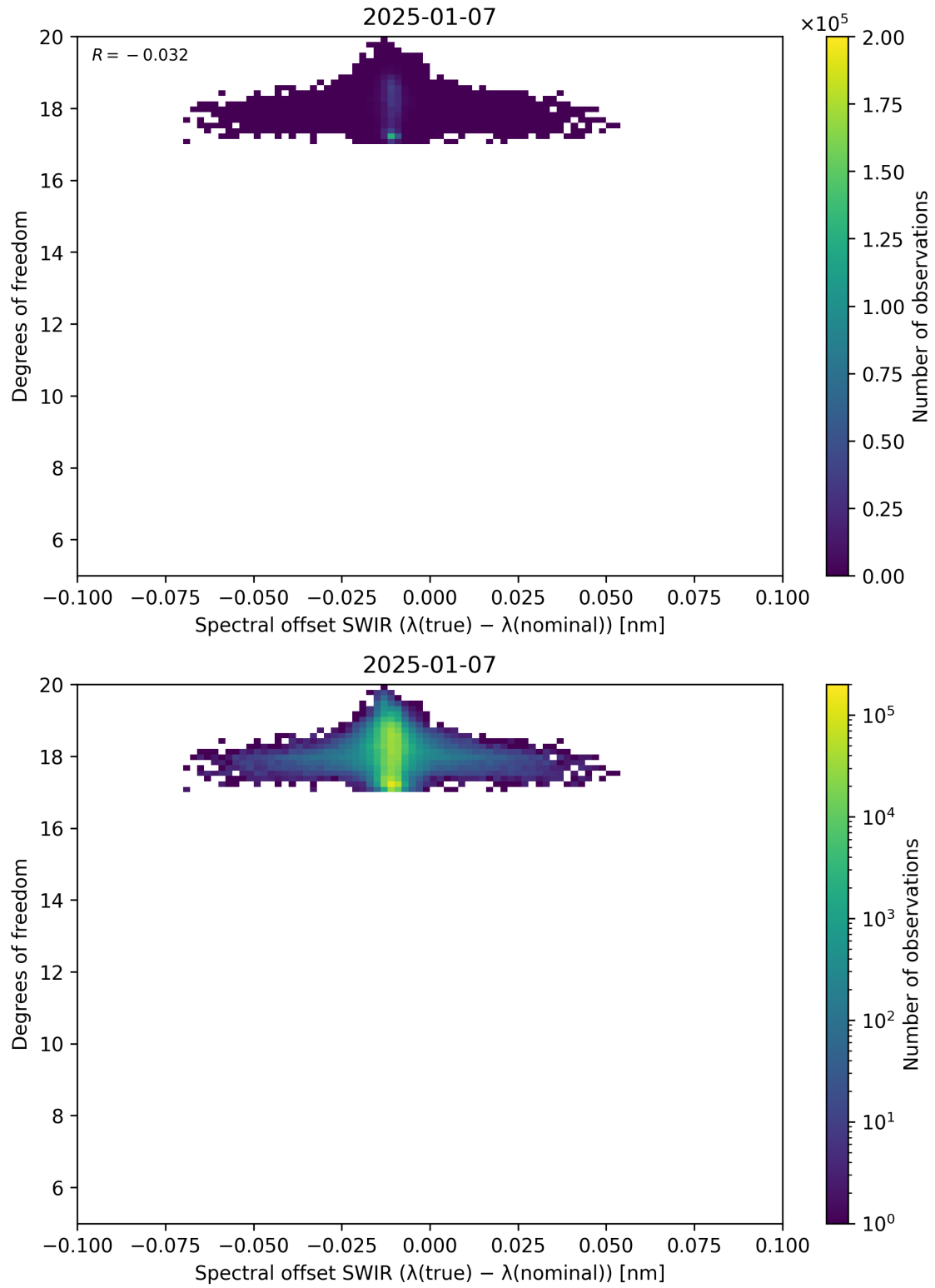
Figure 119: Scatter density plot of “Spectral offset SWIR ( \lambda_{\text{true}} - \lambda_{\text{nominal}} )” against “Degrees of freedom” for 2025-01-07 to 2025-01-08.
