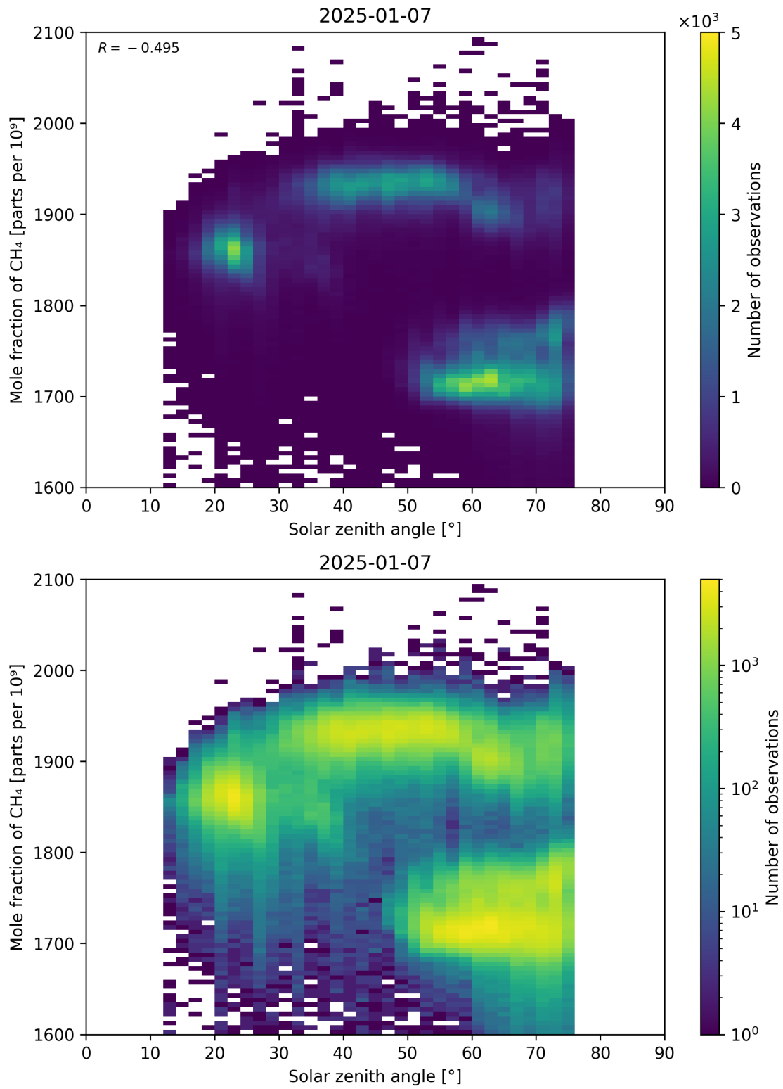
Figure 99: Scatter density plot of “Solar zenith angle” against “Mole fraction of CH 4 ” for 2025-01-07 to 2025-01-08.
