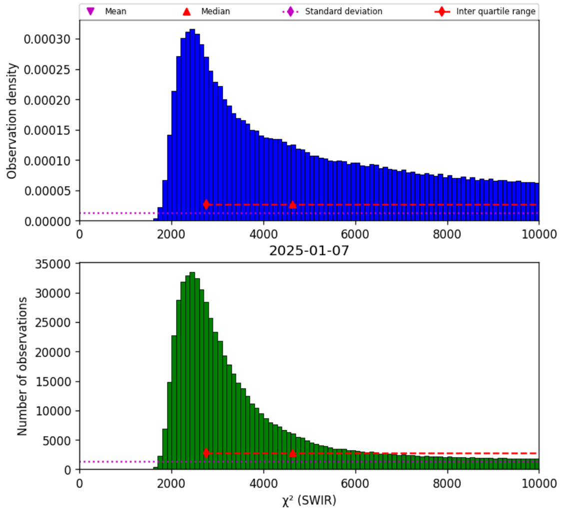
Figure 28: Histogram of “ \chi^2 (SWIR)” for 2025-01-07 to 2025-01-08
