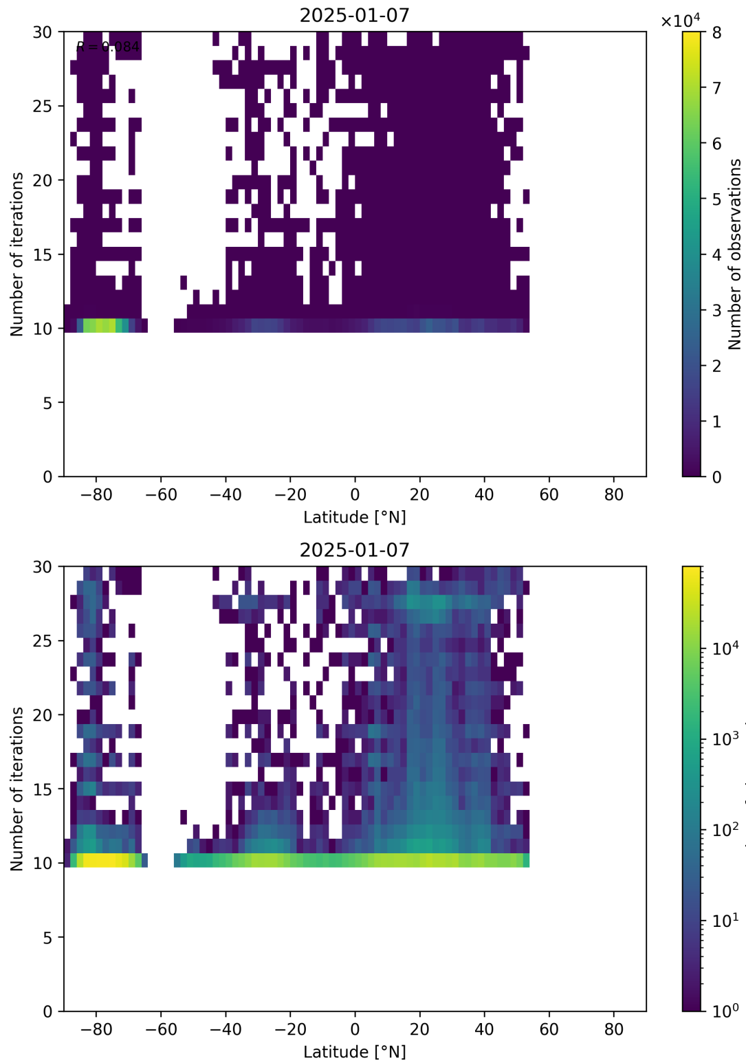
Figure 60: Scatter density plot of “Latitude” against “Number of iterations” for 2025-01-07 to 2025-01-08.
