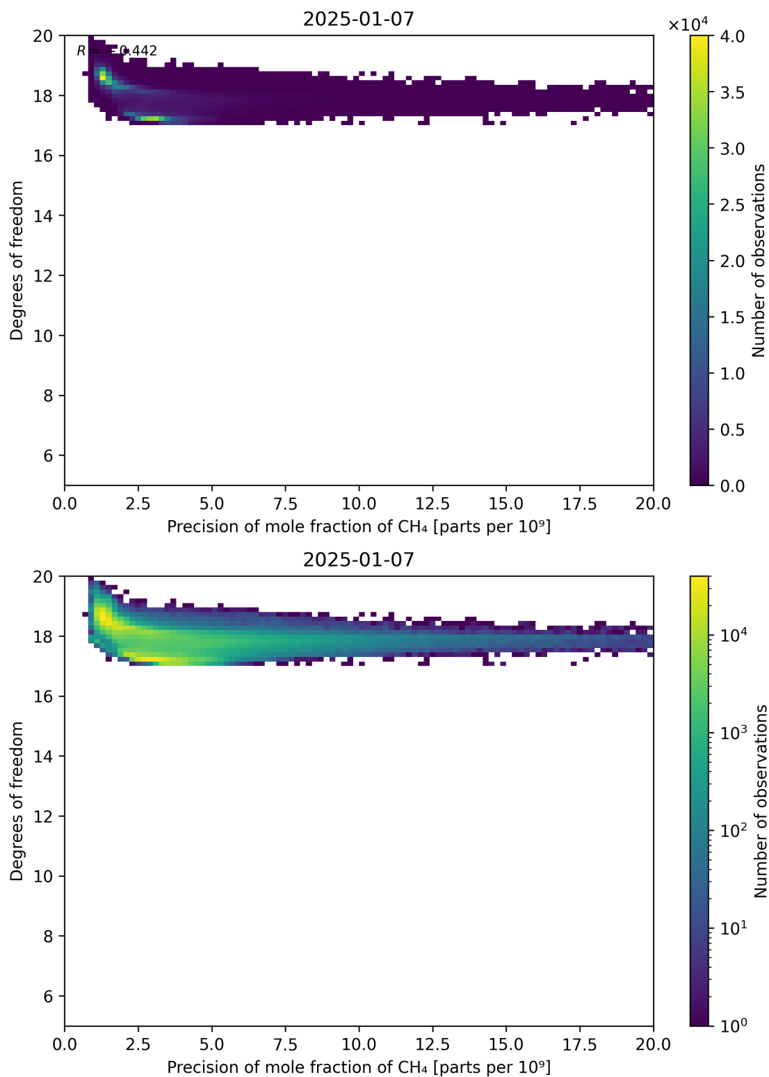
Figure 80: Scatter density plot of “Precision of mole fraction of CH 4 ” against “Degrees of freedom” for 2025-01-07 to 2025-01-08.
