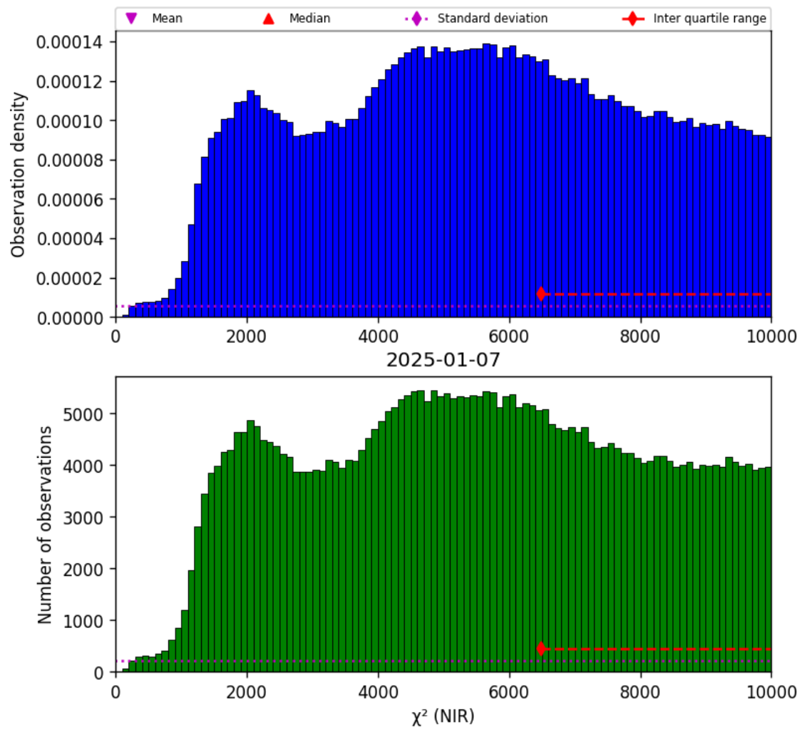
Figure 29: Histogram of “ \chi^2 (NIR)” for 2025-01-07 to 2025-01-08
