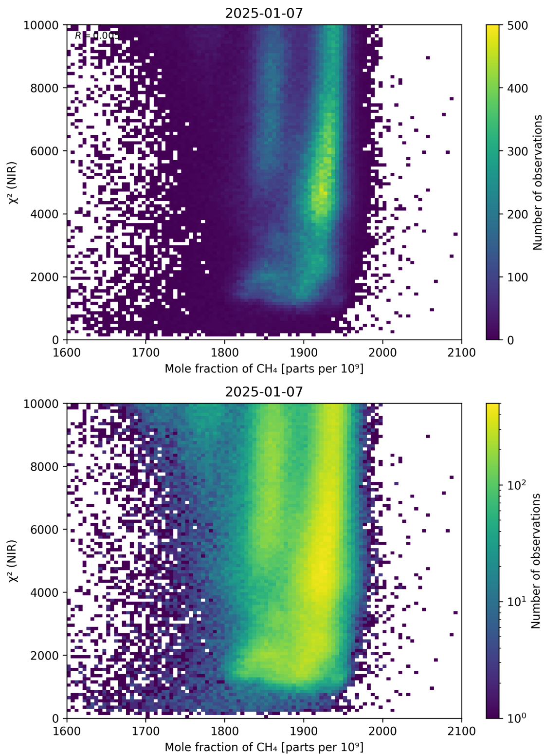
Figure 70: Scatter density plot of “Mole fraction of \text{CH}_4 ” against “ \chi^2 (NIR)” for 2025-01-07 to 2025-01-08.
