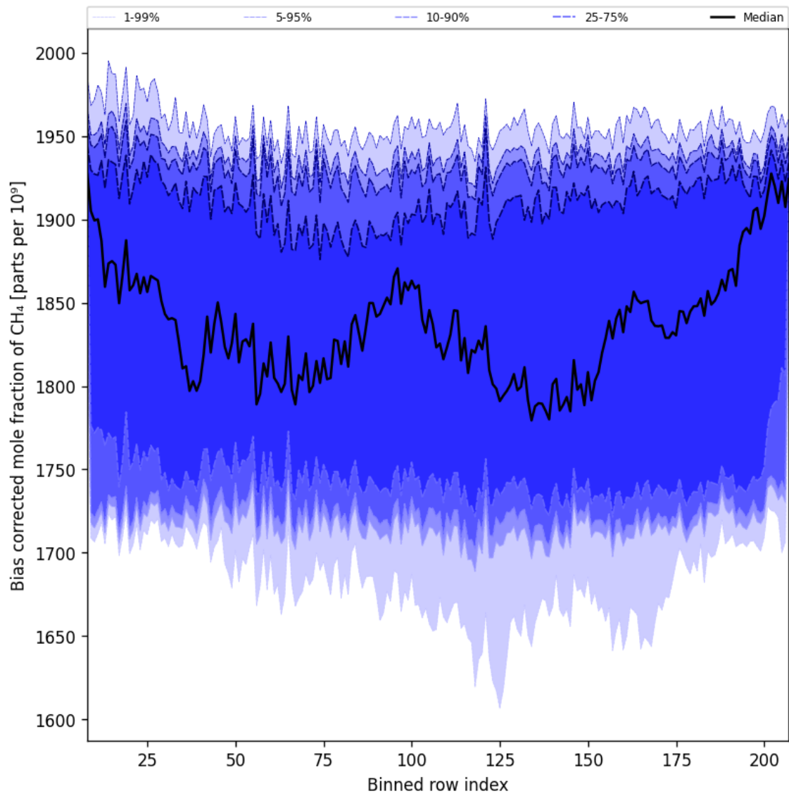
Figure 36: Along track statistics of “Bias corrected mole fraction of CH 4 ” for 2025-01-07 to 2025-01-08
