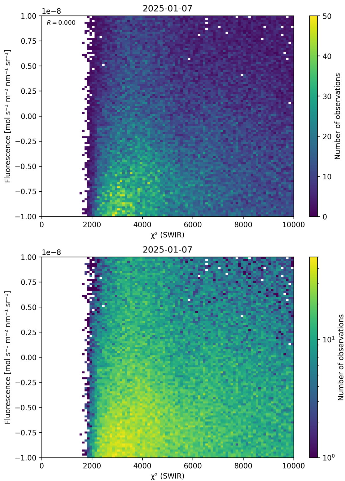
Figure 49: Scatter density plot of “ \chi^2 (SWIR)” against “Fluorescence” for 2025-01-07 to 2025-01-08.
