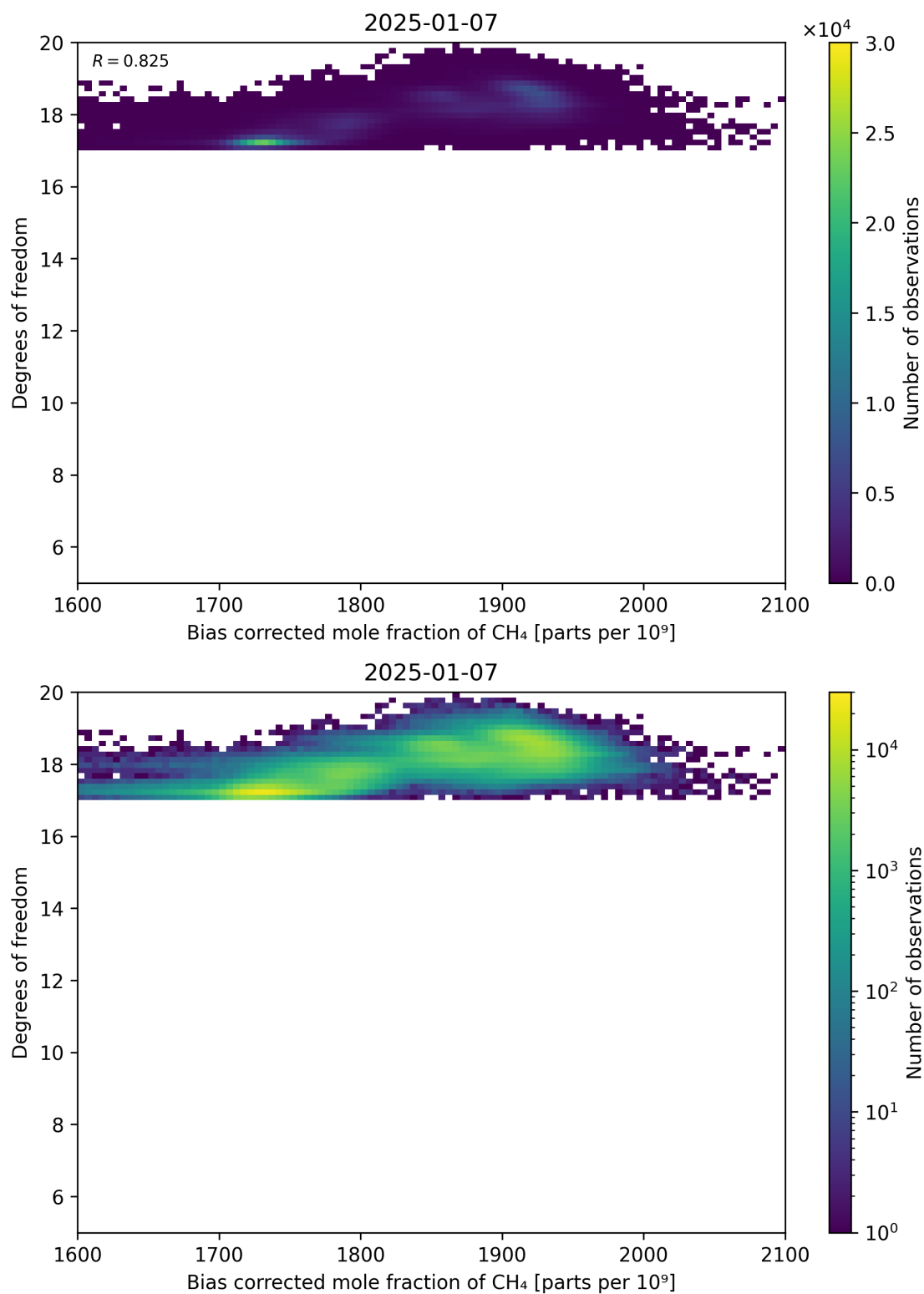
Figure 65: Scatter density plot of “Bias corrected mole fraction of CH 4 ” against “Degrees of freedom” for 2025-01-07 to 2025-01-08.
