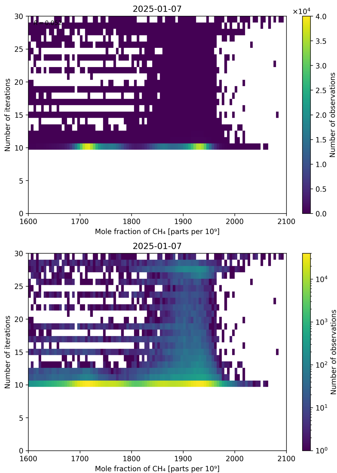
Figure 76: Scatter density plot of “Mole fraction of CH 4 ” against “Number of iterations” for 2025-01-07 to 2025-01-08.
