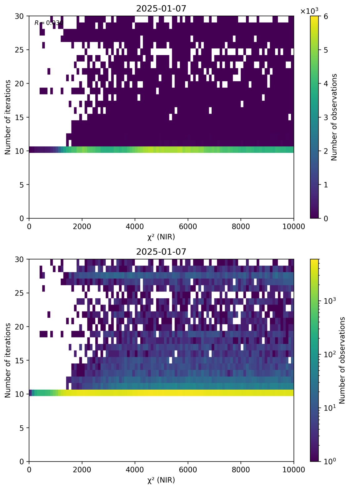
Figure 46: Scatter density plot of “ \chi^2 (NIR)” against “Number of iterations” for 2025-01-07 to 2025-01-08.
