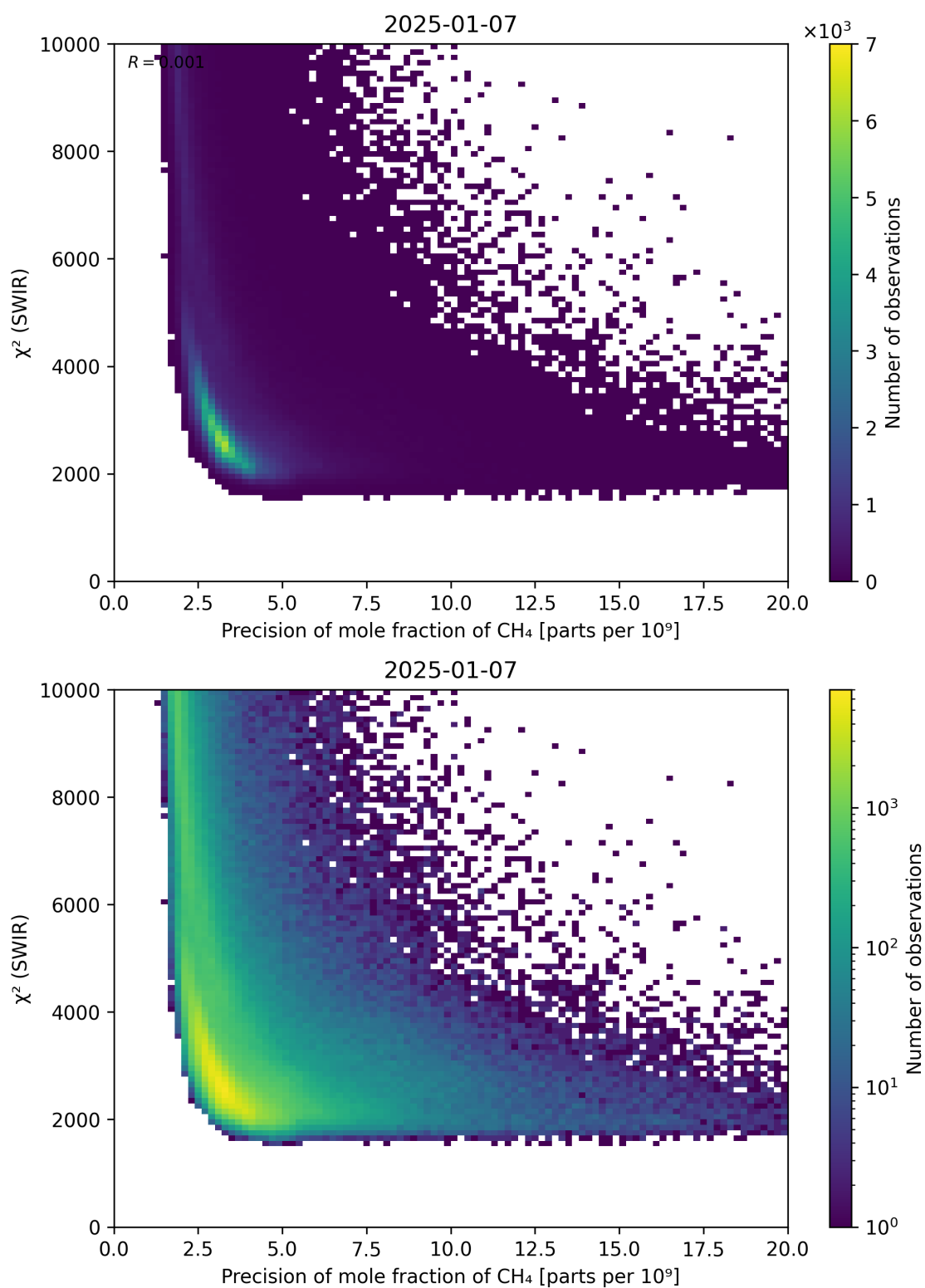
Figure 79: Scatter density plot of “Precision of mole fraction of CH 4 ” against “ \chi^2 (SWIR)” for 2025-01-07 to 2025-01-08.
