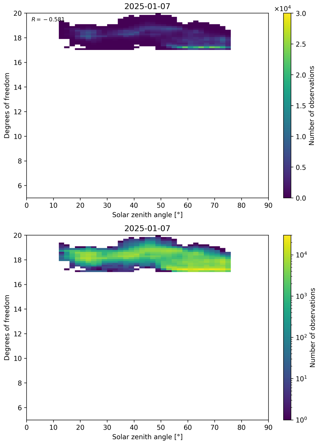
Figure 96: Scatter density plot of “Solar zenith angle” against “Degrees of freedom” for 2025-01-07 to 2025-01-08.
