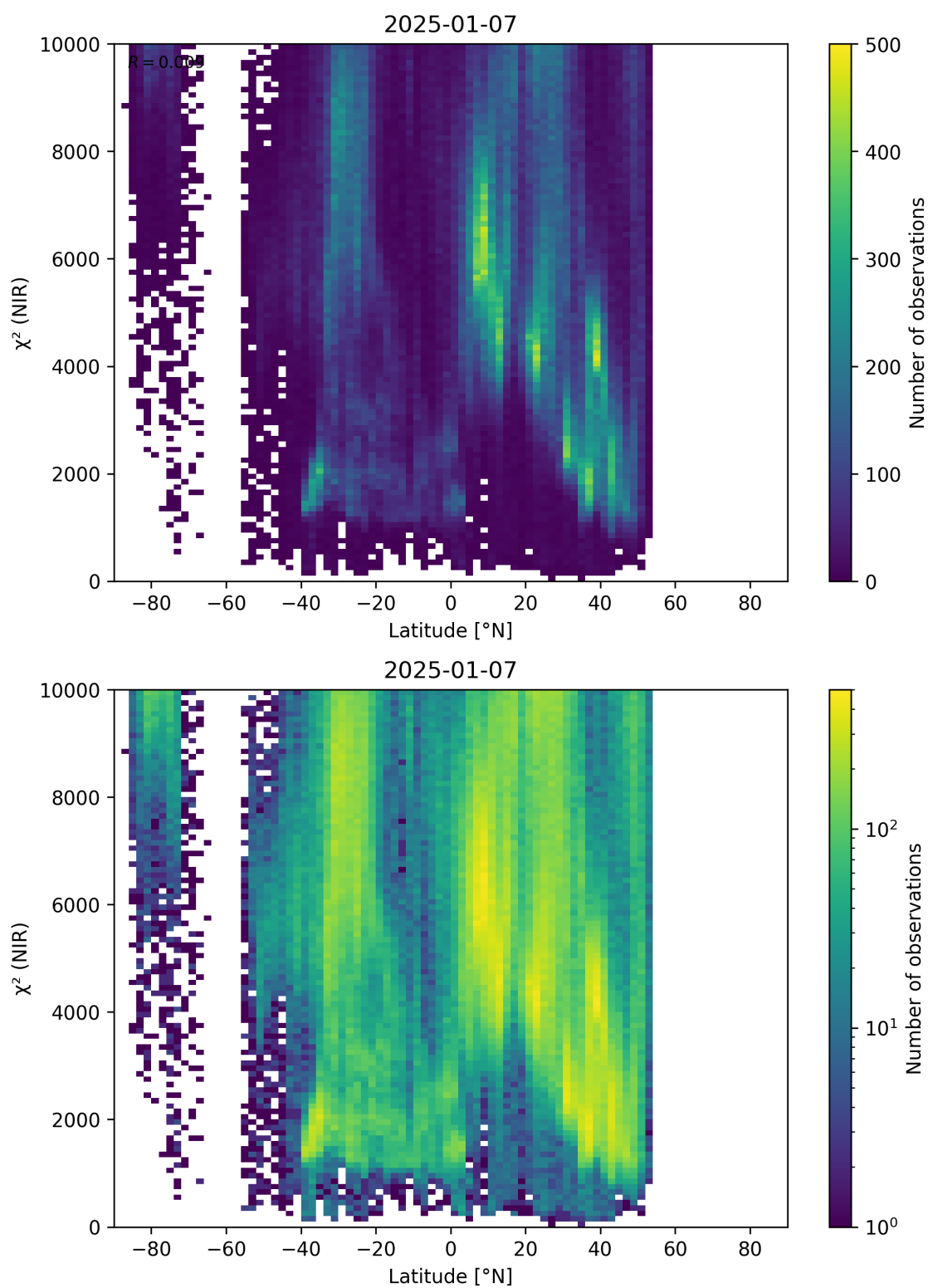
Figure 53: Scatter density plot of “Latitude” against “ \chi^2 (NIR)” for 2025-01-07 to 2025-01-08.
