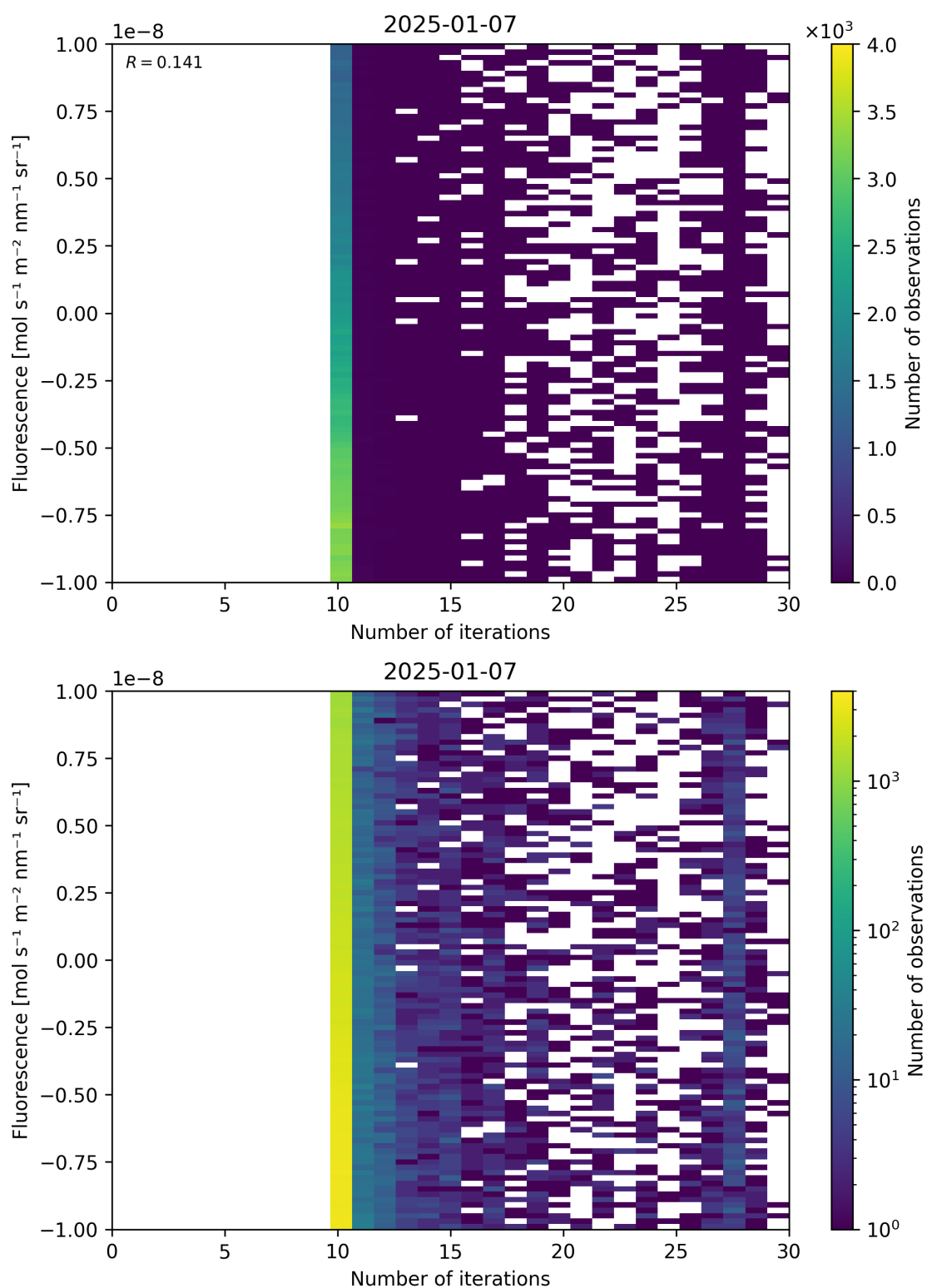
Figure 87: Scatter density plot of “Number of iterations” against “Fluorescence” for 2025-01-07 to 2025-01-08.
