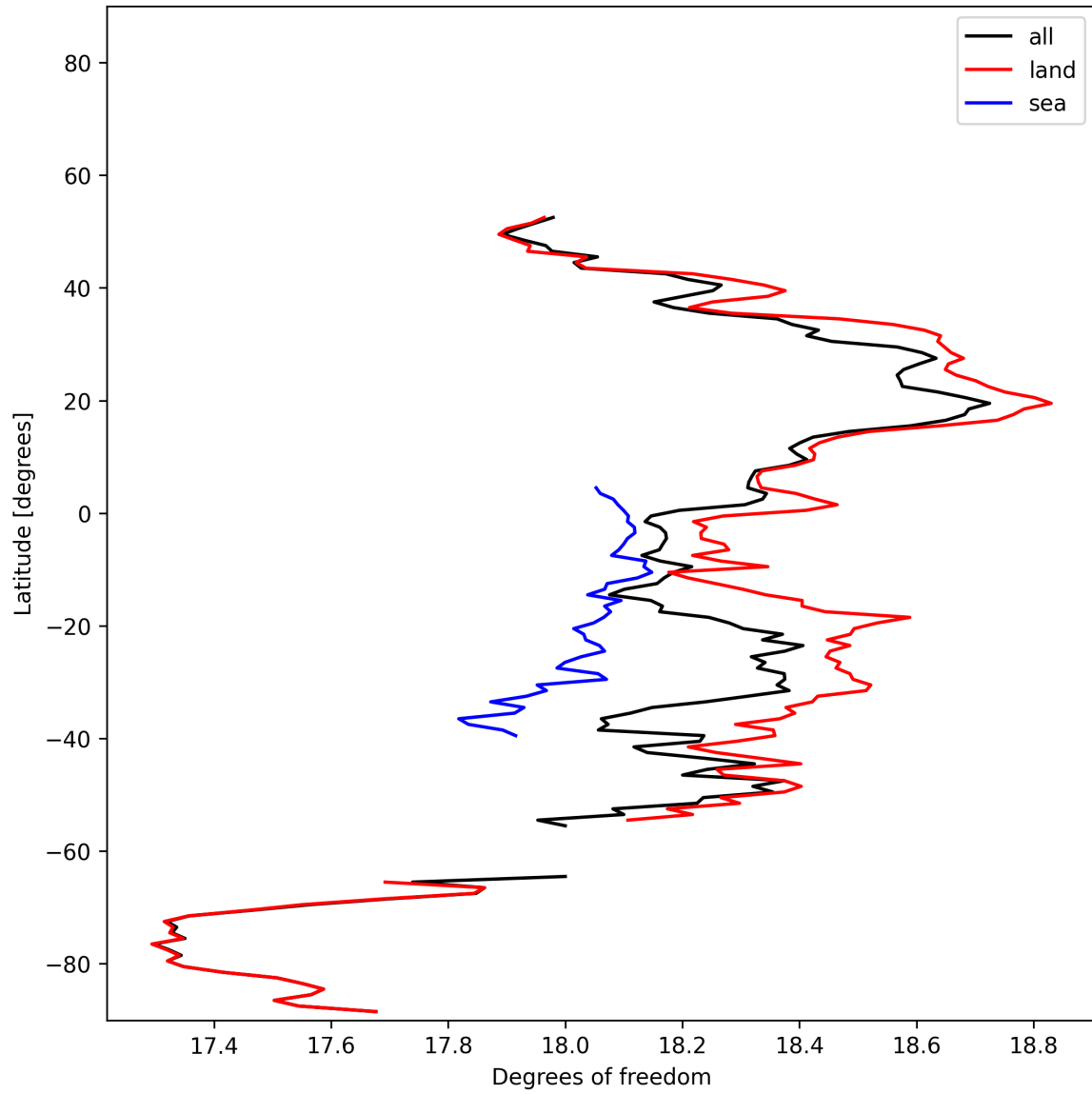
Figure 19: Zonal average of “Degrees of freedom” for 2025-01-07 to 2025-01-08.
