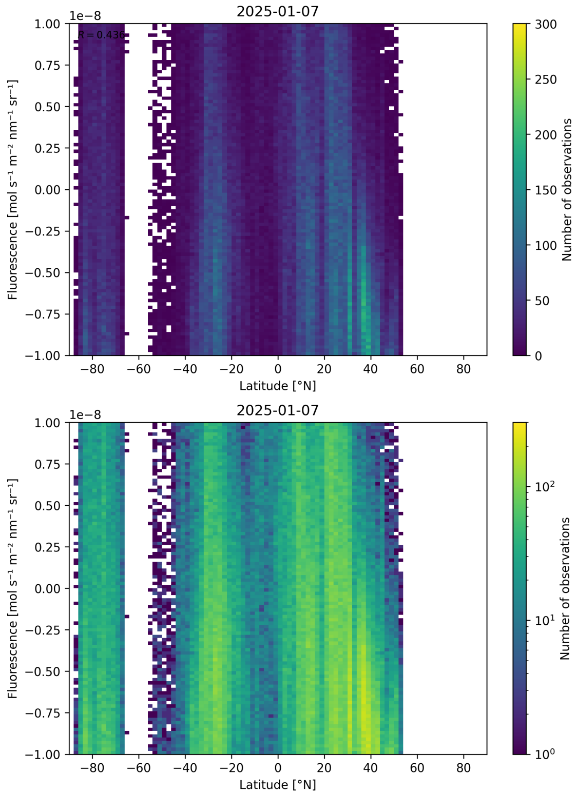
Figure 56: Scatter density plot of “Latitude” against “Fluorescence” for 2025-01-07 to 2025-01-08.
