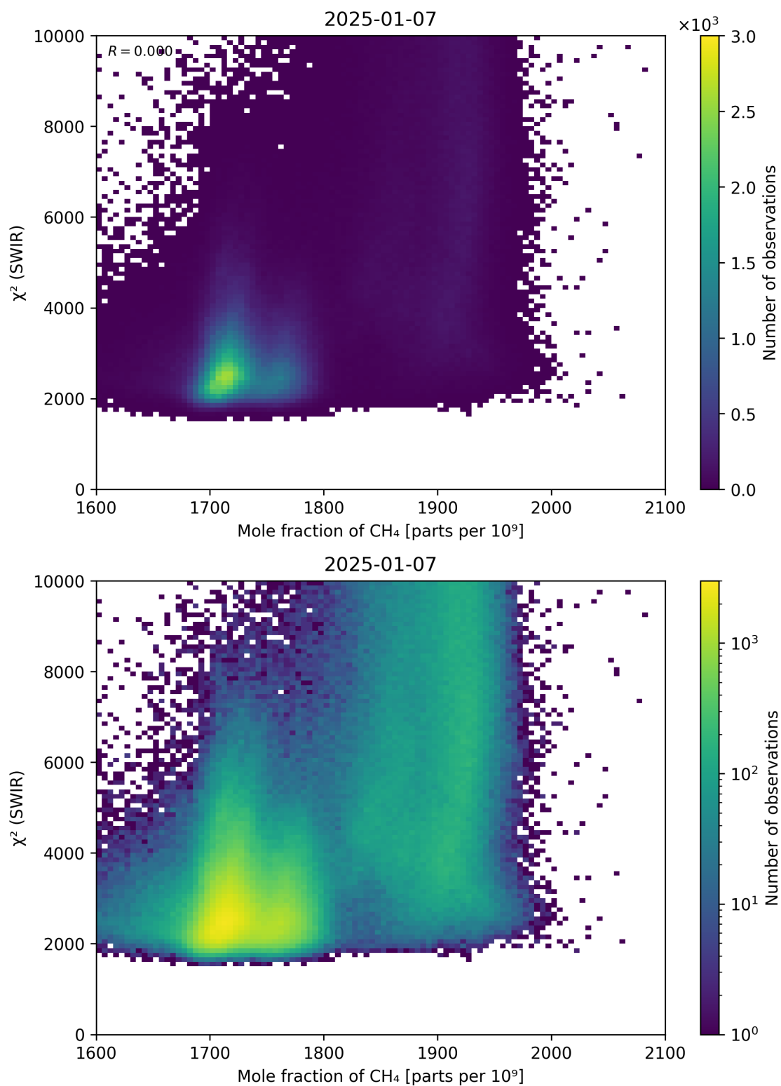
Figure 71: Scatter density plot of “Mole fraction of CH 4 ” against “ \chi^2 (SWIR)” for 2025-01-07 to 2025-01-08.
