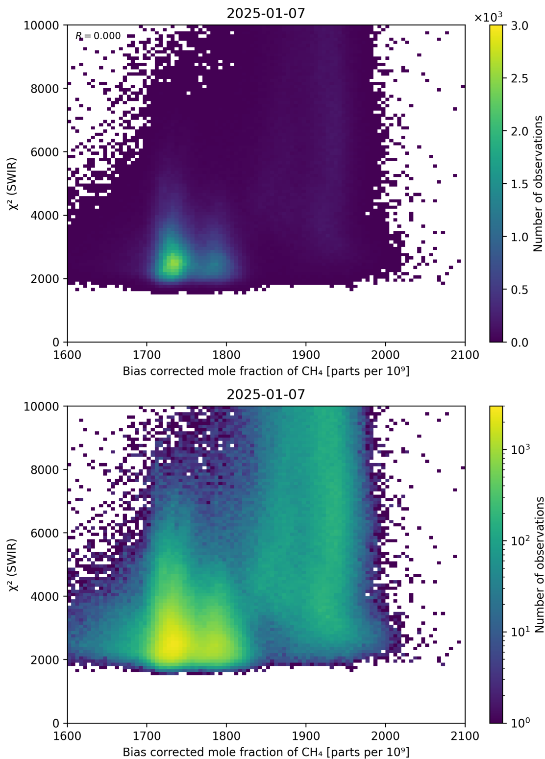
Figure 64: Scatter density plot of “Bias corrected mole fraction of \text{CH}_4 ” against “ \chi^2 (SWIR)” for 2025-01-07 to 2025-01-08.
