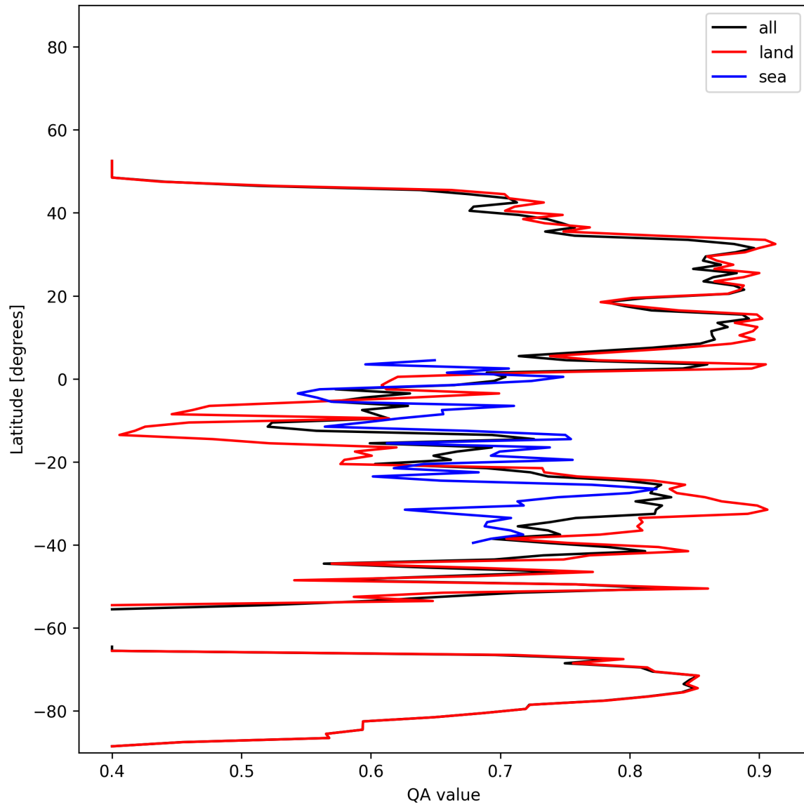
Figure 11: Zonal average of “QA value” for 2025-01-07 to 2025-01-08.
