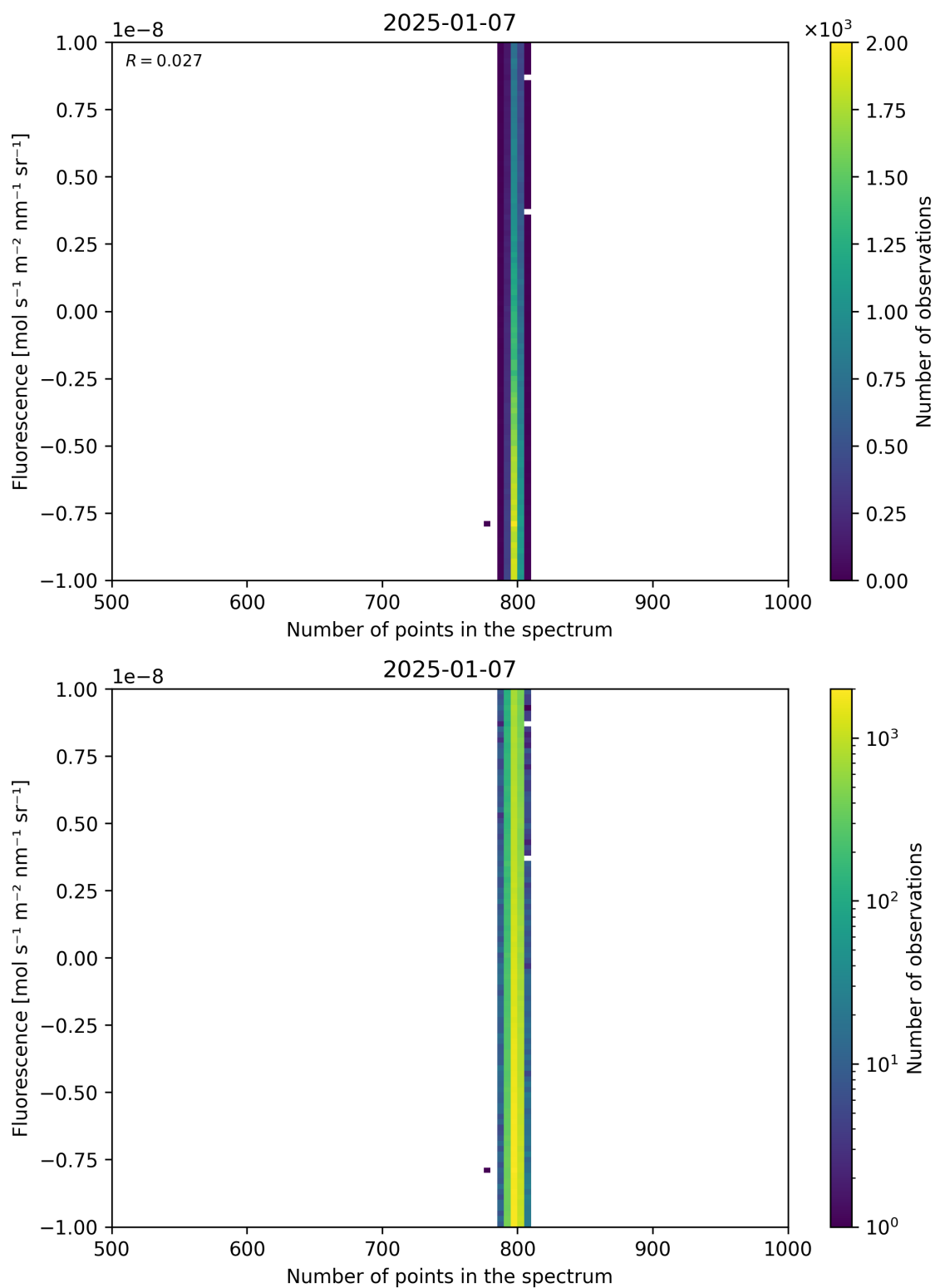
Figure 91: Scatter density plot of “Number of points in the spectrum” against “Fluorescence” for 2025-01-07 to 2025-01-08.
