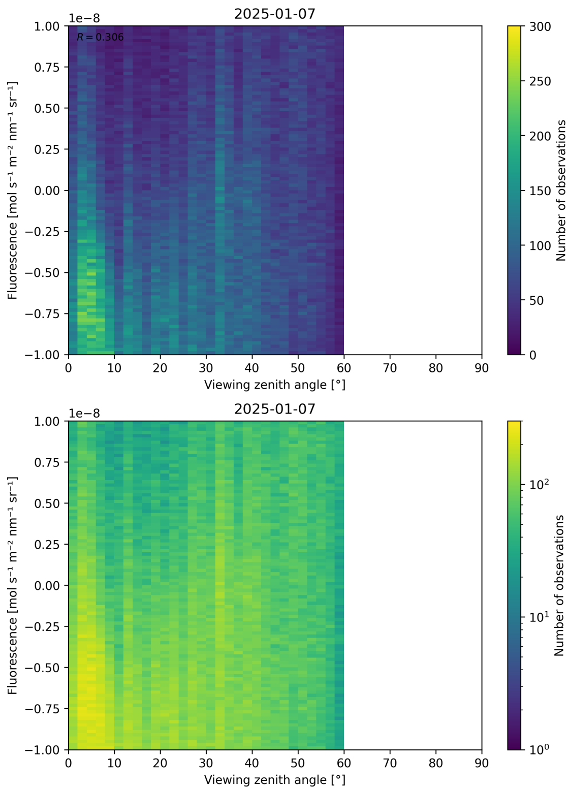
Figure 108: Scatter density plot of “Viewing zenith angle” against “Fluorescence” for 2025-01-07 to 2025-01-08.
