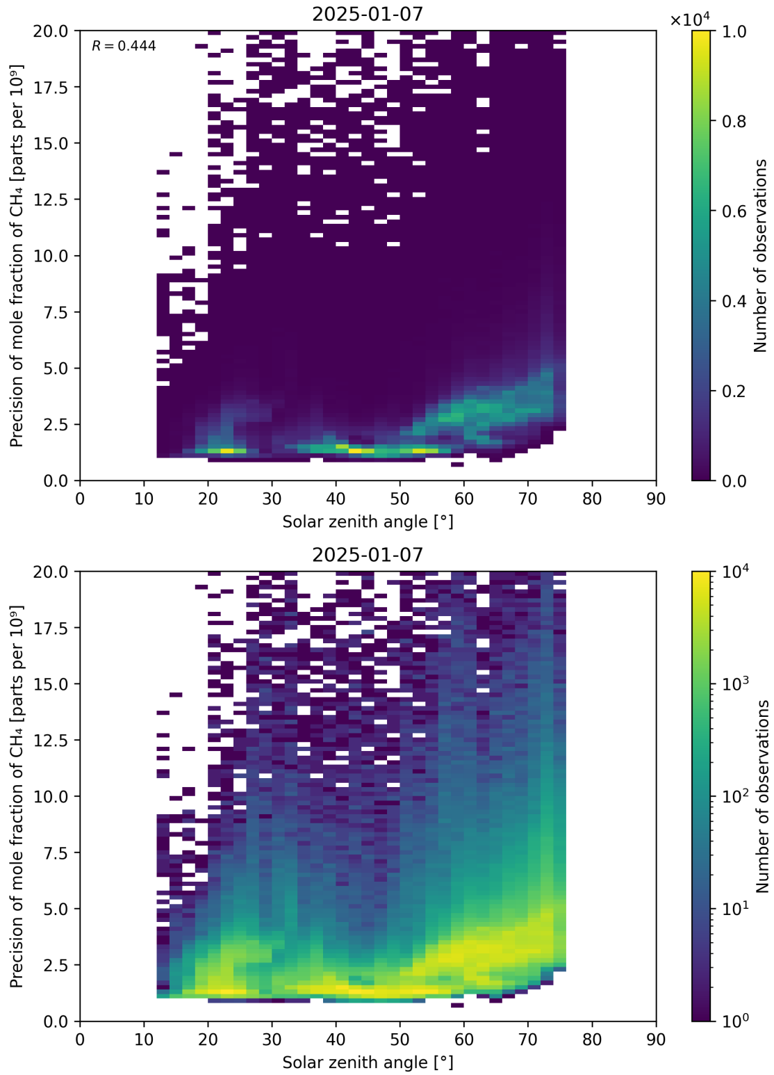
Figure 101: Scatter density plot of “Solar zenith angle” against “Precision of mole fraction of CH 4 ” for 2025-01-07 to 2025-01-08.
