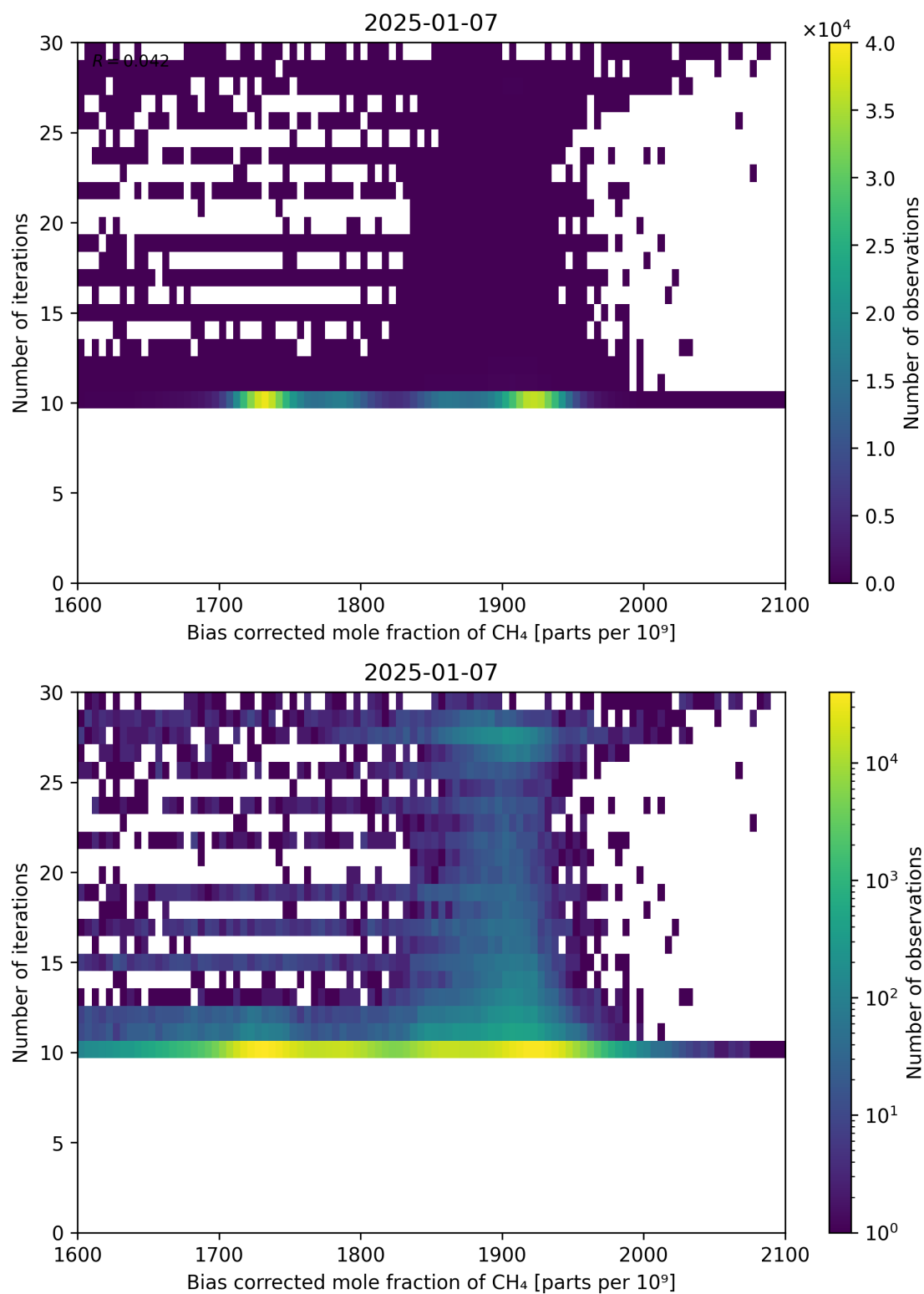
Figure 67: Scatter density plot of “Bias corrected mole fraction of CH 4 ” against “Number of iterations” for 2025-01-07 to 2025-01-08.
