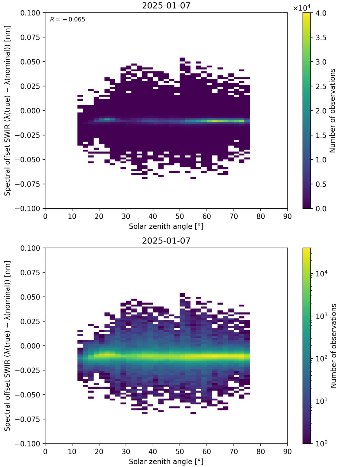
Figure 104: Scatter density plot of “Solar zenith angle” against “Spectral offset SWIR ( \lambda_{\text{true}} - \lambda_{\text{nominal}} )” for 2025-01-07 to 2025-01-08.
