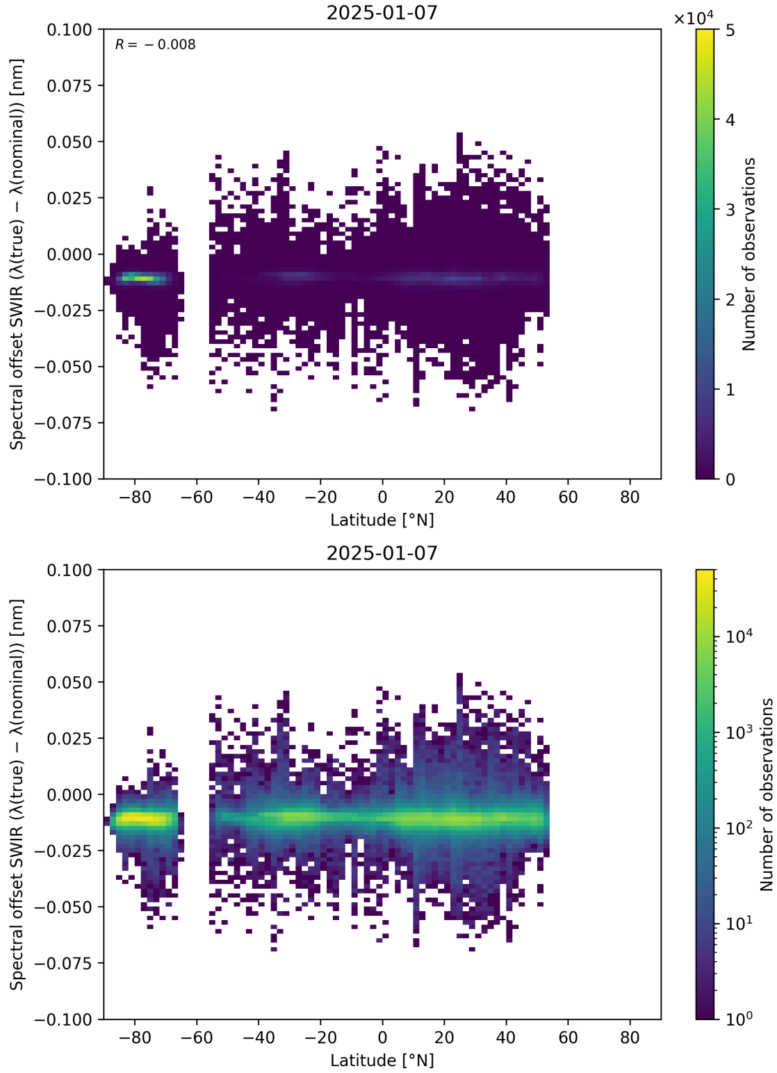
Figure 62: Scatter density plot of “Latitude” against “Spectral offset SWIR ( \lambda_{\text{true}} - \lambda_{\text{nominal}} )” for 2025-01-07 to 2025-01-08.
