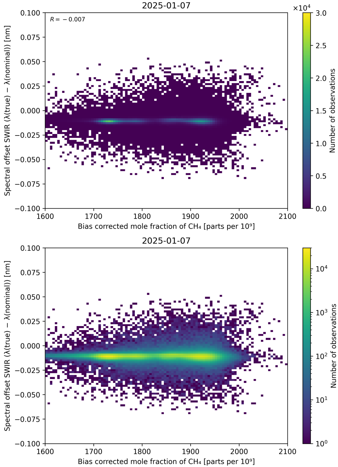
Figure 69: Scatter density plot of “Bias corrected mole fraction of \text{CH}_4 ” against “Spectral offset SWIR ( \lambda_{\text{true}} - \lambda_{\text{nominal}} )” for 2025-01-07 to 2025-01-08.
