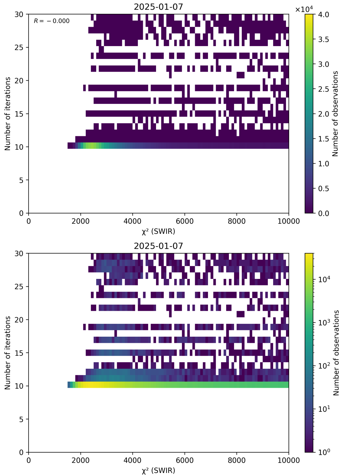
Figure 50: Scatter density plot of “ \chi^2 (SWIR)” against “Number of iterations” for 2025-01-07 to 2025-01-08.
