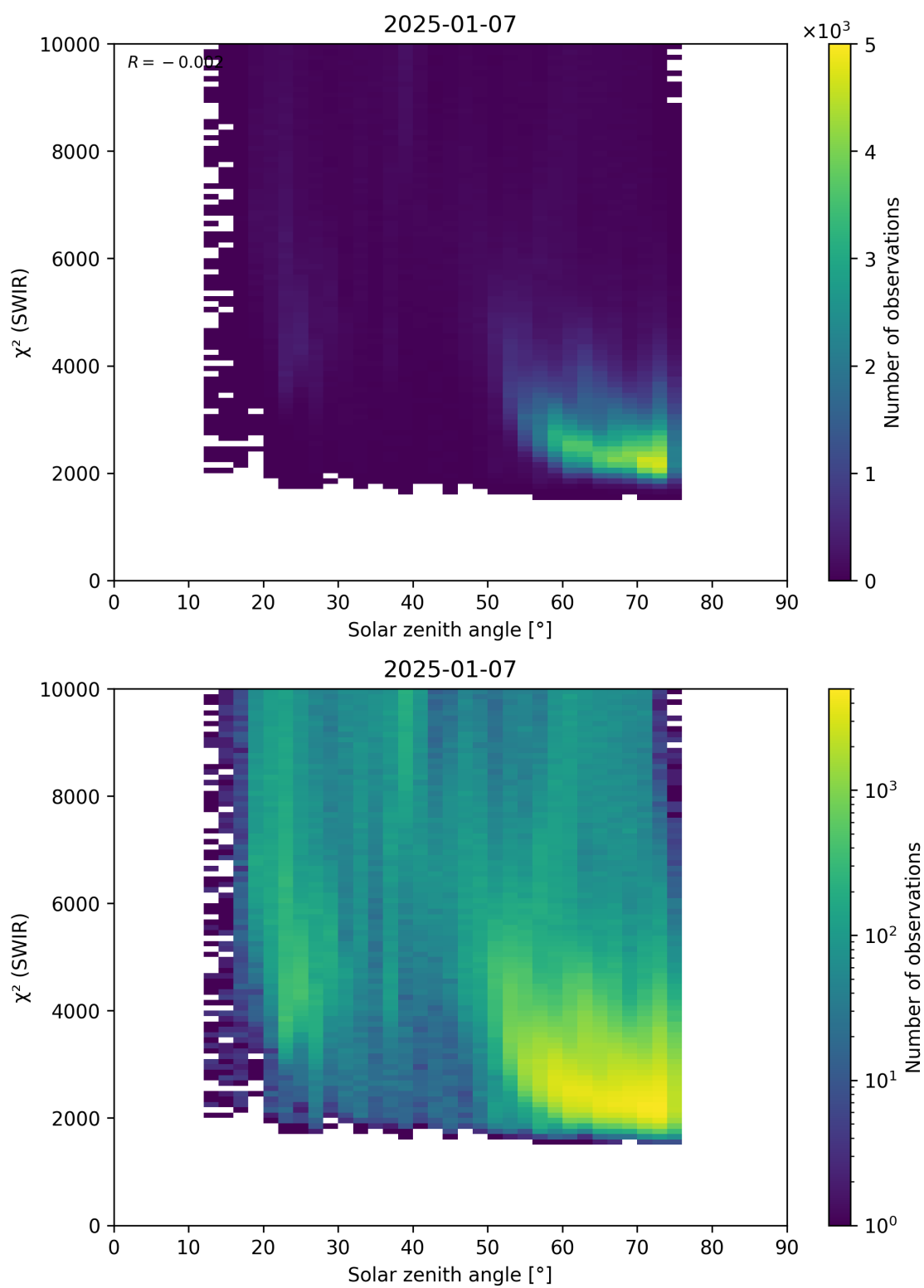
Figure 95: Scatter density plot of “Solar zenith angle” against “ \chi^2 (SWIR)” for 2025-01-07 to 2025-01-08.
