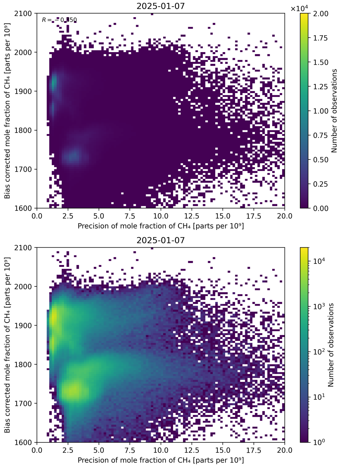
Figure 82: Scatter density plot of “Precision of mole fraction of CH 4 ” against “Bias corrected mole fraction of CH 4 ” for 2025-01-07 to 2025-01-08.
