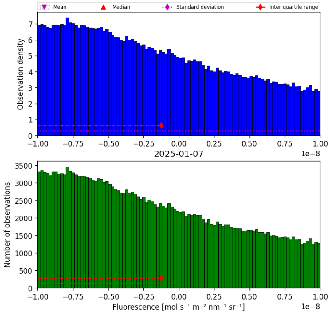
Figure 32: Histogram of “Fluorescence” for 2025-01-07 to 2025-01-08
