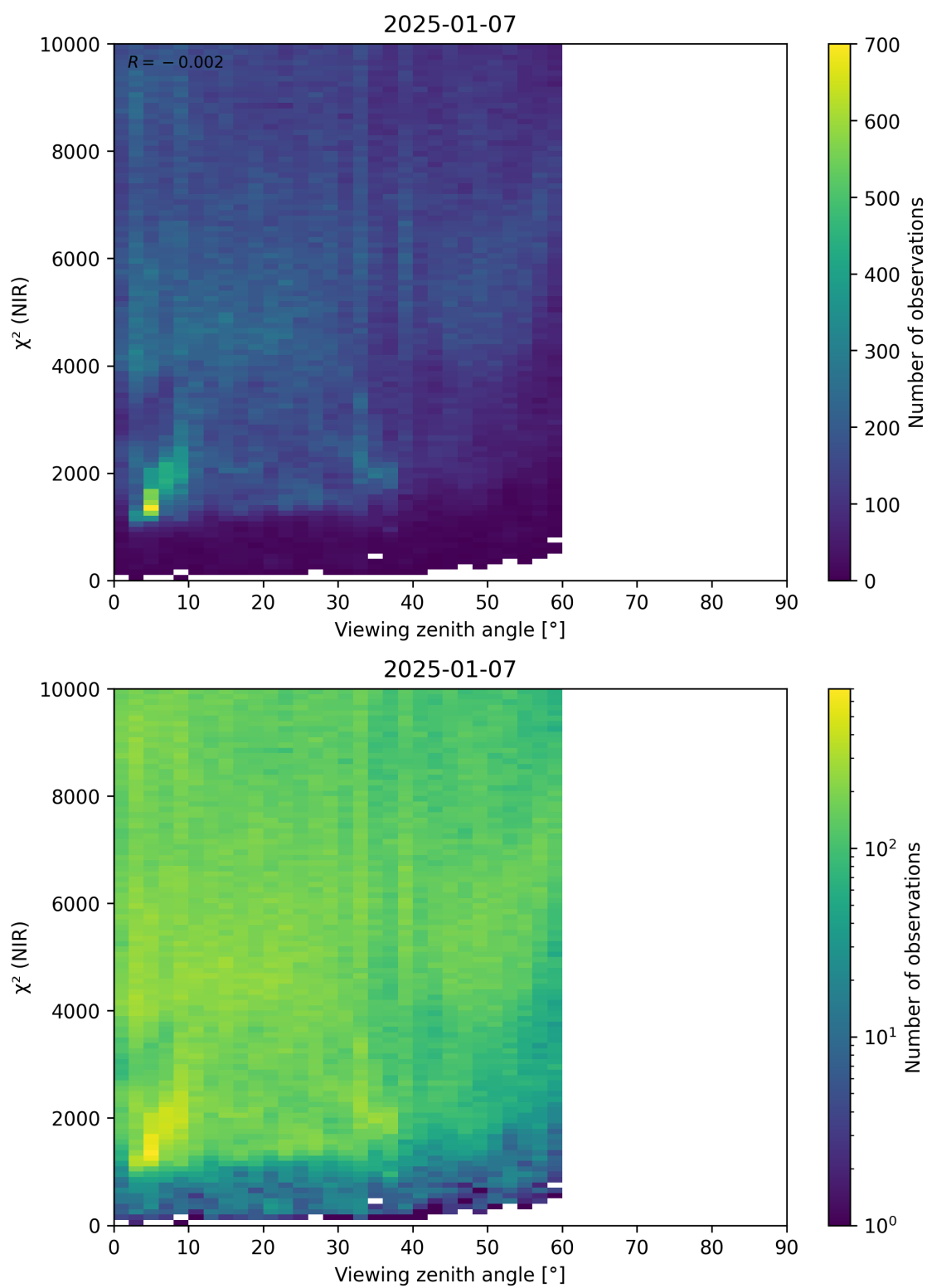
Figure 105: Scatter density plot of “Viewing zenith angle” against “ \chi^2 (NIR)” for 2025-01-07 to 2025-01-08.
