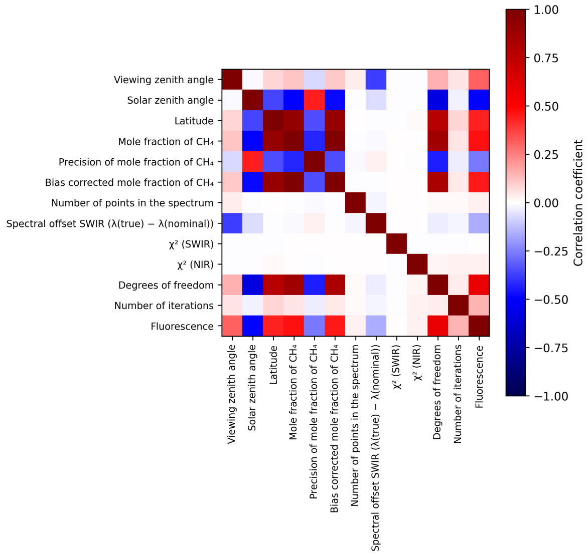
Figure 2: Map of correlation matrix for 2025-01-07 to 2025-01-08.
