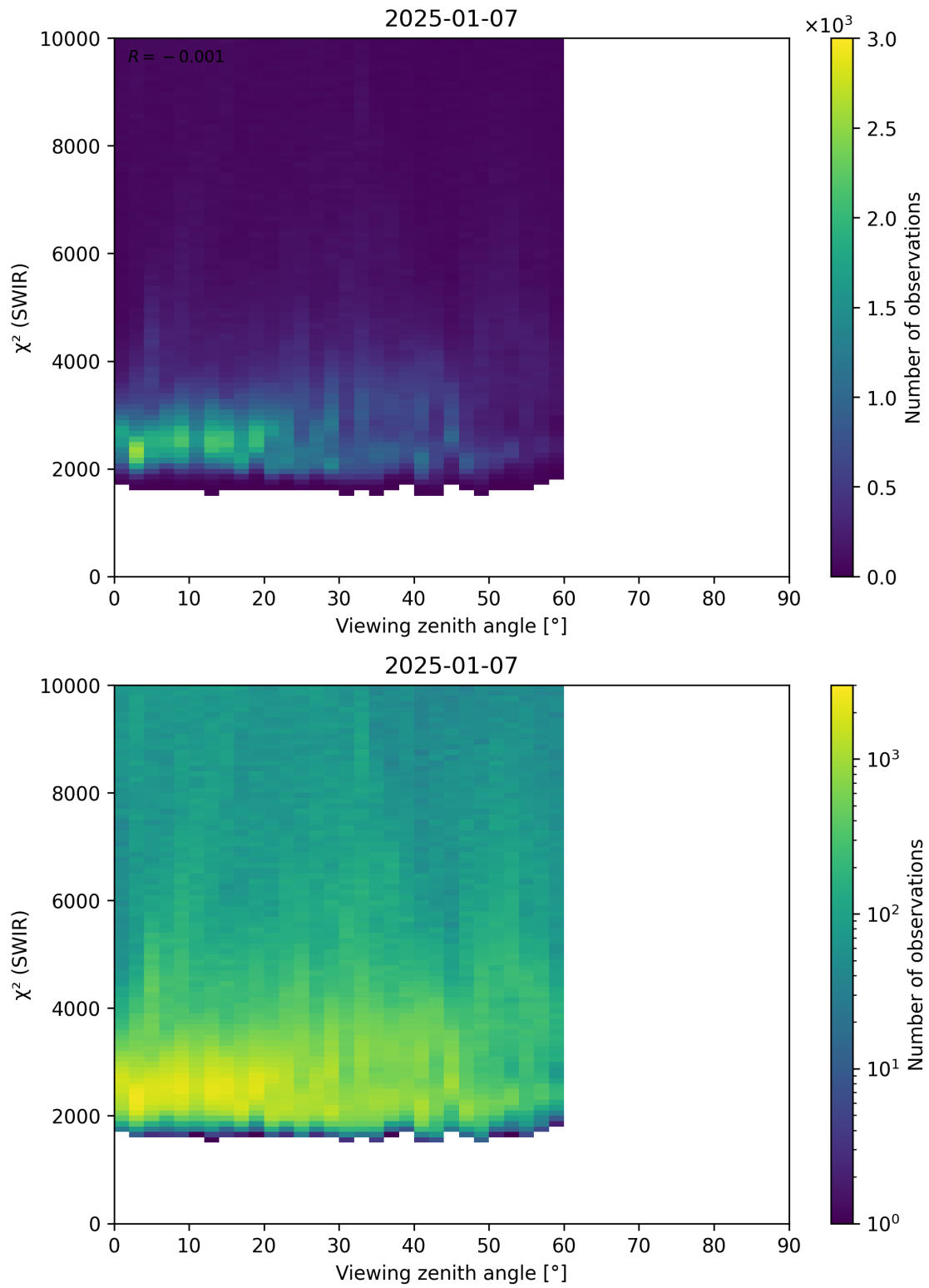
Figure 106: Scatter density plot of “Viewing zenith angle” against “ \chi^2 (SWIR)” for 2025-01-07 to 2025-01-08.
