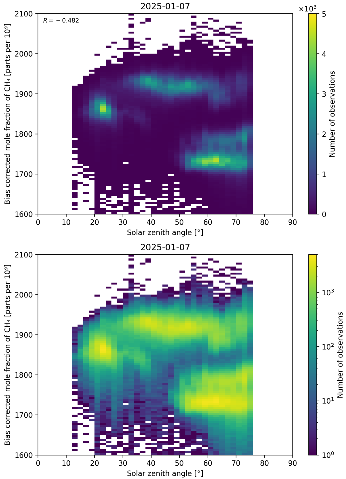
Figure 100: Scatter density plot of “Solar zenith angle” against “Bias corrected mole fraction of CH 4 ” for 2025-01-07 to 2025-01-08.
