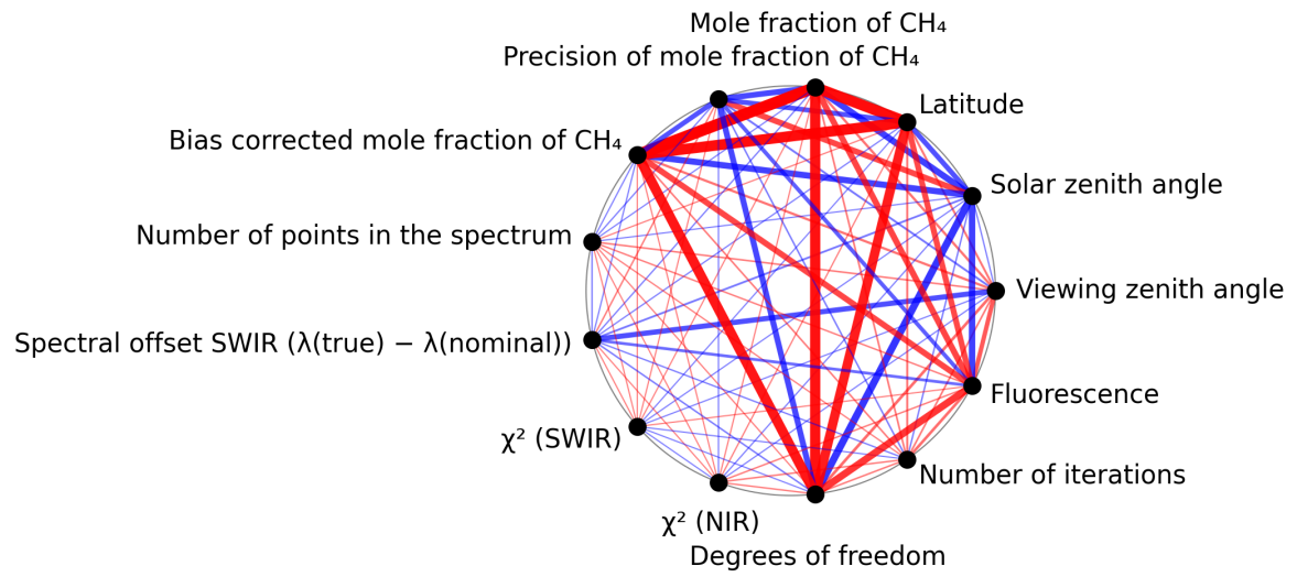
Figure 1: Map of correlation graph for 2025-01-07 to 2025-01-08.
