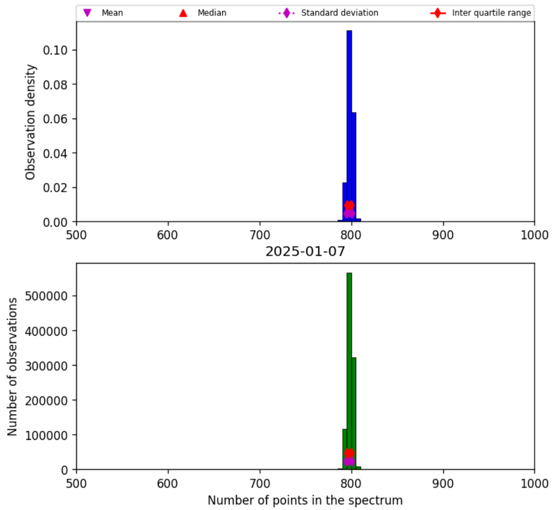
Figure 26: Histogram of “Number of points in the spectrum” for 2025-01-07 to 2025-01-08
