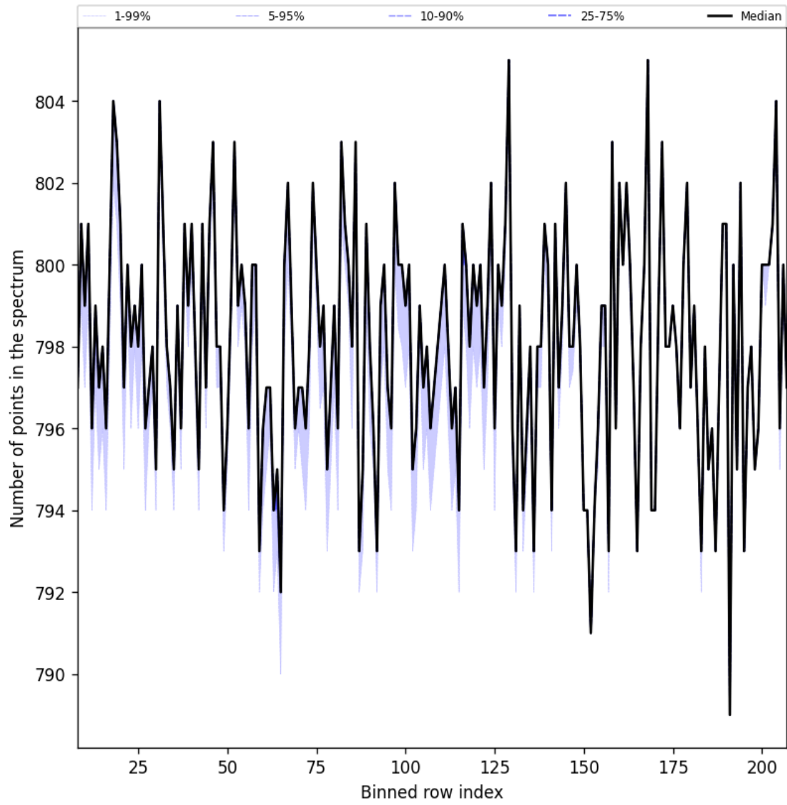
Figure 37: Along track statistics of “Number of points in the spectrum” for 2025-01-07 to 2025-01-08
