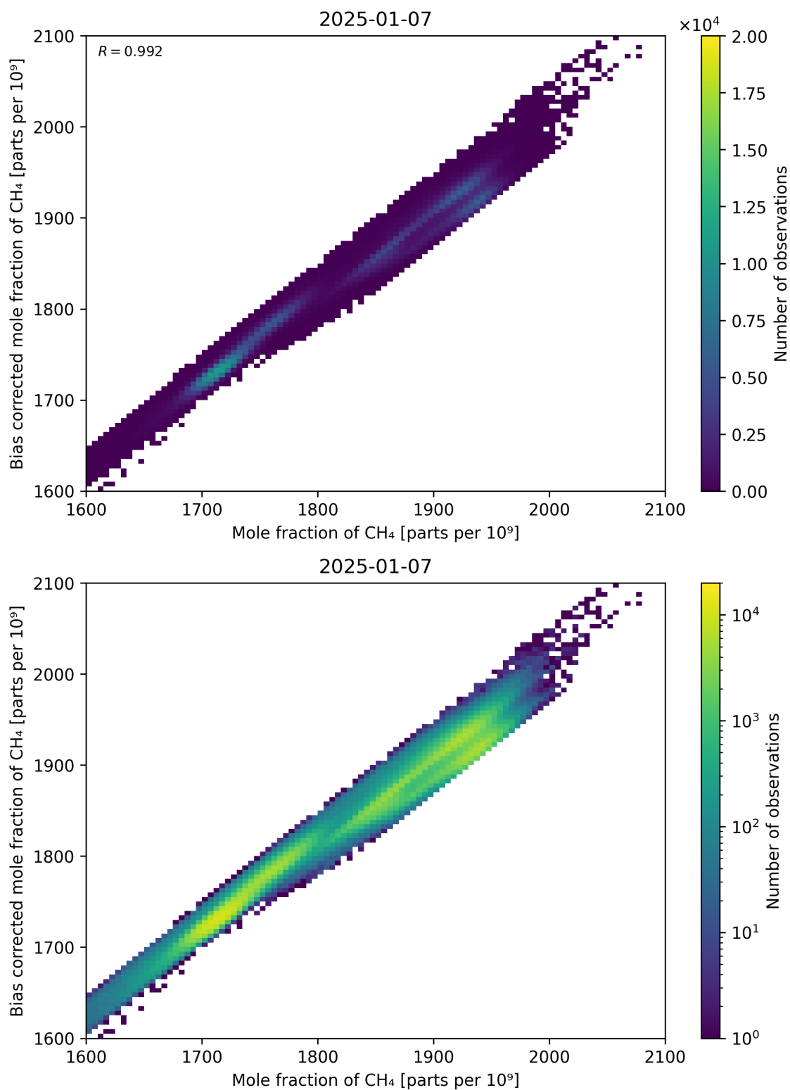
Figure 74: Scatter density plot of “Mole fraction of CH 4 ” against “Bias corrected mole fraction of CH 4 ” for 2025-01-07 to 2025-01-08.
