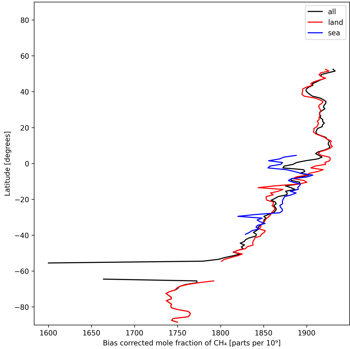
Figure 14: Zonal average of “Bias corrected mole fraction of CH 4 ” for 2025-01-07 to 2025-01-08.
