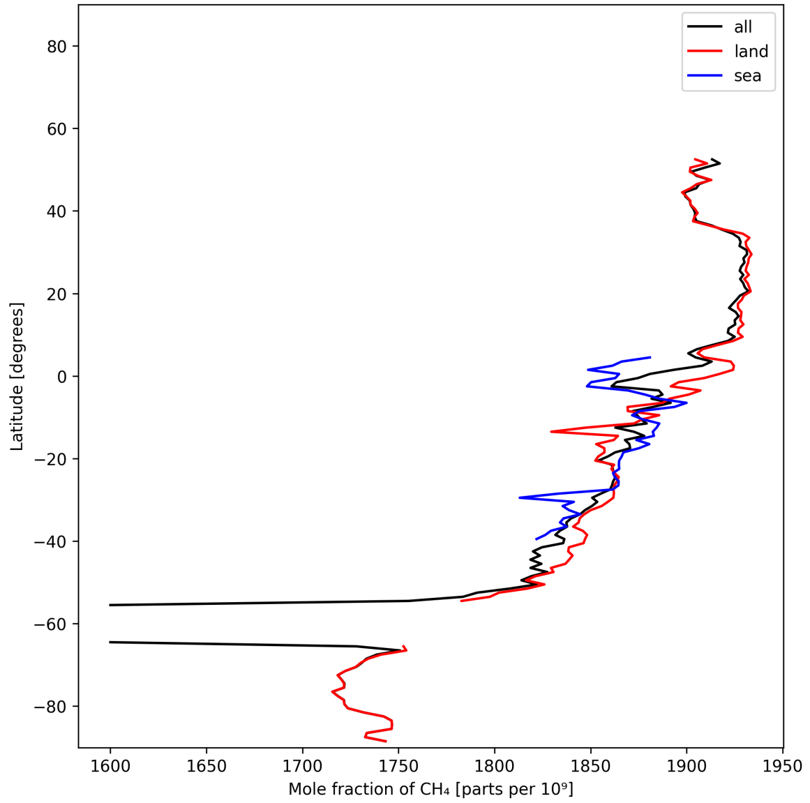
Figure 12: Zonal average of “Mole fraction of \text{CH}_4 ” for 2025-01-07 to 2025-01-08.
