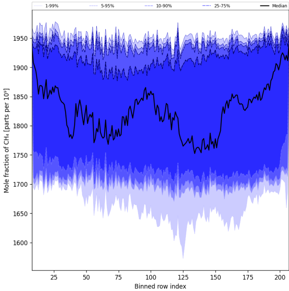
Figure 34: Along track statistics of “Mole fraction of CH 4 ” for 2025-01-07 to 2025-01-08
