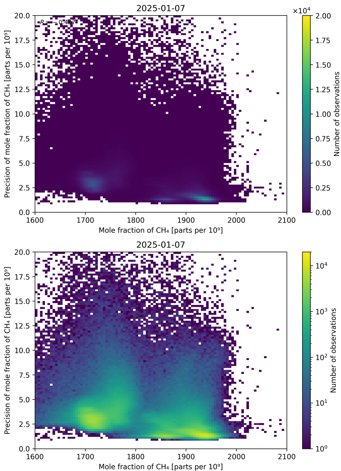
Figure 75: Scatter density plot of “Mole fraction of CH 4 ” against “Precision of mole fraction of CH 4 ” for 2025-01-07 to 2025-01-08.
