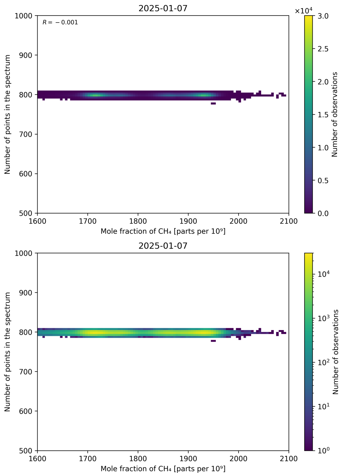
Figure 77: Scatter density plot of “Mole fraction of CH 4 ” against “Number of points in the spectrum” for 2025-01-07 to 2025-01-08.
