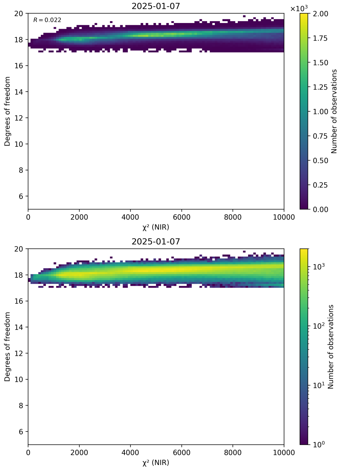
Figure 44: Scatter density plot of “ \chi^2 (NIR)” against “Degrees of freedom” for 2025-01-07 to 2025-01-08.
