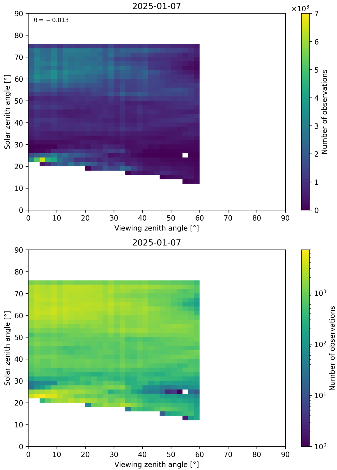
Figure 115: Scatter density plot of “Viewing zenith angle” against “Solar zenith angle” for 2025-01-07 to 2025-01-08.
