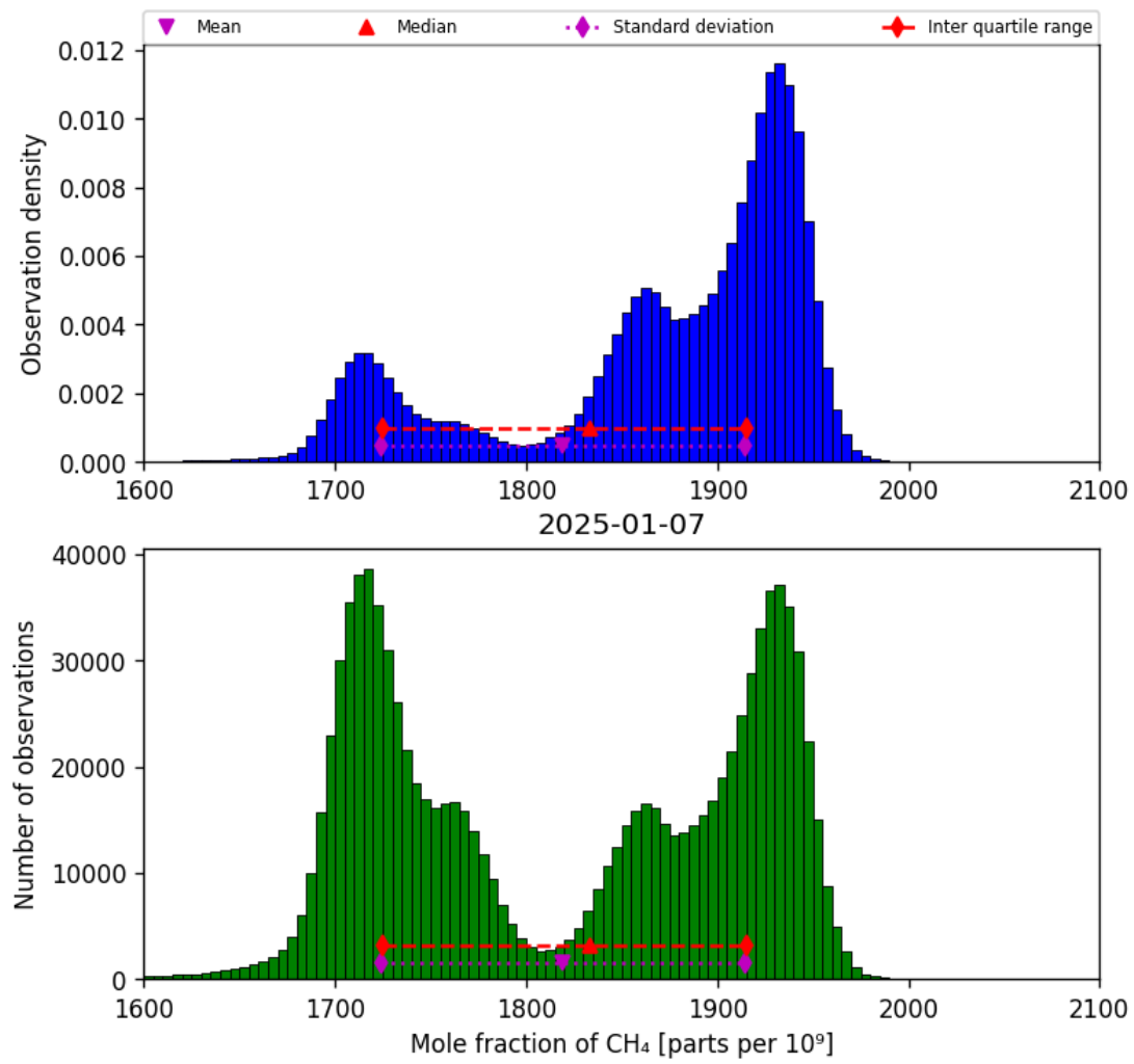
Figure 23: Histogram of “Mole fraction of CH 4 ” for 2025-01-07 to 2025-01-08
