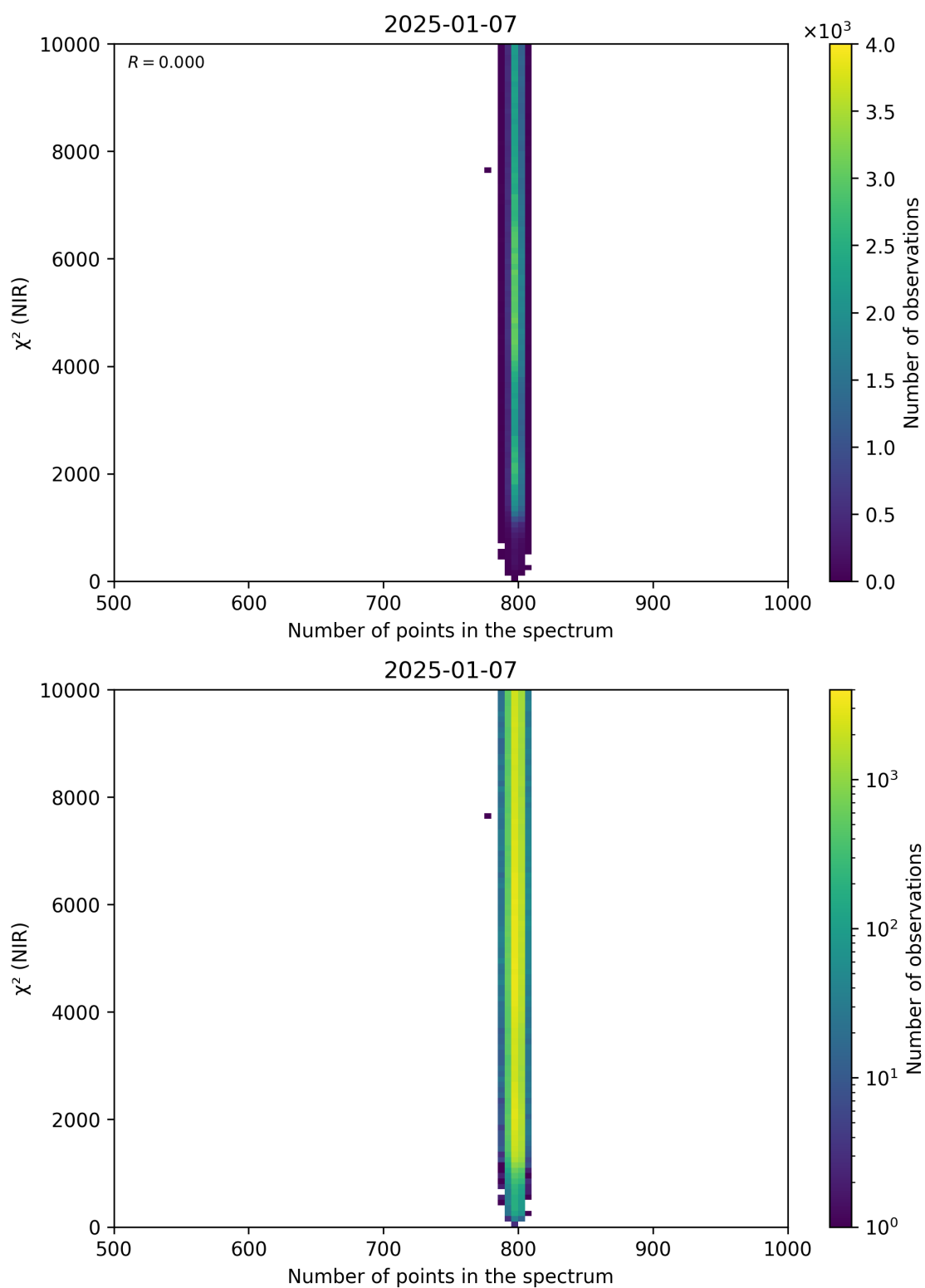
Figure 88: Scatter density plot of “Number of points in the spectrum” against “ \chi^2 (NIR)” for 2025-01-07 to 2025-01-08.
