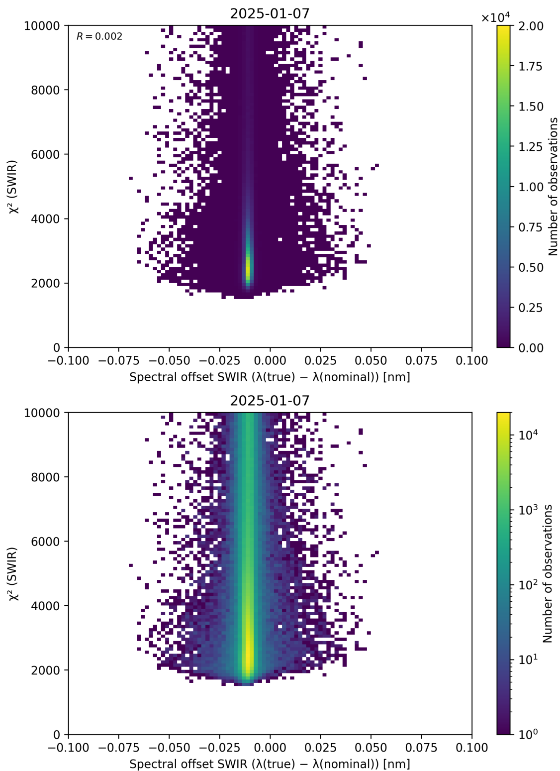
Figure 118: Scatter density plot of “Spectral offset SWIR ( \lambda_{\text{true}} - \lambda_{\text{nominal}} )” against “ \chi^2 (SWIR)” for 2025-01-07 to 2025-01-08.
