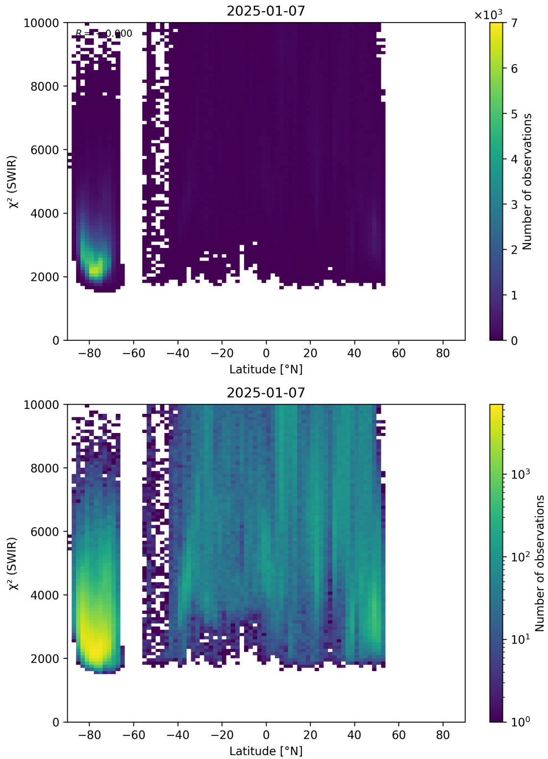
Figure 54: Scatter density plot of “Latitude” against “ \chi^2 (SWIR)” for 2025-01-07 to 2025-01-08.
