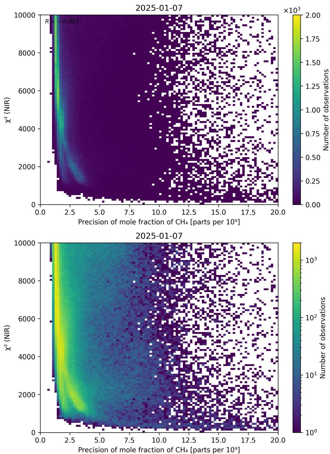
Figure 78: Scatter density plot of “Precision of mole fraction of \text{CH}_4 ” against “ \chi^2 (NIR)” for 2025-01-07 to 2025-01-08.
