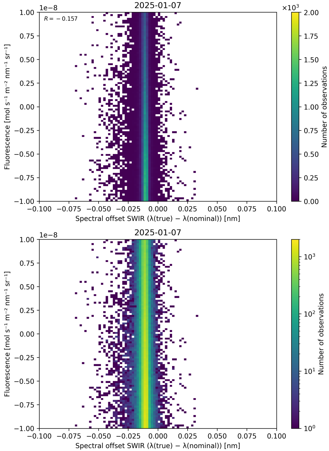
Figure 120: Scatter density plot of “Spectral offset SWIR ( \lambda_{\text{true}} - \lambda_{\text{nominal}} )” against “Fluorescence” for 2025-01-07 to 2025-01-08.
