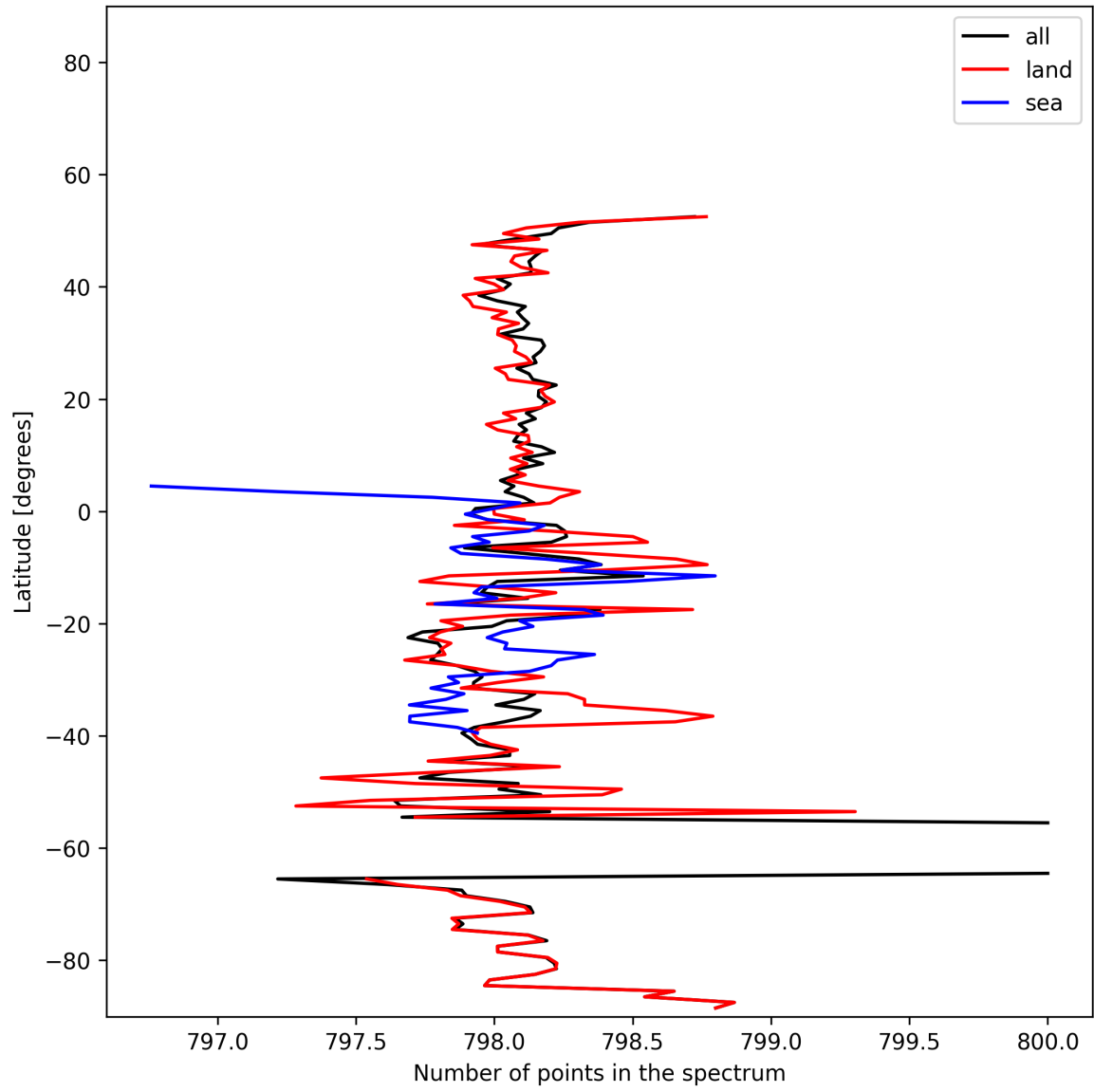
Figure 15: Zonal average of “Number of points in the spectrum” for 2025-01-07 to 2025-01-08.
