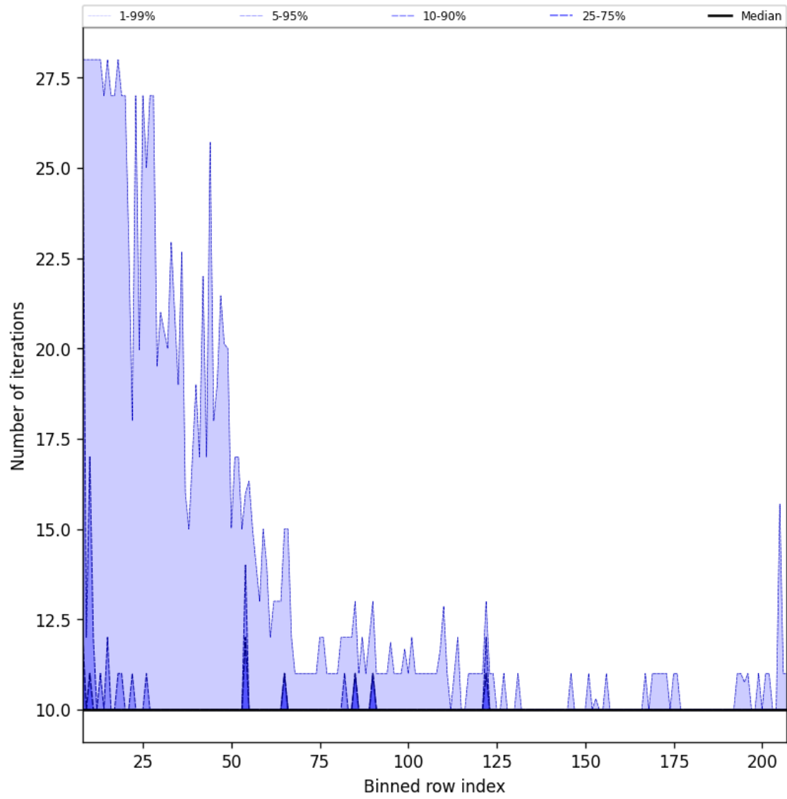
Figure 42: Along track statistics of “Number of iterations” for 2025-01-07 to 2025-01-08
