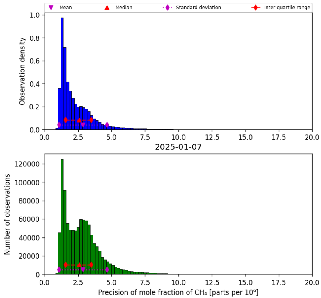
Figure 24: Histogram of “Precision of mole fraction of CH 4 ” for 2025-01-07 to 2025-01-08
