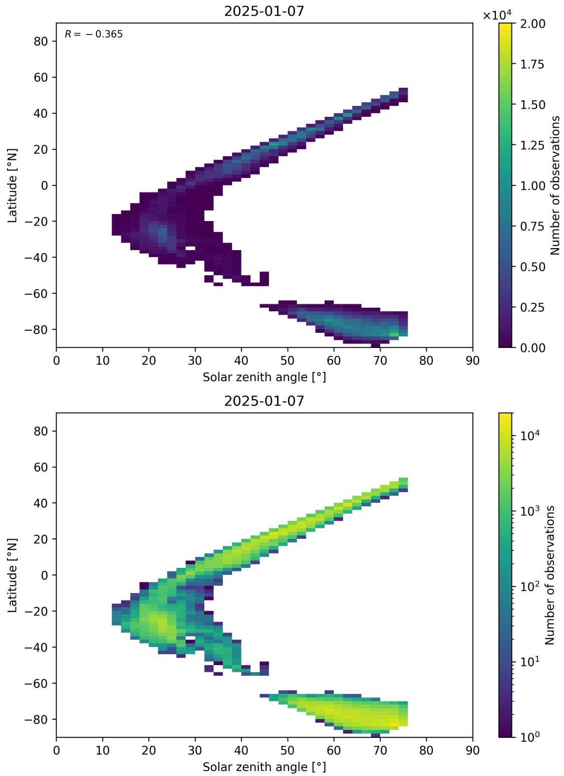
Figure 98: Scatter density plot of “Solar zenith angle” against “Latitude” for 2025-01-07 to 2025-01-08.
