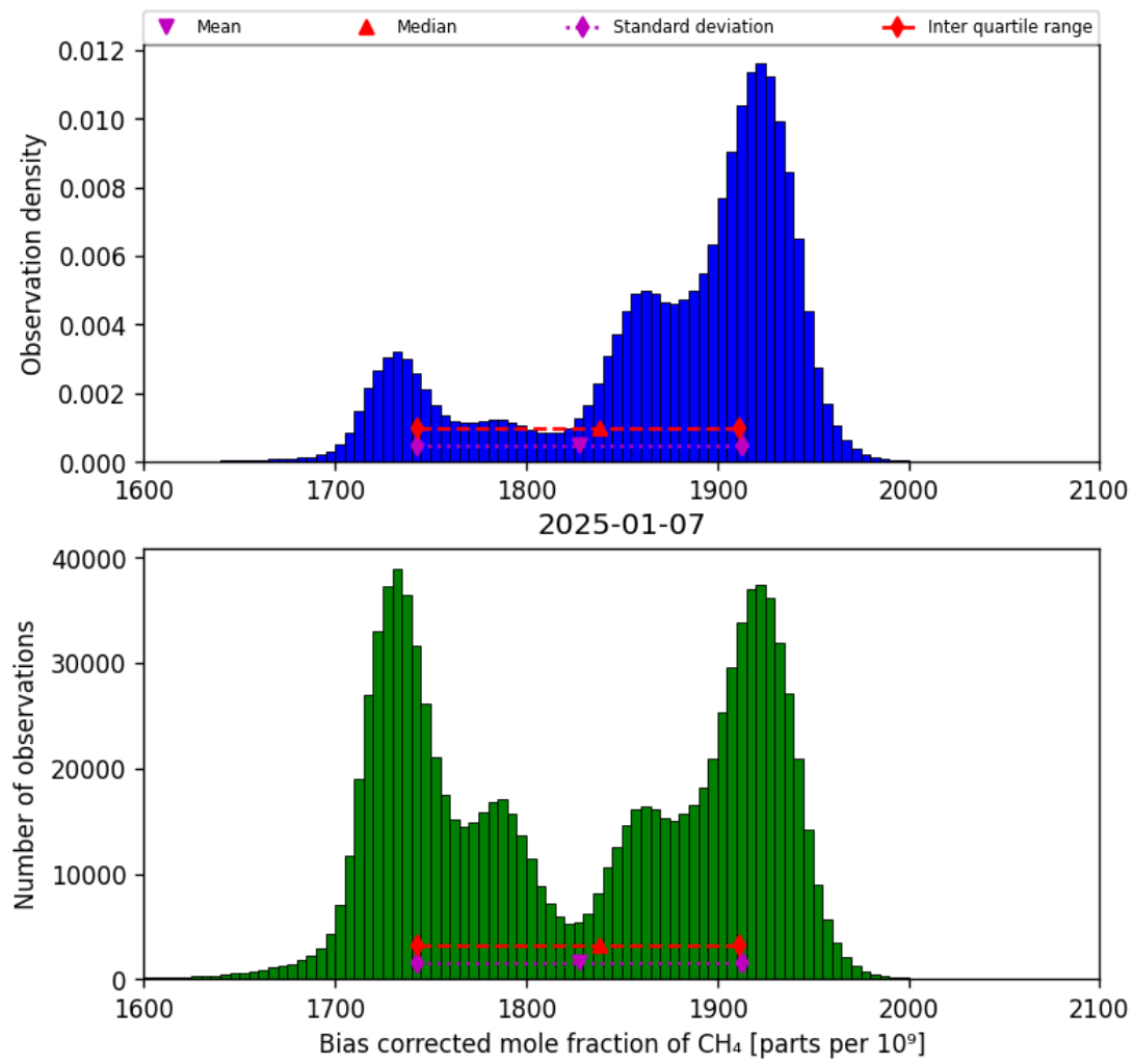
Figure 25: Histogram of “Bias corrected mole fraction of CH 4 ” for 2025-01-07 to 2025-01-08
