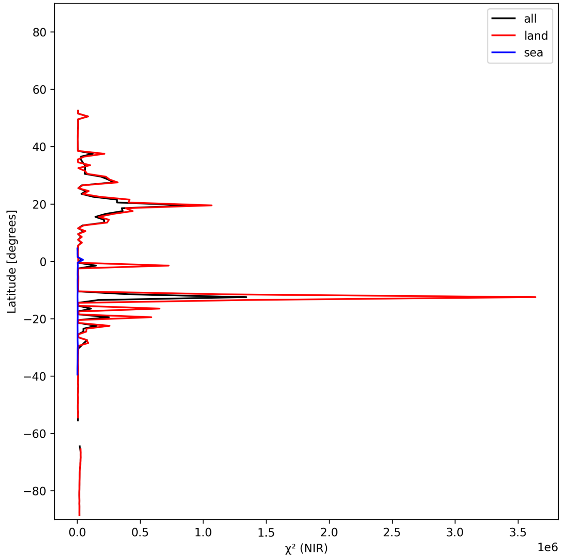
Figure 18: Zonal average of “ \chi^2 (NIR)” for 2025-01-07 to 2025-01-08.
