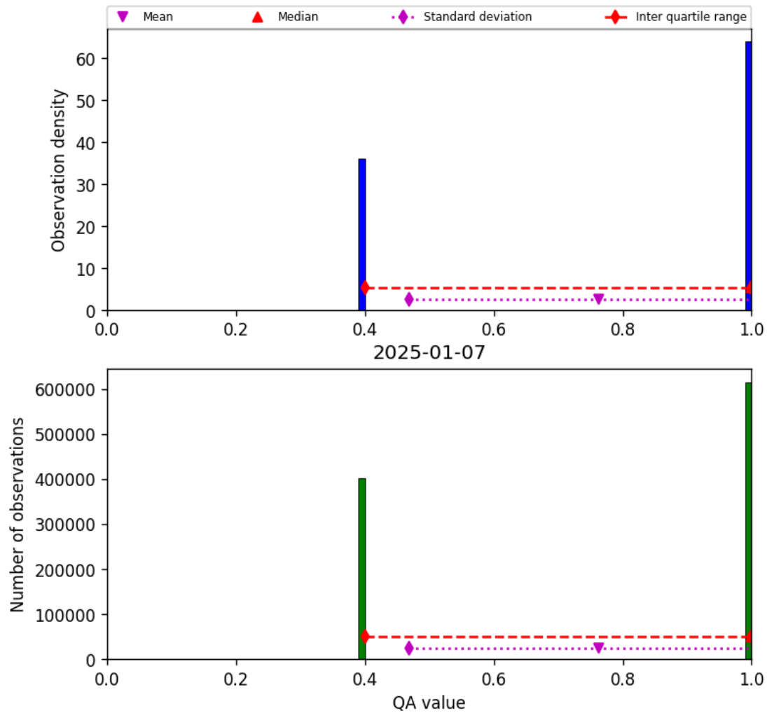
Figure 22: Histogram of “QA value” for 2025-01-07 to 2025-01-08
