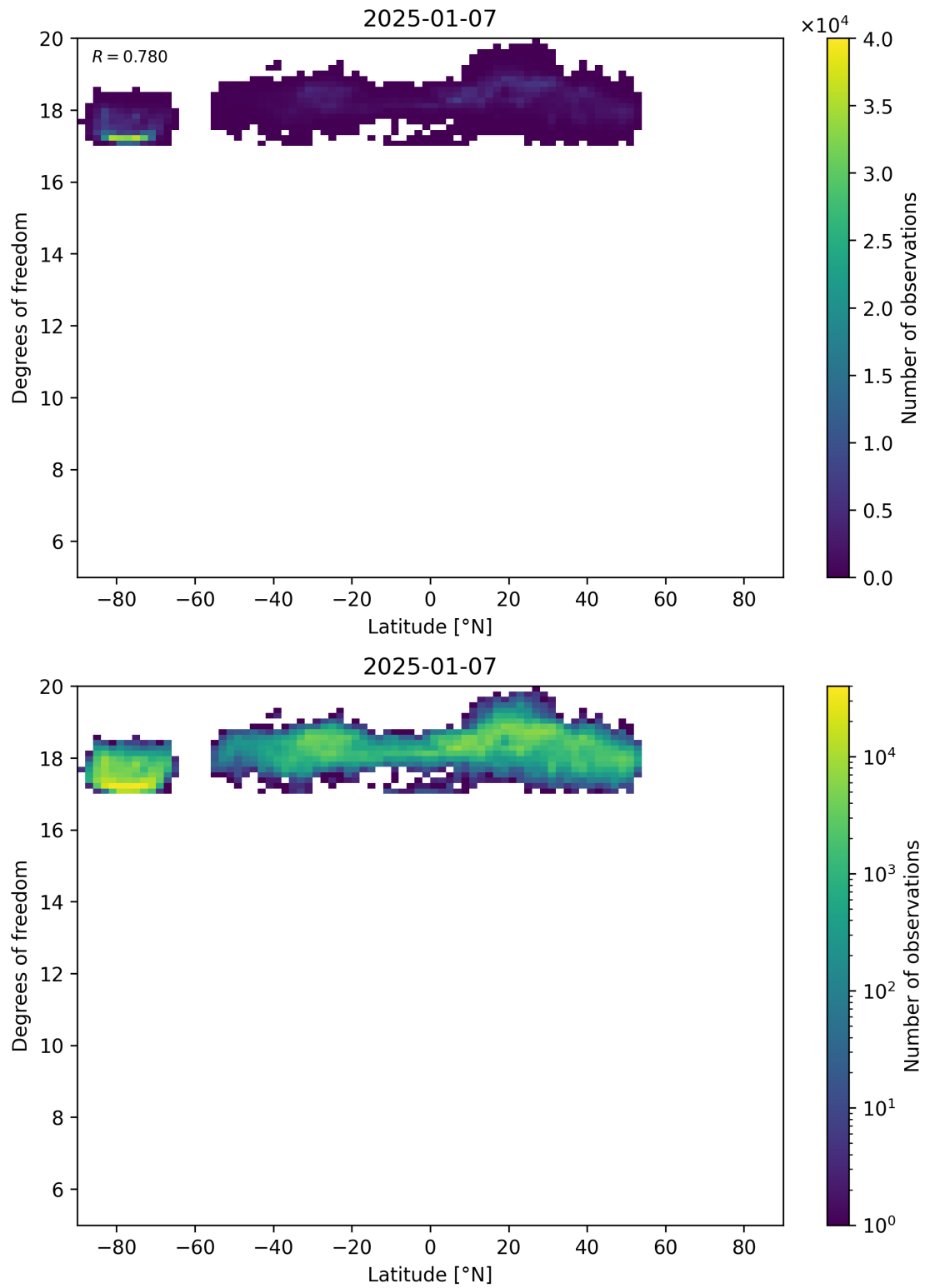
Figure 55: Scatter density plot of “Latitude” against “Degrees of freedom” for 2025-01-07 to 2025-01-08.
