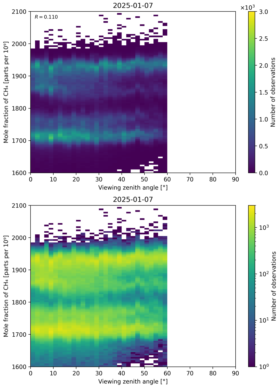
Figure 110: Scatter density plot of “Viewing zenith angle” against “Mole fraction of CH 4 ” for 2025-01-07 to 2025-01-08.
