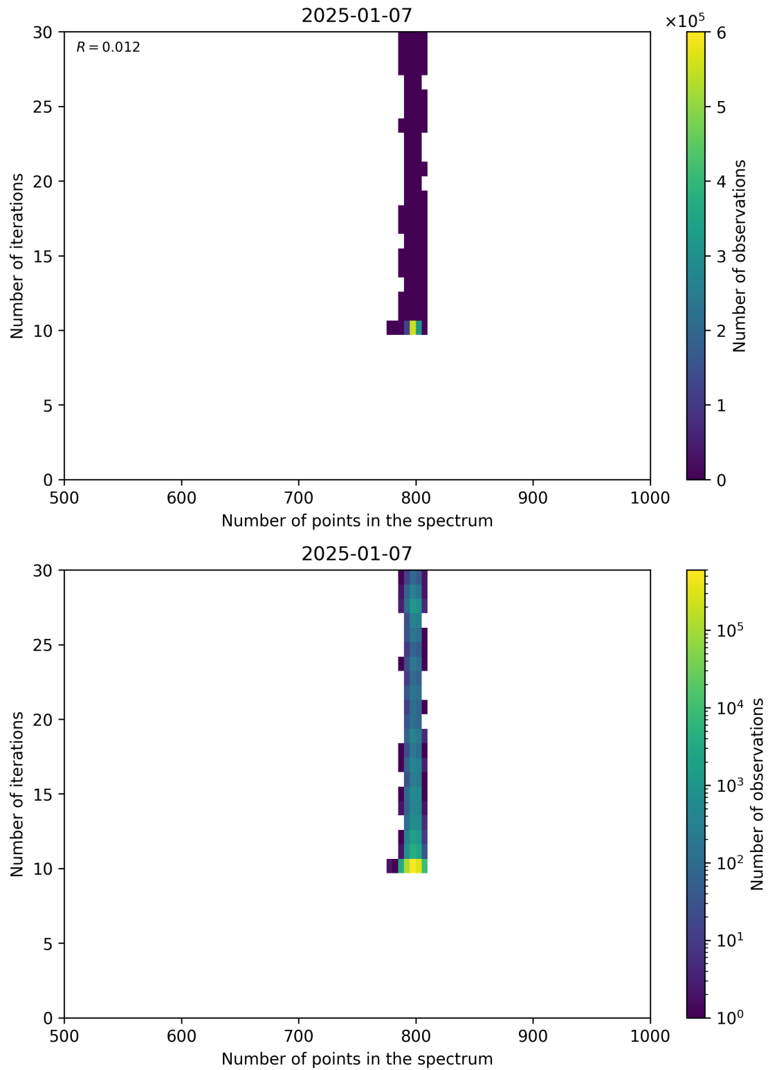
Figure 92: Scatter density plot of “Number of points in the spectrum” against “Number of iterations” for 2025-01-07 to 2025-01-08.
