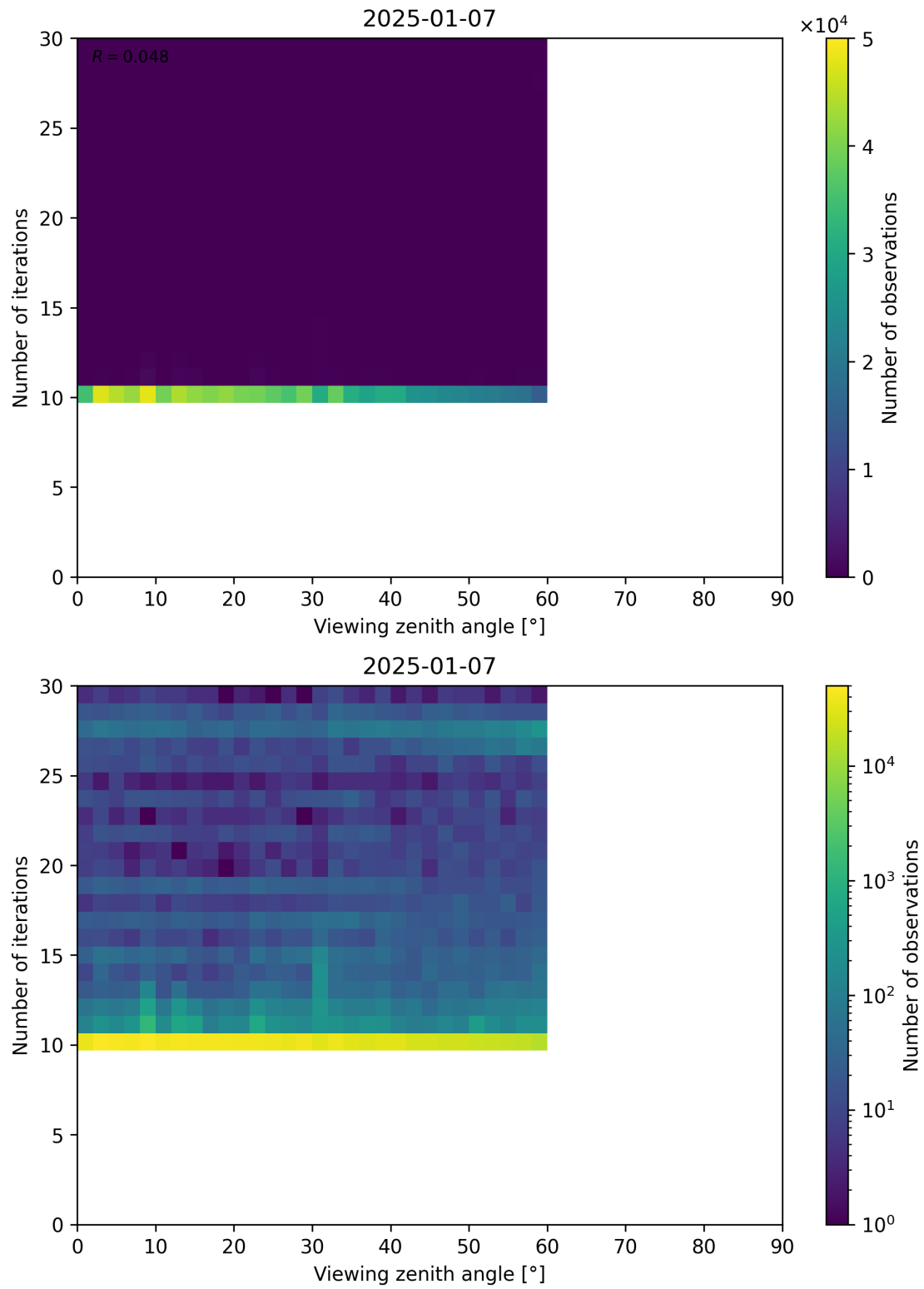
Figure 113: Scatter density plot of “Viewing zenith angle” against “Number of iterations” for 2025-01-07 to 2025-01-08.
