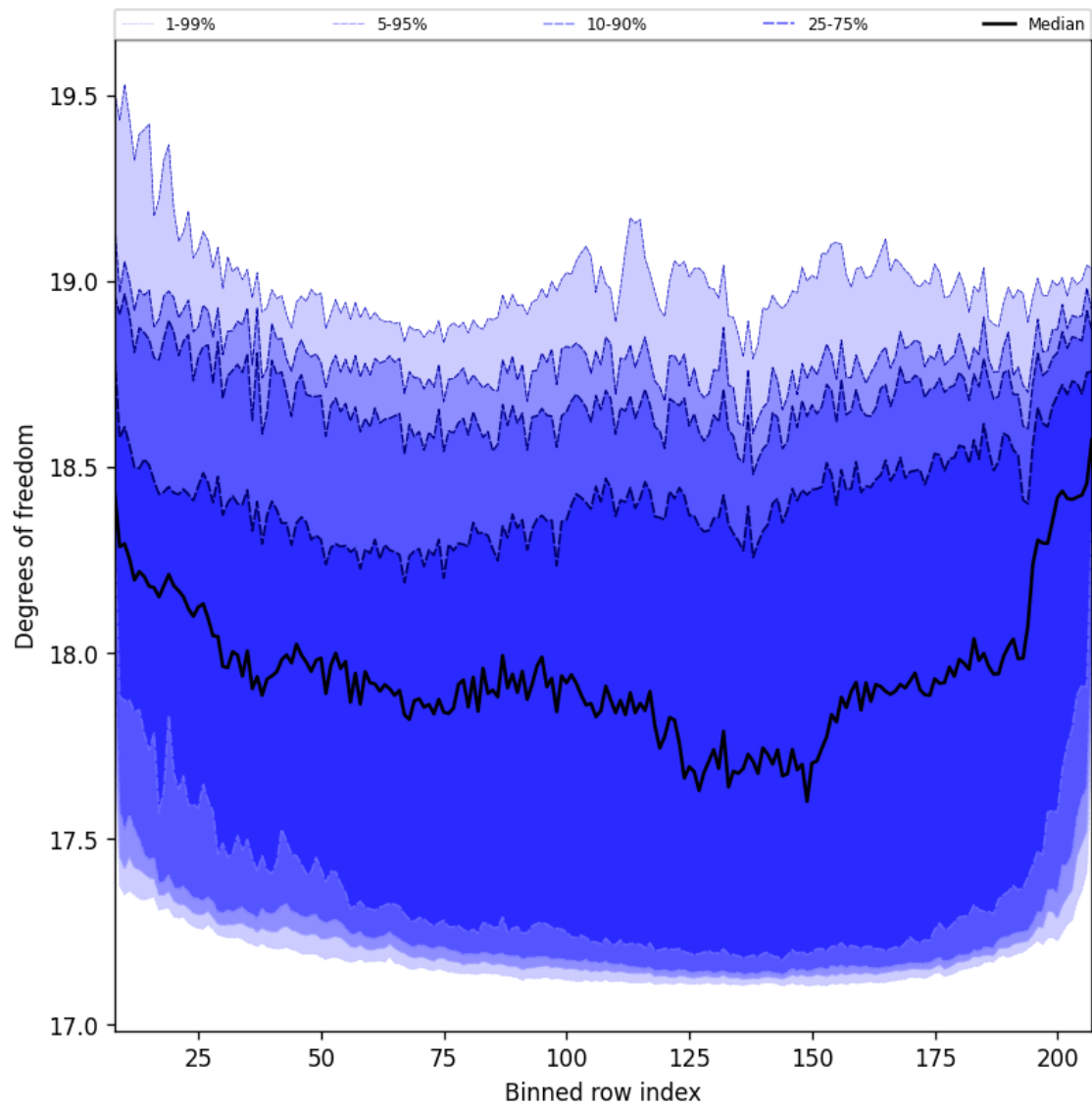
Figure 41: Along track statistics of “Degrees of freedom” for 2025-01-07 to 2025-01-08
