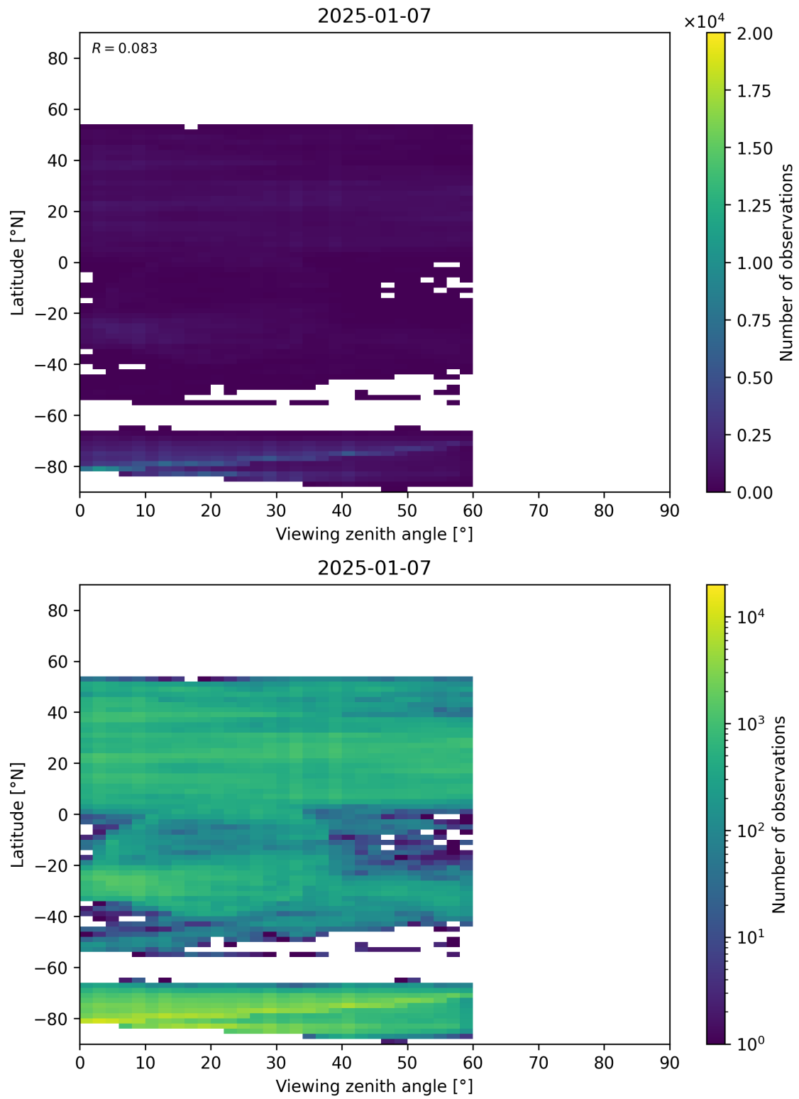
Figure 109: Scatter density plot of “Viewing zenith angle” against “Latitude” for 2025-01-07 to 2025-01-08.
