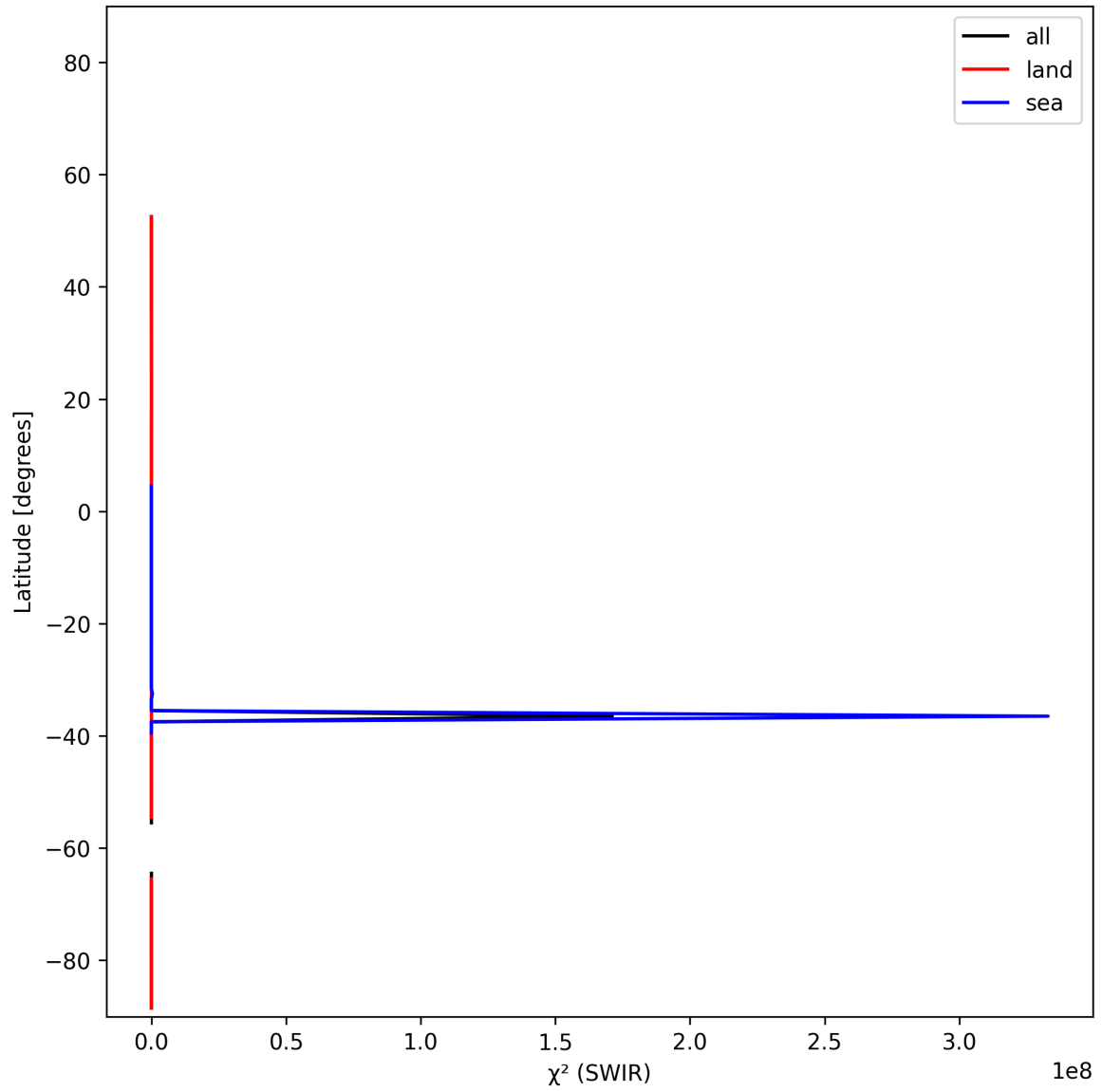
Figure 17: Zonal average of “ \chi^2 (SWIR)” for 2025-01-07 to 2025-01-08.
