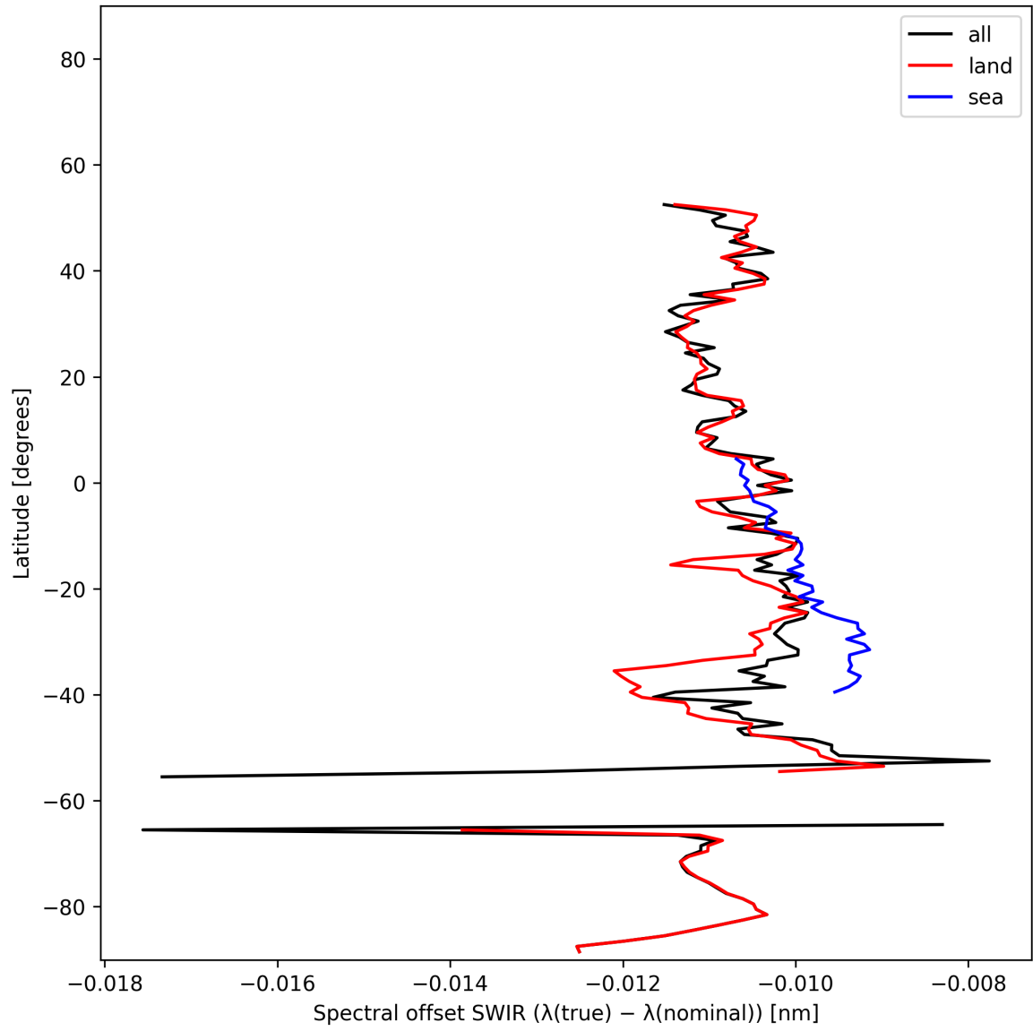
Figure 16: Zonal average of “Spectral offset SWIR ( \lambda_{\text{true}} - \lambda_{\text{nominal}} )” for 2025-01-07 to 2025-01-08.
