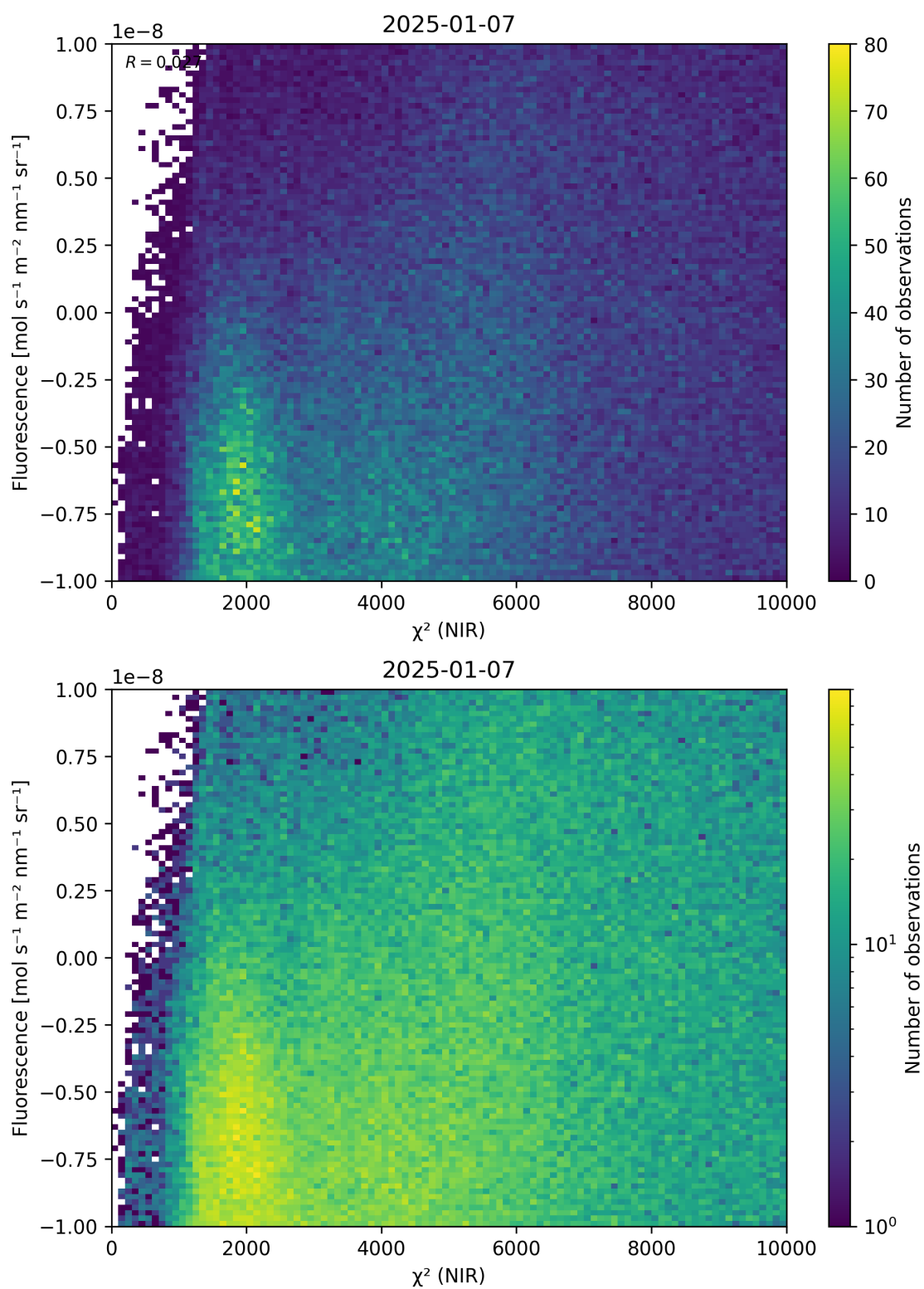
Figure 45: Scatter density plot of “ \chi^2 (NIR)” against “Fluorescence” for 2025-01-07 to 2025-01-08.
