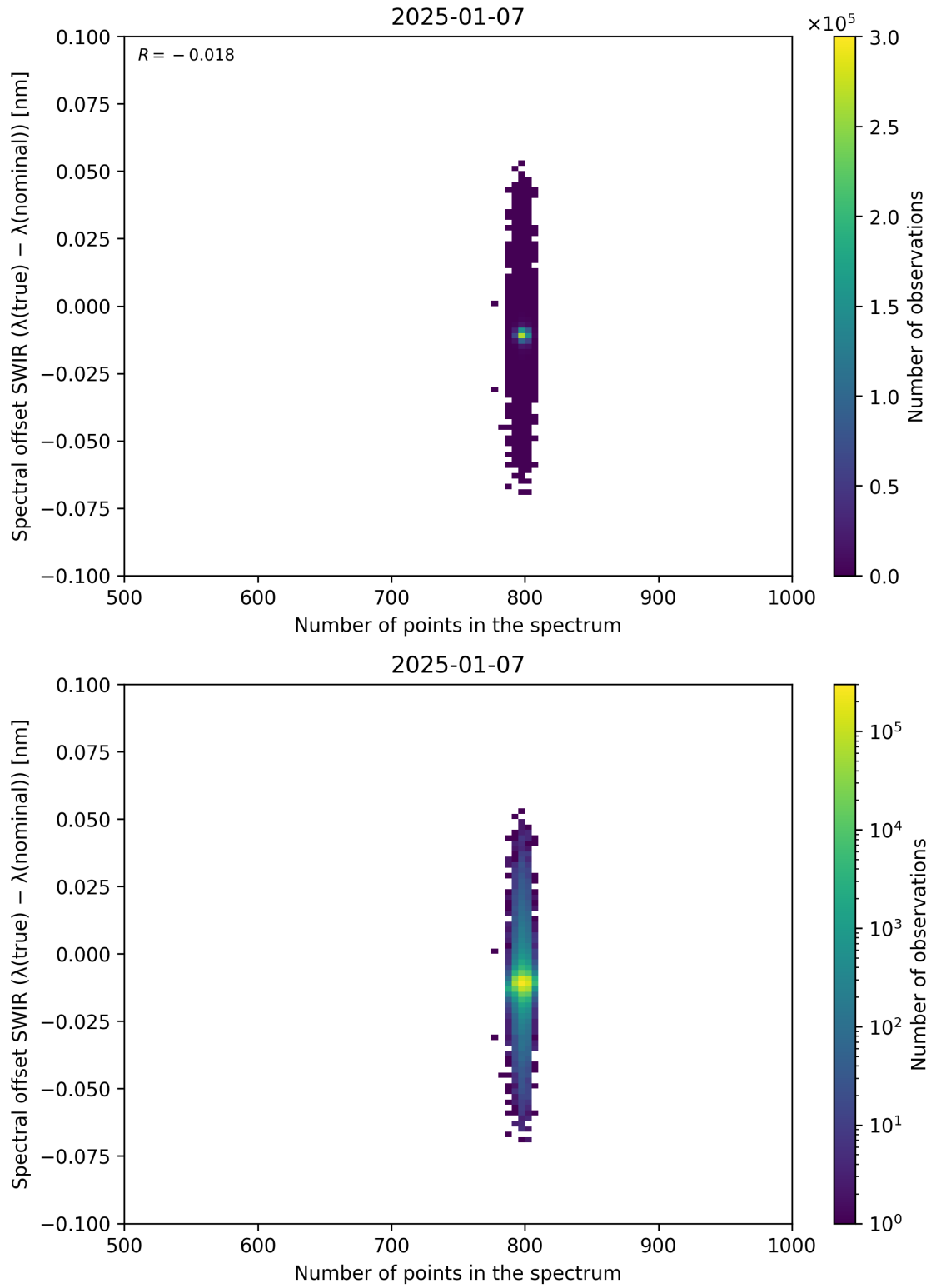
Figure 93: Scatter density plot of “Number of points in the spectrum” against “Spectral offset SWIR ( \lambda_{\text{true}} - \lambda_{\text{nominal}} )” for 2025-01-07 to 2025-01-08.
