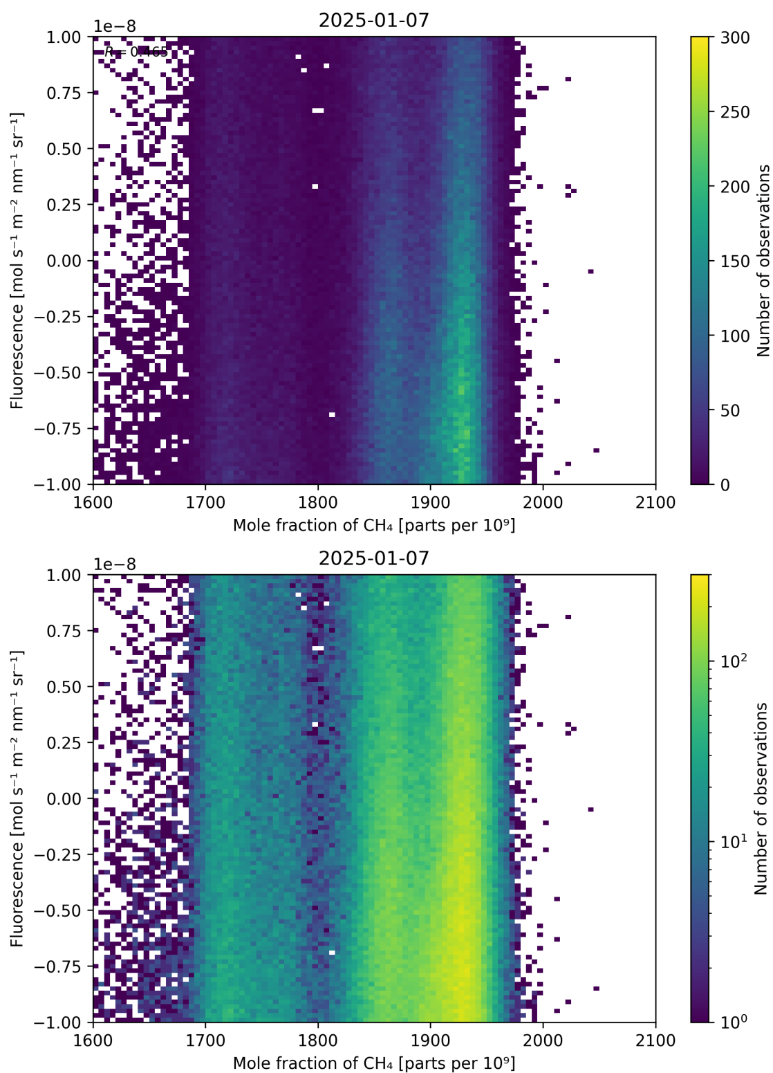
Figure 73: Scatter density plot of “Mole fraction of \text{CH}_4 ” against “Fluorescence” for 2025-01-07 to 2025-01-08.
