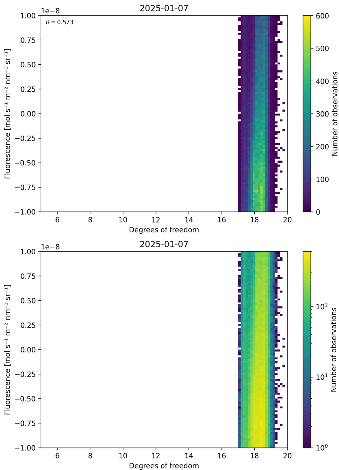
Figure 51: Scatter density plot of “Degrees of freedom” against “Fluorescence” for 2025-01-07 to 2025-01-08.
