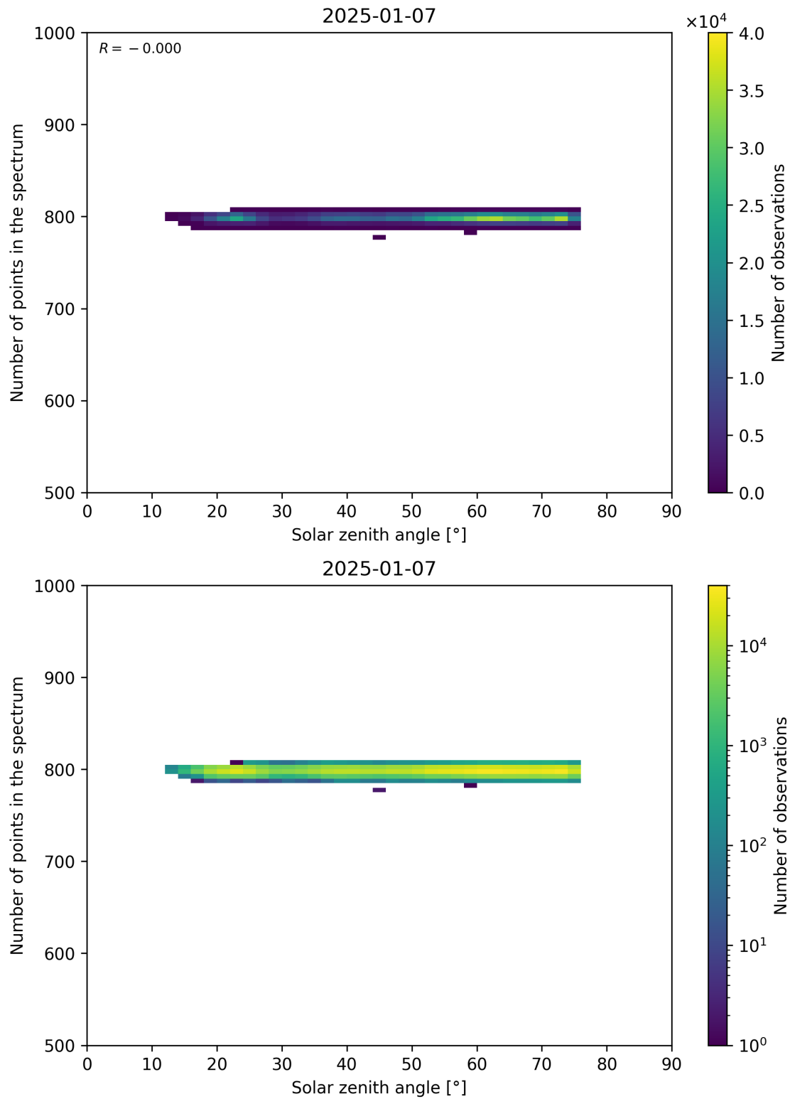
Figure 103: Scatter density plot of “Solar zenith angle” against “Number of points in the spectrum” for 2025-01-07 to 2025-01-08.
