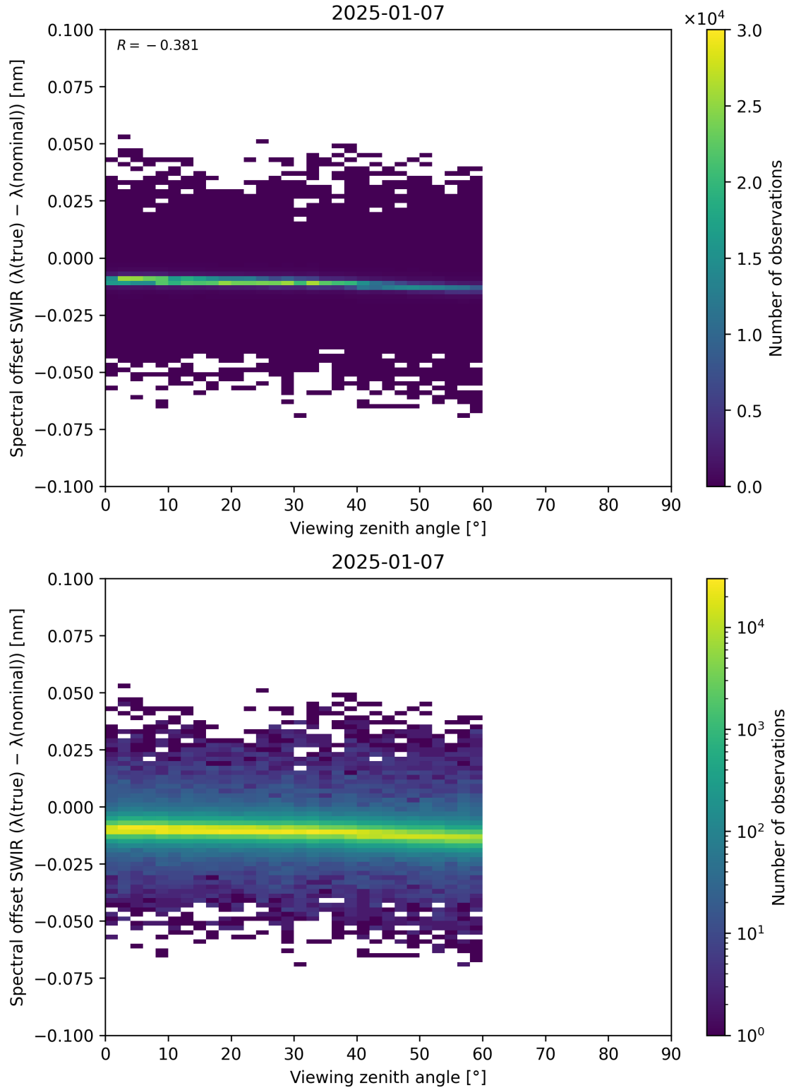
Figure 116: Scatter density plot of “Viewing zenith angle” against “Spectral offset SWIR ( \lambda_{\text{true}} - \lambda_{\text{nominal}} )” for 2025-01-07 to 2025-01-08.
