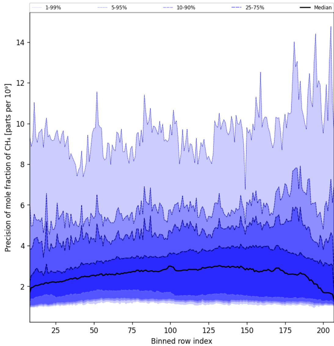
Figure 35: Along track statistics of “Precision of mole fraction of CH 4 ” for 2025-01-07 to 2025-01-08
