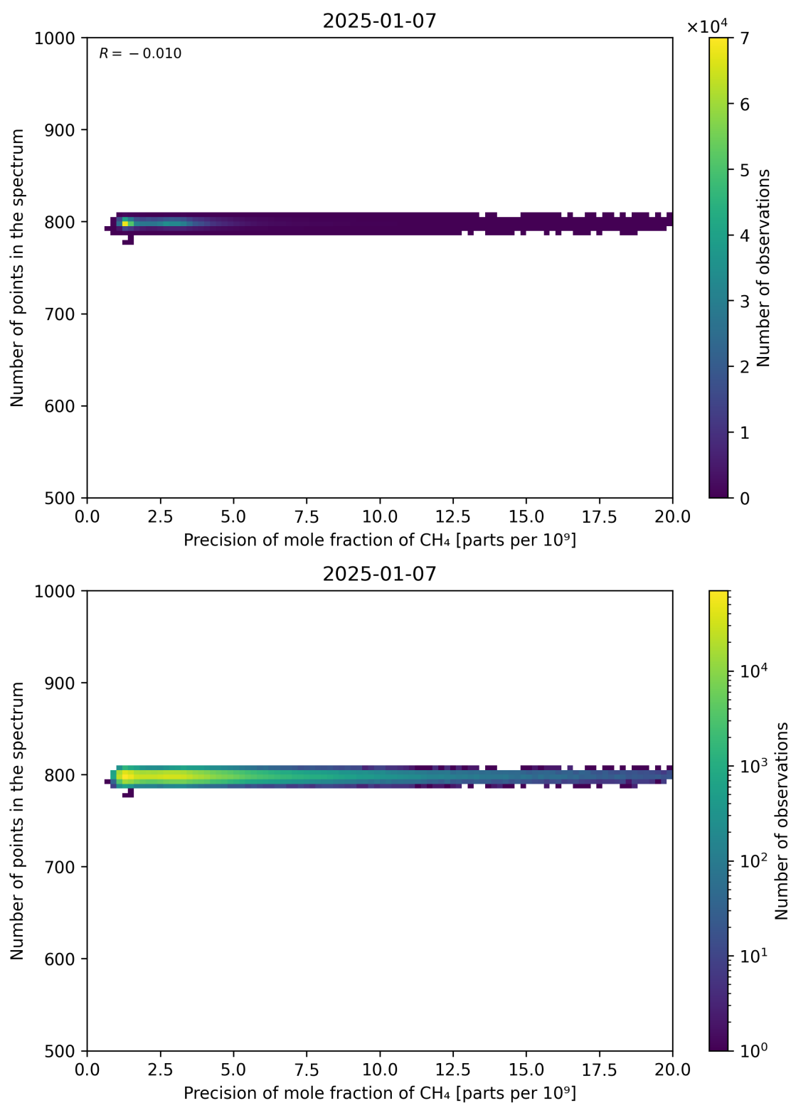
Figure 84: Scatter density plot of “Precision of mole fraction of CH 4 ” against “Number of points in the spectrum” for 2025-01-07 to 2025-01-08.
