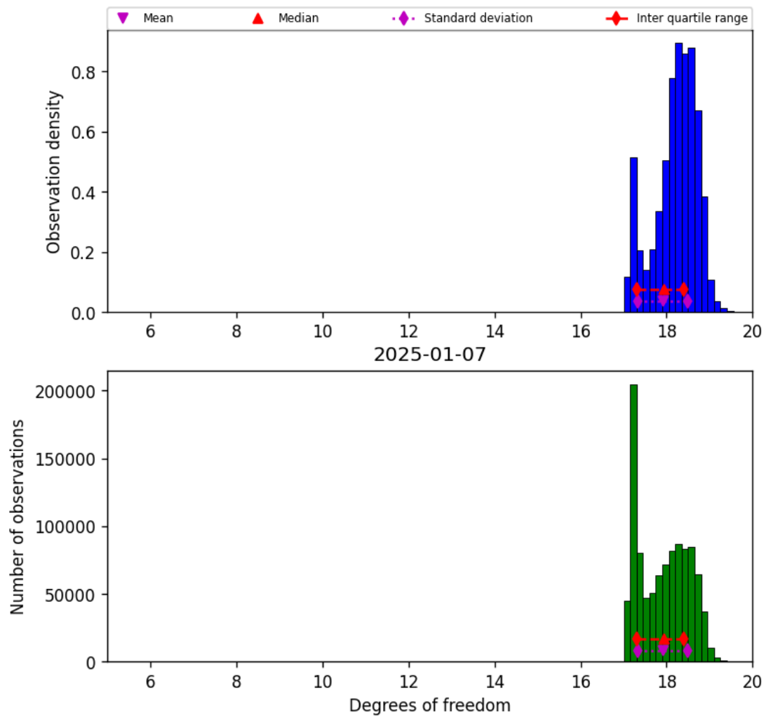
Figure 30: Histogram of “Degrees of freedom” for 2025-01-07 to 2025-01-08
