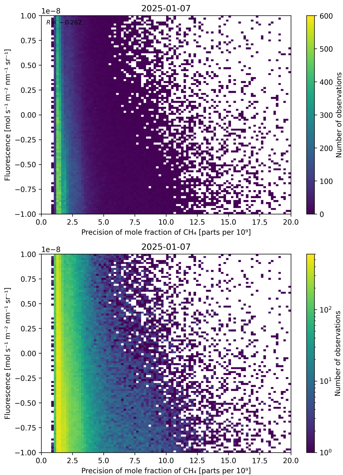
Figure 81: Scatter density plot of “Precision of mole fraction of CH 4 ” against “Fluorescence” for 2025-01-07 to 2025-01-08.
