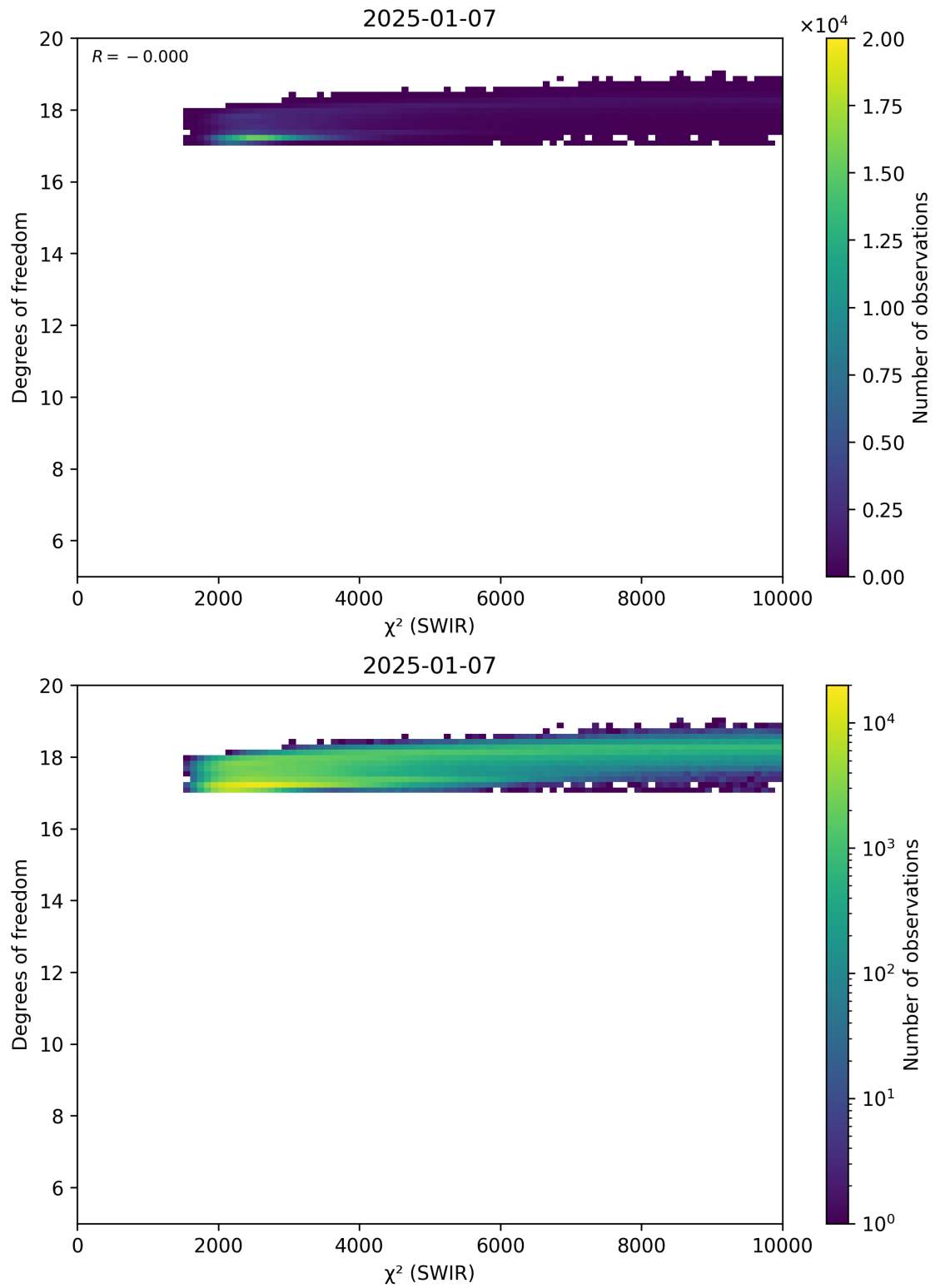
Figure 48: Scatter density plot of “ \chi^2 (SWIR)” against “Degrees of freedom” for 2025-01-07 to 2025-01-08.
