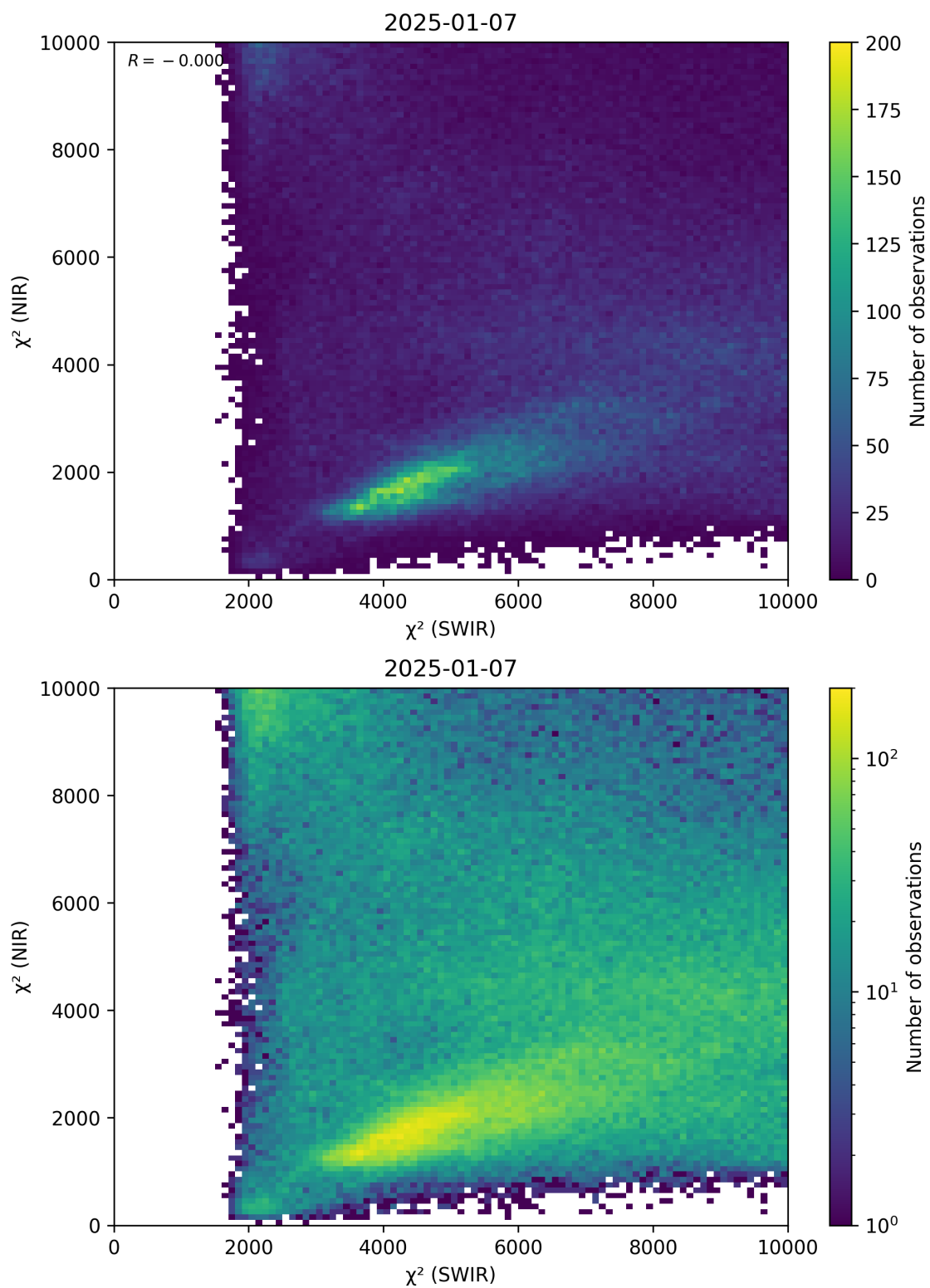
Figure 47: Scatter density plot of “ \chi^2 (SWIR)” against “ \chi^2 (NIR)” for 2025-01-07 to 2025-01-08.
