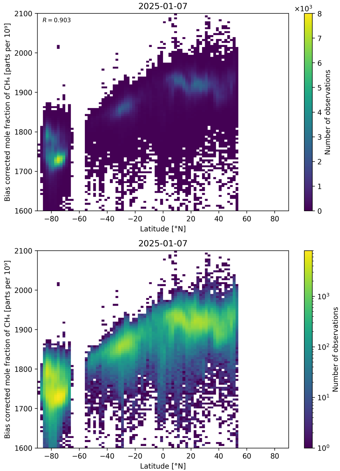
Figure 58: Scatter density plot of “Latitude” against “Bias corrected mole fraction of CH 4 ” for 2025-01-07 to 2025-01-08.
