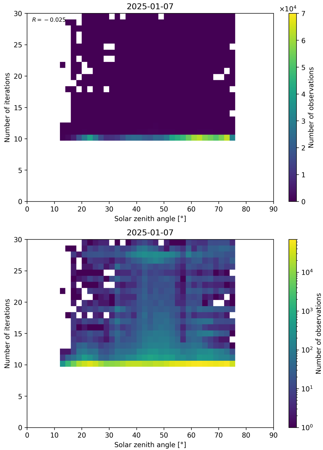
Figure 102: Scatter density plot of “Solar zenith angle” against “Number of iterations” for 2025-01-07 to 2025-01-08.
