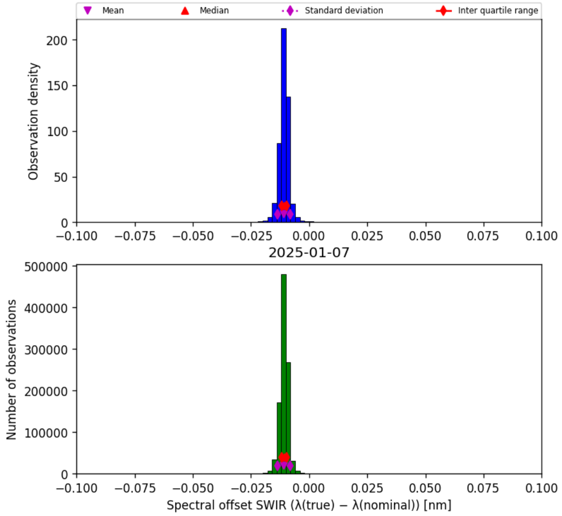
Figure 27: Histogram of “Spectral offset SWIR ( \lambda_{\text{true}} - \lambda_{\text{nominal}} )” for 2025-01-07 to 2025-01-08
