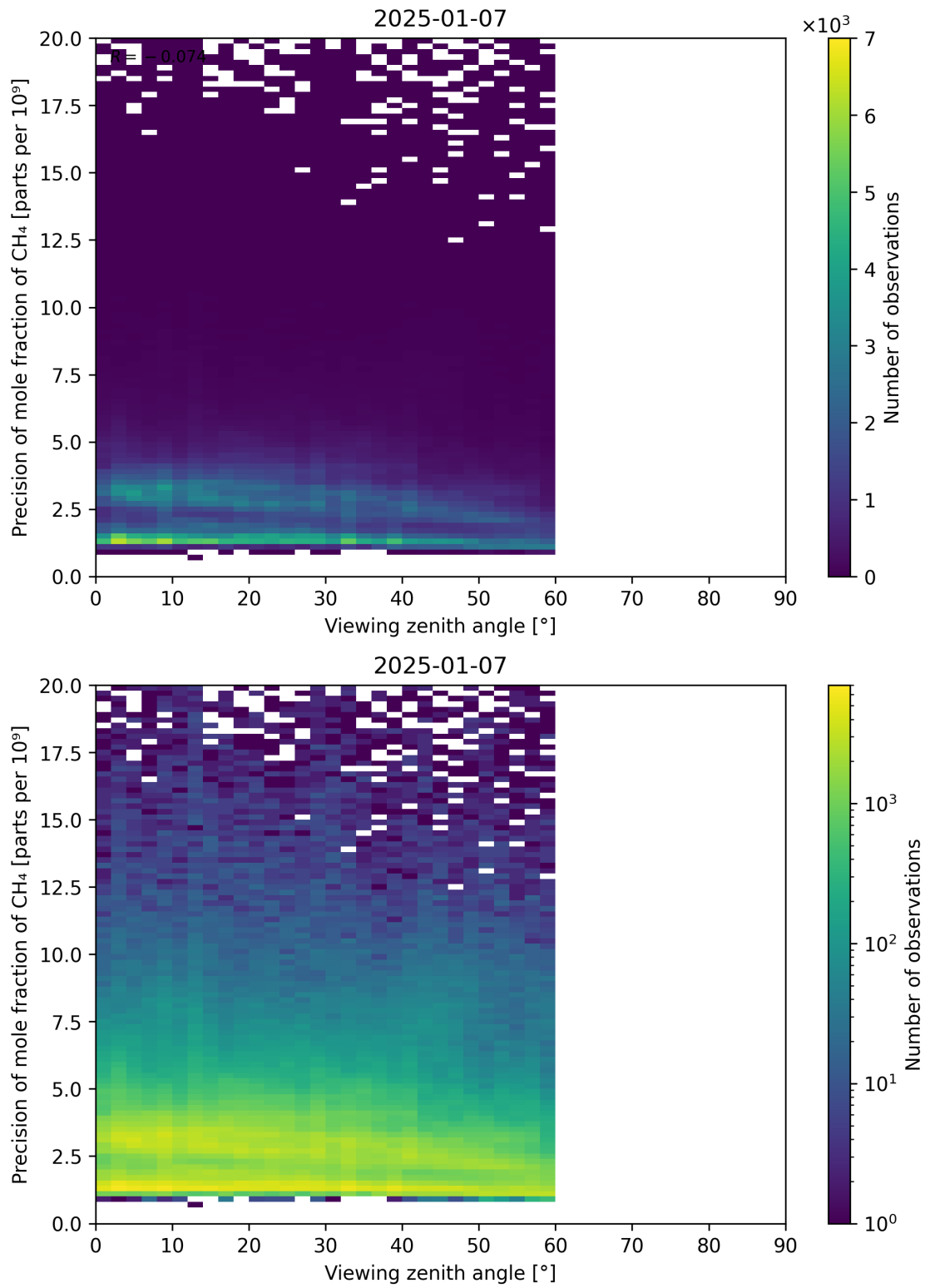
Figure 112: Scatter density plot of “Viewing zenith angle” against “Precision of mole fraction of CH 4 ” for 2025-01-07 to 2025-01-08.
