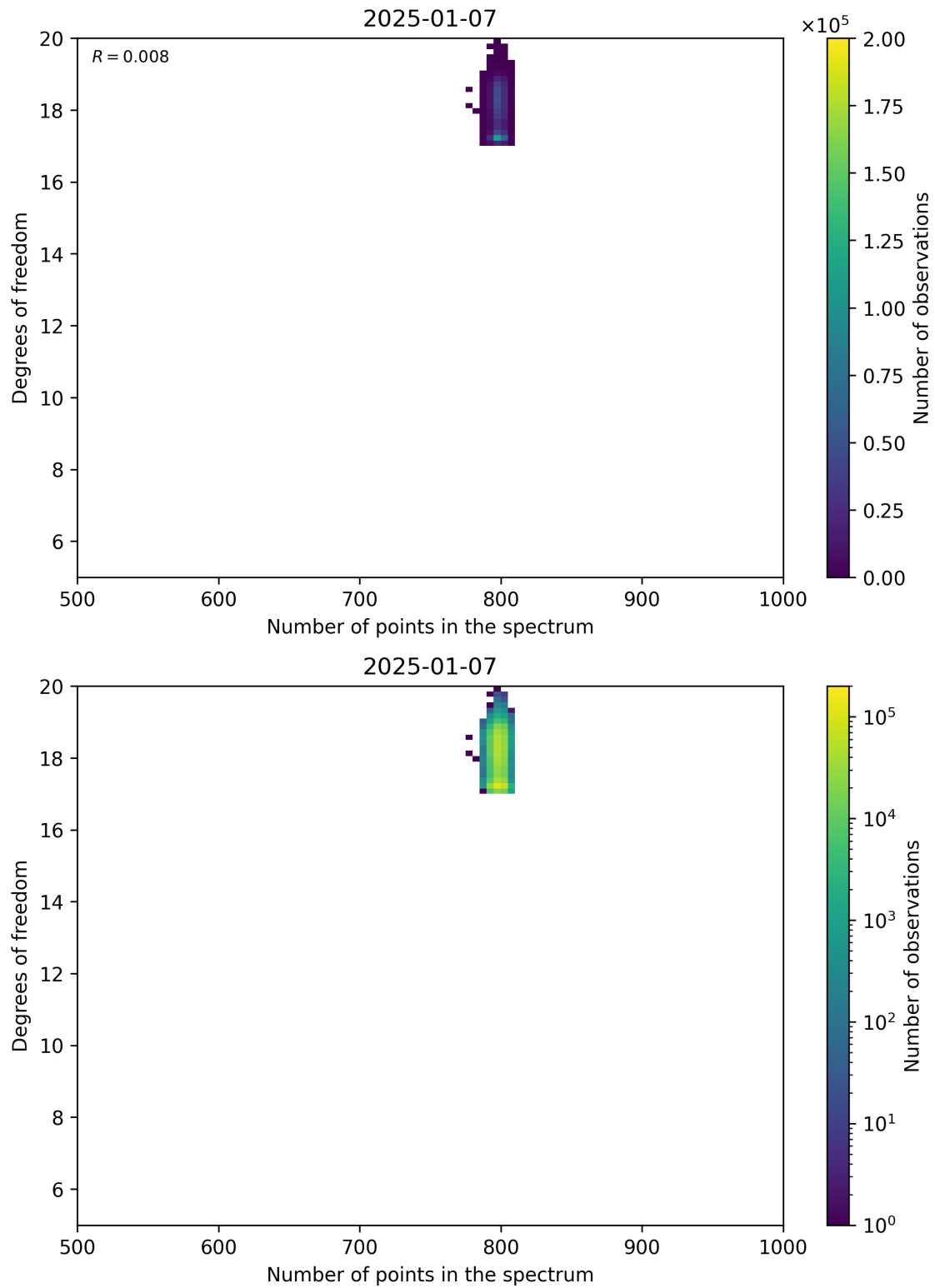
Figure 90: Scatter density plot of “Number of points in the spectrum” against “Degrees of freedom” for 2025-01-07 to 2025-01-08.
