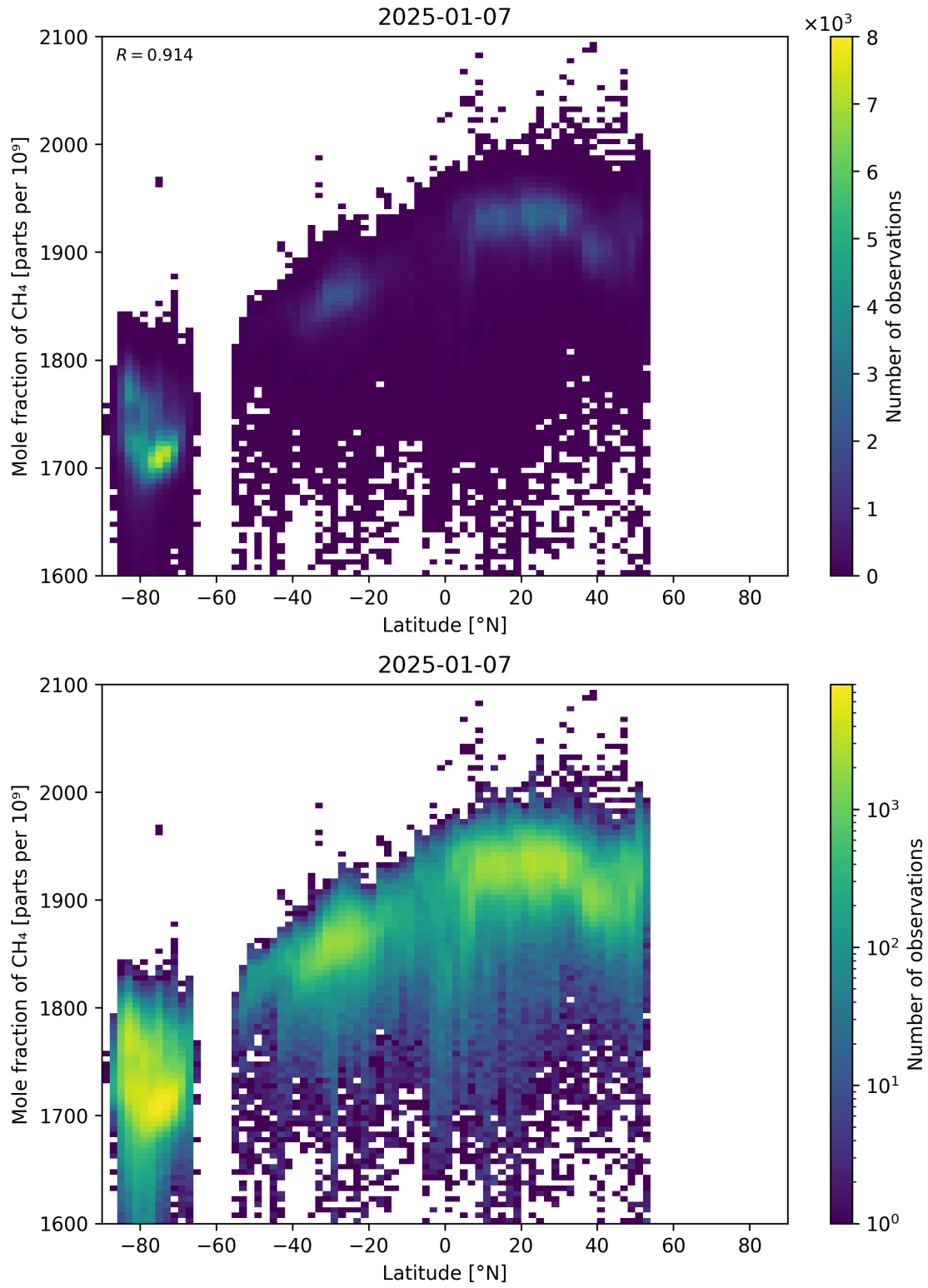
Figure 57: Scatter density plot of “Latitude” against “Mole fraction of CH 4 ” for 2025-01-07 to 2025-01-08.
