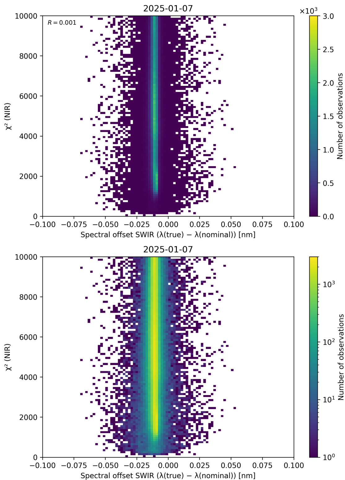
Figure 117: Scatter density plot of “Spectral offset SWIR ( \lambda_{\text{true}} - \lambda_{\text{nominal}} )” against “ \chi^2 (NIR)” for 2025-01-07 to 2025-01-08.
