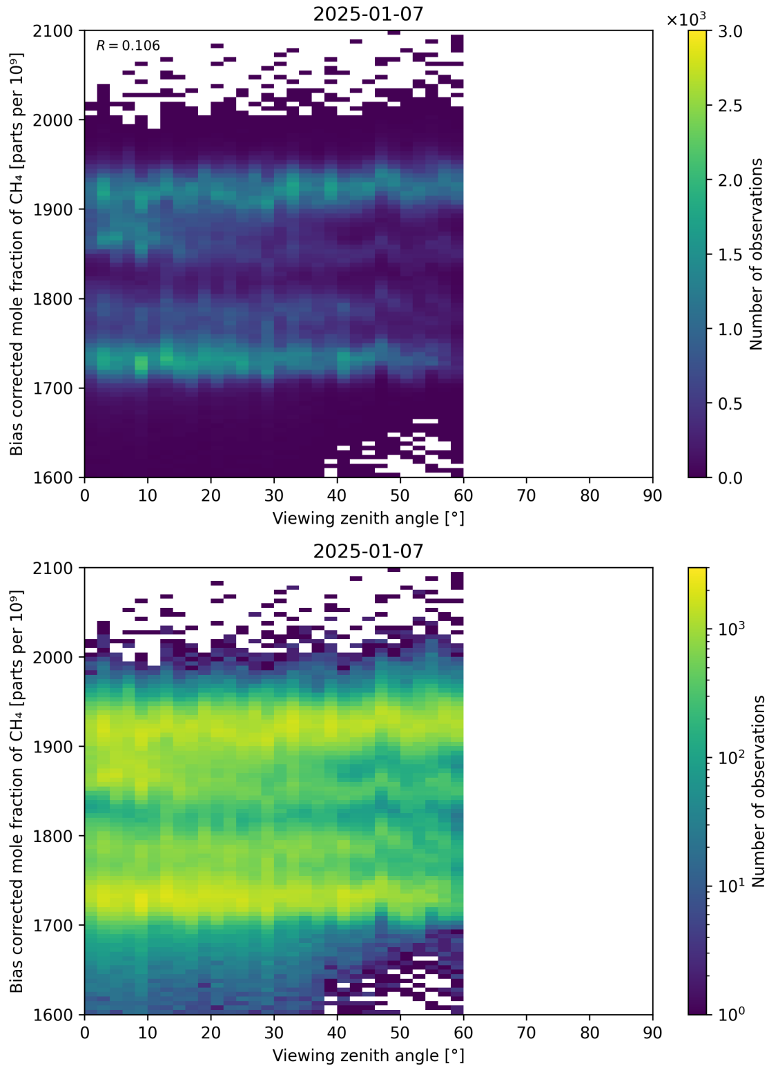
Figure 111: Scatter density plot of “Viewing zenith angle” against “Bias corrected mole fraction of CH 4 ” for 2025-01-07 to 2025-01-08.
