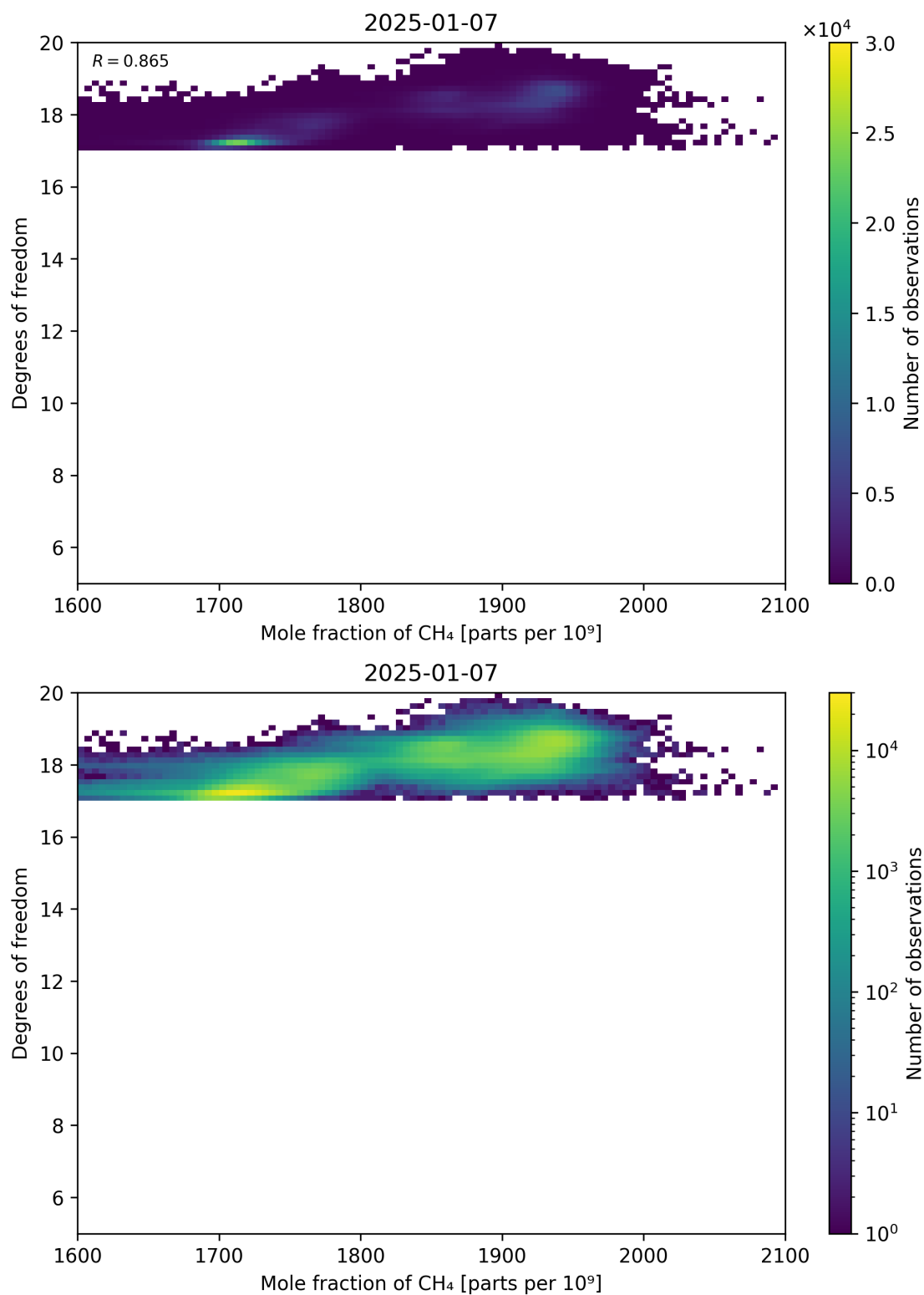
Figure 72: Scatter density plot of “Mole fraction of CH 4 ” against “Degrees of freedom” for 2025-01-07 to 2025-01-08.
