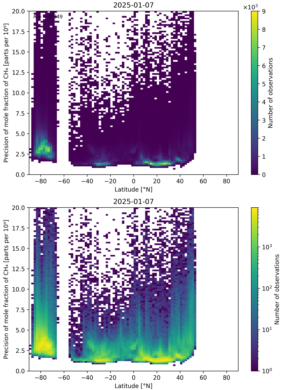
Figure 59: Scatter density plot of “Latitude” against “Precision of mole fraction of CH 4 ” for 2025-01-07 to 2025-01-08.
