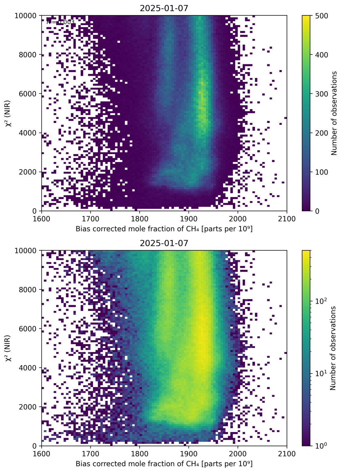
Figure 63: Scatter density plot of “Bias corrected mole fraction of \text{CH}_4 ” against “ \chi^2 (NIR)” for 2025-01-07 to 2025-01-08.
