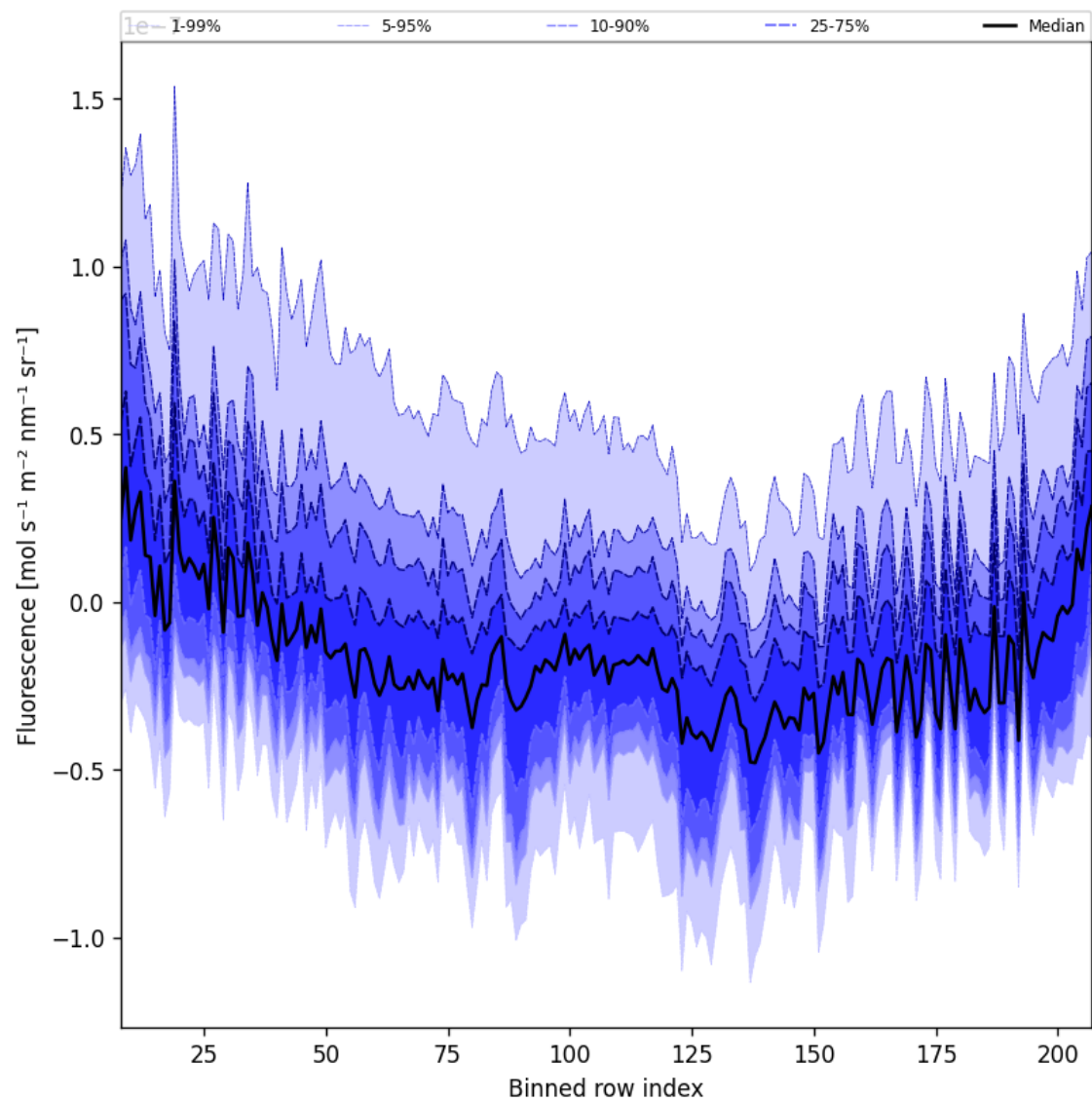
Figure 43: Along track statistics of “Fluorescence” for 2025-01-07 to 2025-01-08
