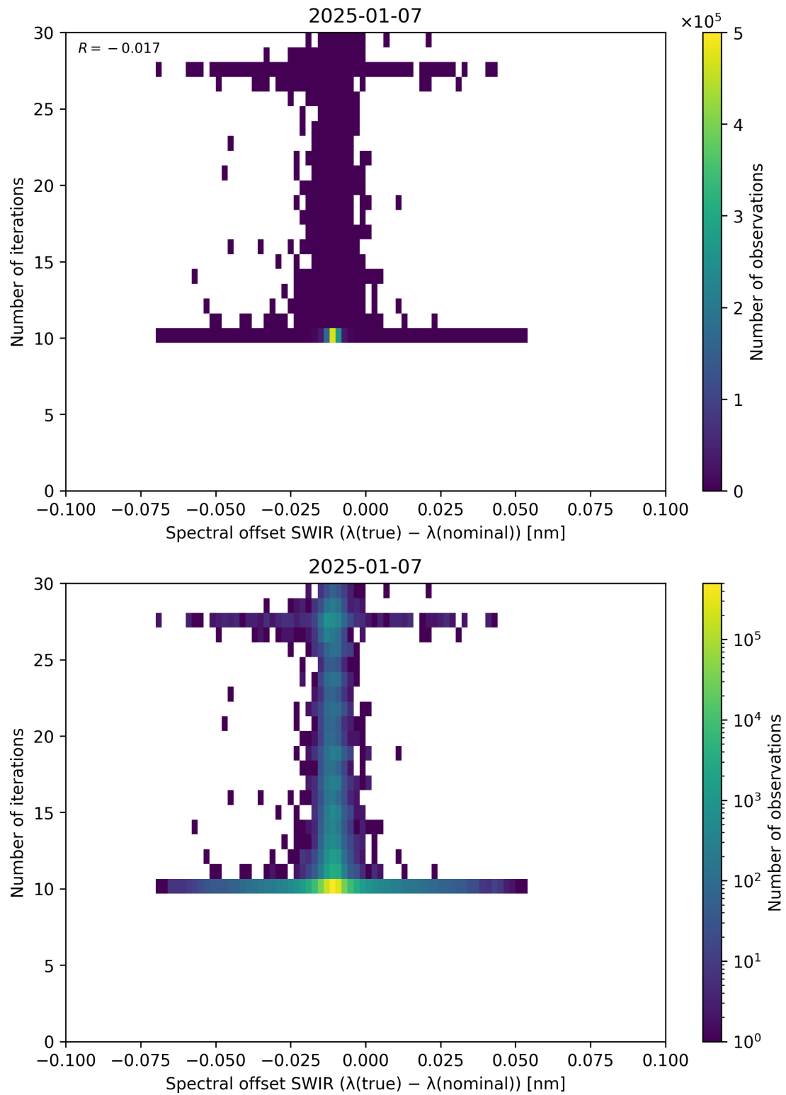
Figure 121: Scatter density plot of “Spectral offset SWIR ( \lambda_{\text{true}} - \lambda_{\text{nominal}} )” against “Number of iterations” for 2025-01-07 to 2025-01-08.
