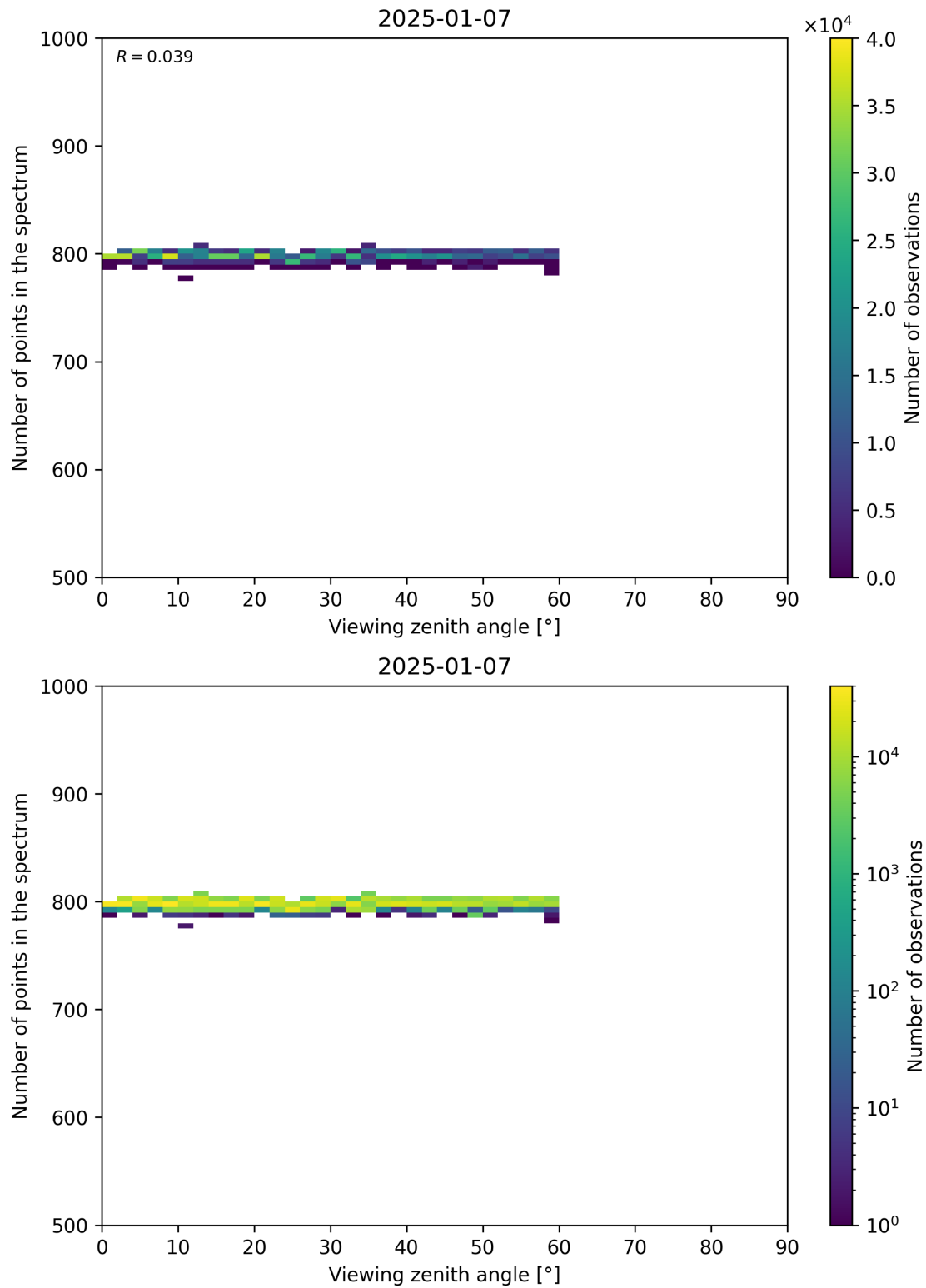
Figure 114: Scatter density plot of “Viewing zenith angle” against “Number of points in the spectrum” for 2025-01-07 to 2025-01-08.
