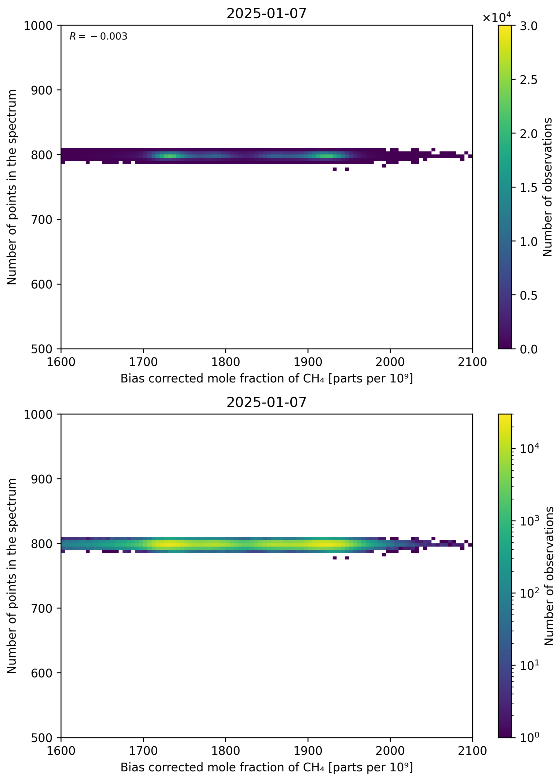
Figure 68: Scatter density plot of “Bias corrected mole fraction of CH 4 ” against “Number of points in the spectrum” for 2025-01-07 to 2025-01-08.
