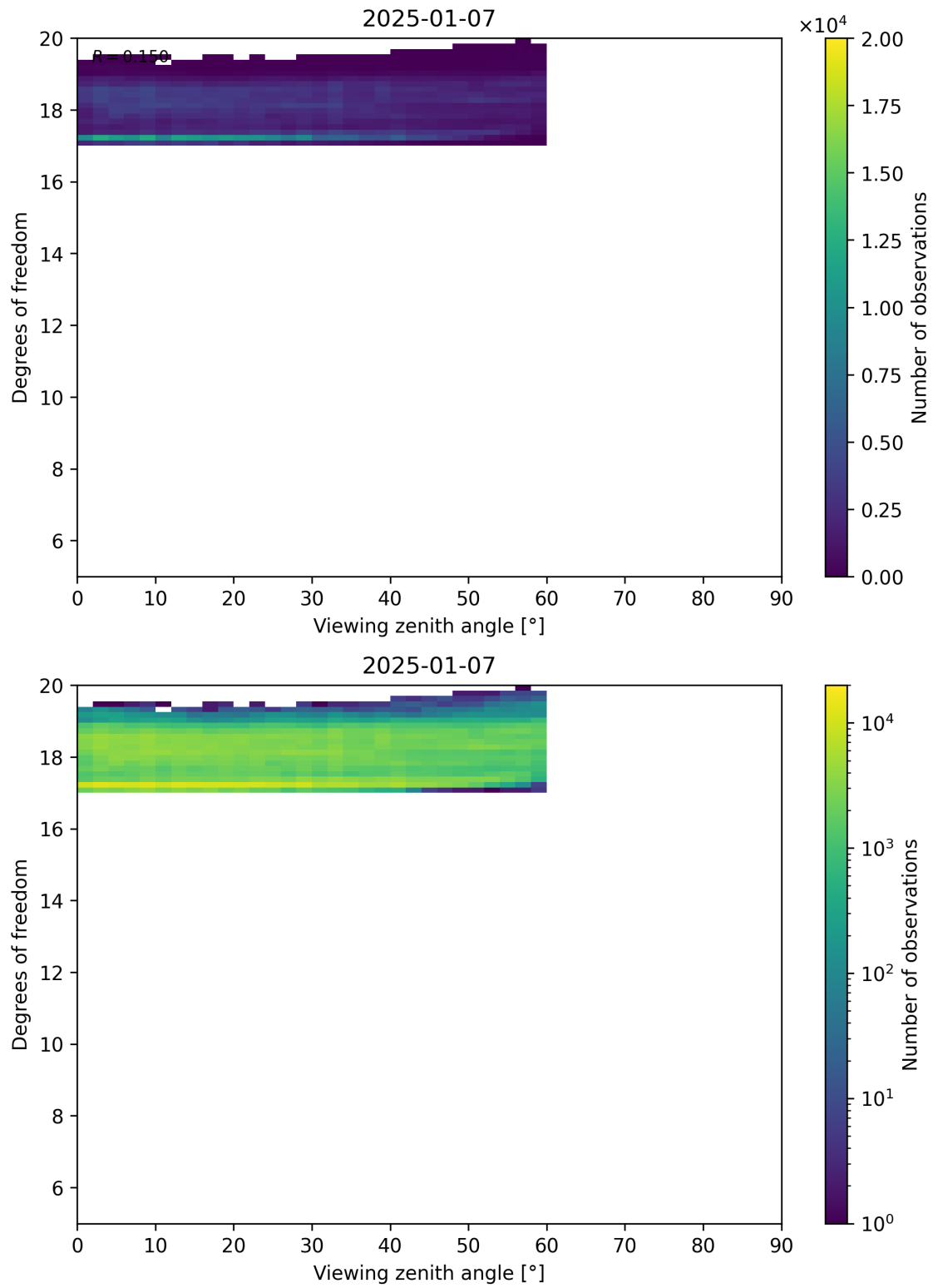
Figure 107: Scatter density plot of “Viewing zenith angle” against “Degrees of freedom” for 2025-01-07 to 2025-01-08.
