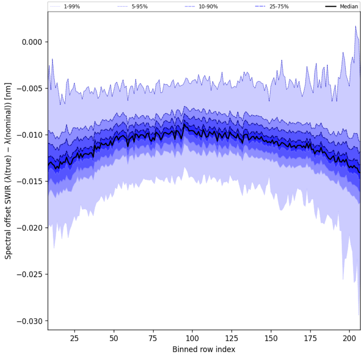
Figure 38: Along track statistics of “Spectral offset SWIR ( \lambda_{\text{true}} - \lambda_{\text{nominal}} )” for 2025-01-07 to 2025-01-08
