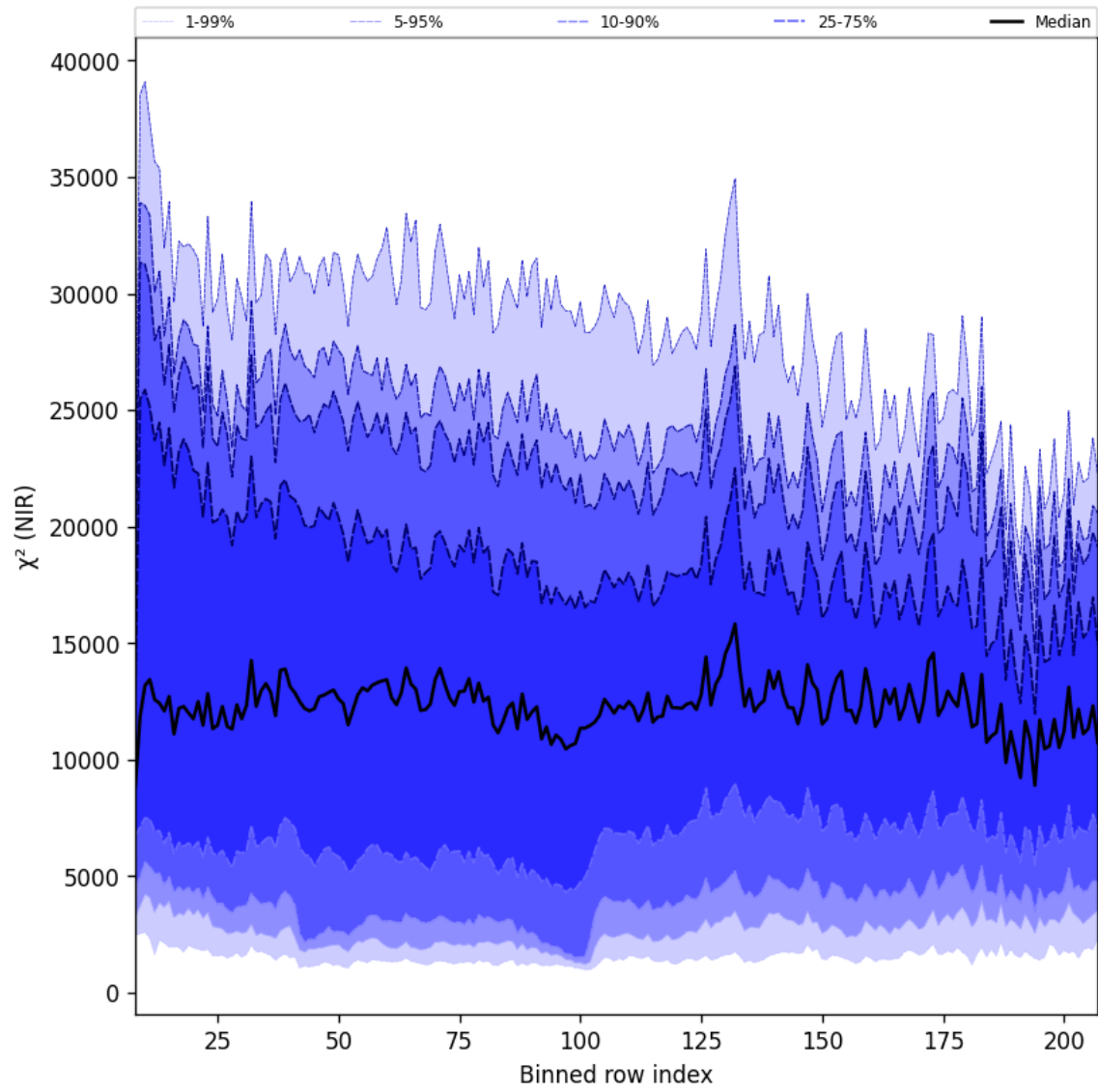
Figure 40: Along track statistics of " \chi^2 (NIR)" for 2025-01-07 to 2025-01-08
