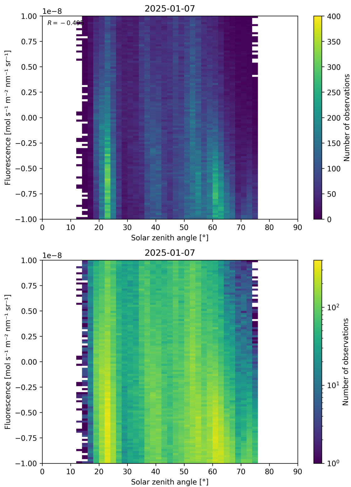
Figure 97: Scatter density plot of “Solar zenith angle” against “Fluorescence” for 2025-01-07 to 2025-01-08.
