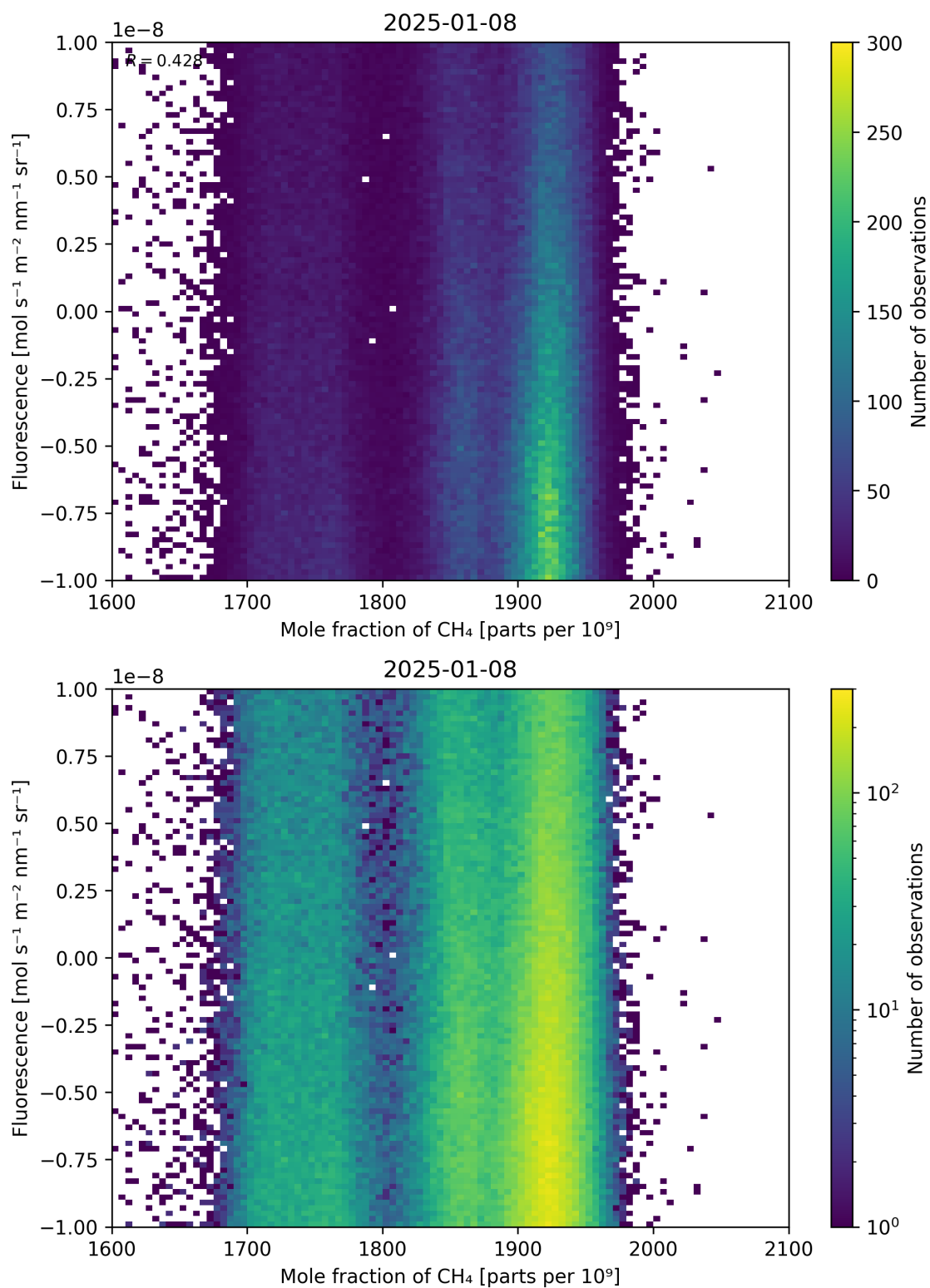
Figure 73: Scatter density plot of “Mole fraction of \text{CH}_4 ” against “Fluorescence” for 2025-01-07 to 2025-01-09.
