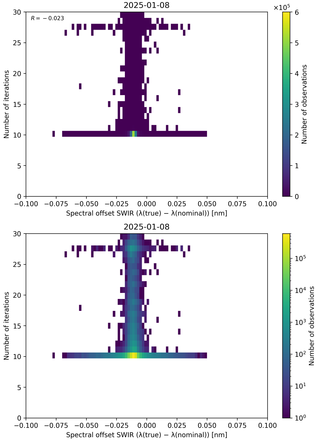
Figure 121: Scatter density plot of “Spectral offset SWIR ( \lambda_{\text{true}} - \lambda_{\text{nominal}} )” against “Number of iterations” for 2025-01-07 to 2025-01-09.
