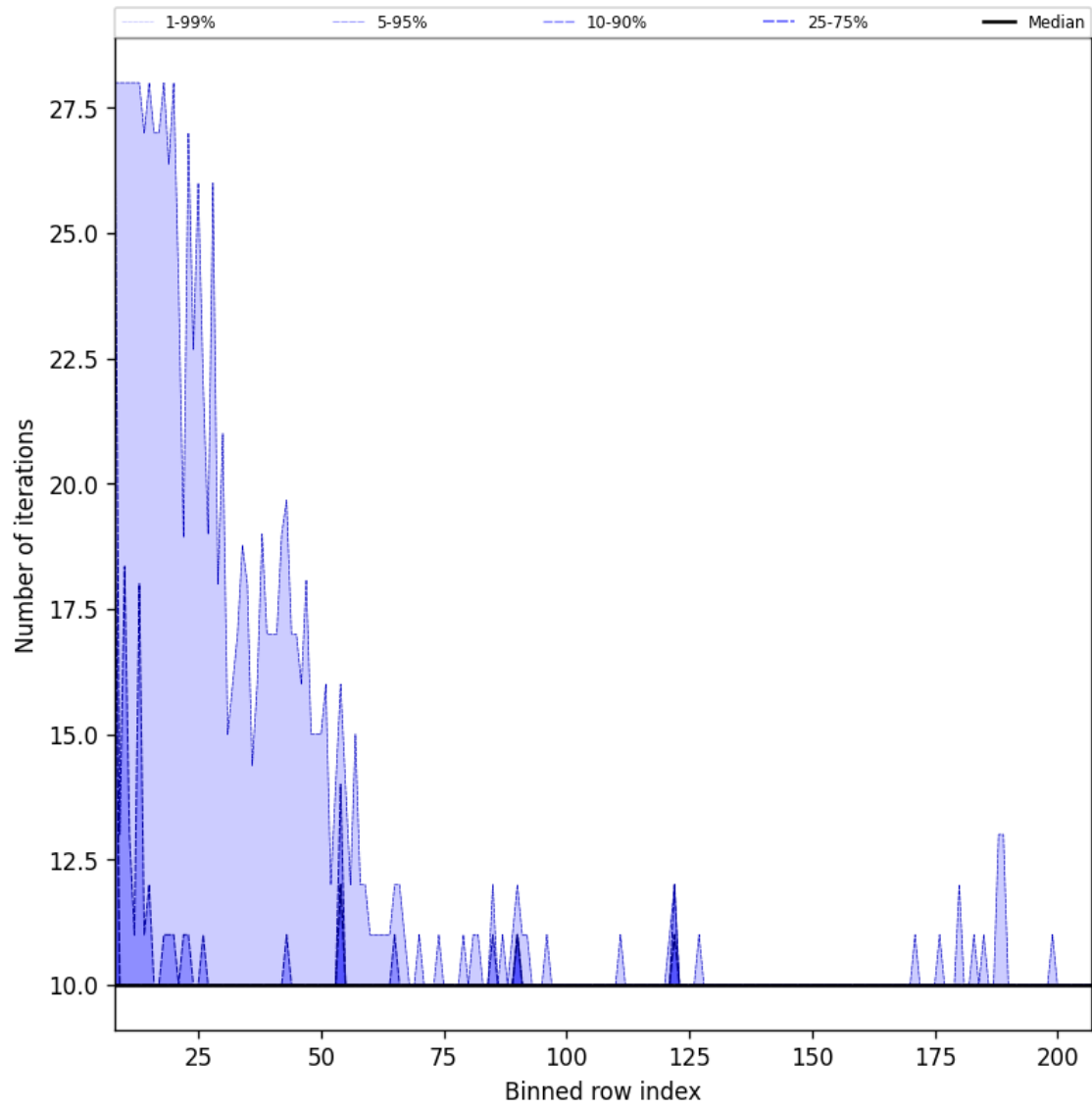
Figure 42: Along track statistics of “Number of iterations” for 2025-01-07 to 2025-01-09
