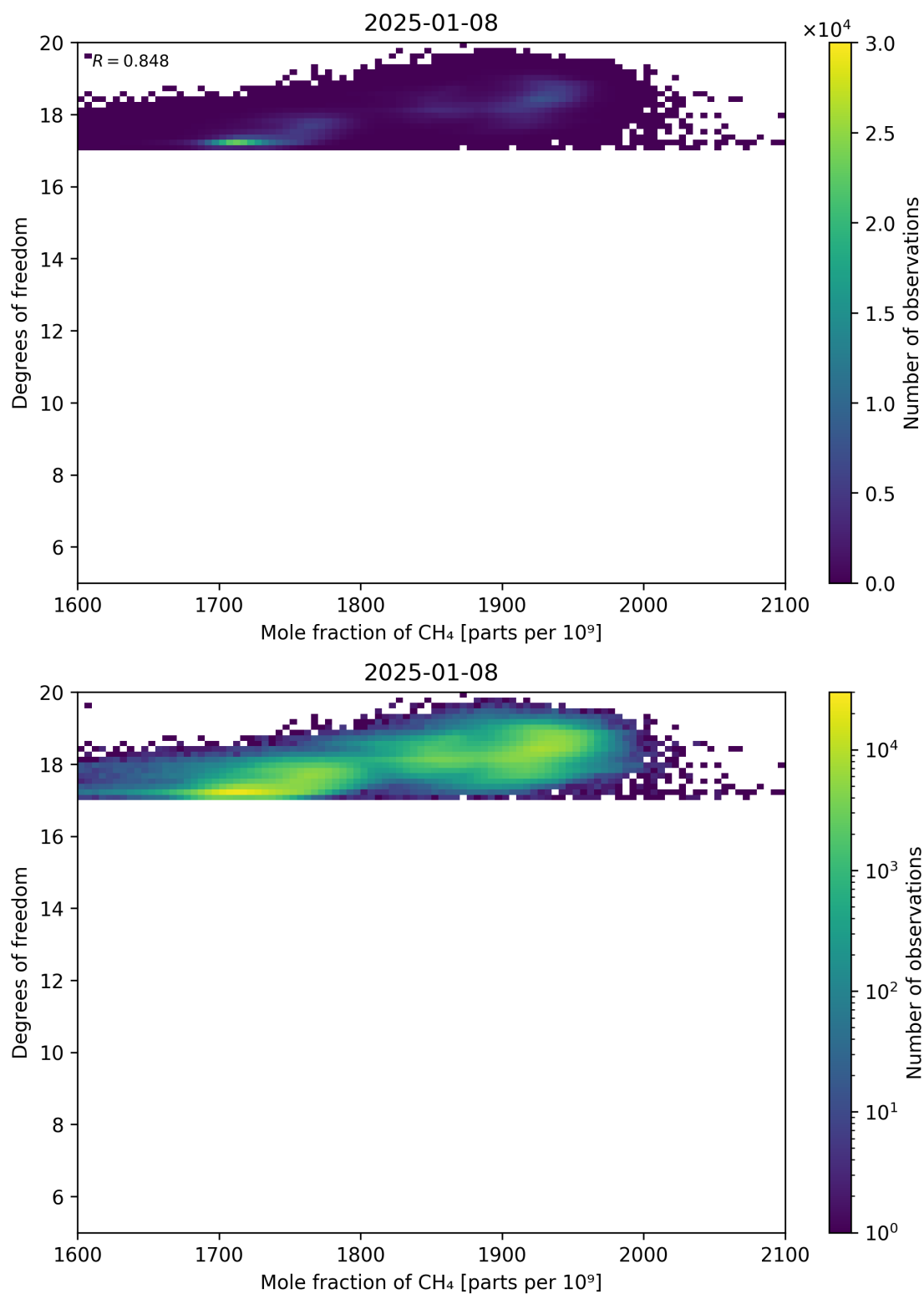
Figure 72: Scatter density plot of “Mole fraction of CH 4 ” against “Degrees of freedom” for 2025-01-07 to 2025-01-09.
