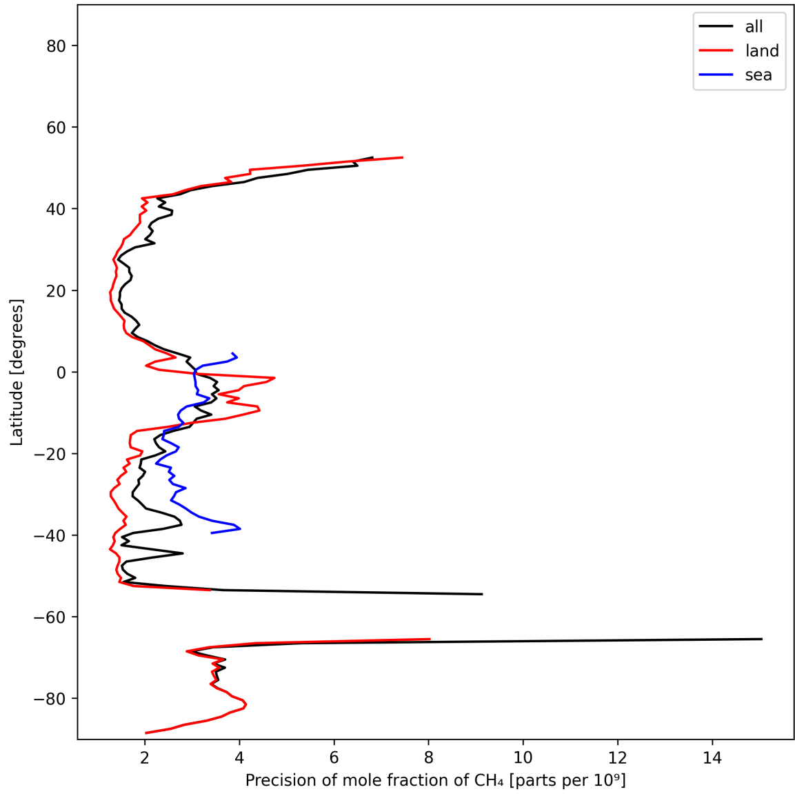
Figure 13: Zonal average of “Precision of mole fraction of CH 4 ” for 2025-01-07 to 2025-01-09.
