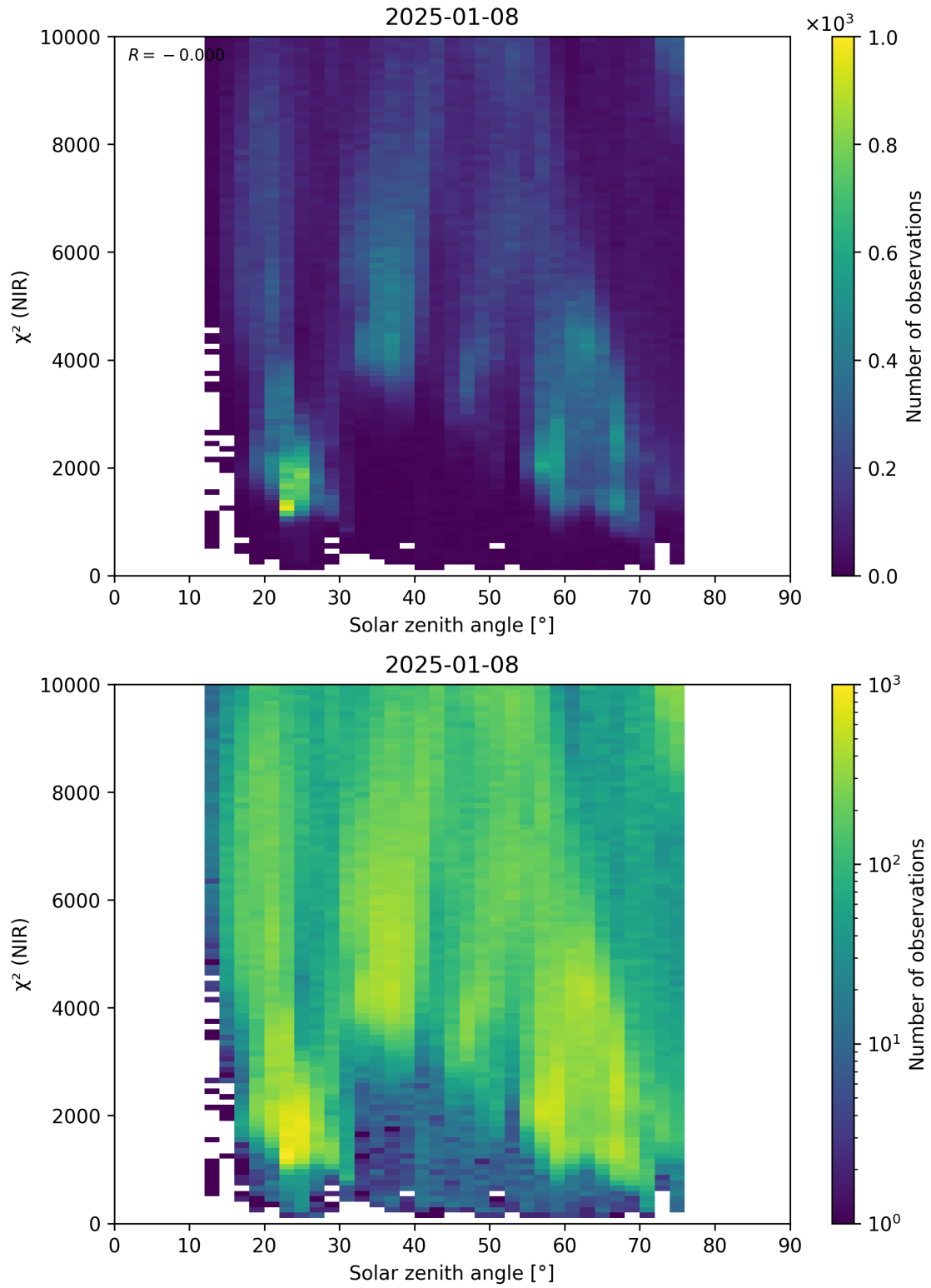
Figure 94: Scatter density plot of “Solar zenith angle” against “ \chi^2 (NIR)” for 2025-01-07 to 2025-01-09.
