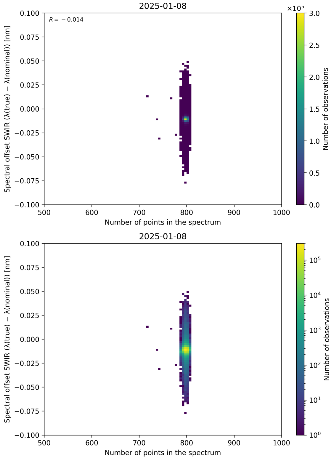
Figure 93: Scatter density plot of “Number of points in the spectrum” against “Spectral offset SWIR ( \lambda_{\text{true}} - \lambda_{\text{nominal}} )” for 2025-01-07 to 2025-01-09.
