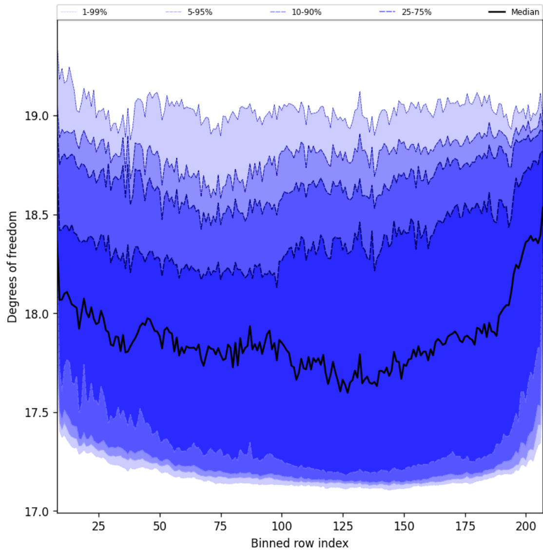
Figure 41: Along track statistics of “Degrees of freedom” for 2025-01-07 to 2025-01-09
