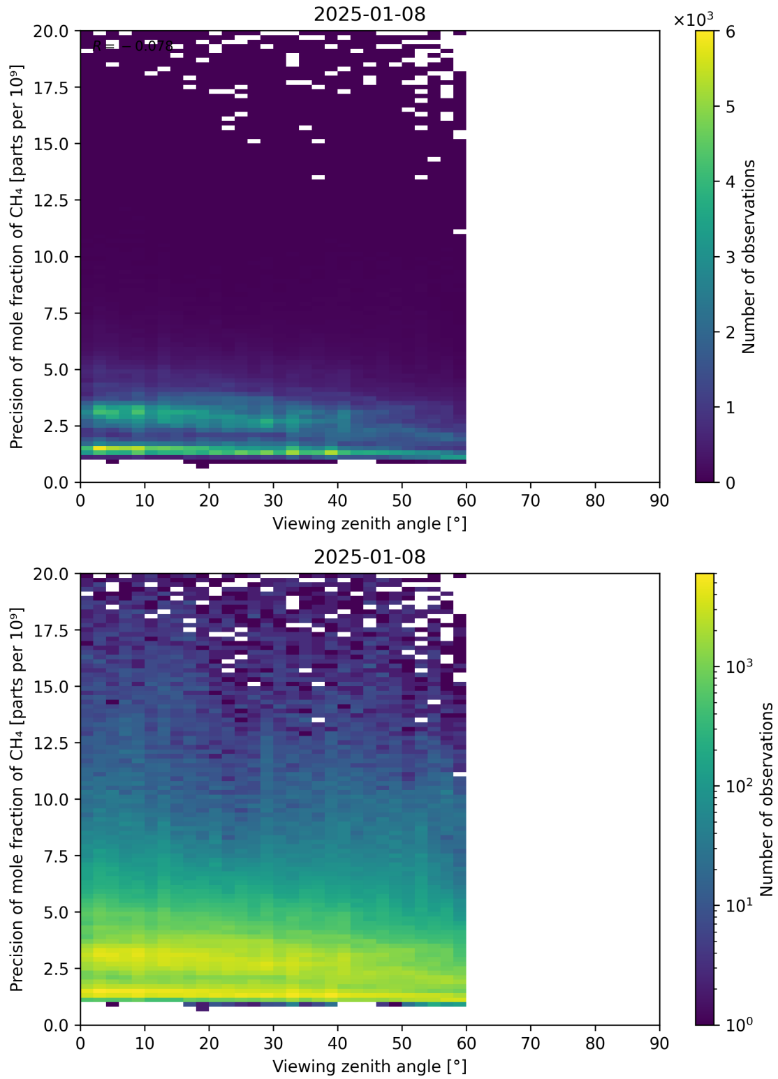
Figure 112: Scatter density plot of “Viewing zenith angle” against “Precision of mole fraction of CH 4 ” for 2025-01-07 to 2025-01-09.
