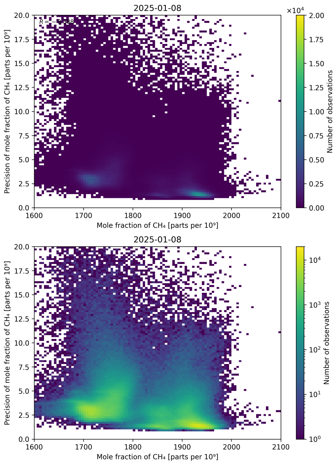
Figure 75: Scatter density plot of “Mole fraction of CH 4 ” against “Precision of mole fraction of CH 4 ” for 2025-01-07 to 2025-01-09.
