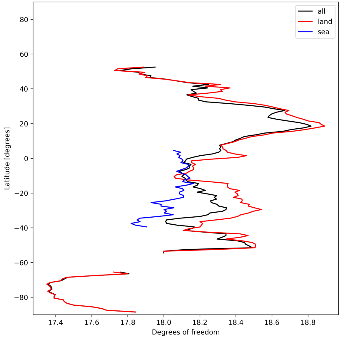
Figure 19: Zonal average of “Degrees of freedom” for 2025-01-07 to 2025-01-09.
