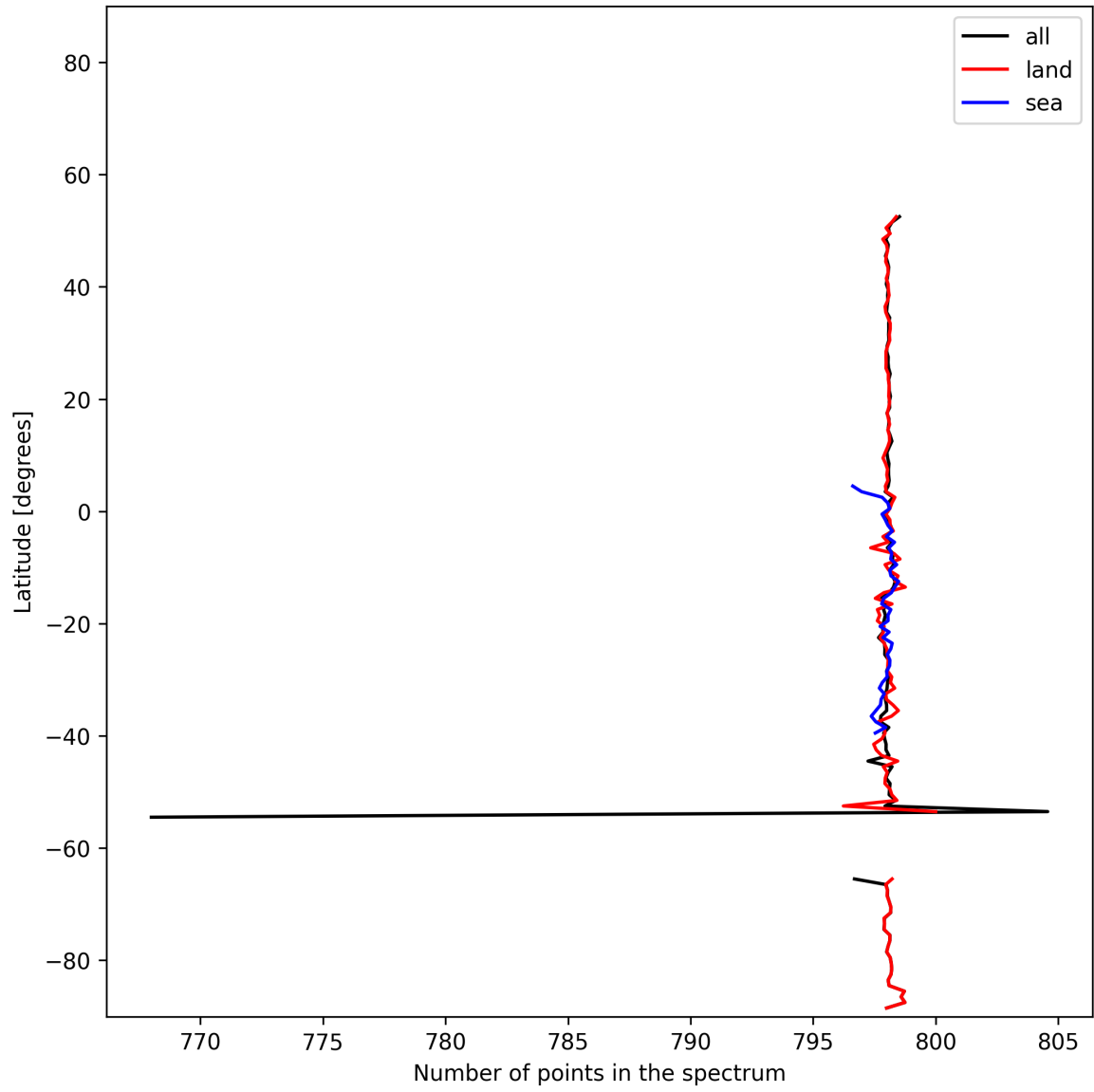
Figure 15: Zonal average of “Number of points in the spectrum” for 2025-01-07 to 2025-01-09.
