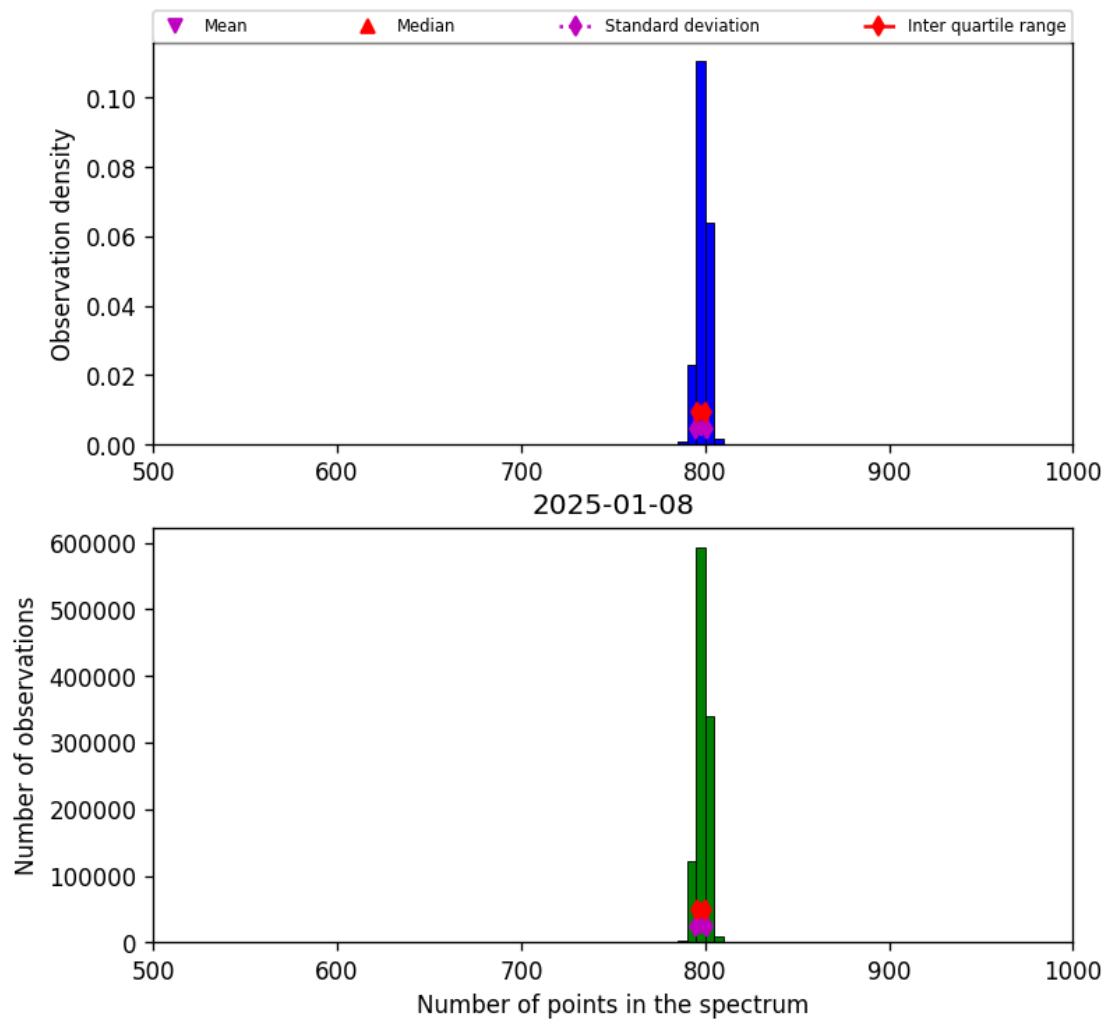
Figure 26: Histogram of “Number of points in the spectrum” for 2025-01-07 to 2025-01-09
