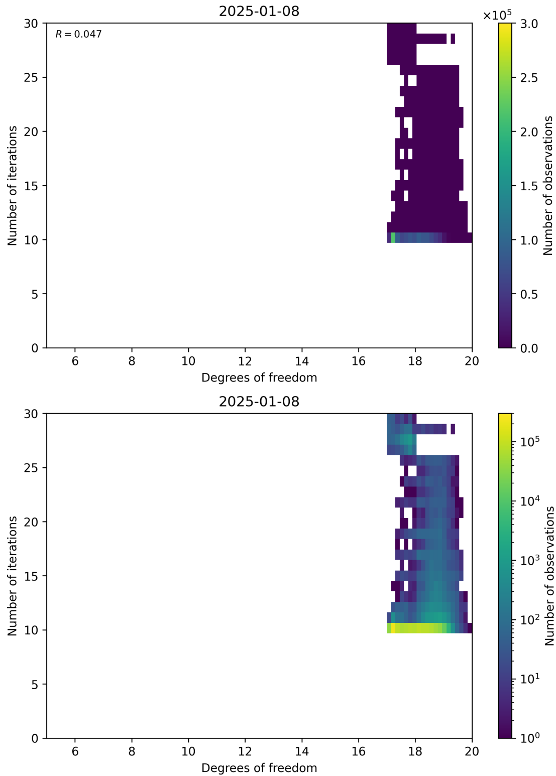
Figure 52: Scatter density plot of “Degrees of freedom” against “Number of iterations” for 2025-01-07 to 2025-01-09.
