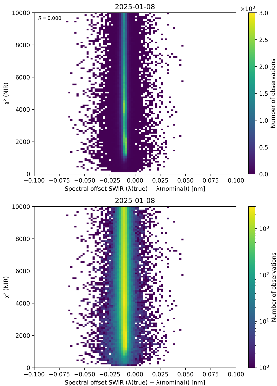
Figure 117: Scatter density plot of “Spectral offset SWIR ( \lambda_{\text{true}} - \lambda_{\text{nominal}} )” against “ \chi^2 (NIR)” for 2025-01-07 to 2025-01-09.
