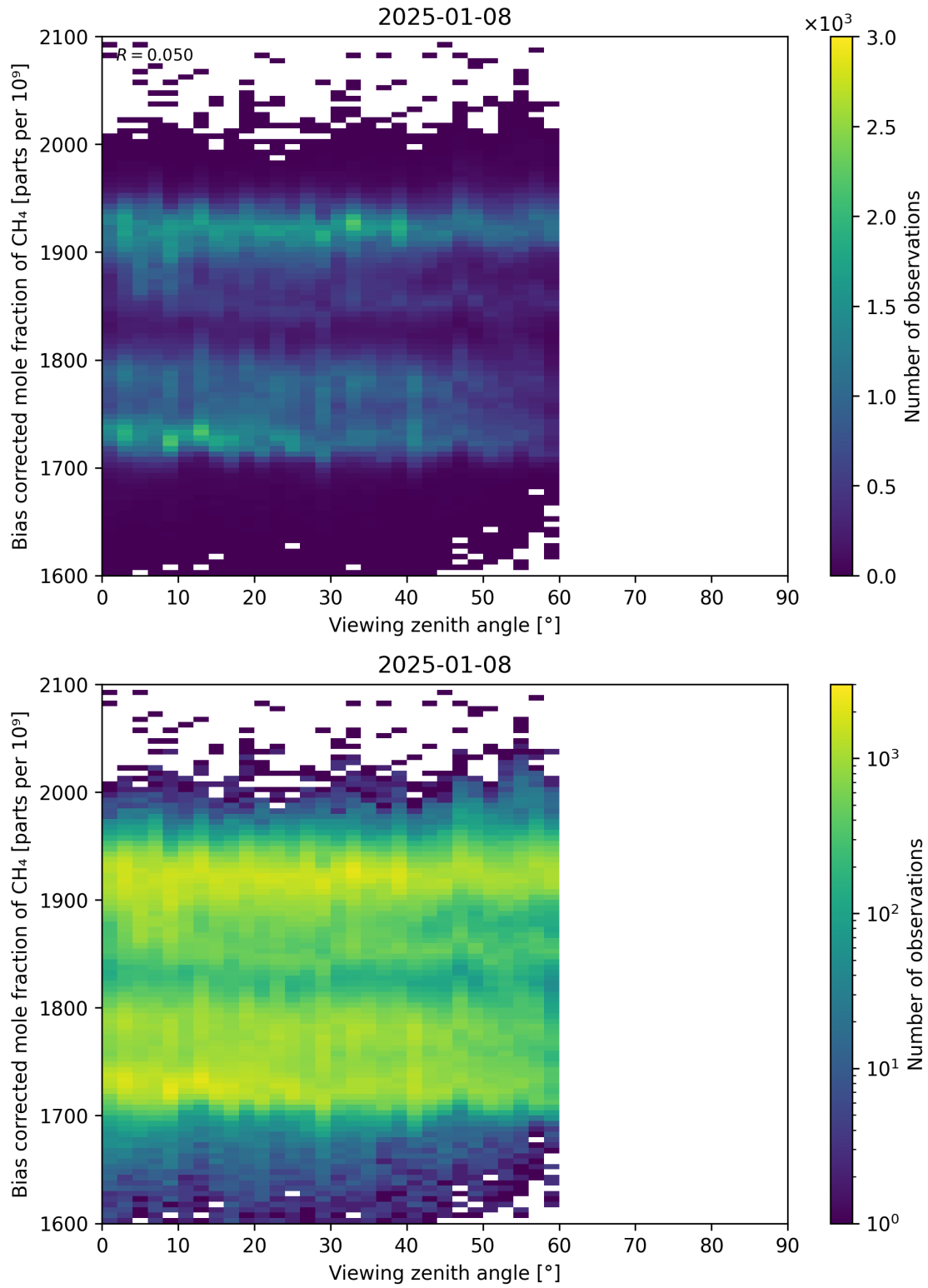
Figure 111: Scatter density plot of “Viewing zenith angle” against “Bias corrected mole fraction of CH 4 ” for 2025-01-07 to 2025-01-09.
