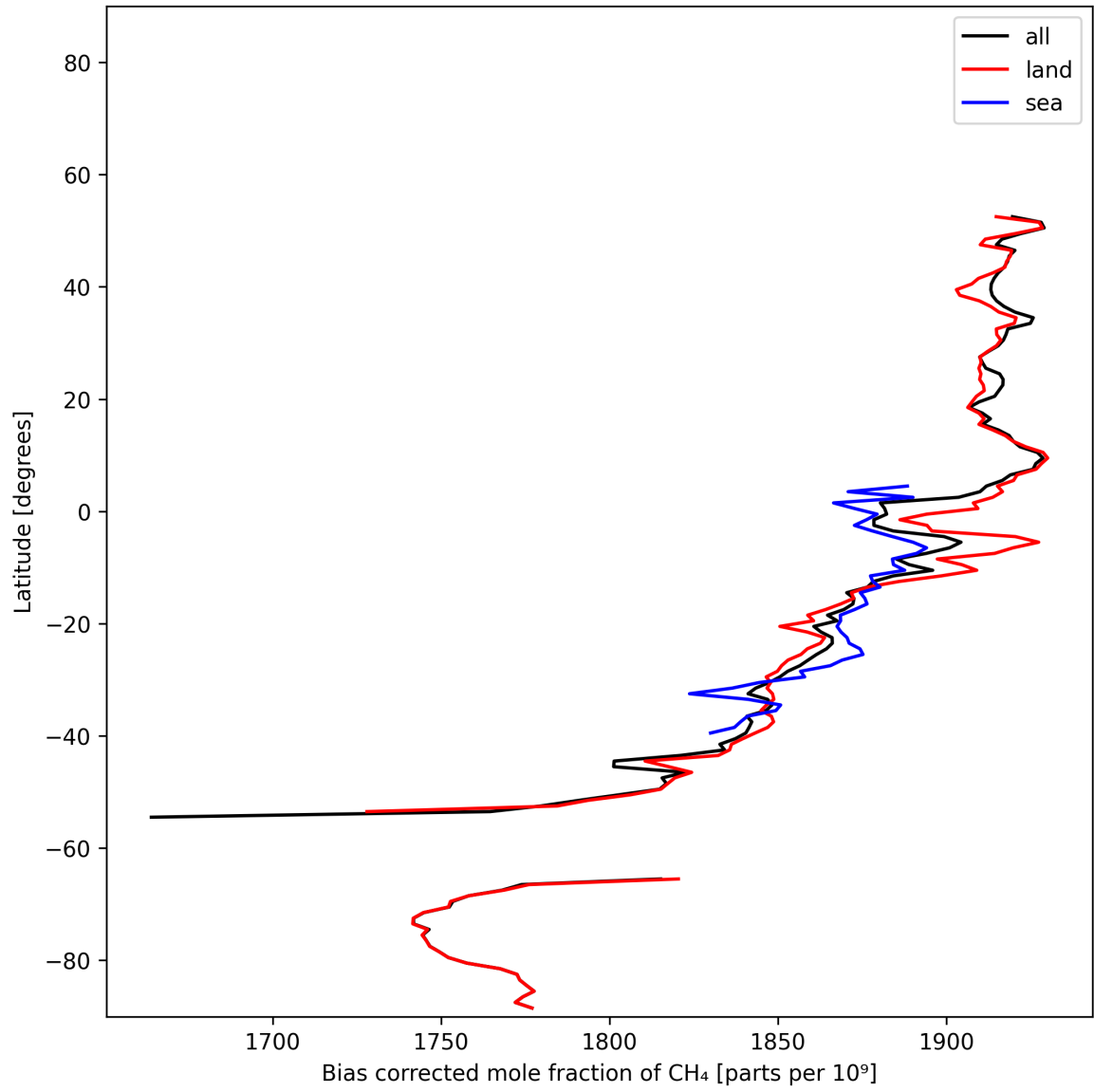
Figure 14: Zonal average of “Bias corrected mole fraction of CH 4 ” for 2025-01-07 to 2025-01-09.
