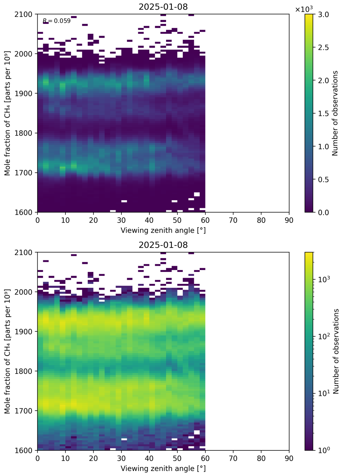
Figure 110: Scatter density plot of “Viewing zenith angle” against “Mole fraction of CH 4 ” for 2025-01-07 to 2025-01-09.
