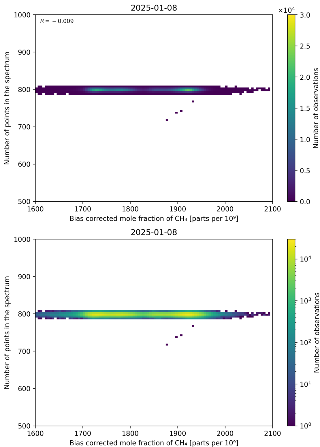
Figure 68: Scatter density plot of “Bias corrected mole fraction of CH 4 ” against “Number of points in the spectrum” for 2025-01-07 to 2025-01-09.
