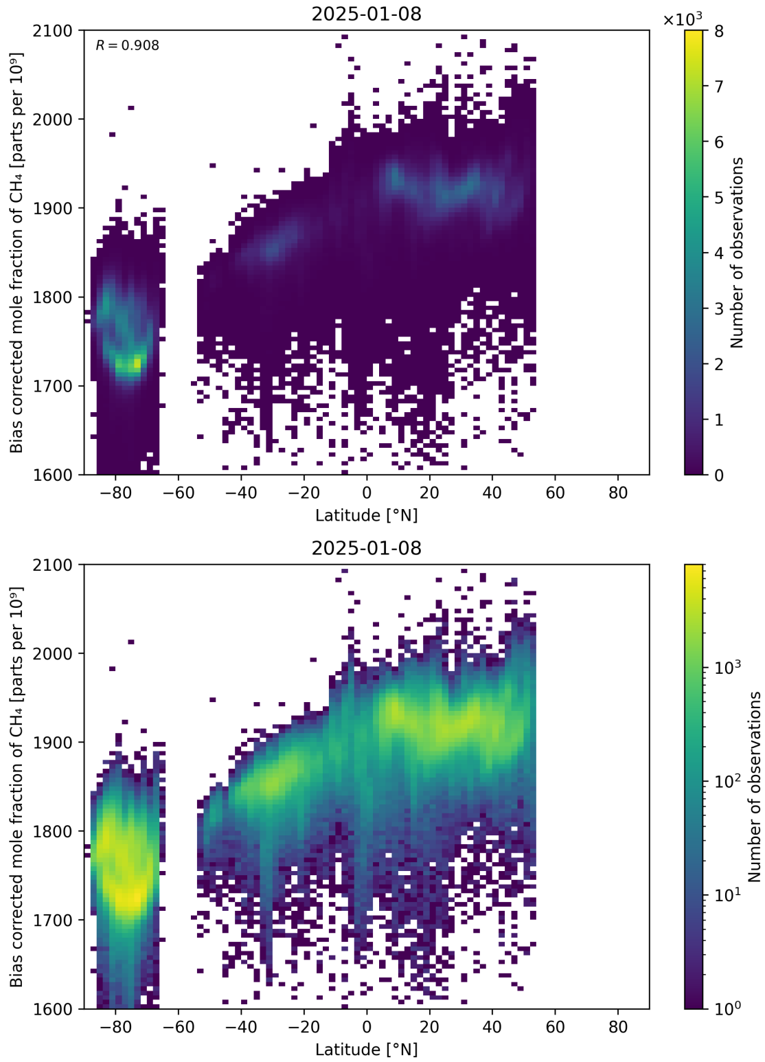
Figure 58: Scatter density plot of “Latitude” against “Bias corrected mole fraction of CH 4 ” for 2025-01-07 to 2025-01-09.
