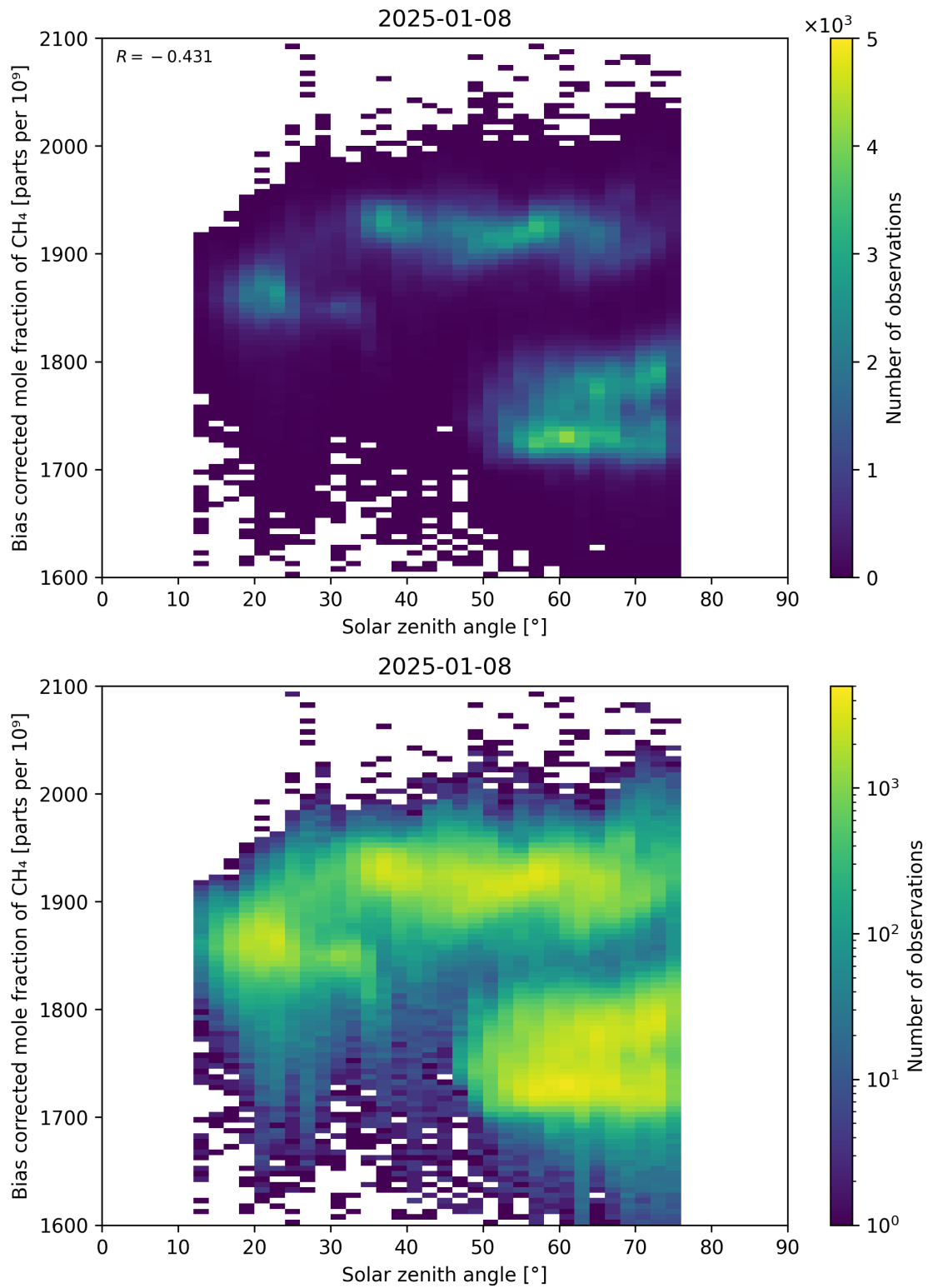
Figure 100: Scatter density plot of “Solar zenith angle” against “Bias corrected mole fraction of CH 4 ” for 2025-01-07 to 2025-01-09.
