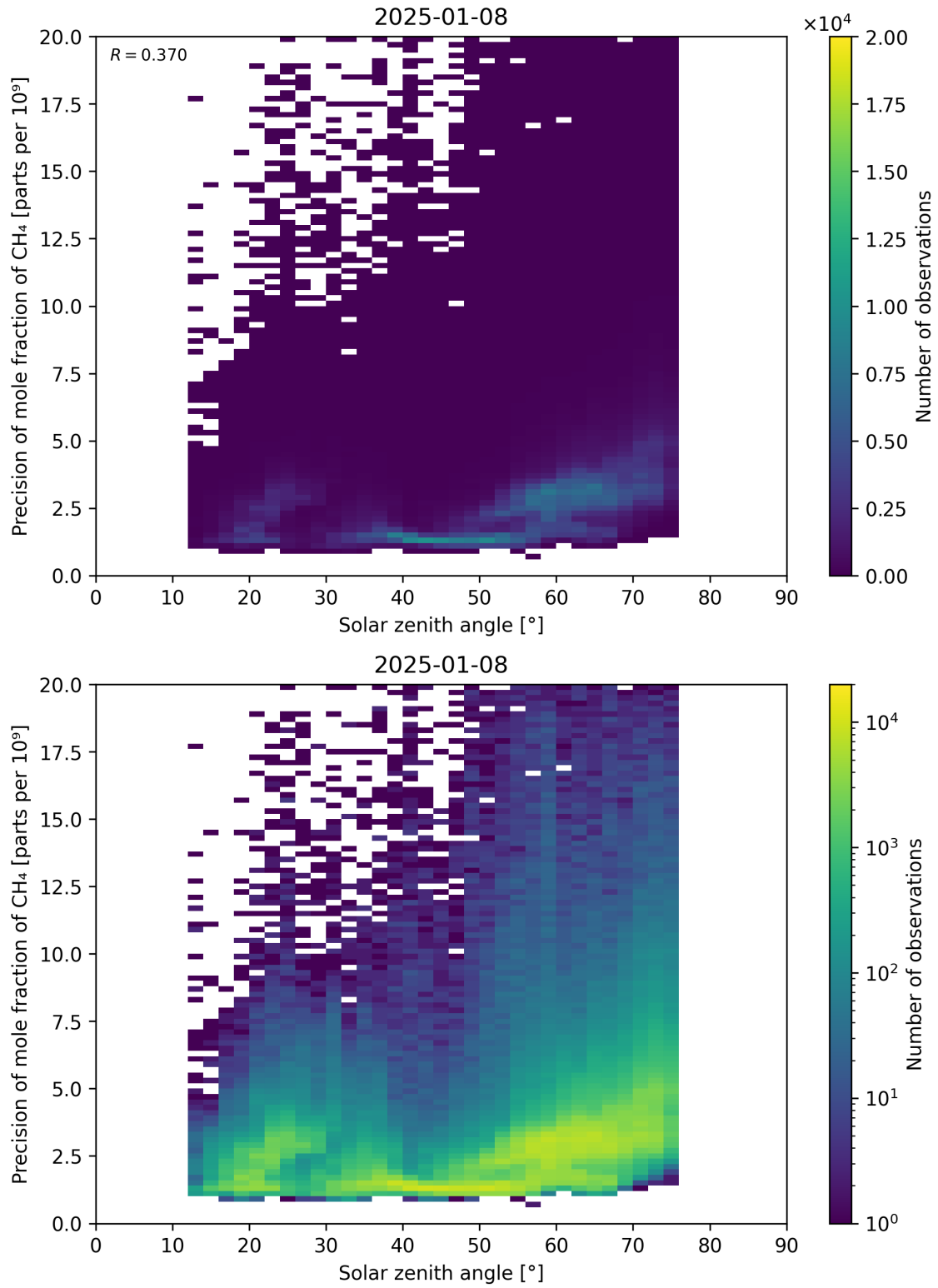
Figure 101: Scatter density plot of “Solar zenith angle” against “Precision of mole fraction of CH 4 ” for 2025-01-07 to 2025-01-09.
