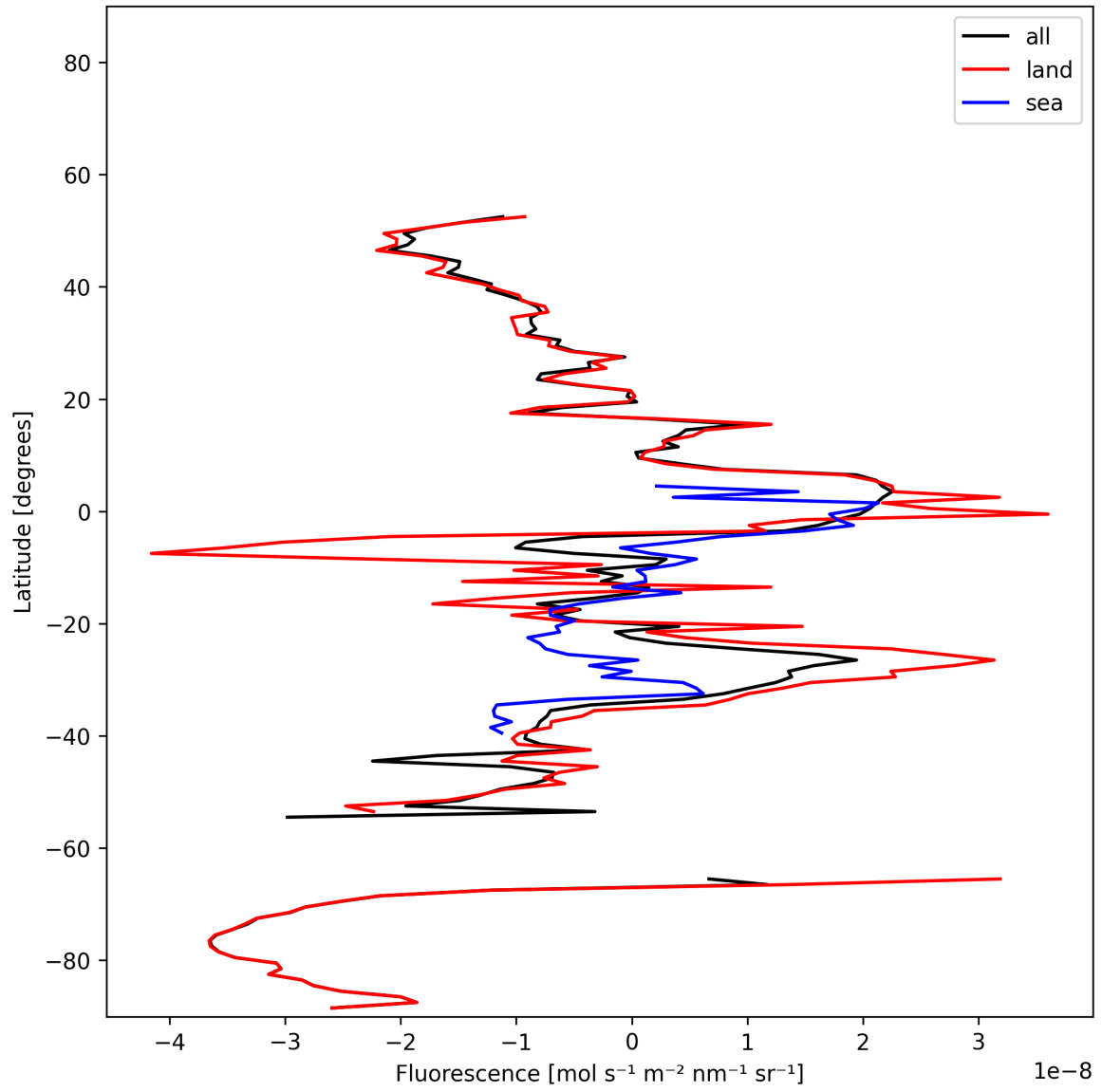
Figure 21: Zonal average of “Fluorescence” for 2025-01-07 to 2025-01-09.
