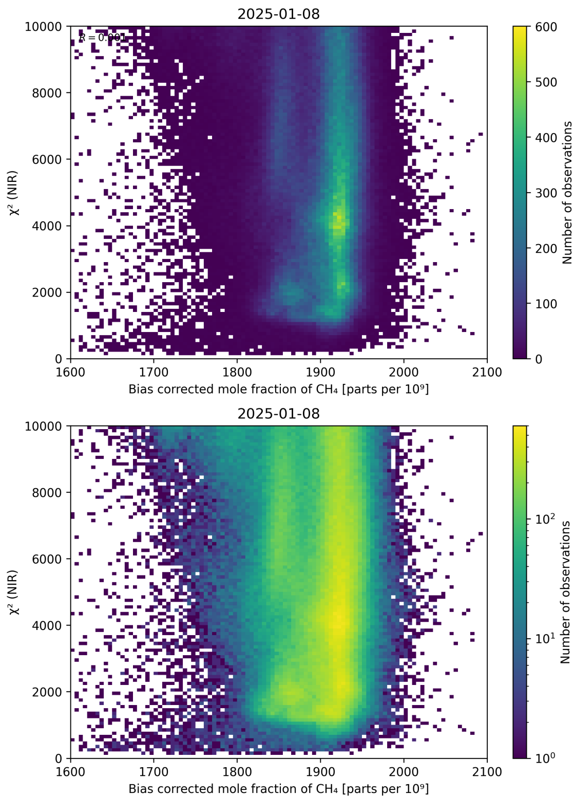
Figure 63: Scatter density plot of “Bias corrected mole fraction of CH 4 ” against “ \chi^2 (NIR)” for 2025-01-07 to 2025-01-09.
