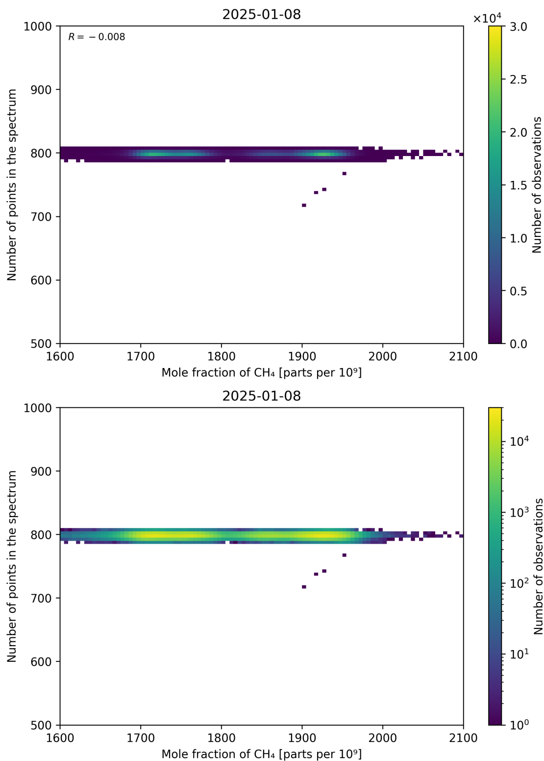
Figure 77: Scatter density plot of “Mole fraction of CH 4 ” against “Number of points in the spectrum” for 2025-01-07 to 2025-01-09.
