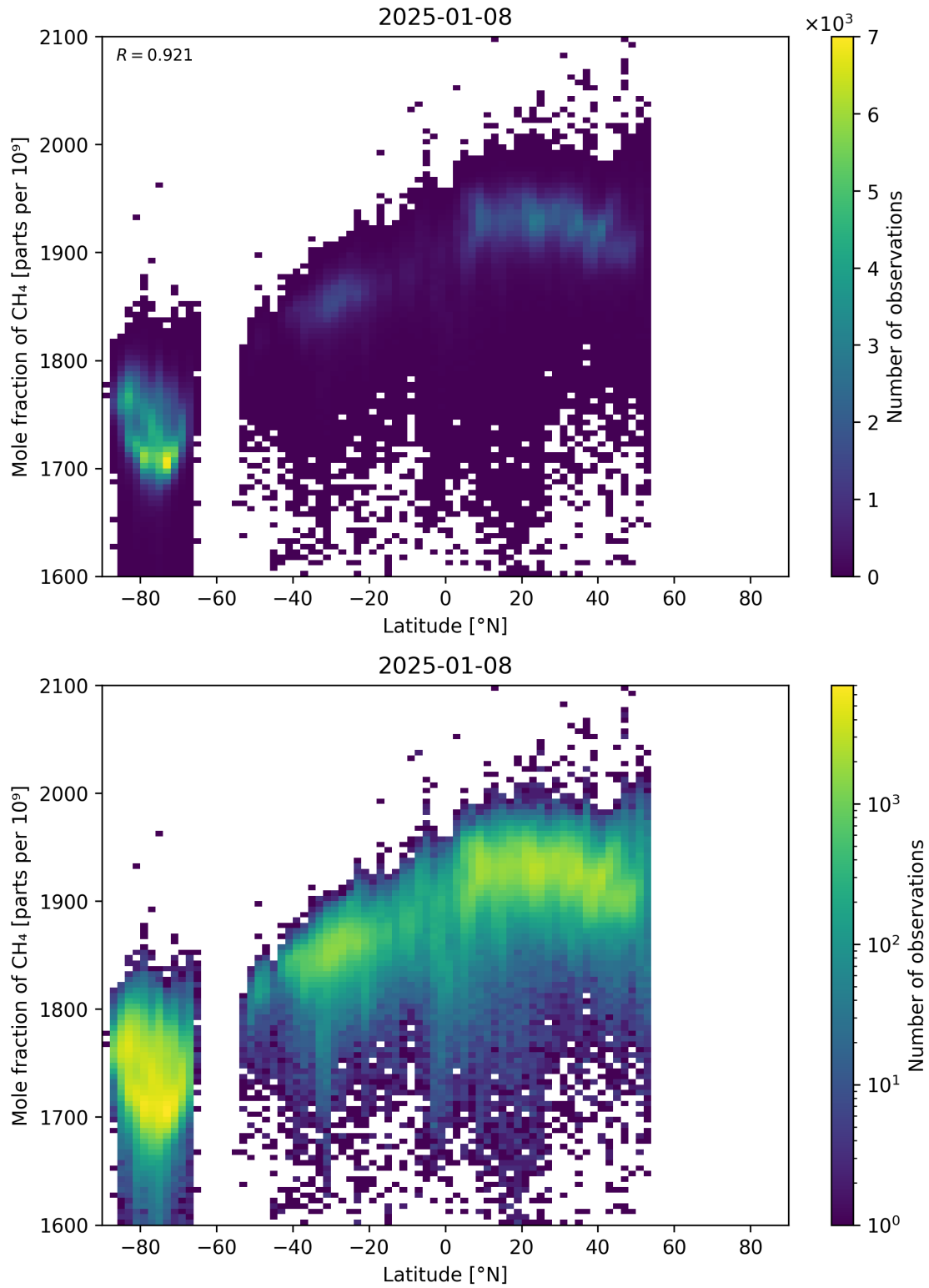
Figure 57: Scatter density plot of “Latitude” against “Mole fraction of \text{CH}_4 ” for 2025-01-07 to 2025-01-09.
