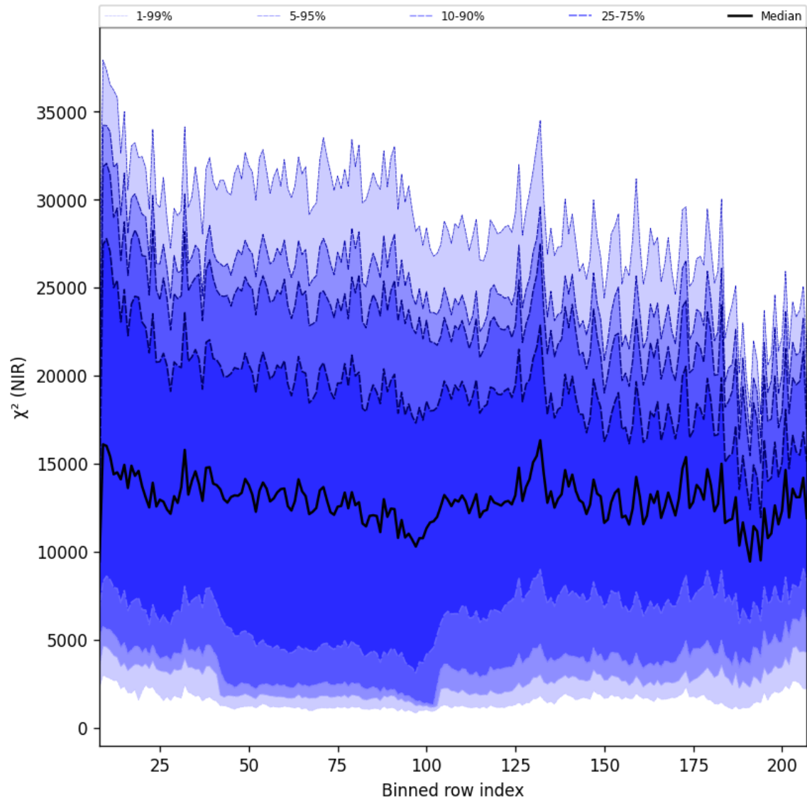
Figure 40: Along track statistics of “ \chi^2 (NIR)” for 2025-01-07 to 2025-01-09
