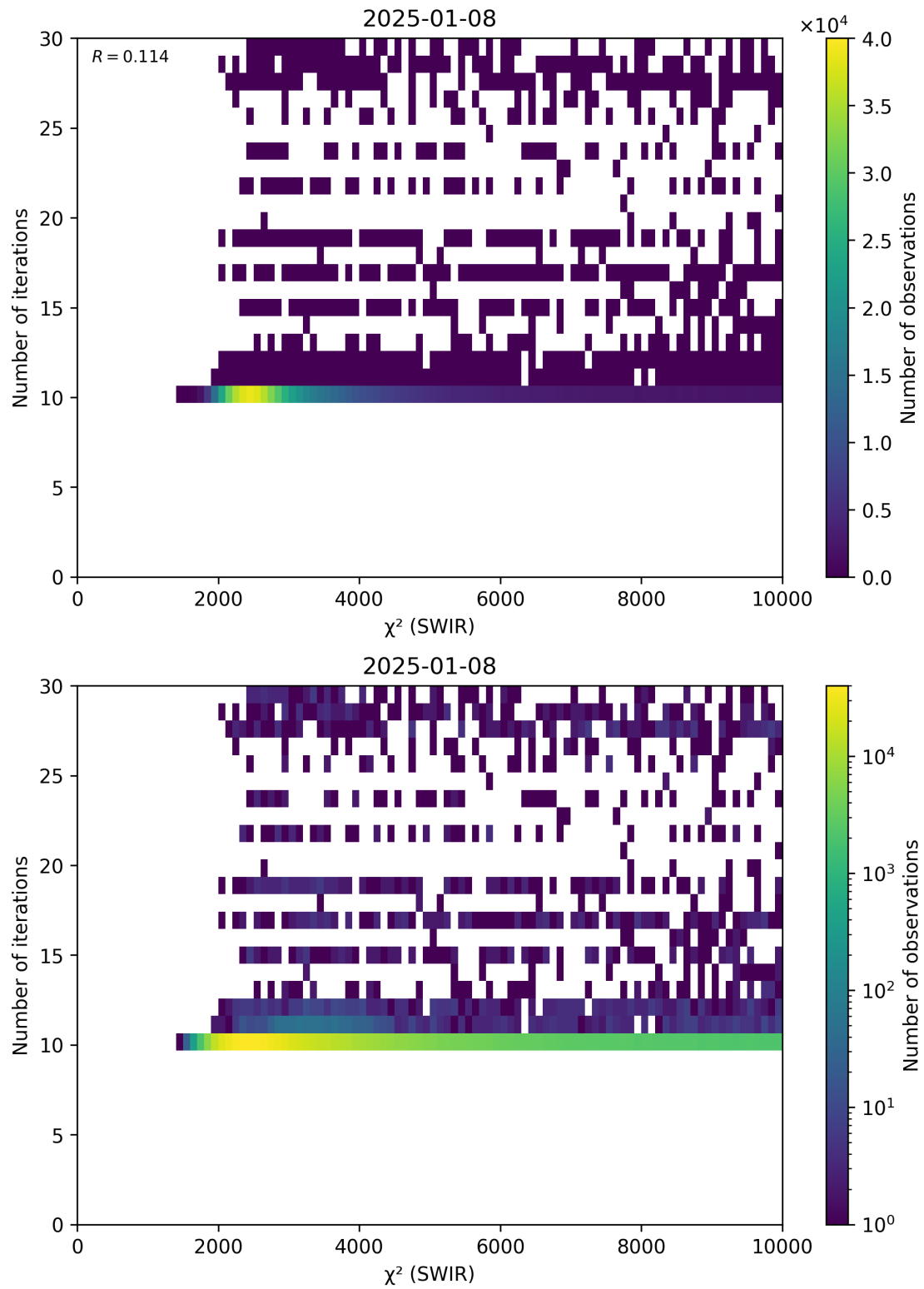
Figure 50: Scatter density plot of “ \chi^2 (SWIR)” against “Number of iterations” for 2025-01-07 to 2025-01-09.
