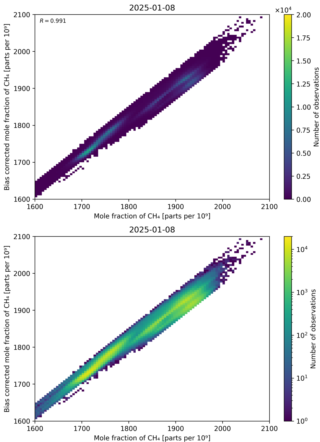
Figure 74: Scatter density plot of “Mole fraction of CH 4 ” against “Bias corrected mole fraction of CH 4 ” for 2025-01-07 to 2025-01-09.
