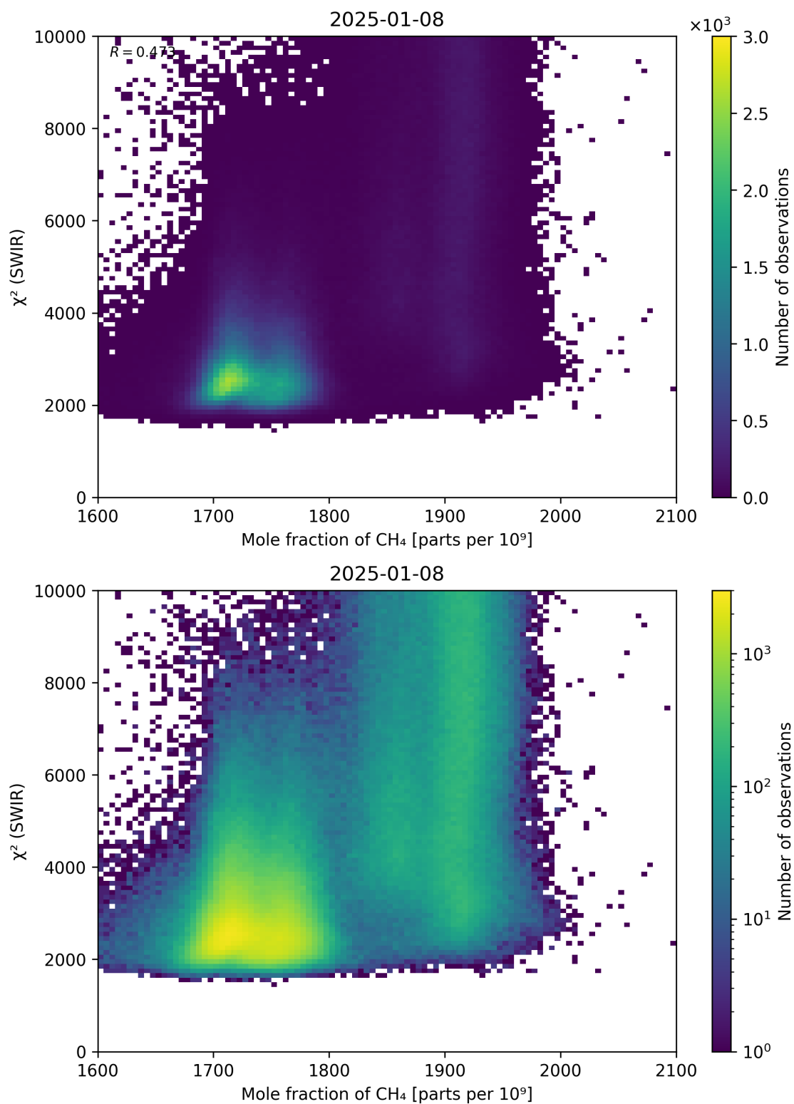
Figure 71: Scatter density plot of “Mole fraction of \text{CH}_4 ” against “ \chi^2 (SWIR)” for 2025-01-07 to 2025-01-09.
