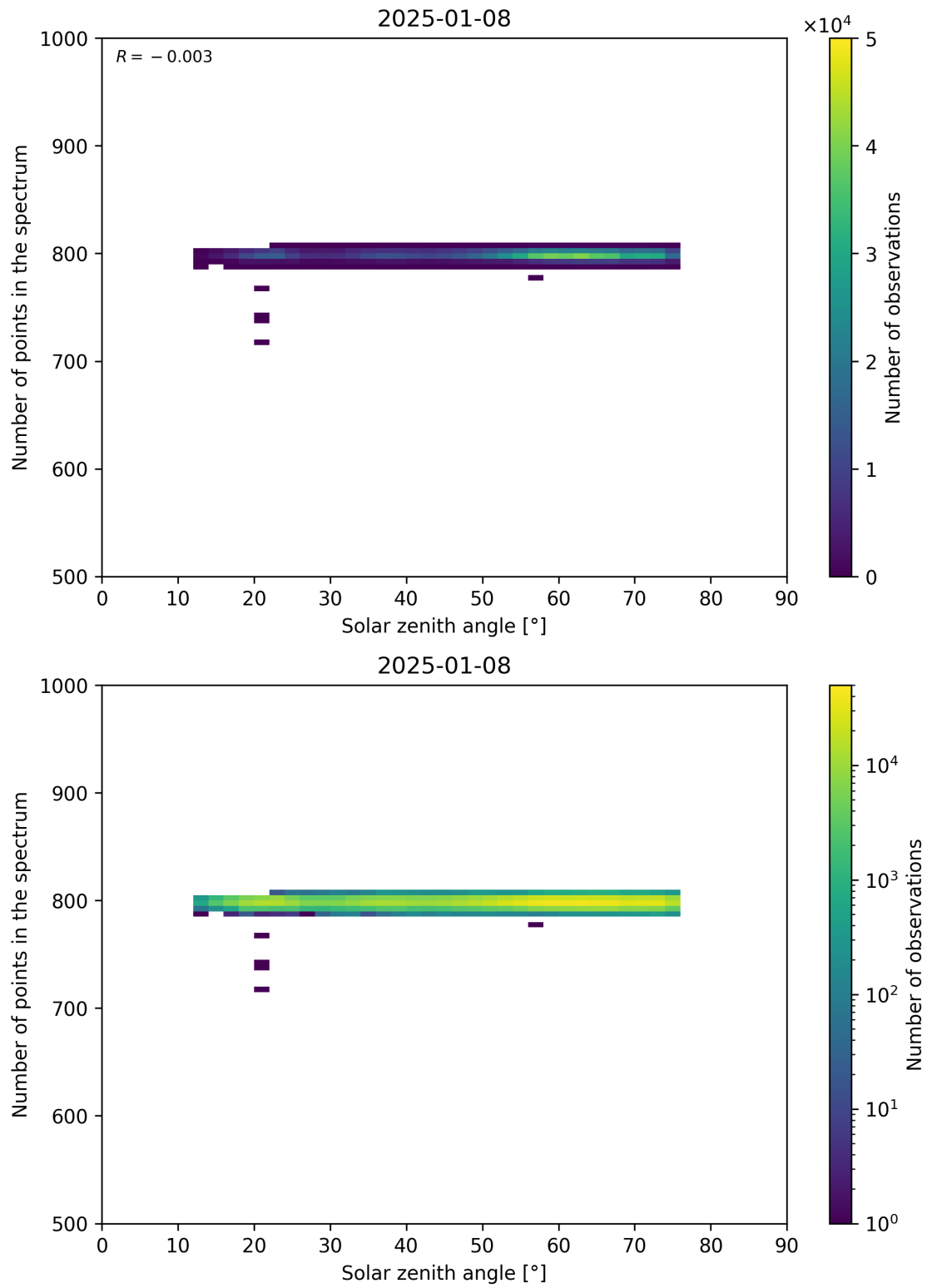
Figure 103: Scatter density plot of “Solar zenith angle” against “Number of points in the spectrum” for 2025-01-07 to 2025-01-09.
