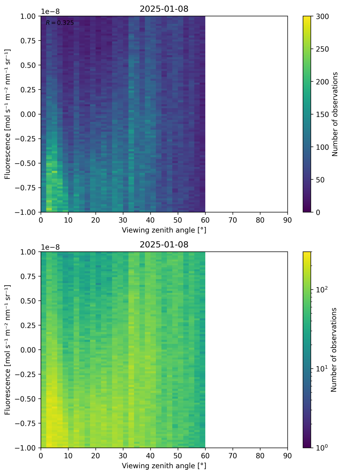
Figure 108: Scatter density plot of “Viewing zenith angle” against “Fluorescence” for 2025-01-07 to 2025-01-09.
