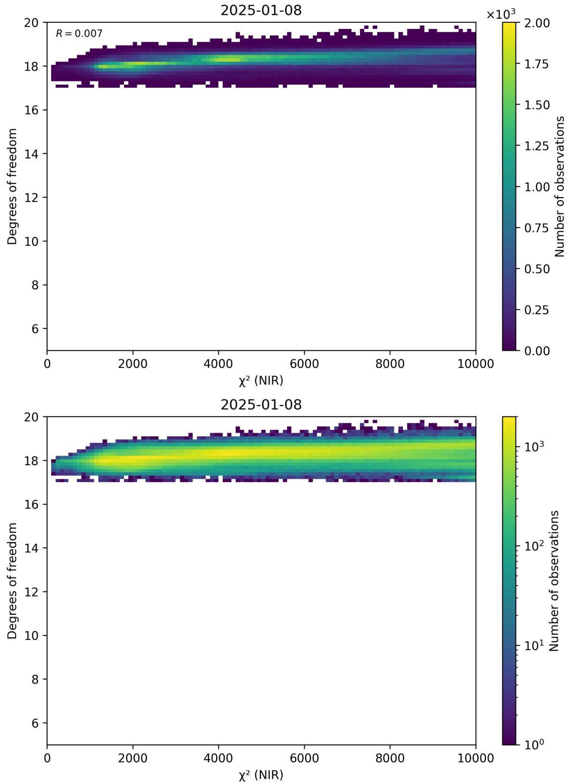
Figure 44: Scatter density plot of “ \chi^2 (NIR)” against “Degrees of freedom” for 2025-01-07 to 2025-01-09.
