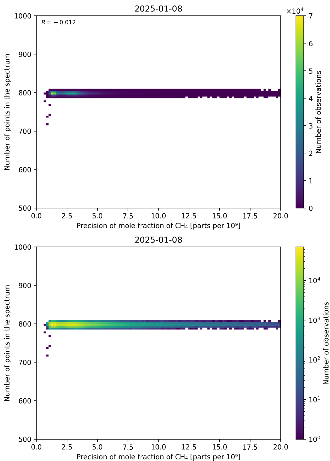
Figure 84: Scatter density plot of “Precision of mole fraction of CH 4 ” against “Number of points in the spectrum” for 2025-01-07 to 2025-01-09.
