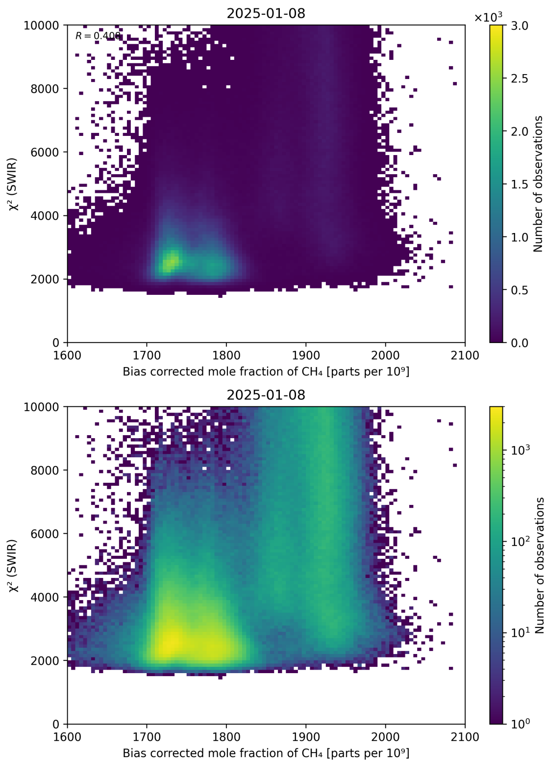
Figure 64: Scatter density plot of “Bias corrected mole fraction of \text{CH}_4 ” against “ \chi^2 (SWIR)” for 2025-01-07 to 2025-01-09.
