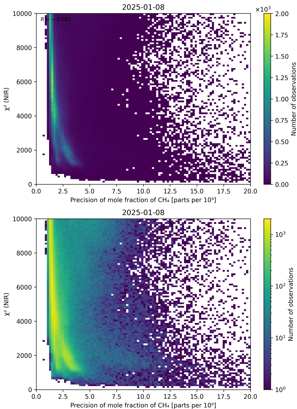
Figure 78: Scatter density plot of “Precision of mole fraction of CH 4 ” against “ \chi^2 (NIR)” for 2025-01-07 to 2025-01-09.
