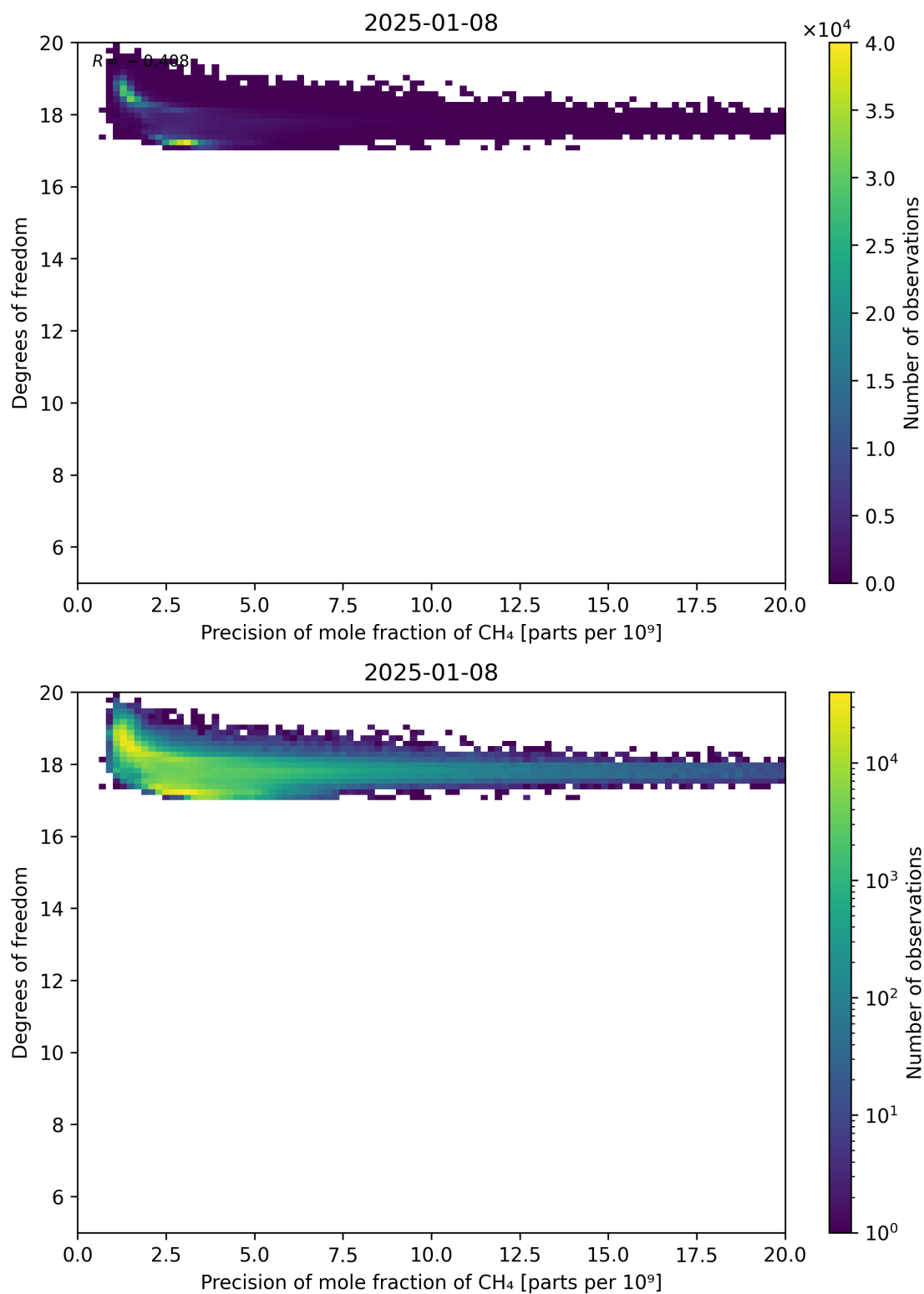
Figure 80: Scatter density plot of “Precision of mole fraction of CH 4 ” against “Degrees of freedom” for 2025-01-07 to 2025-01-09.
