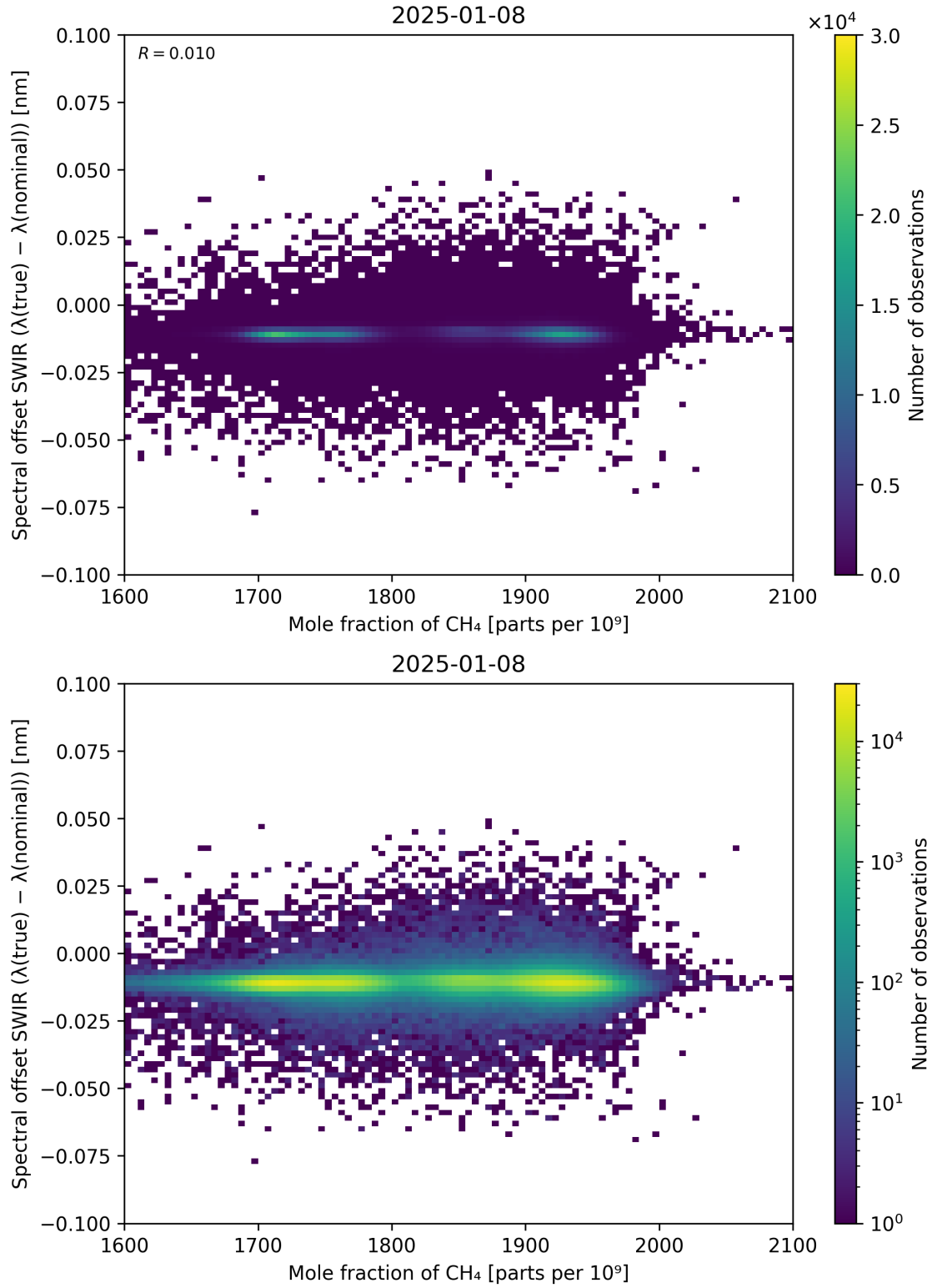
Figure 86: Scatter density plot of “Mole fraction of \text{CH}_4 ” against “Spectral offset SWIR ( \lambda_{\text{true}} - \lambda_{\text{nominal}} )” for 2025-01-07 to 2025-01-09.
