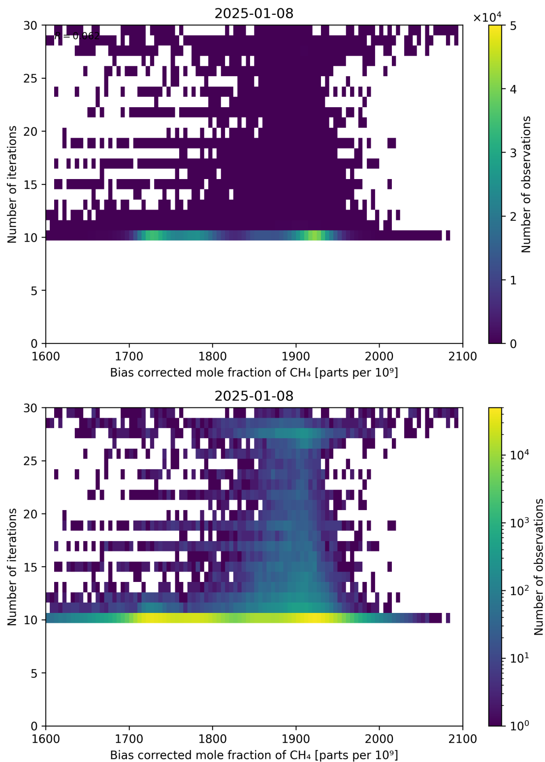
Figure 67: Scatter density plot of “Bias corrected mole fraction of CH 4 ” against “Number of iterations” for 2025-01-07 to 2025-01-09.
