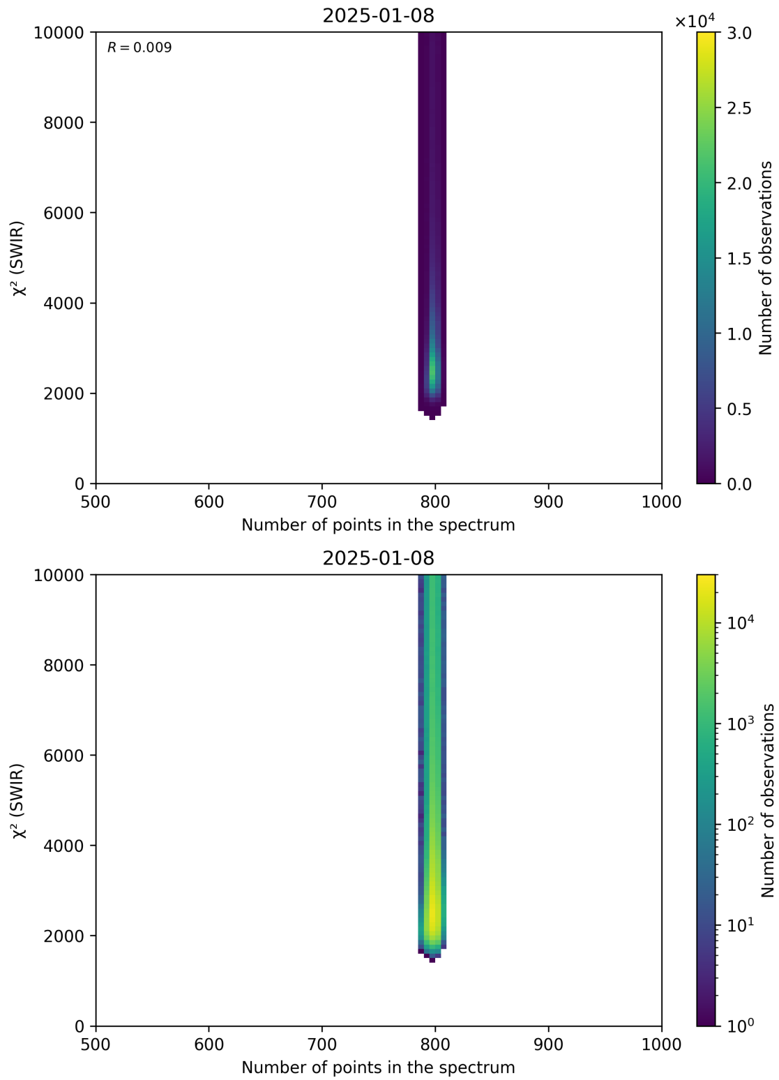
Figure 89: Scatter density plot of “Number of points in the spectrum” against “ \chi^2 (SWIR)” for 2025-01-07 to 2025-01-09.
