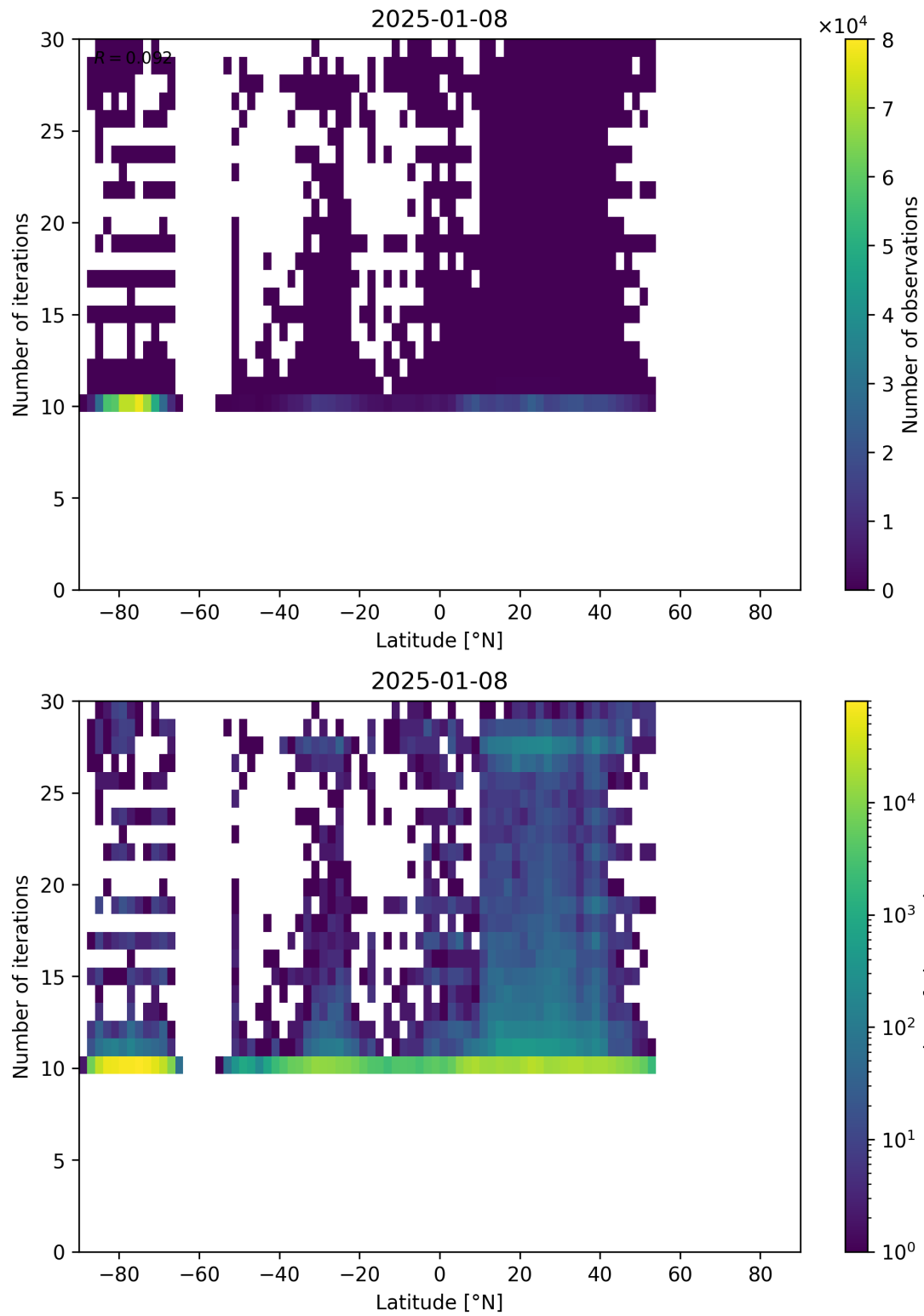
Figure 60: Scatter density plot of “Latitude” against “Number of iterations” for 2025-01-07 to 2025-01-09.
