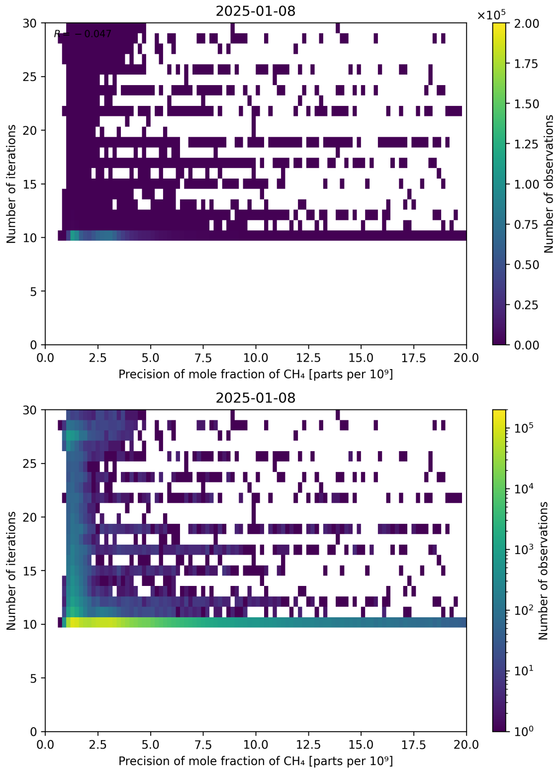
Figure 83: Scatter density plot of “Precision of mole fraction of CH 4 ” against “Number of iterations” for 2025-01-07 to 2025-01-09.
