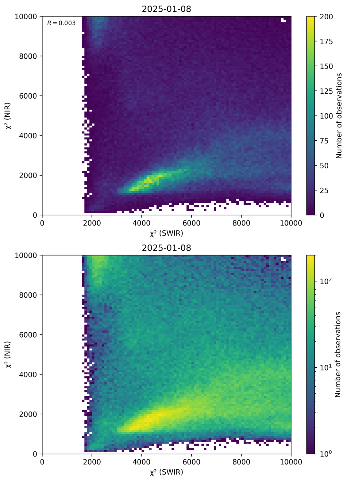
Figure 47: Scatter density plot of “ \chi^2 (SWIR)” against “ \chi^2 (NIR)” for 2025-01-07 to 2025-01-09.
