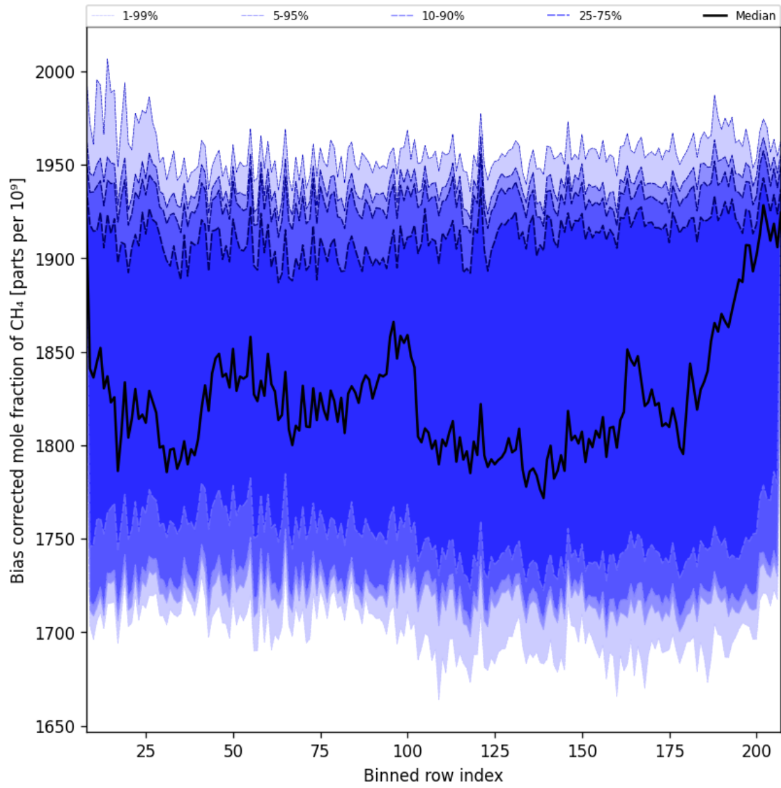
Figure 36: Along track statistics of “Bias corrected mole fraction of CH 4 ” for 2025-01-07 to 2025-01-09
