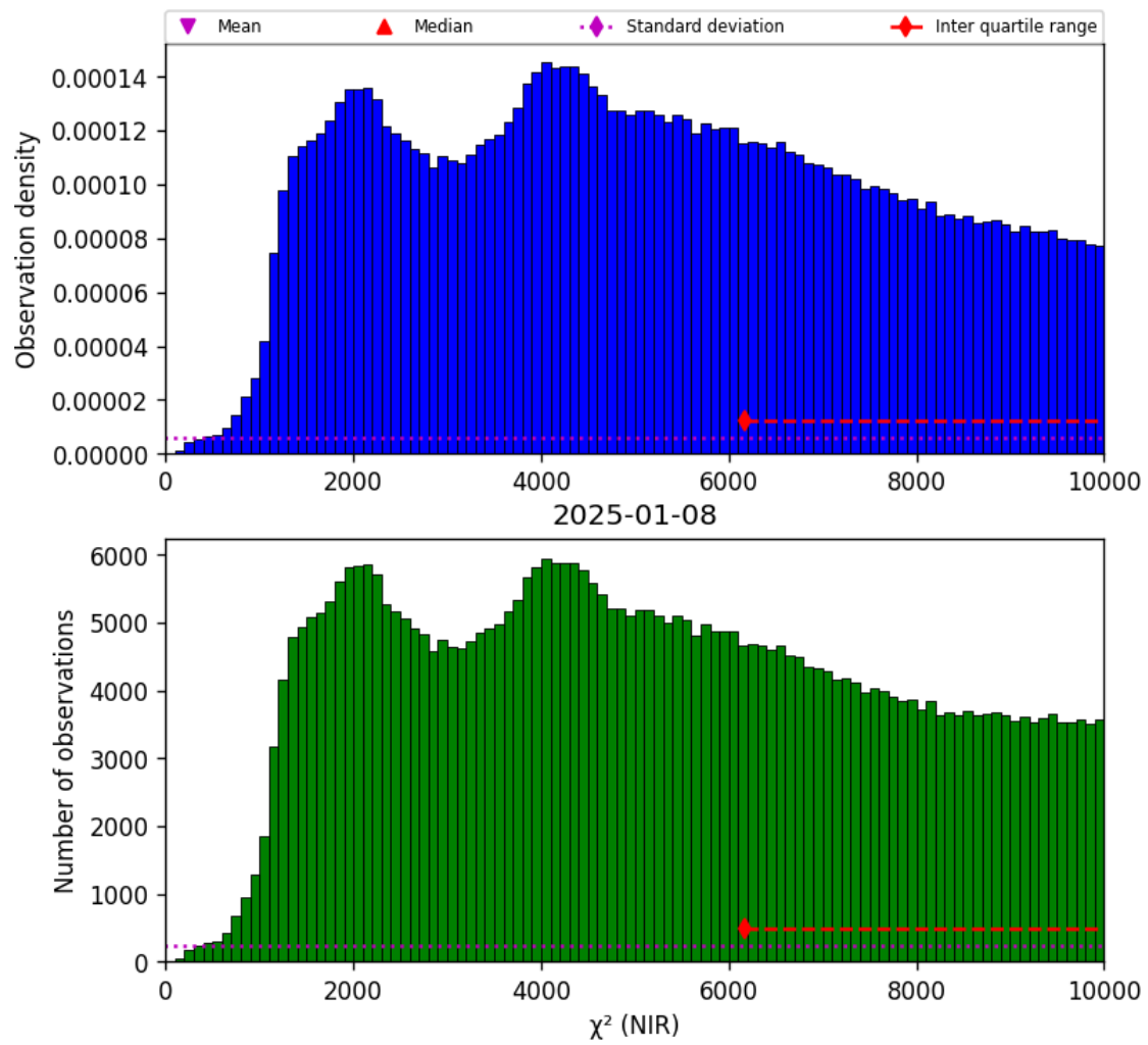
Figure 29: Histogram of “ \chi^2 (NIR)” for 2025-01-07 to 2025-01-09
