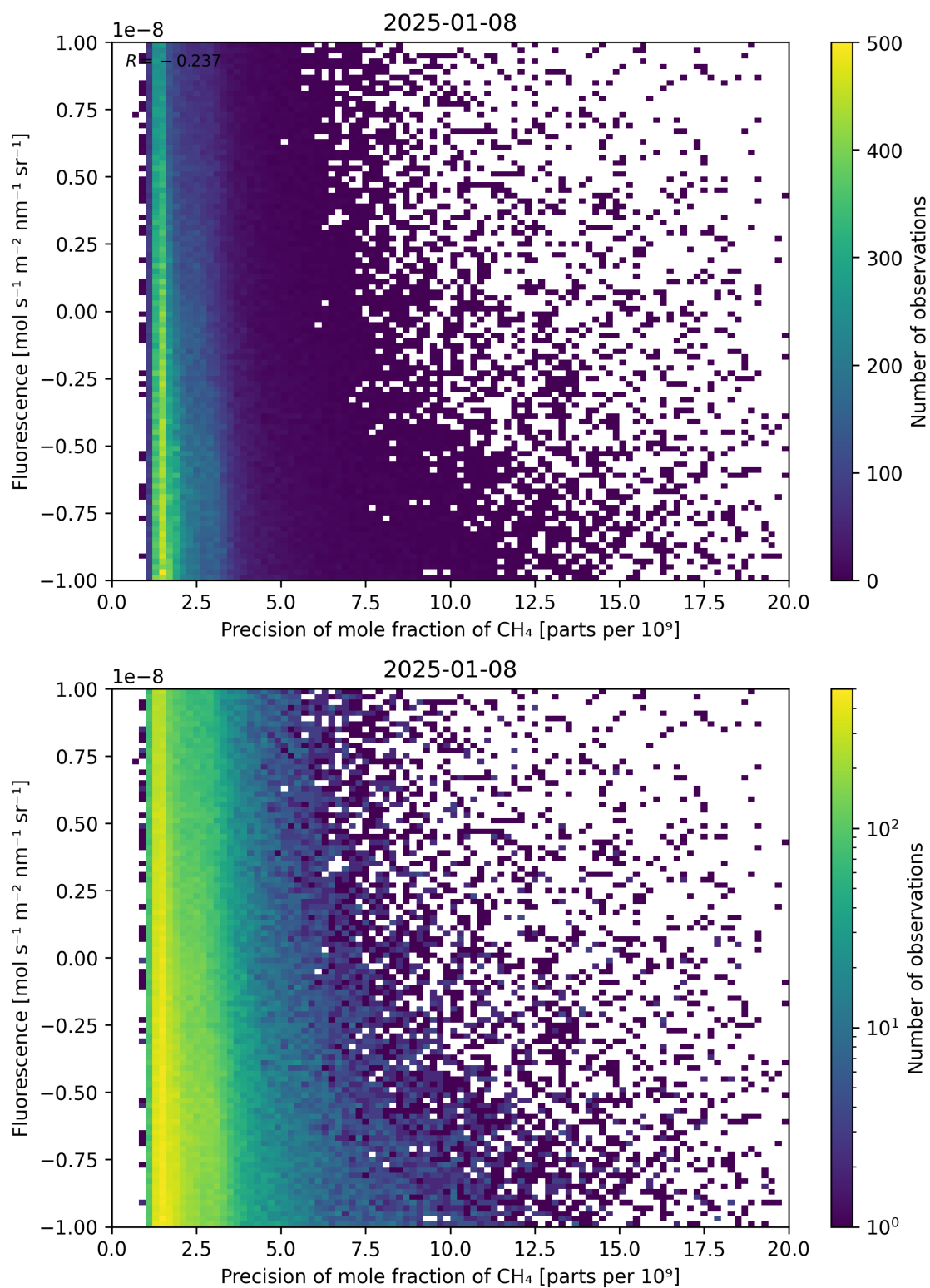
Figure 81: Scatter density plot of “Precision of mole fraction of CH 4 ” against “Fluorescence” for 2025-01-07 to 2025-01-09.
