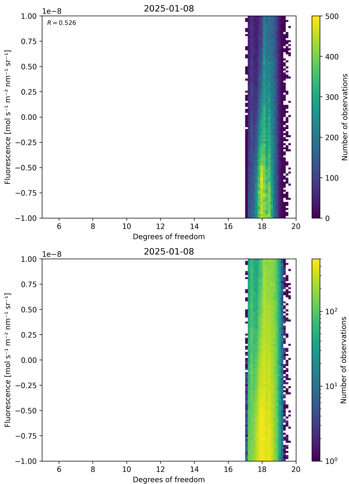
Figure 51: Scatter density plot of “Degrees of freedom” against “Fluorescence” for 2025-01-07 to 2025-01-09.
