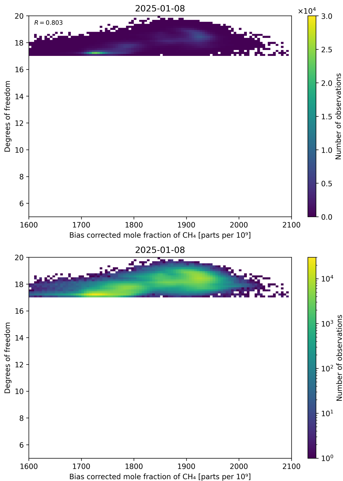
Figure 65: Scatter density plot of “Bias corrected mole fraction of CH 4 ” against “Degrees of freedom” for 2025-01-07 to 2025-01-09.
