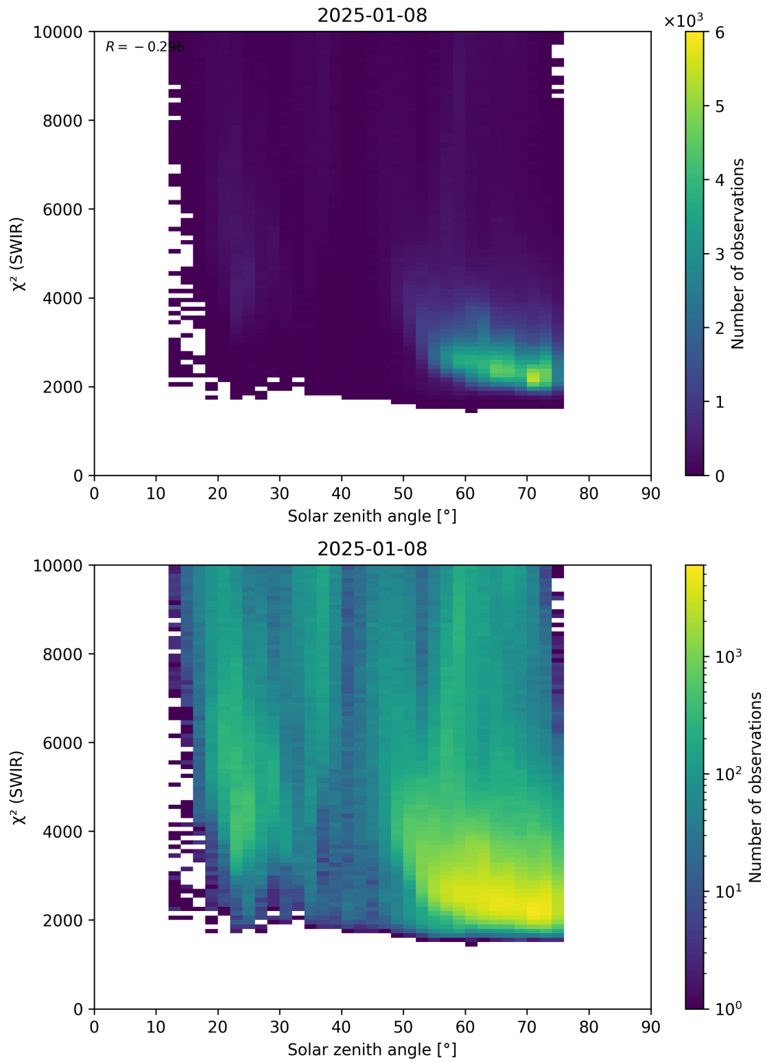
Figure 95: Scatter density plot of “Solar zenith angle” against “ \chi^2 (SWIR)” for 2025-01-07 to 2025-01-09.
