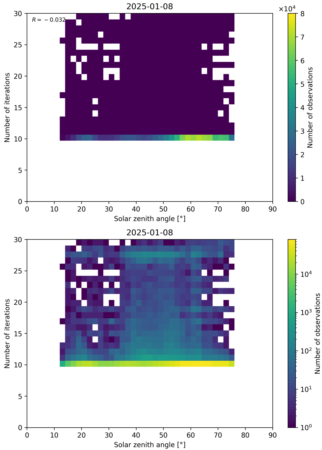
Figure 102: Scatter density plot of “Solar zenith angle” against “Number of iterations” for 2025-01-07 to 2025-01-09.
