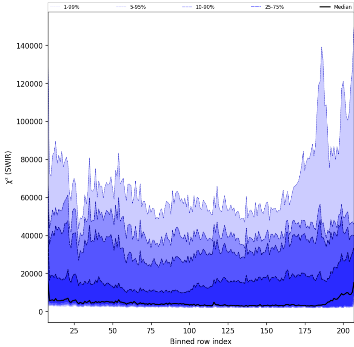
Figure 39: Along track statistics of “ \chi^2 (SWIR)” for 2025-01-07 to 2025-01-09
