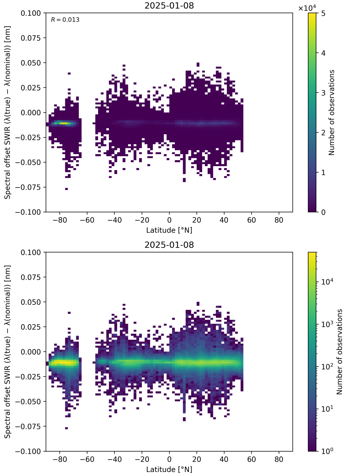
Figure 62: Scatter density plot of “Latitude” against “Spectral offset SWIR ( \lambda_{\text{true}} - \lambda_{\text{nominal}} )” for 2025-01-07 to 2025-01-09.
