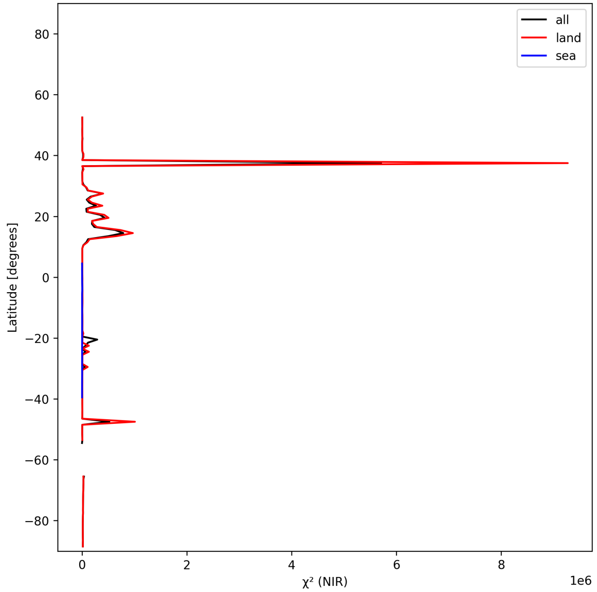
Figure 18: Zonal average of “ \chi^2 (NIR)” for 2025-01-07 to 2025-01-09.
