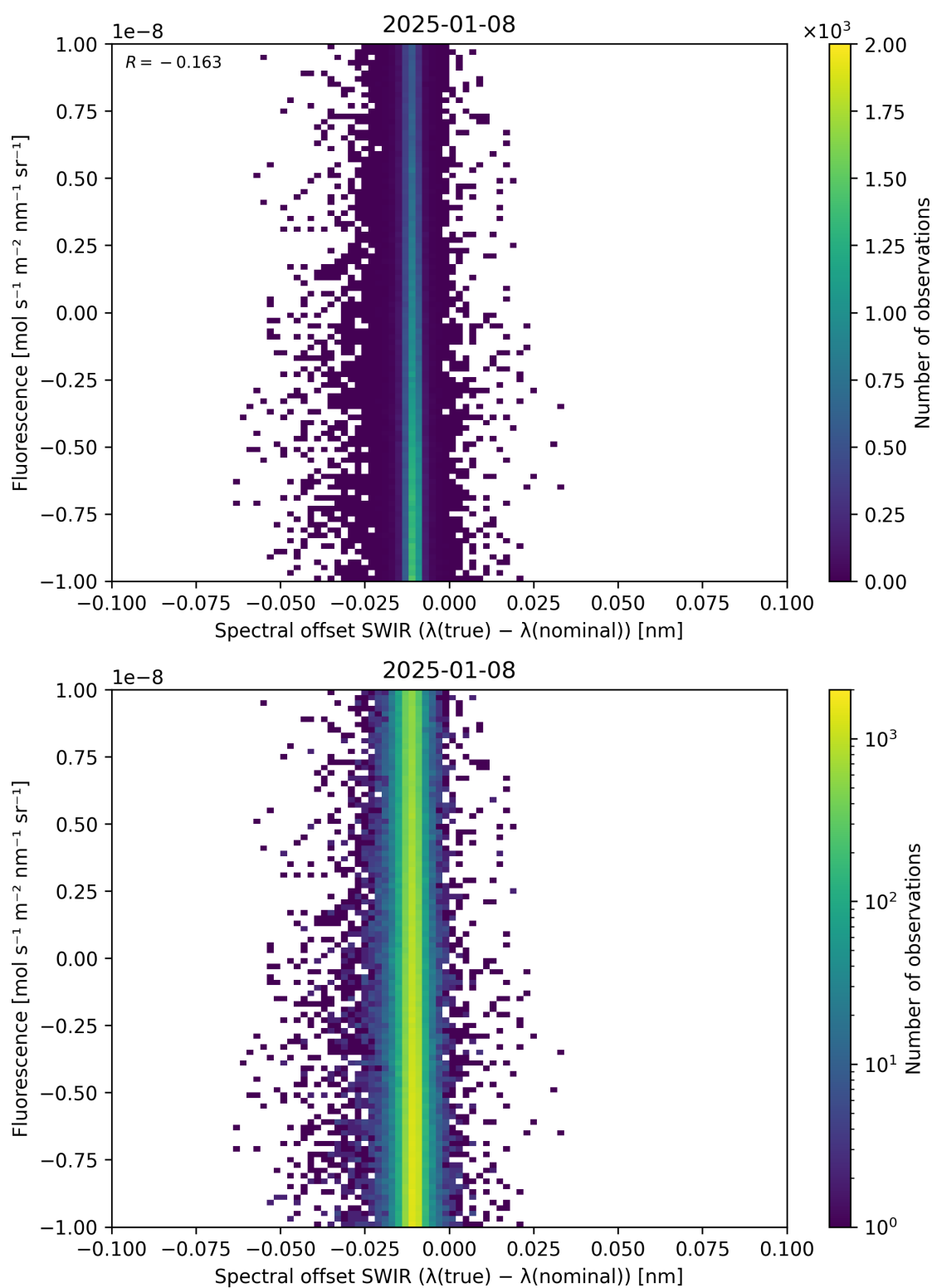
Figure 120: Scatter density plot of “Spectral offset SWIR ( \lambda_{\text{true}} - \lambda_{\text{nominal}} )” against “Fluorescence” for 2025-01-07 to 2025-01-09.
