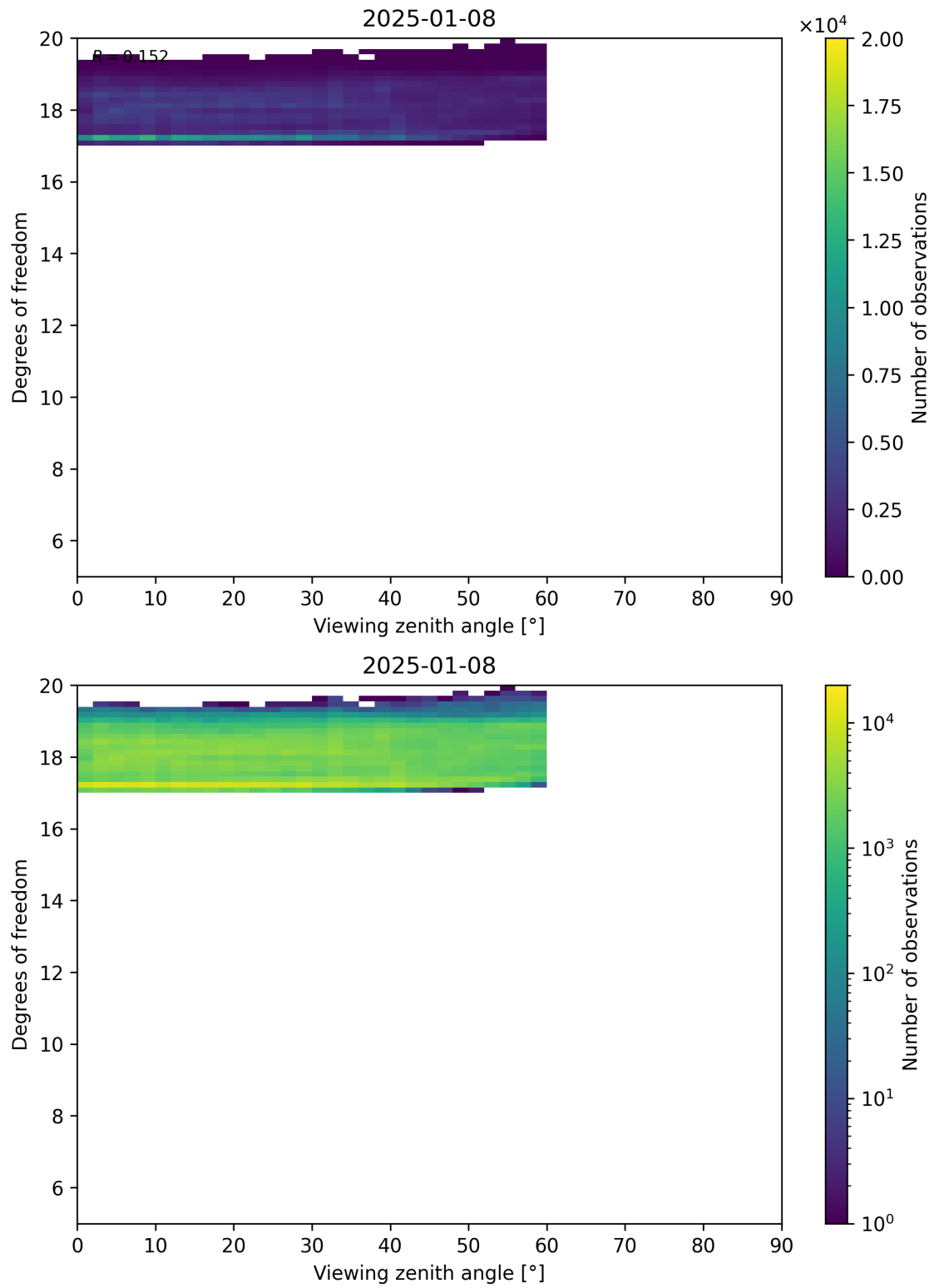
Figure 107: Scatter density plot of “Viewing zenith angle” against “Degrees of freedom” for 2025-01-07 to 2025-01-09.
