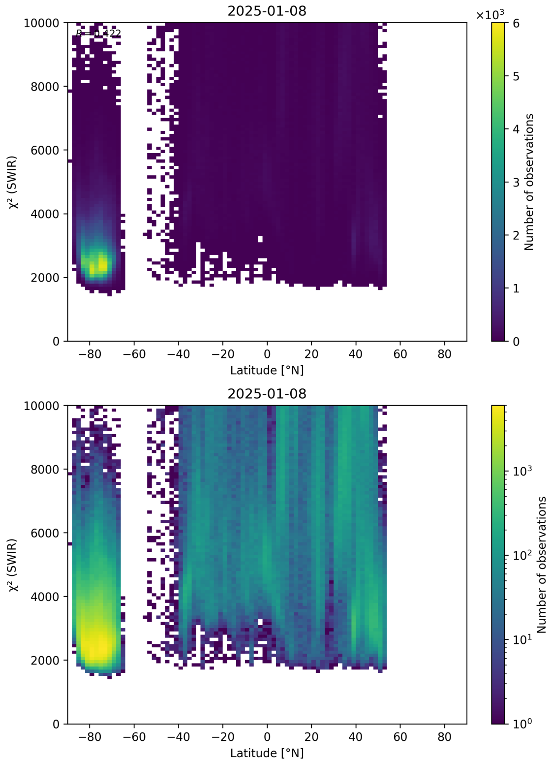
Figure 54: Scatter density plot of “Latitude” against “ \chi^2 (SWIR)” for 2025-01-07 to 2025-01-09.
