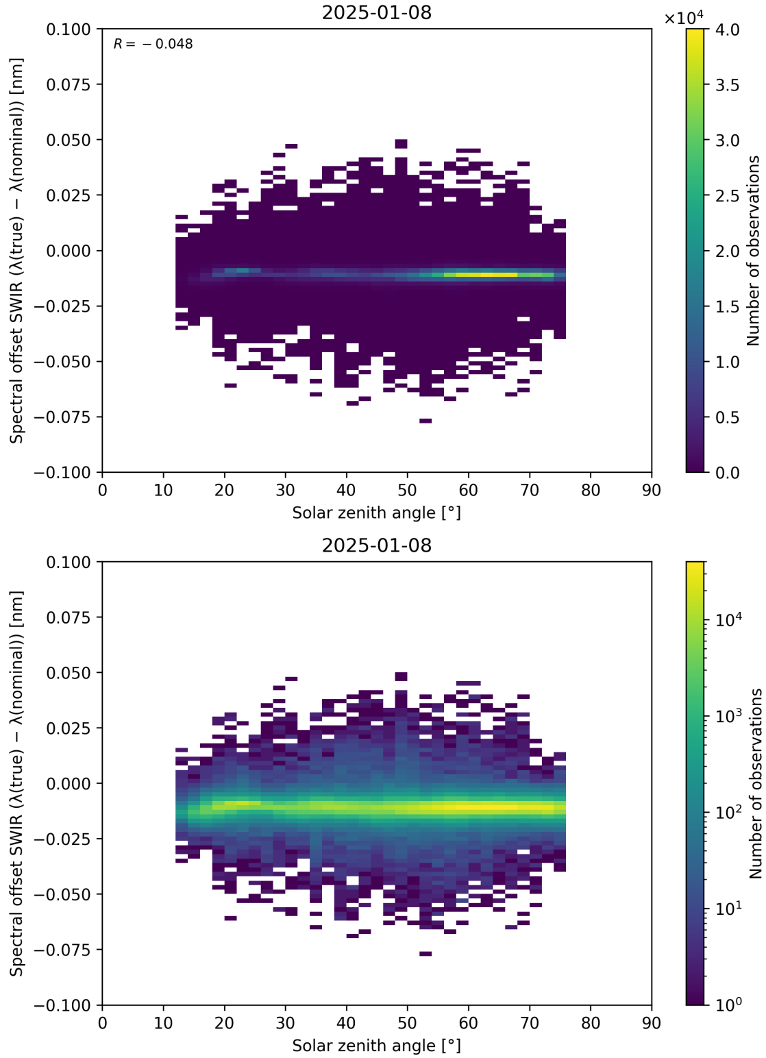
Figure 104: Scatter density plot of “Solar zenith angle” against “Spectral offset SWIR ( \lambda_{\text{true}} - \lambda_{\text{nominal}} )” for 2025-01-07 to 2025-01-09.
