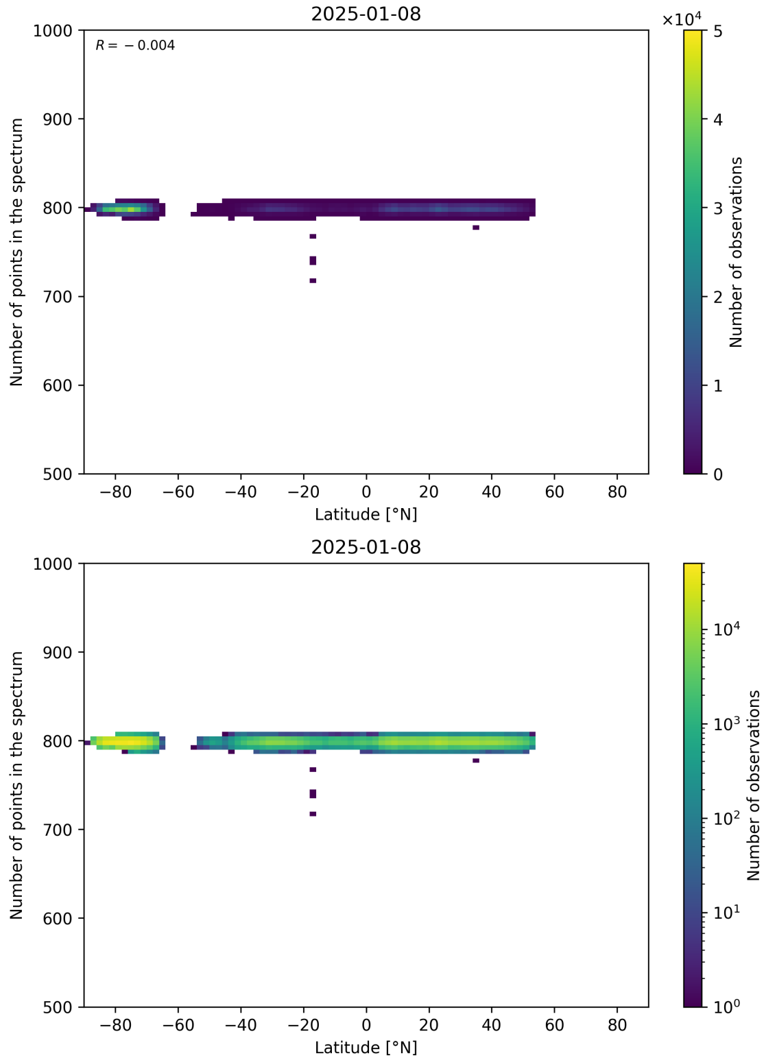
Figure 61: Scatter density plot of “Latitude” against “Number of points in the spectrum” for 2025-01-07 to 2025-01-09.
