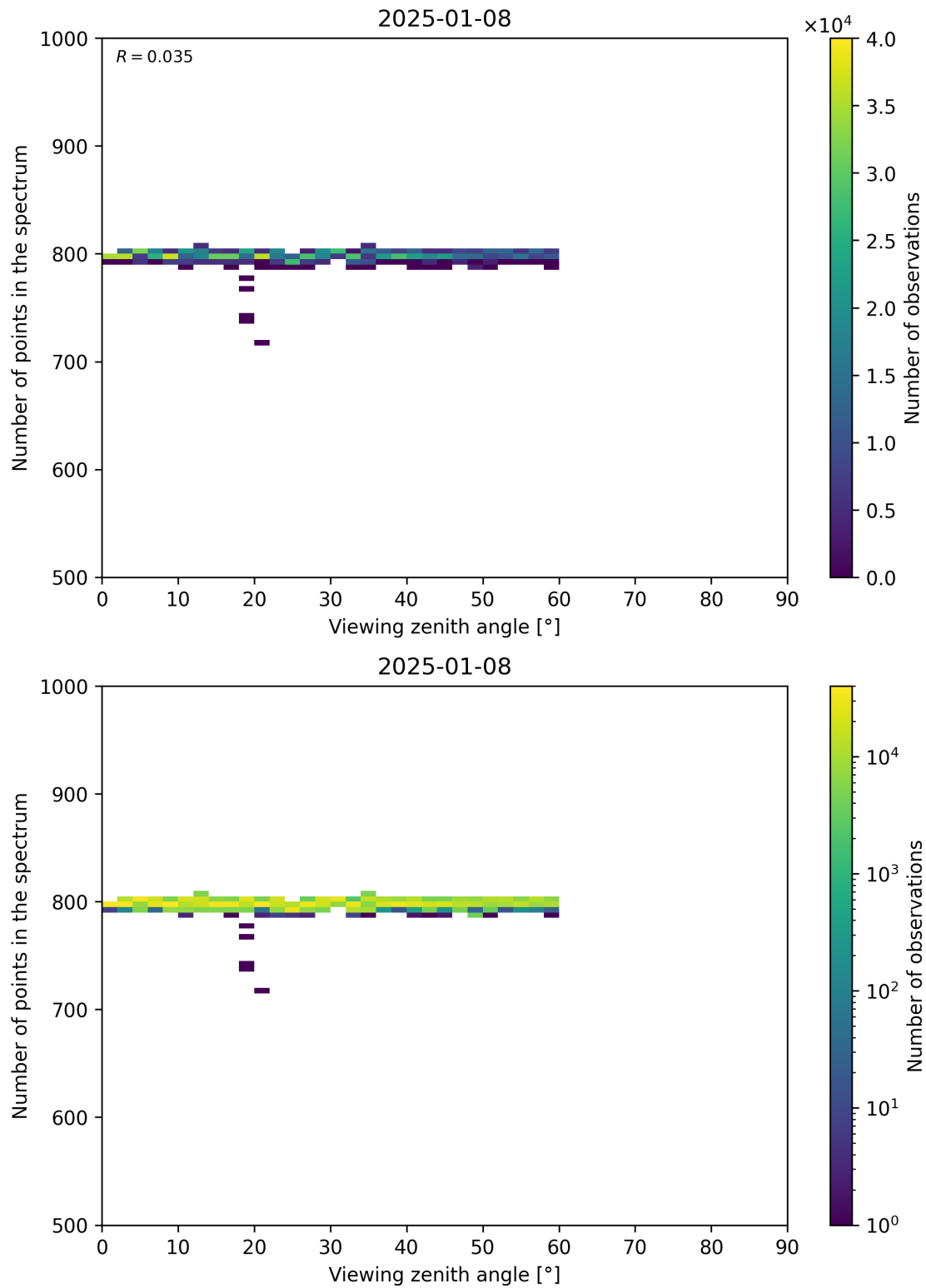
Figure 114: Scatter density plot of “Viewing zenith angle” against “Number of points in the spectrum” for 2025-01-07 to 2025-01-09.
