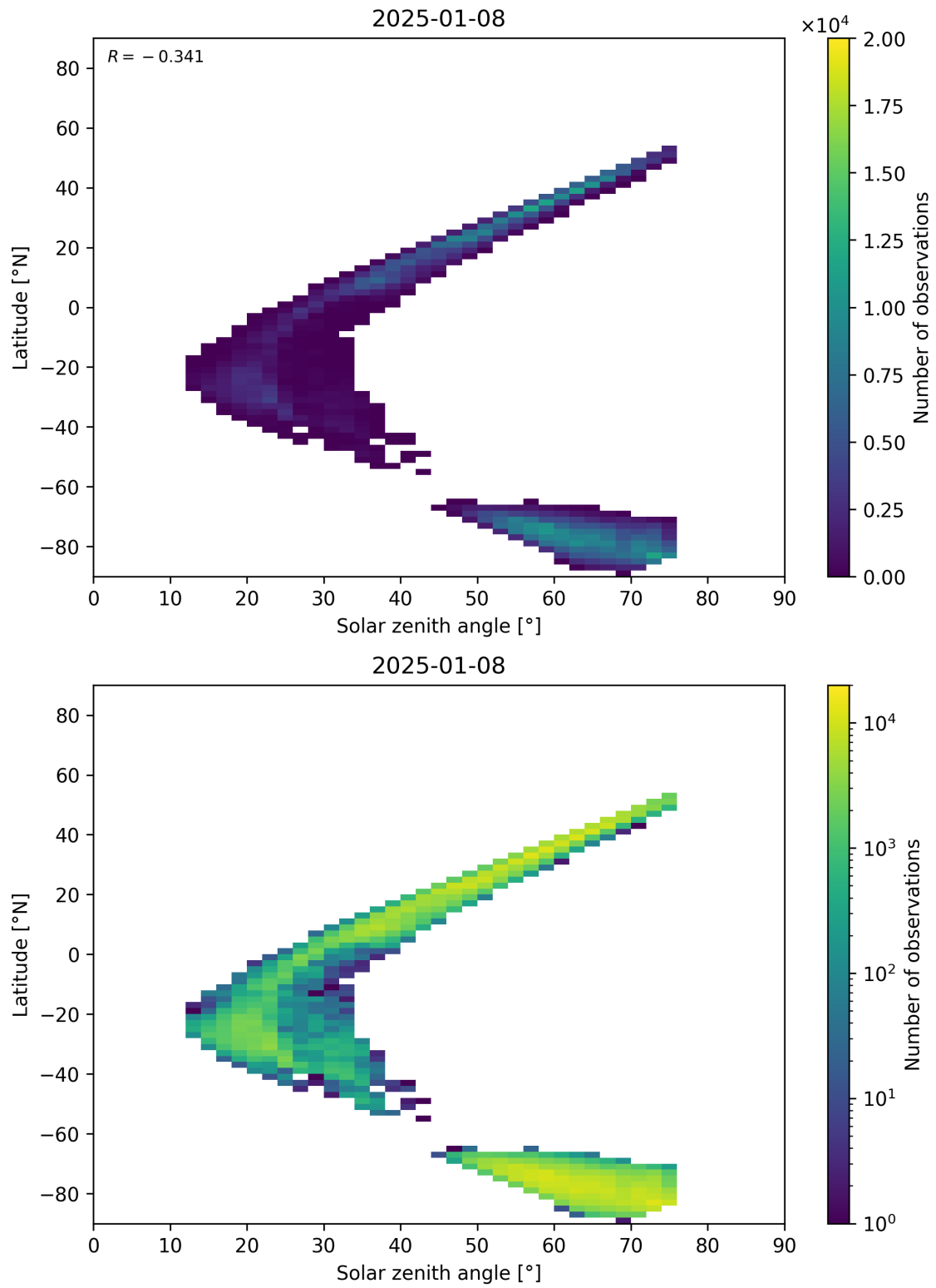
Figure 98: Scatter density plot of “Solar zenith angle” against “Latitude” for 2025-01-07 to 2025-01-09.
