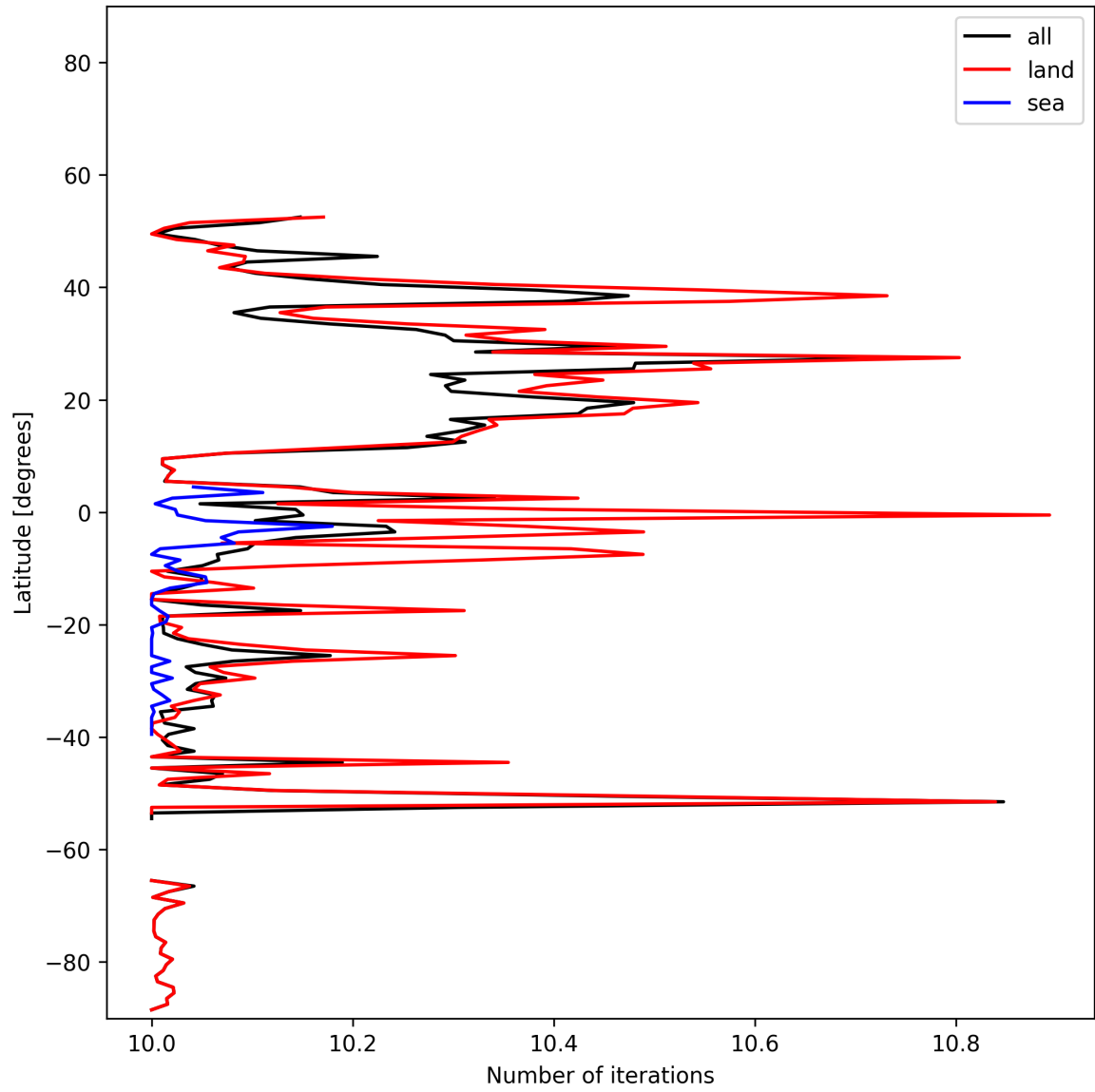
Figure 20: Zonal average of “Number of iterations” for 2025-01-07 to 2025-01-09.
