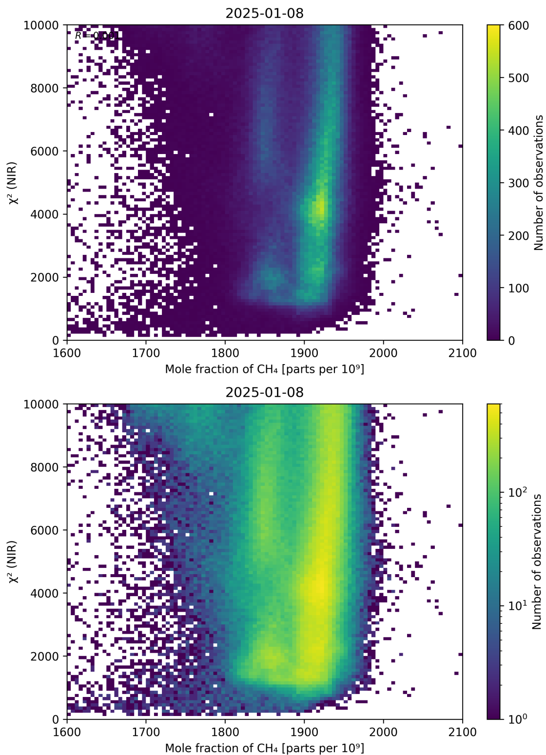
Figure 70: Scatter density plot of “Mole fraction of \text{CH}_4 ” against “ \chi^2 (NIR)” for 2025-01-07 to 2025-01-09.
