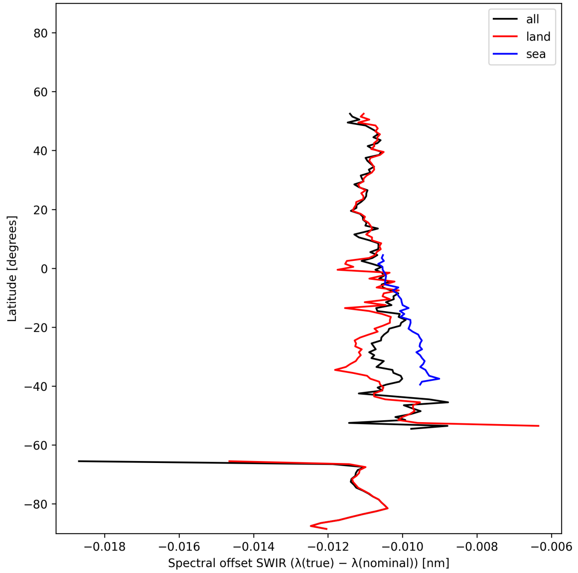
Figure 16: Zonal average of “Spectral offset SWIR ( \lambda_{\text{true}} - \lambda_{\text{nominal}} )” for 2025-01-07 to 2025-01-09.
