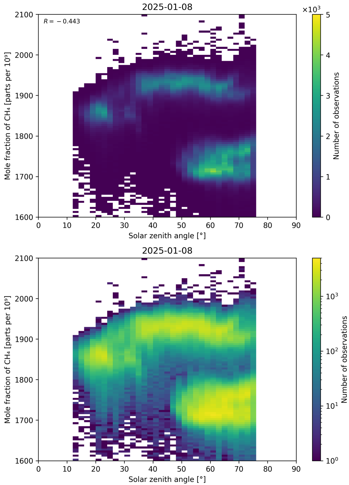
Figure 99: Scatter density plot of “Solar zenith angle” against “Mole fraction of CH 4 ” for 2025-01-07 to 2025-01-09.
