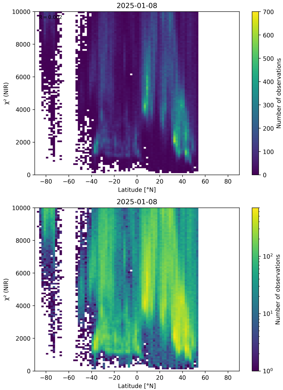
Figure 53: Scatter density plot of “Latitude” against “ \chi^2 (NIR)” for 2025-01-07 to 2025-01-09.
