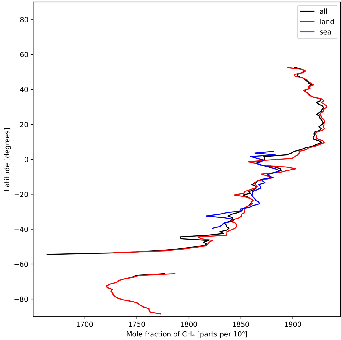
Figure 12: Zonal average of “Mole fraction of CH 4 ” for 2025-01-07 to 2025-01-09.
