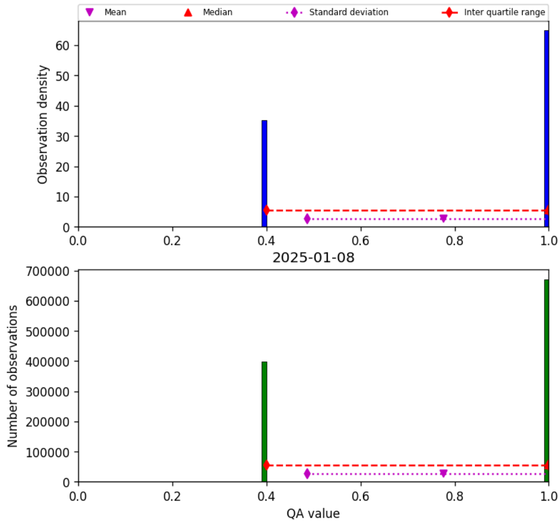
Figure 22: Histogram of “QA value” for 2025-01-07 to 2025-01-09
