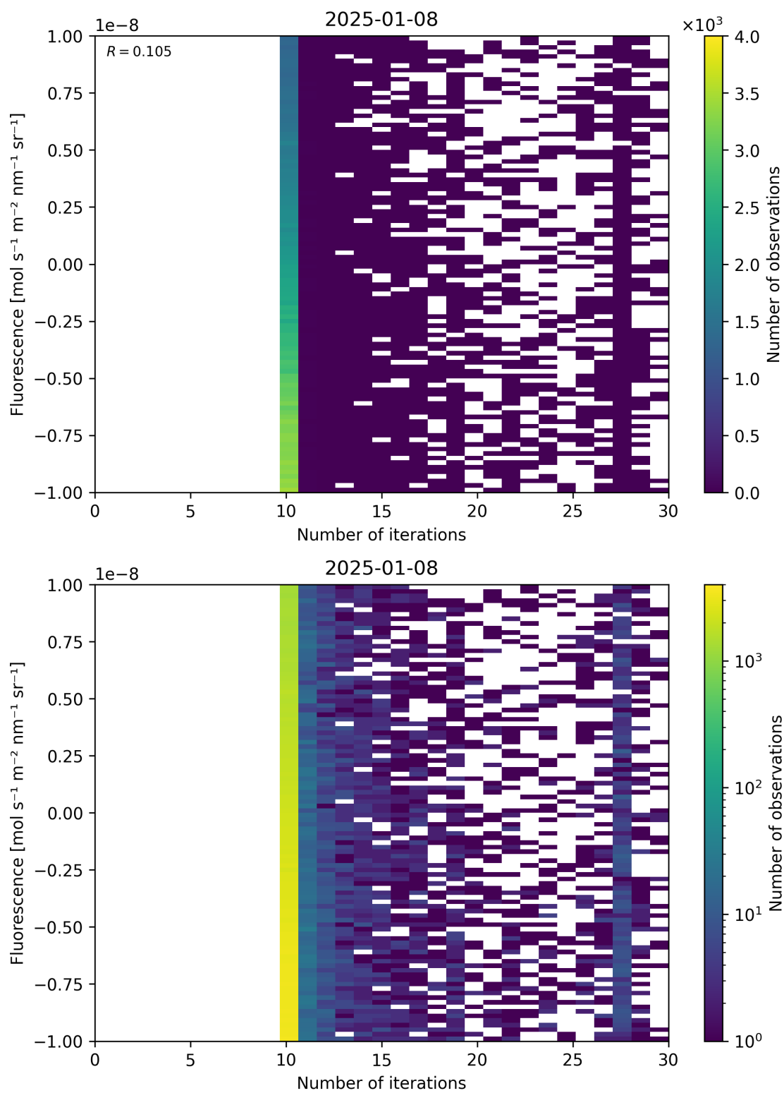
Figure 87: Scatter density plot of “Number of iterations” against “Fluorescence” for 2025-01-07 to 2025-01-09.
