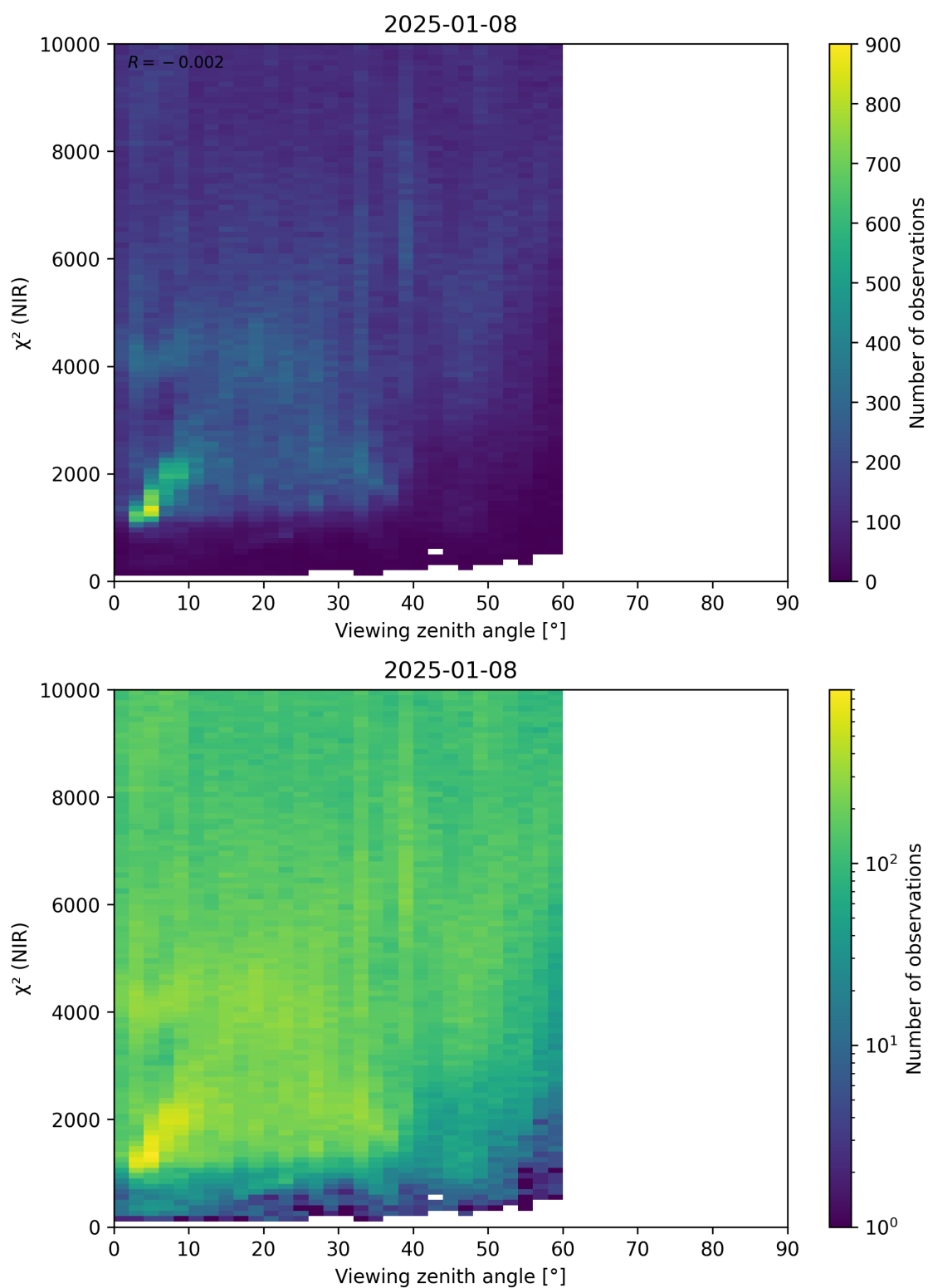
Figure 105: Scatter density plot of “Viewing zenith angle” against “ \chi^2 (NIR)” for 2025-01-07 to 2025-01-09.
