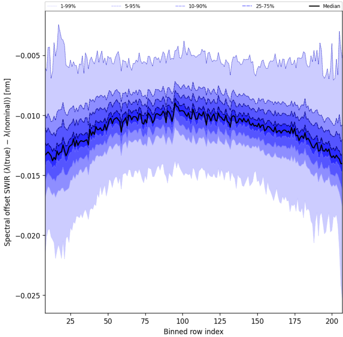
Figure 38: Along track statistics of “Spectral offset SWIR ( \lambda_{\text{true}} - \lambda_{\text{nominal}} )” for 2025-01-07 to 2025-01-09
