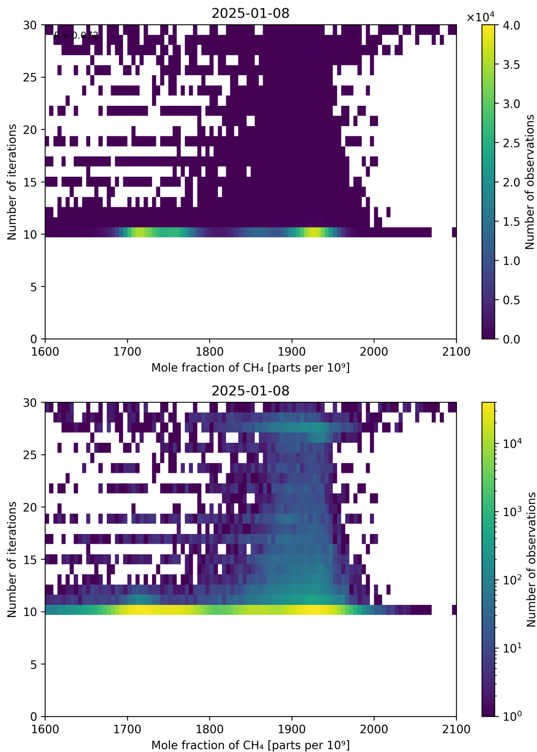
Figure 76: Scatter density plot of “Mole fraction of CH 4 ” against “Number of iterations” for 2025-01-07 to 2025-01-09.
