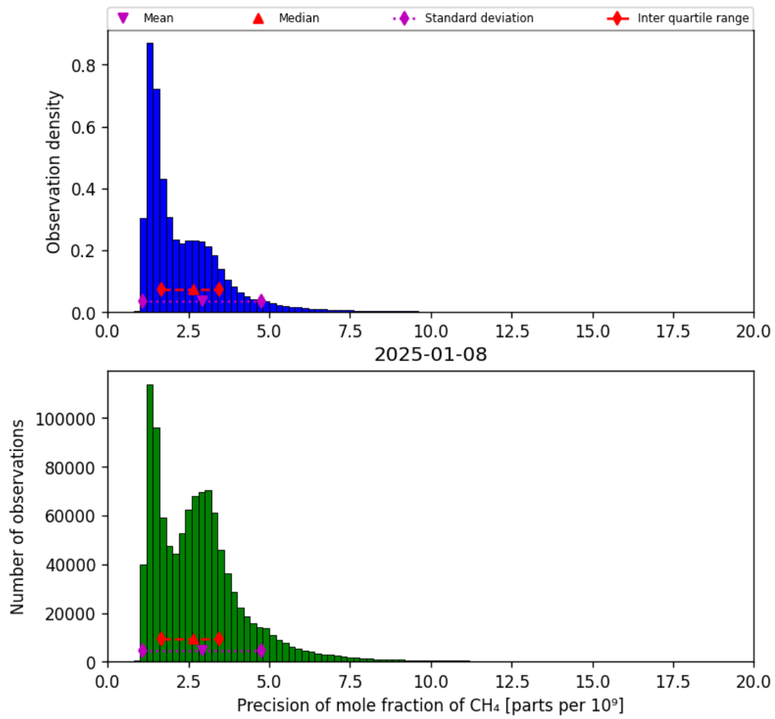
Figure 24: Histogram of “Precision of mole fraction of CH 4 ” for 2025-01-07 to 2025-01-09
