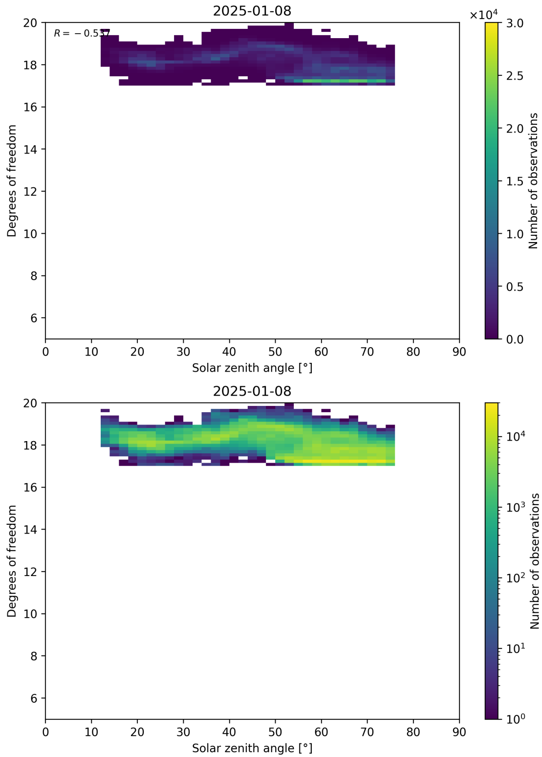
Figure 96: Scatter density plot of “Solar zenith angle” against “Degrees of freedom” for 2025-01-07 to 2025-01-09.
