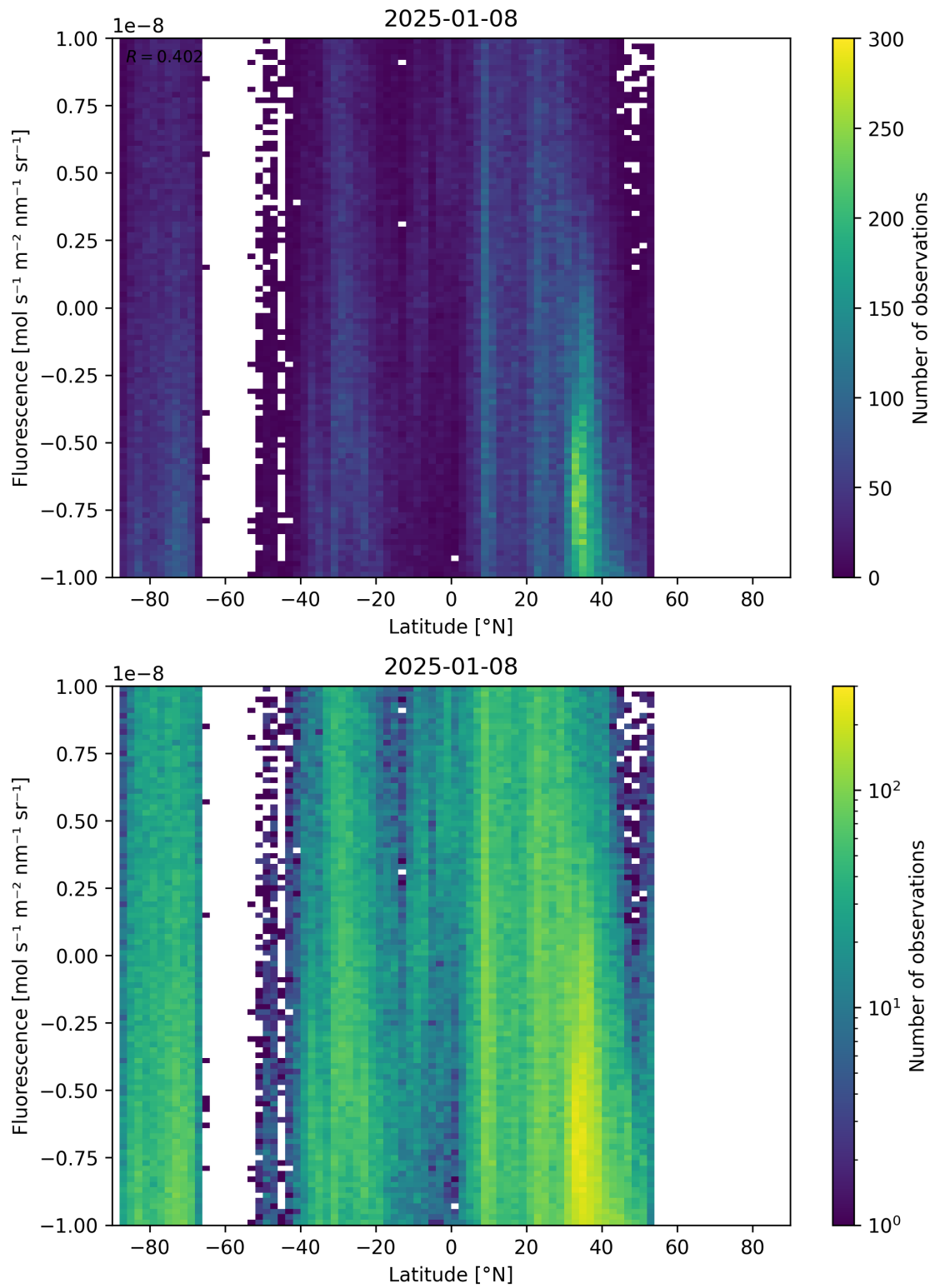
Figure 56: Scatter density plot of “Latitude” against “Fluorescence” for 2025-01-07 to 2025-01-09.
