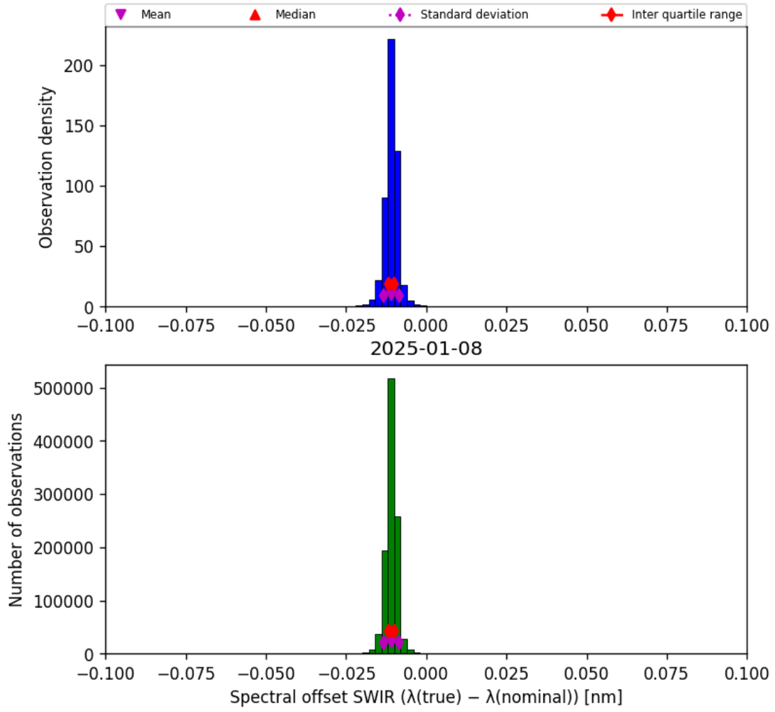
Figure 27: Histogram of “Spectral offset SWIR ( \lambda_{\text{true}} - \lambda_{\text{nominal}} )” for 2025-01-07 to 2025-01-09
