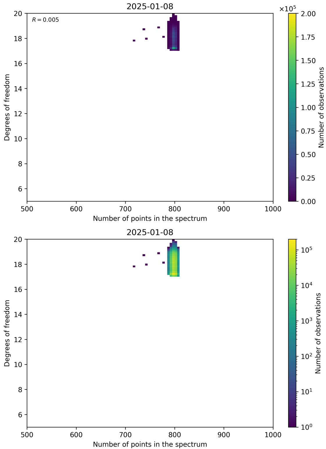
Figure 90: Scatter density plot of “Number of points in the spectrum” against “Degrees of freedom” for 2025-01-07 to 2025-01-09.
