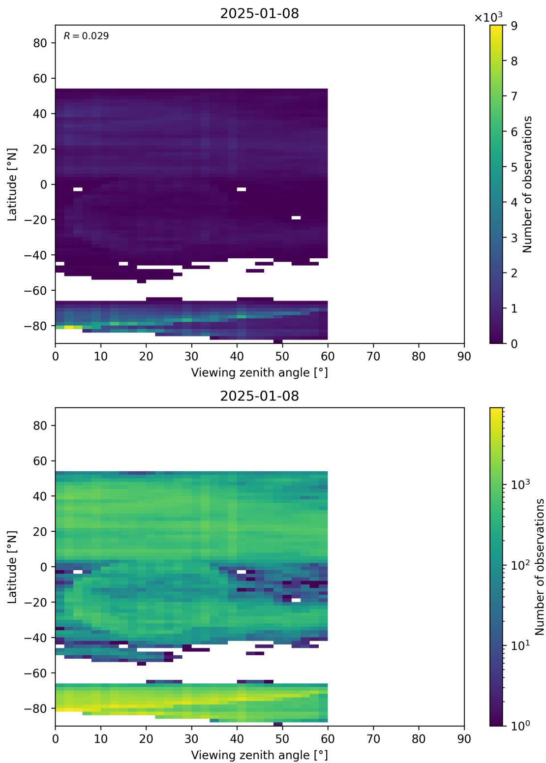
Figure 109: Scatter density plot of “Viewing zenith angle” against “Latitude” for 2025-01-07 to 2025-01-09.
