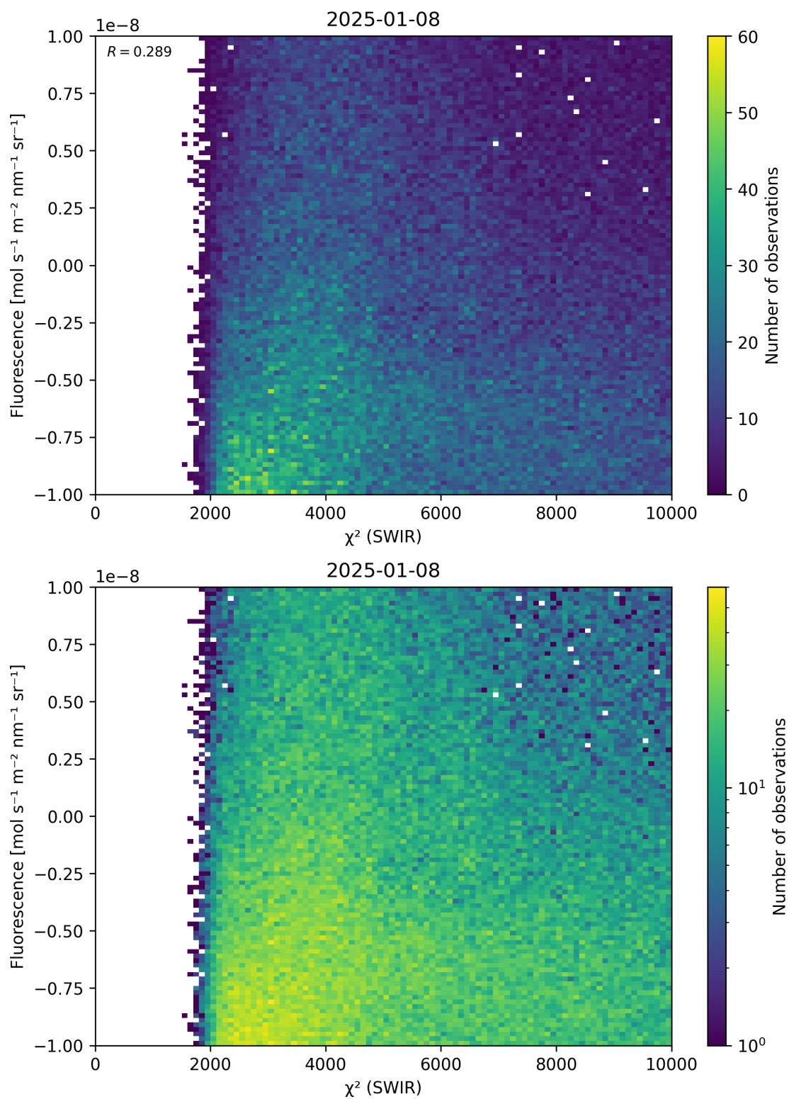
Figure 49: Scatter density plot of “ \chi^2 (SWIR)” against “Fluorescence” for 2025-01-07 to 2025-01-09.
