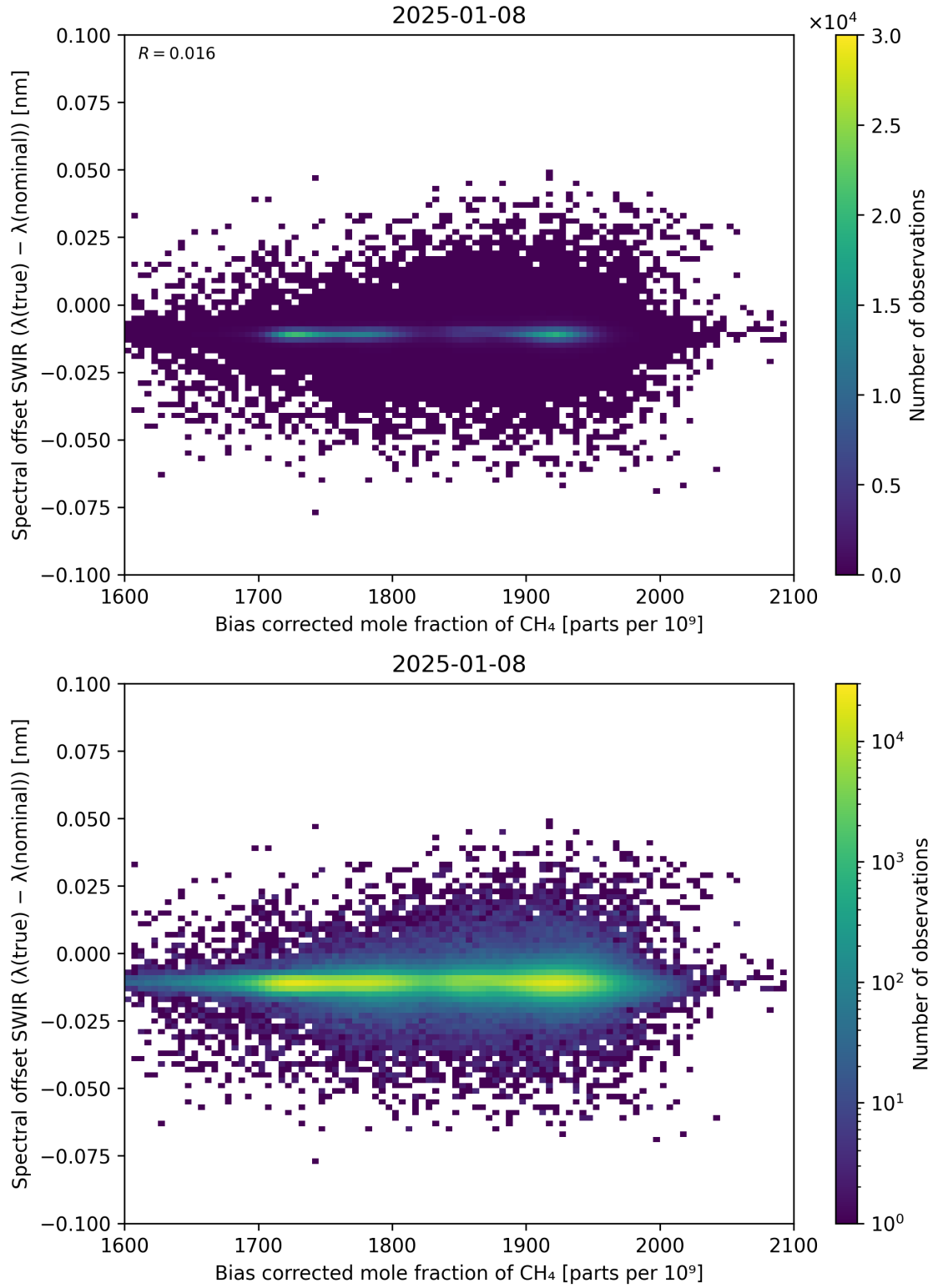
Figure 69: Scatter density plot of “Bias corrected mole fraction of CH 4 ” against “Spectral offset SWIR ( \lambda_{\text{true}} - \lambda_{\text{nominal}} )” for 2025-01-07 to 2025-01-09.
