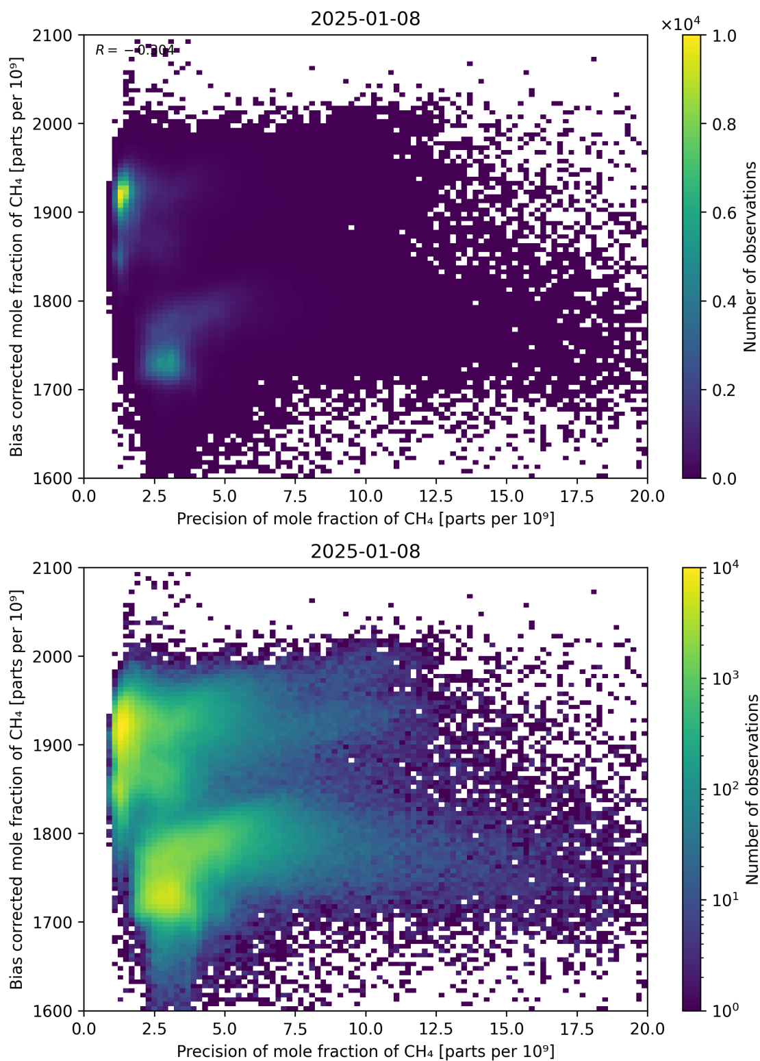
Figure 82: Scatter density plot of “Precision of mole fraction of CH 4 ” against “Bias corrected mole fraction of CH 4 ” for 2025-01-07 to 2025-01-09.
