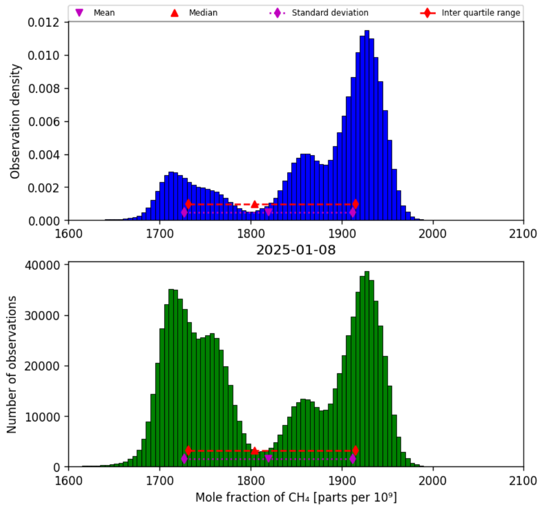
Figure 23: Histogram of “Mole fraction of CH 4 ” for 2025-01-07 to 2025-01-09
