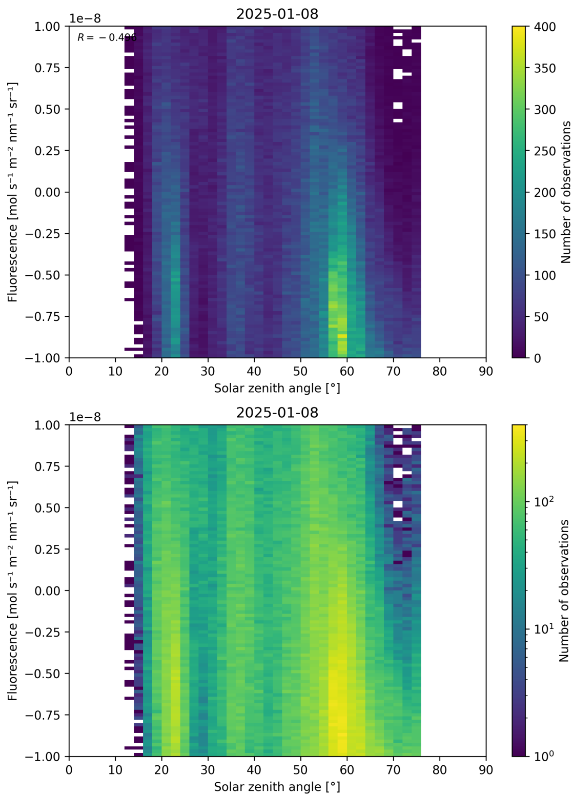
Figure 97: Scatter density plot of “Solar zenith angle” against “Fluorescence” for 2025-01-07 to 2025-01-09.
