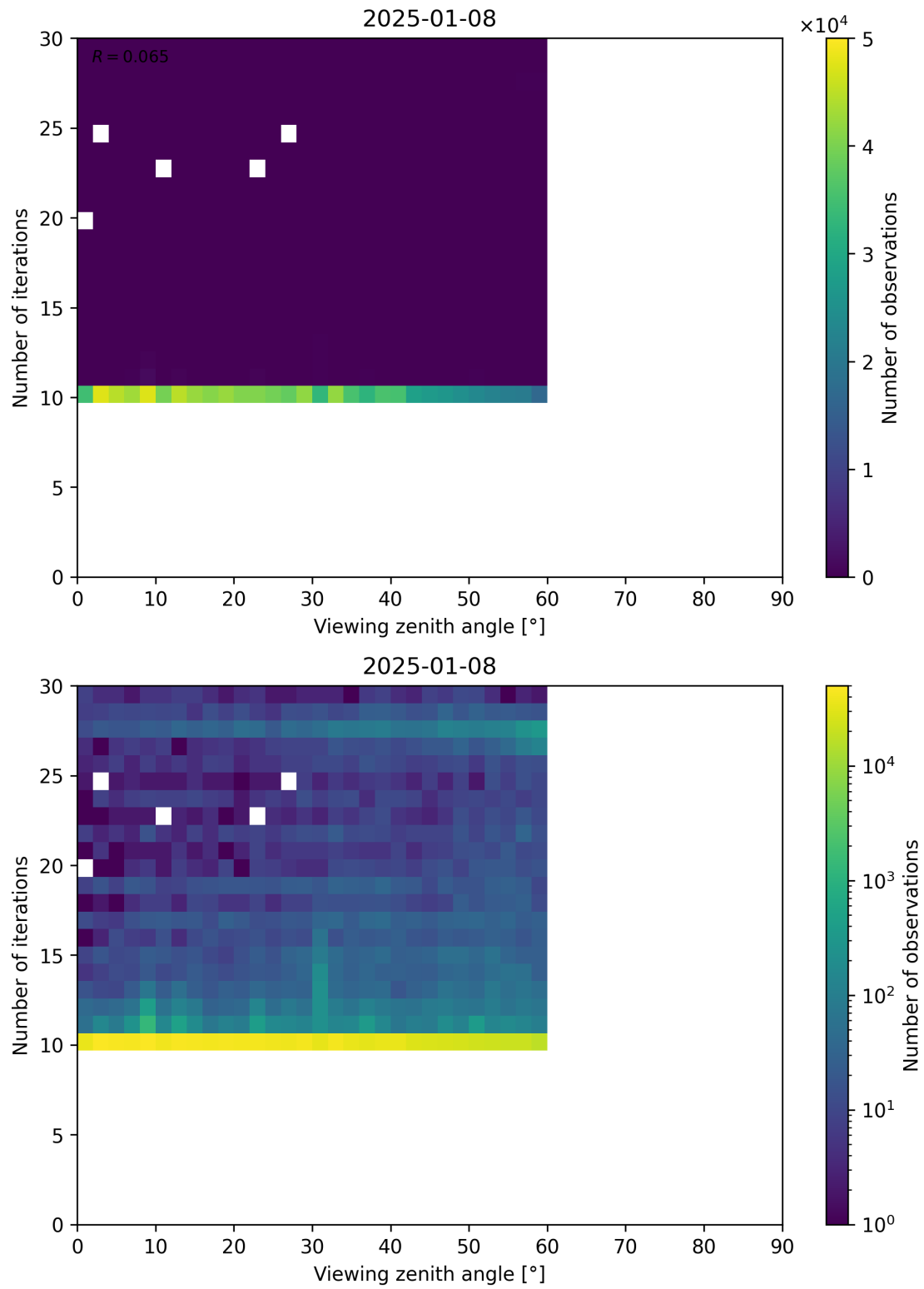
Figure 113: Scatter density plot of “Viewing zenith angle” against “Number of iterations” for 2025-01-07 to 2025-01-09.
