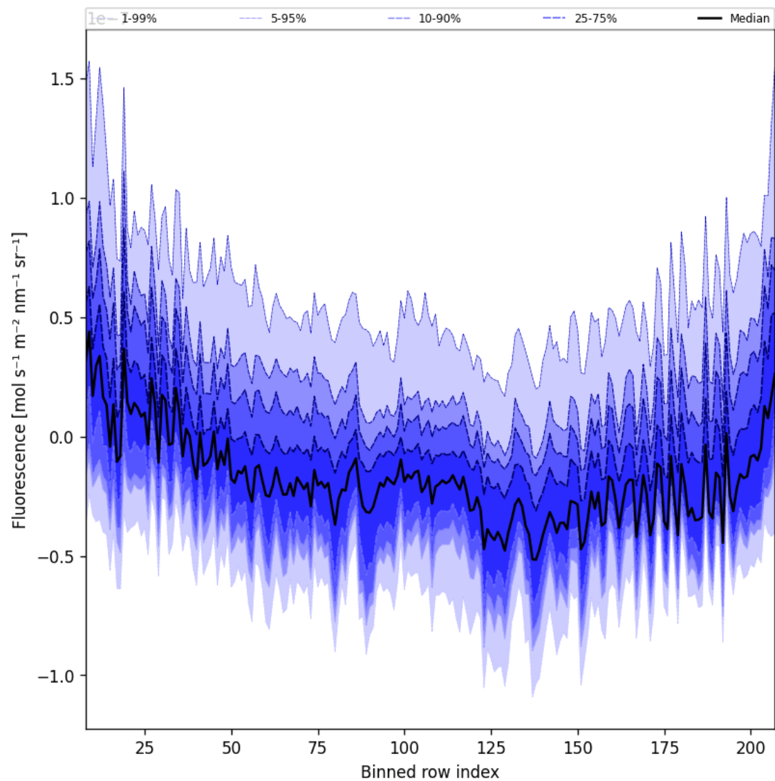
Figure 43: Along track statistics of “Fluorescence” for 2025-01-07 to 2025-01-09
