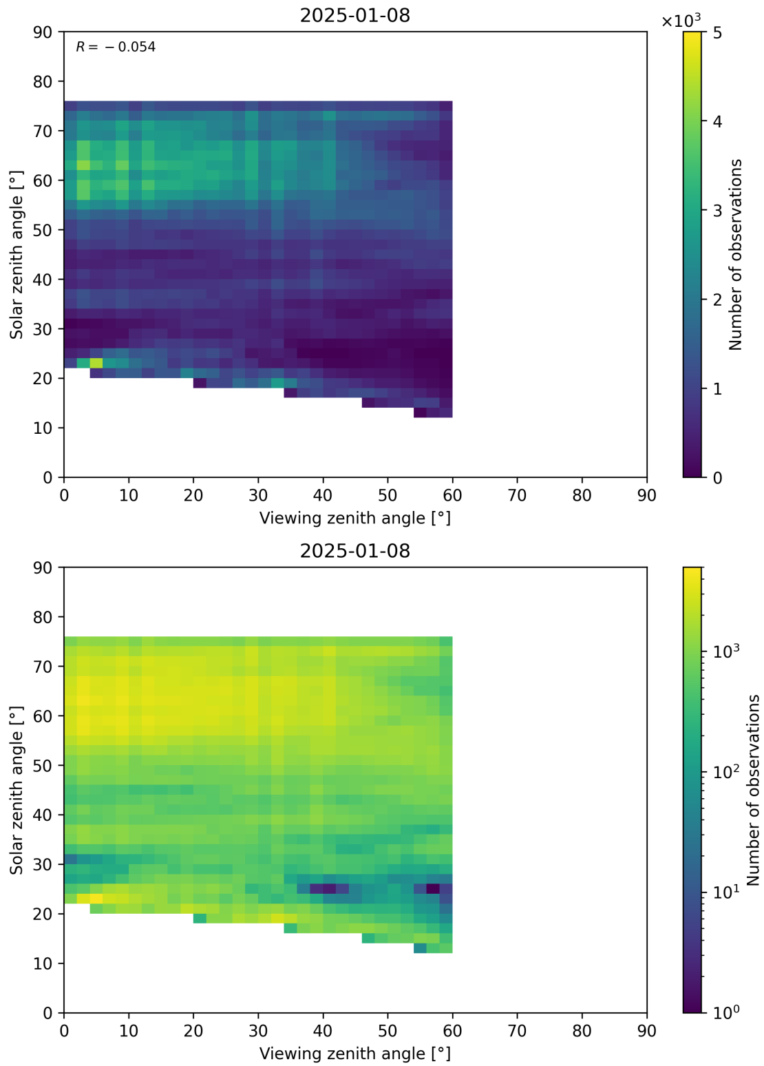
Figure 115: Scatter density plot of “Viewing zenith angle” against “Solar zenith angle” for 2025-01-07 to 2025-01-09.
