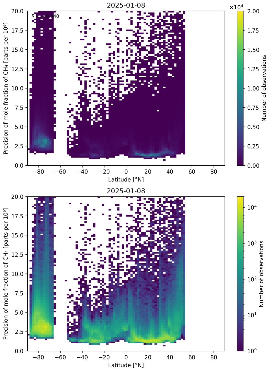
Figure 59: Scatter density plot of “Latitude” against “Precision of mole fraction of CH 4 ” for 2025-01-07 to 2025-01-09.
