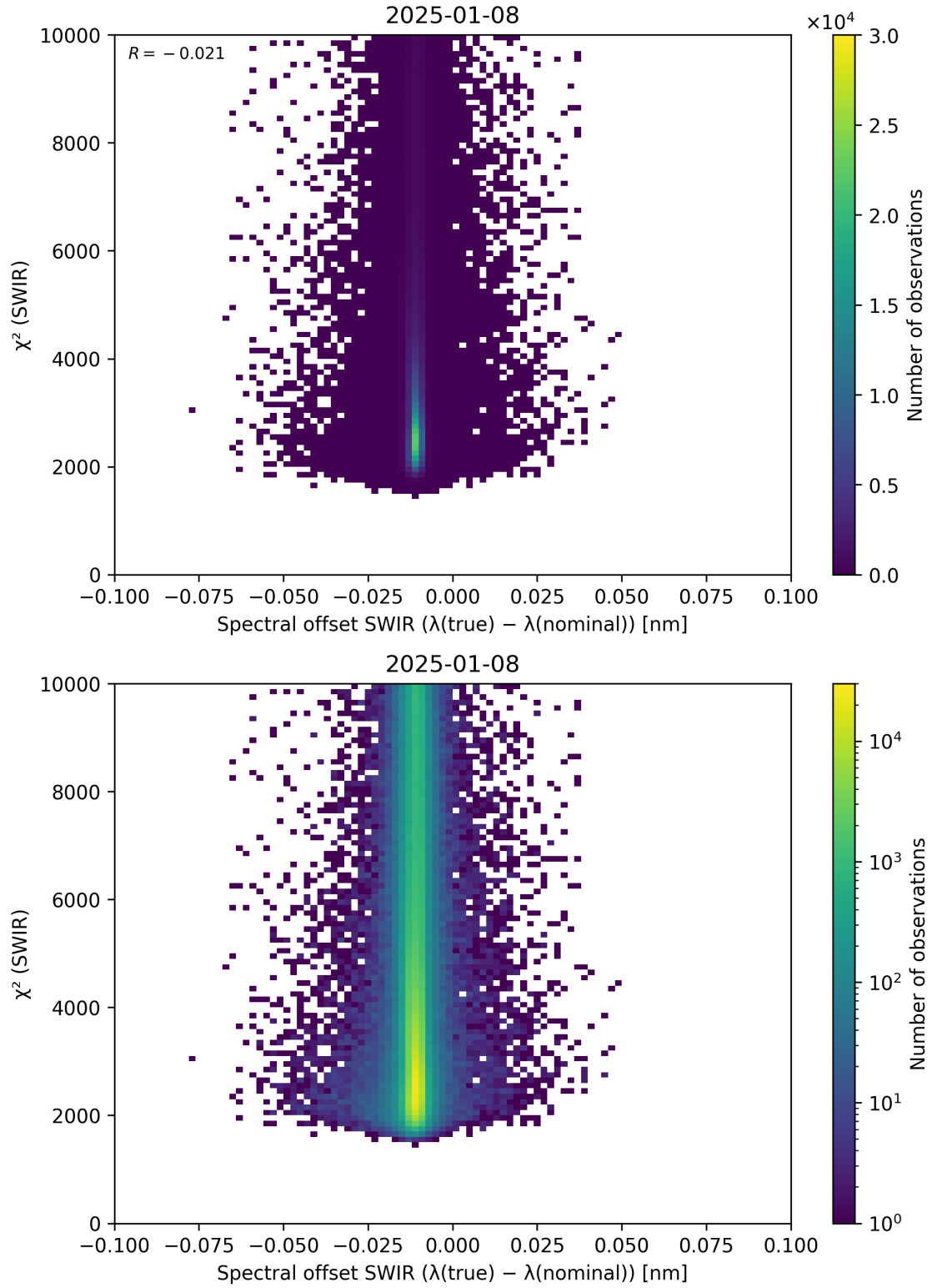
Figure 118: Scatter density plot of “Spectral offset SWIR ( \lambda_{\text{true}} - \lambda_{\text{nominal}} )” against “ \chi^2 (SWIR)” for 2025-01-07 to 2025-01-09.
