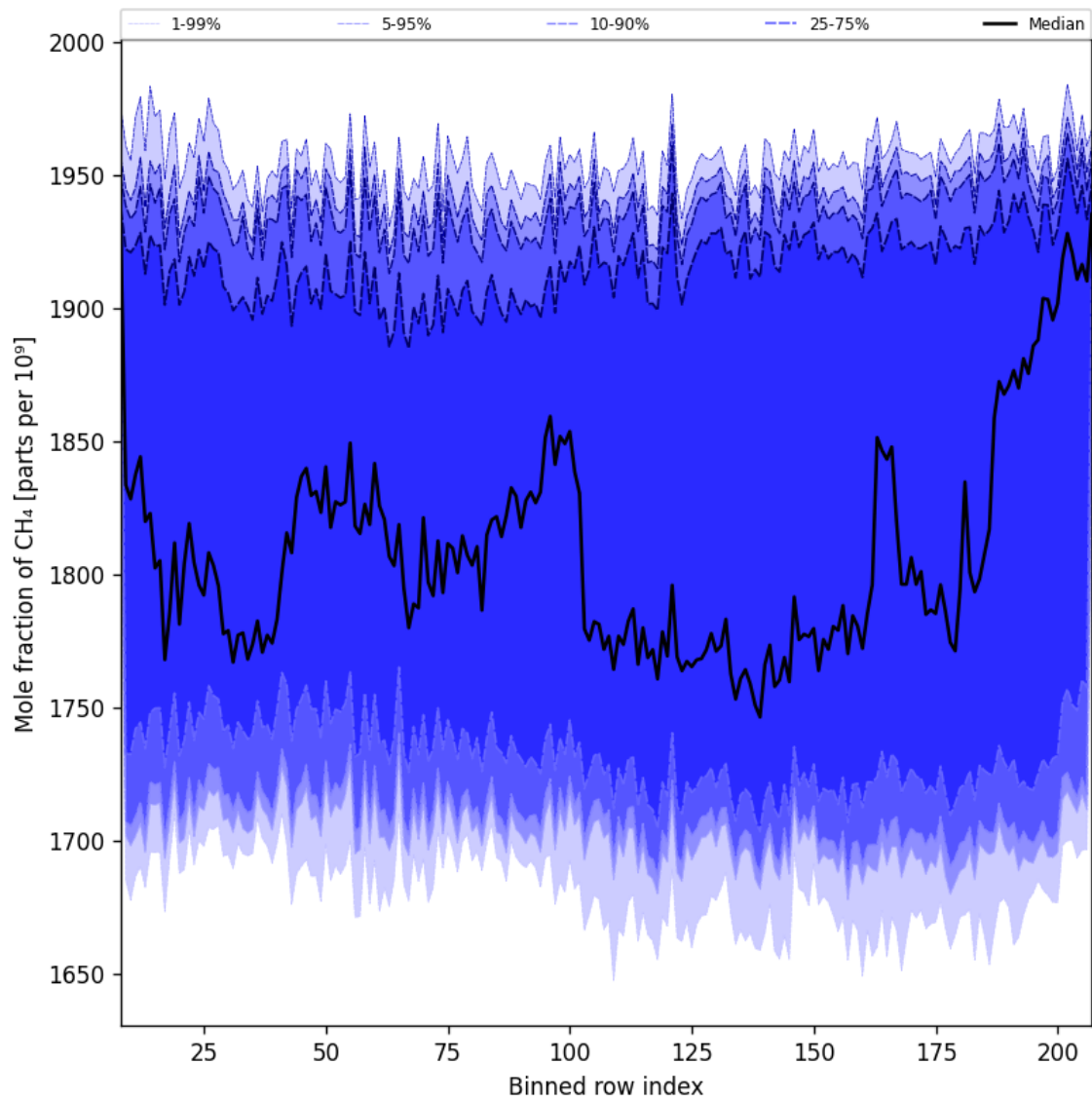
Figure 34: Along track statistics of “Mole fraction of CH 4 ” for 2025-01-07 to 2025-01-09
