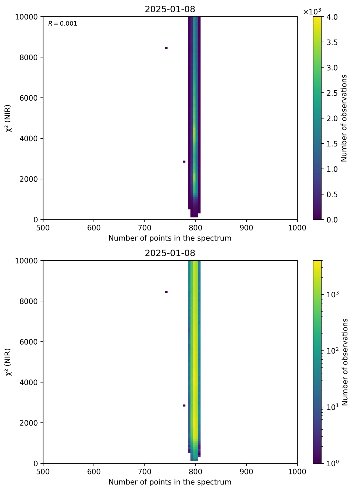
Figure 88: Scatter density plot of “Number of points in the spectrum” against “ \chi^2 (NIR)” for 2025-01-07 to 2025-01-09.
