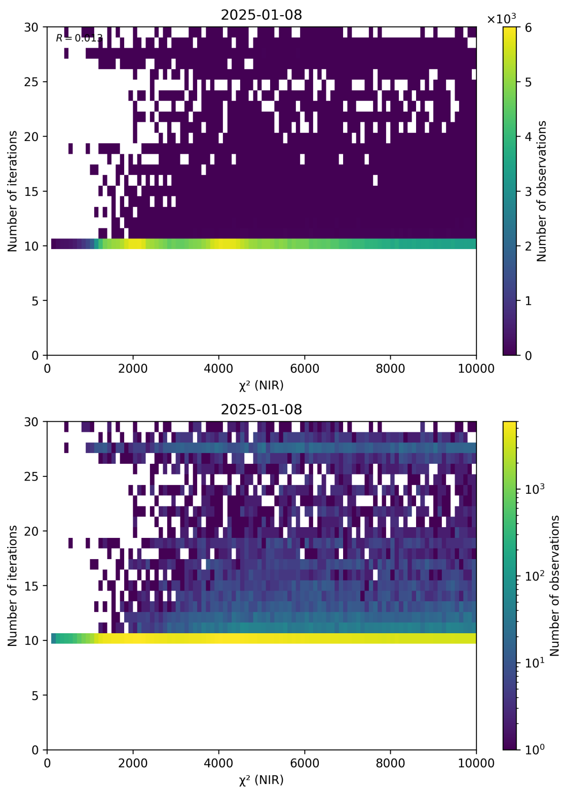
Figure 46: Scatter density plot of “ \chi^2 (NIR)” against “Number of iterations” for 2025-01-07 to 2025-01-09.
