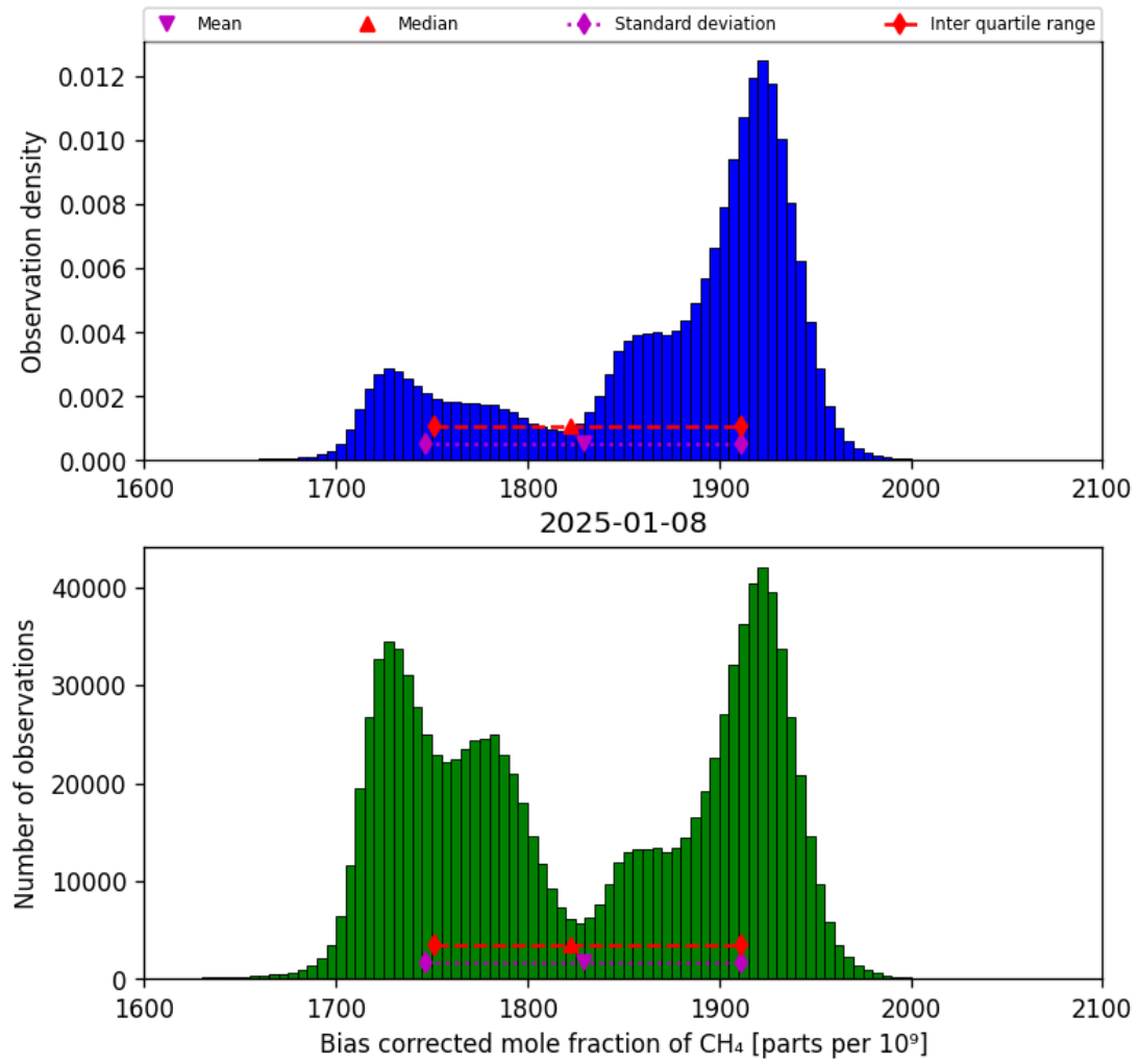
Figure 25: Histogram of “Bias corrected mole fraction of CH 4 ” for 2025-01-07 to 2025-01-09
