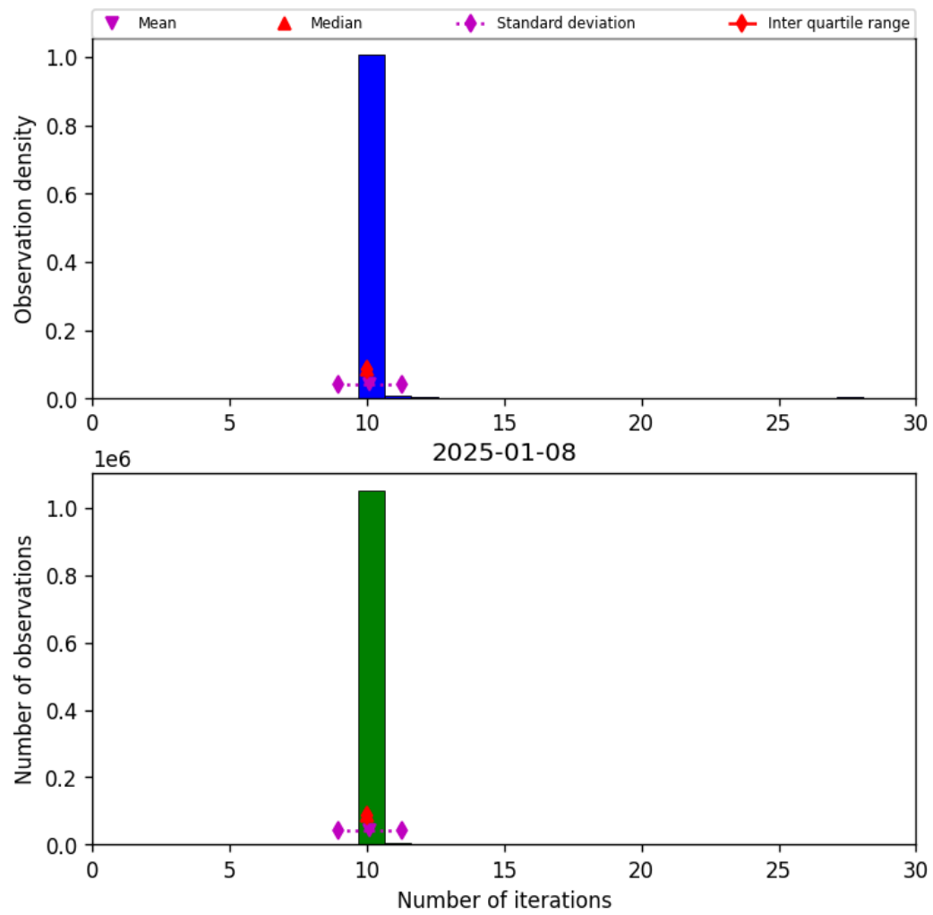
Figure 31: Histogram of “Number of iterations” for 2025-01-07 to 2025-01-09
