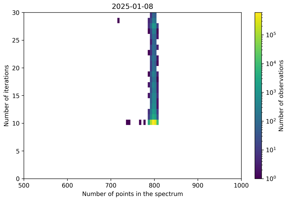
Figure 92: Scatter density plot of “Number of points in the spectrum” against “Number of iterations” for 2025-01-07 to 2025-01-09.
