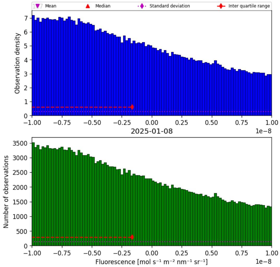
Figure 32: Histogram of “Fluorescence” for 2025-01-07 to 2025-01-09
