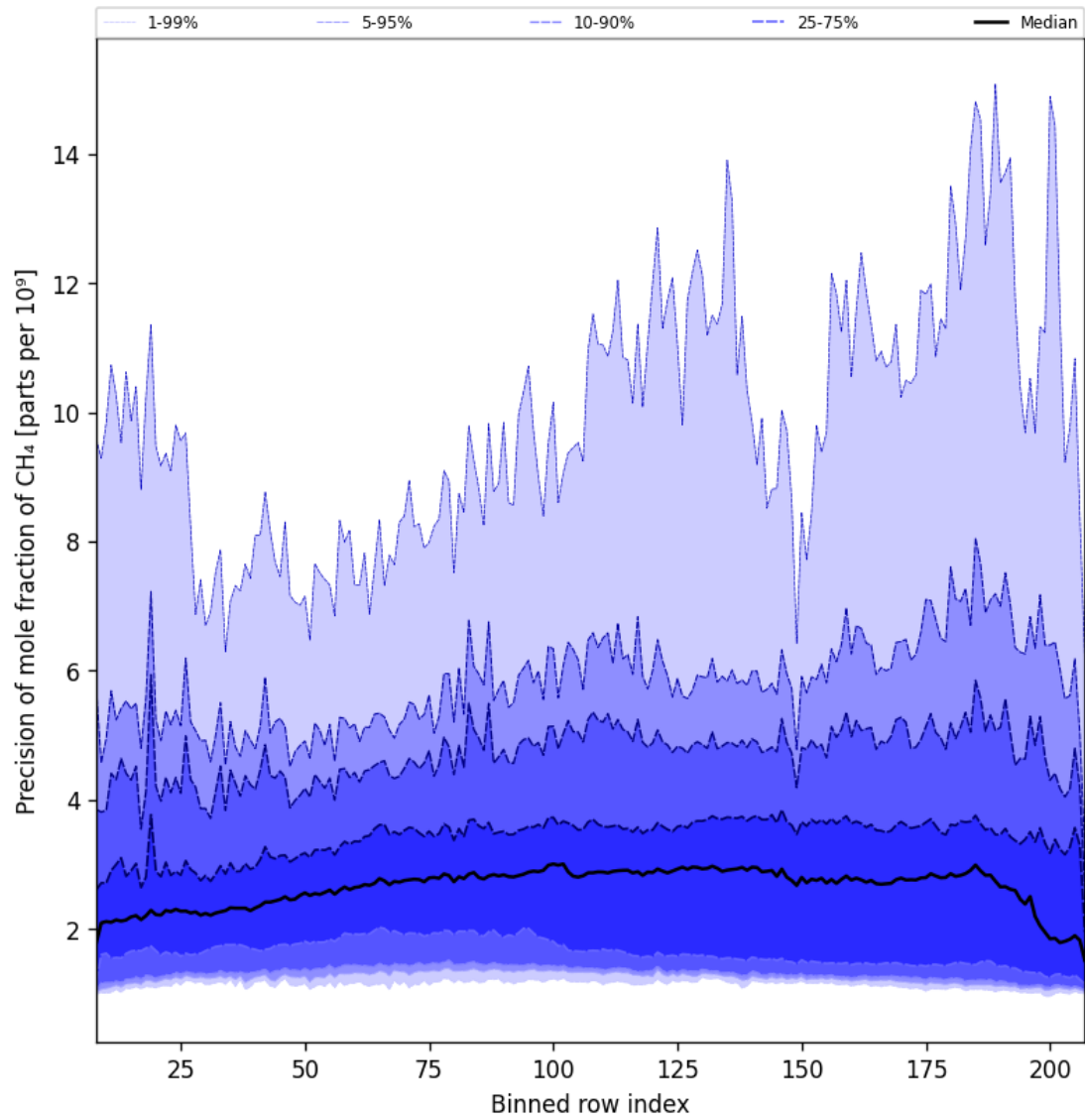
Figure 35: Along track statistics of “Precision of mole fraction of CH 4 ” for 2025-01-07 to 2025-01-09
