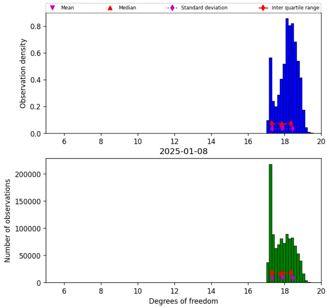
Figure 30: Histogram of “Degrees of freedom” for 2025-01-07 to 2025-01-09
