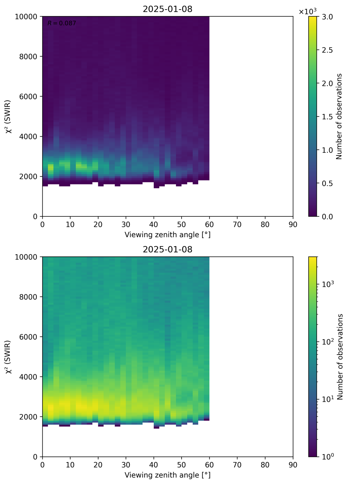
Figure 106: Scatter density plot of “Viewing zenith angle” against “ \chi^2 (SWIR)” for 2025-01-07 to 2025-01-09.
