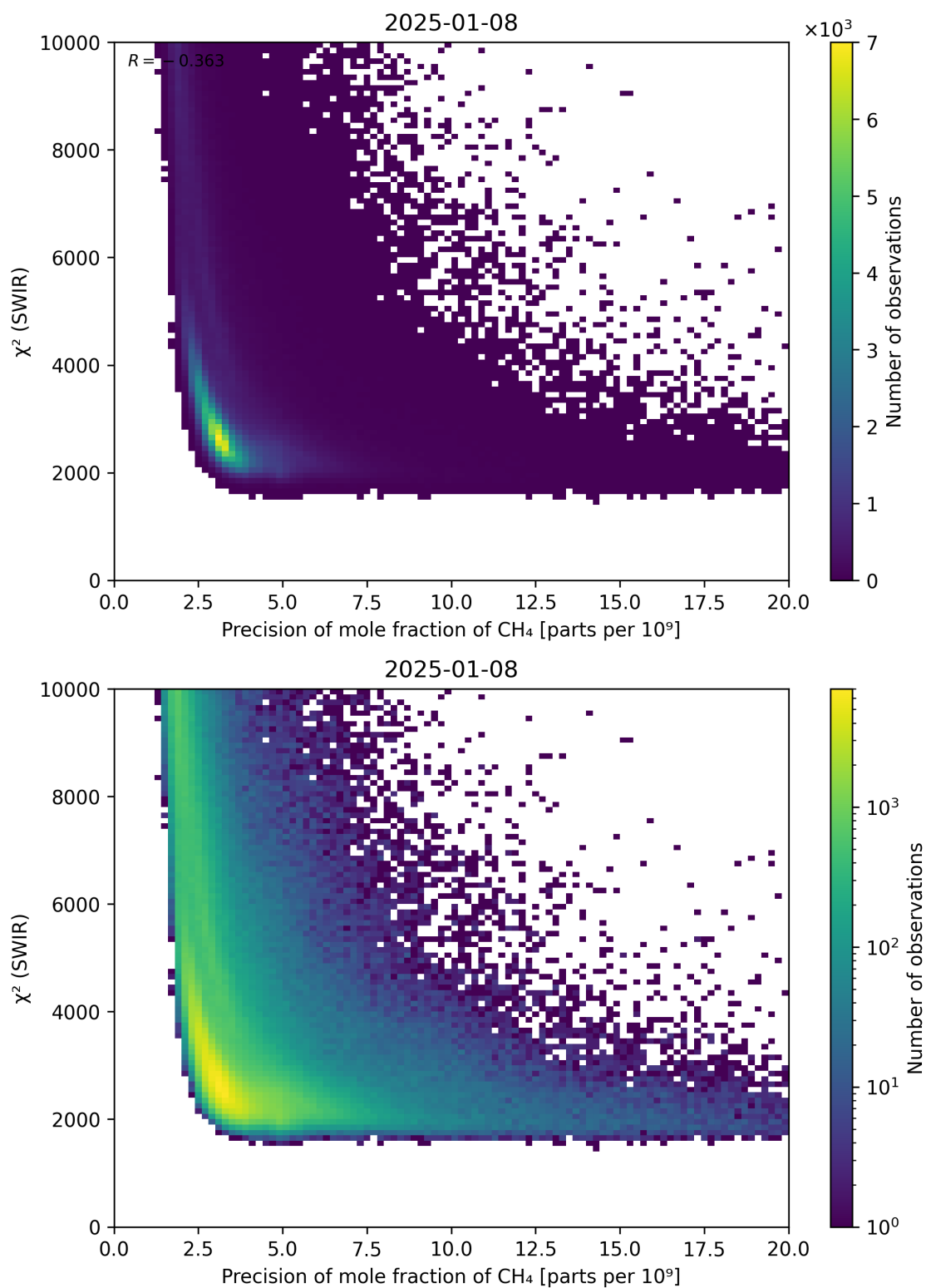
Figure 79: Scatter density plot of “Precision of mole fraction of \text{CH}_4 ” against “ \chi^2 (SWIR)” for 2025-01-07 to 2025-01-09.
