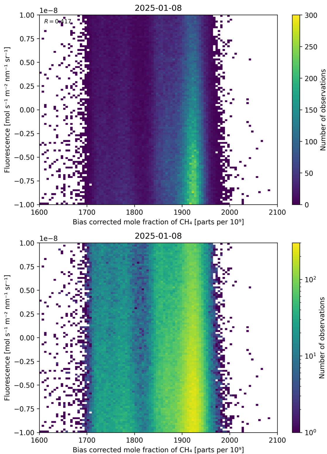
Figure 66: Scatter density plot of “Bias corrected mole fraction of \text{CH}_4 ” against “Fluorescence” for 2025-01-07 to 2025-01-09.
