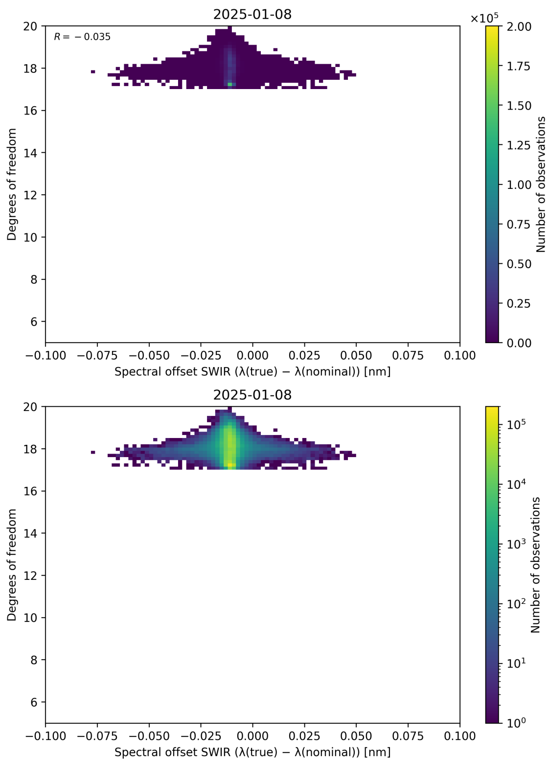
Figure 119: Scatter density plot of “Spectral offset SWIR ( \lambda_{\text{true}} - \lambda_{\text{nominal}} )” against “Degrees of freedom” for 2025-01-07 to 2025-01-09.
