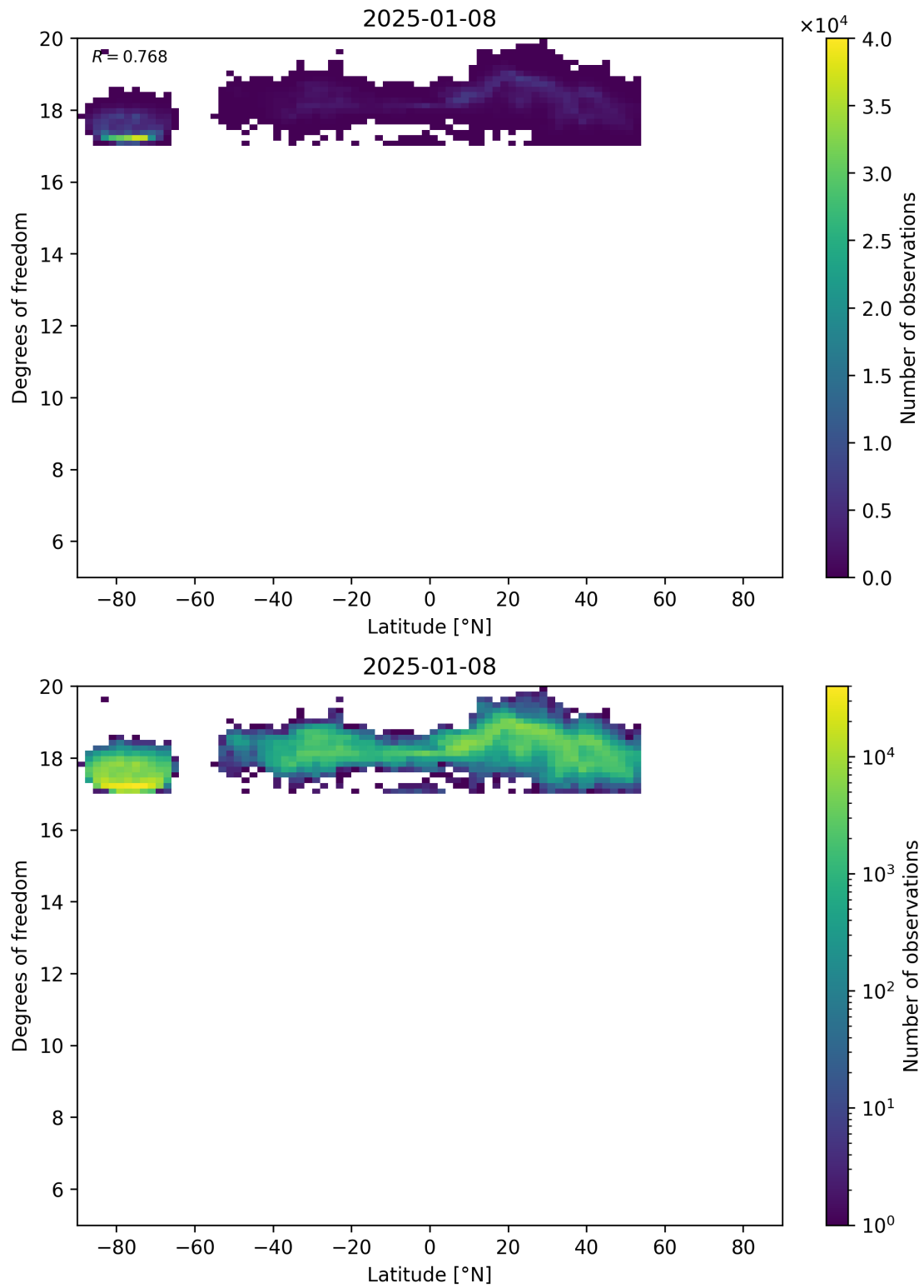
Figure 55: Scatter density plot of “Latitude” against “Degrees of freedom” for 2025-01-07 to 2025-01-09.
