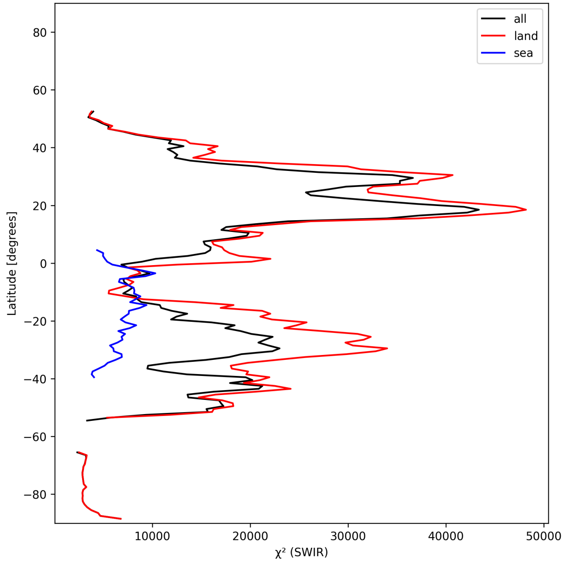
Figure 17: Zonal average of “ \chi^2 (SWIR)” for 2025-01-07 to 2025-01-09.
