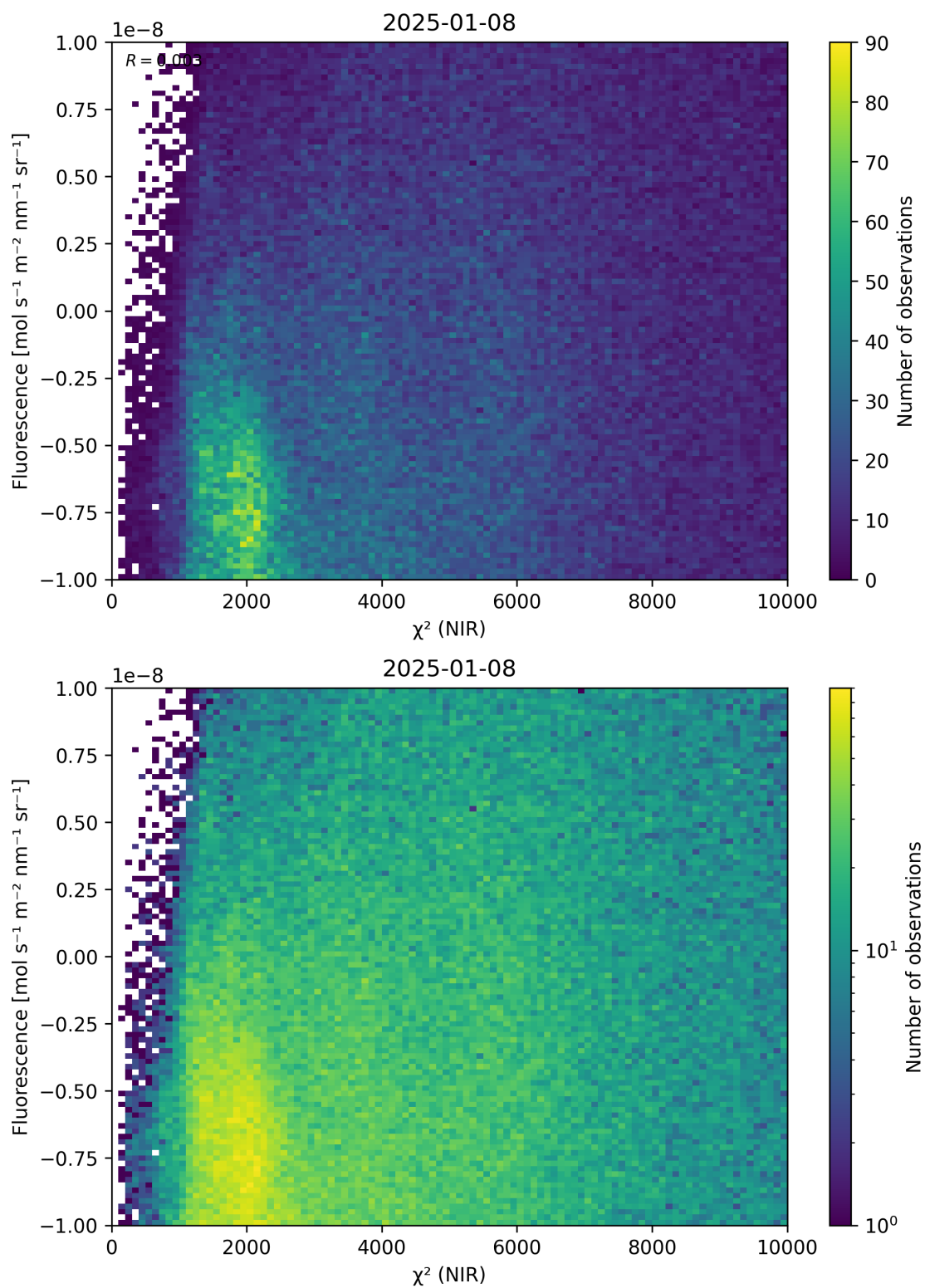
Figure 45: Scatter density plot of “ \chi^2 (NIR)” against “Fluorescence” for 2025-01-07 to 2025-01-09.
