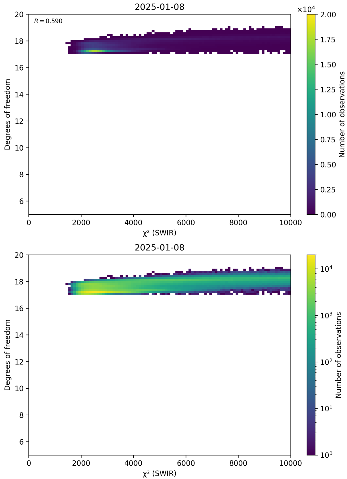
Figure 48: Scatter density plot of “ \chi^2 (SWIR)” against “Degrees of freedom” for 2025-01-07 to 2025-01-09.
