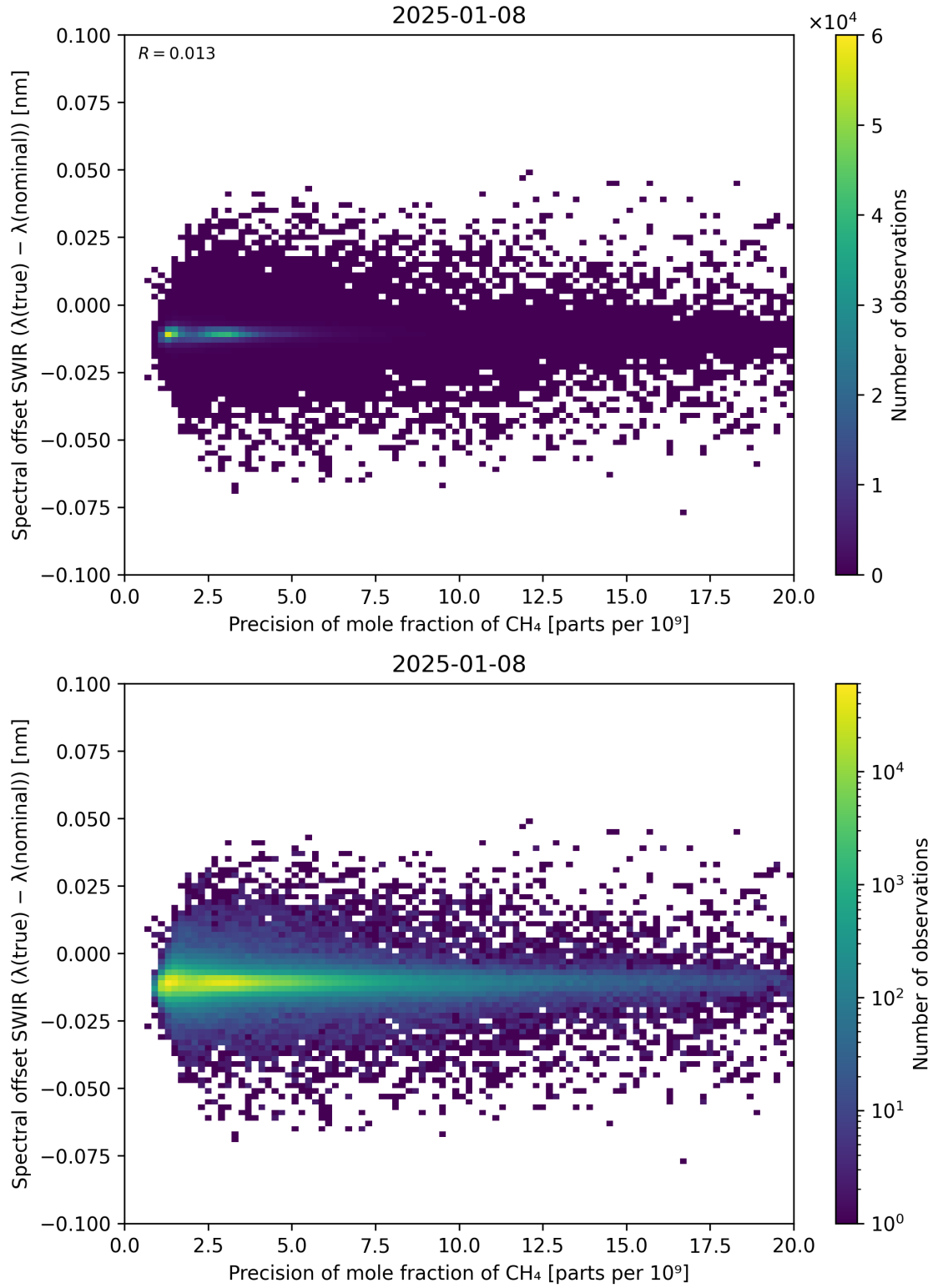
Figure 85: Scatter density plot of “Precision of mole fraction of CH 4 ” against “Spectral offset SWIR ( \lambda_{\text{true}} - \lambda_{\text{nominal}} )” for 2025-01-07 to 2025-01-09.
