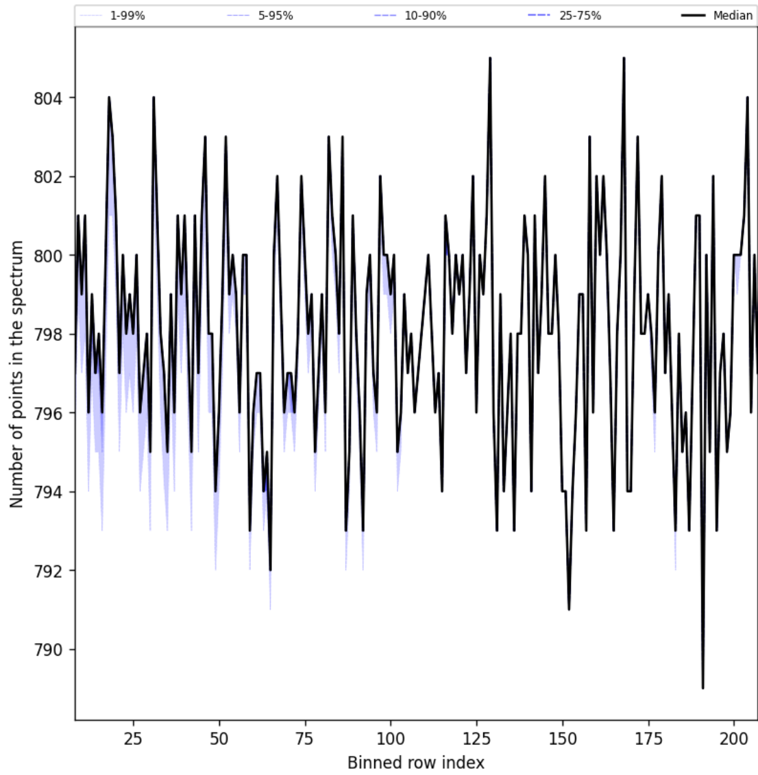
Figure 37: Along track statistics of “Number of points in the spectrum” for 2025-01-07 to 2025-01-09
