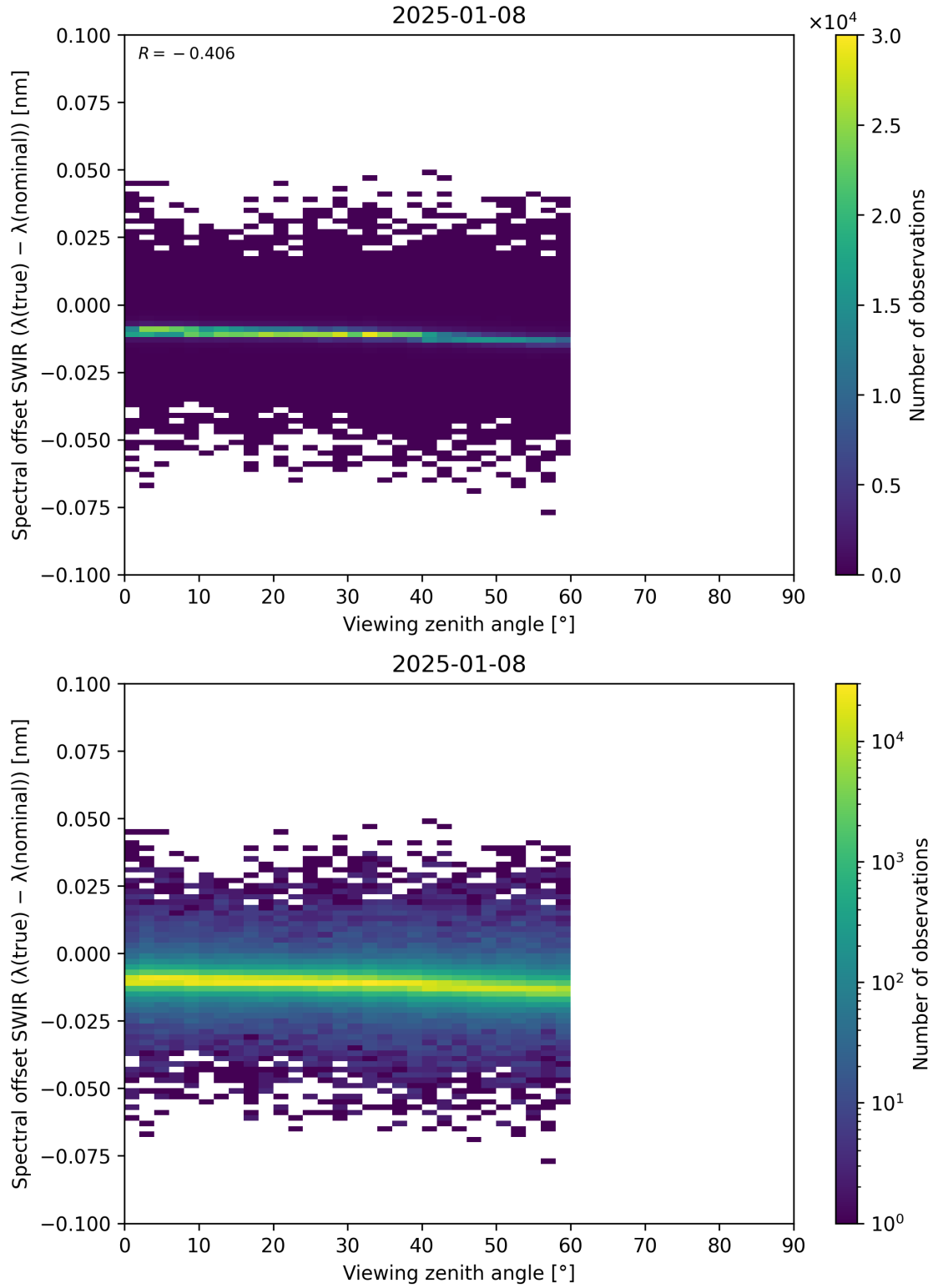
Figure 116: Scatter density plot of “Viewing zenith angle” against “Spectral offset SWIR ( \lambda_{\text{true}} - \lambda_{\text{nominal}} )” for 2025-01-07 to 2025-01-09.
