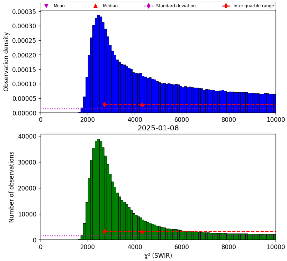
Figure 28: Histogram of “ \chi^2 (SWIR)” for 2025-01-07 to 2025-01-09
