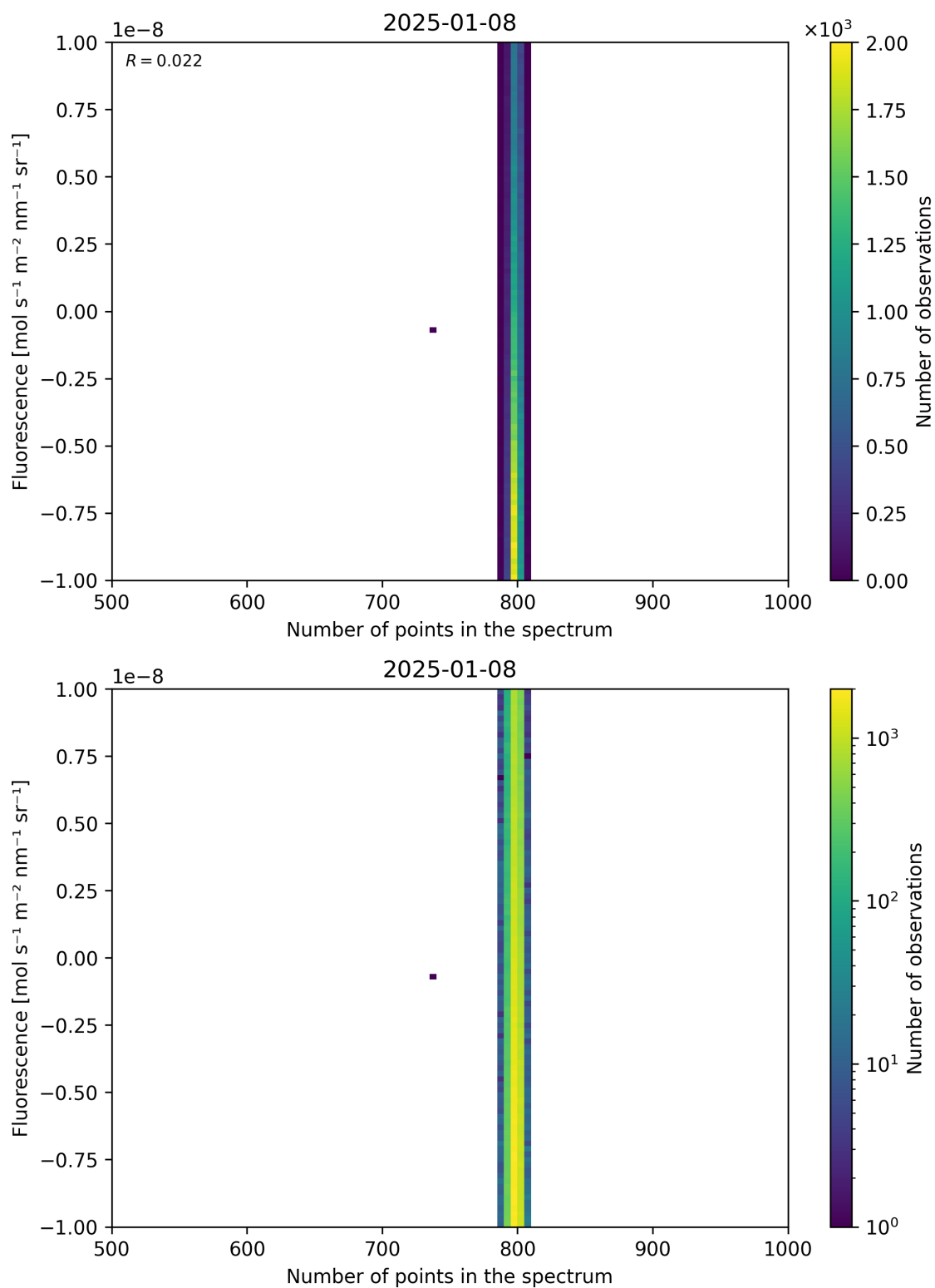
Figure 91: Scatter density plot of “Number of points in the spectrum” against “Fluorescence” for 2025-01-07 to 2025-01-09.
