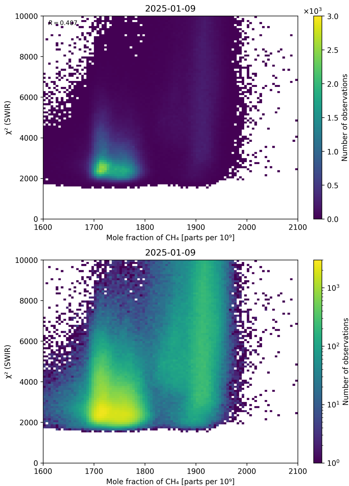
Figure 71: Scatter density plot of “Mole fraction of \text{CH}_4 ” against “ \chi^2 (SWIR)” for 2025-01-08 to 2025-01-10.
