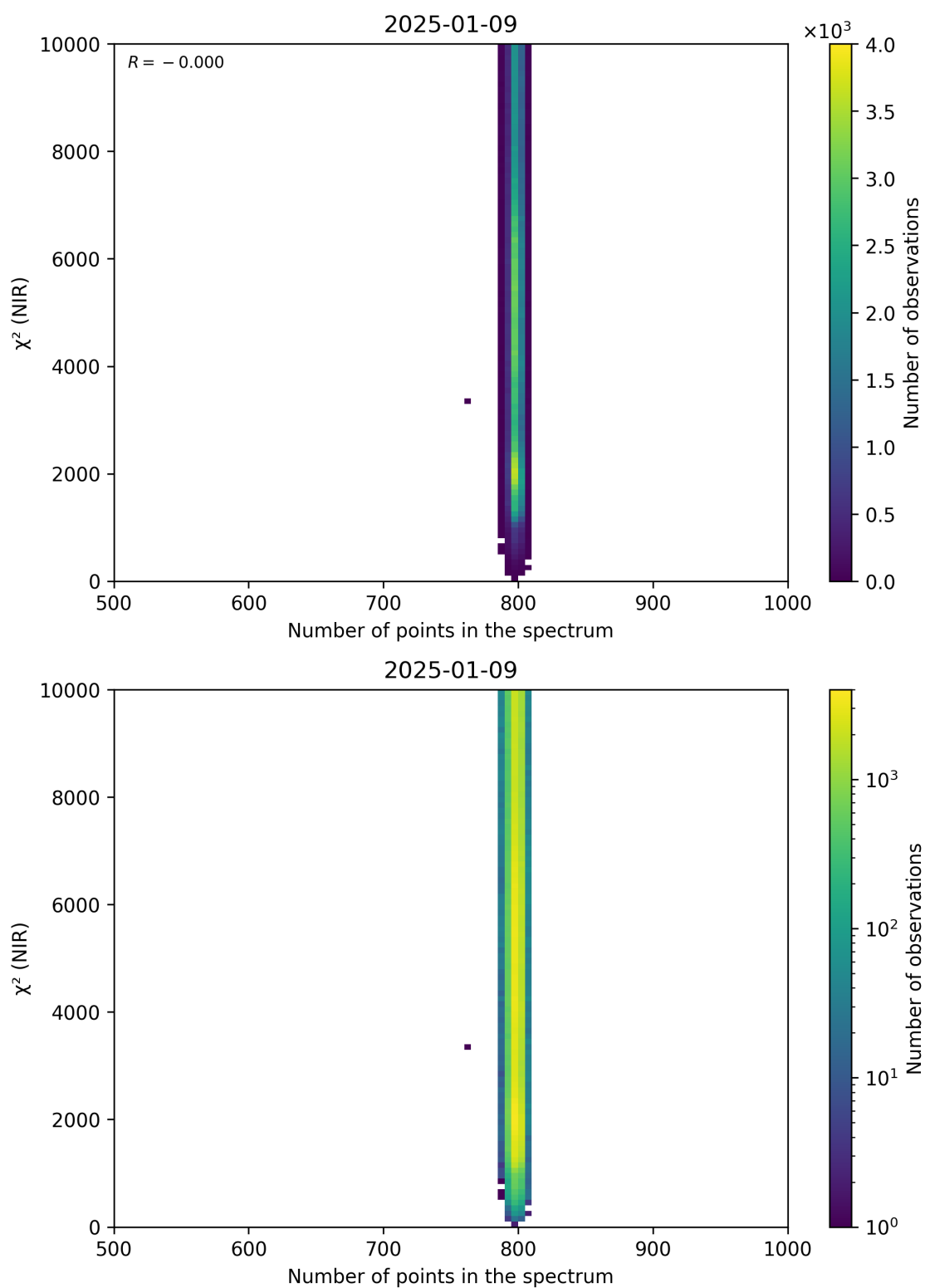
Figure 88: Scatter density plot of “Number of points in the spectrum” against “ \chi^2 (NIR)” for 2025-01-08 to 2025-01-10.
