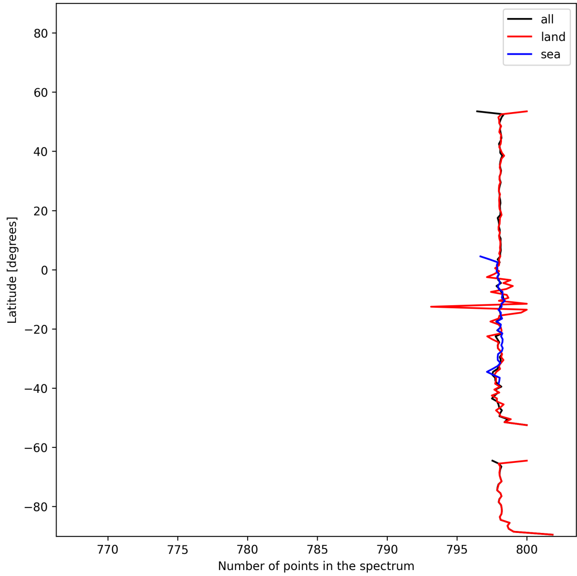
Figure 15: Zonal average of “Number of points in the spectrum” for 2025-01-08 to 2025-01-10.
