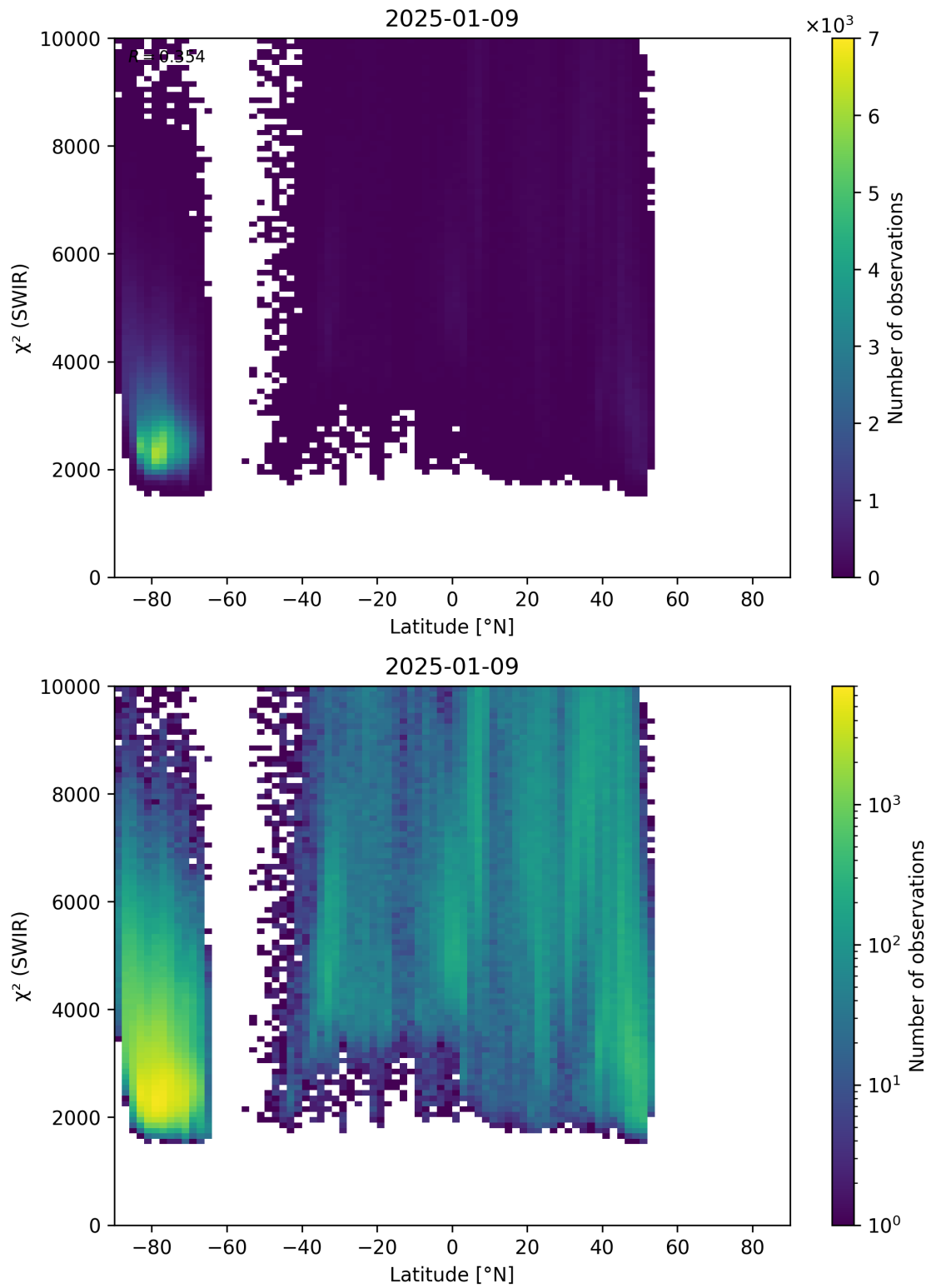
Figure 54: Scatter density plot of “Latitude” against “ \chi^2 (SWIR)” for 2025-01-08 to 2025-01-10.
