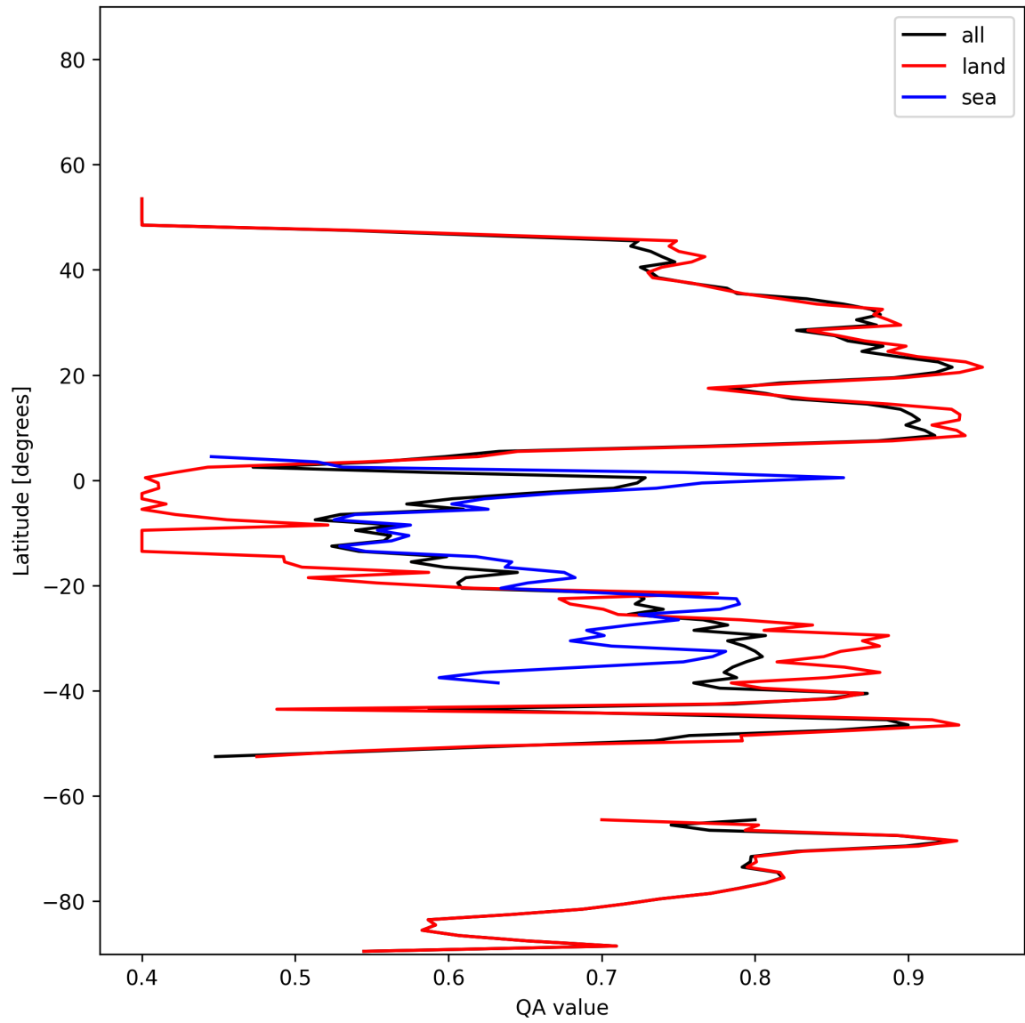
Figure 11: Zonal average of “QA value” for 2025-01-08 to 2025-01-10.
