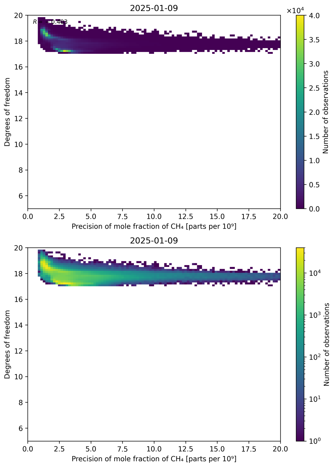
Figure 80: Scatter density plot of “Precision of mole fraction of CH 4 ” against “Degrees of freedom” for 2025-01-08 to 2025-01-10.
