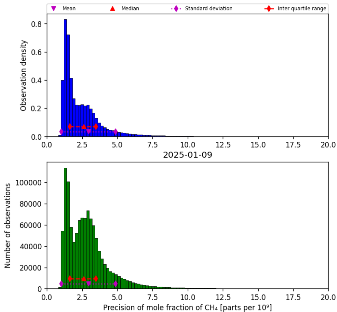
Figure 24: Histogram of “Precision of mole fraction of CH 4 ” for 2025-01-08 to 2025-01-10
