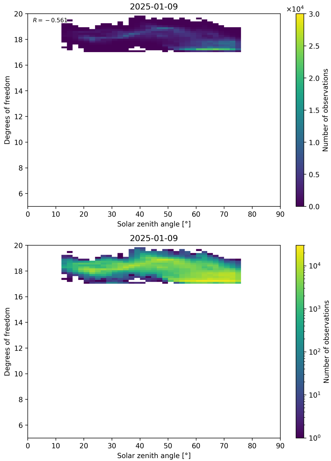
Figure 96: Scatter density plot of “Solar zenith angle” against “Degrees of freedom” for 2025-01-08 to 2025-01-10.
