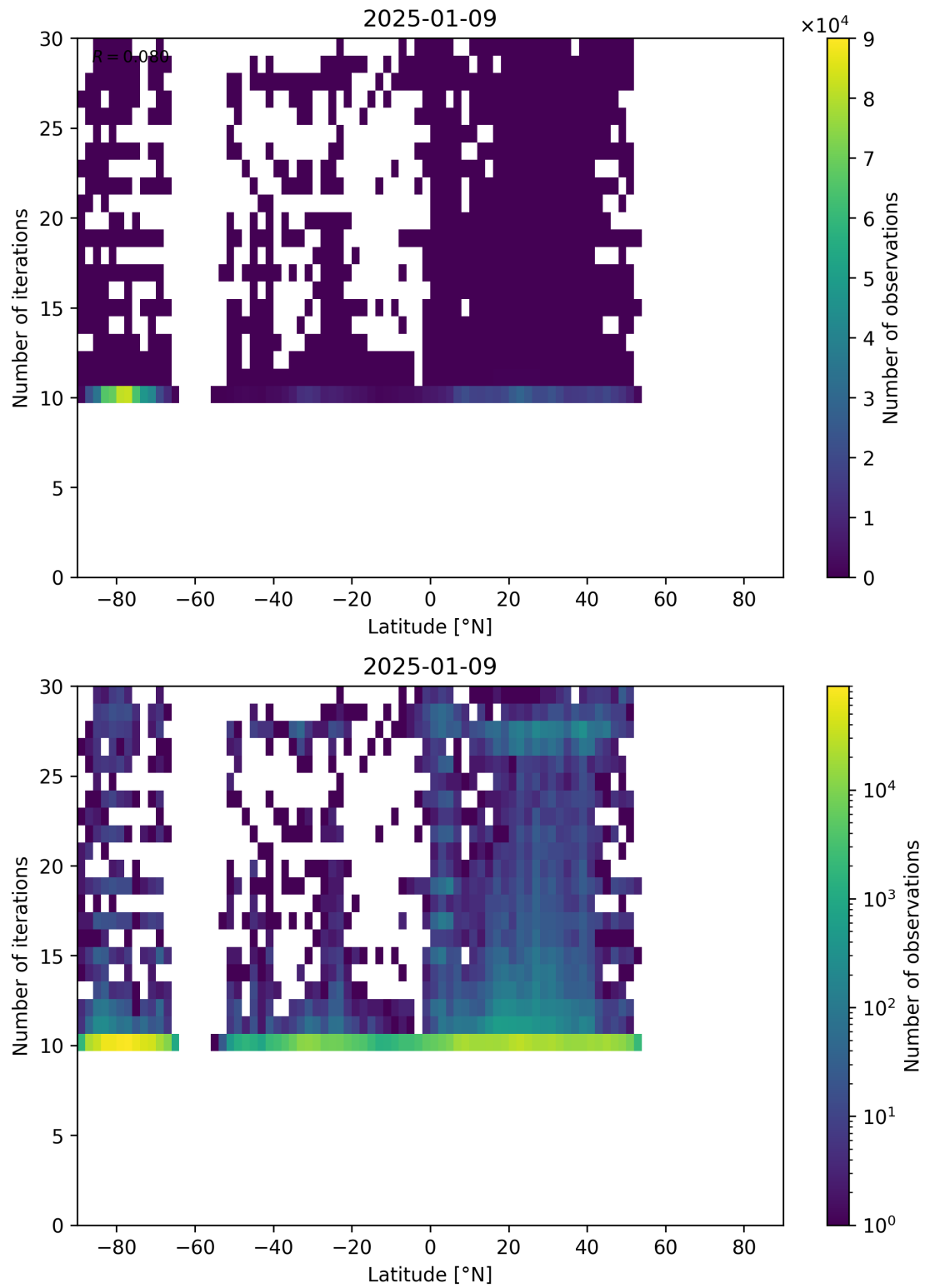
Figure 60: Scatter density plot of “Latitude” against “Number of iterations” for 2025-01-08 to 2025-01-10.
