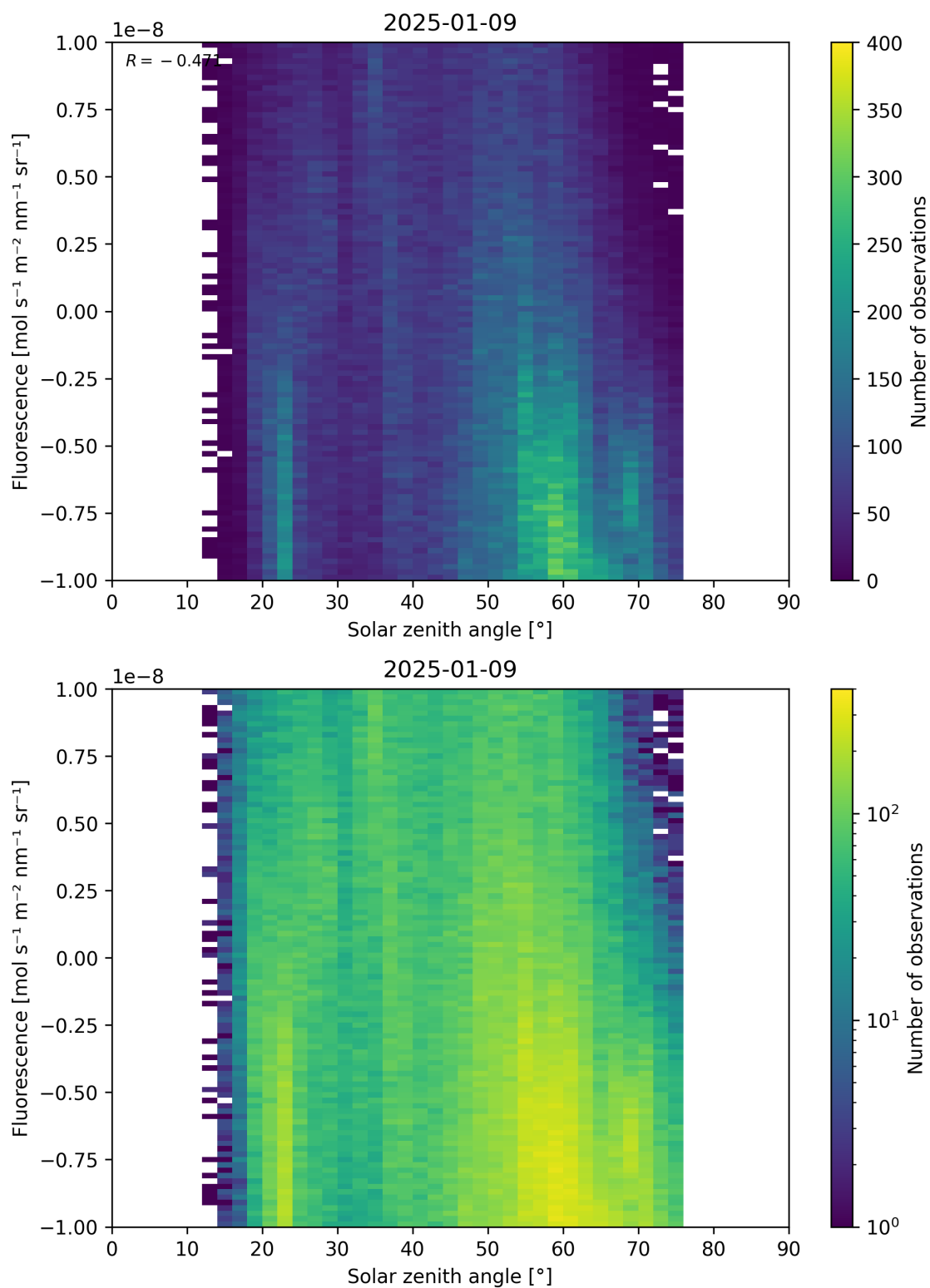
Figure 97: Scatter density plot of “Solar zenith angle” against “Fluorescence” for 2025-01-08 to 2025-01-10.
