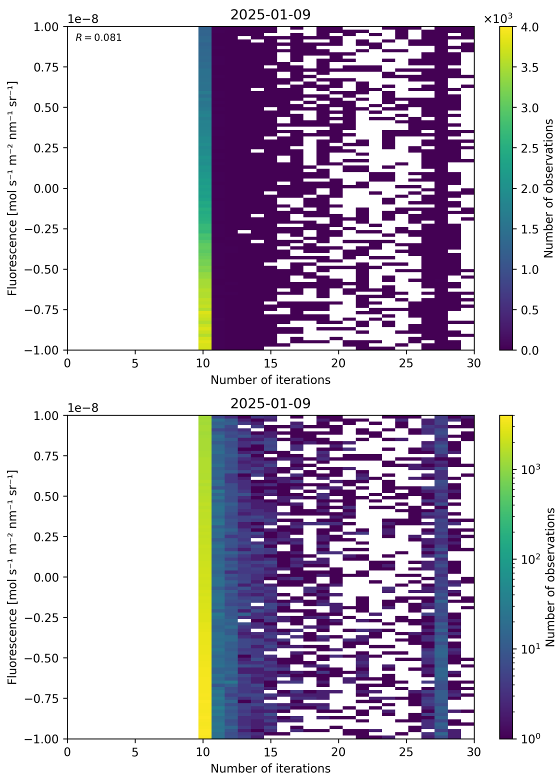
Figure 87: Scatter density plot of “Number of iterations” against “Fluorescence” for 2025-01-08 to 2025-01-10.
