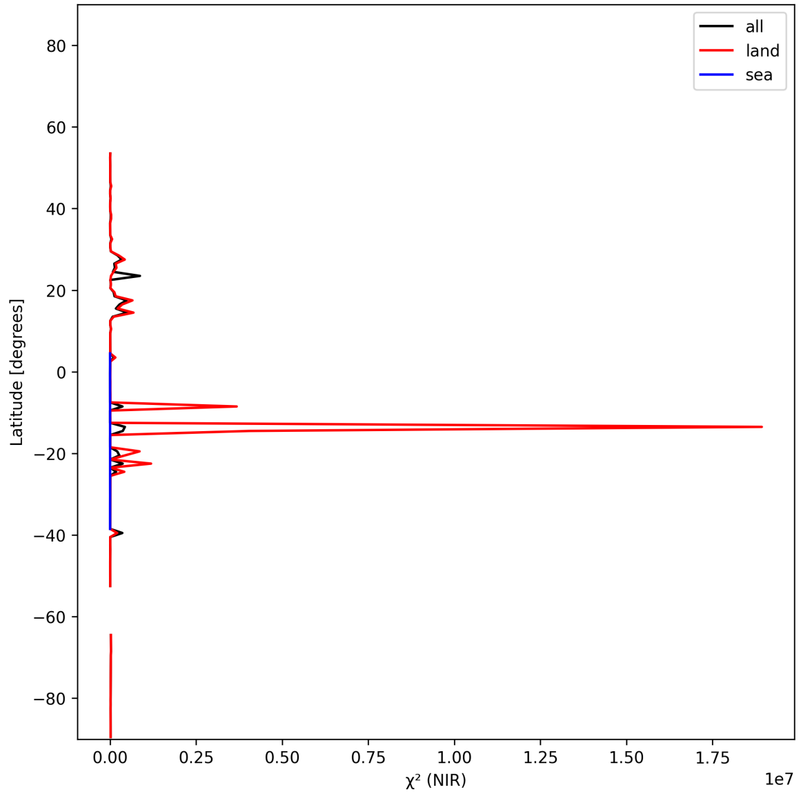
Figure 18: Zonal average of “ \chi^2 (NIR)” for 2025-01-08 to 2025-01-10.
