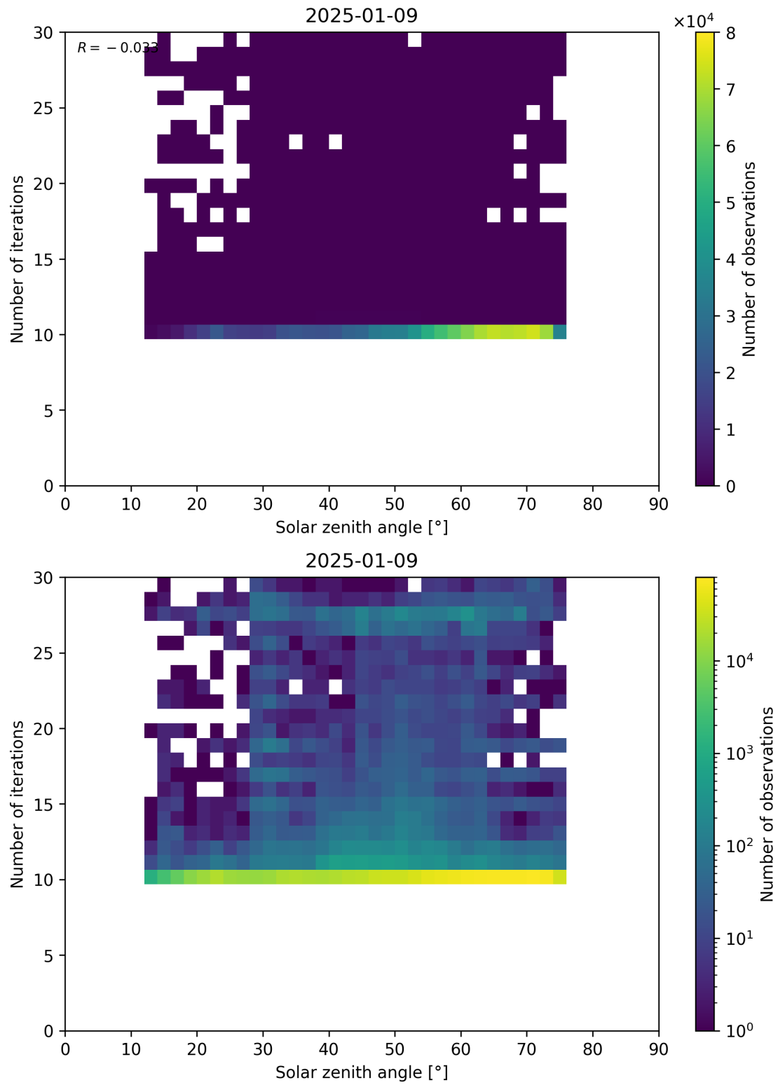
Figure 102: Scatter density plot of “Solar zenith angle” against “Number of iterations” for 2025-01-08 to 2025-01-10.
