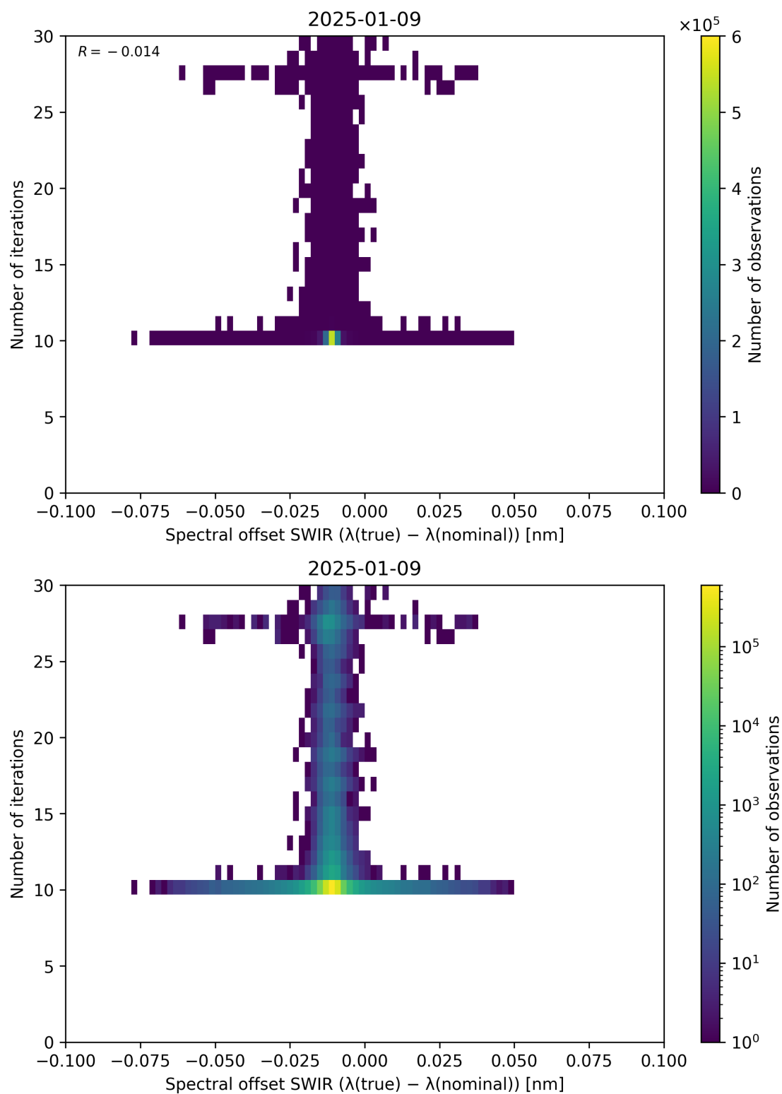
Figure 121: Scatter density plot of “Spectral offset SWIR ( \lambda_{\text{true}} - \lambda_{\text{nominal}} )” against “Number of iterations” for 2025-01-08 to 2025-01-10.
