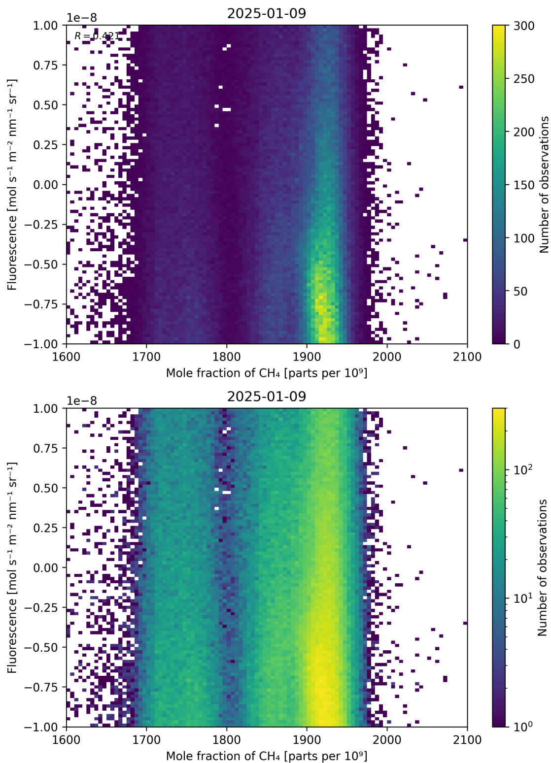
Figure 73: Scatter density plot of “Mole fraction of \text{CH}_4 ” against “Fluorescence” for 2025-01-08 to 2025-01-10.
