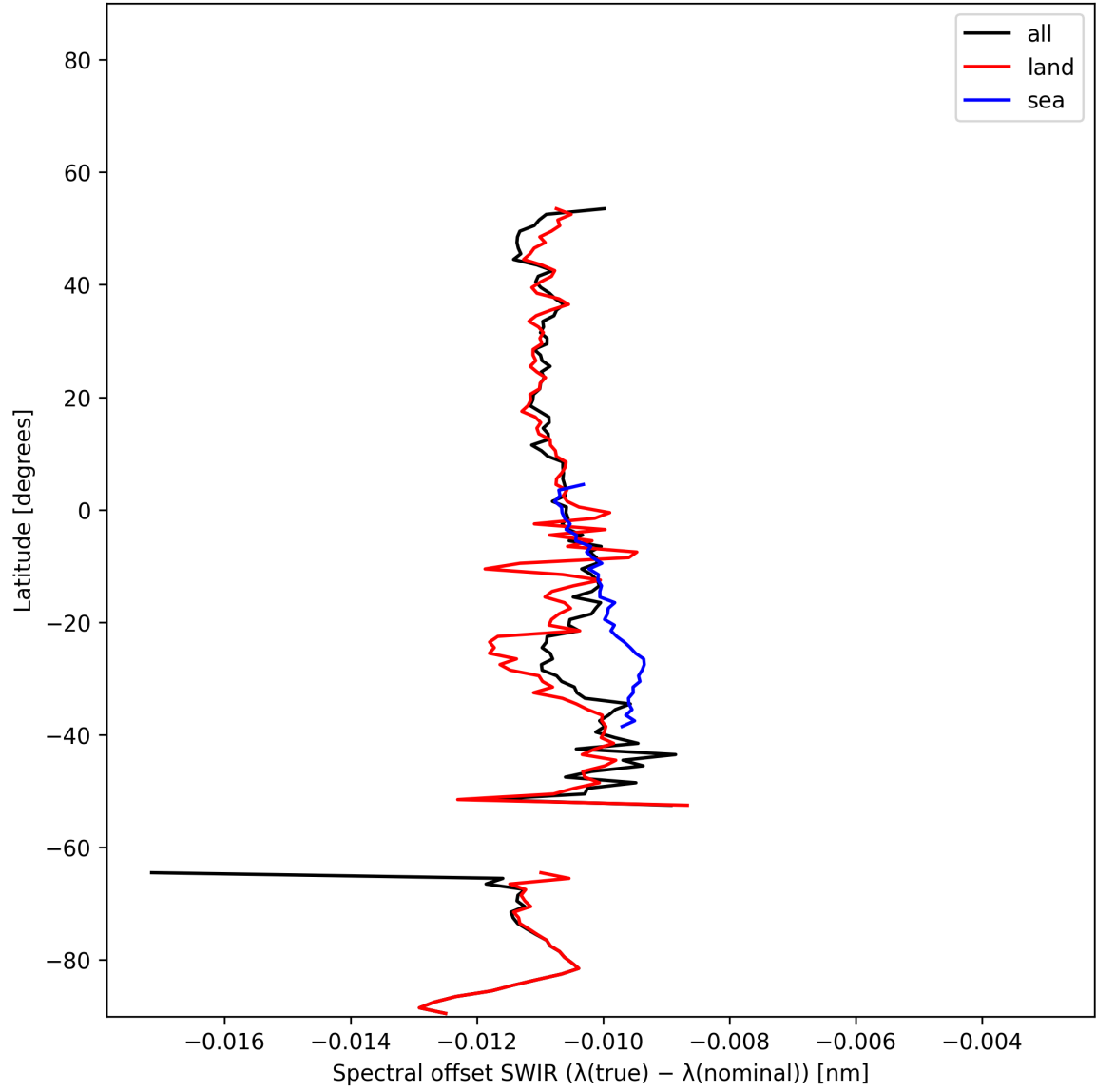
Figure 16: Zonal average of “Spectral offset SWIR ( \lambda_{\text{true}} - \lambda_{\text{nominal}} )” for 2025-01-08 to 2025-01-10.
