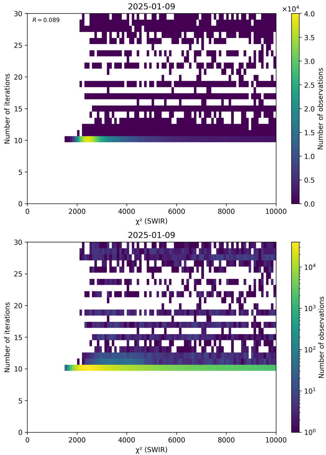
Figure 50: Scatter density plot of “ \chi^2 (SWIR)” against “Number of iterations” for 2025-01-08 to 2025-01-10.
