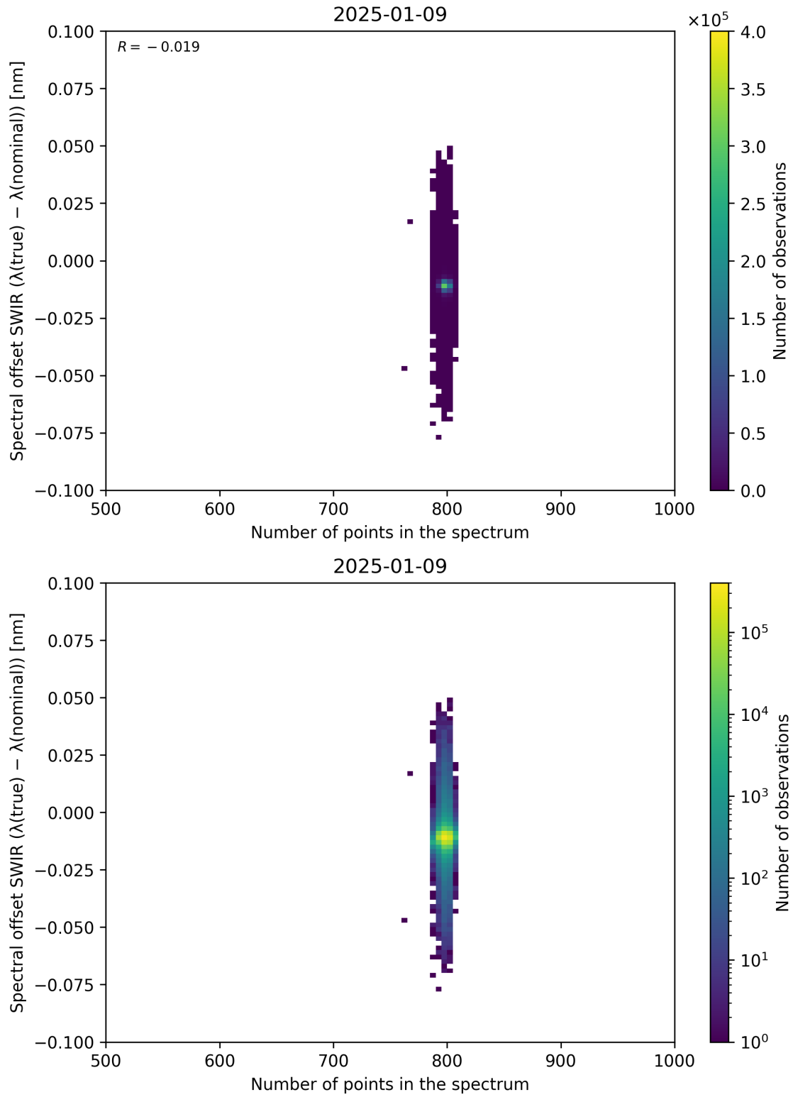
Figure 93: Scatter density plot of “Number of points in the spectrum” against “Spectral offset SWIR ( \lambda_{\text{true}} - \lambda_{\text{nominal}} )” for 2025-01-08 to 2025-01-10.
