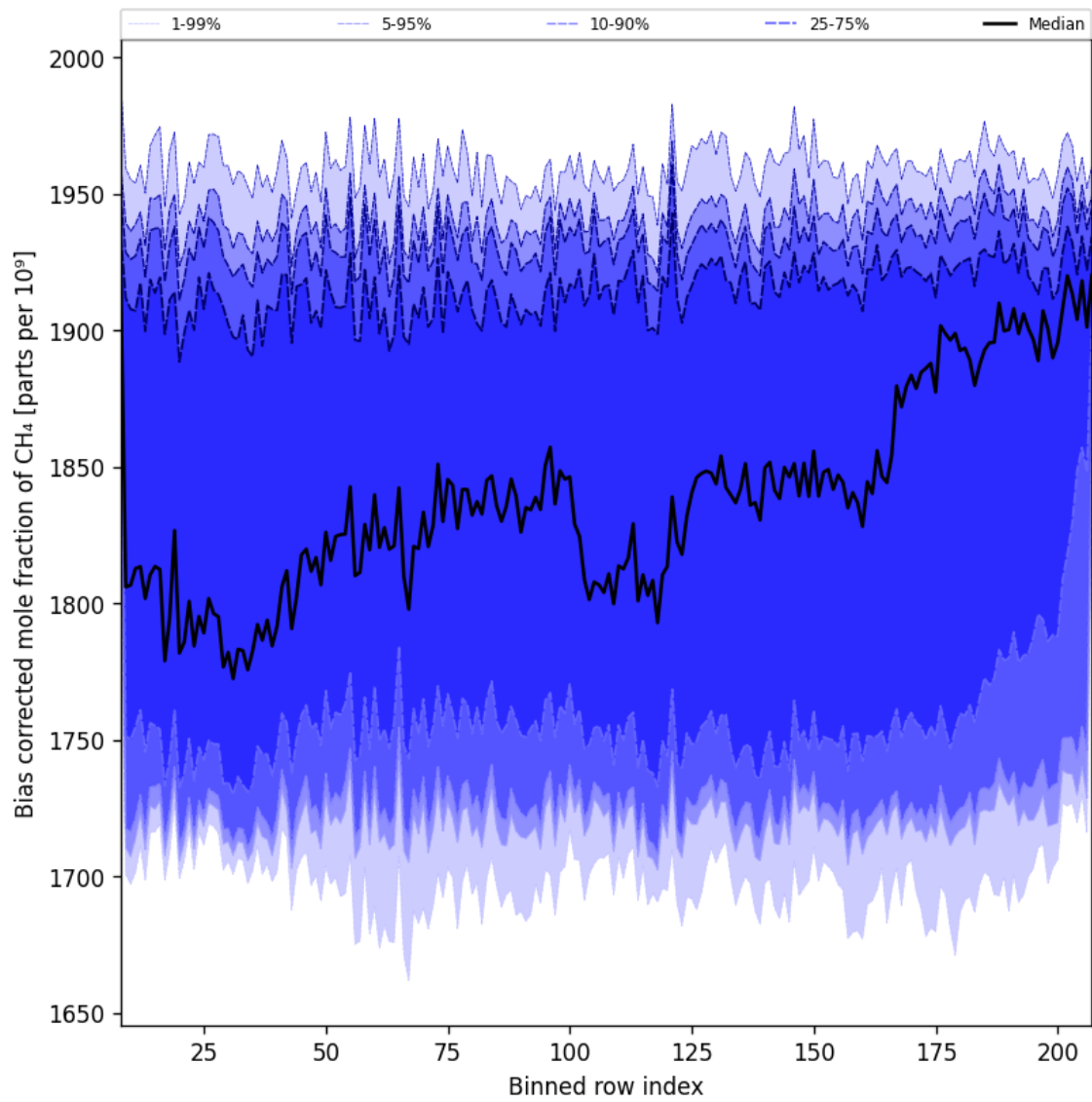
Figure 36: Along track statistics of “Bias corrected mole fraction of CH 4 ” for 2025-01-08 to 2025-01-10
