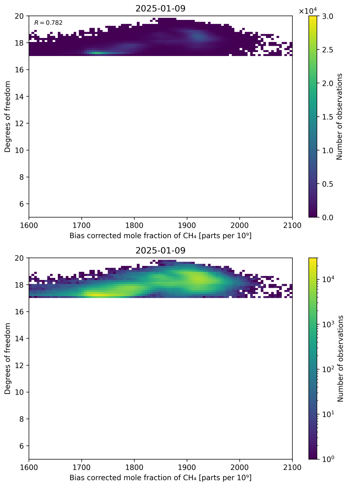
Figure 65: Scatter density plot of “Bias corrected mole fraction of CH 4 ” against “Degrees of freedom” for 2025-01-08 to 2025-01-10.
