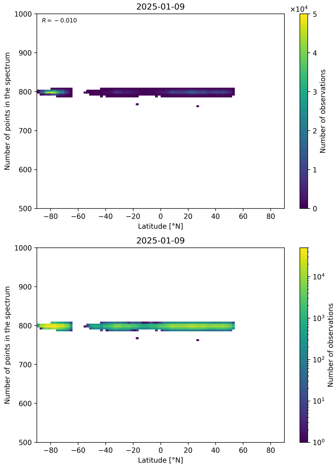
Figure 61: Scatter density plot of “Latitude” against “Number of points in the spectrum” for 2025-01-08 to 2025-01-10.
