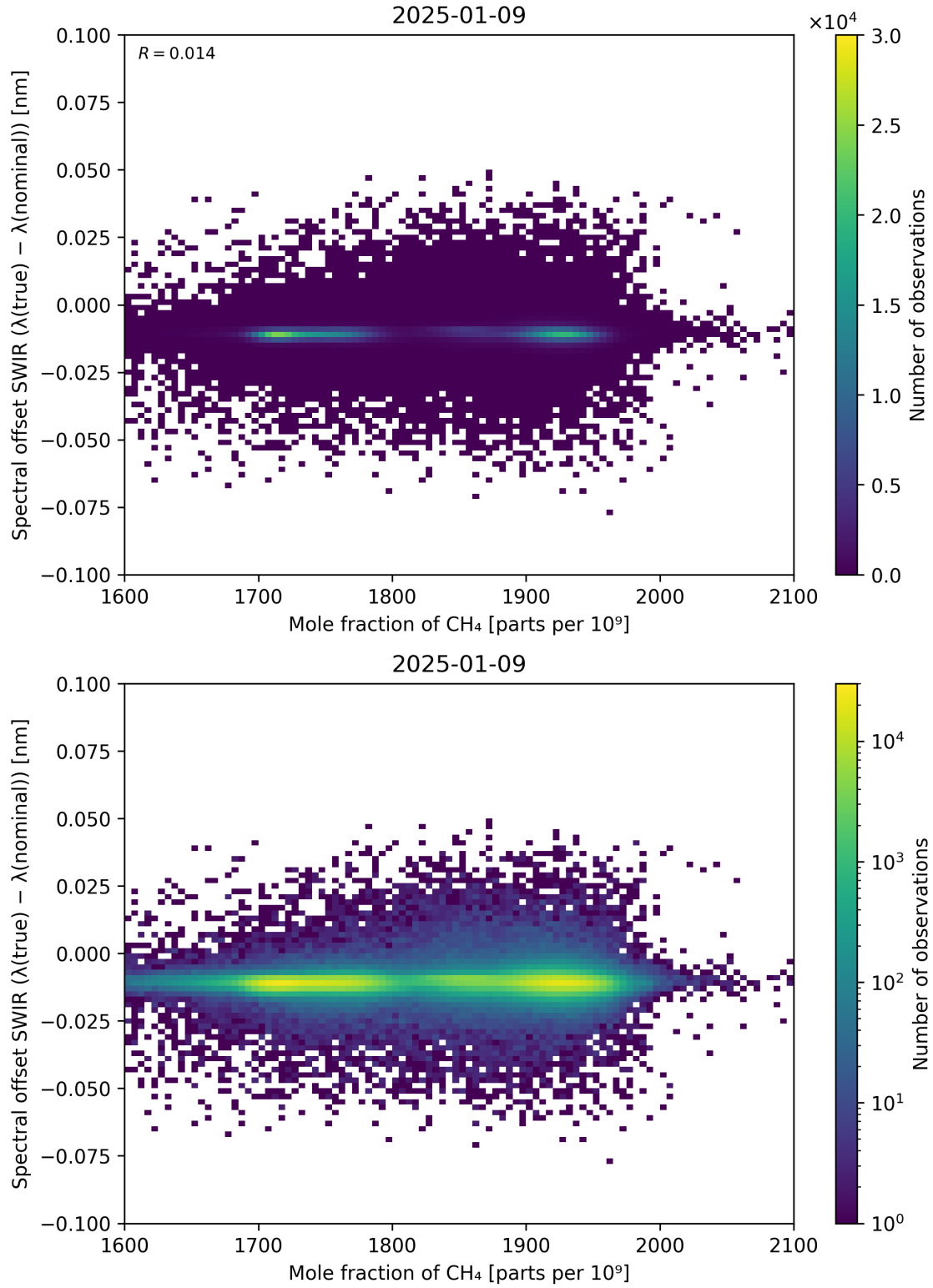
Figure 86: Scatter density plot of “Mole fraction of CH 4 ” against “Spectral offset SWIR ( \lambda_{\text{true}} - \lambda_{\text{nominal}} )” for 2025-01-08 to 2025-01-10.
