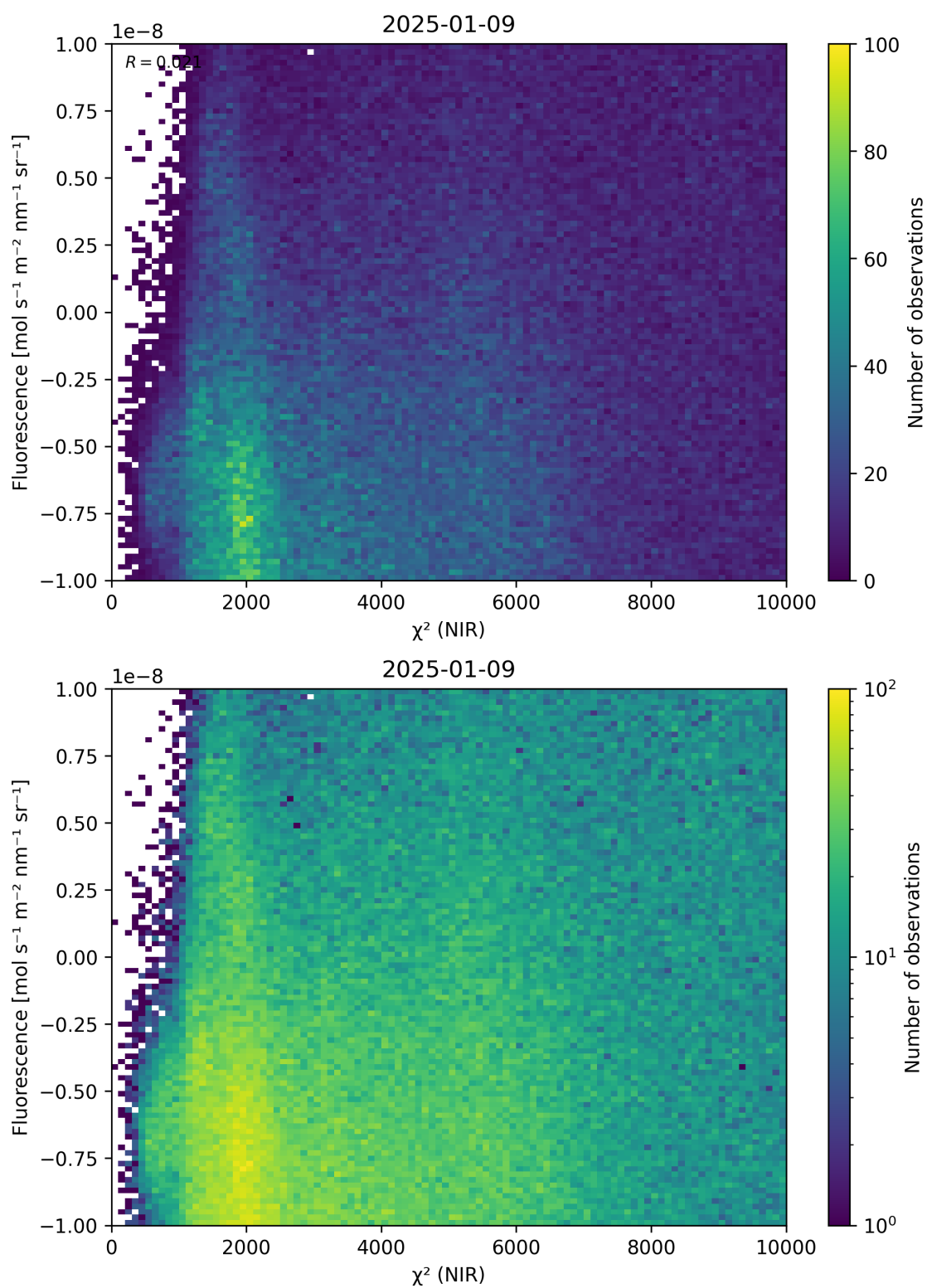
Figure 45: Scatter density plot of “ \chi^2 (NIR)” against “Fluorescence” for 2025-01-08 to 2025-01-10.
