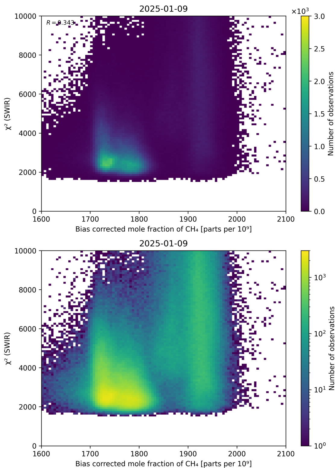
Figure 64: Scatter density plot of “Bias corrected mole fraction of \text{CH}_4 ” against “ \chi^2 (SWIR)” for 2025-01-08 to 2025-01-10.
