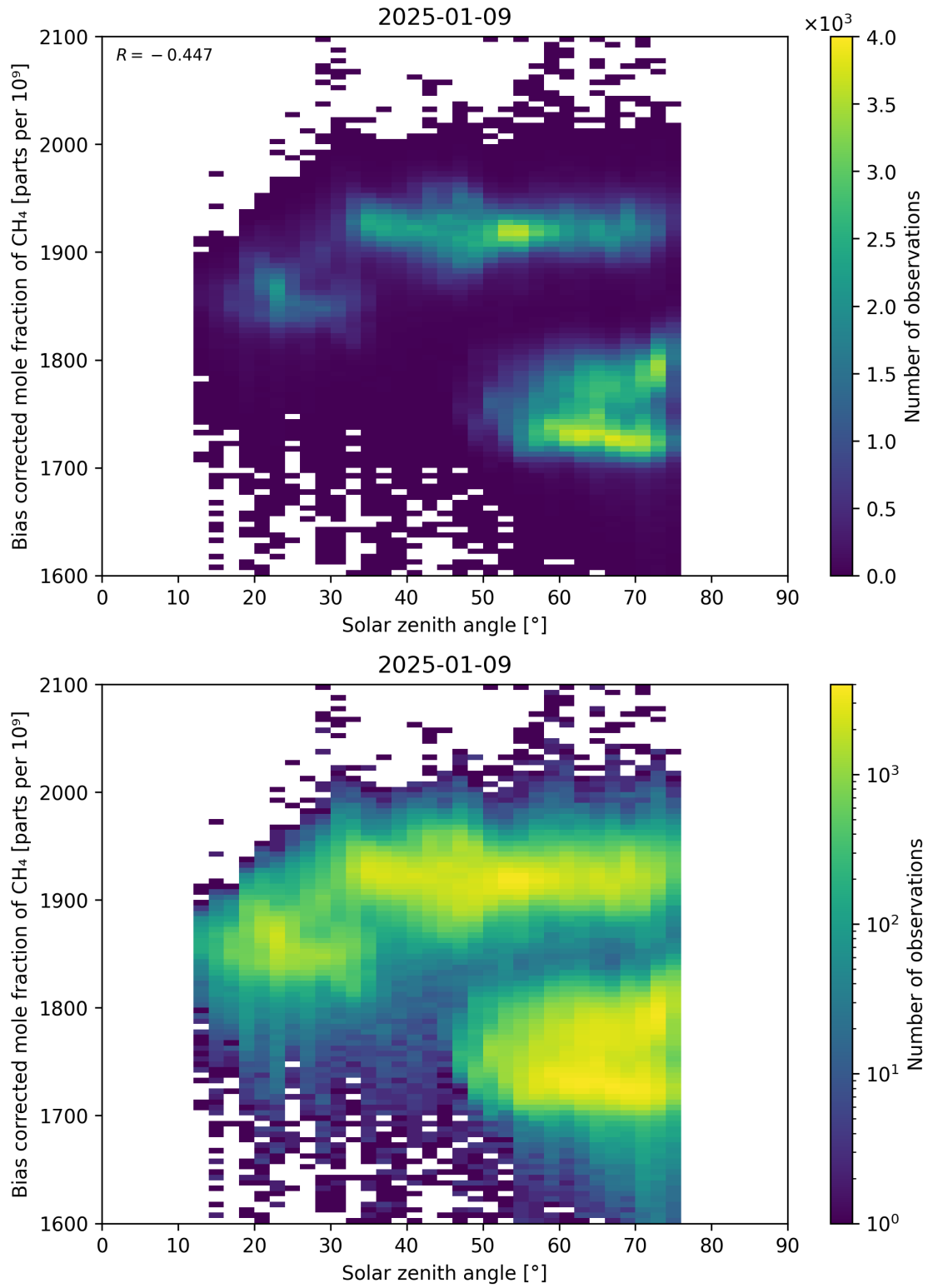
Figure 100: Scatter density plot of “Solar zenith angle” against “Bias corrected mole fraction of \text{CH}_4 ” for 2025-01-08 to 2025-01-10.
