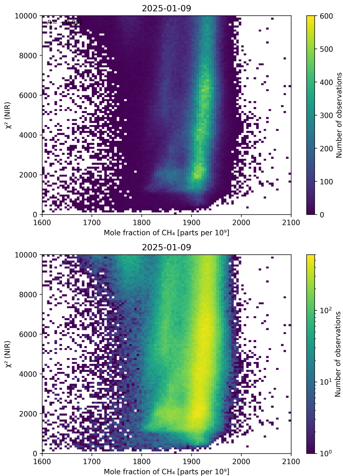
Figure 70: Scatter density plot of “Mole fraction of \text{CH}_4 ” against “ \chi^2 (NIR)” for 2025-01-08 to 2025-01-10.
