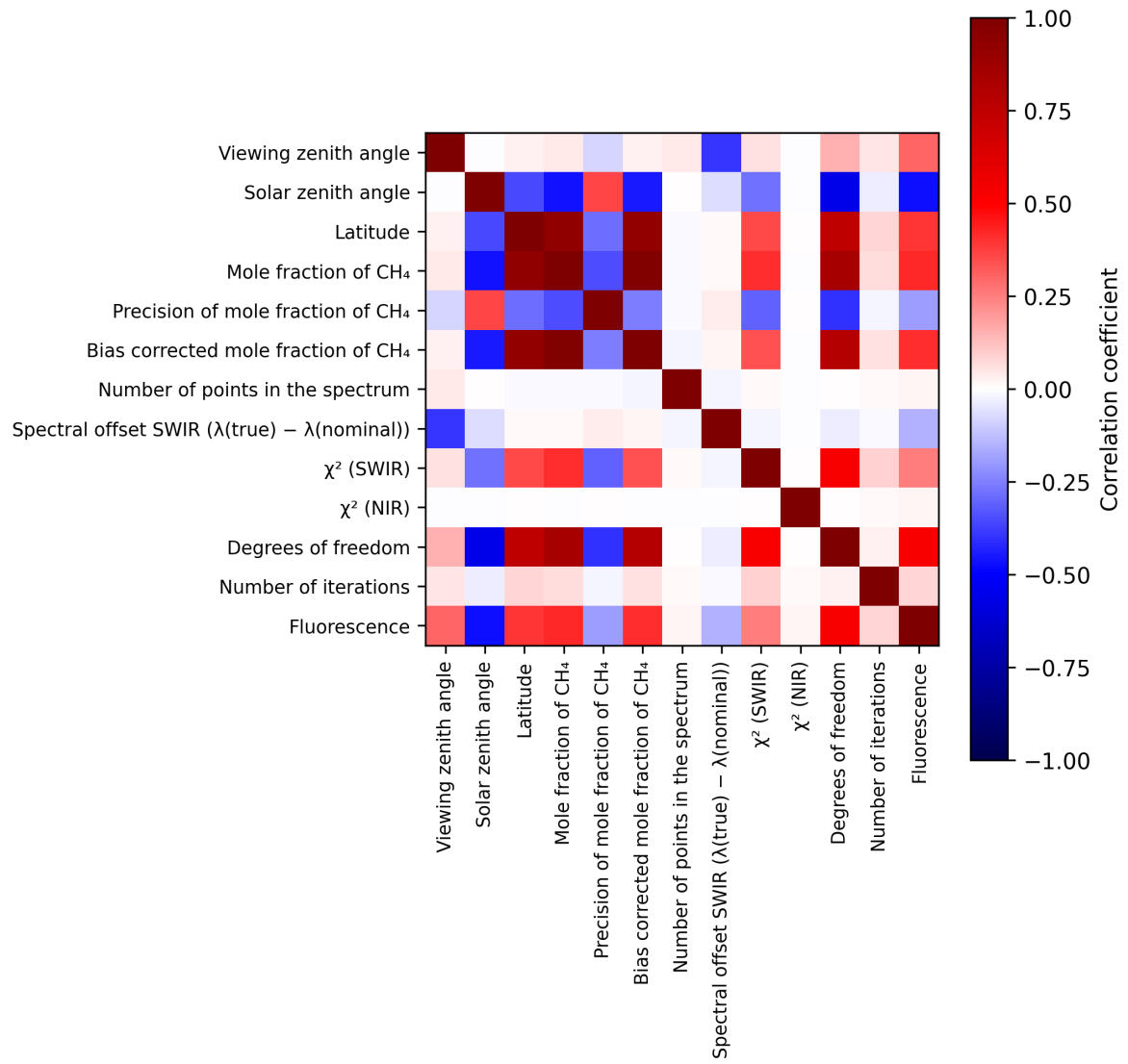
Figure 2: Map of correlation matrix for 2025-01-08 to 2025-01-10.
