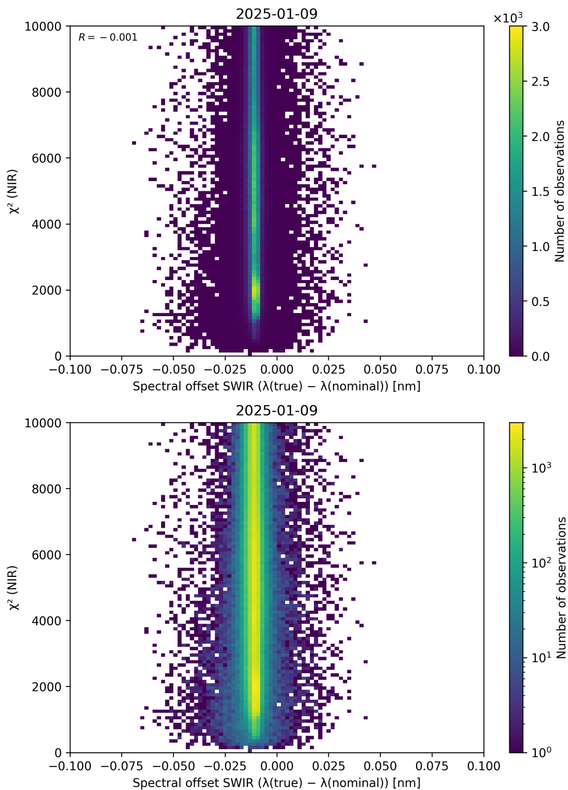
Figure 117: Scatter density plot of “Spectral offset SWIR ( \lambda_{\text{true}} - \lambda_{\text{nominal}} )” against “ \chi^2 (NIR)” for 2025-01-08 to 2025-01-10.
