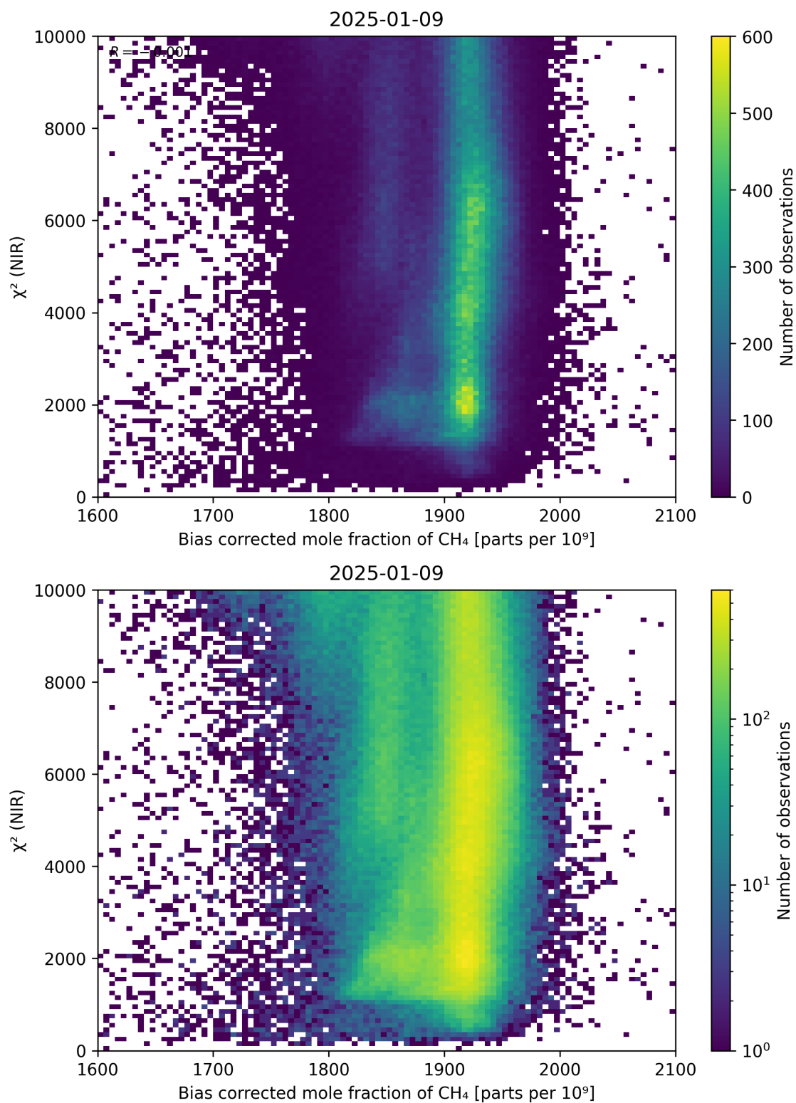
Figure 63: Scatter density plot of “Bias corrected mole fraction of \text{CH}_4 ” against “ \chi^2 (NIR)” for 2025-01-08 to 2025-01-10.
