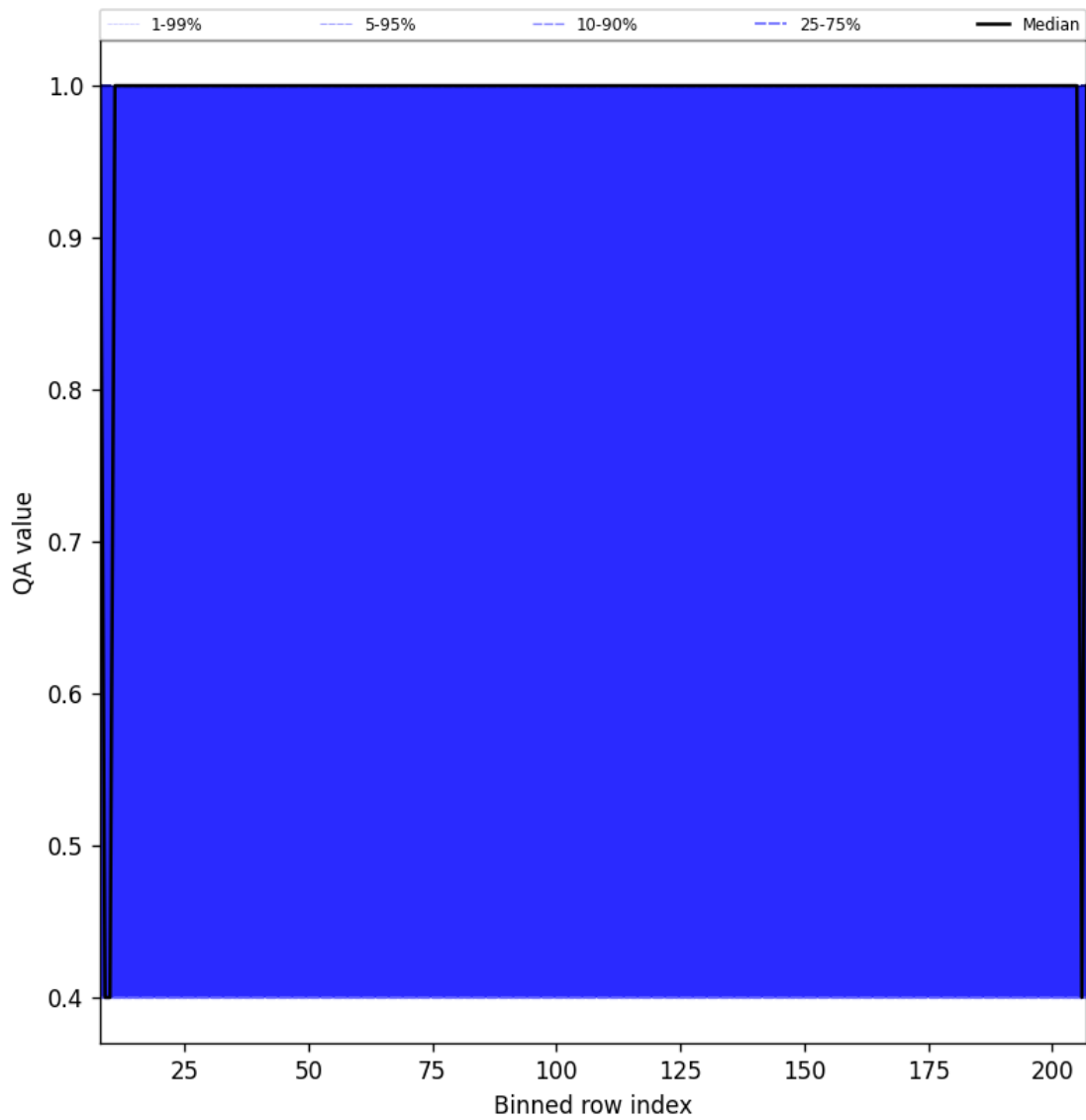
Figure 33: Along track statistics of “QA value” for 2025-01-08 to 2025-01-10
