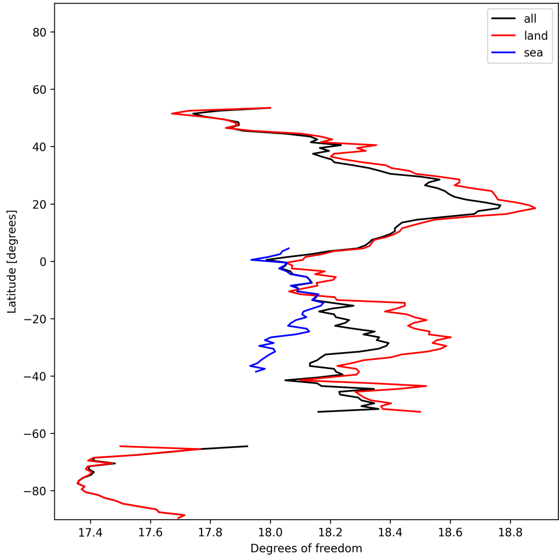
Figure 19: Zonal average of “Degrees of freedom” for 2025-01-08 to 2025-01-10.
