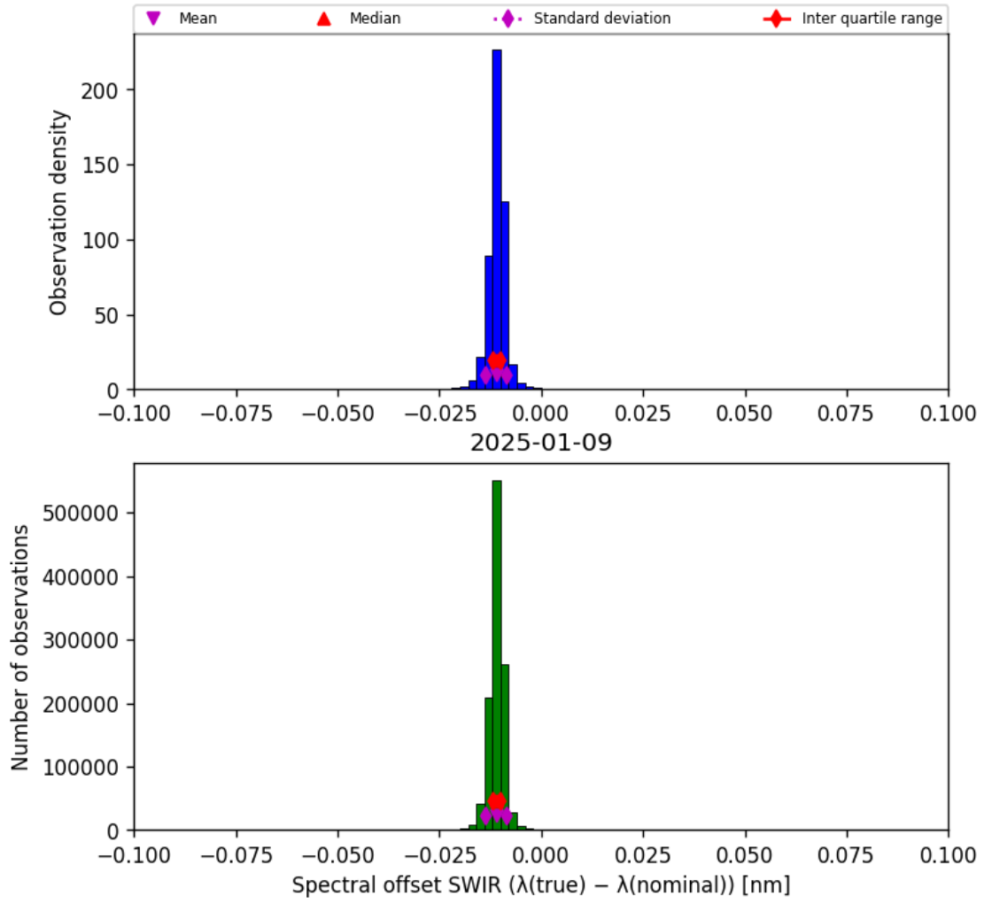
Figure 27: Histogram of “Spectral offset SWIR ( \lambda_{\text{true}} - \lambda_{\text{nominal}} )” for 2025-01-08 to 2025-01-10
