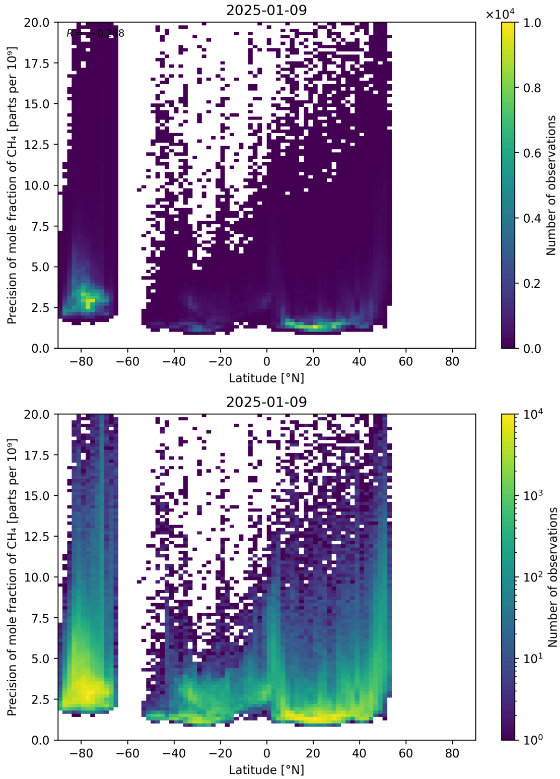
Figure 59: Scatter density plot of “Latitude” against “Precision of mole fraction of CH 4 ” for 2025-01-08 to 2025-01-10.
