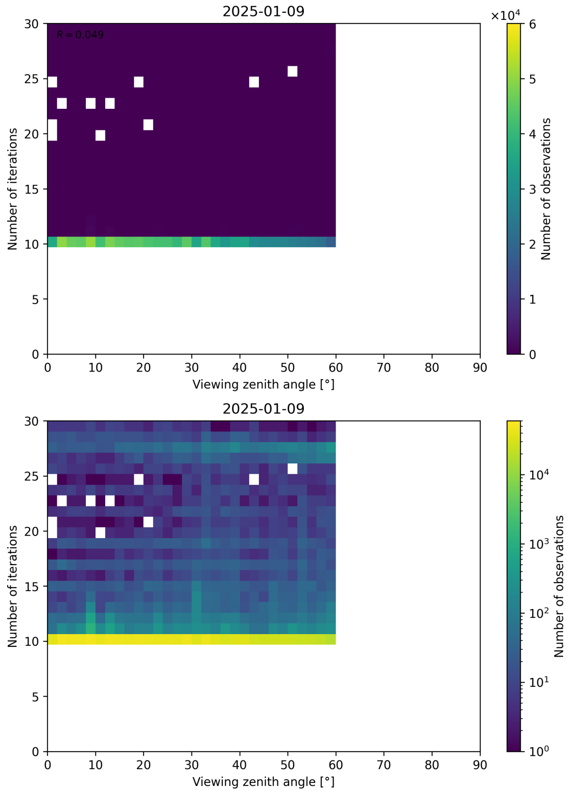
Figure 113: Scatter density plot of “Viewing zenith angle” against “Number of iterations” for 2025-01-08 to 2025-01-10.
