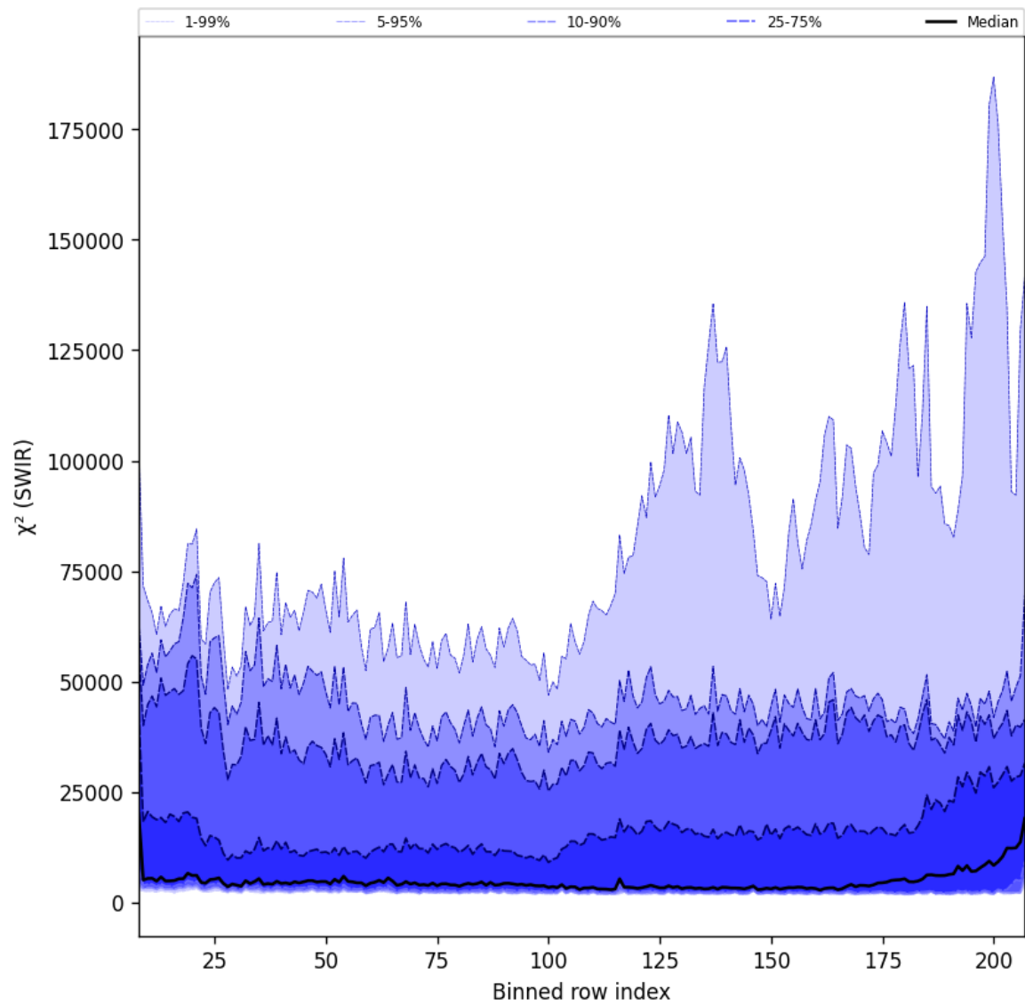
Figure 39: Along track statistics of “ \chi^2 (SWIR)” for 2025-01-08 to 2025-01-10
