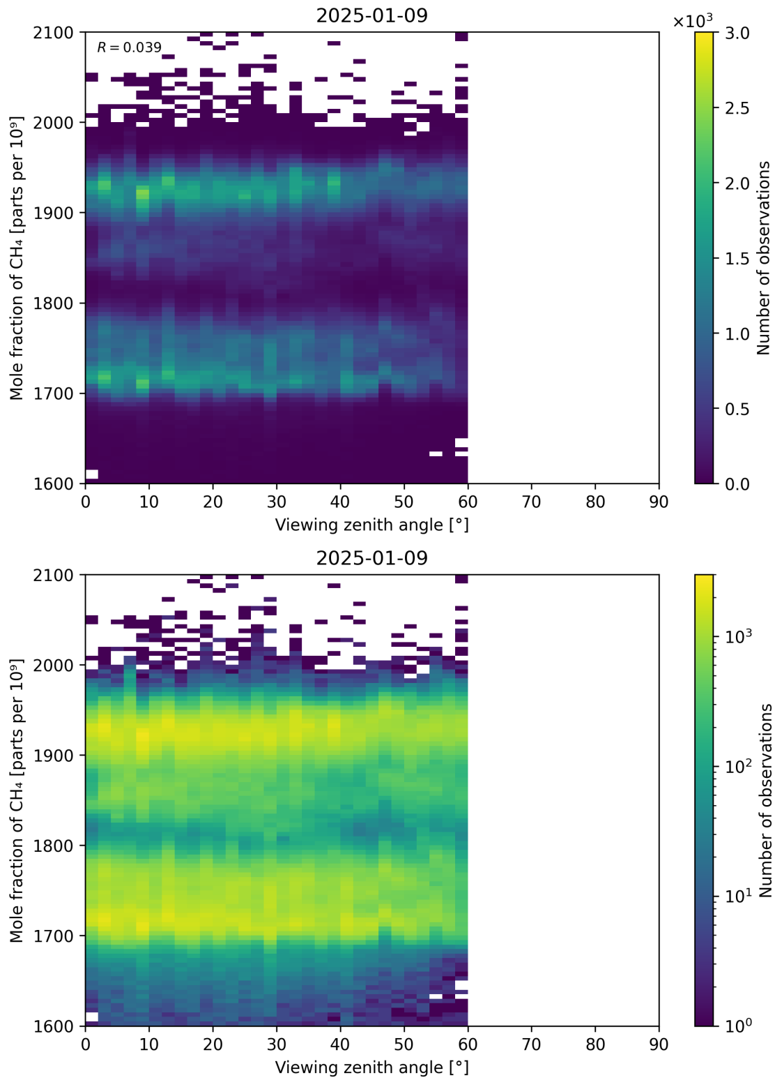
Figure 110: Scatter density plot of “Viewing zenith angle” against “Mole fraction of CH 4 ” for 2025-01-08 to 2025-01-10.
