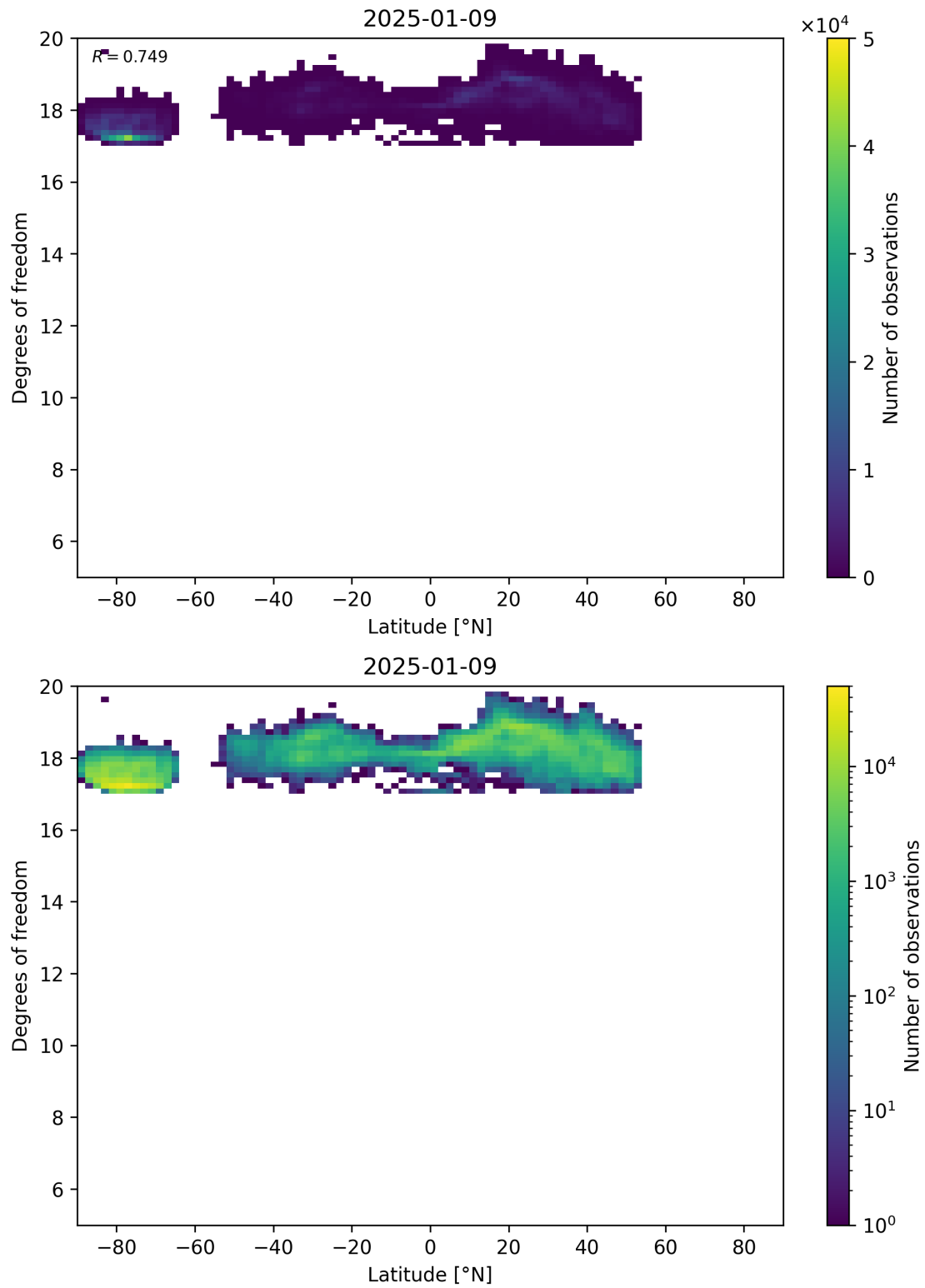
Figure 55: Scatter density plot of “Latitude” against “Degrees of freedom” for 2025-01-08 to 2025-01-10.
