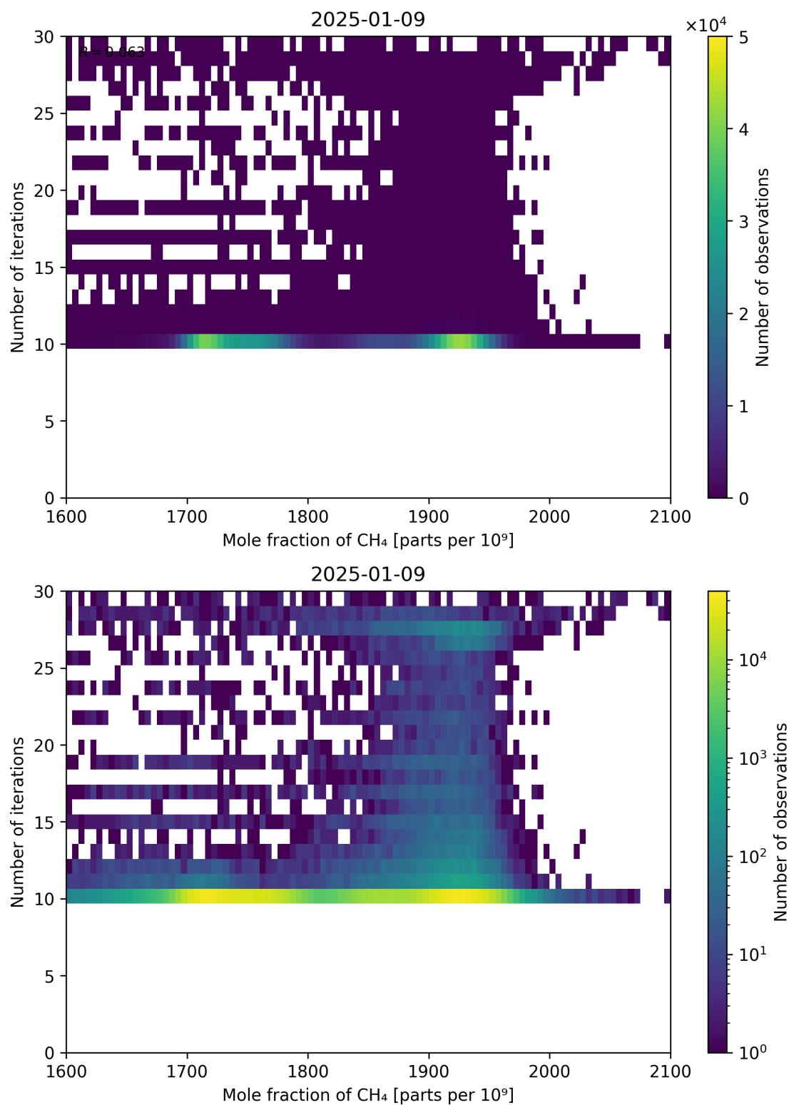
Figure 76: Scatter density plot of “Mole fraction of CH 4 ” against “Number of iterations” for 2025-01-08 to 2025-01-10.
