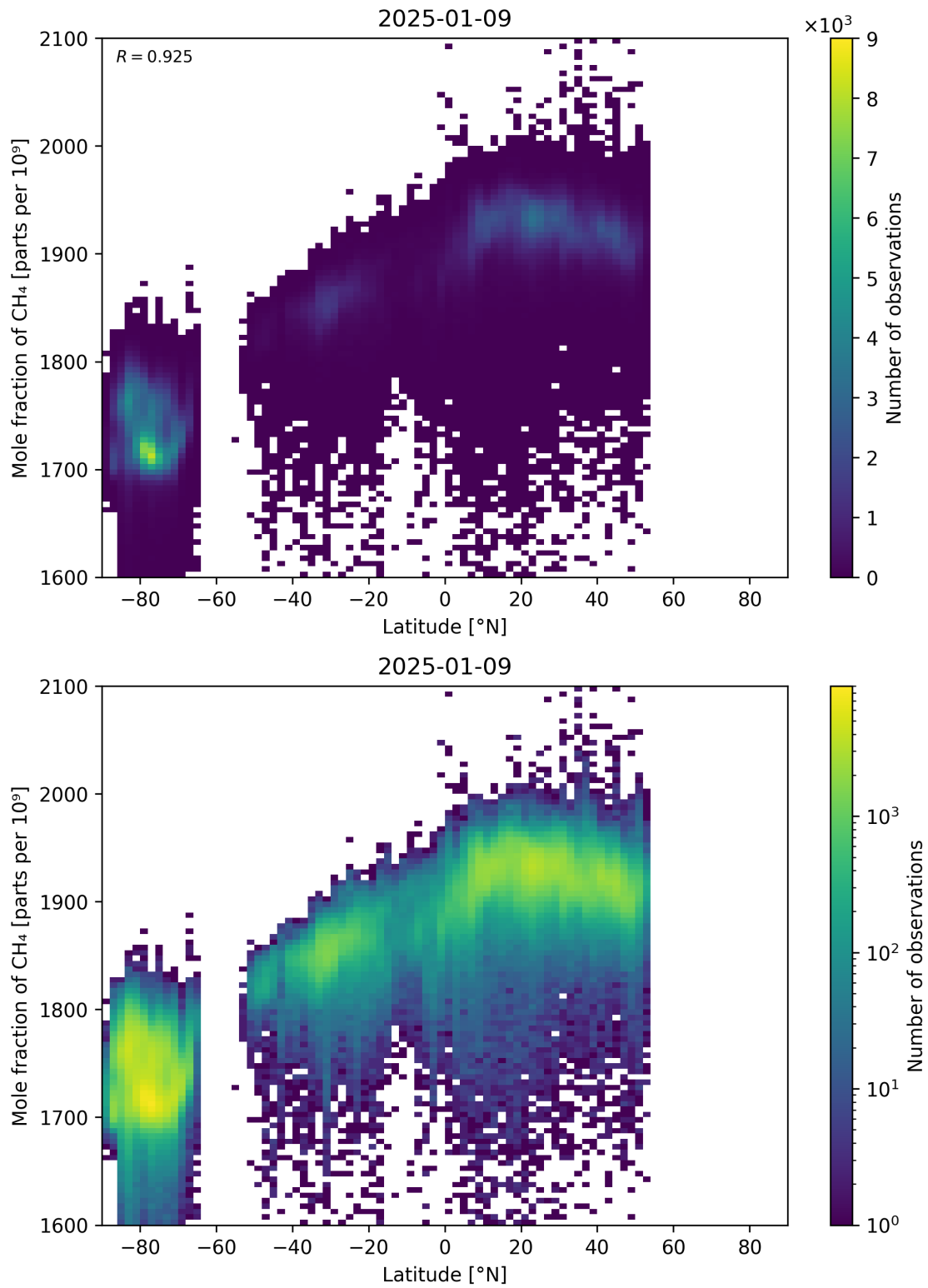
Figure 57: Scatter density plot of “Latitude” against “Mole fraction of \text{CH}_4 ” for 2025-01-08 to 2025-01-10.
