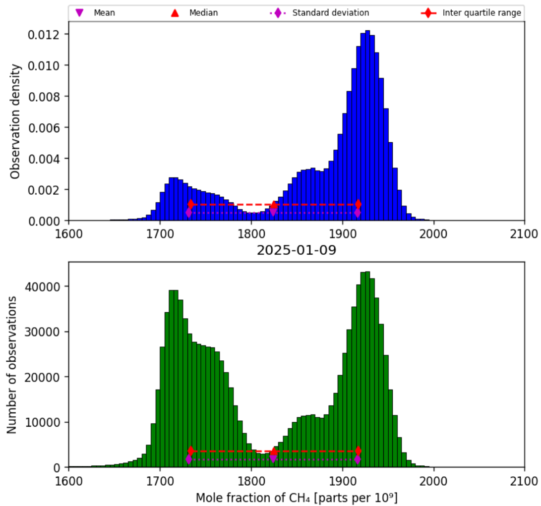
Figure 23: Histogram of “Mole fraction of CH 4 ” for 2025-01-08 to 2025-01-10
