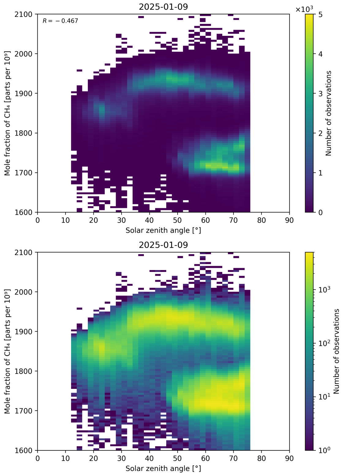
Figure 99: Scatter density plot of “Solar zenith angle” against “Mole fraction of CH 4 ” for 2025-01-08 to 2025-01-10.
