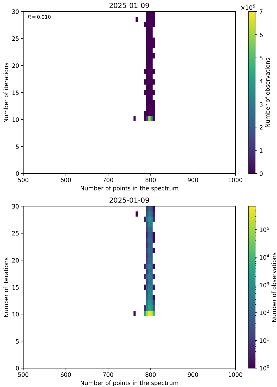
Figure 92: Scatter density plot of “Number of points in the spectrum” against “Number of iterations” for 2025-01-08 to 2025-01-10.
