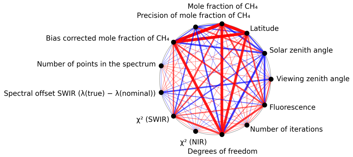
Figure 1: Map of correlation graph for 2025-01-08 to 2025-01-10.
