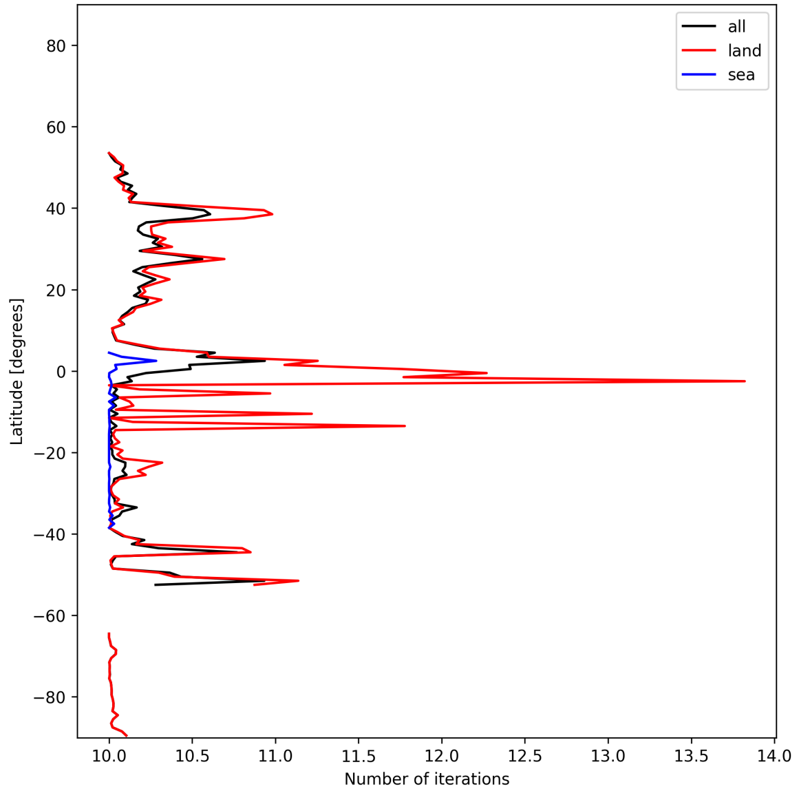
Figure 20: Zonal average of “Number of iterations” for 2025-01-08 to 2025-01-10.
