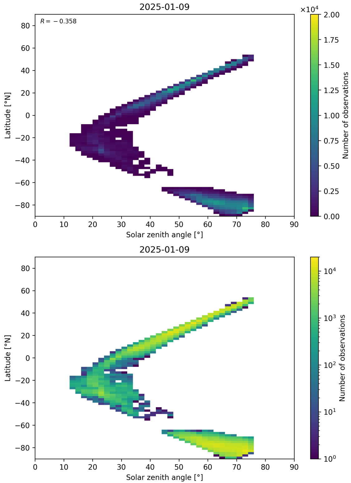
Figure 98: Scatter density plot of “Solar zenith angle” against “Latitude” for 2025-01-08 to 2025-01-10.
