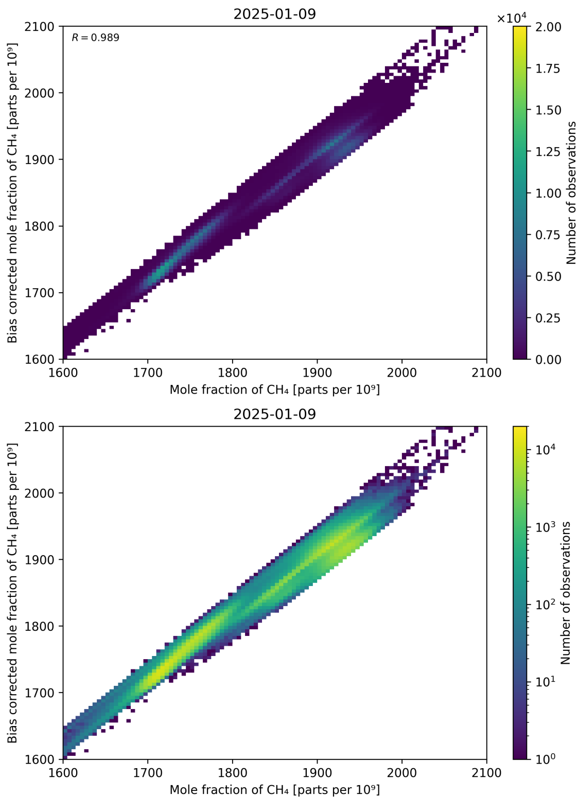
Figure 74: Scatter density plot of “Mole fraction of CH 4 ” against “Bias corrected mole fraction of CH 4 ” for 2025-01-08 to 2025-01-10.
