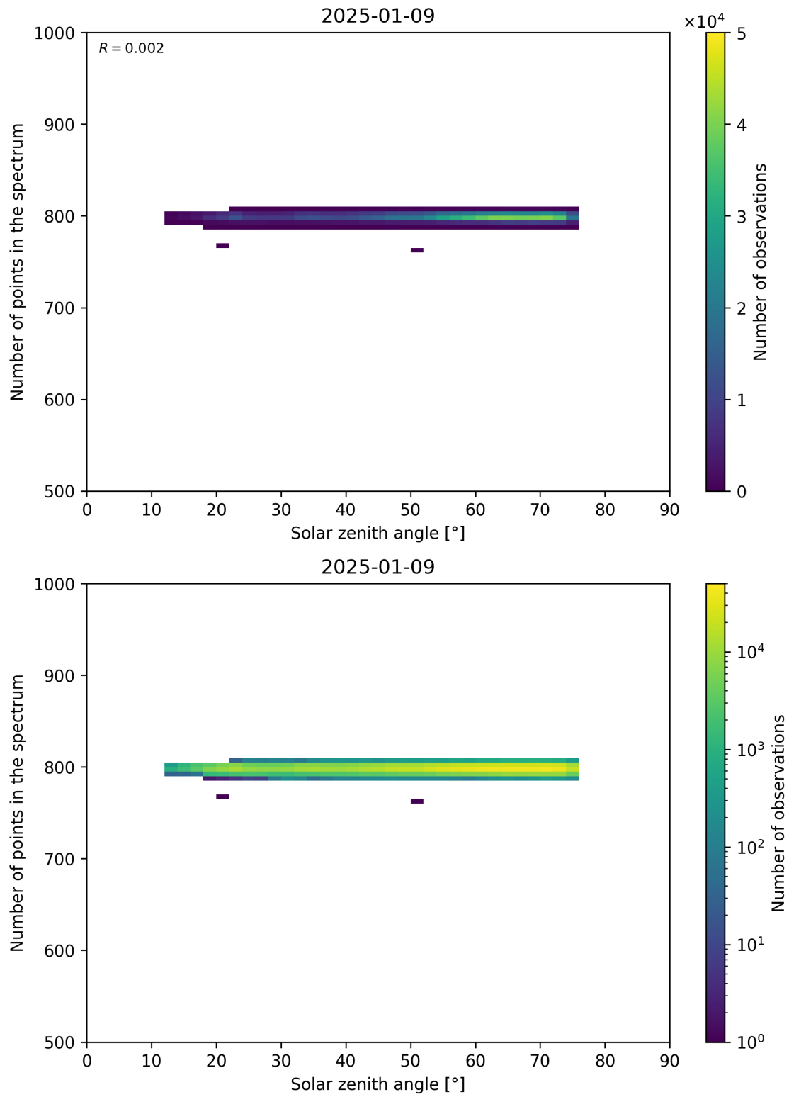
Figure 103: Scatter density plot of “Solar zenith angle” against “Number of points in the spectrum” for 2025-01-08 to 2025-01-10.
