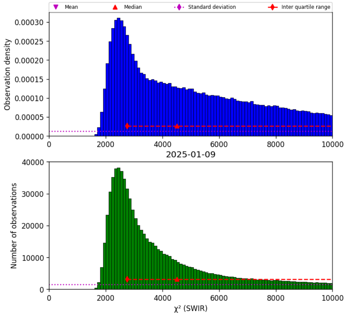
Figure 28: Histogram of “ \chi^2 (SWIR)” for 2025-01-08 to 2025-01-10
