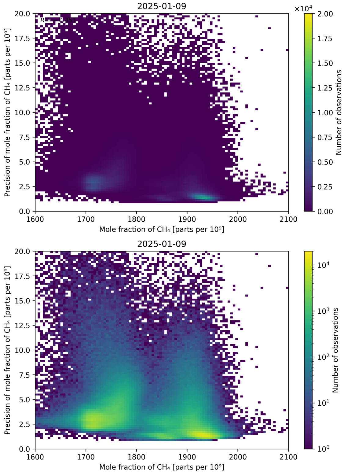
Figure 75: Scatter density plot of “Mole fraction of CH 4 ” against “Precision of mole fraction of CH 4 ” for 2025-01-08 to 2025-01-10.
