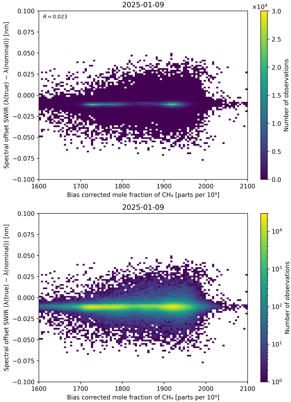
Figure 69: Scatter density plot of “Bias corrected mole fraction of \text{CH}_4 ” against “Spectral offset SWIR ( \lambda_{\text{true}} - \lambda_{\text{nominal}} )” for 2025-01-08 to 2025-01-10.
