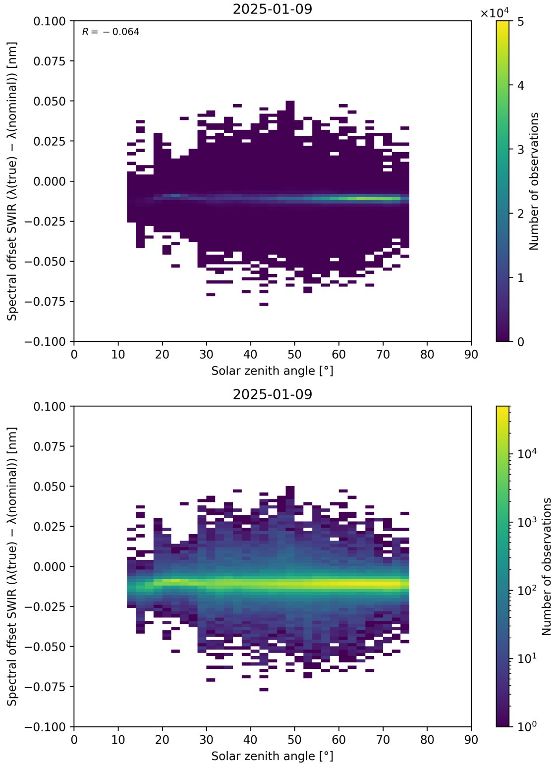
Figure 104: Scatter density plot of “Solar zenith angle” against “Spectral offset SWIR ( \lambda_{\text{true}} - \lambda_{\text{nominal}} )” for 2025-01-08 to 2025-01-10.
