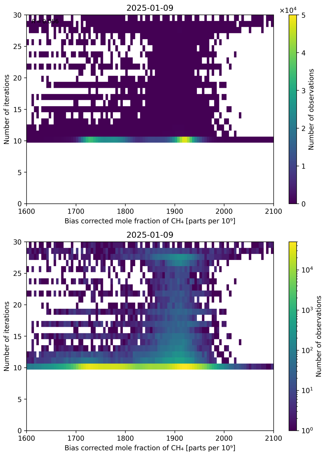
Figure 67: Scatter density plot of “Bias corrected mole fraction of \text{CH}_4 ” against “Number of iterations” for 2025-01-08 to 2025-01-10.
