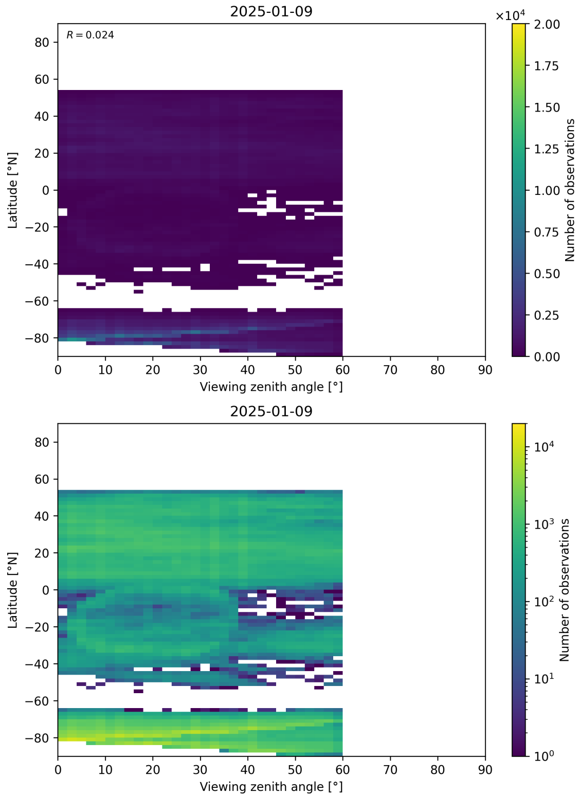
Figure 109: Scatter density plot of “Viewing zenith angle” against “Latitude” for 2025-01-08 to 2025-01-10.
