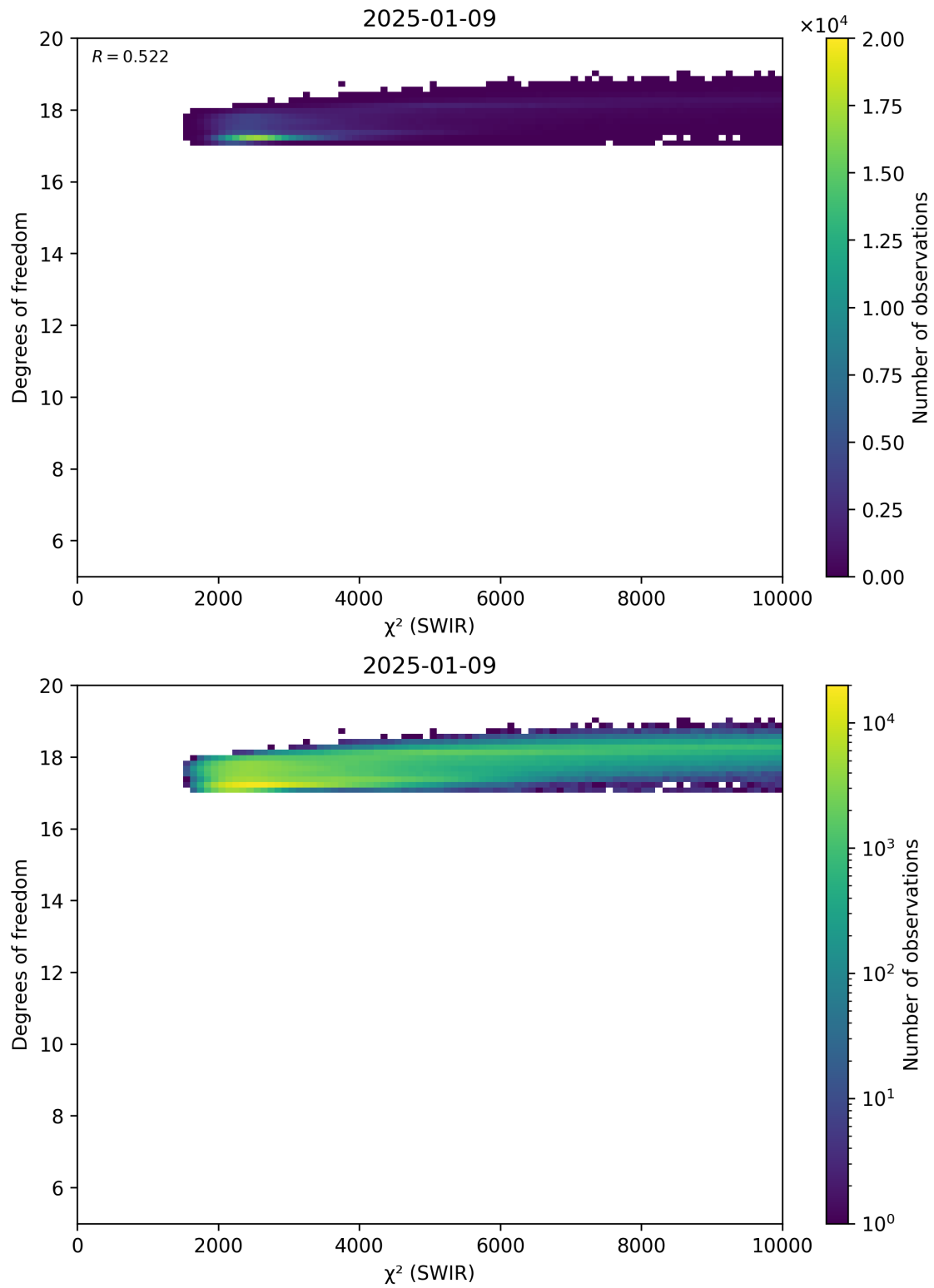
Figure 48: Scatter density plot of “ \chi^2 (SWIR)” against “Degrees of freedom” for 2025-01-08 to 2025-01-10.
