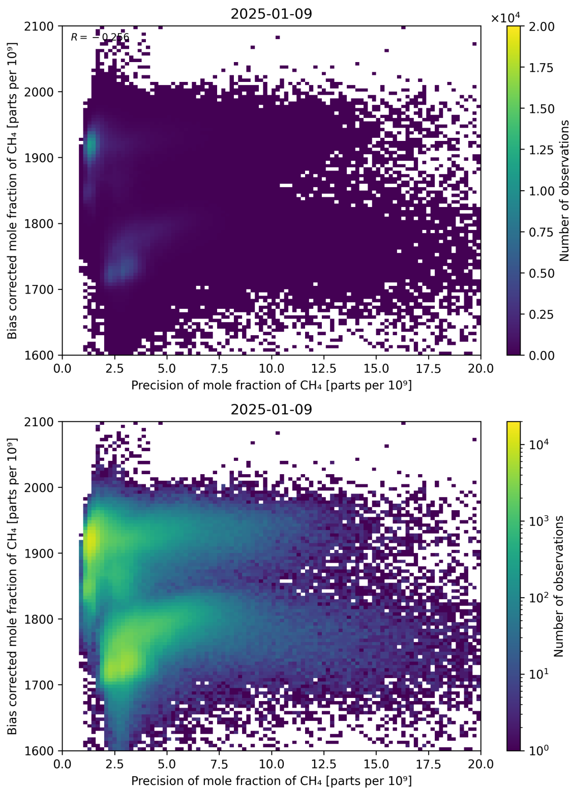
Figure 82: Scatter density plot of “Precision of mole fraction of CH 4 ” against “Bias corrected mole fraction of CH 4 ” for 2025-01-08 to 2025-01-10.
