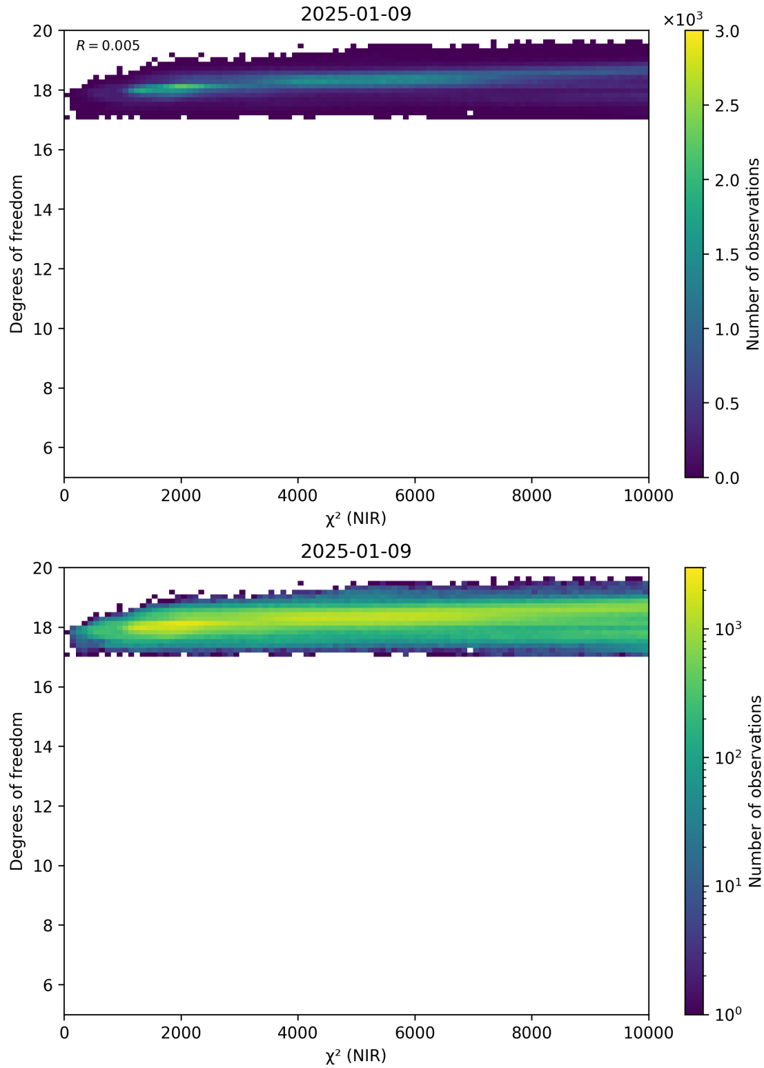
Figure 44: Scatter density plot of “ \chi^2 (NIR)” against “Degrees of freedom” for 2025-01-08 to 2025-01-10.
