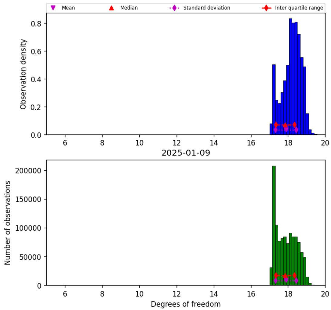
Figure 30: Histogram of “Degrees of freedom” for 2025-01-08 to 2025-01-10
