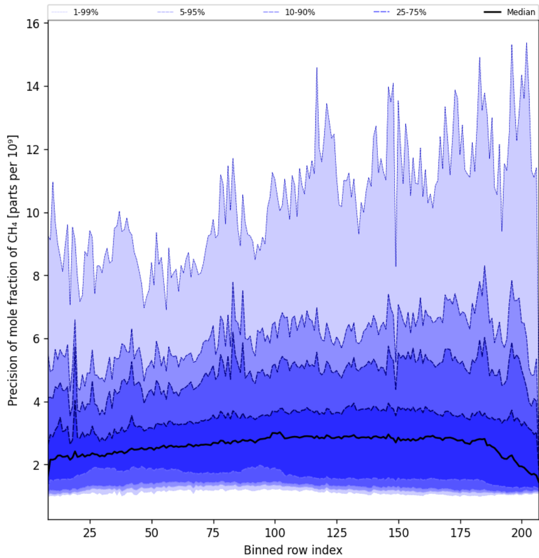
Figure 35: Along track statistics of “Precision of mole fraction of CH 4 ” for 2025-01-08 to 2025-01-10
