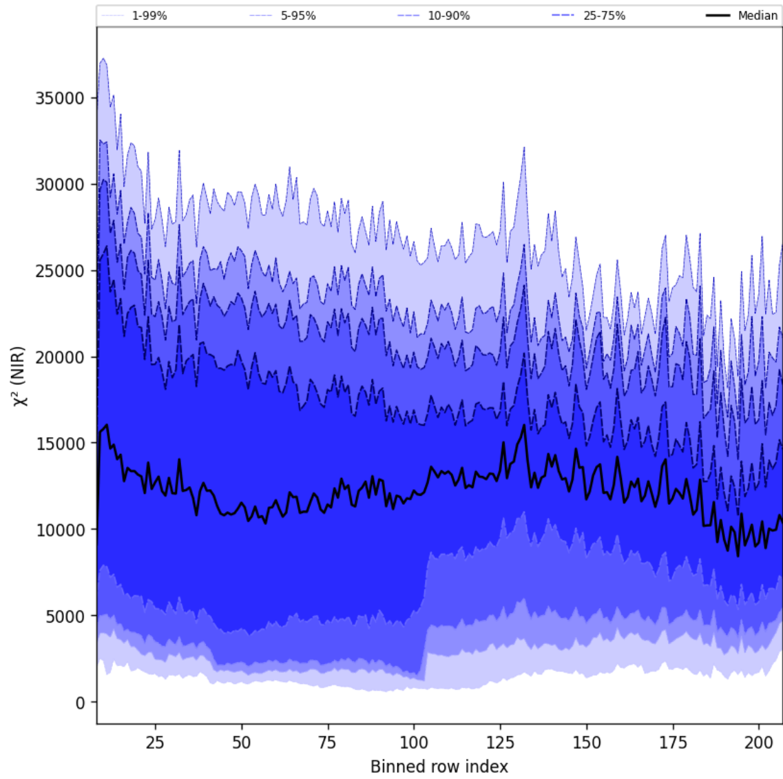
Figure 40: Along track statistics of “ \chi^2 (NIR)” for 2025-01-09 to 2025-01-11
