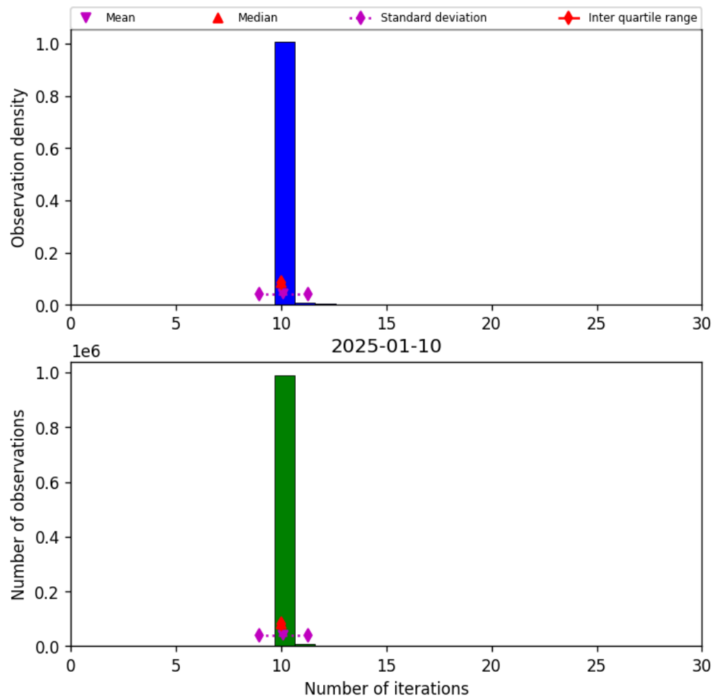
Figure 31: Histogram of “Number of iterations” for 2025-01-09 to 2025-01-11
