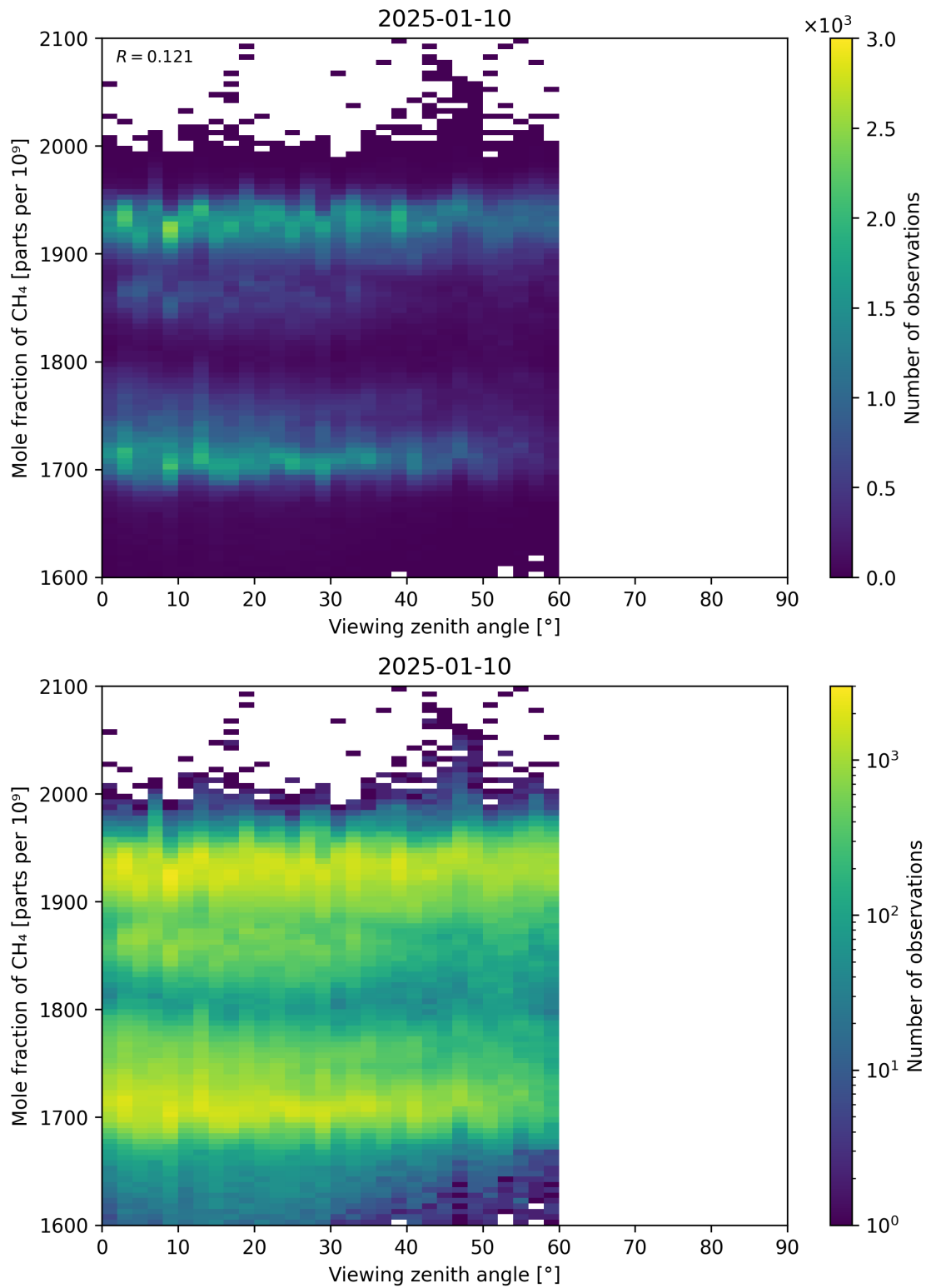
Figure 110: Scatter density plot of “Viewing zenith angle” against “Mole fraction of \text{CH}_4 ” for 2025-01-09 to 2025-01-11.
