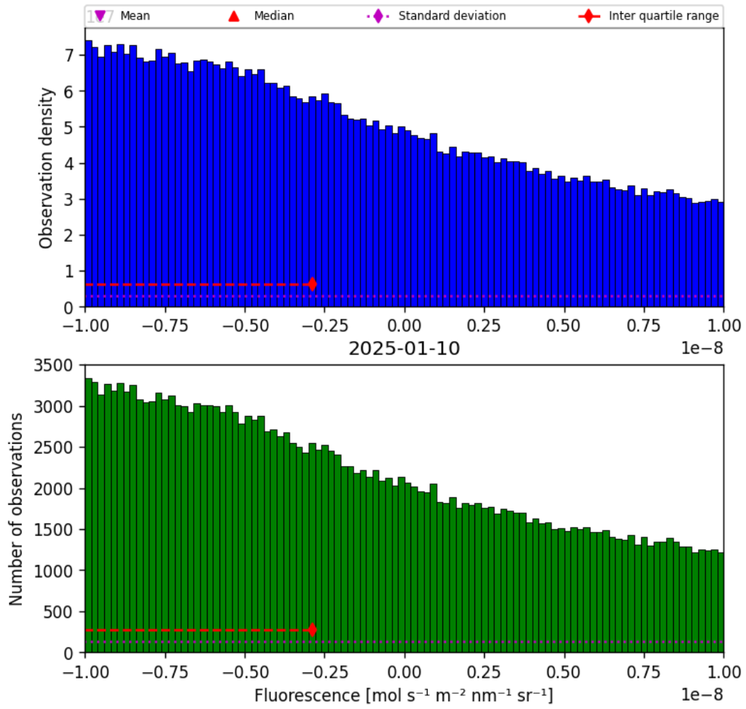
Figure 32: Histogram of “Fluorescence” for 2025-01-09 to 2025-01-11
