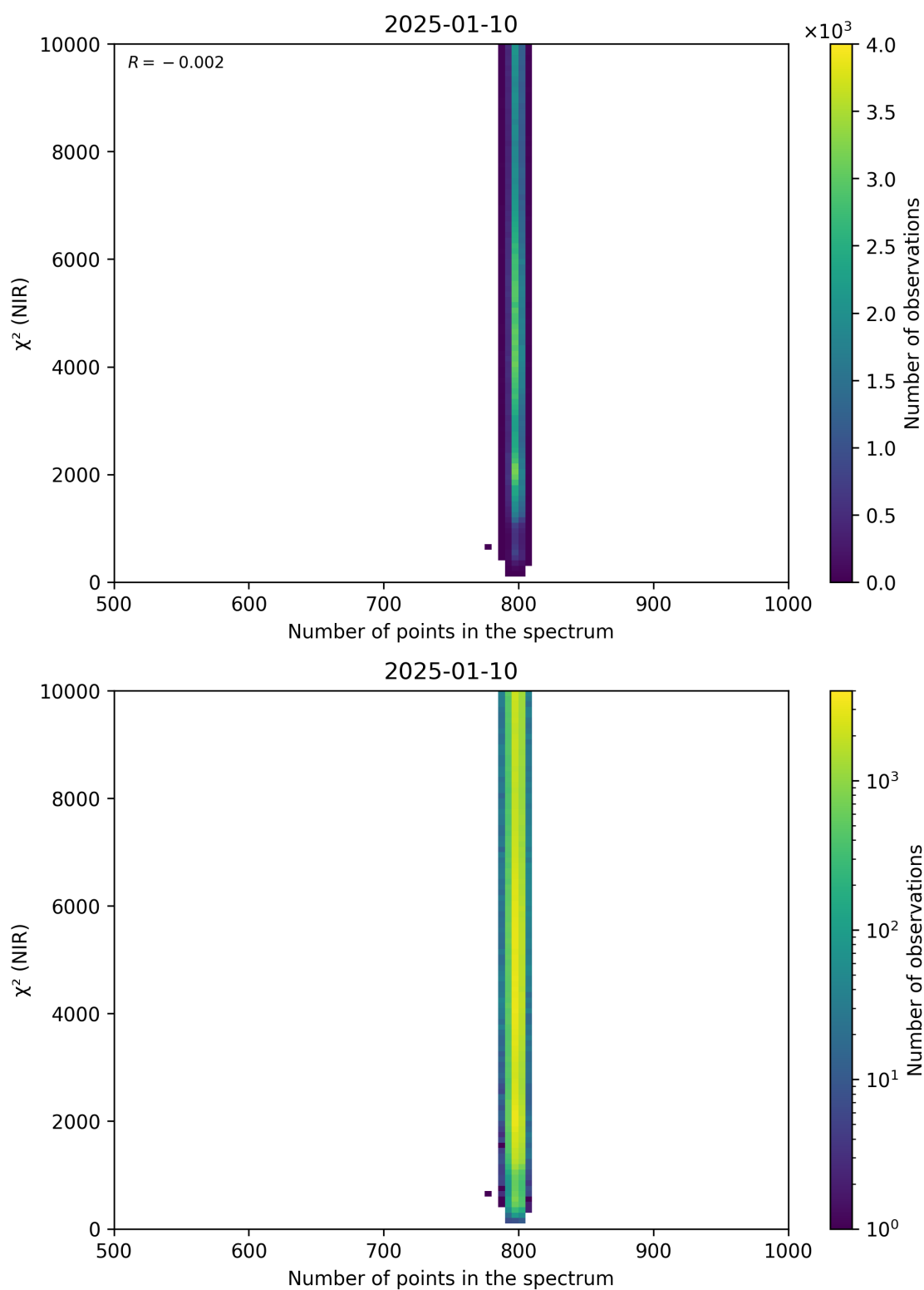
Figure 88: Scatter density plot of “Number of points in the spectrum” against “ \chi^2 (NIR)” for 2025-01-09 to 2025-01-11.
