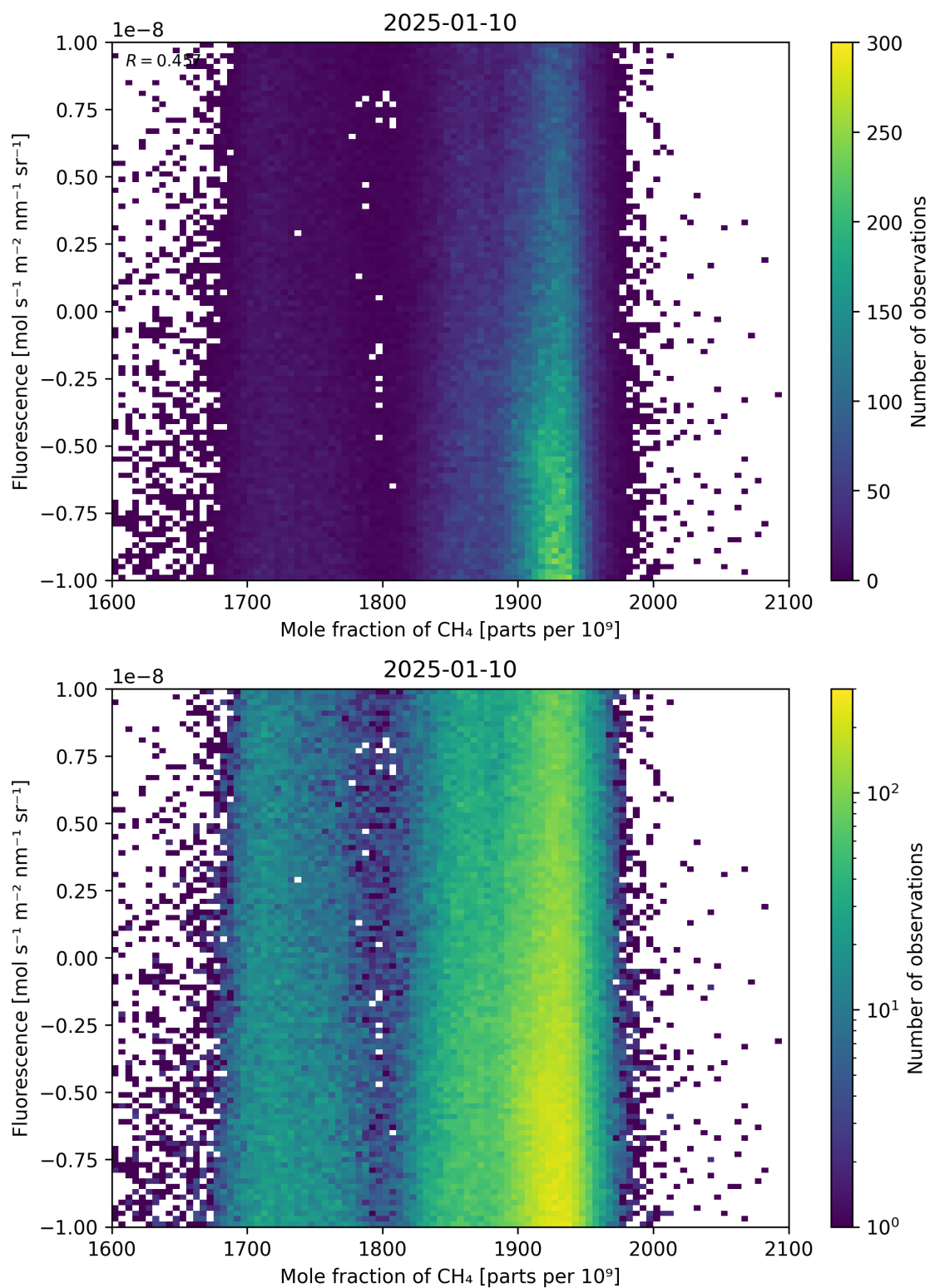
Figure 73: Scatter density plot of “Mole fraction of \text{CH}_4 ” against “Fluorescence” for 2025-01-09 to 2025-01-11.
