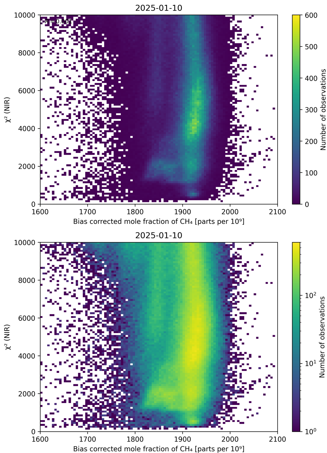
Figure 63: Scatter density plot of “Bias corrected mole fraction of CH 4 ” against “ \chi^2 (NIR)” for 2025-01-09 to 2025-01-11.
