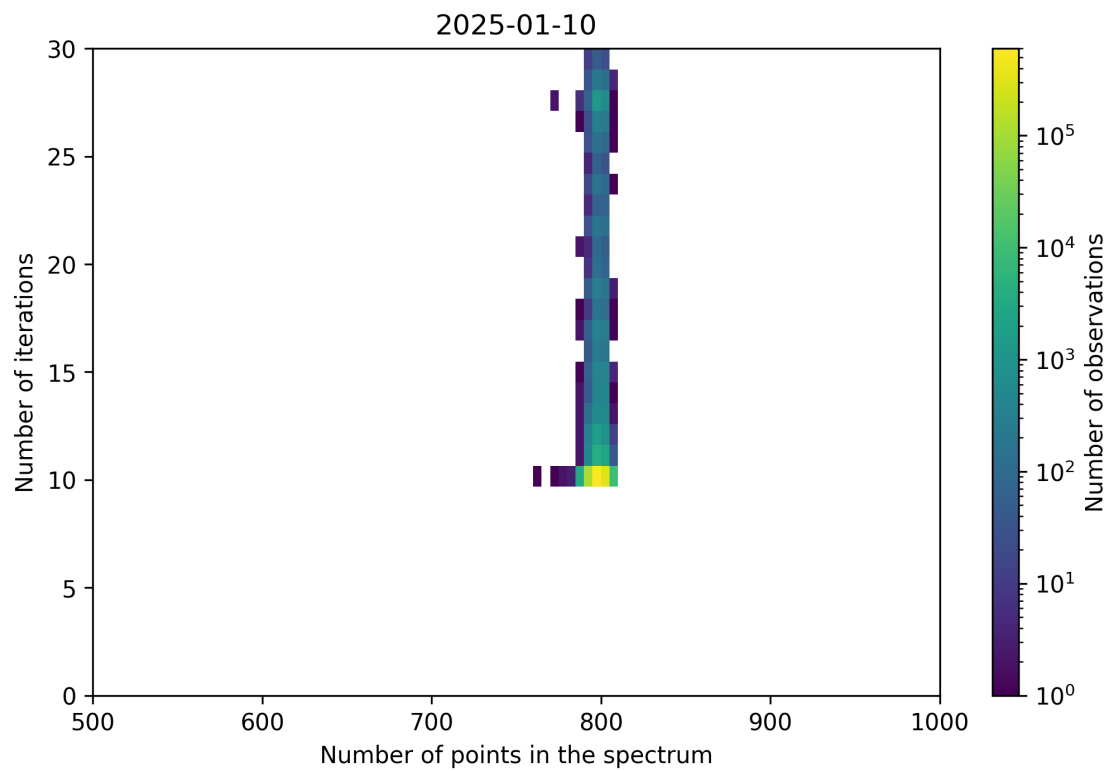
Figure 92: Scatter density plot of “Number of points in the spectrum” against “Number of iterations” for 2025-01-09 to 2025-01-11.
