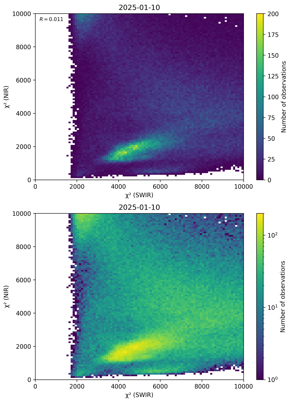
Figure 47: Scatter density plot of “ \chi^2 (SWIR)” against “ \chi^2 (NIR)” for 2025-01-09 to 2025-01-11.
