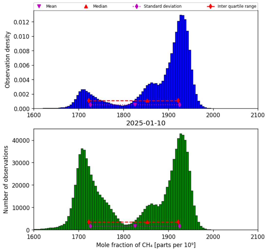
Figure 23: Histogram of “Mole fraction of CH 4 ” for 2025-01-09 to 2025-01-11
