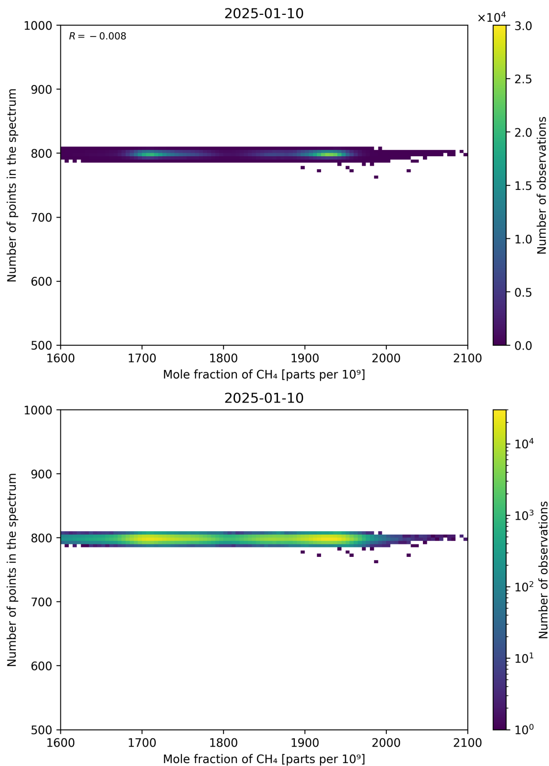
Figure 77: Scatter density plot of “Mole fraction of CH 4 ” against “Number of points in the spectrum” for 2025-01-09 to 2025-01-11.
