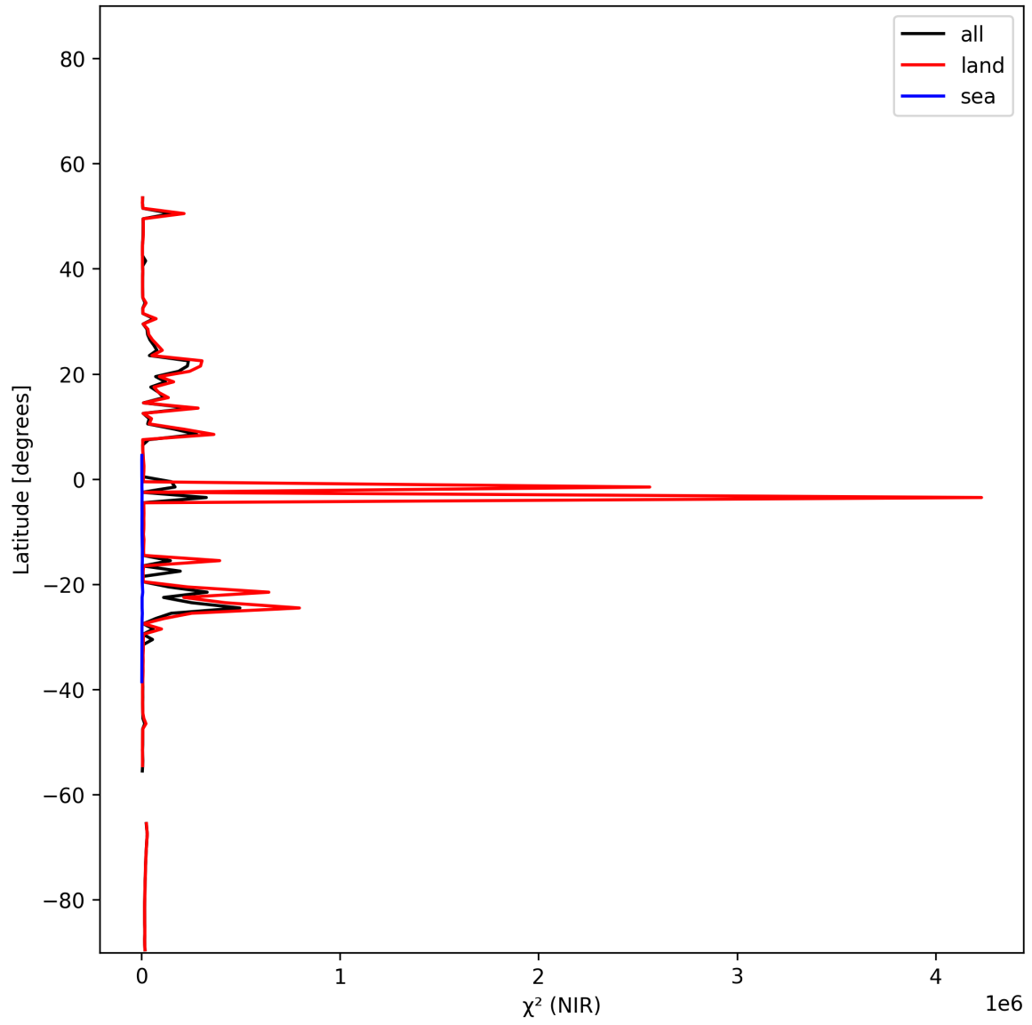
Figure 18: Zonal average of “ \chi^2 (NIR)” for 2025-01-09 to 2025-01-11.
