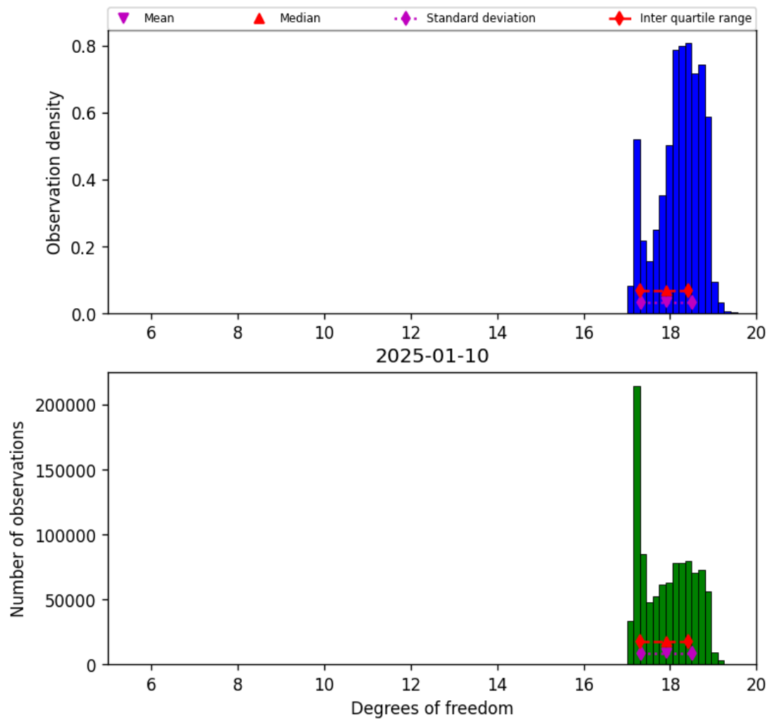
Figure 30: Histogram of “Degrees of freedom” for 2025-01-09 to 2025-01-11
