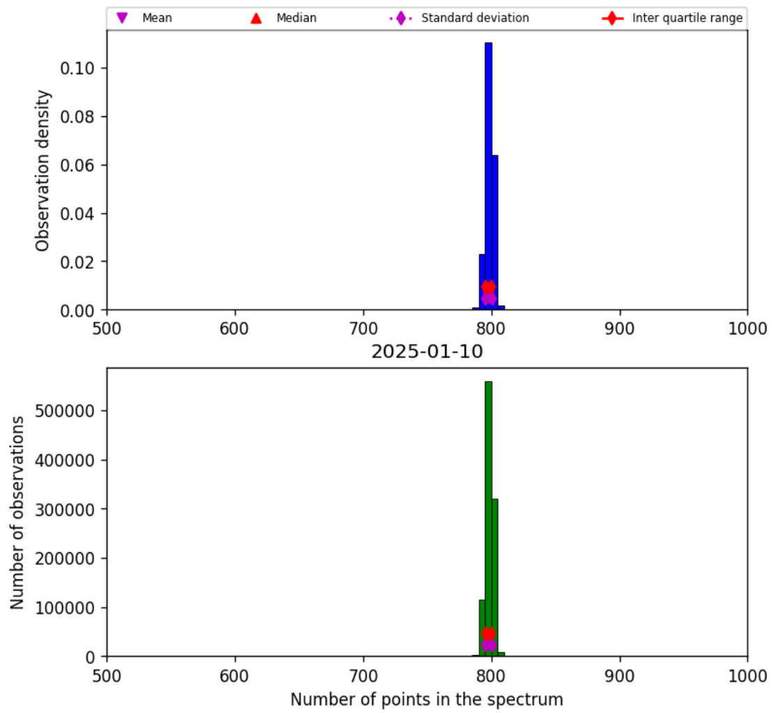
Figure 26: Histogram of “Number of points in the spectrum” for 2025-01-09 to 2025-01-11
