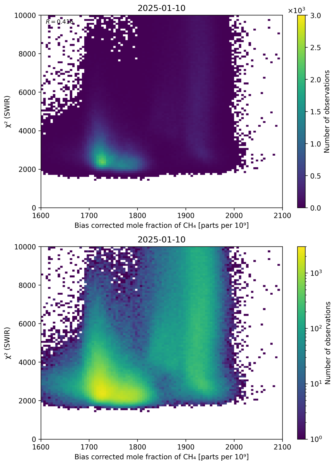
Figure 64: Scatter density plot of “Bias corrected mole fraction of \text{CH}_4 ” against “ \chi^2 (SWIR)” for 2025-01-09 to 2025-01-11.
