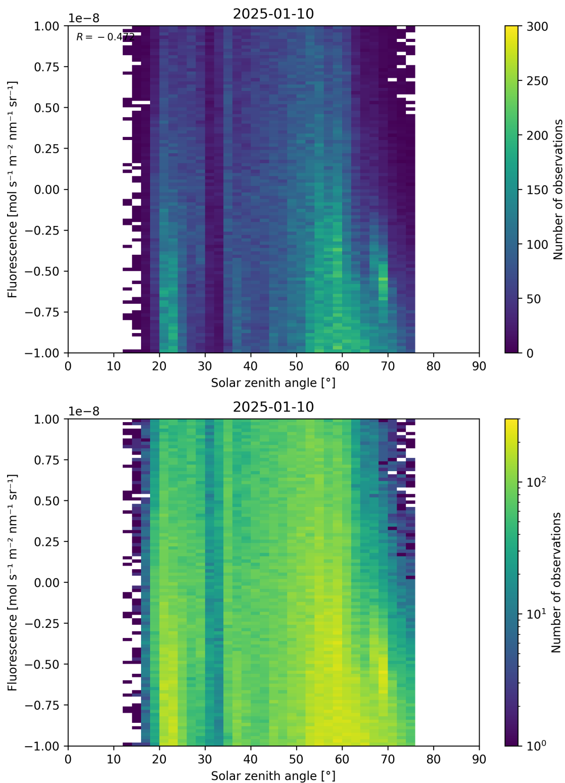
Figure 97: Scatter density plot of “Solar zenith angle” against “Fluorescence” for 2025-01-09 to 2025-01-11.
