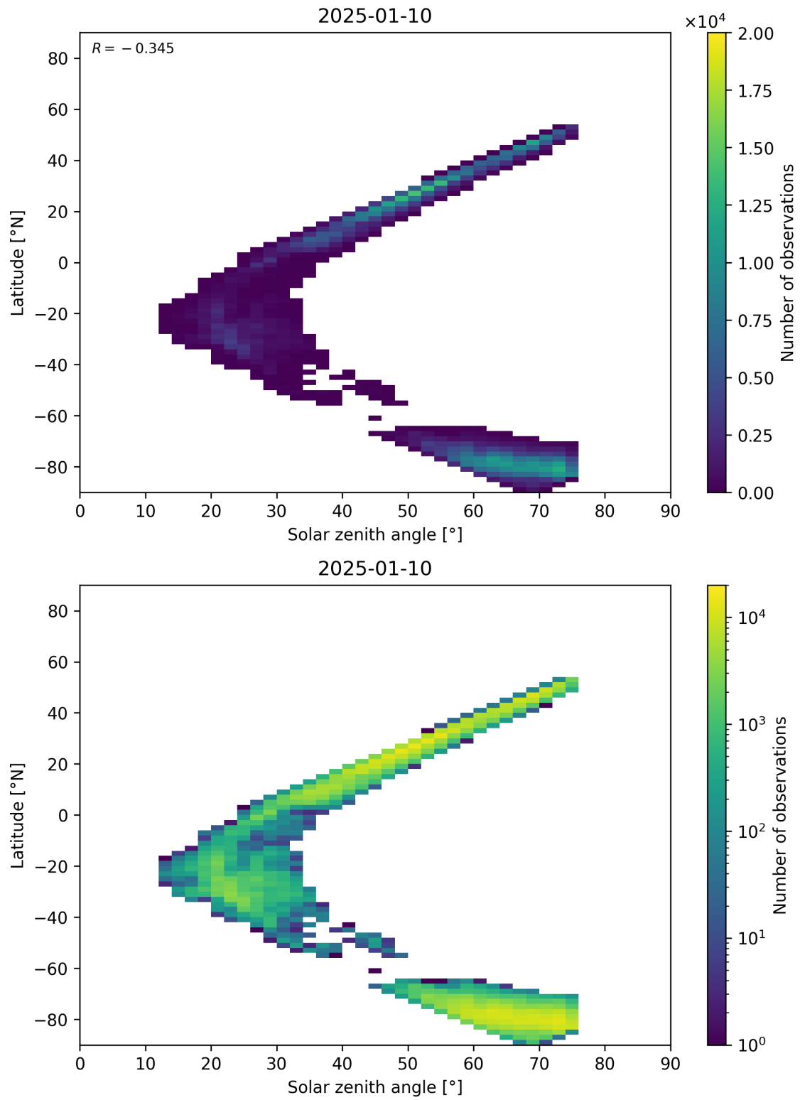
Figure 98: Scatter density plot of “Solar zenith angle” against “Latitude” for 2025-01-09 to 2025-01-11.
