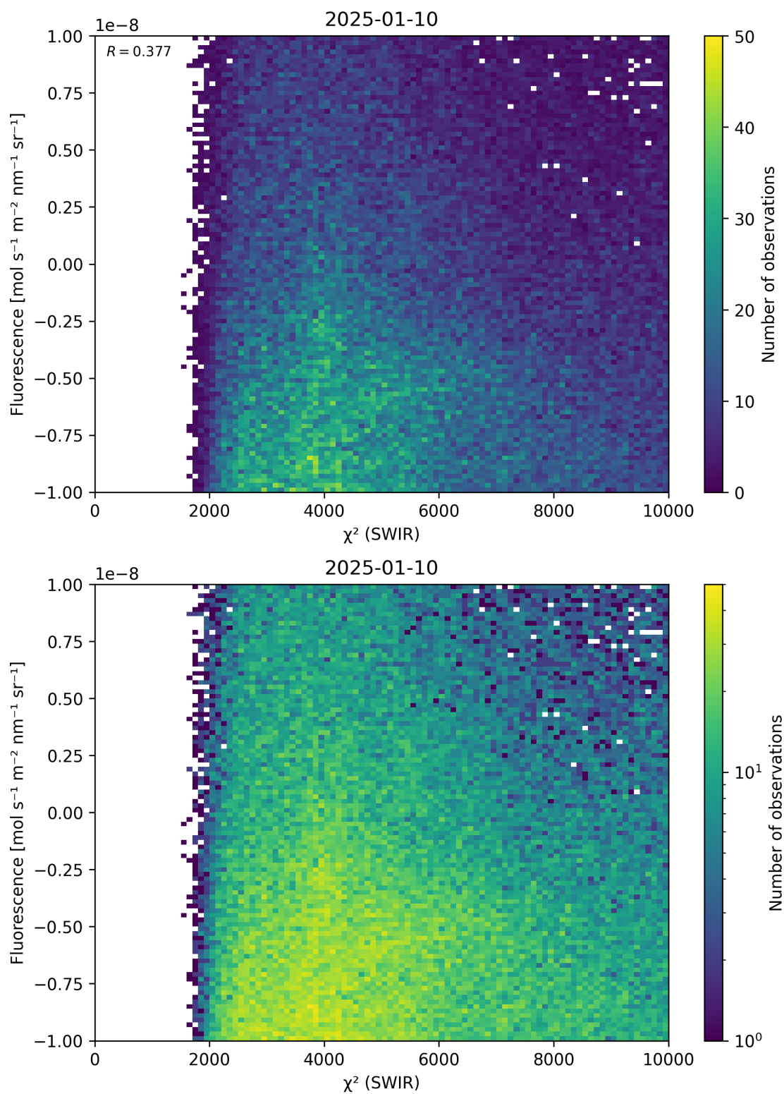
Figure 49: Scatter density plot of “ \chi^2 (SWIR)” against “Fluorescence” for 2025-01-09 to 2025-01-11.
