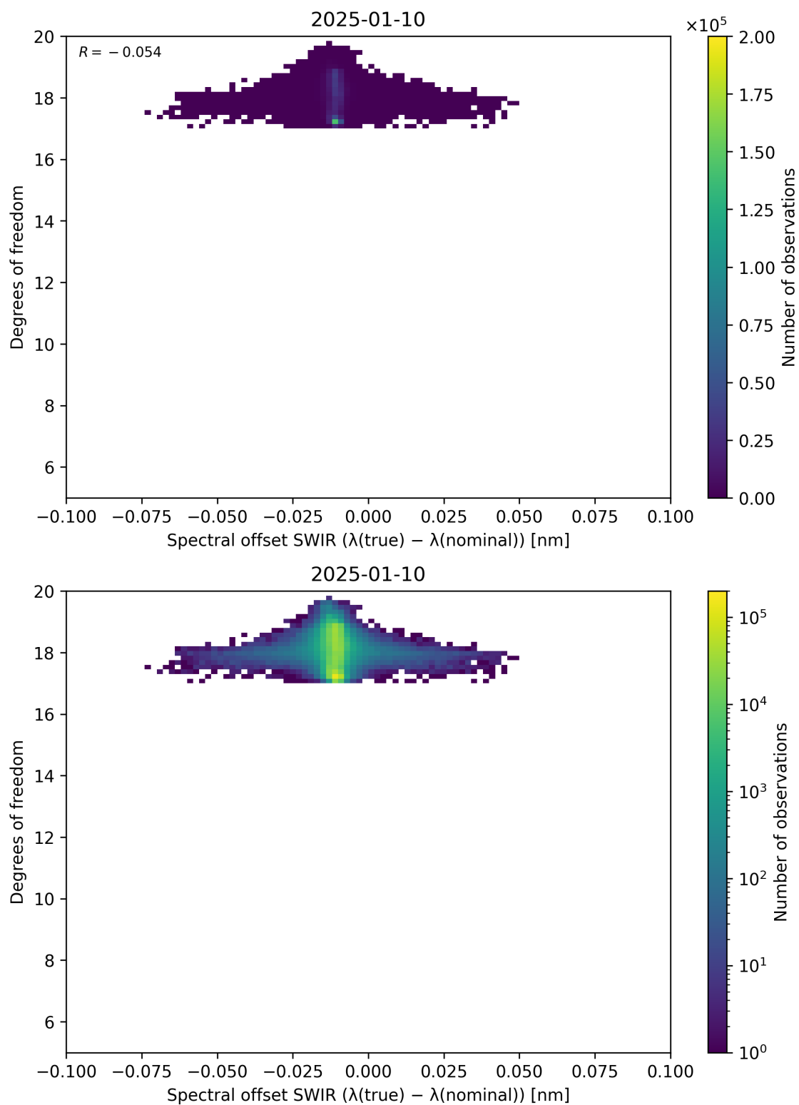
Figure 119: Scatter density plot of “Spectral offset SWIR ( \lambda_{\text{true}} - \lambda_{\text{nominal}} )” against “Degrees of freedom” for 2025-01-09 to 2025-01-11.
