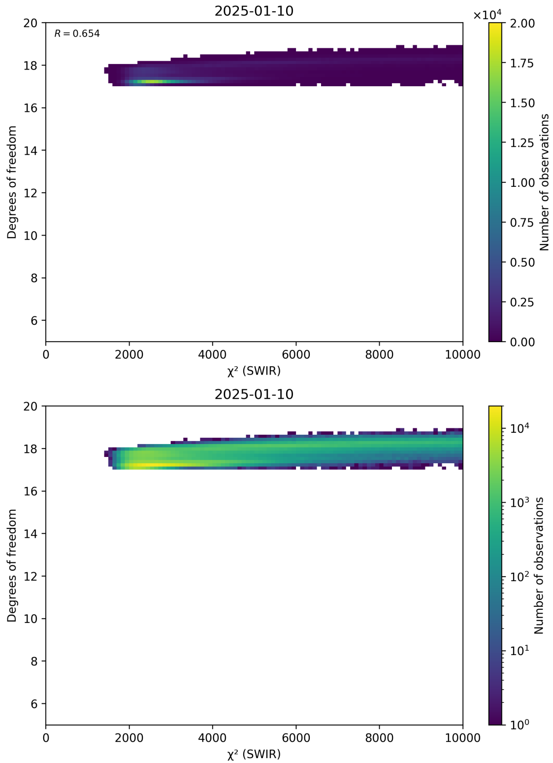
Figure 48: Scatter density plot of “ \chi^2 (SWIR)” against “Degrees of freedom” for 2025-01-09 to 2025-01-11.
