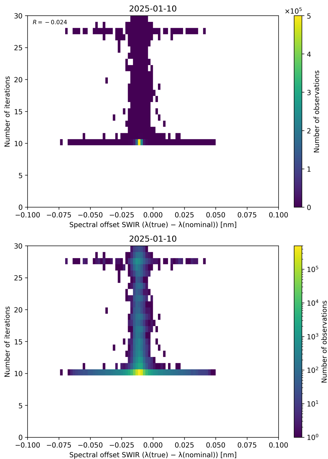
Figure 121: Scatter density plot of “Spectral offset SWIR ( \lambda_{\text{true}} - \lambda_{\text{nominal}} )” against “Number of iterations” for 2025-01-09 to 2025-01-11.
