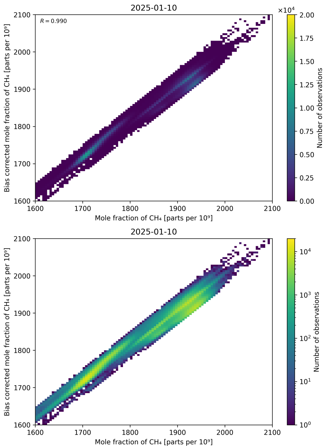
Figure 74: Scatter density plot of “Mole fraction of CH 4 ” against “Bias corrected mole fraction of CH 4 ” for 2025-01-09 to 2025-01-11.
