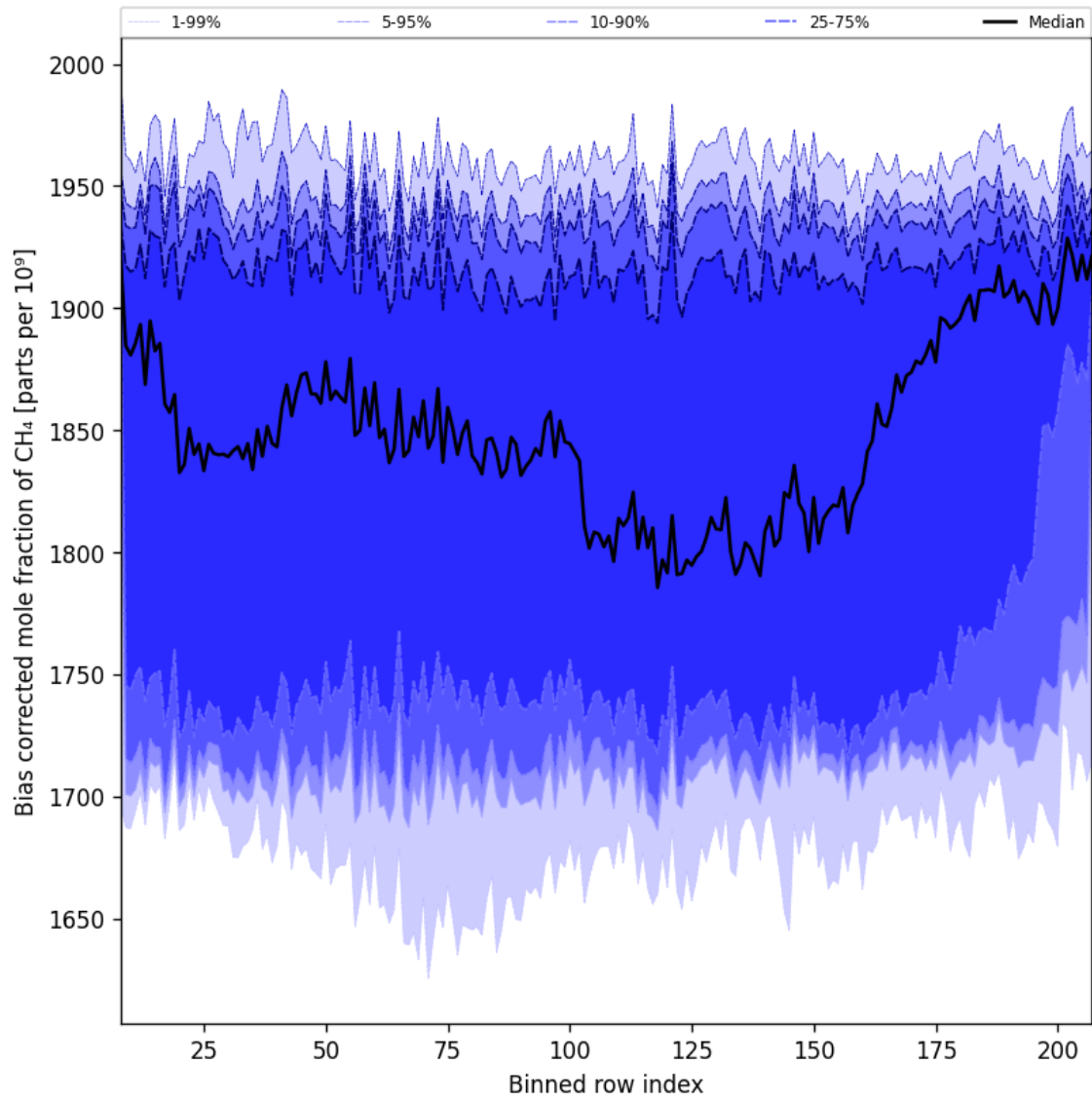
Figure 36: Along track statistics of “Bias corrected mole fraction of CH 4 ” for 2025-01-09 to 2025-01-11
