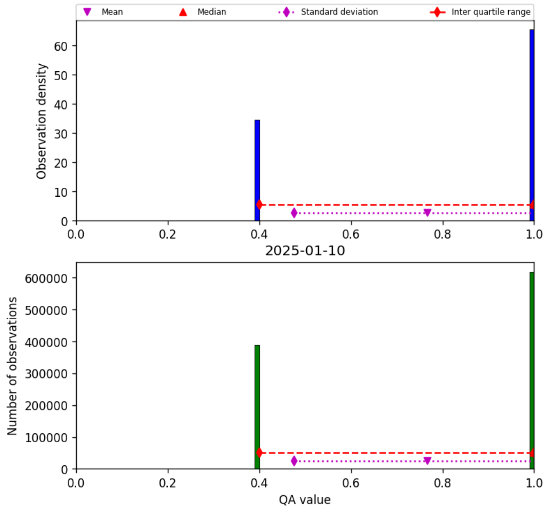
Figure 22: Histogram of “QA value” for 2025-01-09 to 2025-01-11
