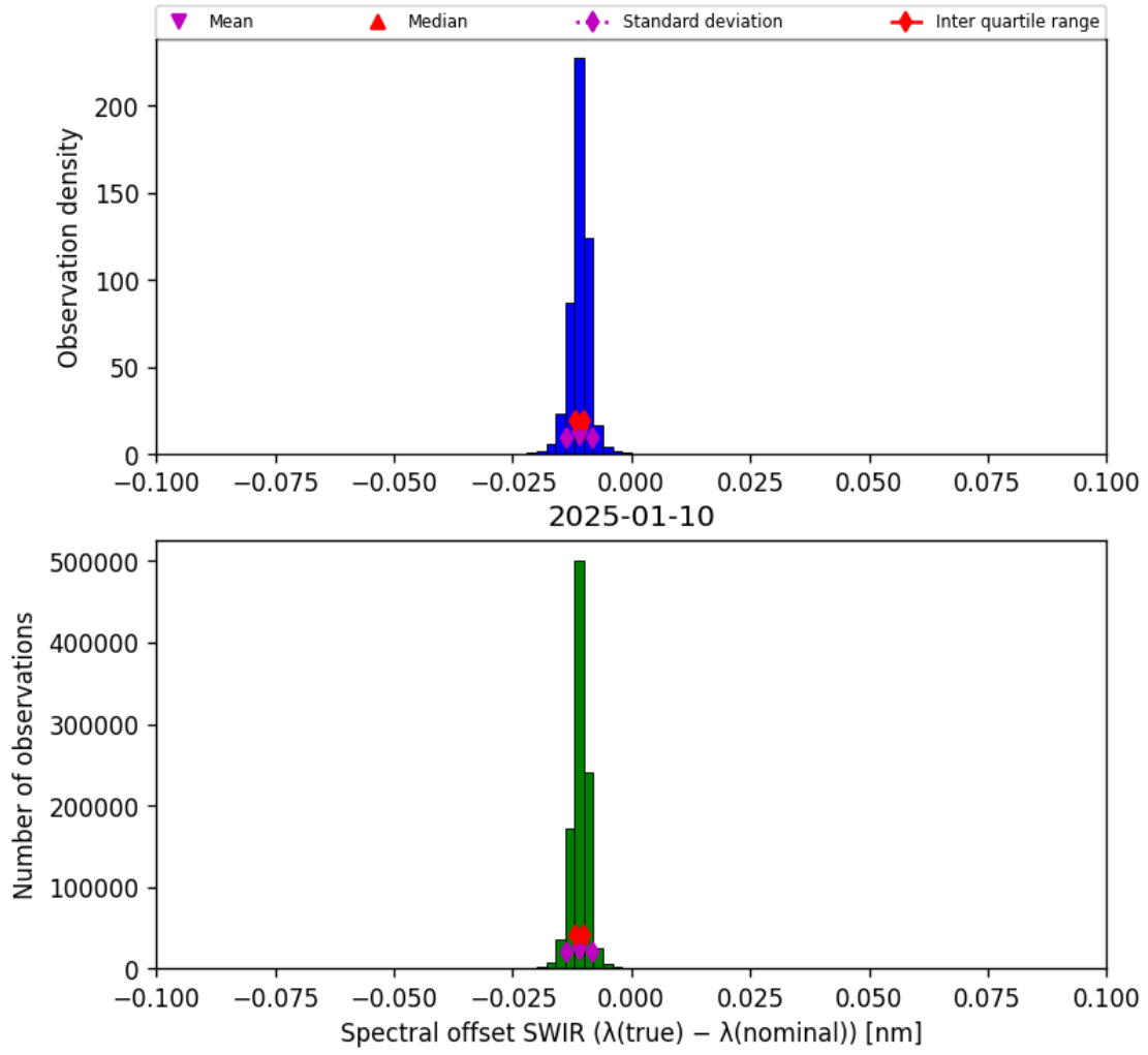
Figure 27: Histogram of “Spectral offset SWIR ( \lambda_{\text{true}} - \lambda_{\text{nominal}} )” for 2025-01-09 to 2025-01-11
