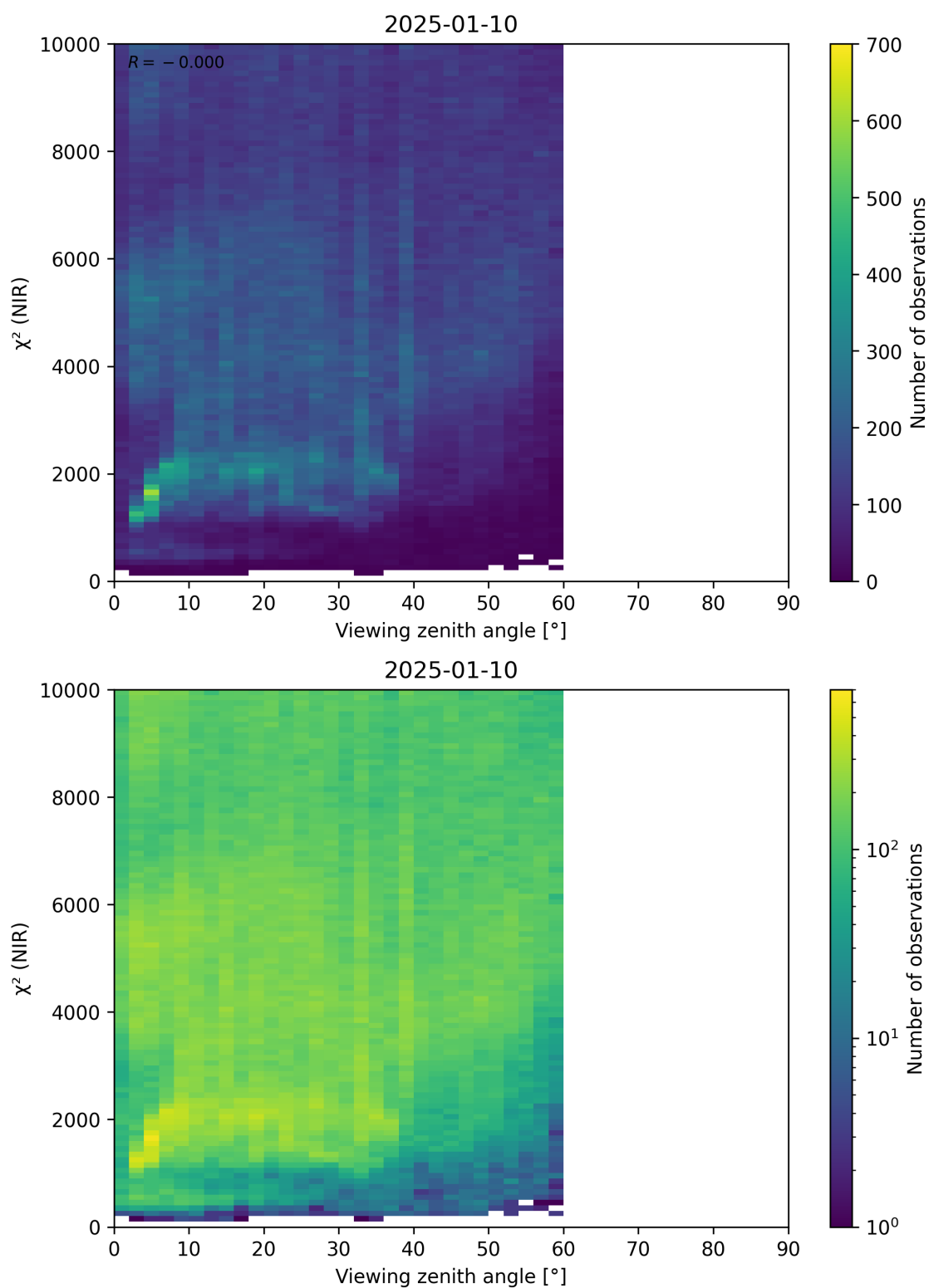
Figure 105: Scatter density plot of “Viewing zenith angle” against “ \chi^2 (NIR)” for 2025-01-09 to 2025-01-11.
