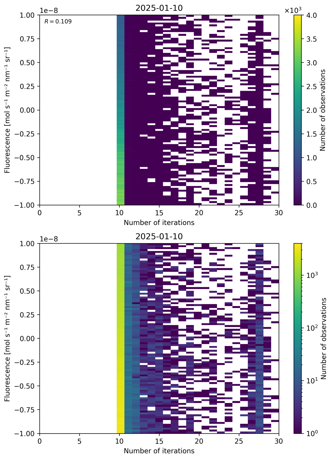
Figure 87: Scatter density plot of “Number of iterations” against “Fluorescence” for 2025-01-09 to 2025-01-11.
