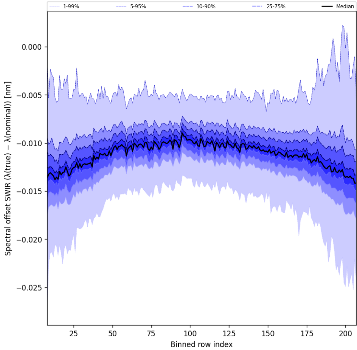
Figure 38: Along track statistics of “Spectral offset SWIR ( \lambda_{\text{true}} - \lambda_{\text{nominal}} )” for 2025-01-09 to 2025-01-11
