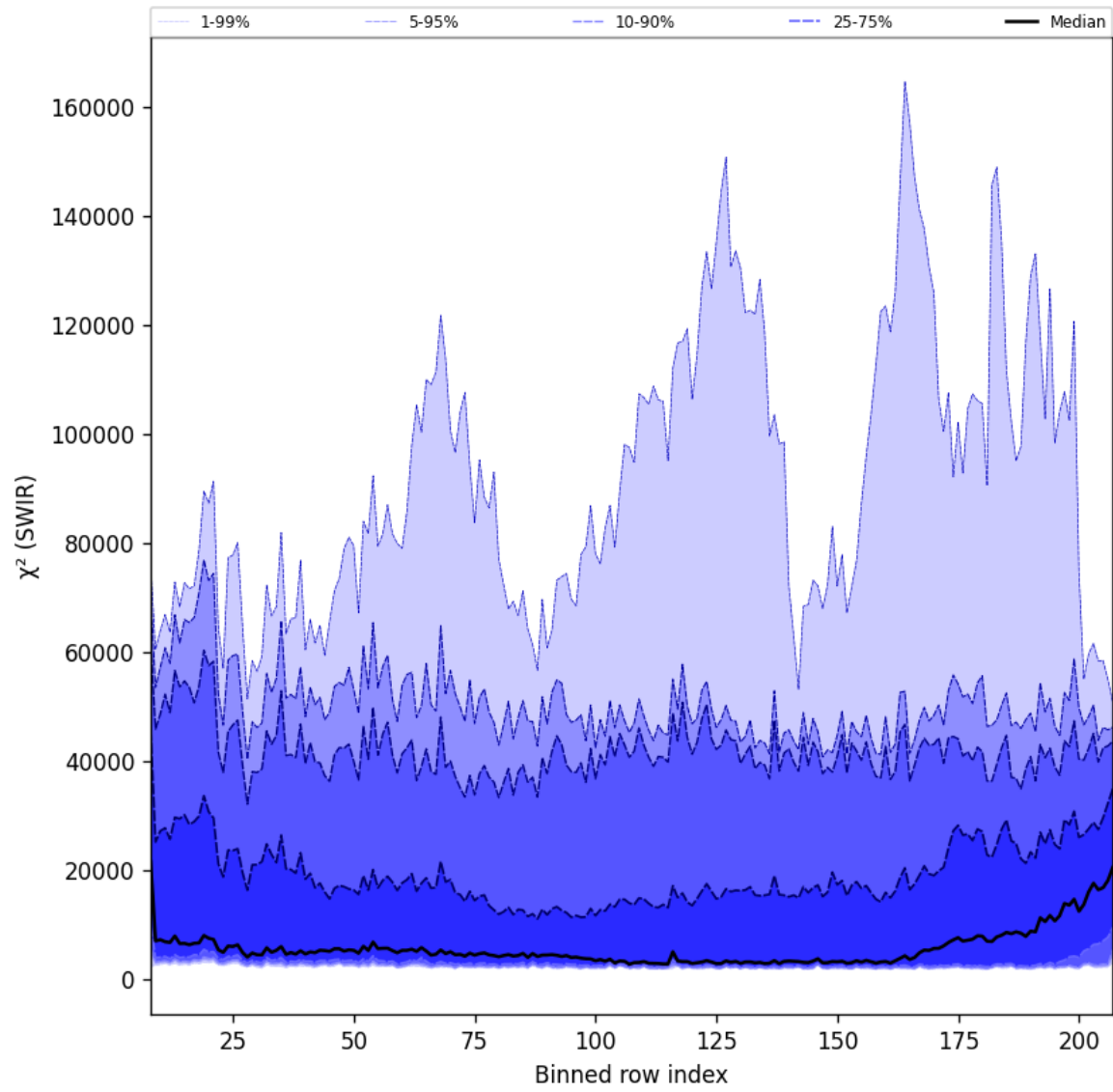
Figure 39: Along track statistics of “ \chi^2 (SWIR)” for 2025-01-09 to 2025-01-11
