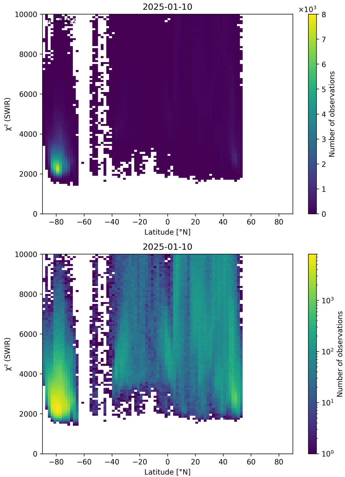
Figure 54: Scatter density plot of “Latitude” against “ \chi^2 (SWIR)” for 2025-01-09 to 2025-01-11.
