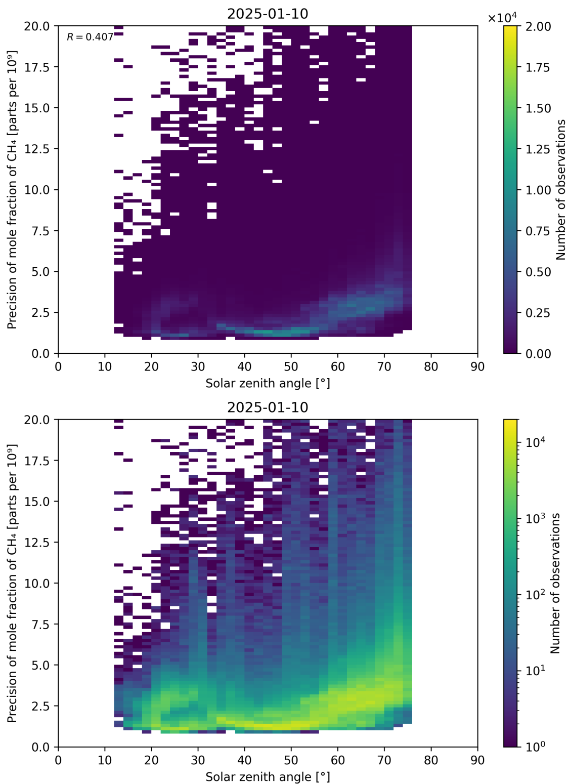
Figure 101: Scatter density plot of “Solar zenith angle” against “Precision of mole fraction of CH 4 ” for 2025-01-09 to 2025-01-11.
