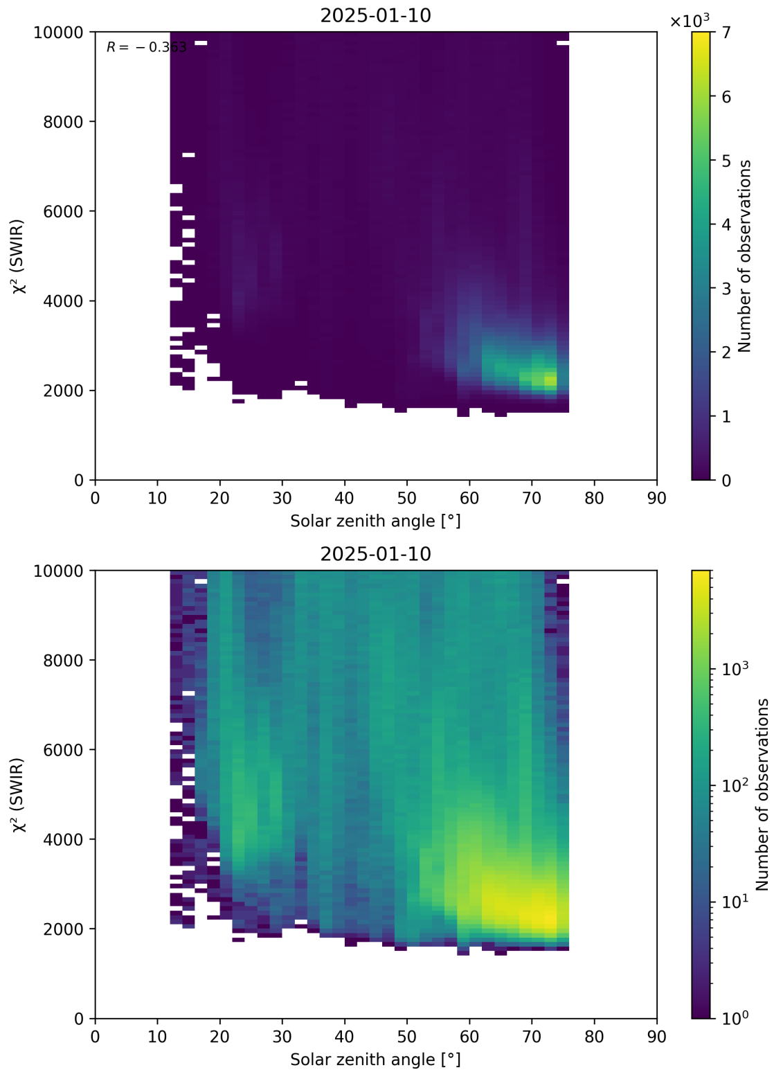
Figure 95: Scatter density plot of “Solar zenith angle” against “ \chi^2 (SWIR)” for 2025-01-09 to 2025-01-11.
