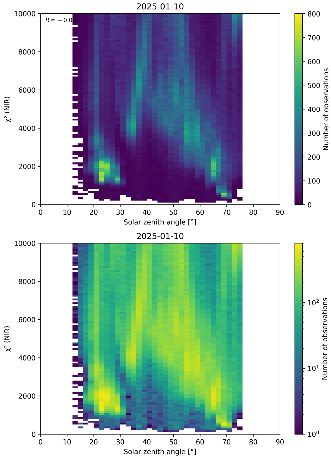
Figure 94: Scatter density plot of “Solar zenith angle” against “ \chi^2 (NIR)” for 2025-01-09 to 2025-01-11.
