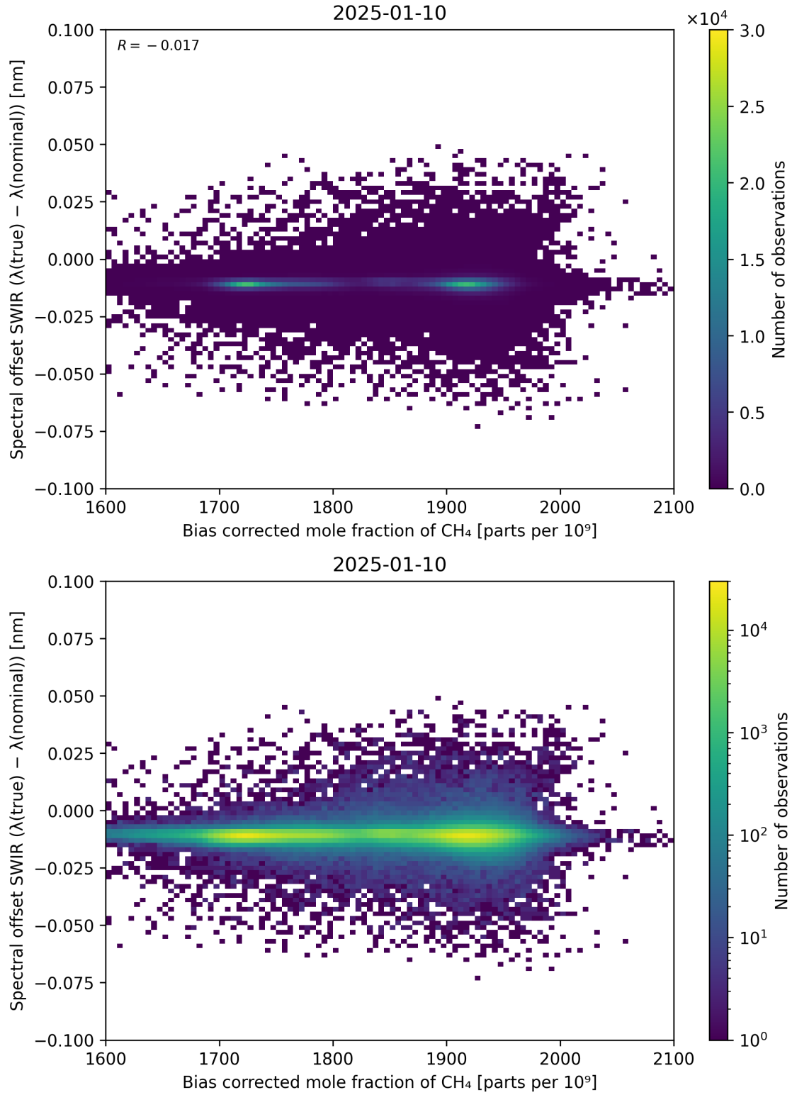
Figure 69: Scatter density plot of “Bias corrected mole fraction of \text{CH}_4 ” against “Spectral offset SWIR ( \lambda_{\text{true}} - \lambda_{\text{nominal}} )” for 2025-01-09 to 2025-01-11.
