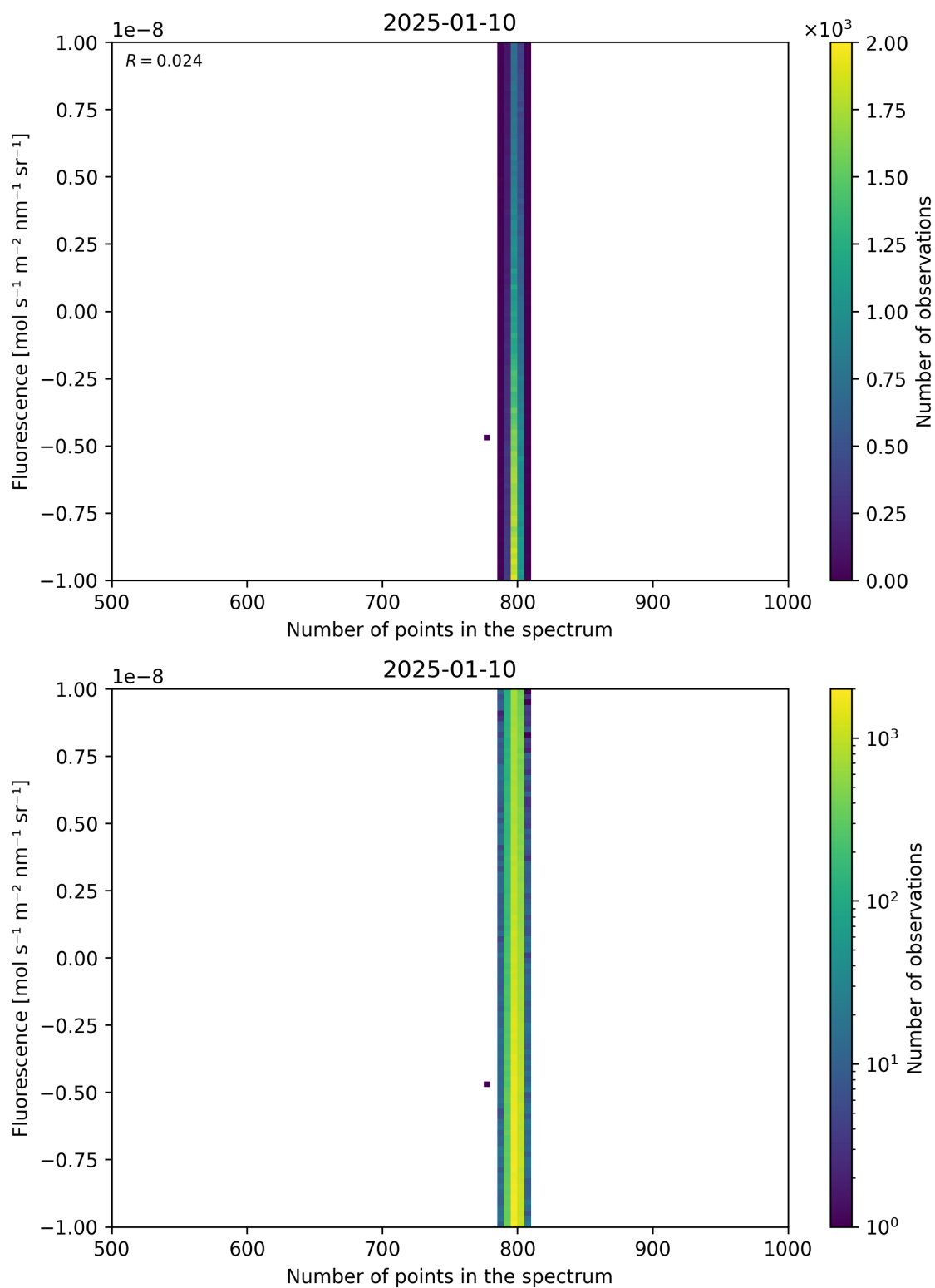
Figure 91: Scatter density plot of “Number of points in the spectrum” against “Fluorescence” for 2025-01-09 to 2025-01-11.
