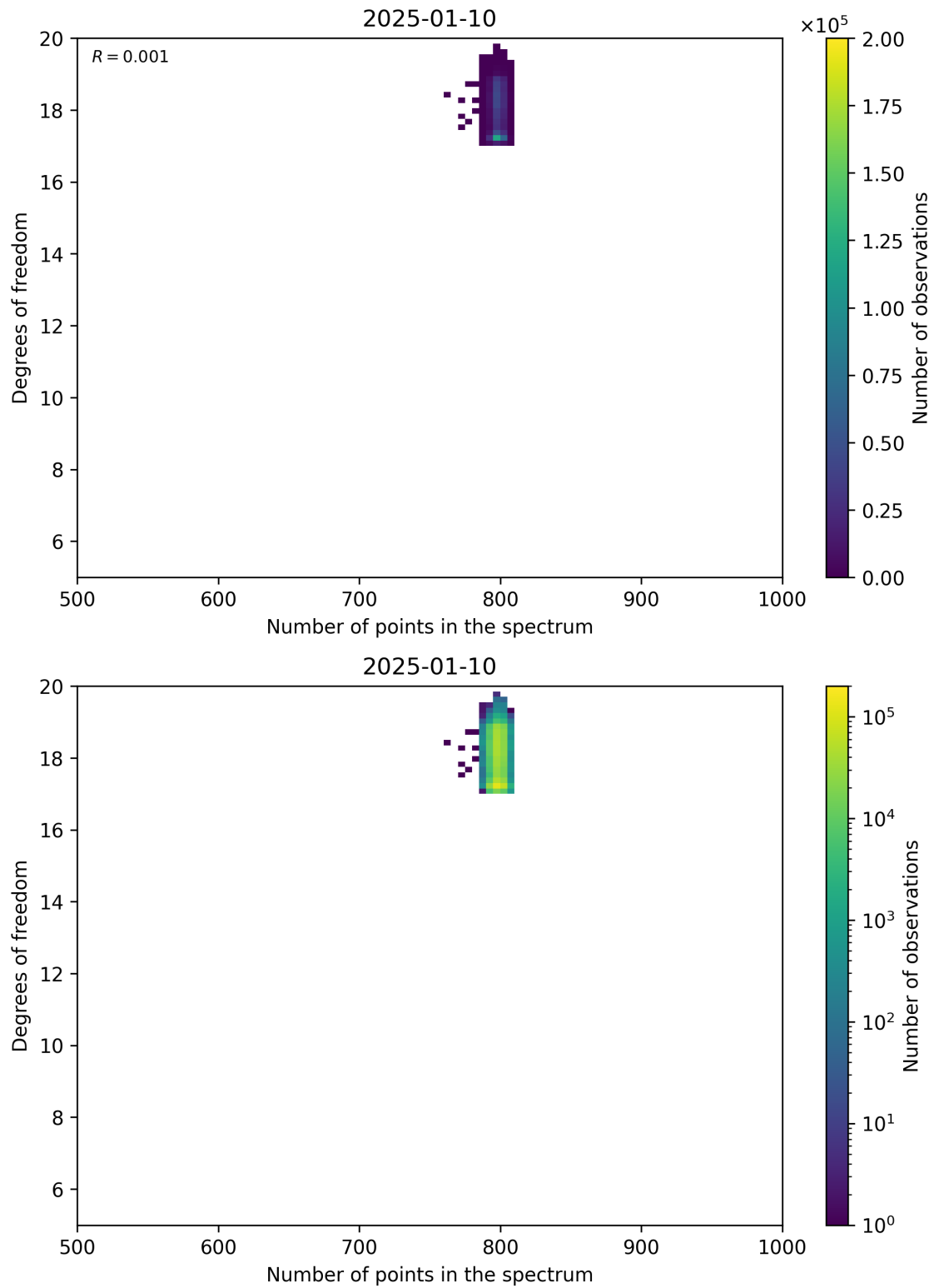
Figure 90: Scatter density plot of “Number of points in the spectrum” against “Degrees of freedom” for 2025-01-09 to 2025-01-11.
