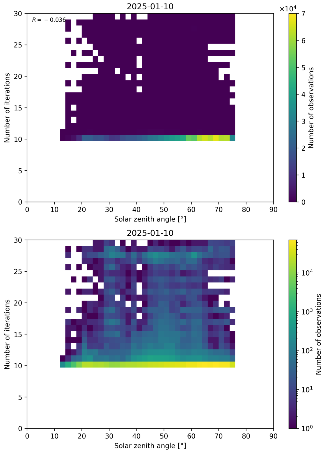
Figure 102: Scatter density plot of “Solar zenith angle” against “Number of iterations” for 2025-01-09 to 2025-01-11.
