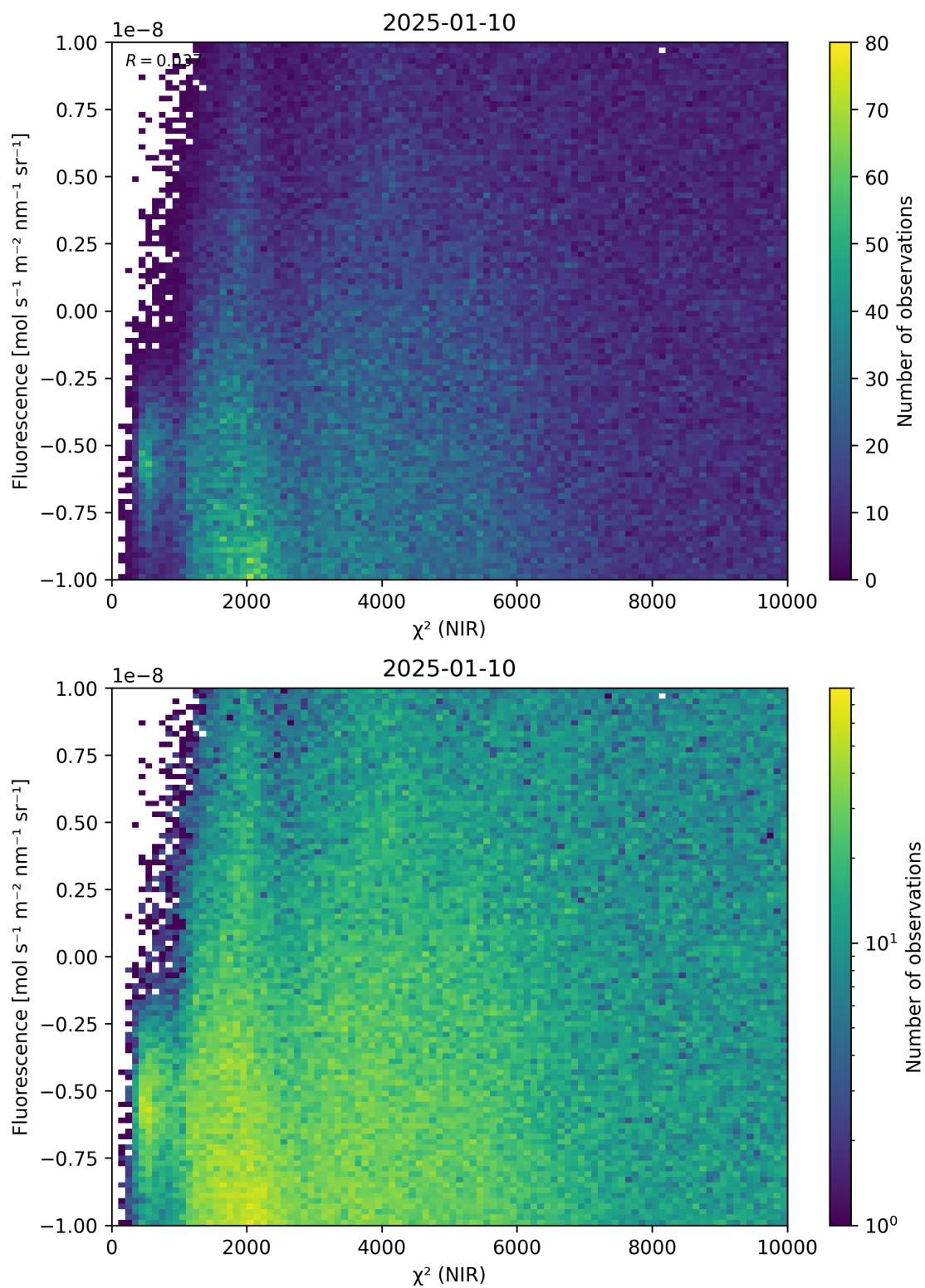
Figure 45: Scatter density plot of “ \chi^2 (NIR)” against “Fluorescence” for 2025-01-09 to 2025-01-11.
