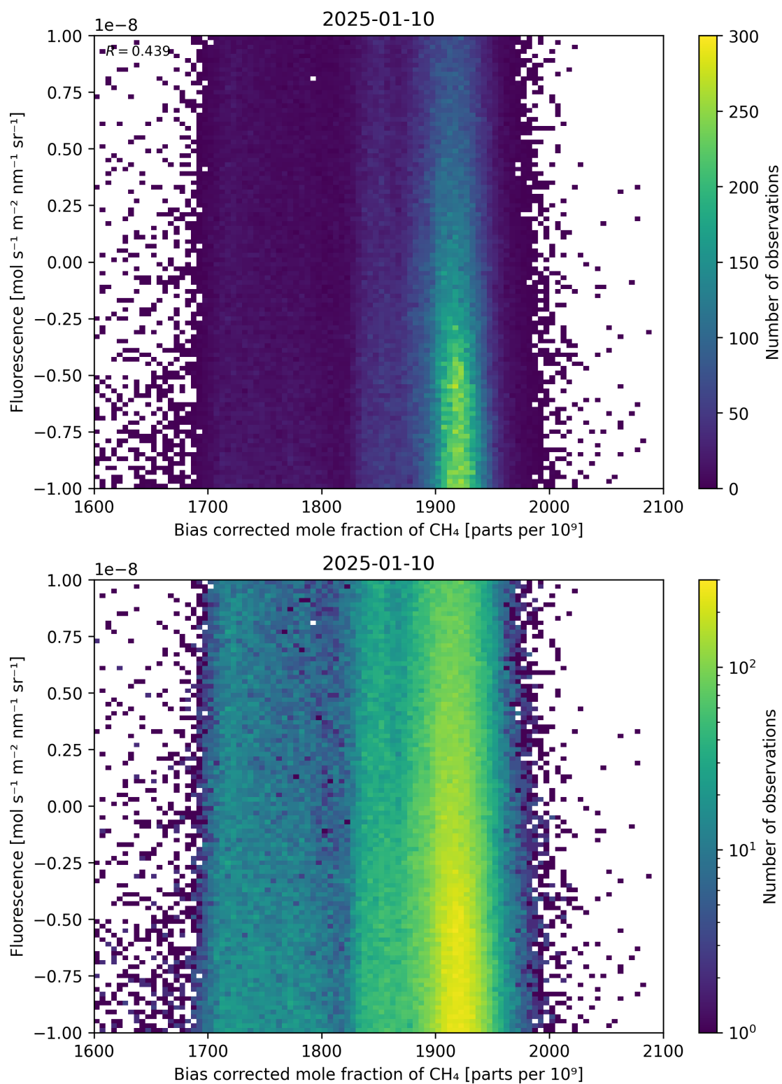
Figure 66: Scatter density plot of “Bias corrected mole fraction of \text{CH}_4 ” against “Fluorescence” for 2025-01-09 to 2025-01-11.
