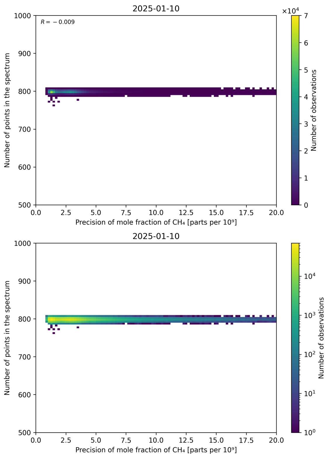
Figure 84: Scatter density plot of “Precision of mole fraction of CH 4 ” against “Number of points in the spectrum” for 2025-01-09 to 2025-01-11.
