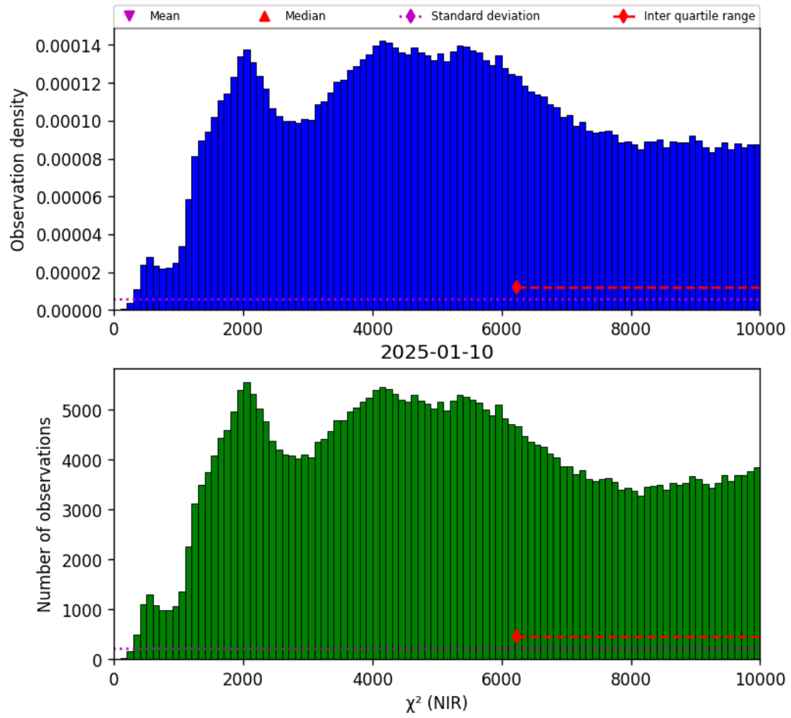
Figure 29: Histogram of “ \chi^2 (NIR)” for 2025-01-09 to 2025-01-11
