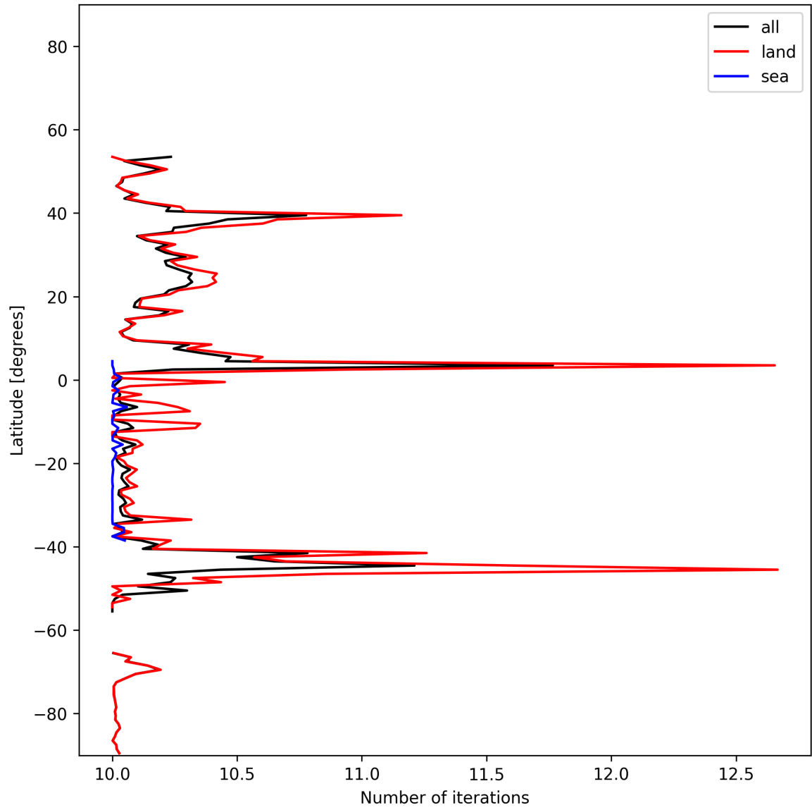
Figure 20: Zonal average of “Number of iterations” for 2025-01-09 to 2025-01-11.
