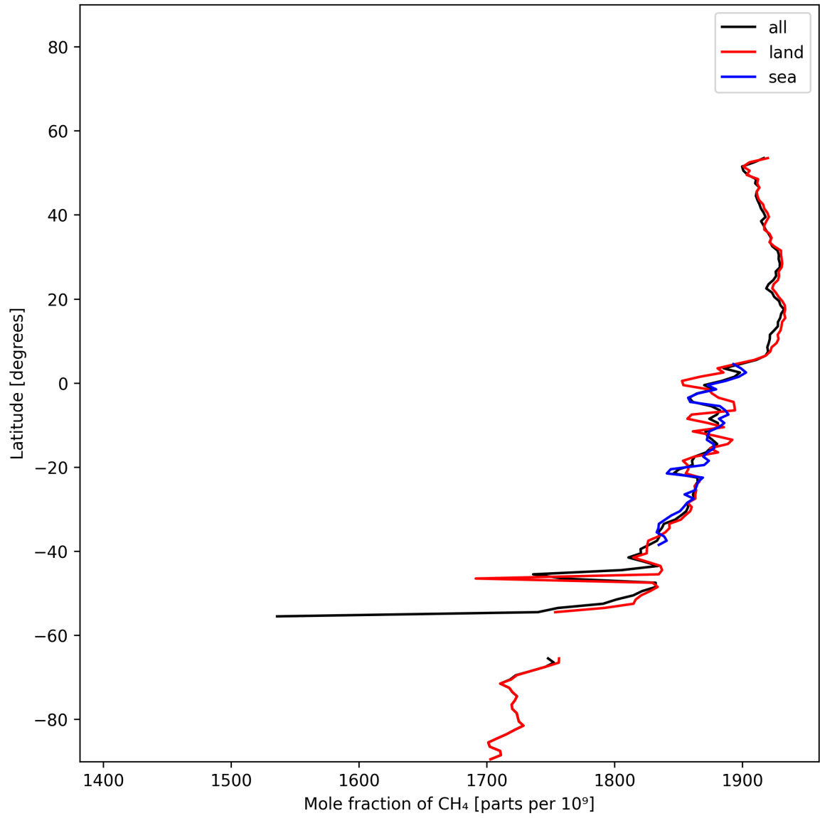
Figure 12: Zonal average of “Mole fraction of \text{CH}_4 ” for 2025-01-09 to 2025-01-11.
