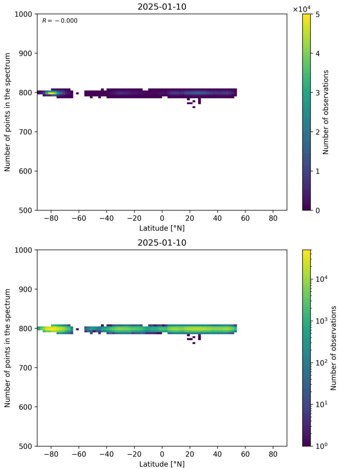
Figure 61: Scatter density plot of “Latitude” against “Number of points in the spectrum” for 2025-01-09 to 2025-01-11.
