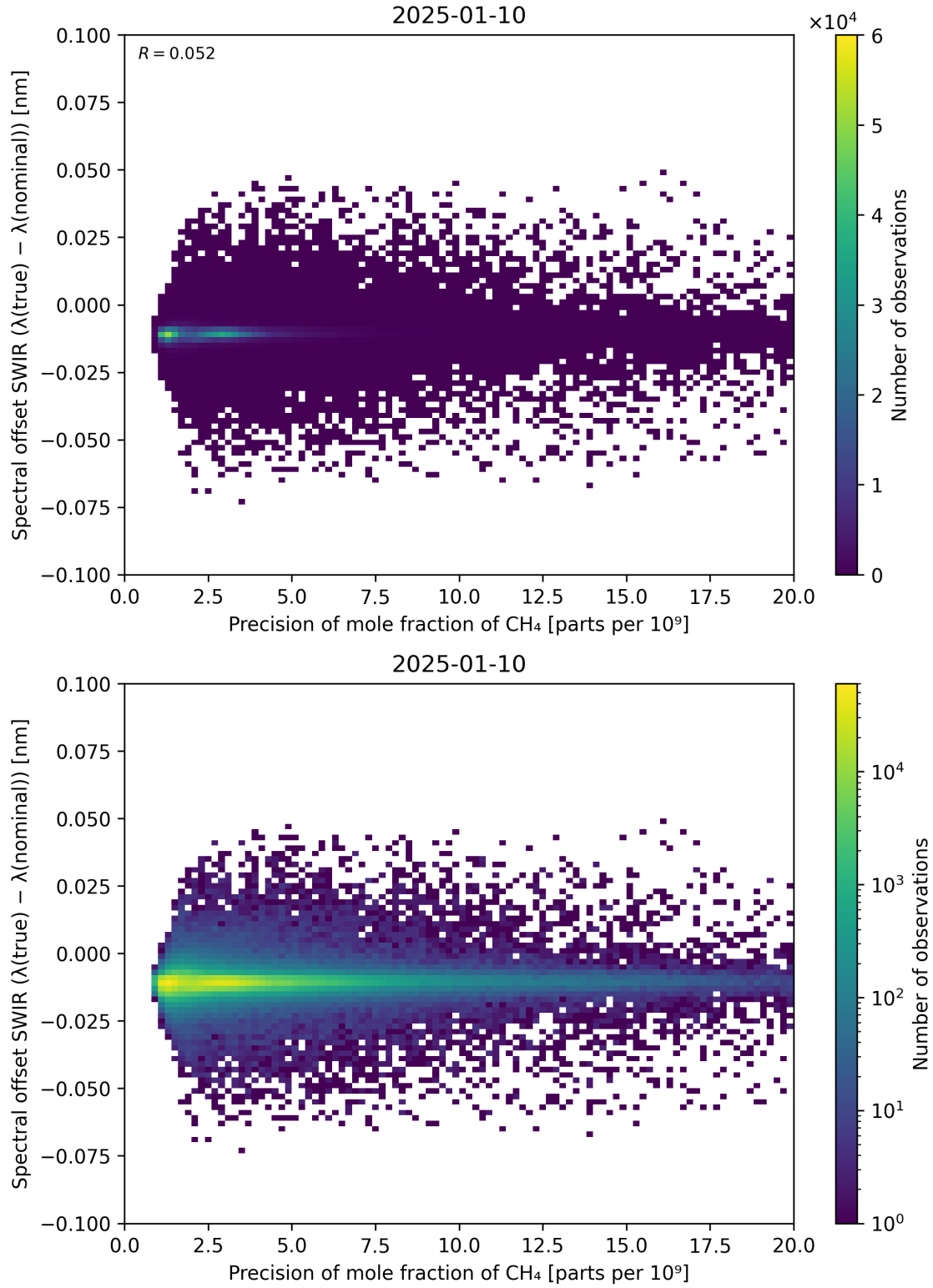
Figure 85: Scatter density plot of “Precision of mole fraction of \text{CH}_4 ” against “Spectral offset SWIR ( \lambda_{\text{true}} - \lambda_{\text{nominal}} )” for 2025-01-09 to 2025-01-11.
