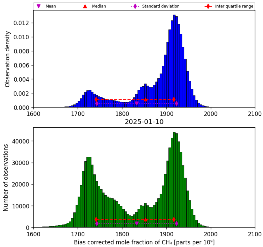
Figure 25: Histogram of “Bias corrected mole fraction of CH 4 ” for 2025-01-09 to 2025-01-11
