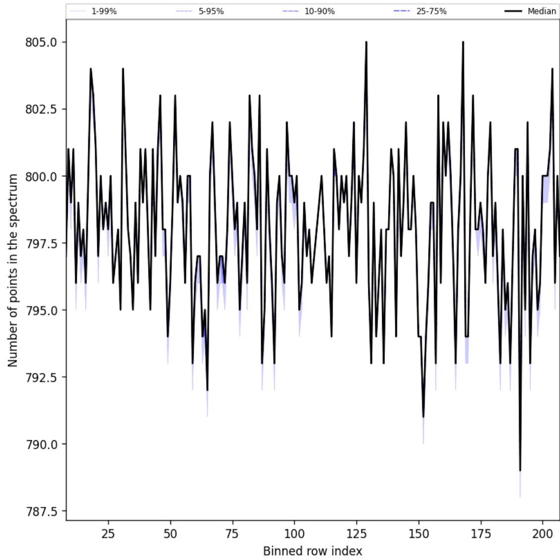
Figure 37: Along track statistics of “Number of points in the spectrum” for 2025-01-09 to 2025-01-11
