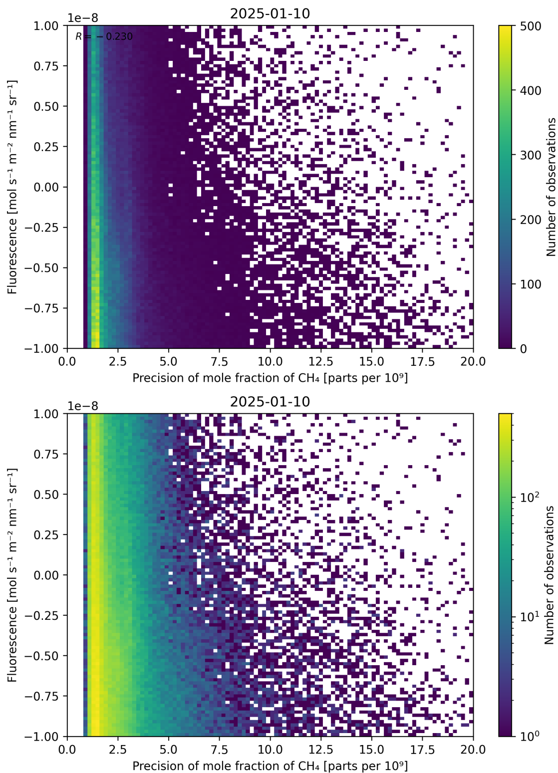
Figure 81: Scatter density plot of “Precision of mole fraction of \text{CH}_4 ” against “Fluorescence” for 2025-01-09 to 2025-01-11.
