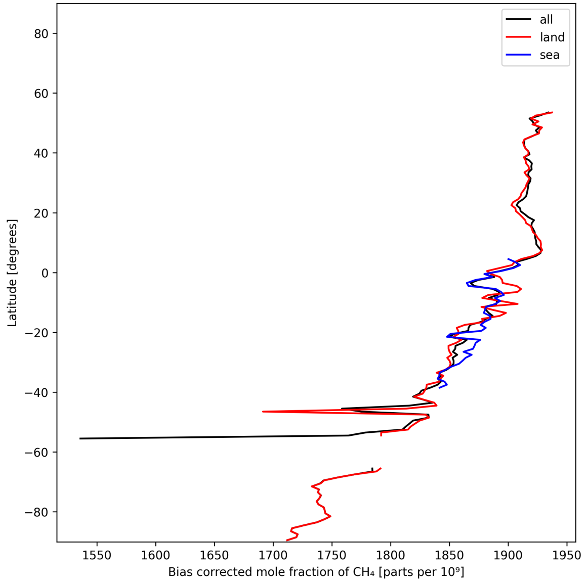
Figure 14: Zonal average of “Bias corrected mole fraction of CH 4 ” for 2025-01-09 to 2025-01-11.
