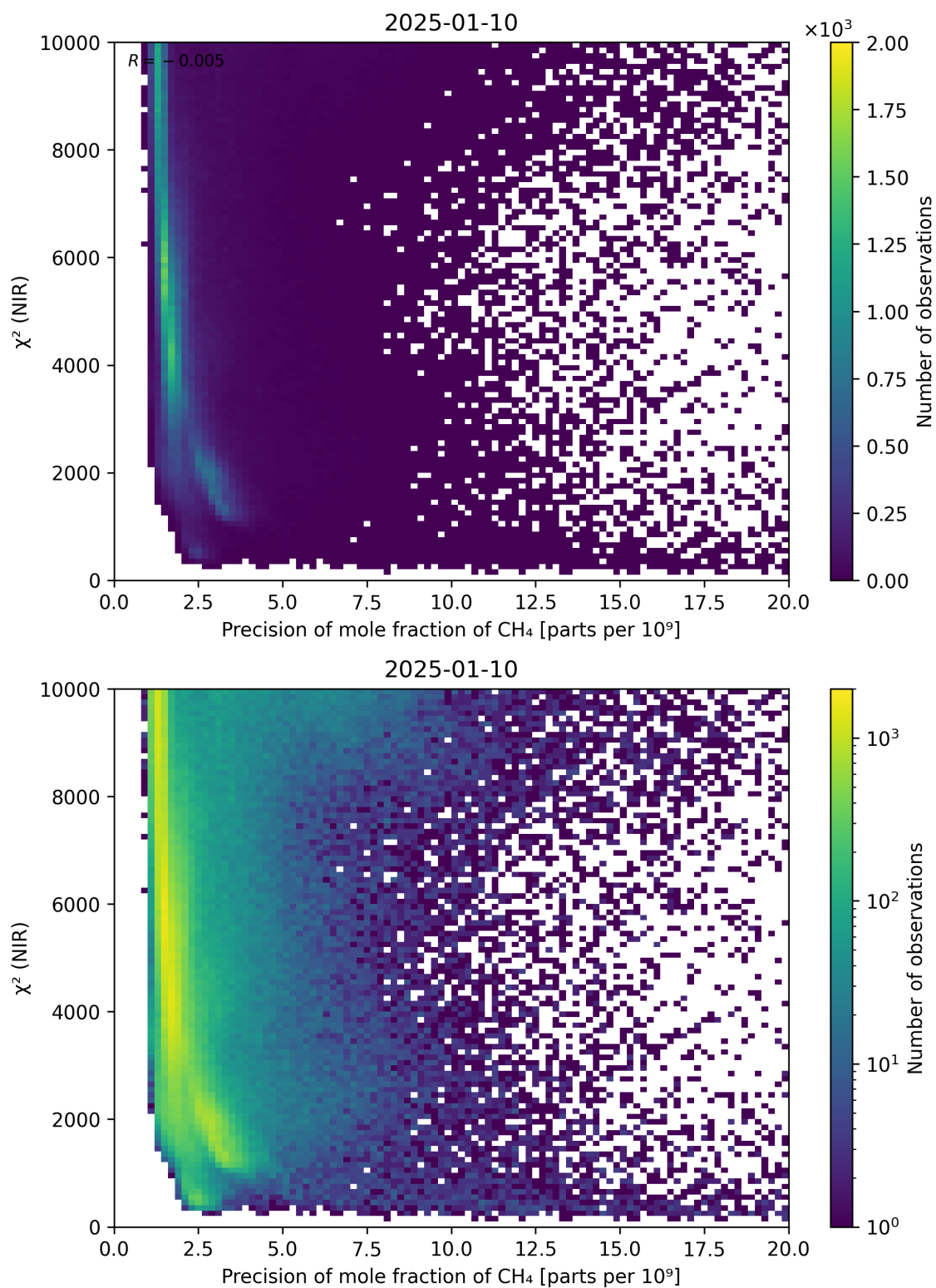
Figure 78: Scatter density plot of “Precision of mole fraction of CH 4 ” against “ \chi^2 (NIR)” for 2025-01-09 to 2025-01-11.
