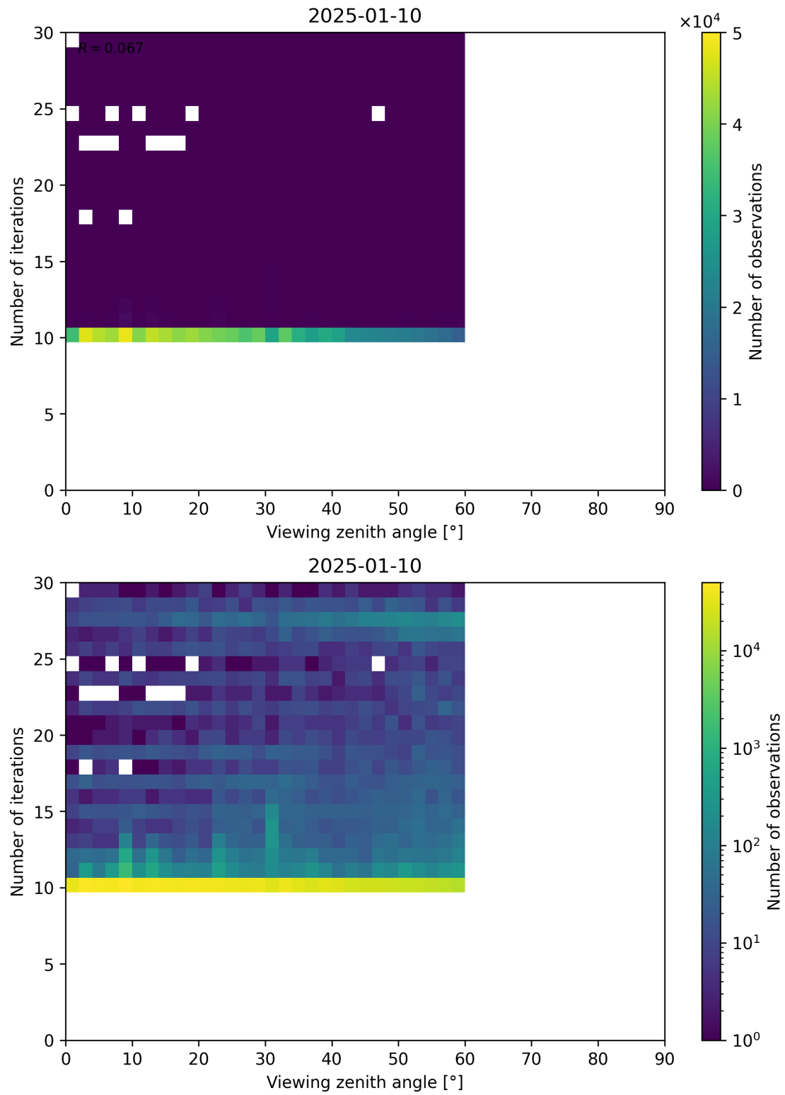
Figure 113: Scatter density plot of “Viewing zenith angle” against “Number of iterations” for 2025-01-09 to 2025-01-11.
