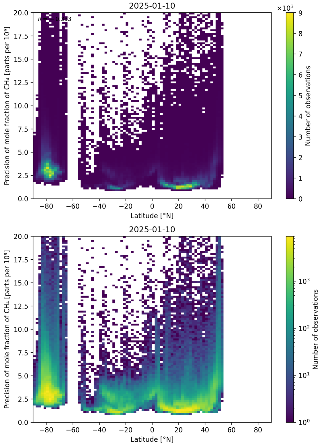
Figure 59: Scatter density plot of “Latitude” against “Precision of mole fraction of CH 4 ” for 2025-01-09 to 2025-01-11.
