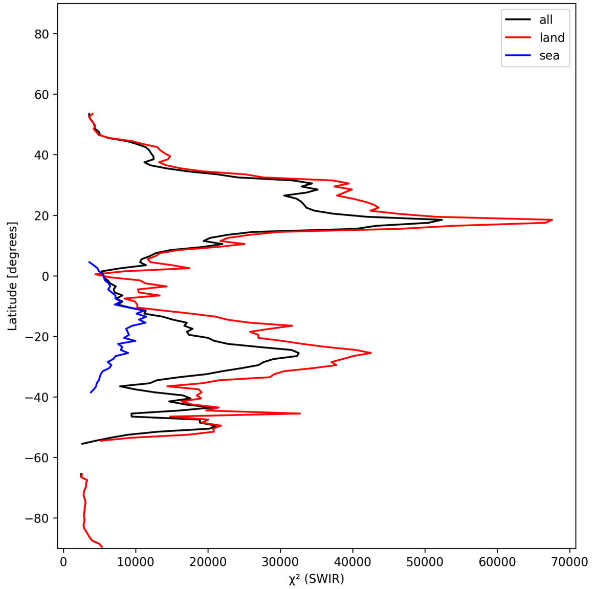
Figure 17: Zonal average of “ \chi^2 (SWIR)” for 2025-01-09 to 2025-01-11.
