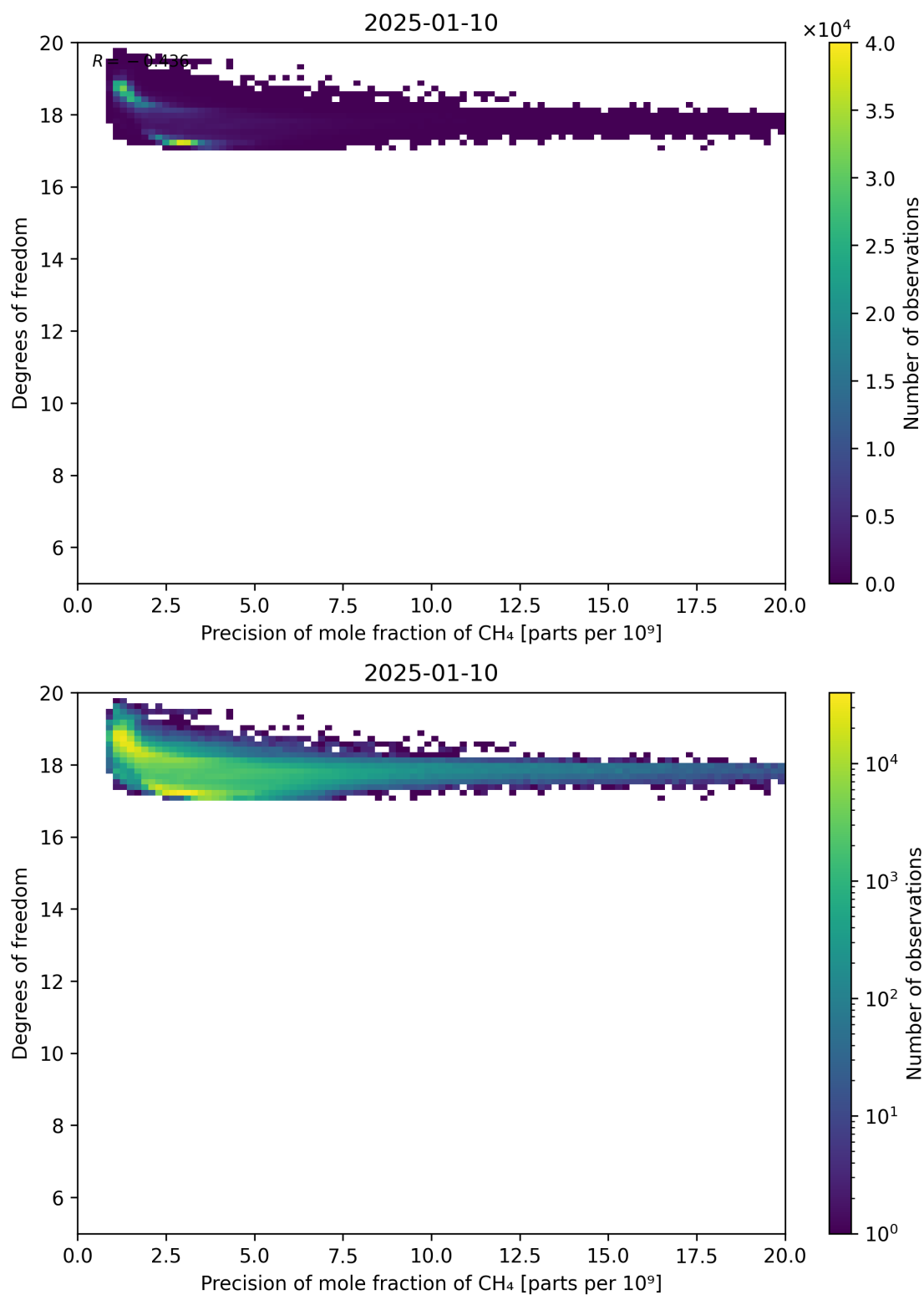
Figure 80: Scatter density plot of “Precision of mole fraction of CH 4 ” against “Degrees of freedom” for 2025-01-09 to 2025-01-11.
