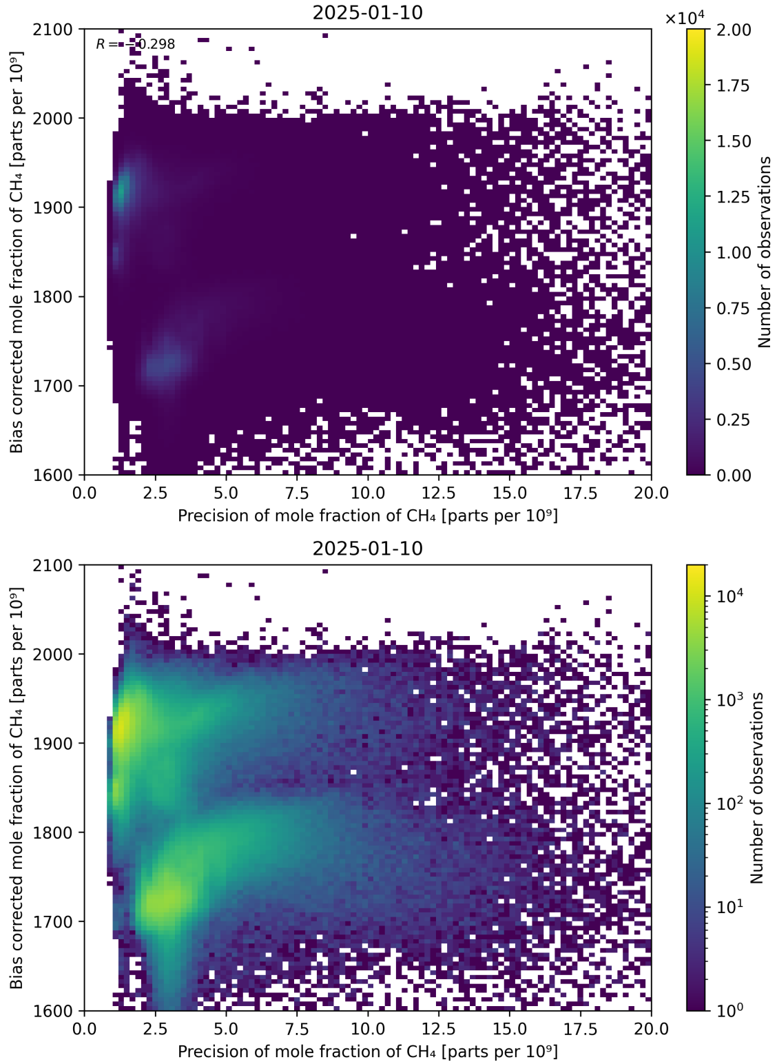
Figure 82: Scatter density plot of “Precision of mole fraction of \text{CH}_4 ” against “Bias corrected mole fraction of \text{CH}_4 ” for 2025-01-09 to 2025-01-11.
