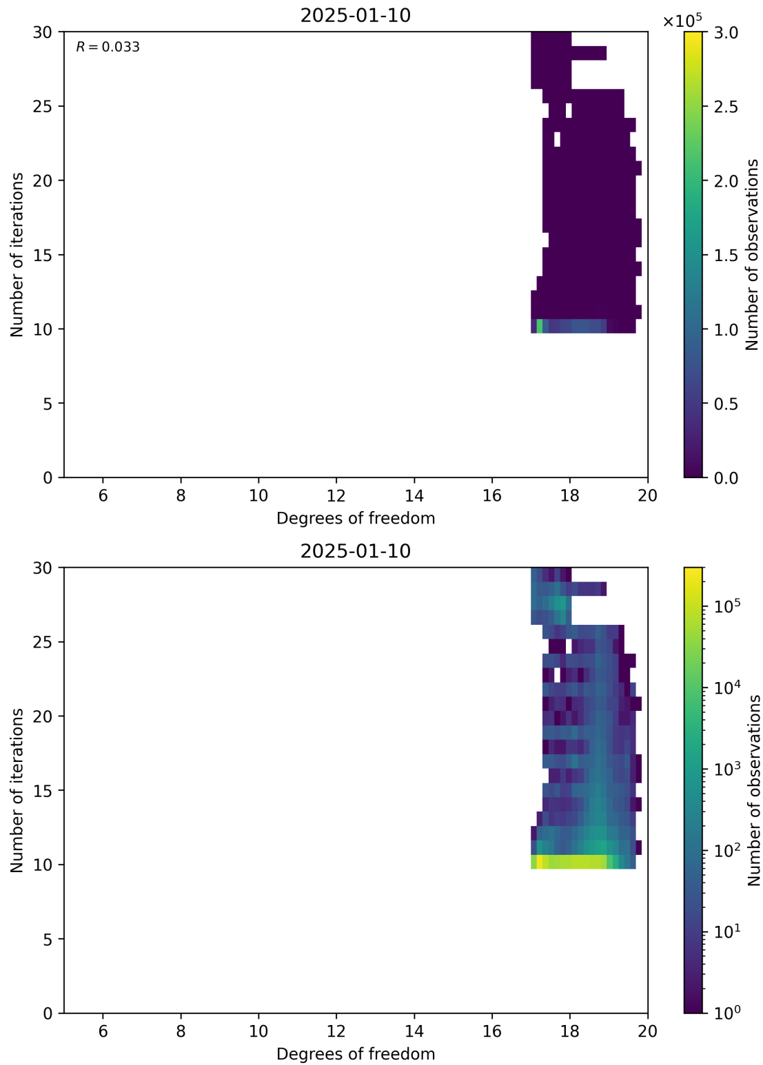
Figure 52: Scatter density plot of “Degrees of freedom” against “Number of iterations” for 2025-01-09 to 2025-01-11.
