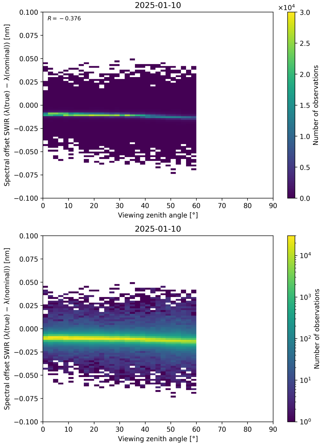
Figure 116: Scatter density plot of “Viewing zenith angle” against “Spectral offset SWIR ( \lambda_{\text{true}} - \lambda_{\text{nominal}} )” for 2025-01-09 to 2025-01-11.
