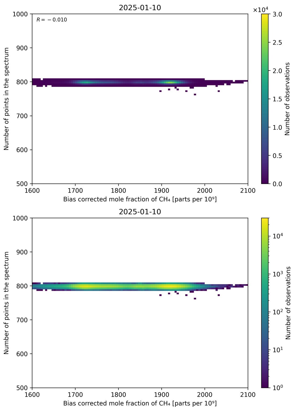
Figure 68: Scatter density plot of “Bias corrected mole fraction of CH 4 ” against “Number of points in the spectrum” for 2025-01-09 to 2025-01-11.
