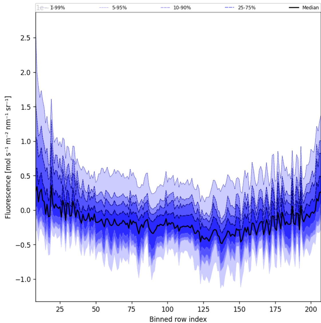
Figure 43: Along track statistics of "Fluorescence" for 2025-01-09 to 2025-01-11
