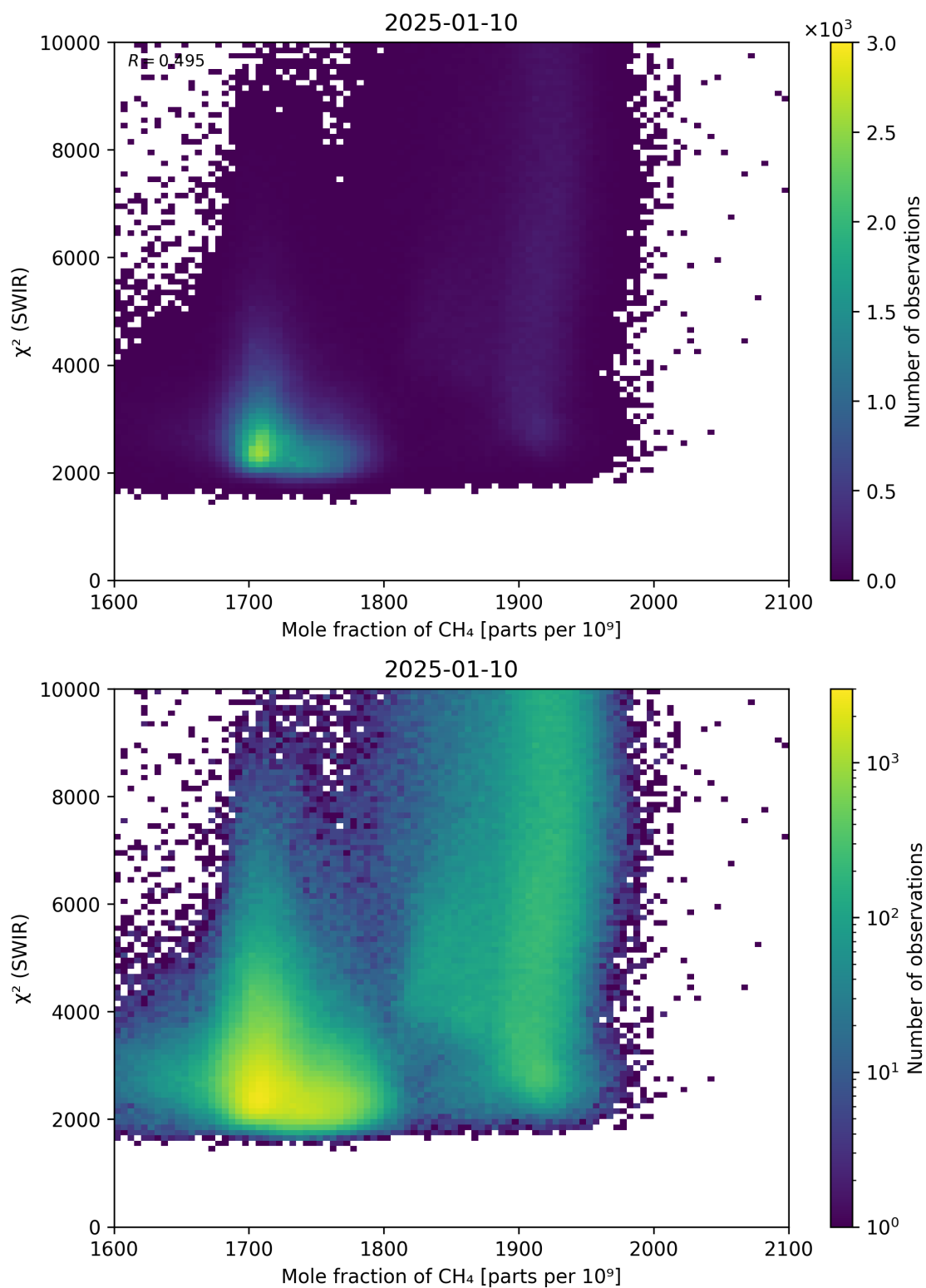
Figure 71: Scatter density plot of “Mole fraction of \text{CH}_4 ” against “ \chi^2 (SWIR)” for 2025-01-09 to 2025-01-11.
