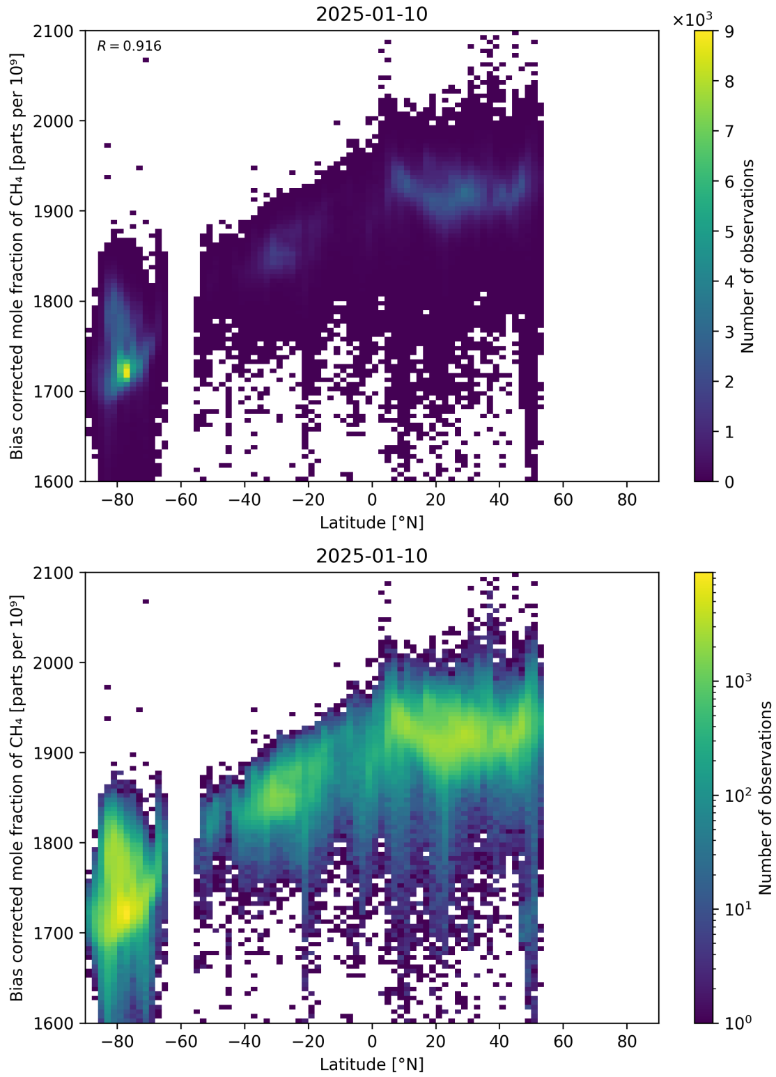
Figure 58: Scatter density plot of “Latitude” against “Bias corrected mole fraction of \text{CH}_4 ” for 2025-01-09 to 2025-01-11.
