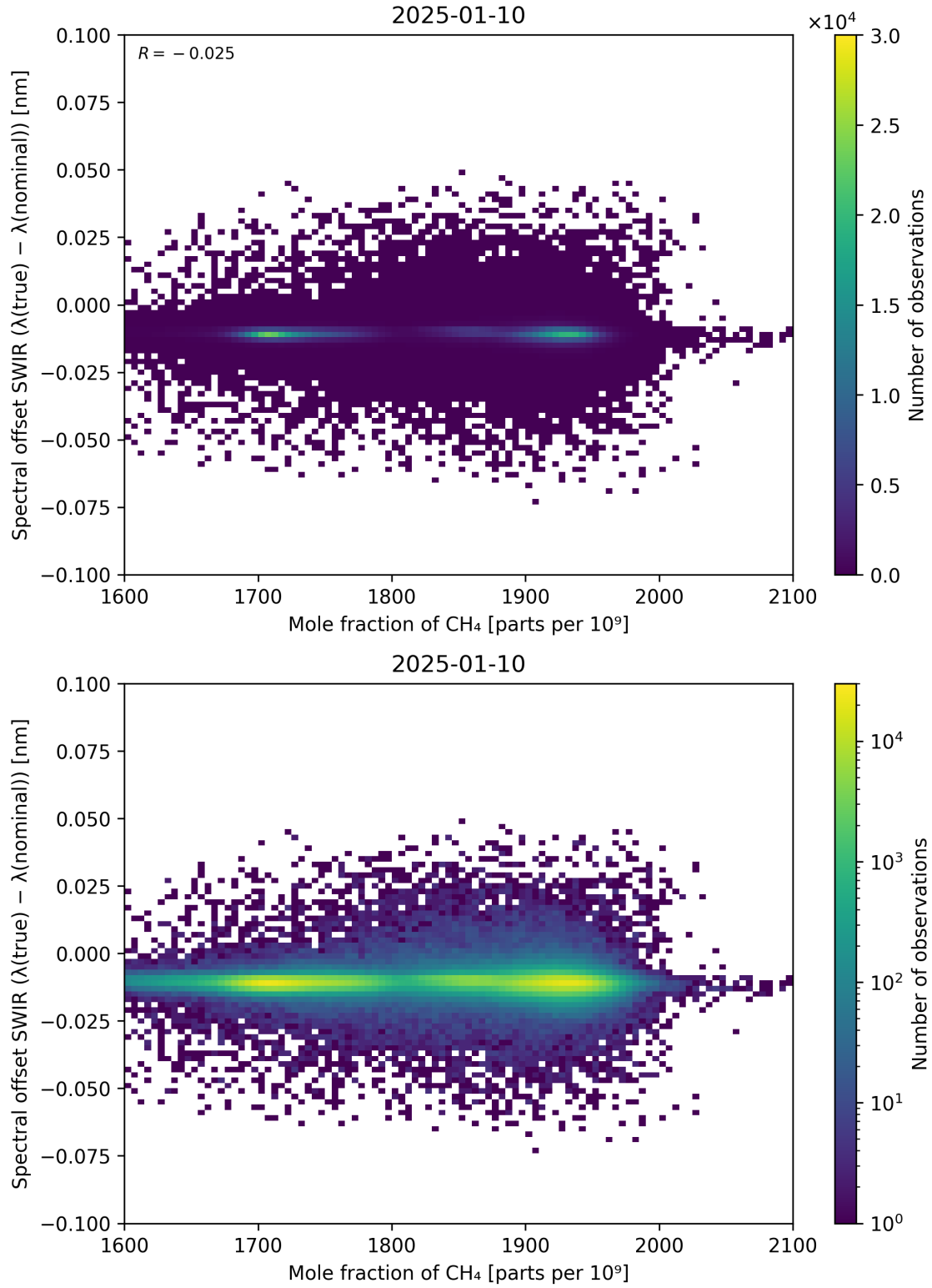
Figure 86: Scatter density plot of “Mole fraction of \text{CH}_4 ” against “Spectral offset SWIR ( \lambda_{\text{true}} - \lambda_{\text{nominal}} )” for 2025-01-09 to 2025-01-11.
