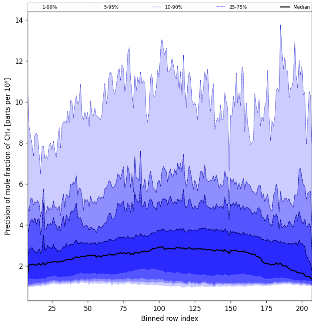
Figure 35: Along track statistics of “Precision of mole fraction of CH 4 ” for 2025-01-09 to 2025-01-11
