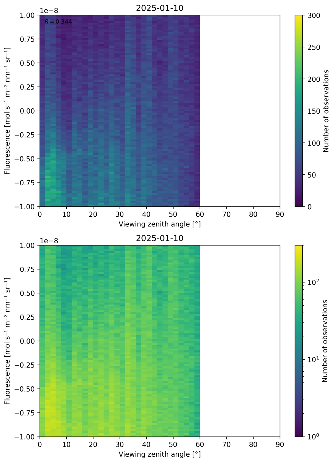
Figure 108: Scatter density plot of “Viewing zenith angle” against “Fluorescence” for 2025-01-09 to 2025-01-11.
