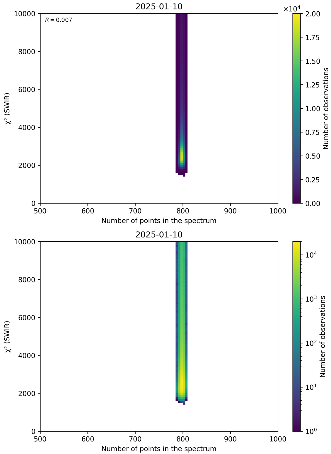
Figure 89: Scatter density plot of “Number of points in the spectrum” against “ \chi^2 (SWIR)” for 2025-01-09 to 2025-01-11.
