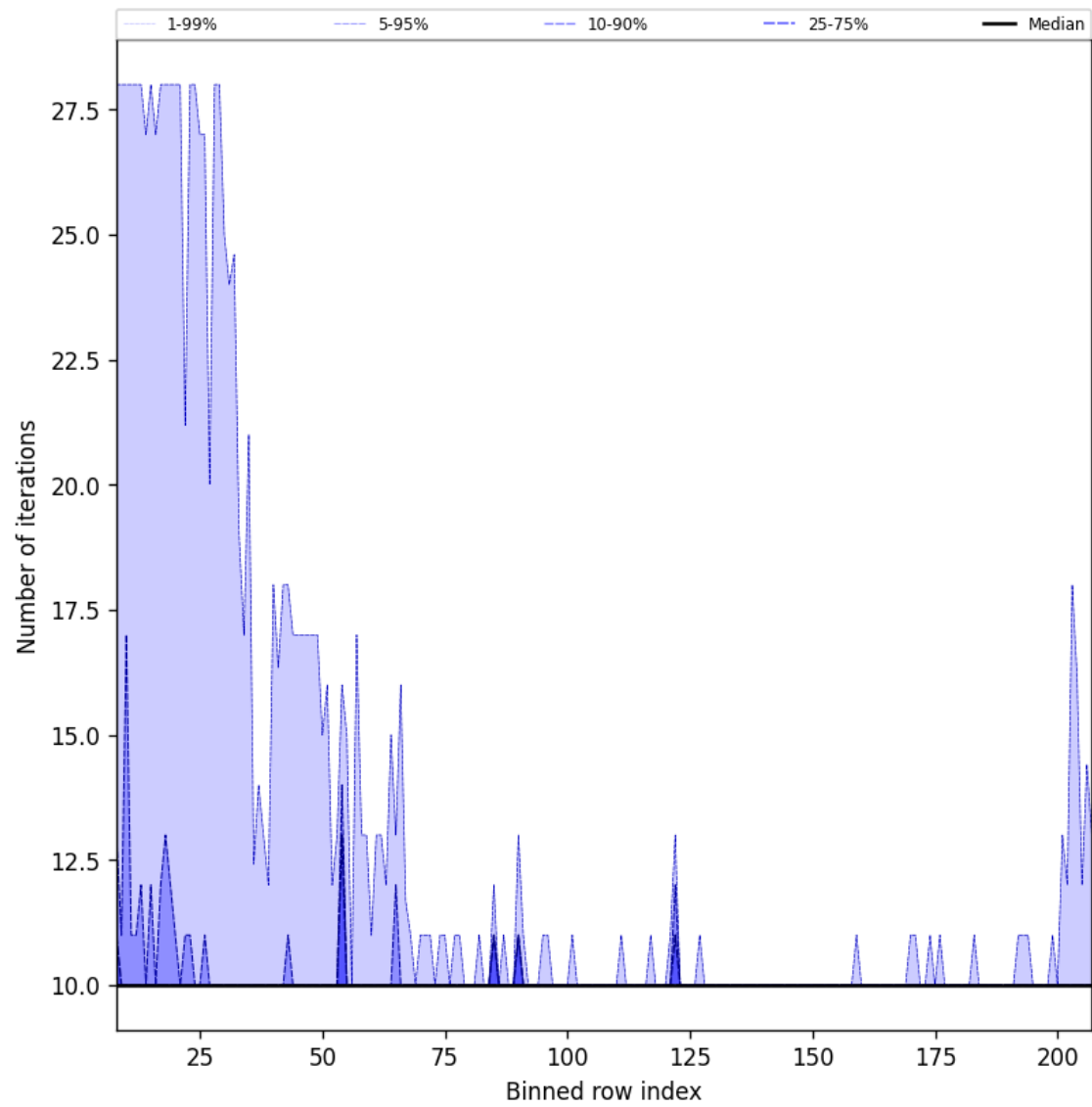
Figure 42: Along track statistics of “Number of iterations” for 2025-01-09 to 2025-01-11
