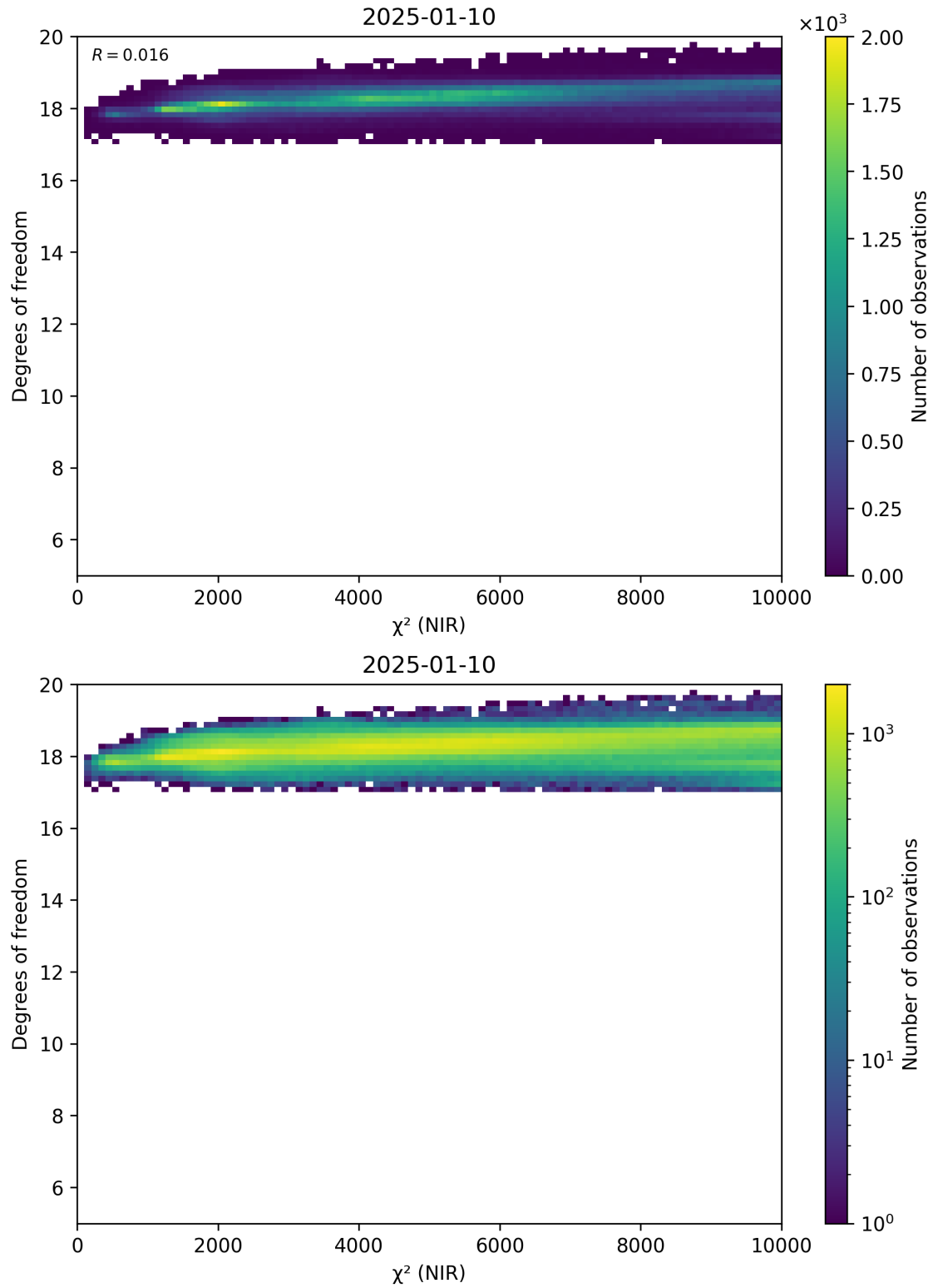
Figure 44: Scatter density plot of “ \chi^2 (NIR)” against “Degrees of freedom” for 2025-01-09 to 2025-01-11.
