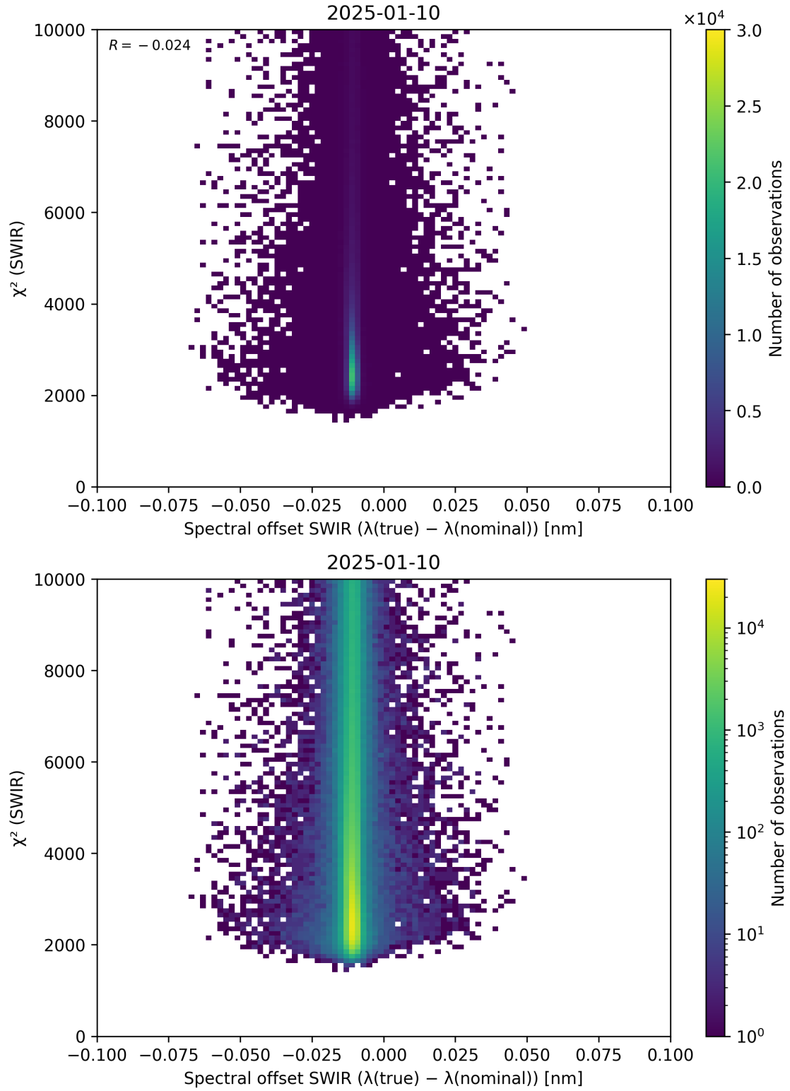
Figure 118: Scatter density plot of “Spectral offset SWIR ( \lambda_{\text{true}} - \lambda_{\text{nominal}} )” against “ \chi^2 (SWIR)” for 2025-01-09 to 2025-01-11.
