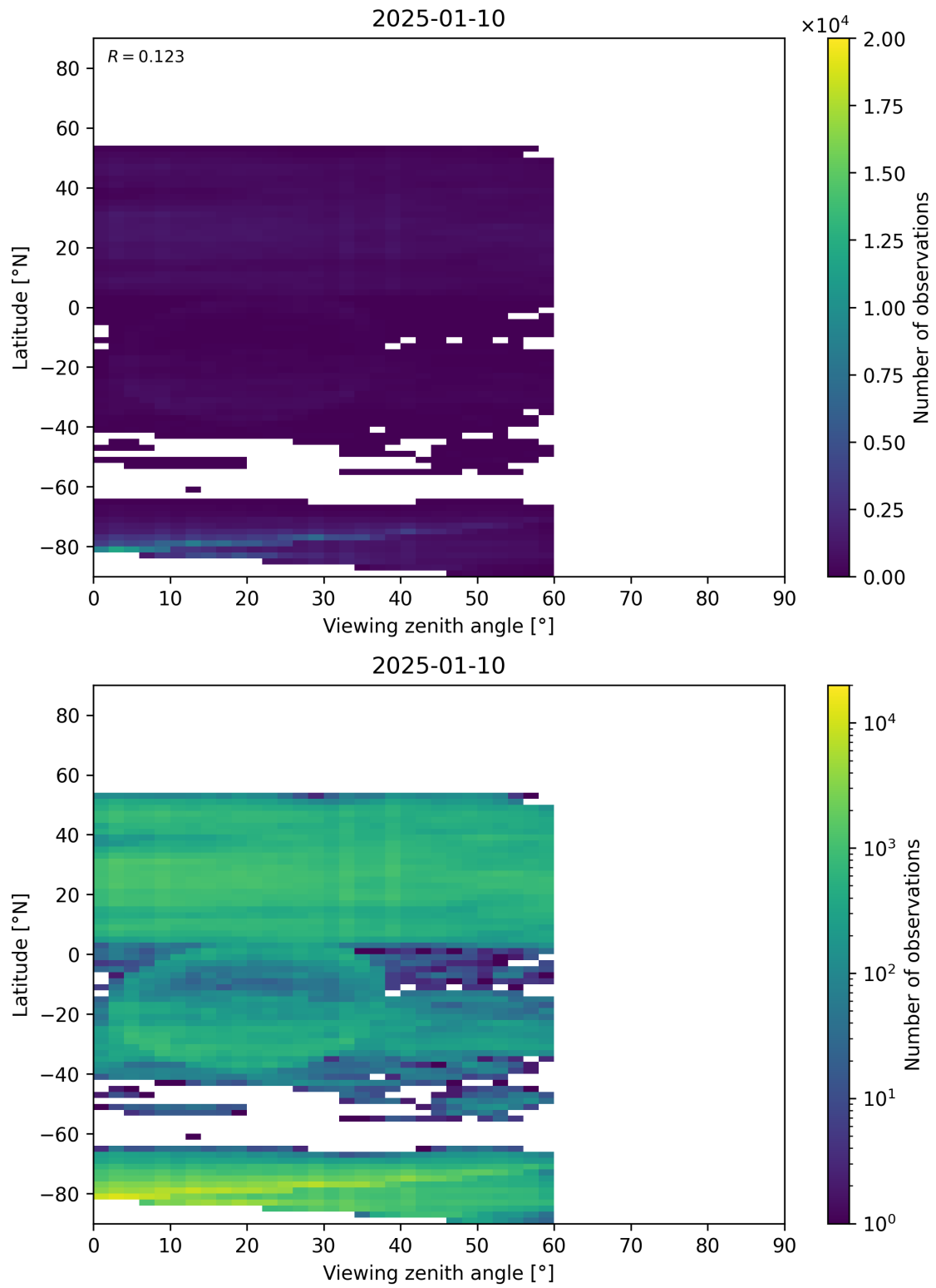
Figure 109: Scatter density plot of “Viewing zenith angle” against “Latitude” for 2025-01-09 to 2025-01-11.
