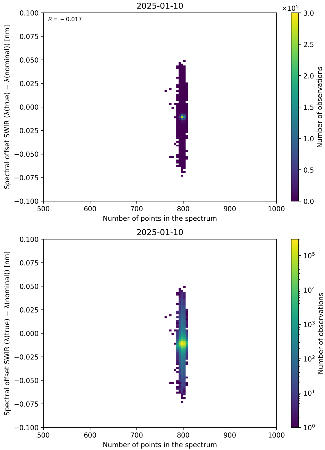
Figure 93: Scatter density plot of “Number of points in the spectrum” against “Spectral offset SWIR ( \lambda_{\text{true}} - \lambda_{\text{nominal}} )” for 2025-01-09 to 2025-01-11.
