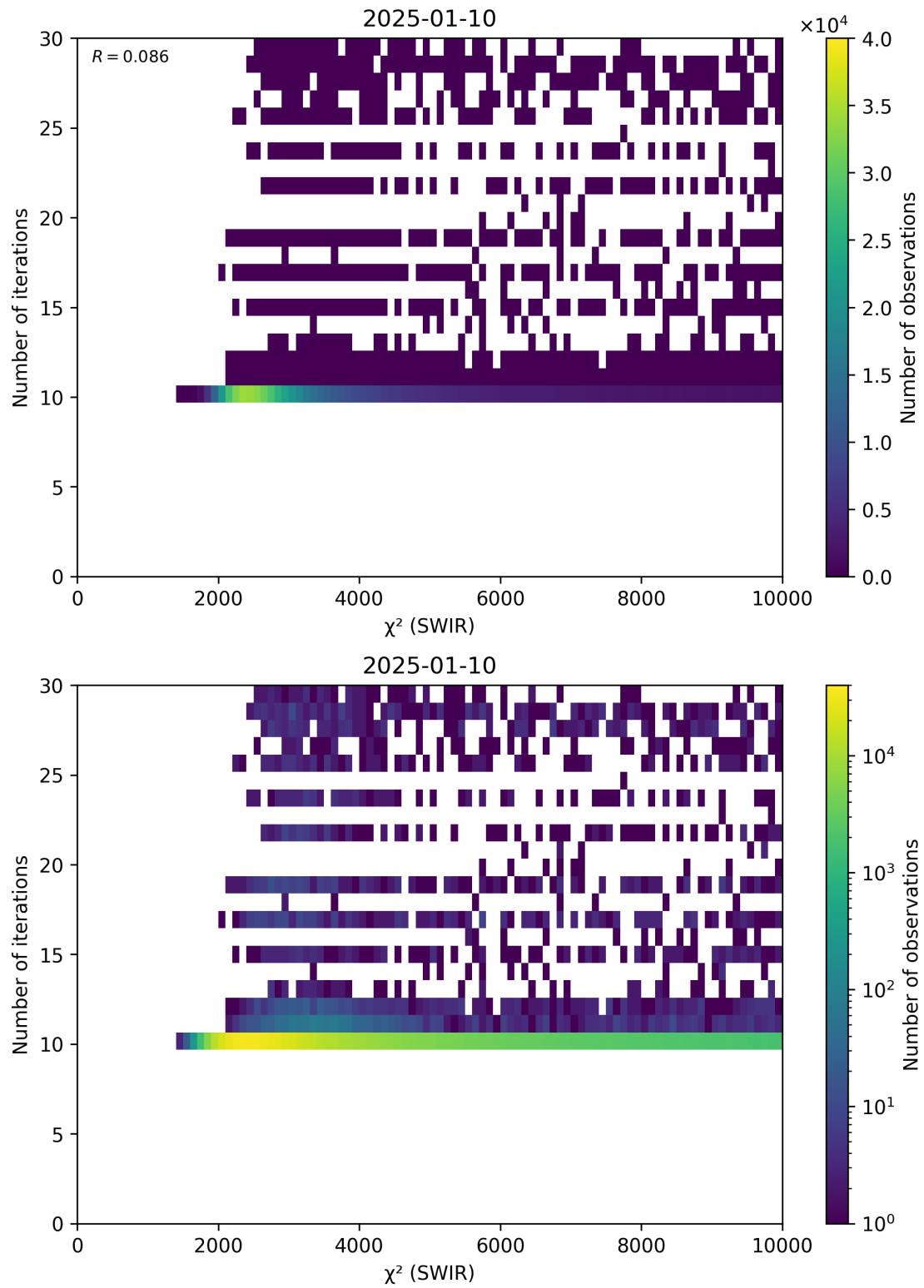
Figure 50: Scatter density plot of “ \chi^2 (SWIR)” against “Number of iterations” for 2025-01-09 to 2025-01-11.
