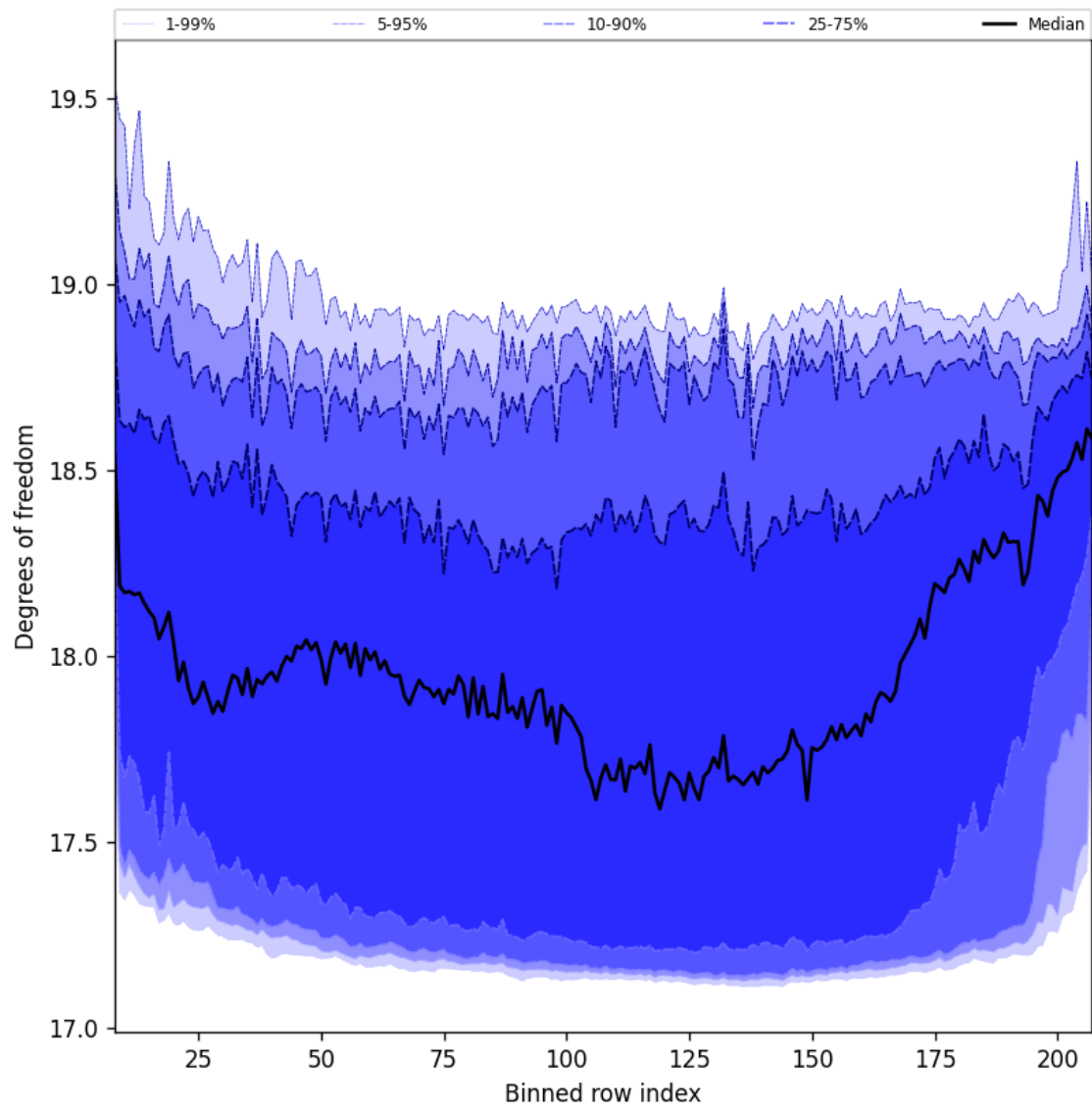
Figure 41: Along track statistics of “Degrees of freedom” for 2025-01-09 to 2025-01-11
