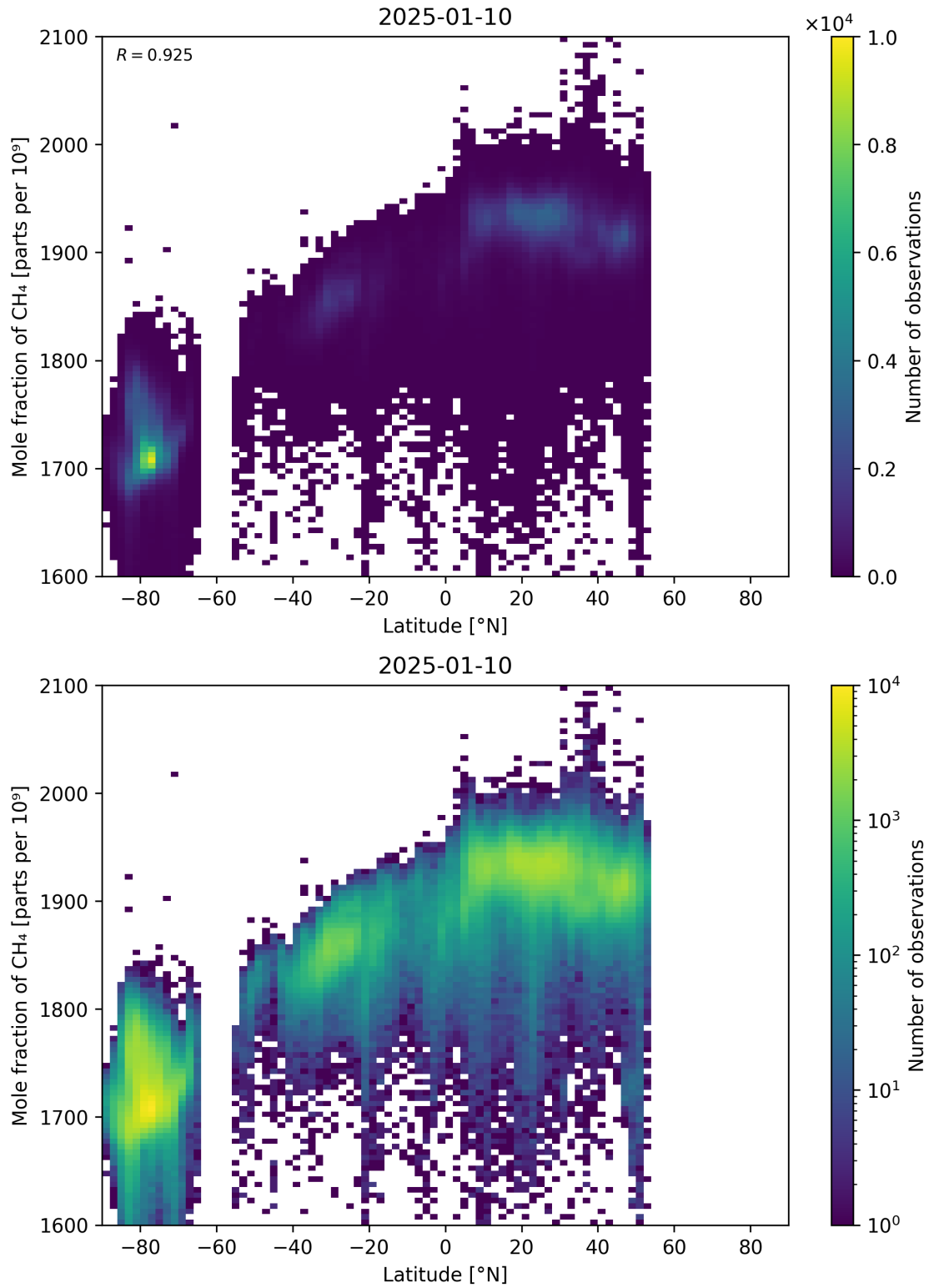
Figure 57: Scatter density plot of “Latitude” against “Mole fraction of \text{CH}_4 ” for 2025-01-09 to 2025-01-11.
