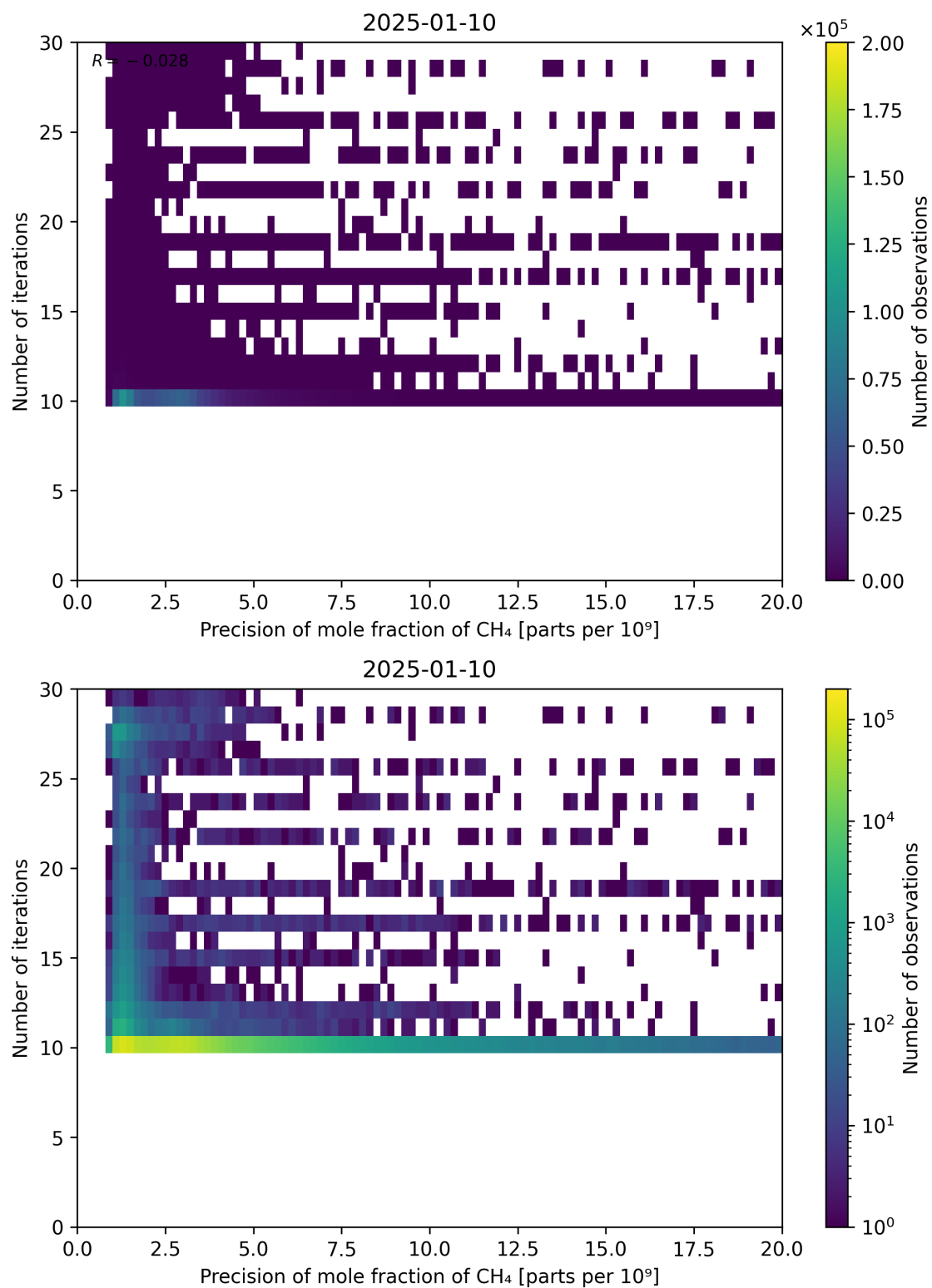
Figure 83: Scatter density plot of “Precision of mole fraction of CH 4 ” against “Number of iterations” for 2025-01-09 to 2025-01-11.
