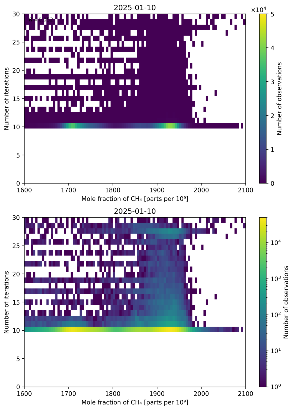
Figure 76: Scatter density plot of “Mole fraction of CH 4 ” against “Number of iterations” for 2025-01-09 to 2025-01-11.
