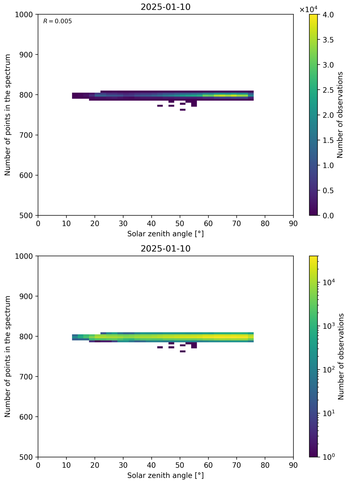
Figure 103: Scatter density plot of “Solar zenith angle” against “Number of points in the spectrum” for 2025-01-09 to 2025-01-11.
