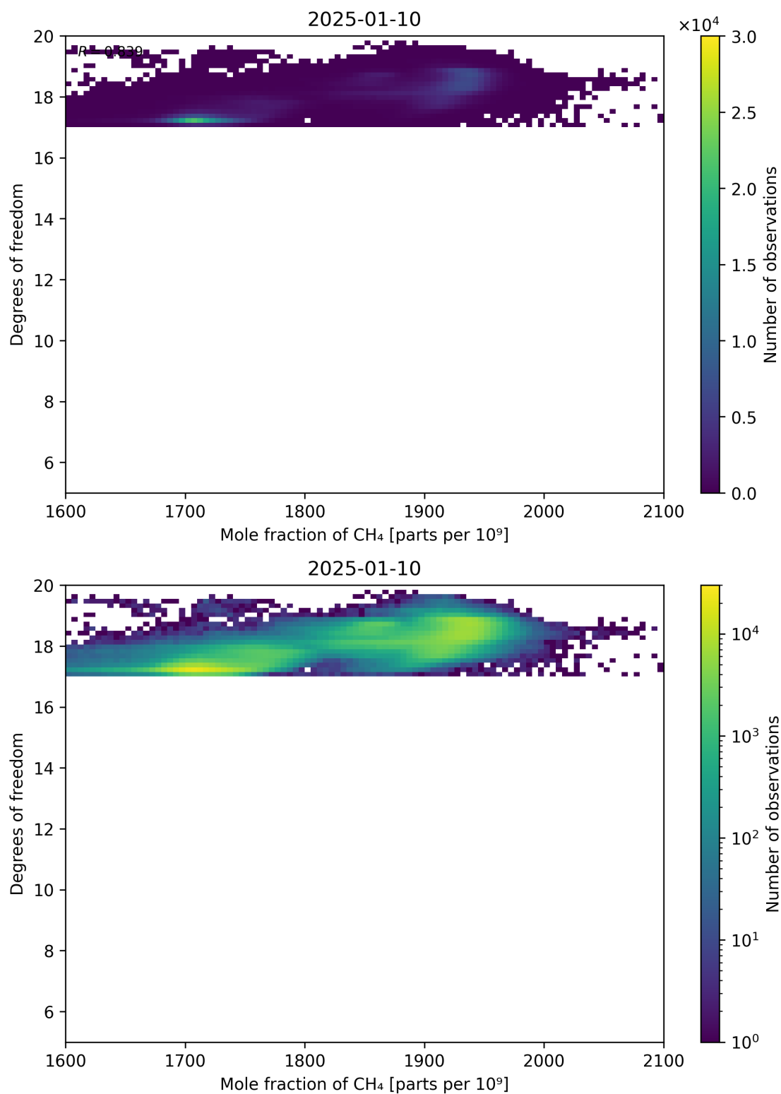
Figure 72: Scatter density plot of “Mole fraction of CH 4 ” against “Degrees of freedom” for 2025-01-09 to 2025-01-11.
