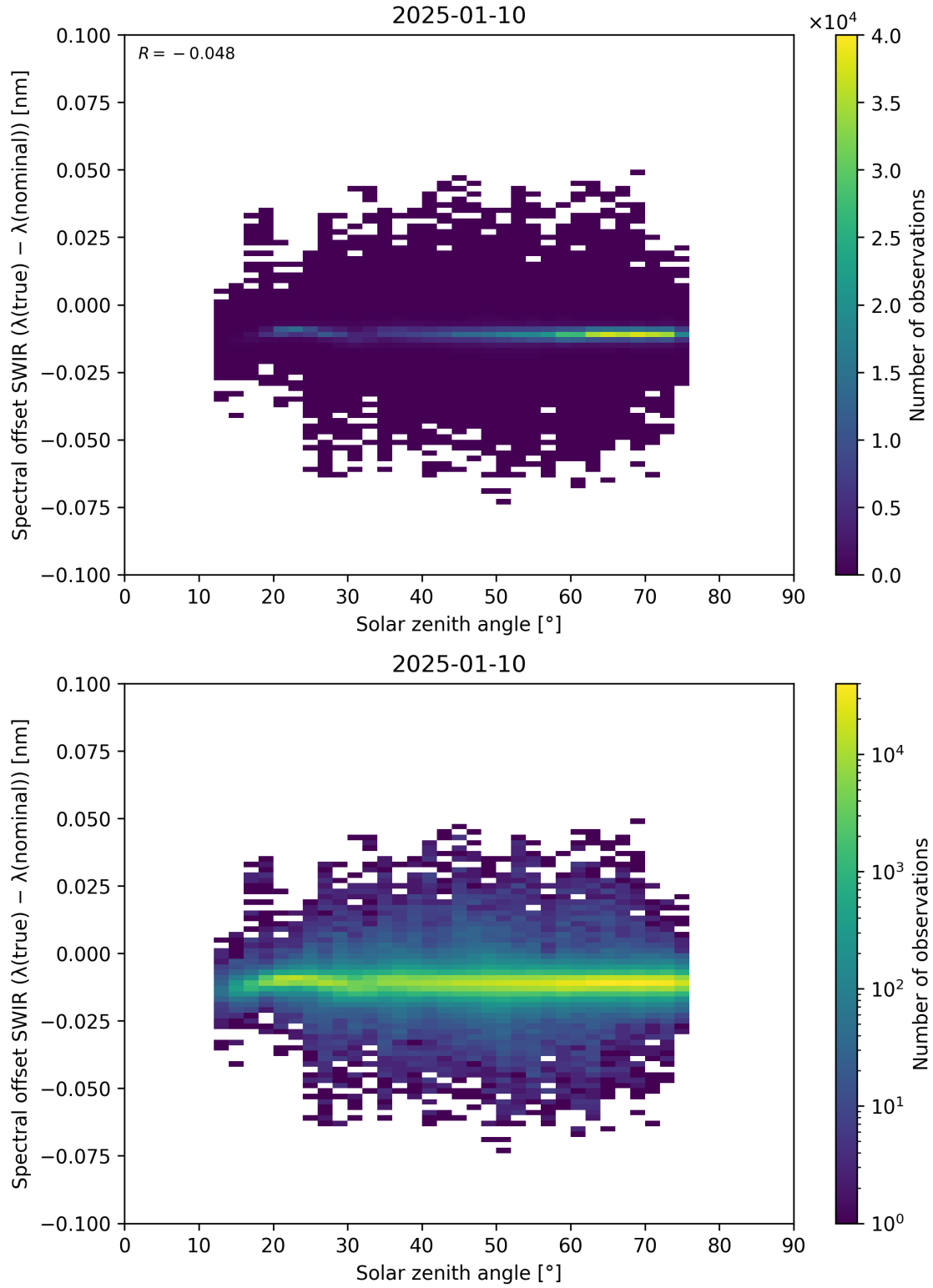
Figure 104: Scatter density plot of “Solar zenith angle” against “Spectral offset SWIR ( \lambda_{\text{true}} - \lambda_{\text{nominal}} )” for 2025-01-09 to 2025-01-11.
