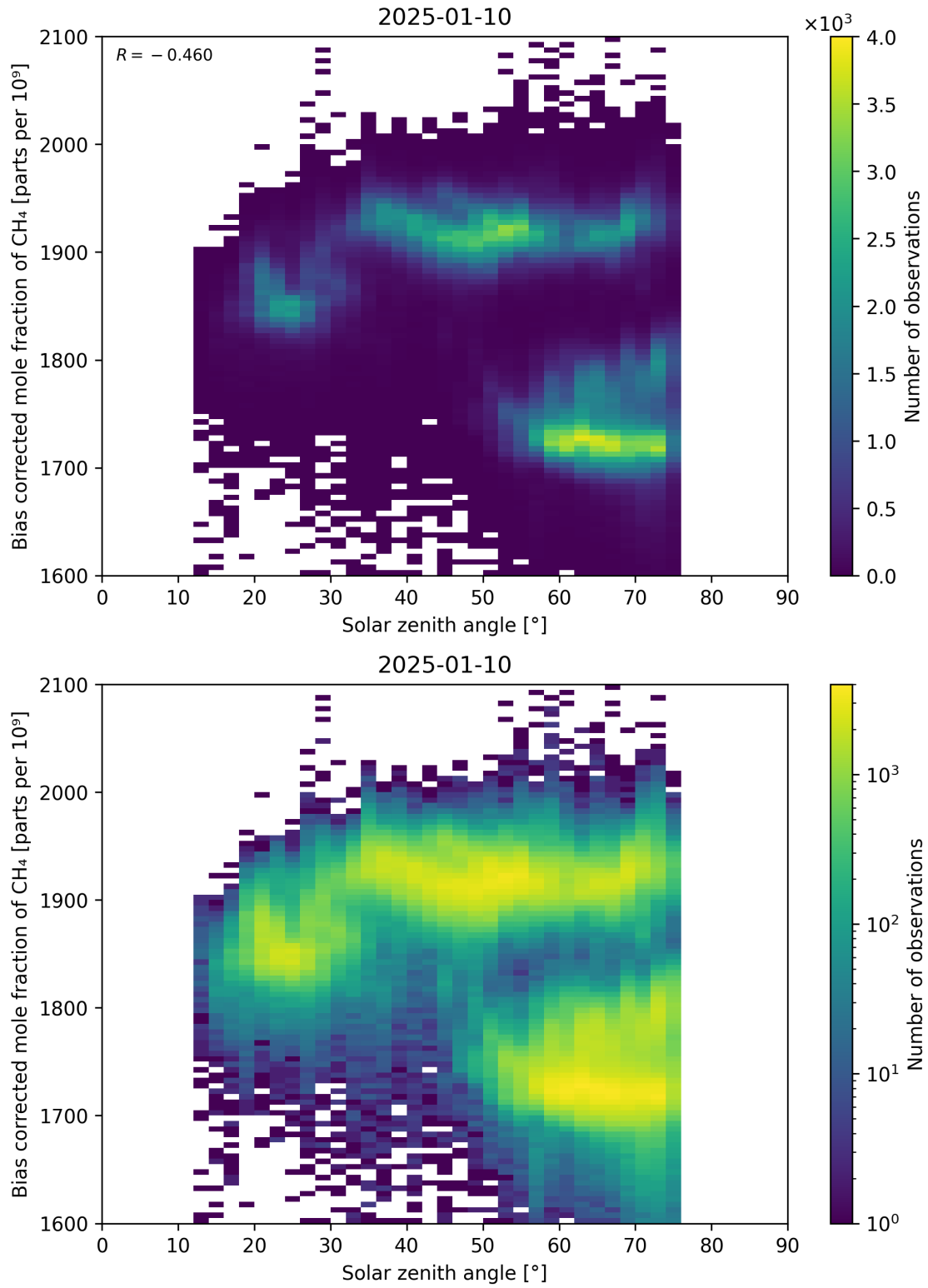
Figure 100: Scatter density plot of “Solar zenith angle” against “Bias corrected mole fraction of \text{CH}_4 ” for 2025-01-09 to 2025-01-11.
