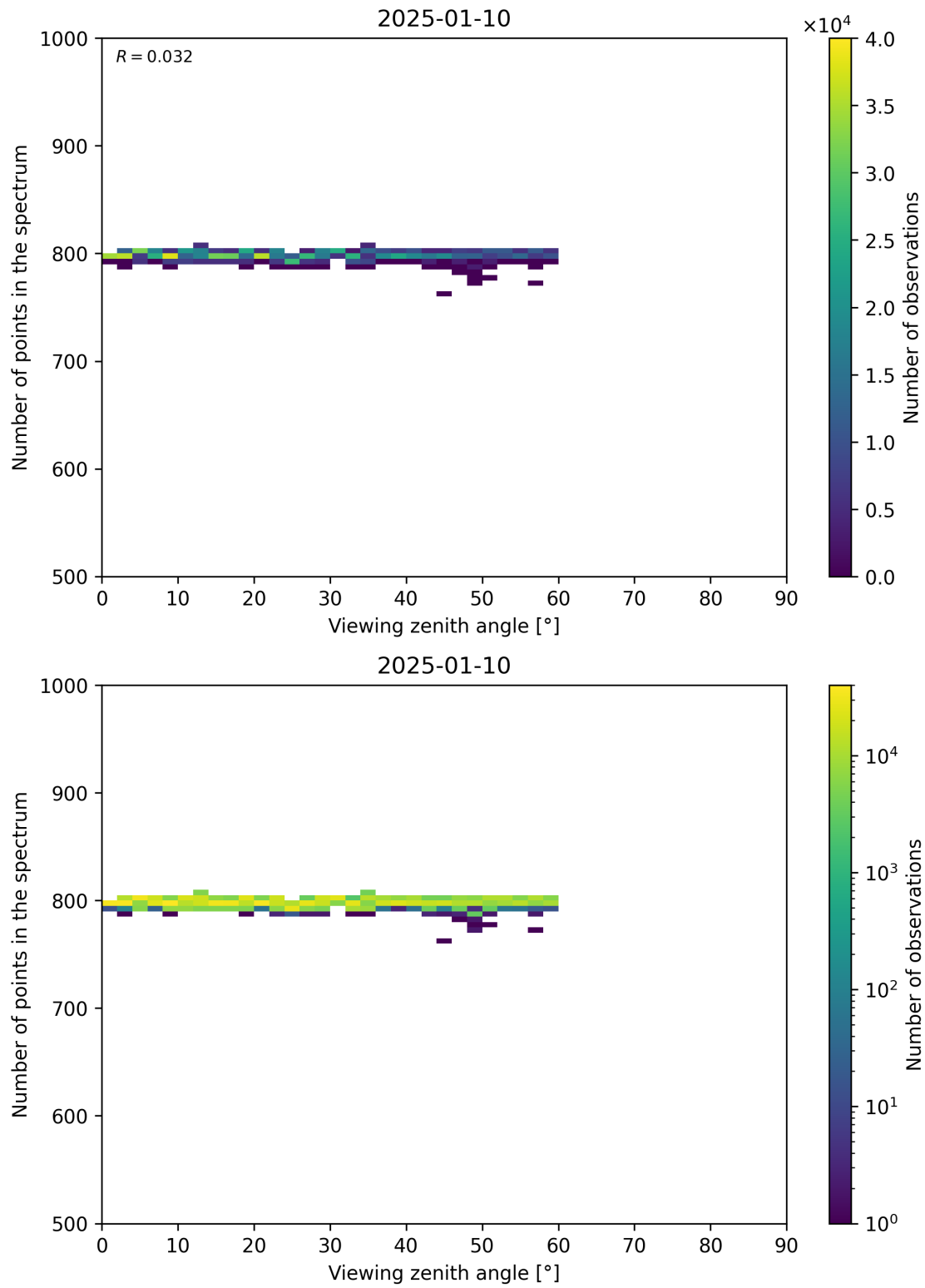
Figure 114: Scatter density plot of “Viewing zenith angle” against “Number of points in the spectrum” for 2025-01-09 to 2025-01-11.
