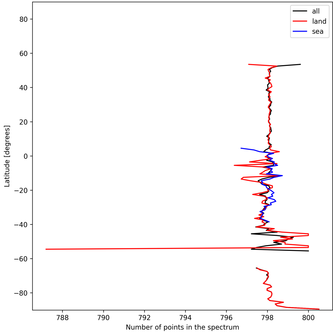
Figure 15: Zonal average of “Number of points in the spectrum” for 2025-01-09 to 2025-01-11.
