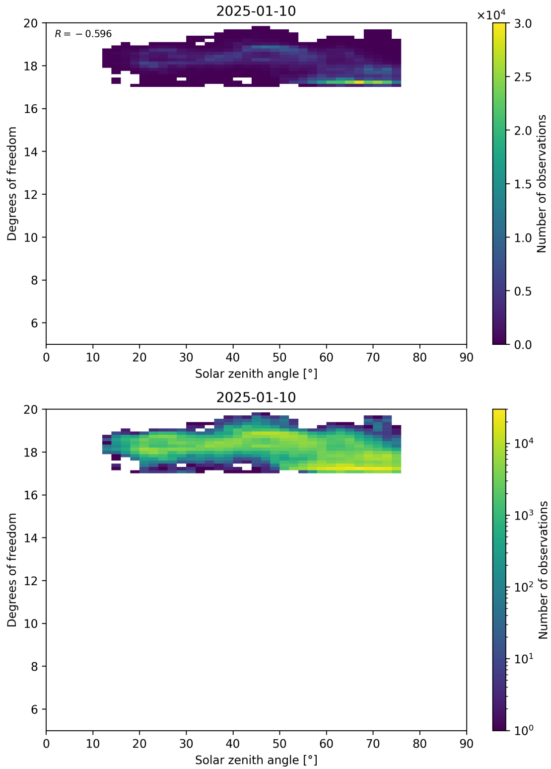
Figure 96: Scatter density plot of “Solar zenith angle” against “Degrees of freedom” for 2025-01-09 to 2025-01-11.
