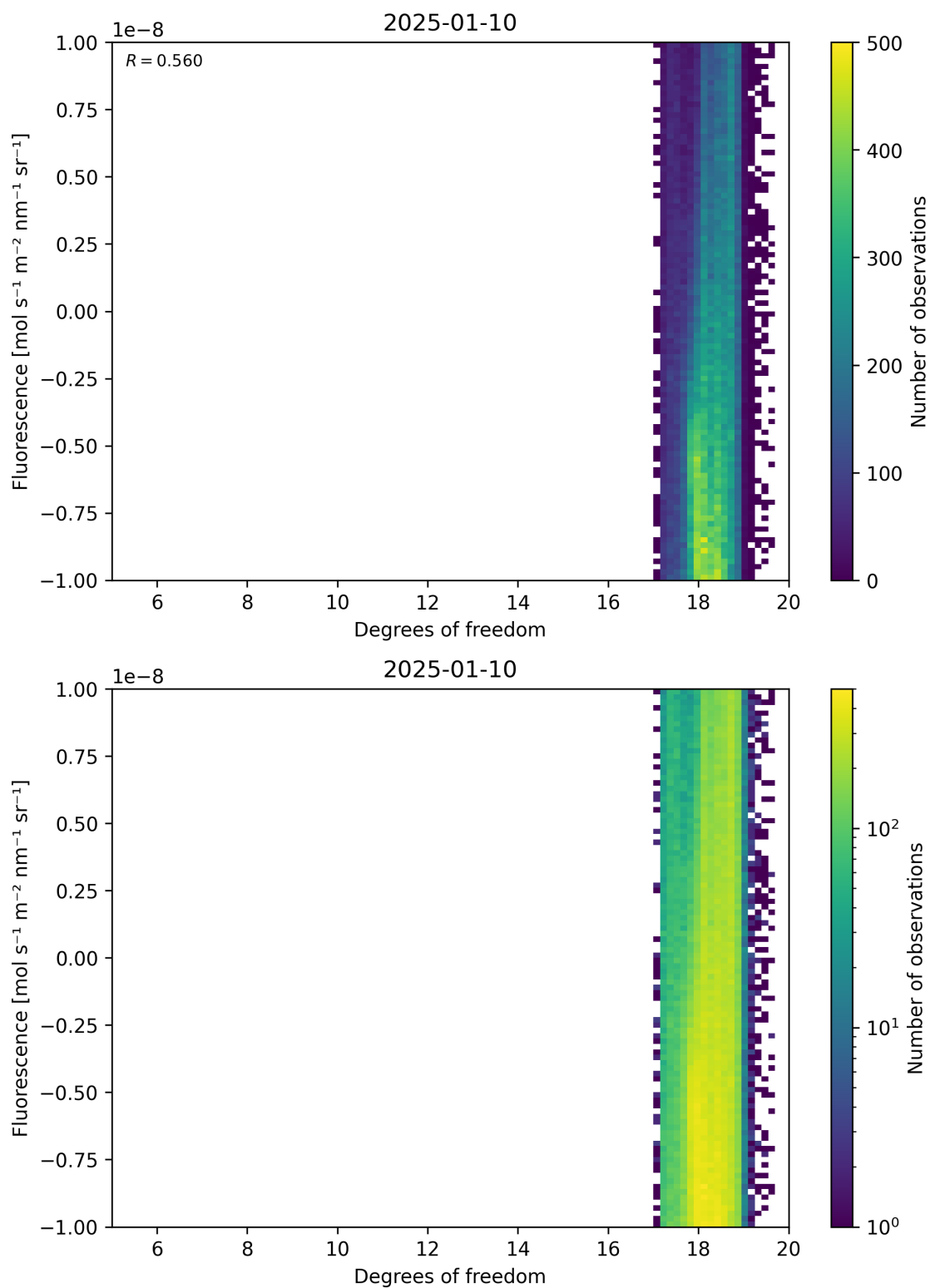
Figure 51: Scatter density plot of “Degrees of freedom” against “Fluorescence” for 2025-01-09 to 2025-01-11.
