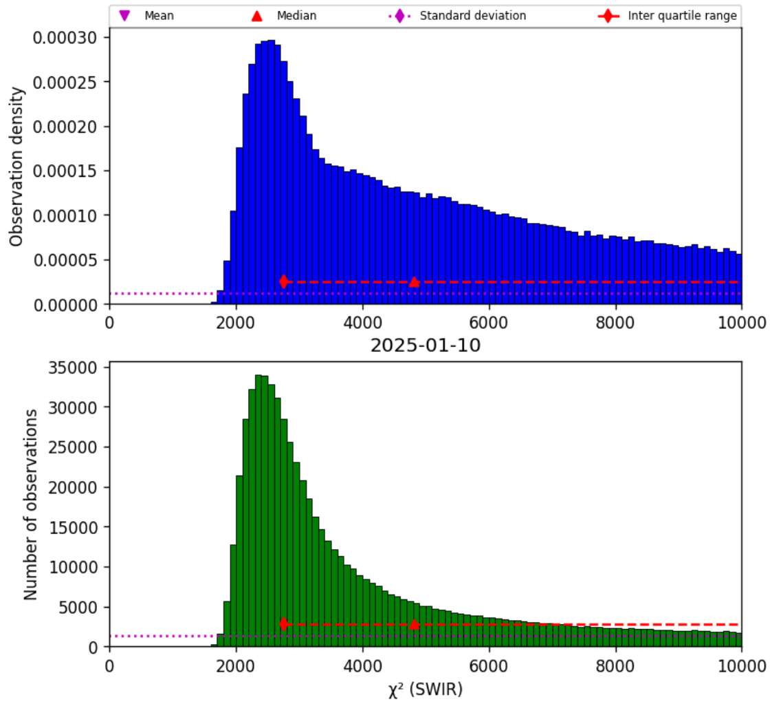
Figure 28: Histogram of “ \chi^2 (SWIR)” for 2025-01-09 to 2025-01-11
