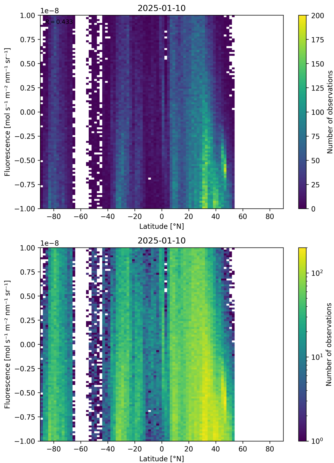
Figure 56: Scatter density plot of “Latitude” against “Fluorescence” for 2025-01-09 to 2025-01-11.
