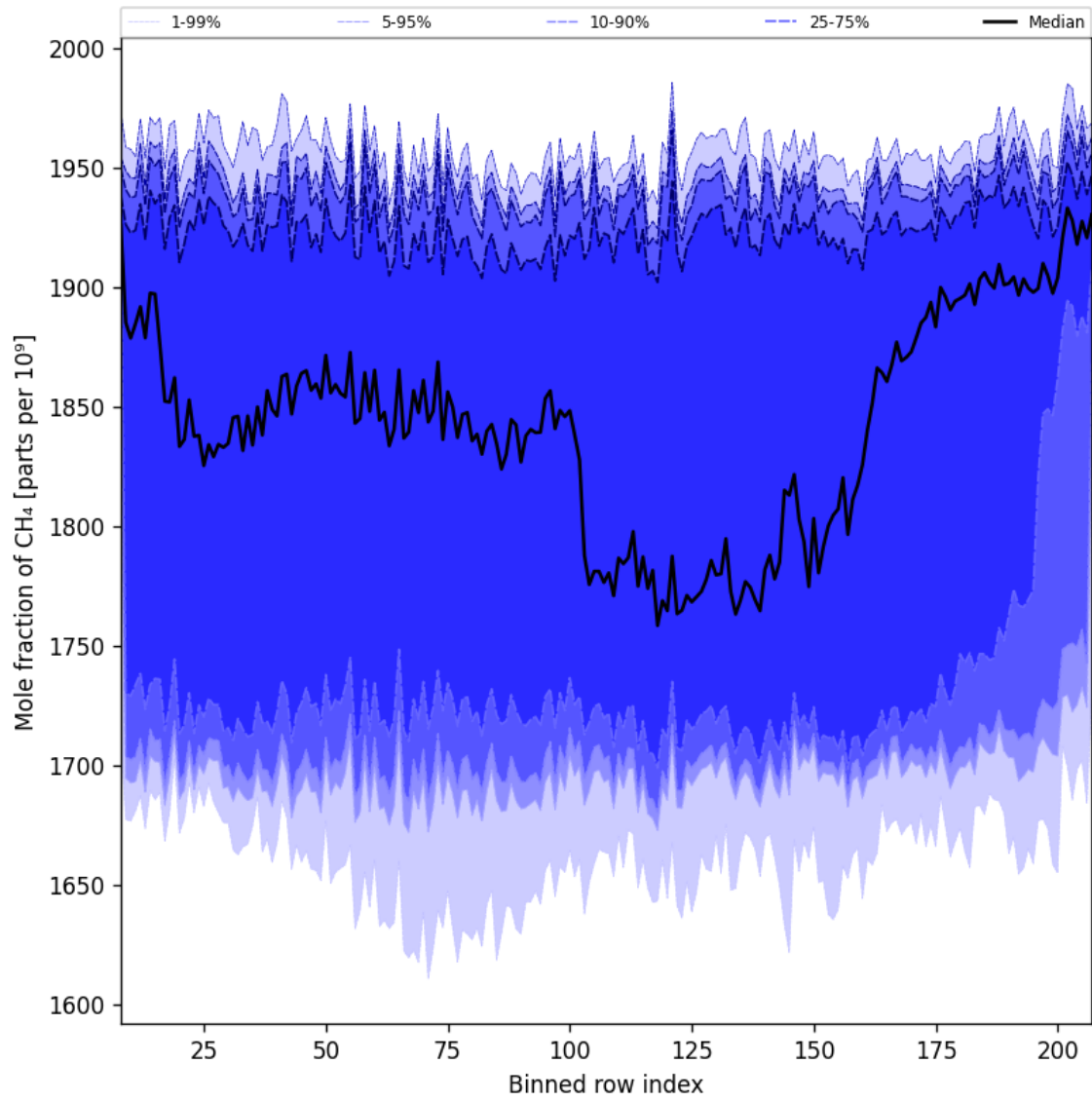
Figure 34: Along track statistics of “Mole fraction of CH 4 ” for 2025-01-09 to 2025-01-11
