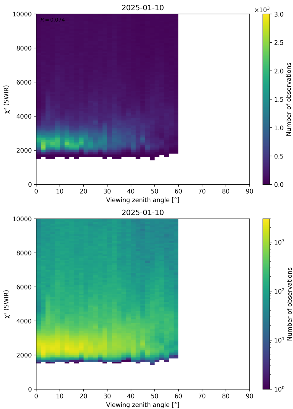
Figure 106: Scatter density plot of “Viewing zenith angle” against “ \chi^2 (SWIR)” for 2025-01-09 to 2025-01-11.
