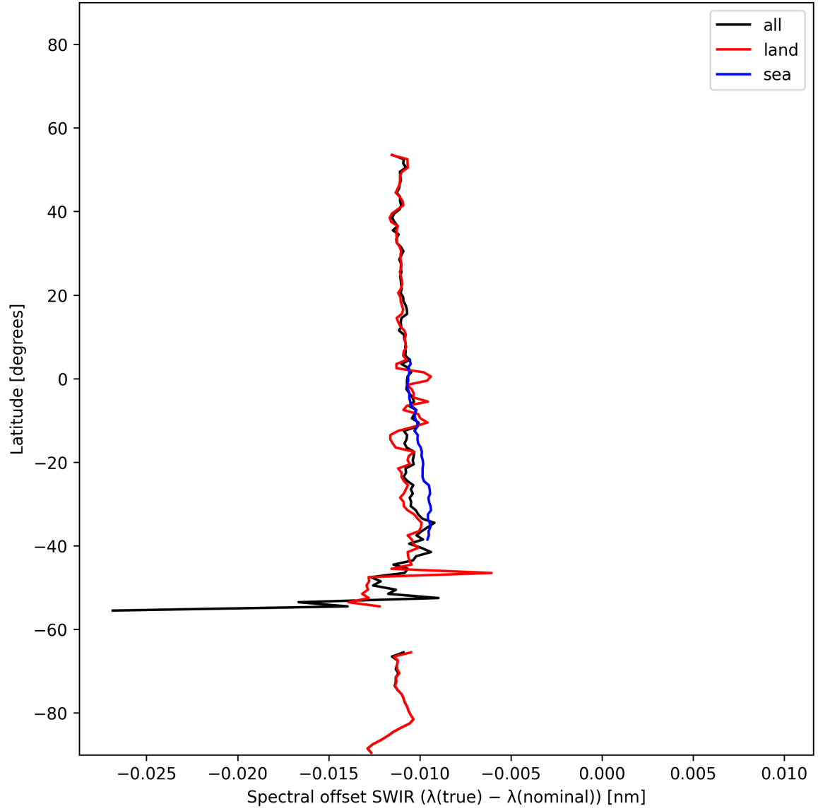
Figure 16: Zonal average of “Spectral offset SWIR ( \lambda_{\text{true}} - \lambda_{\text{nominal}} )” for 2025-01-09 to 2025-01-11.
