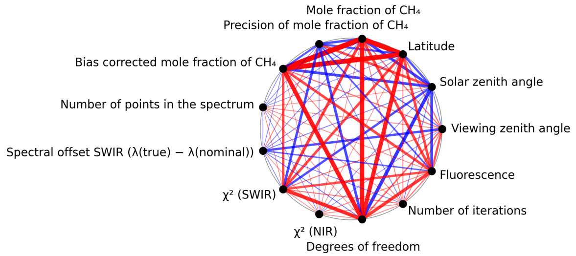
Figure 1: Map of correlation graph for 2025-01-09 to 2025-01-11.
