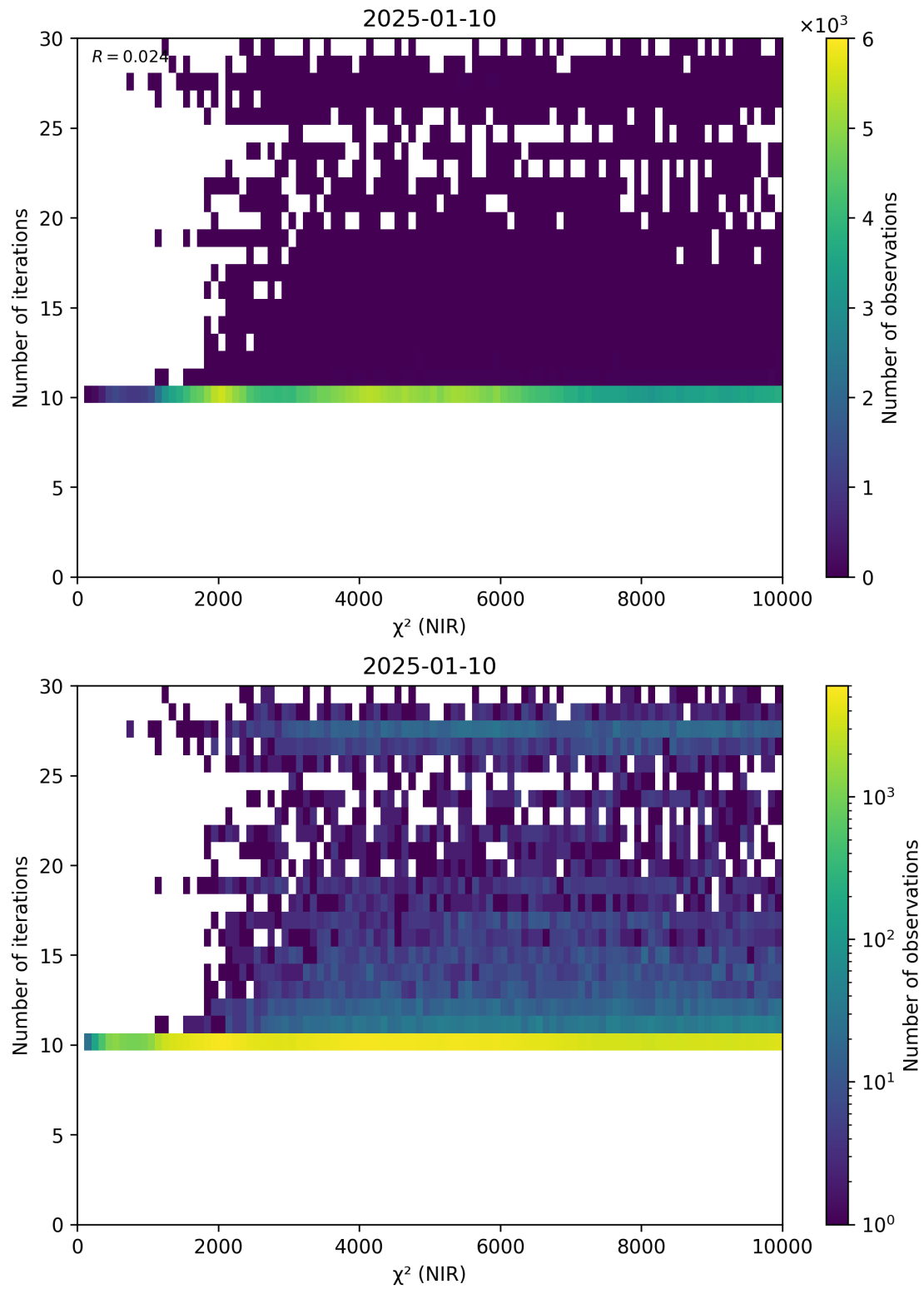
Figure 46: Scatter density plot of “ \chi^2 (NIR)” against “Number of iterations” for 2025-01-09 to 2025-01-11.
