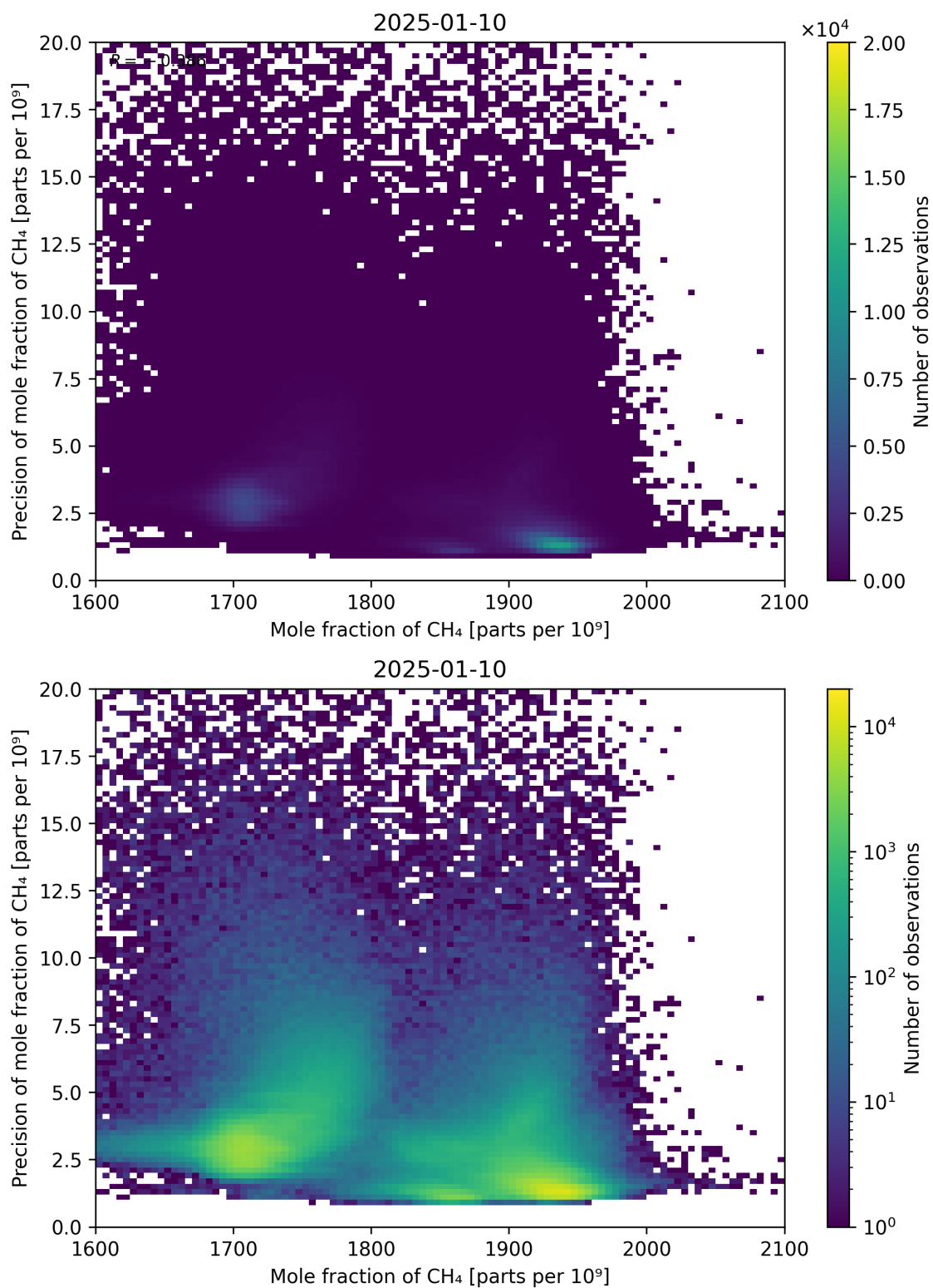
Figure 75: Scatter density plot of “Mole fraction of CH 4 ” against “Precision of mole fraction of CH 4 ” for 2025-01-09 to 2025-01-11.
