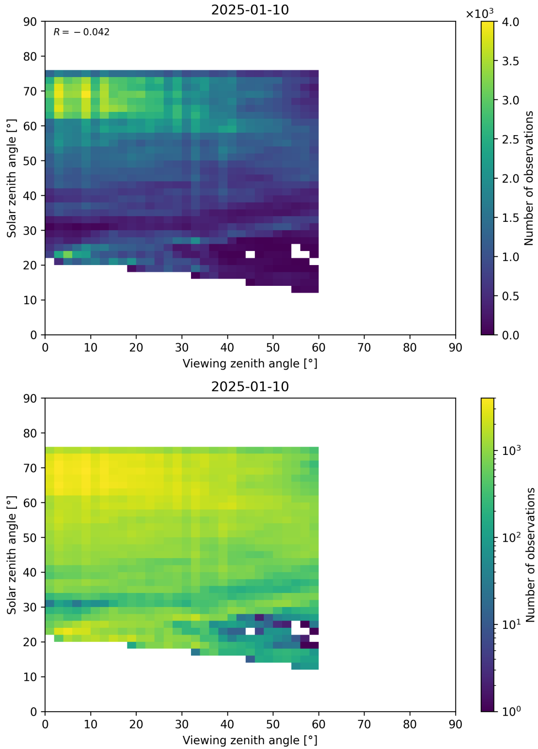
Figure 115: Scatter density plot of “Viewing zenith angle” against “Solar zenith angle” for 2025-01-09 to 2025-01-11.
