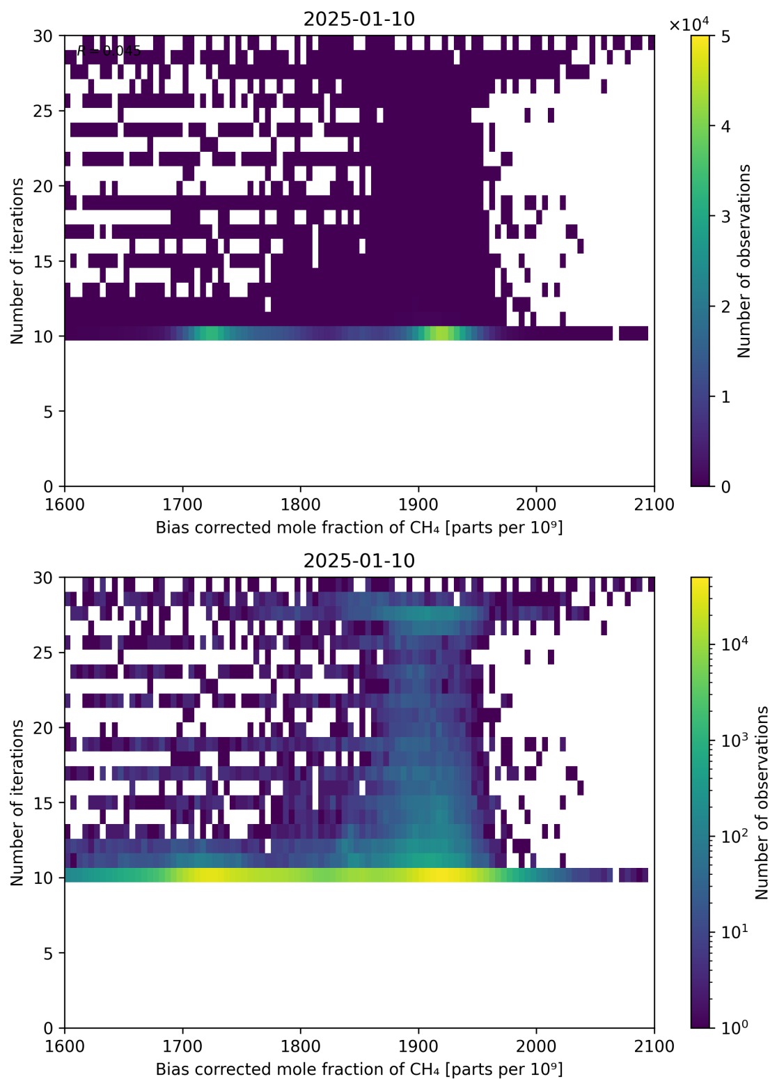
Figure 67: Scatter density plot of “Bias corrected mole fraction of CH 4 ” against “Number of iterations” for 2025-01-09 to 2025-01-11.
