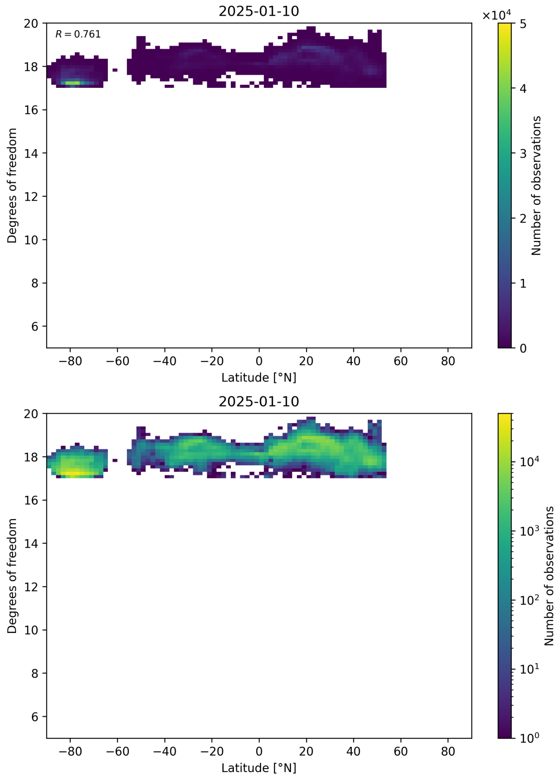
Figure 55: Scatter density plot of “Latitude” against “Degrees of freedom” for 2025-01-09 to 2025-01-11.
