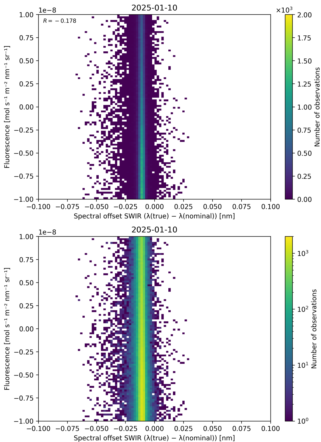
Figure 120: Scatter density plot of “Spectral offset SWIR ( \lambda_{\text{true}} - \lambda_{\text{nominal}} )” against “Fluorescence” for 2025-01-09 to 2025-01-11.
