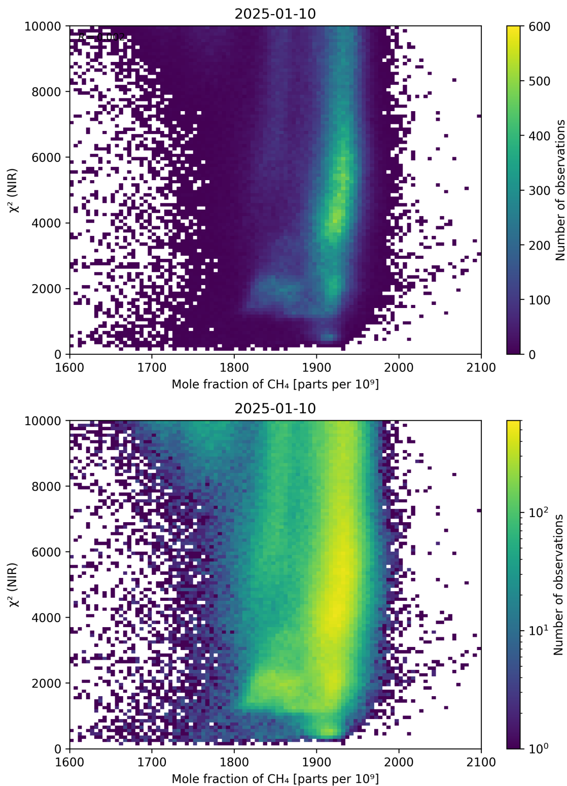
Figure 70: Scatter density plot of “Mole fraction of \text{CH}_4 ” against “ \chi^2 (NIR)” for 2025-01-09 to 2025-01-11.
