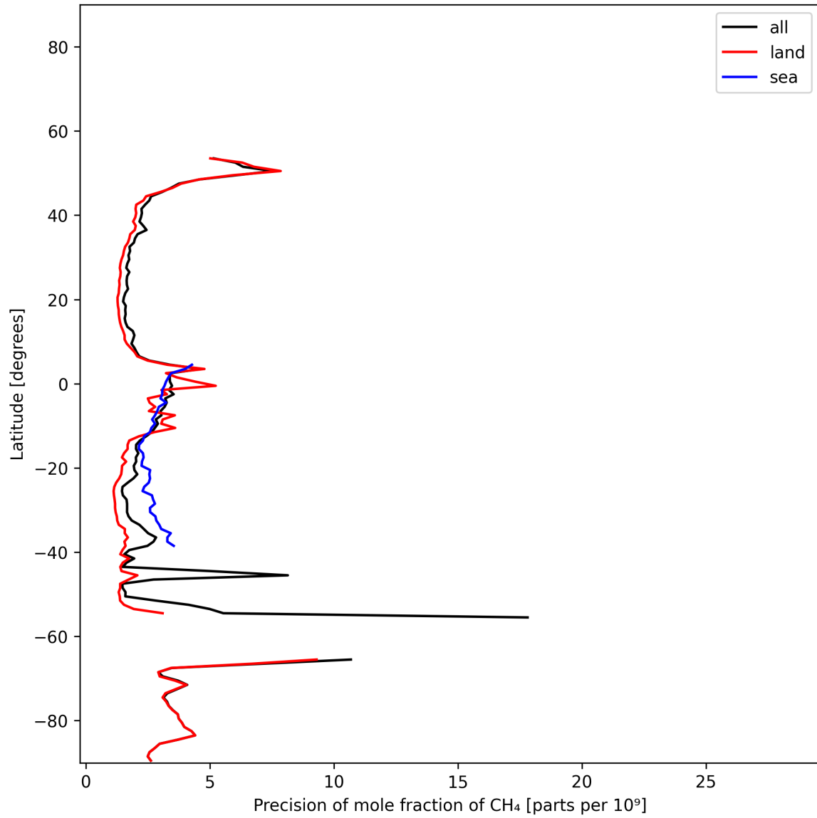
Figure 13: Zonal average of “Precision of mole fraction of CH 4 ” for 2025-01-09 to 2025-01-11.
