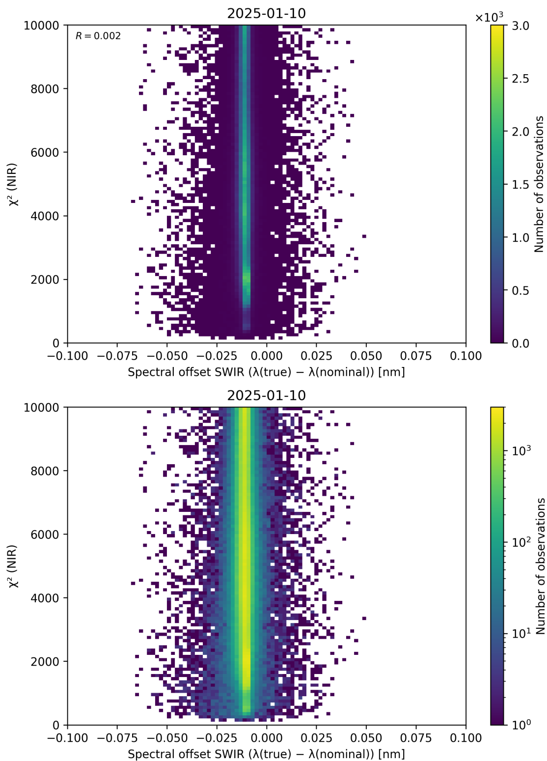
Figure 117: Scatter density plot of “Spectral offset SWIR ( \lambda_{\text{true}} - \lambda_{\text{nominal}} )” against “ \chi^2 (NIR)” for 2025-01-09 to 2025-01-11.
