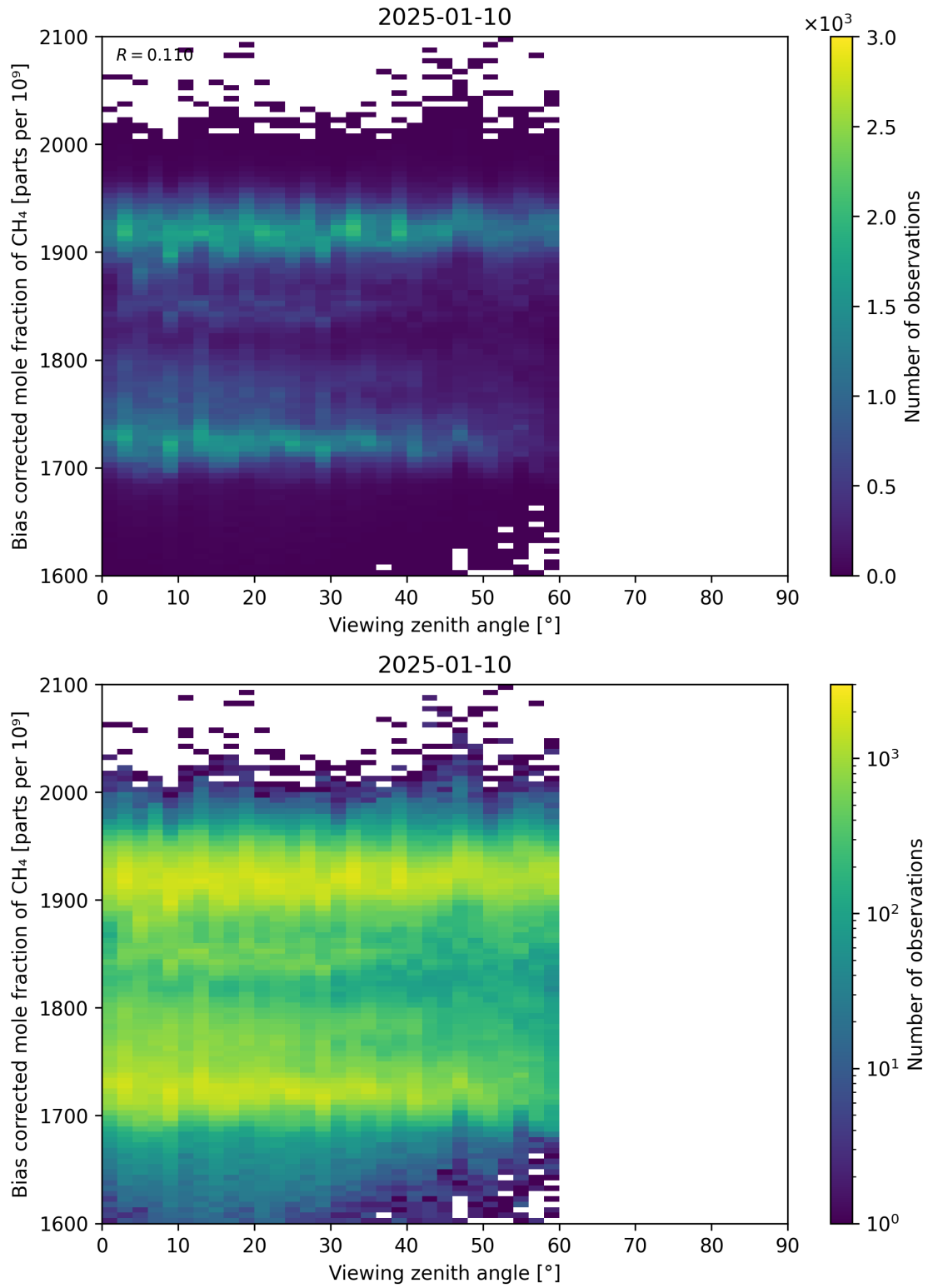
Figure 111: Scatter density plot of “Viewing zenith angle” against “Bias corrected mole fraction of CH 4 ” for 2025-01-09 to 2025-01-11.
