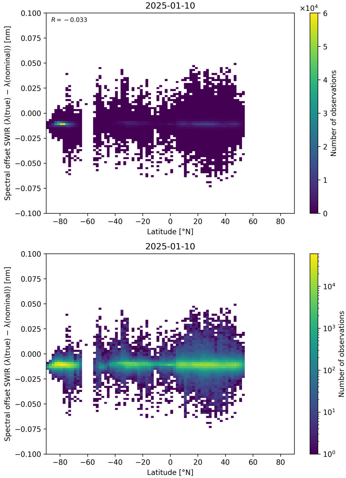
Figure 62: Scatter density plot of “Latitude” against “Spectral offset SWIR ( \lambda_{\text{true}} - \lambda_{\text{nominal}} )” for 2025-01-09 to 2025-01-11.
