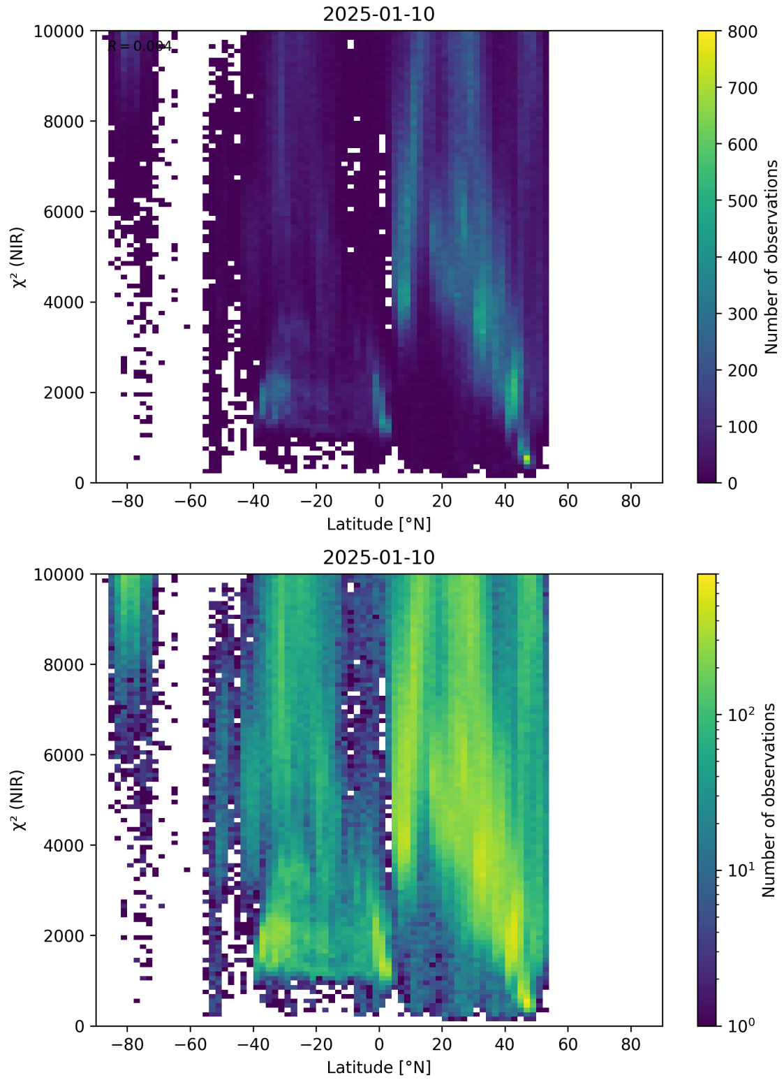
Figure 53: Scatter density plot of “Latitude” against “ \chi^2 (NIR)” for 2025-01-09 to 2025-01-11.
