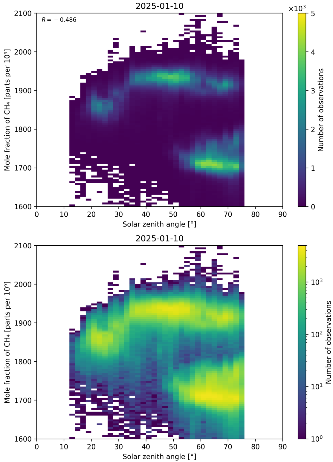
Figure 99: Scatter density plot of “Solar zenith angle” against “Mole fraction of CH 4 ” for 2025-01-09 to 2025-01-11.
