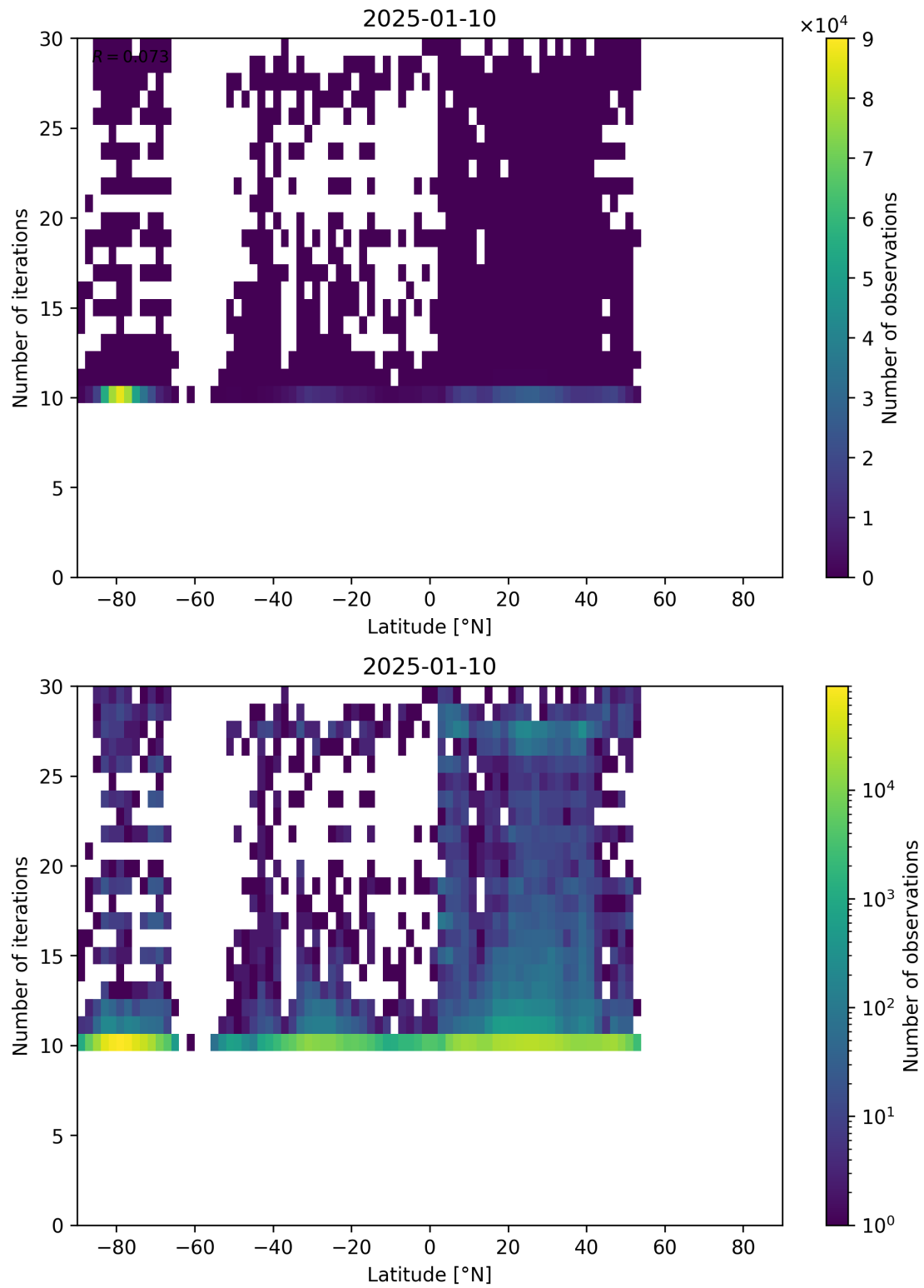
Figure 60: Scatter density plot of “Latitude” against “Number of iterations” for 2025-01-09 to 2025-01-11.
