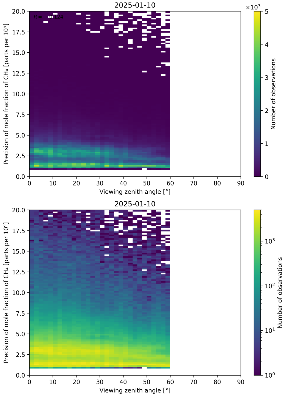
Figure 112: Scatter density plot of “Viewing zenith angle” against “Precision of mole fraction of CH 4 ” for 2025-01-09 to 2025-01-11.
