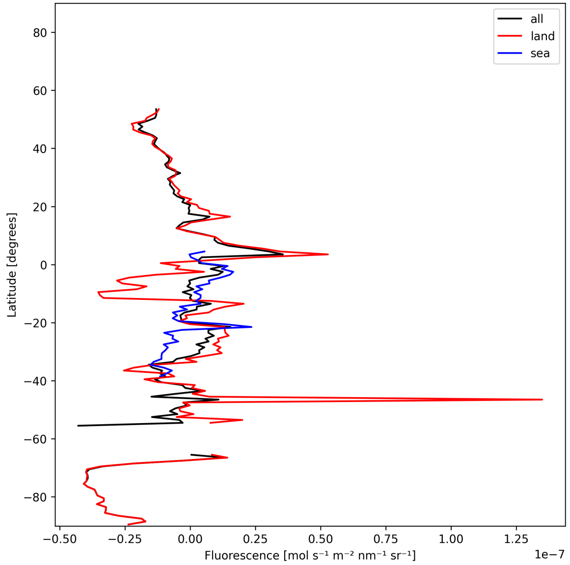
Figure 21: Zonal average of “Fluorescence” for 2025-01-09 to 2025-01-11.
