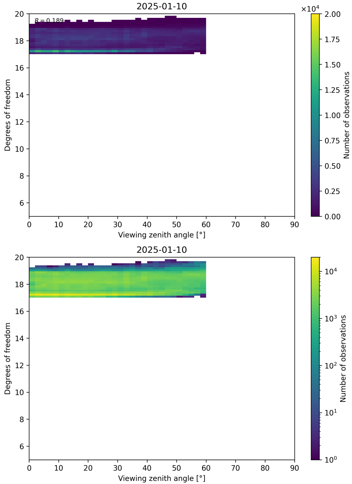
Figure 107: Scatter density plot of “Viewing zenith angle” against “Degrees of freedom” for 2025-01-09 to 2025-01-11.
