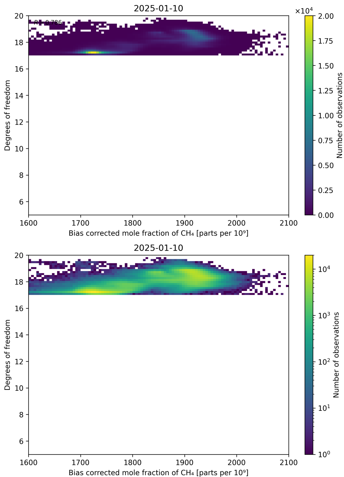
Figure 65: Scatter density plot of “Bias corrected mole fraction of CH 4 ” against “Degrees of freedom” for 2025-01-09 to 2025-01-11.
