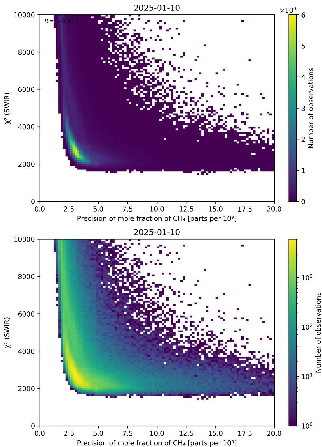
Figure 79: Scatter density plot of “Precision of mole fraction of \text{CH}_4 ” against “ \chi^2 (SWIR)” for 2025-01-09 to 2025-01-11.
