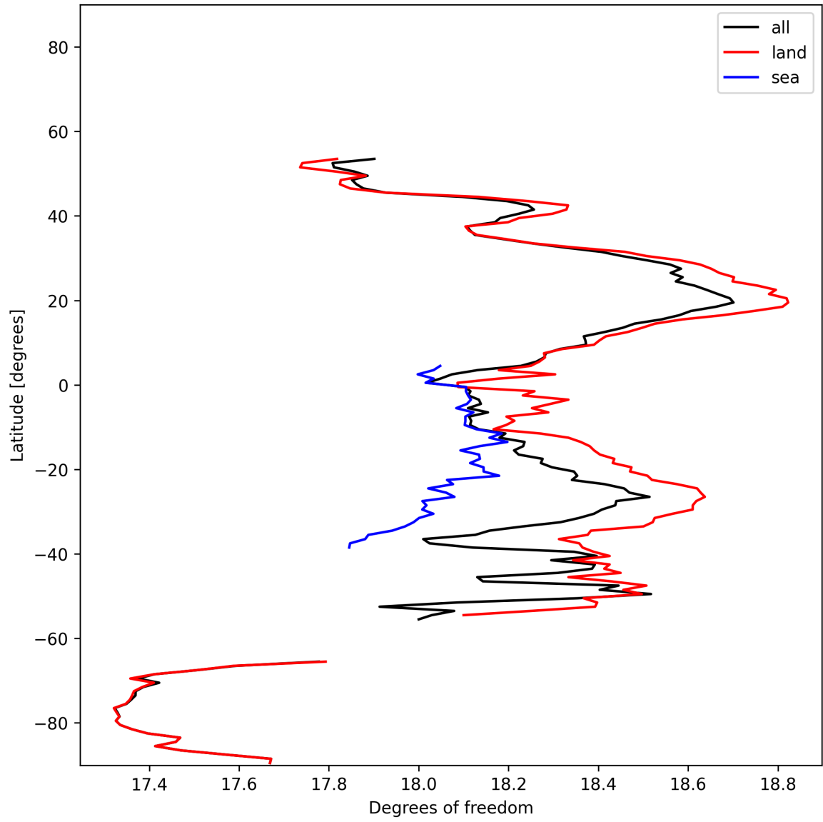
Figure 19: Zonal average of “Degrees of freedom” for 2025-01-09 to 2025-01-11.
