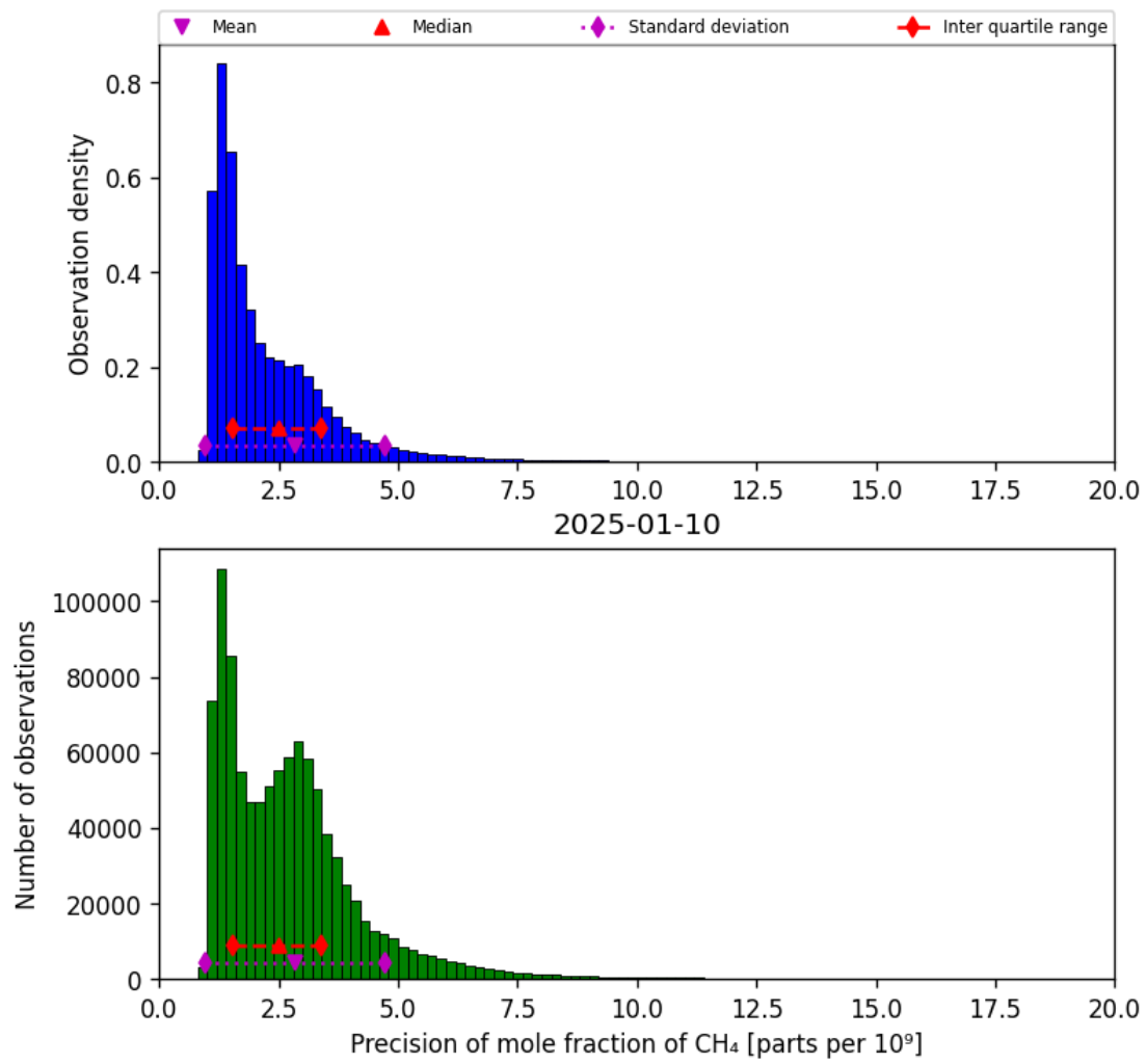
Figure 24: Histogram of “Precision of mole fraction of CH 4 ” for 2025-01-09 to 2025-01-11
