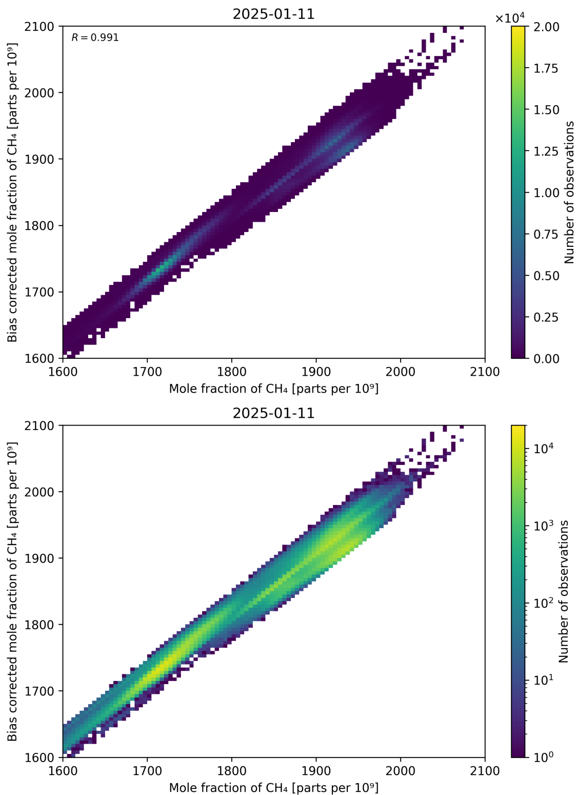
Figure 74: Scatter density plot of “Mole fraction of CH 4 ” against “Bias corrected mole fraction of CH 4 ” for 2025-01-10 to 2025-01-12.
