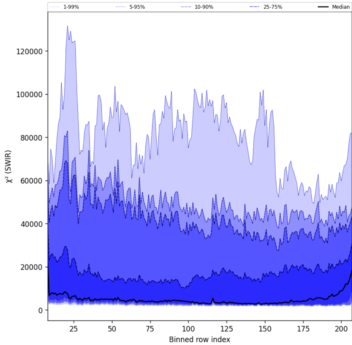
Figure 39: Along track statistics of “ \chi^2 (SWIR)” for 2025-01-10 to 2025-01-12
