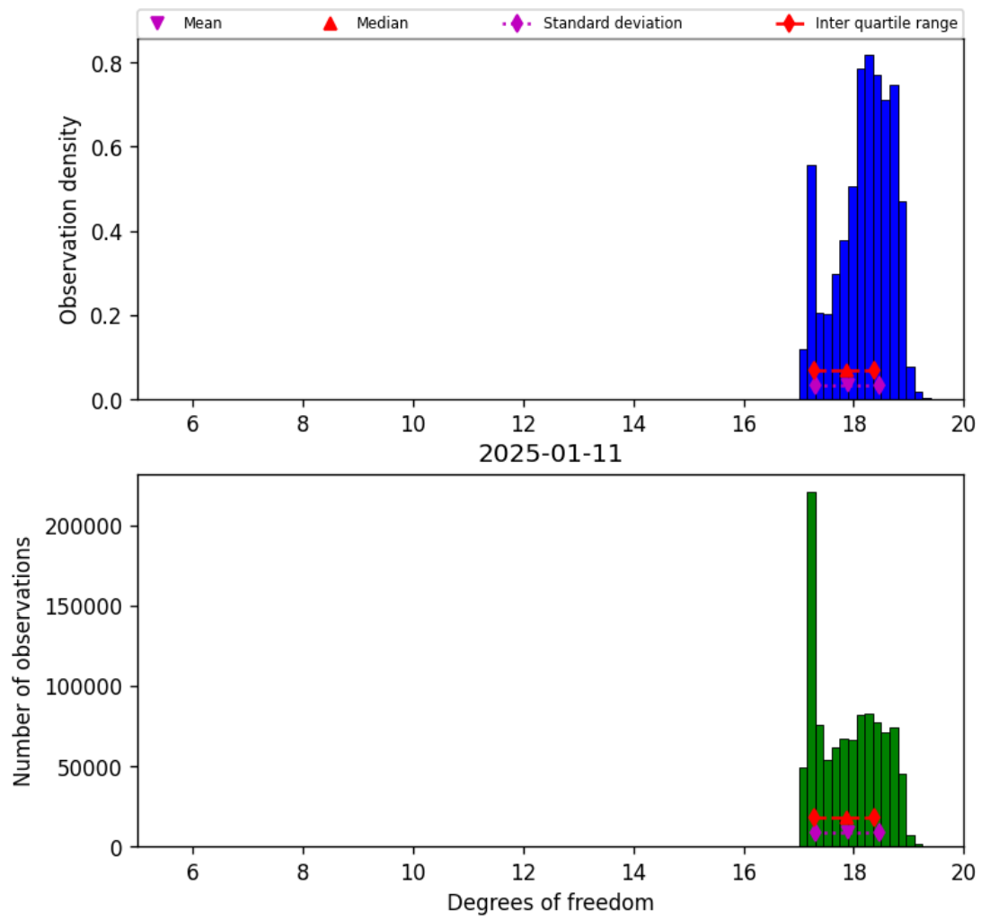
Figure 30: Histogram of “Degrees of freedom” for 2025-01-10 to 2025-01-12
