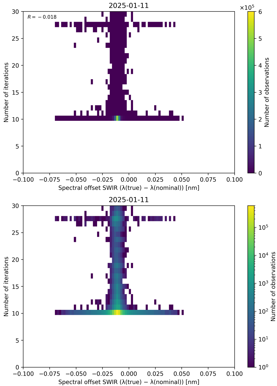
Figure 121: Scatter density plot of “Spectral offset SWIR ( \lambda_{\text{true}} - \lambda_{\text{nominal}} )” against “Number of iterations” for 2025-01-10 to 2025-01-12.
