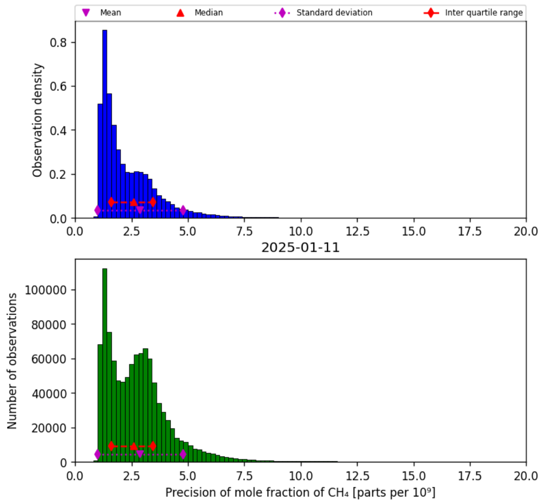
Figure 24: Histogram of “Precision of mole fraction of CH 4 ” for 2025-01-10 to 2025-01-12
