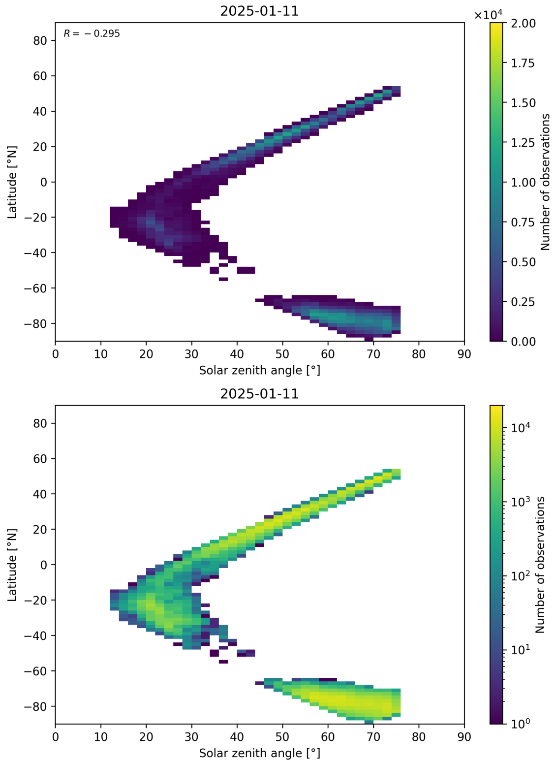
Figure 98: Scatter density plot of “Solar zenith angle” against “Latitude” for 2025-01-10 to 2025-01-12.
