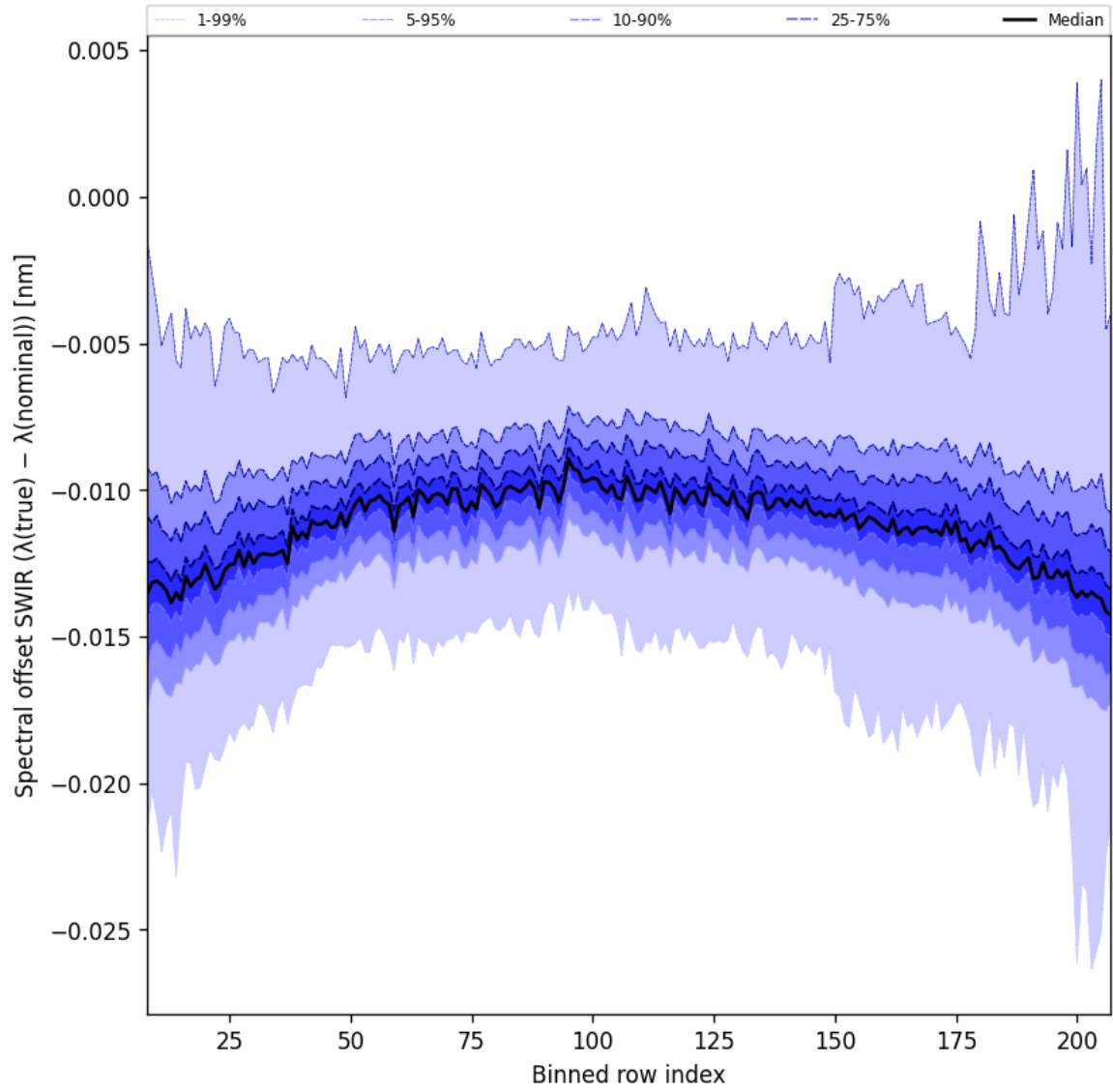
Figure 38: Along track statistics of “Spectral offset SWIR ( \lambda_{\text{true}} - \lambda_{\text{nominal}} )” for 2025-01-10 to 2025-01-12
