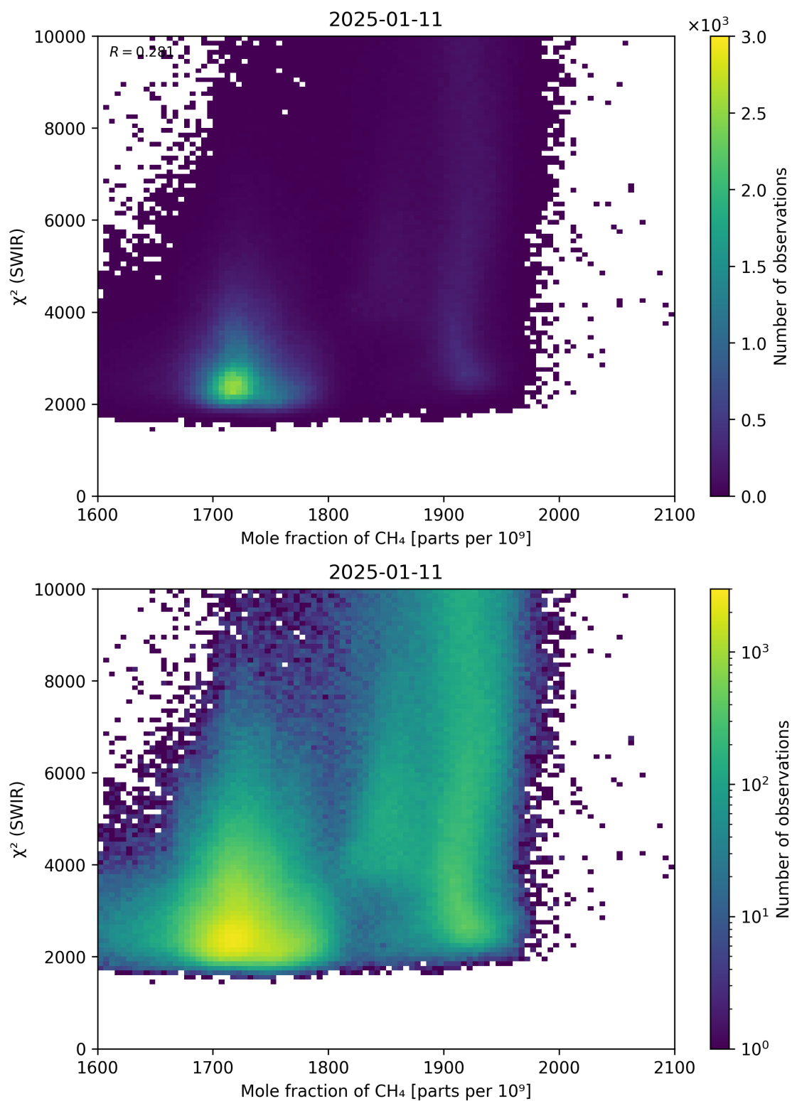
Figure 71: Scatter density plot of “Mole fraction of \text{CH}_4 ” against “ \chi^2 (SWIR)” for 2025-01-10 to 2025-01-12.
