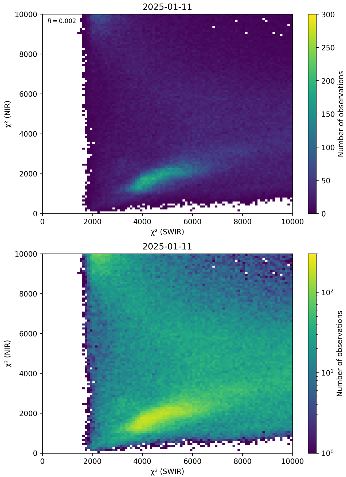
Figure 47: Scatter density plot of “ \chi^2 (SWIR)” against “ \chi^2 (NIR)” for 2025-01-10 to 2025-01-12.
