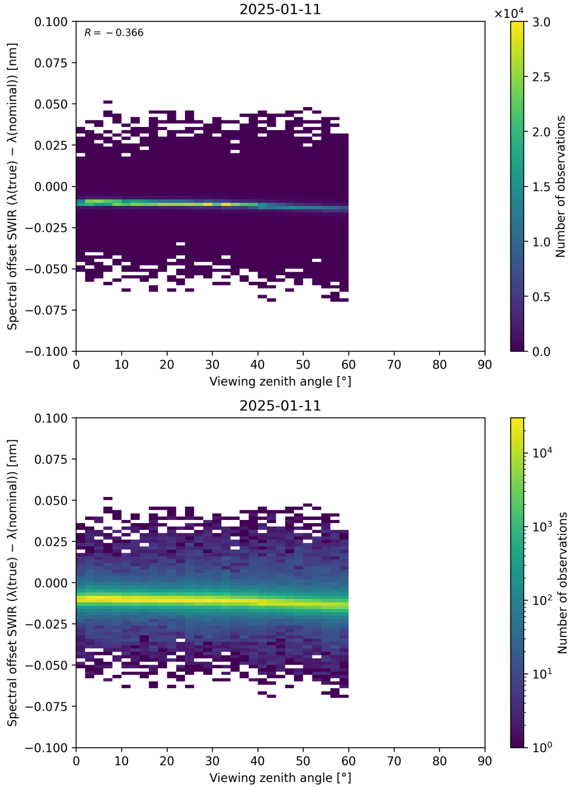
Figure 116: Scatter density plot of “Viewing zenith angle” against “Spectral offset SWIR ( \lambda_{\text{true}} - \lambda_{\text{nominal}} )” for 2025-01-10 to 2025-01-12.
