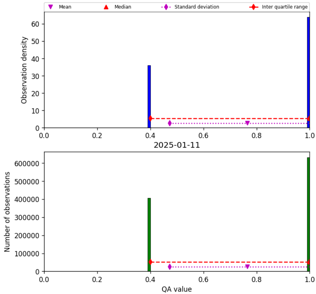
Figure 22: Histogram of “QA value” for 2025-01-10 to 2025-01-12
