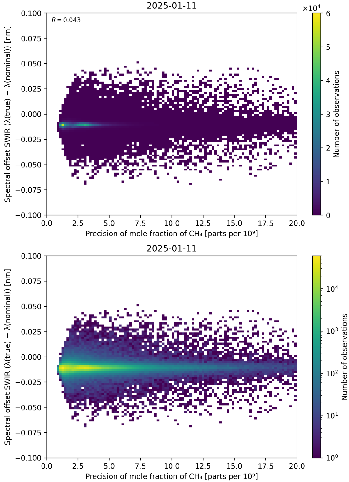
Figure 85: Scatter density plot of “Precision of mole fraction of CH 4 ” against “Spectral offset SWIR ( \lambda_{\text{true}} - \lambda_{\text{nominal}} )” for 2025-01-10 to 2025-01-12.
