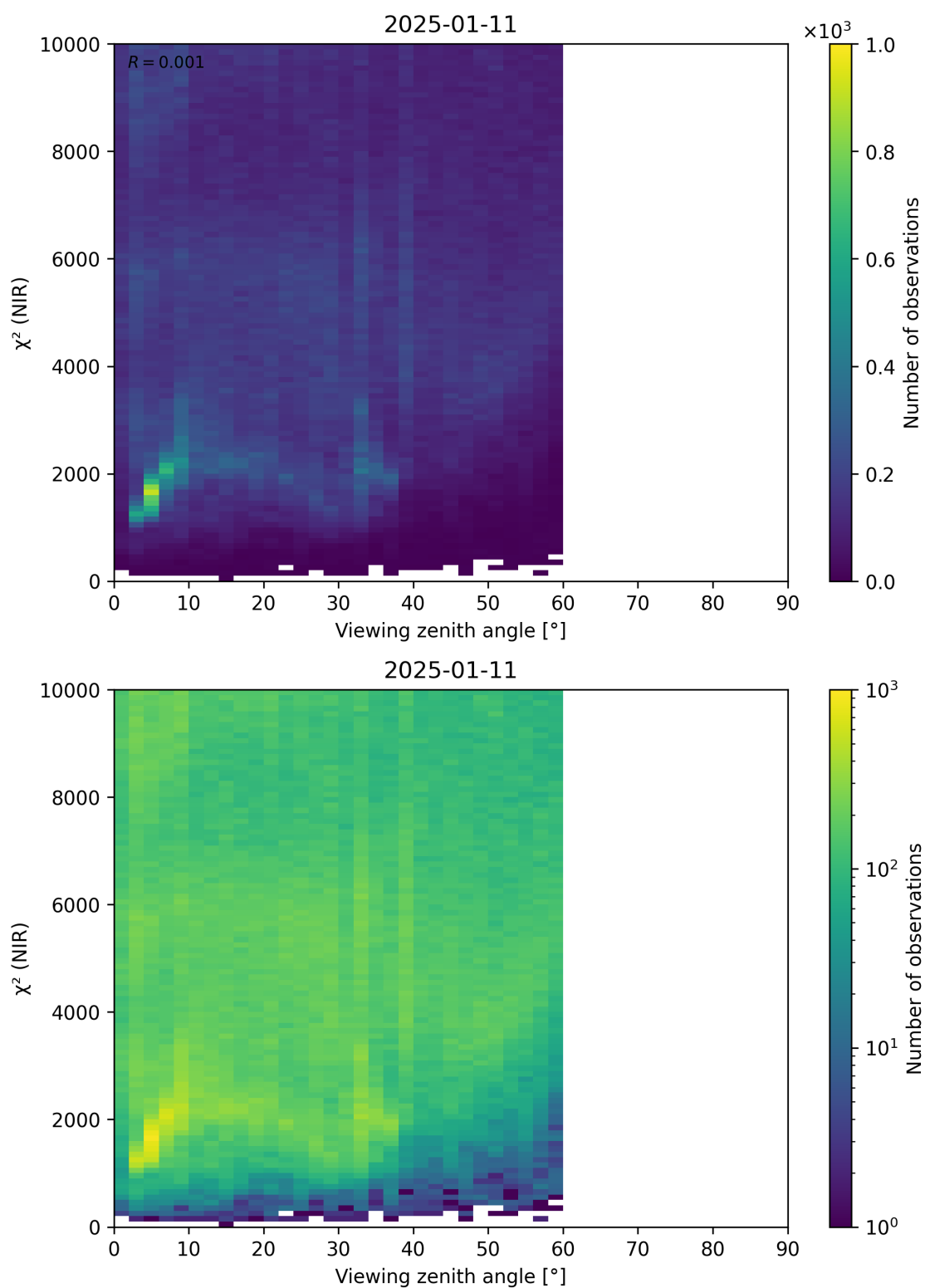
Figure 105: Scatter density plot of “Viewing zenith angle” against “ \chi^2 (NIR)” for 2025-01-10 to 2025-01-12.
