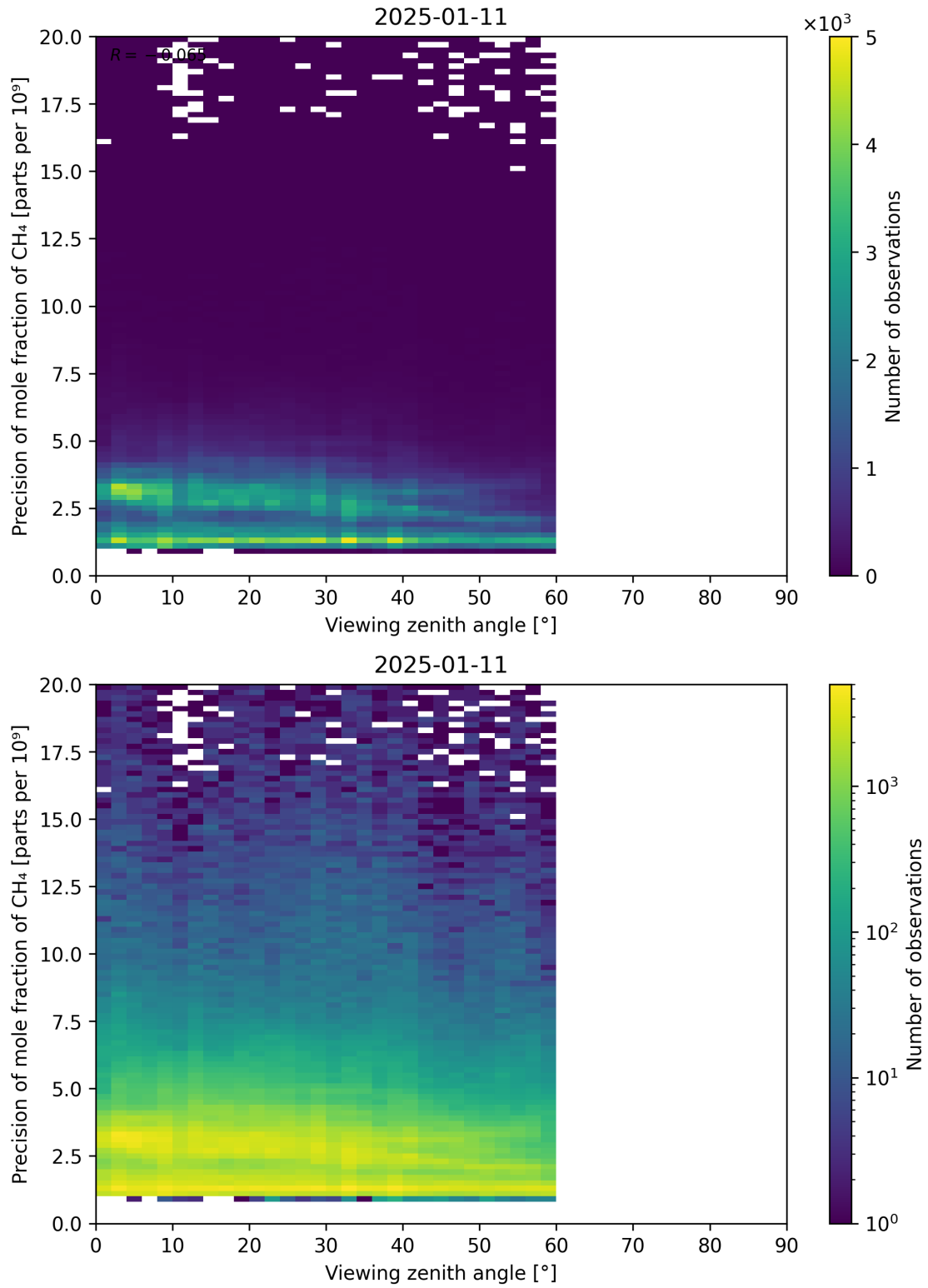
Figure 112: Scatter density plot of “Viewing zenith angle” against “Precision of mole fraction of CH 4 ” for 2025-01-10 to 2025-01-12.
