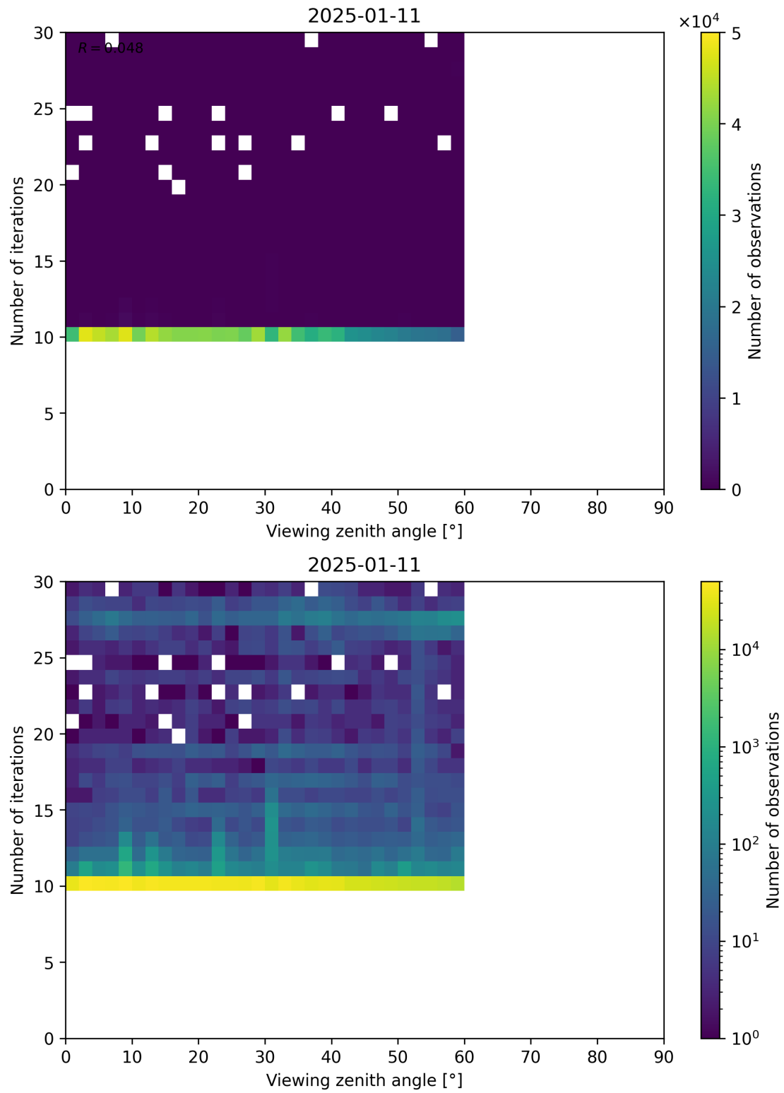
Figure 113: Scatter density plot of “Viewing zenith angle” against “Number of iterations” for 2025-01-10 to 2025-01-12.
