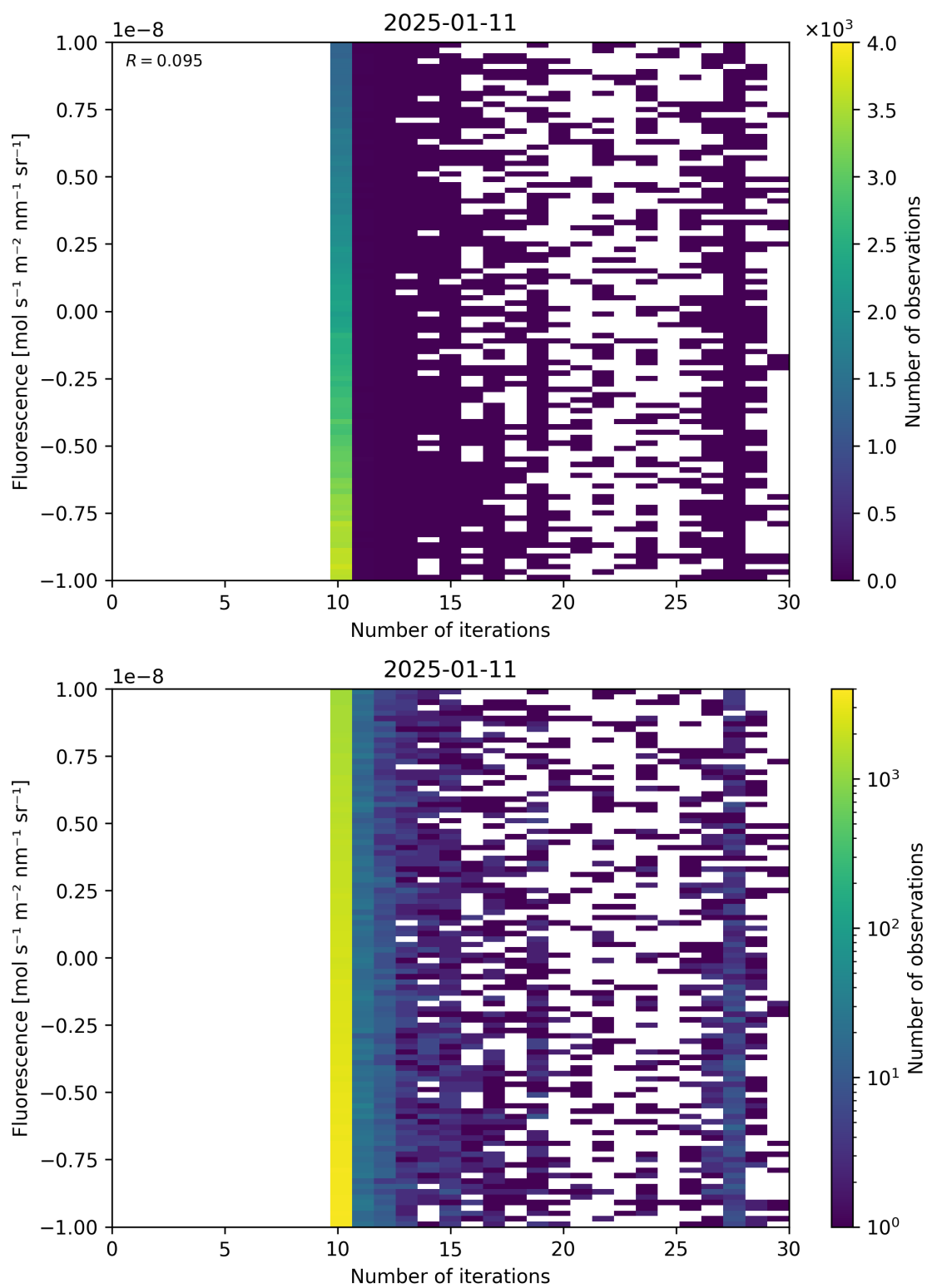
Figure 87: Scatter density plot of “Number of iterations” against “Fluorescence” for 2025-01-10 to 2025-01-12.
