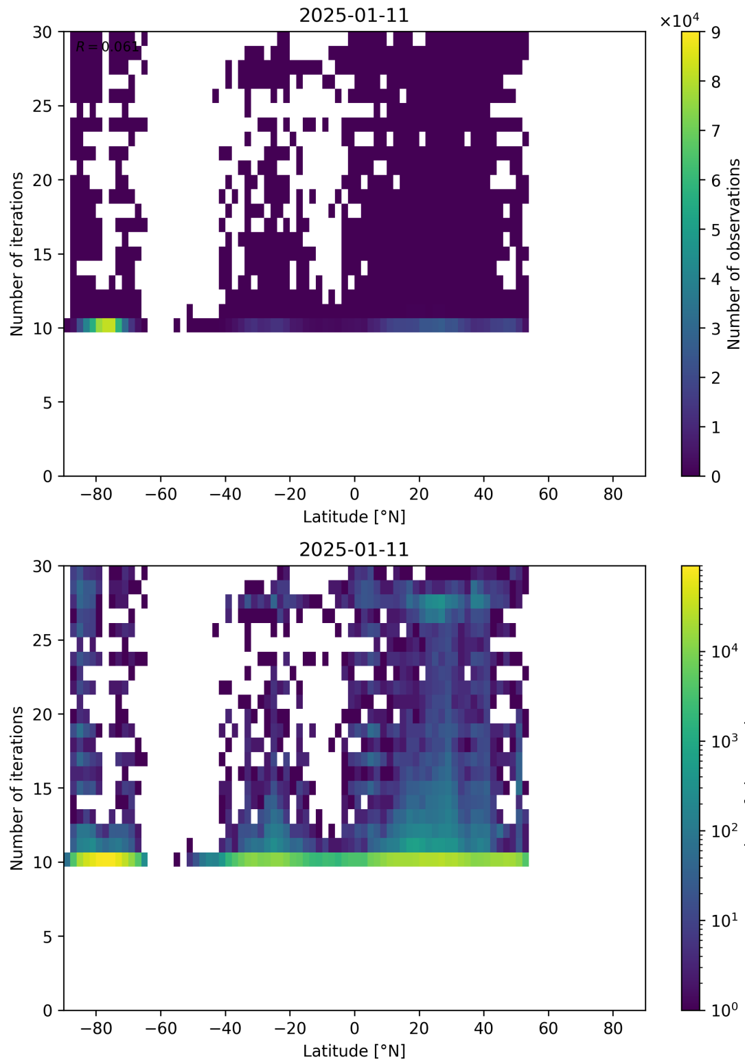
Figure 60: Scatter density plot of “Latitude” against “Number of iterations” for 2025-01-10 to 2025-01-12.
