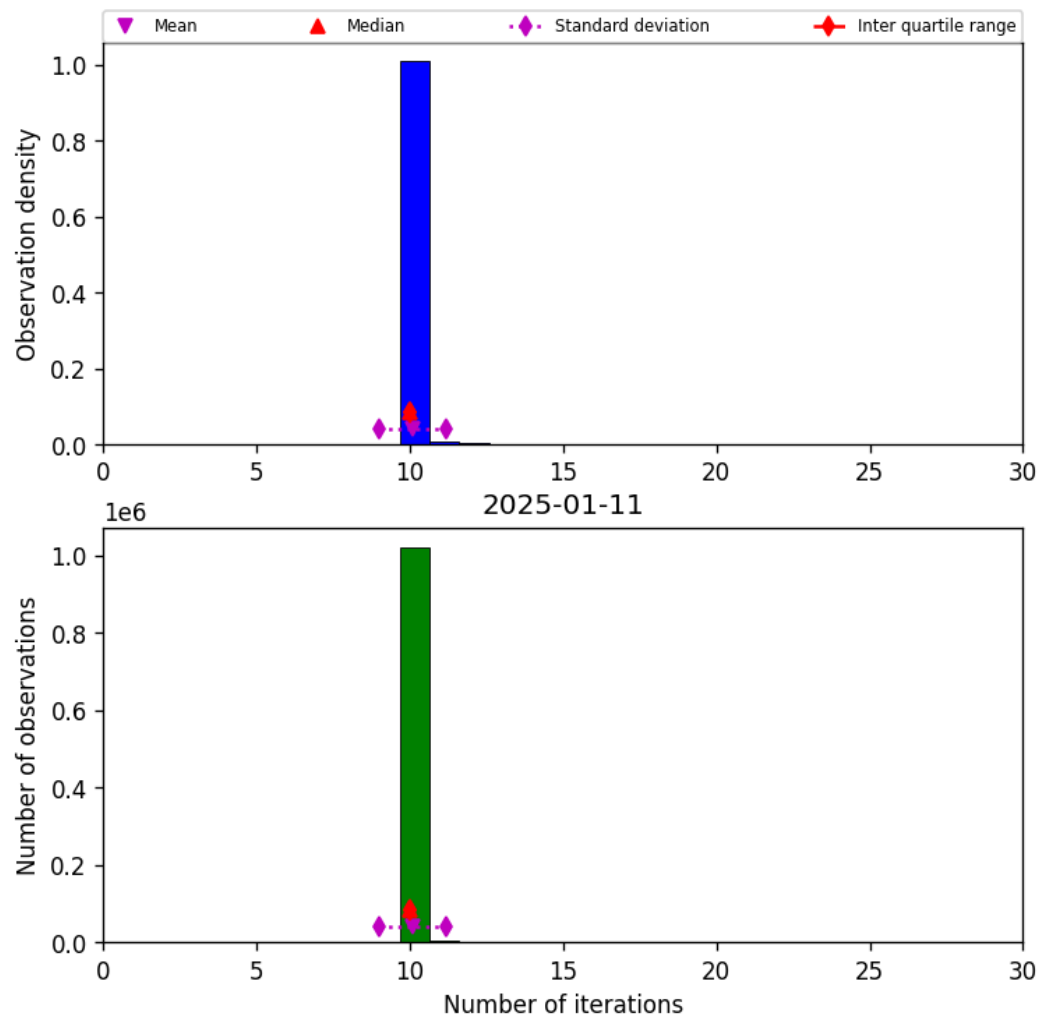
Figure 31: Histogram of "Number of iterations" for 2025-01-10 to 2025-01-12
