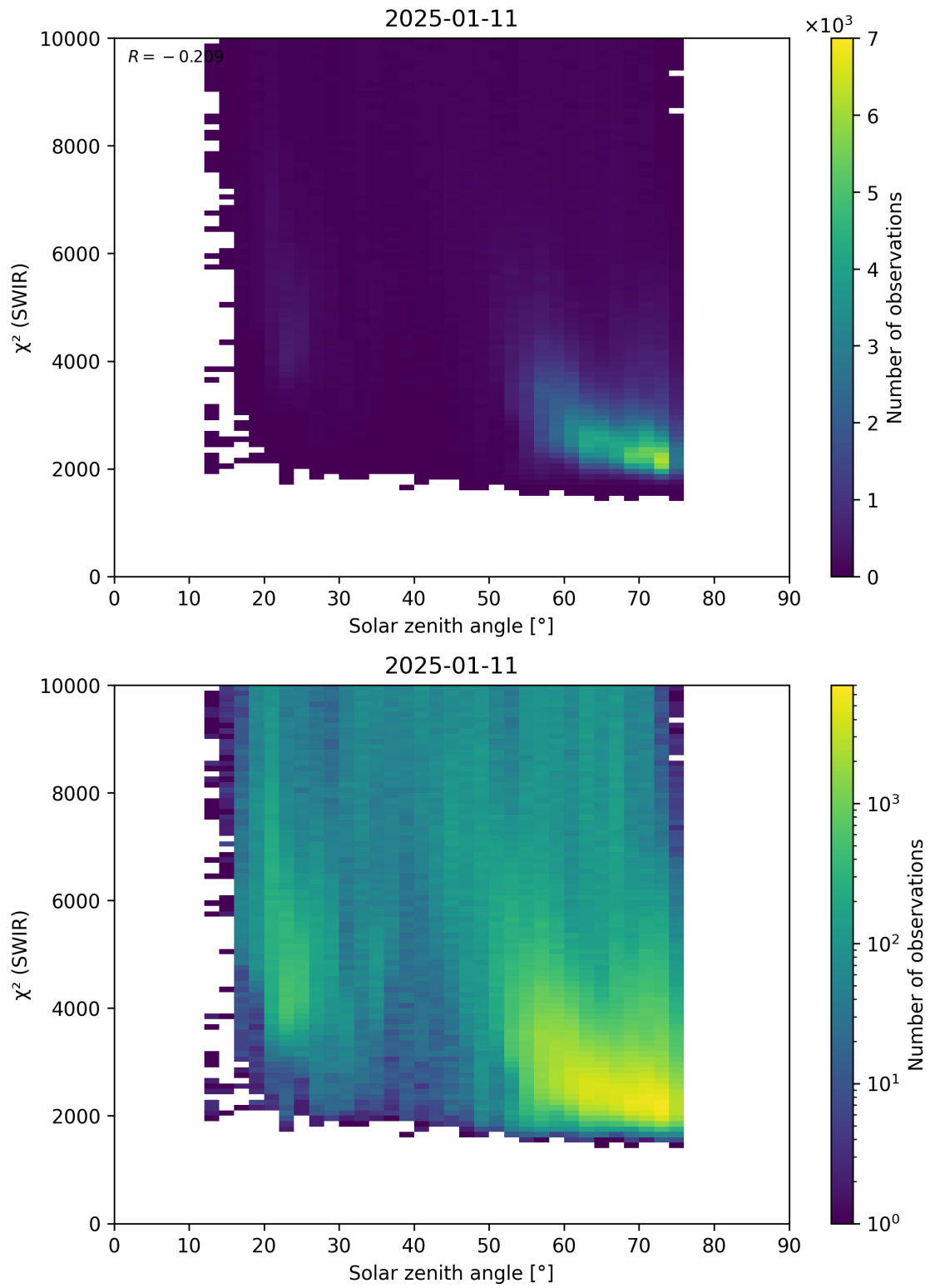
Figure 95: Scatter density plot of “Solar zenith angle” against “ \chi^2 (SWIR)” for 2025-01-10 to 2025-01-12.
