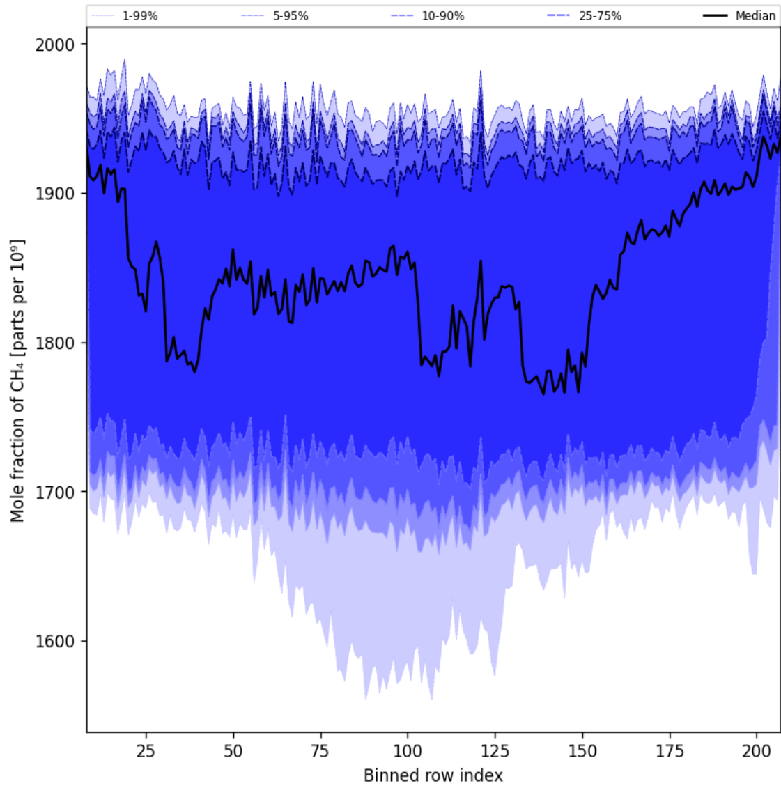
Figure 34: Along track statistics of “Mole fraction of CH 4 ” for 2025-01-10 to 2025-01-12
