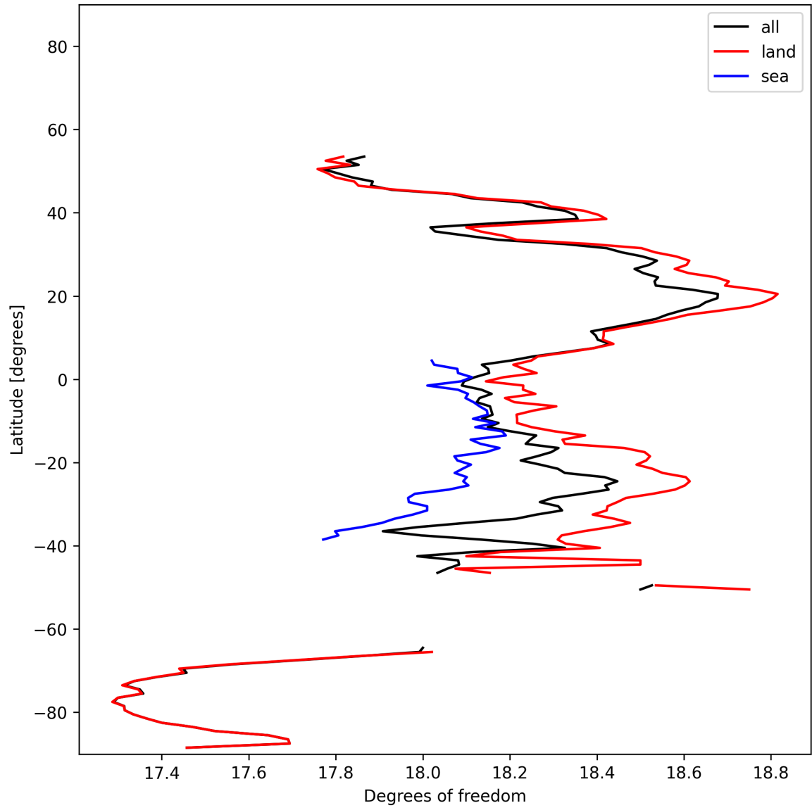
Figure 19: Zonal average of “Degrees of freedom” for 2025-01-10 to 2025-01-12.
