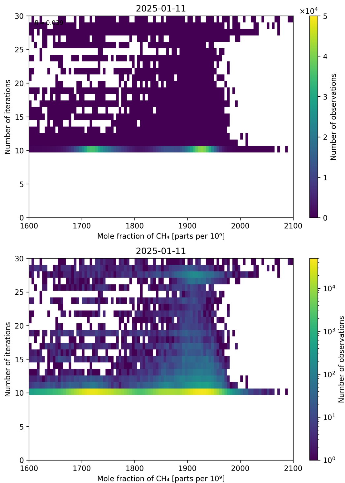
Figure 76: Scatter density plot of “Mole fraction of CH 4 ” against “Number of iterations” for 2025-01-10 to 2025-01-12.
