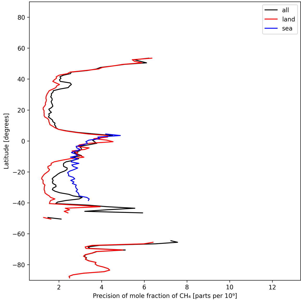
Figure 13: Zonal average of “Precision of mole fraction of CH 4 ” for 2025-01-10 to 2025-01-12.
