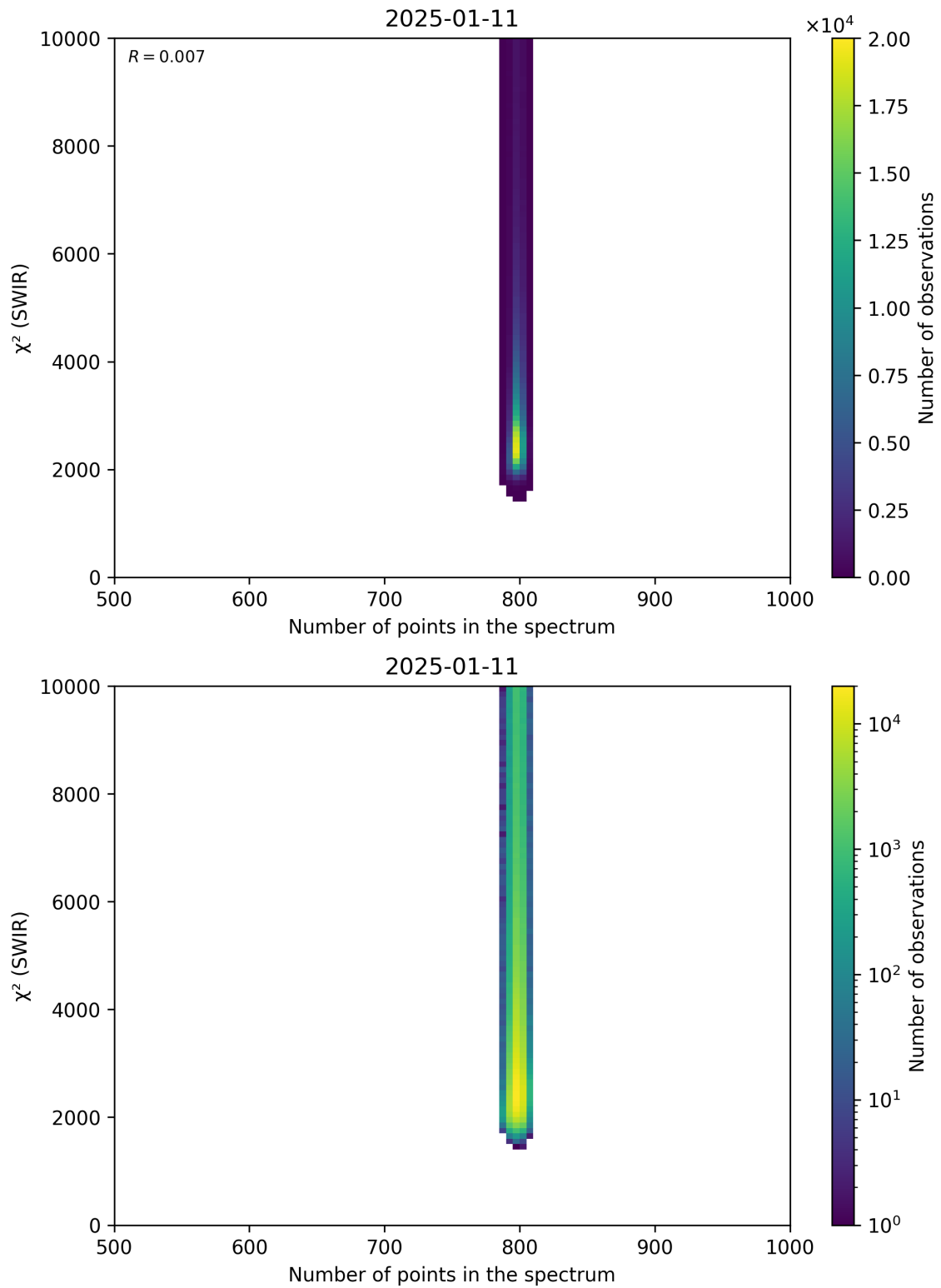
Figure 89: Scatter density plot of “Number of points in the spectrum” against “ \chi^2 (SWIR)” for 2025-01-10 to 2025-01-12.
