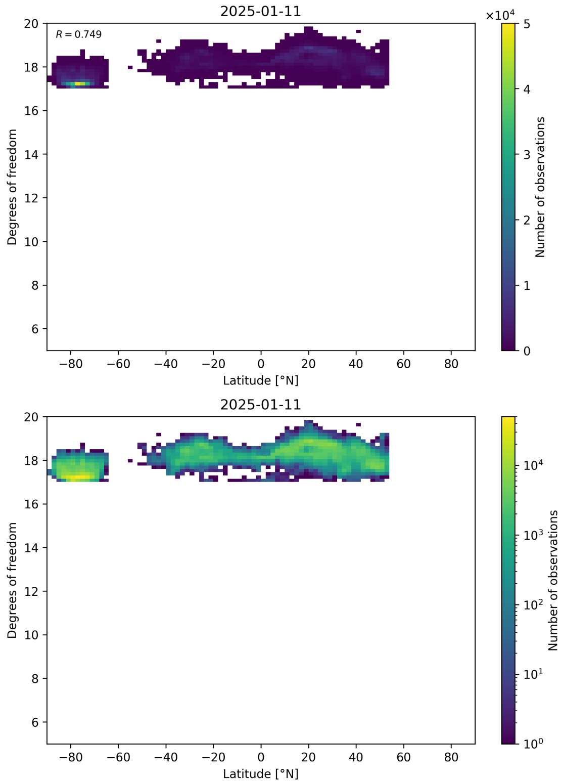
Figure 55: Scatter density plot of “Latitude” against “Degrees of freedom” for 2025-01-10 to 2025-01-12.
