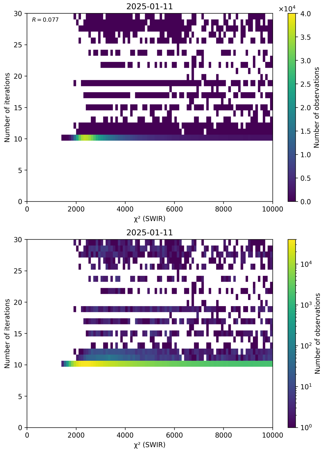
Figure 50: Scatter density plot of “ \chi^2 (SWIR)” against “Number of iterations” for 2025-01-10 to 2025-01-12.
