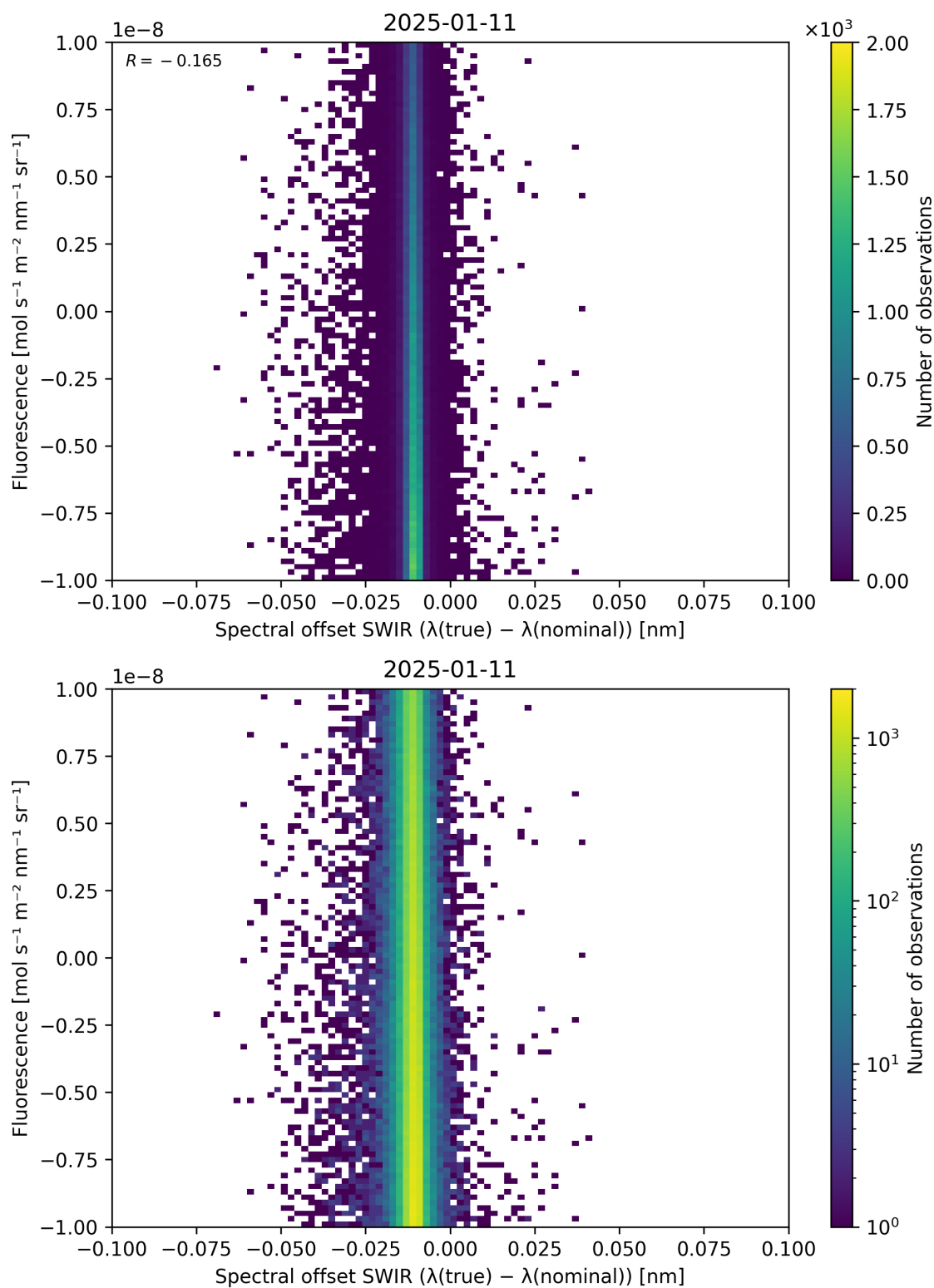
Figure 120: Scatter density plot of “Spectral offset SWIR ( \lambda_{\text{true}} - \lambda_{\text{nominal}} )” against “Fluorescence” for 2025-01-10 to 2025-01-12.
