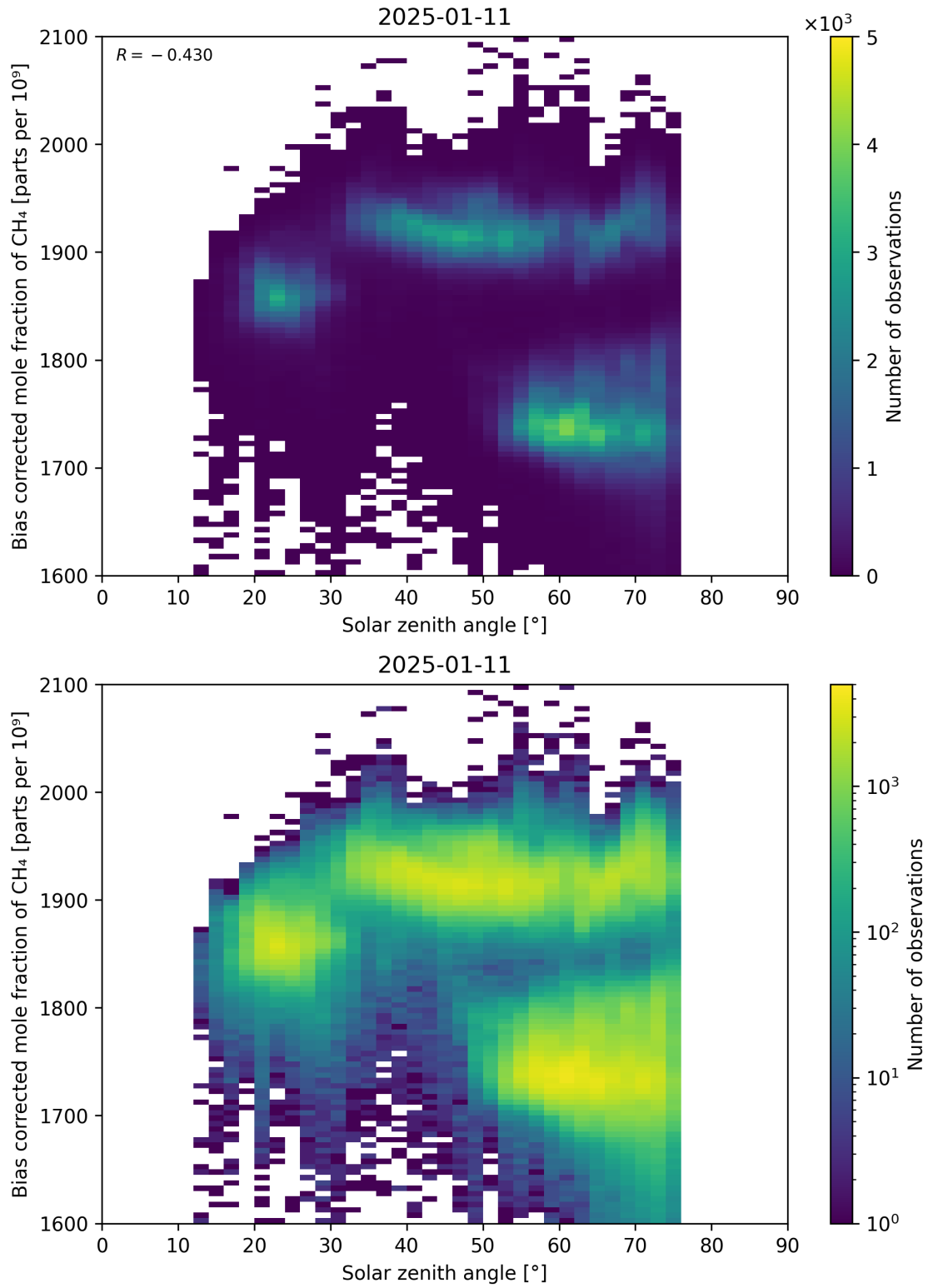
Figure 100: Scatter density plot of “Solar zenith angle” against “Bias corrected mole fraction of CH 4 ” for 2025-01-10 to 2025-01-12.
