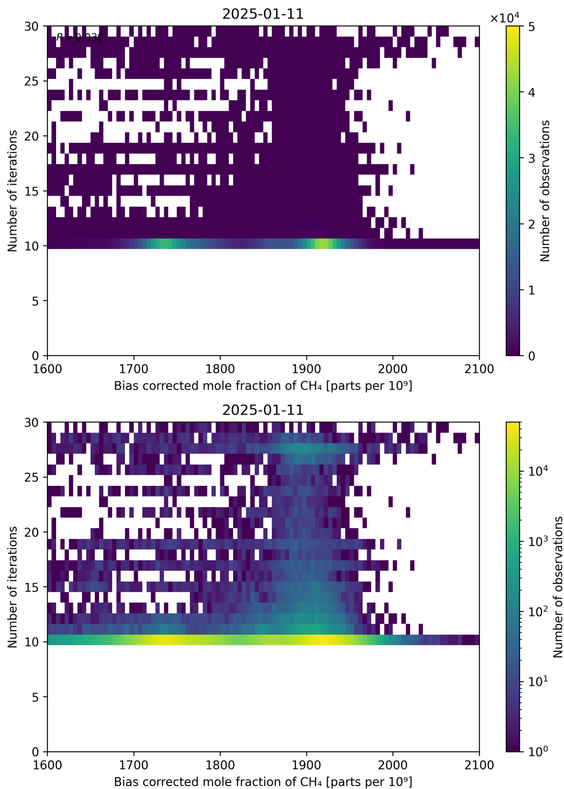
Figure 67: Scatter density plot of “Bias corrected mole fraction of CH 4 ” against “Number of iterations” for 2025-01-10 to 2025-01-12.
