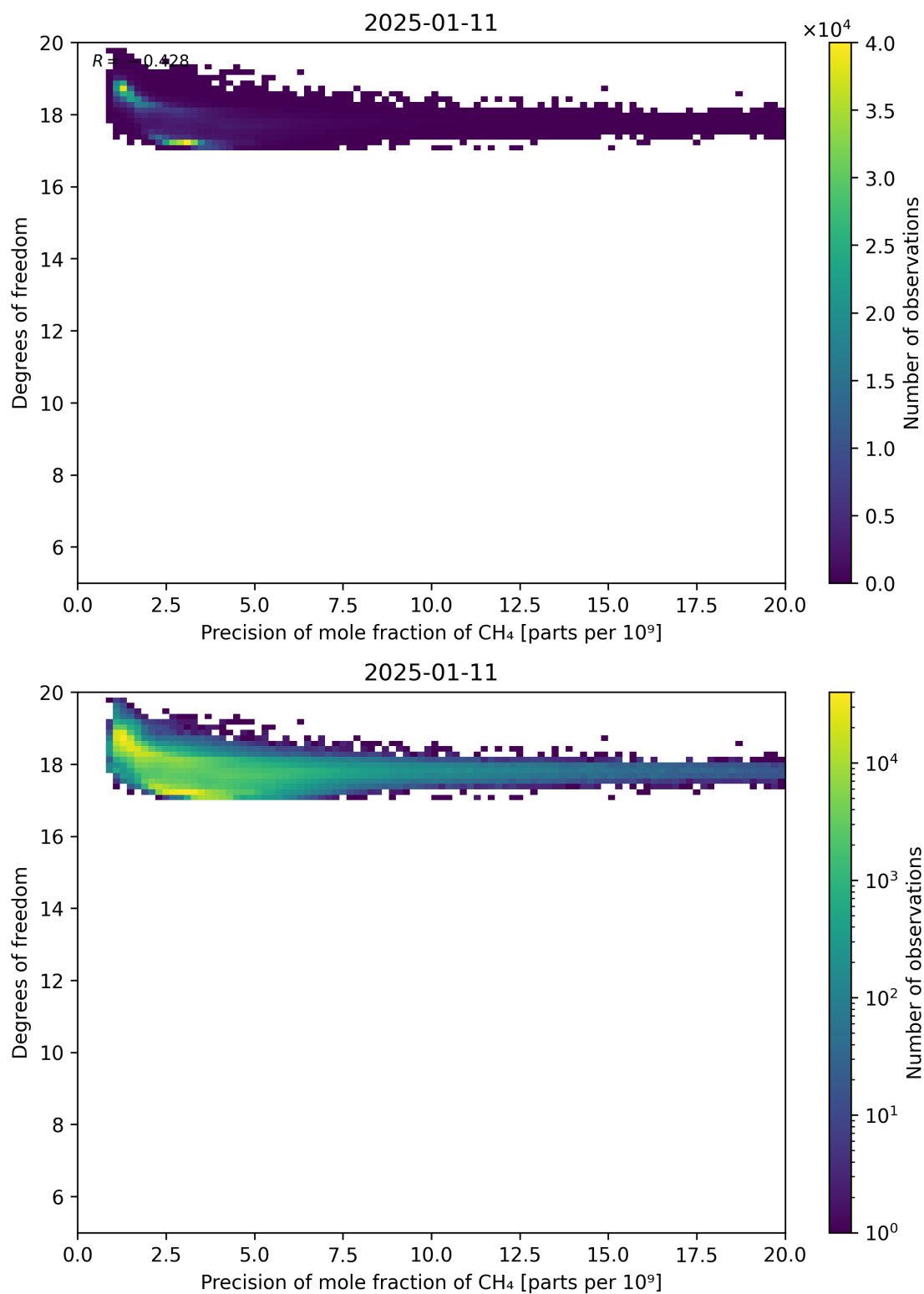
Figure 80: Scatter density plot of “Precision of mole fraction of CH 4 ” against “Degrees of freedom” for 2025-01-10 to 2025-01-12.
