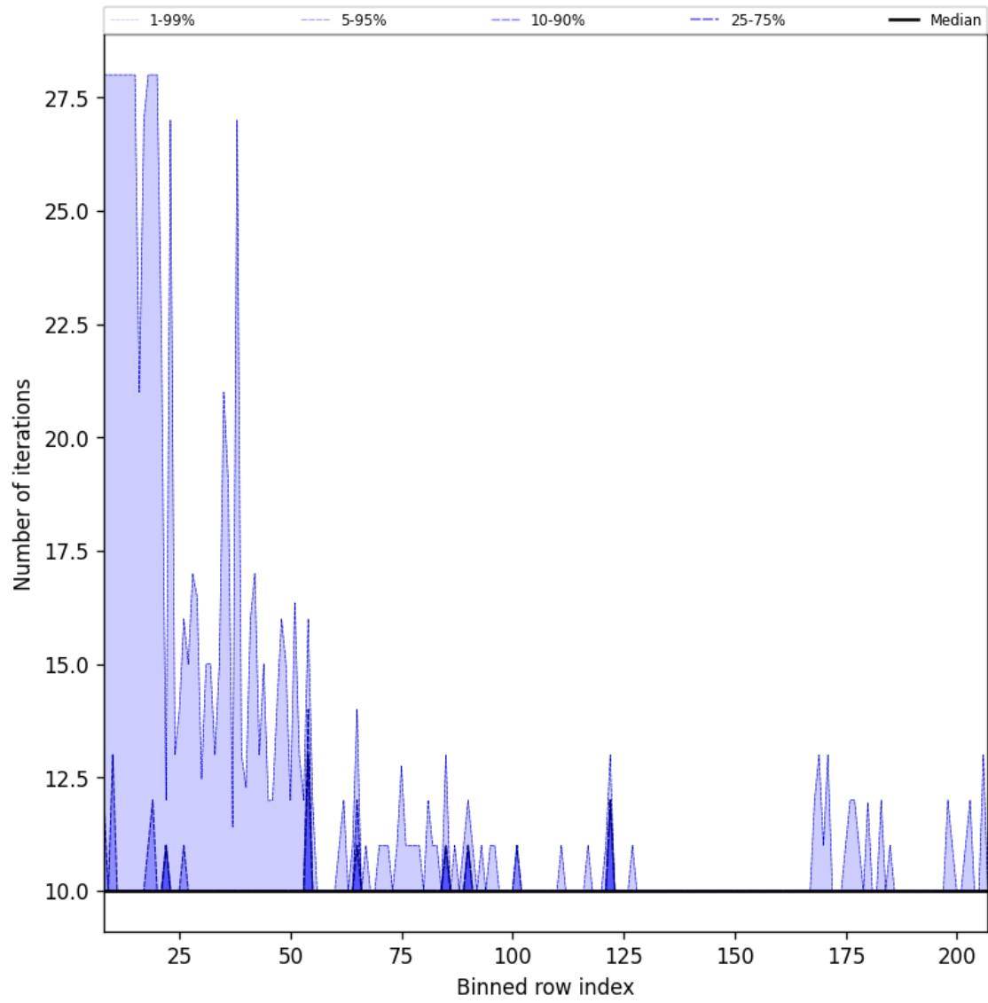
Figure 42: Along track statistics of “Number of iterations” for 2025-01-10 to 2025-01-12
