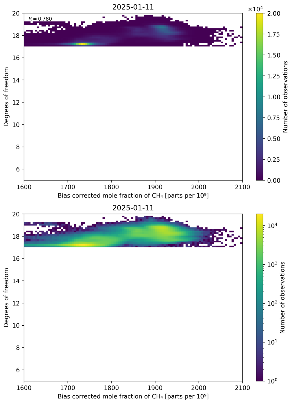
Figure 65: Scatter density plot of “Bias corrected mole fraction of CH 4 ” against “Degrees of freedom” for 2025-01-10 to 2025-01-12.
