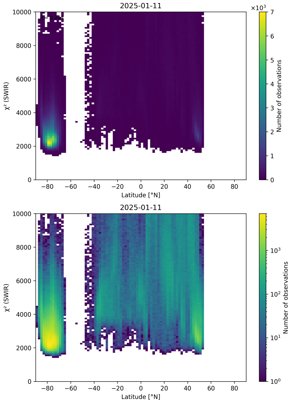
Figure 54: Scatter density plot of “Latitude” against “ \chi^2 (SWIR)” for 2025-01-10 to 2025-01-12.
