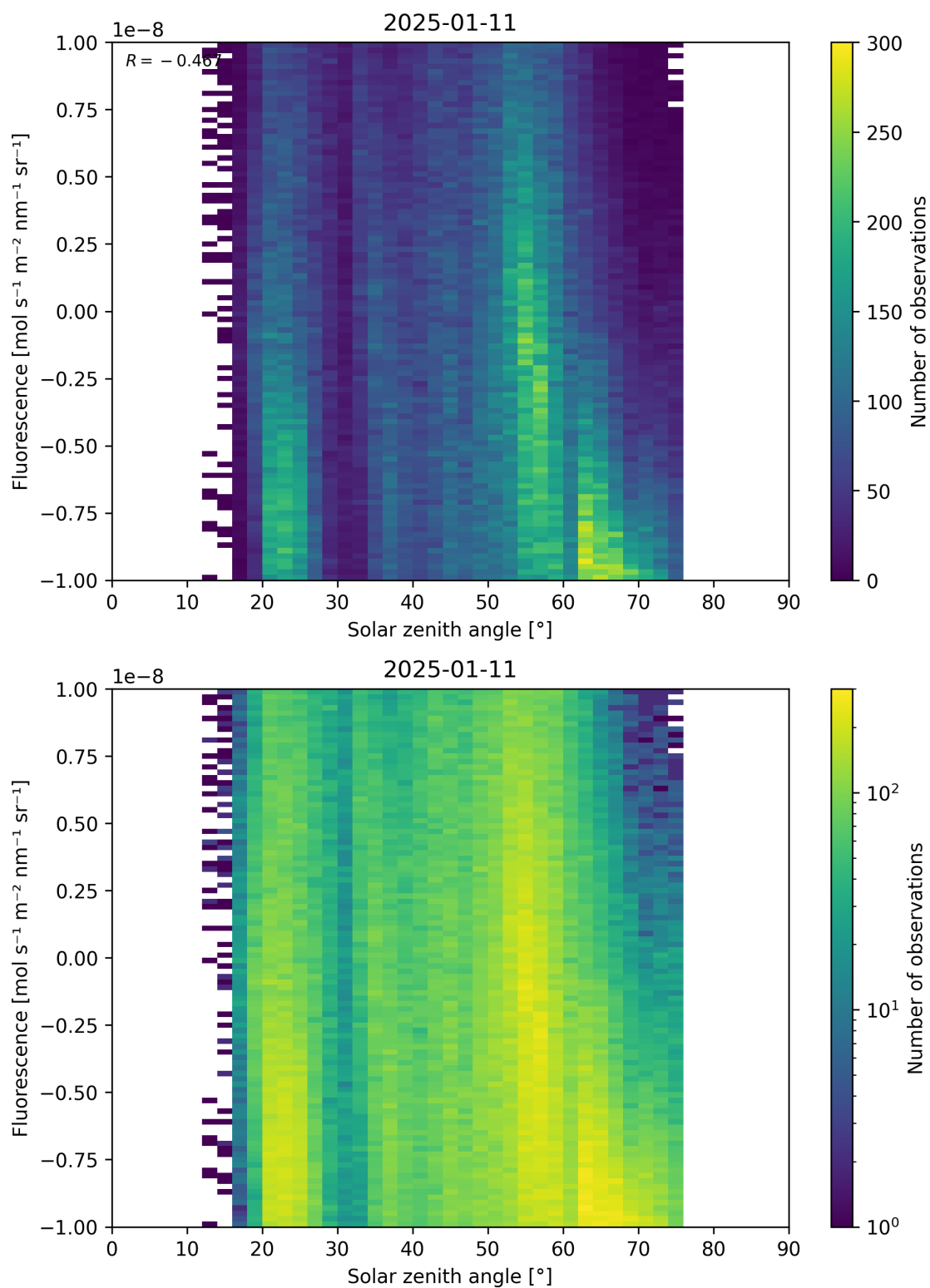
Figure 97: Scatter density plot of “Solar zenith angle” against “Fluorescence” for 2025-01-10 to 2025-01-12.
