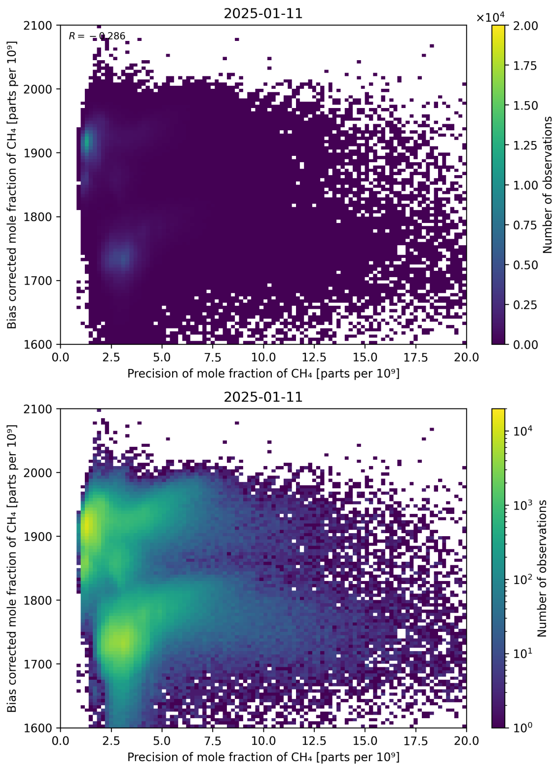
Figure 82: Scatter density plot of “Precision of mole fraction of CH 4 ” against “Bias corrected mole fraction of CH 4 ” for 2025-01-10 to 2025-01-12.
