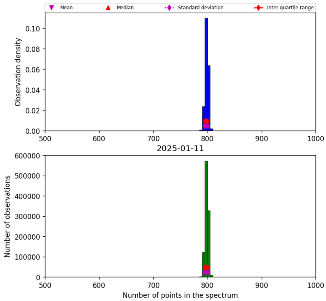
Figure 26: Histogram of “Number of points in the spectrum” for 2025-01-10 to 2025-01-12
