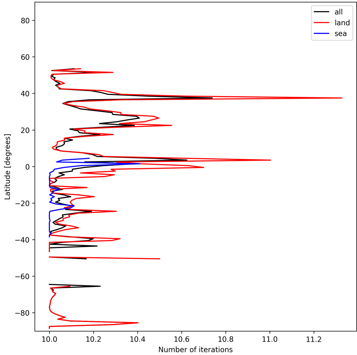
Figure 20: Zonal average of “Number of iterations” for 2025-01-10 to 2025-01-12.
