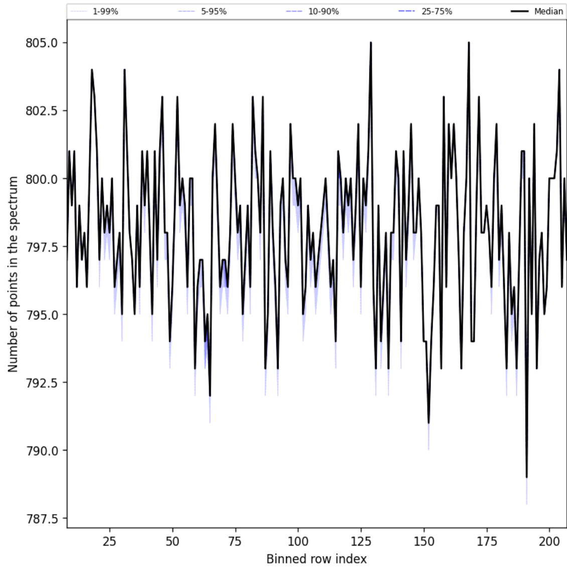
Figure 37: Along track statistics of “Number of points in the spectrum” for 2025-01-10 to 2025-01-12
