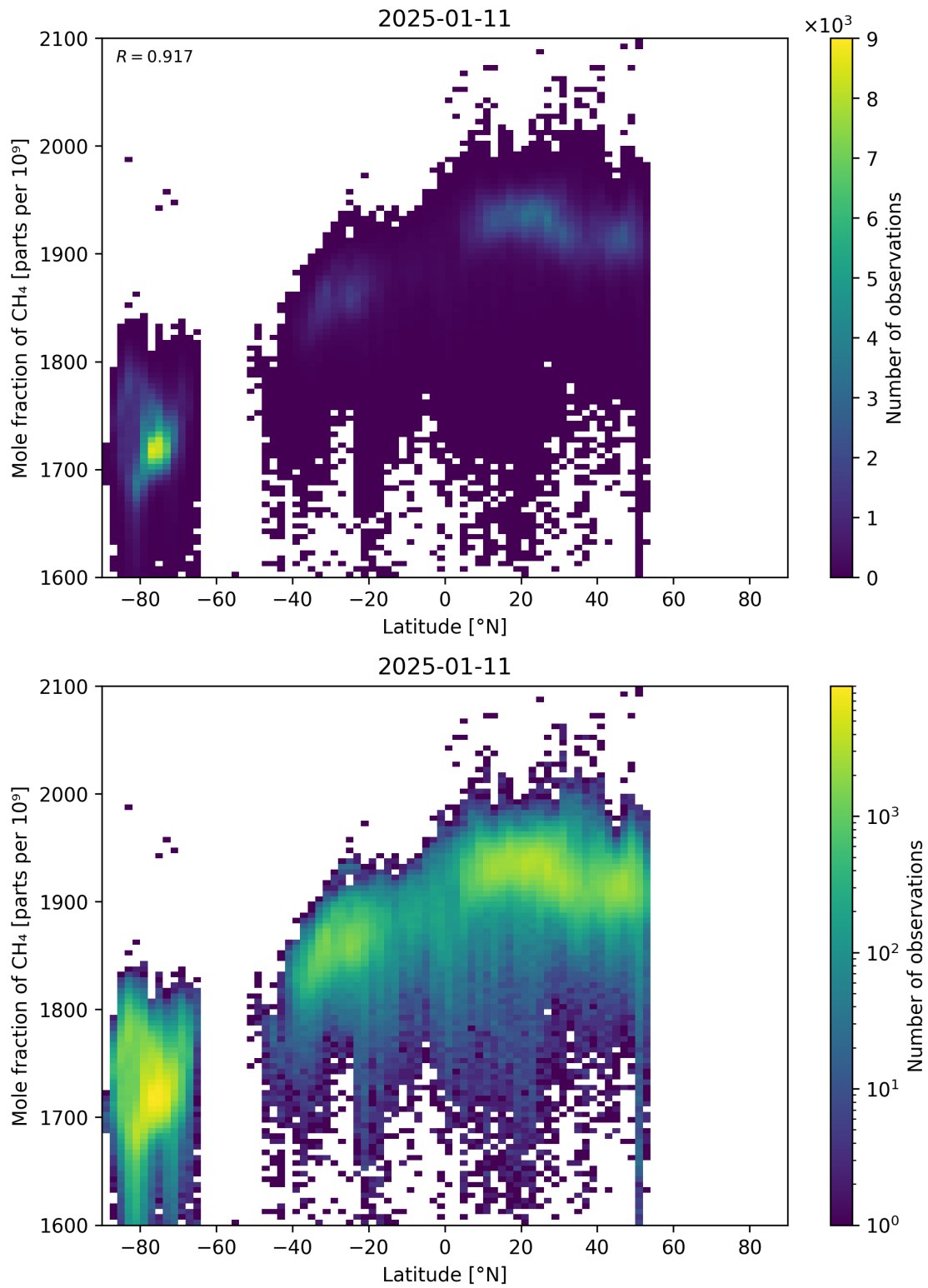
Figure 57: Scatter density plot of “Latitude” against “Mole fraction of \text{CH}_4 ” for 2025-01-10 to 2025-01-12.
