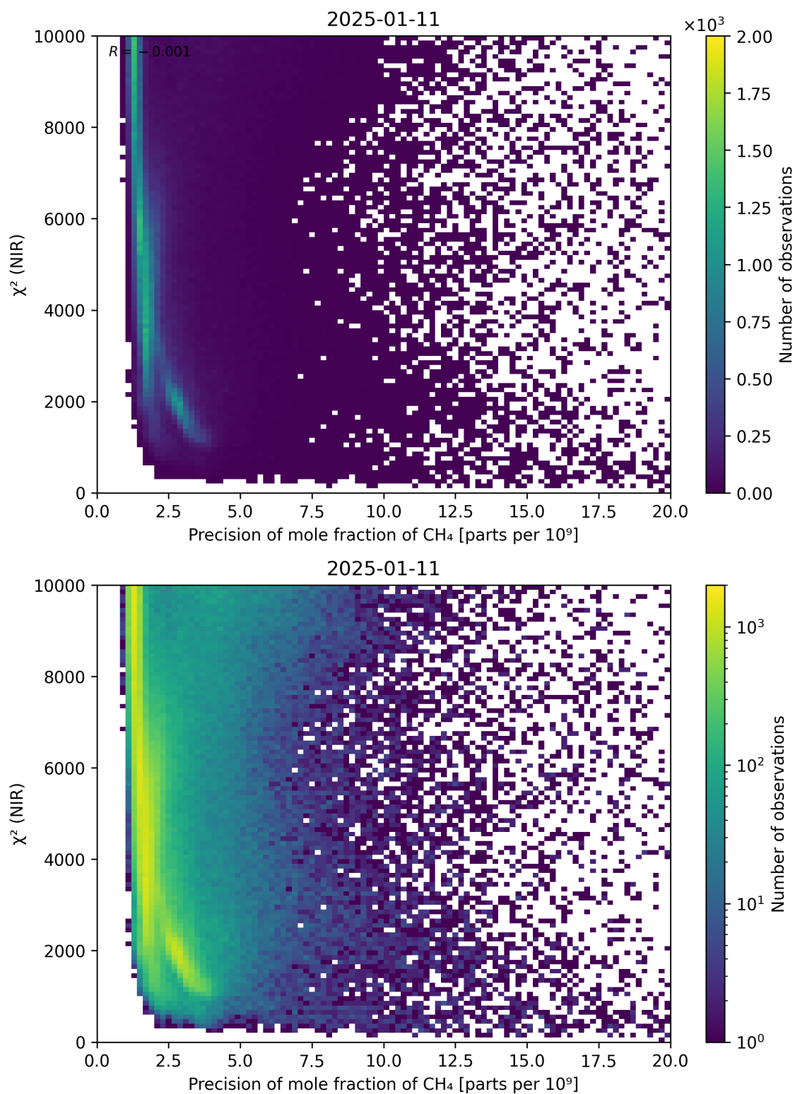
Figure 78: Scatter density plot of “Precision of mole fraction of CH 4 ” against “ \chi^2 (NIR)” for 2025-01-10 to 2025-01-12.
