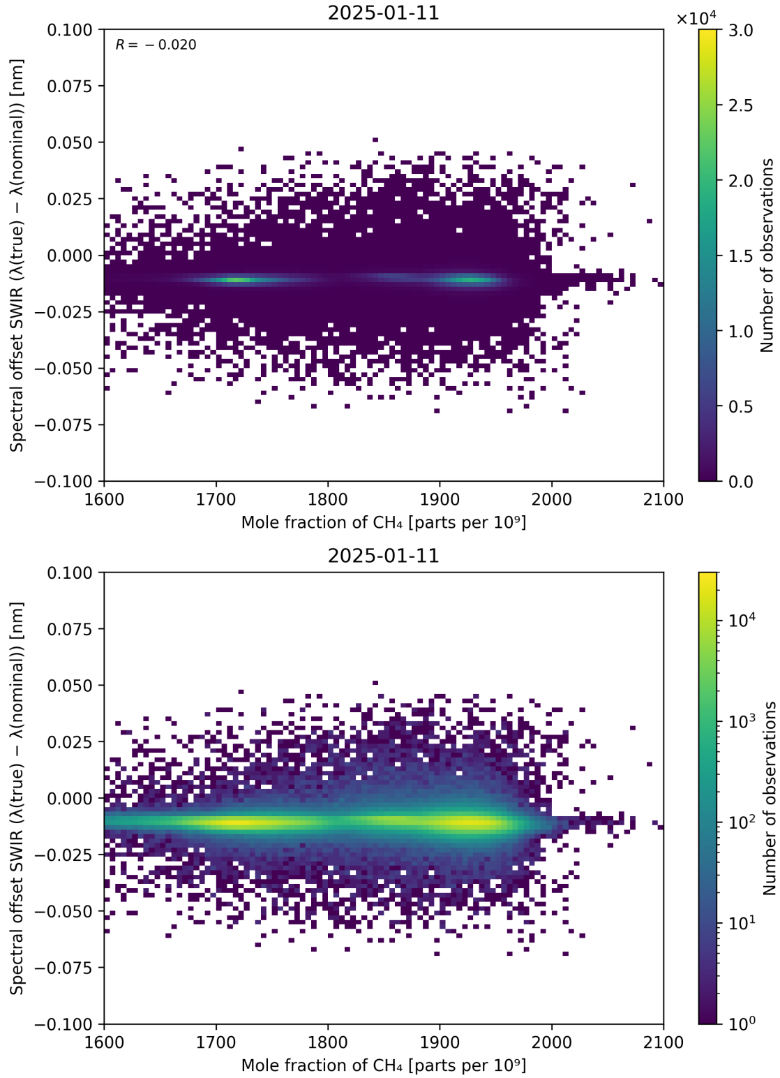
Figure 86: Scatter density plot of “Mole fraction of \text{CH}_4 ” against “Spectral offset SWIR ( \lambda_{\text{true}} - \lambda_{\text{nominal}} )” for 2025-01-10 to 2025-01-12.
