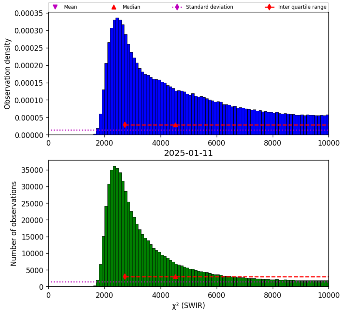
Figure 28: Histogram of “ \chi^2 (SWIR)” for 2025-01-10 to 2025-01-12
