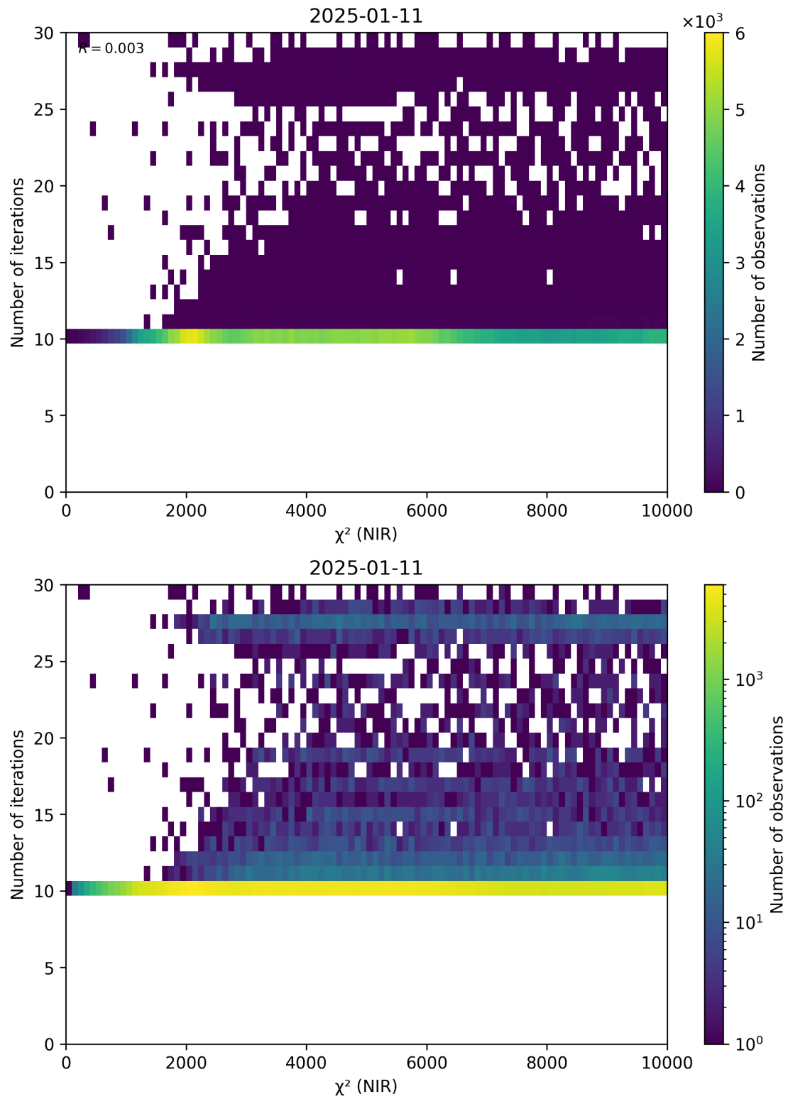
Figure 46: Scatter density plot of “ \chi^2 (NIR)” against “Number of iterations” for 2025-01-10 to 2025-01-12.
