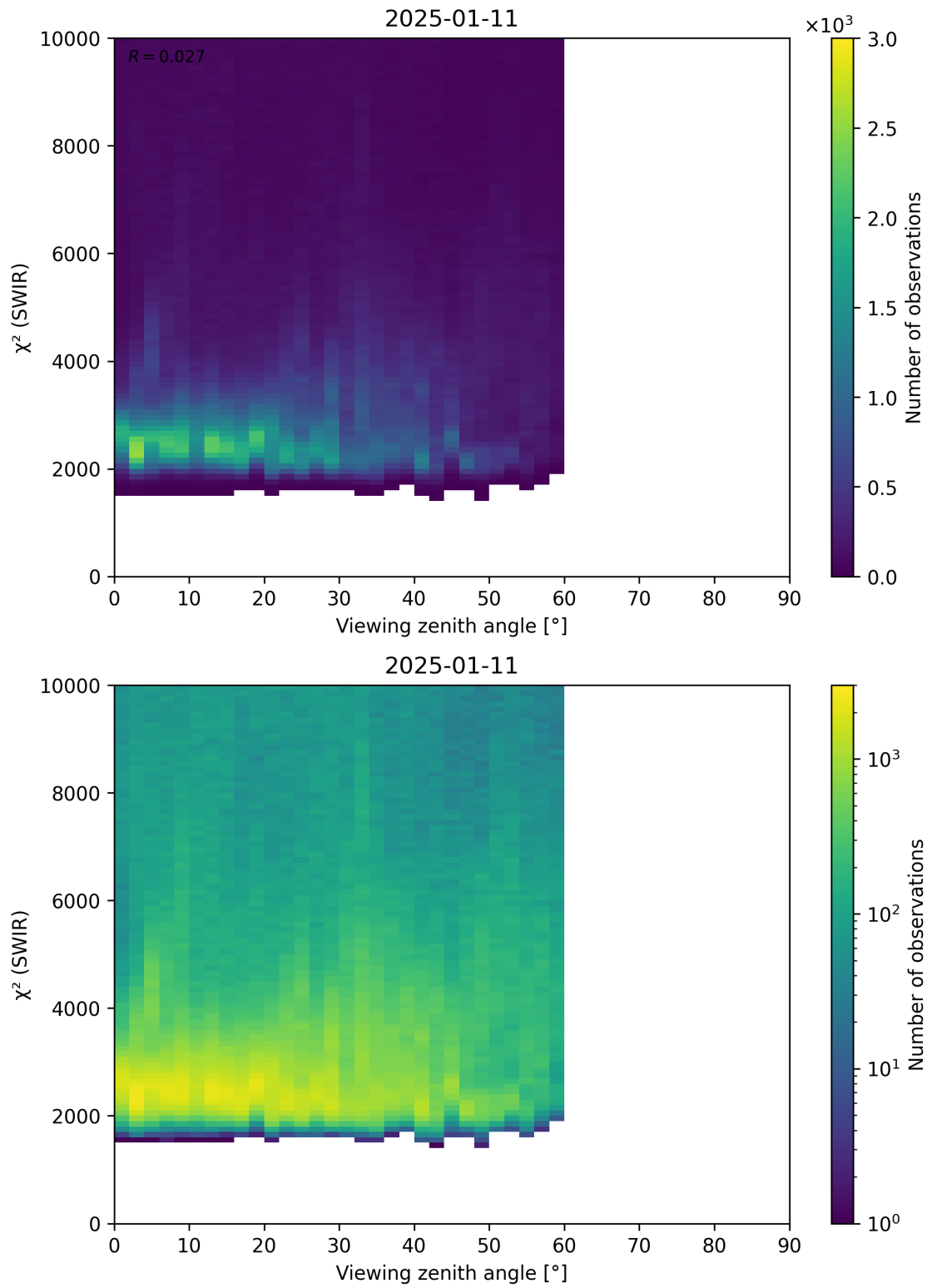
Figure 106: Scatter density plot of “Viewing zenith angle” against “ \chi^2 (SWIR)” for 2025-01-10 to 2025-01-12.
