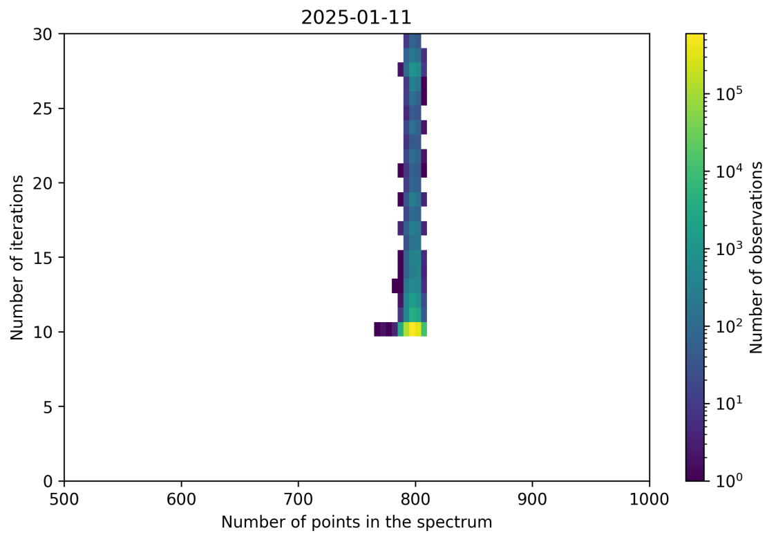
Figure 92: Scatter density plot of “Number of points in the spectrum” against “Number of iterations” for 2025-01-10 to 2025-01-12.
