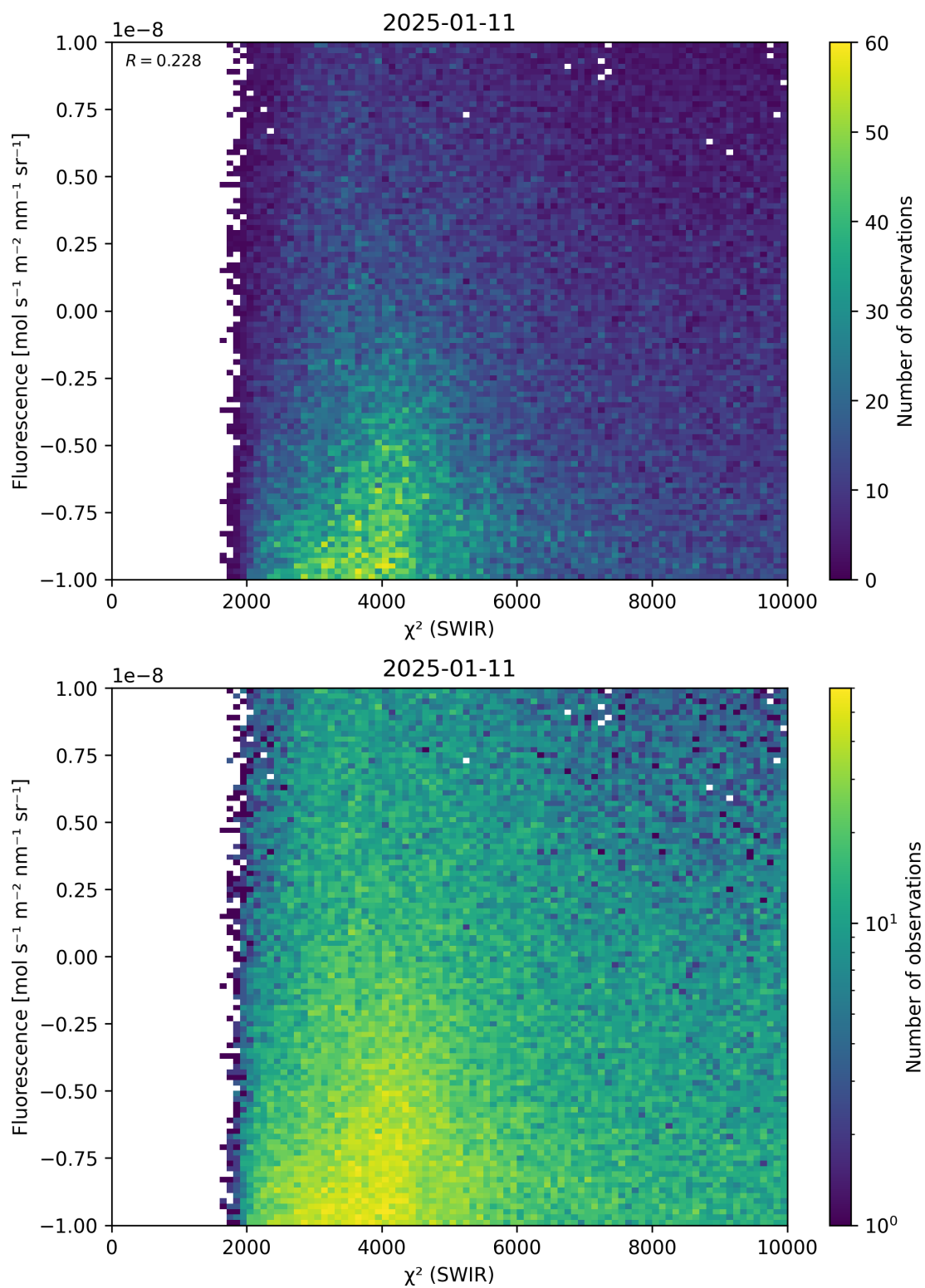
Figure 49: Scatter density plot of “ \chi^2 (SWIR)” against “Fluorescence” for 2025-01-10 to 2025-01-12.
