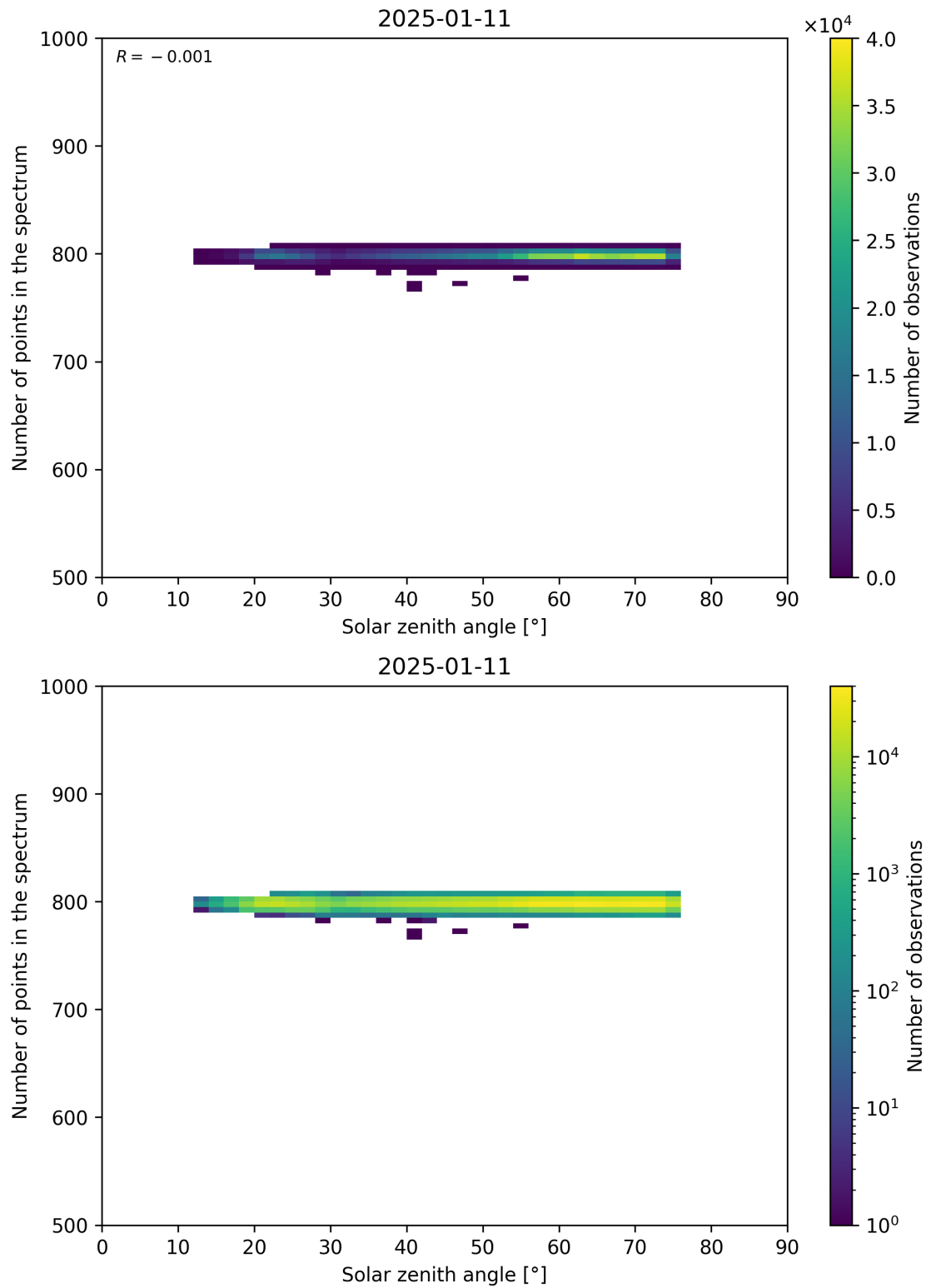
Figure 103: Scatter density plot of “Solar zenith angle” against “Number of points in the spectrum” for 2025-01-10 to 2025-01-12.
