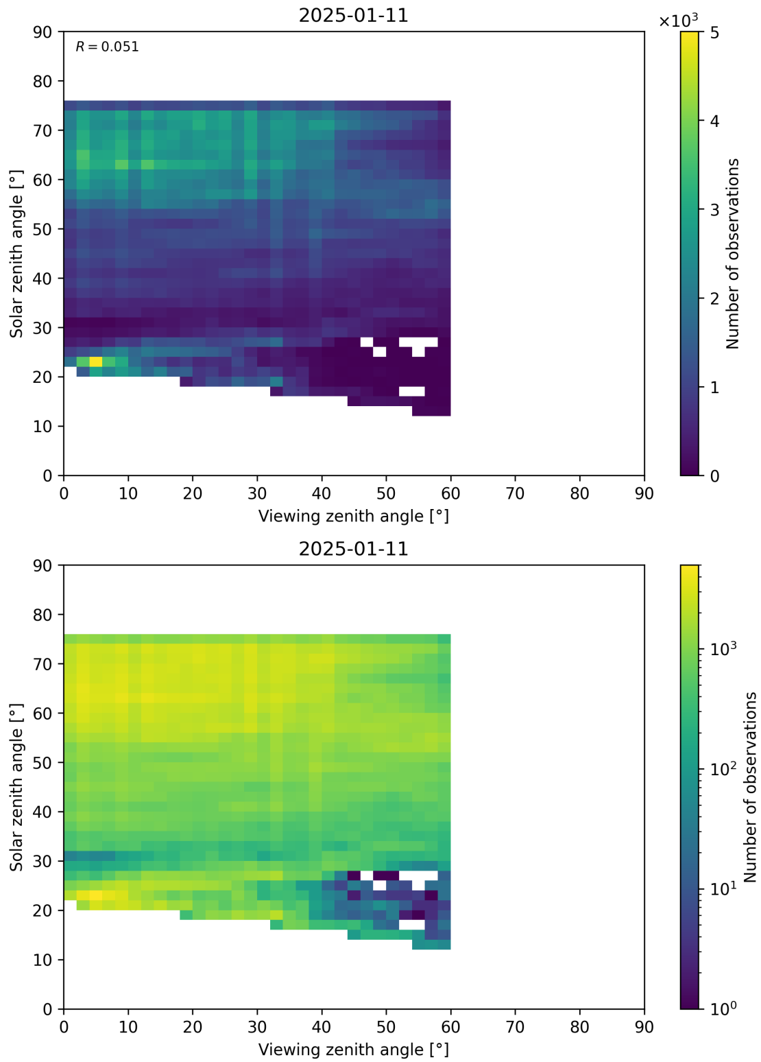
Figure 115: Scatter density plot of “Viewing zenith angle” against “Solar zenith angle” for 2025-01-10 to 2025-01-12.
