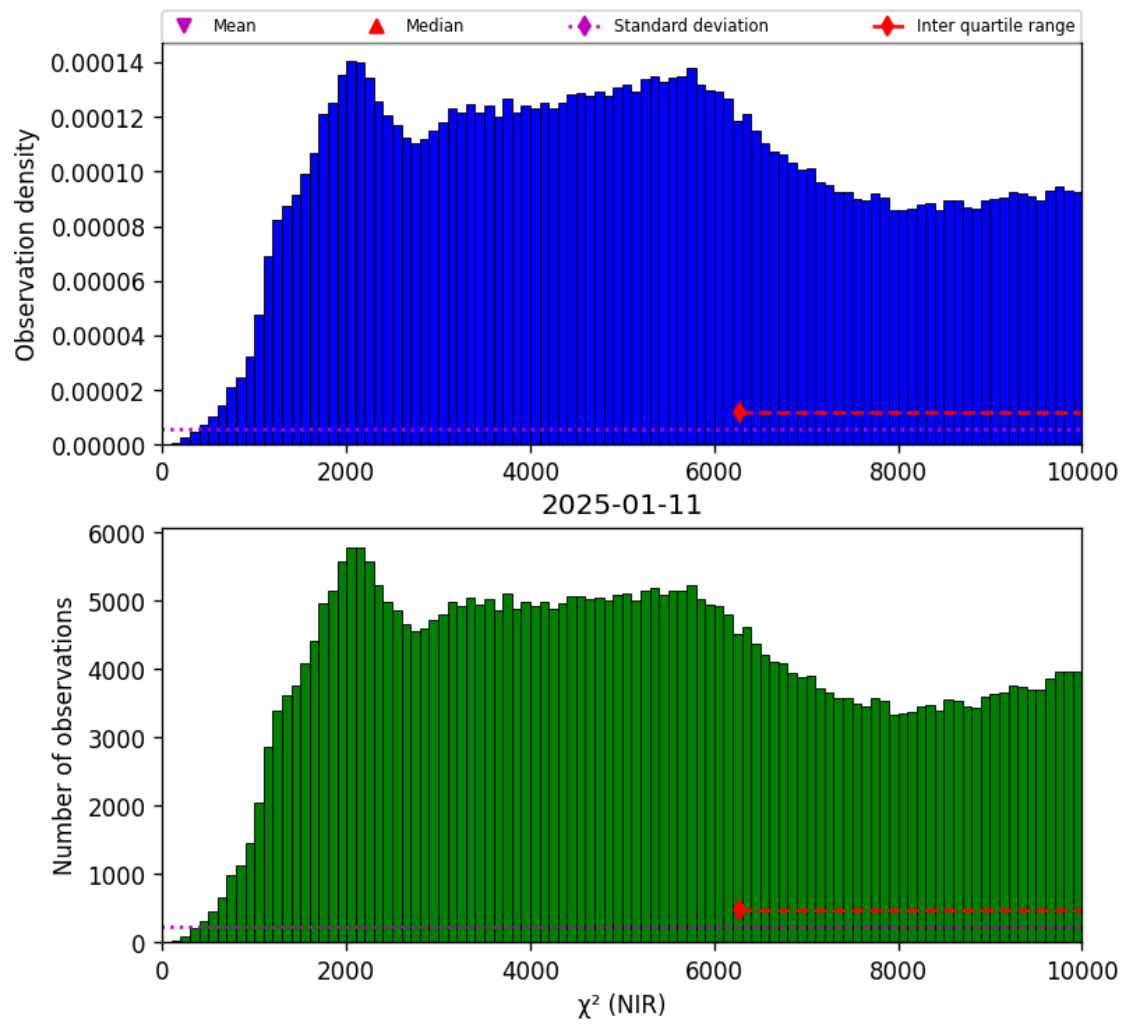
Figure 29: Histogram of “ \chi^2 (NIR)” for 2025-01-10 to 2025-01-12
