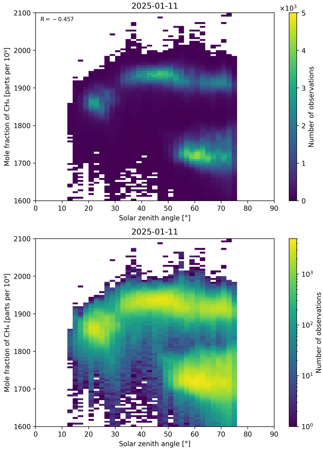
Figure 99: Scatter density plot of “Solar zenith angle” against “Mole fraction of CH 4 ” for 2025-01-10 to 2025-01-12.
