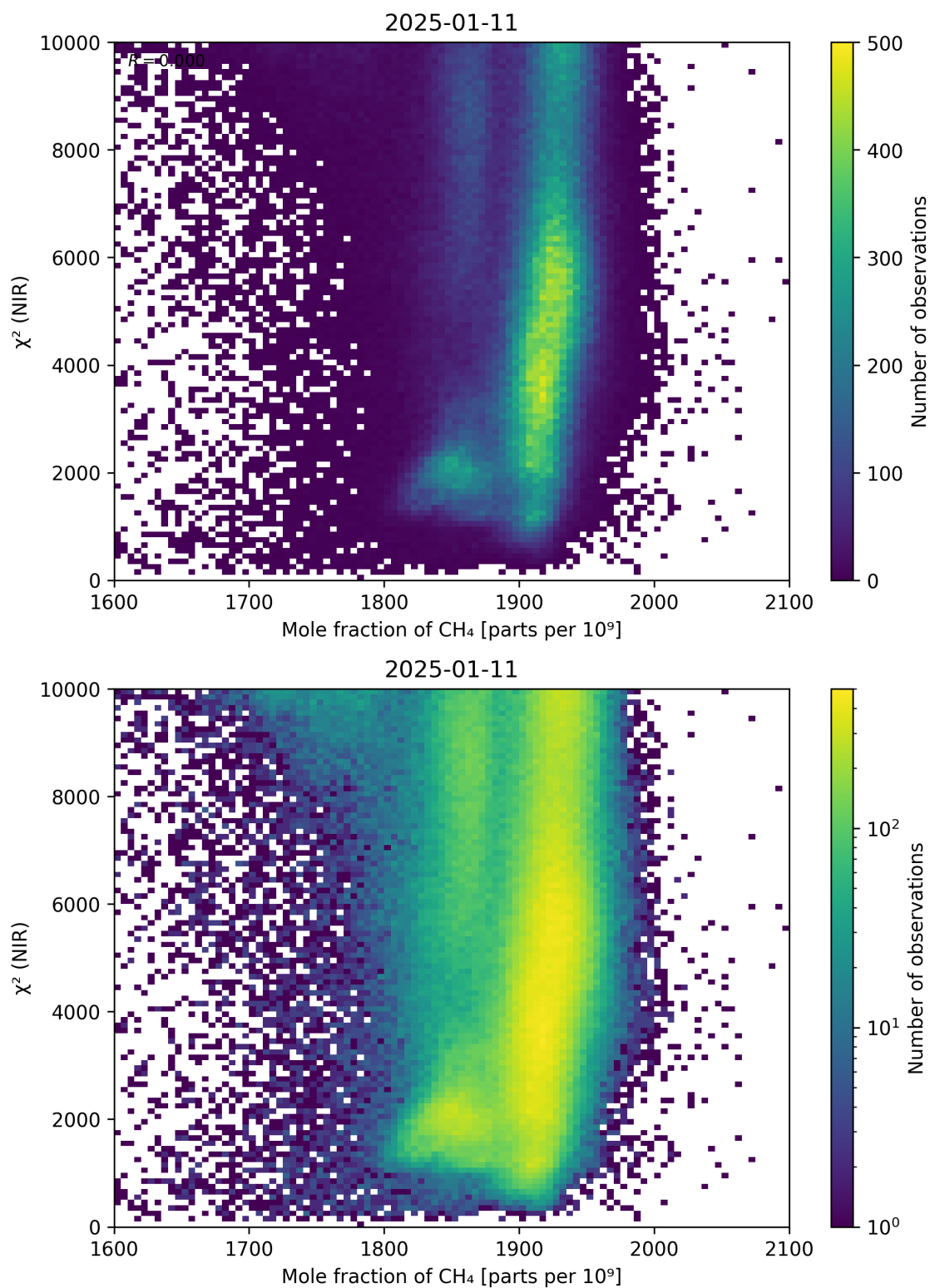
Figure 70: Scatter density plot of “Mole fraction of \text{CH}_4 ” against “ \chi^2 (NIR)” for 2025-01-10 to 2025-01-12.
