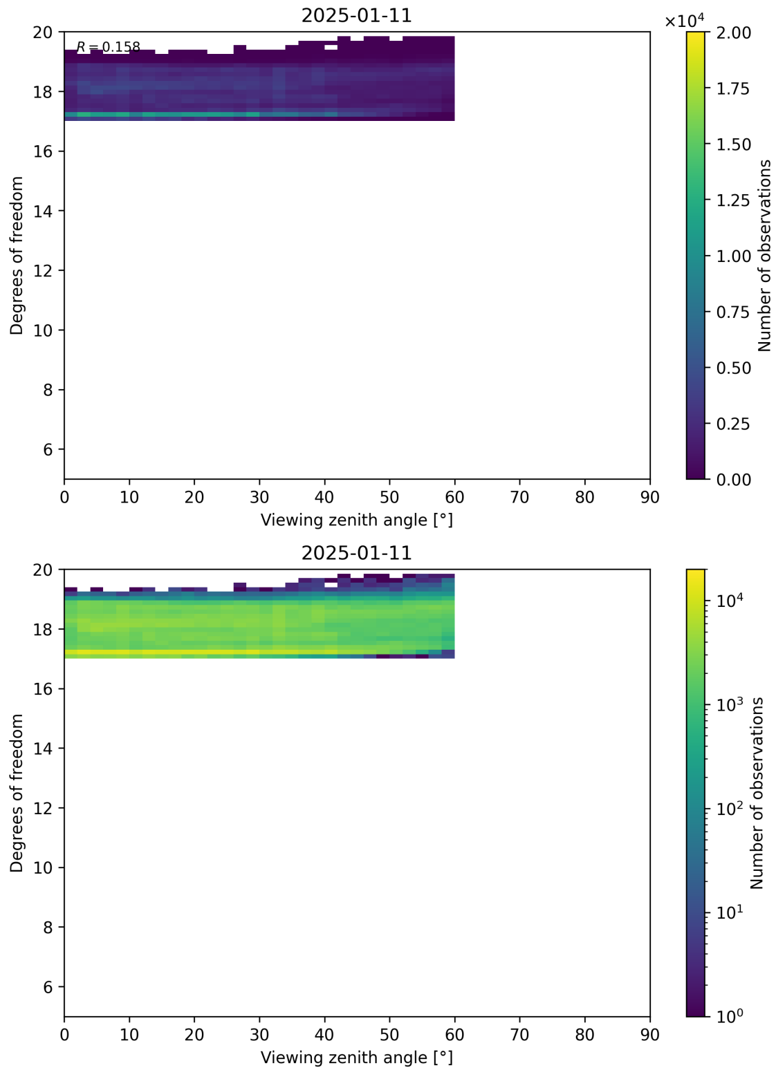
Figure 107: Scatter density plot of “Viewing zenith angle” against “Degrees of freedom” for 2025-01-10 to 2025-01-12.
