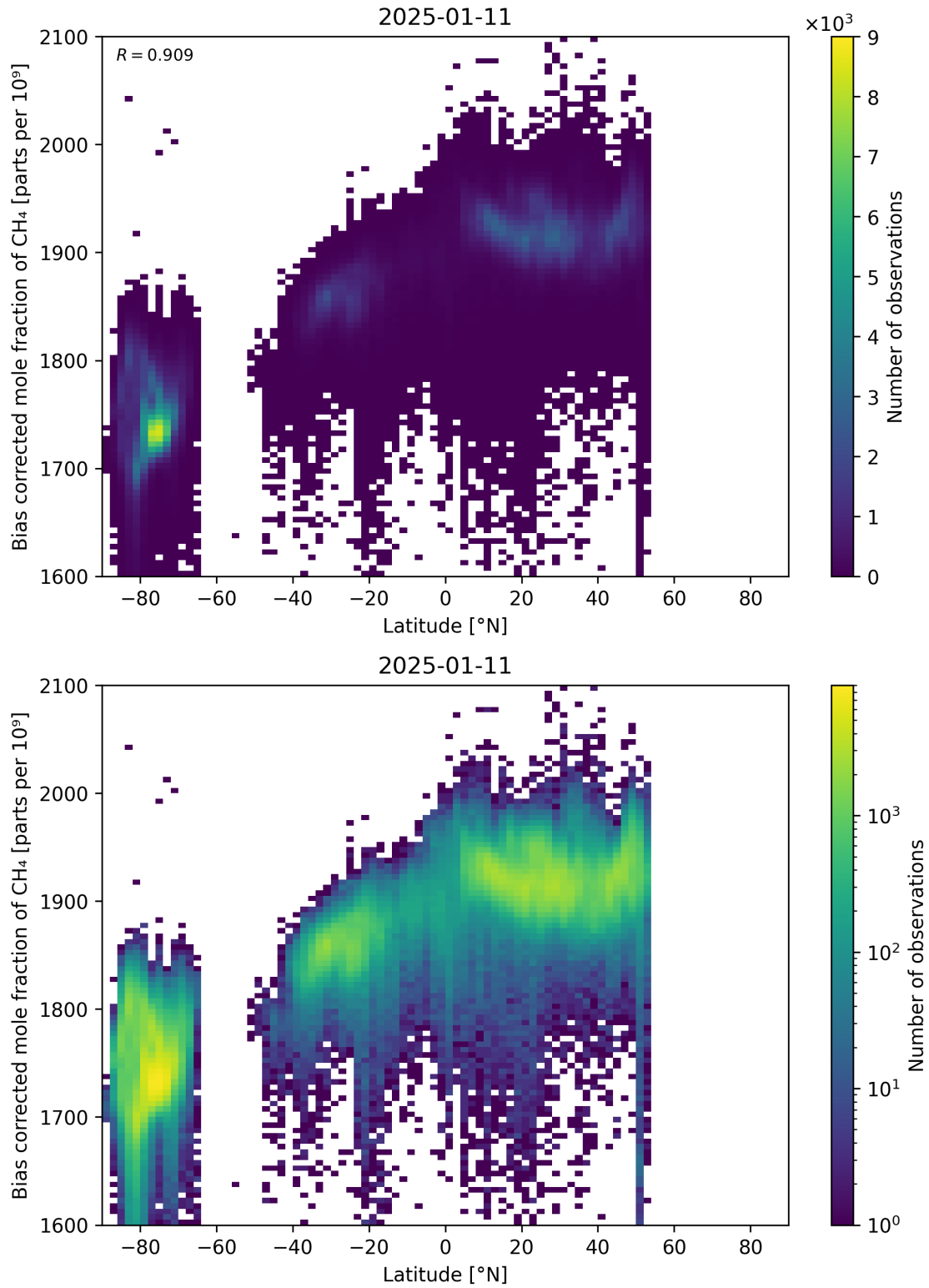
Figure 58: Scatter density plot of “Latitude” against “Bias corrected mole fraction of CH 4 ” for 2025-01-10 to 2025-01-12.
