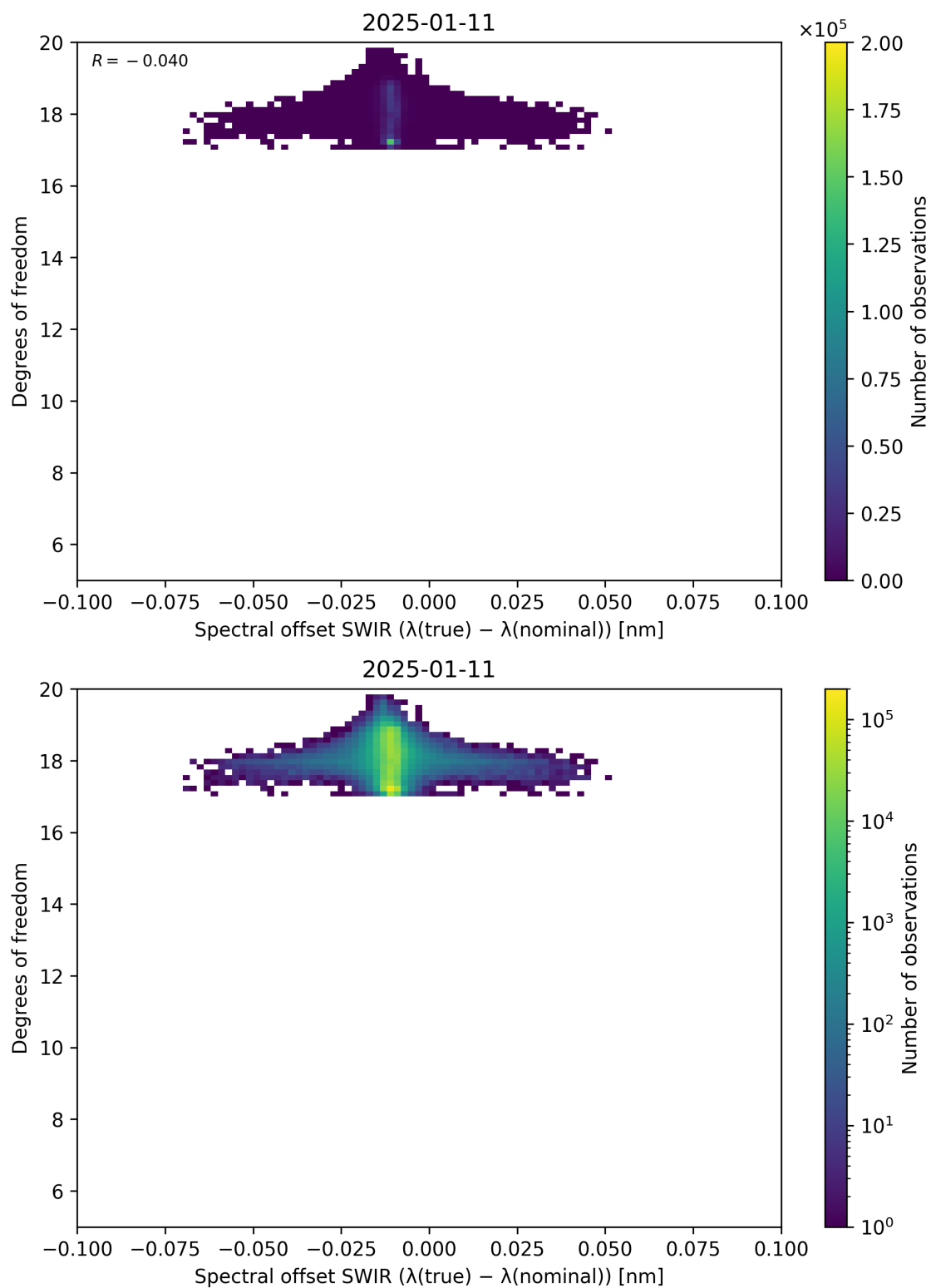
Figure 119: Scatter density plot of “Spectral offset SWIR ( \lambda_{\text{true}} - \lambda_{\text{nominal}} )” against “Degrees of freedom” for 2025-01-10 to 2025-01-12.
