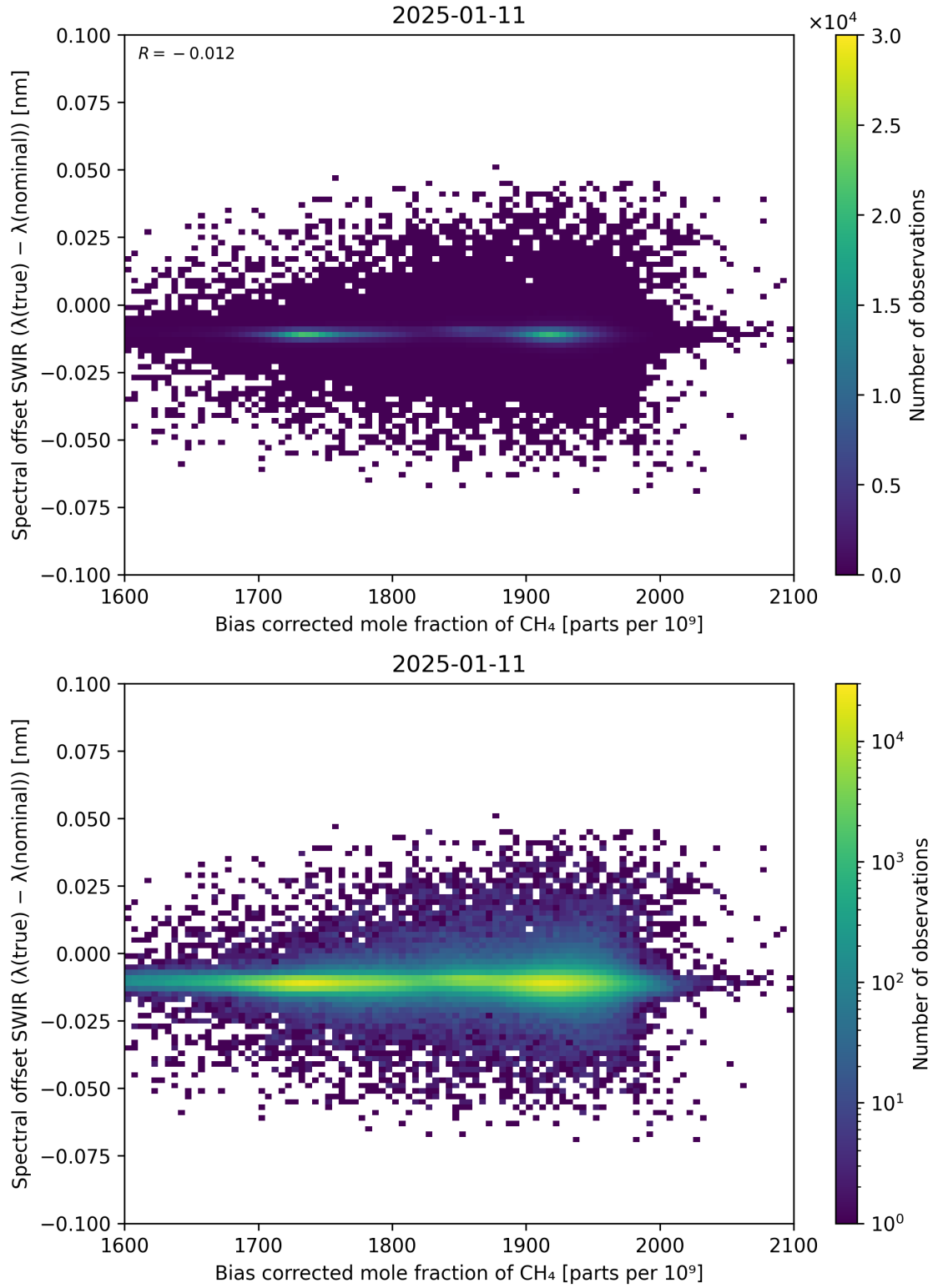
Figure 69: Scatter density plot of “Bias corrected mole fraction of \text{CH}_4 ” against “Spectral offset SWIR ( \lambda_{\text{true}} - \lambda_{\text{nominal}} )” for 2025-01-10 to 2025-01-12.
