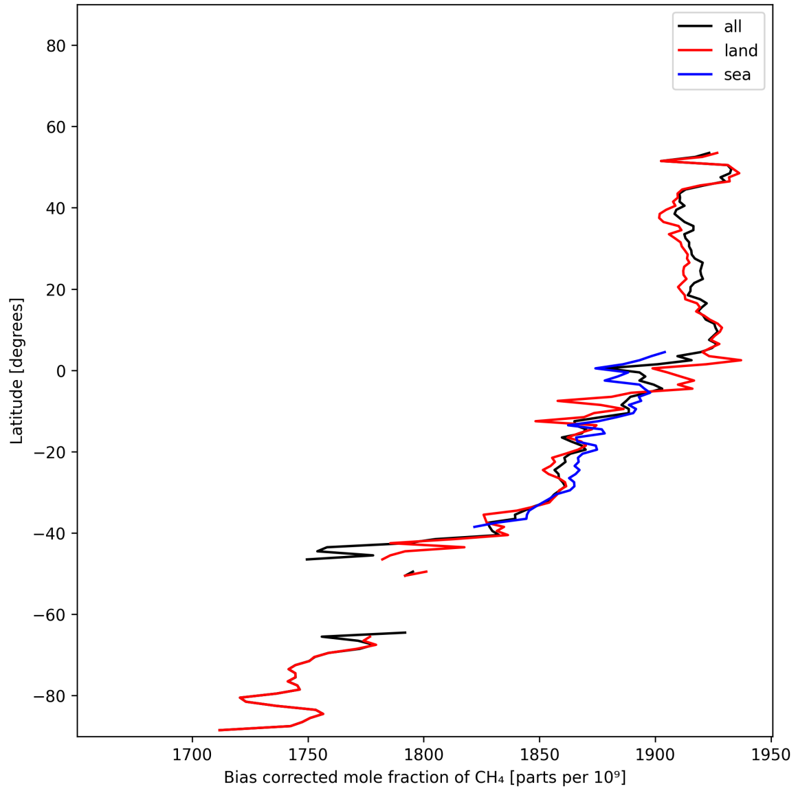
Figure 14: Zonal average of “Bias corrected mole fraction of CH 4 ” for 2025-01-10 to 2025-01-12.
