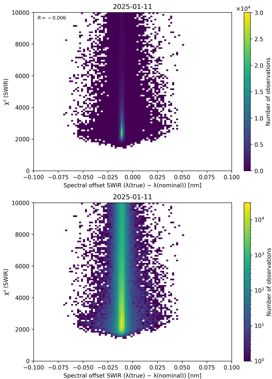
Figure 118: Scatter density plot of “Spectral offset SWIR ( \lambda_{\text{true}} - \lambda_{\text{nominal}} )” against “ \chi^2 (SWIR)” for 2025-01-10 to 2025-01-12.
