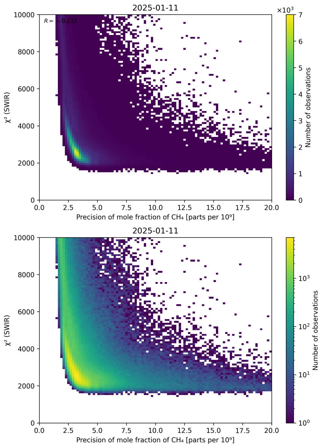
Figure 79: Scatter density plot of “Precision of mole fraction of CH 4 ” against “ \chi^2 (SWIR)” for 2025-01-10 to 2025-01-12.
