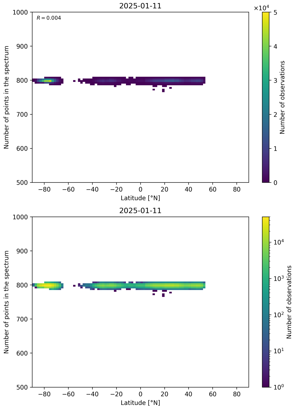
Figure 61: Scatter density plot of “Latitude” against “Number of points in the spectrum” for 2025-01-10 to 2025-01-12.
