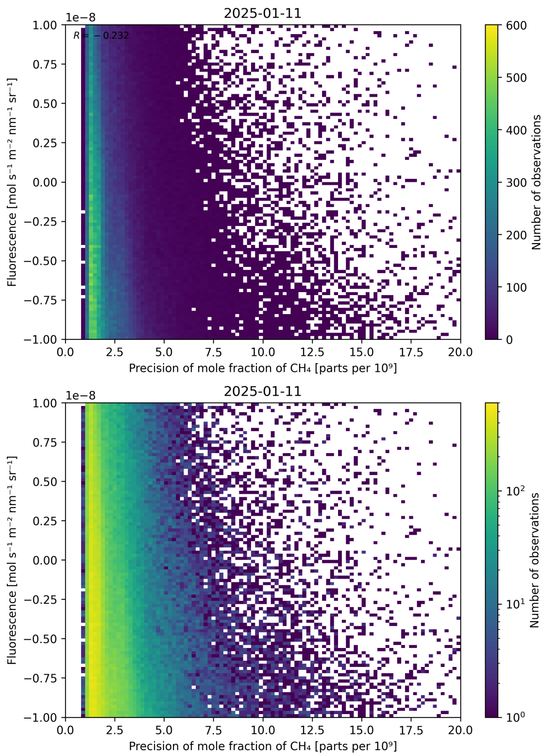
Figure 81: Scatter density plot of “Precision of mole fraction of CH 4 ” against “Fluorescence” for 2025-01-10 to 2025-01-12.
