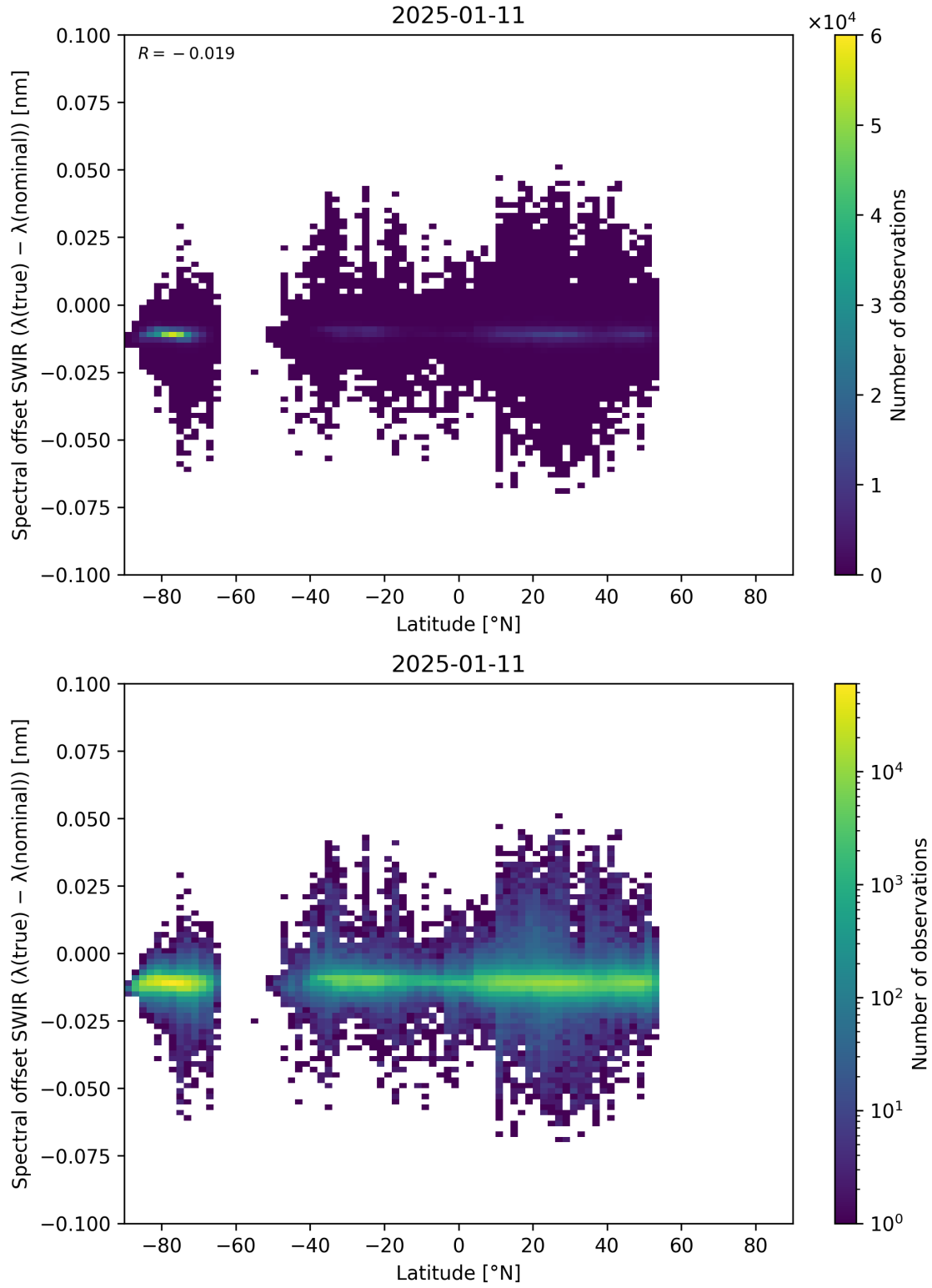
Figure 62: Scatter density plot of “Latitude” against “Spectral offset SWIR ( \lambda_{\text{true}} - \lambda_{\text{nominal}} )” for 2025-01-10 to 2025-01-12.
