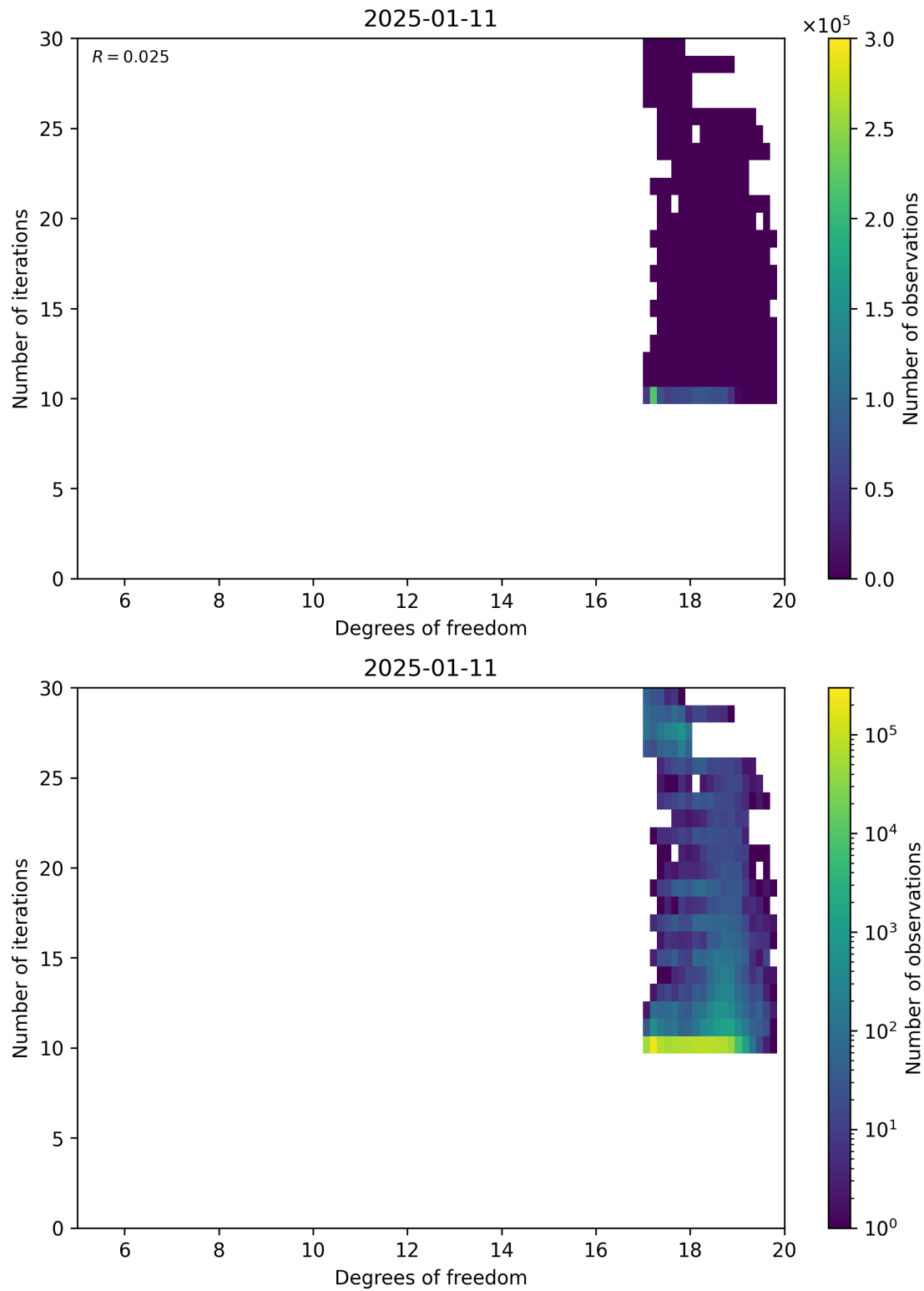
Figure 52: Scatter density plot of “Degrees of freedom” against “Number of iterations” for 2025-01-10 to 2025-01-12.
