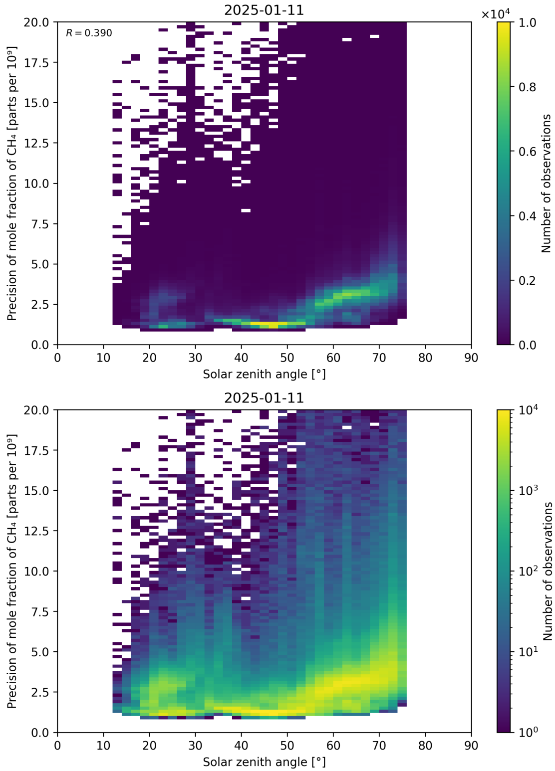
Figure 101: Scatter density plot of “Solar zenith angle” against “Precision of mole fraction of \text{CH}_4 ” for 2025-01-10 to 2025-01-12.
