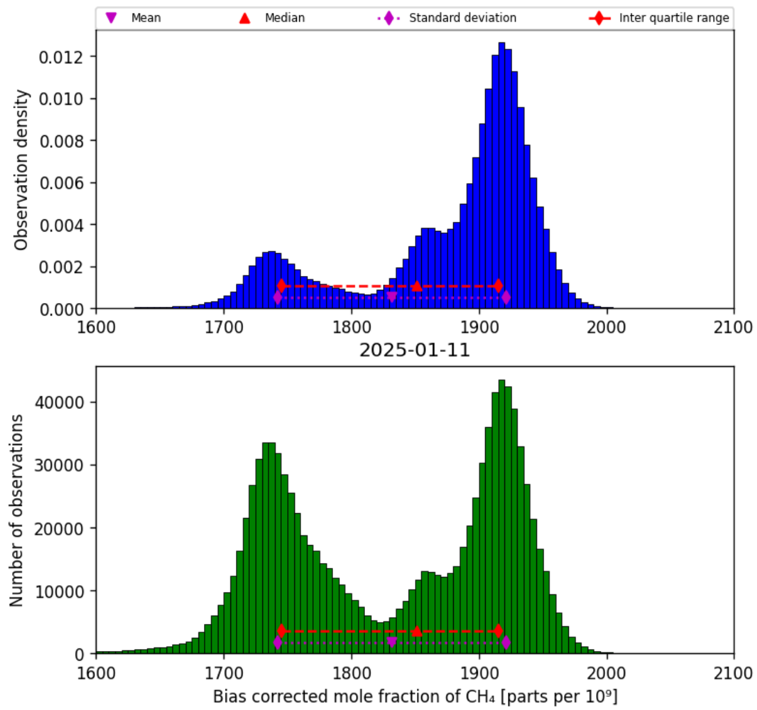
Figure 25: Histogram of “Bias corrected mole fraction of CH 4 ” for 2025-01-10 to 2025-01-12
