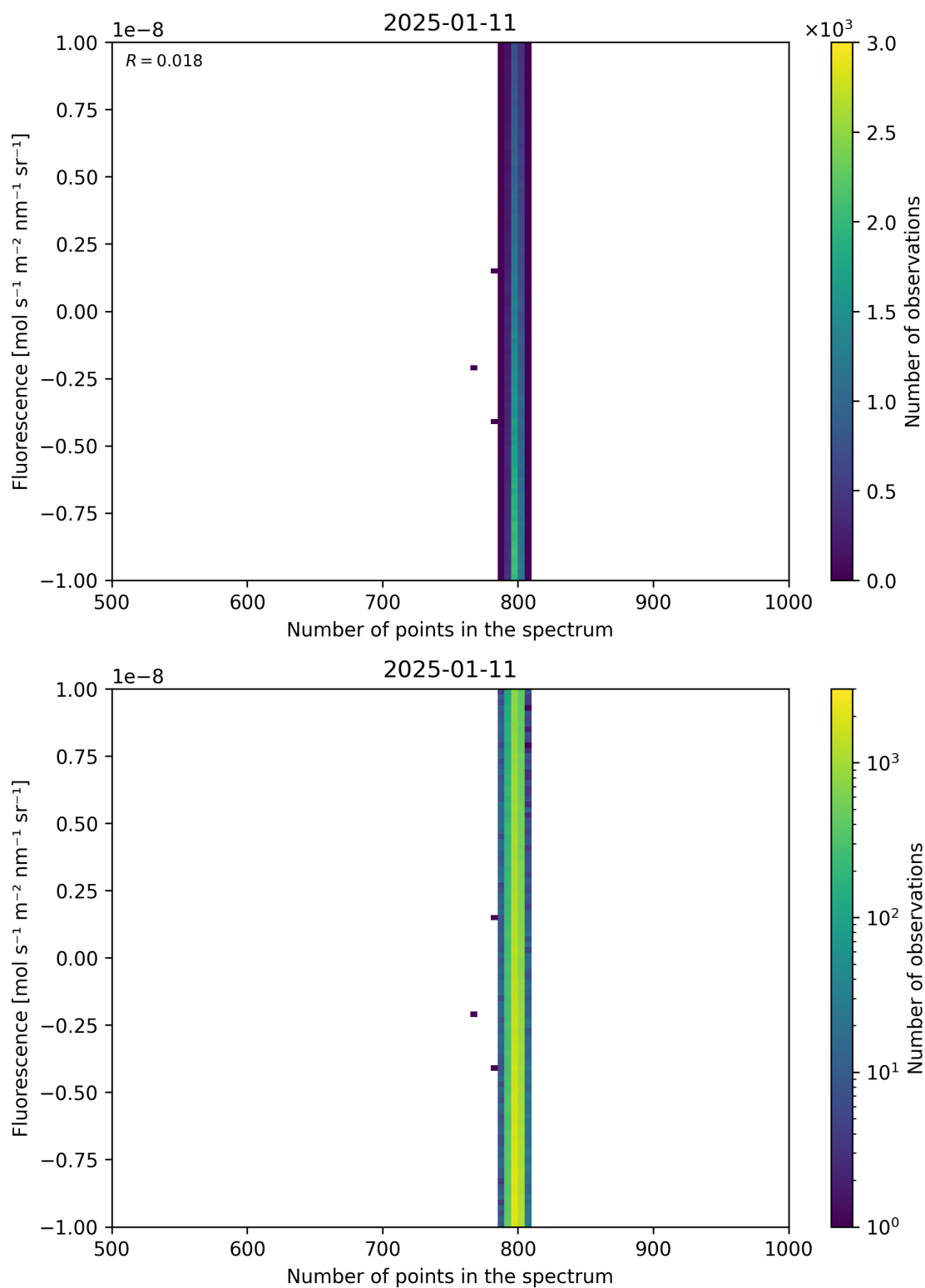
Figure 91: Scatter density plot of “Number of points in the spectrum” against “Fluorescence” for 2025-01-10 to 2025-01-12.
