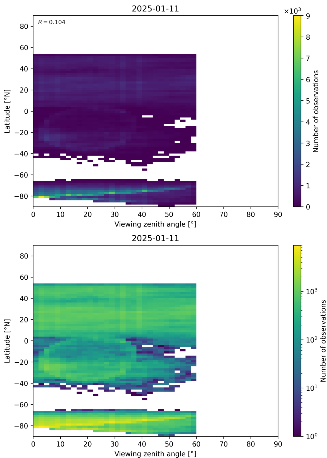
Figure 109: Scatter density plot of “Viewing zenith angle” against “Latitude” for 2025-01-10 to 2025-01-12.
