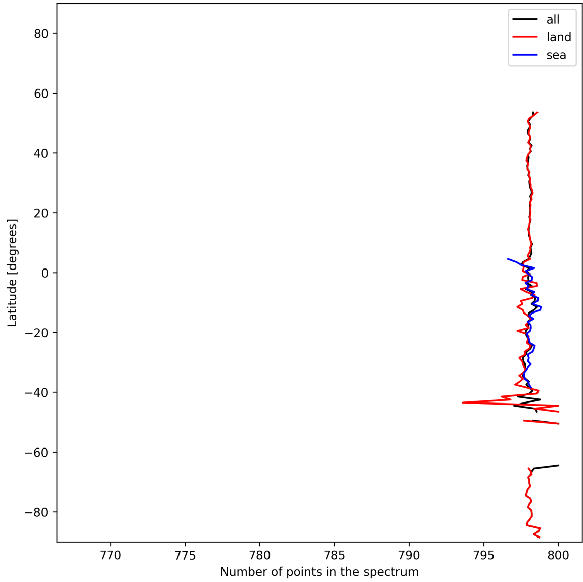
Figure 15: Zonal average of “Number of points in the spectrum” for 2025-01-10 to 2025-01-12.
