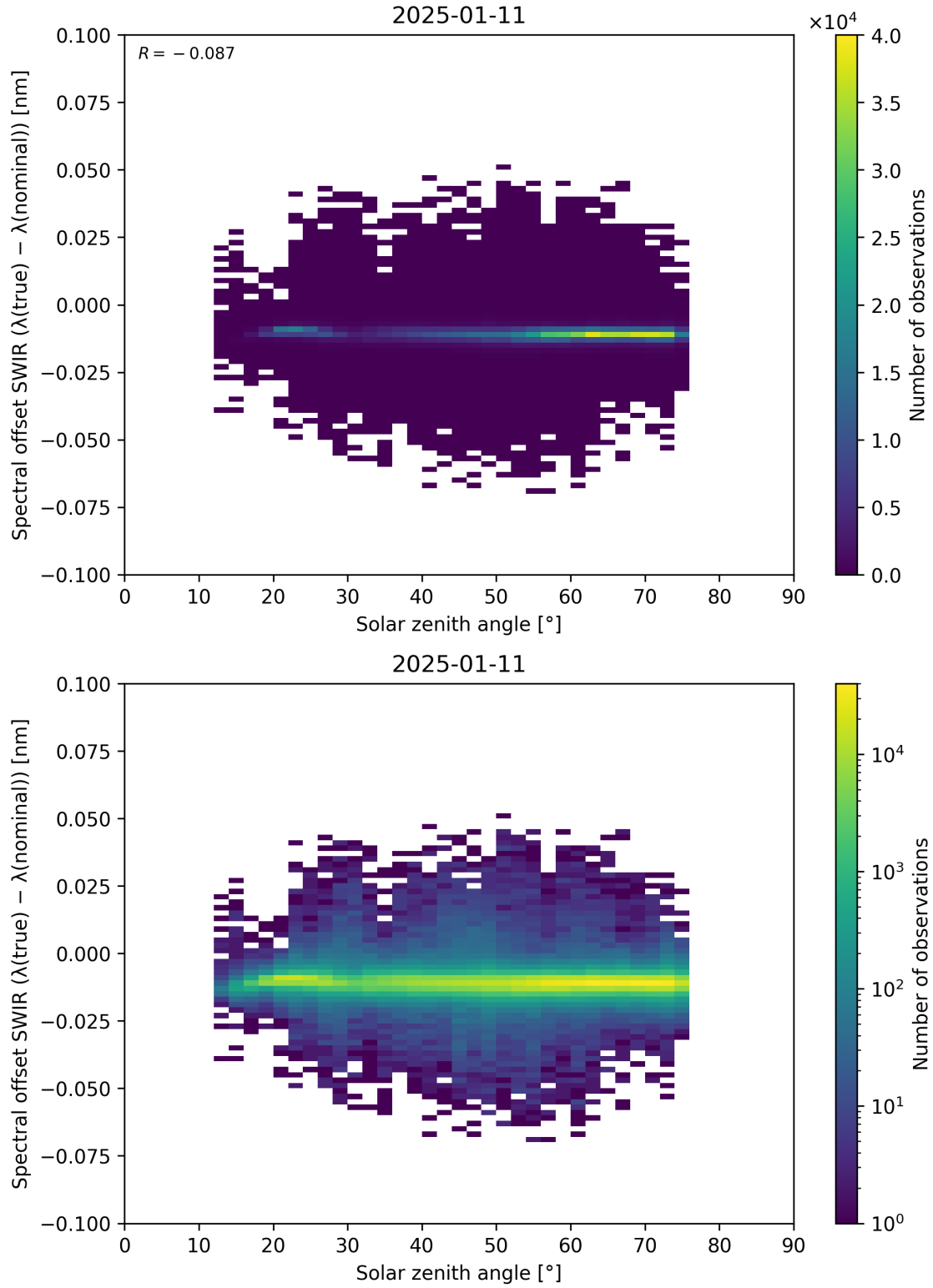
Figure 104: Scatter density plot of “Solar zenith angle” against “Spectral offset SWIR ( \lambda_{\text{true}} - \lambda_{\text{nominal}} )” for 2025-01-10 to 2025-01-12.
