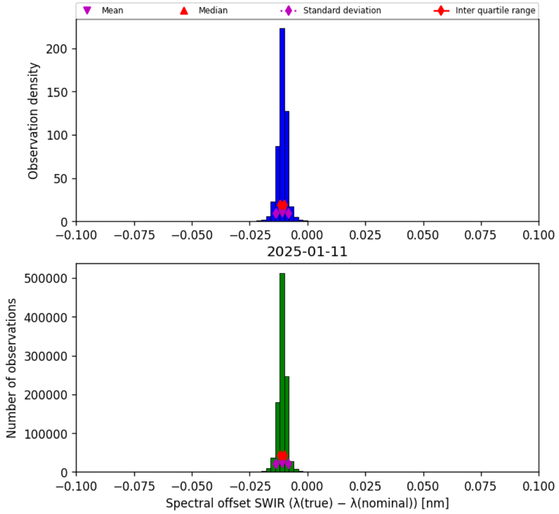
Figure 27: Histogram of “Spectral offset SWIR ( \lambda_{\text{true}} - \lambda_{\text{nominal}} )” for 2025-01-10 to 2025-01-12
