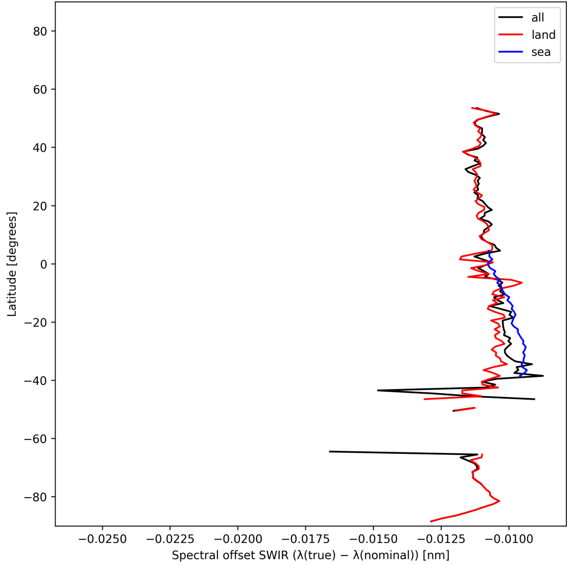
Figure 16: Zonal average of “Spectral offset SWIR ( \lambda_{\text{true}} - \lambda_{\text{nominal}} )” for 2025-01-10 to 2025-01-12.
