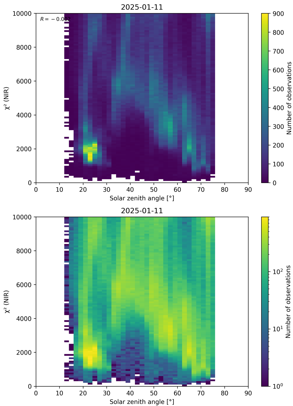
Figure 94: Scatter density plot of “Solar zenith angle” against “ \chi^2 (NIR)” for 2025-01-10 to 2025-01-12.
