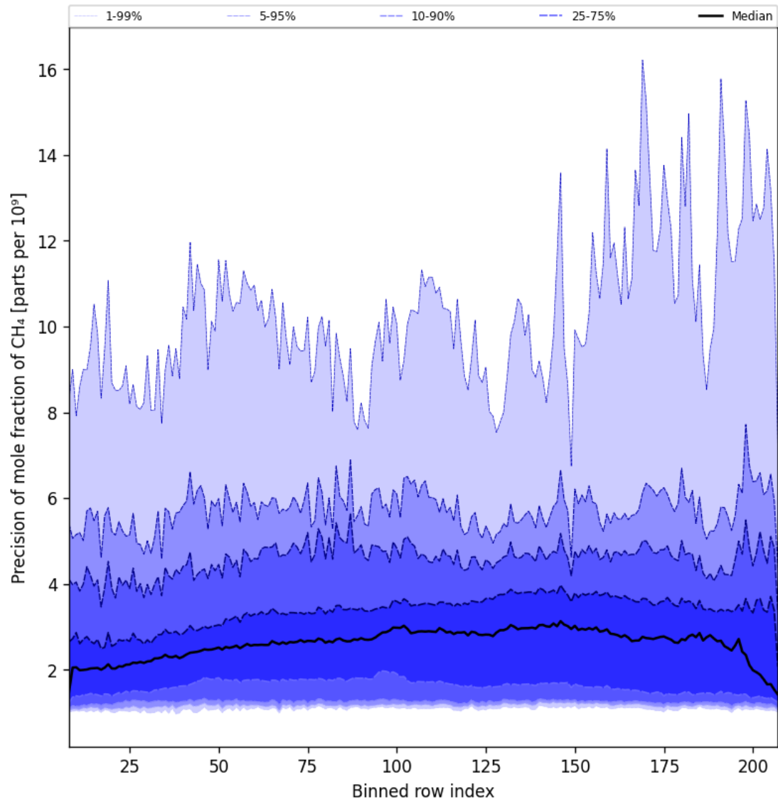
Figure 35: Along track statistics of “Precision of mole fraction of CH 4 ” for 2025-01-10 to 2025-01-12
