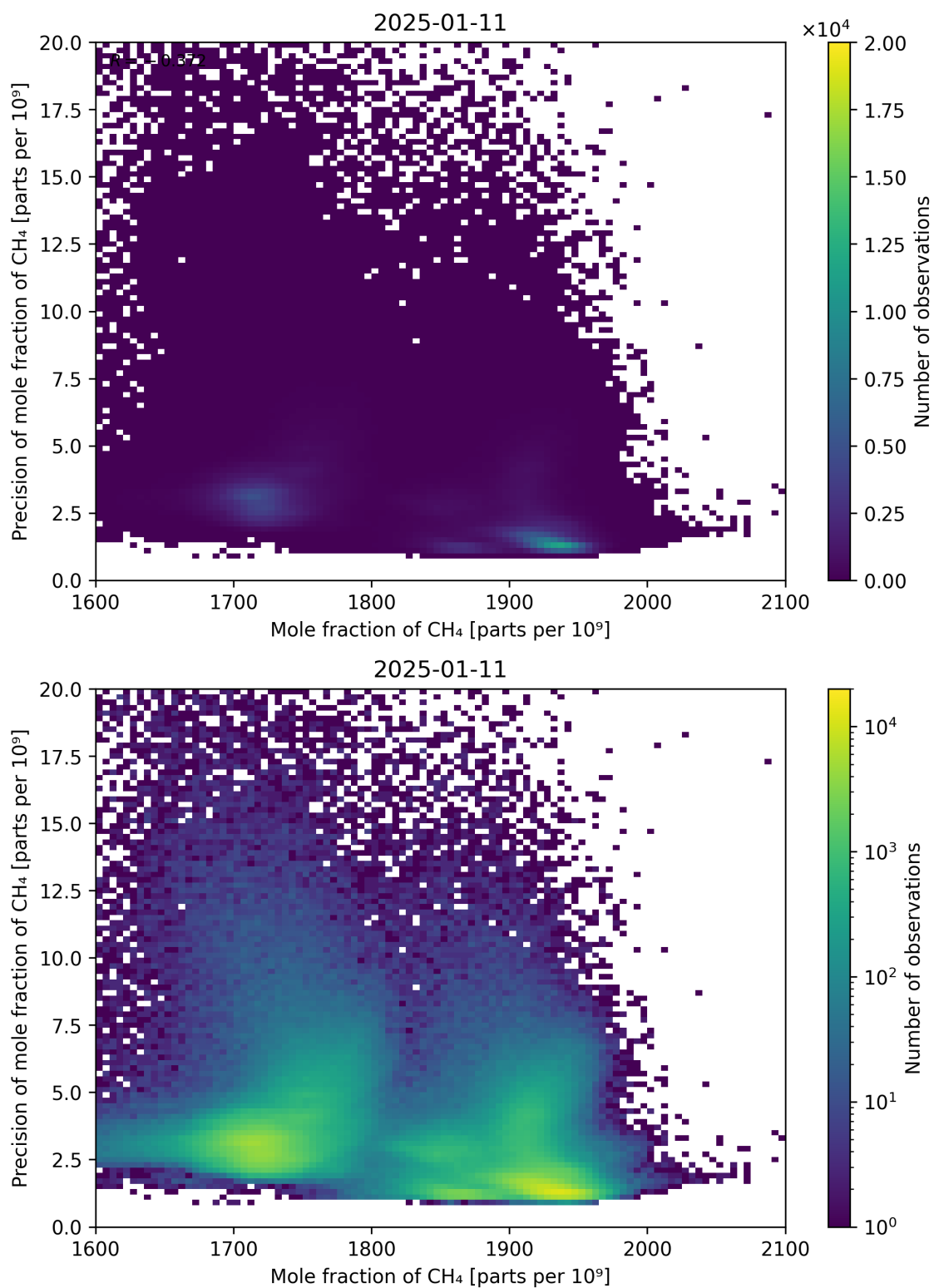
Figure 75: Scatter density plot of “Mole fraction of CH 4 ” against “Precision of mole fraction of CH 4 ” for 2025-01-10 to 2025-01-12.
