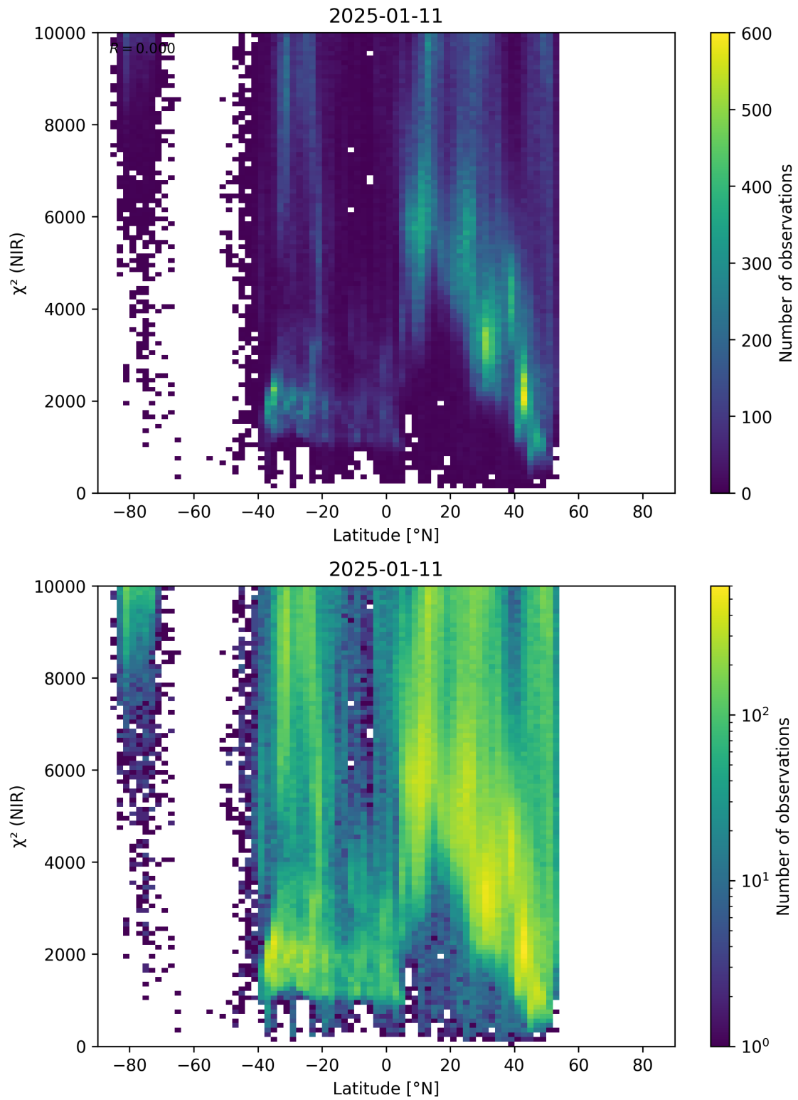
Figure 53: Scatter density plot of “Latitude” against “ \chi^2 (NIR)” for 2025-01-10 to 2025-01-12.
