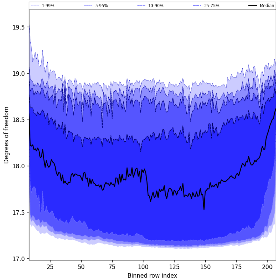
Figure 41: Along track statistics of “Degrees of freedom” for 2025-01-10 to 2025-01-12
