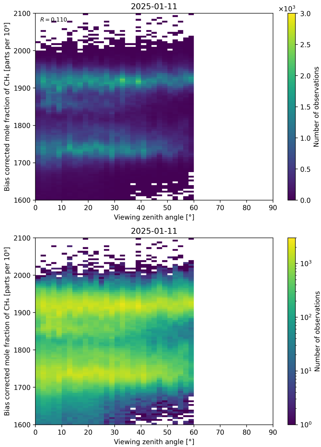
Figure 111: Scatter density plot of “Viewing zenith angle” against “Bias corrected mole fraction of CH 4 ” for 2025-01-10 to 2025-01-12.
