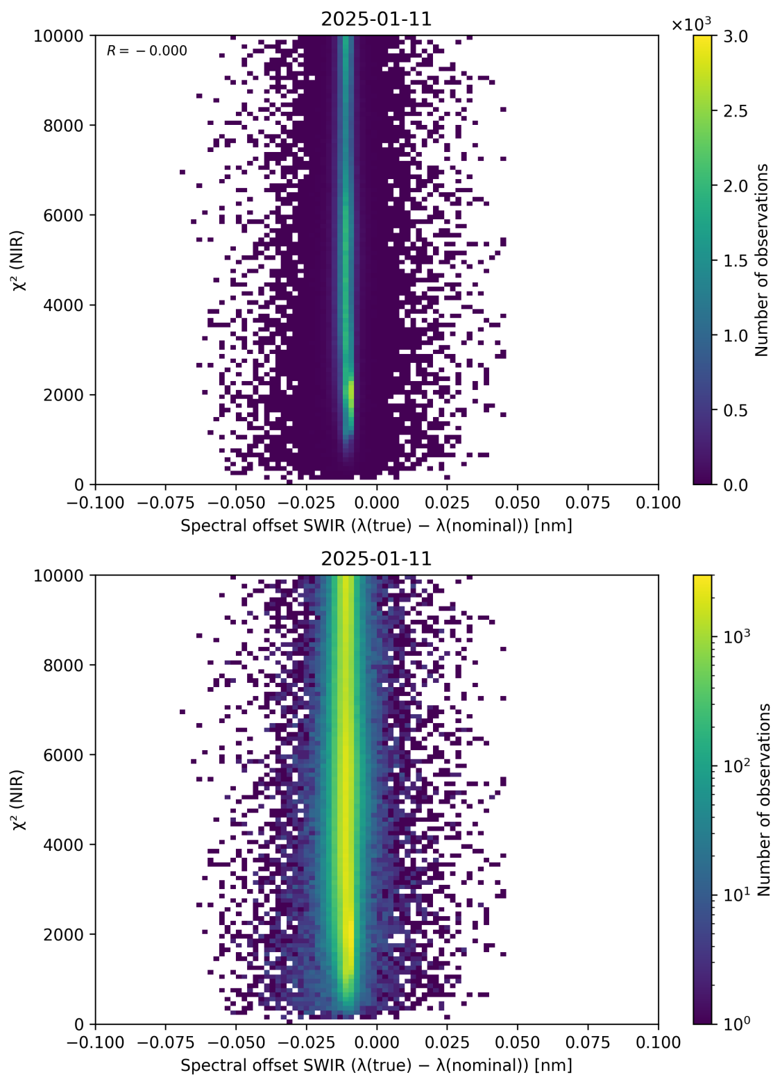
Figure 117: Scatter density plot of “Spectral offset SWIR ( \lambda_{\text{true}} - \lambda_{\text{nominal}} )” against “ \chi^2 (NIR)” for 2025-01-10 to 2025-01-12.
