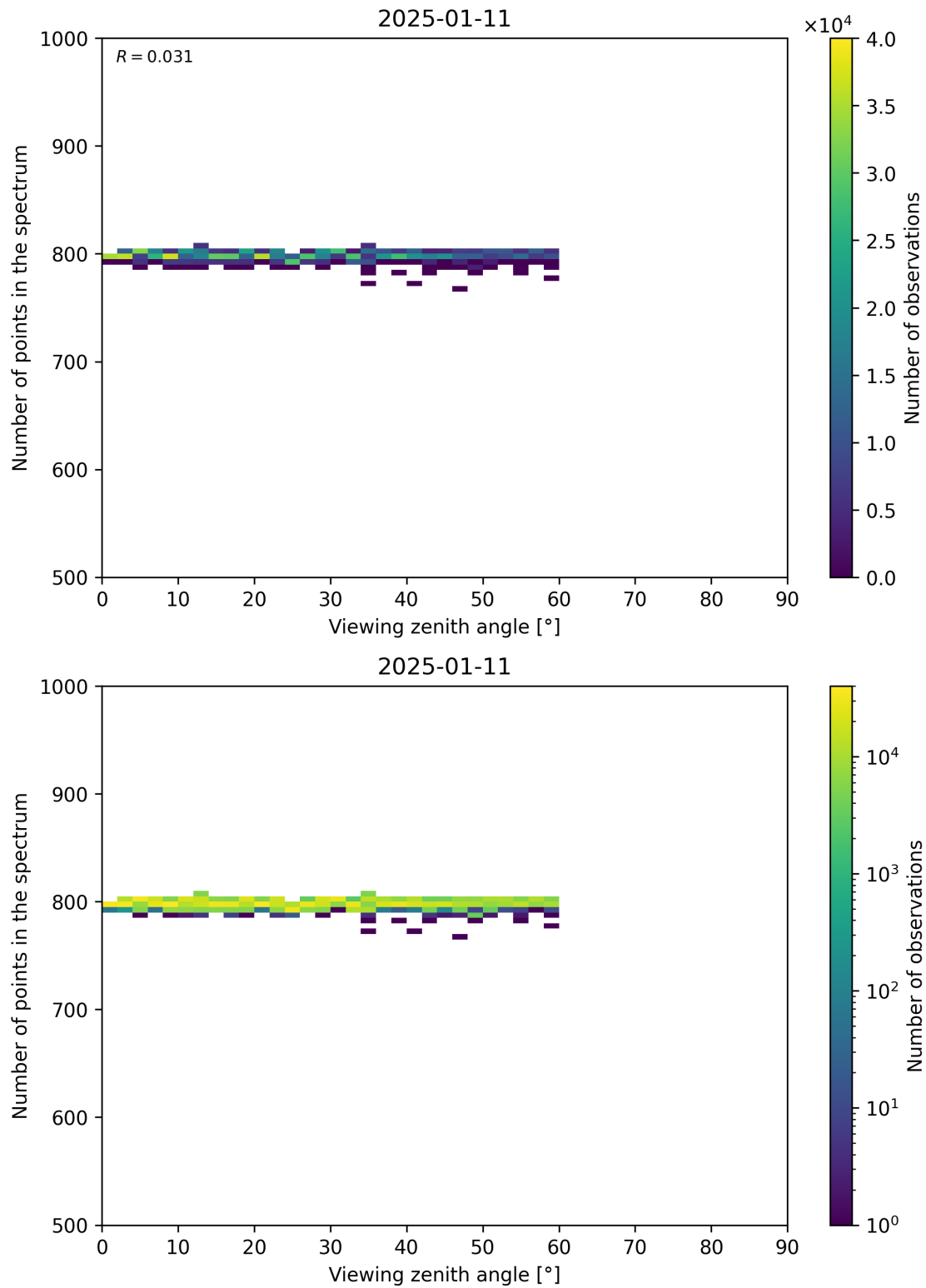
Figure 114: Scatter density plot of “Viewing zenith angle” against “Number of points in the spectrum” for 2025-01-10 to 2025-01-12.
