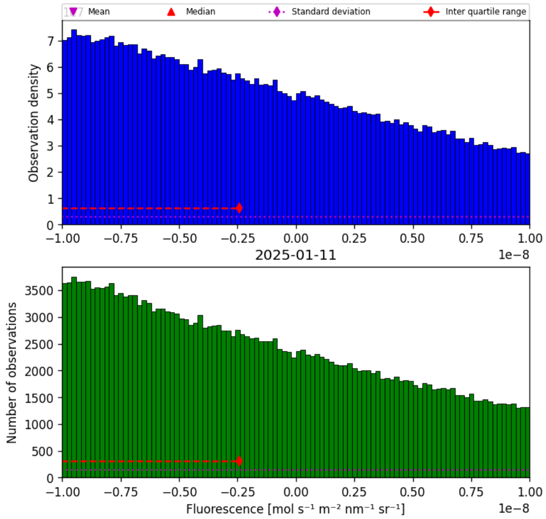
Figure 32: Histogram of “Fluorescence” for 2025-01-10 to 2025-01-12
