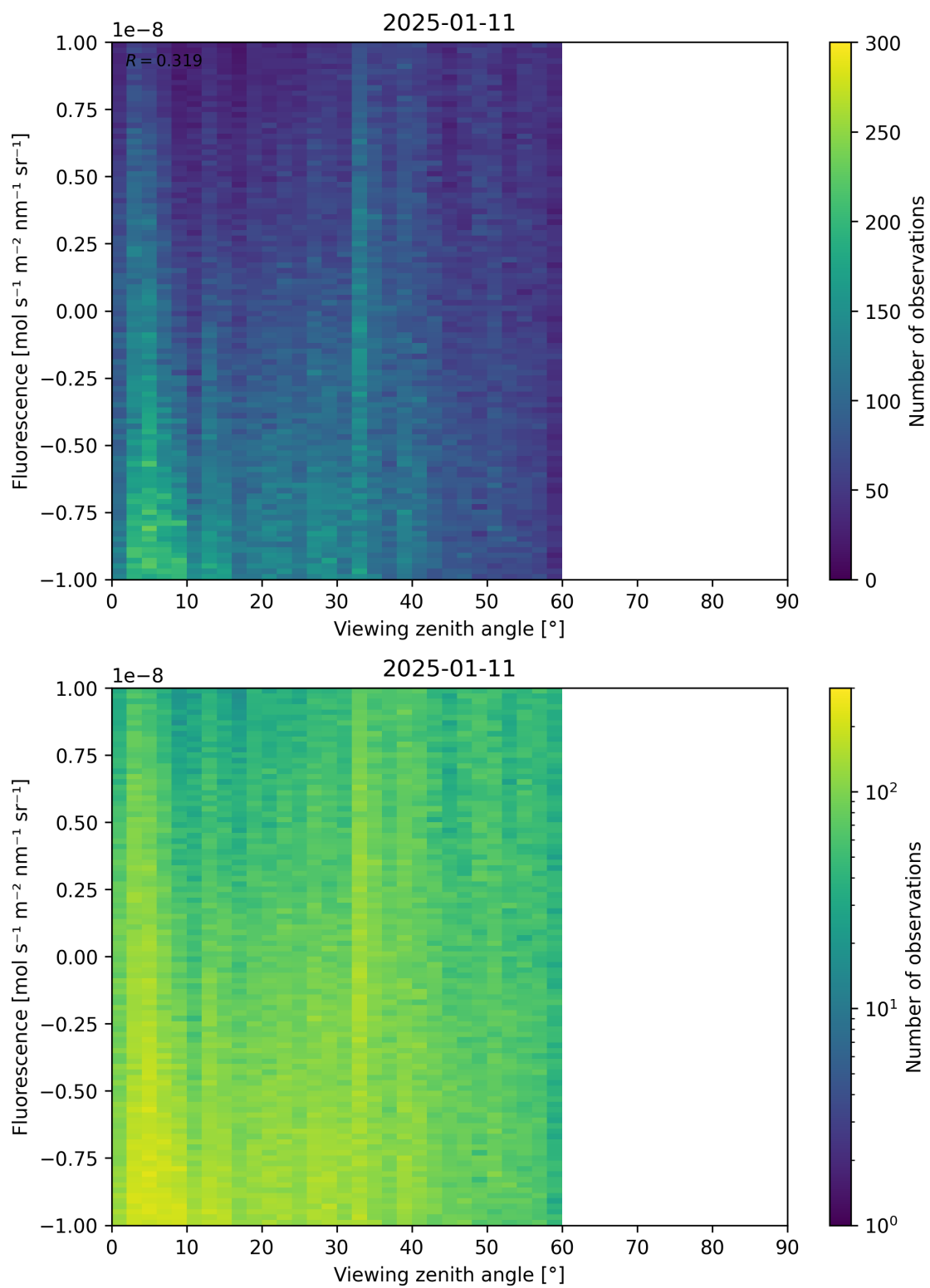
Figure 108: Scatter density plot of “Viewing zenith angle” against “Fluorescence” for 2025-01-10 to 2025-01-12.
