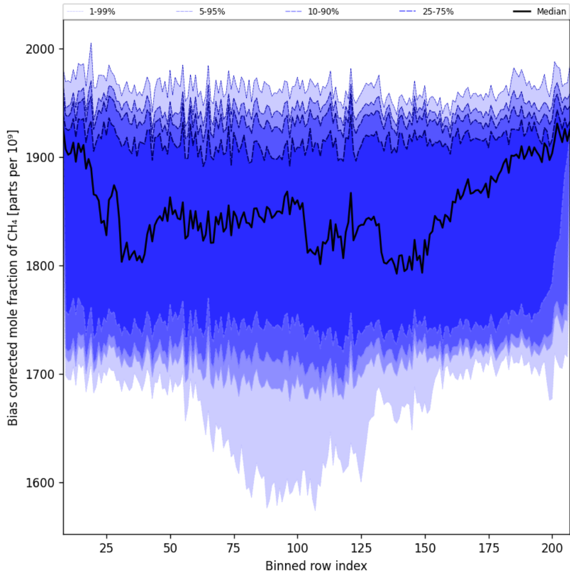
Figure 36: Along track statistics of “Bias corrected mole fraction of CH 4 ” for 2025-01-10 to 2025-01-12
