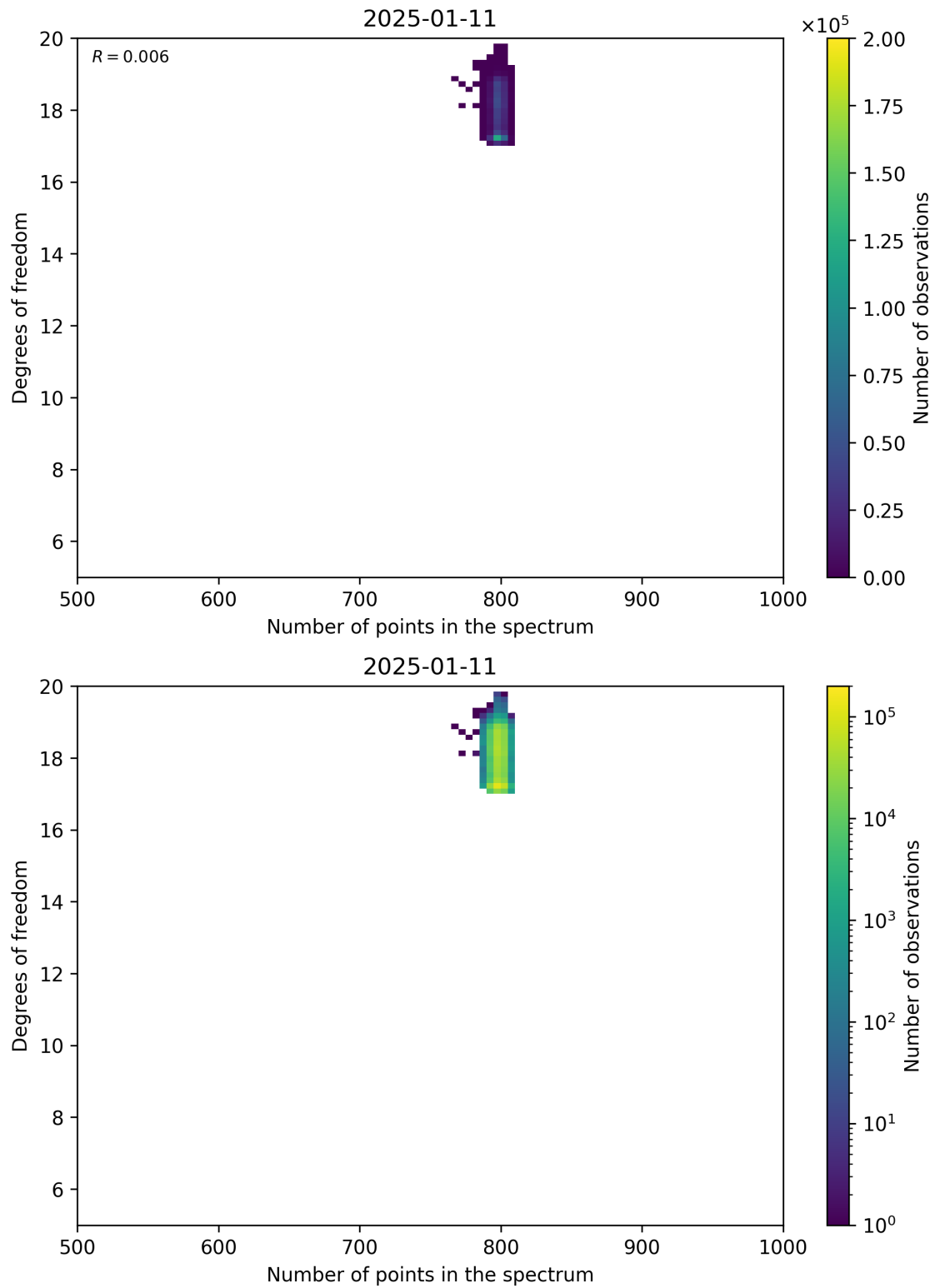
Figure 90: Scatter density plot of “Number of points in the spectrum” against “Degrees of freedom” for 2025-01-10 to 2025-01-12.
