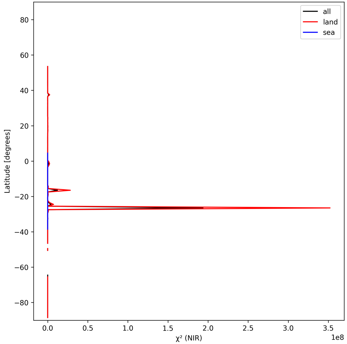
Figure 18: Zonal average of “ \chi^2 (NIR)” for 2025-01-10 to 2025-01-12.
