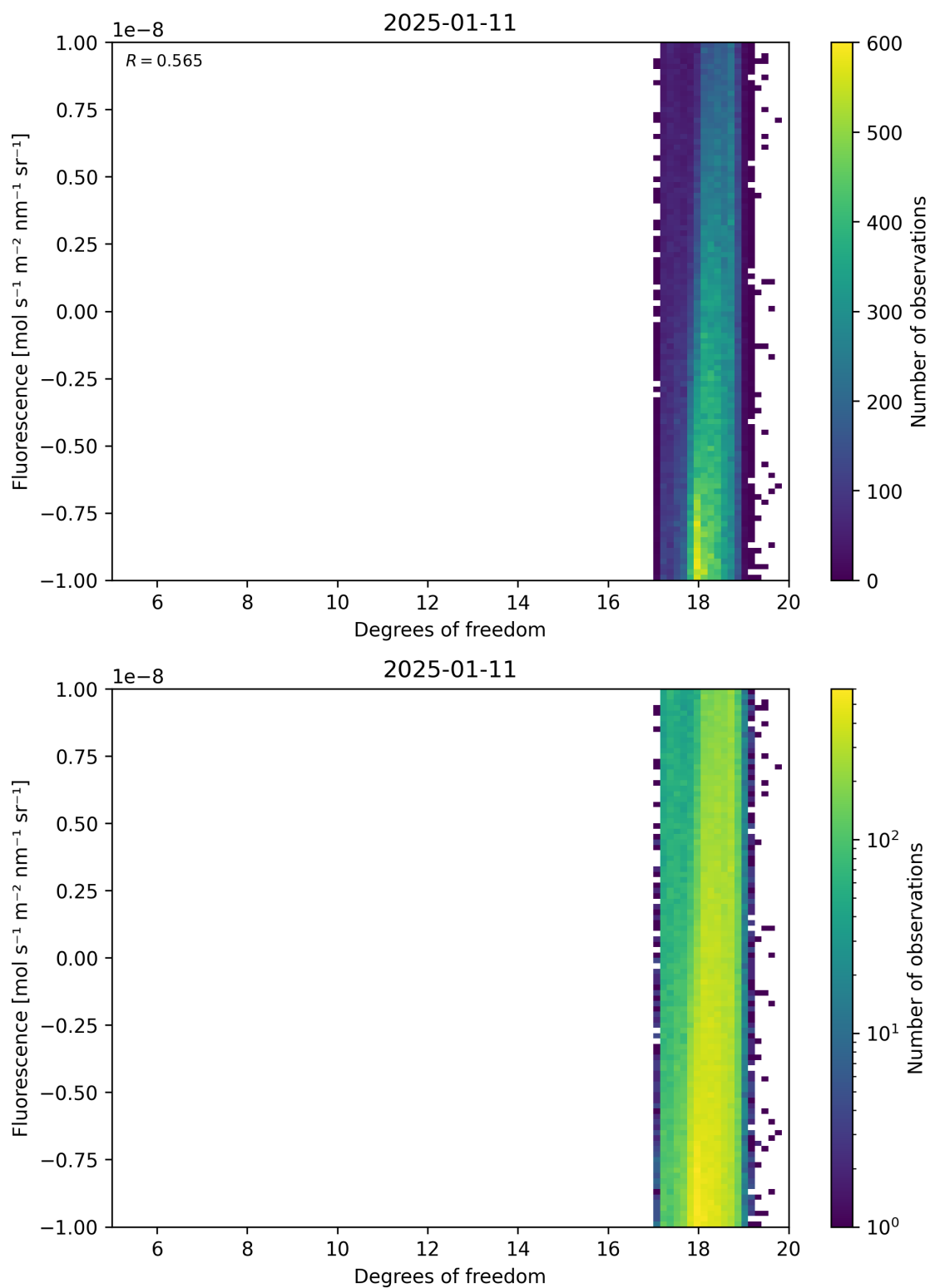
Figure 51: Scatter density plot of “Degrees of freedom” against “Fluorescence” for 2025-01-10 to 2025-01-12.
