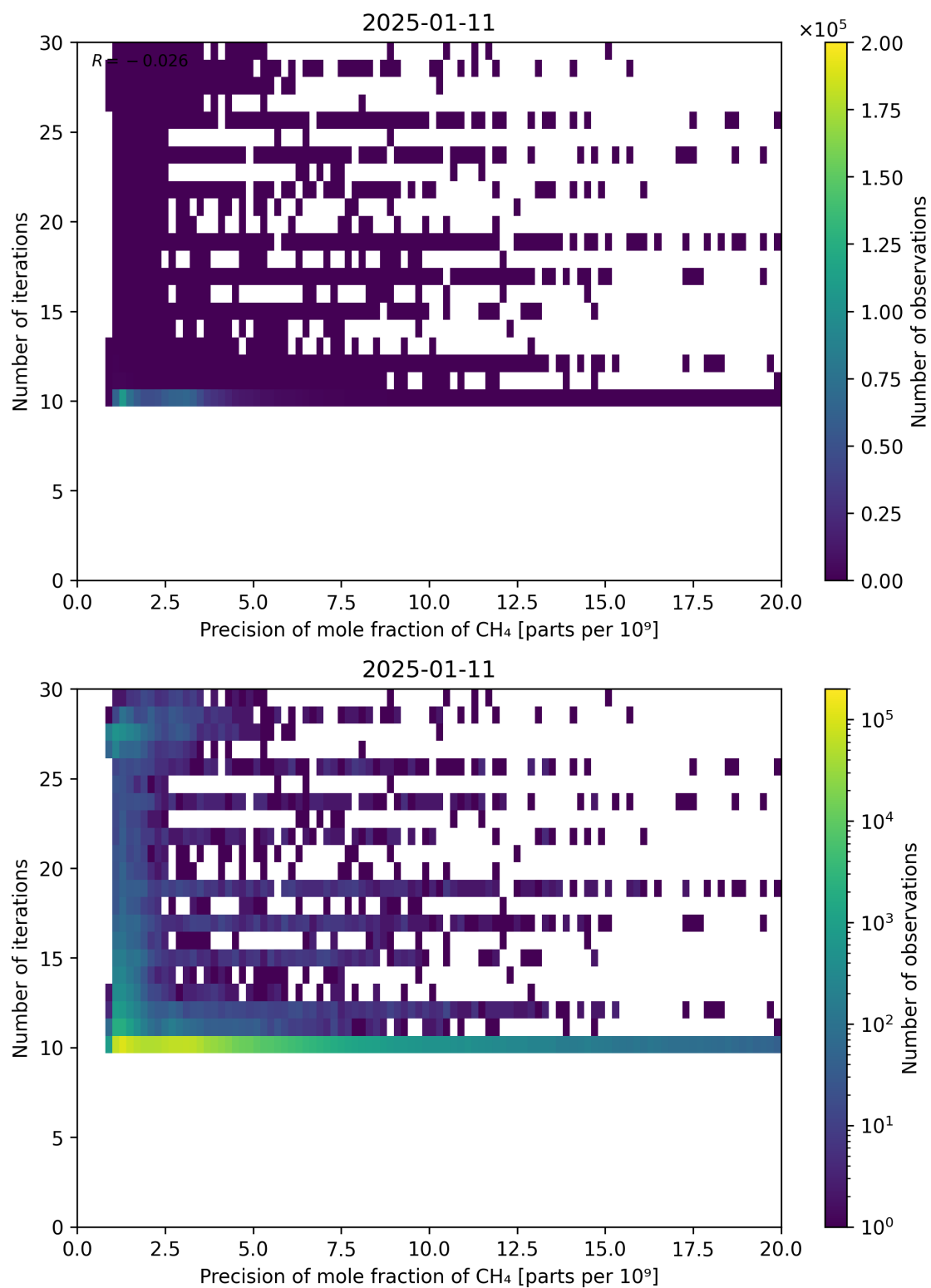
Figure 83: Scatter density plot of “Precision of mole fraction of CH 4 ” against “Number of iterations” for 2025-01-10 to 2025-01-12.
