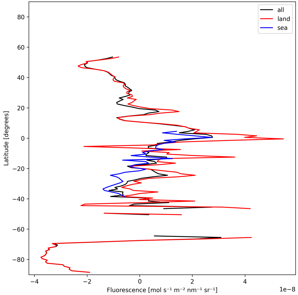
Figure 21: Zonal average of “Fluorescence” for 2025-01-10 to 2025-01-12.
