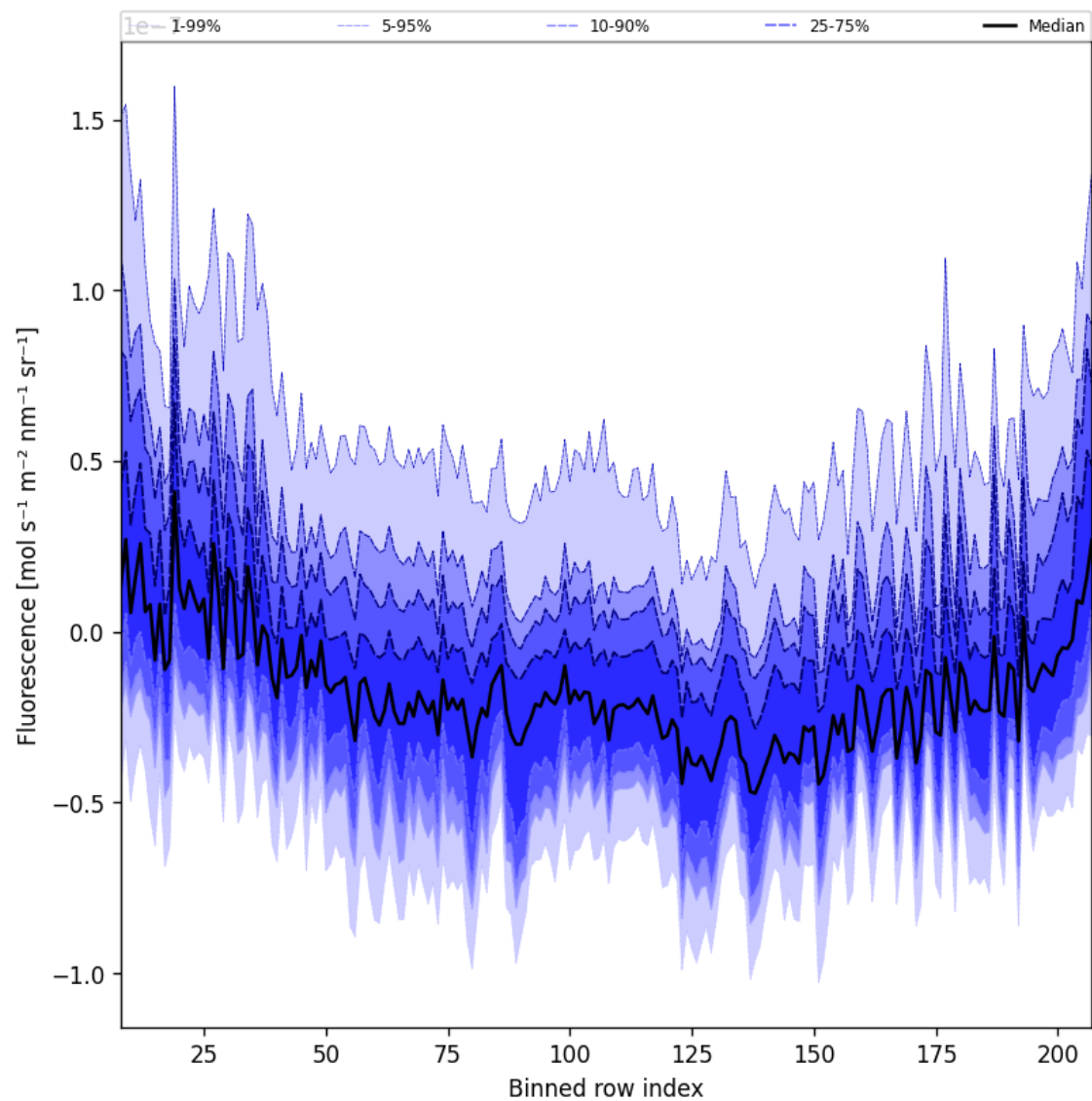
Figure 43: Along track statistics of “Fluorescence” for 2025-01-10 to 2025-01-12
