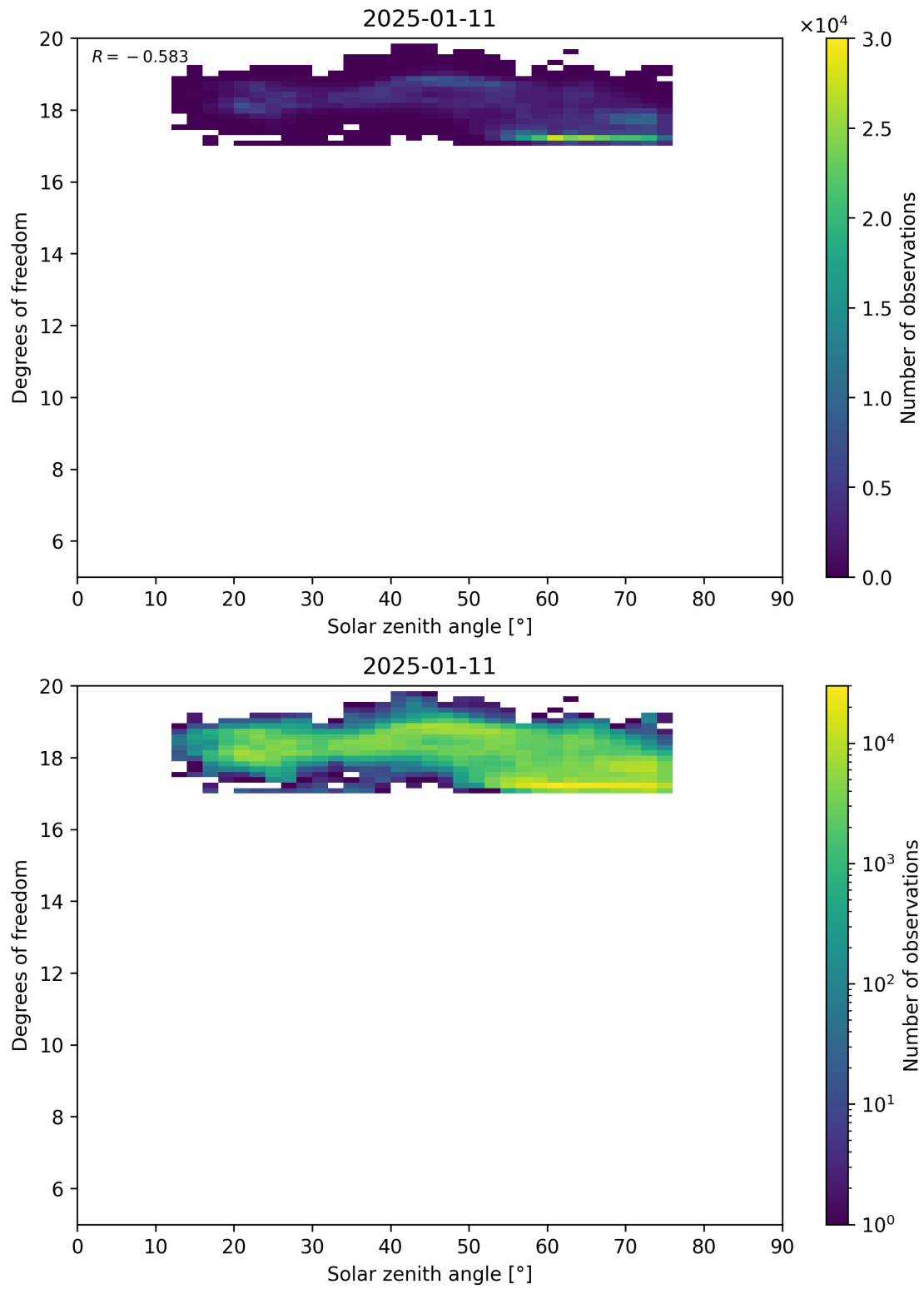
Figure 96: Scatter density plot of “Solar zenith angle” against “Degrees of freedom” for 2025-01-10 to 2025-01-12.
