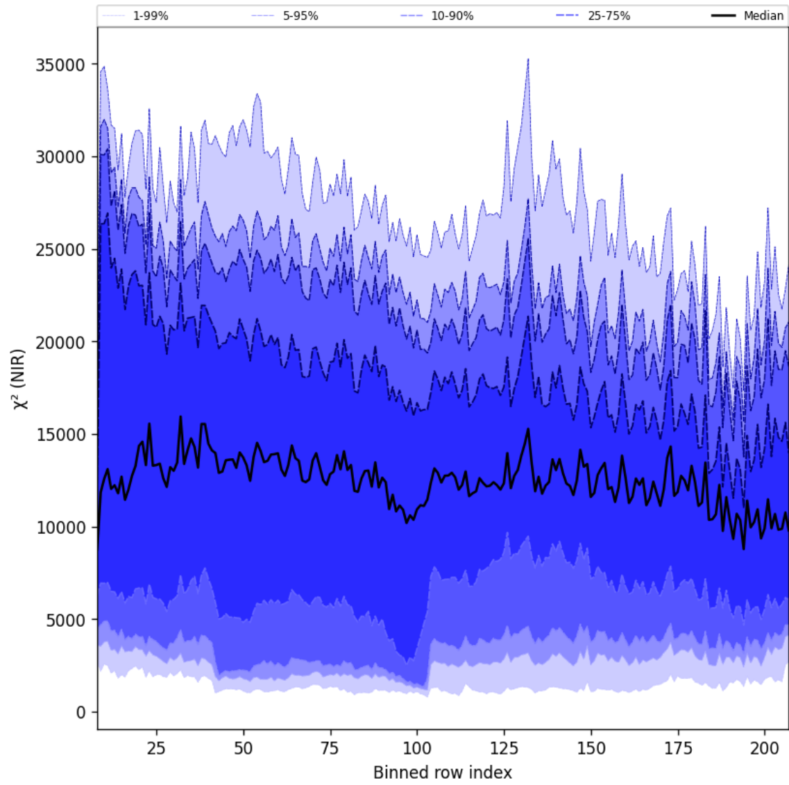
Figure 40: Along track statistics of “ \chi^2 (NIR)” for 2025-01-10 to 2025-01-12
