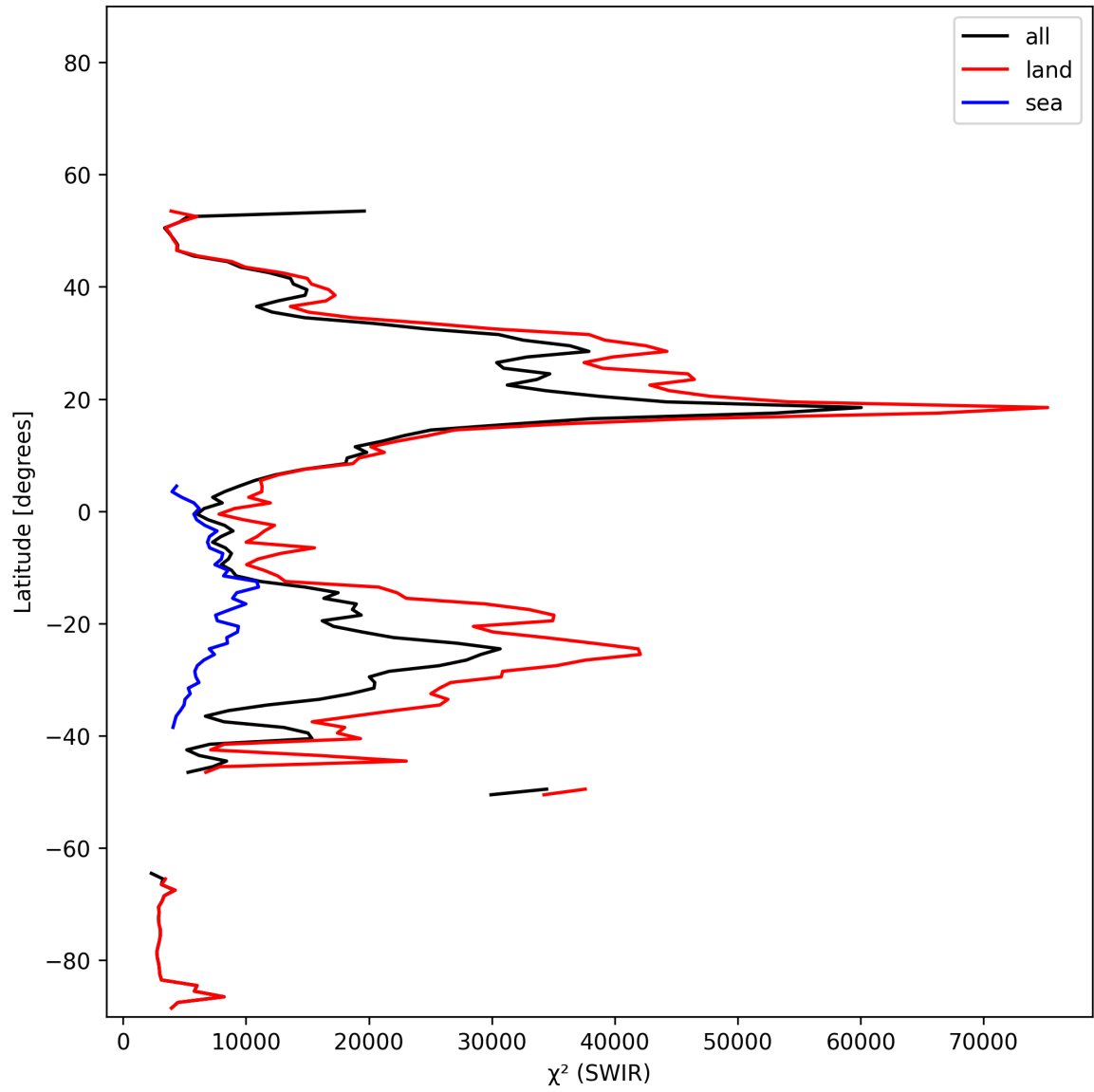
Figure 17: Zonal average of “ \chi^2 (SWIR)” for 2025-01-10 to 2025-01-12.
