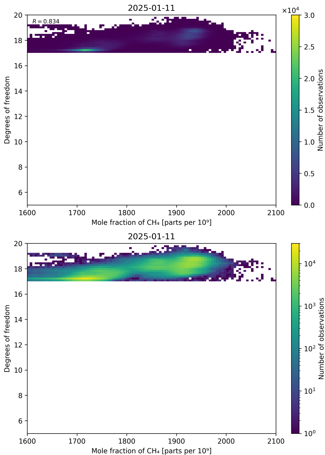
Figure 72: Scatter density plot of “Mole fraction of CH 4 ” against “Degrees of freedom” for 2025-01-10 to 2025-01-12.
