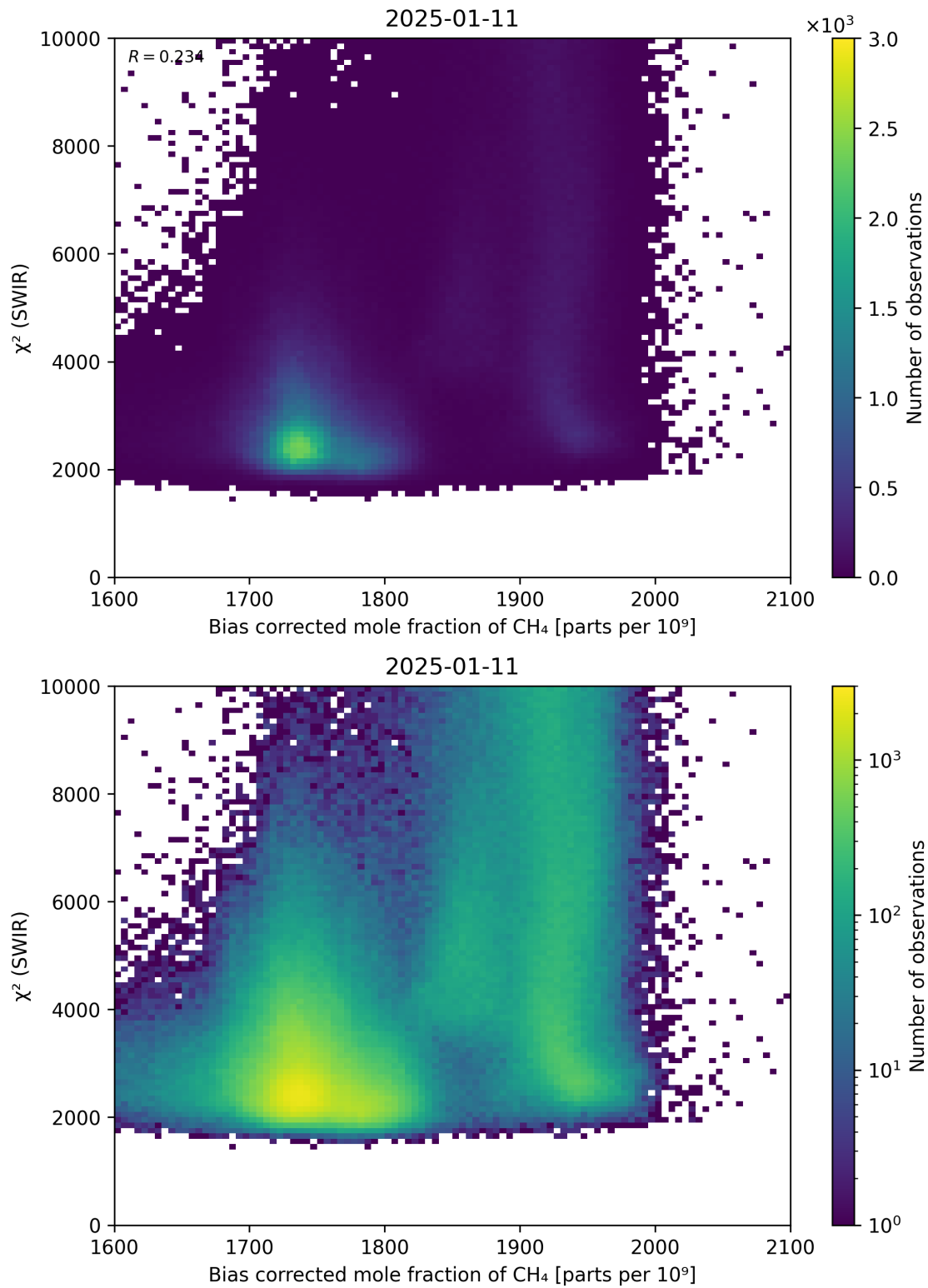
Figure 64: Scatter density plot of “Bias corrected mole fraction of \text{CH}_4 ” against “ \chi^2 (SWIR)” for 2025-01-10 to 2025-01-12.
