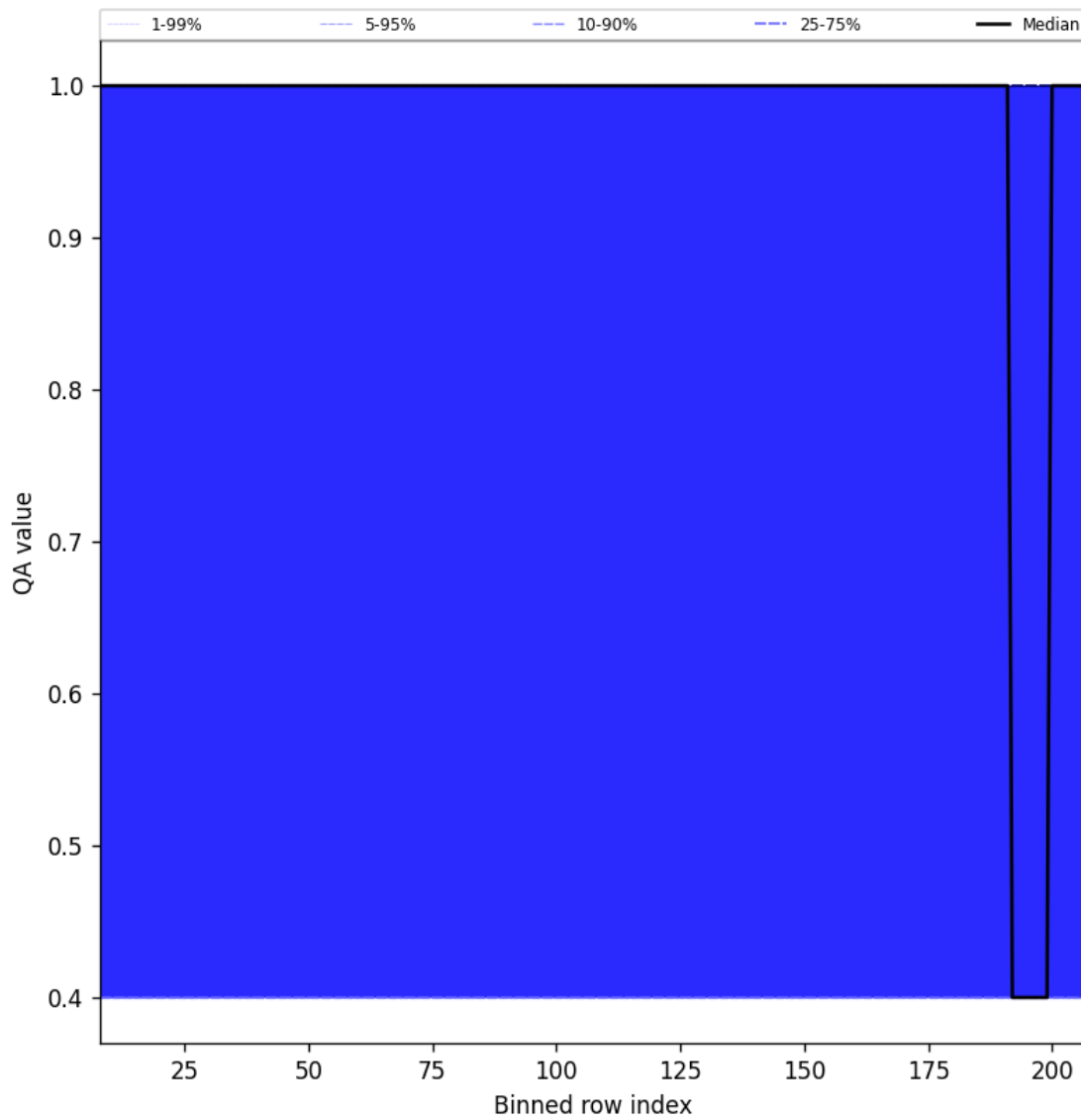
Figure 33: Along track statistics of “QA value” for 2025-01-10 to 2025-01-12
