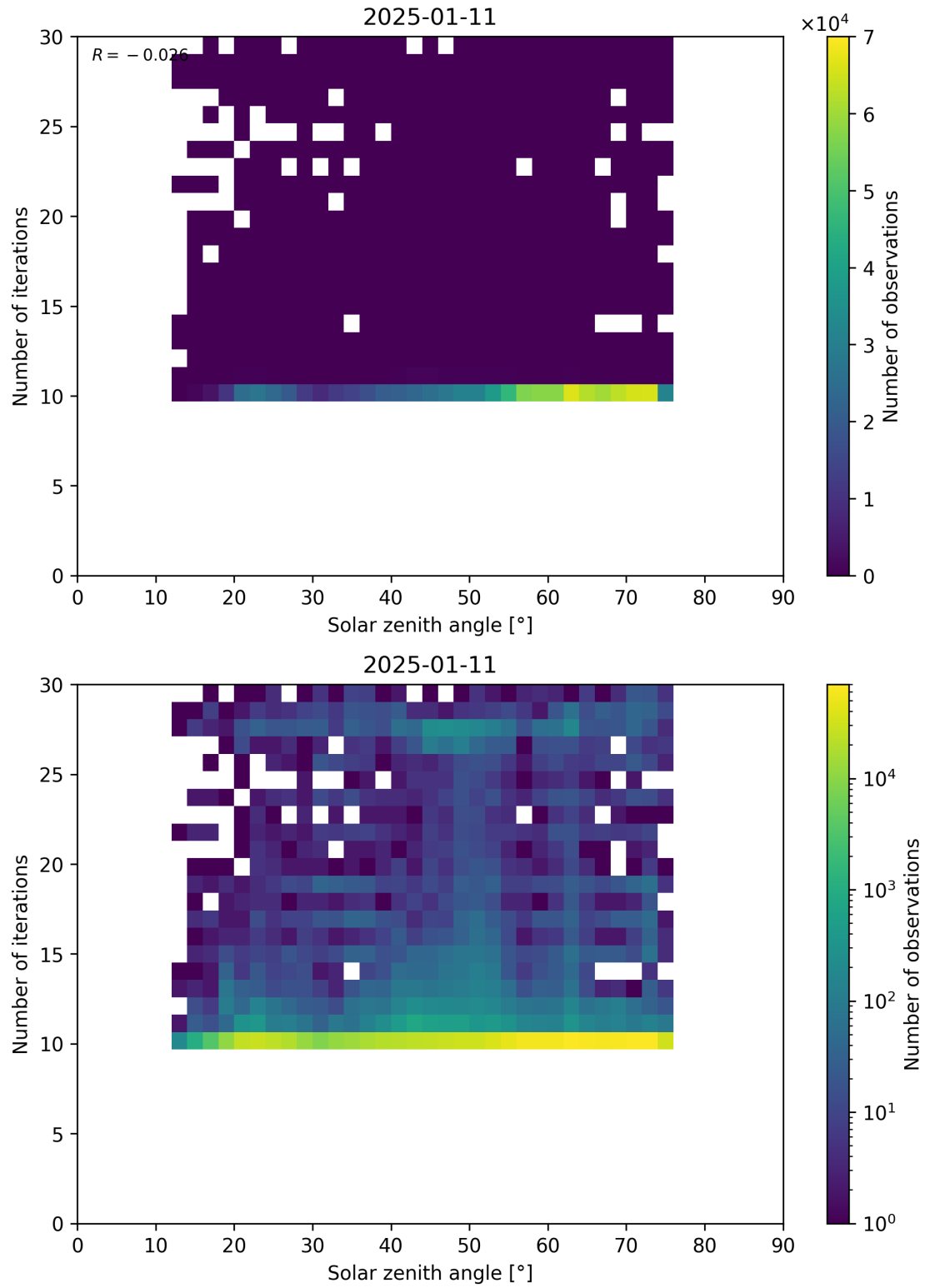
Figure 102: Scatter density plot of “Solar zenith angle” against “Number of iterations” for 2025-01-10 to 2025-01-12.
