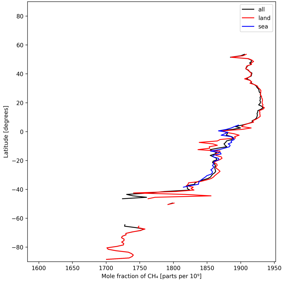
Figure 12: Zonal average of “Mole fraction of \text{CH}_4 ” for 2025-01-10 to 2025-01-12.
