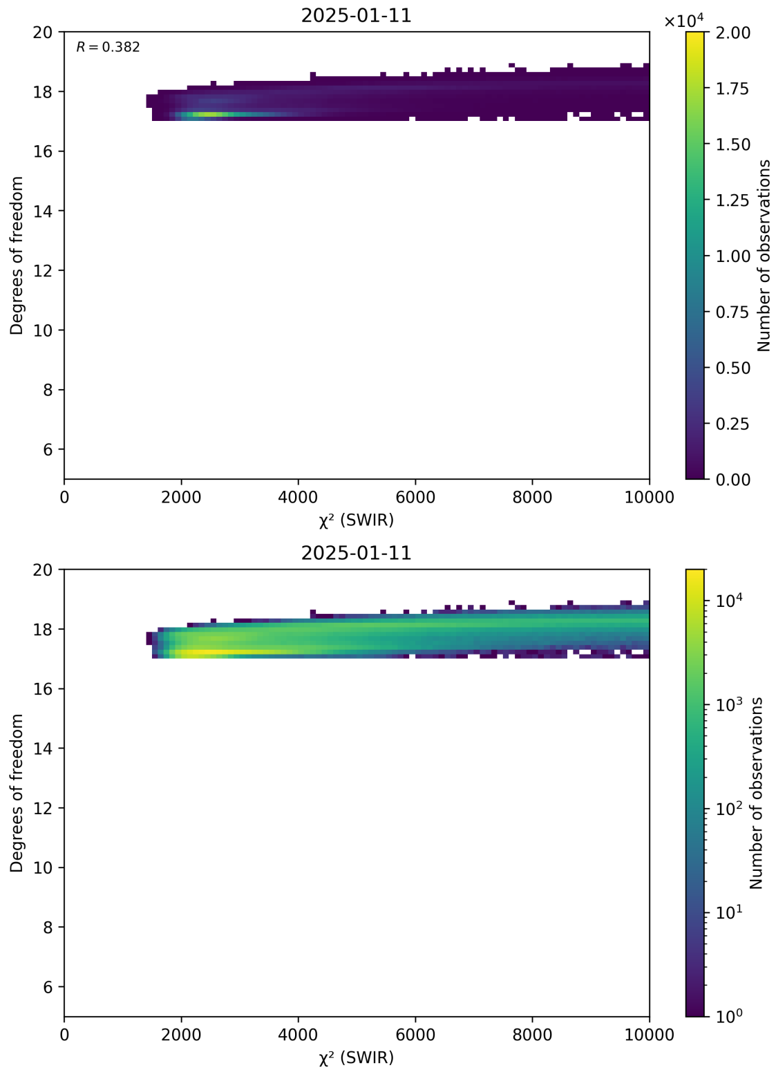
Figure 48: Scatter density plot of “ \chi^2 (SWIR)” against “Degrees of freedom” for 2025-01-10 to 2025-01-12.
