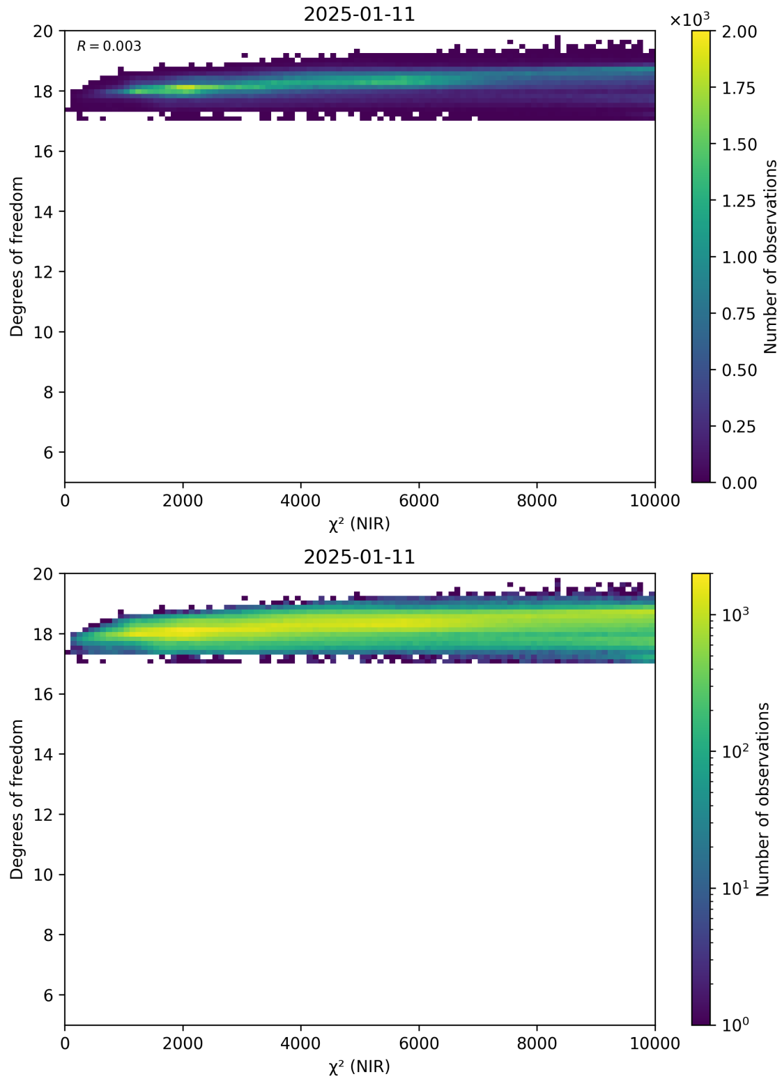
Figure 44: Scatter density plot of “ \chi^2 (NIR)” against “Degrees of freedom” for 2025-01-10 to 2025-01-12.
