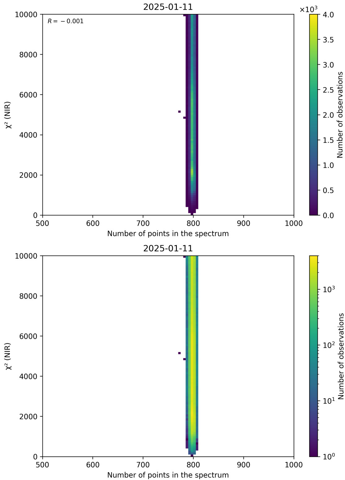
Figure 88: Scatter density plot of “Number of points in the spectrum” against “ \chi^2 (NIR)” for 2025-01-10 to 2025-01-12.
