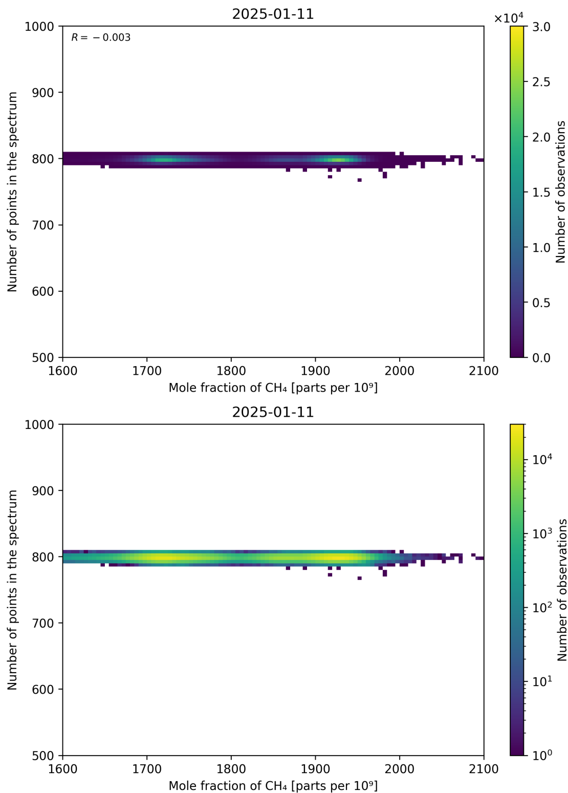
Figure 77: Scatter density plot of “Mole fraction of CH 4 ” against “Number of points in the spectrum” for 2025-01-10 to 2025-01-12.
