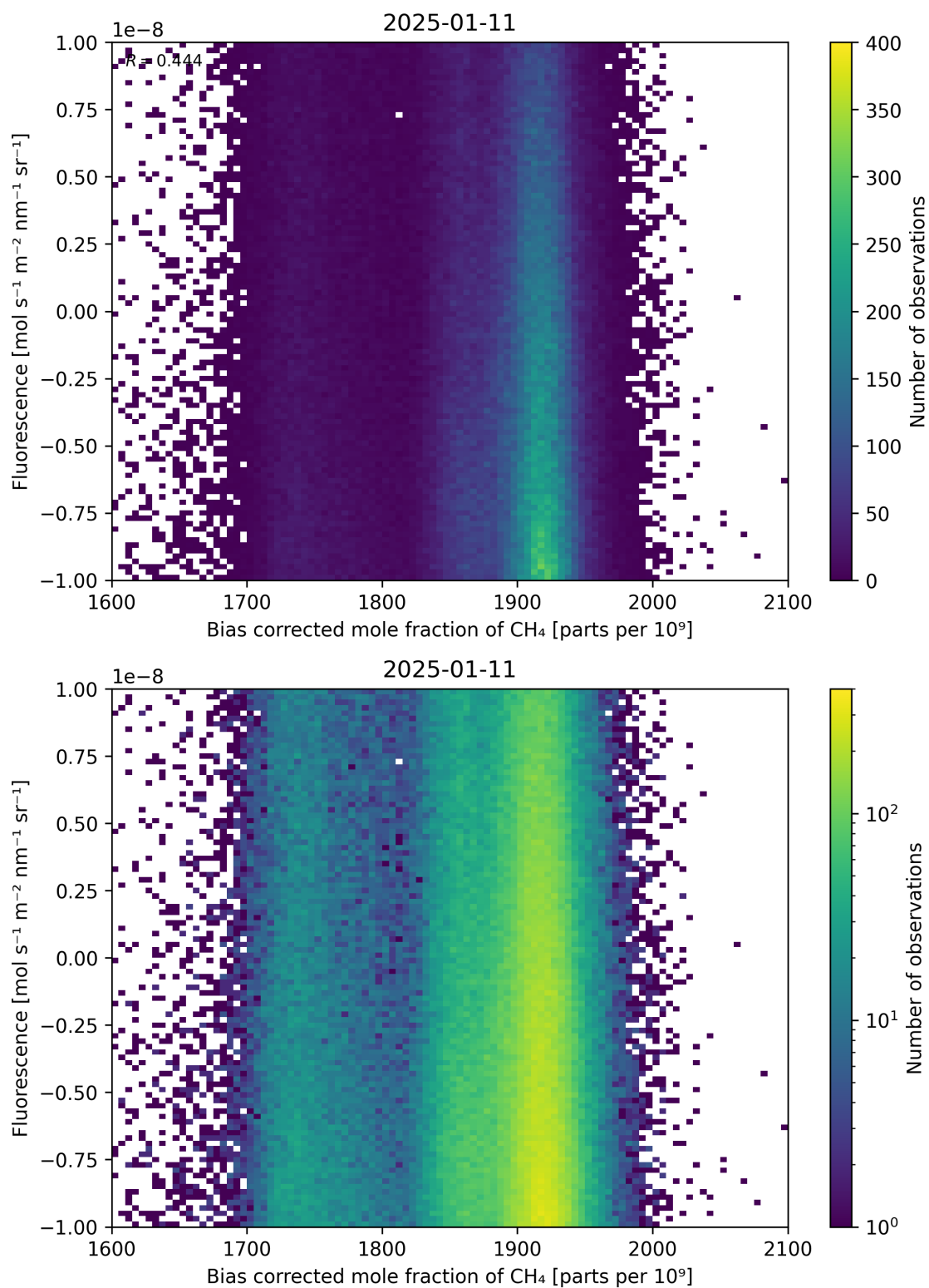
Figure 66: Scatter density plot of “Bias corrected mole fraction of \text{CH}_4 ” against “Fluorescence” for 2025-01-10 to 2025-01-12.
