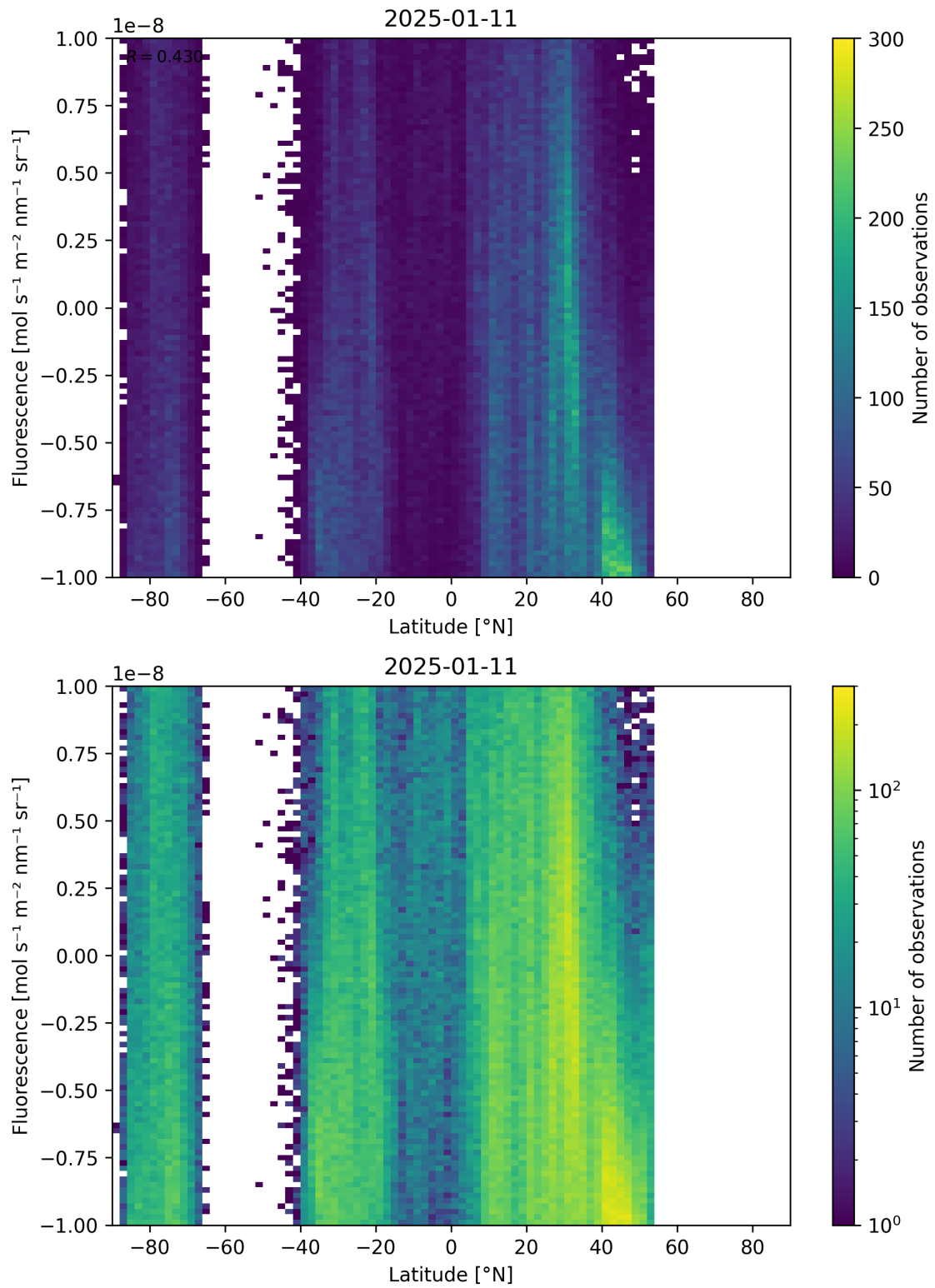
Figure 56: Scatter density plot of “Latitude” against “Fluorescence” for 2025-01-10 to 2025-01-12.
