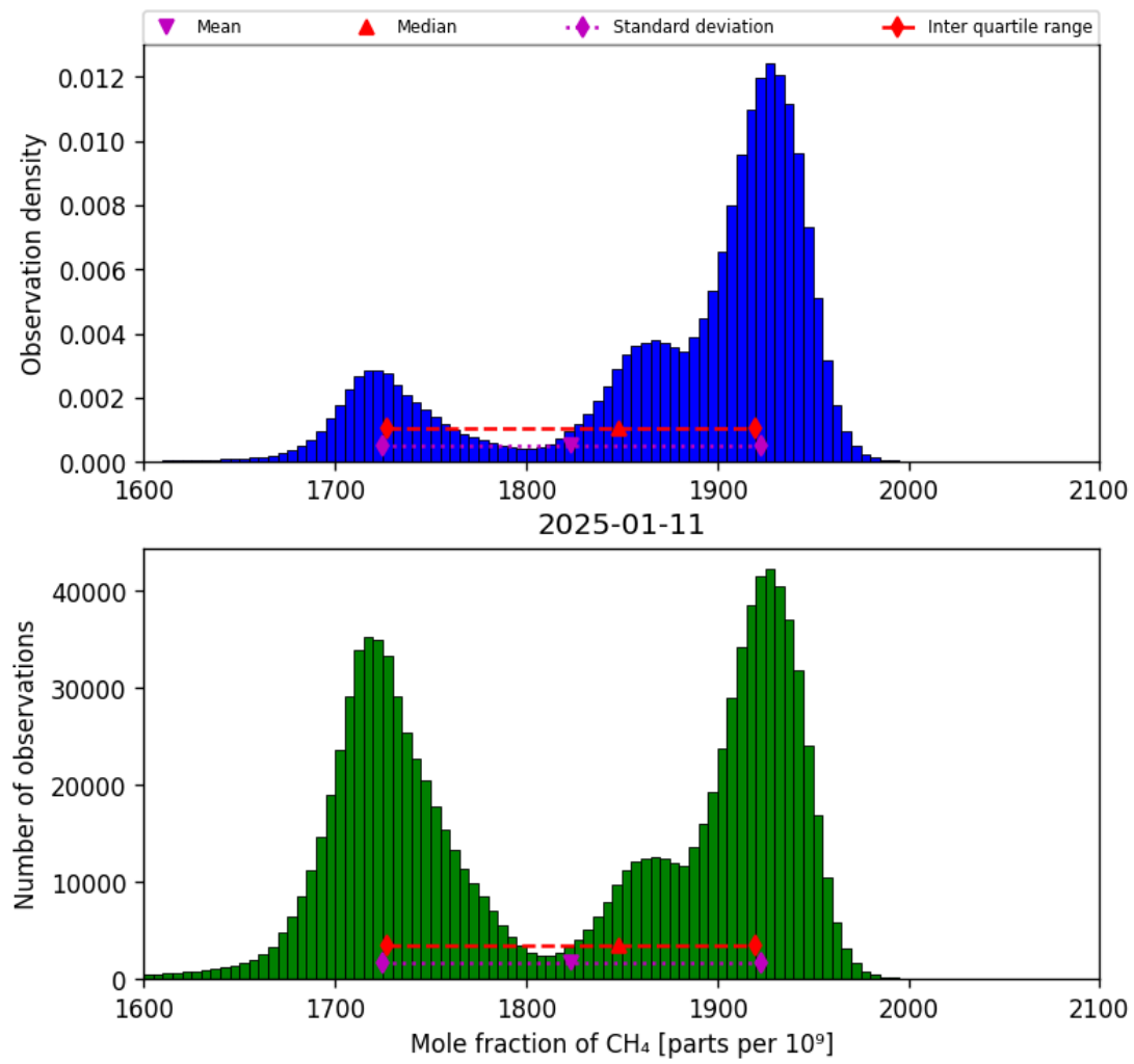
Figure 23: Histogram of “Mole fraction of CH 4 ” for 2025-01-10 to 2025-01-12
