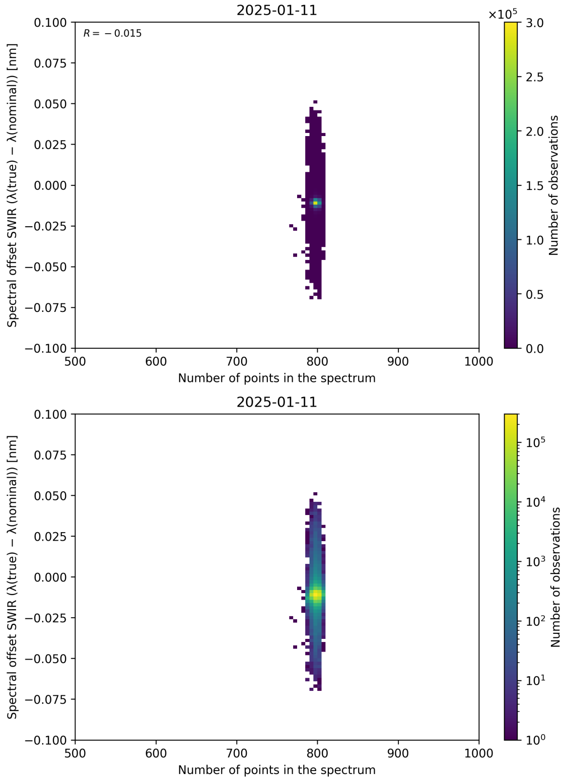
Figure 93: Scatter density plot of “Number of points in the spectrum” against “Spectral offset SWIR ( \lambda_{\text{true}} - \lambda_{\text{nominal}} )” for 2025-01-10 to 2025-01-12.
