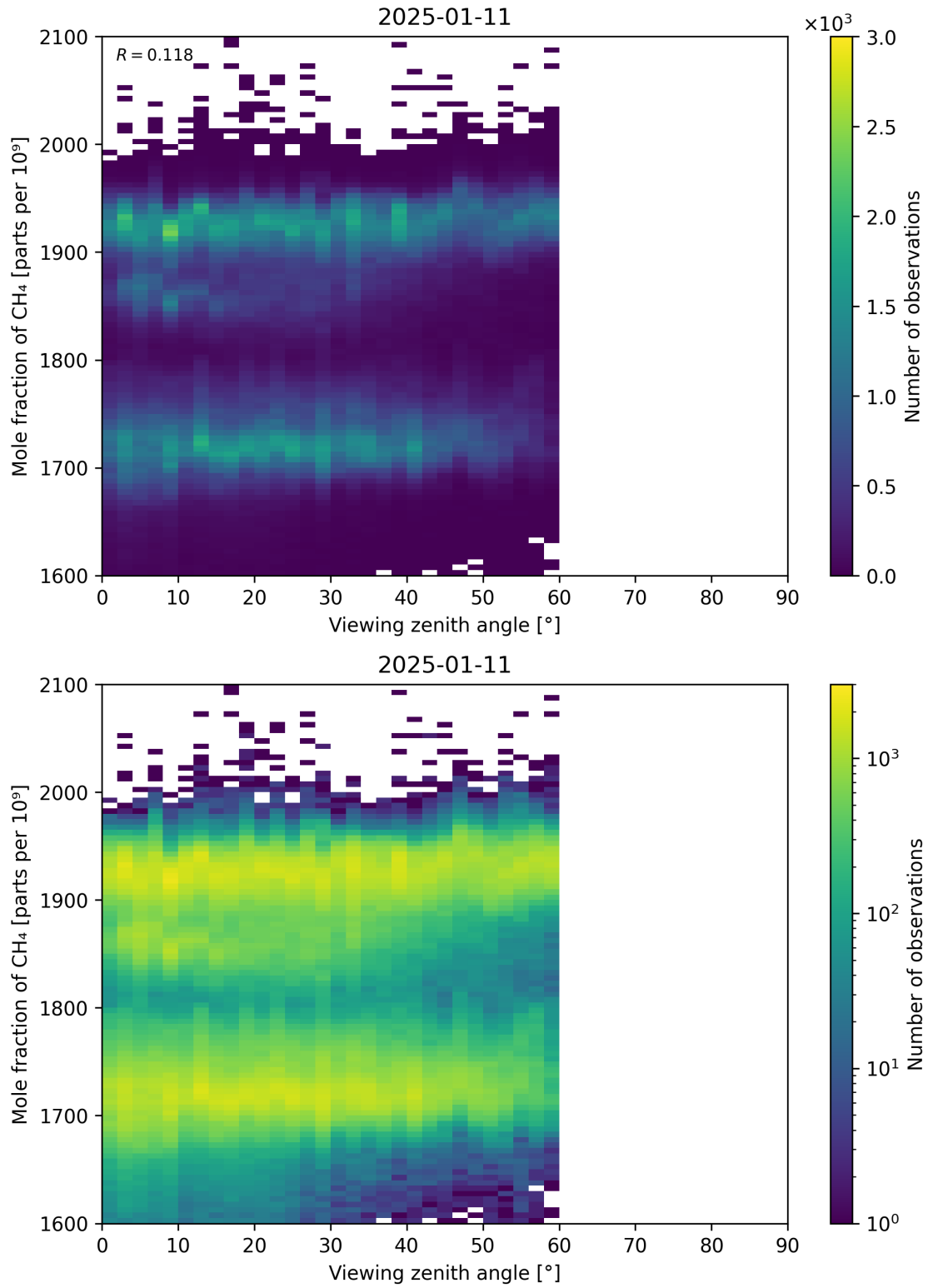
Figure 110: Scatter density plot of “Viewing zenith angle” against “Mole fraction of CH 4 ” for 2025-01-10 to 2025-01-12.
