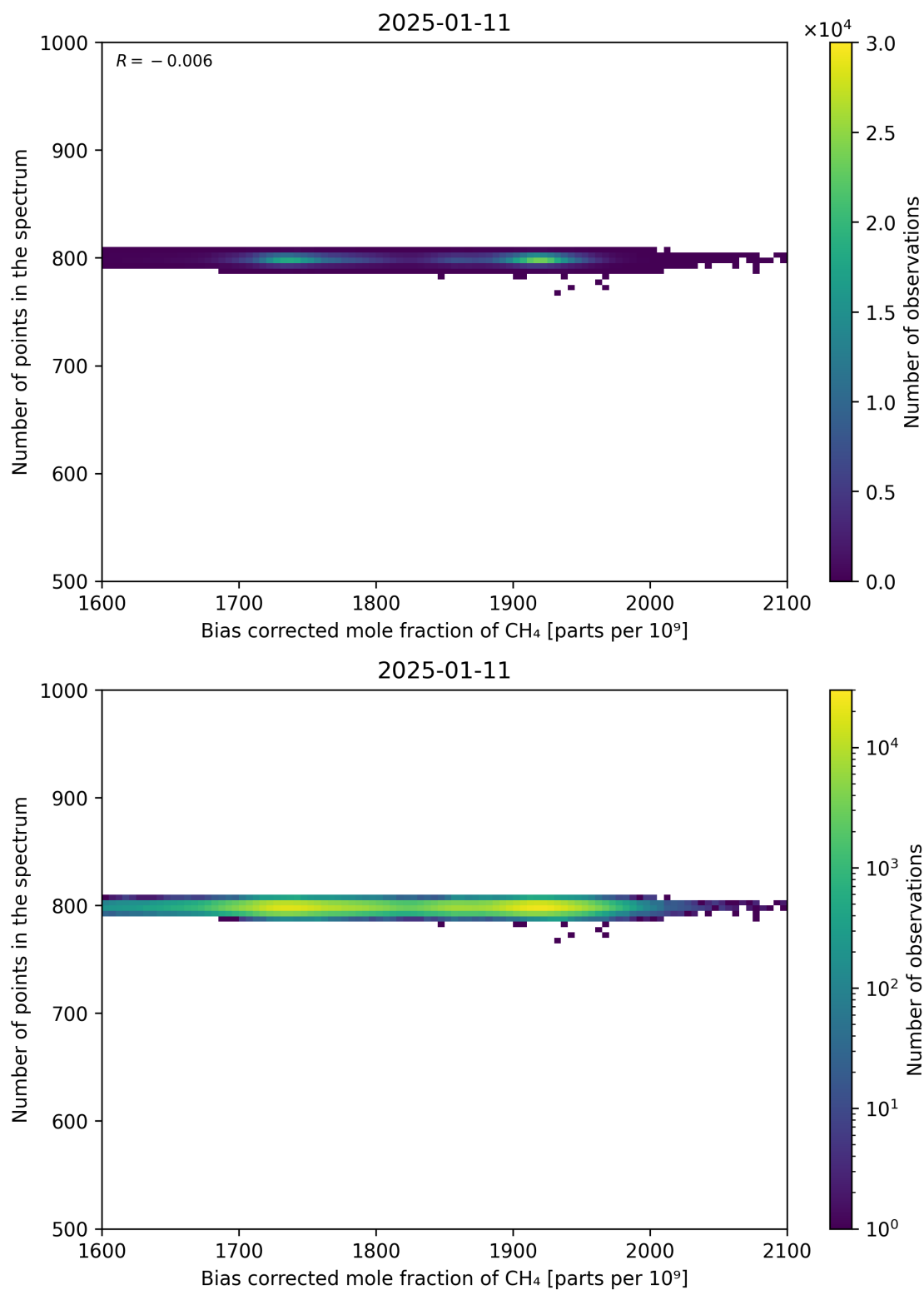
Figure 68: Scatter density plot of “Bias corrected mole fraction of CH 4 ” against “Number of points in the spectrum” for 2025-01-10 to 2025-01-12.
