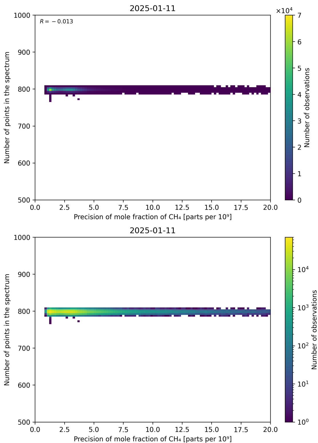
Figure 84: Scatter density plot of “Precision of mole fraction of CH 4 ” against “Number of points in the spectrum” for 2025-01-10 to 2025-01-12.
