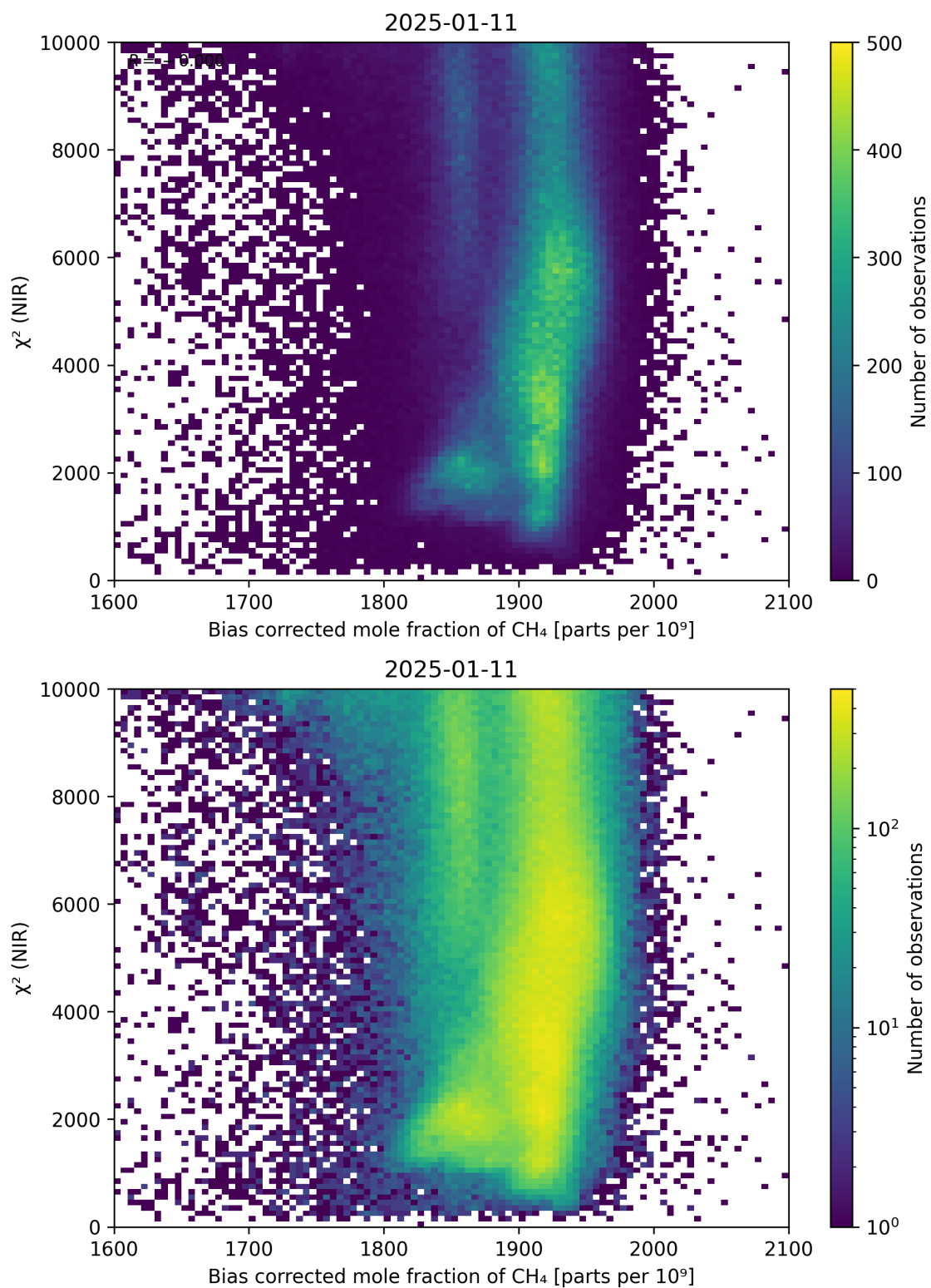
Figure 63: Scatter density plot of “Bias corrected mole fraction of \text{CH}_4 ” against “ \chi^2 (NIR)” for 2025-01-10 to 2025-01-12.
