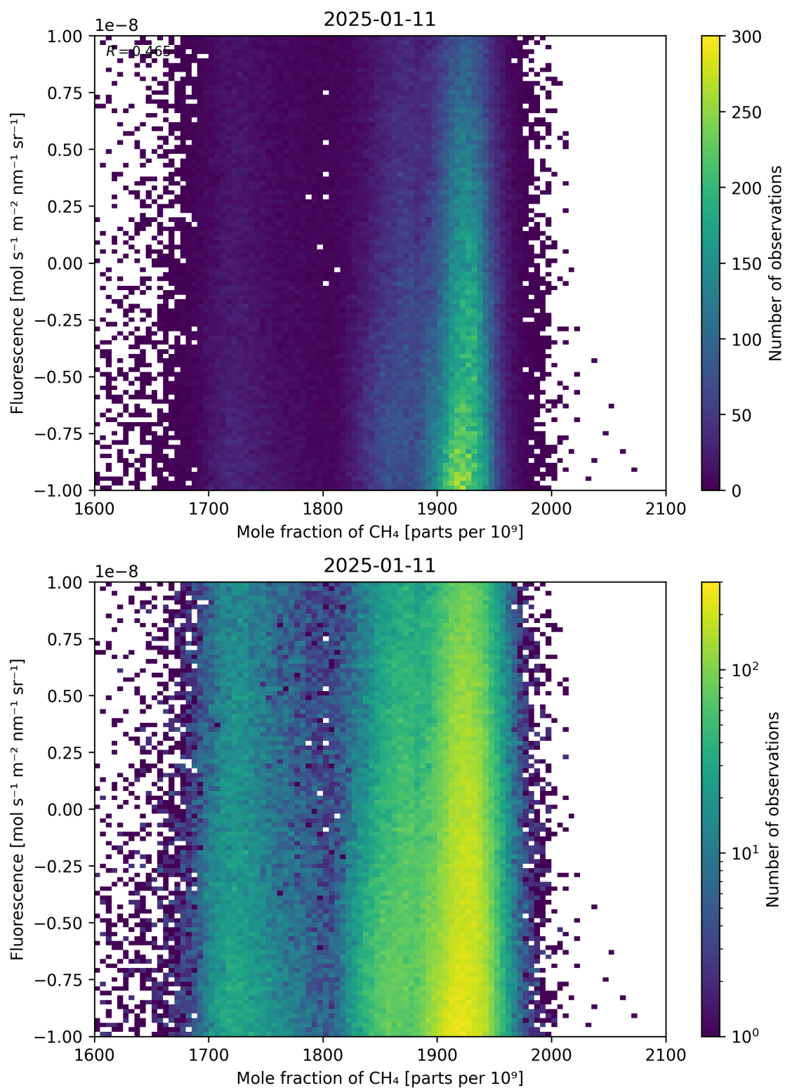
Figure 73: Scatter density plot of “Mole fraction of \text{CH}_4 ” against “Fluorescence” for 2025-01-10 to 2025-01-12.
