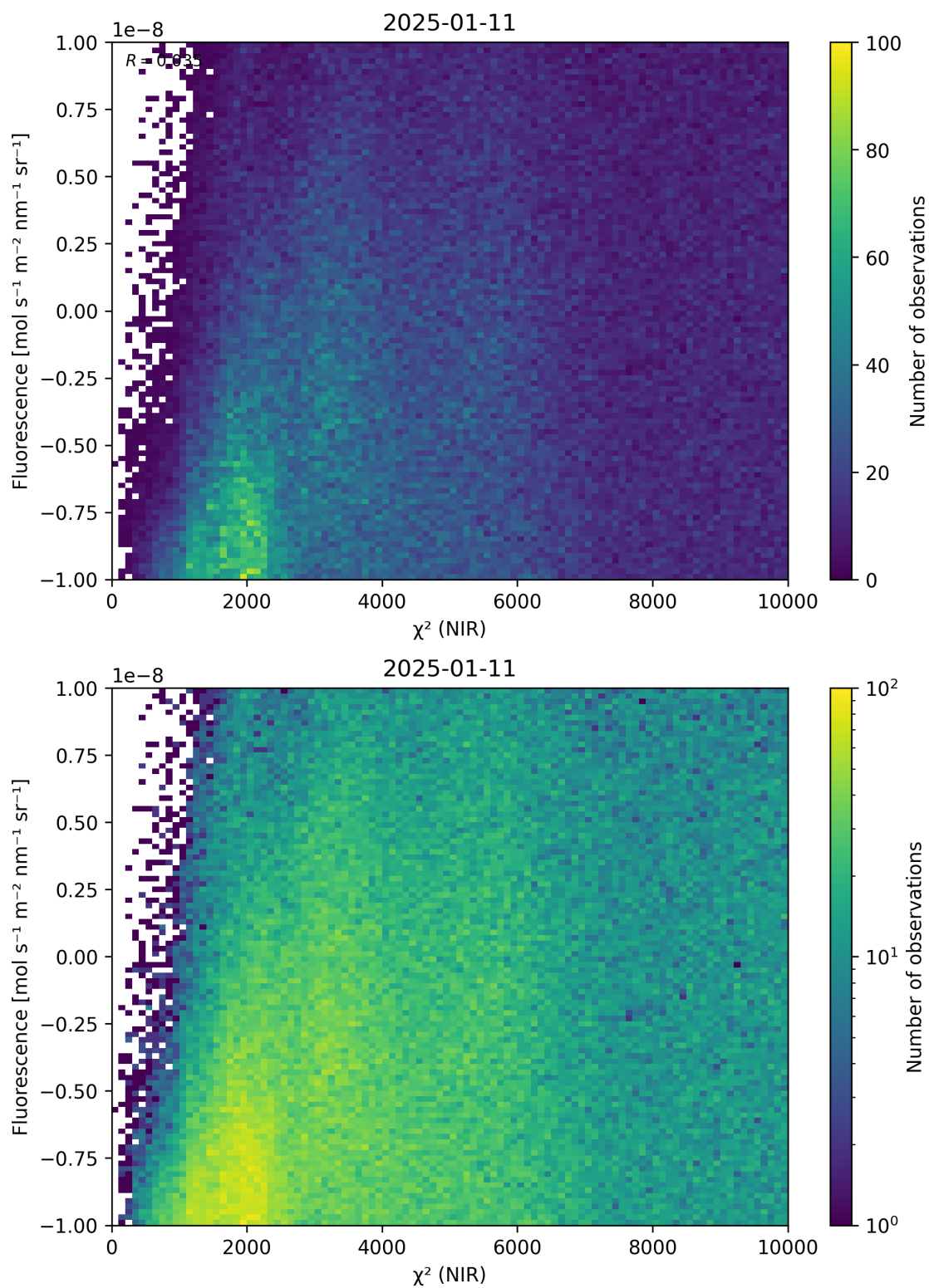
Figure 45: Scatter density plot of “ \chi^2 (NIR)” against “Fluorescence” for 2025-01-10 to 2025-01-12.
