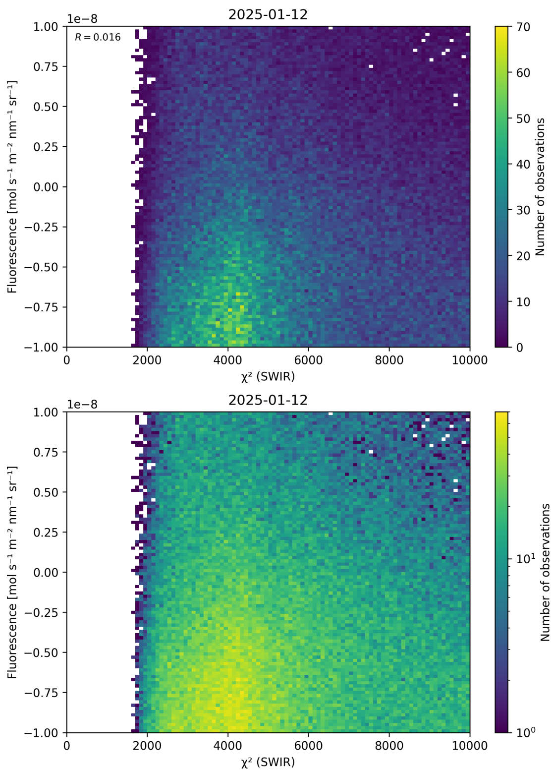
Figure 49: Scatter density plot of “ \chi^2 (SWIR)” against “Fluorescence” for 2025-01-12 to 2025-01-13.
