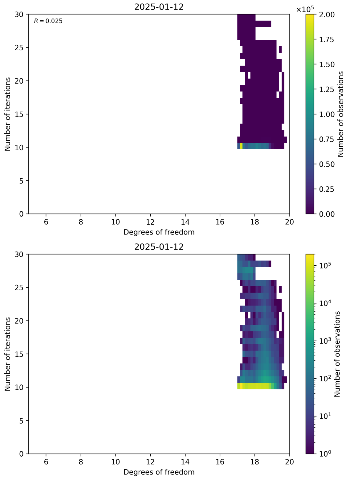
Figure 52: Scatter density plot of “Degrees of freedom” against “Number of iterations” for 2025-01-12 to 2025-01-13.
