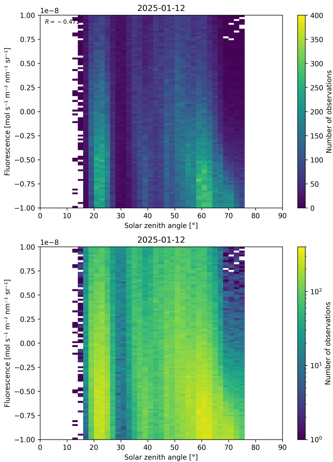
Figure 97: Scatter density plot of “Solar zenith angle” against “Fluorescence” for 2025-01-12 to 2025-01-13.
