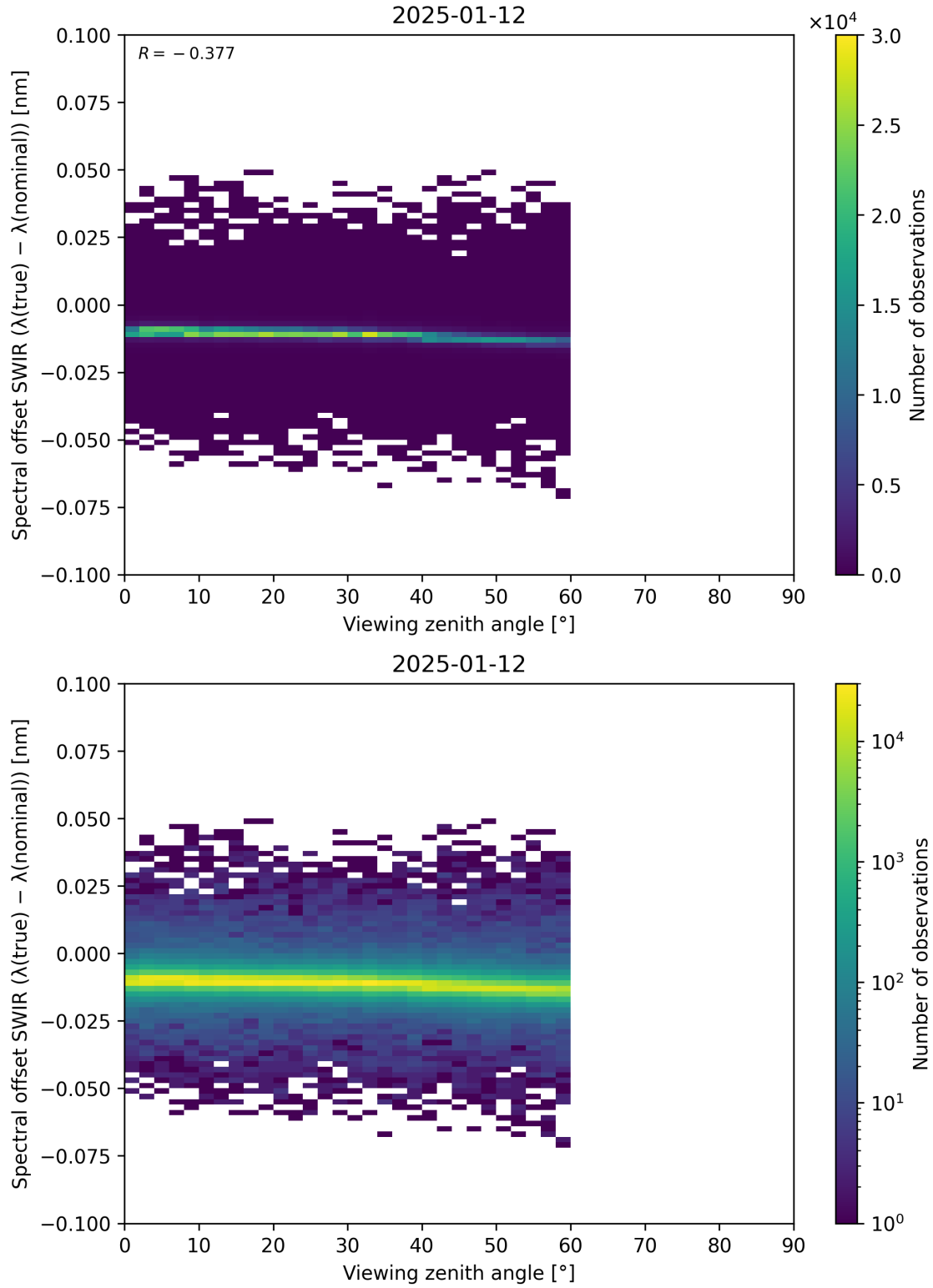
Figure 116: Scatter density plot of “Viewing zenith angle” against “Spectral offset SWIR ( \lambda_{\text{true}} - \lambda_{\text{nominal}} )” for 2025-01-12 to 2025-01-13.
