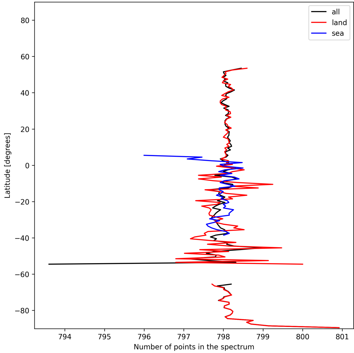
Figure 15: Zonal average of “Number of points in the spectrum” for 2025-01-12 to 2025-01-13.
