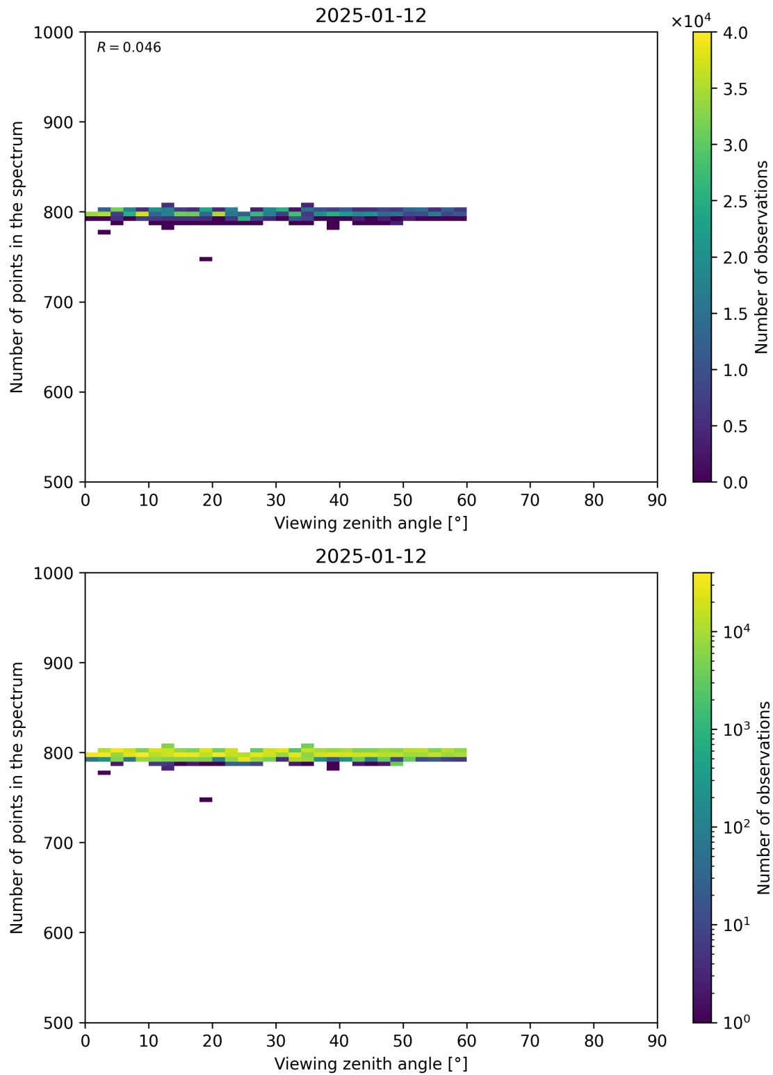
Figure 114: Scatter density plot of “Viewing zenith angle” against “Number of points in the spectrum” for 2025-01-12 to 2025-01-13.
