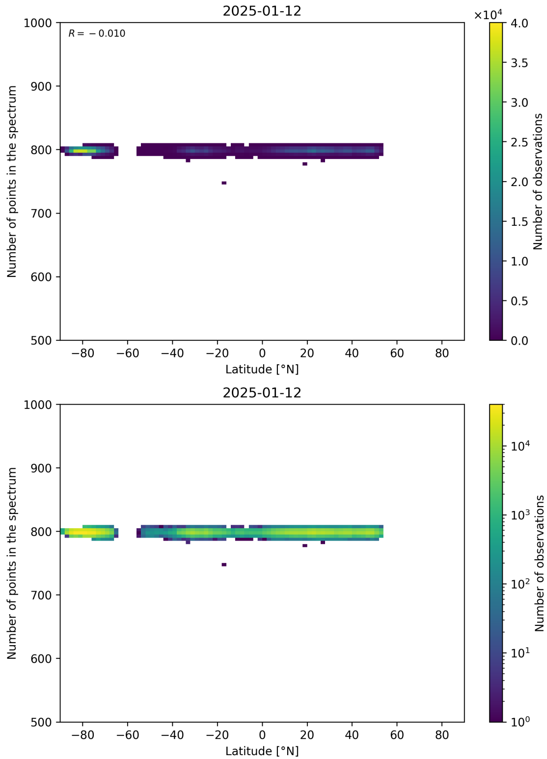
Figure 61: Scatter density plot of “Latitude” against “Number of points in the spectrum” for 2025-01-12 to 2025-01-13.
