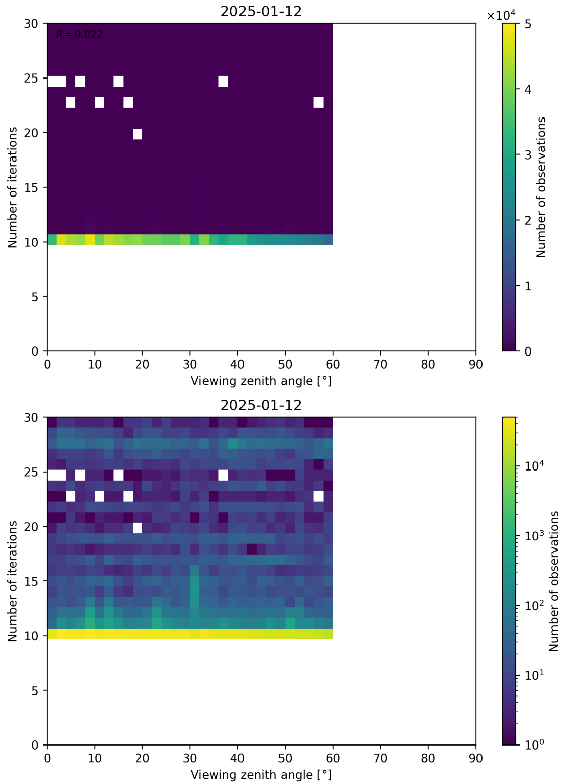
Figure 113: Scatter density plot of “Viewing zenith angle” against “Number of iterations” for 2025-01-12 to 2025-01-13.
