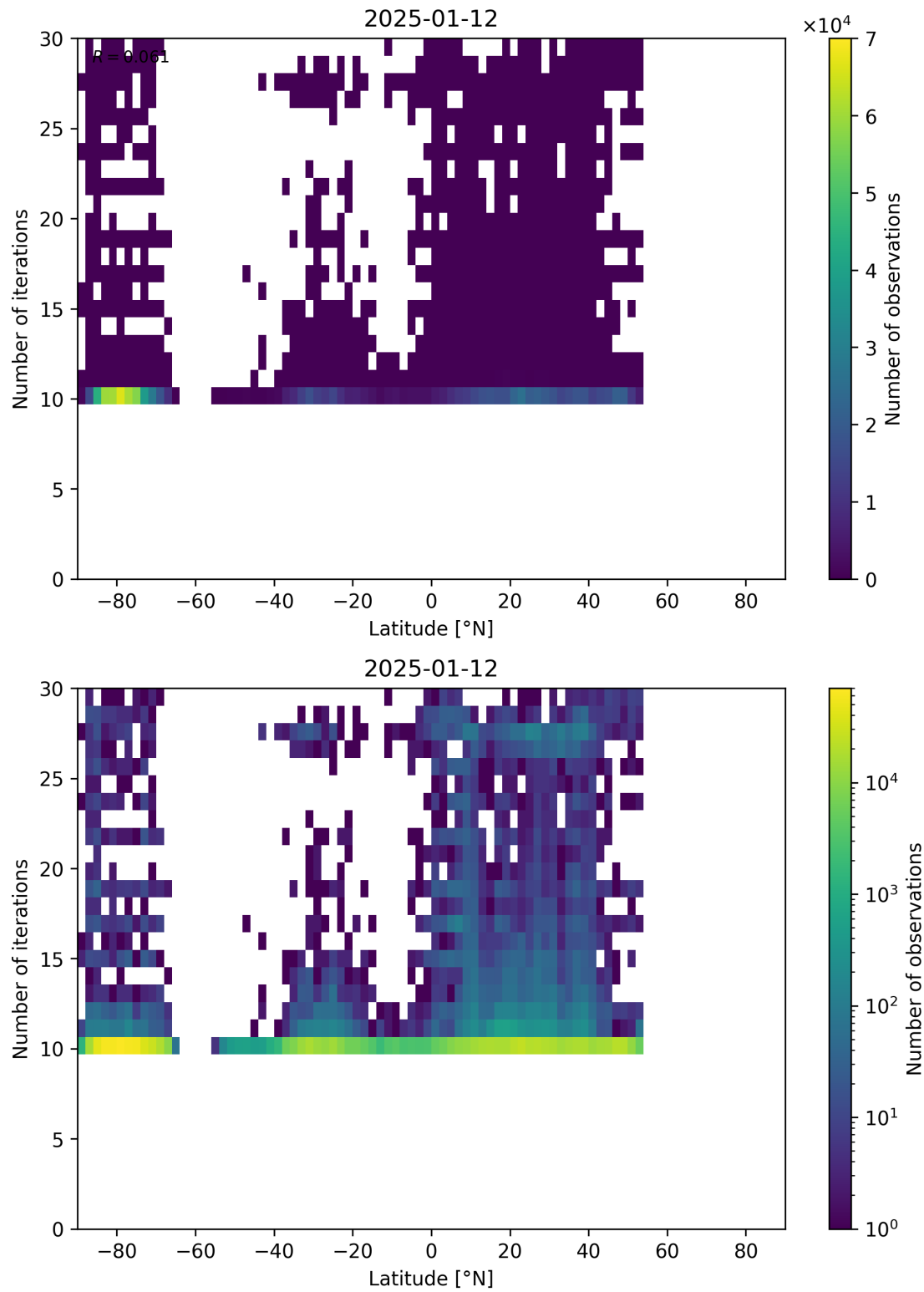
Figure 60: Scatter density plot of “Latitude” against “Number of iterations” for 2025-01-12 to 2025-01-13.
