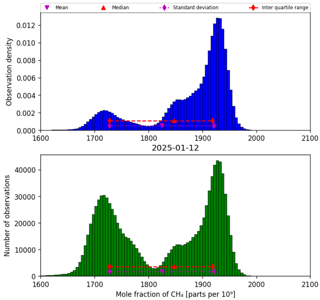
Figure 23: Histogram of “Mole fraction of CH 4 ” for 2025-01-12 to 2025-01-13
