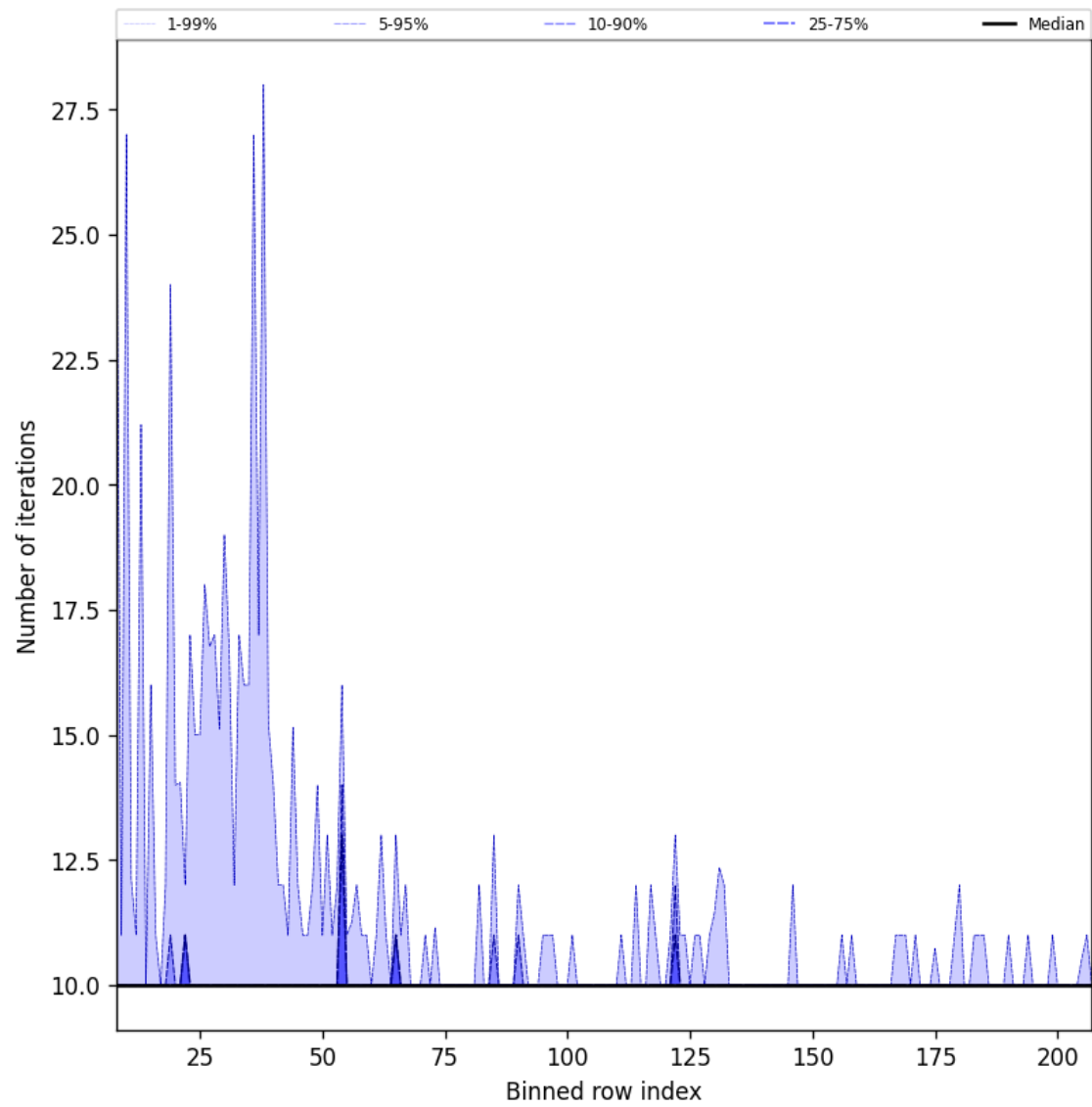
Figure 42: Along track statistics of “Number of iterations” for 2025-01-12 to 2025-01-13
