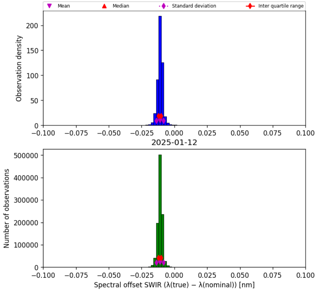
Figure 27: Histogram of “Spectral offset SWIR ( \lambda_{\text{true}} - \lambda_{\text{nominal}} )” for 2025-01-12 to 2025-01-13
