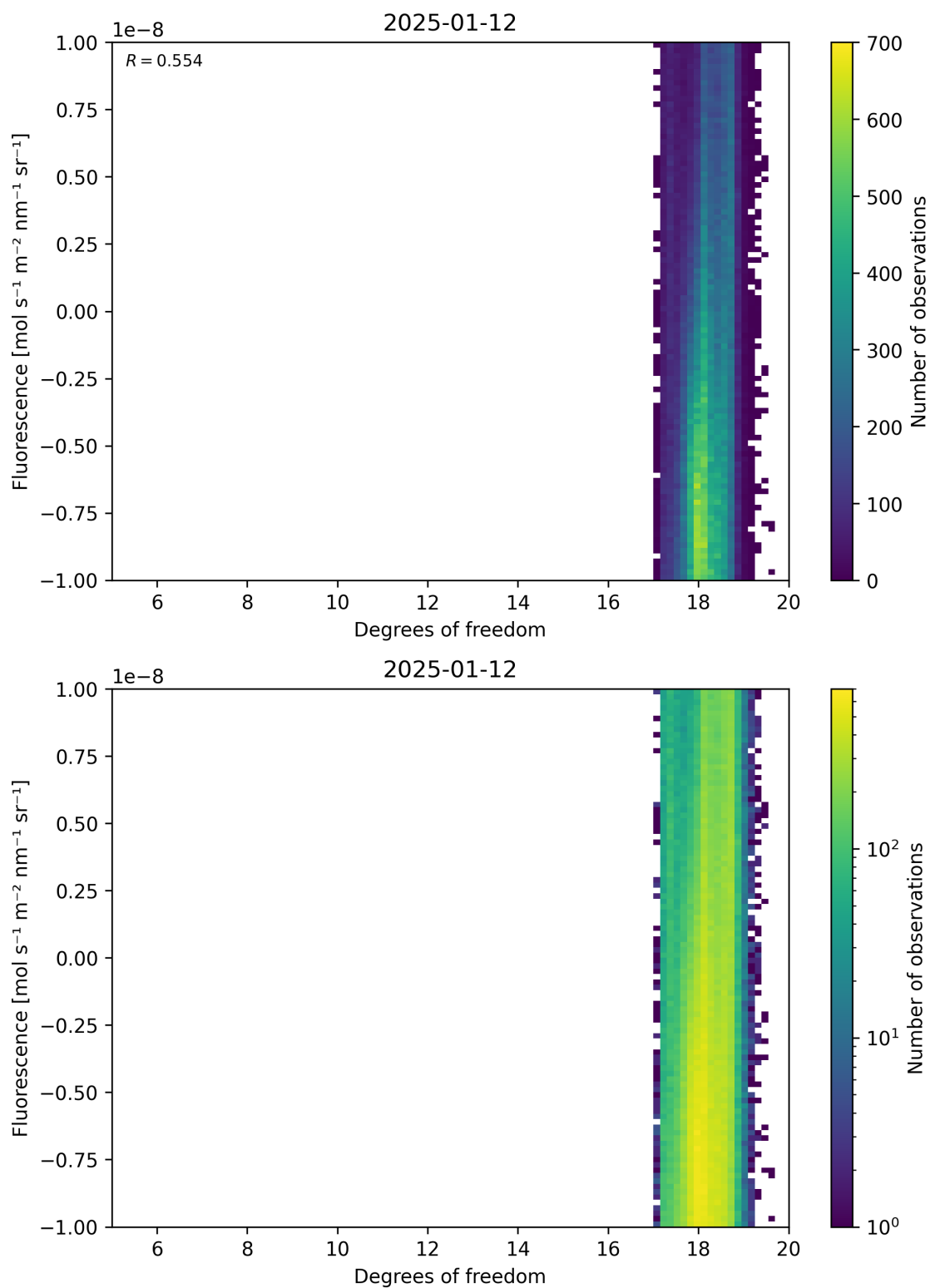
Figure 51: Scatter density plot of “Degrees of freedom” against “Fluorescence” for 2025-01-12 to 2025-01-13.
