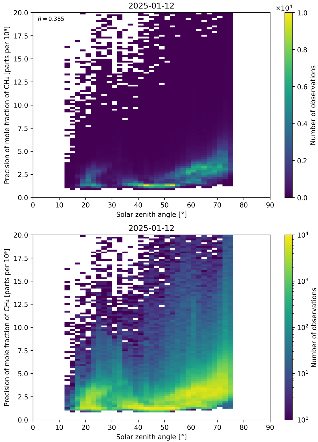
Figure 101: Scatter density plot of “Solar zenith angle” against “Precision of mole fraction of CH 4 ” for 2025-01-12 to 2025-01-13.
