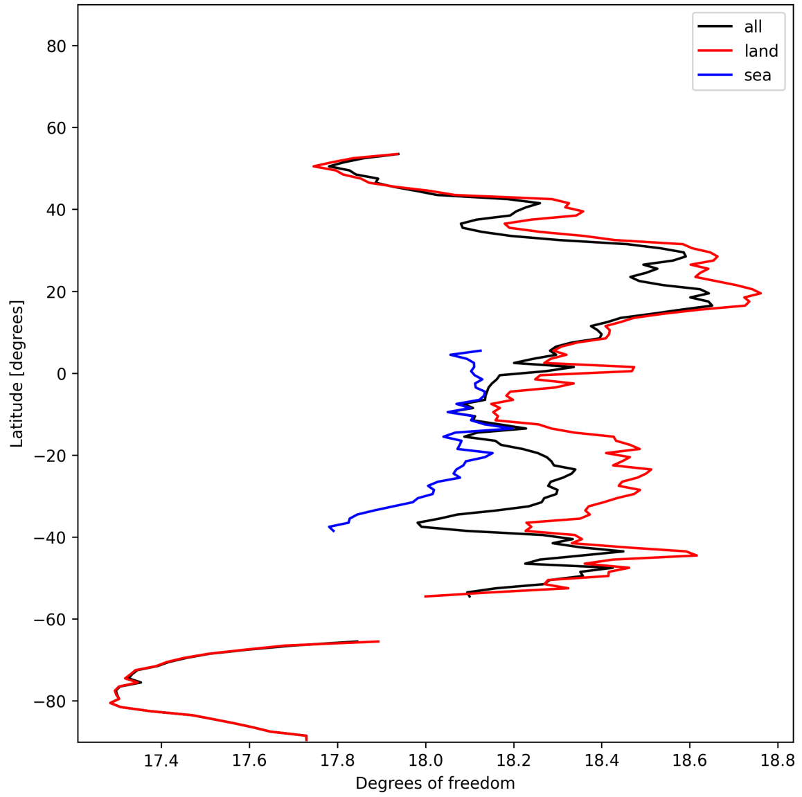
Figure 19: Zonal average of “Degrees of freedom” for 2025-01-12 to 2025-01-13.
