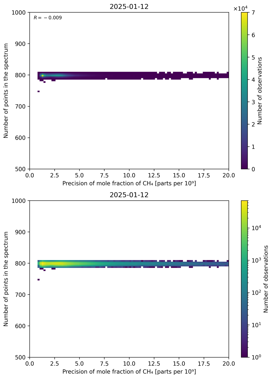
Figure 84: Scatter density plot of “Precision of mole fraction of CH 4 ” against “Number of points in the spectrum” for 2025-01-12 to 2025-01-13.
