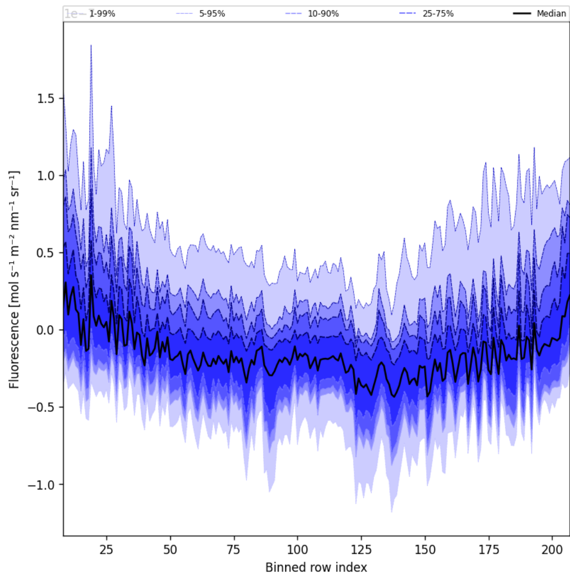
Figure 43: Along track statistics of "Fluorescence" for 2025-01-12 to 2025-01-13
