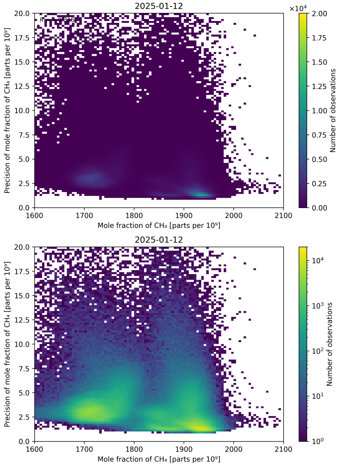
Figure 75: Scatter density plot of “Mole fraction of CH 4 ” against “Precision of mole fraction of CH 4 ” for 2025-01-12 to 2025-01-13.
