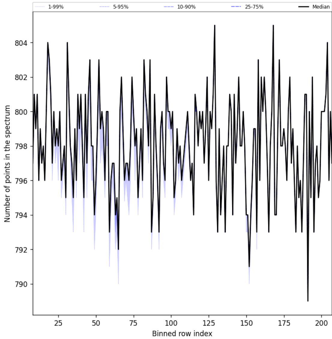
Figure 37: Along track statistics of “Number of points in the spectrum” for 2025-01-12 to 2025-01-13
