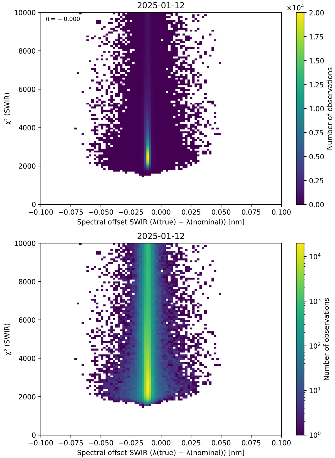
Figure 118: Scatter density plot of “Spectral offset SWIR ( \lambda_{\text{true}} - \lambda_{\text{nominal}} )” against “ \chi^2 (SWIR)” for 2025-01-12 to 2025-01-13.
