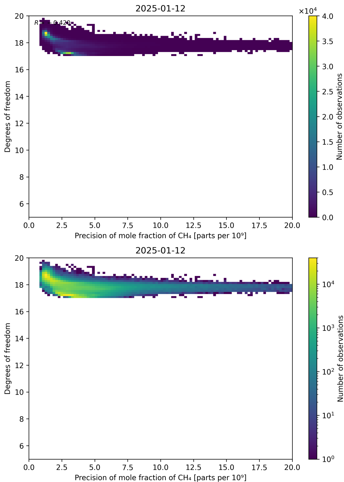
Figure 80: Scatter density plot of “Precision of mole fraction of CH 4 ” against “Degrees of freedom” for 2025-01-12 to 2025-01-13.
