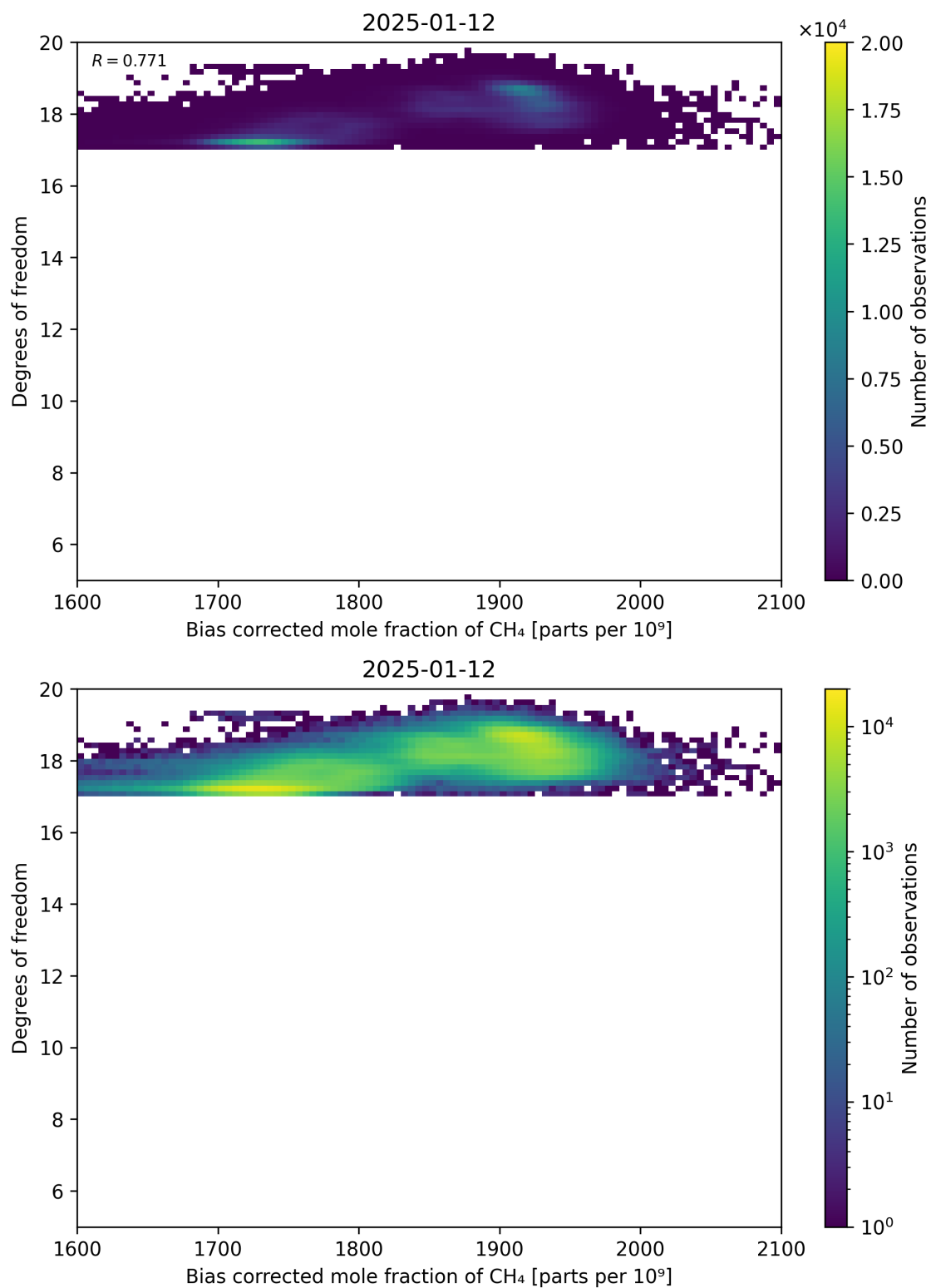
Figure 65: Scatter density plot of “Bias corrected mole fraction of CH 4 ” against “Degrees of freedom” for 2025-01-12 to 2025-01-13.
