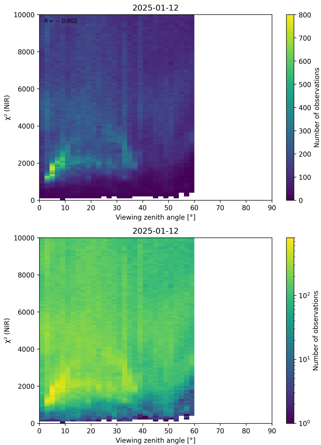
Figure 105: Scatter density plot of “Viewing zenith angle” against “ \chi^2 (NIR)” for 2025-01-12 to 2025-01-13.
