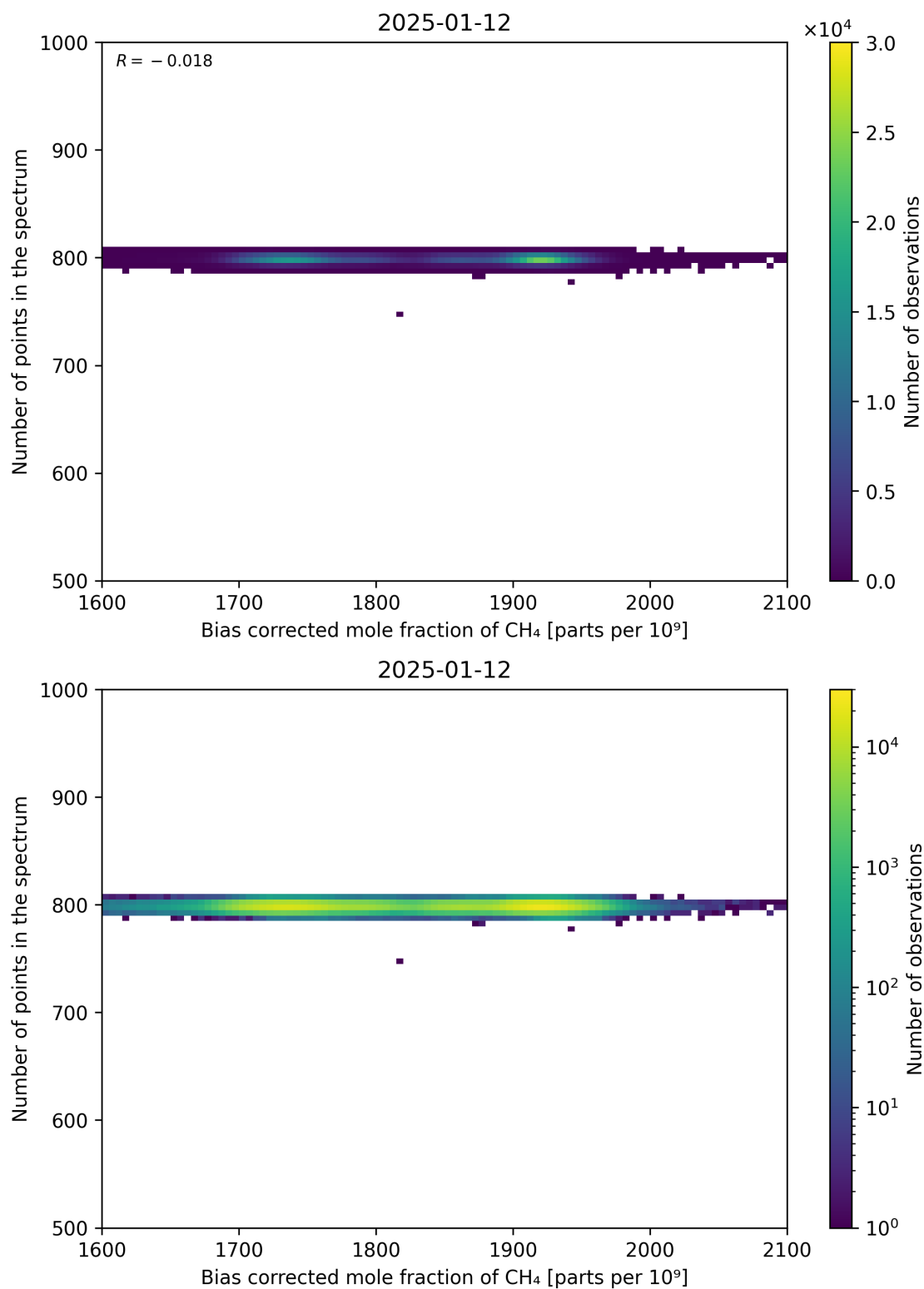
Figure 68: Scatter density plot of “Bias corrected mole fraction of CH 4 ” against “Number of points in the spectrum” for 2025-01-12 to 2025-01-13.
