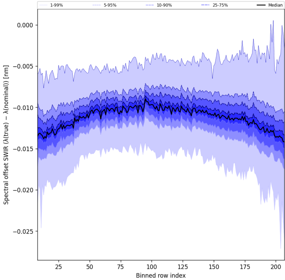
Figure 38: Along track statistics of “Spectral offset SWIR ( \lambda_{\text{true}} - \lambda_{\text{nominal}} )” for 2025-01-12 to 2025-01-13
