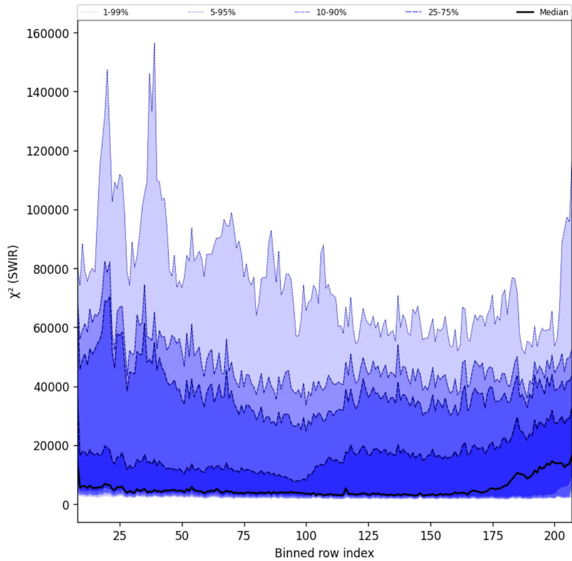
Figure 39: Along track statistics of “ \chi^2 (SWIR)” for 2025-01-12 to 2025-01-13
