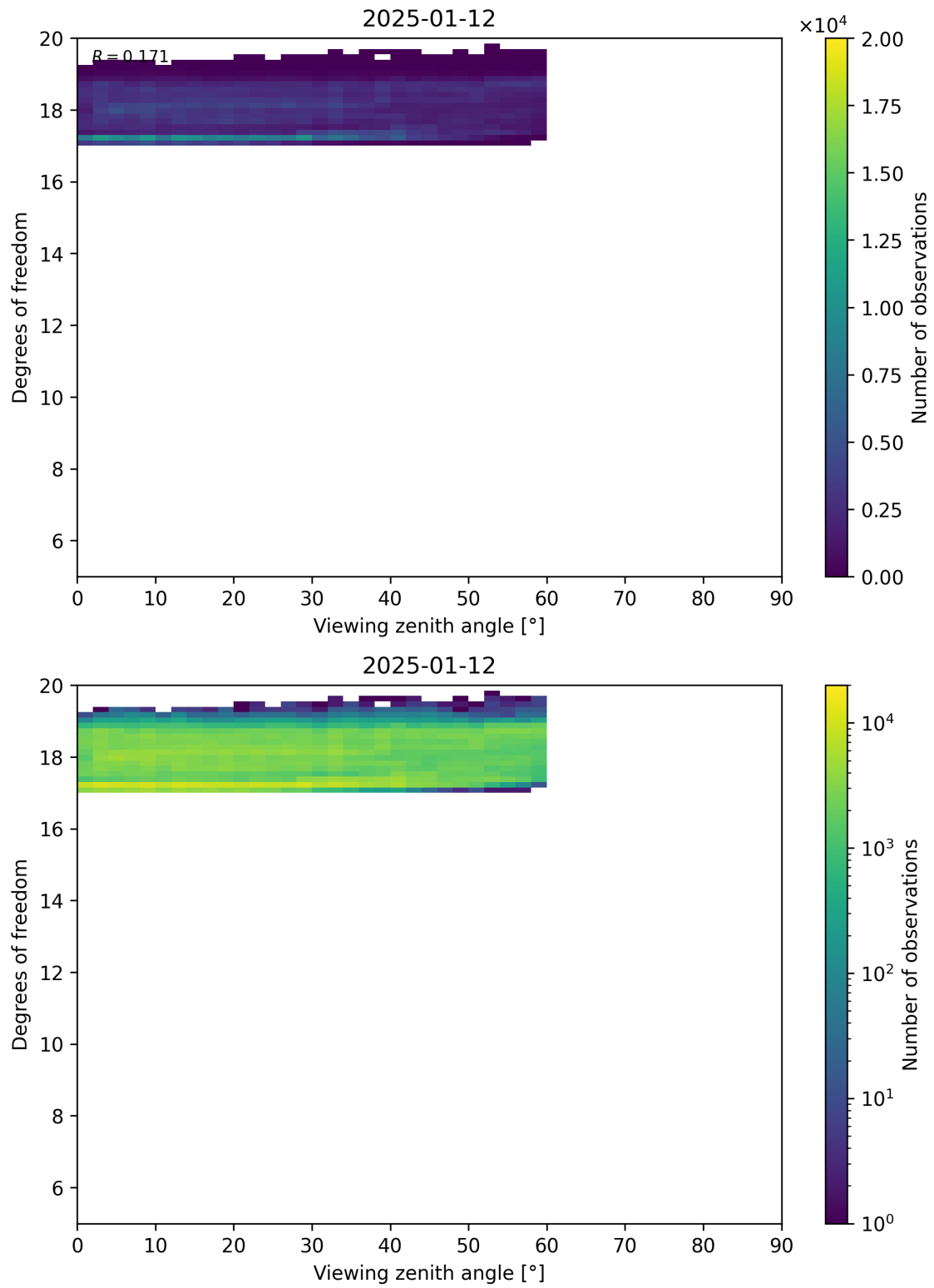
Figure 107: Scatter density plot of “Viewing zenith angle” against “Degrees of freedom” for 2025-01-12 to 2025-01-13.
