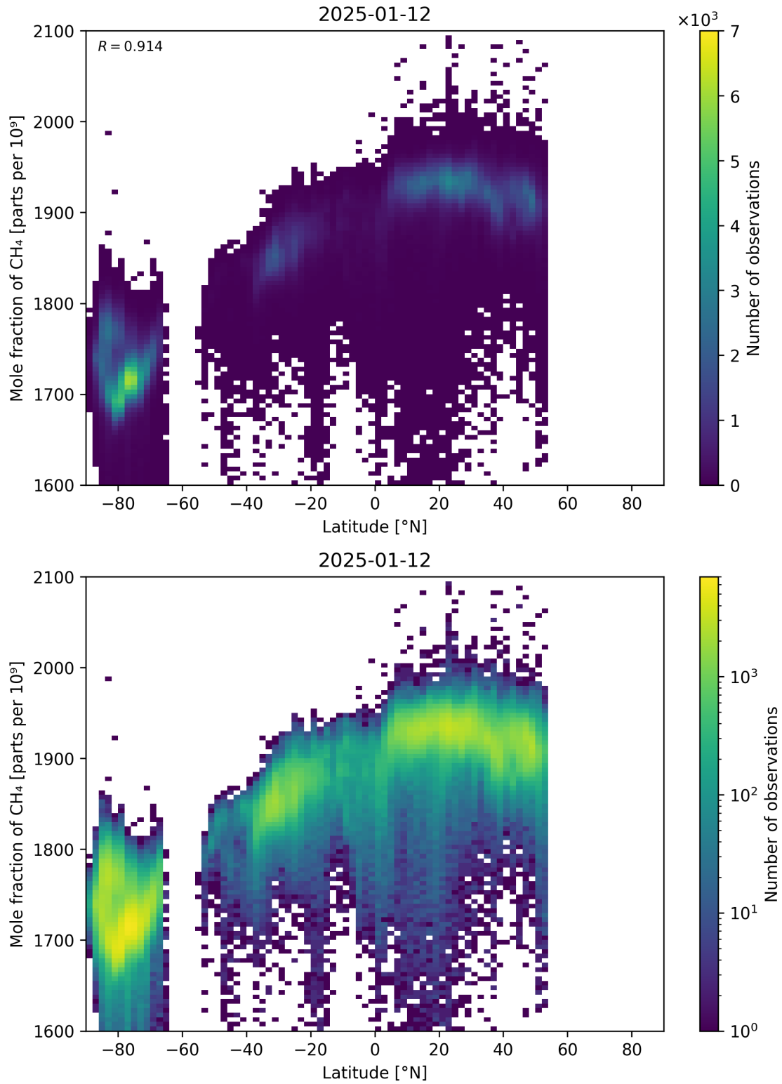
Figure 57: Scatter density plot of “Latitude” against “Mole fraction of CH 4 ” for 2025-01-12 to 2025-01-13.
