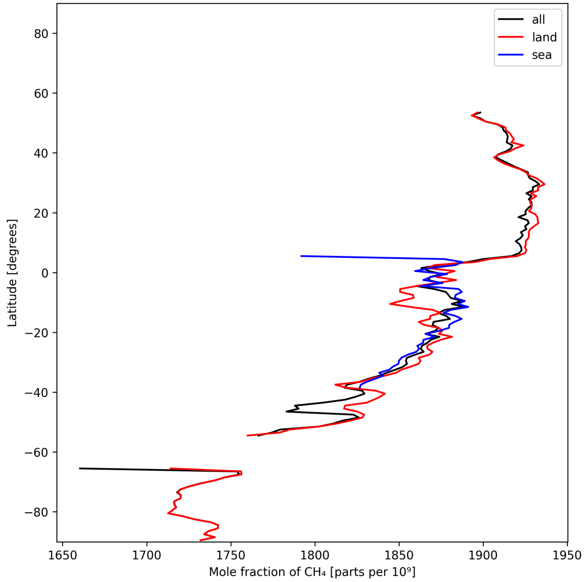
Figure 12: Zonal average of “Mole fraction of CH 4 ” for 2025-01-12 to 2025-01-13.
