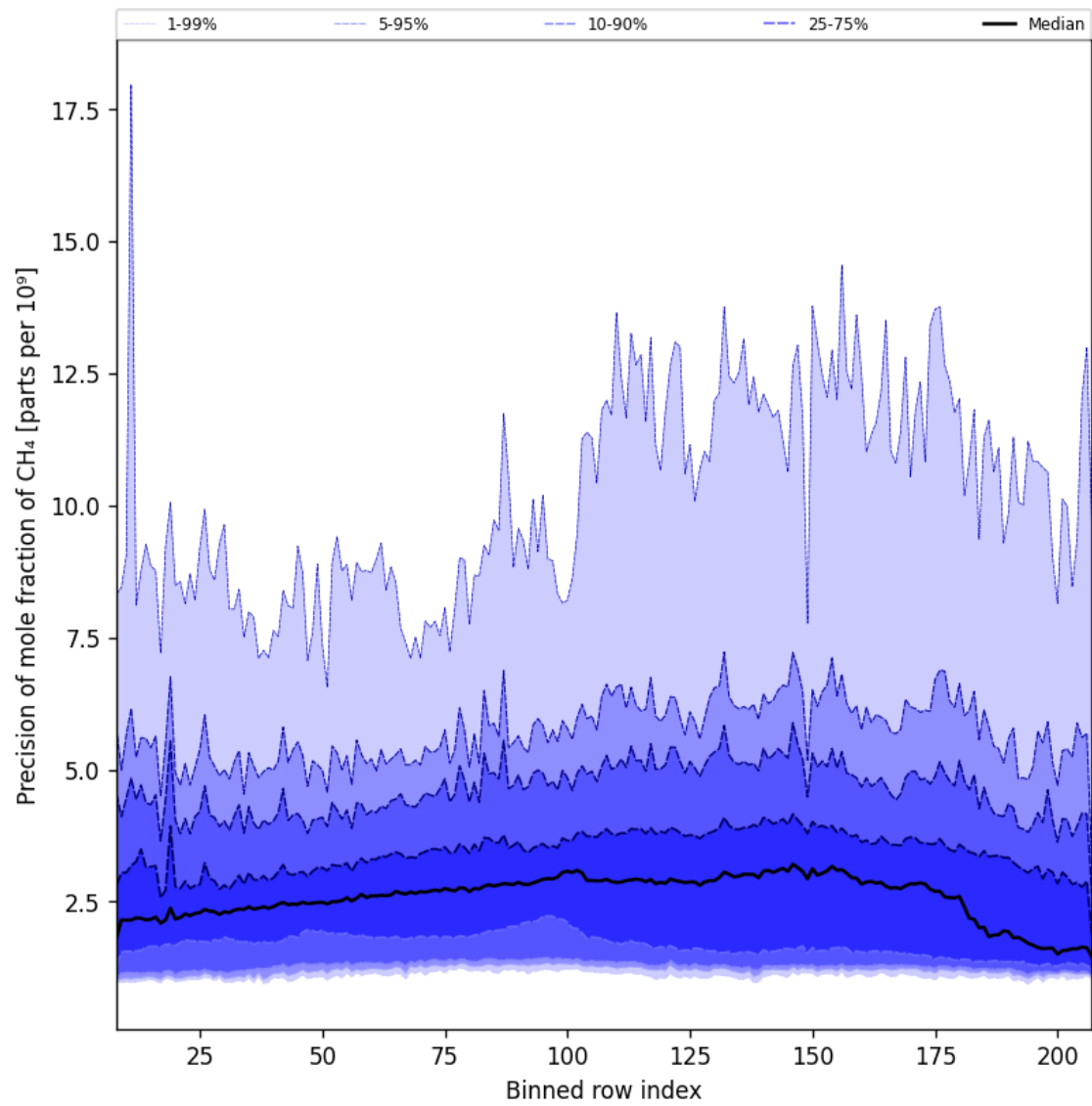
Figure 35: Along track statistics of “Precision of mole fraction of CH 4 ” for 2025-01-12 to 2025-01-13
