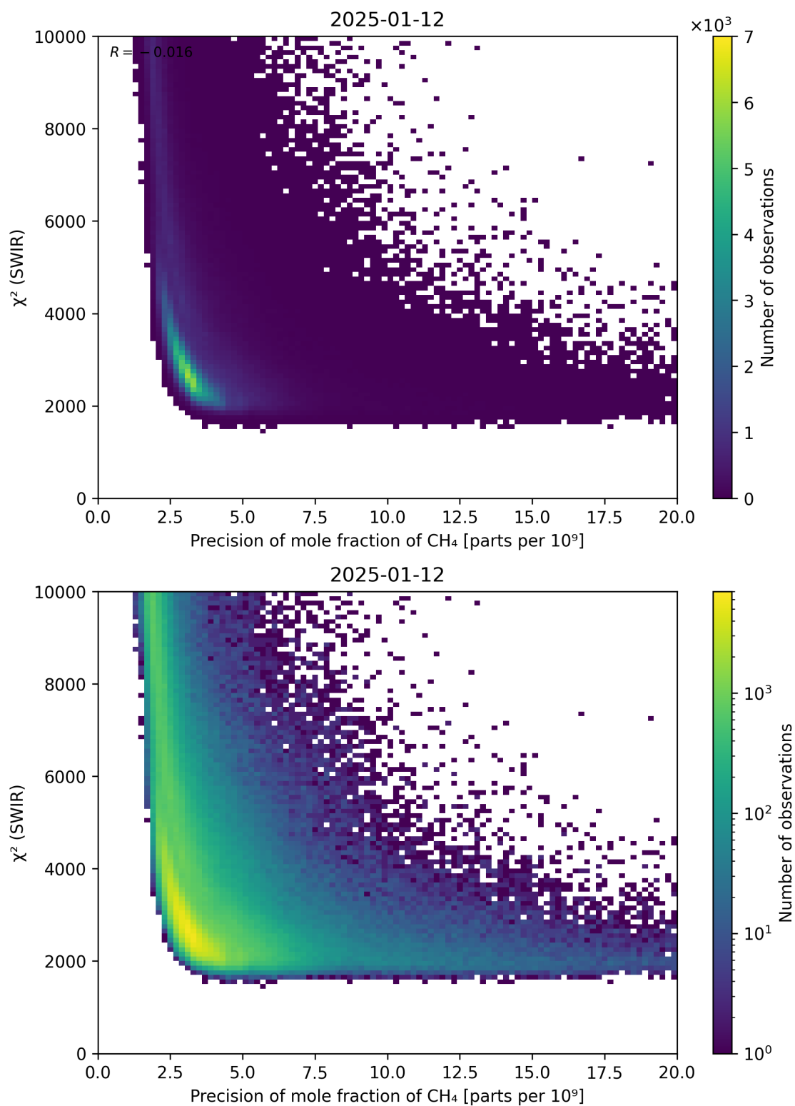
Figure 79: Scatter density plot of “Precision of mole fraction of \text{CH}_4 ” against “ \chi^2 (SWIR)” for 2025-01-12 to 2025-01-13.
