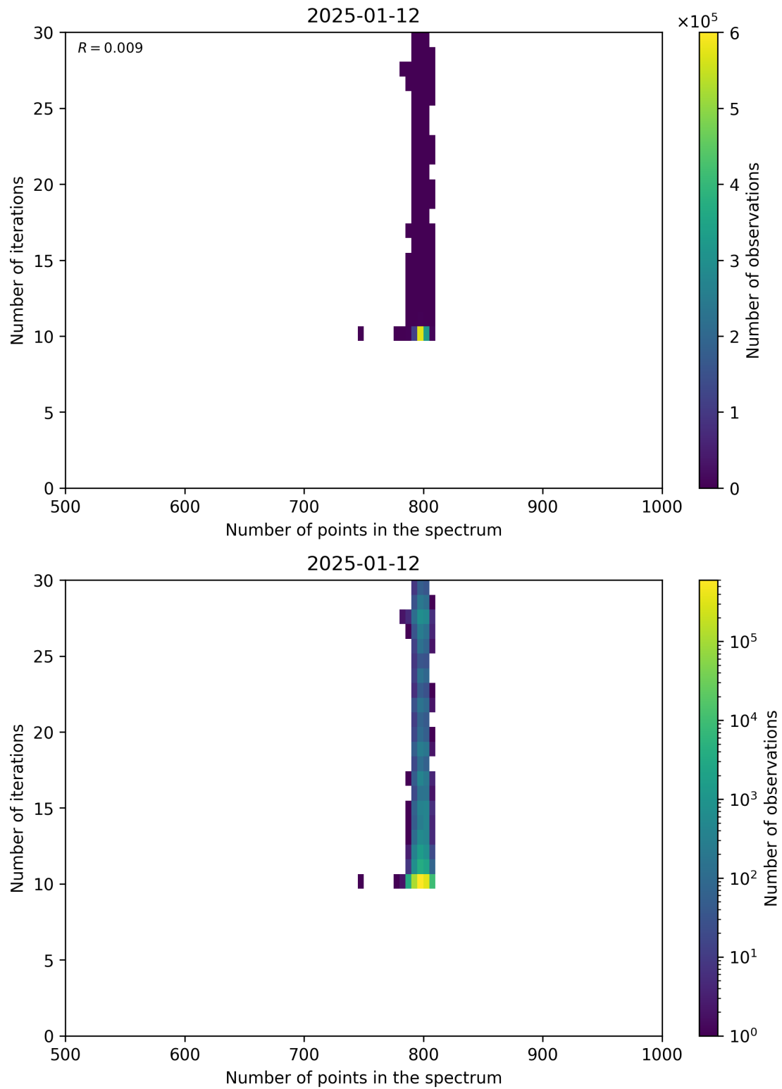
Figure 92: Scatter density plot of “Number of points in the spectrum” against “Number of iterations” for 2025-01-12 to 2025-01-13.
