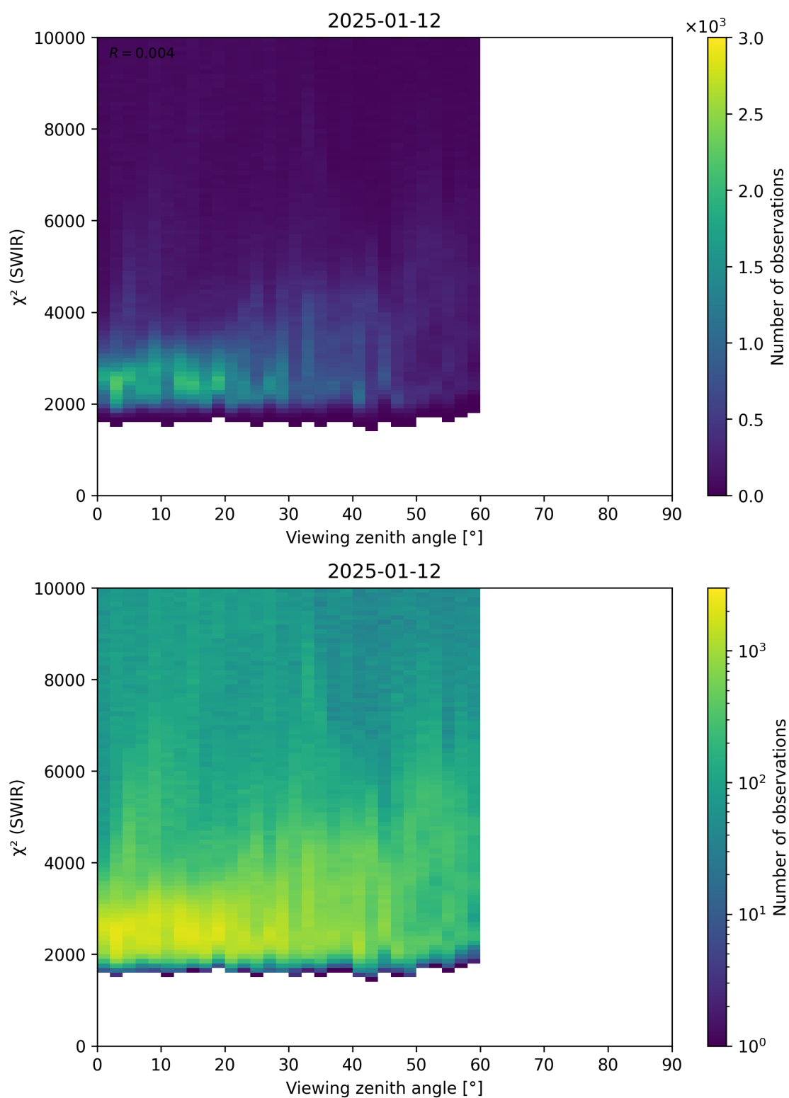
Figure 106: Scatter density plot of “Viewing zenith angle” against “ \chi^2 (SWIR)” for 2025-01-12 to 2025-01-13.
