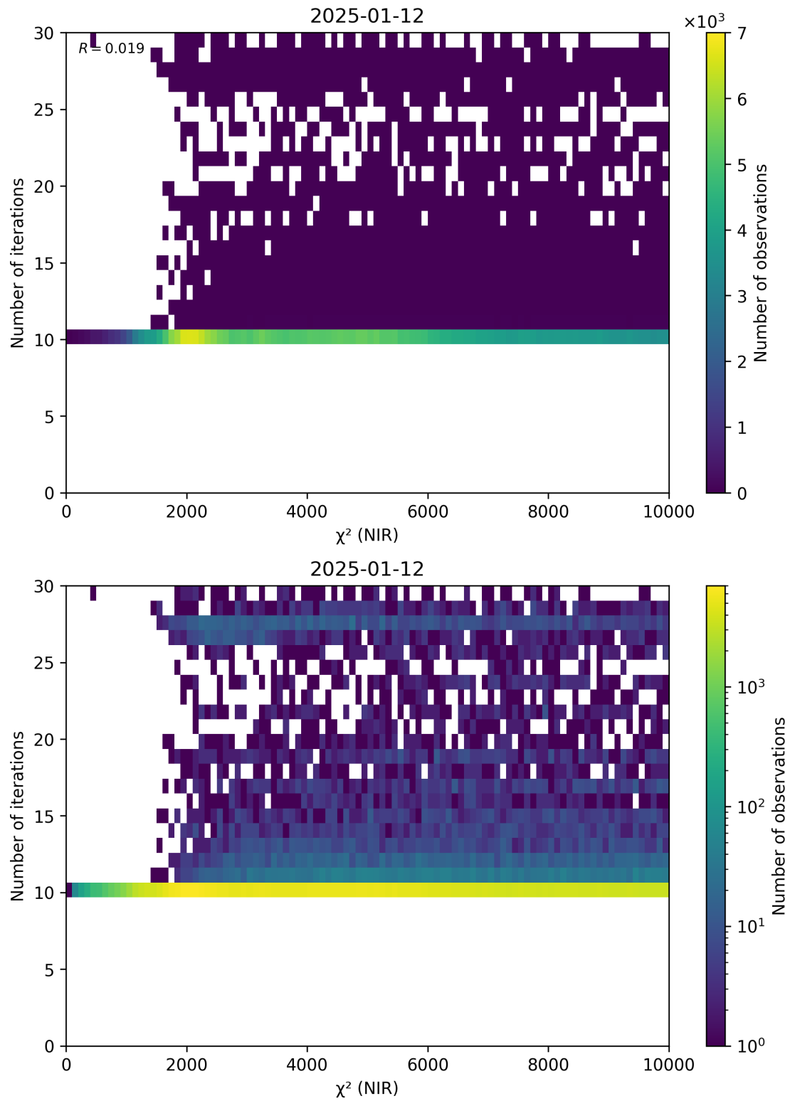
Figure 46: Scatter density plot of “ \chi^2 (NIR)” against “Number of iterations” for 2025-01-12 to 2025-01-13.
