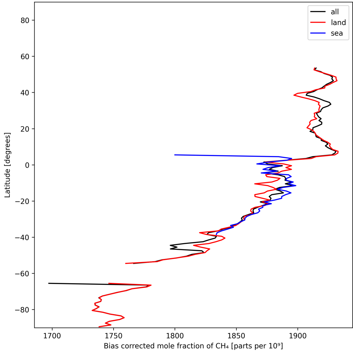
Figure 14: Zonal average of “Bias corrected mole fraction of CH 4 ” for 2025-01-12 to 2025-01-13.
