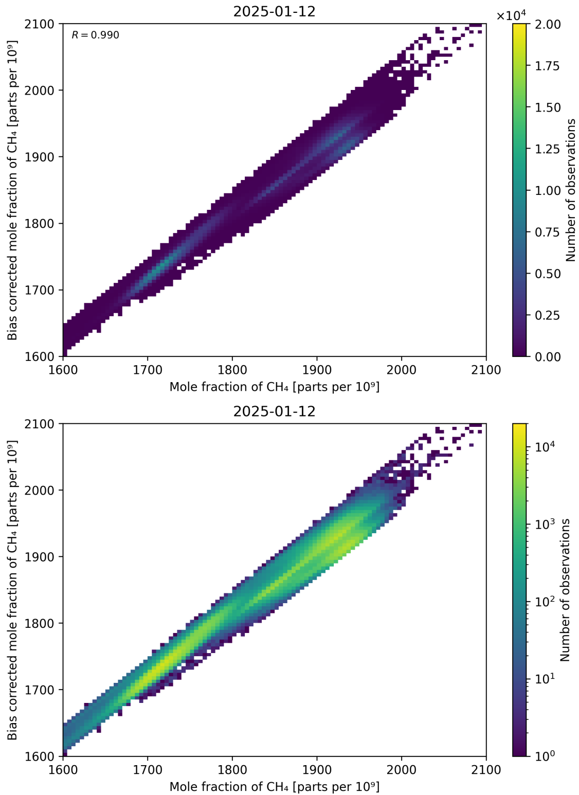
Figure 74: Scatter density plot of “Mole fraction of CH 4 ” against “Bias corrected mole fraction of CH 4 ” for 2025-01-12 to 2025-01-13.
