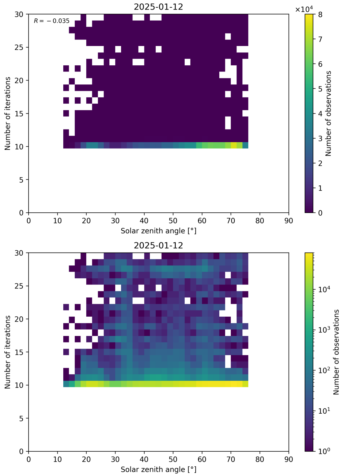
Figure 102: Scatter density plot of “Solar zenith angle” against “Number of iterations” for 2025-01-12 to 2025-01-13.
