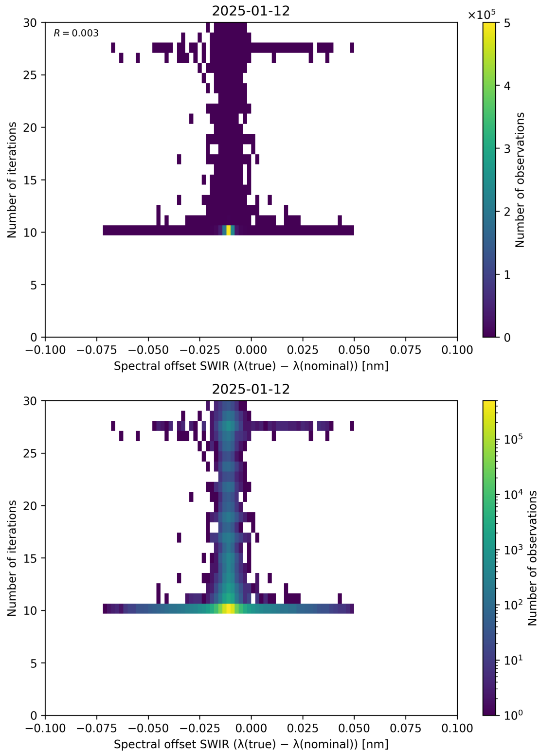
Figure 121: Scatter density plot of “Spectral offset SWIR ( \lambda_{\text{true}} - \lambda_{\text{nominal}} )” against “Number of iterations” for 2025-01-12 to 2025-01-13.
