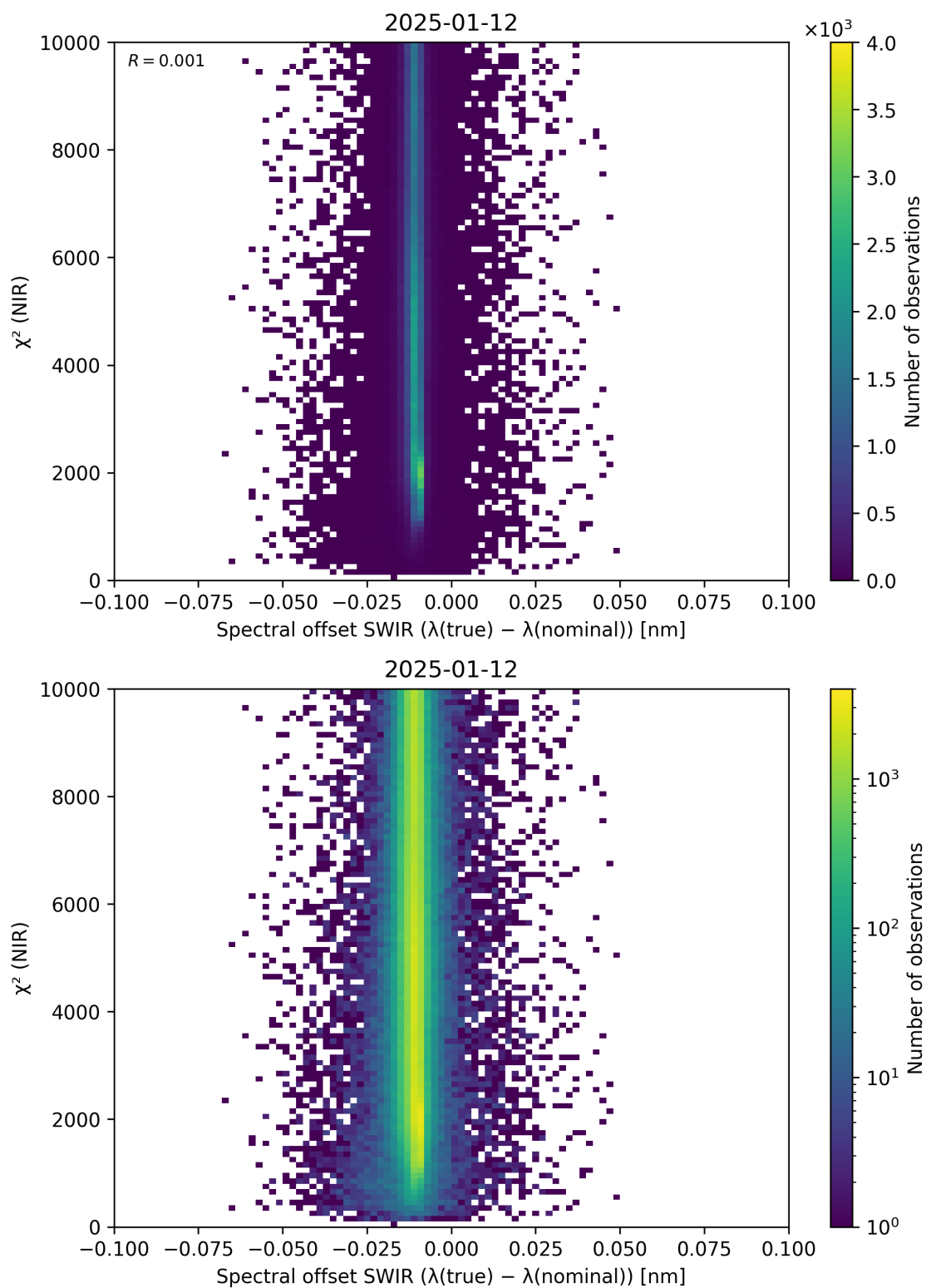
Figure 117: Scatter density plot of “Spectral offset SWIR ( \lambda_{\text{true}} - \lambda_{\text{nominal}} )” against “ \chi^2 (NIR)” for 2025-01-12 to 2025-01-13.
