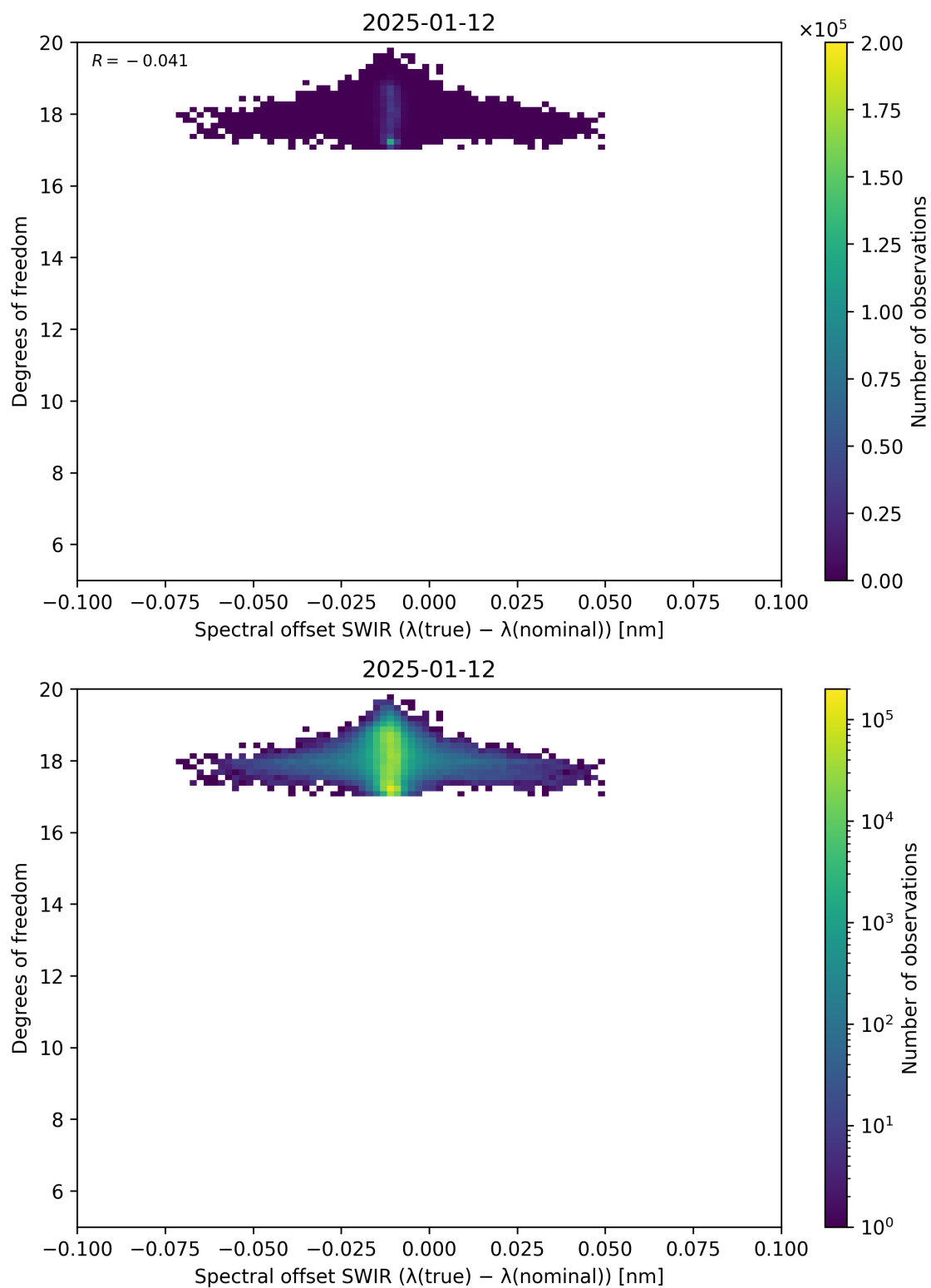
Figure 119: Scatter density plot of “Spectral offset SWIR ( \lambda_{\text{true}} - \lambda_{\text{nominal}} )” against “Degrees of freedom” for 2025-01-12 to 2025-01-13.
