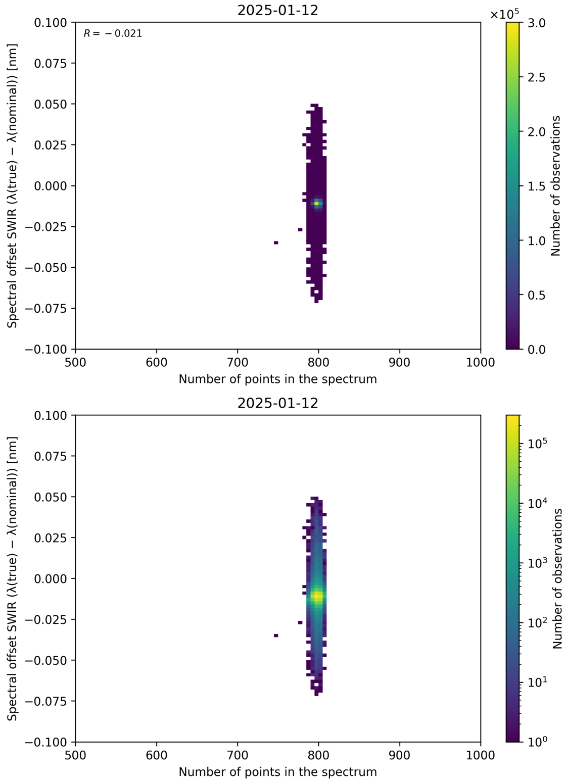
Figure 93: Scatter density plot of “Number of points in the spectrum” against “Spectral offset SWIR ( \lambda_{\text{true}} - \lambda_{\text{nominal}} )” for 2025-01-12 to 2025-01-13.
