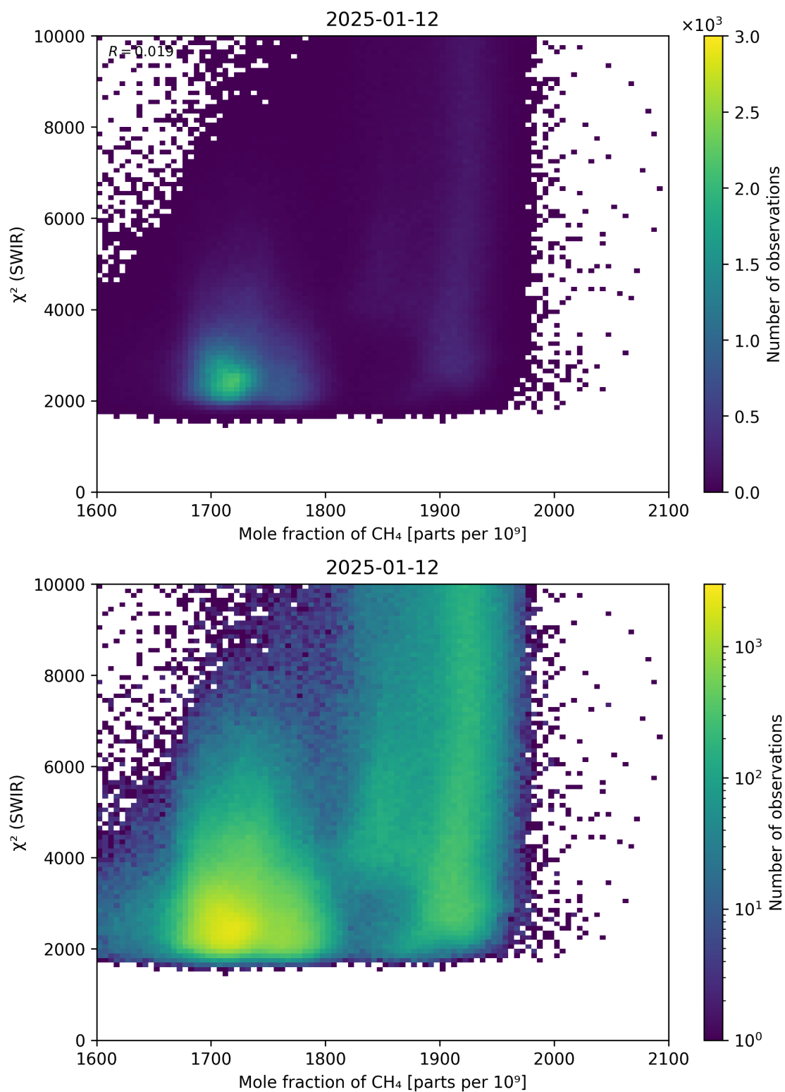
Figure 71: Scatter density plot of “Mole fraction of \text{CH}_4 ” against “ \chi^2 (SWIR)” for 2025-01-12 to 2025-01-13.
