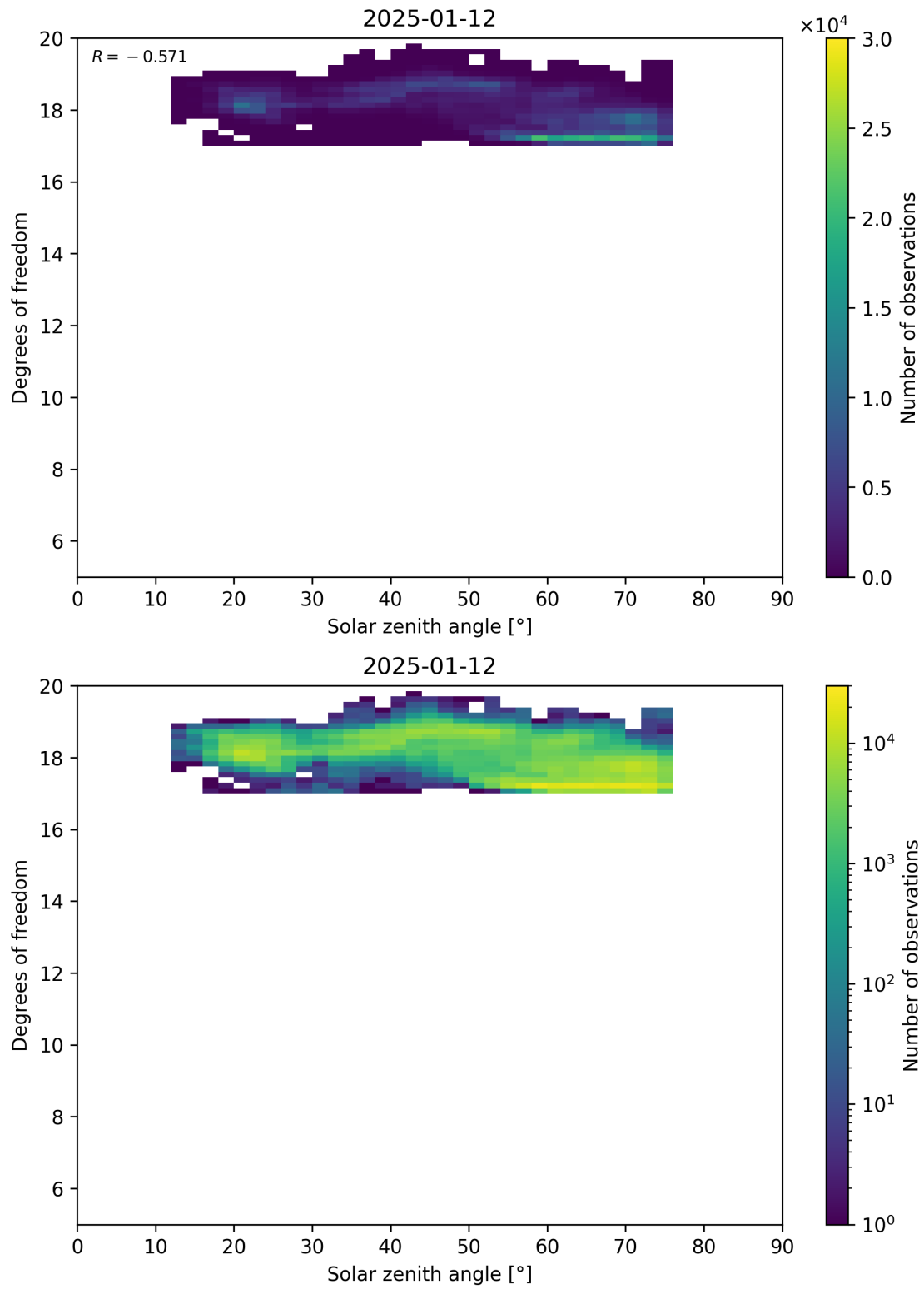
Figure 96: Scatter density plot of “Solar zenith angle” against “Degrees of freedom” for 2025-01-12 to 2025-01-13.
