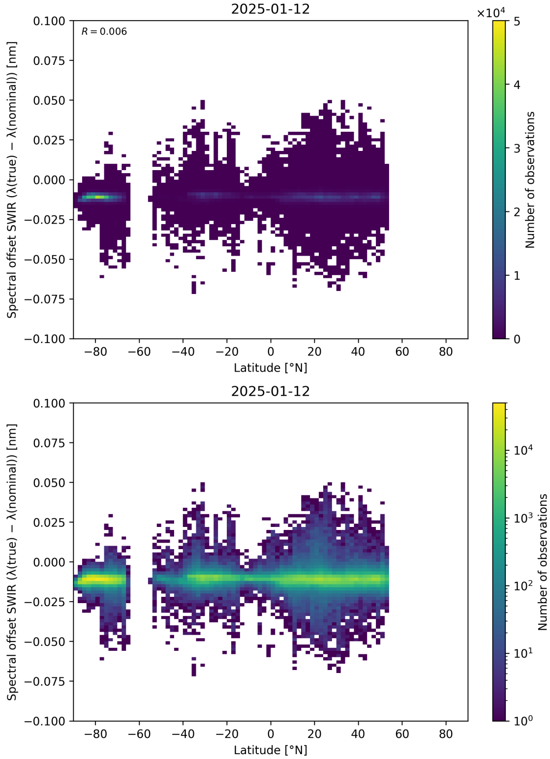
Figure 62: Scatter density plot of “Latitude” against “Spectral offset SWIR ( \lambda_{\text{true}} - \lambda_{\text{nominal}} )” for 2025-01-12 to 2025-01-13.
