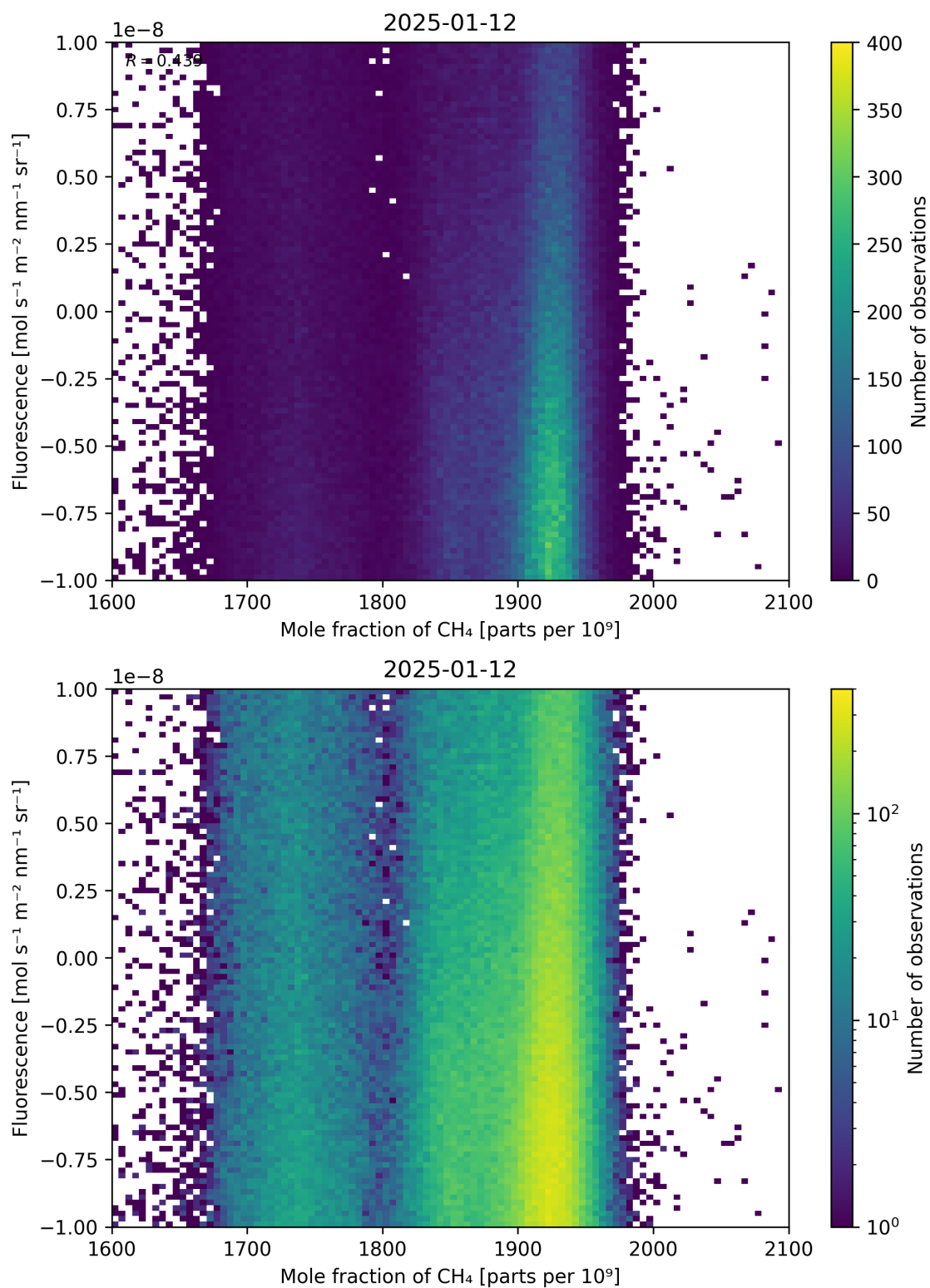
Figure 73: Scatter density plot of “Mole fraction of CH 4 ” against “Fluorescence” for 2025-01-12 to 2025-01-13.
