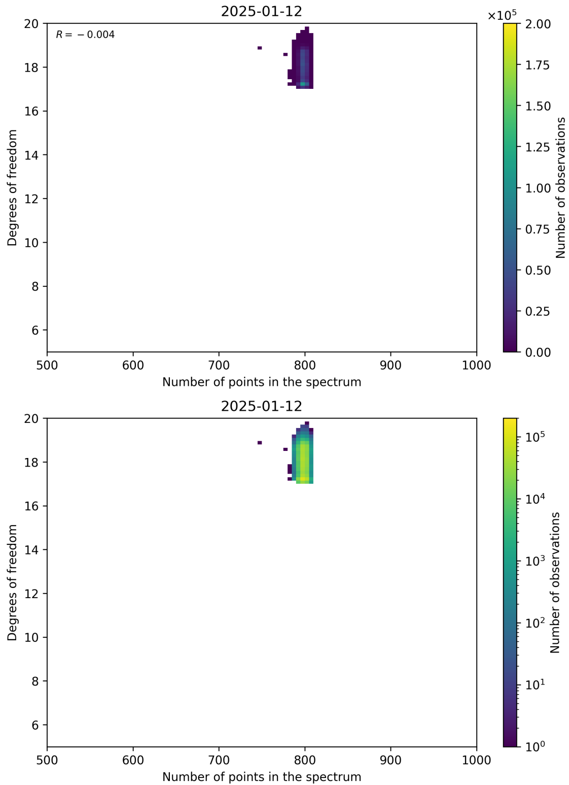
Figure 90: Scatter density plot of “Number of points in the spectrum” against “Degrees of freedom” for 2025-01-12 to 2025-01-13.
