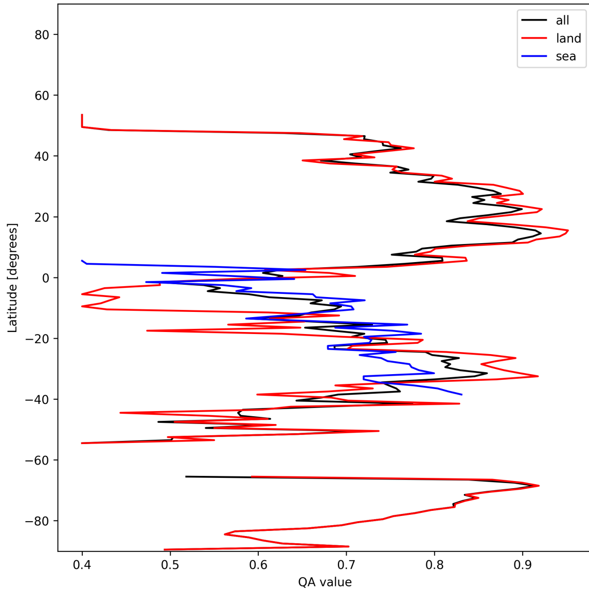
Figure 11: Zonal average of “QA value” for 2025-01-12 to 2025-01-13.
