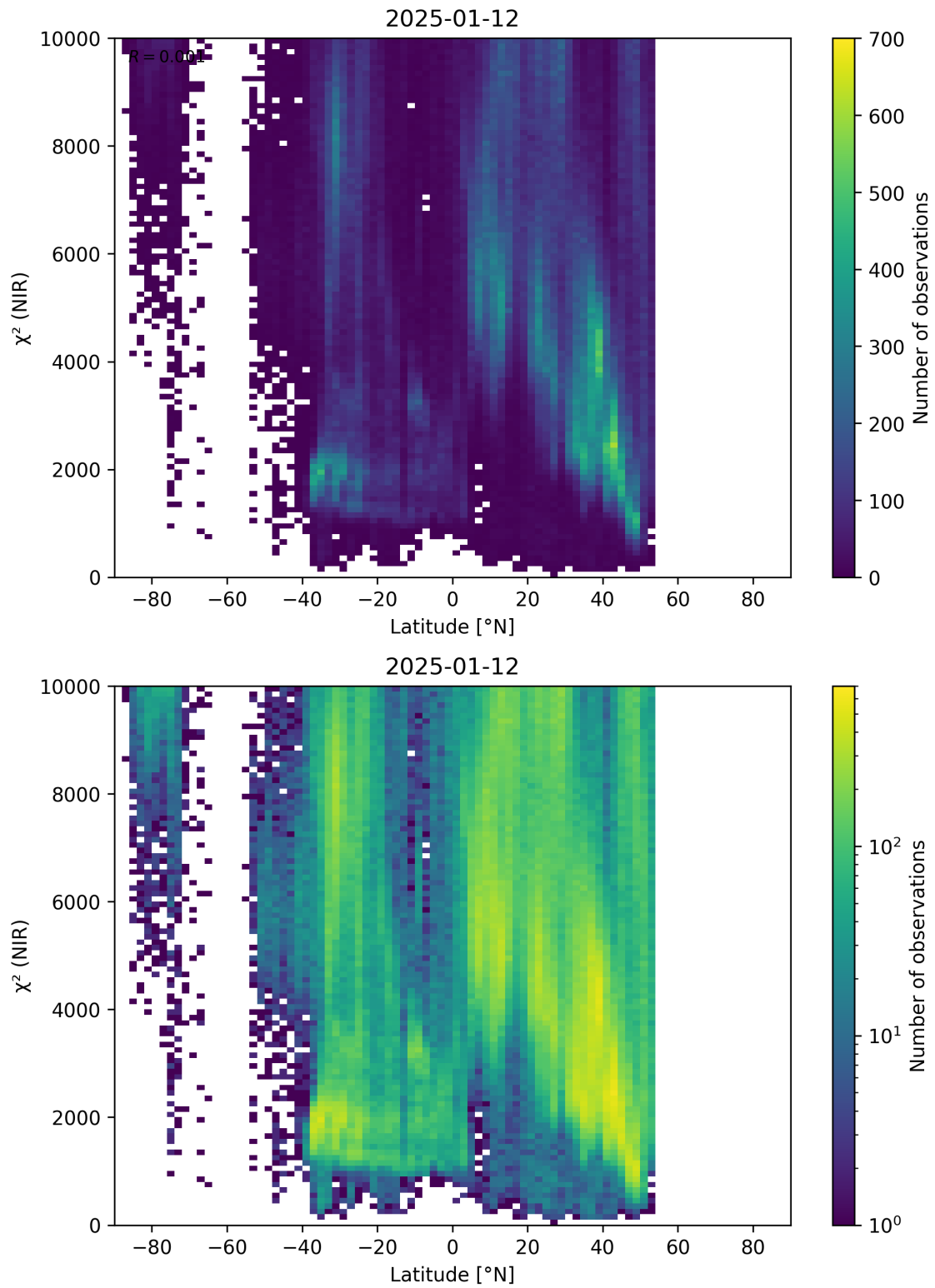
Figure 53: Scatter density plot of “Latitude” against “ \chi^2 (NIR)” for 2025-01-12 to 2025-01-13.
