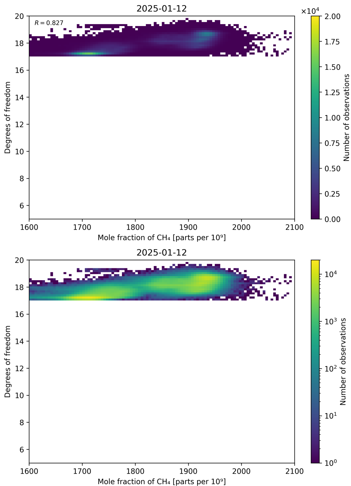
Figure 72: Scatter density plot of “Mole fraction of CH 4 ” against “Degrees of freedom” for 2025-01-12 to 2025-01-13.
