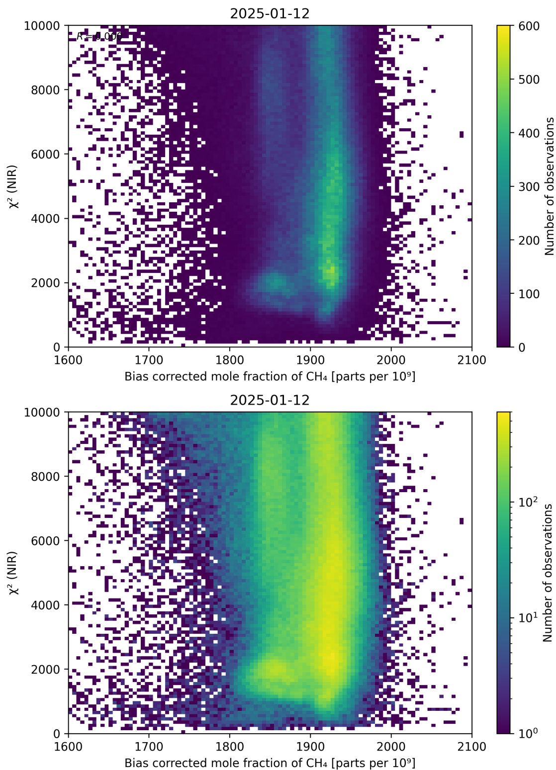
Figure 63: Scatter density plot of “Bias corrected mole fraction of CH 4 ” against “ \chi^2 (NIR)” for 2025-01-12 to 2025-01-13.
