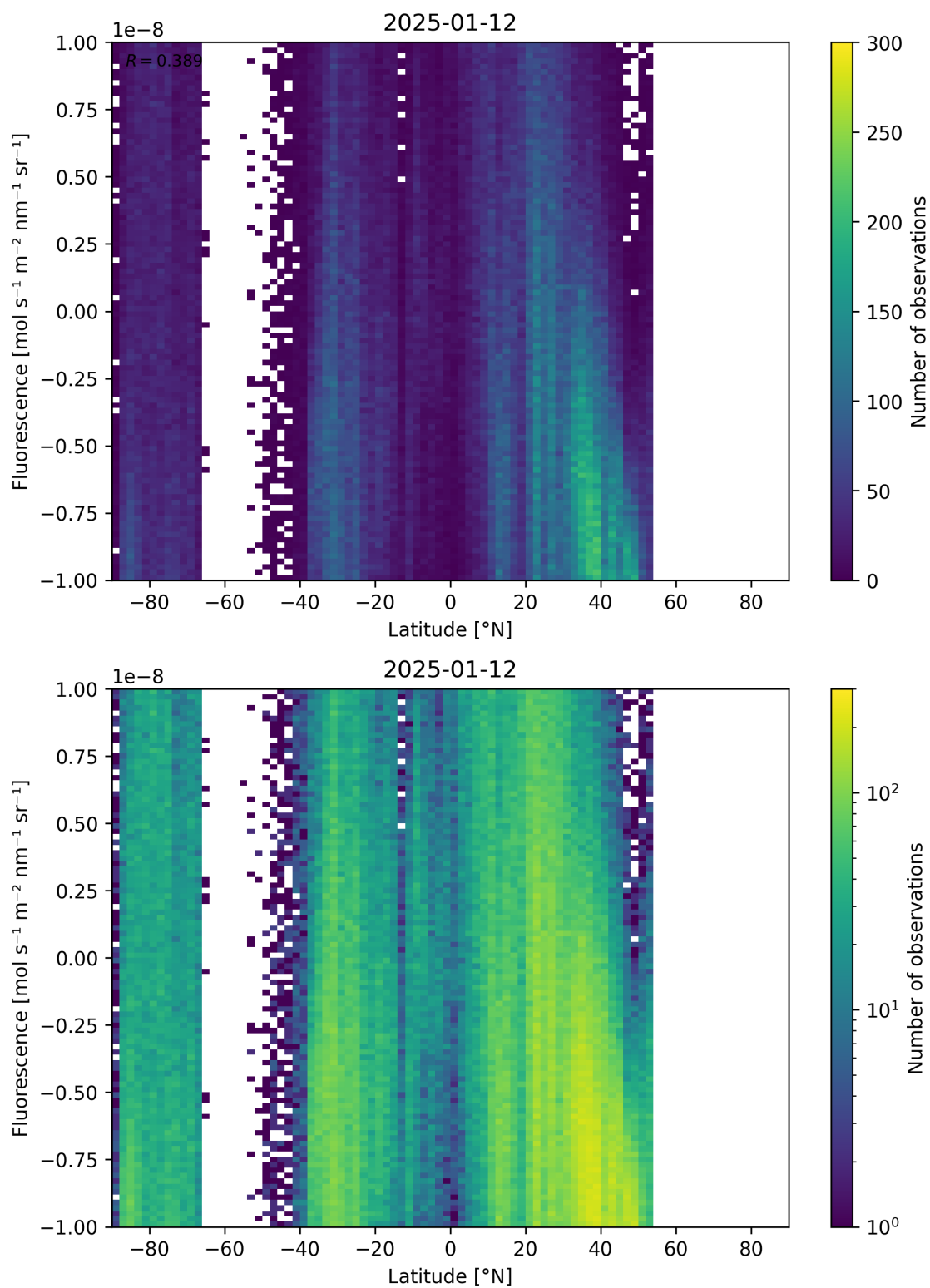
Figure 56: Scatter density plot of “Latitude” against “Fluorescence” for 2025-01-12 to 2025-01-13.
