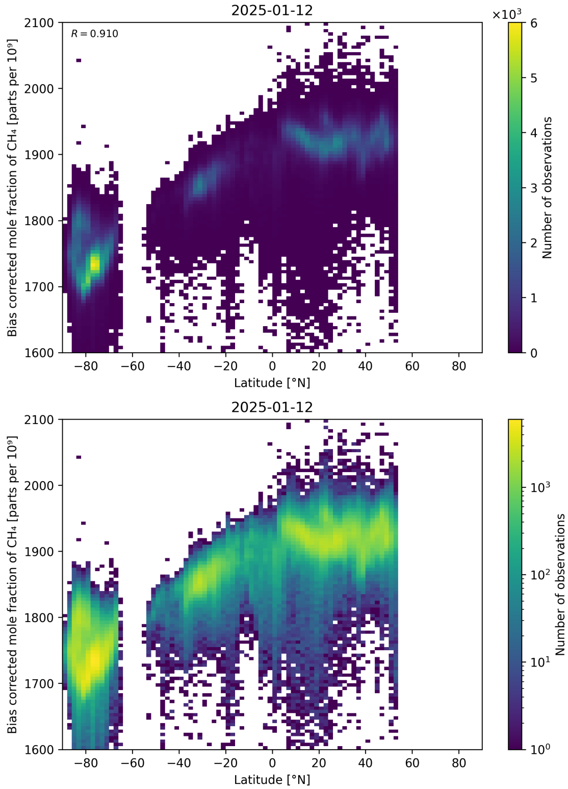
Figure 58: Scatter density plot of “Latitude” against “Bias corrected mole fraction of CH 4 ” for 2025-01-12 to 2025-01-13.
