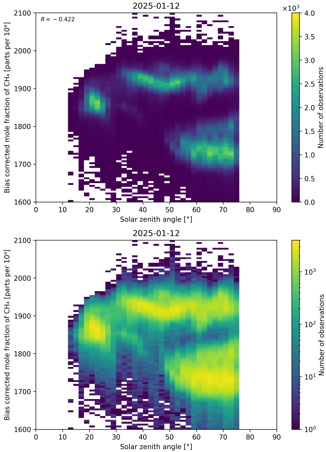
Figure 100: Scatter density plot of “Solar zenith angle” against “Bias corrected mole fraction of CH 4 ” for 2025-01-12 to 2025-01-13.
