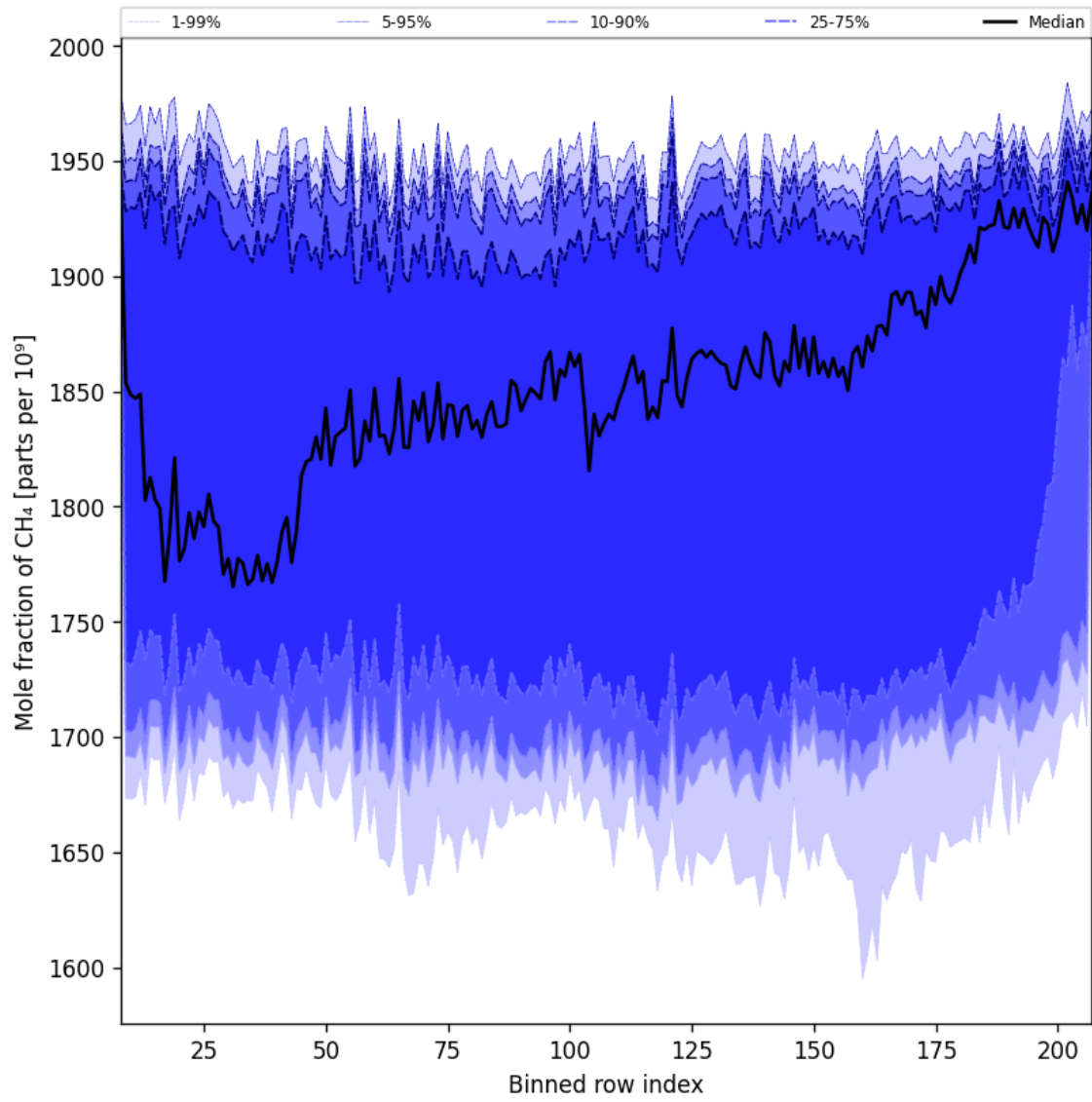
Figure 34: Along track statistics of “Mole fraction of CH 4 ” for 2025-01-12 to 2025-01-13
