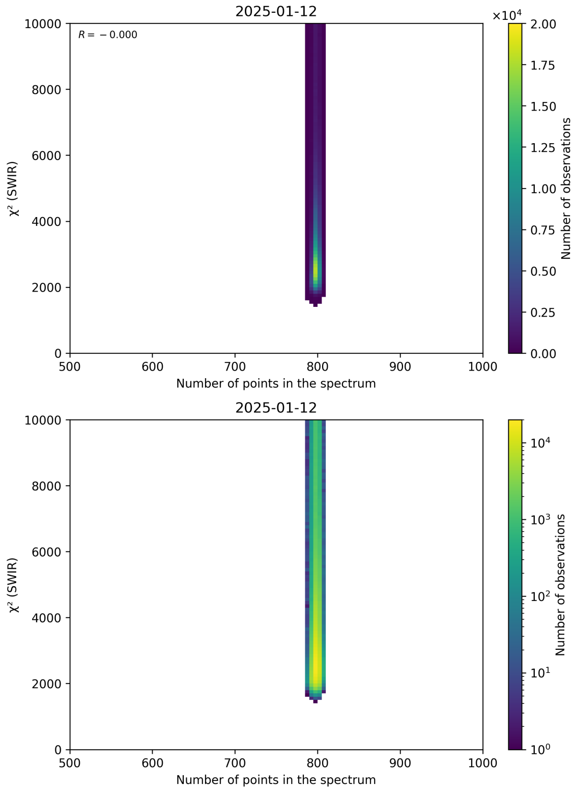
Figure 89: Scatter density plot of “Number of points in the spectrum” against “ \chi^2 (SWIR)” for 2025-01-12 to 2025-01-13.
