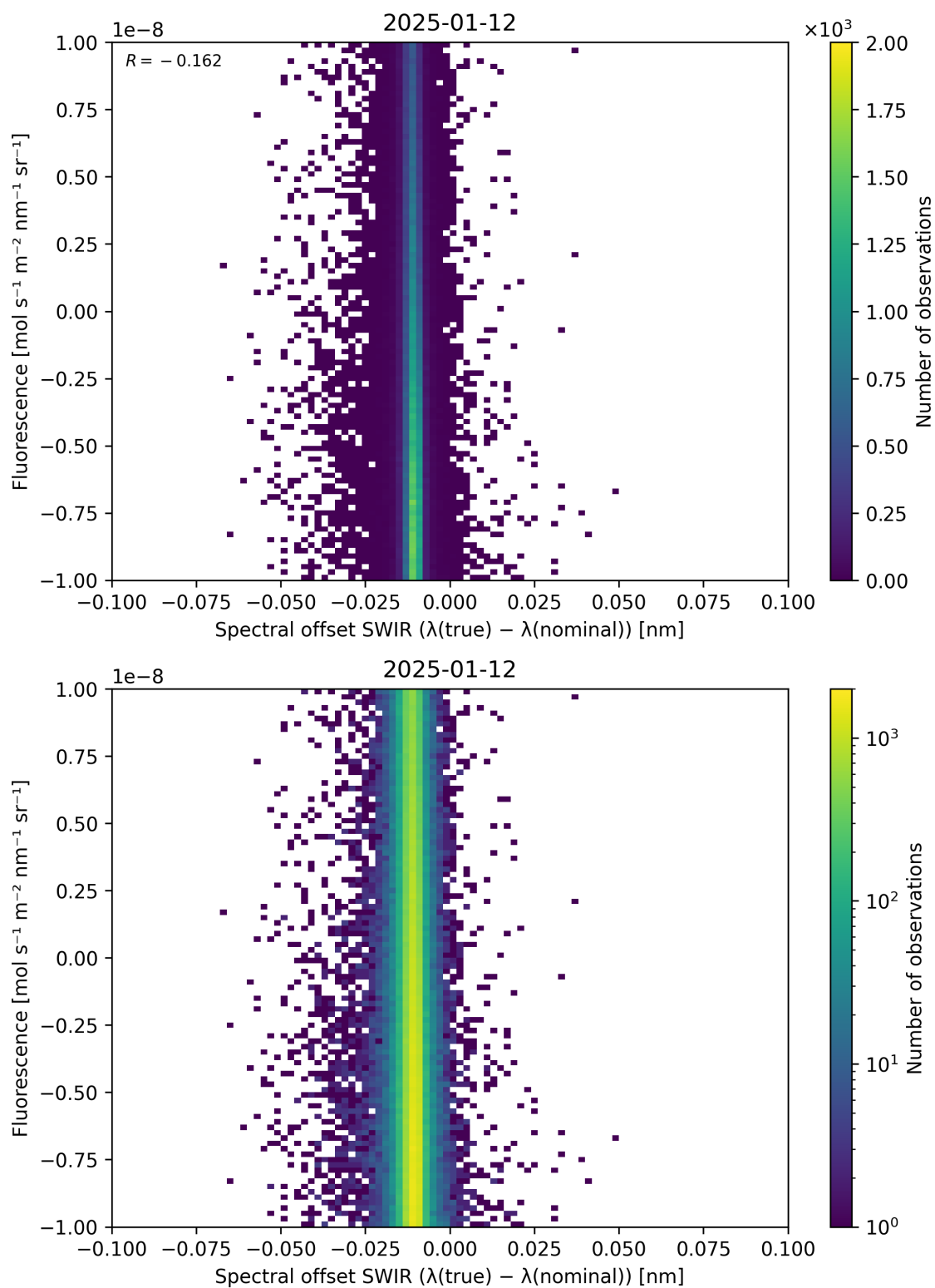
Figure 120: Scatter density plot of “Spectral offset SWIR ( \lambda_{\text{true}} - \lambda_{\text{nominal}} )” against “Fluorescence” for 2025-01-12 to 2025-01-13.
