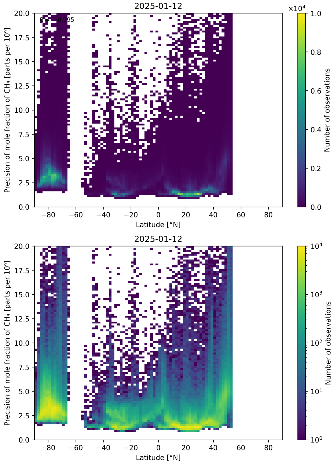
Figure 59: Scatter density plot of “Latitude” against “Precision of mole fraction of CH 4 ” for 2025-01-12 to 2025-01-13.
