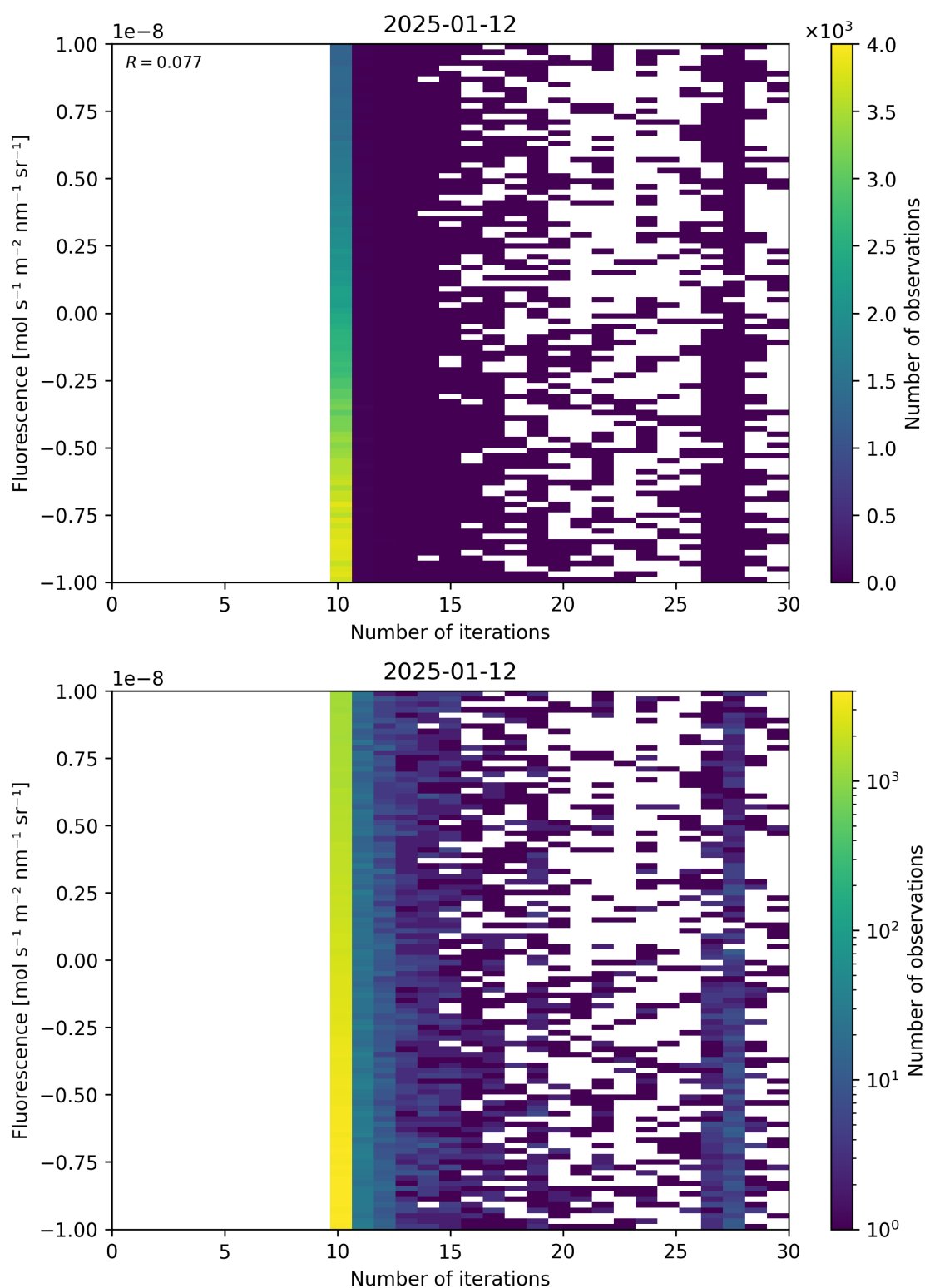
Figure 87: Scatter density plot of “Number of iterations” against “Fluorescence” for 2025-01-12 to 2025-01-13.
