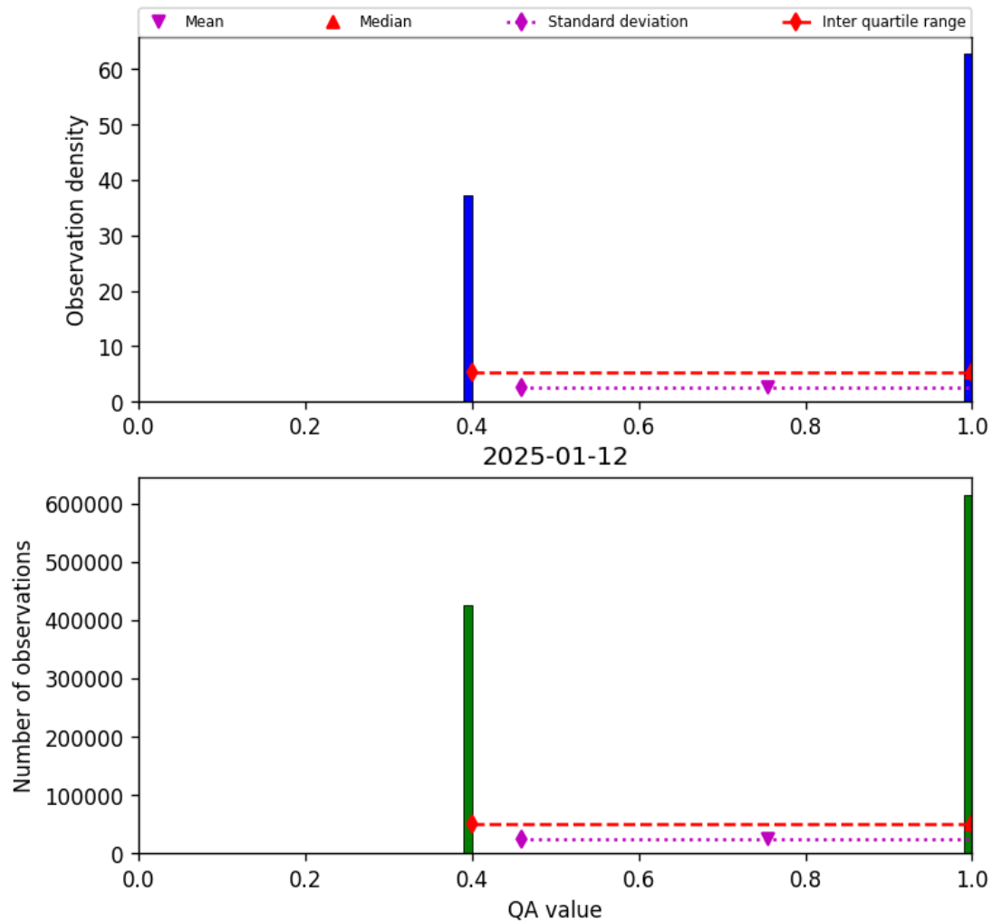
Figure 22: Histogram of “QA value” for 2025-01-12 to 2025-01-13
