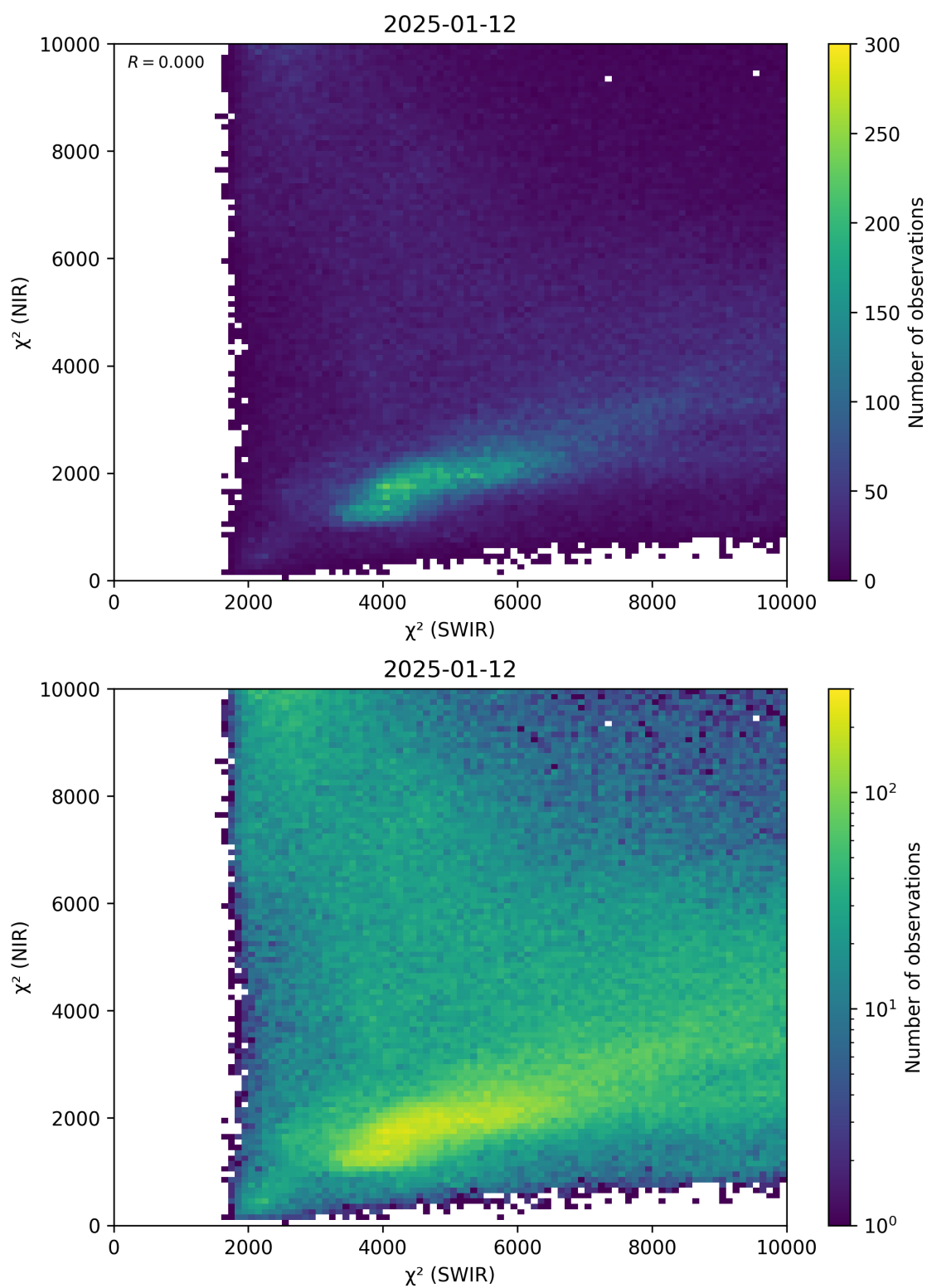
Figure 47: Scatter density plot of “ \chi^2 (SWIR)” against “ \chi^2 (NIR)” for 2025-01-12 to 2025-01-13.
