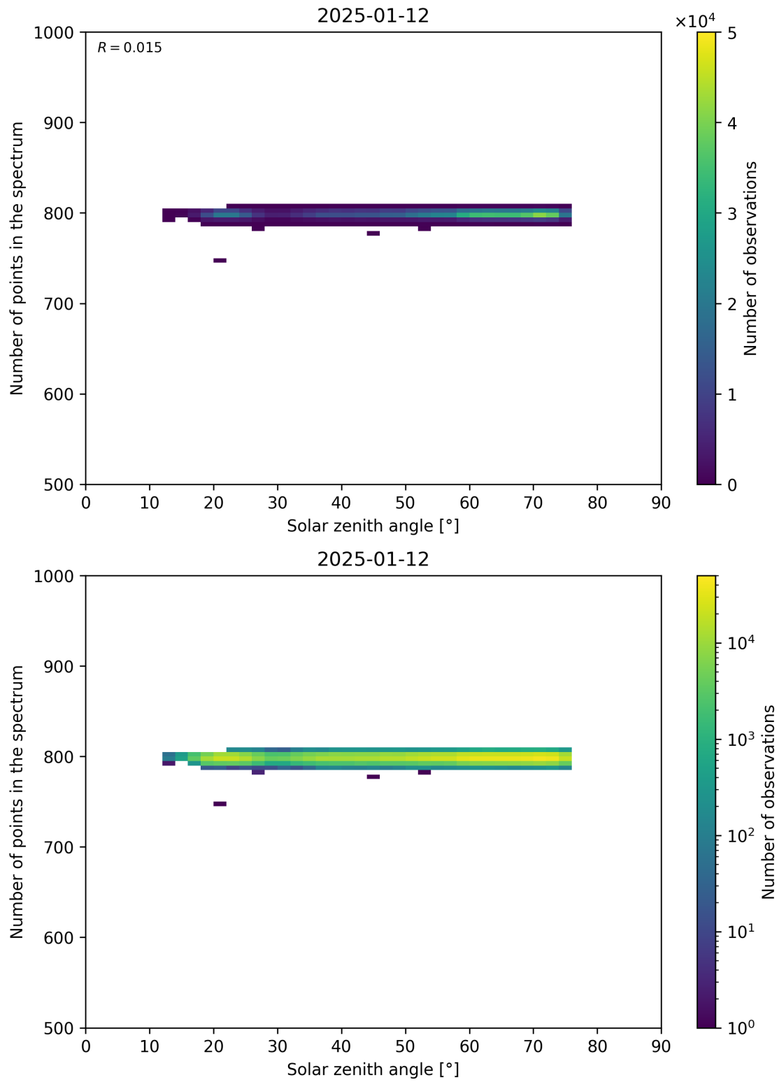
Figure 103: Scatter density plot of “Solar zenith angle” against “Number of points in the spectrum” for 2025-01-12 to 2025-01-13.
