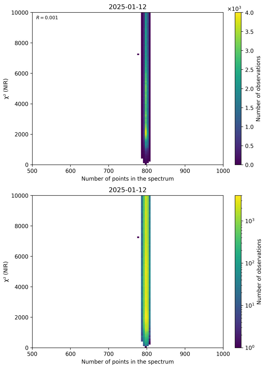
Figure 88: Scatter density plot of “Number of points in the spectrum” against “ \chi^2 (NIR)” for 2025-01-12 to 2025-01-13.
