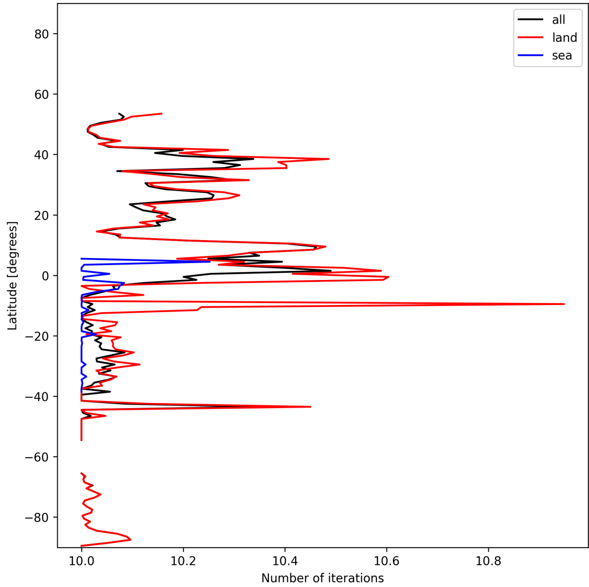
Figure 20: Zonal average of “Number of iterations” for 2025-01-12 to 2025-01-13.
