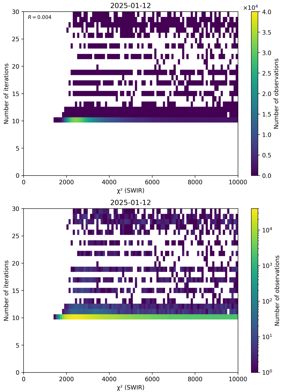
Figure 50: Scatter density plot of " \chi^2 (SWIR)" against "Number of iterations" for 2025-01-12 to 2025-01-13.
