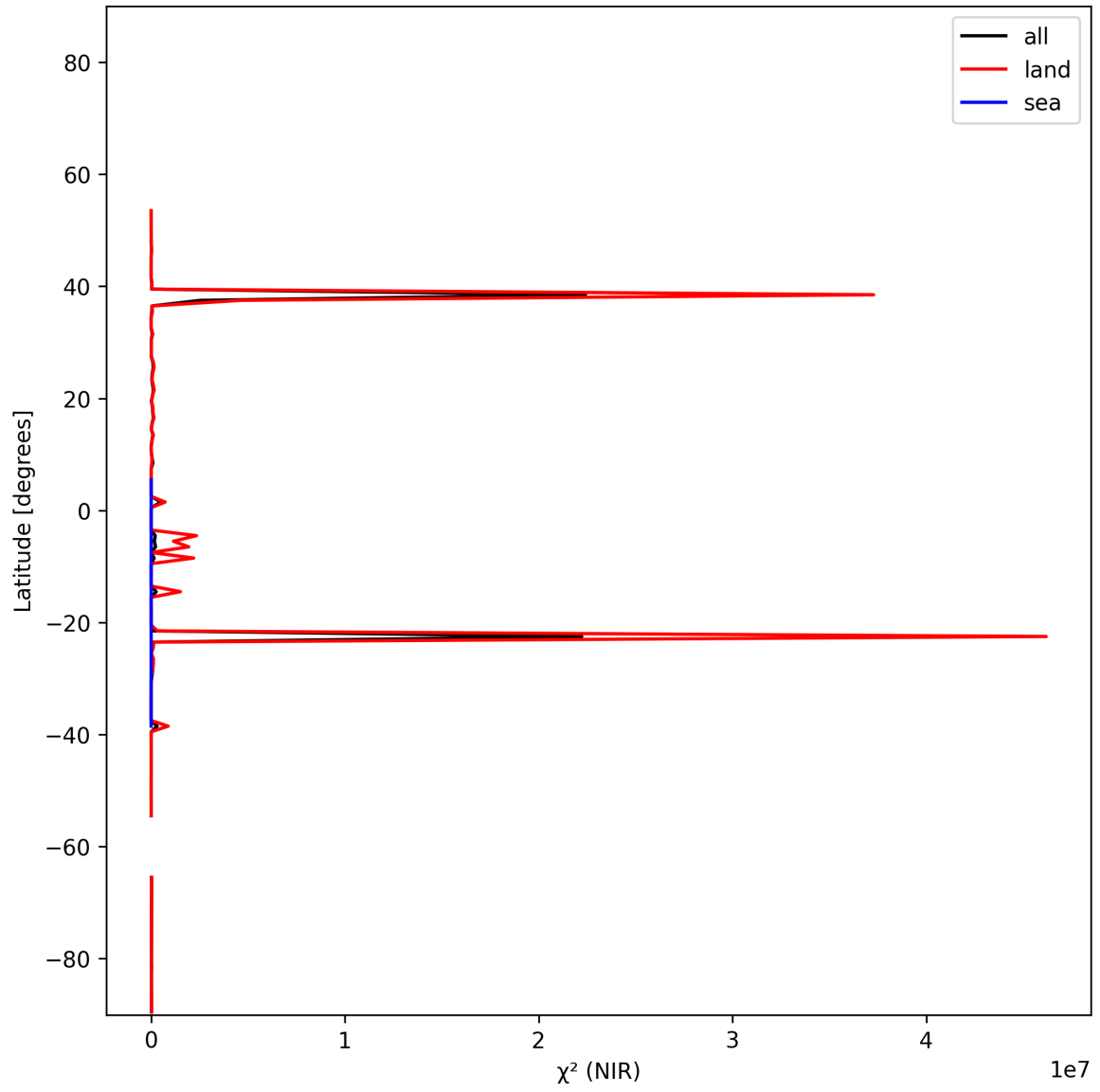
Figure 18: Zonal average of “ \chi^2 (NIR)” for 2025-01-12 to 2025-01-13.
