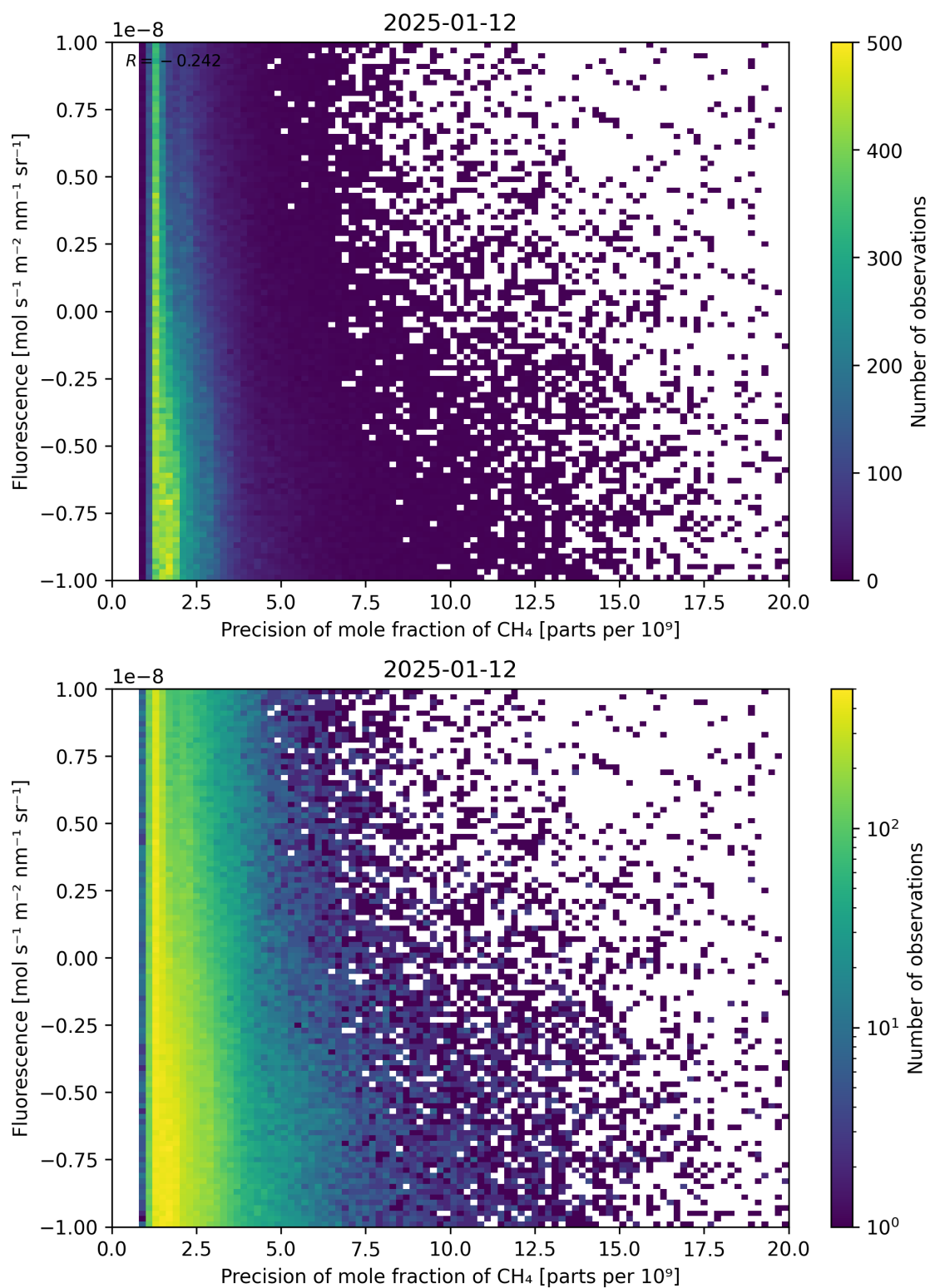
Figure 81: Scatter density plot of “Precision of mole fraction of CH 4 ” against “Fluorescence” for 2025-01-12 to 2025-01-13.
