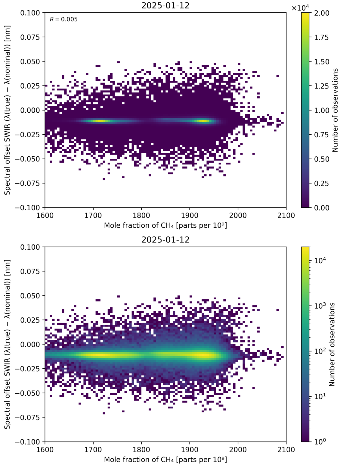
Figure 86: Scatter density plot of “Mole fraction of \text{CH}_4 ” against “Spectral offset SWIR ( \lambda_{\text{true}} - \lambda_{\text{nominal}} )” for 2025-01-12 to 2025-01-13.
