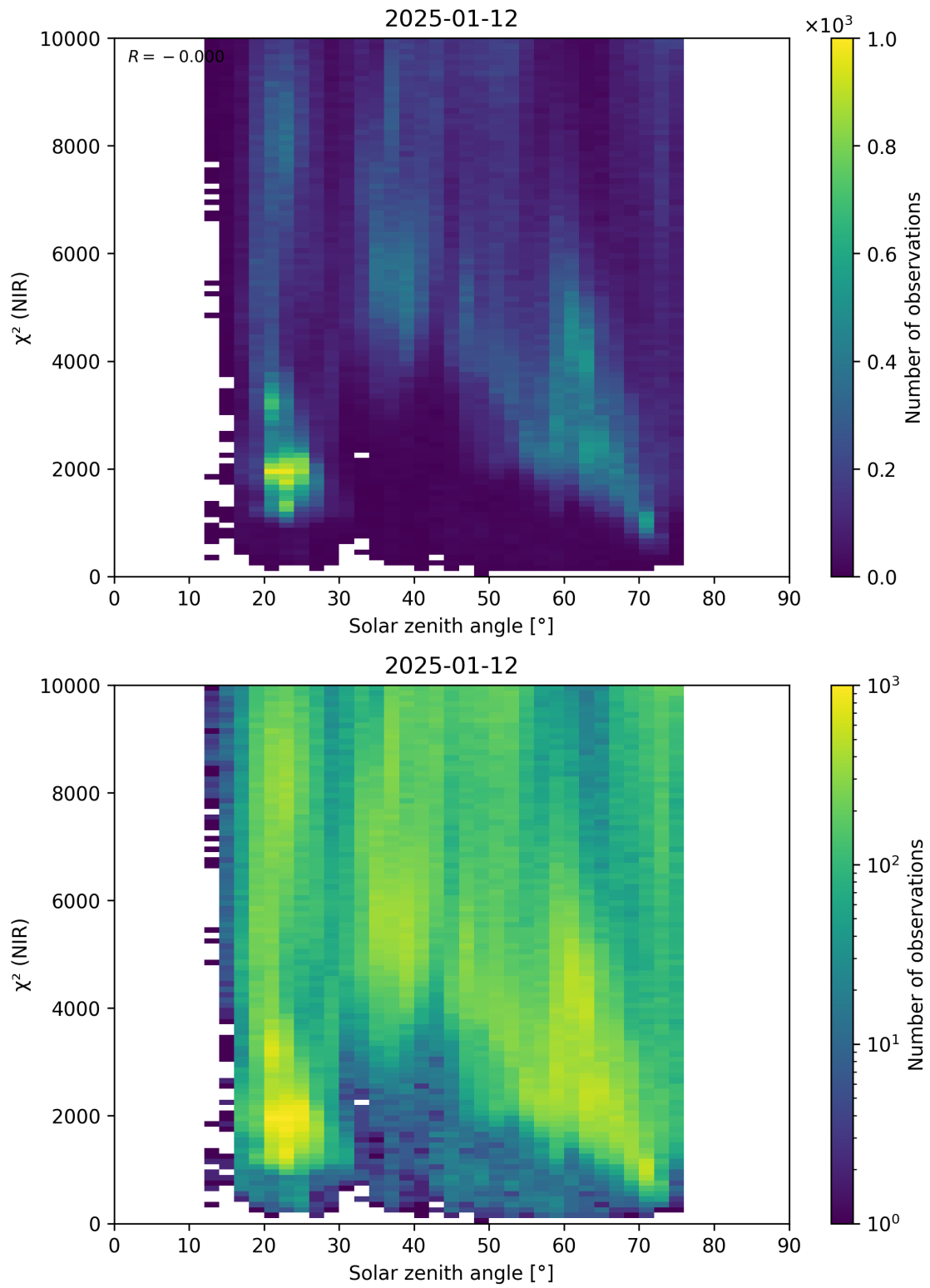
Figure 94: Scatter density plot of “Solar zenith angle” against “ \chi^2 (NIR)” for 2025-01-12 to 2025-01-13.
