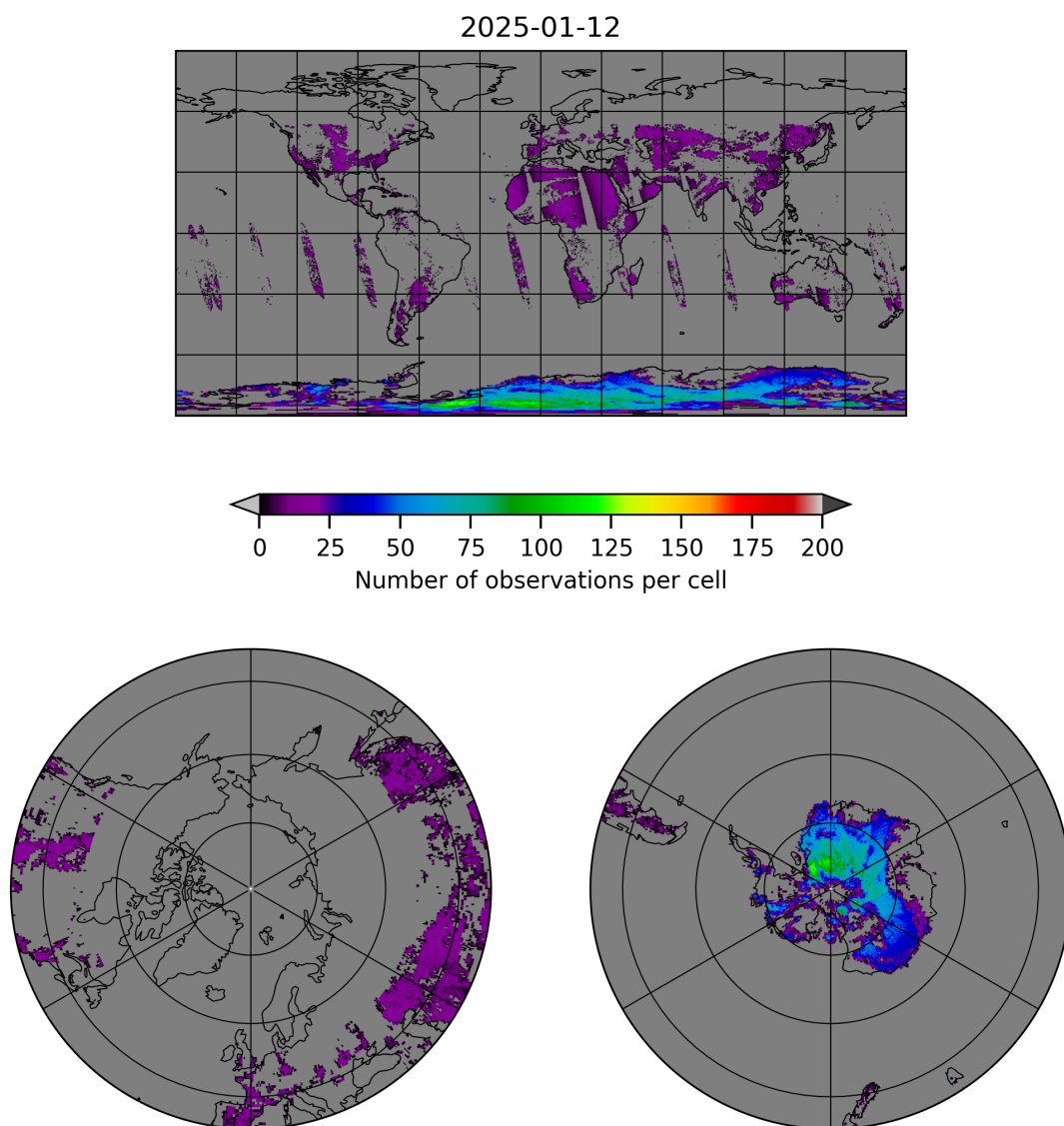
Figure 10: Map of the number of observations for 2025-01-12 to 2025-01-13
