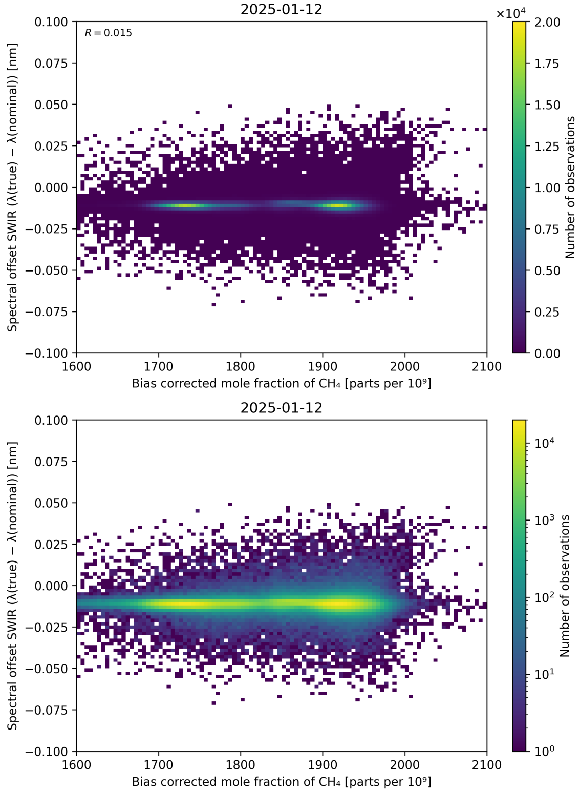
Figure 69: Scatter density plot of “Bias corrected mole fraction of \text{CH}_4 ” against “Spectral offset SWIR ( \lambda_{\text{true}} - \lambda_{\text{nominal}} )” for 2025-01-12 to 2025-01-13.
