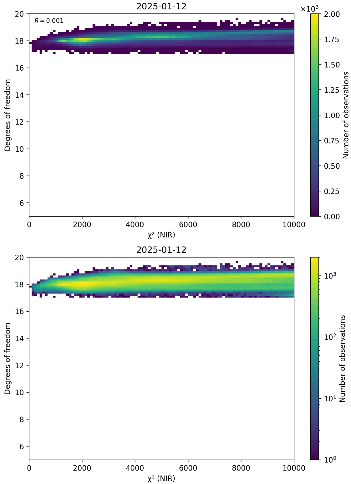
Figure 44: Scatter density plot of “ \chi^2 (NIR)” against “Degrees of freedom” for 2025-01-12 to 2025-01-13.
