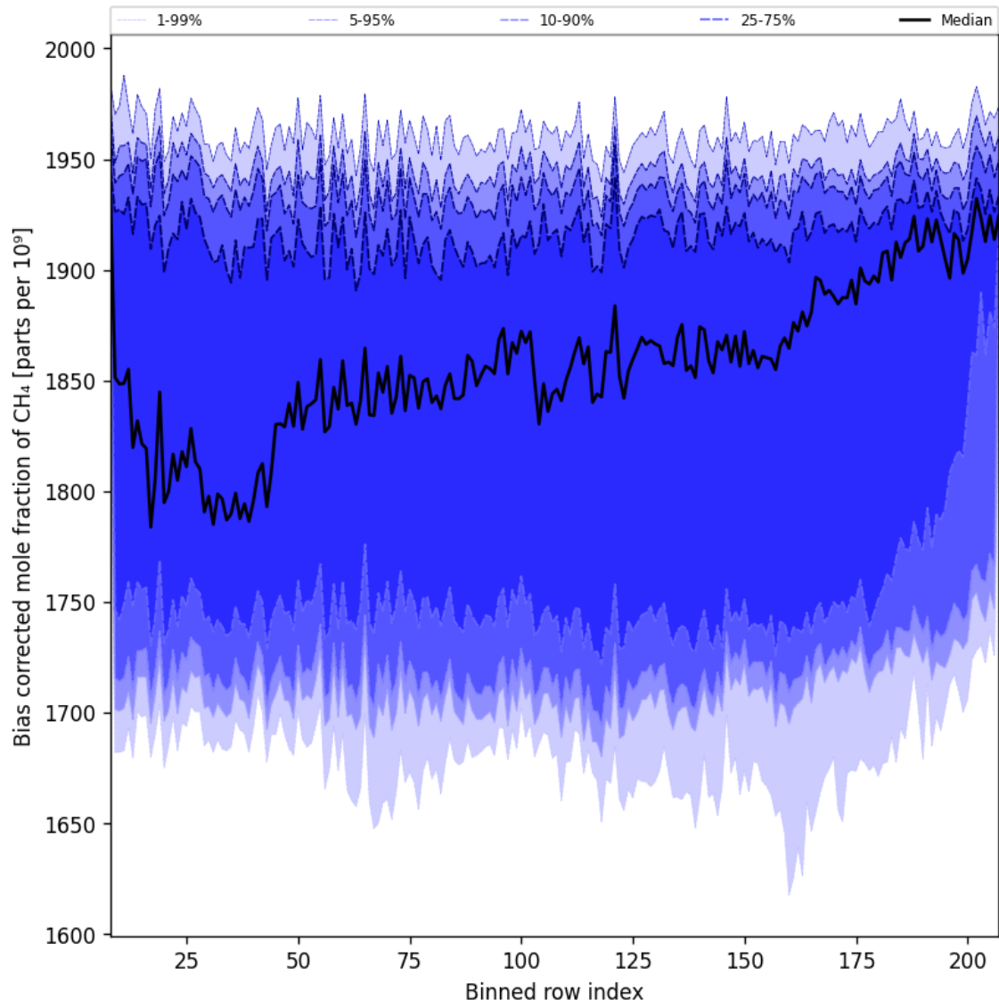
Figure 36: Along track statistics of “Bias corrected mole fraction of CH 4 ” for 2025-01-12 to 2025-01-13
