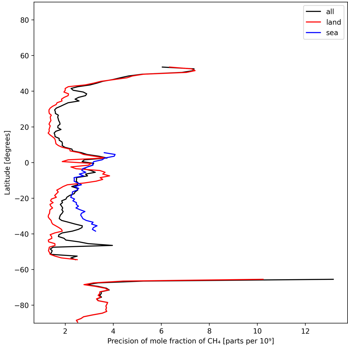
Figure 13: Zonal average of “Precision of mole fraction of CH 4 ” for 2025-01-12 to 2025-01-13.
