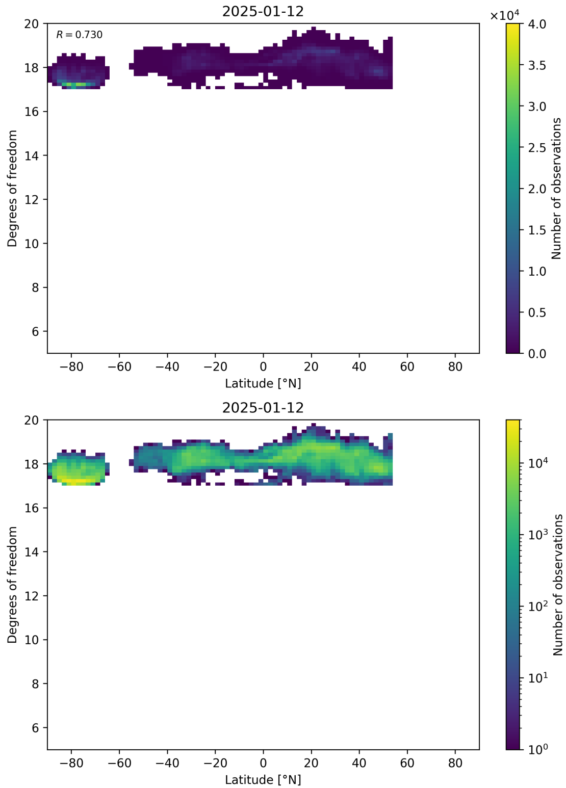
Figure 55: Scatter density plot of “Latitude” against “Degrees of freedom” for 2025-01-12 to 2025-01-13.
