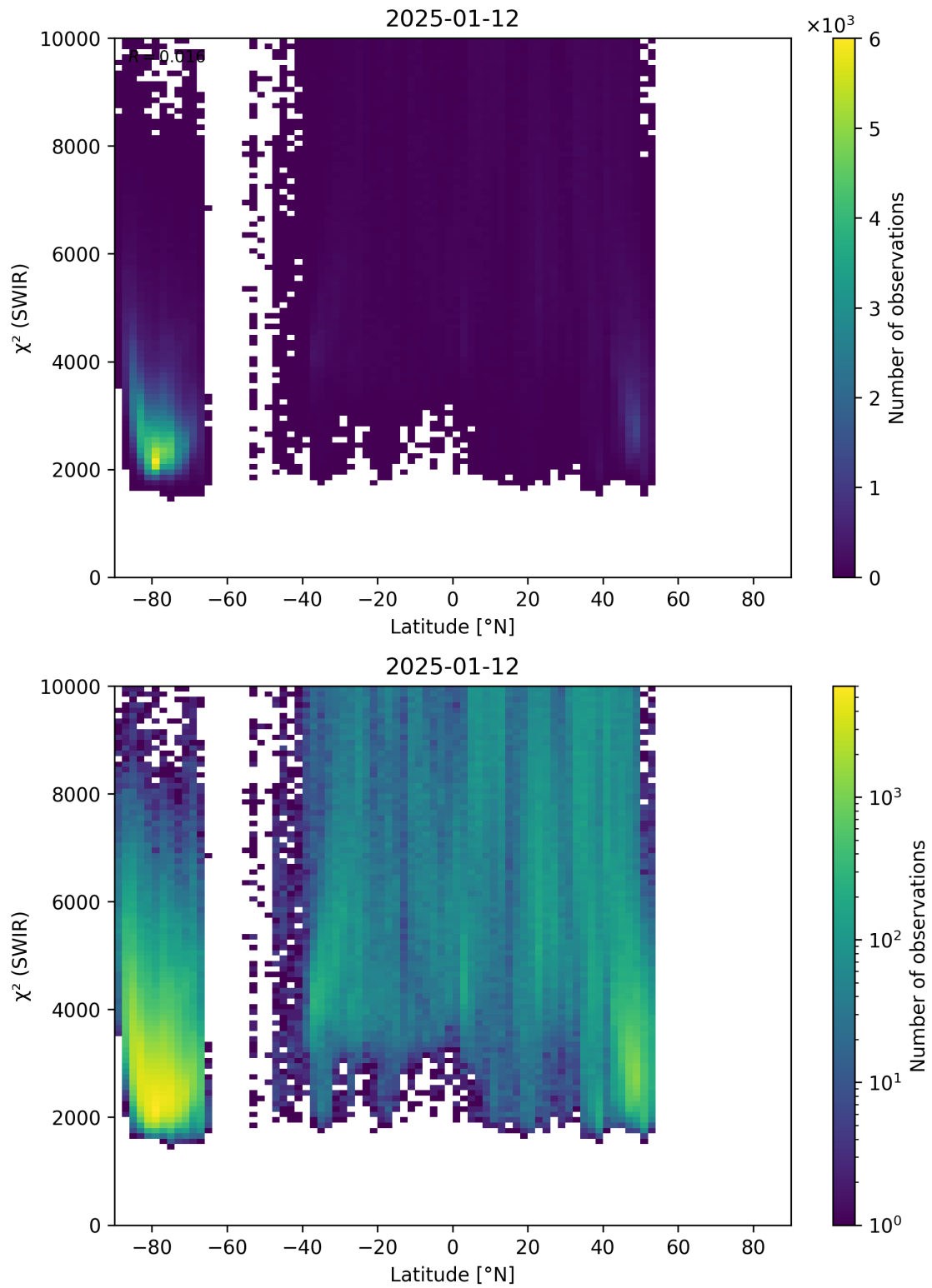
Figure 54: Scatter density plot of “Latitude” against “ \chi^2 (SWIR)” for 2025-01-12 to 2025-01-13.
