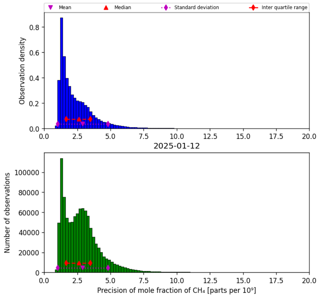
Figure 24: Histogram of “Precision of mole fraction of CH 4 ” for 2025-01-12 to 2025-01-13
