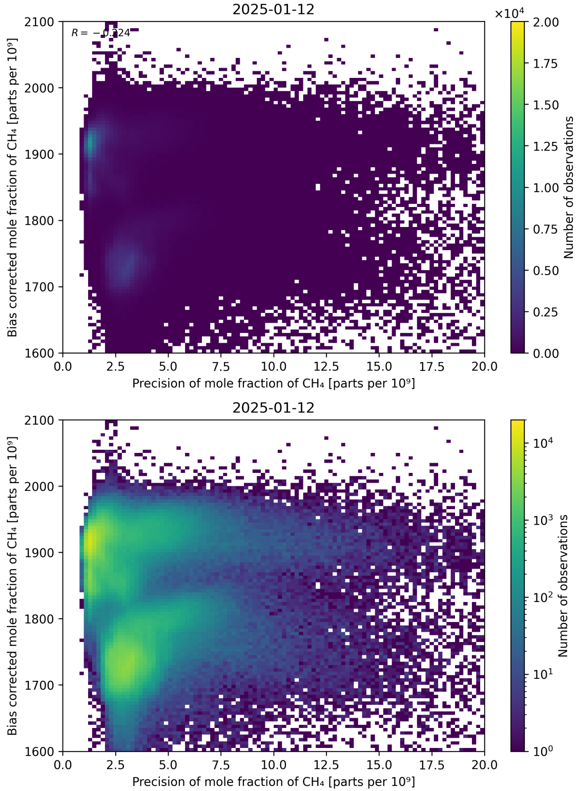
Figure 82: Scatter density plot of “Precision of mole fraction of CH 4 ” against “Bias corrected mole fraction of CH 4 ” for 2025-01-12 to 2025-01-13.
