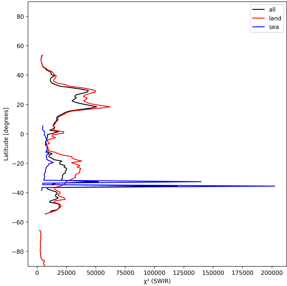
Figure 17: Zonal average of “ \chi^2 (SWIR)” for 2025-01-12 to 2025-01-13.
