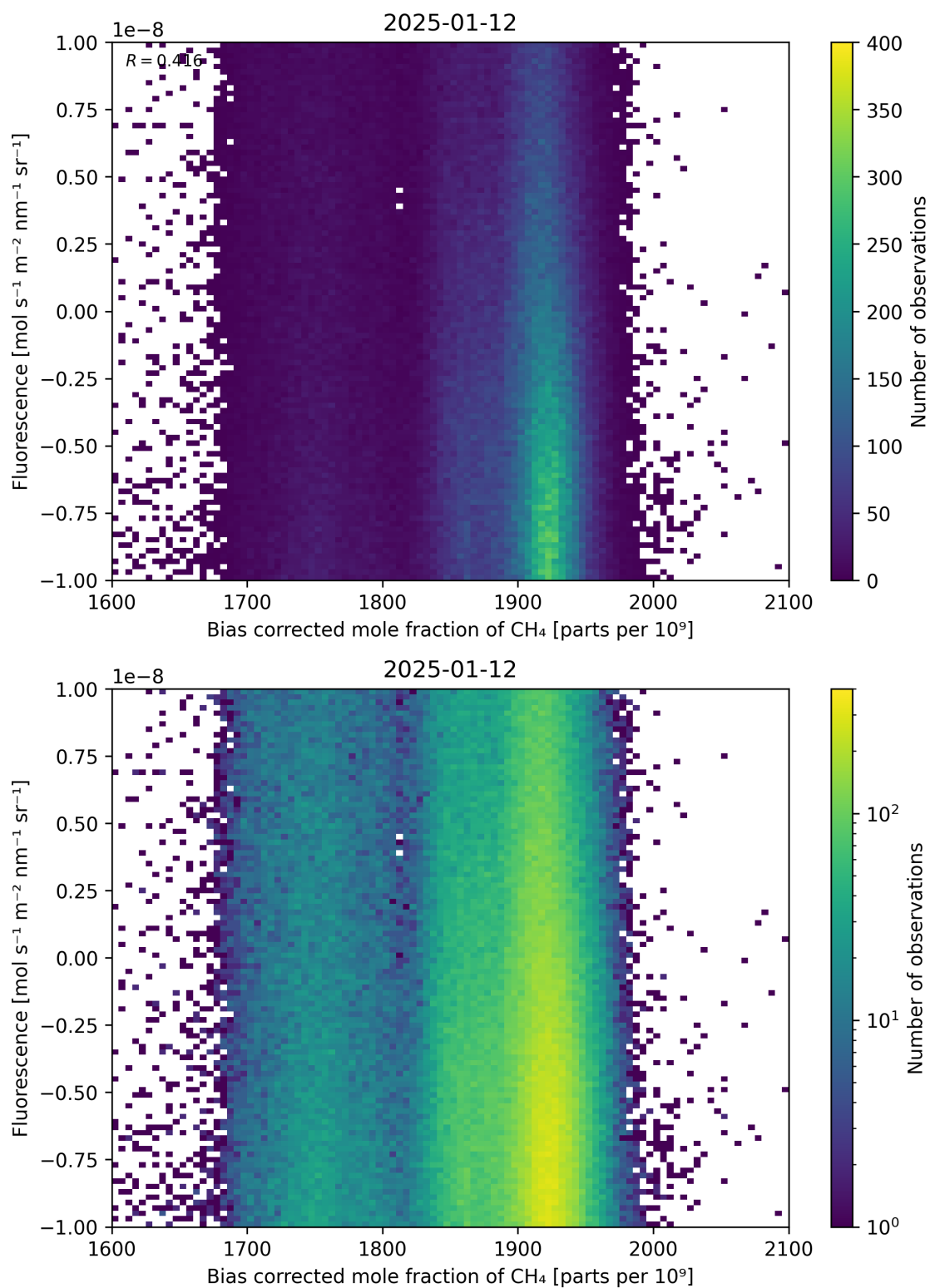
Figure 66: Scatter density plot of “Bias corrected mole fraction of \text{CH}_4 ” against “Fluorescence” for 2025-01-12 to 2025-01-13.
