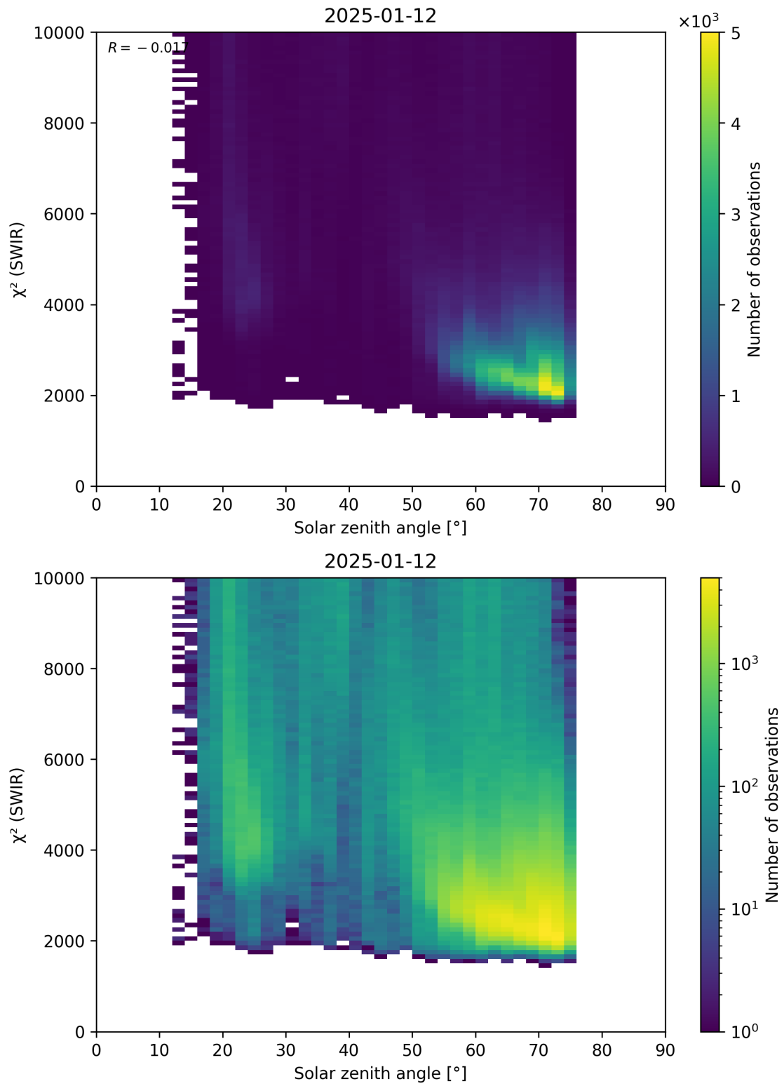
Figure 95: Scatter density plot of “Solar zenith angle” against “ \chi^2 (SWIR)” for 2025-01-12 to 2025-01-13.
