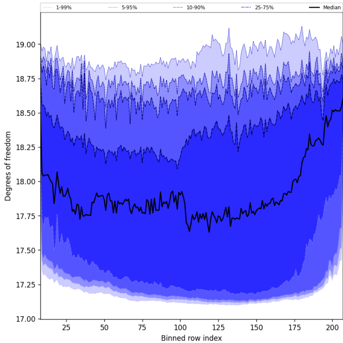
Figure 41: Along track statistics of “Degrees of freedom” for 2025-01-12 to 2025-01-13
