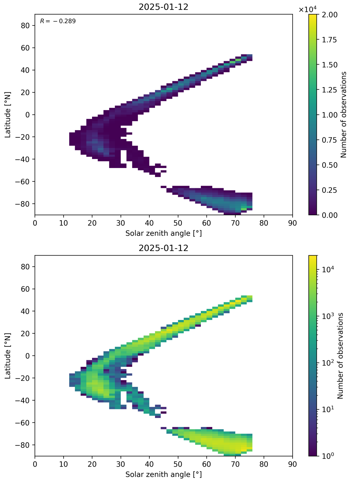
Figure 98: Scatter density plot of “Solar zenith angle” against “Latitude” for 2025-01-12 to 2025-01-13.
