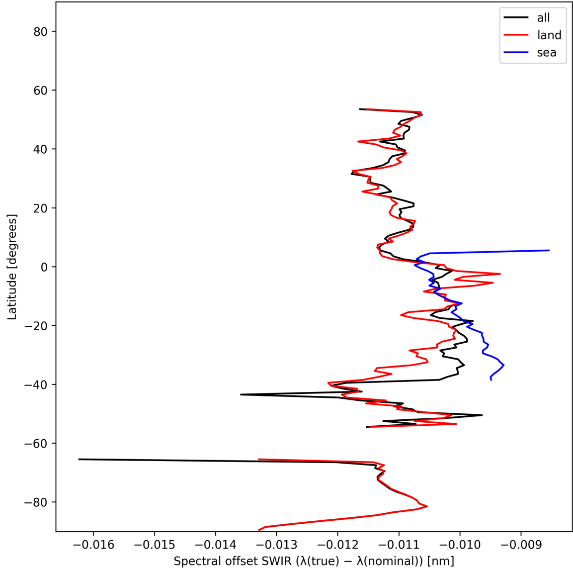
Figure 16: Zonal average of “Spectral offset SWIR ( \lambda_{\text{true}} - \lambda_{\text{nominal}} )” for 2025-01-12 to 2025-01-13.
