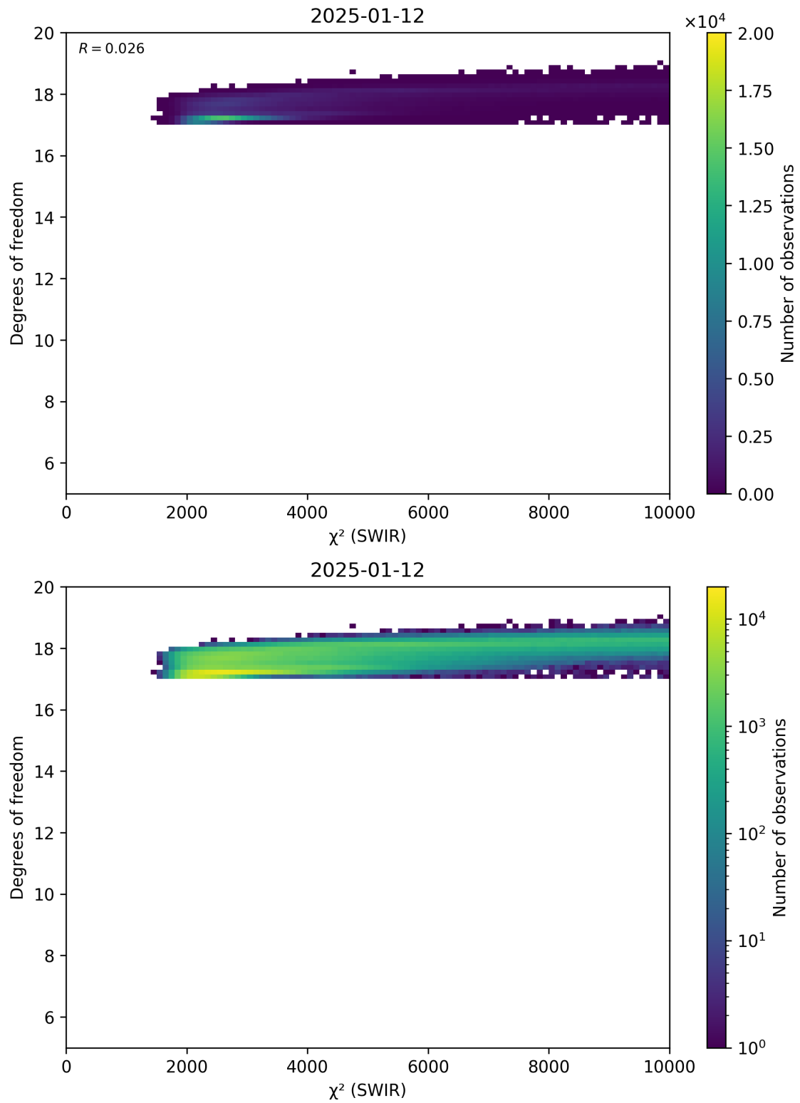
Figure 48: Scatter density plot of “ \chi^2 (SWIR)” against “Degrees of freedom” for 2025-01-12 to 2025-01-13.
