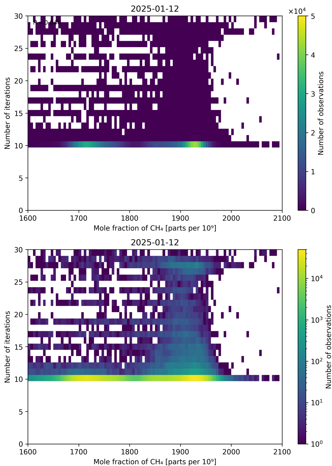
Figure 76: Scatter density plot of “Mole fraction of CH 4 ” against “Number of iterations” for 2025-01-12 to 2025-01-13.
