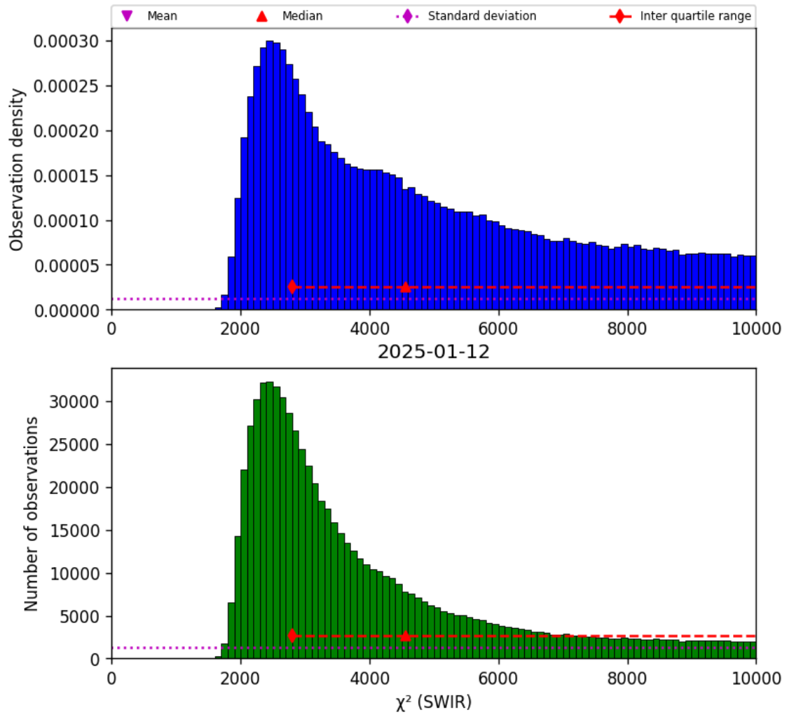
Figure 28: Histogram of “ \chi^2 (SWIR)” for 2025-01-12 to 2025-01-13
