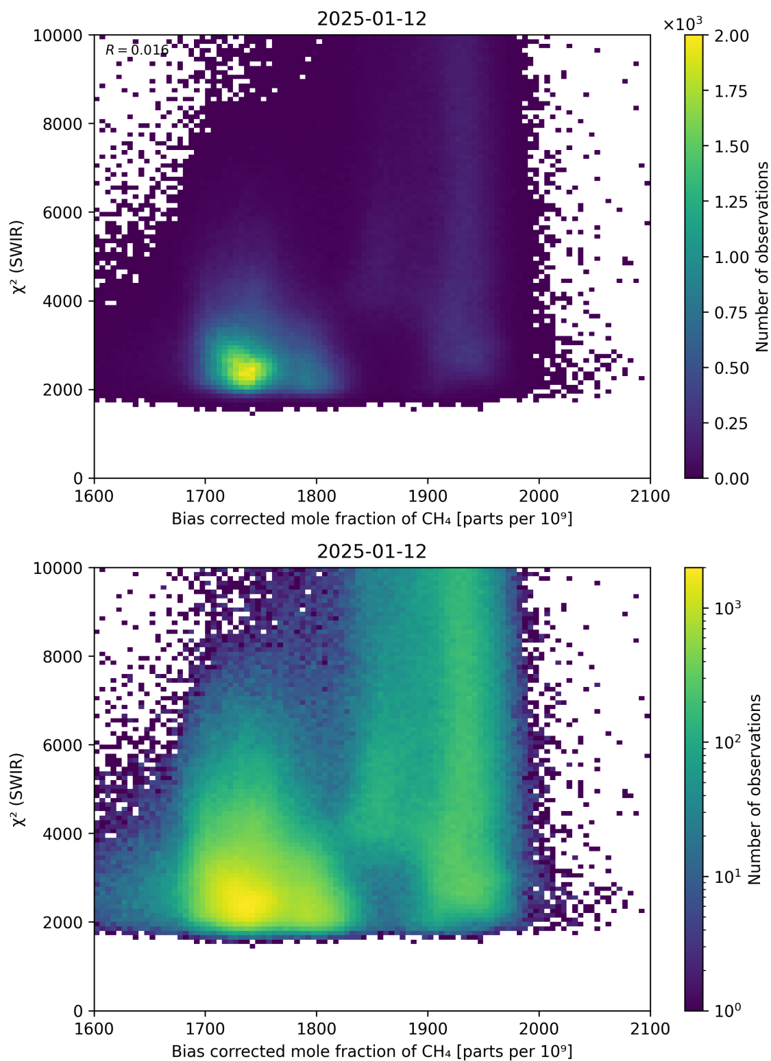
Figure 64: Scatter density plot of “Bias corrected mole fraction of CH 4 ” against “ \chi^2 (SWIR)” for 2025-01-12 to 2025-01-13.
