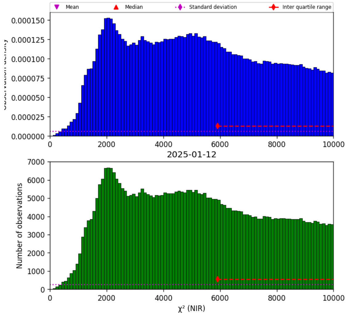
Figure 29: Histogram of “ \chi^2 (NIR)” for 2025-01-12 to 2025-01-13
