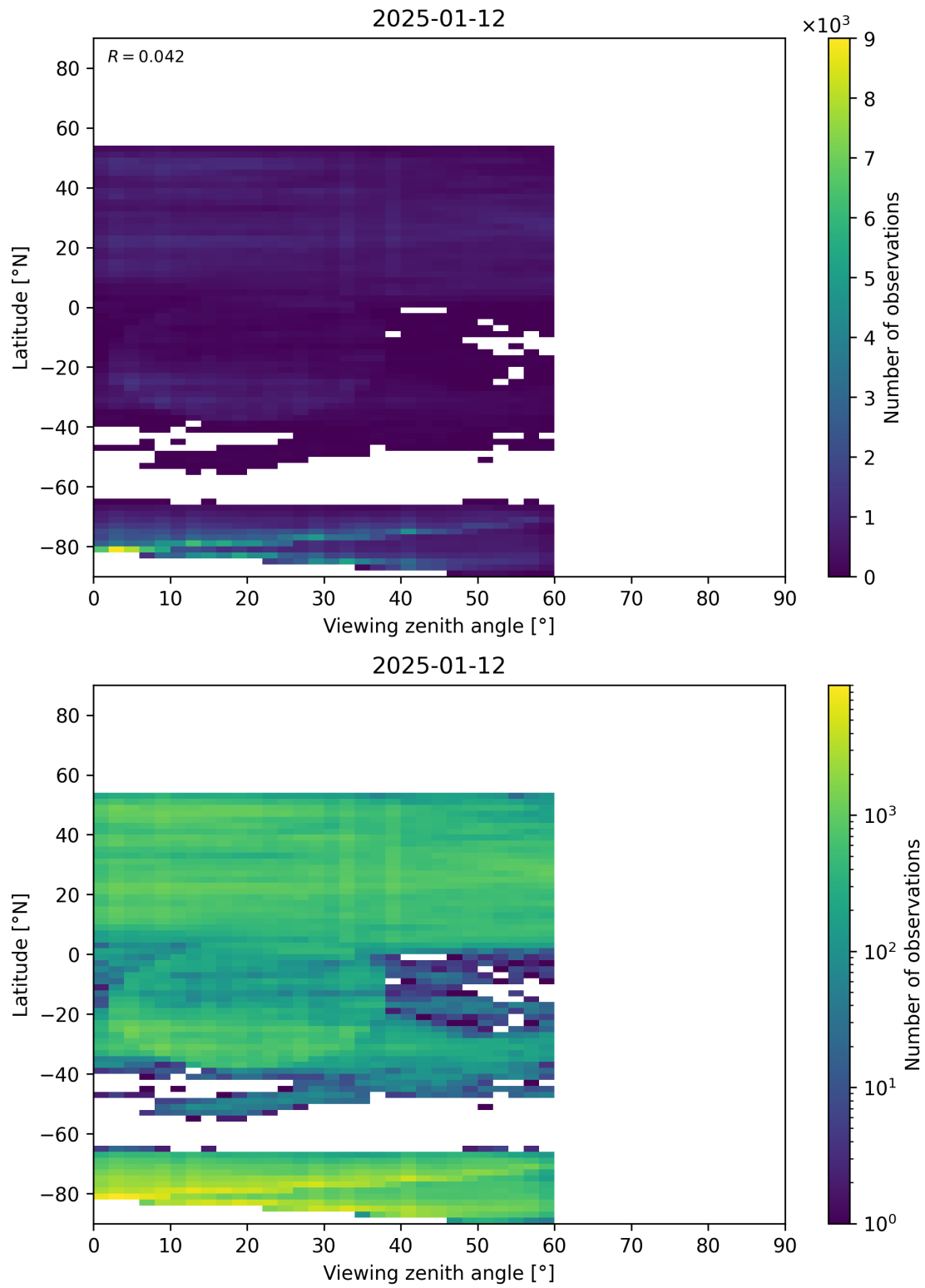
Figure 109: Scatter density plot of “Viewing zenith angle” against “Latitude” for 2025-01-12 to 2025-01-13.
