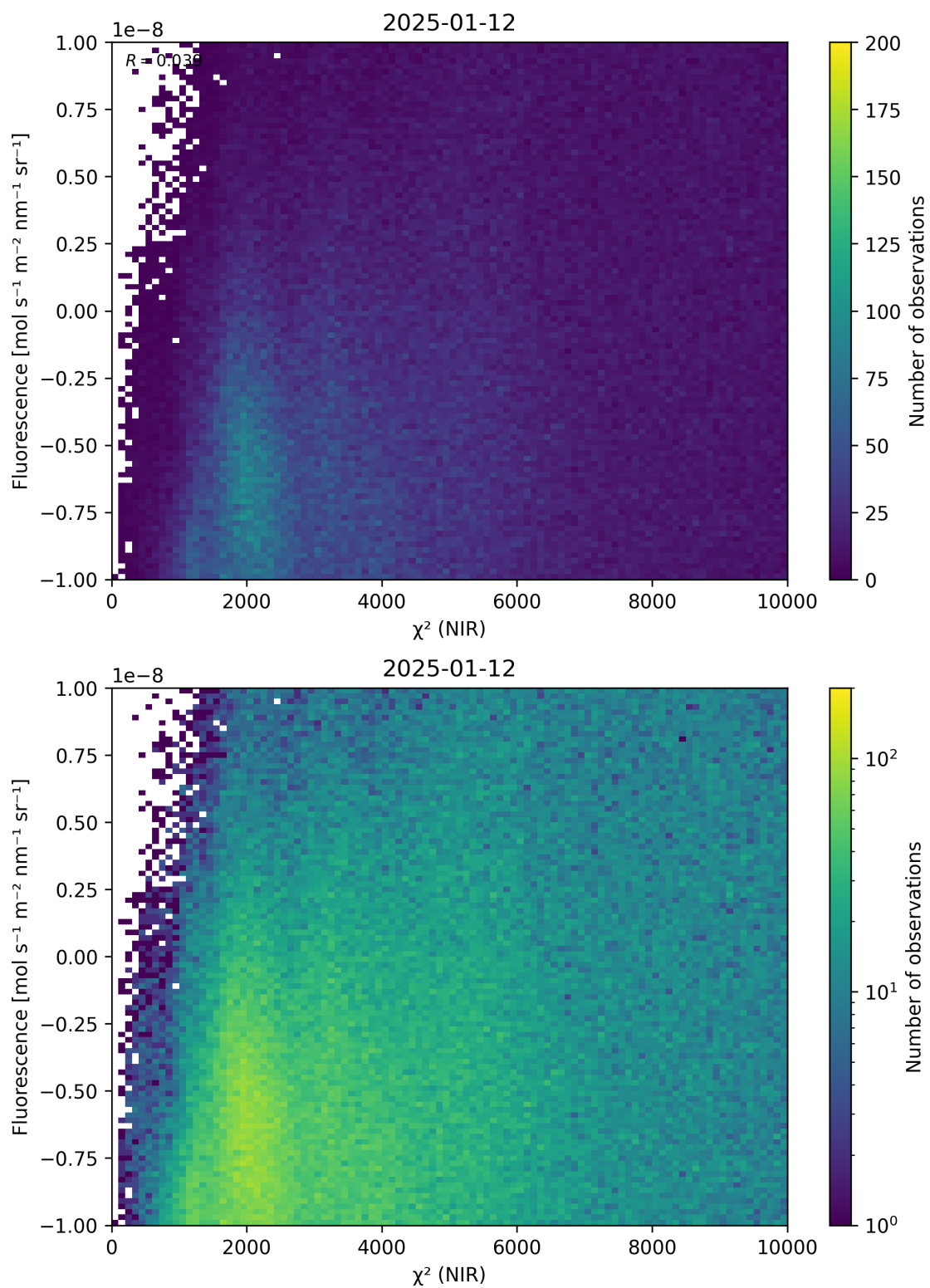
Figure 45: Scatter density plot of “ \chi^2 (NIR)” against “Fluorescence” for 2025-01-12 to 2025-01-13.
