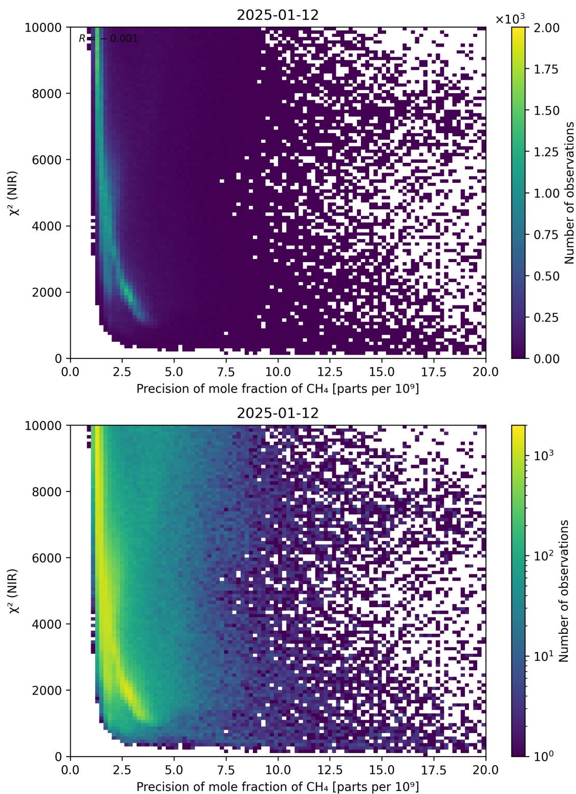
Figure 78: Scatter density plot of “Precision of mole fraction of CH 4 ” against “ \chi^2 (NIR)” for 2025-01-12 to 2025-01-13.
