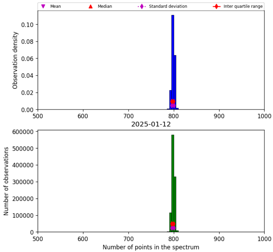
Figure 26: Histogram of “Number of points in the spectrum” for 2025-01-12 to 2025-01-13
