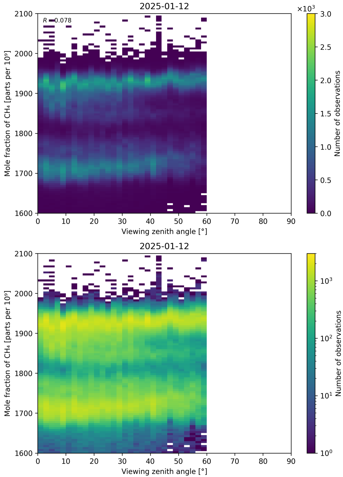
Figure 110: Scatter density plot of “Viewing zenith angle” against “Mole fraction of CH 4 ” for 2025-01-12 to 2025-01-13.
