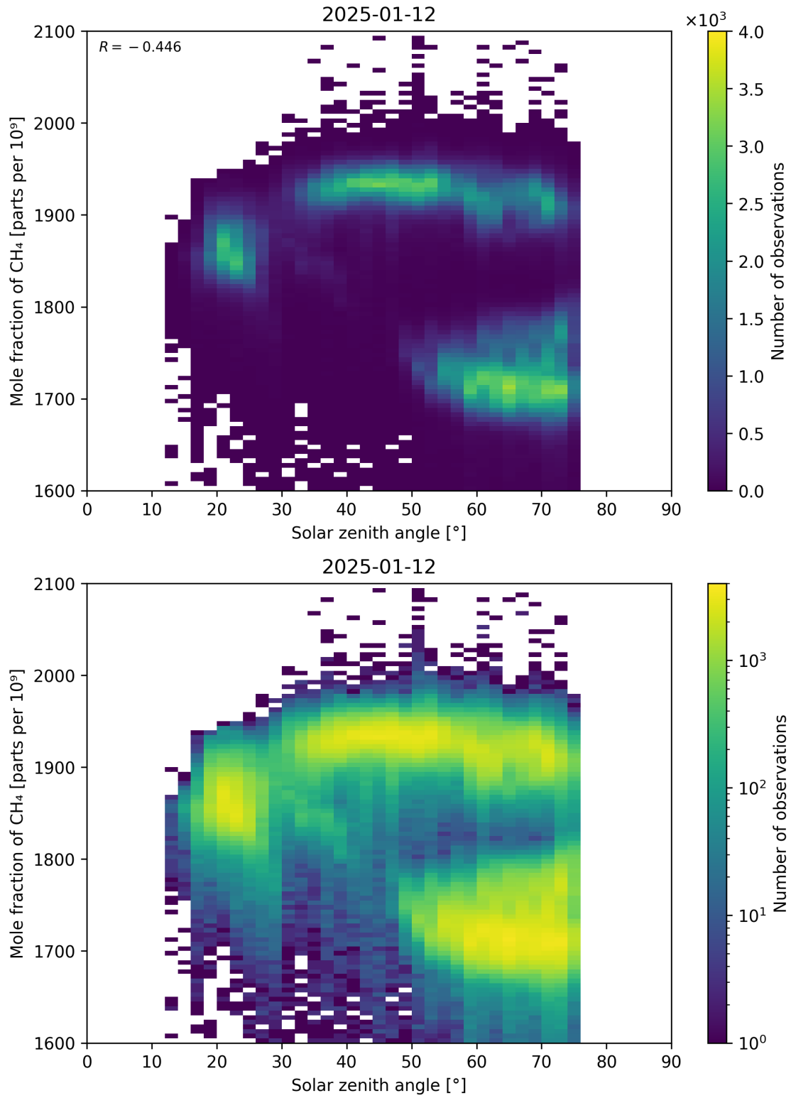
Figure 99: Scatter density plot of “Solar zenith angle” against “Mole fraction of CH 4 ” for 2025-01-12 to 2025-01-13.
