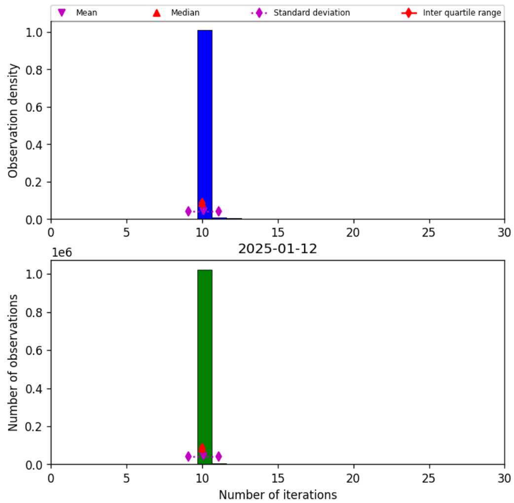
Figure 31: Histogram of “Number of iterations” for 2025-01-12 to 2025-01-13
