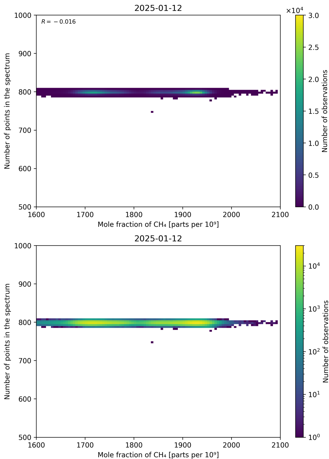
Figure 77: Scatter density plot of “Mole fraction of CH 4 ” against “Number of points in the spectrum” for 2025-01-12 to 2025-01-13.
