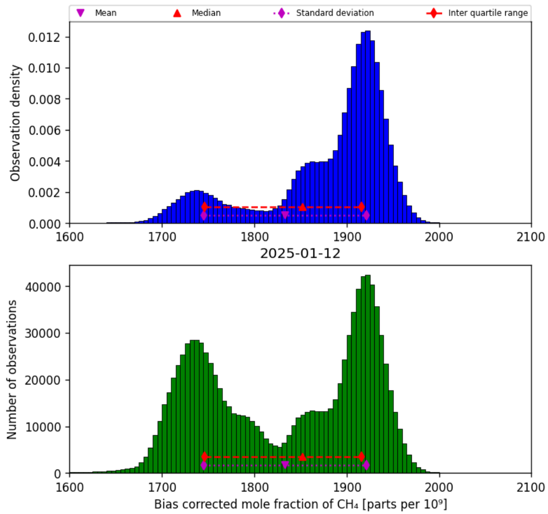
Figure 25: Histogram of “Bias corrected mole fraction of CH 4 ” for 2025-01-12 to 2025-01-13
