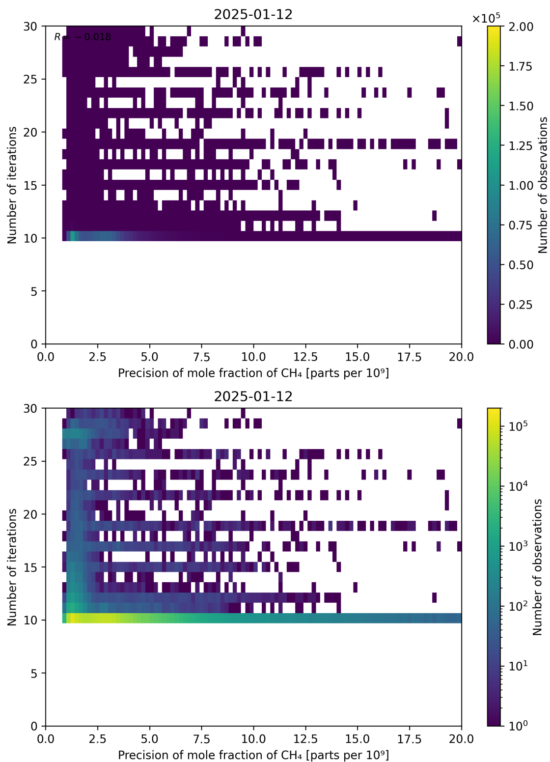
Figure 83: Scatter density plot of “Precision of mole fraction of CH 4 ” against “Number of iterations” for 2025-01-12 to 2025-01-13.
