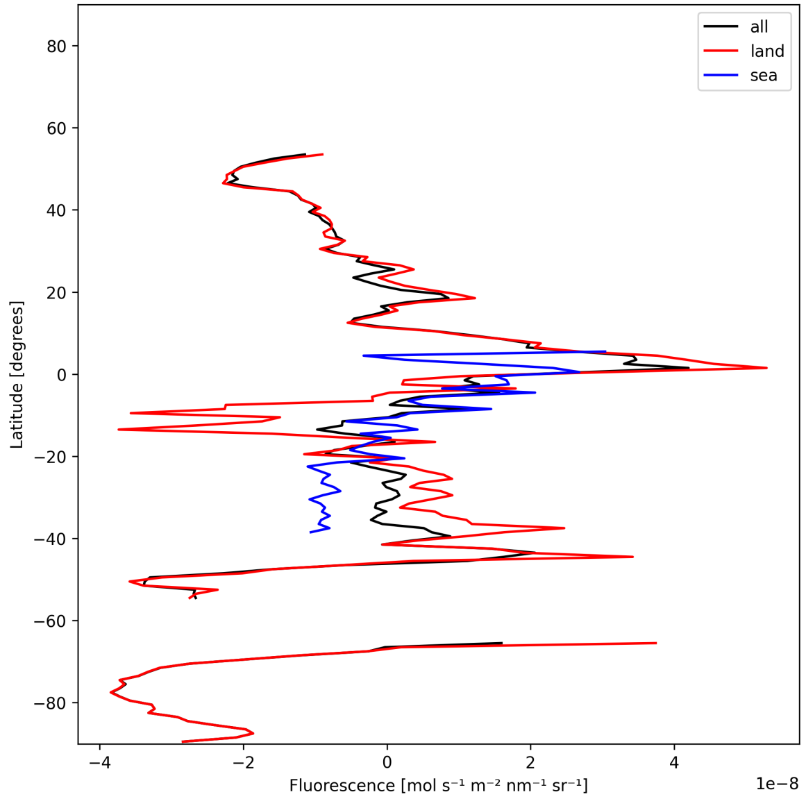
Figure 21: Zonal average of “Fluorescence” for 2025-01-12 to 2025-01-13.
