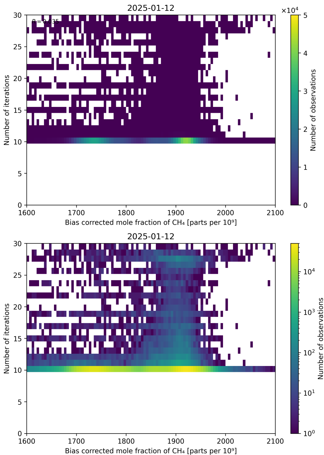
Figure 67: Scatter density plot of “Bias corrected mole fraction of \text{CH}_4 ” against “Number of iterations” for 2025-01-12 to 2025-01-13.
