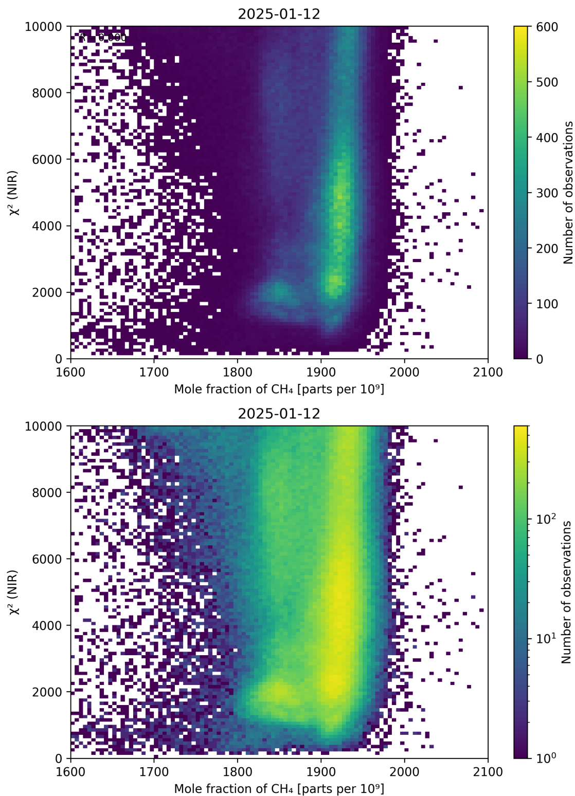
Figure 70: Scatter density plot of “Mole fraction of CH 4 ” against “ \chi^2 (NIR)” for 2025-01-12 to 2025-01-13.
