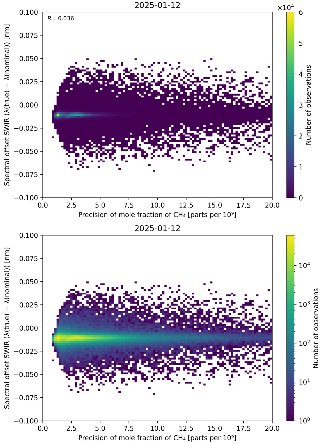
Figure 85: Scatter density plot of “Precision of mole fraction of \text{CH}_4 ” against “Spectral offset SWIR ( \lambda_{\text{true}} - \lambda_{\text{nominal}} )” for 2025-01-12 to 2025-01-13.
