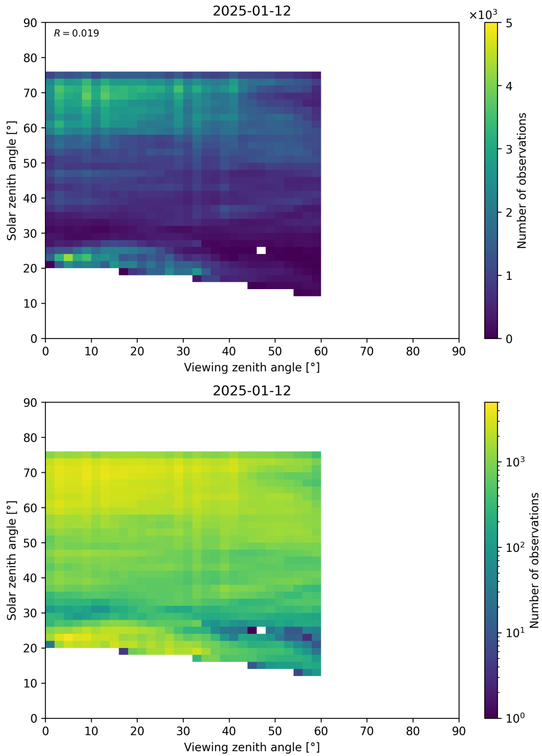
Figure 115: Scatter density plot of “Viewing zenith angle” against “Solar zenith angle” for 2025-01-12 to 2025-01-13.
