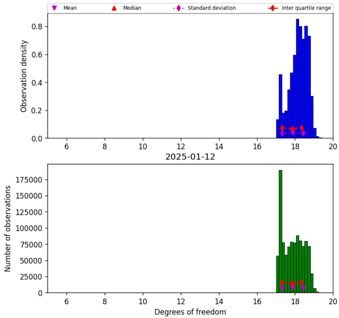
Figure 30: Histogram of “Degrees of freedom” for 2025-01-12 to 2025-01-13
