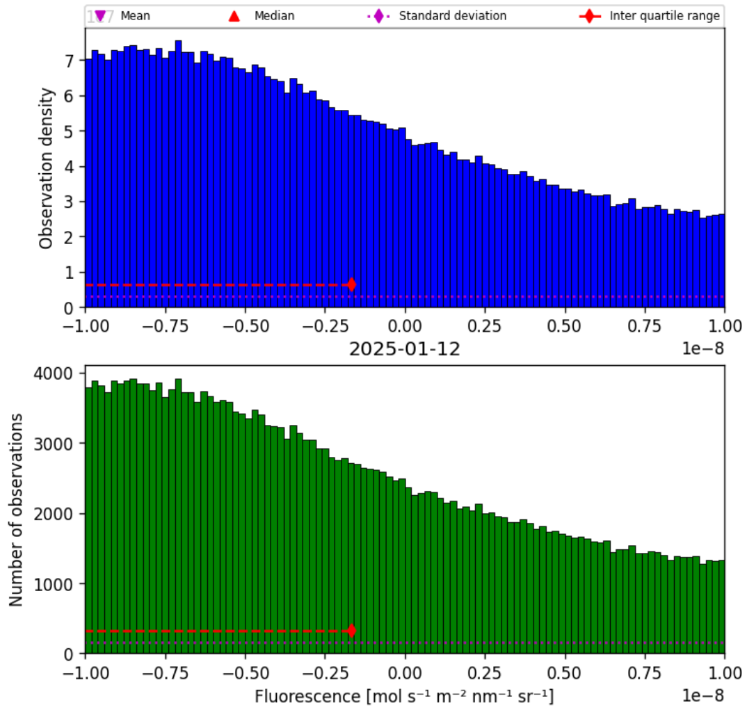
Figure 32: Histogram of “Fluorescence” for 2025-01-12 to 2025-01-13
