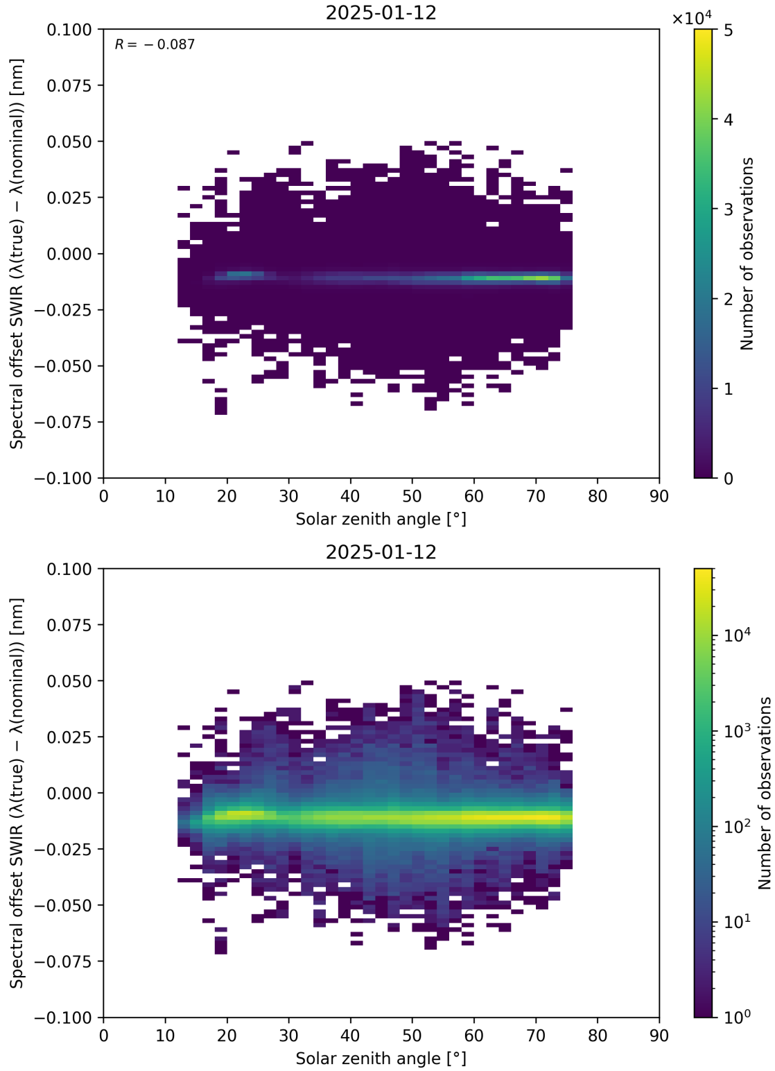
Figure 104: Scatter density plot of “Solar zenith angle” against “Spectral offset SWIR ( \lambda_{\text{true}} - \lambda_{\text{nominal}} )” for 2025-01-12 to 2025-01-13.
