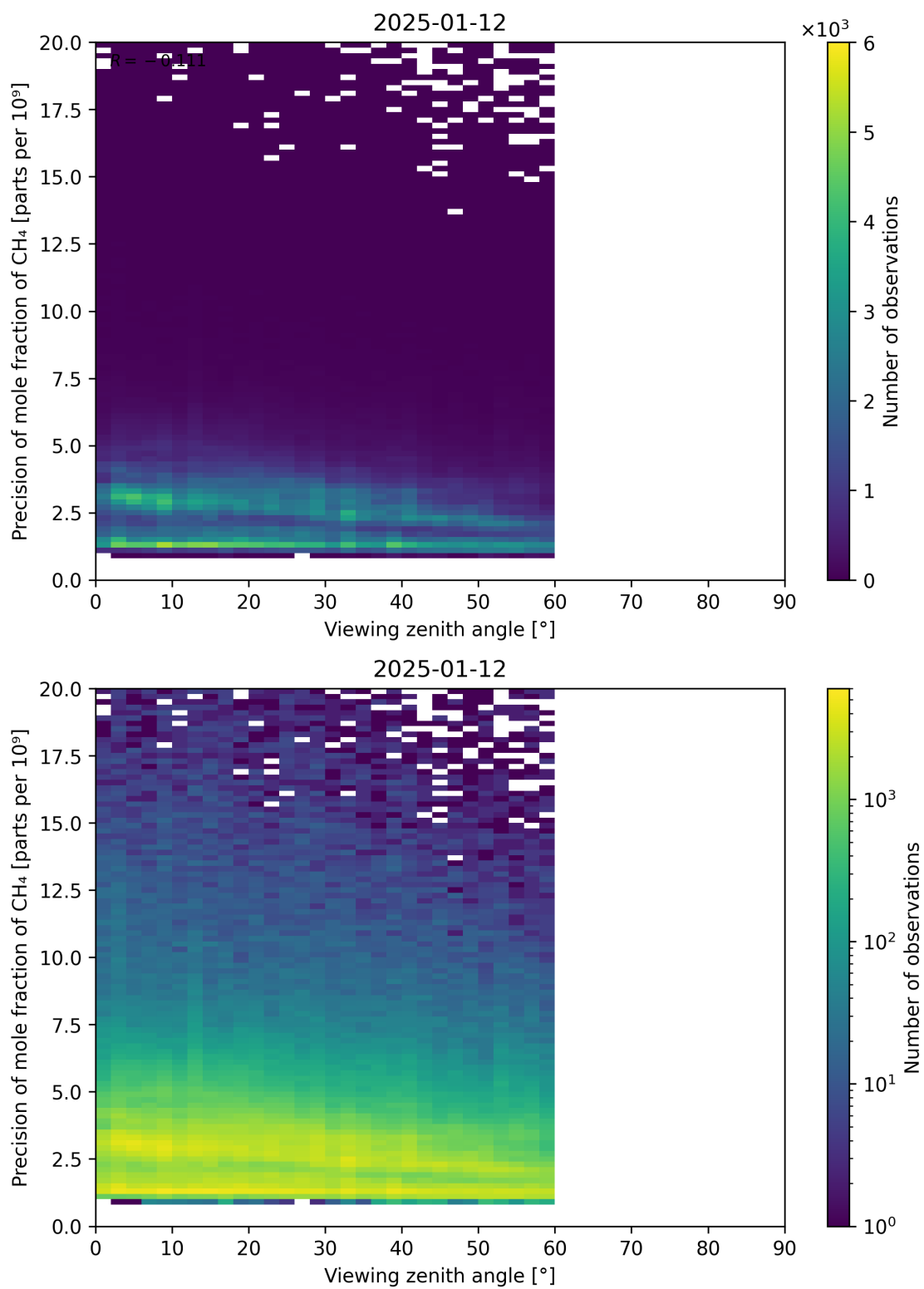
Figure 112: Scatter density plot of “Viewing zenith angle” against “Precision of mole fraction of CH 4 ” for 2025-01-12 to 2025-01-13.
