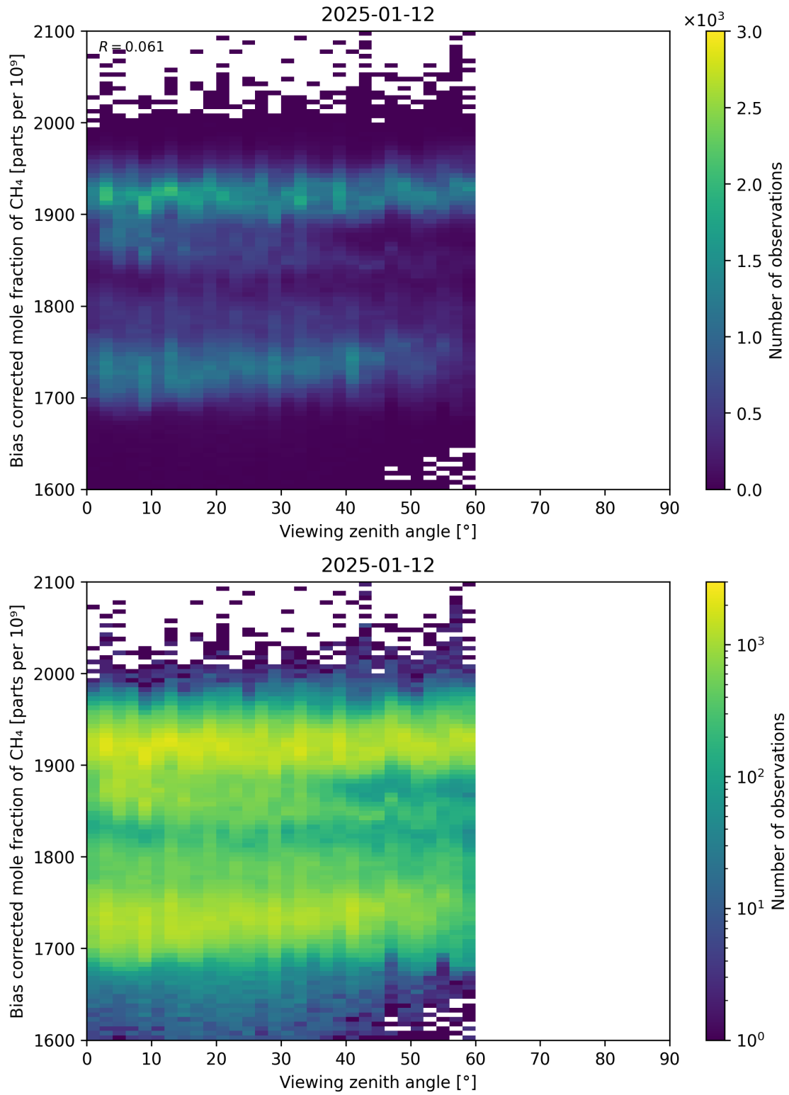
Figure 111: Scatter density plot of “Viewing zenith angle” against “Bias corrected mole fraction of CH 4 ” for 2025-01-12 to 2025-01-13.
