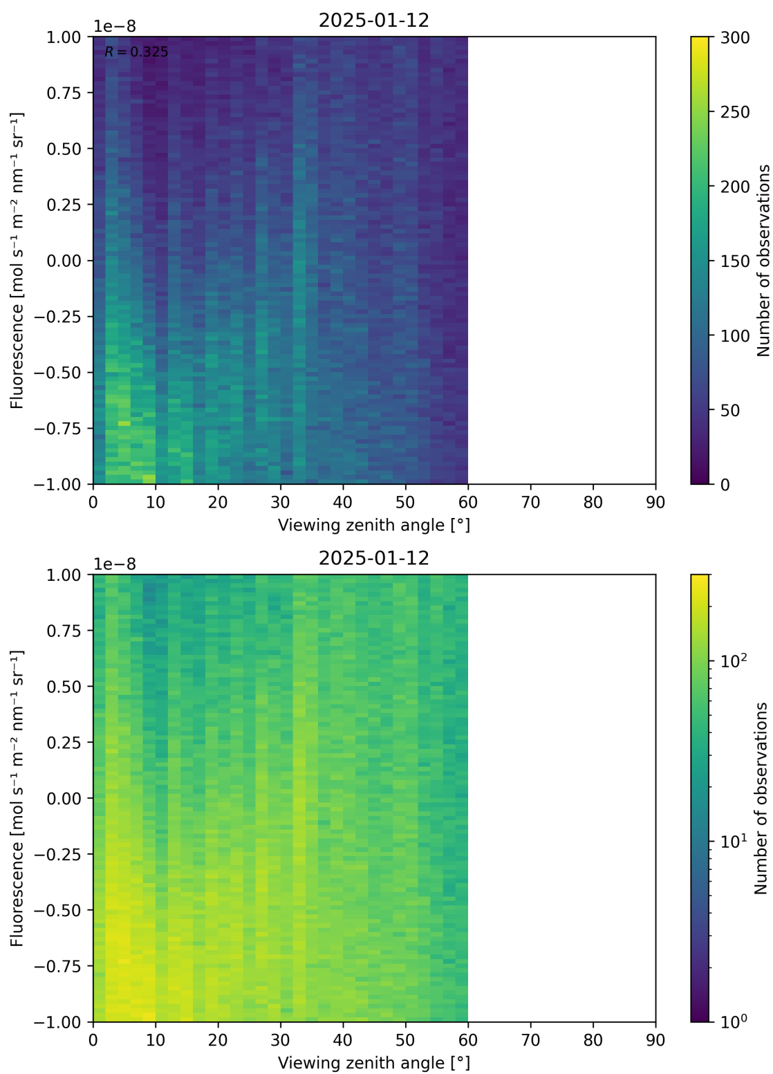
Figure 108: Scatter density plot of “Viewing zenith angle” against “Fluorescence” for 2025-01-12 to 2025-01-13.
