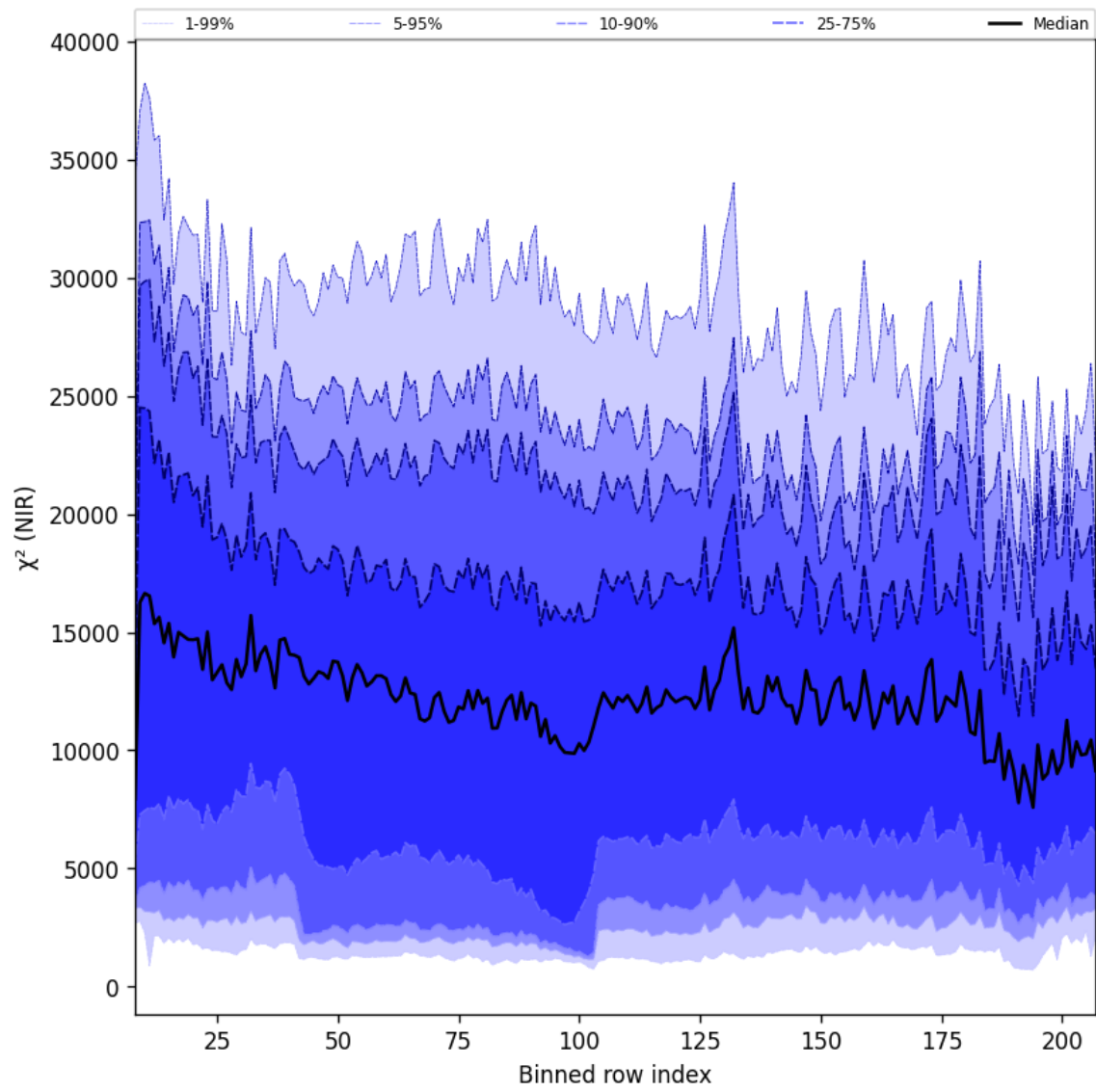
Figure 40: Along track statistics of “ \chi^2 (NIR)” for 2025-01-12 to 2025-01-13
