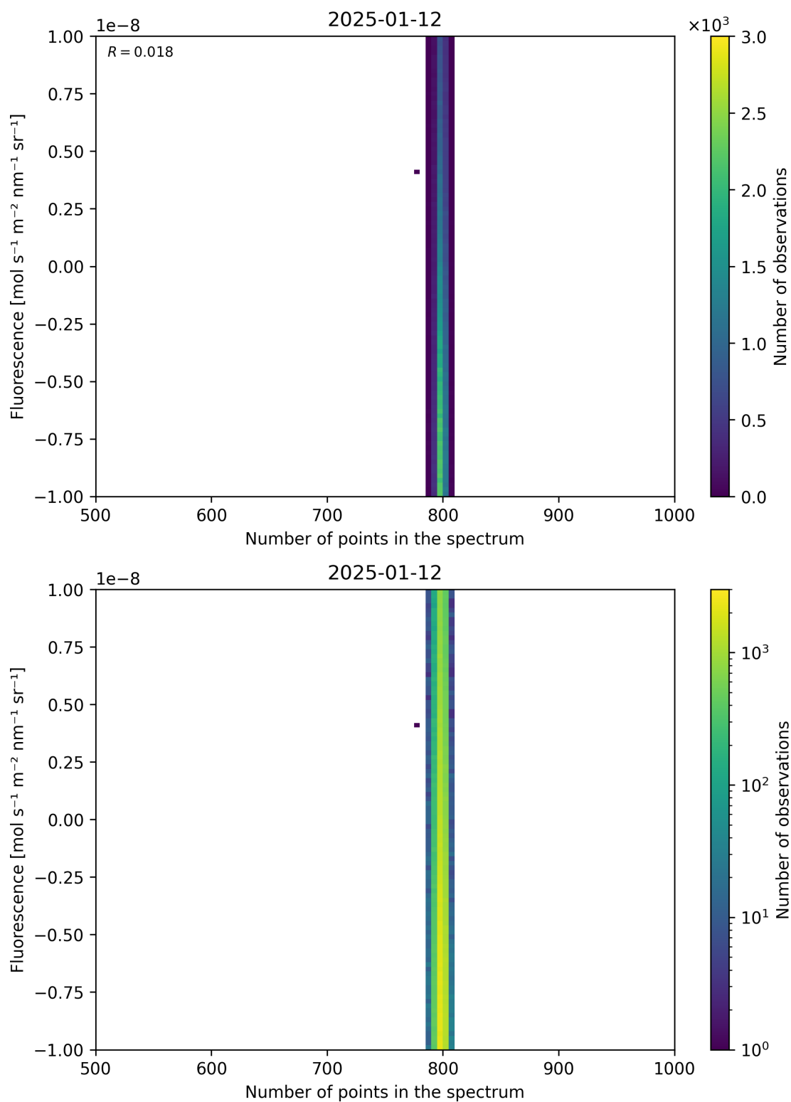
Figure 91: Scatter density plot of “Number of points in the spectrum” against “Fluorescence” for 2025-01-12 to 2025-01-13.
