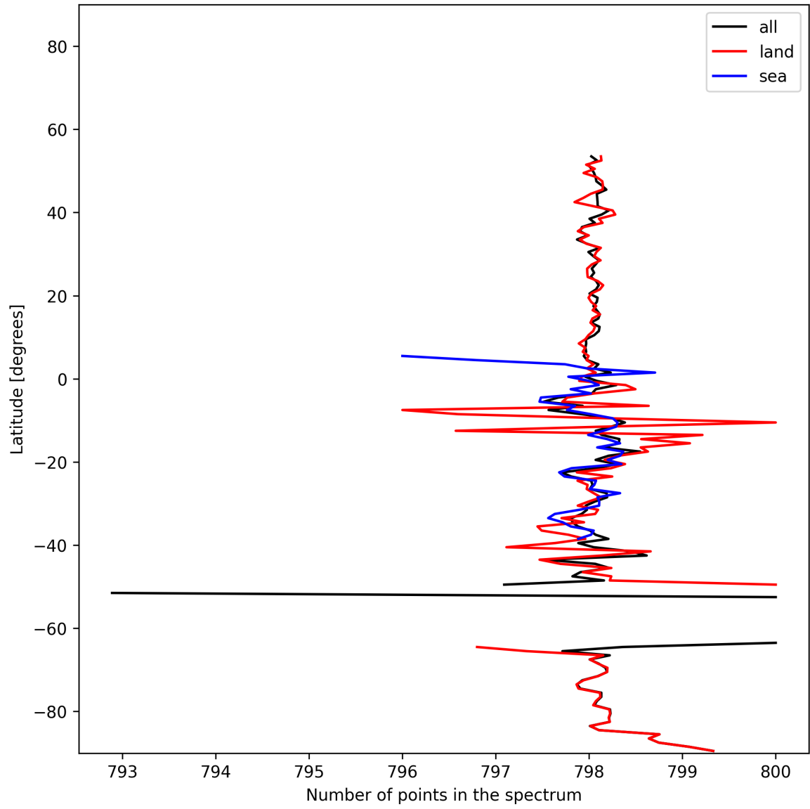
Figure 15: Zonal average of “Number of points in the spectrum” for 2025-01-12 to 2025-01-14.
