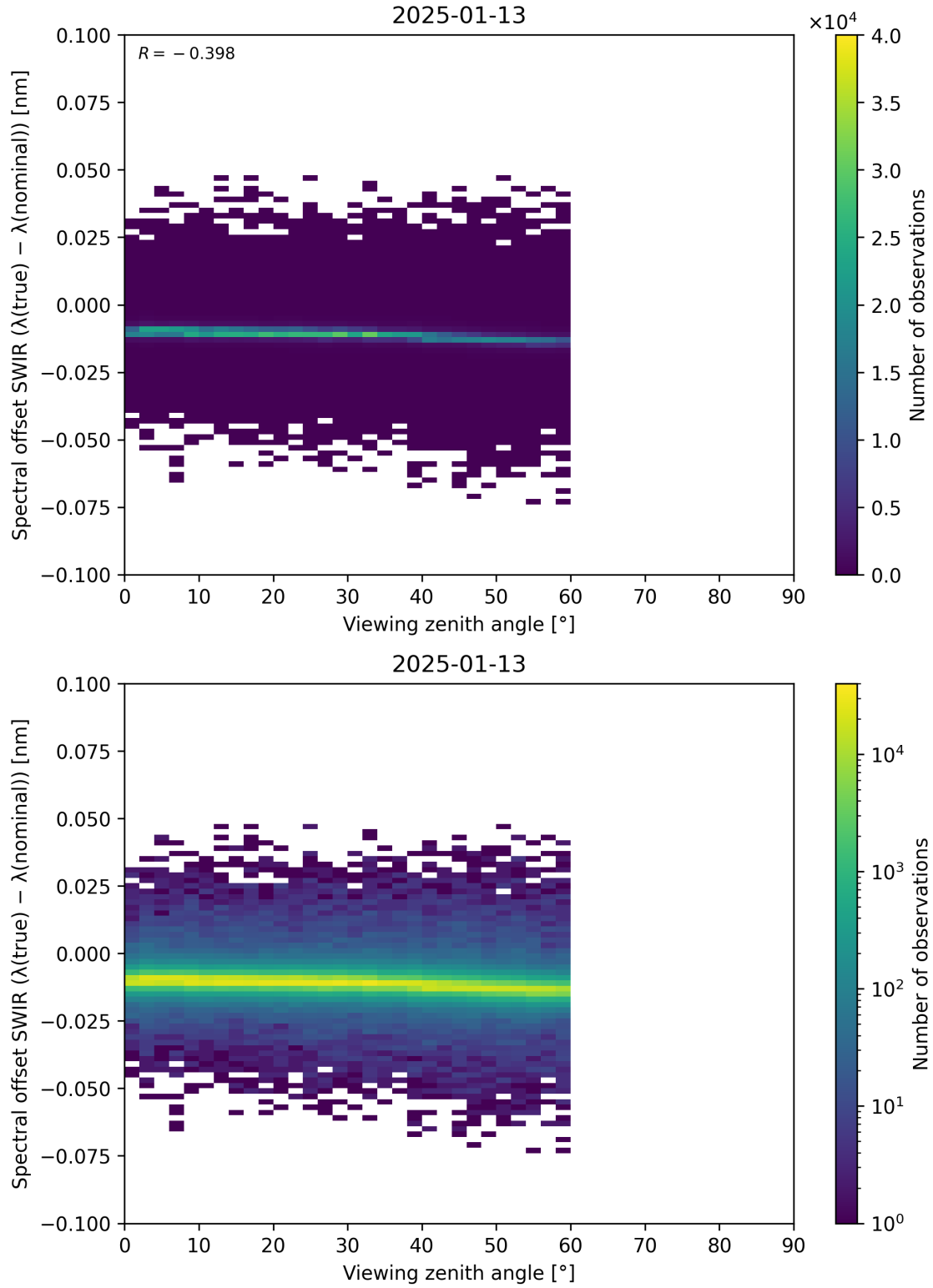
Figure 116: Scatter density plot of “Viewing zenith angle” against “Spectral offset SWIR ( \lambda_{\text{true}} - \lambda_{\text{nominal}} )” for 2025-01-12 to 2025-01-14.
