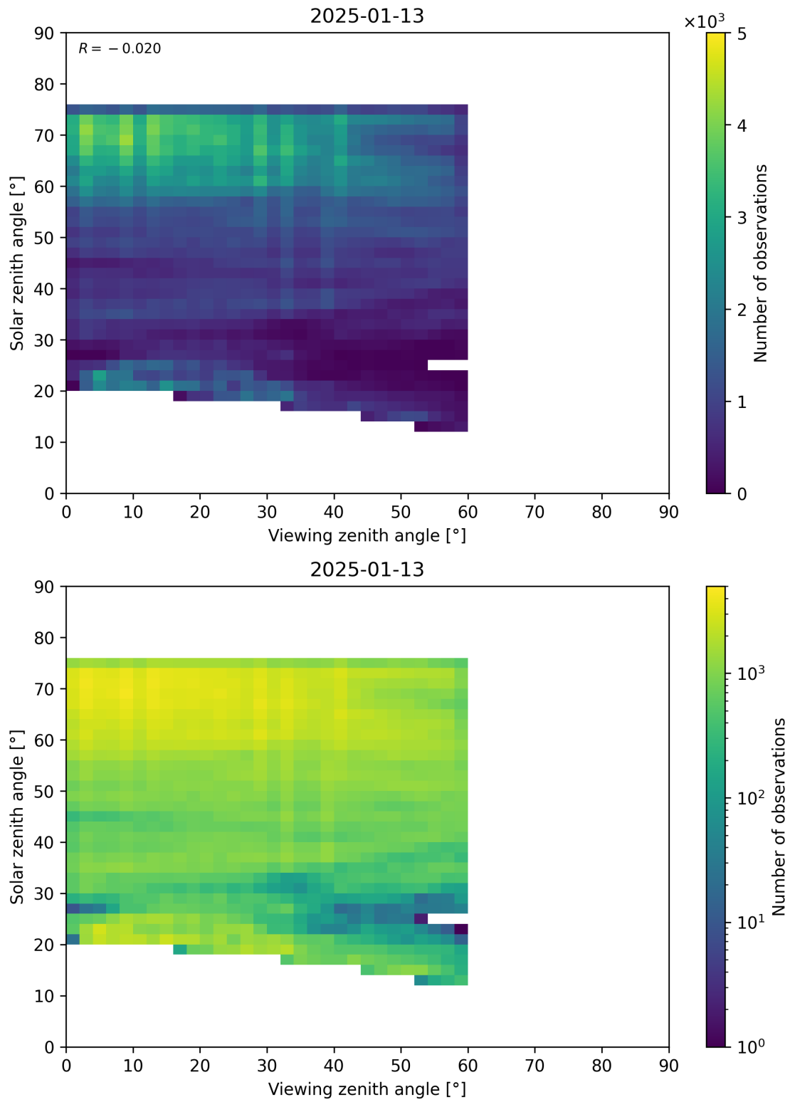
Figure 115: Scatter density plot of “Viewing zenith angle” against “Solar zenith angle” for 2025-01-12 to 2025-01-14.
