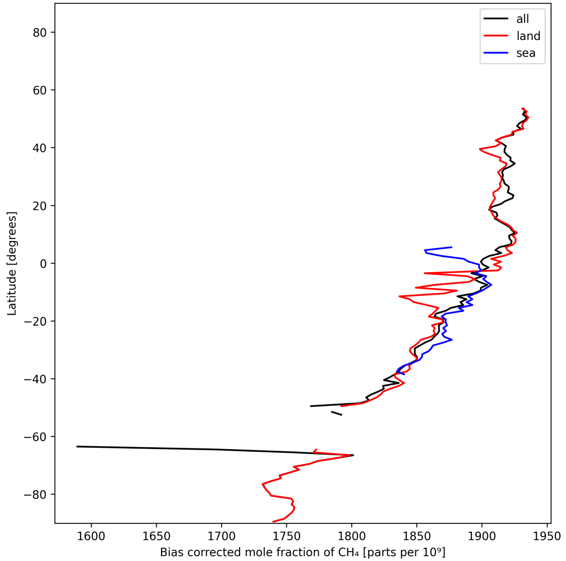
Figure 14: Zonal average of “Bias corrected mole fraction of CH 4 ” for 2025-01-12 to 2025-01-14.
