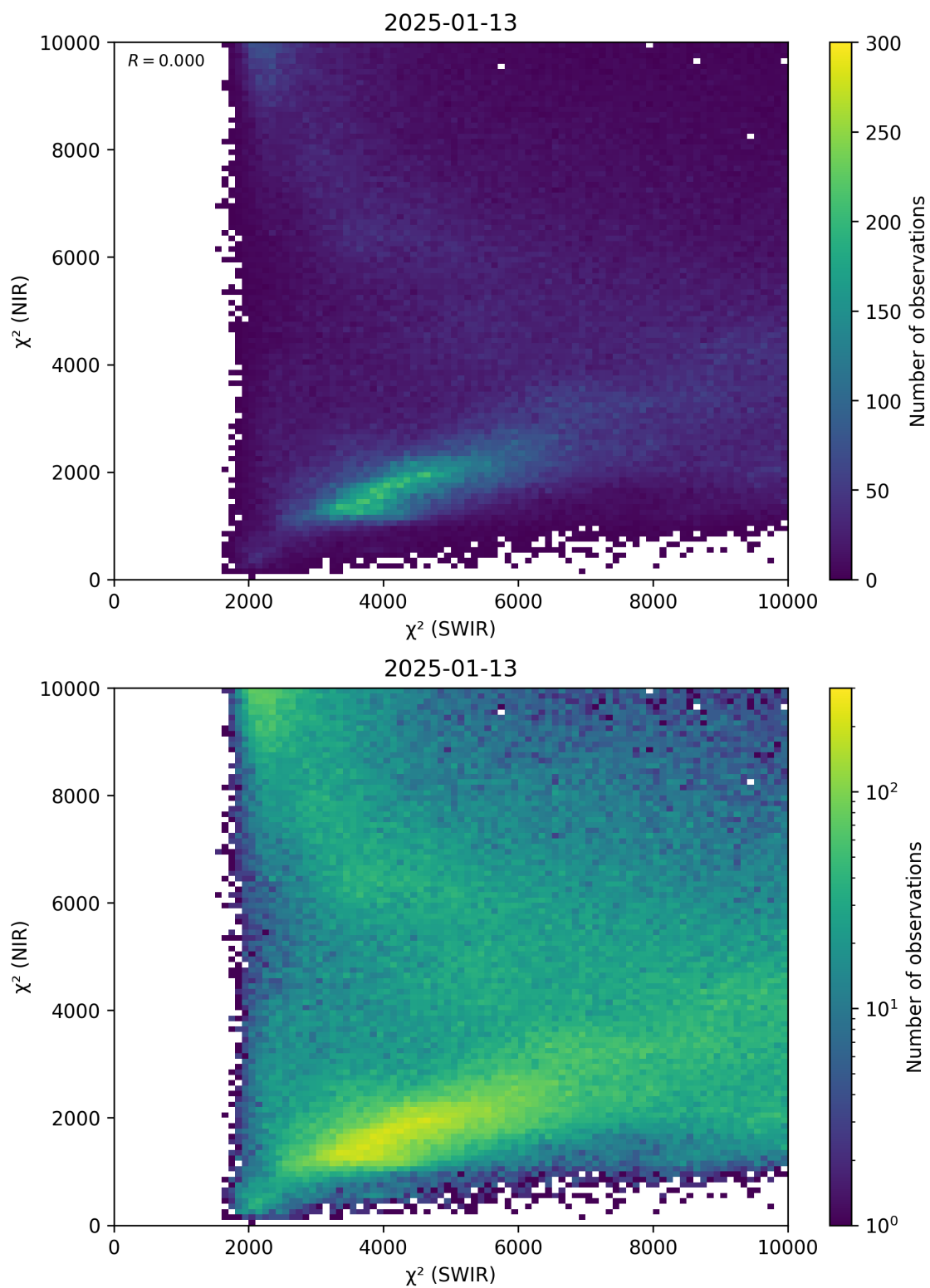
Figure 47: Scatter density plot of “ \chi^2 (SWIR)” against “ \chi^2 (NIR)” for 2025-01-12 to 2025-01-14.
