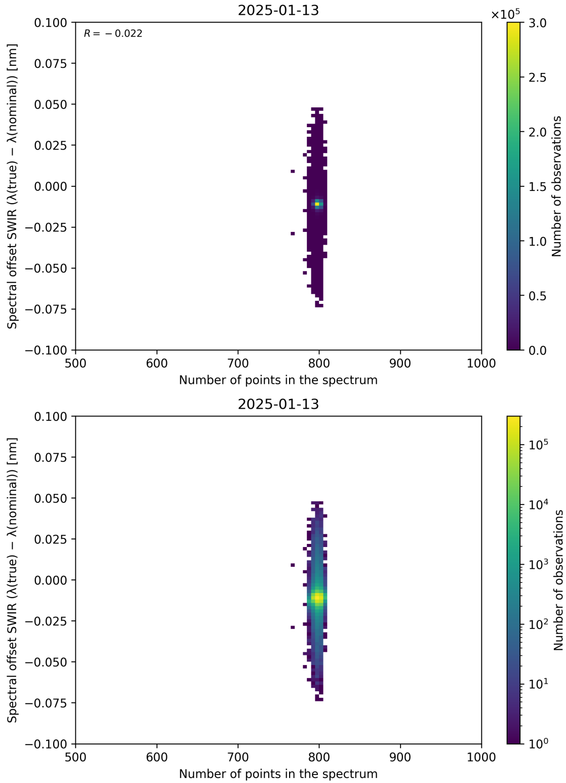
Figure 93: Scatter density plot of “Number of points in the spectrum” against “Spectral offset SWIR ( \lambda_{\text{true}} - \lambda_{\text{nominal}} )” for 2025-01-12 to 2025-01-14.
