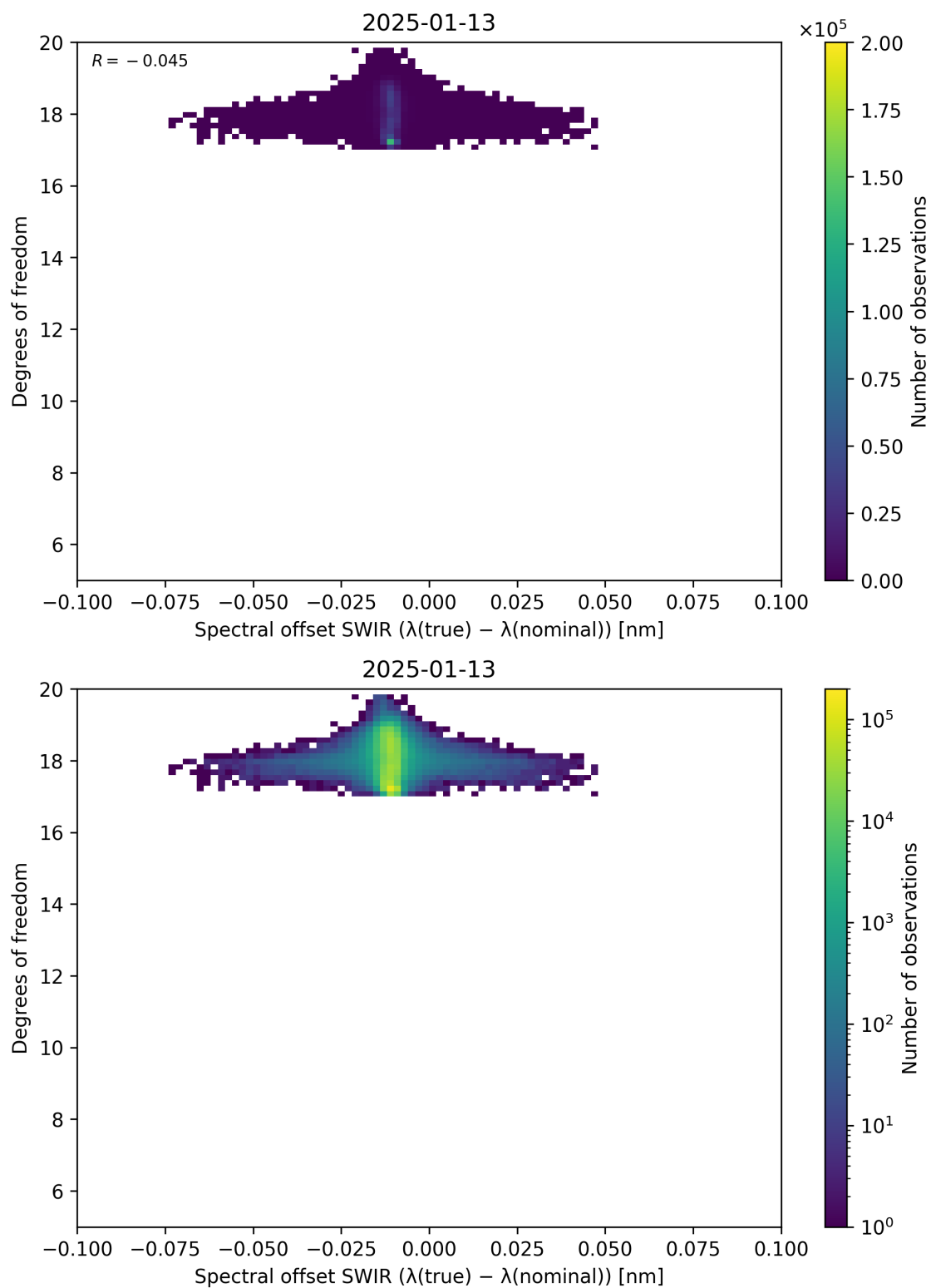
Figure 119: Scatter density plot of “Spectral offset SWIR ( \lambda_{\text{true}} - \lambda_{\text{nominal}} )” against “Degrees of freedom” for 2025-01-12 to 2025-01-14.
