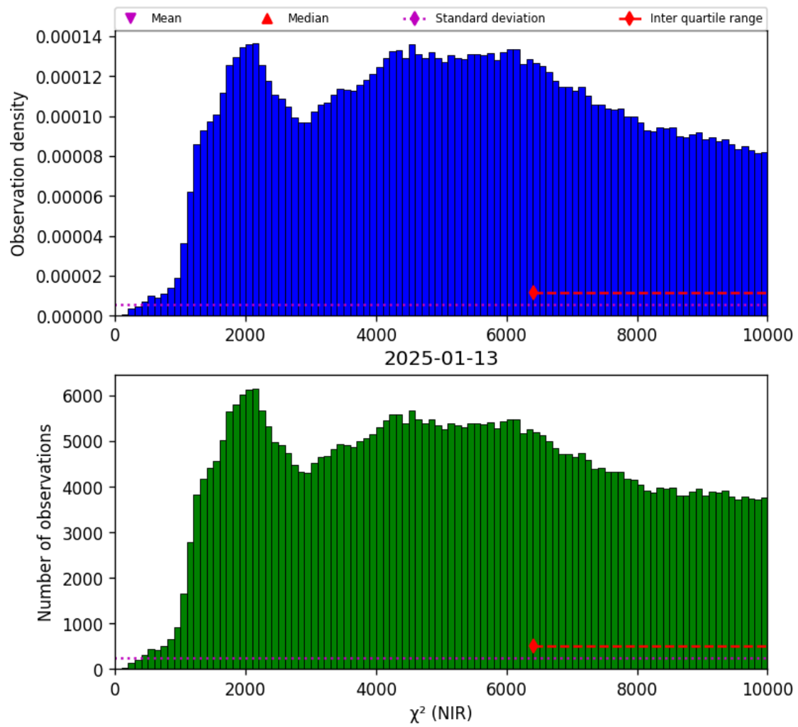
Figure 29: Histogram of “ \chi^2 (NIR)” for 2025-01-12 to 2025-01-14
