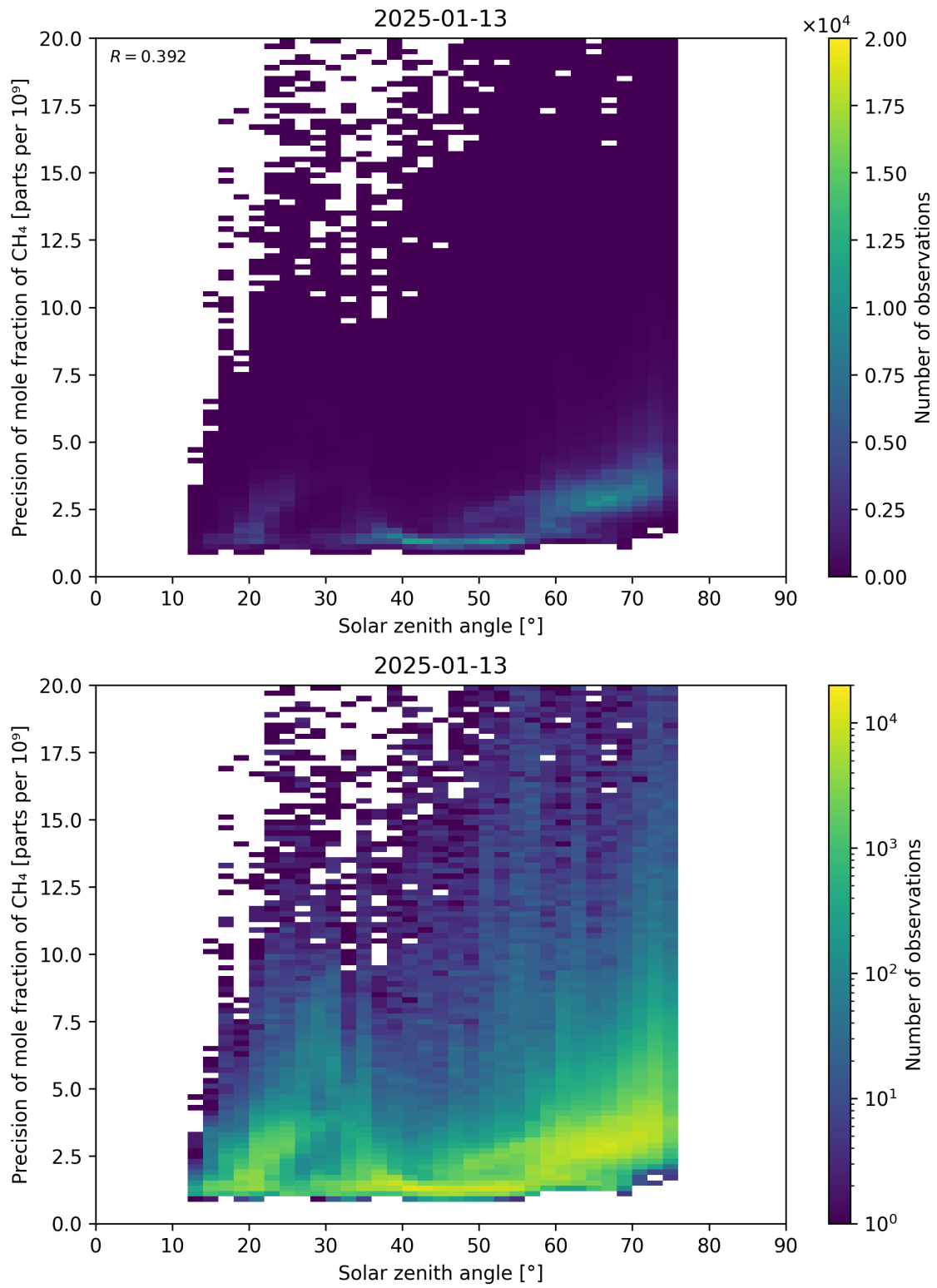
Figure 101: Scatter density plot of “Solar zenith angle” against “Precision of mole fraction of CH 4 ” for 2025-01-12 to 2025-01-14.
