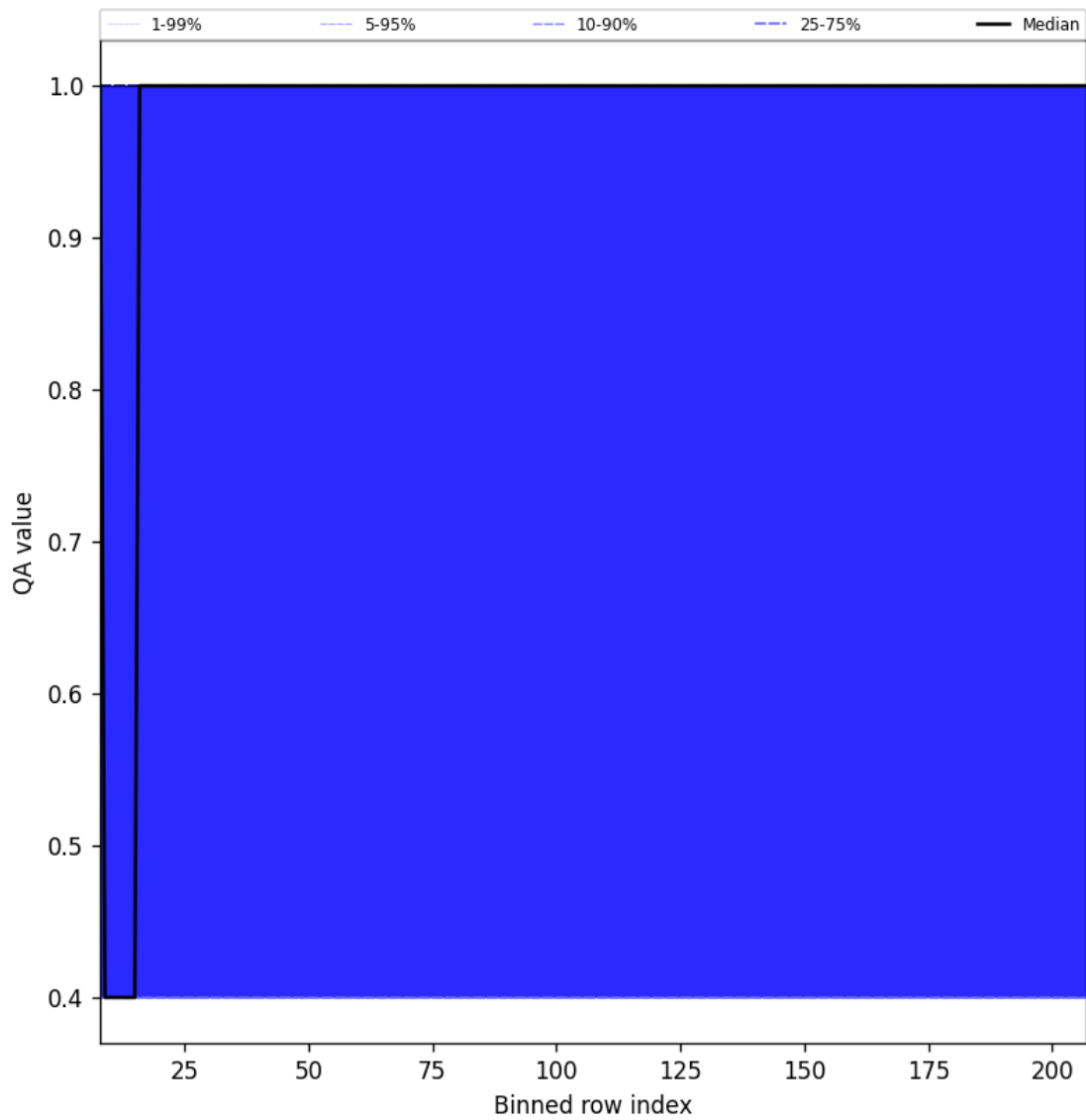
Figure 33: Along track statistics of “QA value” for 2025-01-12 to 2025-01-14
