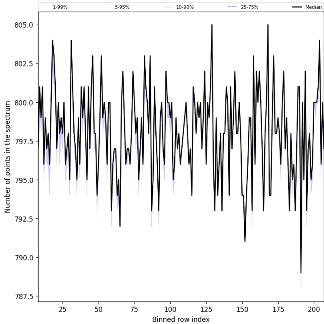
Figure 37: Along track statistics of “Number of points in the spectrum” for 2025-01-12 to 2025-01-14
