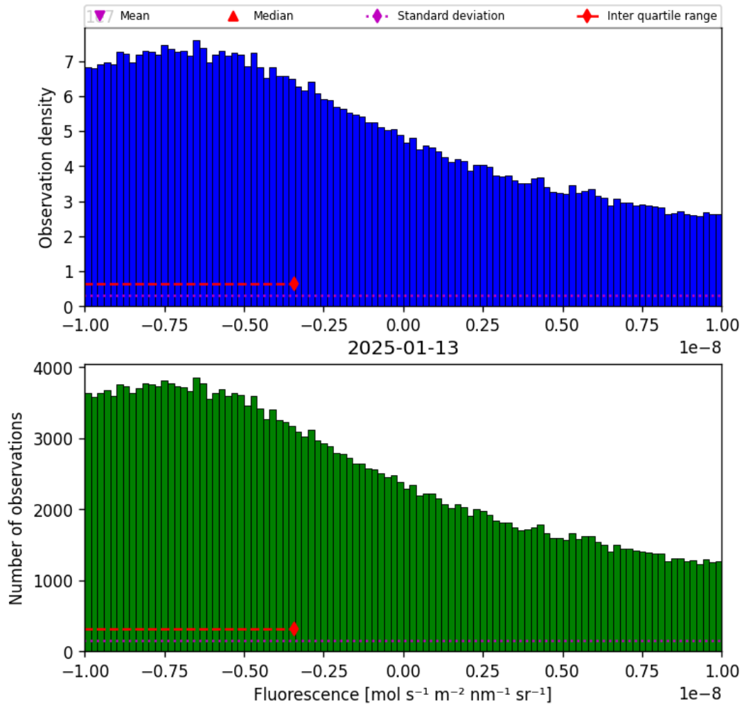
Figure 32: Histogram of “Fluorescence” for 2025-01-12 to 2025-01-14
