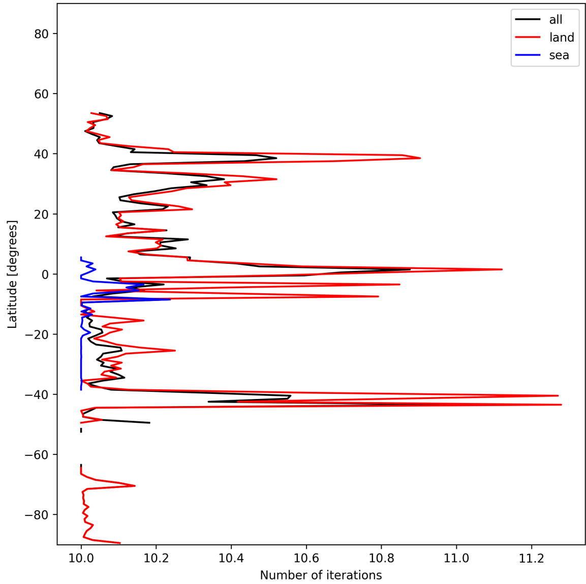
Figure 20: Zonal average of “Number of iterations” for 2025-01-12 to 2025-01-14.
