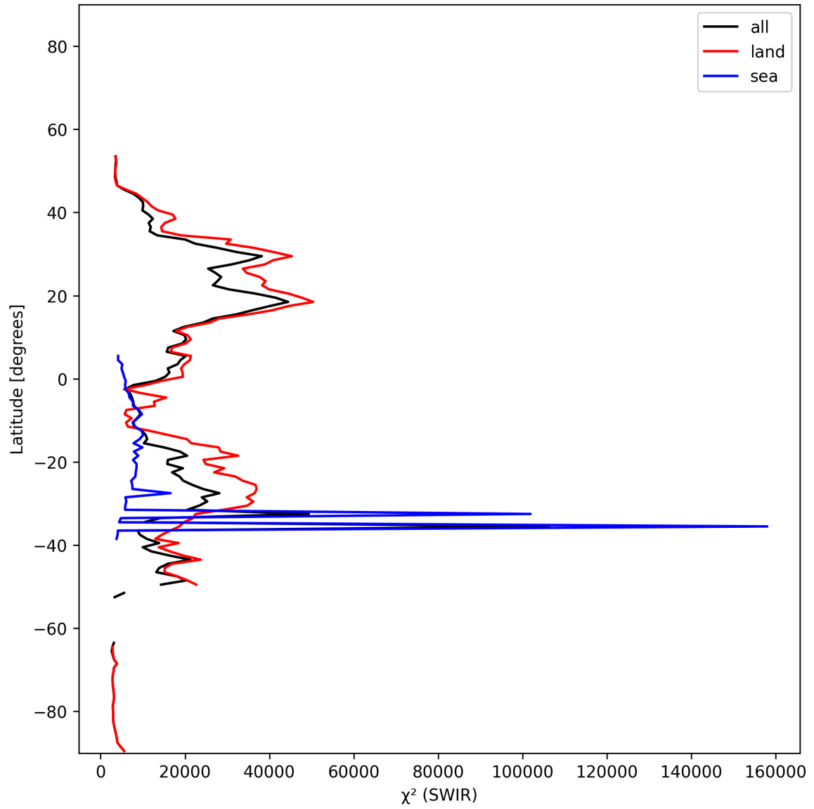
Figure 17: Zonal average of “ \chi^2 (SWIR)” for 2025-01-12 to 2025-01-14.
