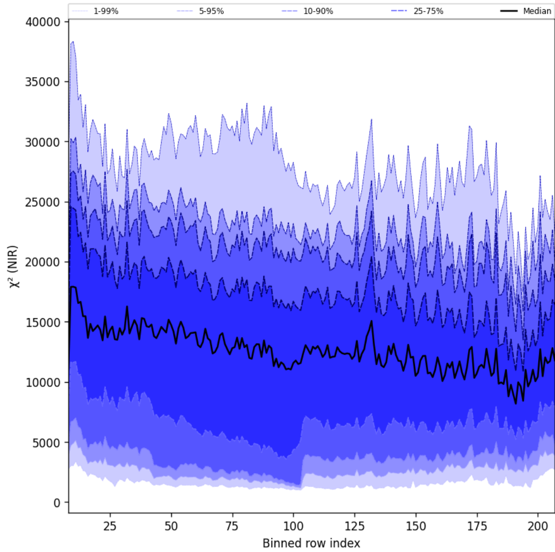
Figure 40: Along track statistics of “ \chi^2 (NIR)” for 2025-01-12 to 2025-01-14
