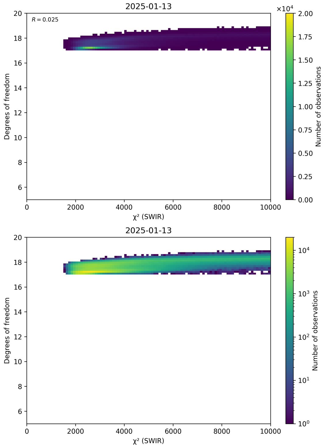
Figure 48: Scatter density plot of “ \chi^2 (SWIR)” against “Degrees of freedom” for 2025-01-12 to 2025-01-14.
