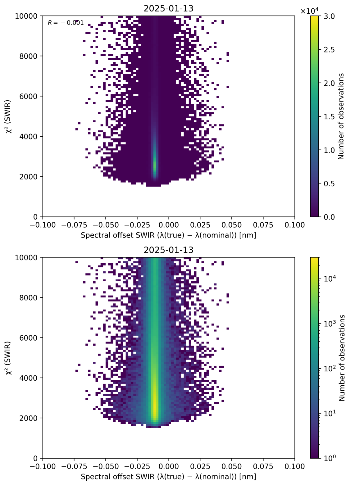
Figure 118: Scatter density plot of “Spectral offset SWIR ( \lambda_{\text{true}} - \lambda_{\text{nominal}} )” against “ \chi^2 (SWIR)” for 2025-01-12 to 2025-01-14.
