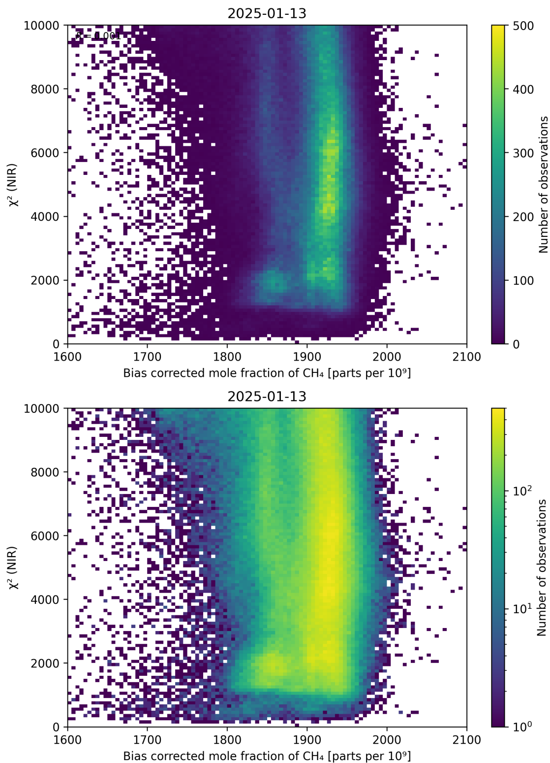
Figure 63: Scatter density plot of “Bias corrected mole fraction of CH 4 ” against “ \chi^2 (NIR)” for 2025-01-12 to 2025-01-14.
