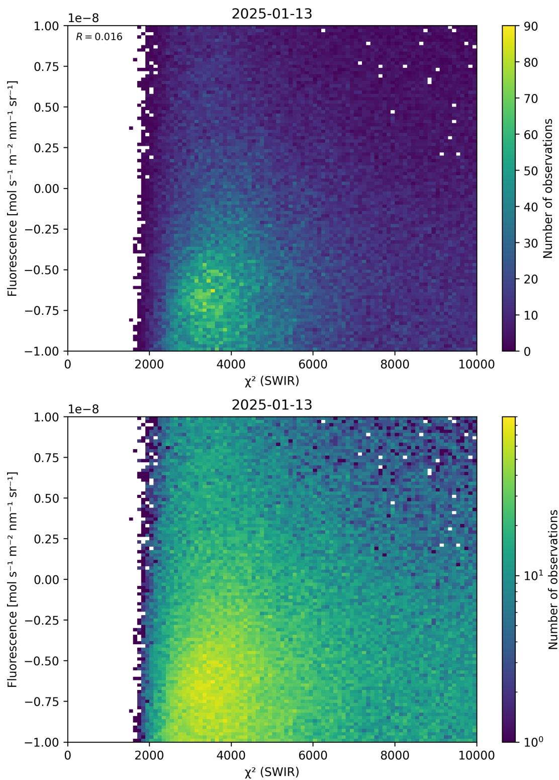
Figure 49: Scatter density plot of “ \chi^2 (SWIR)” against “Fluorescence” for 2025-01-12 to 2025-01-14.
