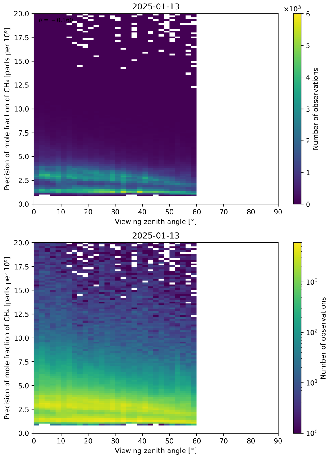
Figure 112: Scatter density plot of “Viewing zenith angle” against “Precision of mole fraction of CH 4 ” for 2025-01-12 to 2025-01-14.
