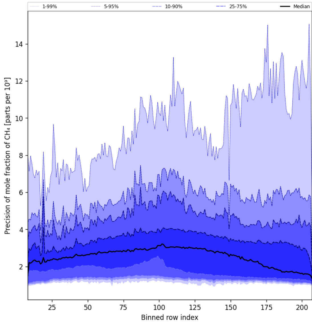
Figure 35: Along track statistics of “Precision of mole fraction of CH 4 ” for 2025-01-12 to 2025-01-14
