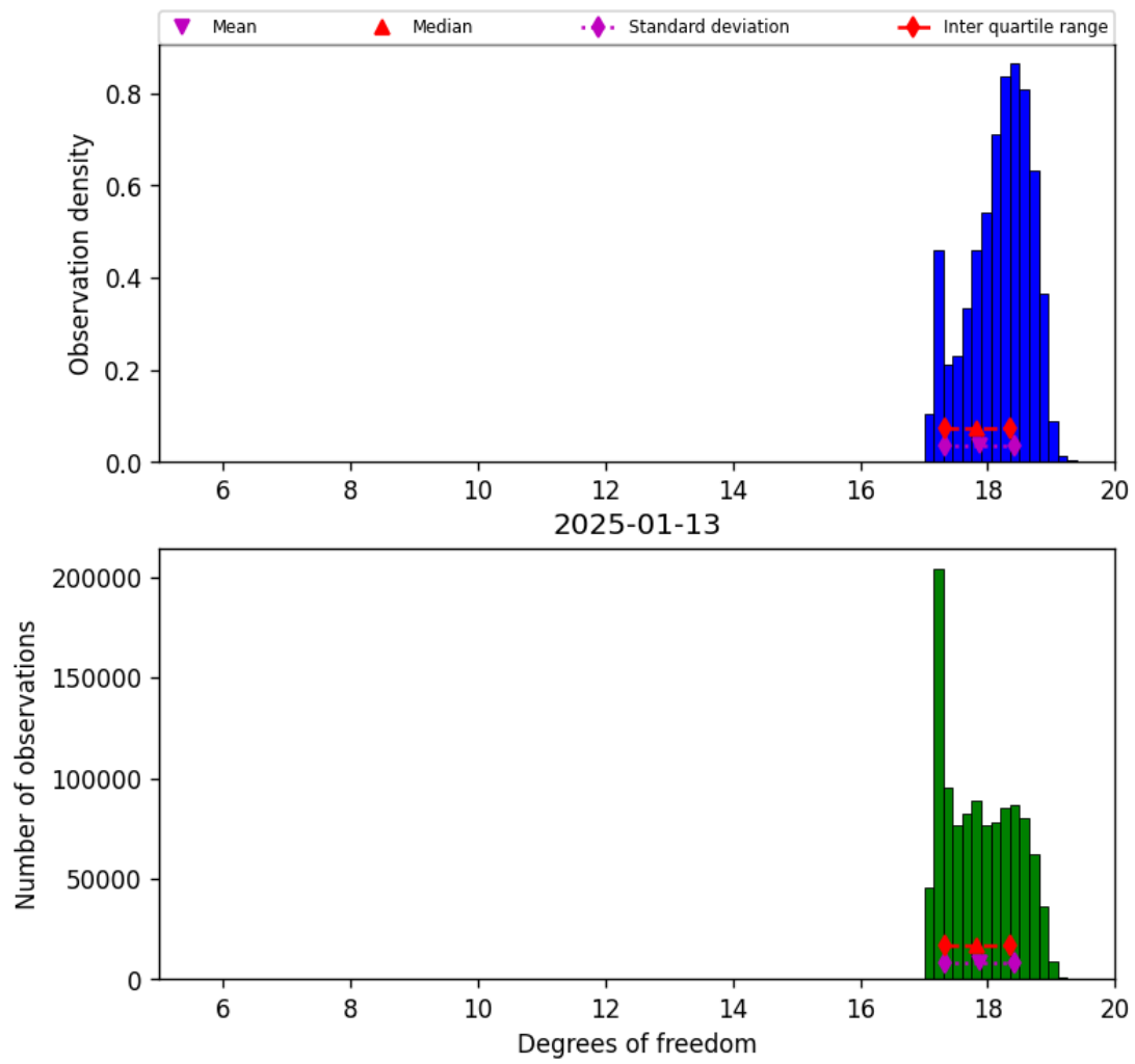
Figure 30: Histogram of “Degrees of freedom” for 2025-01-12 to 2025-01-14
