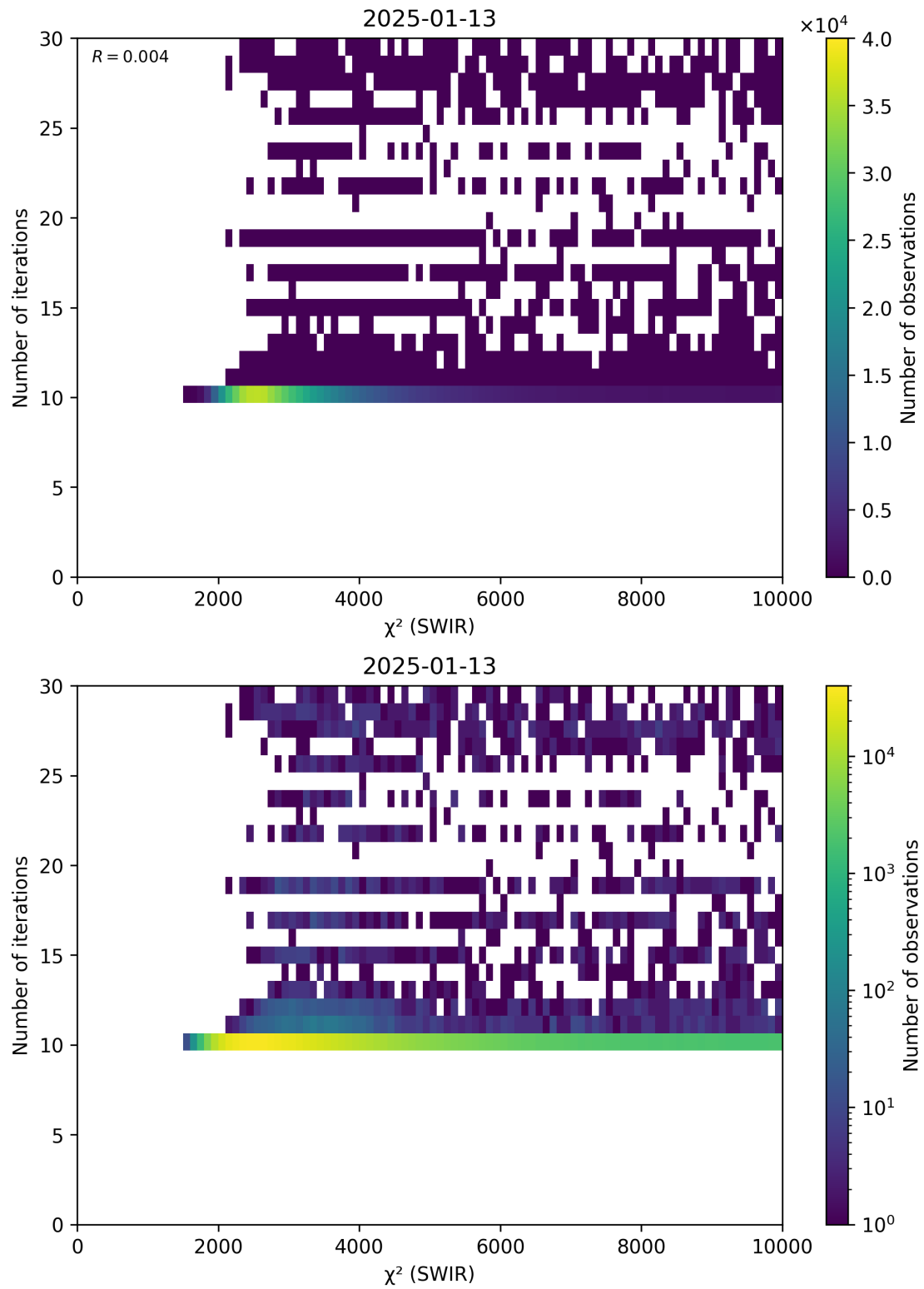
Figure 50: Scatter density plot of “ \chi^2 (SWIR)” against “Number of iterations” for 2025-01-12 to 2025-01-14.
