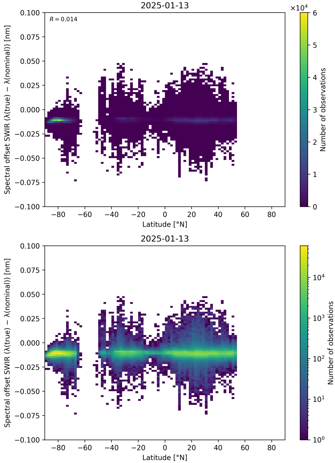
Figure 62: Scatter density plot of “Latitude” against “Spectral offset SWIR ( \lambda_{\text{true}} - \lambda_{\text{nominal}} )” for 2025-01-12 to 2025-01-14.
