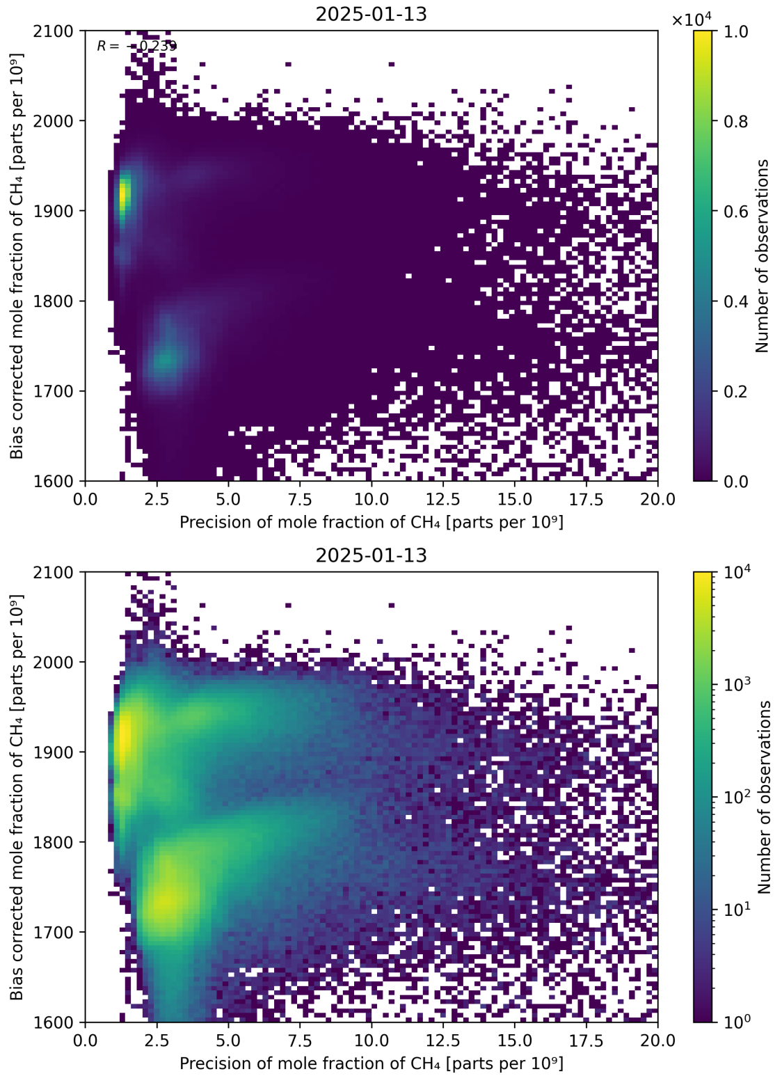
Figure 82: Scatter density plot of “Precision of mole fraction of CH 4 ” against “Bias corrected mole fraction of CH 4 ” for 2025-01-12 to 2025-01-14.
