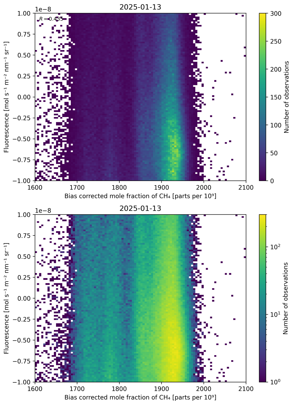
Figure 66: Scatter density plot of “Bias corrected mole fraction of \text{CH}_4 ” against “Fluorescence” for 2025-01-12 to 2025-01-14.
