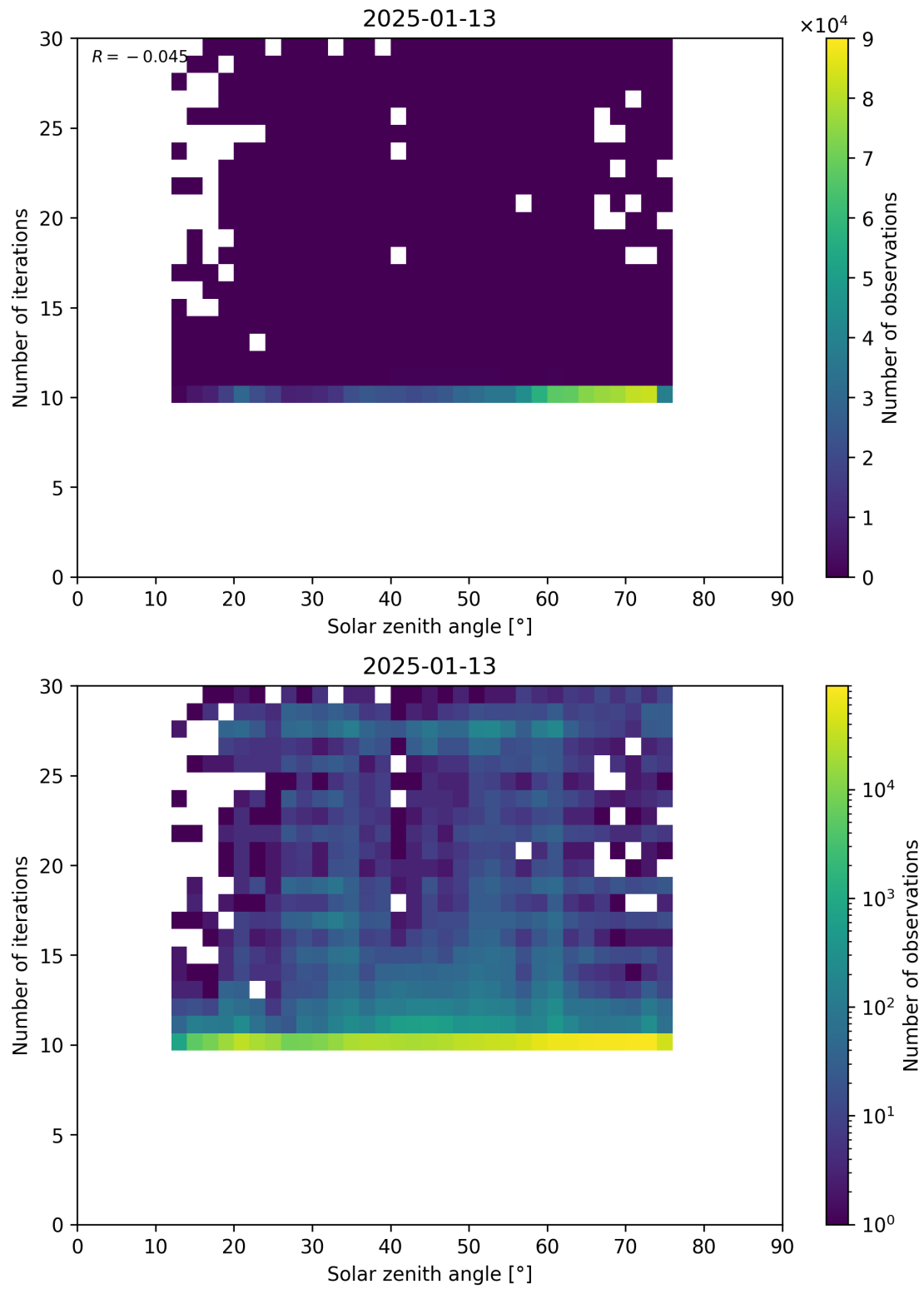
Figure 102: Scatter density plot of “Solar zenith angle” against “Number of iterations” for 2025-01-12 to 2025-01-14.
