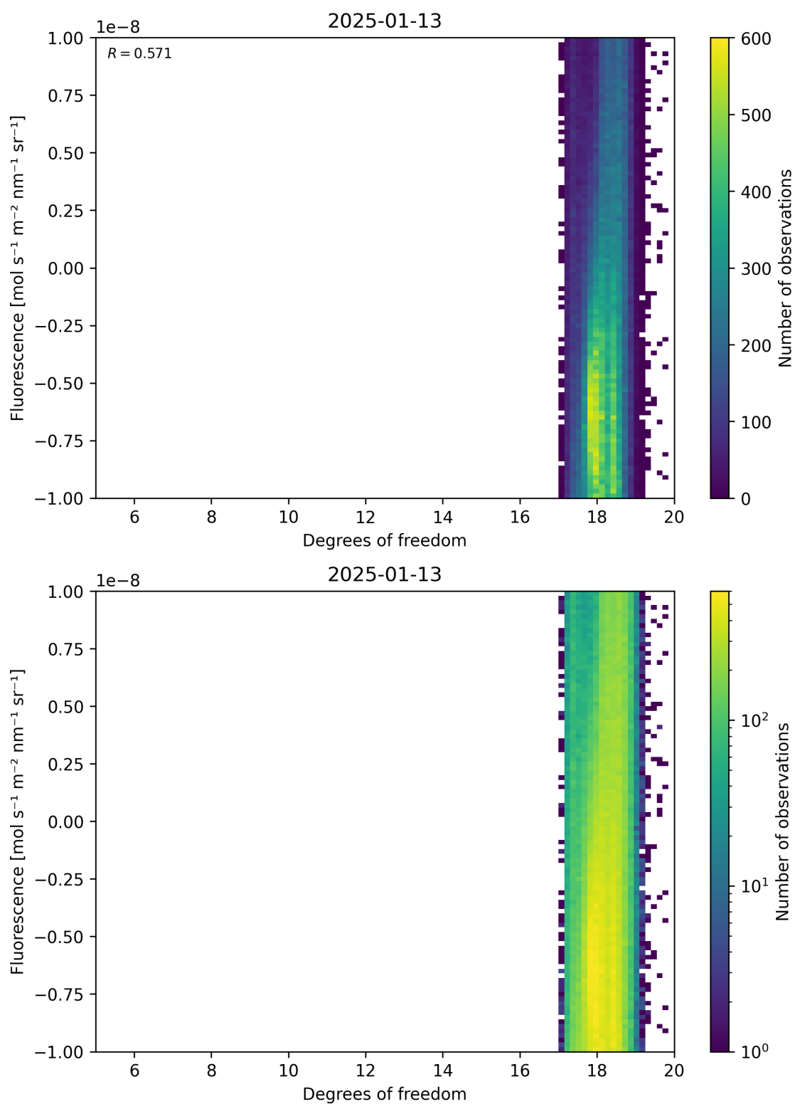
Figure 51: Scatter density plot of “Degrees of freedom” against “Fluorescence” for 2025-01-12 to 2025-01-14.
