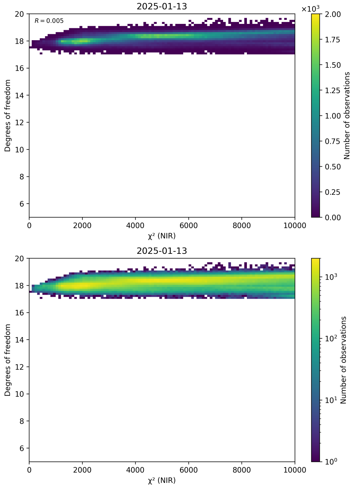
Figure 44: Scatter density plot of “ \chi^2 (NIR)” against “Degrees of freedom” for 2025-01-12 to 2025-01-14.
