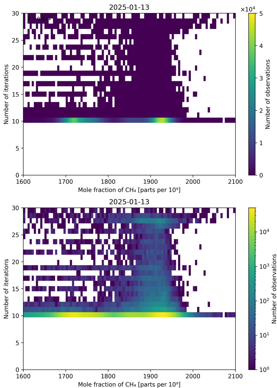
Figure 76: Scatter density plot of “Mole fraction of CH 4 ” against “Number of iterations” for 2025-01-12 to 2025-01-14.
