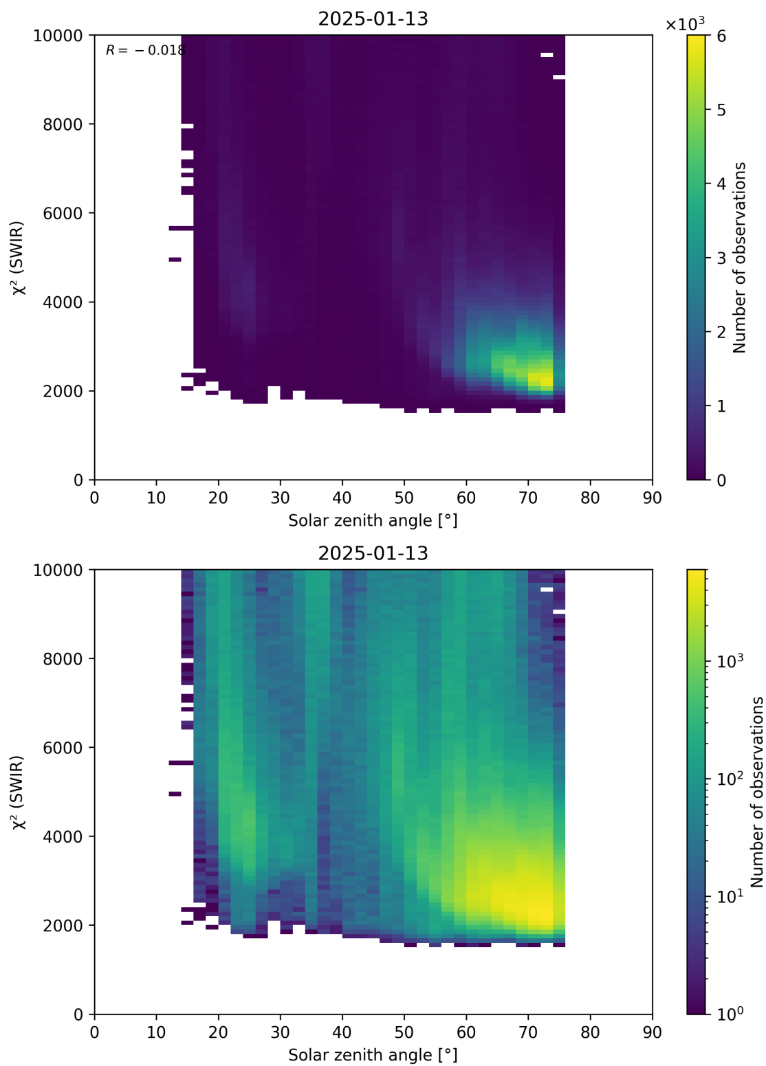
Figure 95: Scatter density plot of “Solar zenith angle” against “ \chi^2 (SWIR)” for 2025-01-12 to 2025-01-14.
