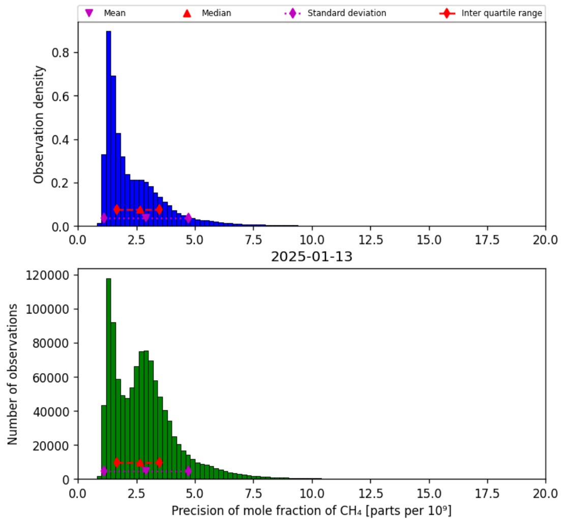
Figure 24: Histogram of “Precision of mole fraction of CH 4 ” for 2025-01-12 to 2025-01-14
