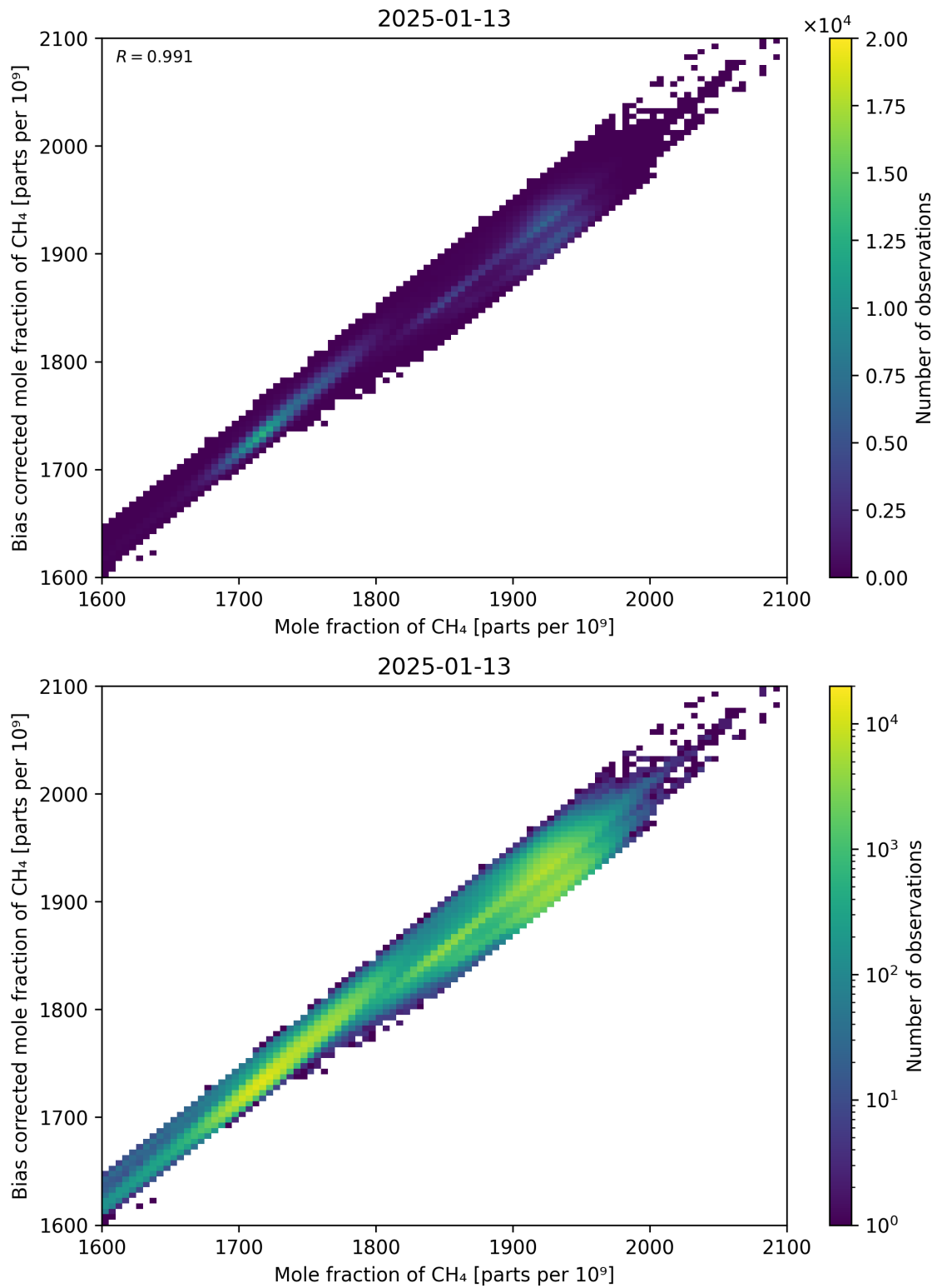
Figure 74: Scatter density plot of “Mole fraction of CH 4 ” against “Bias corrected mole fraction of CH 4 ” for 2025-01-12 to 2025-01-14.
