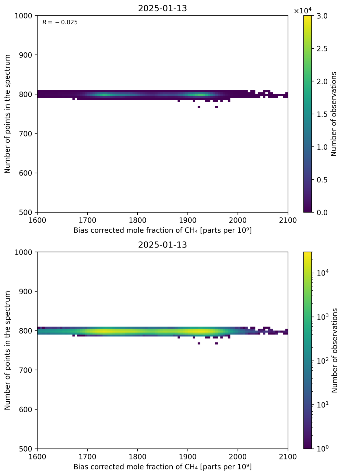
Figure 68: Scatter density plot of “Bias corrected mole fraction of CH 4 ” against “Number of points in the spectrum” for 2025-01-12 to 2025-01-14.
