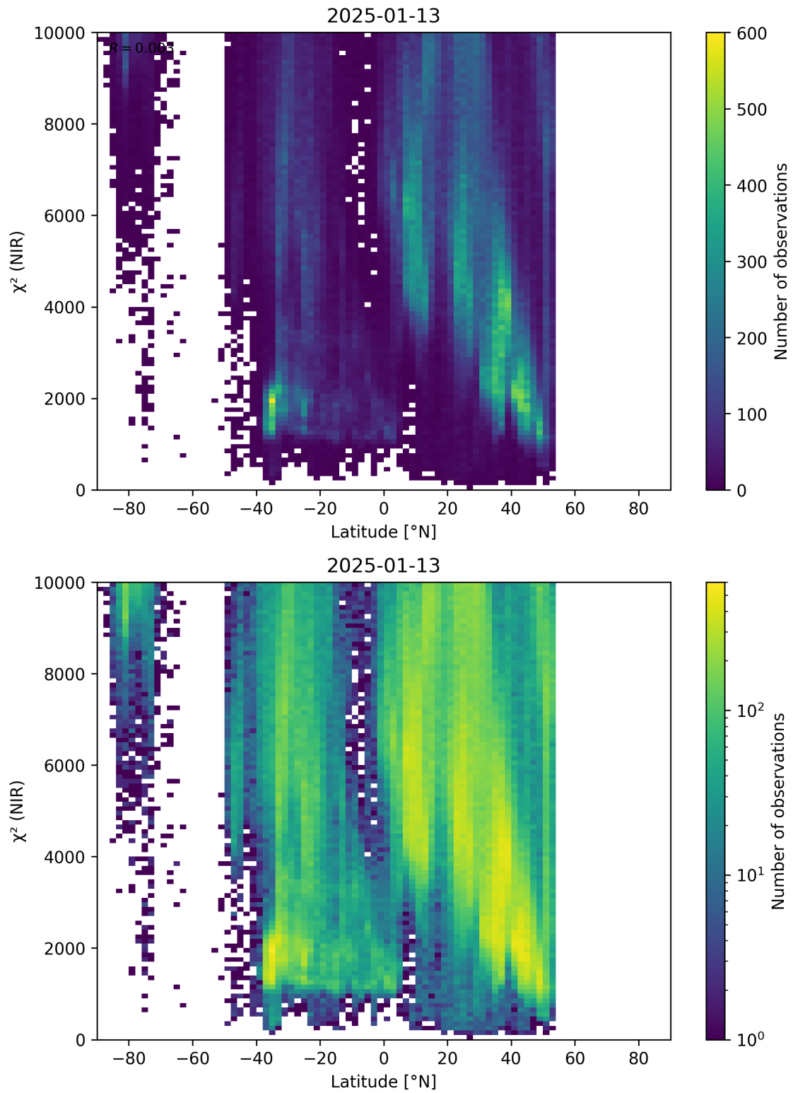
Figure 53: Scatter density plot of “Latitude” against “ \chi^2 (NIR)” for 2025-01-12 to 2025-01-14.
