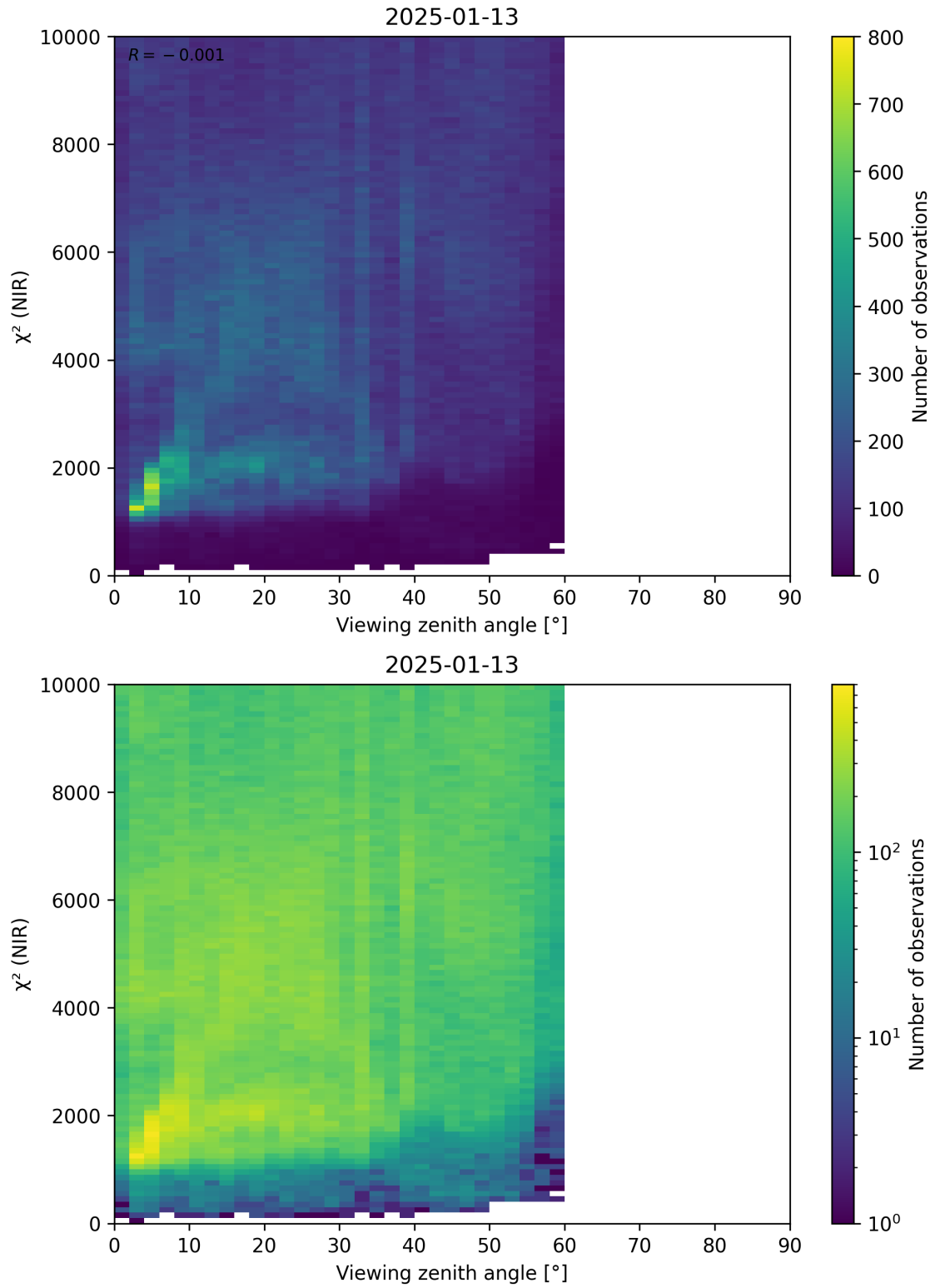
Figure 105: Scatter density plot of “Viewing zenith angle” against “ \chi^2 (NIR)” for 2025-01-12 to 2025-01-14.
