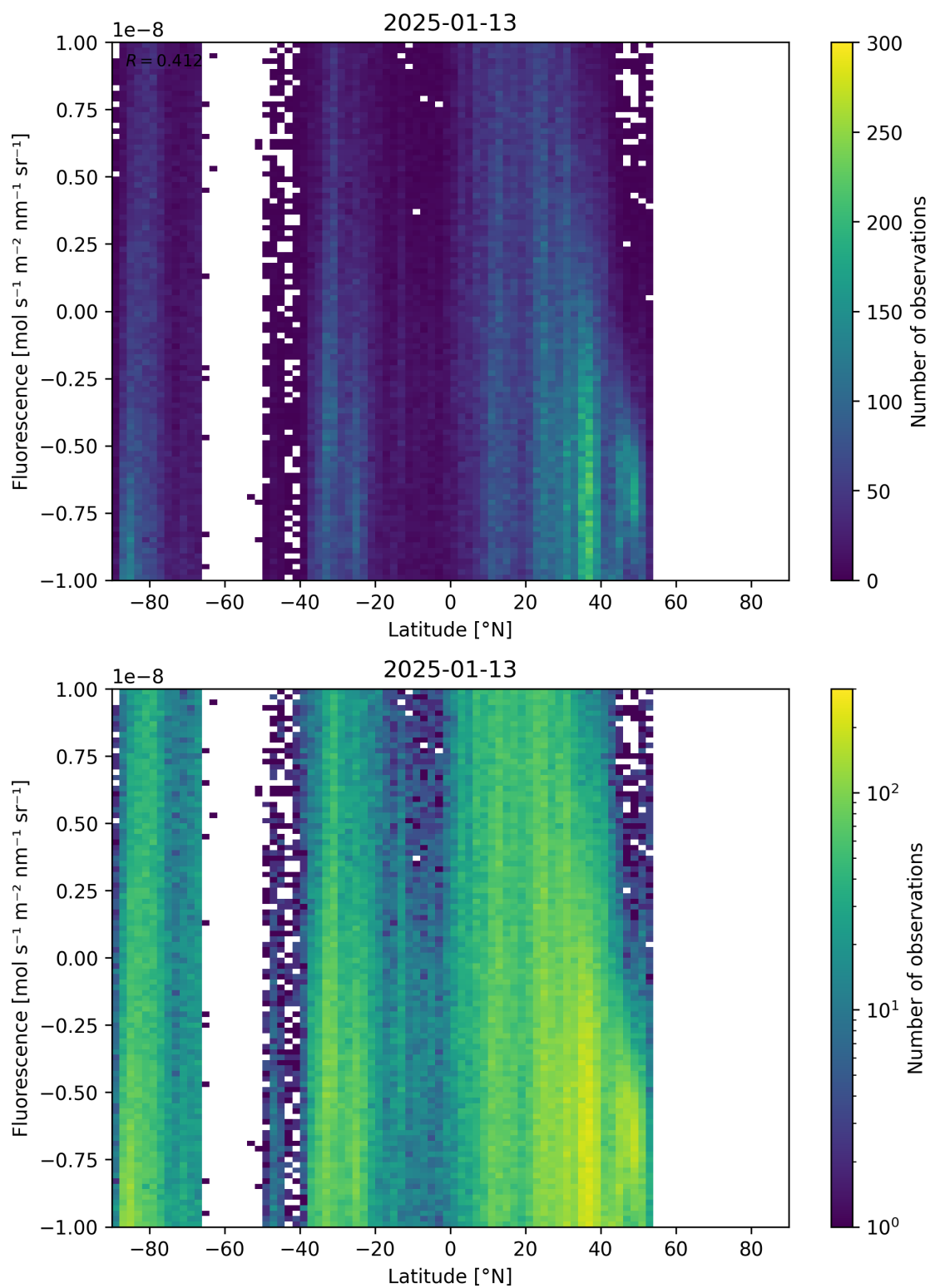
Figure 56: Scatter density plot of “Latitude” against “Fluorescence” for 2025-01-12 to 2025-01-14.
