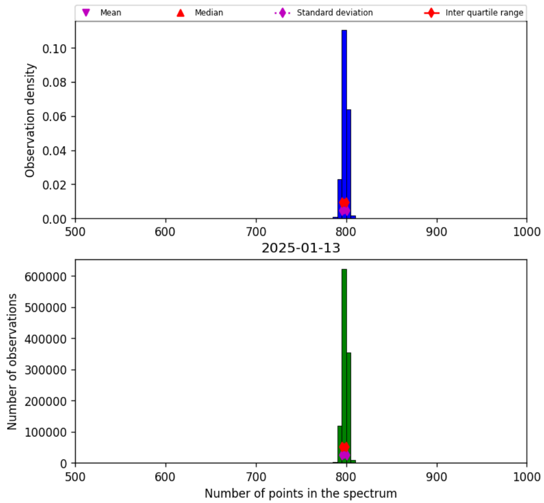
Figure 26: Histogram of “Number of points in the spectrum” for 2025-01-12 to 2025-01-14
