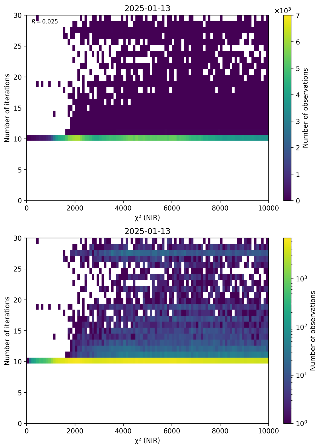
Figure 46: Scatter density plot of “ \chi^2 (NIR)” against “Number of iterations” for 2025-01-12 to 2025-01-14.
