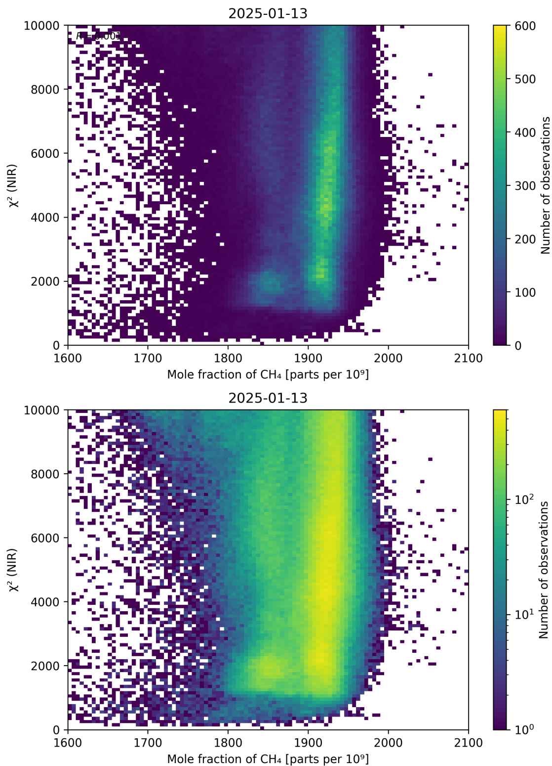
Figure 70: Scatter density plot of “Mole fraction of CH 4 ” against “ \chi^2 (NIR)” for 2025-01-12 to 2025-01-14.
