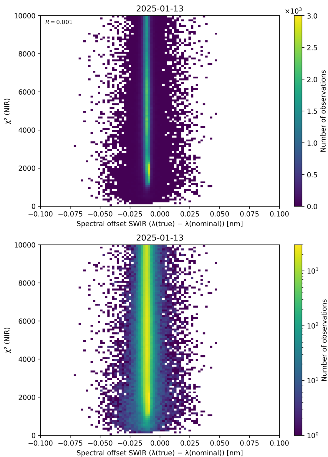
Figure 117: Scatter density plot of “Spectral offset SWIR ( \lambda_{\text{true}} - \lambda_{\text{nominal}} )” against “ \chi^2 (NIR)” for 2025-01-12 to 2025-01-14.
