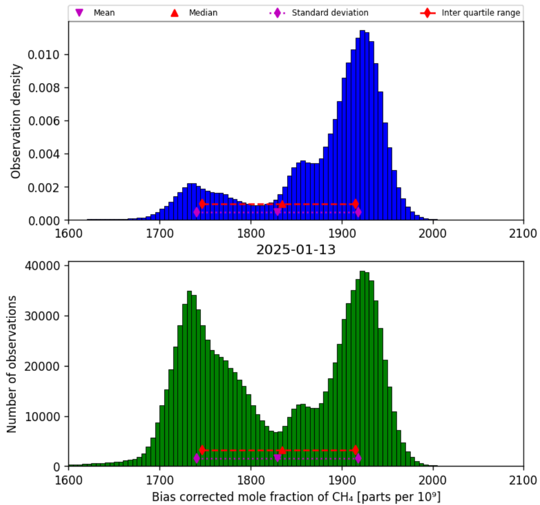
Figure 25: Histogram of “Bias corrected mole fraction of CH 4 ” for 2025-01-12 to 2025-01-14
