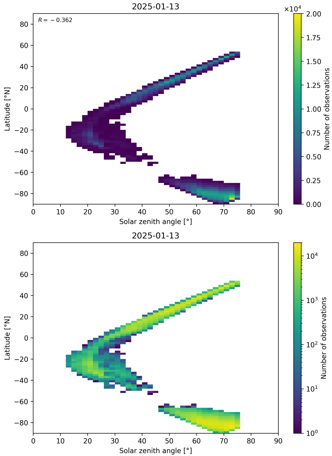
Figure 98: Scatter density plot of “Solar zenith angle” against “Latitude” for 2025-01-12 to 2025-01-14.
