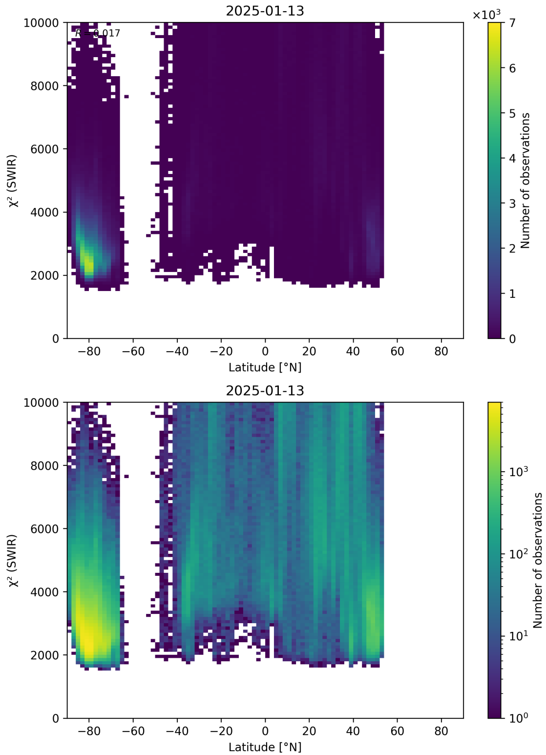
Figure 54: Scatter density plot of “Latitude” against “ \chi^2 (SWIR)” for 2025-01-12 to 2025-01-14.
