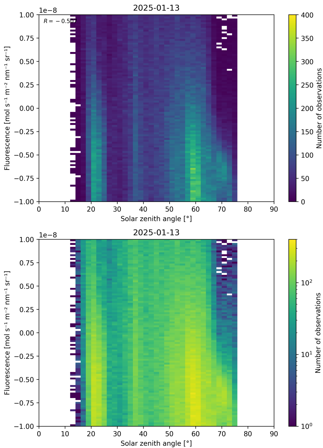
Figure 97: Scatter density plot of “Solar zenith angle” against “Fluorescence” for 2025-01-12 to 2025-01-14.
