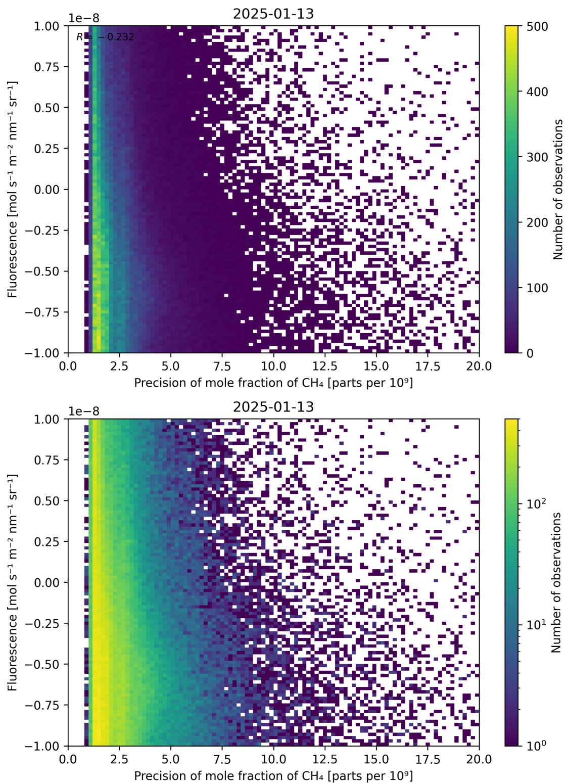
Figure 81: Scatter density plot of “Precision of mole fraction of \text{CH}_4 ” against “Fluorescence” for 2025-01-12 to 2025-01-14.
