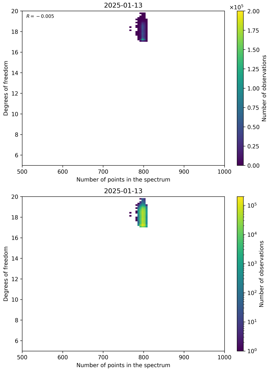
Figure 90: Scatter density plot of “Number of points in the spectrum” against “Degrees of freedom” for 2025-01-12 to 2025-01-14.
