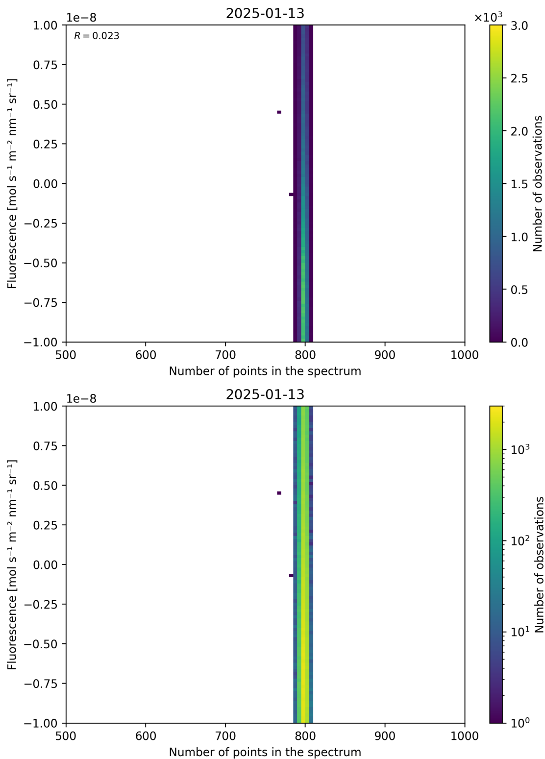
Figure 91: Scatter density plot of “Number of points in the spectrum” against “Fluorescence” for 2025-01-12 to 2025-01-14.
