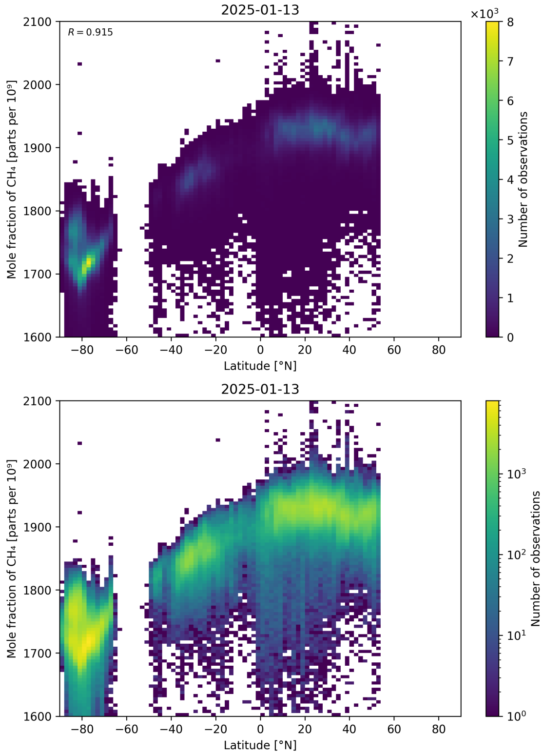
Figure 57: Scatter density plot of “Latitude” against “Mole fraction of \text{CH}_4 ” for 2025-01-12 to 2025-01-14.
