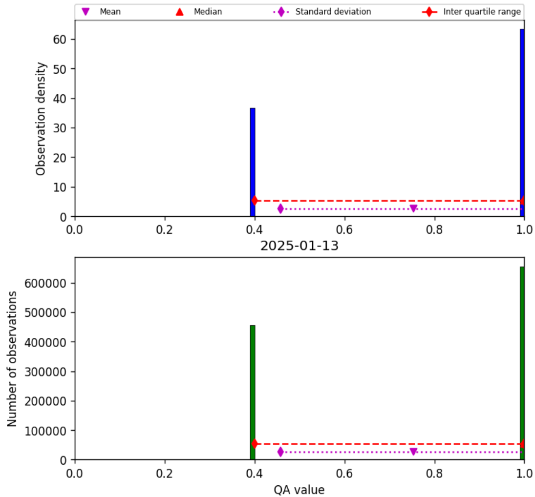
Figure 22: Histogram of “QA value” for 2025-01-12 to 2025-01-14
