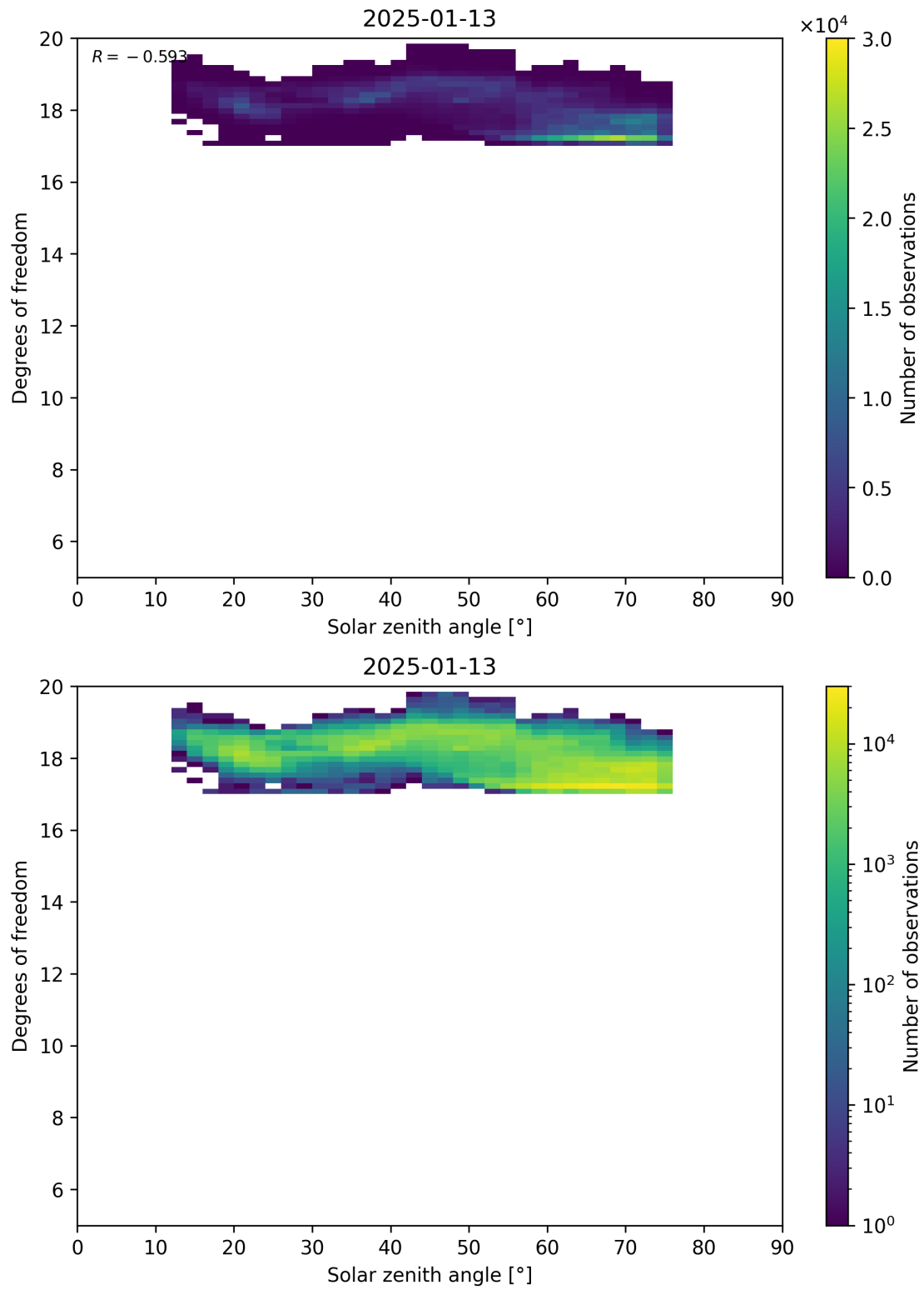
Figure 96: Scatter density plot of “Solar zenith angle” against “Degrees of freedom” for 2025-01-12 to 2025-01-14.
