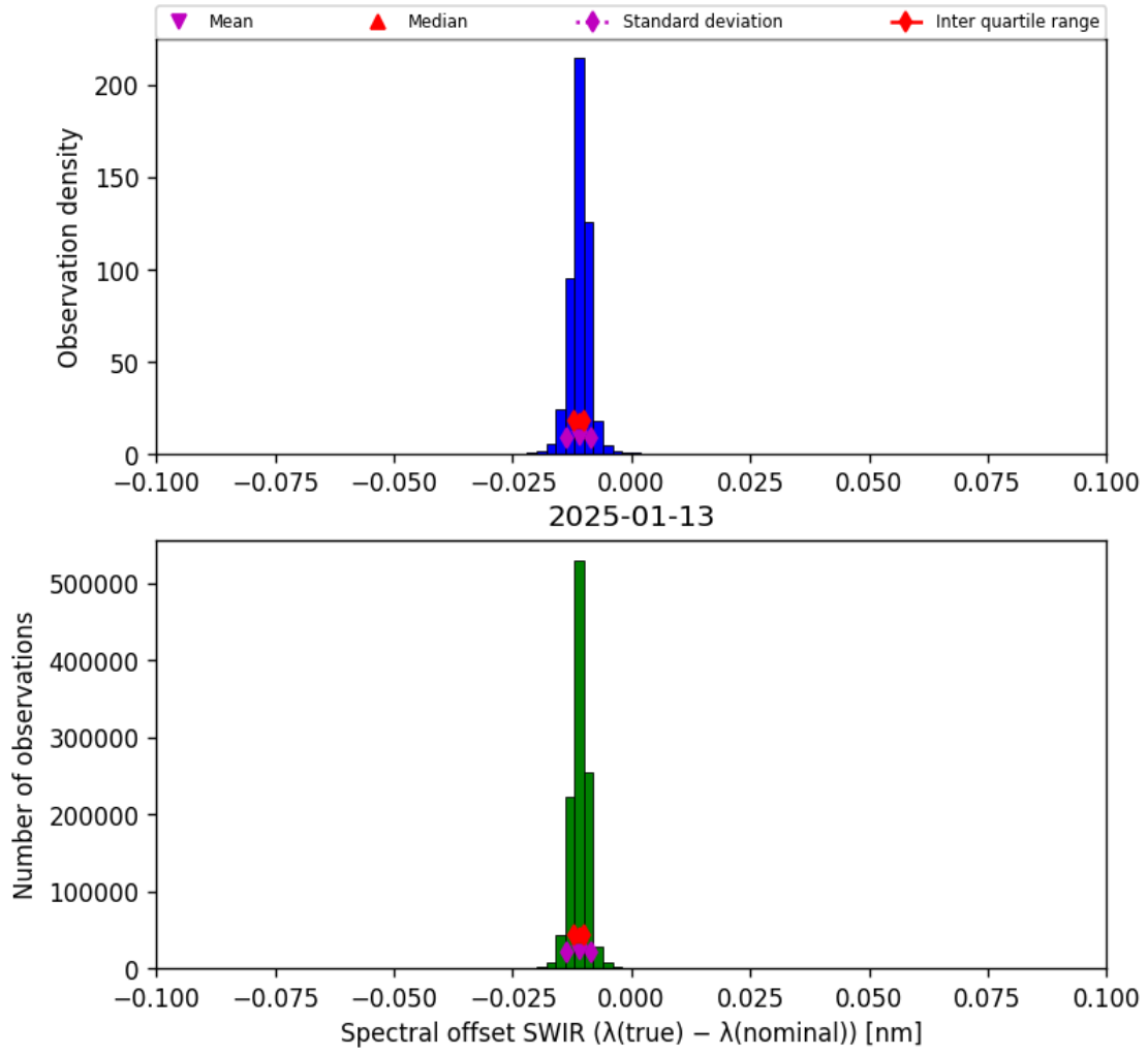
Figure 27: Histogram of “Spectral offset SWIR ( \lambda_{\text{true}} - \lambda_{\text{nominal}} )” for 2025-01-12 to 2025-01-14
