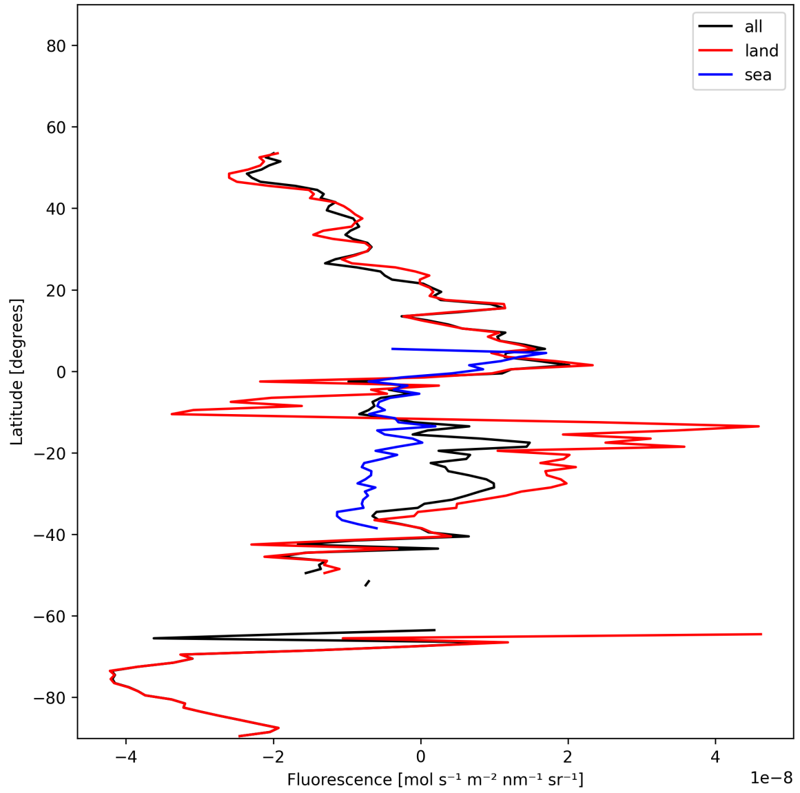
Figure 21: Zonal average of “Fluorescence” for 2025-01-12 to 2025-01-14.
