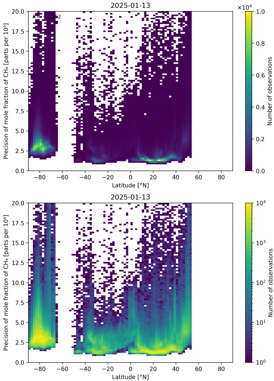
Figure 59: Scatter density plot of “Latitude” against “Precision of mole fraction of CH 4 ” for 2025-01-12 to 2025-01-14.
