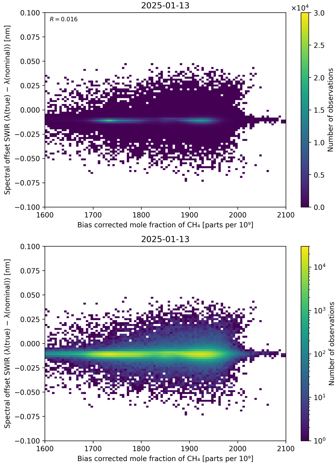
Figure 69: Scatter density plot of “Bias corrected mole fraction of \text{CH}_4 ” against “Spectral offset SWIR ( \lambda_{\text{true}} - \lambda_{\text{nominal}} )” for 2025-01-12 to 2025-01-14.
