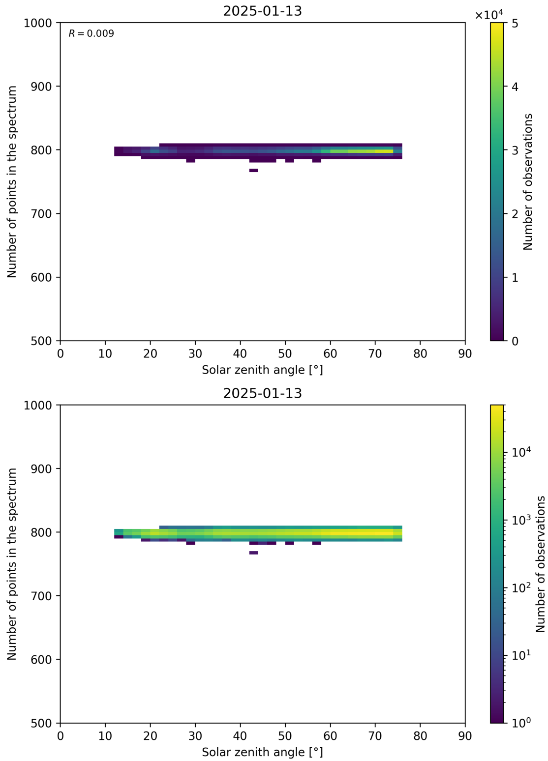
Figure 103: Scatter density plot of “Solar zenith angle” against “Number of points in the spectrum” for 2025-01-12 to 2025-01-14.
