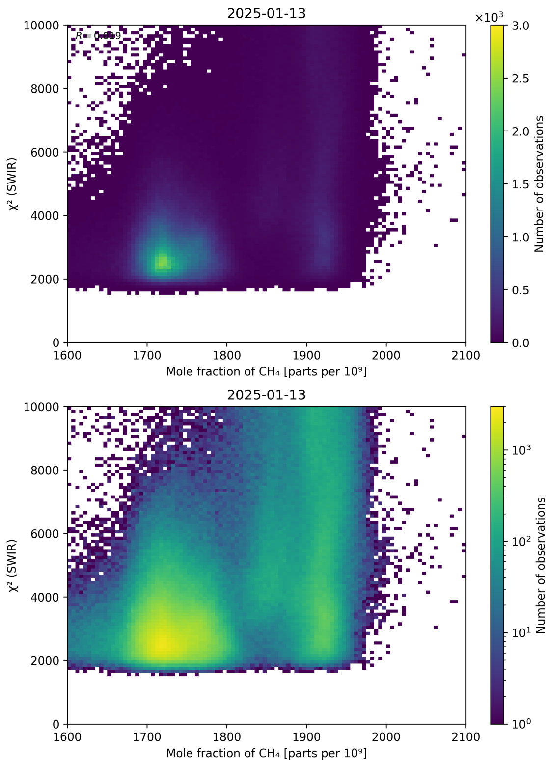
Figure 71: Scatter density plot of “Mole fraction of \text{CH}_4 ” against “ \chi^2 (SWIR)” for 2025-01-12 to 2025-01-14.
