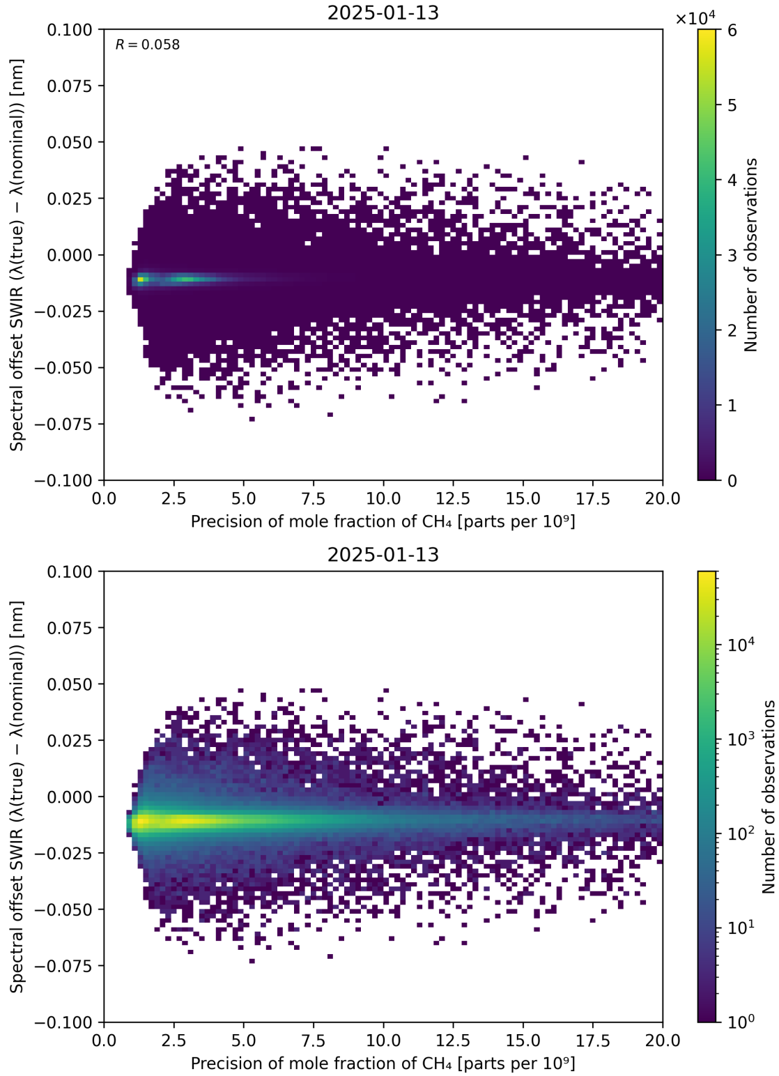
Figure 85: Scatter density plot of “Precision of mole fraction of CH 4 ” against “Spectral offset SWIR ( \lambda_{\text{true}} - \lambda_{\text{nominal}} )” for 2025-01-12 to 2025-01-14.
