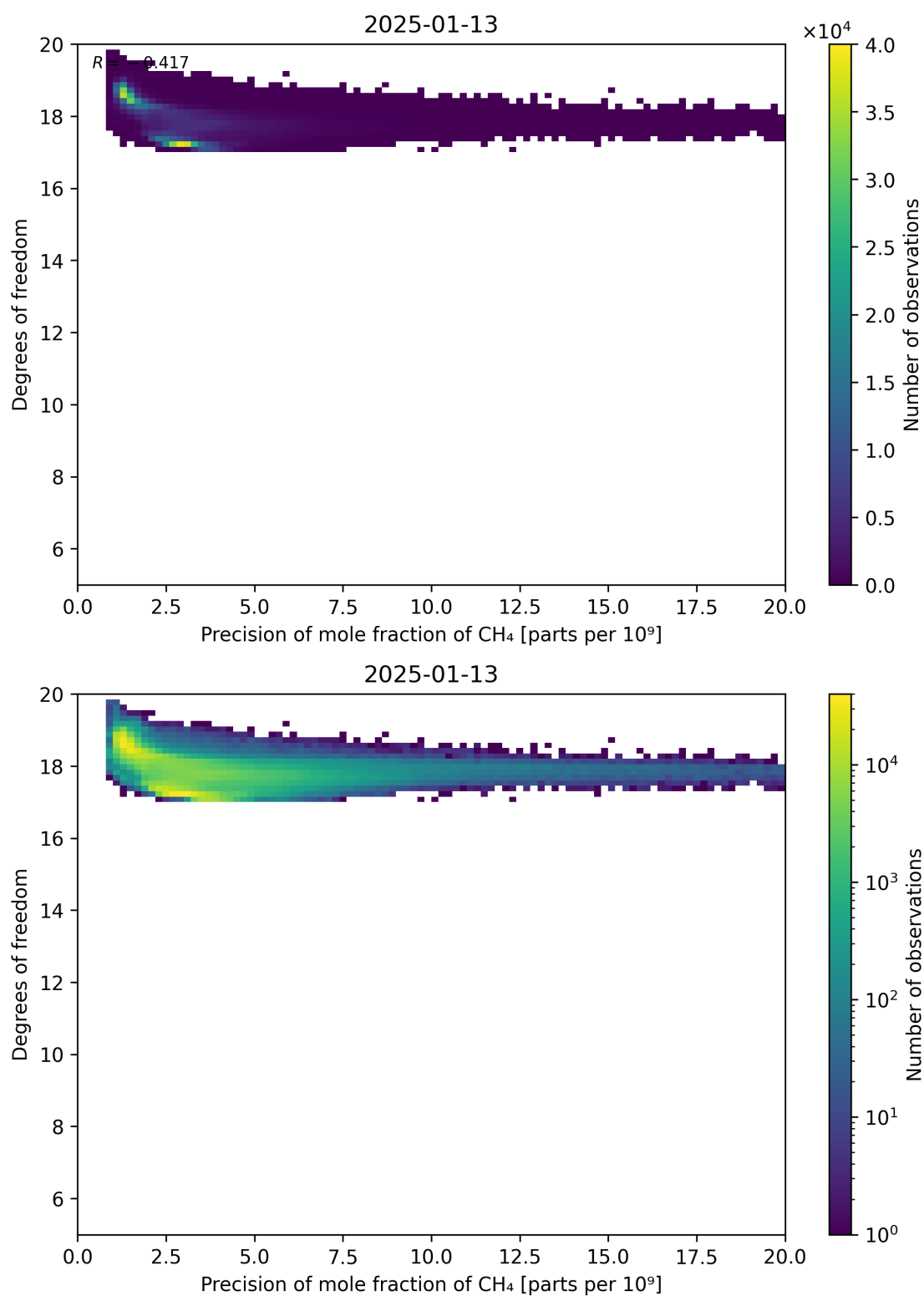
Figure 80: Scatter density plot of “Precision of mole fraction of CH 4 ” against “Degrees of freedom” for 2025-01-12 to 2025-01-14.
