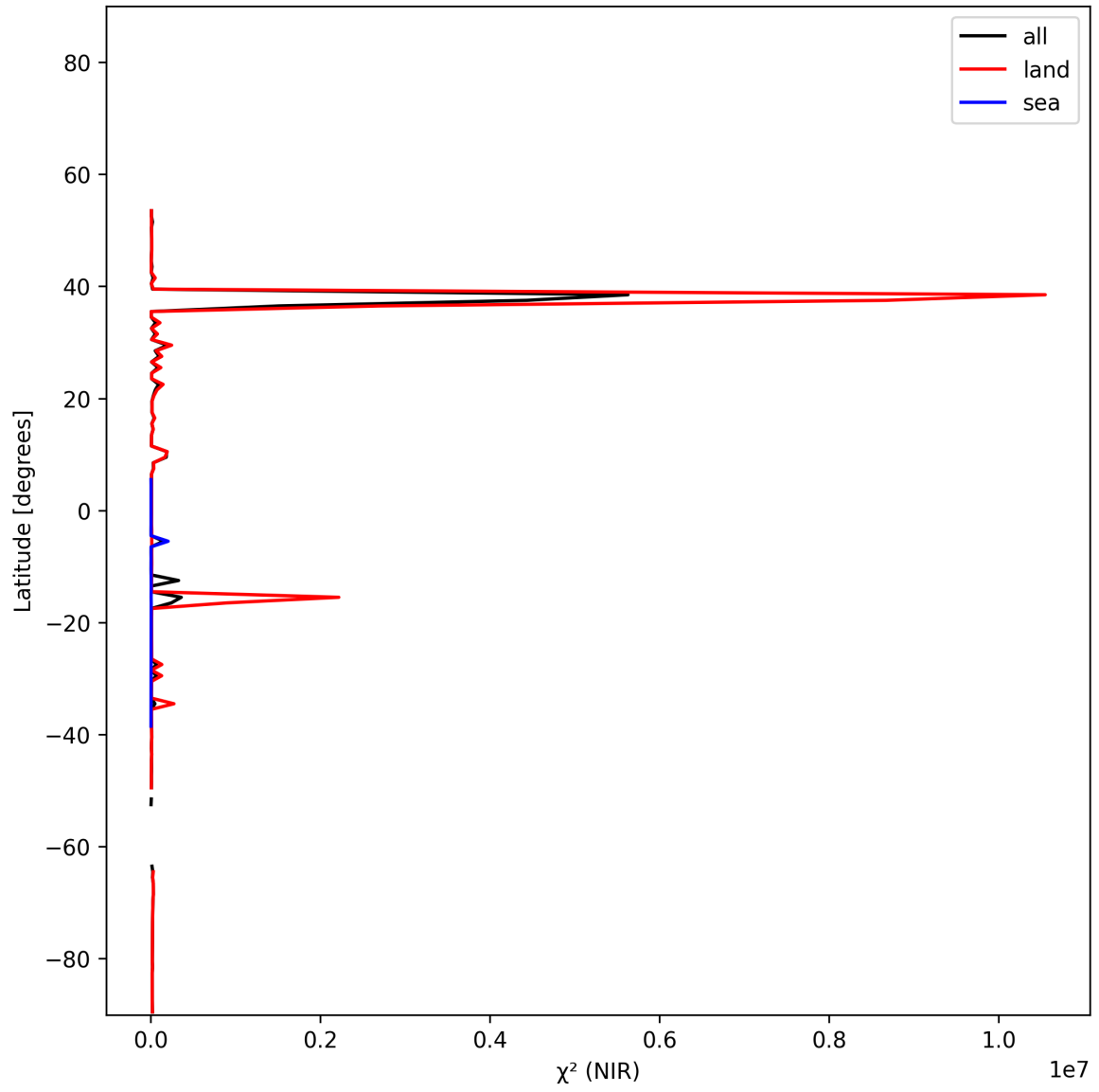
Figure 18: Zonal average of “ \chi^2 (NIR)” for 2025-01-12 to 2025-01-14.
