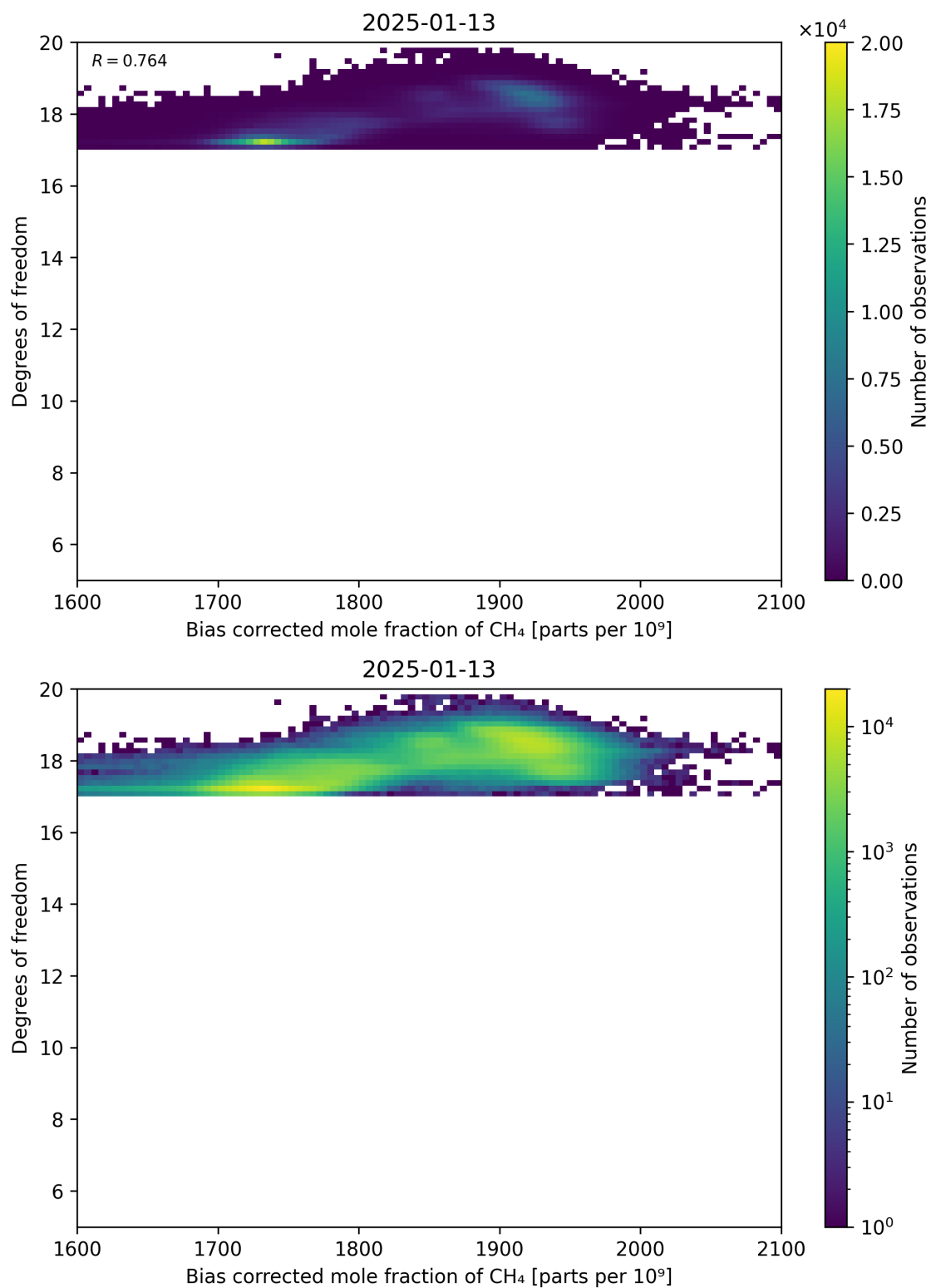
Figure 65: Scatter density plot of “Bias corrected mole fraction of CH 4 ” against “Degrees of freedom” for 2025-01-12 to 2025-01-14.
