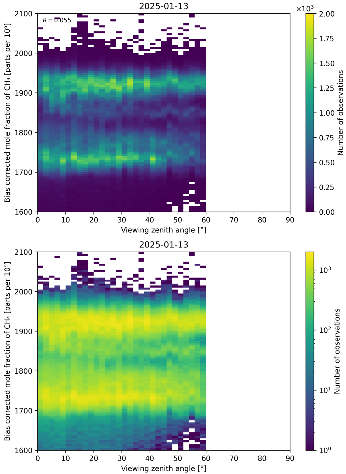
Figure 111: Scatter density plot of “Viewing zenith angle” against “Bias corrected mole fraction of CH 4 ” for 2025-01-12 to 2025-01-14.
