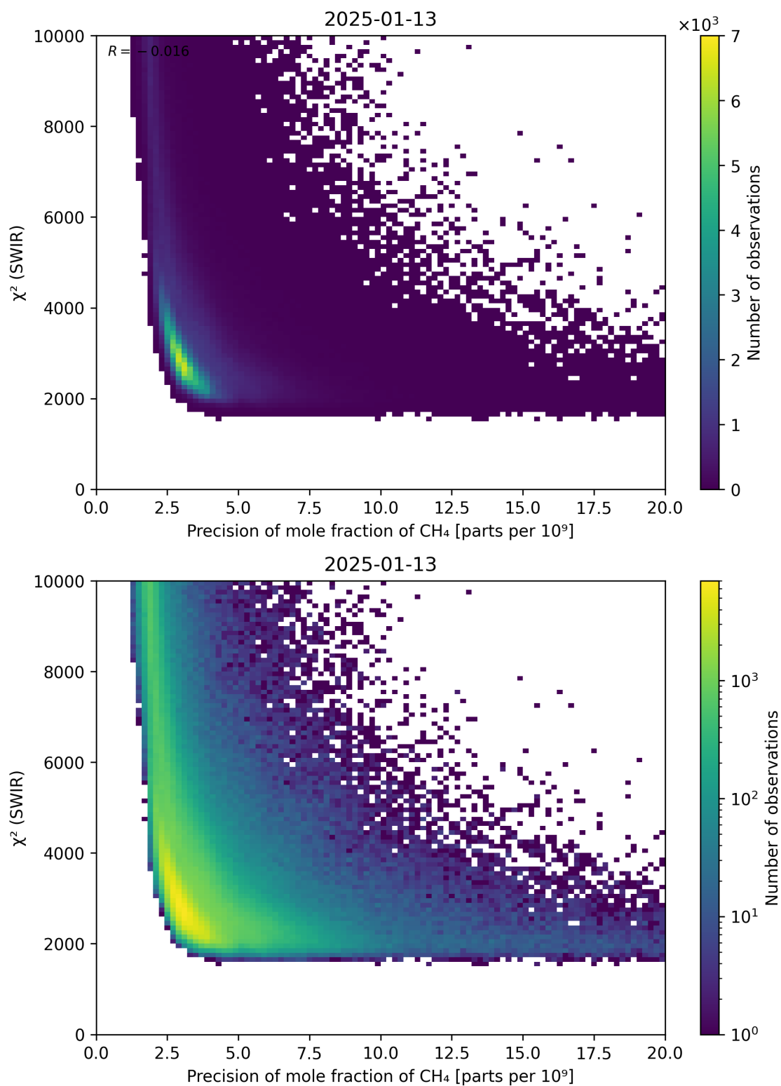
Figure 79: Scatter density plot of “Precision of mole fraction of \text{CH}_4 ” against “ \chi^2 (SWIR)” for 2025-01-12 to 2025-01-14.
