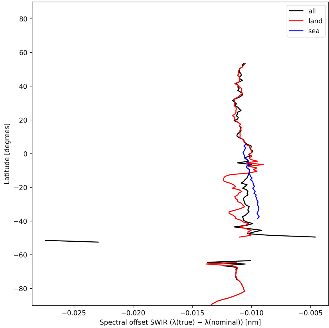
Figure 16: Zonal average of “Spectral offset SWIR ( \lambda_{\text{true}} - \lambda_{\text{nominal}} )” for 2025-01-12 to 2025-01-14.
