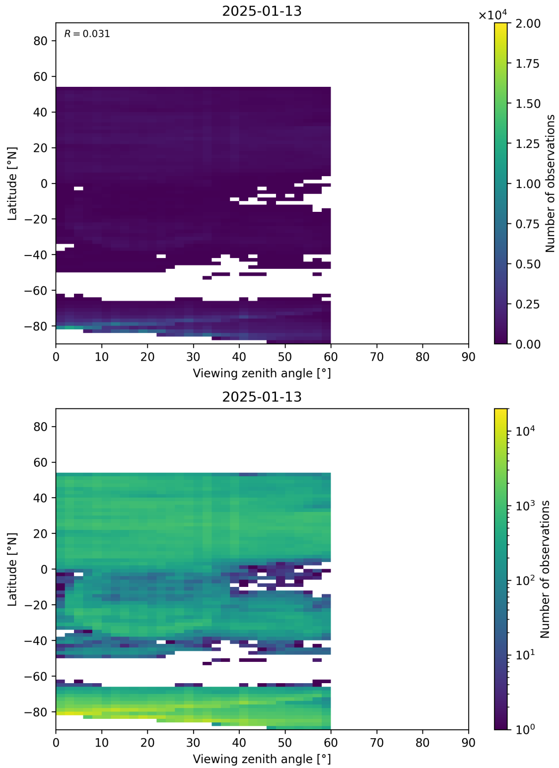
Figure 109: Scatter density plot of “Viewing zenith angle” against “Latitude” for 2025-01-12 to 2025-01-14.
