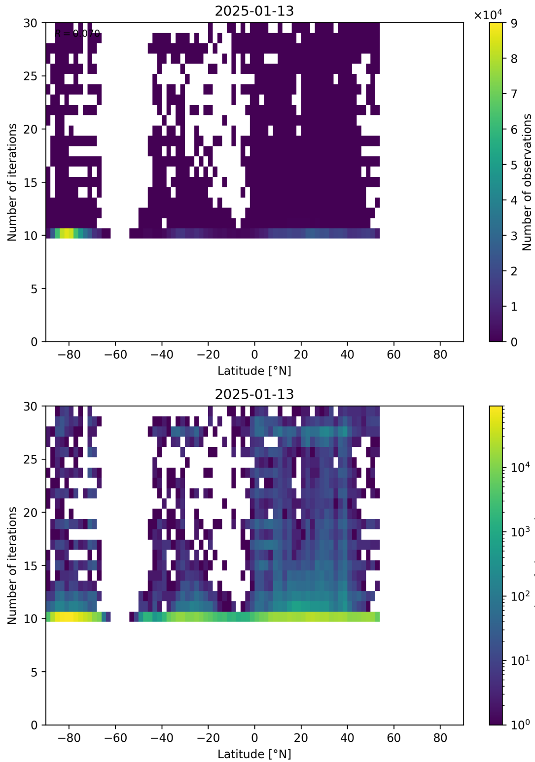
Figure 60: Scatter density plot of “Latitude” against “Number of iterations” for 2025-01-12 to 2025-01-14.
