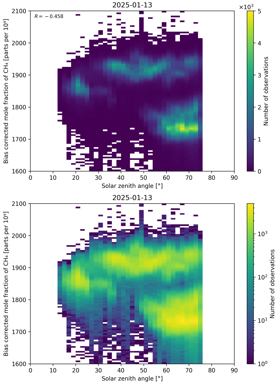
Figure 100: Scatter density plot of “Solar zenith angle” against “Bias corrected mole fraction of CH 4 ” for 2025-01-12 to 2025-01-14.
