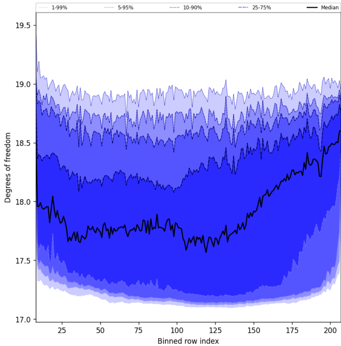
Figure 41: Along track statistics of “Degrees of freedom” for 2025-01-12 to 2025-01-14
