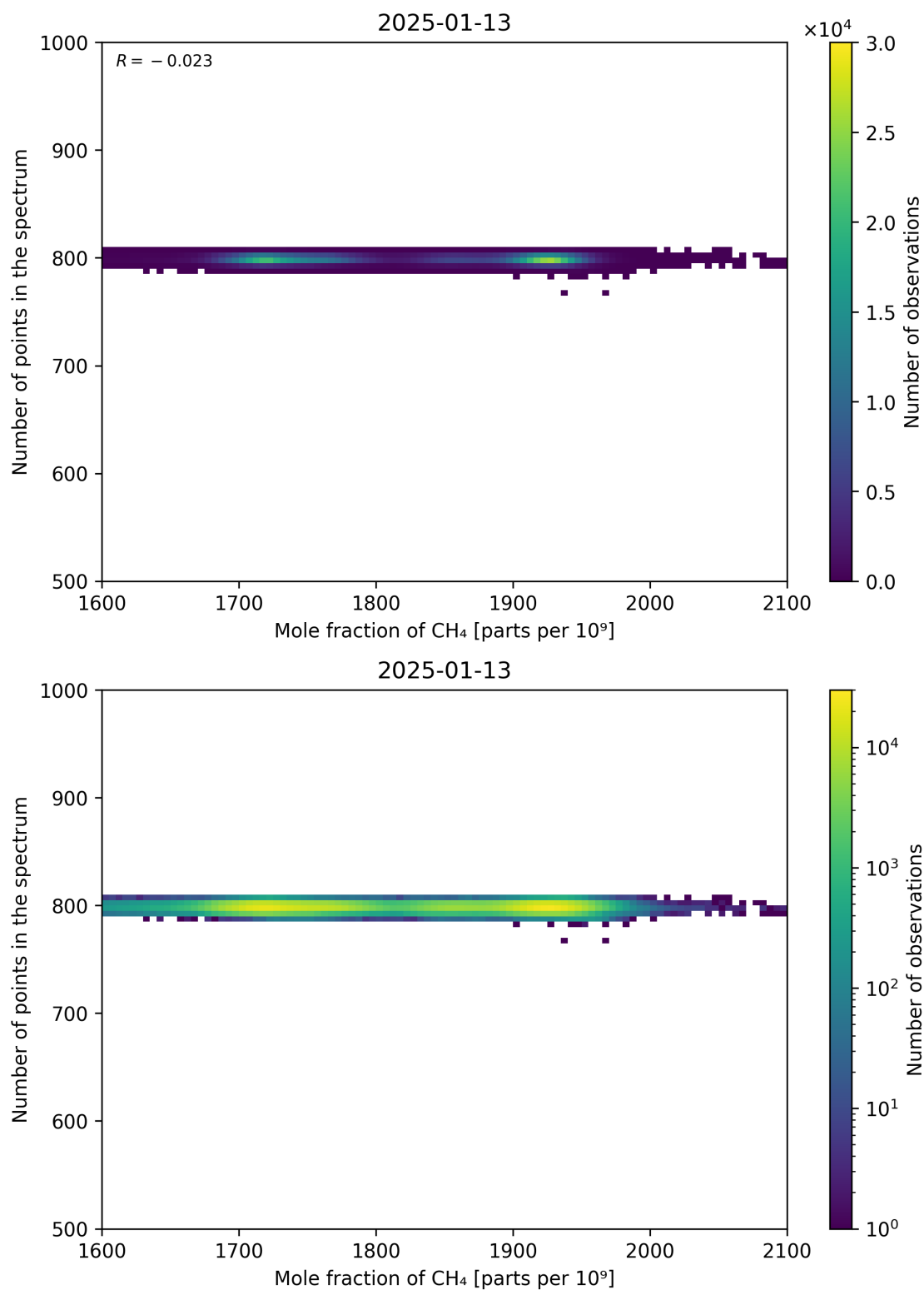
Figure 77: Scatter density plot of “Mole fraction of CH 4 ” against “Number of points in the spectrum” for 2025-01-12 to 2025-01-14.
