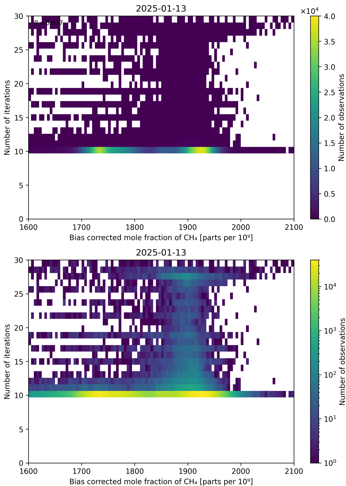
Figure 67: Scatter density plot of “Bias corrected mole fraction of \text{CH}_4 ” against “Number of iterations” for 2025-01-12 to 2025-01-14.
