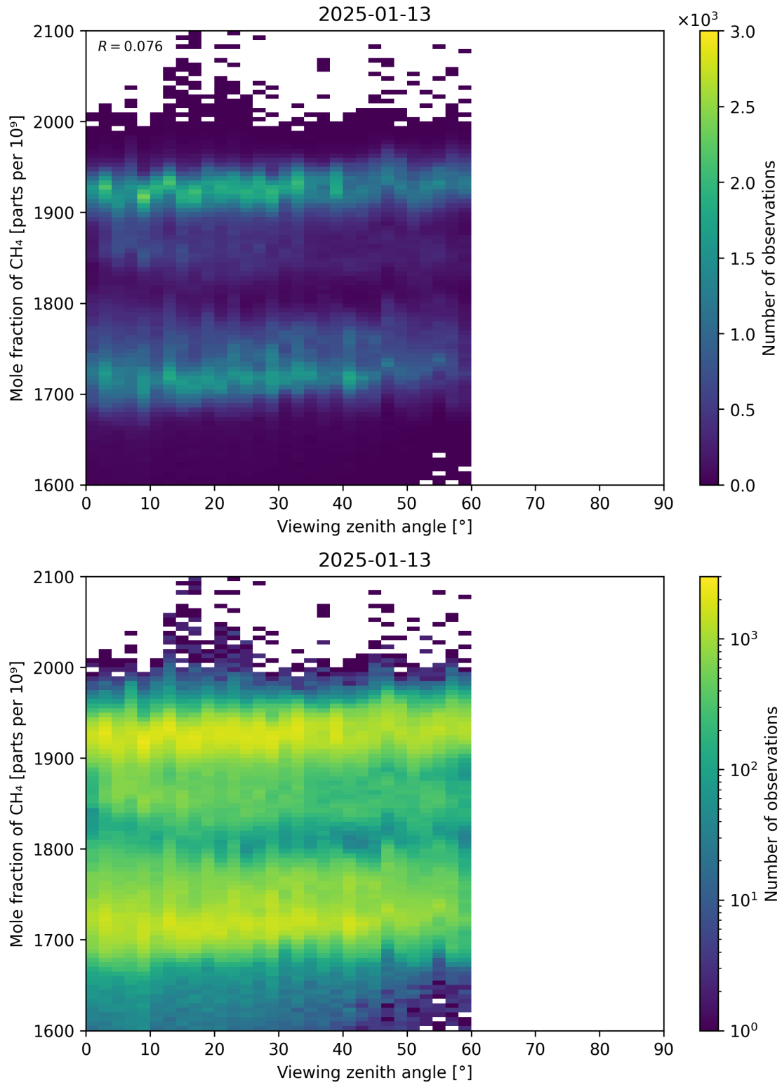
Figure 110: Scatter density plot of “Viewing zenith angle” against “Mole fraction of CH 4 ” for 2025-01-12 to 2025-01-14.
