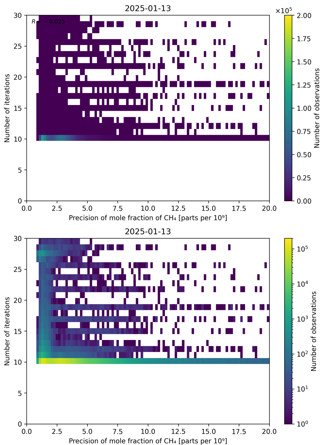
Figure 83: Scatter density plot of “Precision of mole fraction of CH 4 ” against “Number of iterations” for 2025-01-12 to 2025-01-14.
