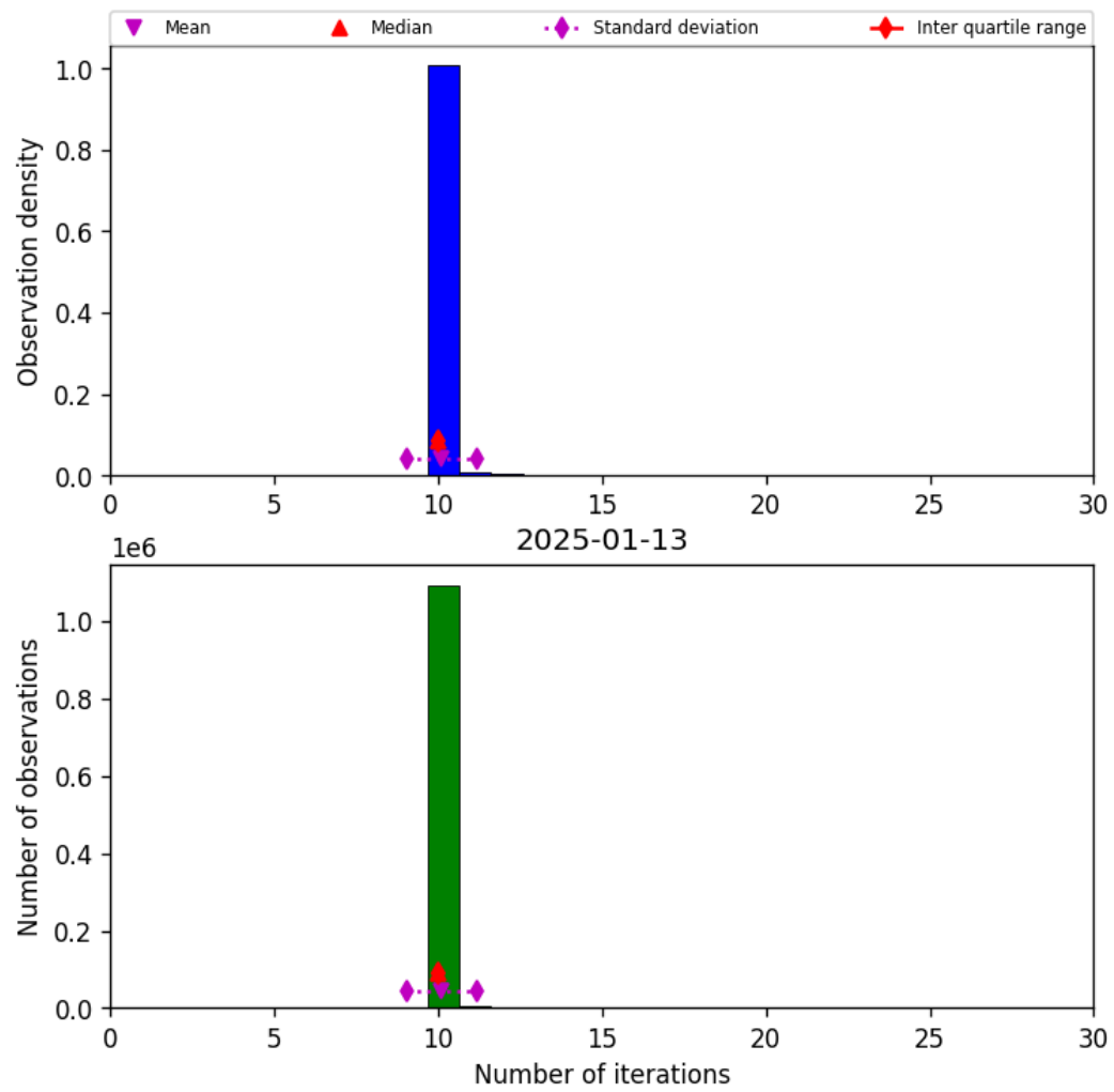
Figure 31: Histogram of “Number of iterations” for 2025-01-12 to 2025-01-14
