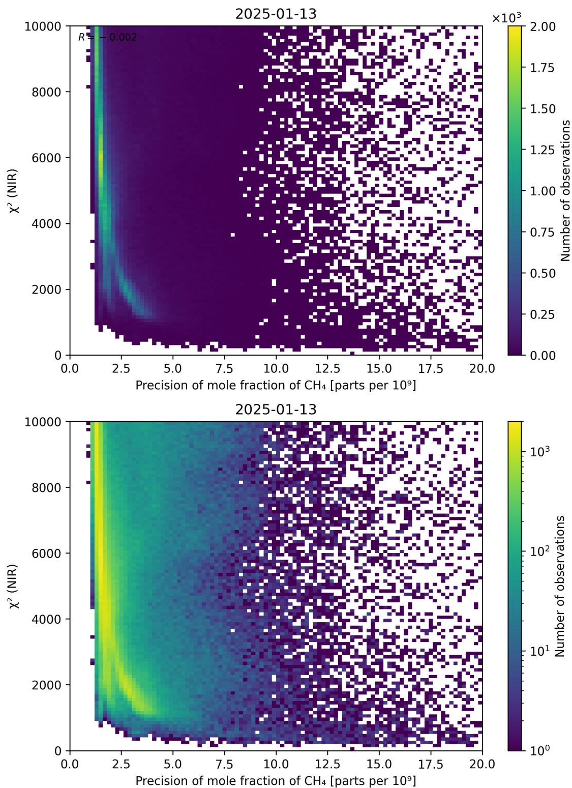
Figure 78: Scatter density plot of “Precision of mole fraction of CH 4 ” against “ \chi^2 (NIR)” for 2025-01-12 to 2025-01-14.
