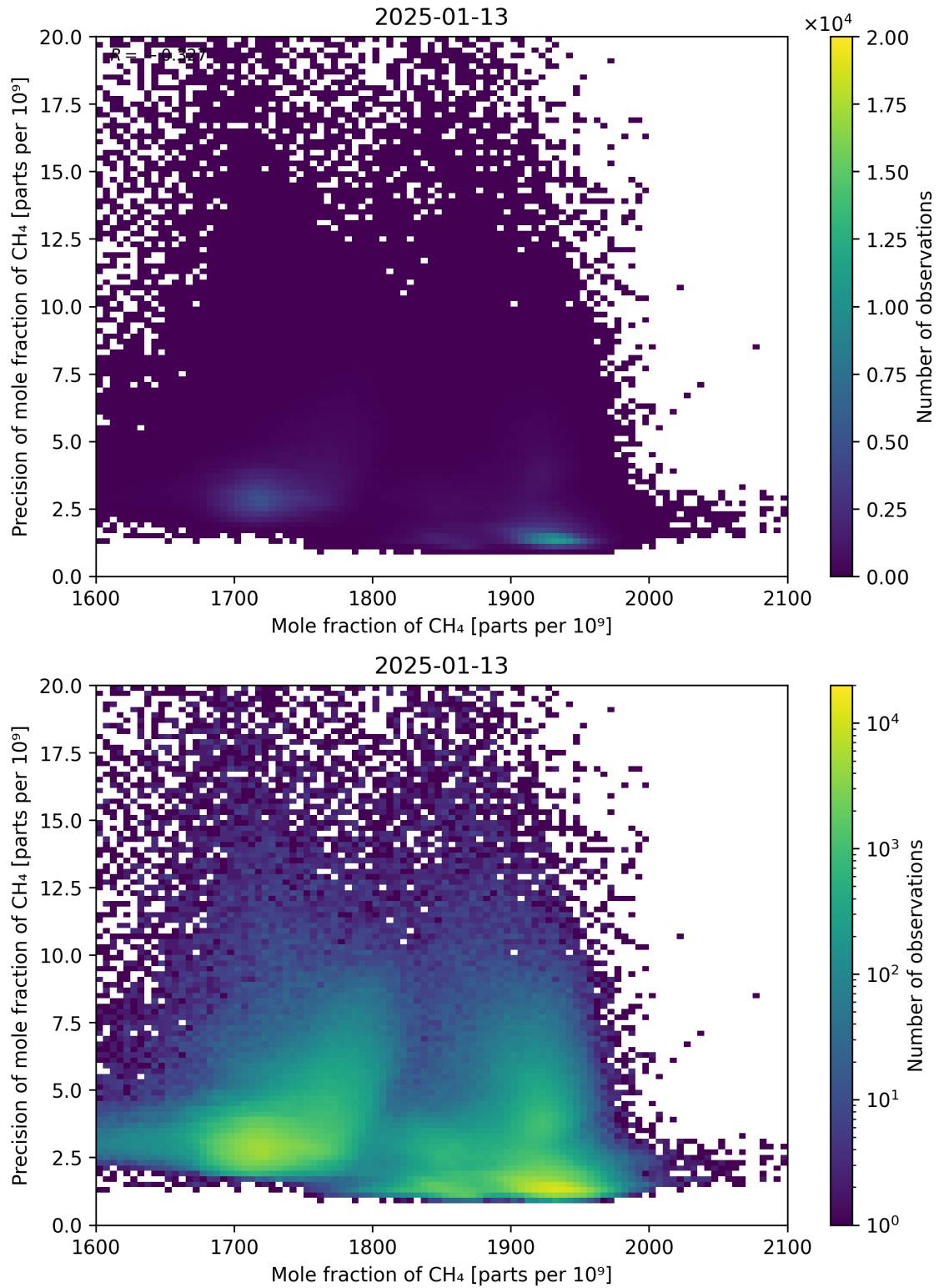
Figure 75: Scatter density plot of “Mole fraction of CH 4 ” against “Precision of mole fraction of CH 4 ” for 2025-01-12 to 2025-01-14.
