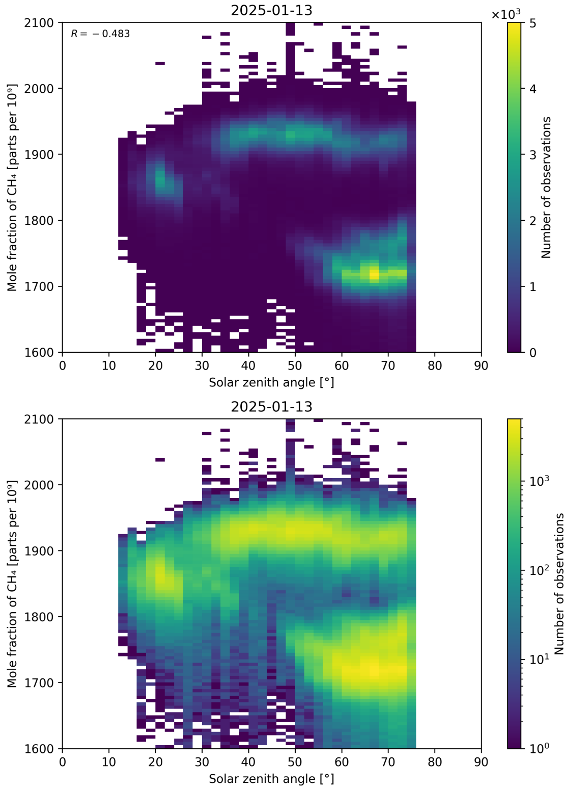
Figure 99: Scatter density plot of “Solar zenith angle” against “Mole fraction of CH 4 ” for 2025-01-12 to 2025-01-14.
