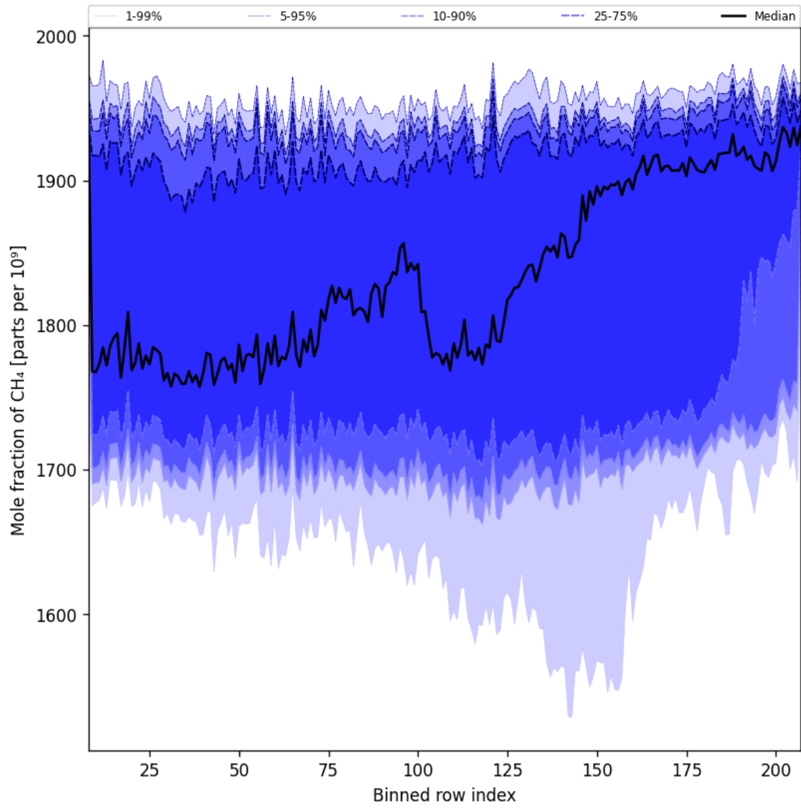
Figure 34: Along track statistics of “Mole fraction of CH 4 ” for 2025-01-12 to 2025-01-14
