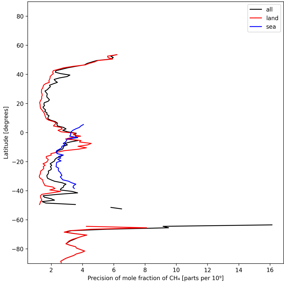
Figure 13: Zonal average of “Precision of mole fraction of CH 4 ” for 2025-01-12 to 2025-01-14.
