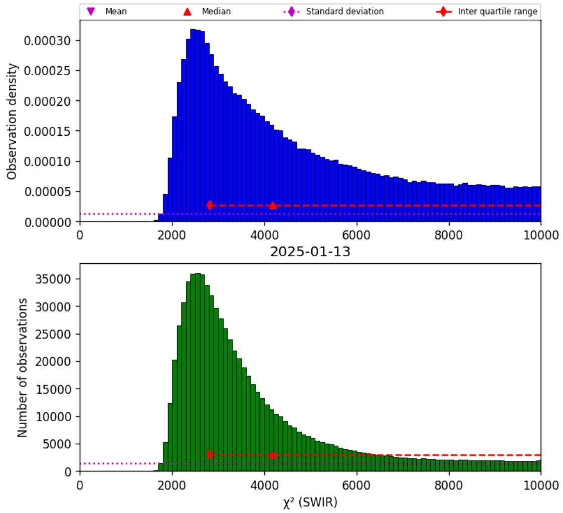
Figure 28: Histogram of “ \chi^2 (SWIR)” for 2025-01-12 to 2025-01-14
