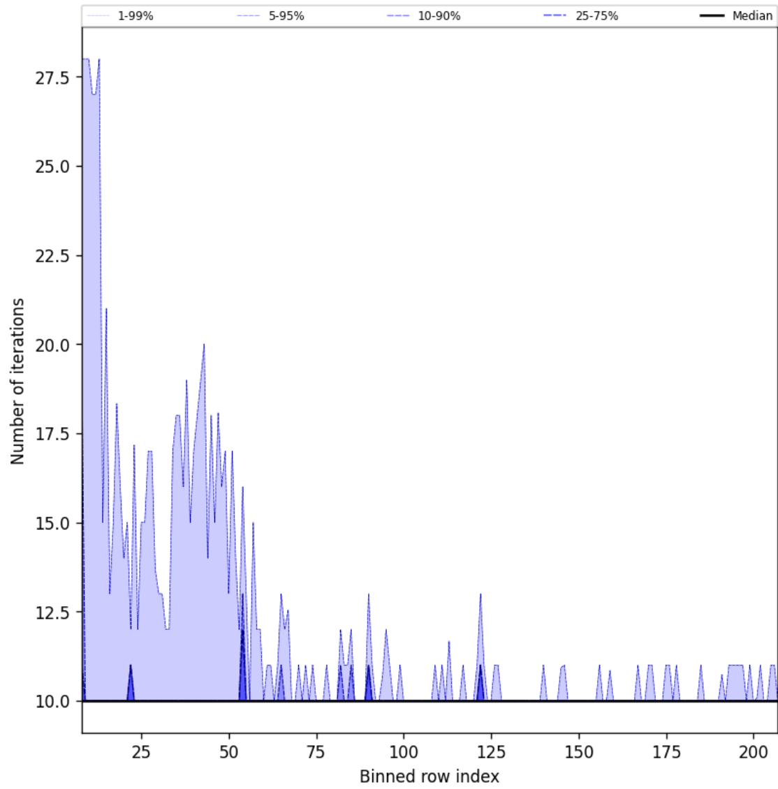
Figure 42: Along track statistics of “Number of iterations” for 2025-01-12 to 2025-01-14
