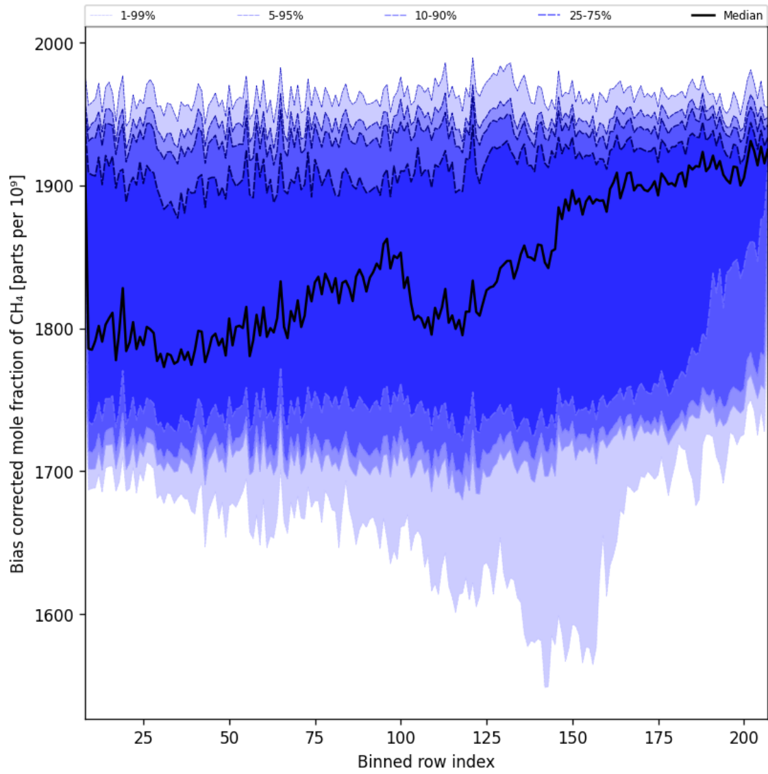
Figure 36: Along track statistics of “Bias corrected mole fraction of CH 4 ” for 2025-01-12 to 2025-01-14
