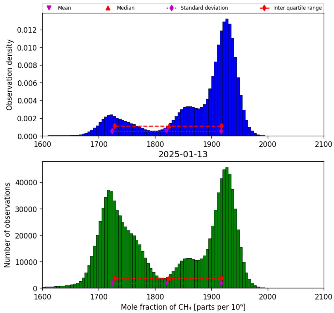
Figure 23: Histogram of “Mole fraction of CH 4 ” for 2025-01-12 to 2025-01-14
