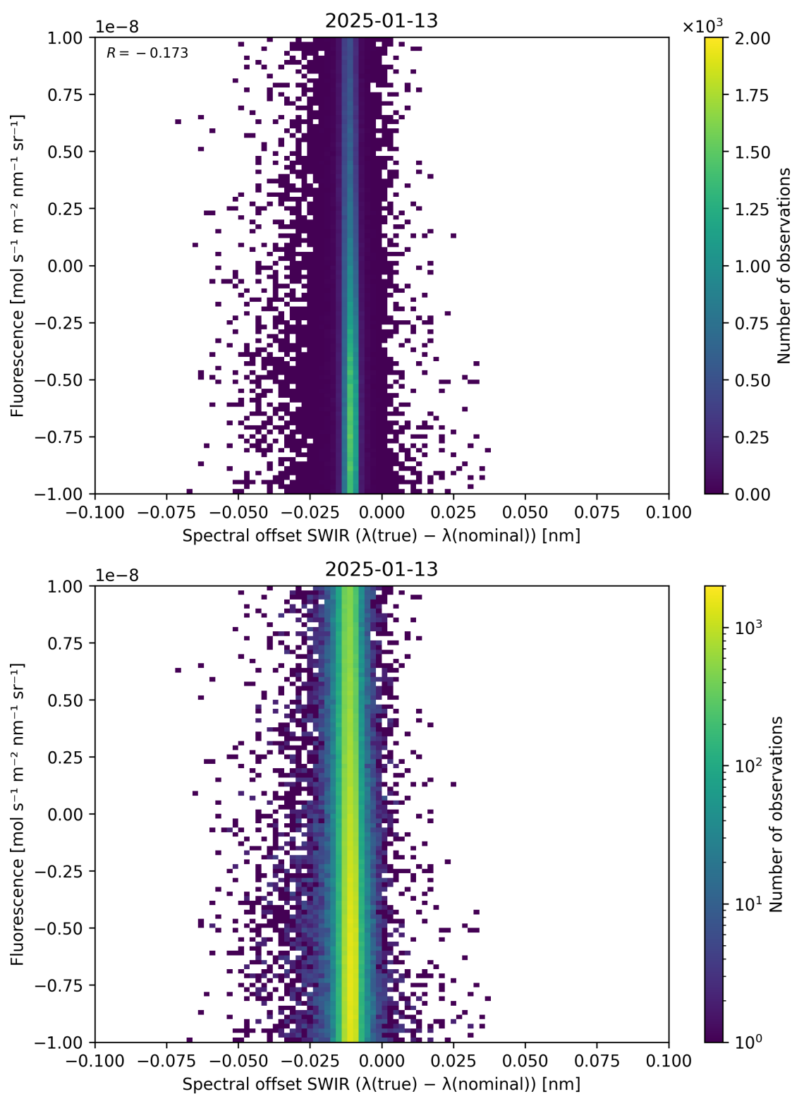
Figure 120: Scatter density plot of “Spectral offset SWIR ( \lambda_{\text{true}} - \lambda_{\text{nominal}} )” against “Fluorescence” for 2025-01-12 to 2025-01-14.
