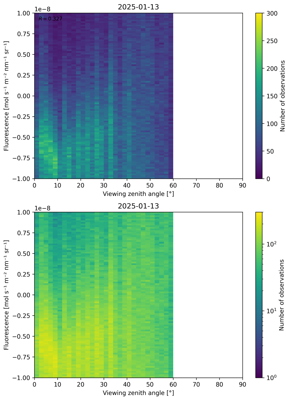
Figure 108: Scatter density plot of “Viewing zenith angle” against “Fluorescence” for 2025-01-12 to 2025-01-14.
