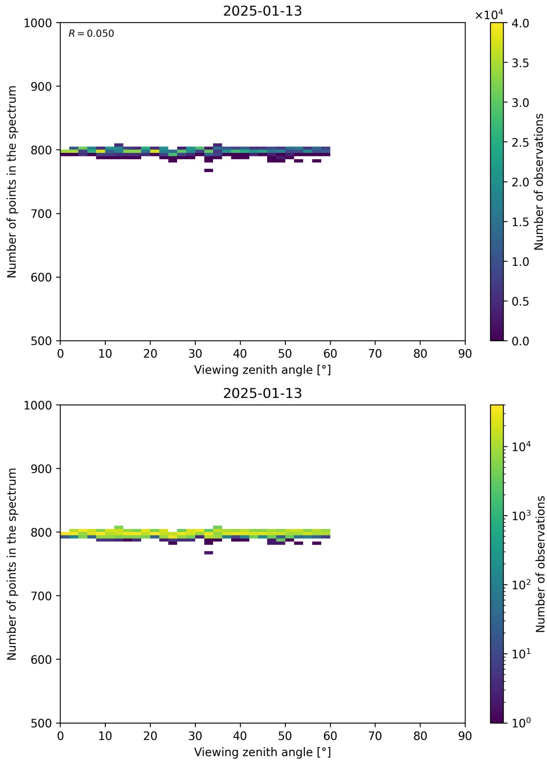
Figure 114: Scatter density plot of “Viewing zenith angle” against “Number of points in the spectrum” for 2025-01-12 to 2025-01-14.
