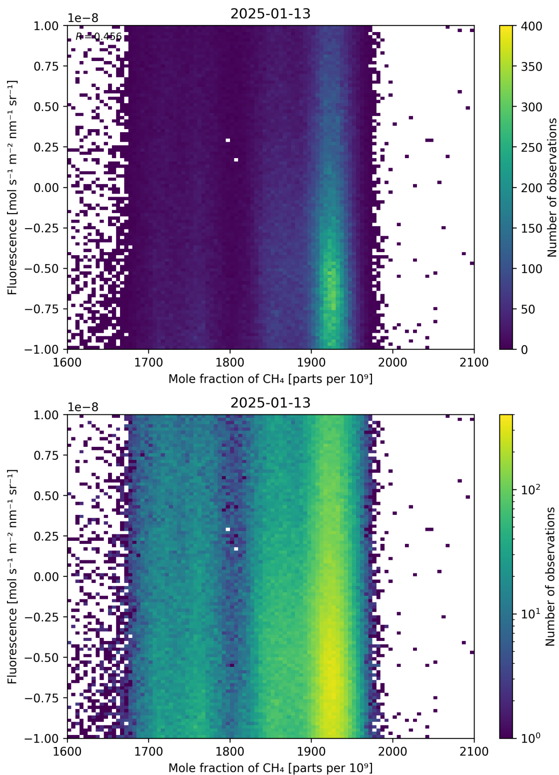
Figure 73: Scatter density plot of “Mole fraction of \text{CH}_4 ” against “Fluorescence” for 2025-01-12 to 2025-01-14.
