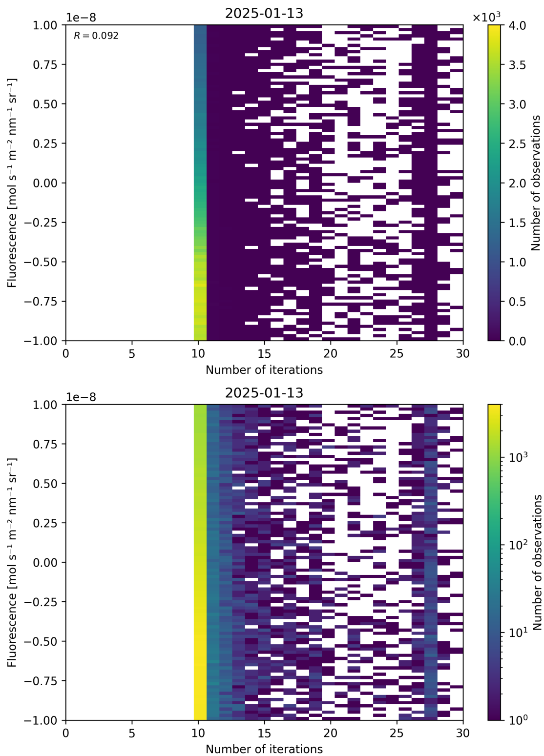
Figure 87: Scatter density plot of “Number of iterations” against “Fluorescence” for 2025-01-12 to 2025-01-14.
