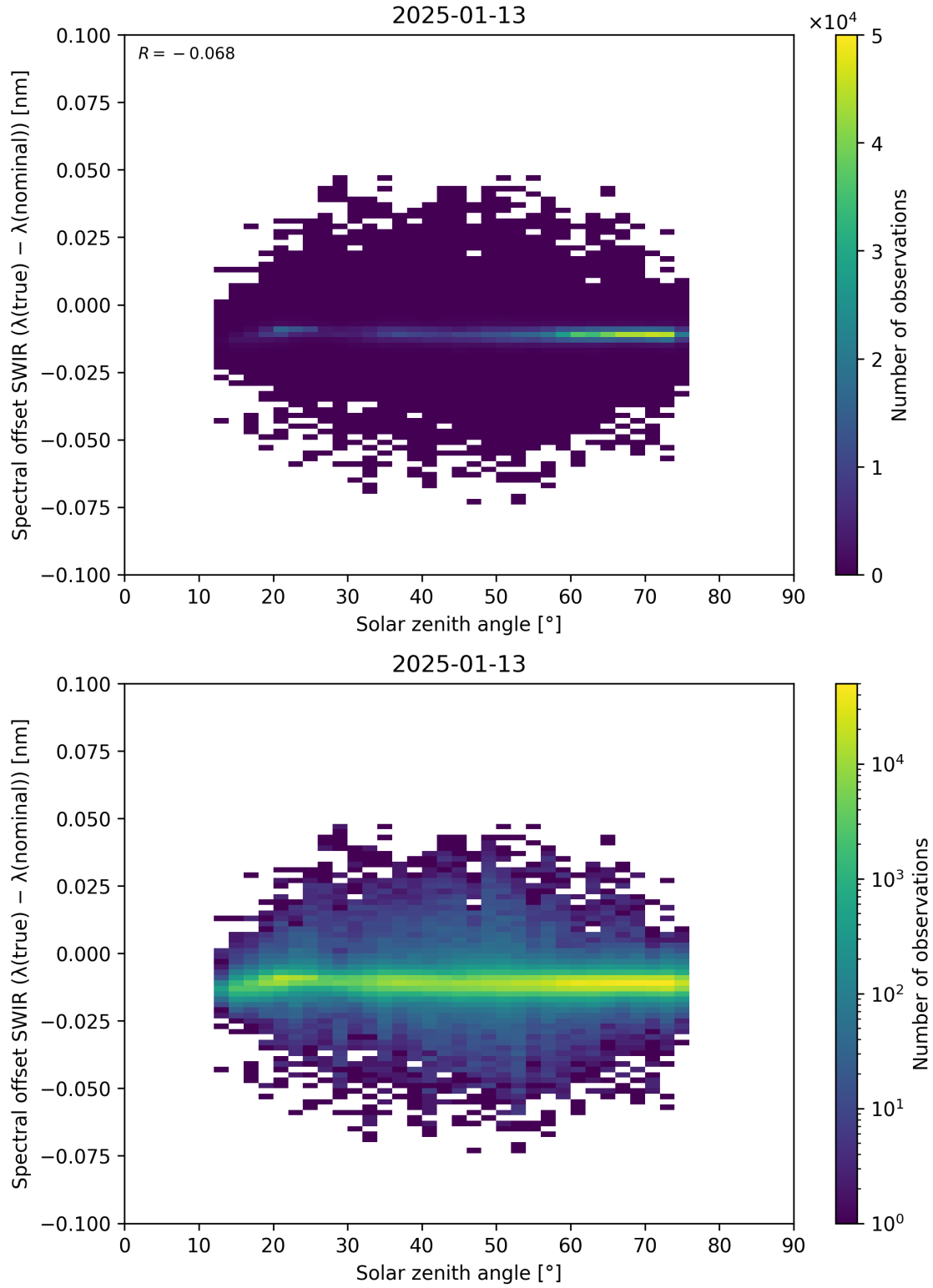
Figure 104: Scatter density plot of “Solar zenith angle” against “Spectral offset SWIR ( \lambda_{\text{true}} - \lambda_{\text{nominal}} )” for 2025-01-12 to 2025-01-14.
