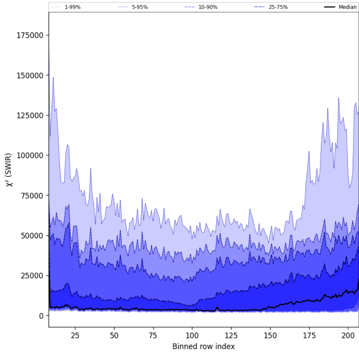
Figure 39: Along track statistics of “ \chi^2 (SWIR)” for 2025-01-12 to 2025-01-14
