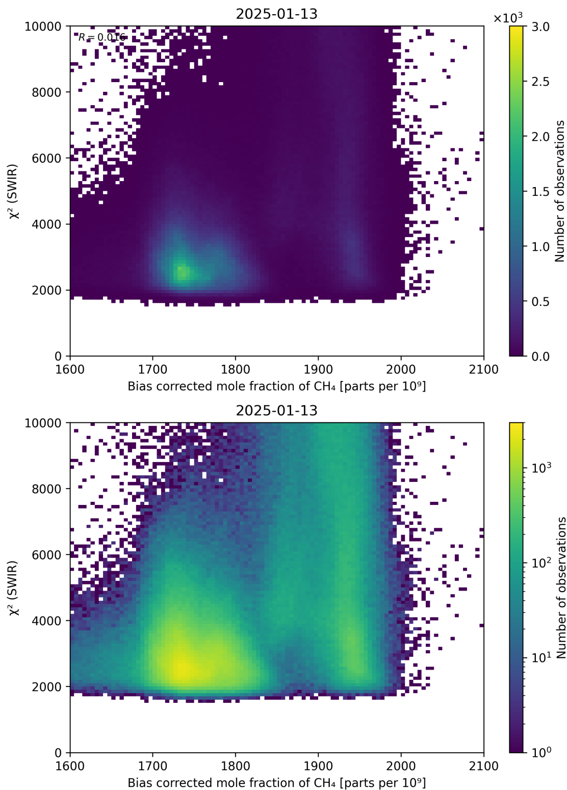
Figure 64: Scatter density plot of “Bias corrected mole fraction of \text{CH}_4 ” against “ \chi^2 (SWIR)” for 2025-01-12 to 2025-01-14.
