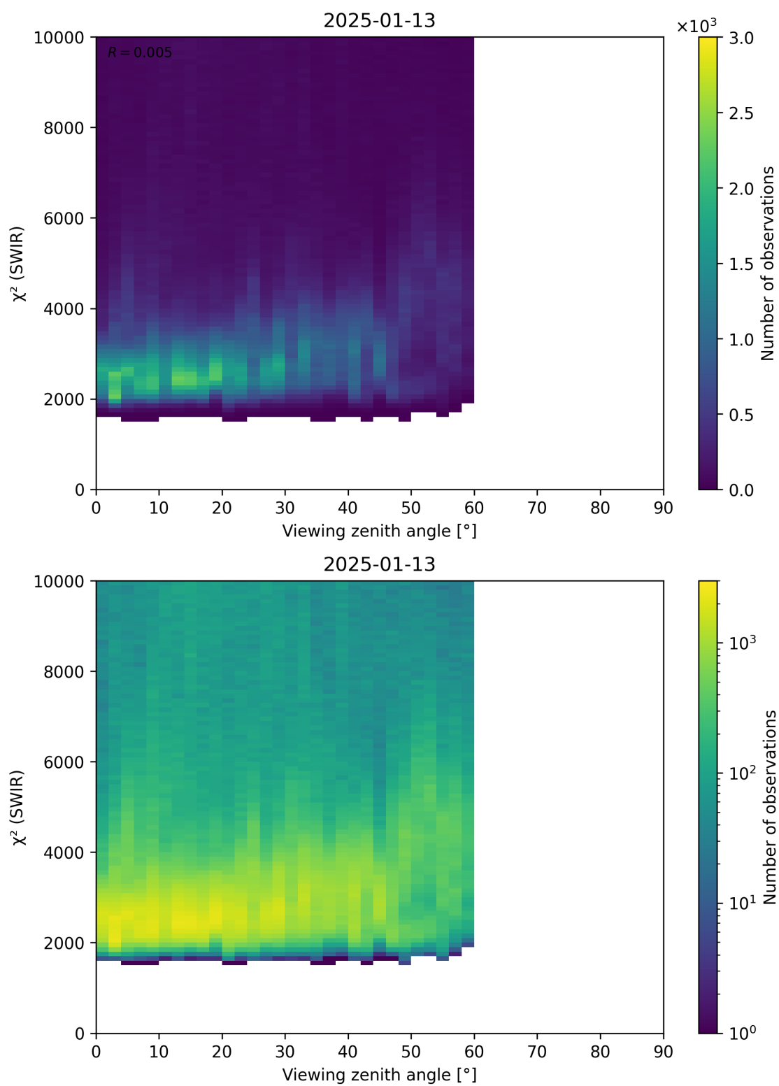
Figure 106: Scatter density plot of “Viewing zenith angle” against “ \chi^2 (SWIR)” for 2025-01-12 to 2025-01-14.
