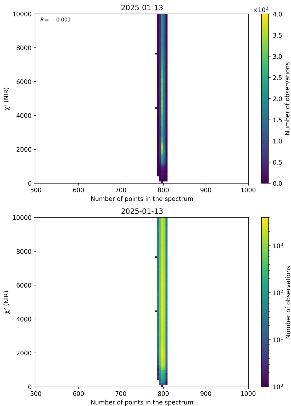
Figure 88: Scatter density plot of “Number of points in the spectrum” against “ \chi^2 (NIR)” for 2025-01-12 to 2025-01-14.
