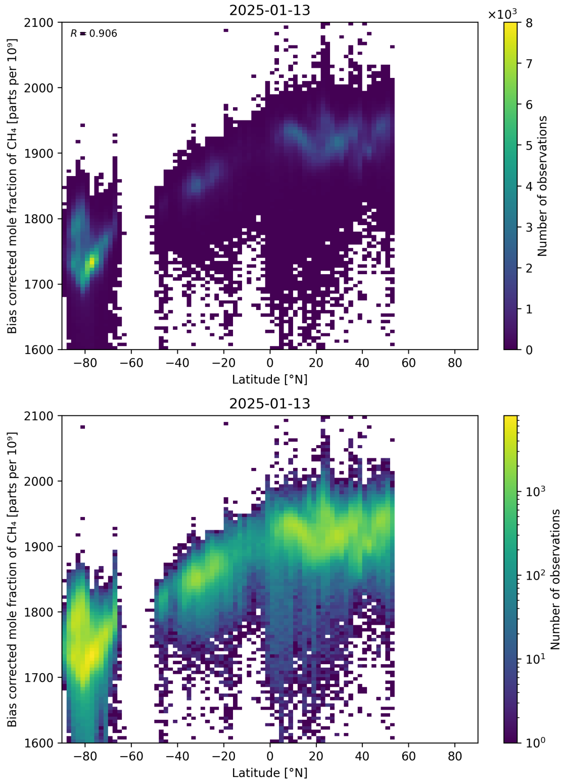
Figure 58: Scatter density plot of “Latitude” against “Bias corrected mole fraction of \text{CH}_4 ” for 2025-01-12 to 2025-01-14.
