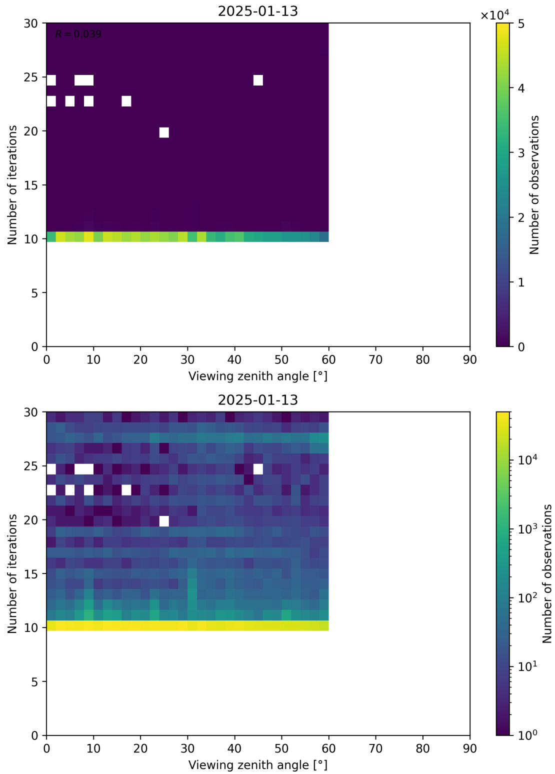
Figure 113: Scatter density plot of “Viewing zenith angle” against “Number of iterations” for 2025-01-12 to 2025-01-14.
