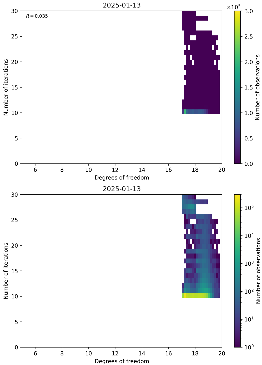
Figure 52: Scatter density plot of “Degrees of freedom” against “Number of iterations” for 2025-01-12 to 2025-01-14.
