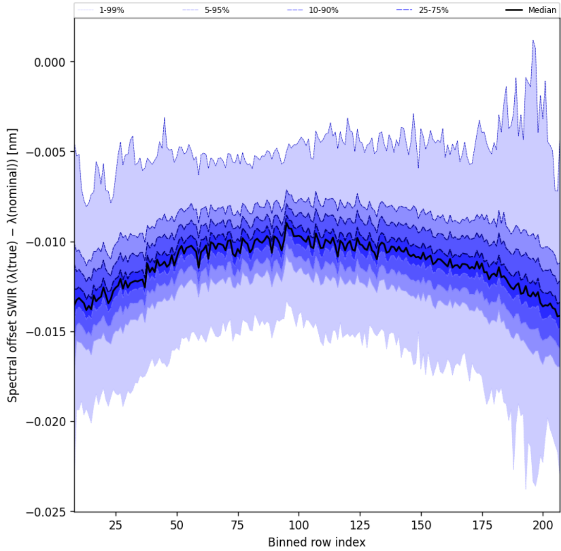
Figure 38: Along track statistics of “Spectral offset SWIR ( \lambda_{\text{true}} - \lambda_{\text{nominal}} )” for 2025-01-12 to 2025-01-14
