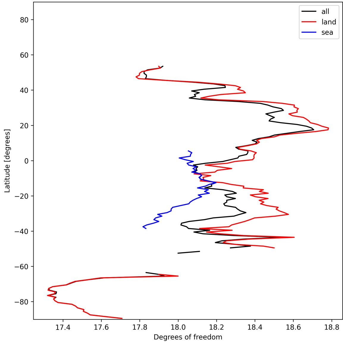
Figure 19: Zonal average of “Degrees of freedom” for 2025-01-12 to 2025-01-14.
