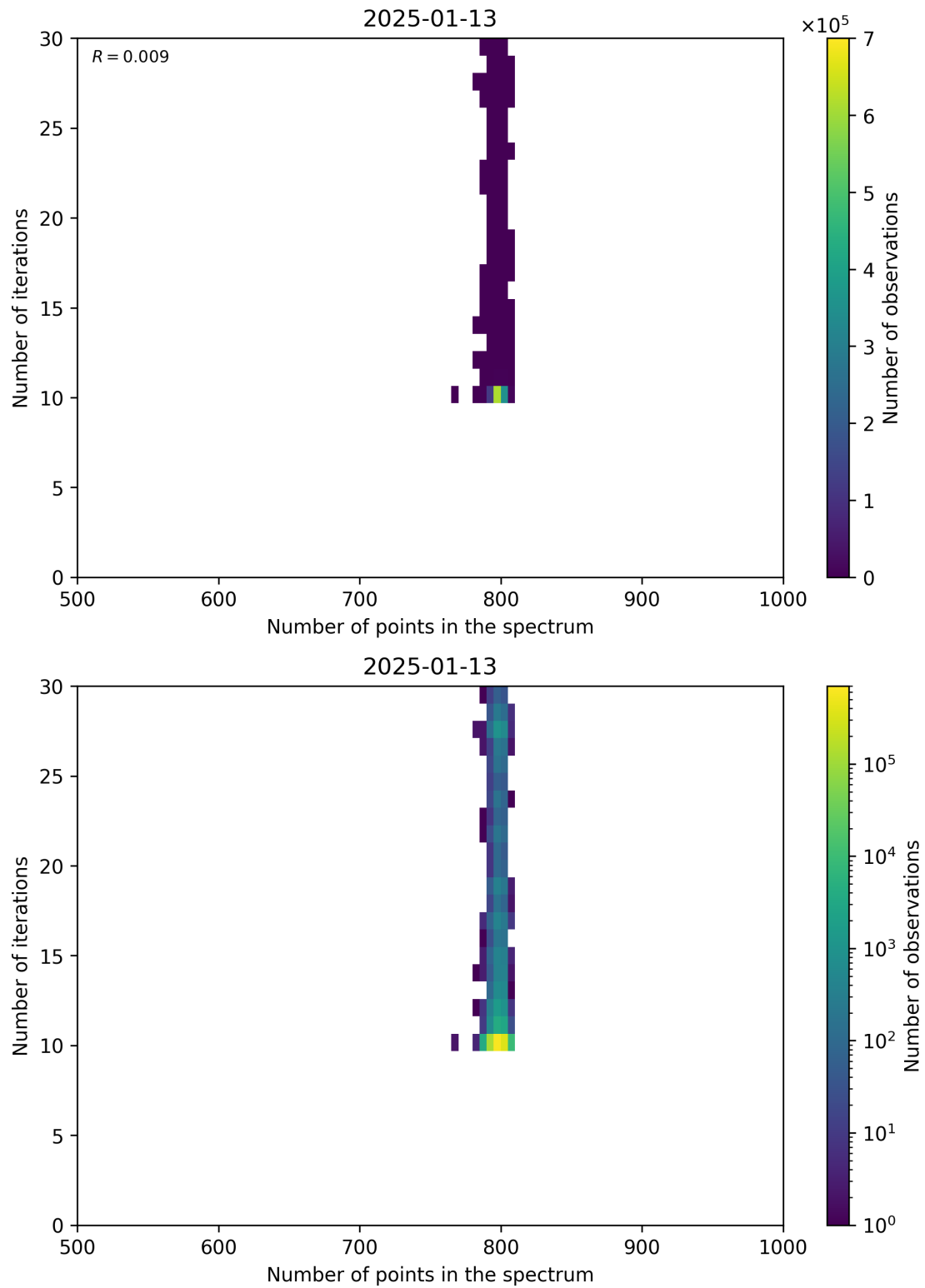
Figure 92: Scatter density plot of “Number of points in the spectrum” against “Number of iterations” for 2025-01-12 to 2025-01-14.
