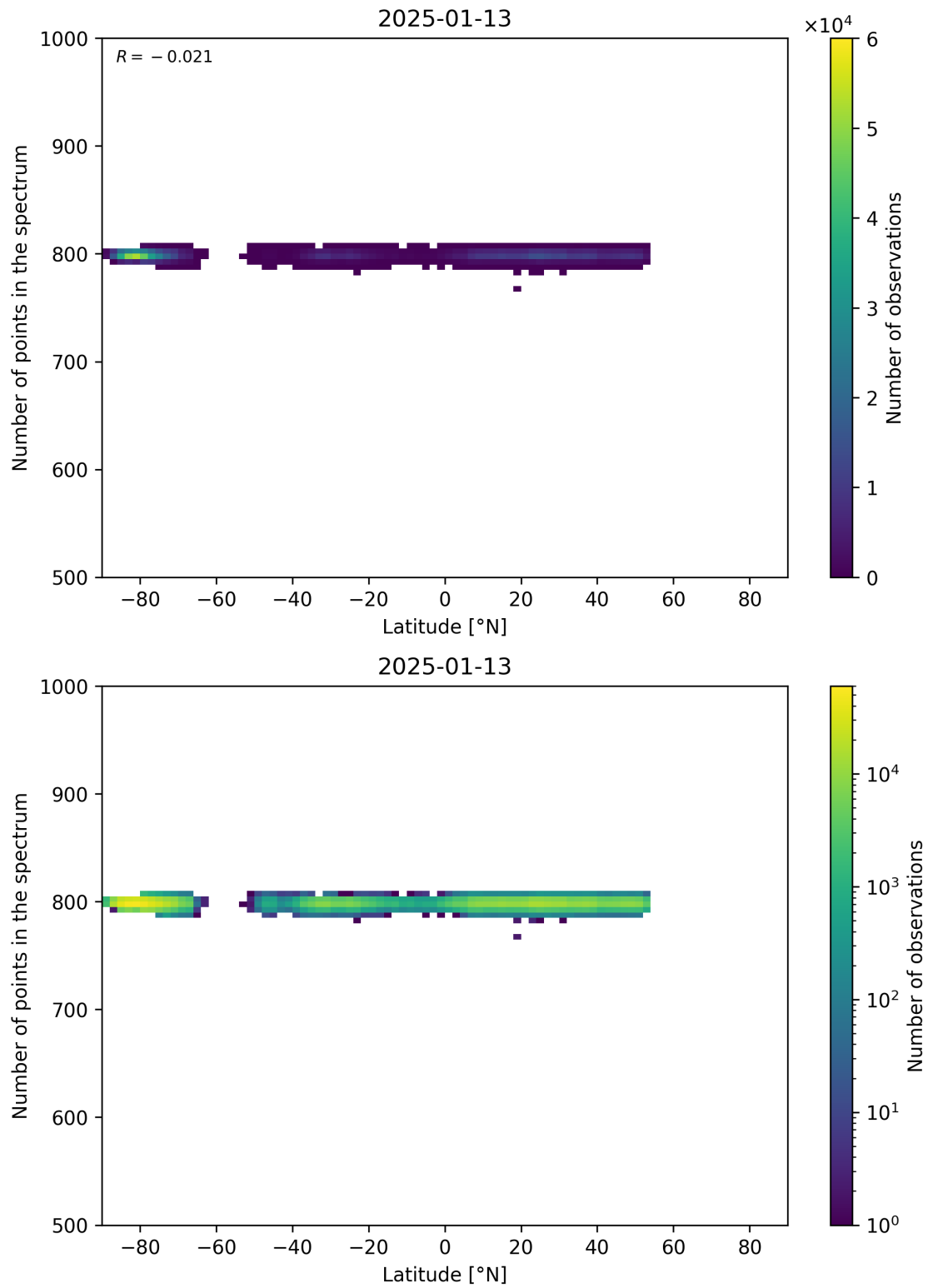
Figure 61: Scatter density plot of “Latitude” against “Number of points in the spectrum” for 2025-01-12 to 2025-01-14.
