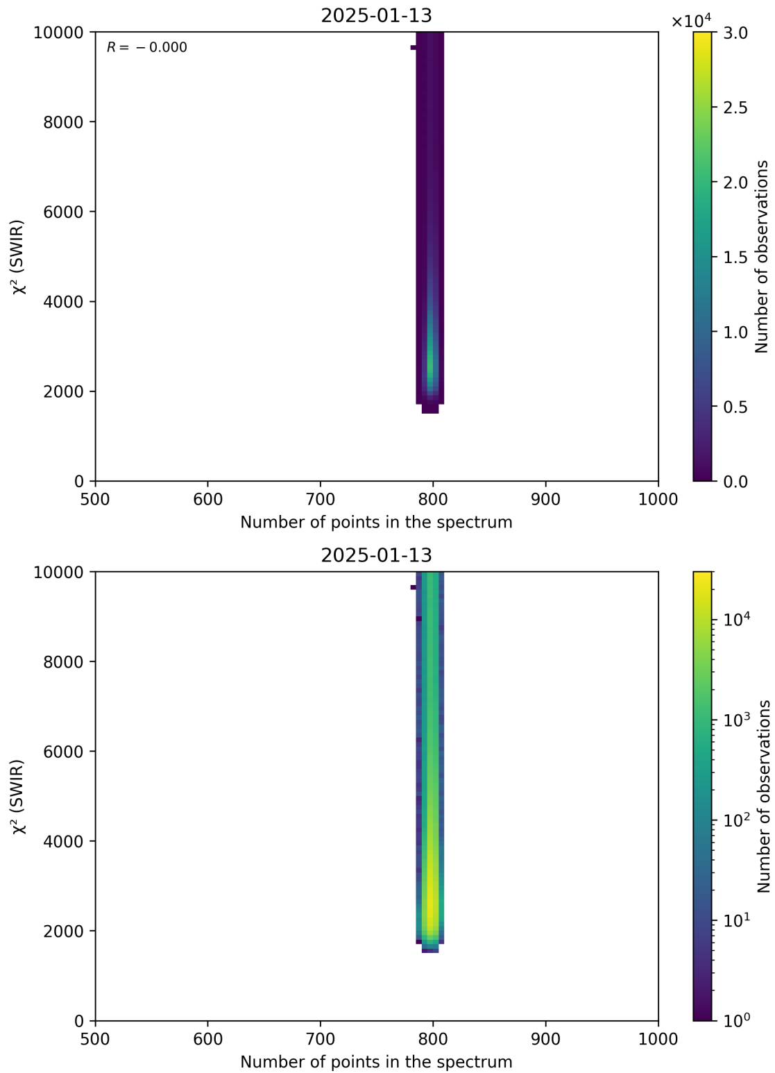
Figure 89: Scatter density plot of “Number of points in the spectrum” against “ \chi^2 (SWIR)” for 2025-01-12 to 2025-01-14.
