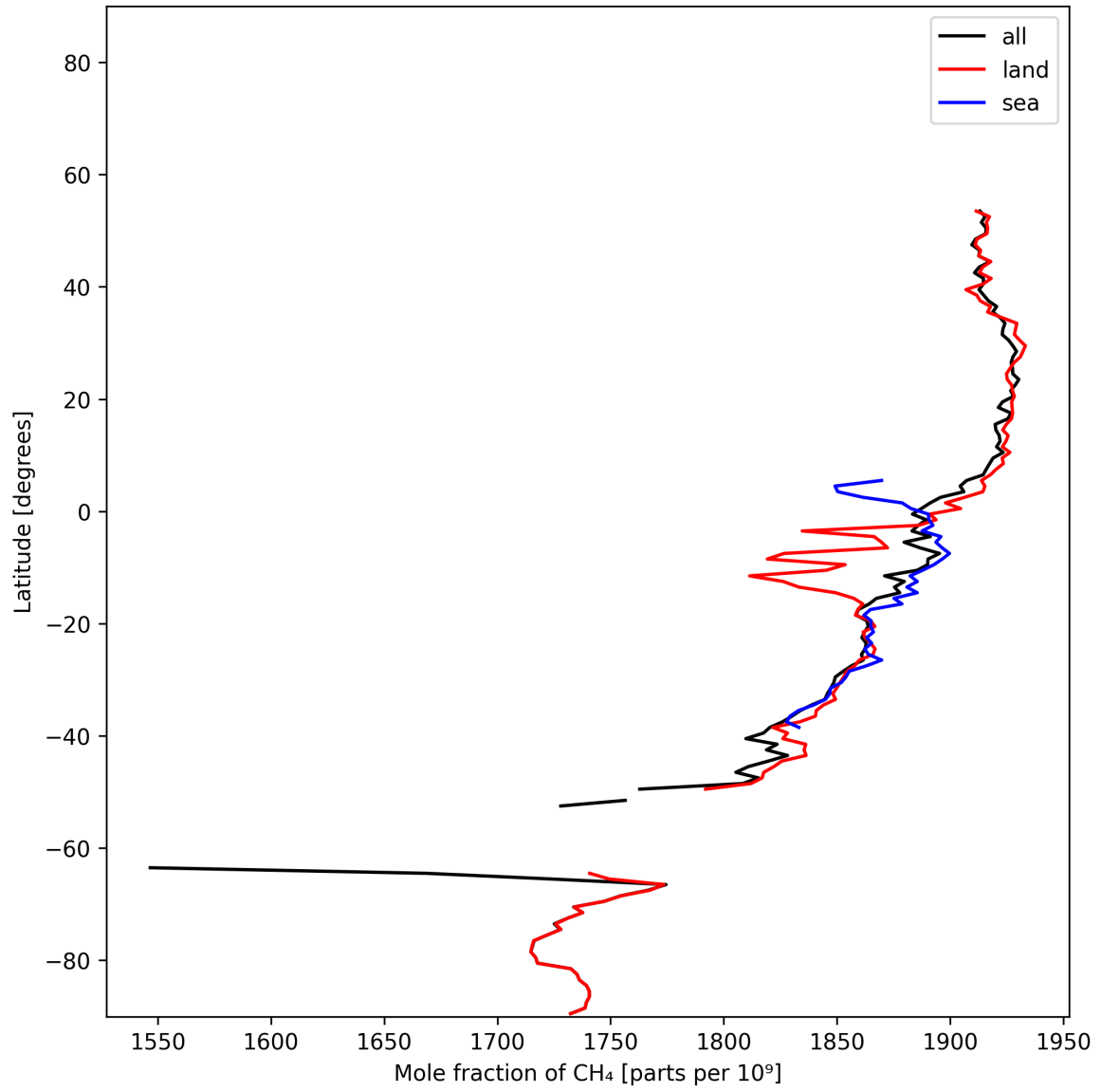
Figure 12: Zonal average of “Mole fraction of CH 4 ” for 2025-01-12 to 2025-01-14.
