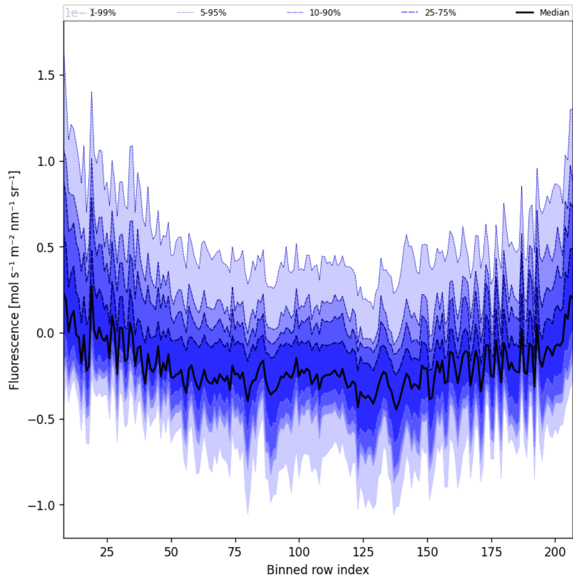
Figure 43: Along track statistics of “Fluorescence” for 2025-01-12 to 2025-01-14
