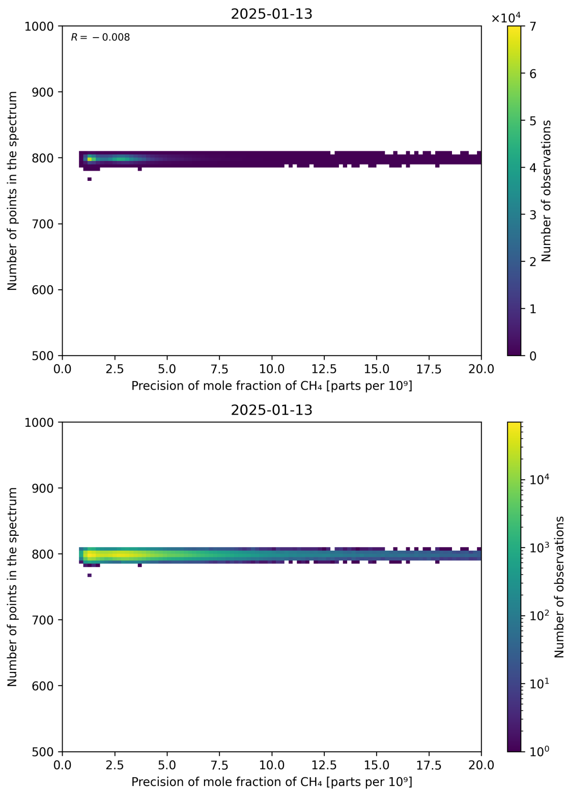
Figure 84: Scatter density plot of “Precision of mole fraction of CH 4 ” against “Number of points in the spectrum” for 2025-01-12 to 2025-01-14.
