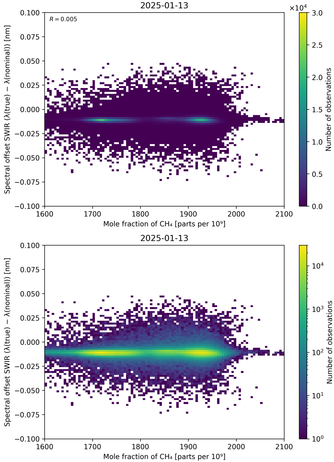
Figure 86: Scatter density plot of “Mole fraction of CH 4 ” against “Spectral offset SWIR ( \lambda_{\text{true}} - \lambda_{\text{nominal}} )” for 2025-01-12 to 2025-01-14.
