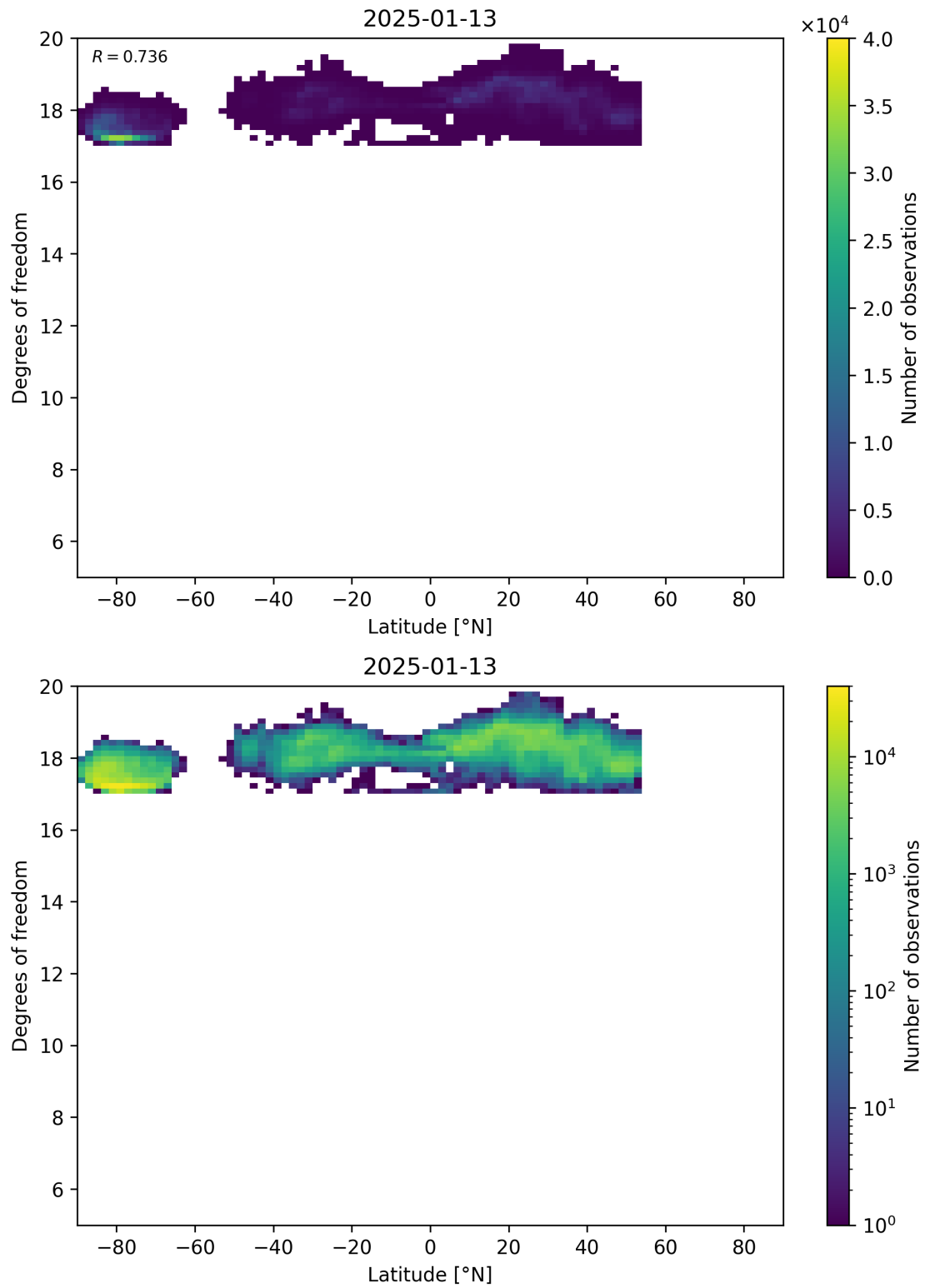
Figure 55: Scatter density plot of “Latitude” against “Degrees of freedom” for 2025-01-12 to 2025-01-14.
