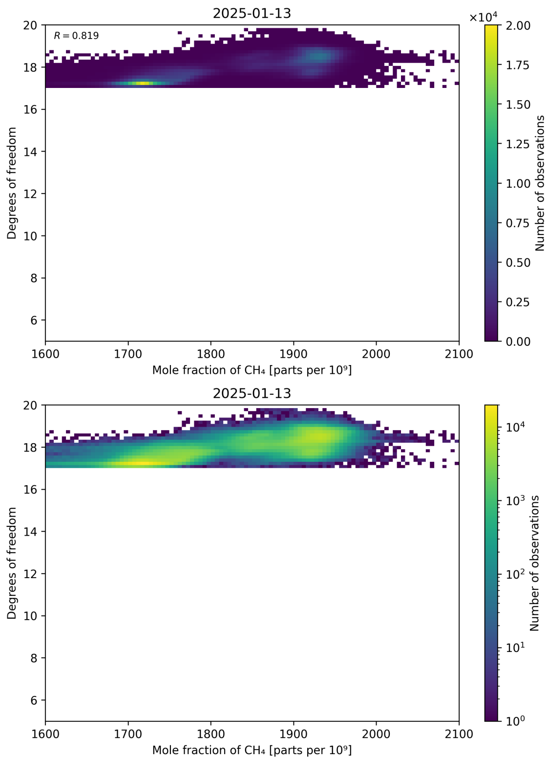
Figure 72: Scatter density plot of “Mole fraction of CH 4 ” against “Degrees of freedom” for 2025-01-12 to 2025-01-14.
