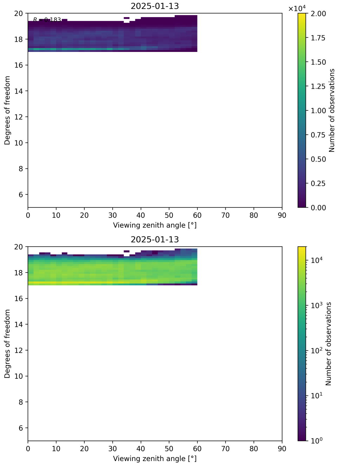
Figure 107: Scatter density plot of “Viewing zenith angle” against “Degrees of freedom” for 2025-01-12 to 2025-01-14.
