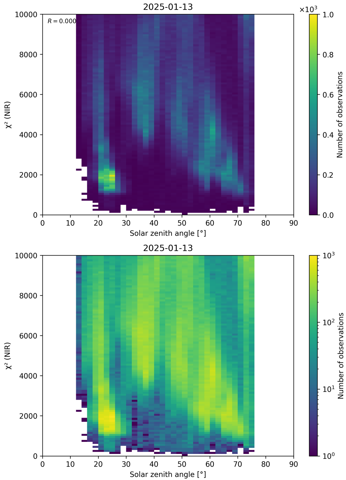
Figure 94: Scatter density plot of “Solar zenith angle” against “ \chi^2 (NIR)” for 2025-01-12 to 2025-01-14.
