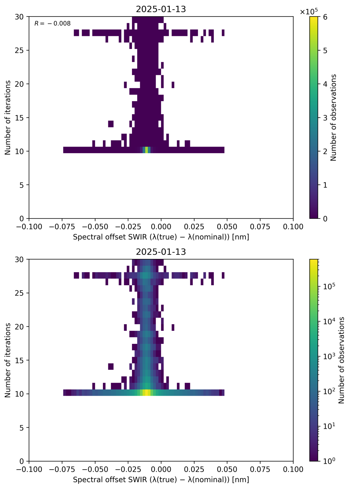
Figure 121: Scatter density plot of “Spectral offset SWIR ( \lambda_{\text{true}} - \lambda_{\text{nominal}} )” against “Number of iterations” for 2025-01-12 to 2025-01-14.
