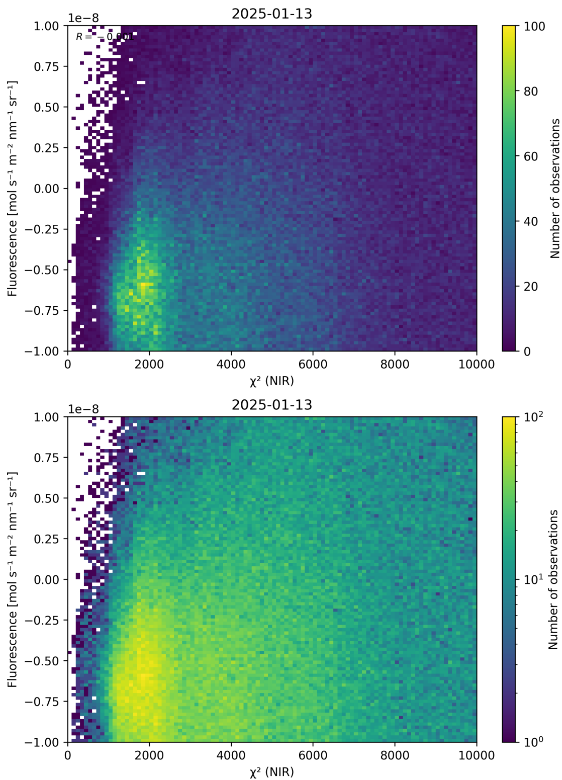
Figure 45: Scatter density plot of “ \chi^2 (NIR)” against “Fluorescence” for 2025-01-12 to 2025-01-14.
