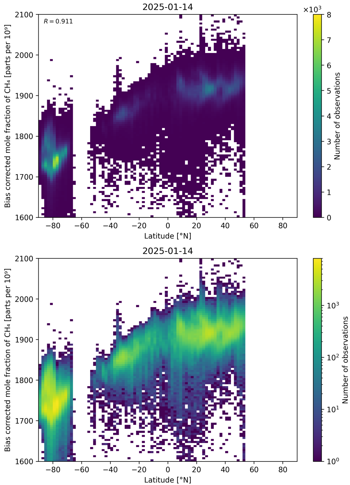
Figure 58: Scatter density plot of “Latitude” against “Bias corrected mole fraction of CH 4 ” for 2025-01-13 to 2025-01-15.
