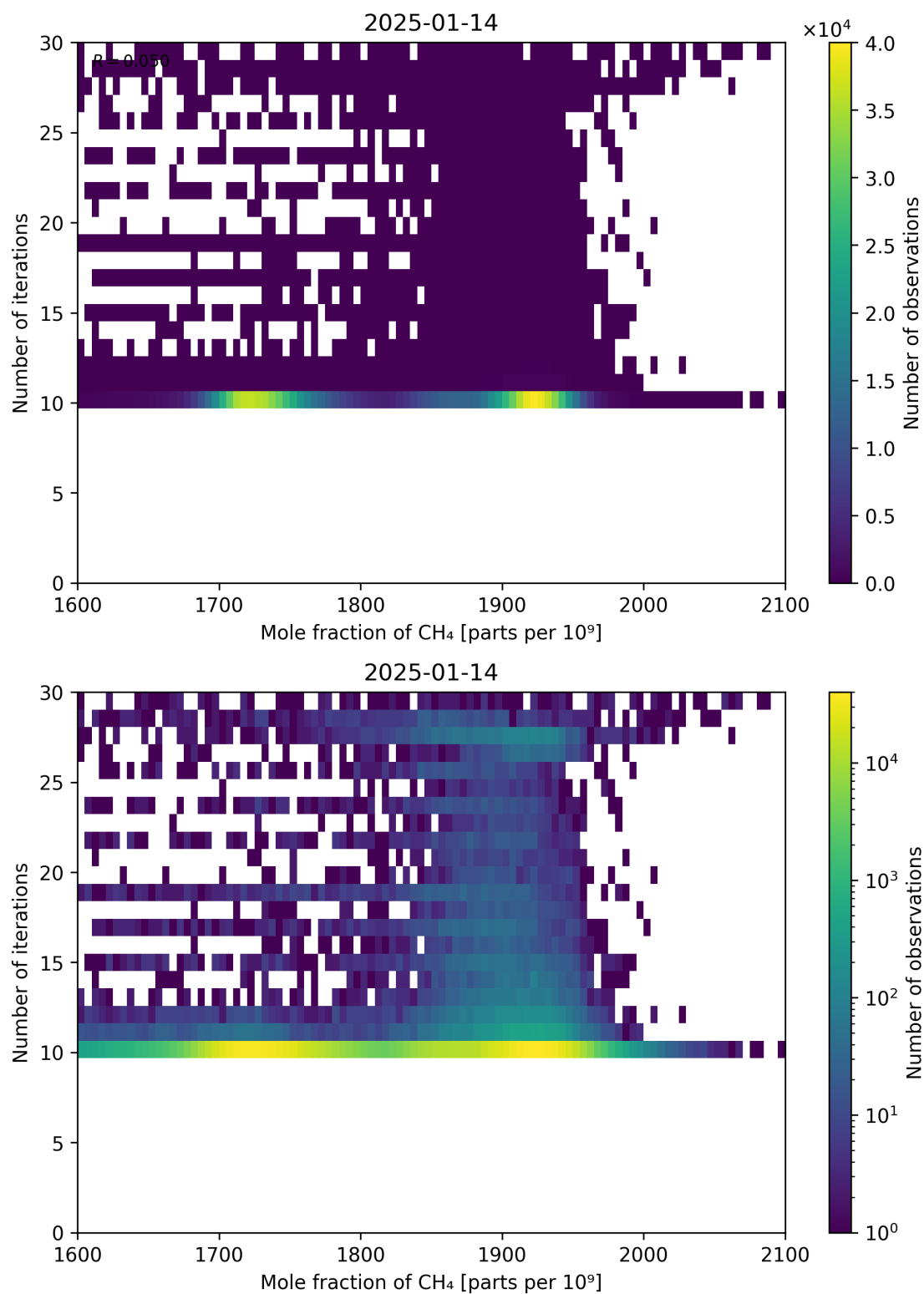
Figure 76: Scatter density plot of “Mole fraction of CH 4 ” against “Number of iterations” for 2025-01-13 to 2025-01-15.
