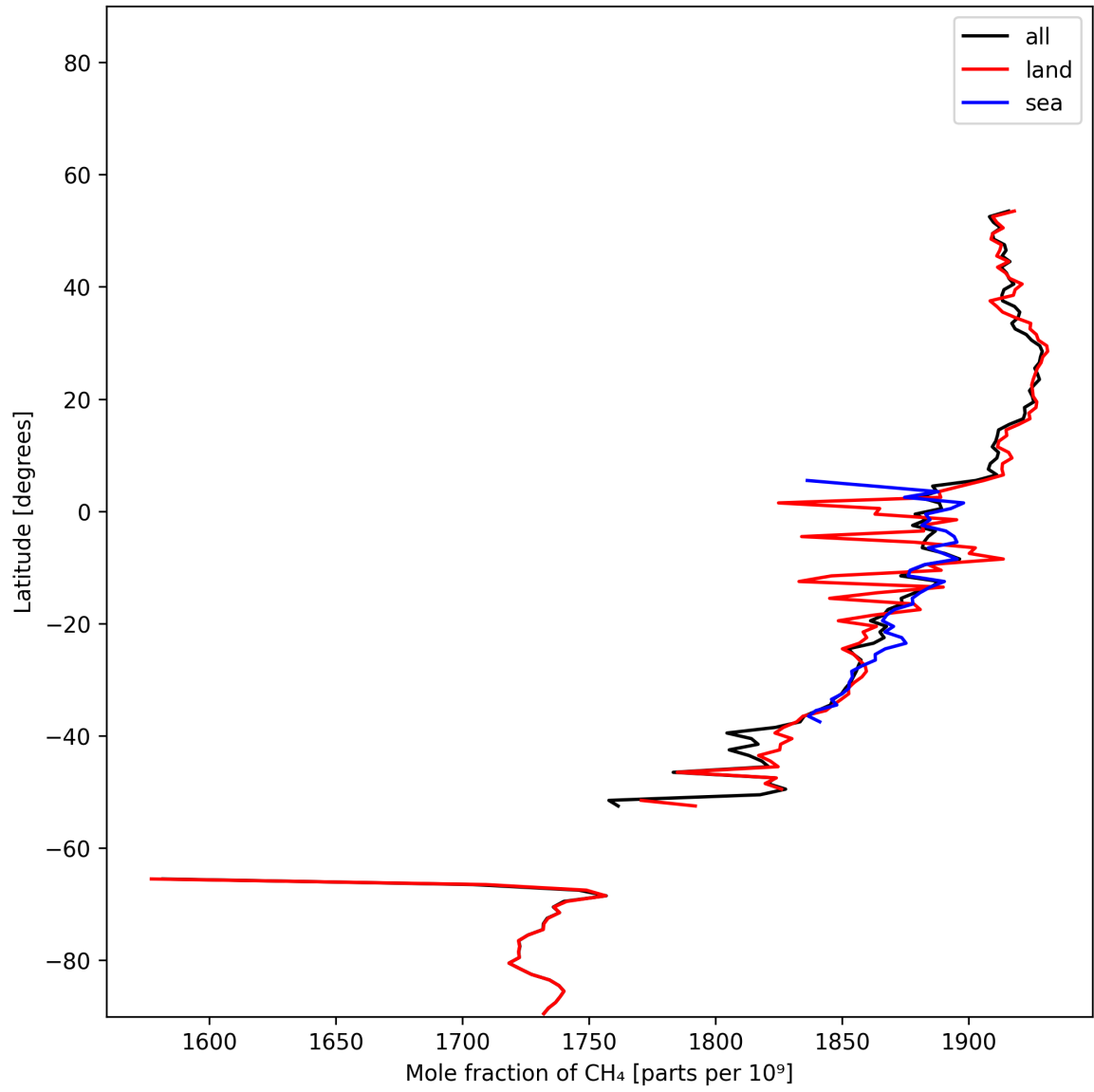
Figure 12: Zonal average of “Mole fraction of \text{CH}_4 ” for 2025-01-13 to 2025-01-15.
