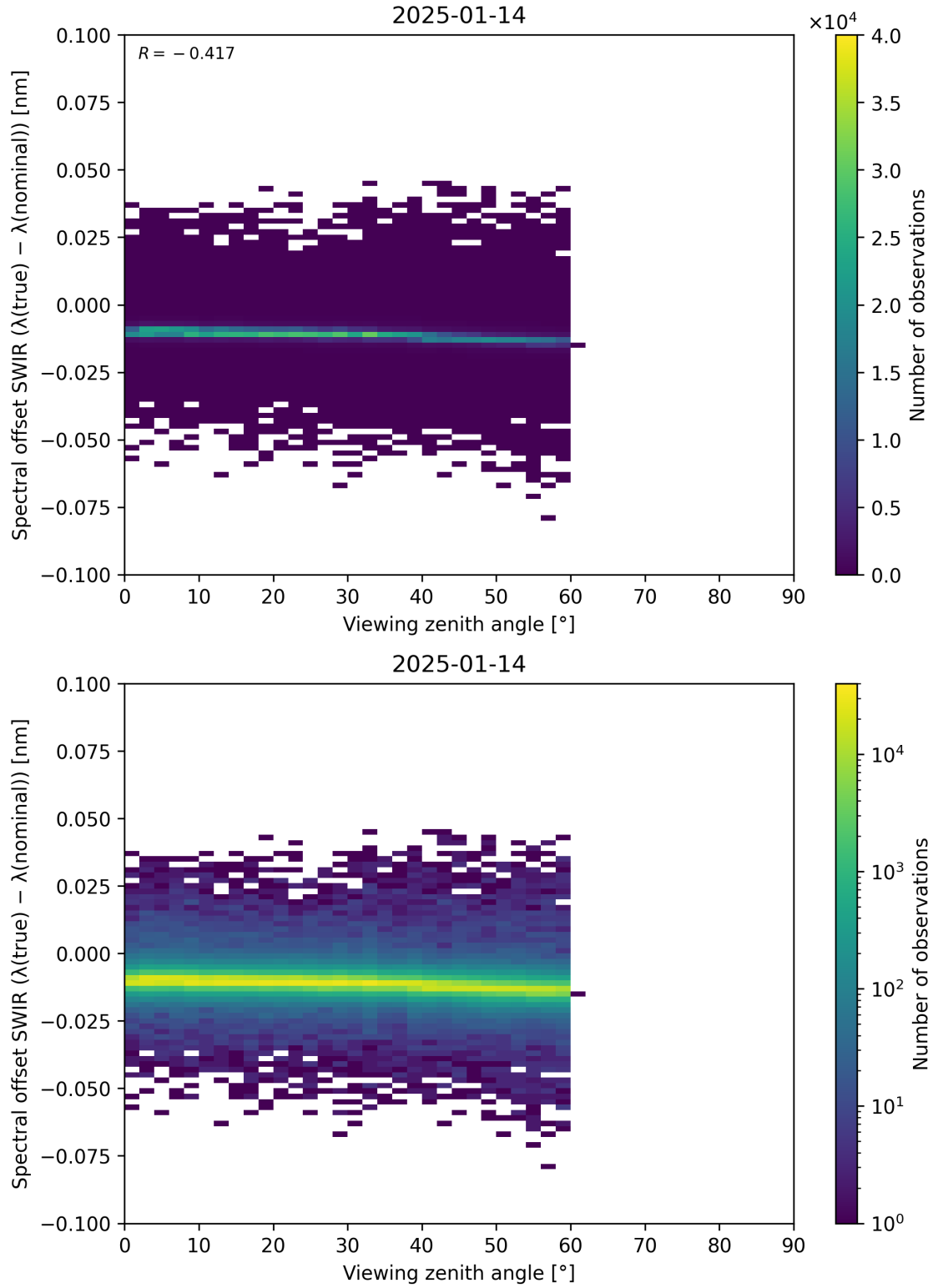
Figure 116: Scatter density plot of “Viewing zenith angle” against “Spectral offset SWIR ( \lambda_{\text{true}} - \lambda_{\text{nominal}} )” for 2025-01-13 to 2025-01-15.
