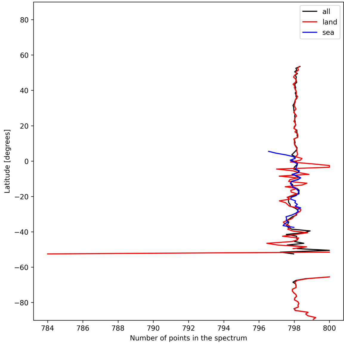
Figure 15: Zonal average of “Number of points in the spectrum” for 2025-01-13 to 2025-01-15.
