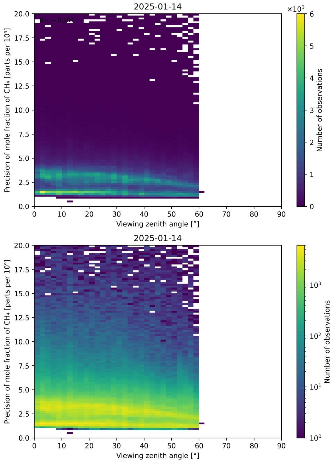
Figure 112: Scatter density plot of “Viewing zenith angle” against “Precision of mole fraction of CH 4 ” for 2025-01-13 to 2025-01-15.
