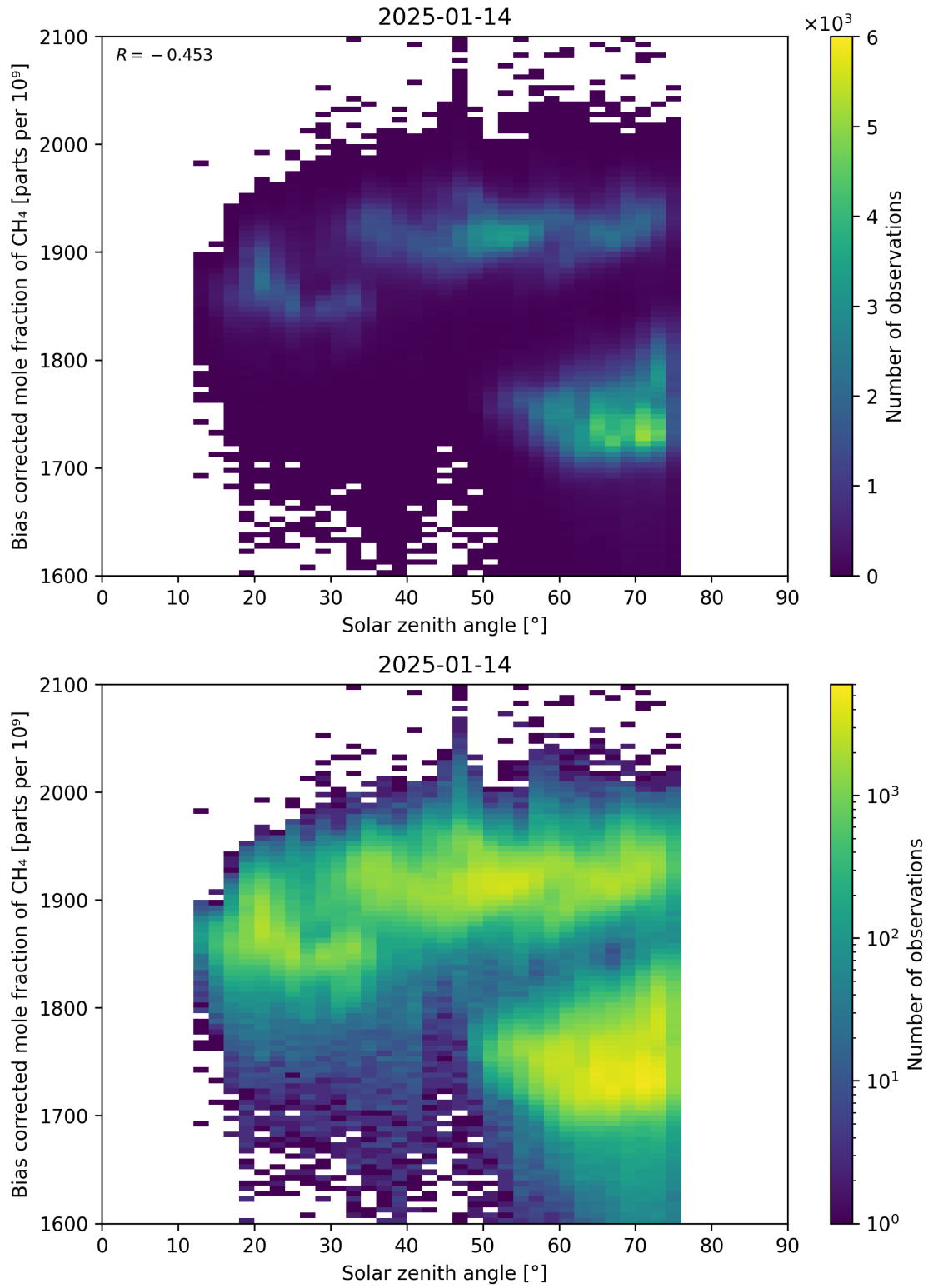
Figure 100: Scatter density plot of “Solar zenith angle” against “Bias corrected mole fraction of CH 4 ” for 2025-01-13 to 2025-01-15.
