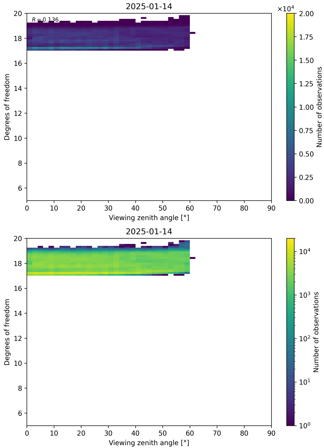
Figure 107: Scatter density plot of “Viewing zenith angle” against “Degrees of freedom” for 2025-01-13 to 2025-01-15.
