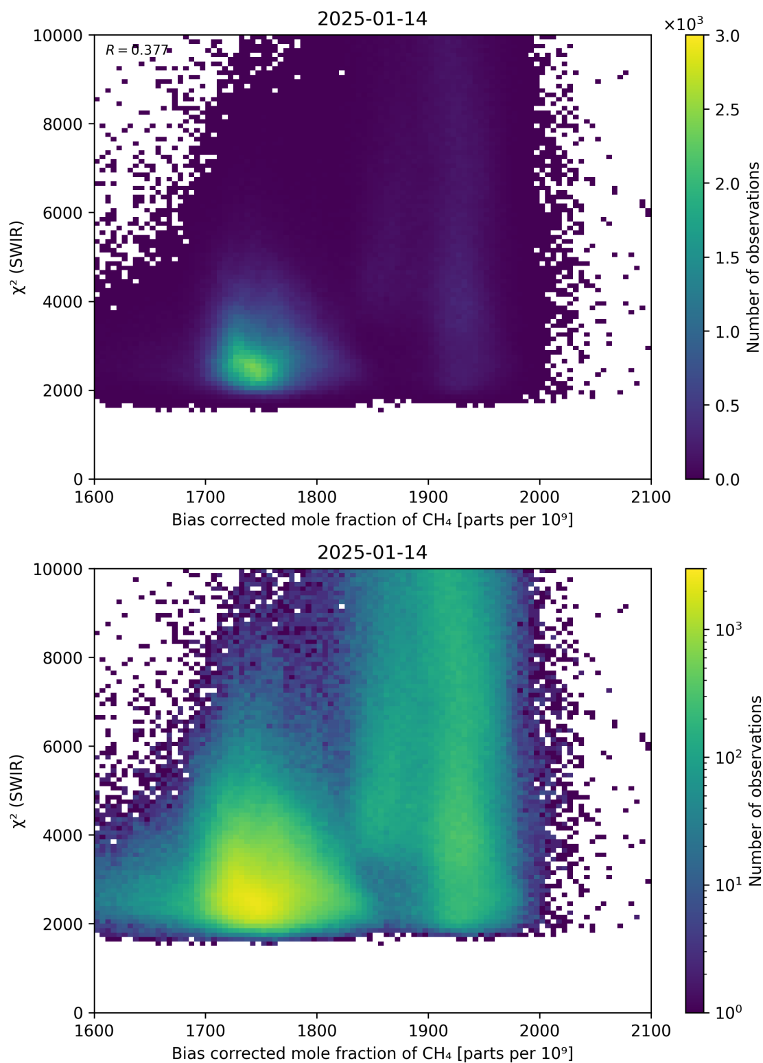
Figure 64: Scatter density plot of “Bias corrected mole fraction of \text{CH}_4 ” against “ \chi^2 (SWIR)” for 2025-01-13 to 2025-01-15.
