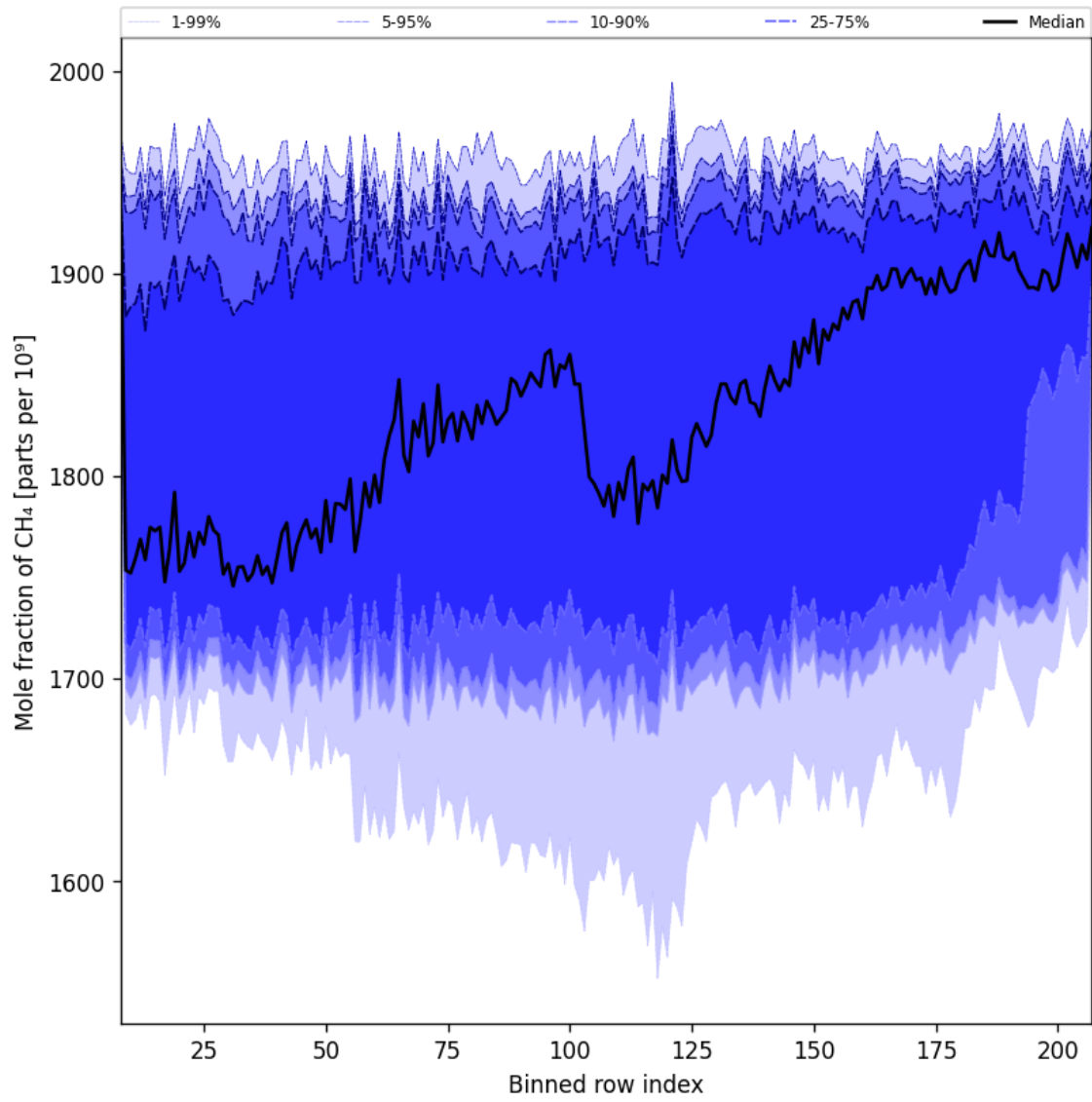
Figure 34: Along track statistics of “Mole fraction of CH 4 ” for 2025-01-13 to 2025-01-15
