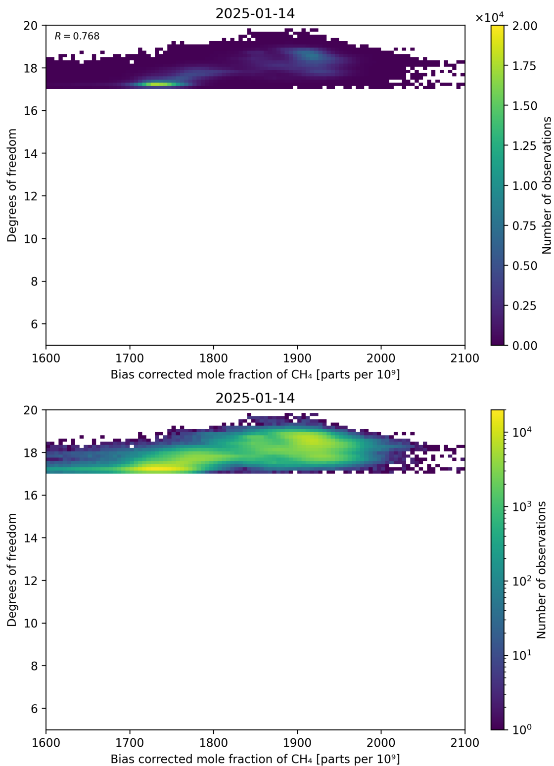
Figure 65: Scatter density plot of “Bias corrected mole fraction of \text{CH}_4 ” against “Degrees of freedom” for 2025-01-13 to 2025-01-15.
