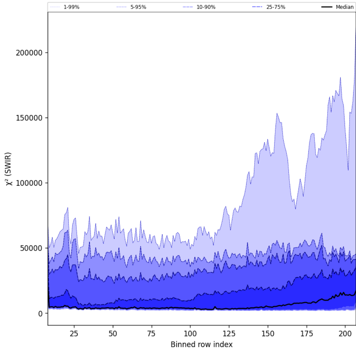
Figure 39: Along track statistics of “ \chi^2 (SWIR)” for 2025-01-13 to 2025-01-15
