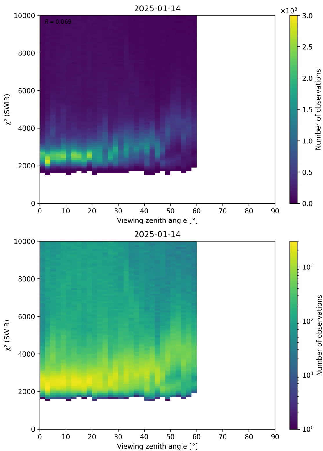
Figure 106: Scatter density plot of “Viewing zenith angle” against “ \chi^2 (SWIR)” for 2025-01-13 to 2025-01-15.
