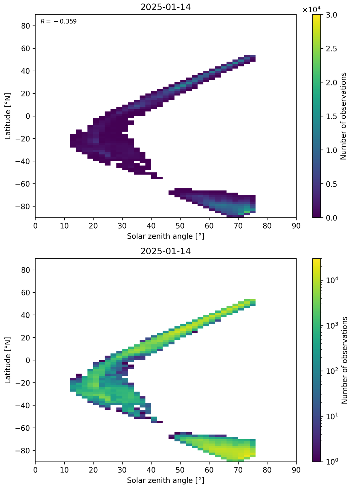
Figure 98: Scatter density plot of “Solar zenith angle” against “Latitude” for 2025-01-13 to 2025-01-15.
