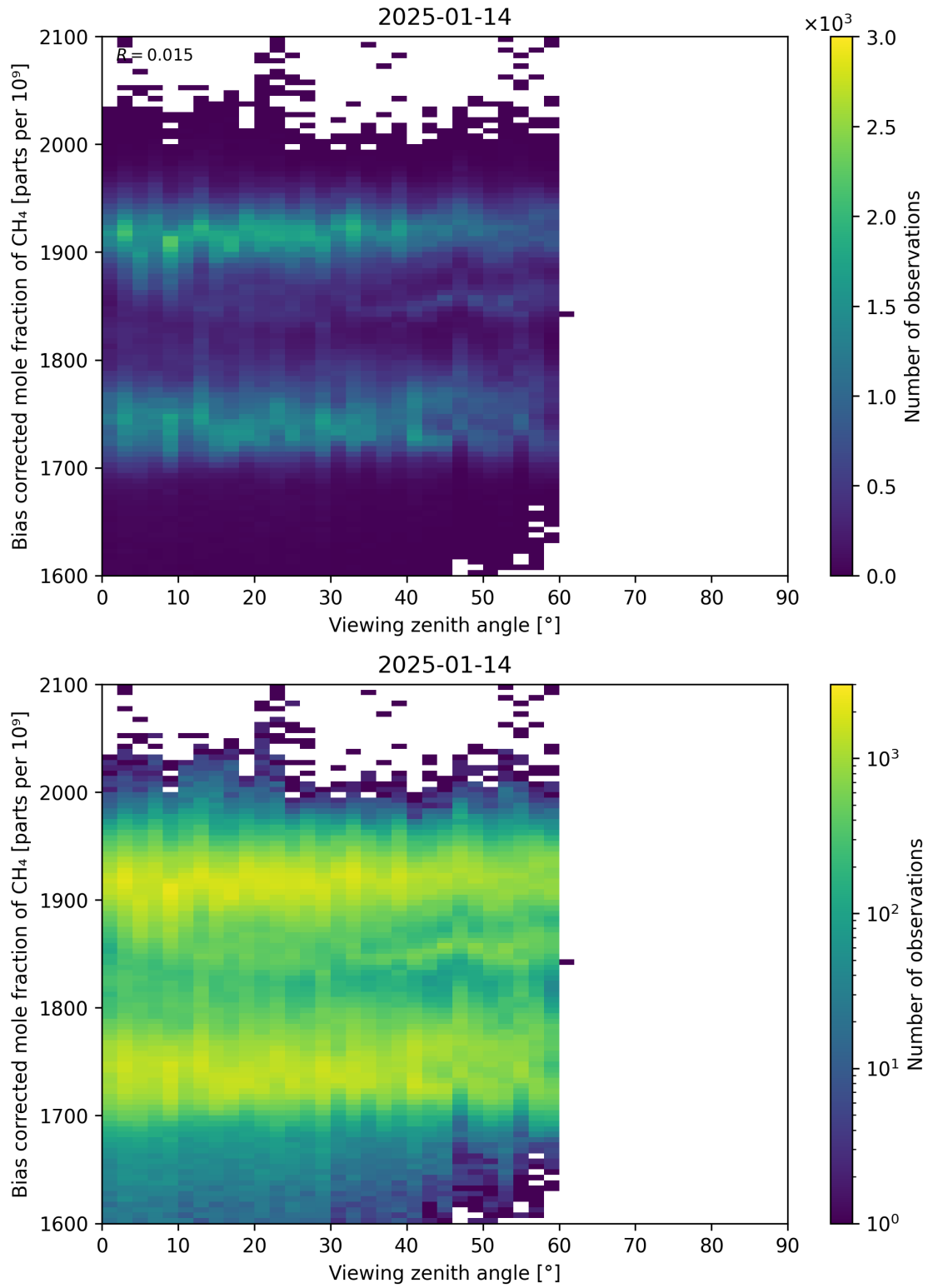
Figure 111: Scatter density plot of “Viewing zenith angle” against “Bias corrected mole fraction of CH 4 ” for 2025-01-13 to 2025-01-15.
