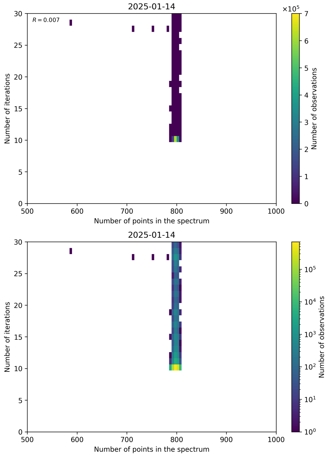
Figure 92: Scatter density plot of “Number of points in the spectrum” against “Number of iterations” for 2025-01-13 to 2025-01-15.
