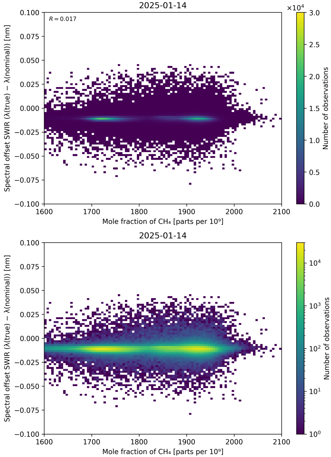
Figure 86: Scatter density plot of “Mole fraction of CH 4 ” against “Spectral offset SWIR ( \lambda_{\text{true}} - \lambda_{\text{nominal}} )” for 2025-01-13 to 2025-01-15.
