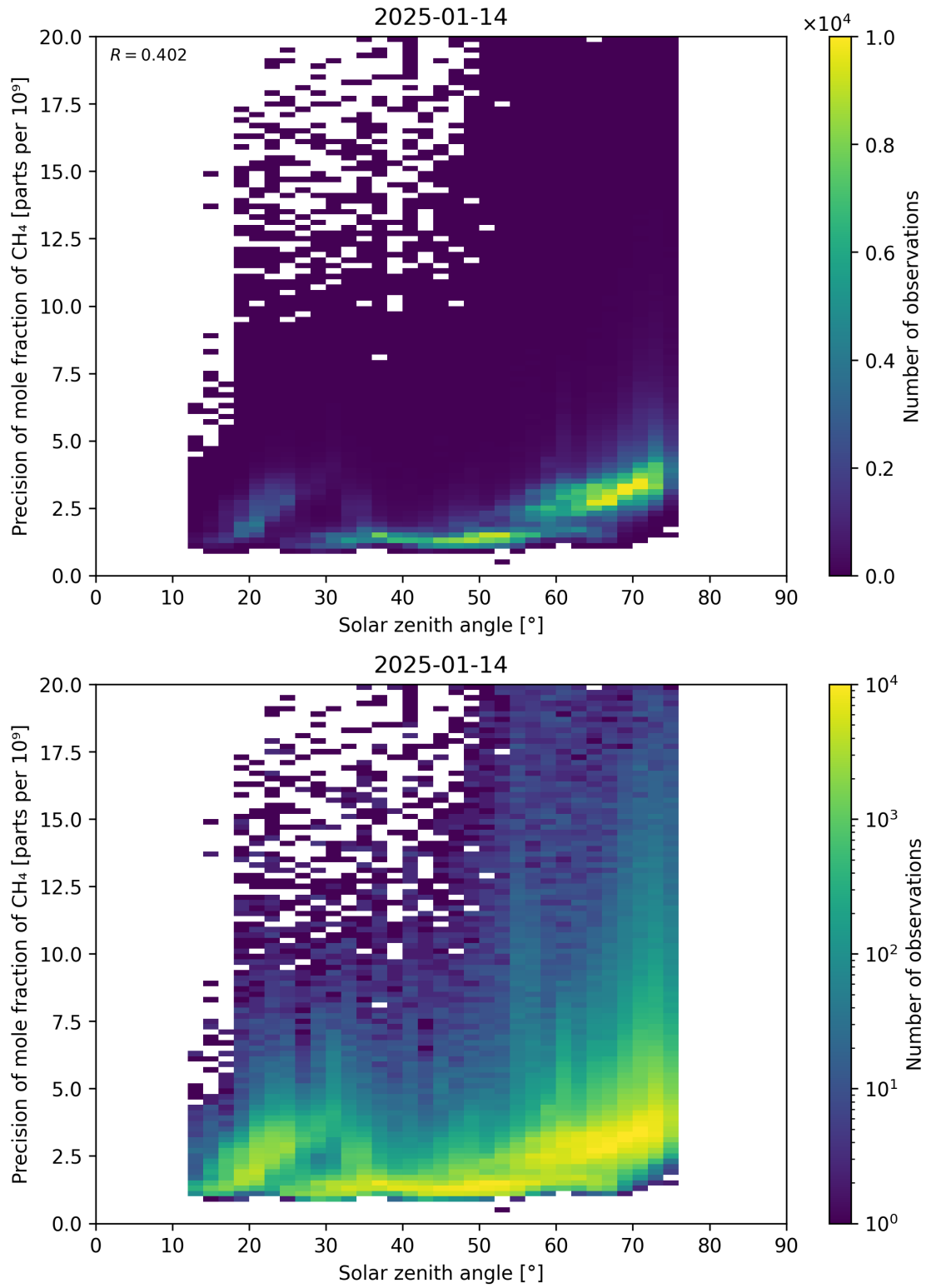
Figure 101: Scatter density plot of “Solar zenith angle” against “Precision of mole fraction of CH 4 ” for 2025-01-13 to 2025-01-15.
