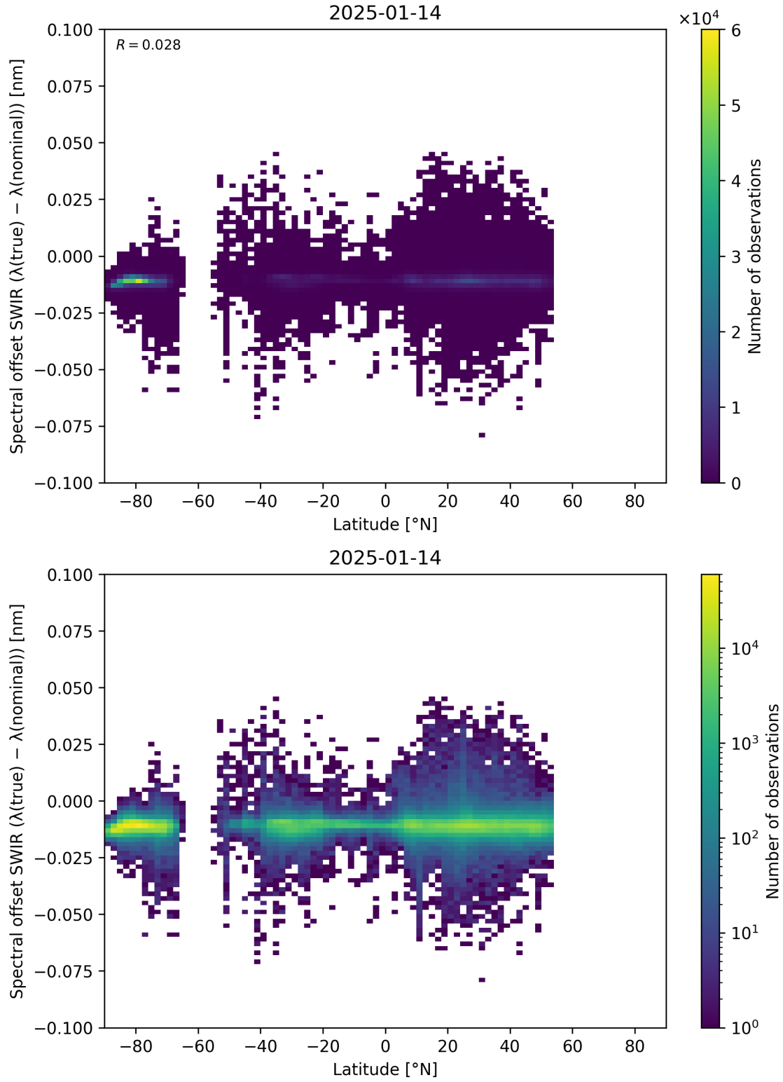
Figure 62: Scatter density plot of “Latitude” against “Spectral offset SWIR ( \lambda_{\text{true}} - \lambda_{\text{nominal}} )” for 2025-01-13 to 2025-01-15.
