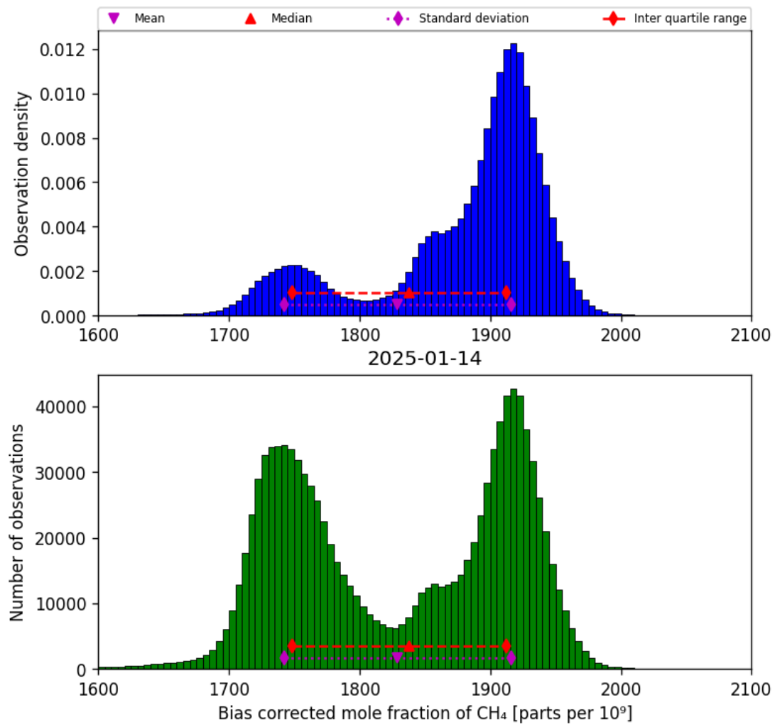
Figure 25: Histogram of “Bias corrected mole fraction of CH 4 ” for 2025-01-13 to 2025-01-15
