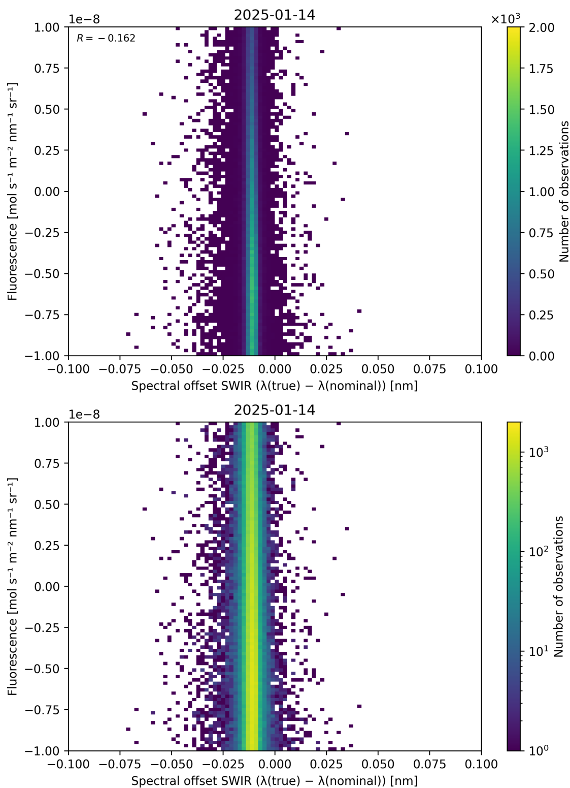
Figure 120: Scatter density plot of “Spectral offset SWIR ( \lambda_{\text{true}} - \lambda_{\text{nominal}} )” against “Fluorescence” for 2025-01-13 to 2025-01-15.
