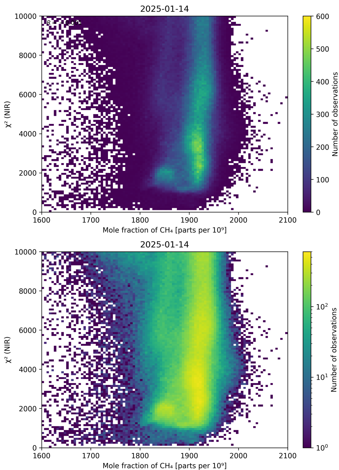
Figure 70: Scatter density plot of “Mole fraction of CH 4 ” against “ \chi^2 (NIR)” for 2025-01-13 to 2025-01-15.
