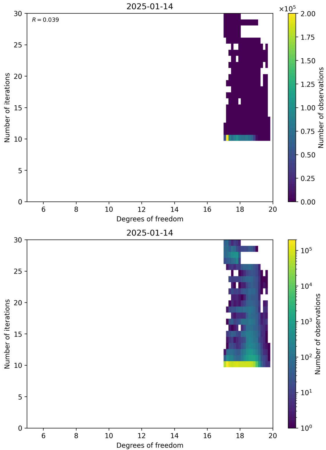
Figure 52: Scatter density plot of “Degrees of freedom” against “Number of iterations” for 2025-01-13 to 2025-01-15.
