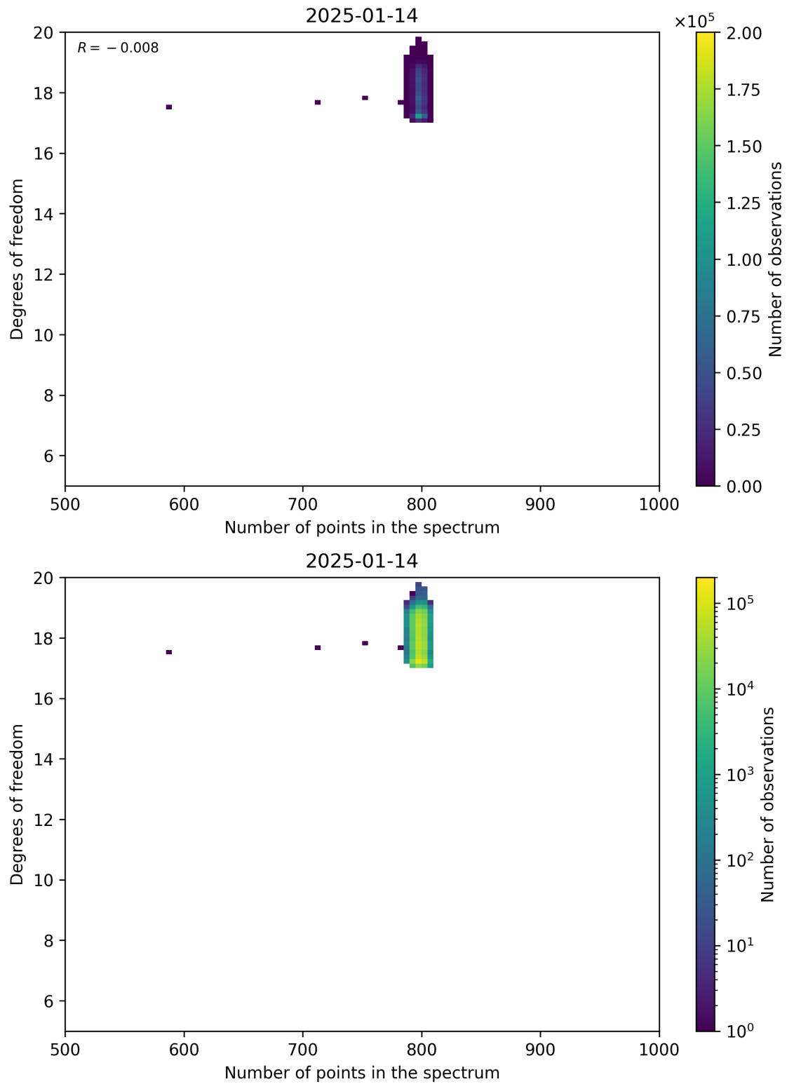
Figure 90: Scatter density plot of “Number of points in the spectrum” against “Degrees of freedom” for 2025-01-13 to 2025-01-15.
