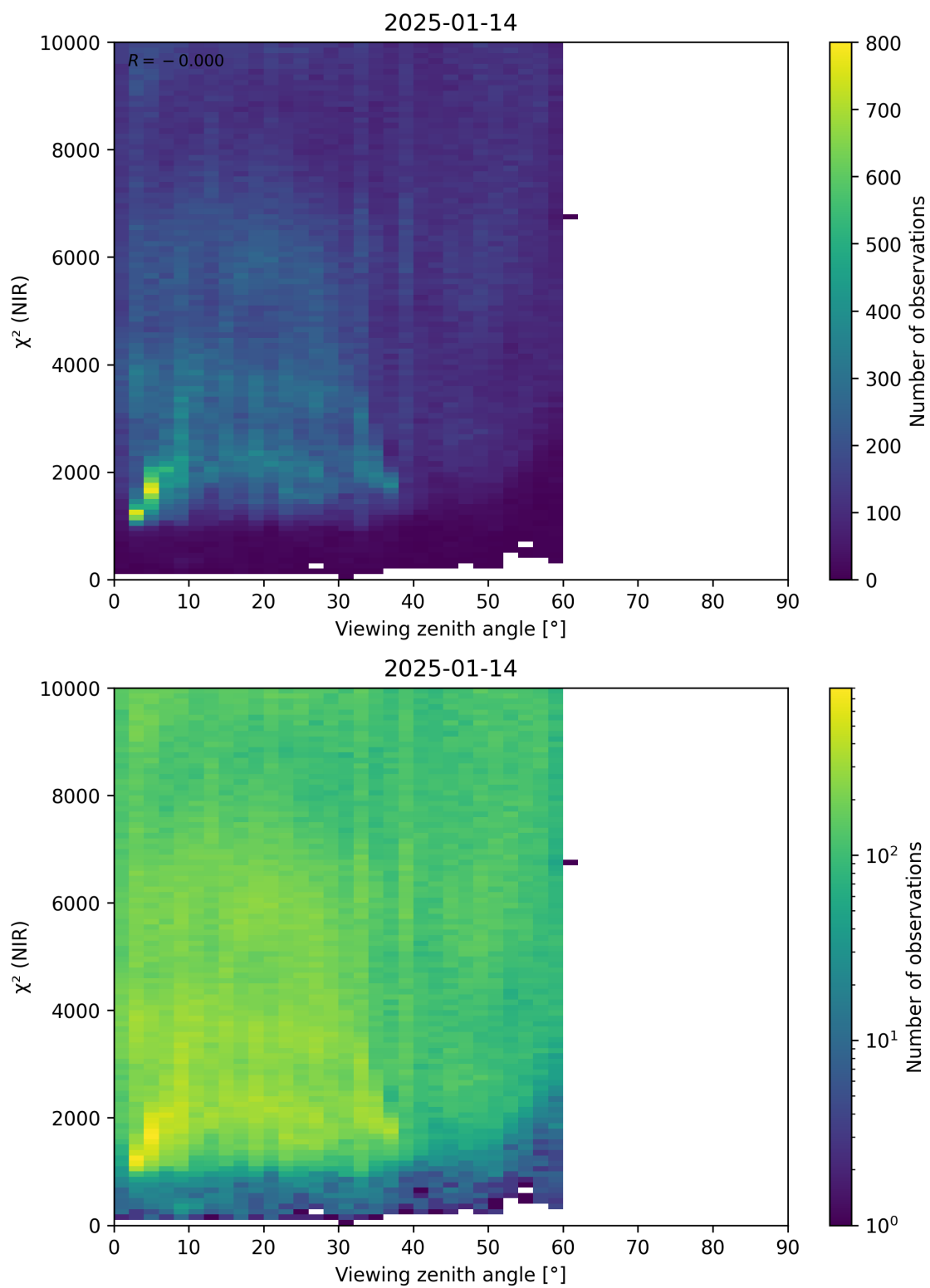
Figure 105: Scatter density plot of “Viewing zenith angle” against “ \chi^2 (NIR)” for 2025-01-13 to 2025-01-15.
