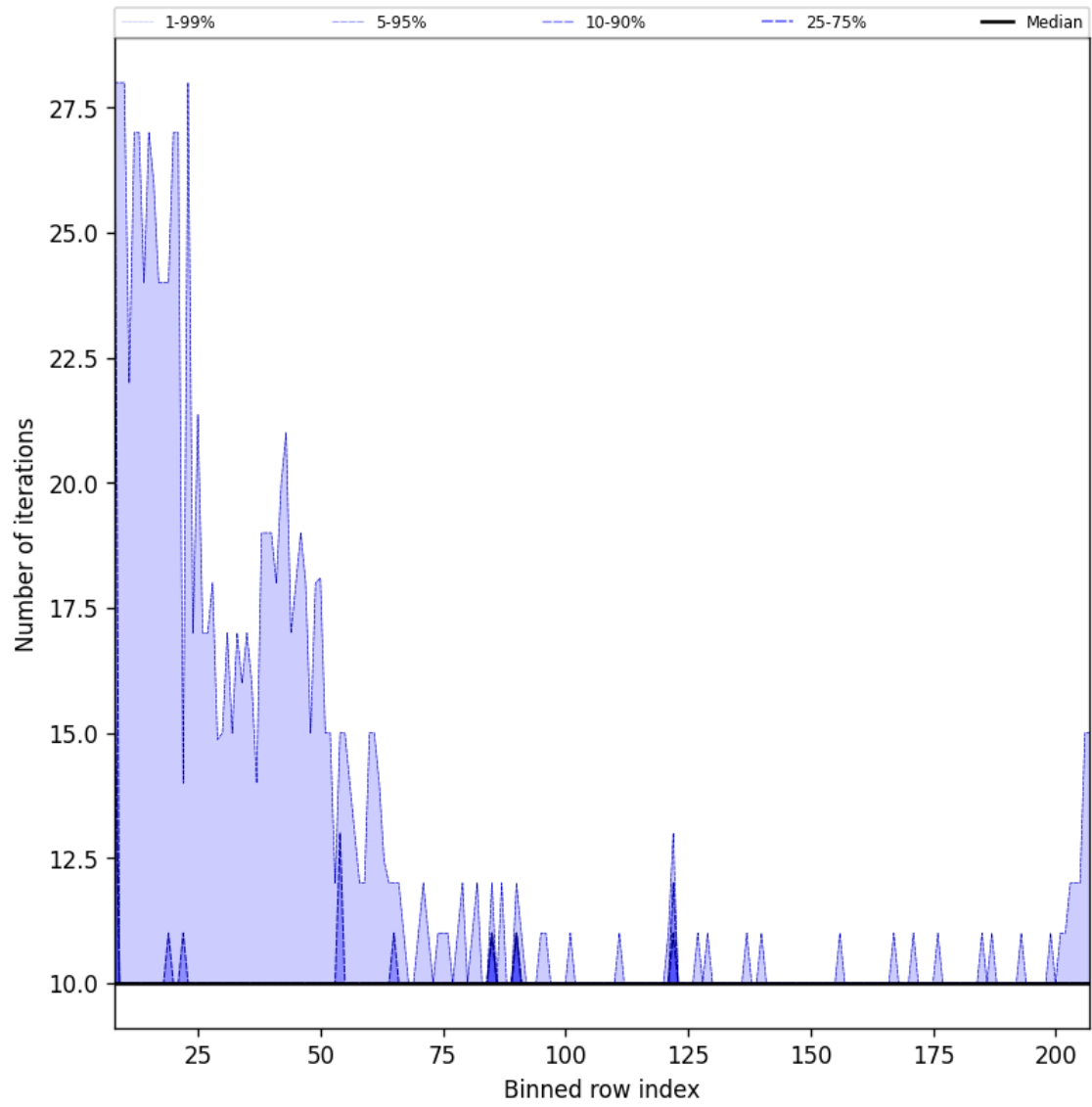
Figure 42: Along track statistics of “Number of iterations” for 2025-01-13 to 2025-01-15
