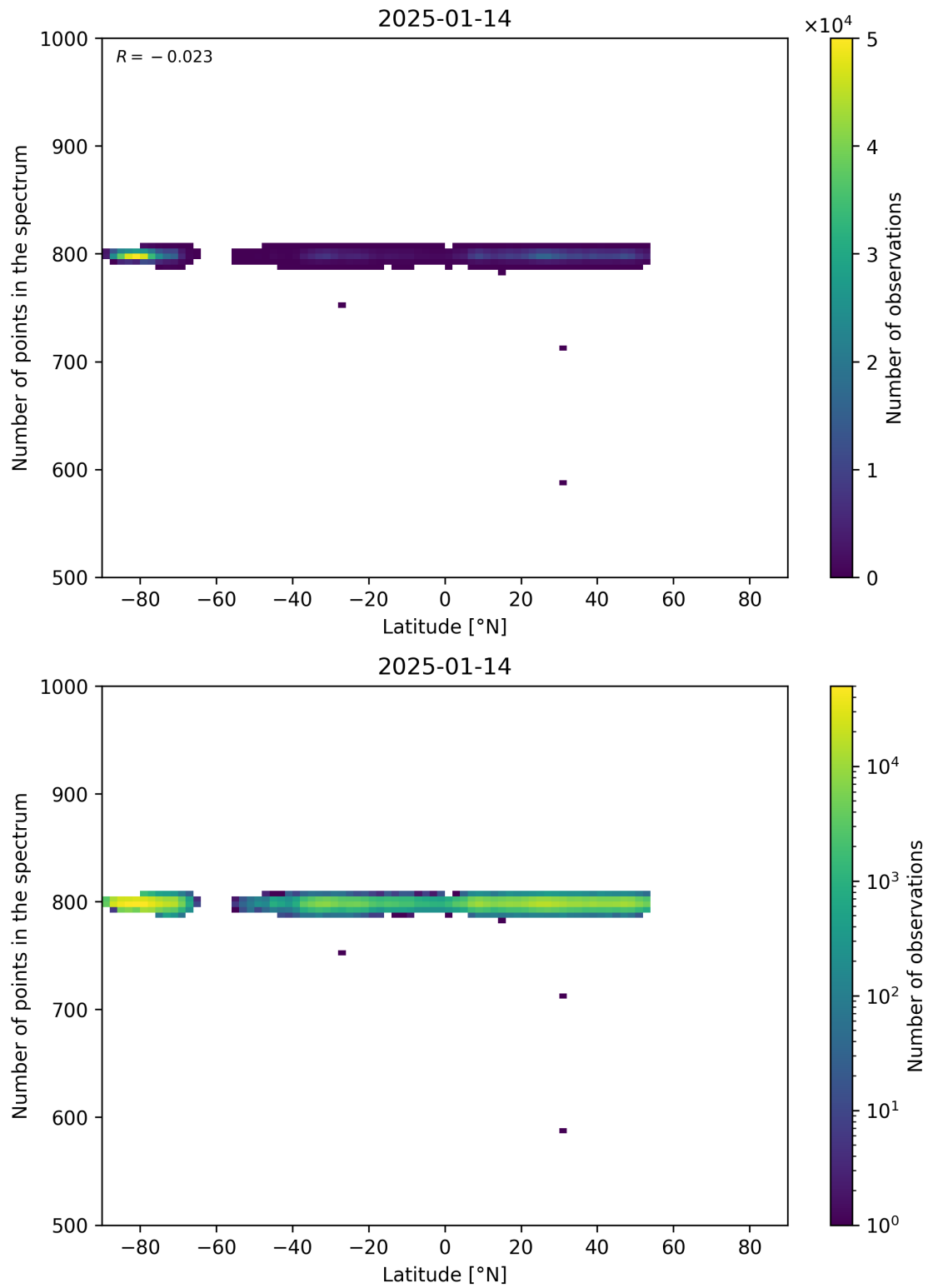
Figure 61: Scatter density plot of “Latitude” against “Number of points in the spectrum” for 2025-01-13 to 2025-01-15.
