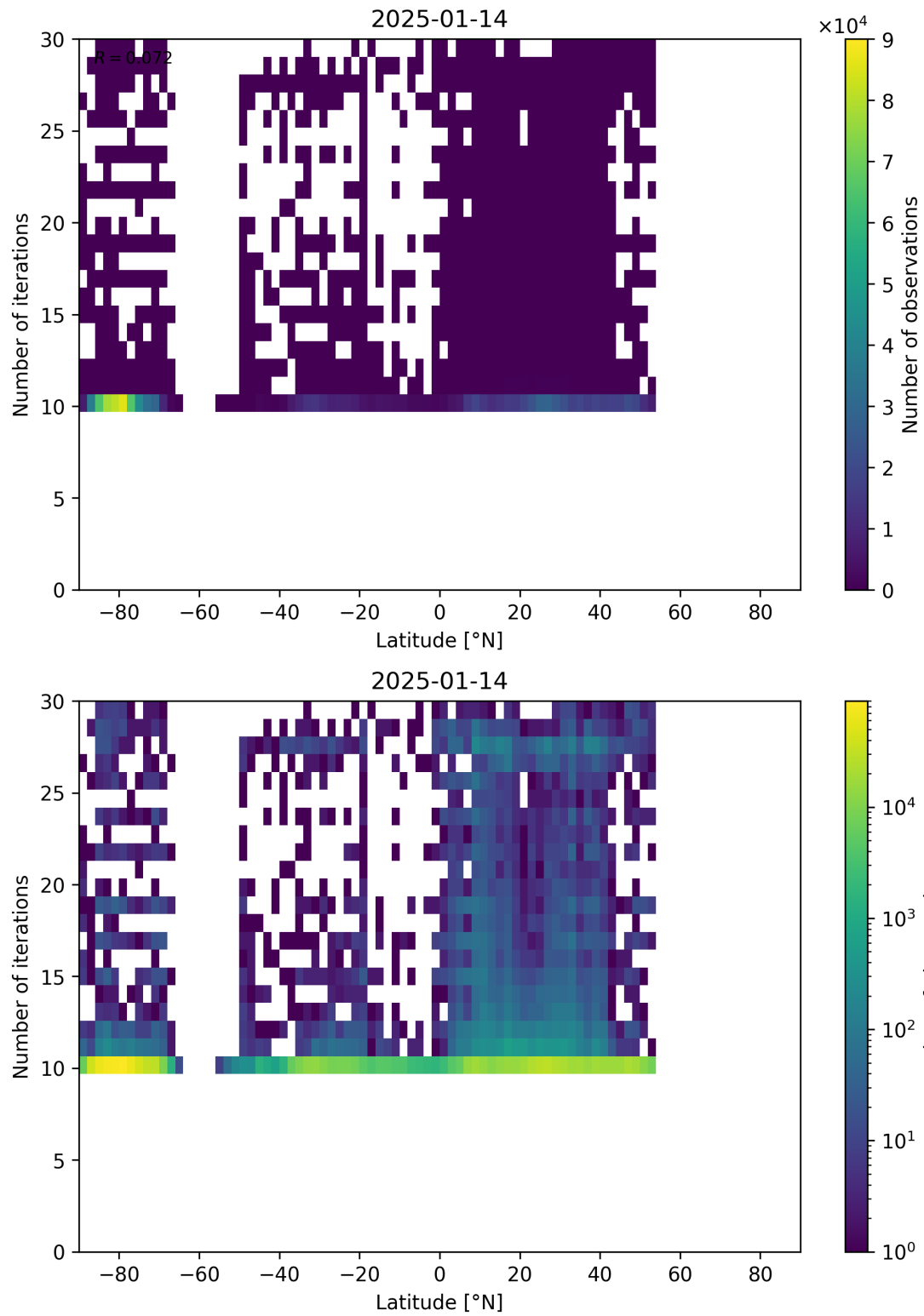
Figure 60: Scatter density plot of “Latitude” against “Number of iterations” for 2025-01-13 to 2025-01-15.
