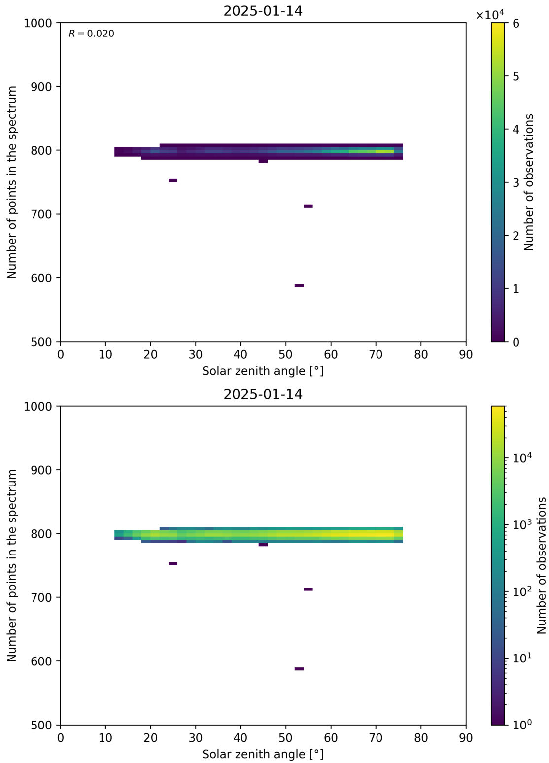
Figure 103: Scatter density plot of “Solar zenith angle” against “Number of points in the spectrum” for 2025-01-13 to 2025-01-15.
