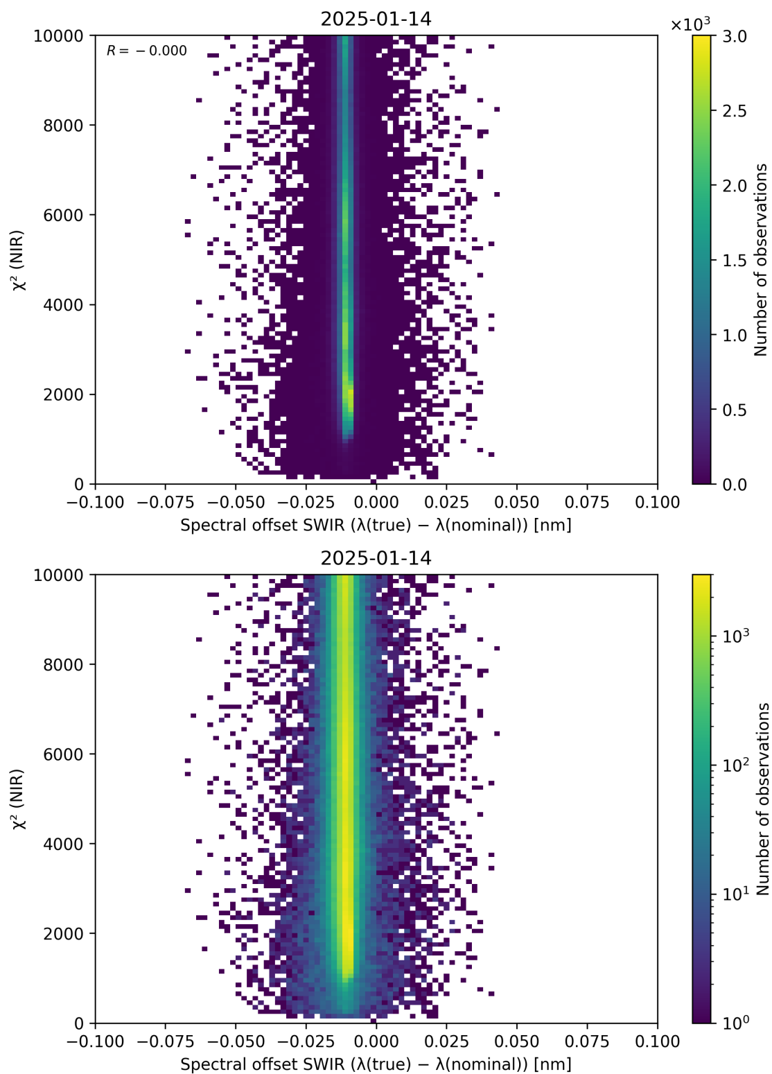
Figure 117: Scatter density plot of “Spectral offset SWIR ( \lambda_{\text{true}} - \lambda_{\text{nominal}} )” against “ \chi^2 (NIR)” for 2025-01-13 to 2025-01-15.
