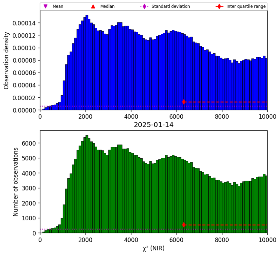
Figure 29: Histogram of " \chi^2 (NIR)" for 2025-01-13 to 2025-01-15
