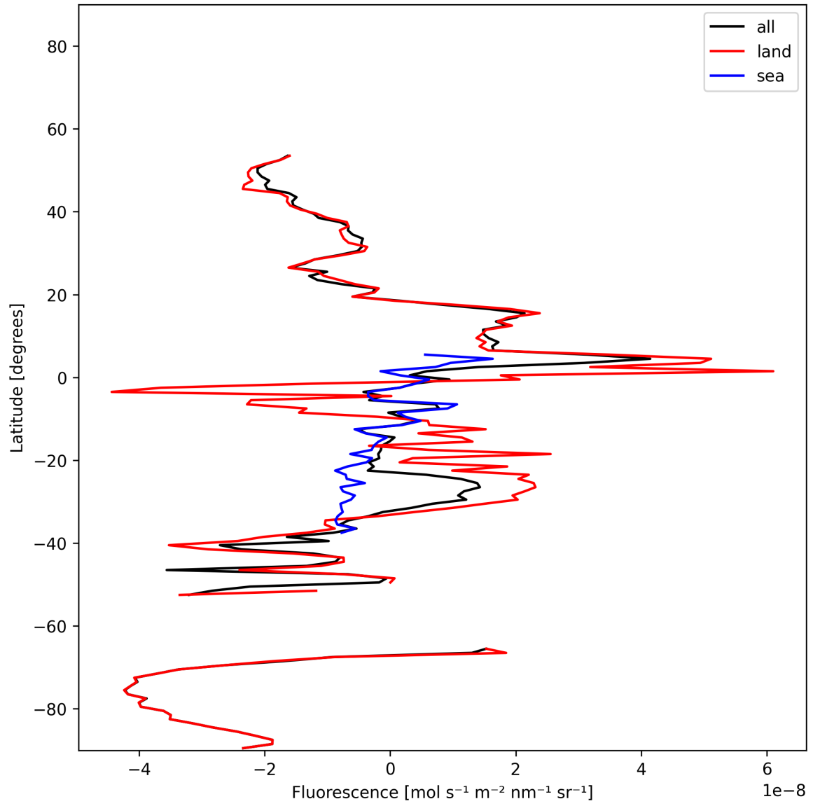
Figure 21: Zonal average of “Fluorescence” for 2025-01-13 to 2025-01-15.
