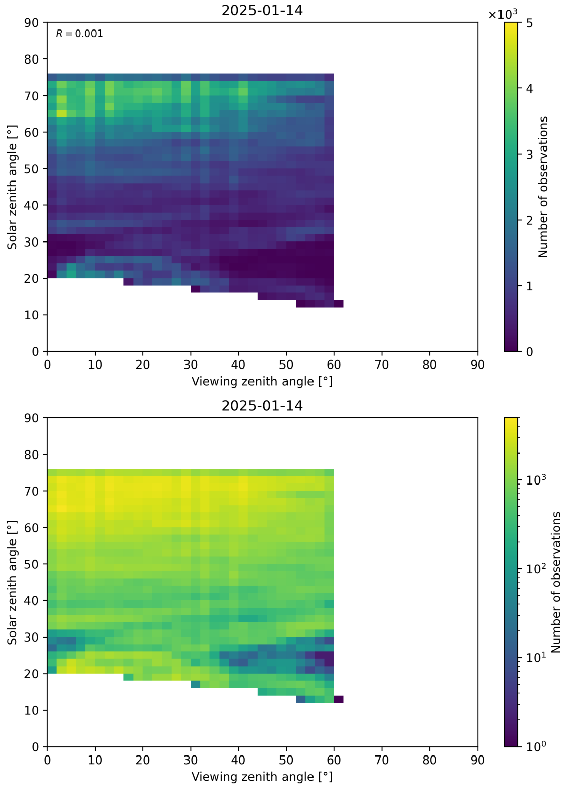
Figure 115: Scatter density plot of “Viewing zenith angle” against “Solar zenith angle” for 2025-01-13 to 2025-01-15.
