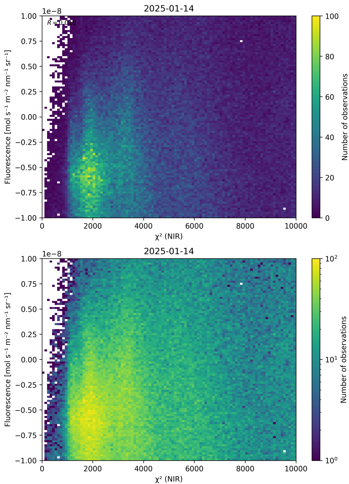
Figure 45: Scatter density plot of “ \chi^2 (NIR)” against “Fluorescence” for 2025-01-13 to 2025-01-15.
