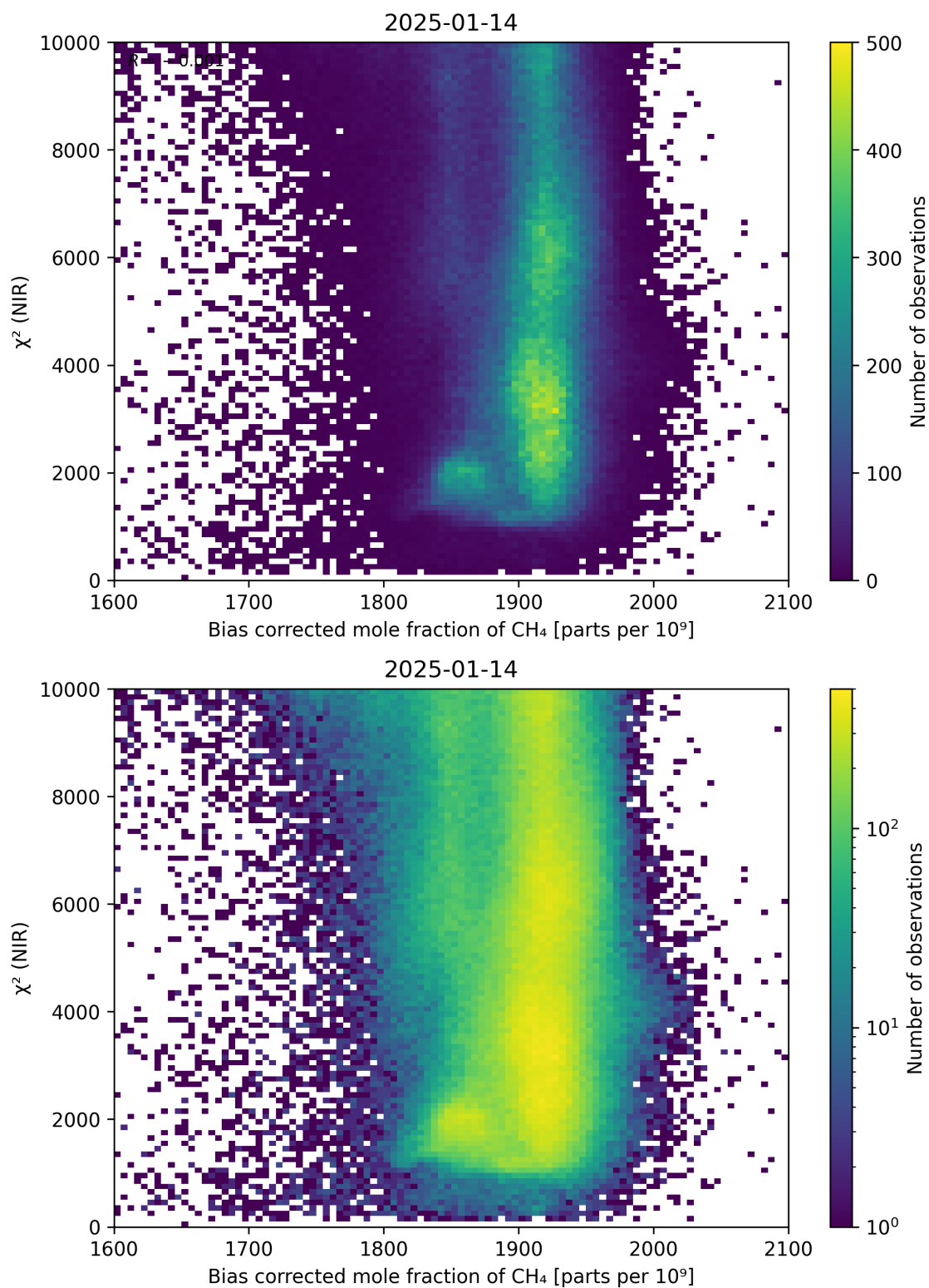
Figure 63: Scatter density plot of “Bias corrected mole fraction of \text{CH}_4 ” against “ \chi^2 (NIR)” for 2025-01-13 to 2025-01-15.
