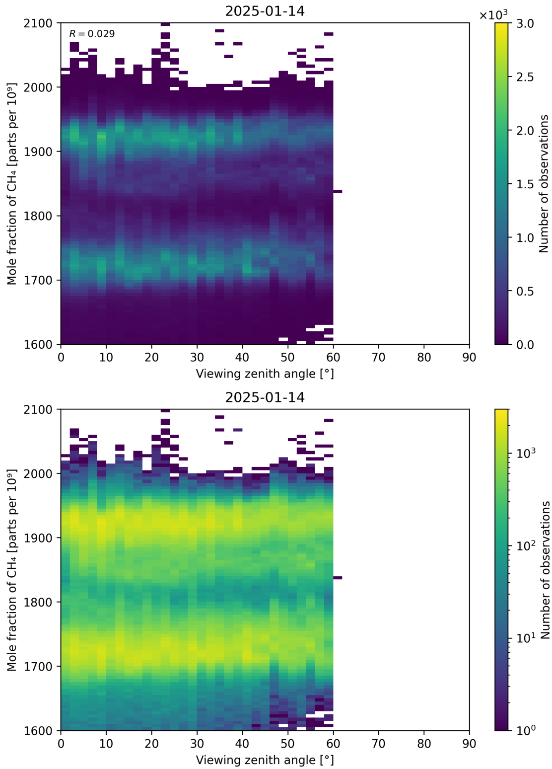
Figure 110: Scatter density plot of “Viewing zenith angle” against “Mole fraction of CH 4 ” for 2025-01-13 to 2025-01-15.
