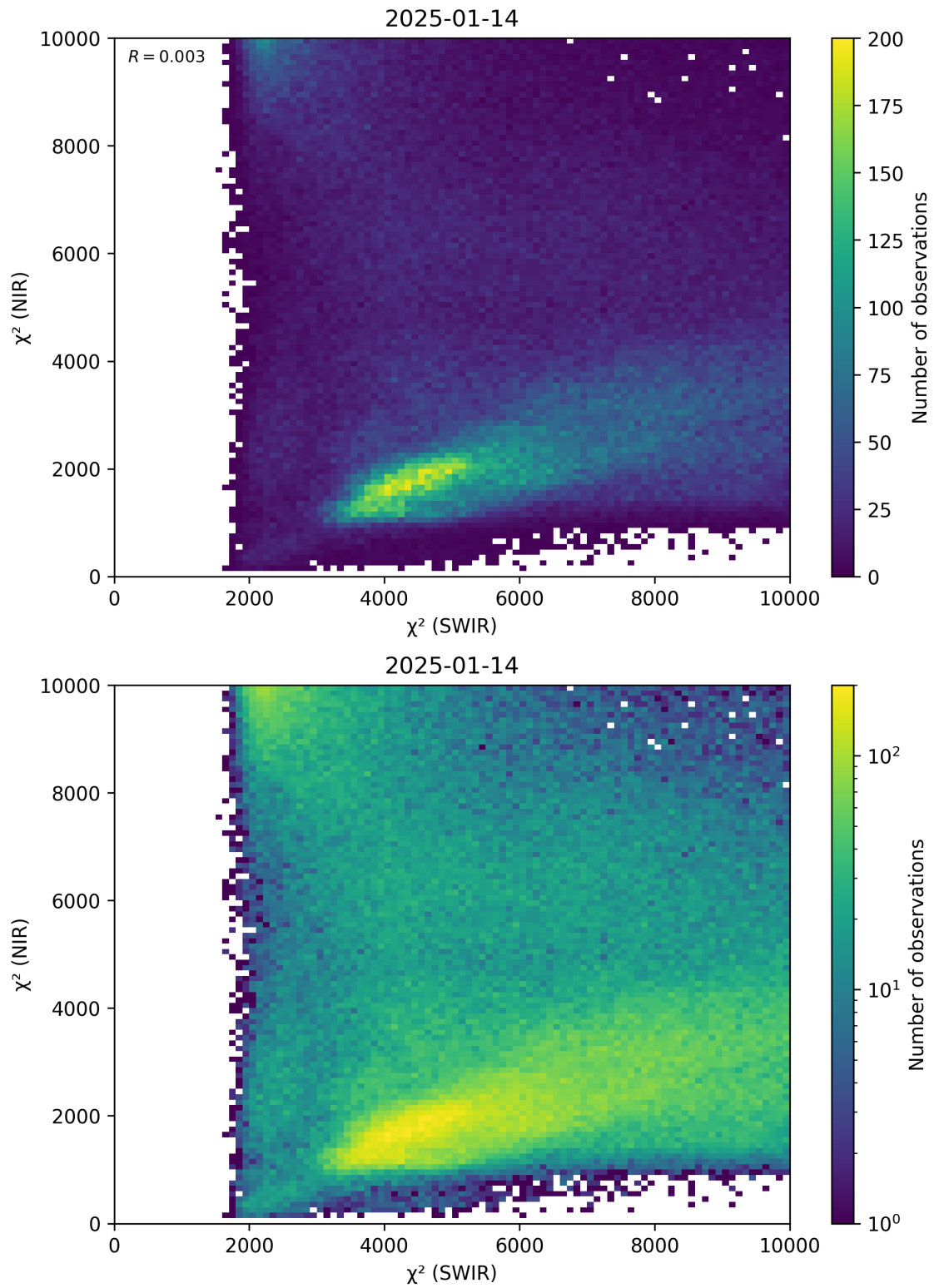
Figure 47: Scatter density plot of “ \chi^2 (SWIR)” against “ \chi^2 (NIR)” for 2025-01-13 to 2025-01-15.
