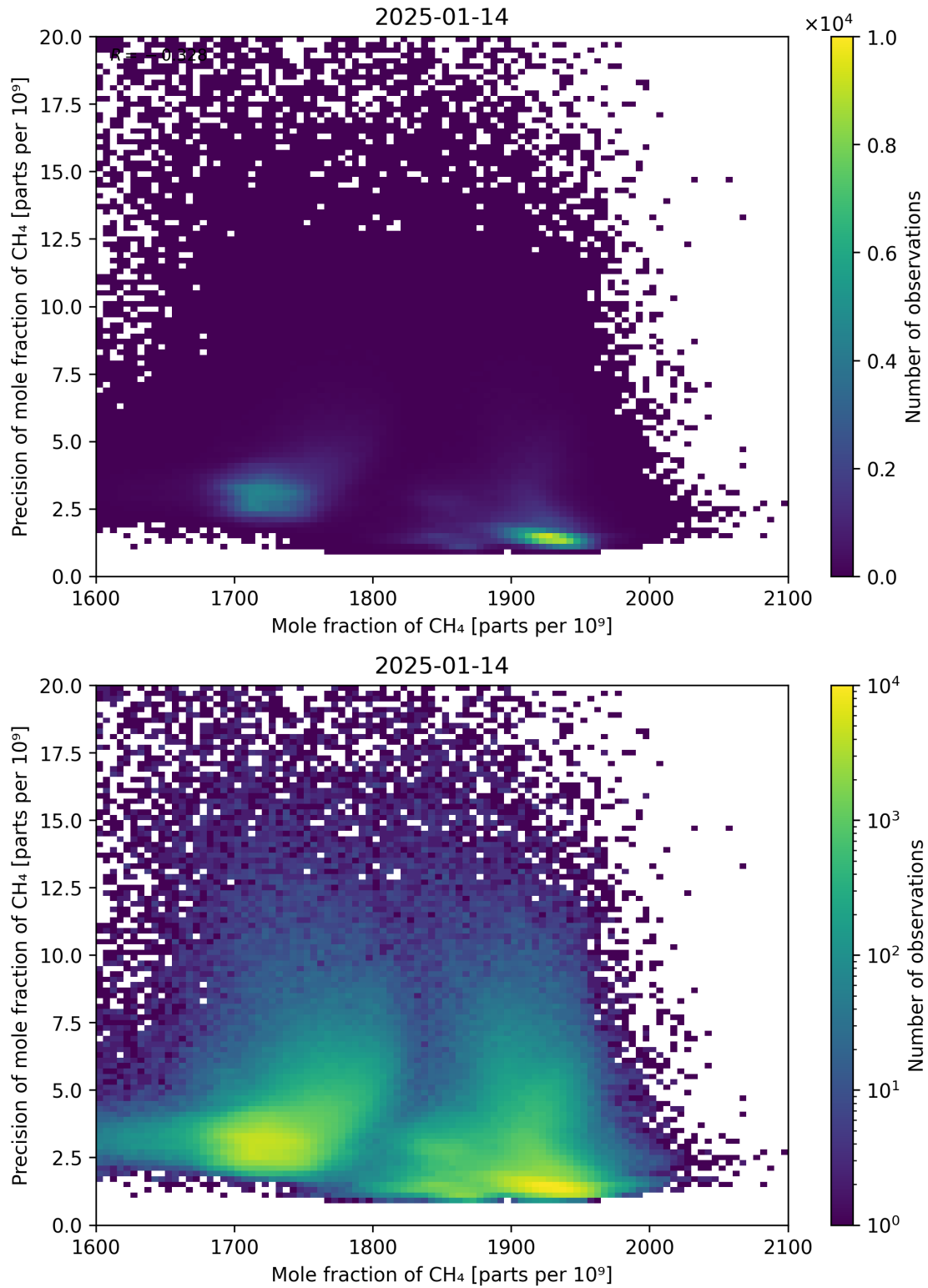
Figure 75: Scatter density plot of “Mole fraction of CH 4 ” against “Precision of mole fraction of CH 4 ” for 2025-01-13 to 2025-01-15.
