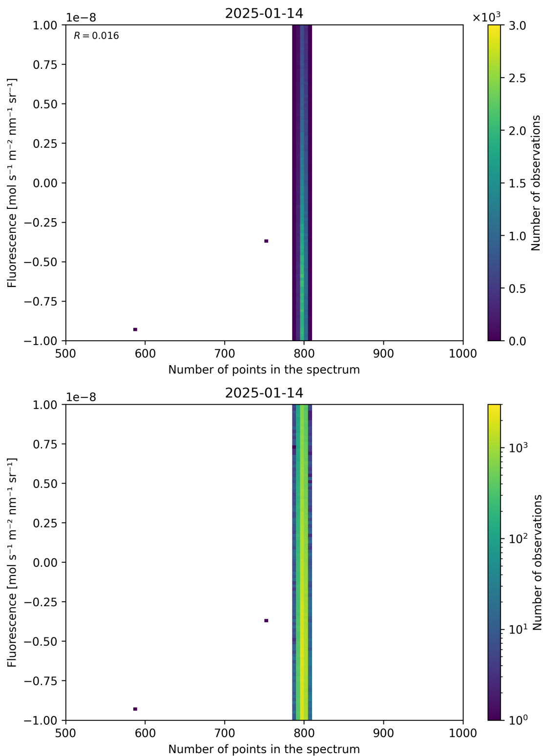
Figure 91: Scatter density plot of “Number of points in the spectrum” against “Fluorescence” for 2025-01-13 to 2025-01-15.
