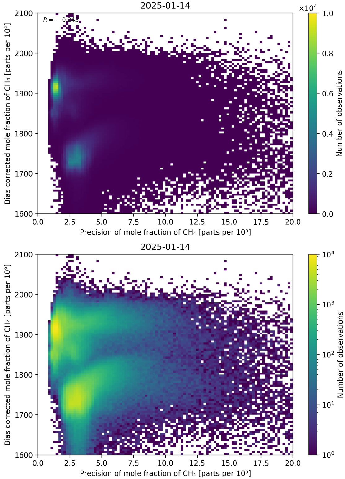
Figure 82: Scatter density plot of “Precision of mole fraction of CH 4 ” against “Bias corrected mole fraction of CH 4 ” for 2025-01-13 to 2025-01-15.
