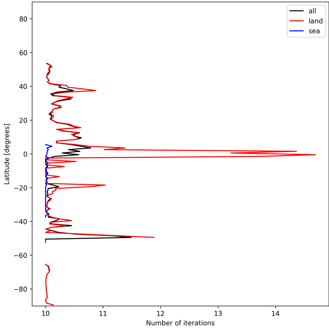
Figure 20: Zonal average of “Number of iterations” for 2025-01-13 to 2025-01-15.
