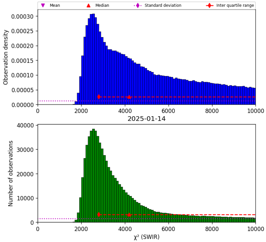
Figure 28: Histogram of “ \chi^2 (SWIR)” for 2025-01-13 to 2025-01-15
