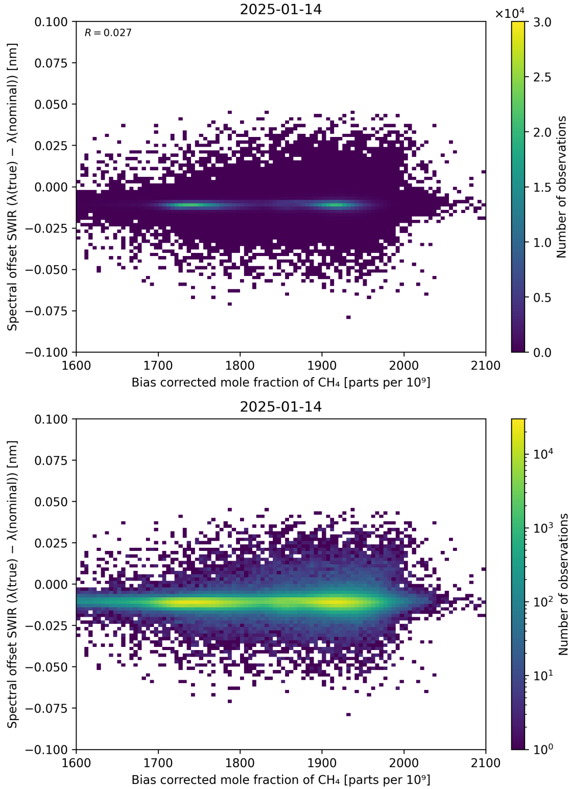
Figure 69: Scatter density plot of “Bias corrected mole fraction of \text{CH}_4 ” against “Spectral offset SWIR ( \lambda_{\text{true}} - \lambda_{\text{nominal}} )” for 2025-01-13 to 2025-01-15.
