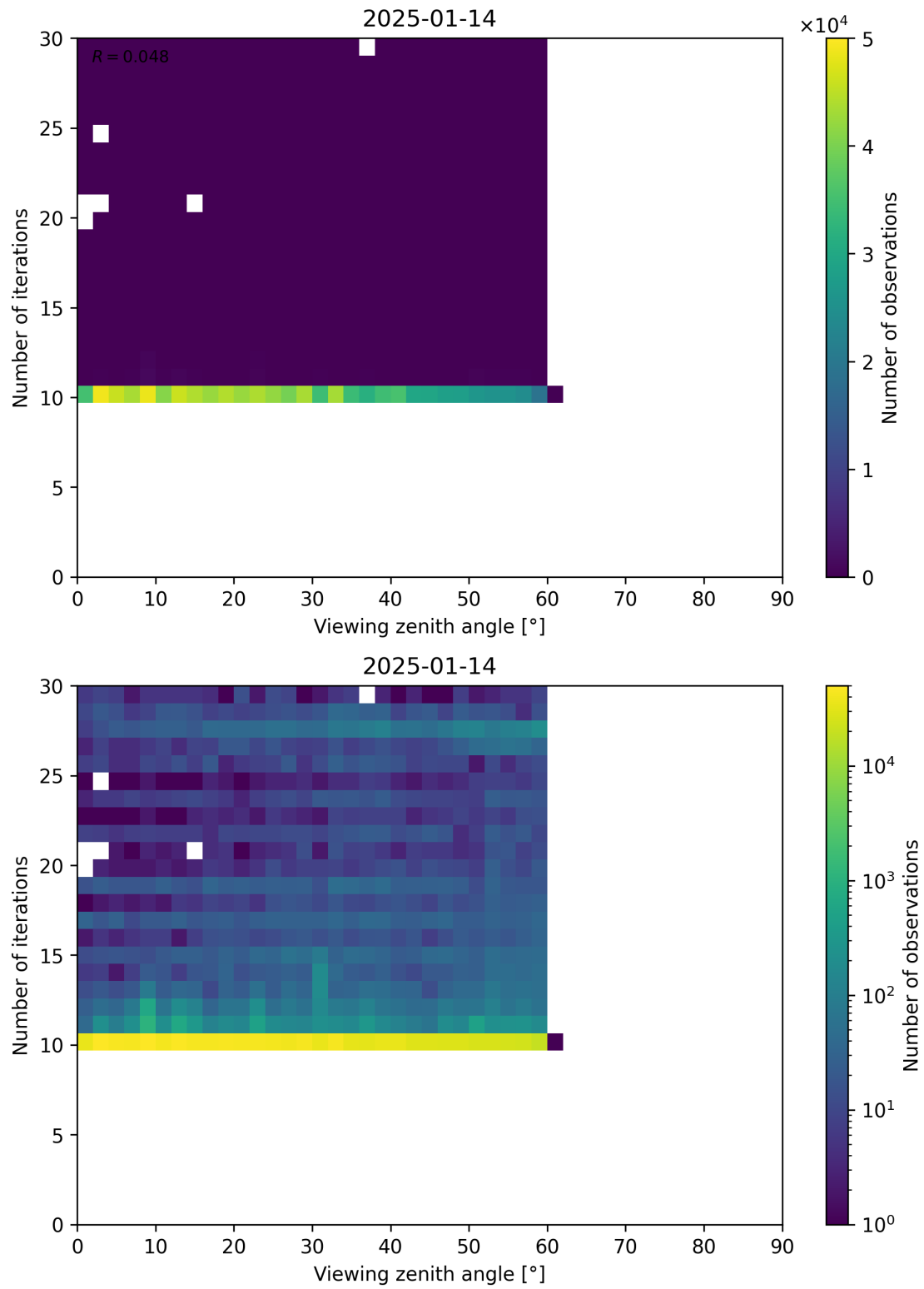
Figure 113: Scatter density plot of “Viewing zenith angle” against “Number of iterations” for 2025-01-13 to 2025-01-15.
