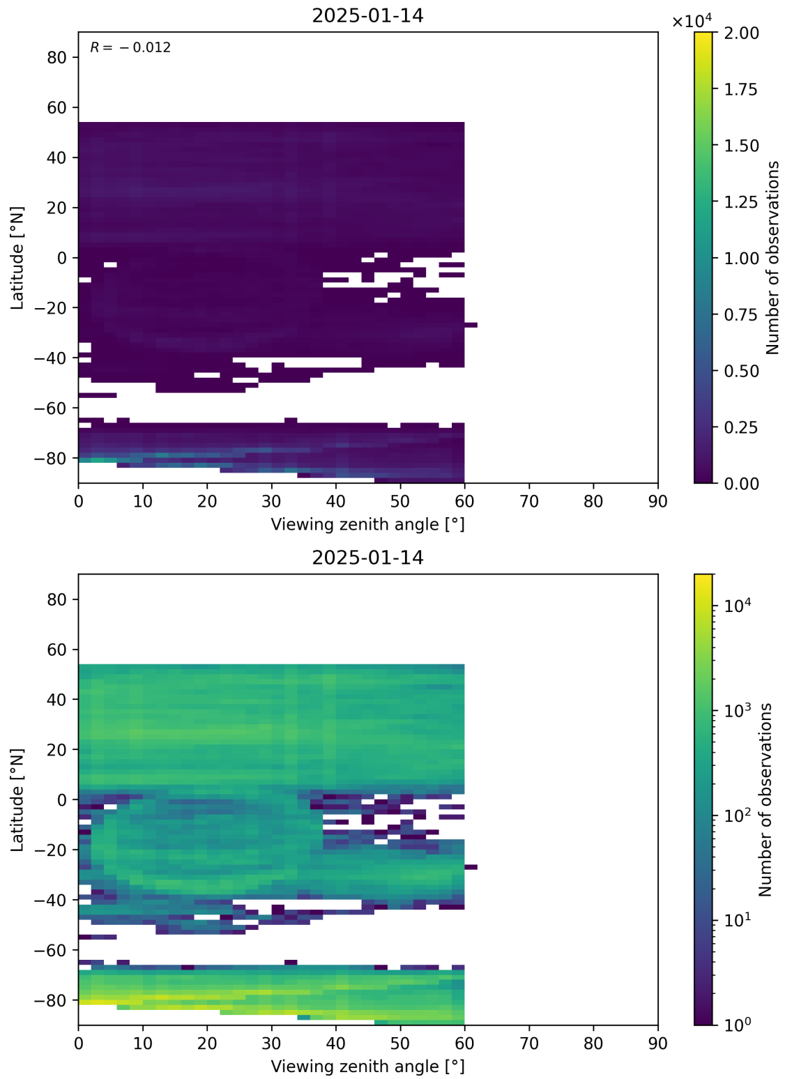
Figure 109: Scatter density plot of “Viewing zenith angle” against “Latitude” for 2025-01-13 to 2025-01-15.
