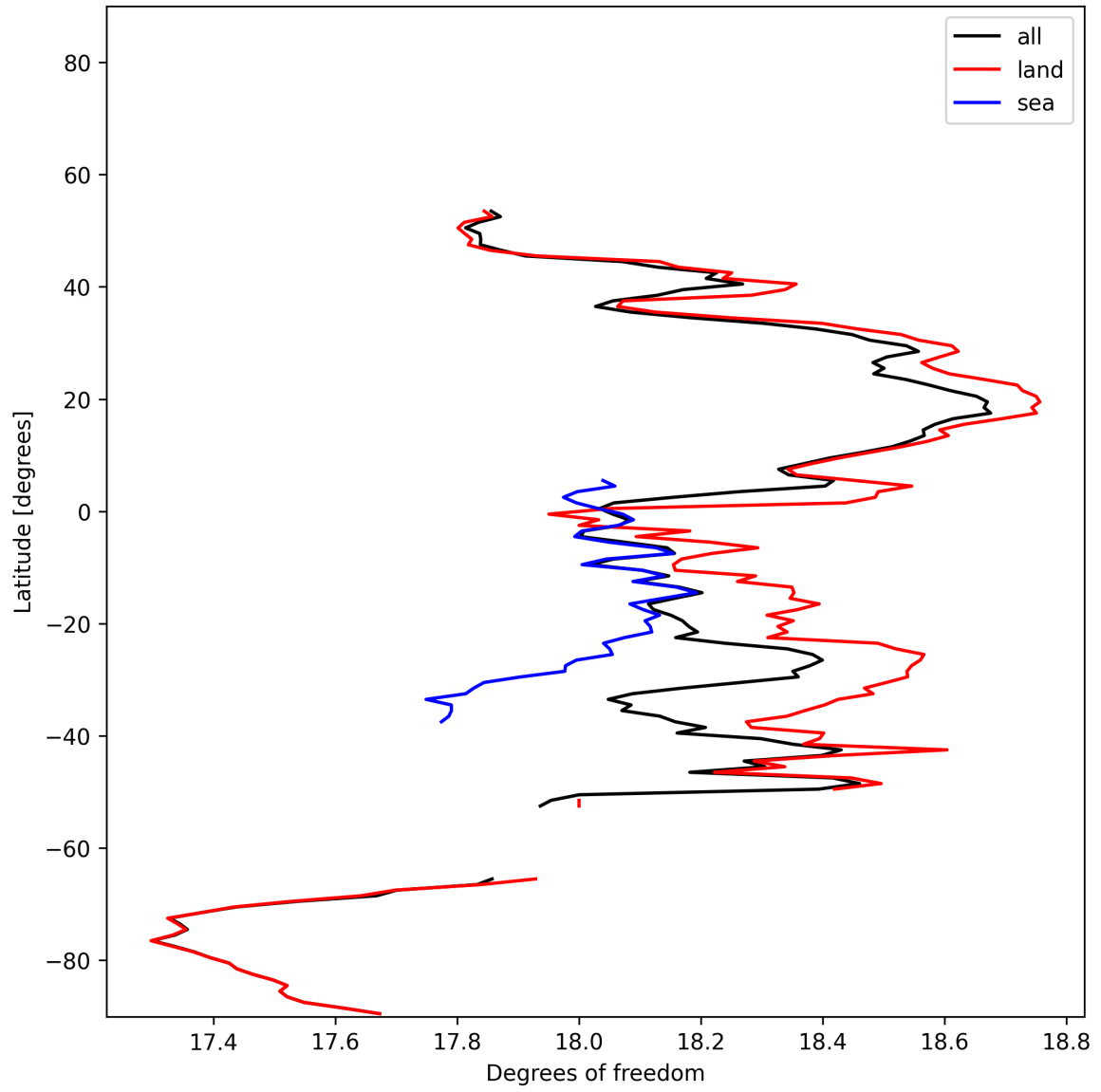
Figure 19: Zonal average of “Degrees of freedom” for 2025-01-13 to 2025-01-15.
