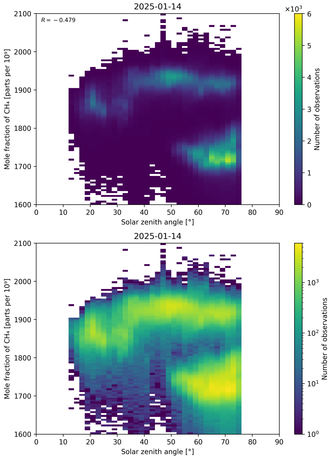
Figure 99: Scatter density plot of “Solar zenith angle” against “Mole fraction of CH 4 ” for 2025-01-13 to 2025-01-15.
