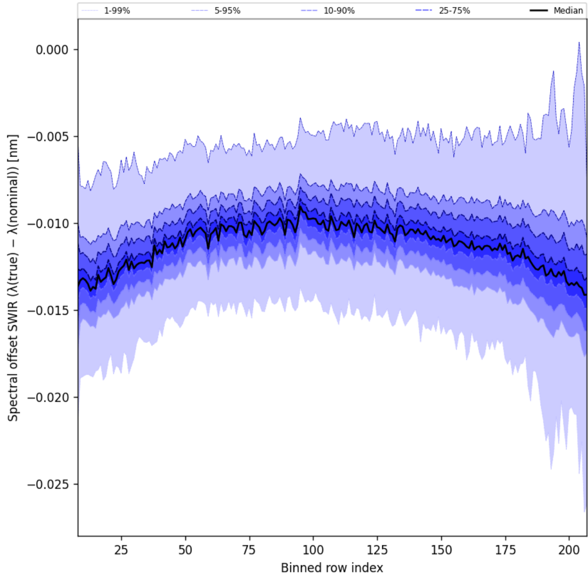
Figure 38: Along track statistics of “Spectral offset SWIR ( \lambda_{\text{true}} - \lambda_{\text{nominal}} )” for 2025-01-13 to 2025-01-15
