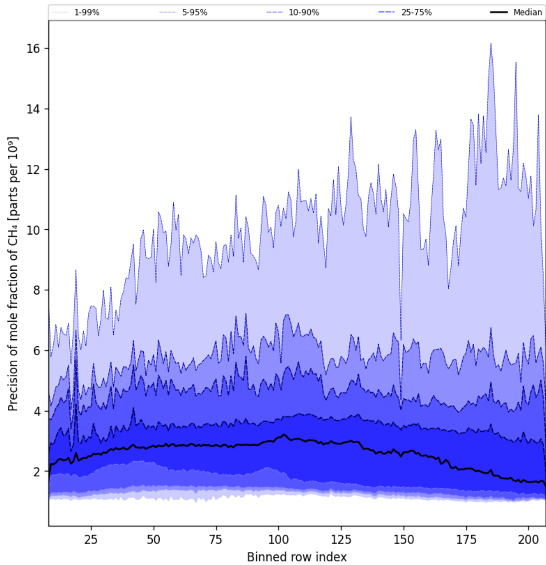
Figure 35: Along track statistics of “Precision of mole fraction of CH 4 ” for 2025-01-13 to 2025-01-15
