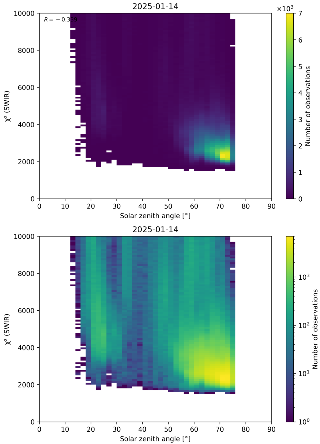
Figure 95: Scatter density plot of “Solar zenith angle” against “ \chi^2 (SWIR)” for 2025-01-13 to 2025-01-15.
