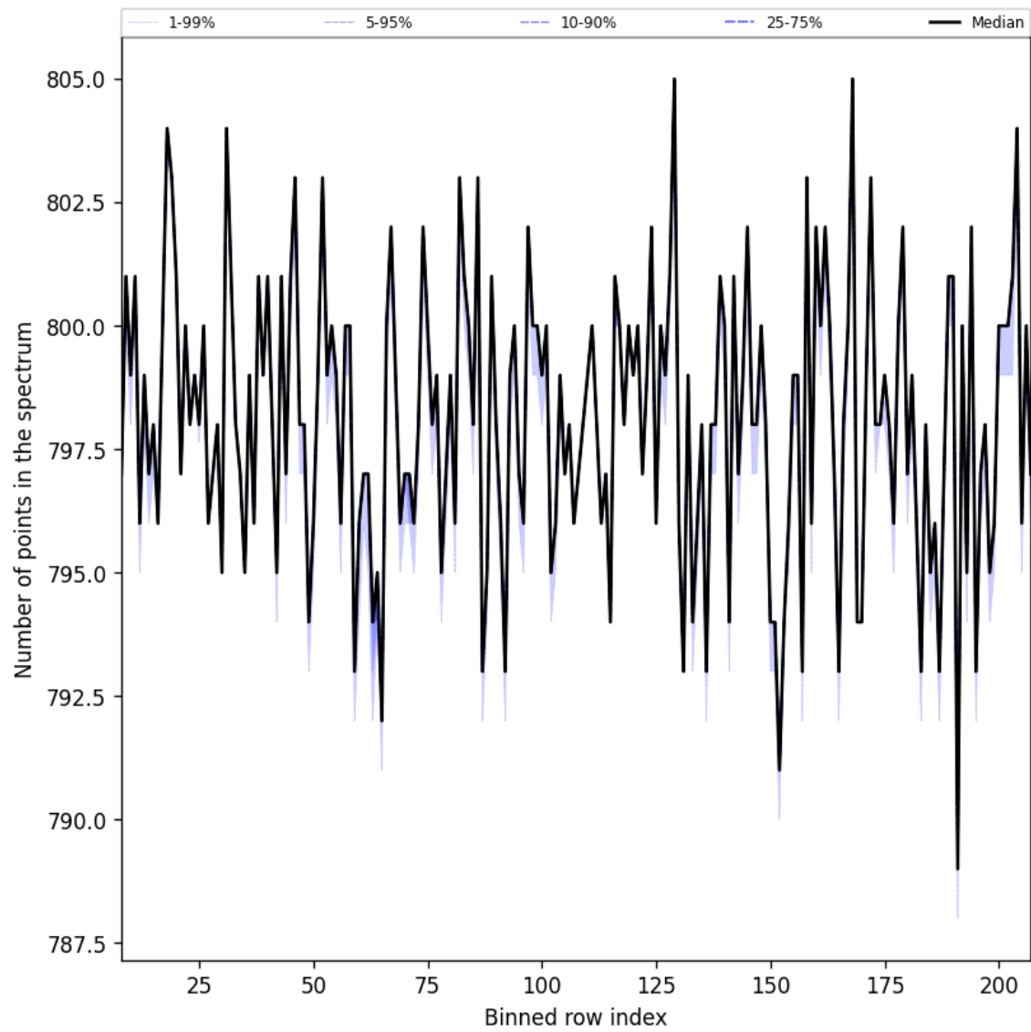
Figure 37: Along track statistics of “Number of points in the spectrum” for 2025-01-13 to 2025-01-15
