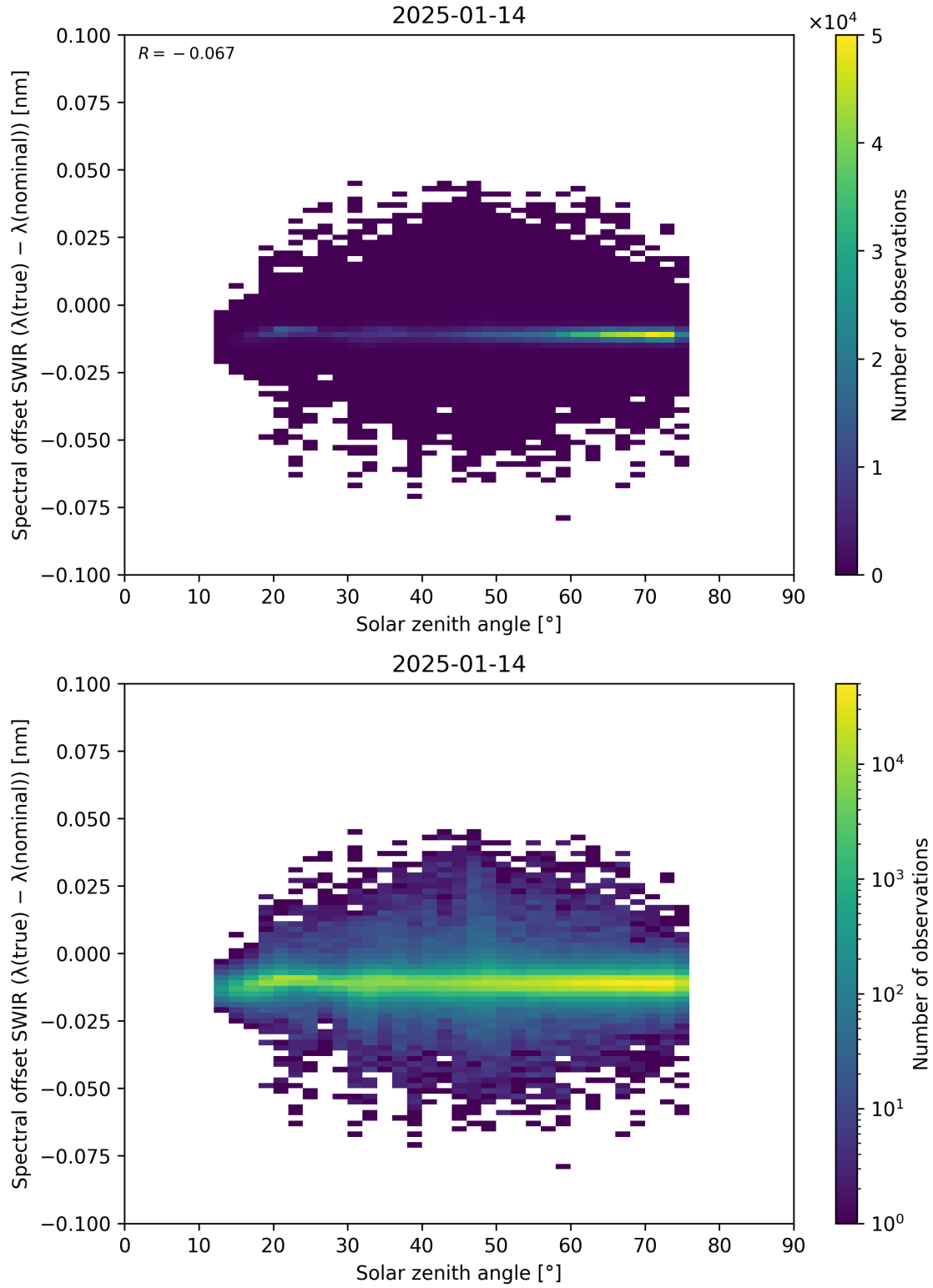
Figure 104: Scatter density plot of “Solar zenith angle” against “Spectral offset SWIR ( \lambda_{\text{true}} - \lambda_{\text{nominal}} )” for 2025-01-13 to 2025-01-15.
