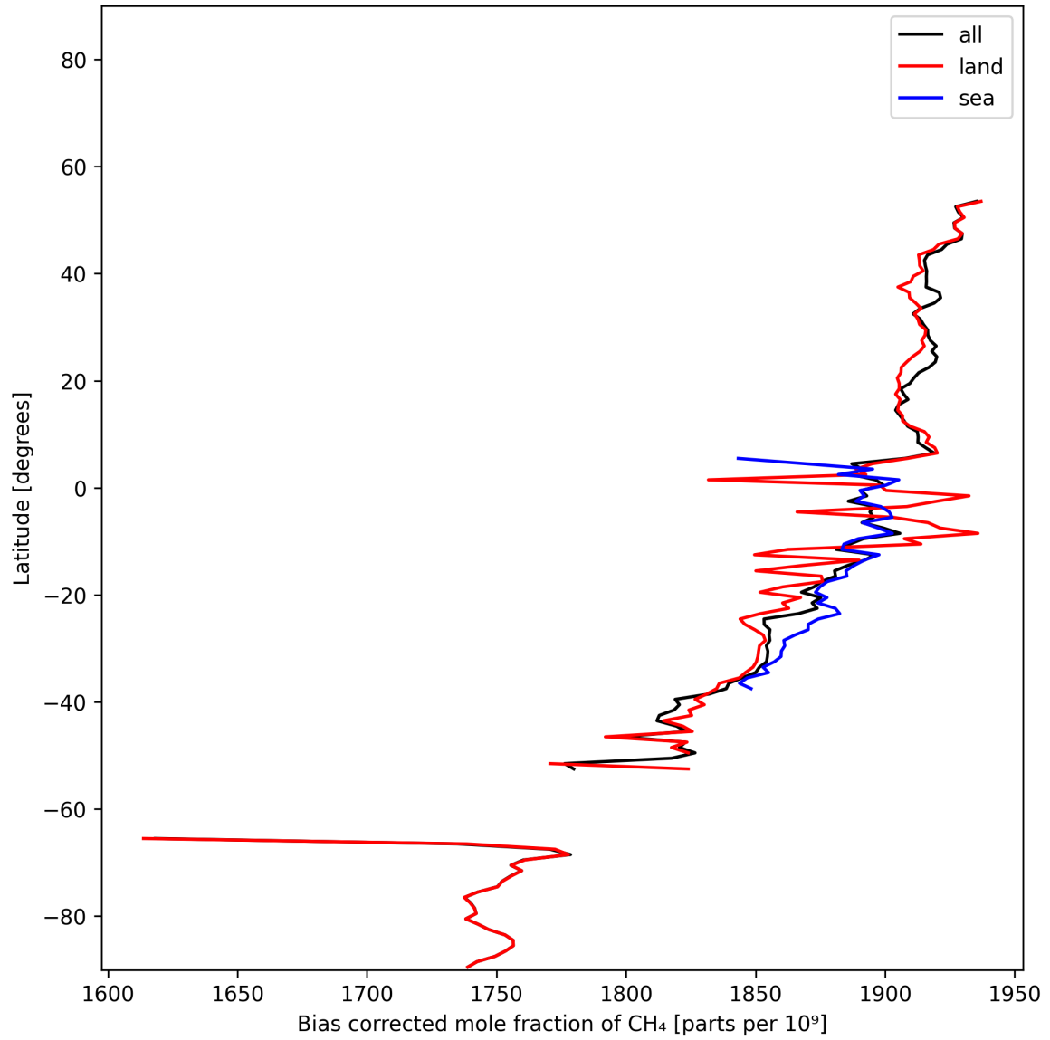
Figure 14: Zonal average of “Bias corrected mole fraction of CH 4 ” for 2025-01-13 to 2025-01-15.
