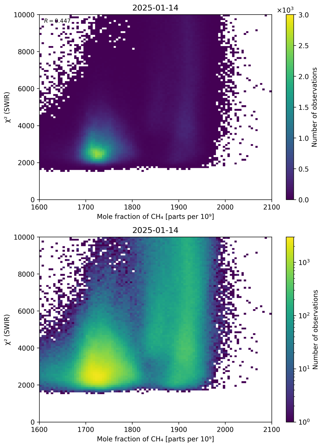
Figure 71: Scatter density plot of “Mole fraction of \text{CH}_4 ” against “ \chi^2 (SWIR)” for 2025-01-13 to 2025-01-15.
