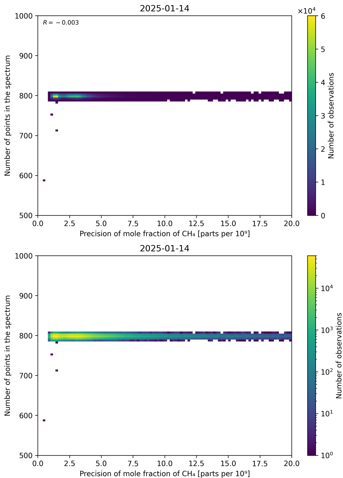
Figure 84: Scatter density plot of “Precision of mole fraction of CH 4 ” against “Number of points in the spectrum” for 2025-01-13 to 2025-01-15.
