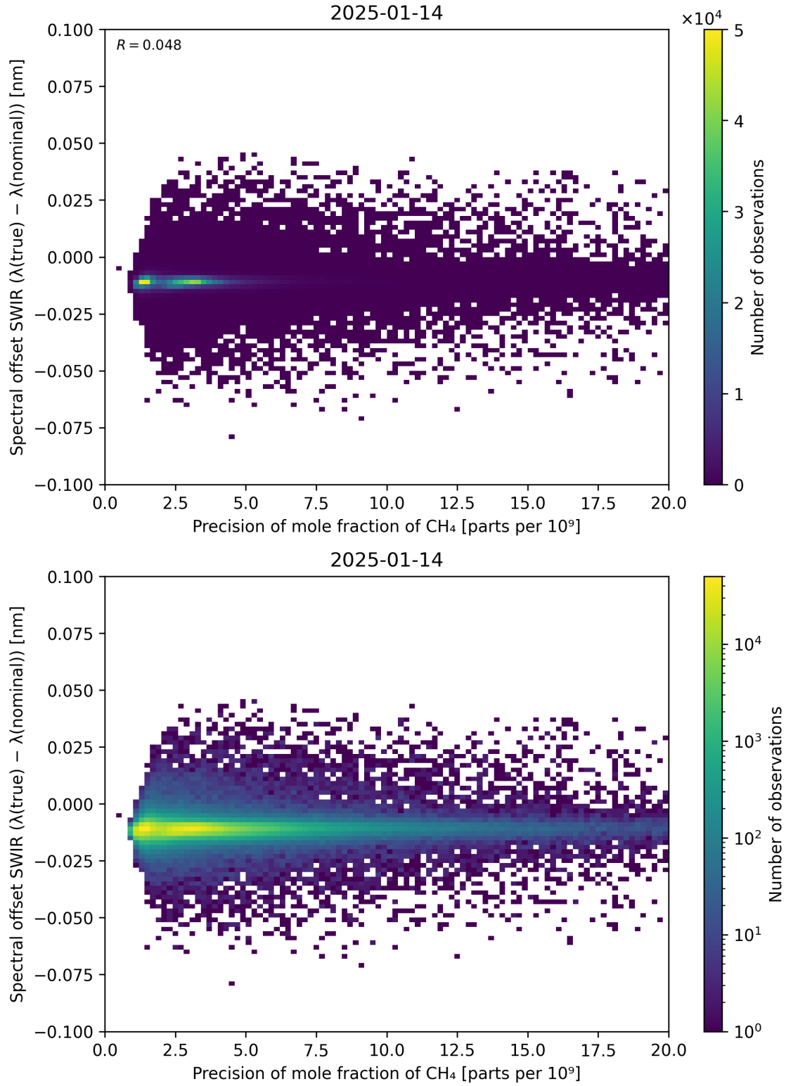
Figure 85: Scatter density plot of “Precision of mole fraction of CH 4 ” against “Spectral offset SWIR ( \lambda_{\text{true}} - \lambda_{\text{nominal}} )” for 2025-01-13 to 2025-01-15.
