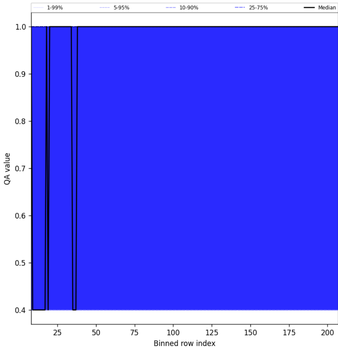
Figure 33: Along track statistics of “QA value” for 2025-01-13 to 2025-01-15
