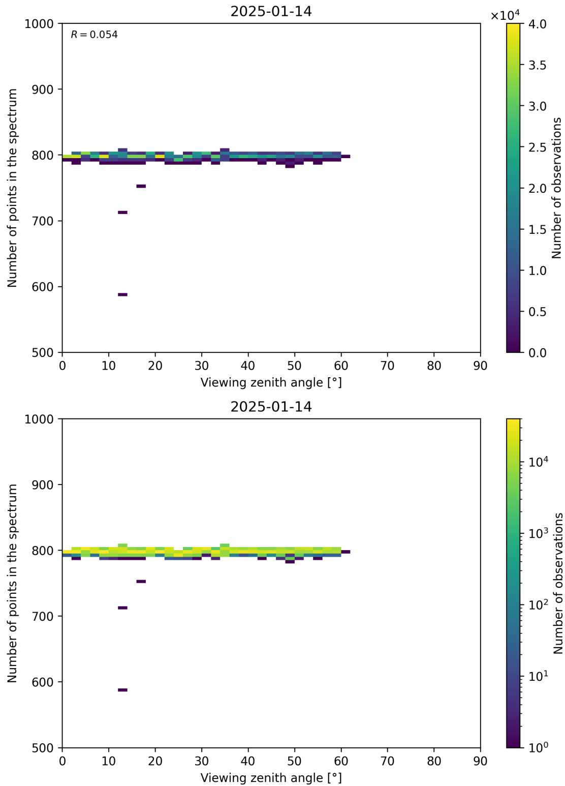
Figure 114: Scatter density plot of “Viewing zenith angle” against “Number of points in the spectrum” for 2025-01-13 to 2025-01-15.
