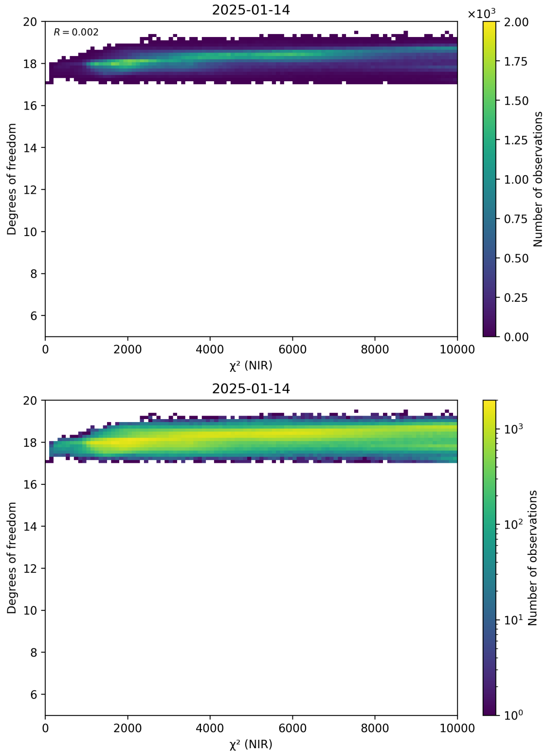
Figure 44: Scatter density plot of “ \chi^2 (NIR)” against “Degrees of freedom” for 2025-01-13 to 2025-01-15.
