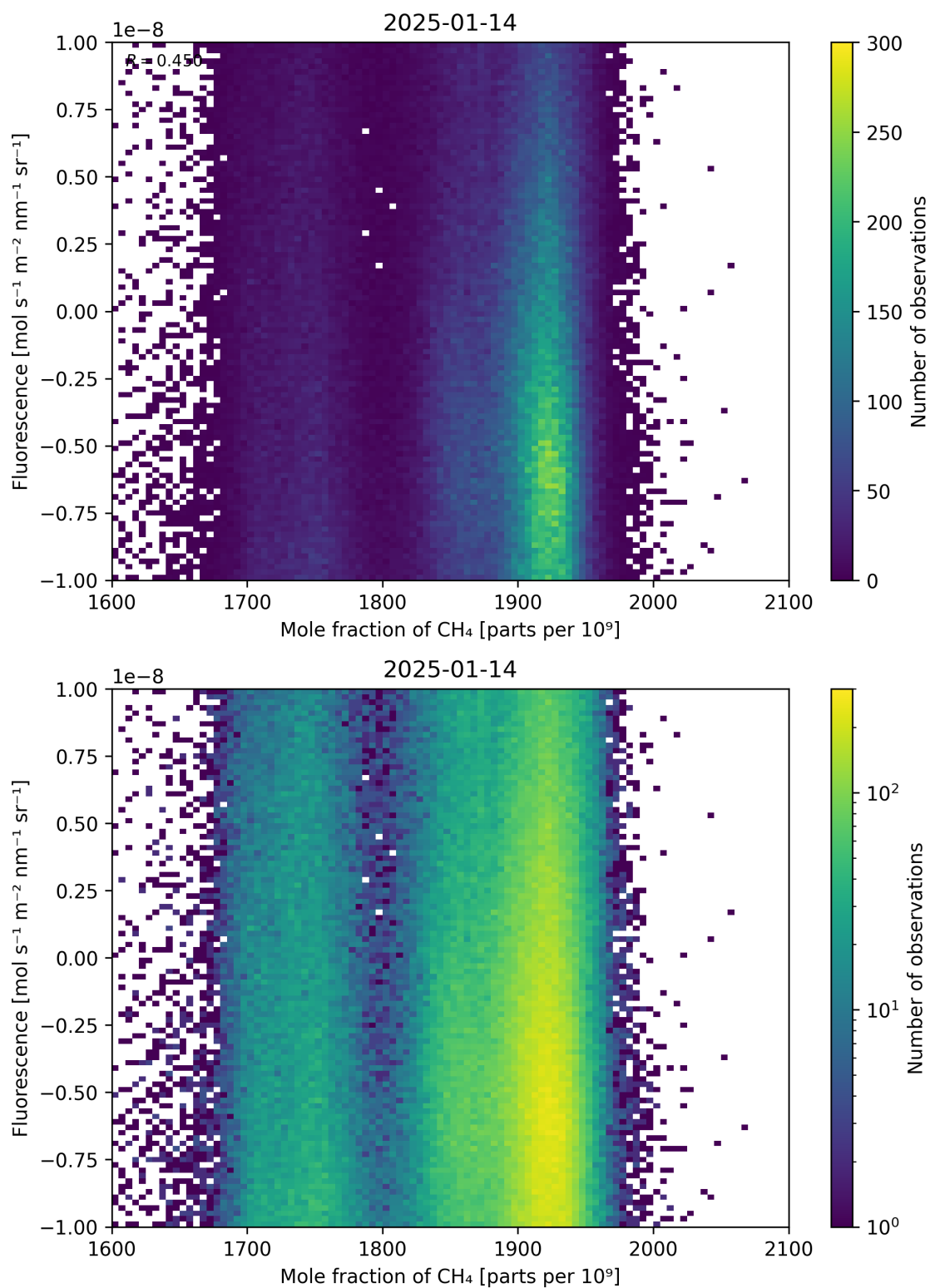
Figure 73: Scatter density plot of “Mole fraction of \text{CH}_4 ” against “Fluorescence” for 2025-01-13 to 2025-01-15.
