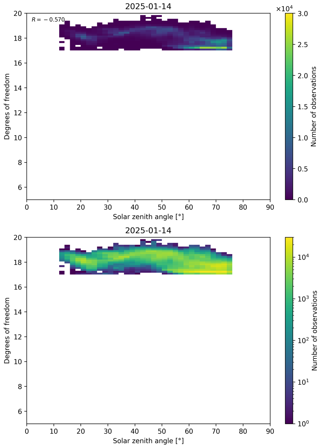
Figure 96: Scatter density plot of “Solar zenith angle” against “Degrees of freedom” for 2025-01-13 to 2025-01-15.
