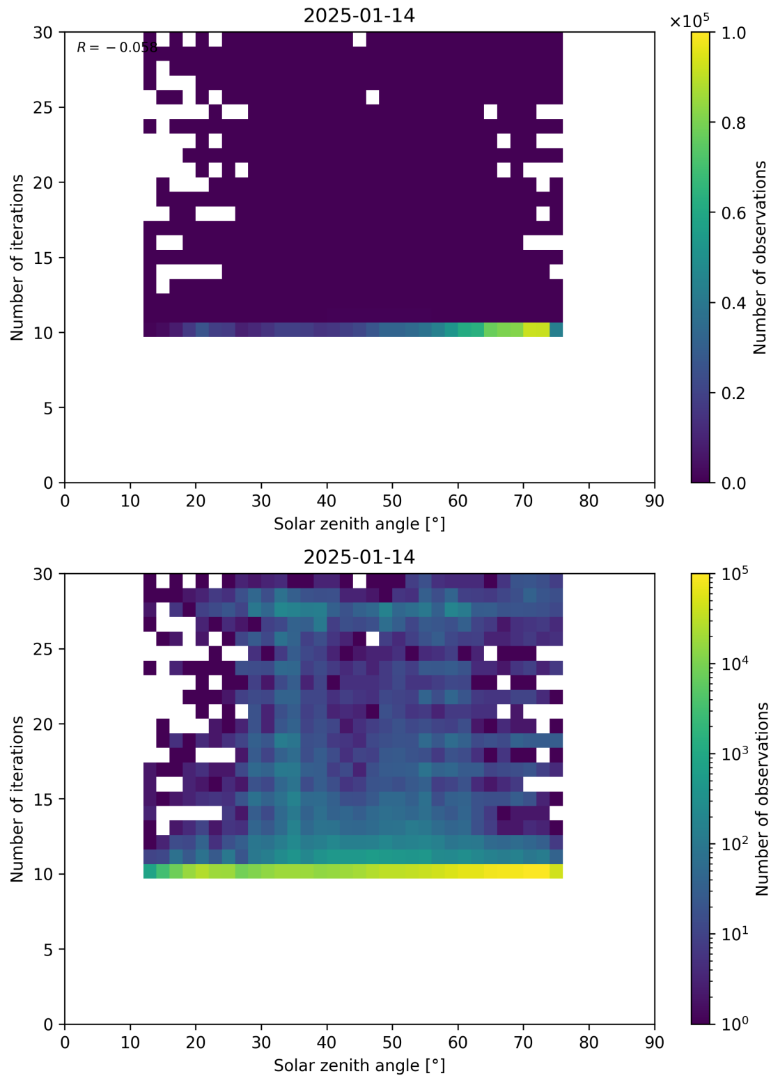
Figure 102: Scatter density plot of “Solar zenith angle” against “Number of iterations” for 2025-01-13 to 2025-01-15.
