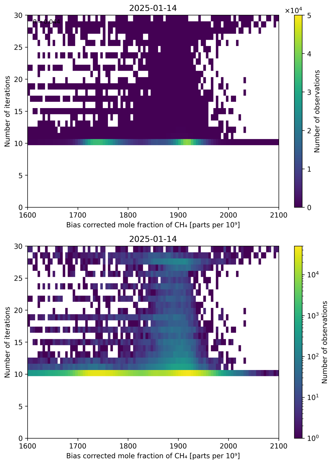
Figure 67: Scatter density plot of “Bias corrected mole fraction of CH 4 ” against “Number of iterations” for 2025-01-13 to 2025-01-15.
