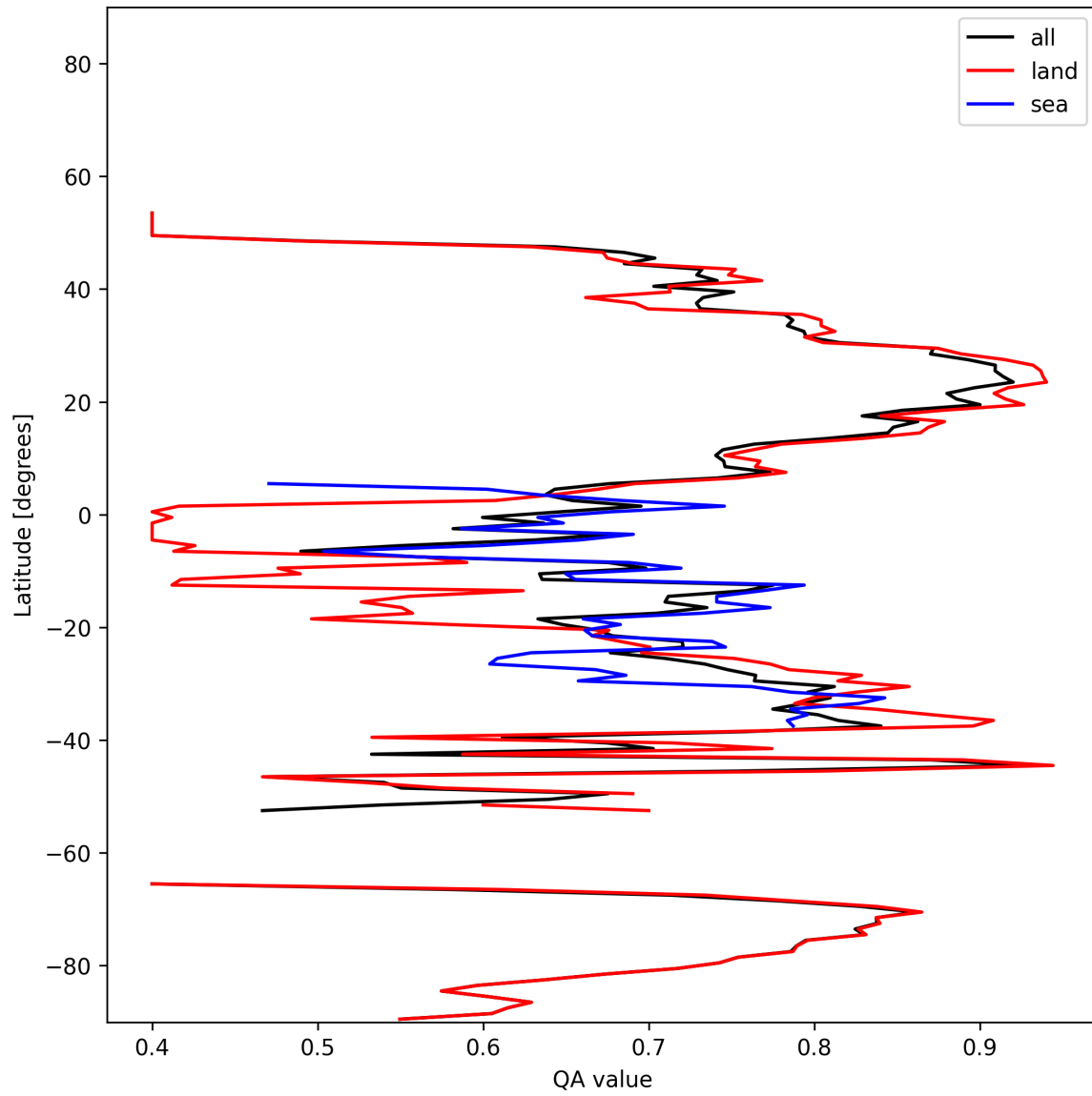
Figure 11: Zonal average of “QA value” for 2025-01-13 to 2025-01-15.
