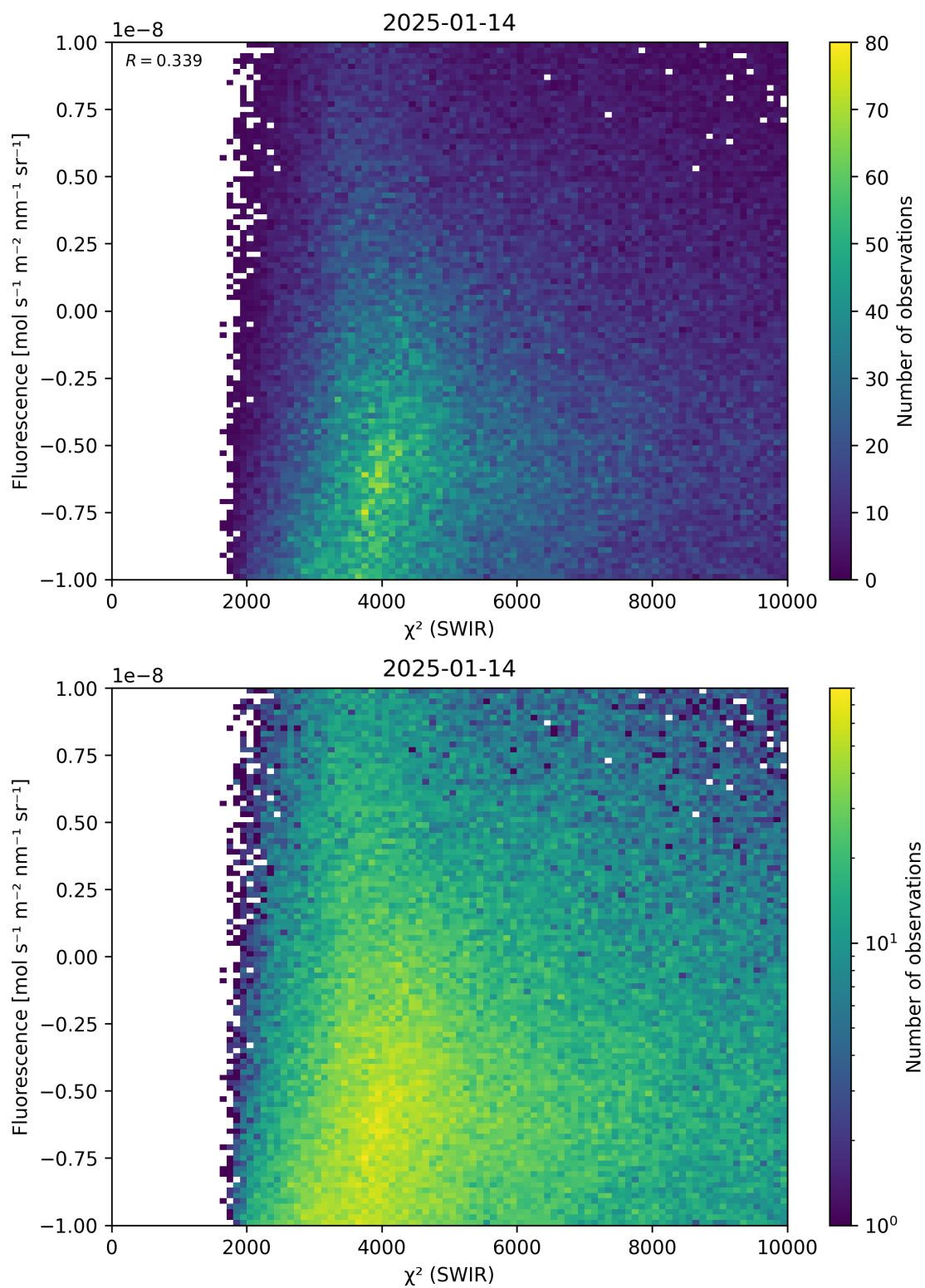
Figure 49: Scatter density plot of “ \chi^2 (SWIR)” against “Fluorescence” for 2025-01-13 to 2025-01-15.
