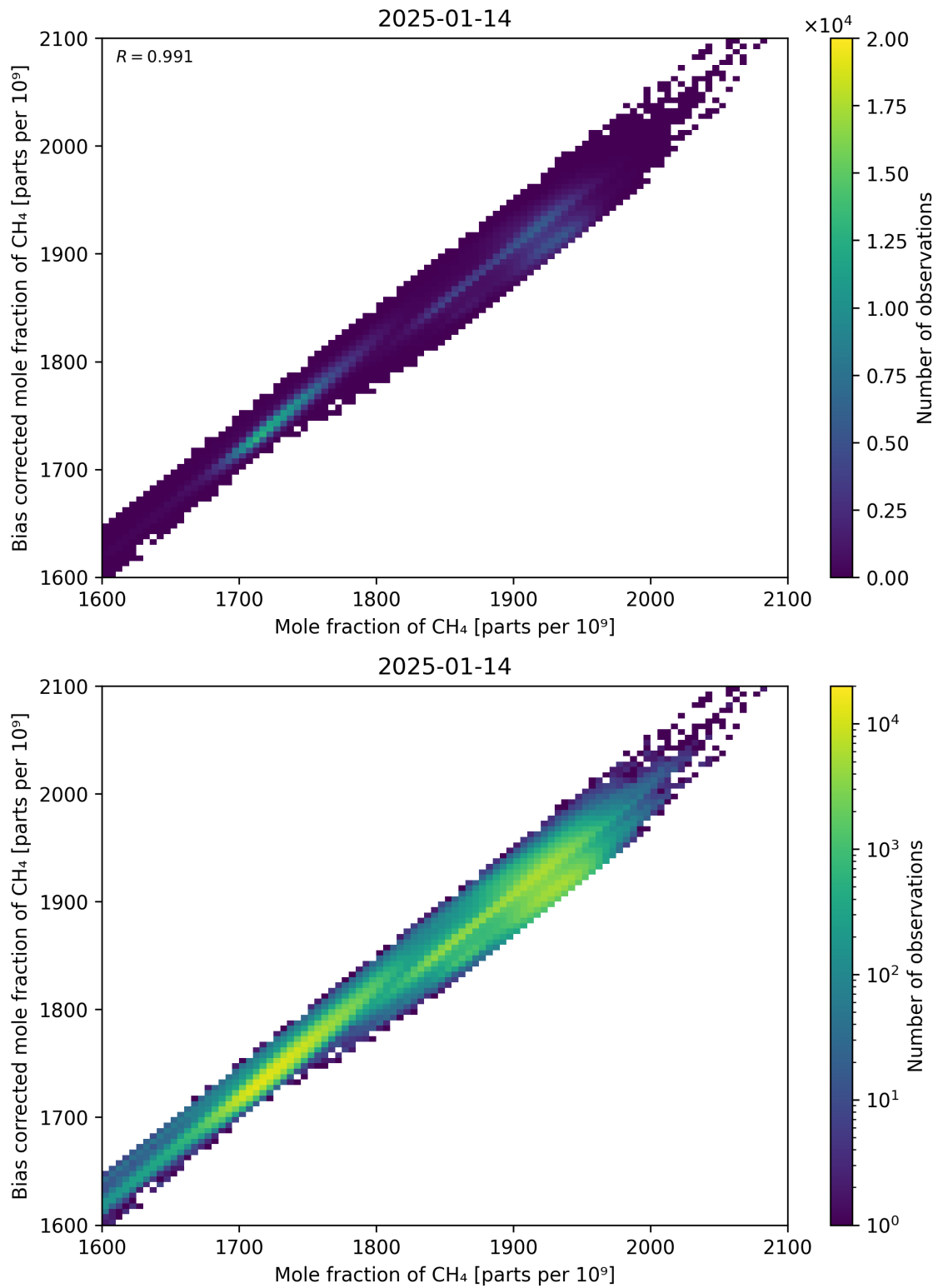
Figure 74: Scatter density plot of “Mole fraction of CH 4 ” against “Bias corrected mole fraction of CH 4 ” for 2025-01-13 to 2025-01-15.
