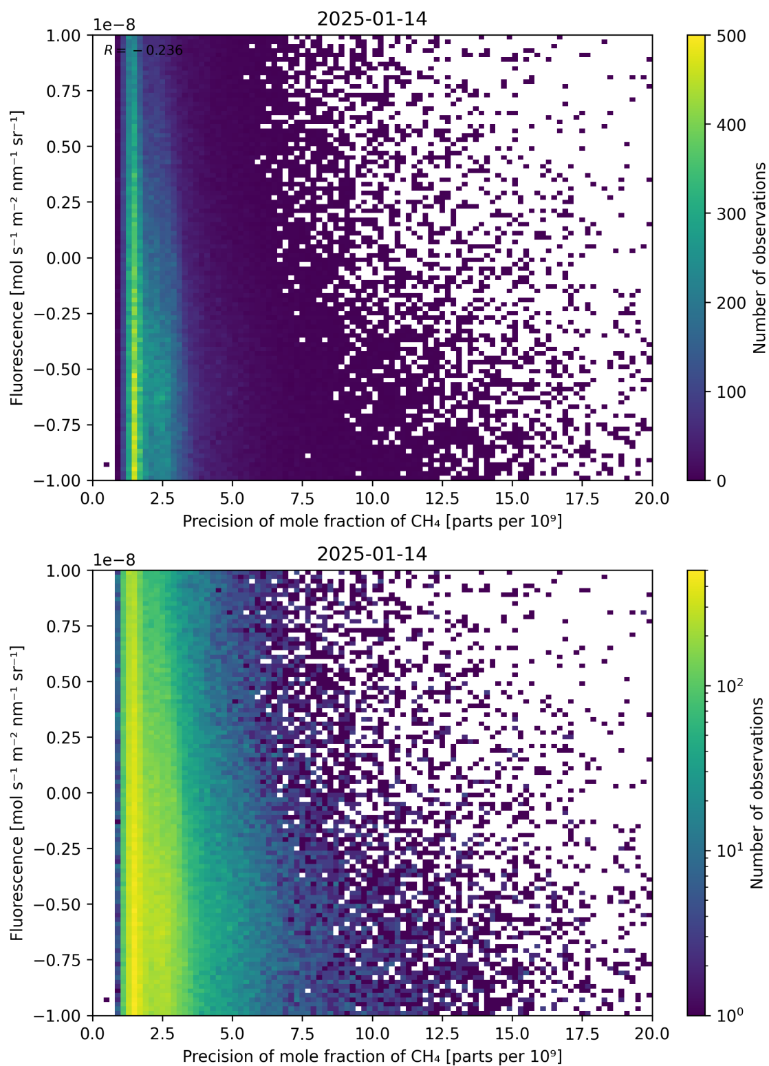
Figure 81: Scatter density plot of “Precision of mole fraction of \text{CH}_4 ” against “Fluorescence” for 2025-01-13 to 2025-01-15.
