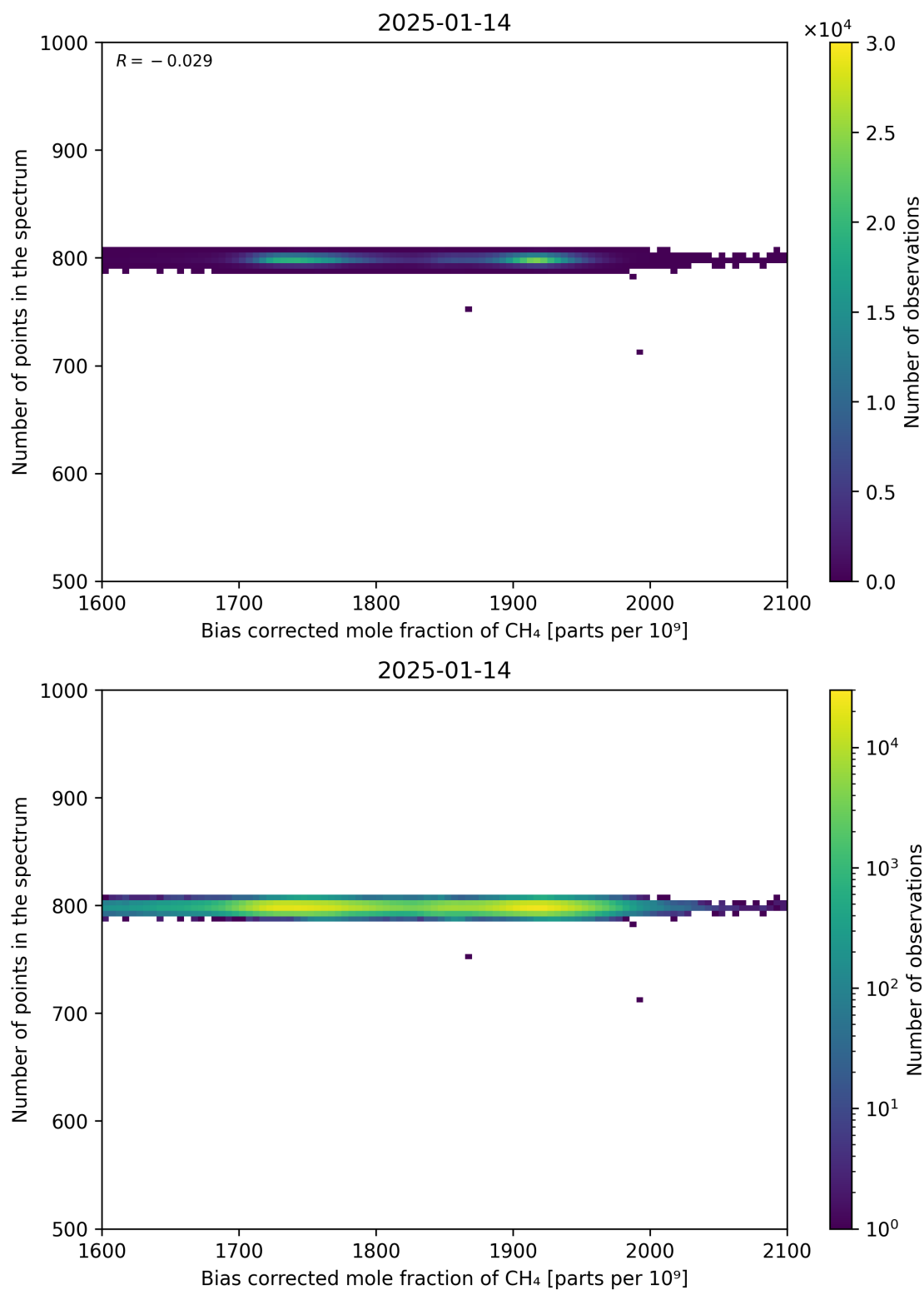
Figure 68: Scatter density plot of “Bias corrected mole fraction of CH 4 ” against “Number of points in the spectrum” for 2025-01-13 to 2025-01-15.
