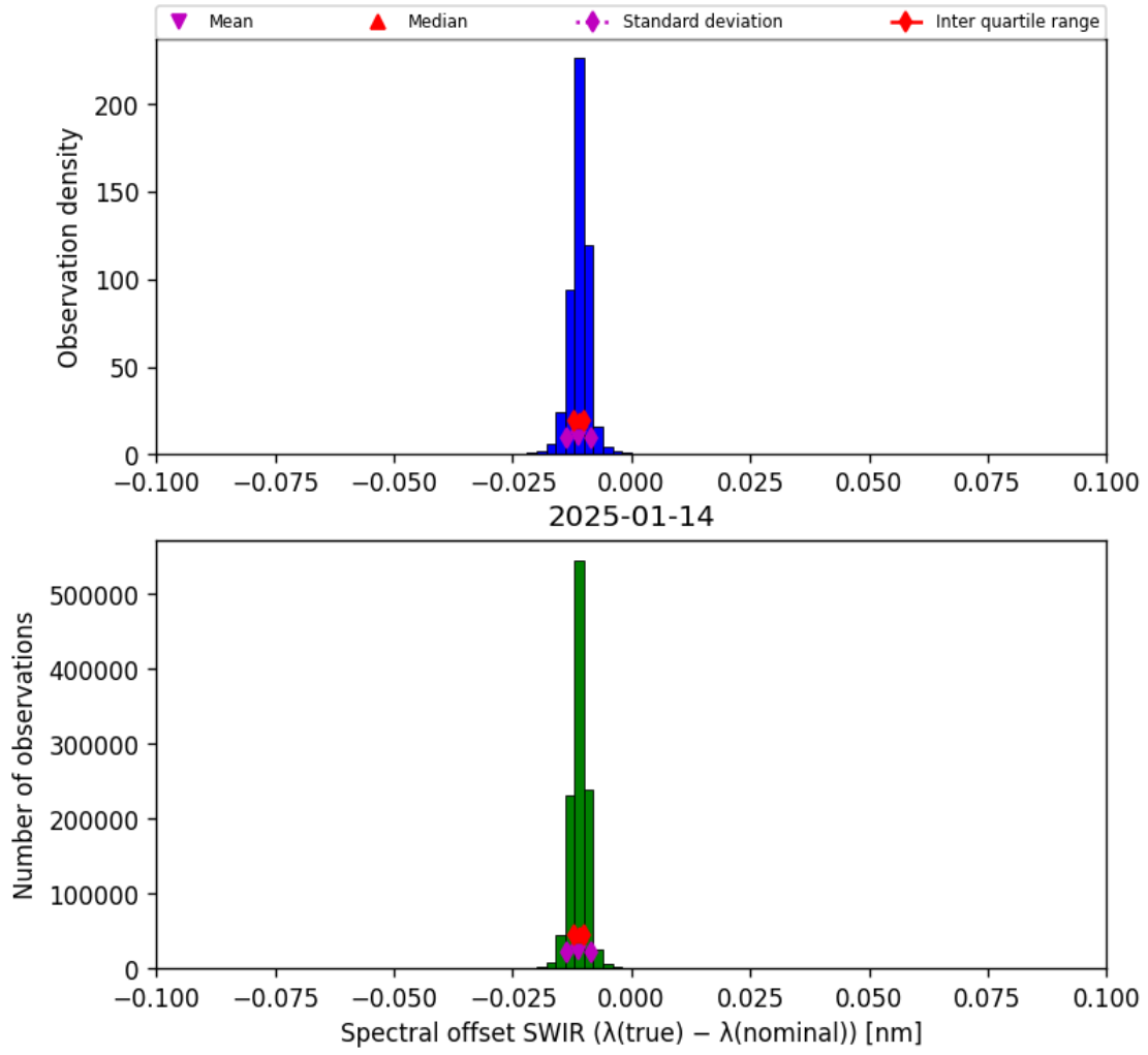
Figure 27: Histogram of “Spectral offset SWIR ( \lambda_{\text{true}} - \lambda_{\text{nominal}} )” for 2025-01-13 to 2025-01-15
