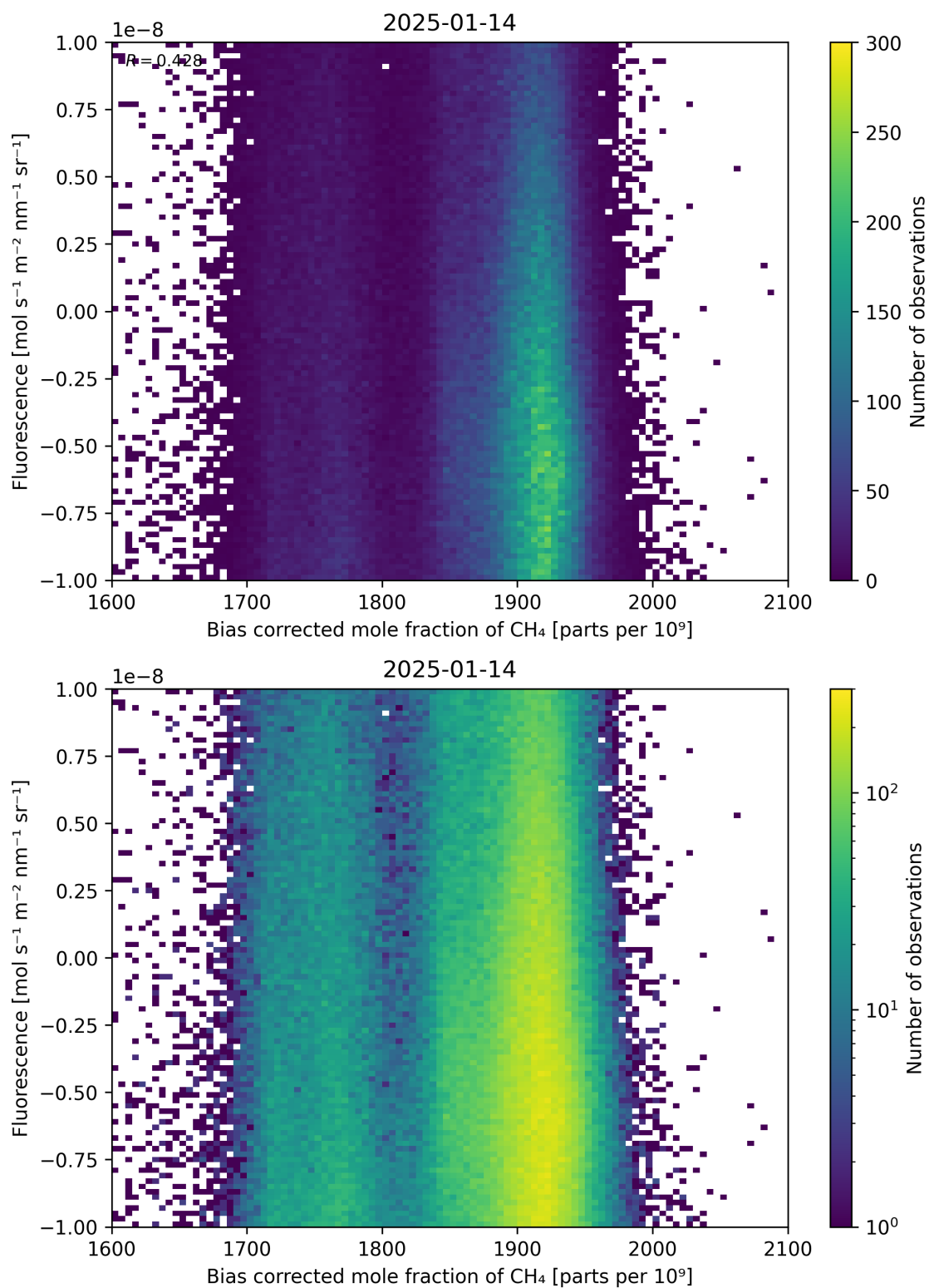
Figure 66: Scatter density plot of “Bias corrected mole fraction of \text{CH}_4 ” against “Fluorescence” for 2025-01-13 to 2025-01-15.
