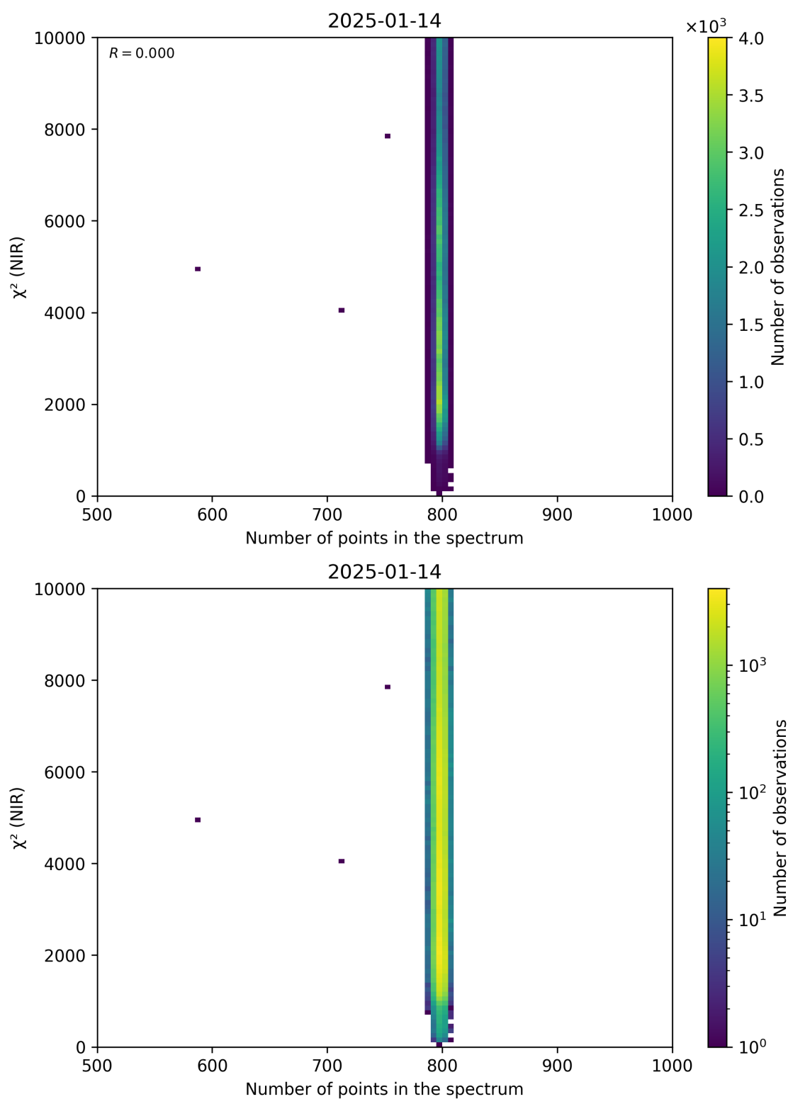
Figure 88: Scatter density plot of “Number of points in the spectrum” against “ \chi^2 (NIR)” for 2025-01-13 to 2025-01-15.
