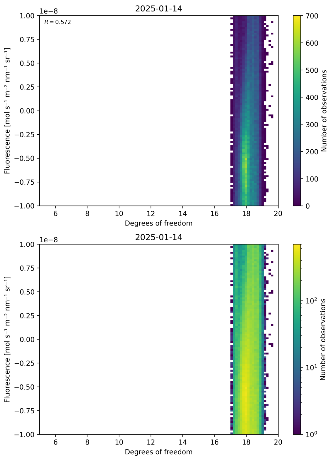
Figure 51: Scatter density plot of “Degrees of freedom” against “Fluorescence” for 2025-01-13 to 2025-01-15.
