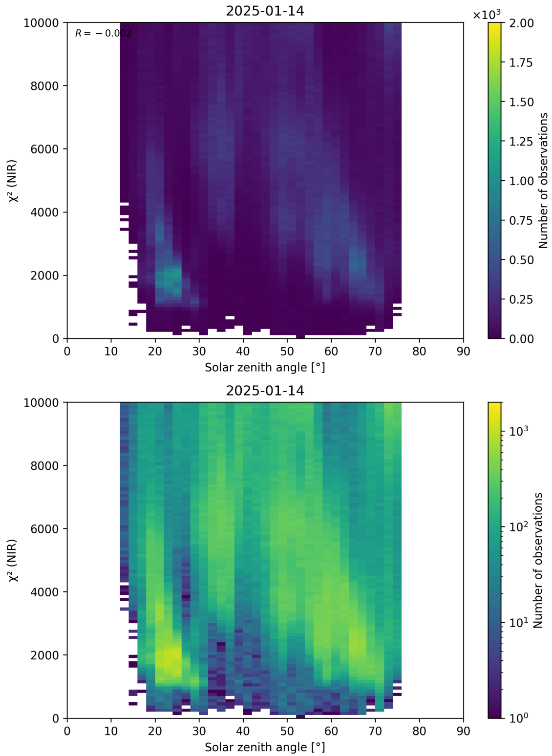
Figure 94: Scatter density plot of “Solar zenith angle” against “ \chi^2 (NIR)” for 2025-01-13 to 2025-01-15.
