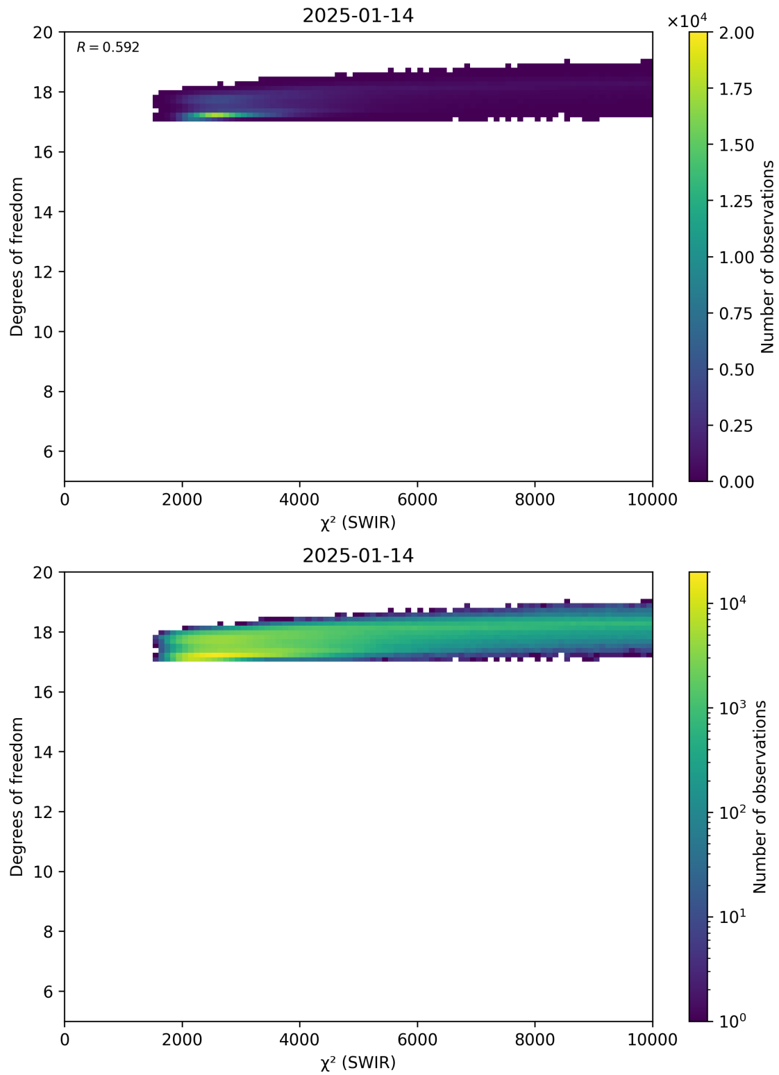
Figure 48: Scatter density plot of “ \chi^2 (SWIR)” against “Degrees of freedom” for 2025-01-13 to 2025-01-15.
