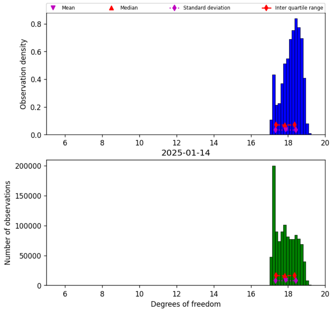
Figure 30: Histogram of “Degrees of freedom” for 2025-01-13 to 2025-01-15
