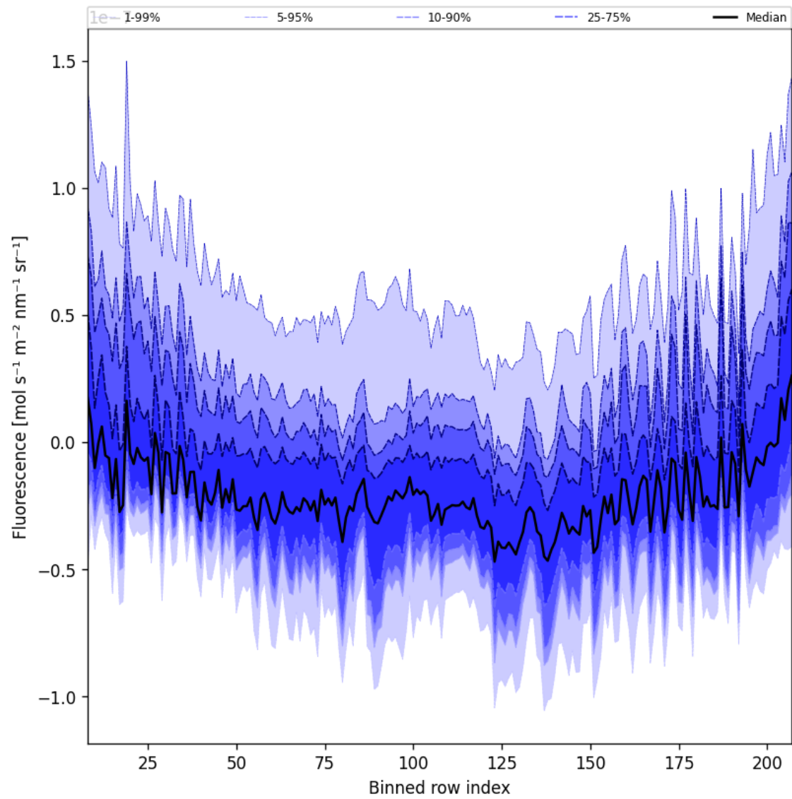
Figure 43: Along track statistics of “Fluorescence” for 2025-01-13 to 2025-01-15
