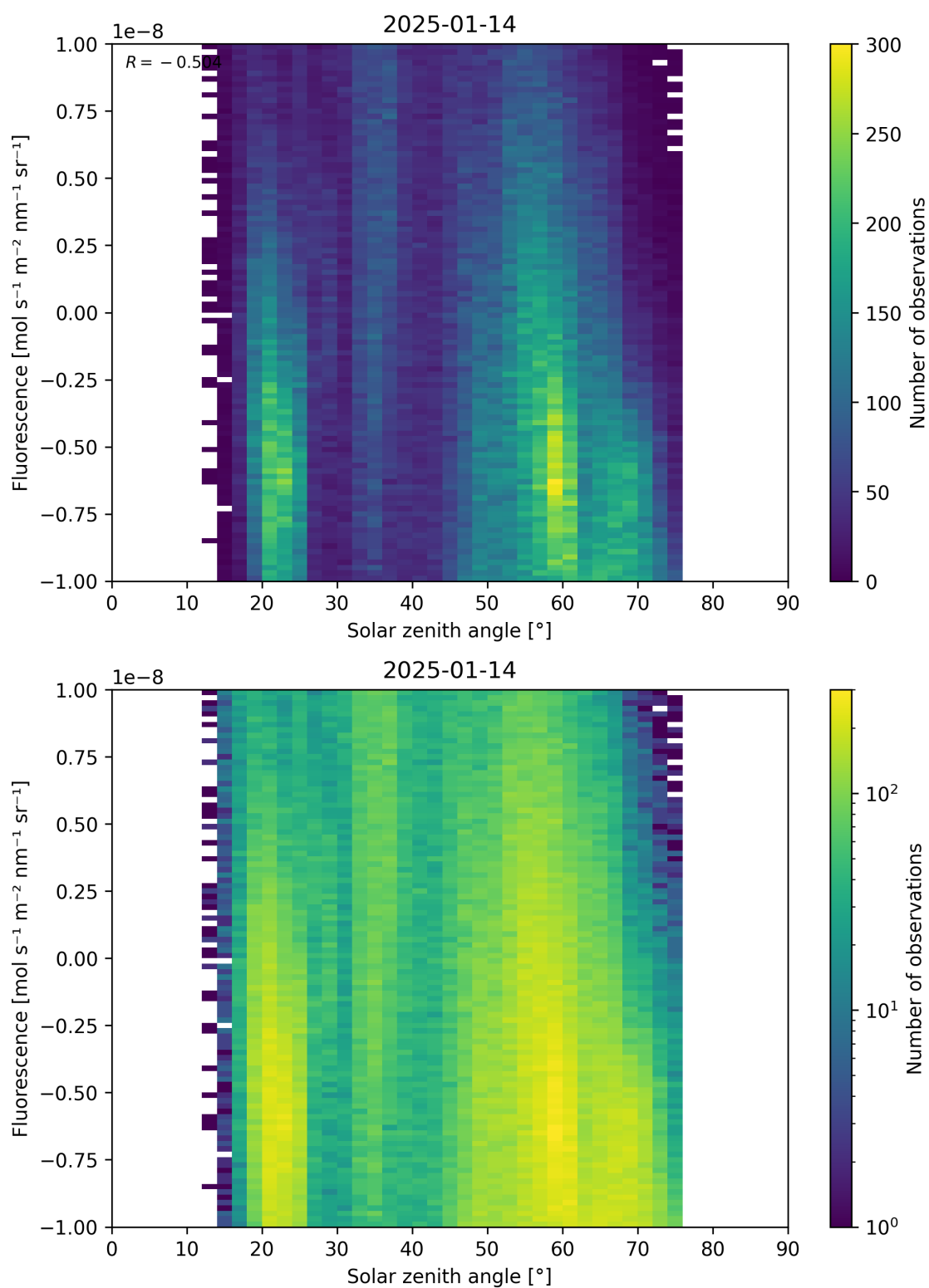
Figure 97: Scatter density plot of “Solar zenith angle” against “Fluorescence” for 2025-01-13 to 2025-01-15.
