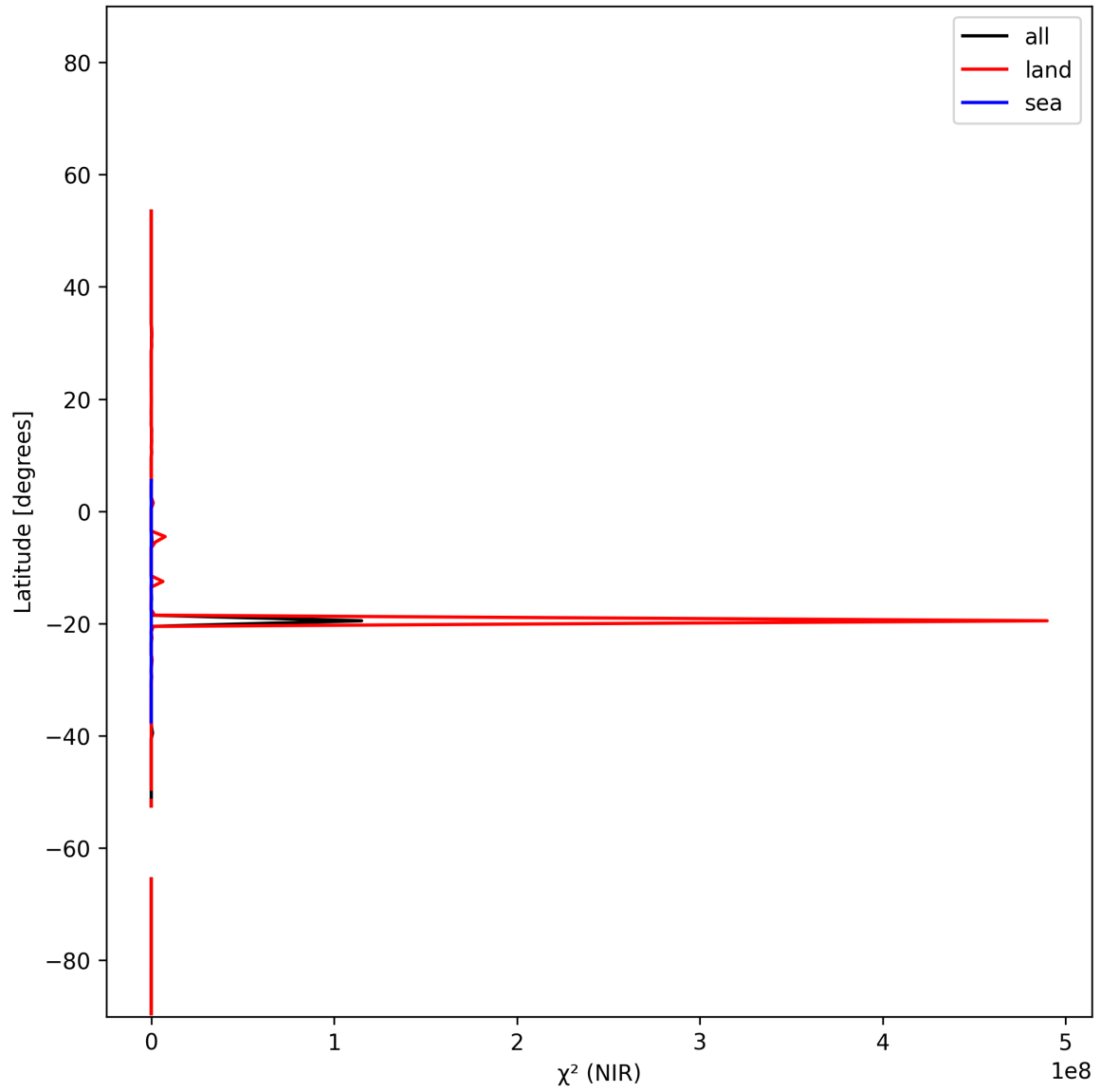
Figure 18: Zonal average of “ \chi^2 (NIR)” for 2025-01-13 to 2025-01-15.
