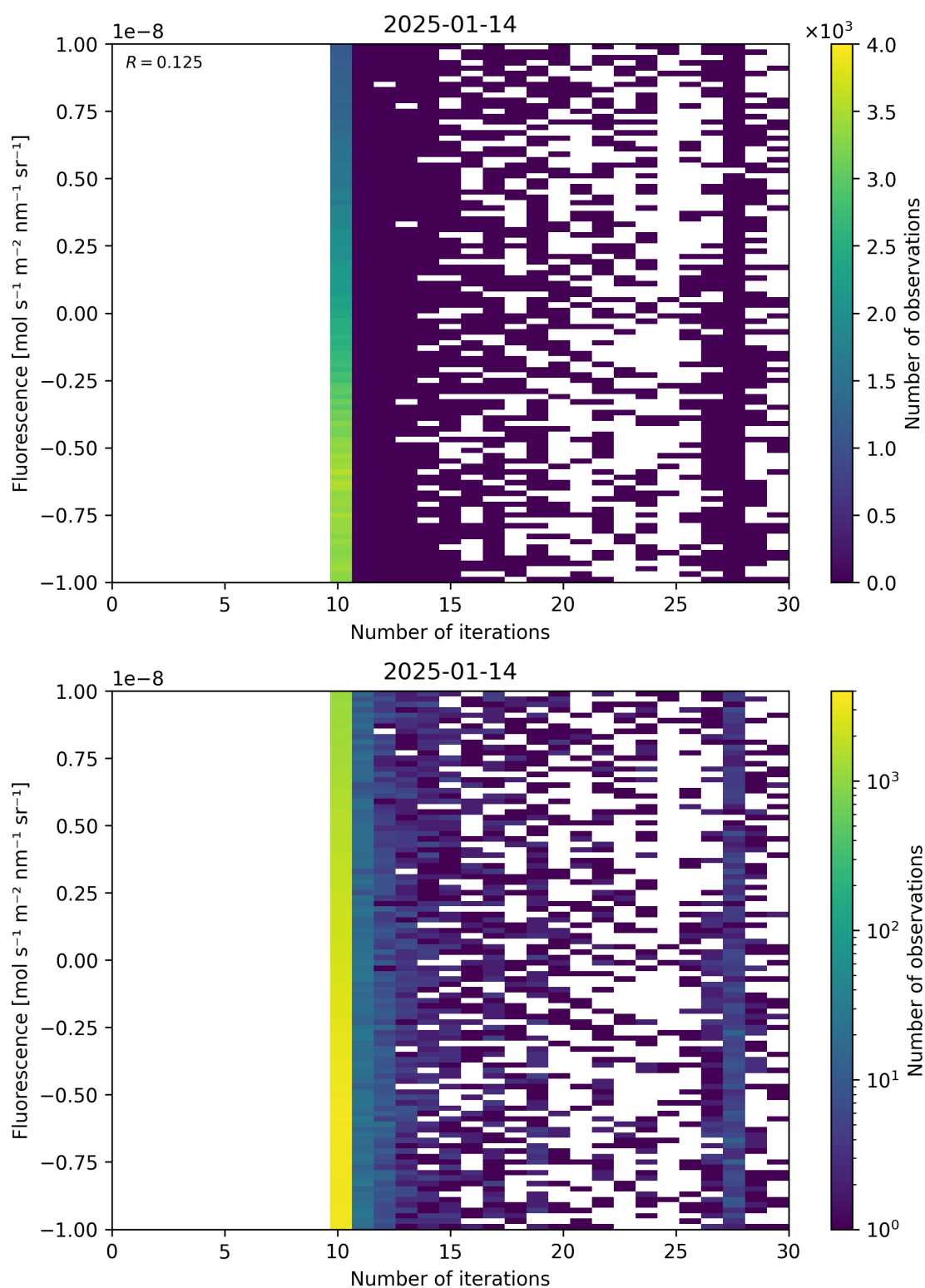
Figure 87: Scatter density plot of “Number of iterations” against “Fluorescence” for 2025-01-13 to 2025-01-15.
