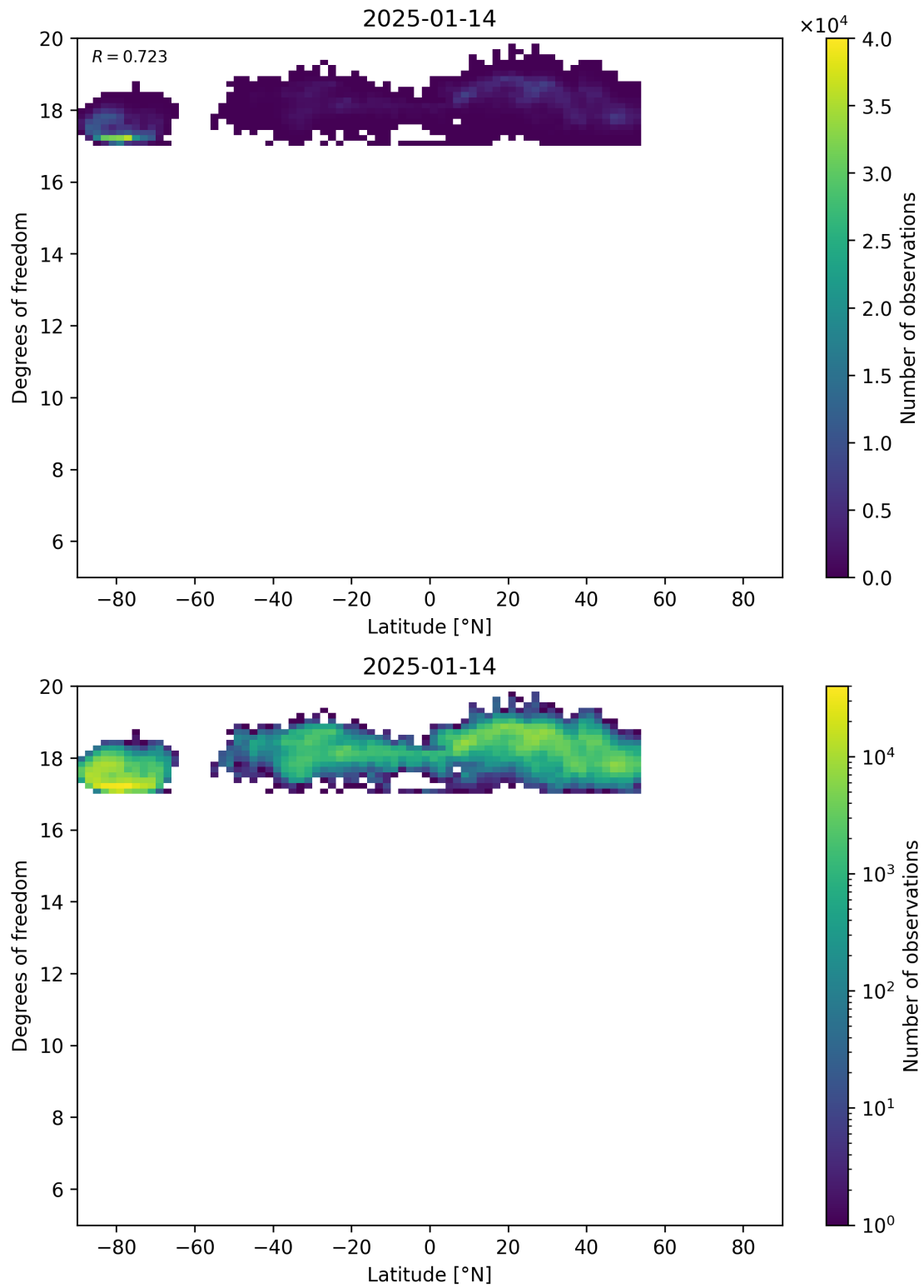
Figure 55: Scatter density plot of “Latitude” against “Degrees of freedom” for 2025-01-13 to 2025-01-15.
