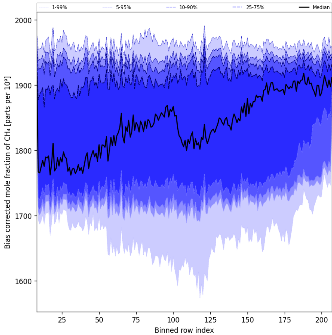
Figure 36: Along track statistics of “Bias corrected mole fraction of CH 4 ” for 2025-01-13 to 2025-01-15
