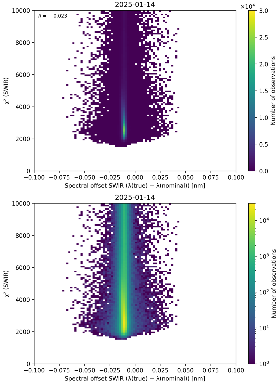
Figure 118: Scatter density plot of “Spectral offset SWIR ( \lambda_{\text{true}} - \lambda_{\text{nominal}} )” against “ \chi^2 (SWIR)” for 2025-01-13 to 2025-01-15.
