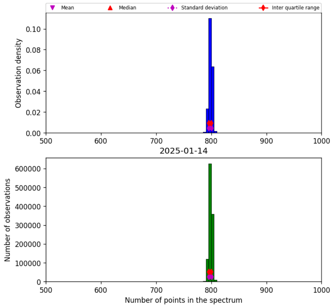
Figure 26: Histogram of “Number of points in the spectrum” for 2025-01-13 to 2025-01-15
