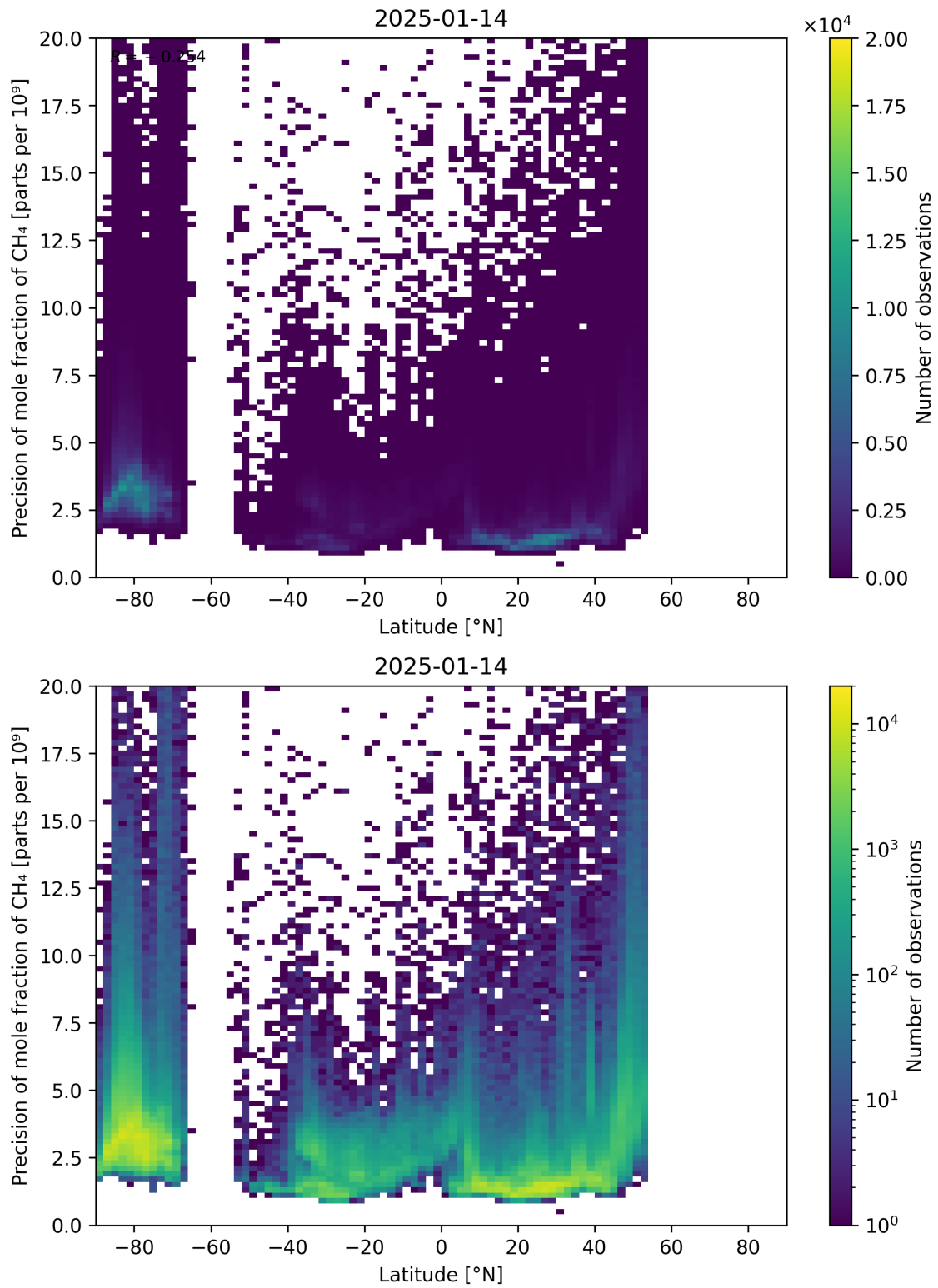
Figure 59: Scatter density plot of “Latitude” against “Precision of mole fraction of CH 4 ” for 2025-01-13 to 2025-01-15.
