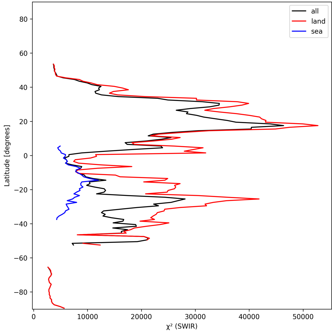
Figure 17: Zonal average of “ \chi^2 (SWIR)” for 2025-01-13 to 2025-01-15.
