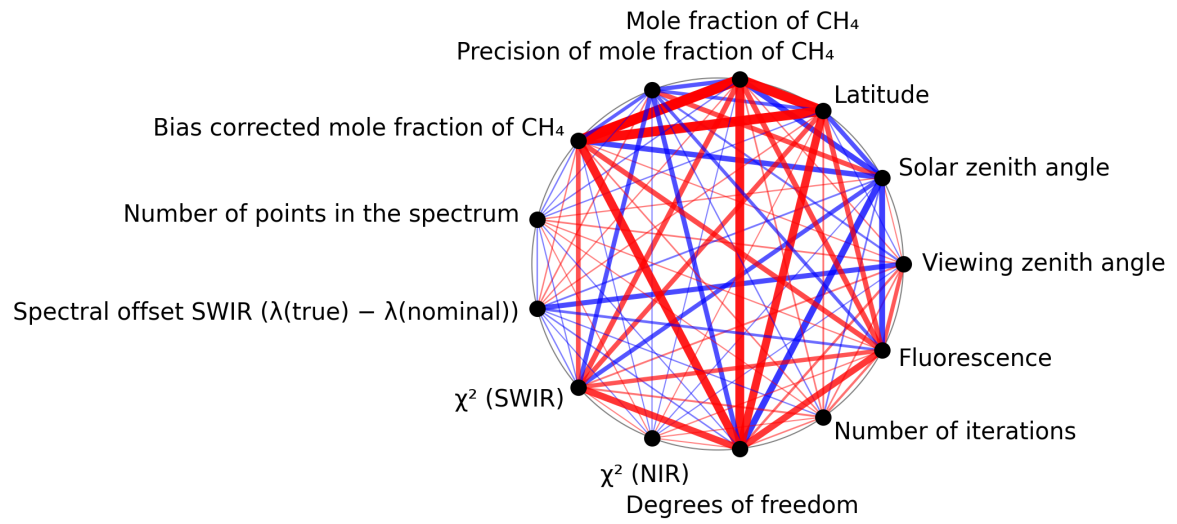
Figure 1: Map of correlation graph for 2025-01-13 to 2025-01-15.
