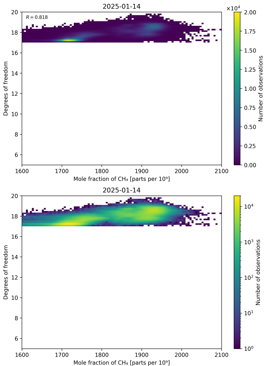
Figure 72: Scatter density plot of “Mole fraction of CH 4 ” against “Degrees of freedom” for 2025-01-13 to 2025-01-15.
