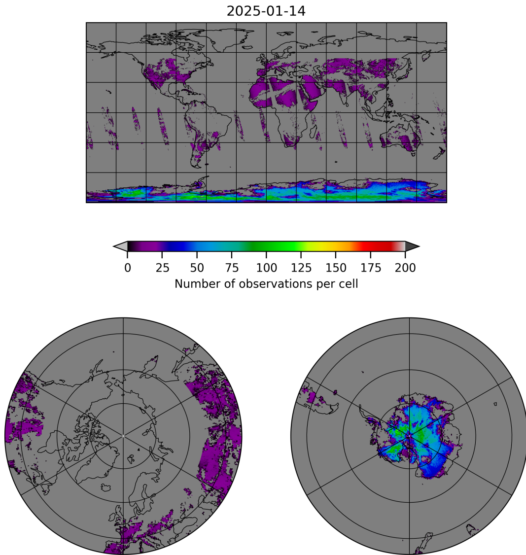
Figure 10: Map of the number of observations for 2025-01-13 to 2025-01-15
