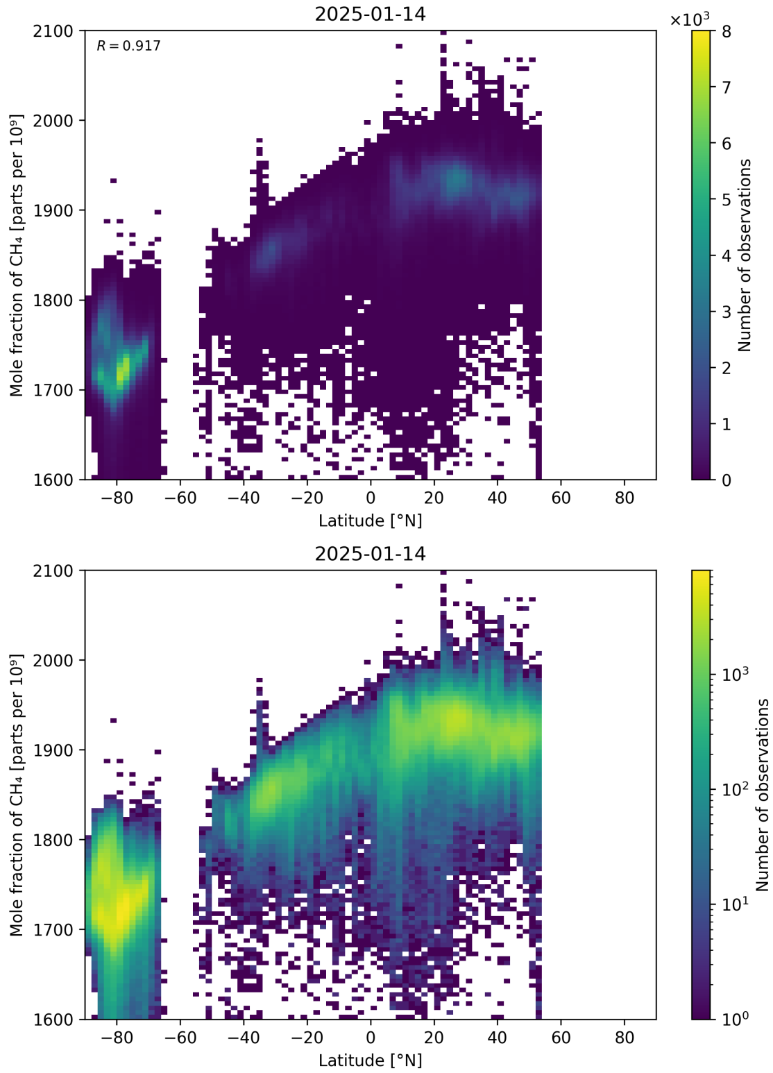
Figure 57: Scatter density plot of “Latitude” against “Mole fraction of \text{CH}_4 ” for 2025-01-13 to 2025-01-15.
