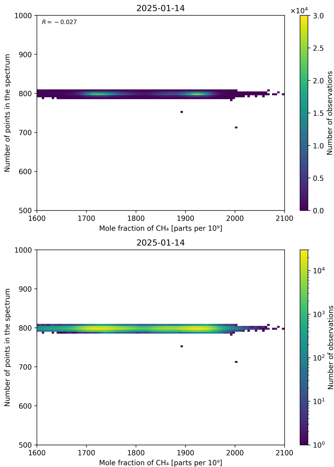
Figure 77: Scatter density plot of “Mole fraction of CH 4 ” against “Number of points in the spectrum” for 2025-01-13 to 2025-01-15.
