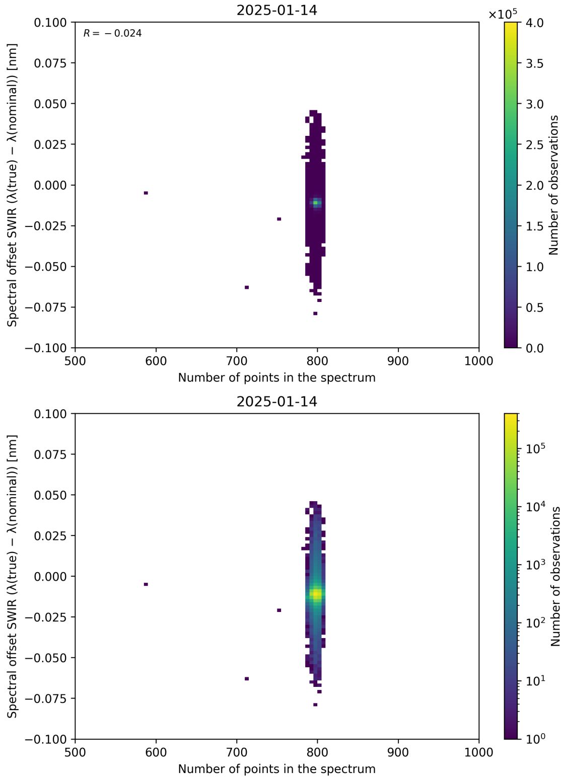
Figure 93: Scatter density plot of “Number of points in the spectrum” against “Spectral offset SWIR ( \lambda_{\text{true}} - \lambda_{\text{nominal}} )” for 2025-01-13 to 2025-01-15.
