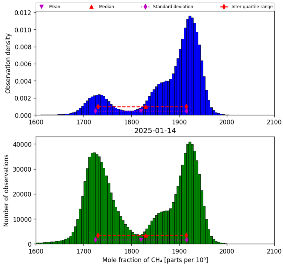
Figure 23: Histogram of “Mole fraction of CH 4 ” for 2025-01-13 to 2025-01-15
