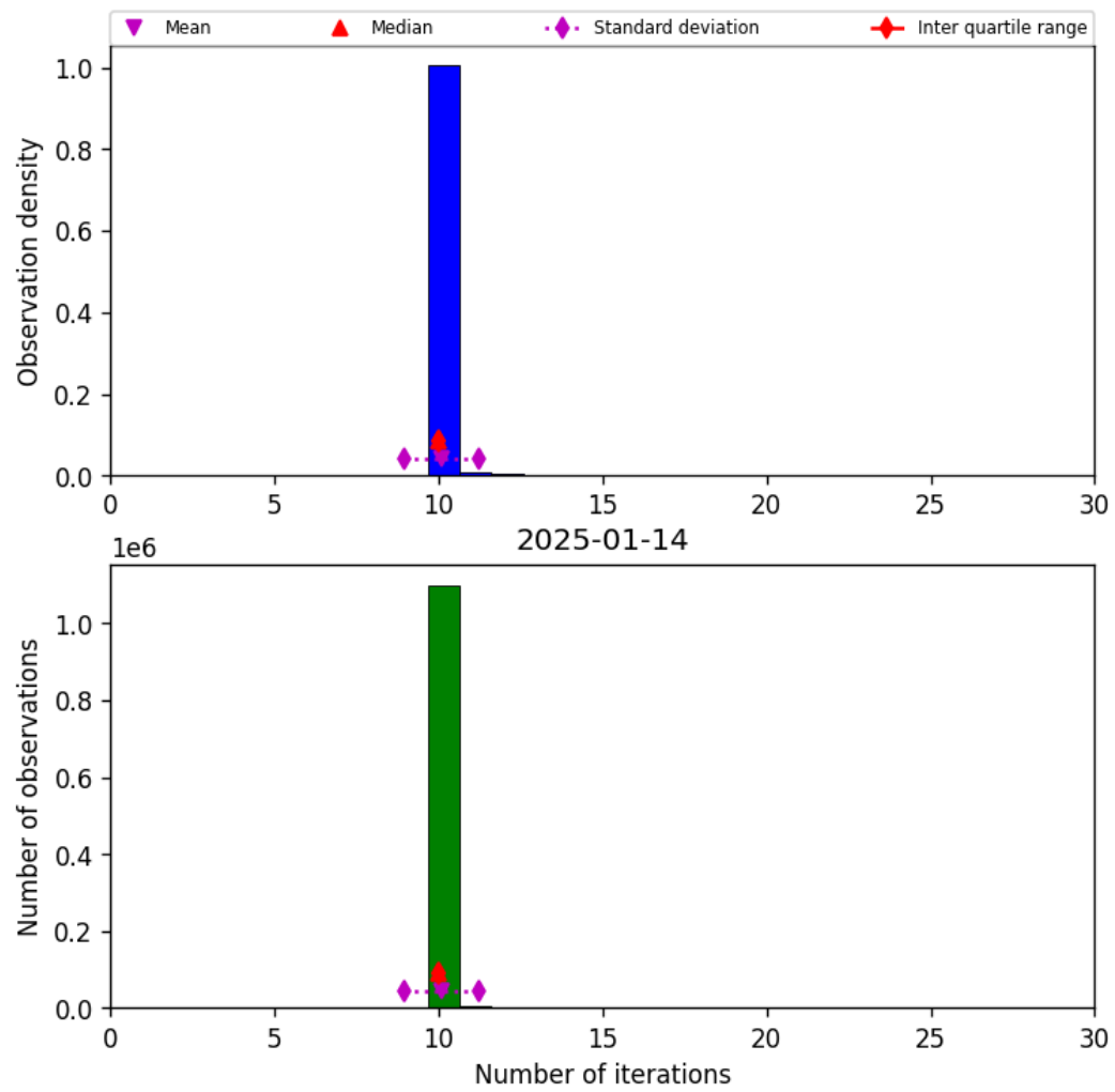
Figure 31: Histogram of “Number of iterations” for 2025-01-13 to 2025-01-15
