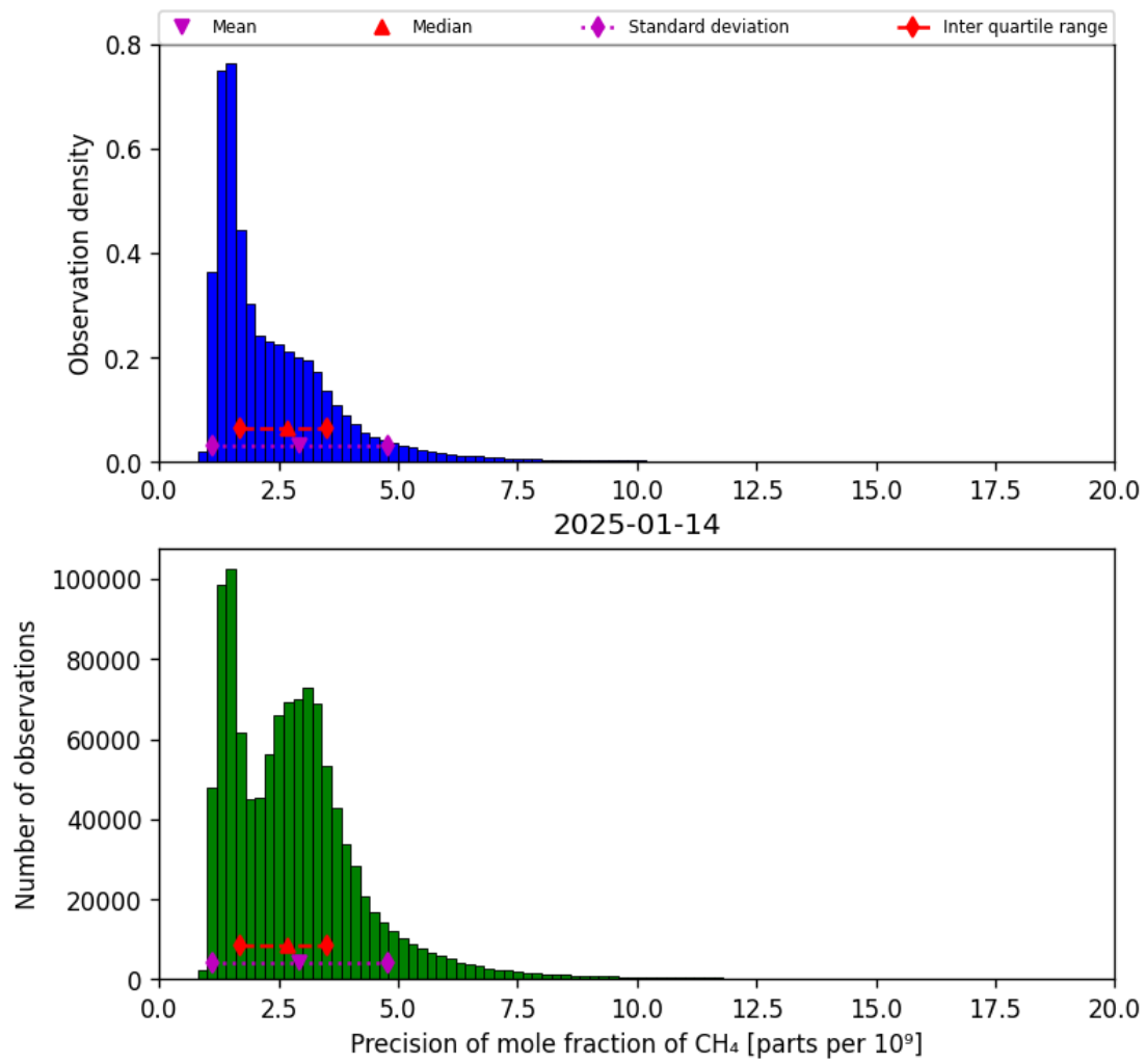
Figure 24: Histogram of “Precision of mole fraction of CH 4 ” for 2025-01-13 to 2025-01-15
