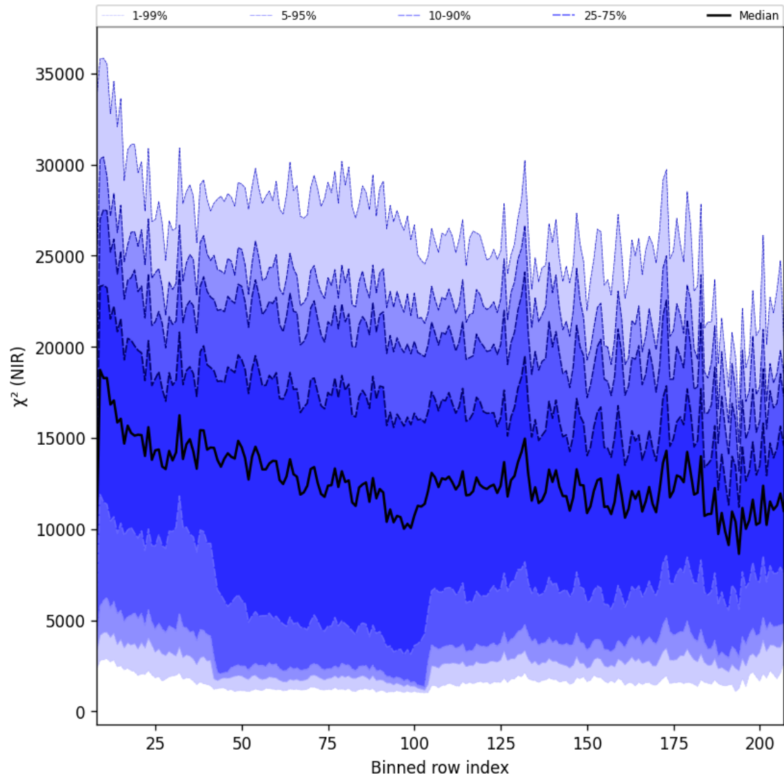
Figure 40: Along track statistics of “ \chi^2 (NIR)” for 2025-01-13 to 2025-01-15
