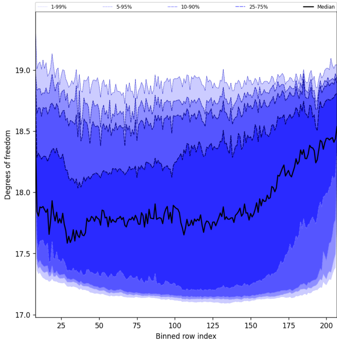
Figure 41: Along track statistics of “Degrees of freedom” for 2025-01-13 to 2025-01-15
