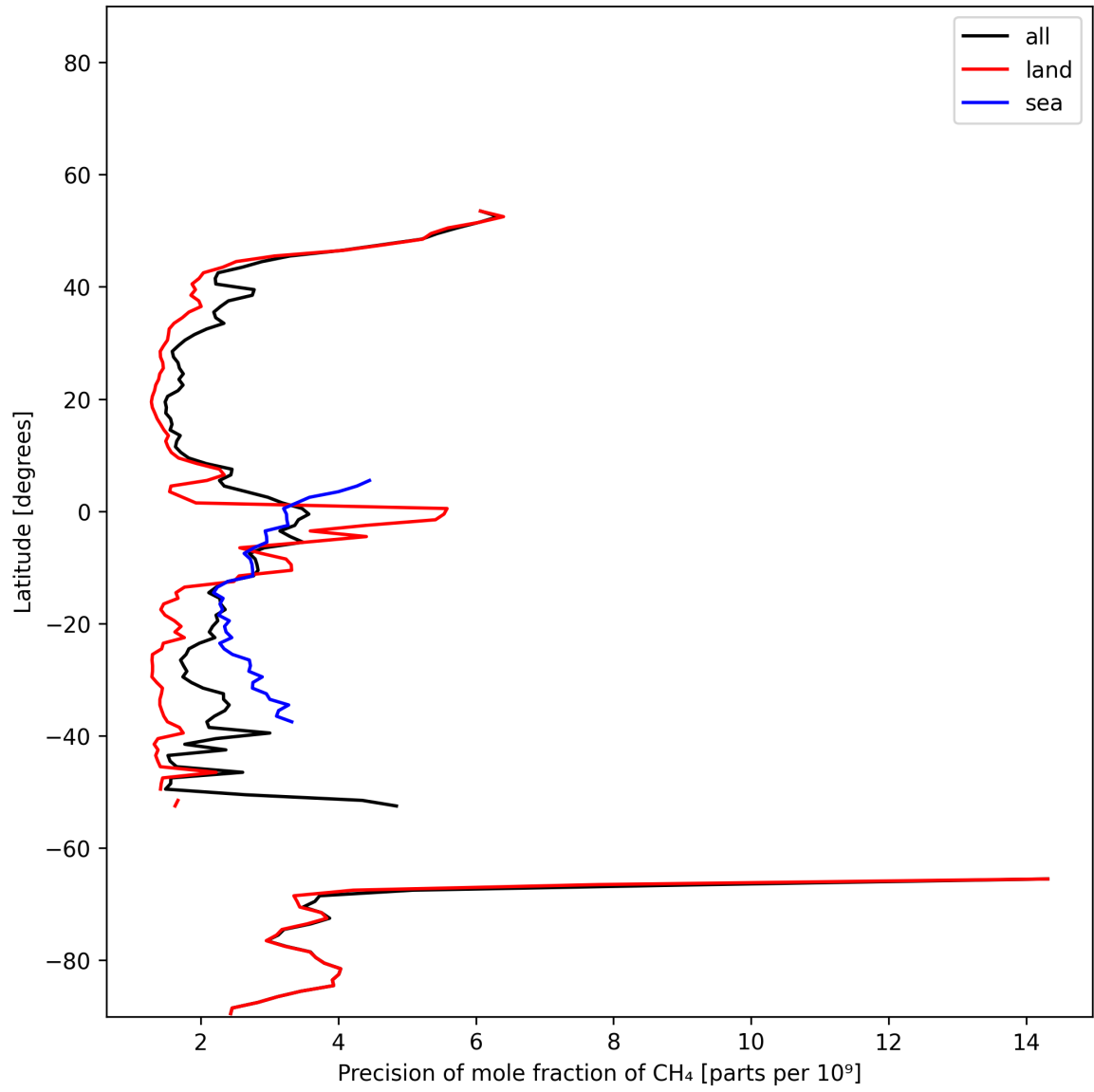
Figure 13: Zonal average of “Precision of mole fraction of CH 4 ” for 2025-01-13 to 2025-01-15.
