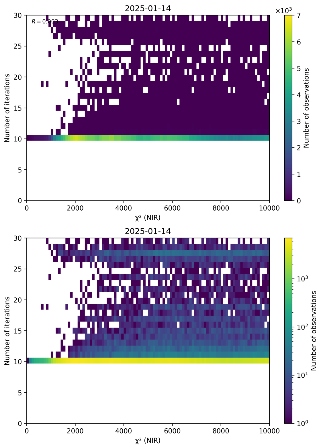
Figure 46: Scatter density plot of “ \chi^2 (NIR)” against “Number of iterations” for 2025-01-13 to 2025-01-15.
