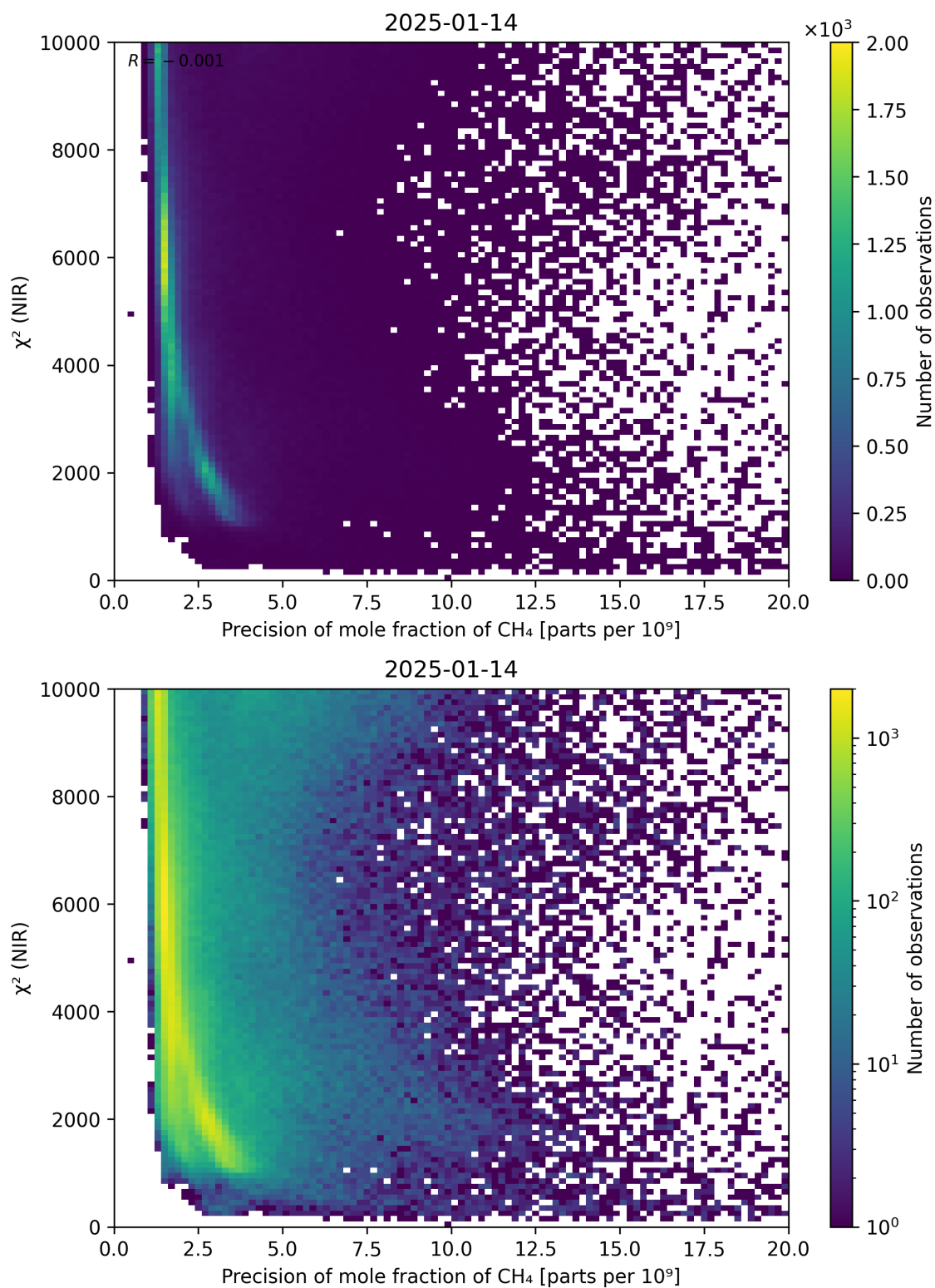
Figure 78: Scatter density plot of “Precision of mole fraction of \text{CH}_4 ” against “ \chi^2 (NIR)” for 2025-01-13 to 2025-01-15.
