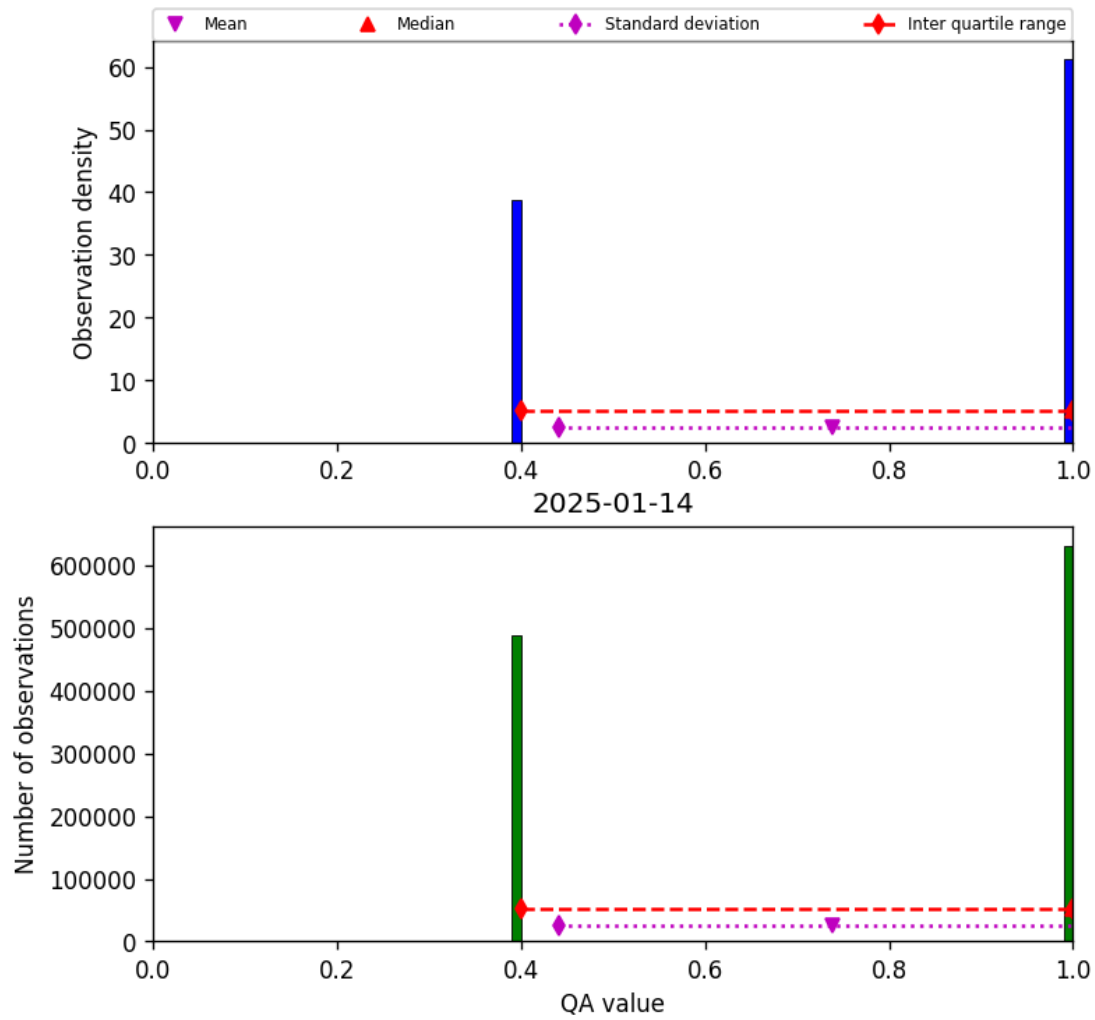
Figure 22: Histogram of “QA value” for 2025-01-13 to 2025-01-15
