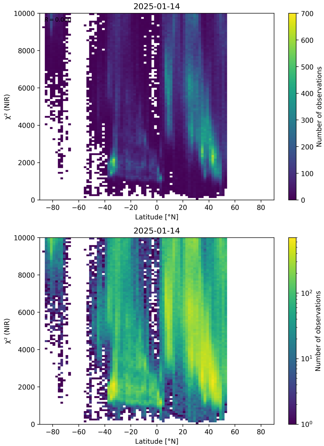
Figure 53: Scatter density plot of “Latitude” against “ \chi^2 (NIR)” for 2025-01-13 to 2025-01-15.
