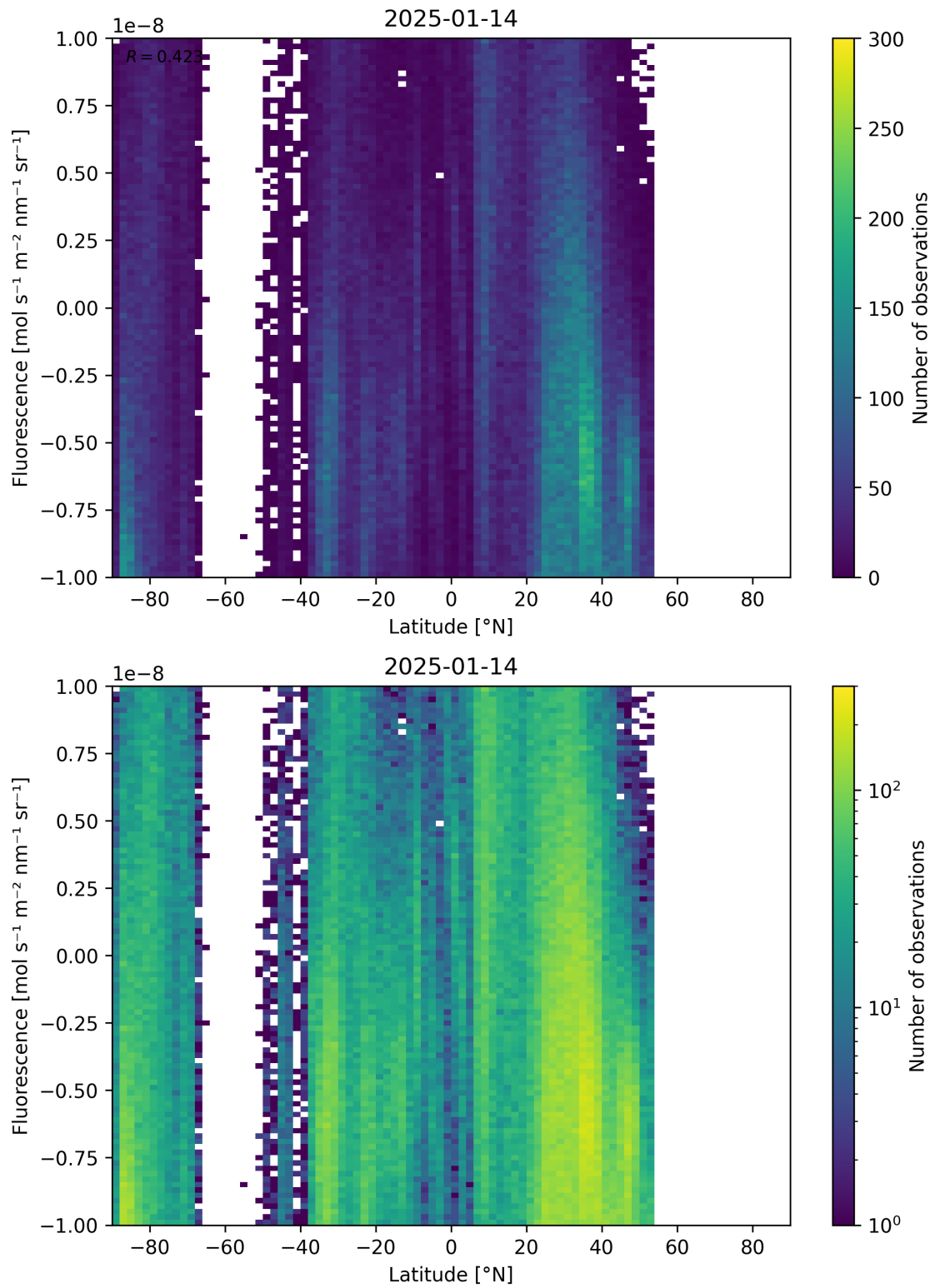
Figure 56: Scatter density plot of “Latitude” against “Fluorescence” for 2025-01-13 to 2025-01-15.
