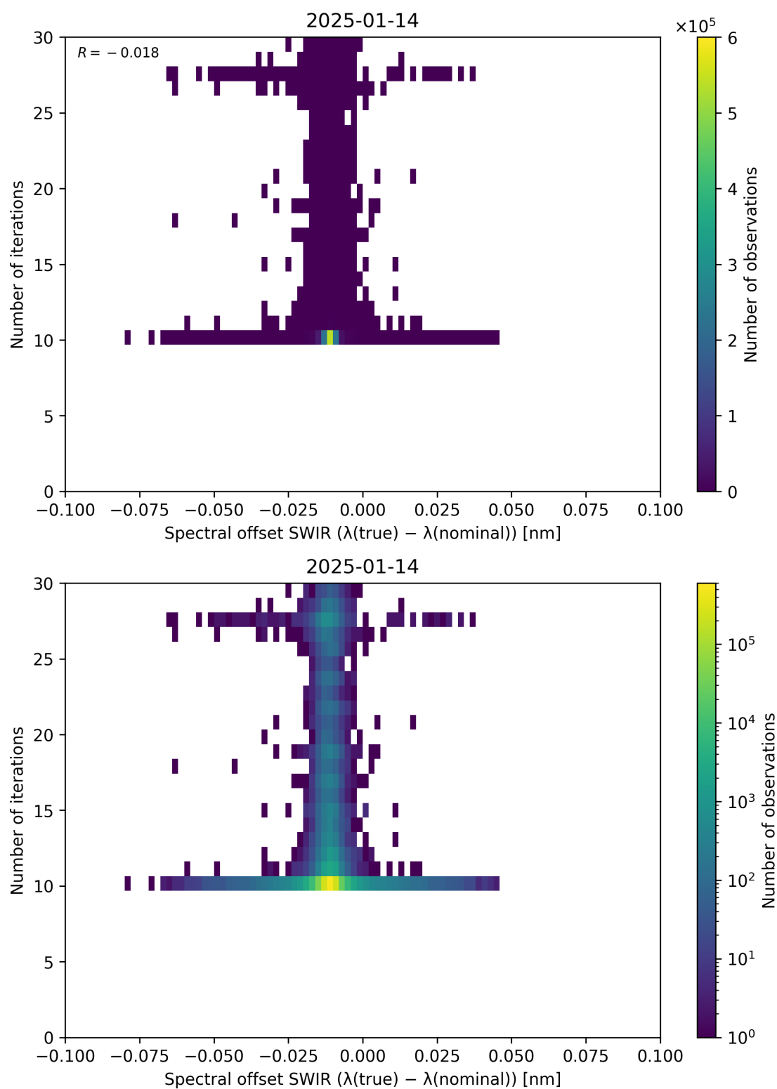
Figure 121: Scatter density plot of “Spectral offset SWIR ( \lambda_{\text{true}} - \lambda_{\text{nominal}} )” against “Number of iterations” for 2025-01-13 to 2025-01-15.
