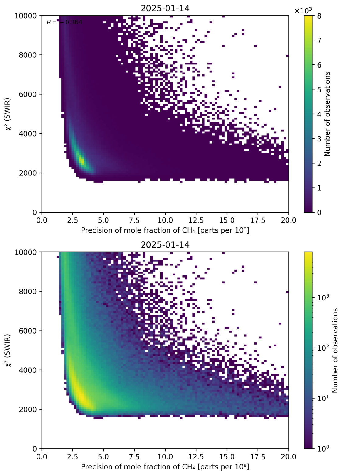
Figure 79: Scatter density plot of “Precision of mole fraction of \text{CH}_4 ” against “ \chi^2 (SWIR)” for 2025-01-13 to 2025-01-15.
