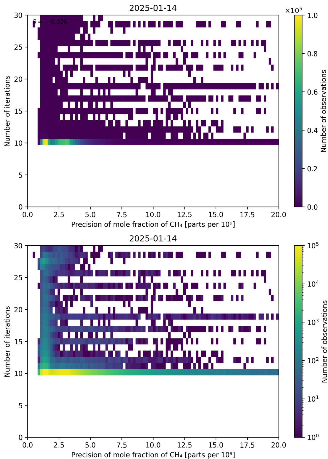
Figure 83: Scatter density plot of “Precision of mole fraction of CH 4 ” against “Number of iterations” for 2025-01-13 to 2025-01-15.
