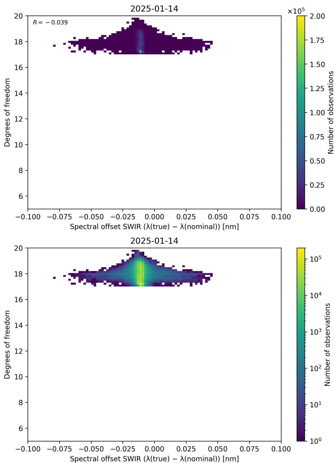
Figure 119: Scatter density plot of “Spectral offset SWIR ( \lambda_{\text{true}} - \lambda_{\text{nominal}} )” against “Degrees of freedom” for 2025-01-13 to 2025-01-15.
