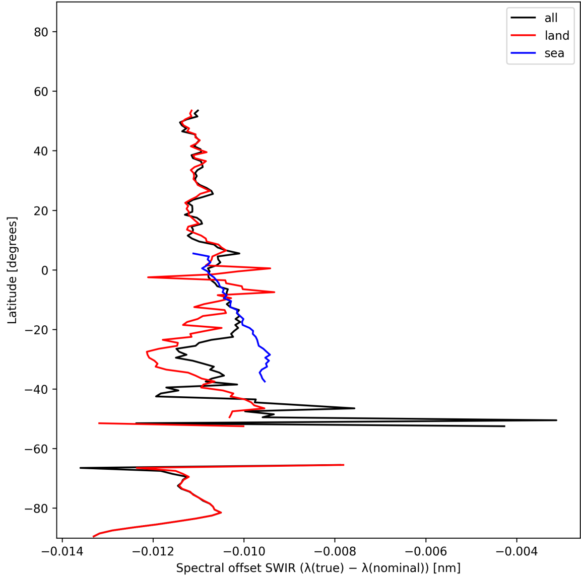
Figure 16: Zonal average of “Spectral offset SWIR ( \lambda_{\text{true}} - \lambda_{\text{nominal}} )” for 2025-01-13 to 2025-01-15.
