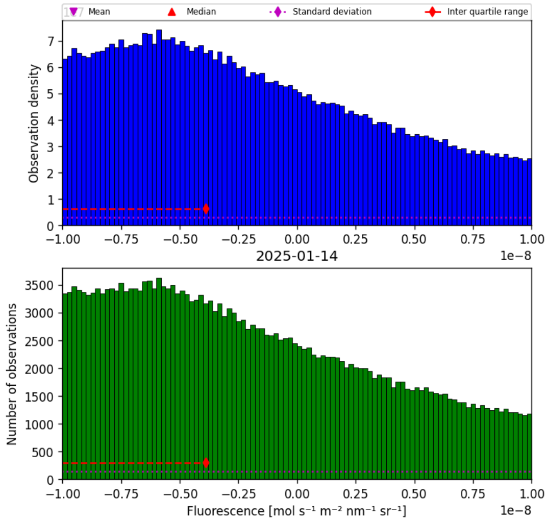
Figure 32: Histogram of “Fluorescence” for 2025-01-13 to 2025-01-15
