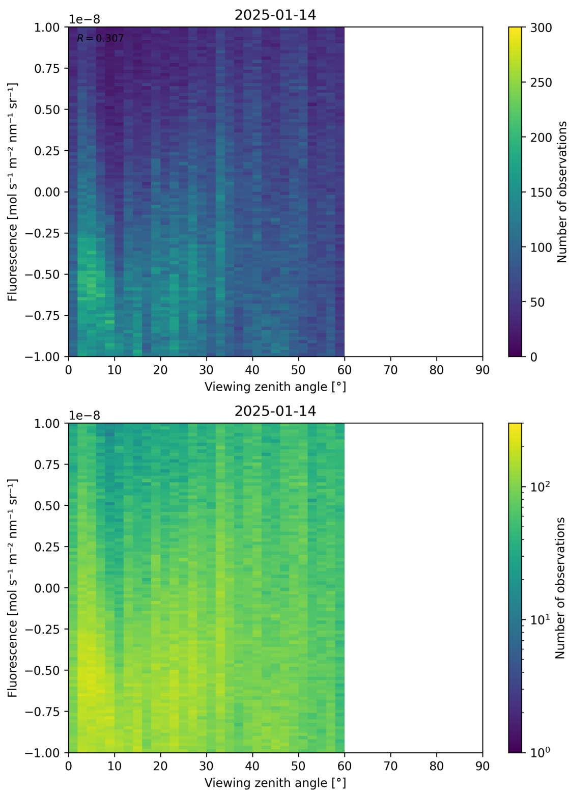
Figure 108: Scatter density plot of “Viewing zenith angle” against “Fluorescence” for 2025-01-13 to 2025-01-15.
