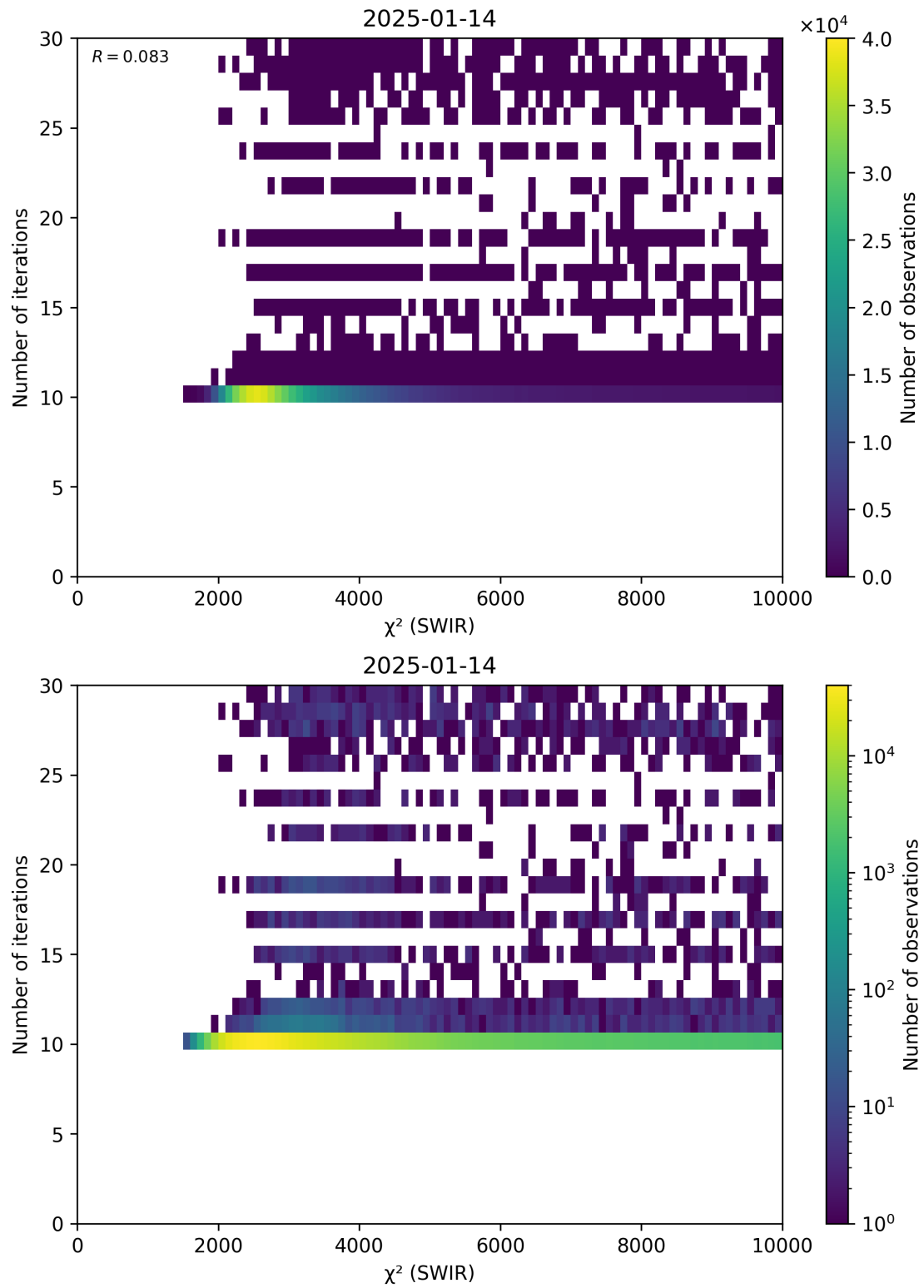
Figure 50: Scatter density plot of “ \chi^2 (SWIR)” against “Number of iterations” for 2025-01-13 to 2025-01-15.
