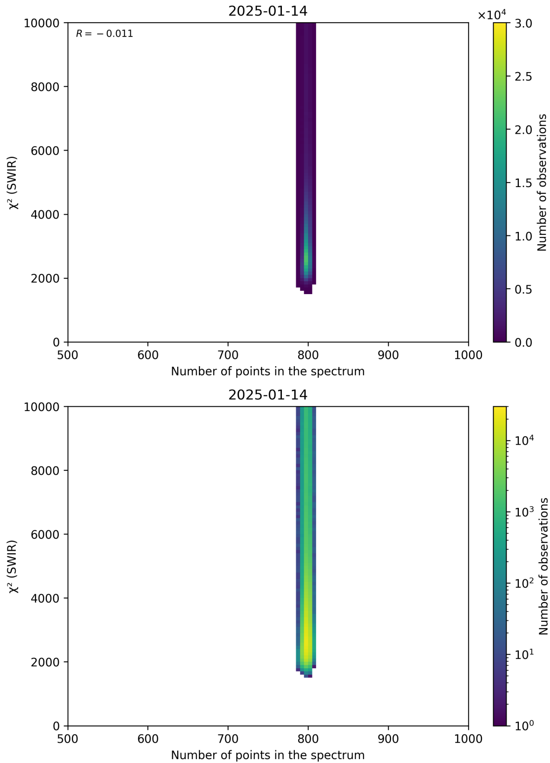
Figure 89: Scatter density plot of “Number of points in the spectrum” against “ \chi^2 (SWIR)” for 2025-01-13 to 2025-01-15.
