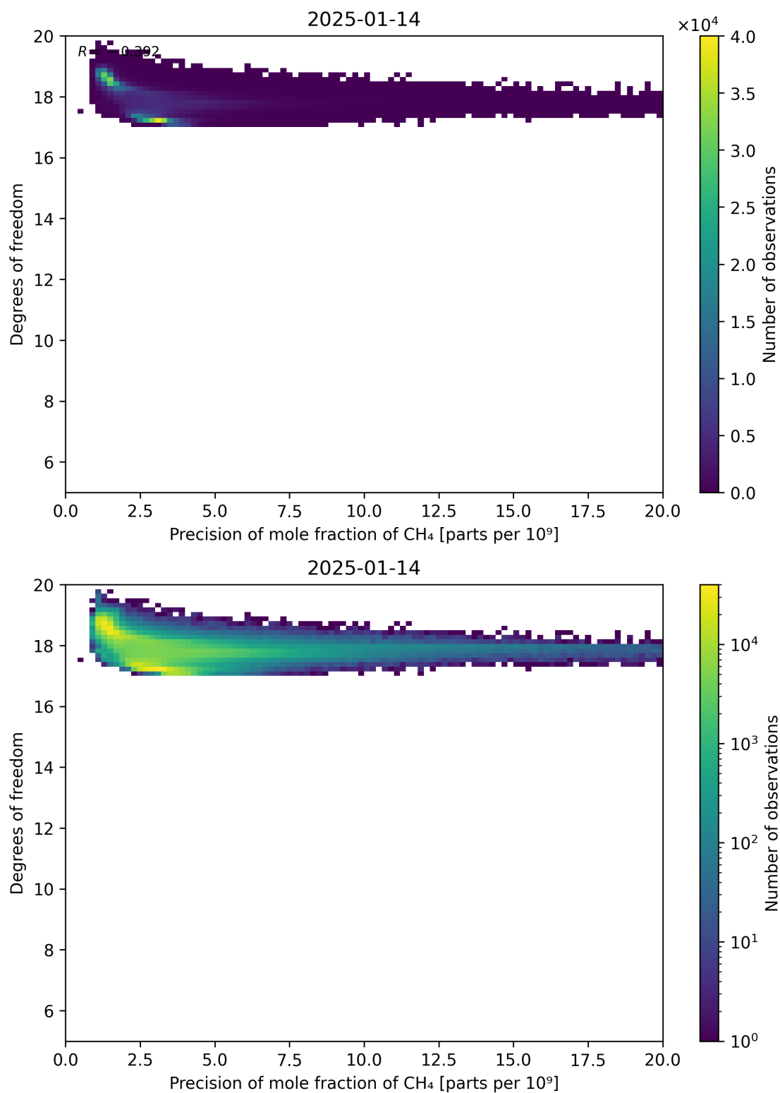
Figure 80: Scatter density plot of “Precision of mole fraction of CH 4 ” against “Degrees of freedom” for 2025-01-13 to 2025-01-15.
