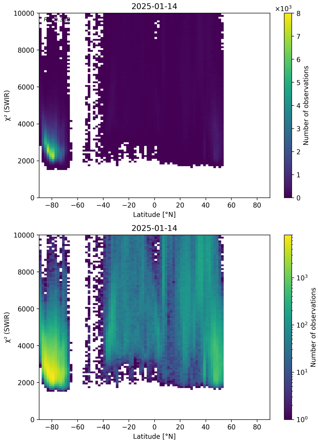
Figure 54: Scatter density plot of “Latitude” against “ \chi^2 (SWIR)” for 2025-01-13 to 2025-01-15.
