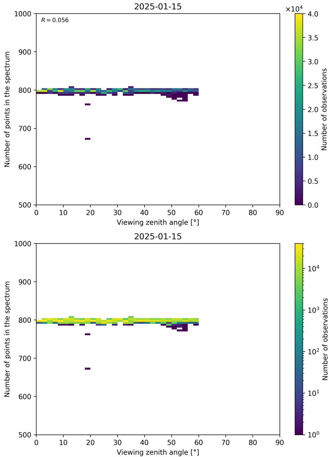
Figure 114: Scatter density plot of “Viewing zenith angle” against “Number of points in the spectrum” for 2025-01-14 to 2025-01-16.
