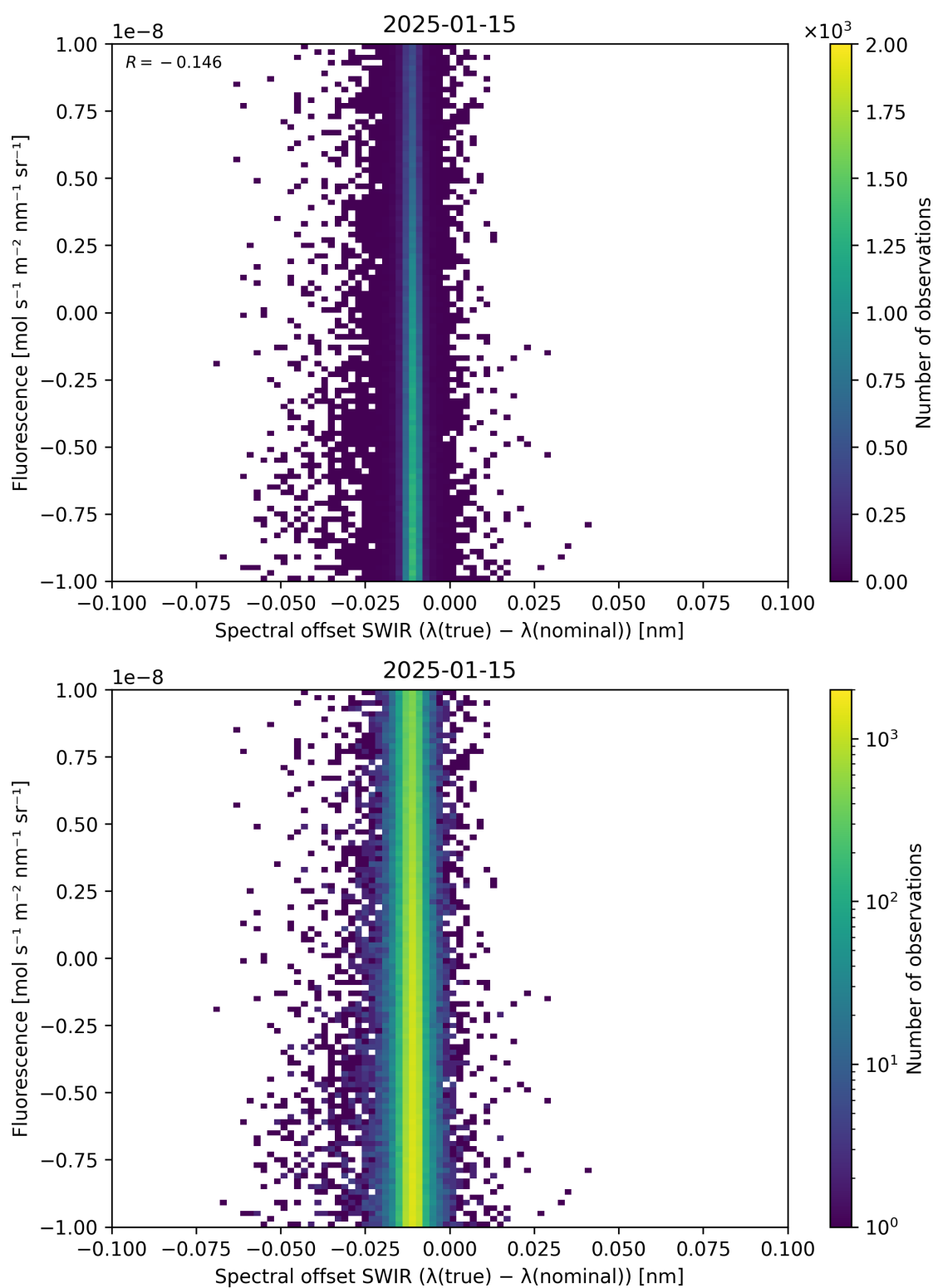
Figure 120: Scatter density plot of “Spectral offset SWIR ( \lambda_{\text{true}} - \lambda_{\text{nominal}} )” against “Fluorescence” for 2025-01-14 to 2025-01-16.
