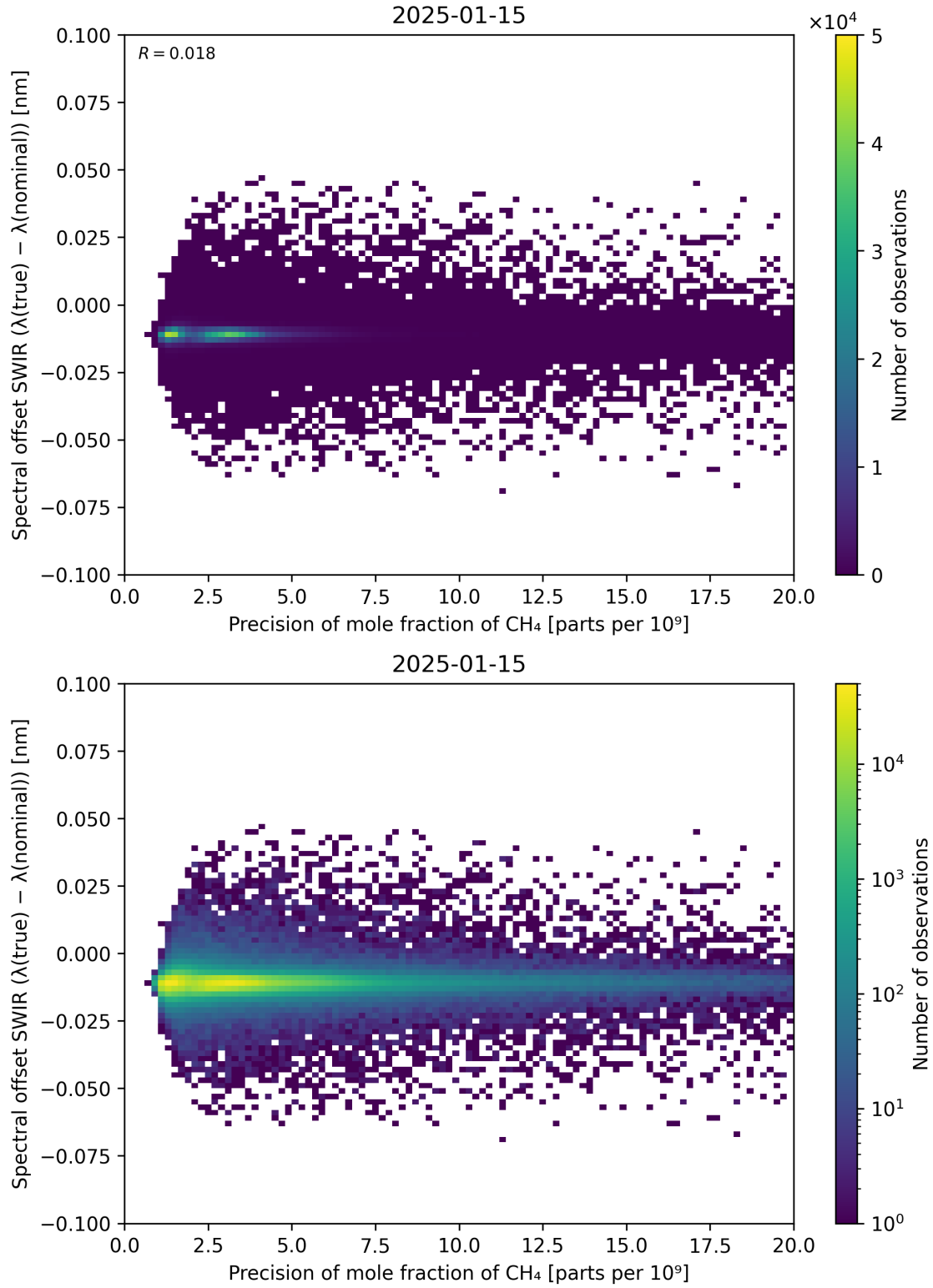
Figure 85: Scatter density plot of “Precision of mole fraction of CH 4 ” against “Spectral offset SWIR ( \lambda_{\text{true}} - \lambda_{\text{nominal}} )” for 2025-01-14 to 2025-01-16.
