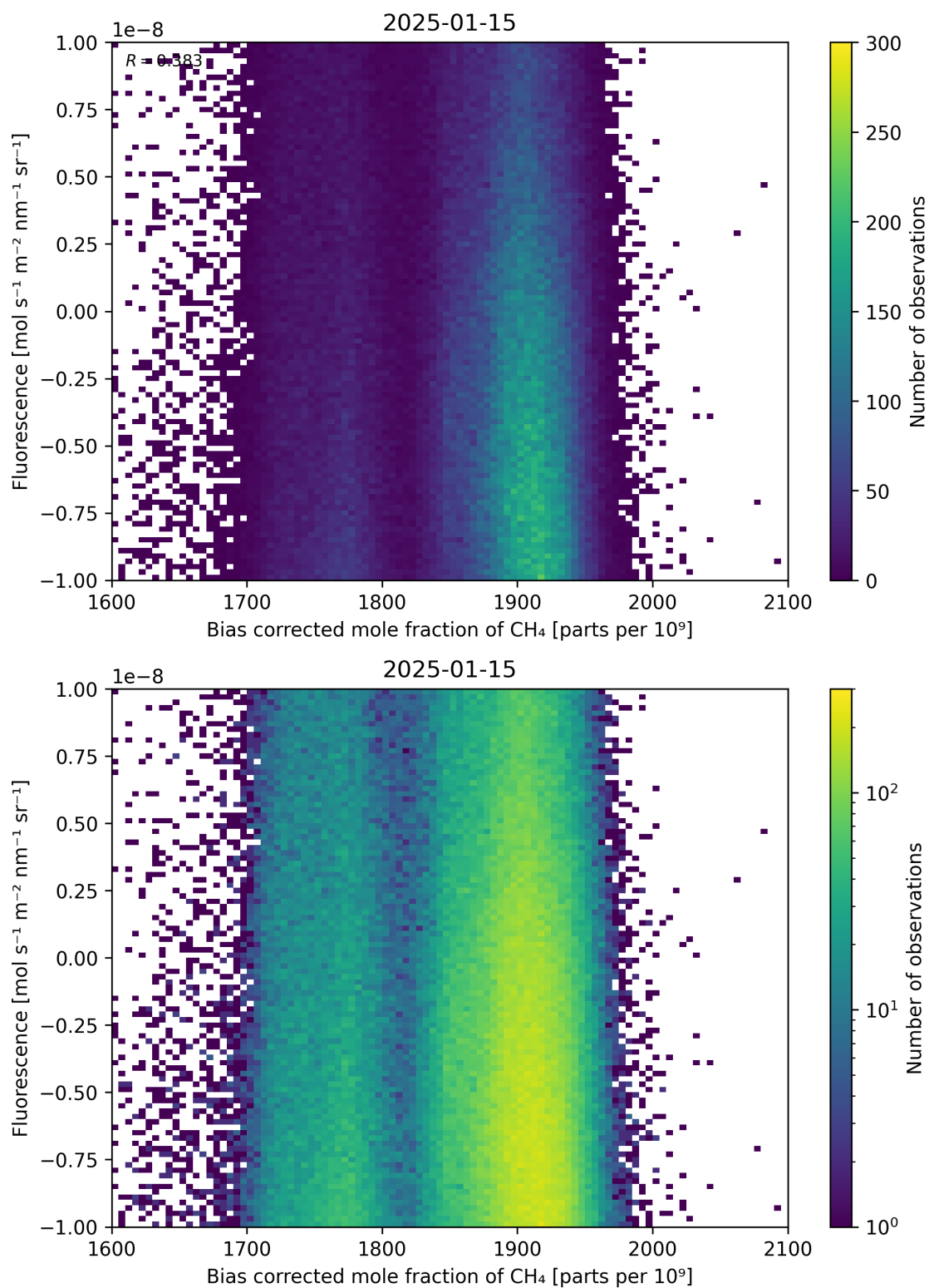
Figure 66: Scatter density plot of “Bias corrected mole fraction of \text{CH}_4 ” against “Fluorescence” for 2025-01-14 to 2025-01-16.
