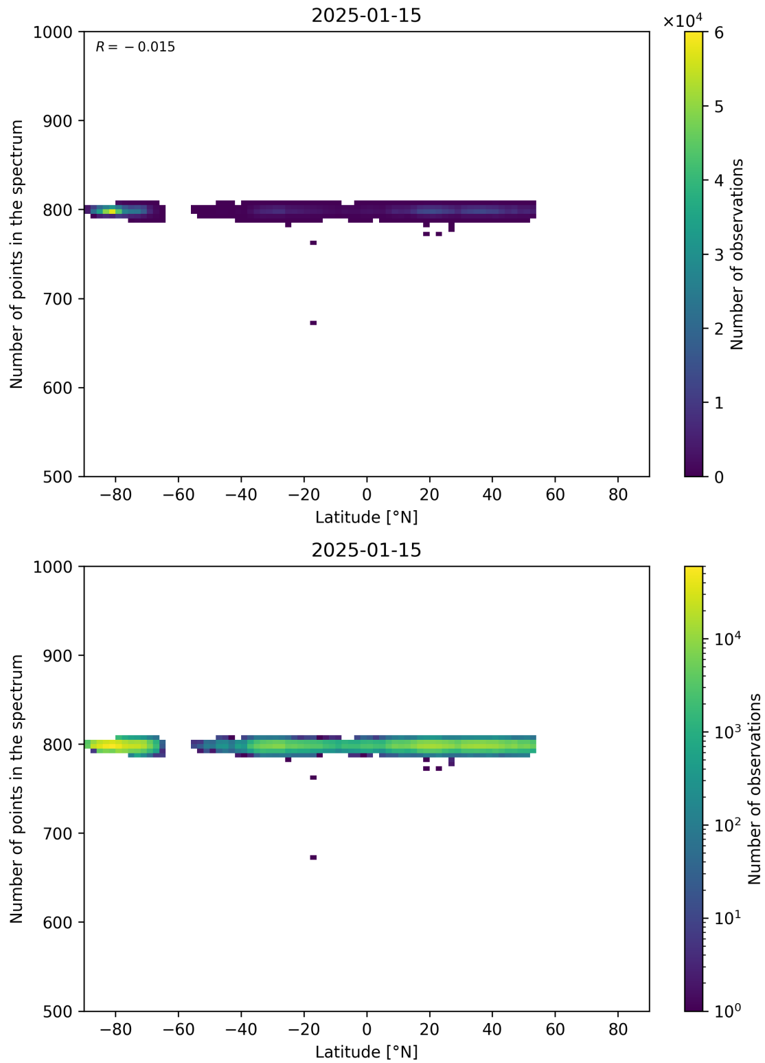
Figure 61: Scatter density plot of “Latitude” against “Number of points in the spectrum” for 2025-01-14 to 2025-01-16.
