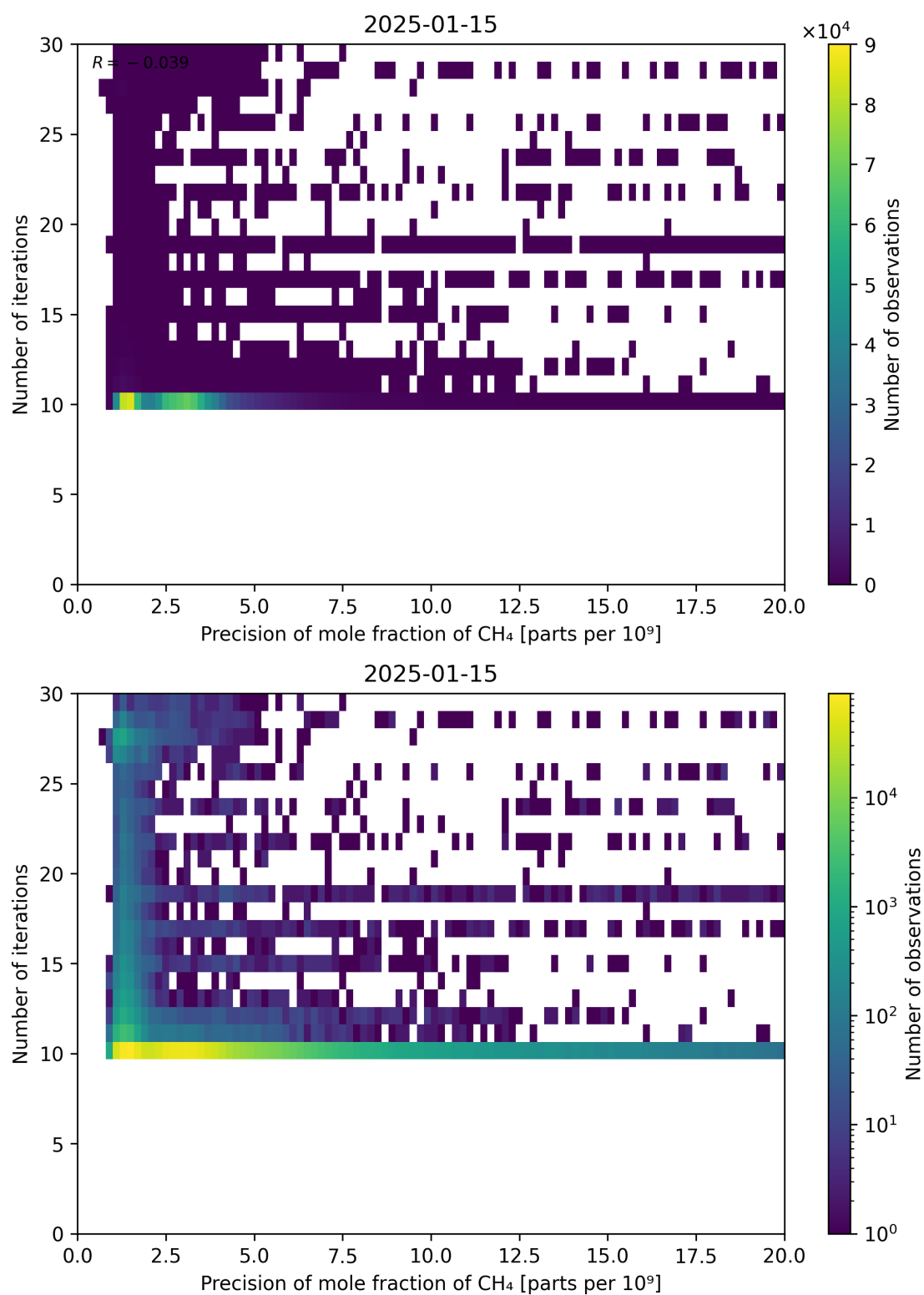
Figure 83: Scatter density plot of “Precision of mole fraction of CH 4 ” against “Number of iterations” for 2025-01-14 to 2025-01-16.
