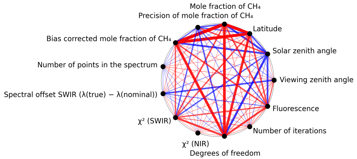
Figure 1: Map of correlation graph for 2025-01-14 to 2025-01-16.
