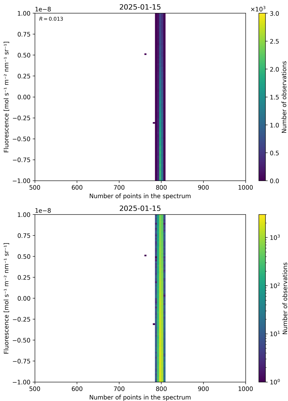
Figure 91: Scatter density plot of “Number of points in the spectrum” against “Fluorescence” for 2025-01-14 to 2025-01-16.
