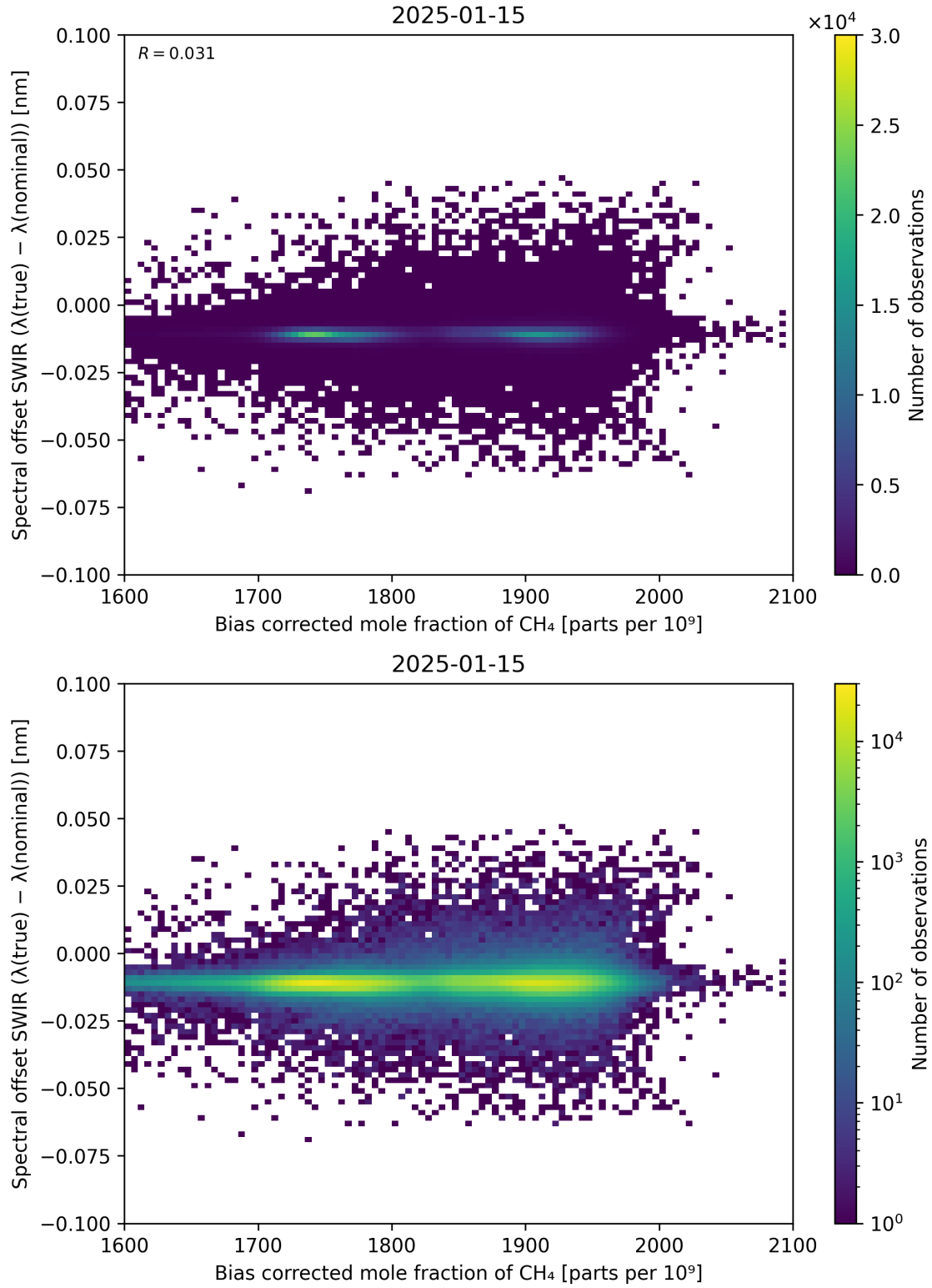
Figure 69: Scatter density plot of “Bias corrected mole fraction of \text{CH}_4 ” against “Spectral offset SWIR ( \lambda_{\text{true}} - \lambda_{\text{nominal}} )” for 2025-01-14 to 2025-01-16.
