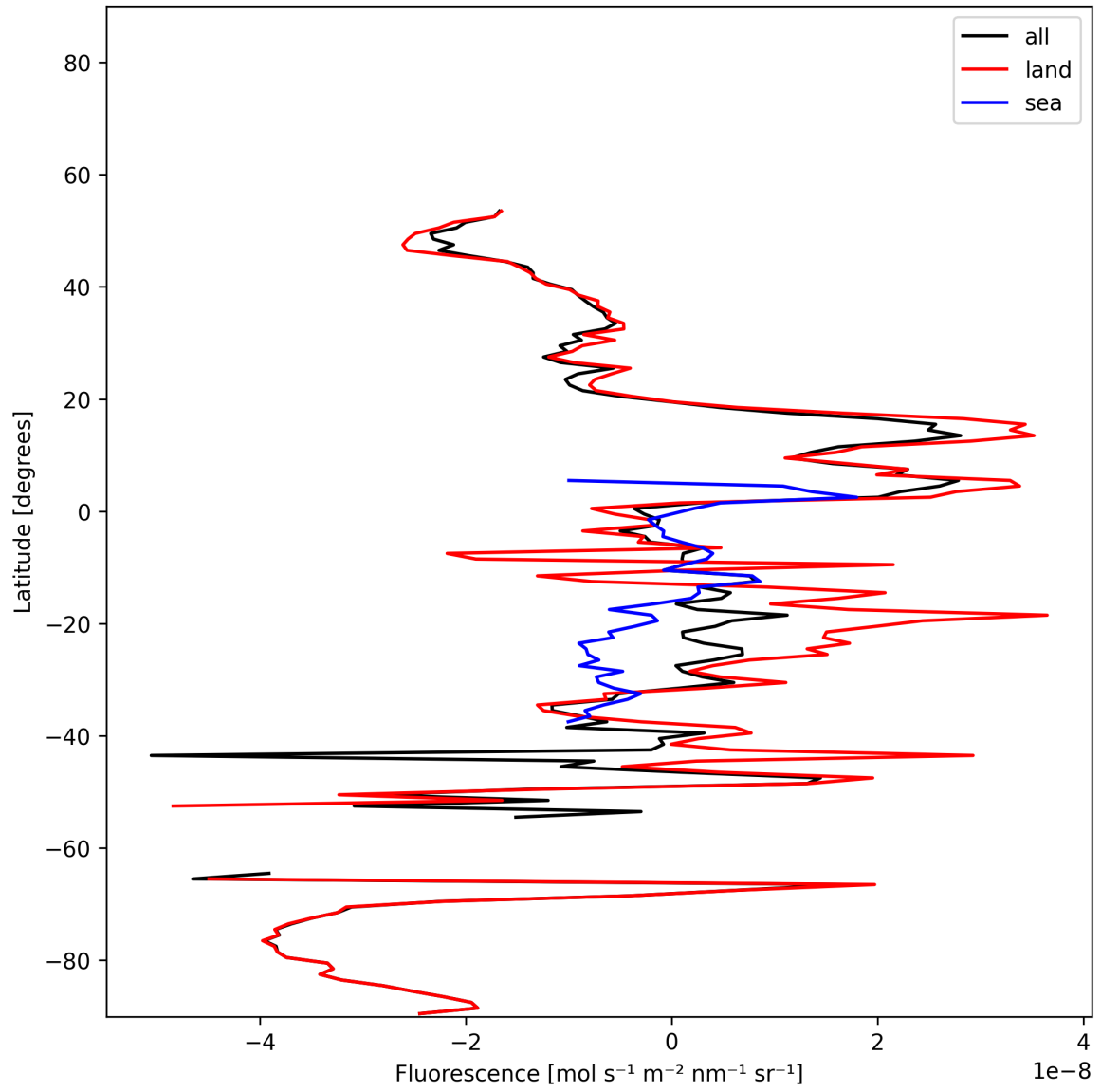
Figure 21: Zonal average of “Fluorescence” for 2025-01-14 to 2025-01-16.
