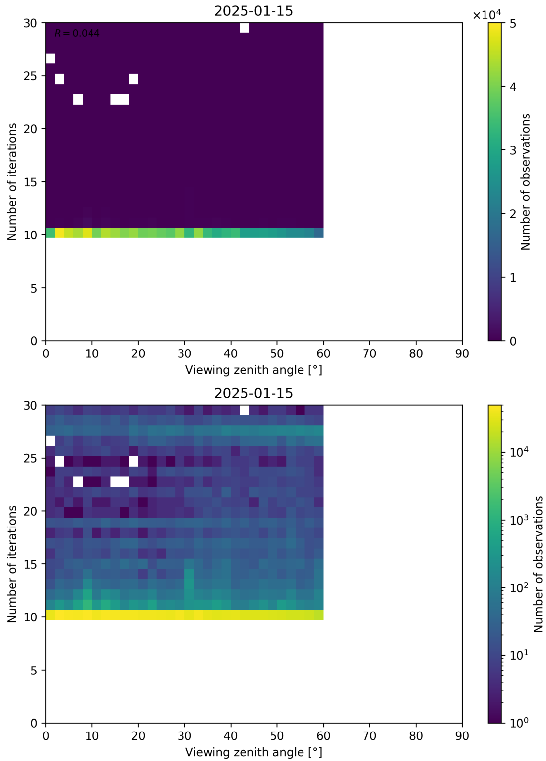
Figure 113: Scatter density plot of “Viewing zenith angle” against “Number of iterations” for 2025-01-14 to 2025-01-16.
