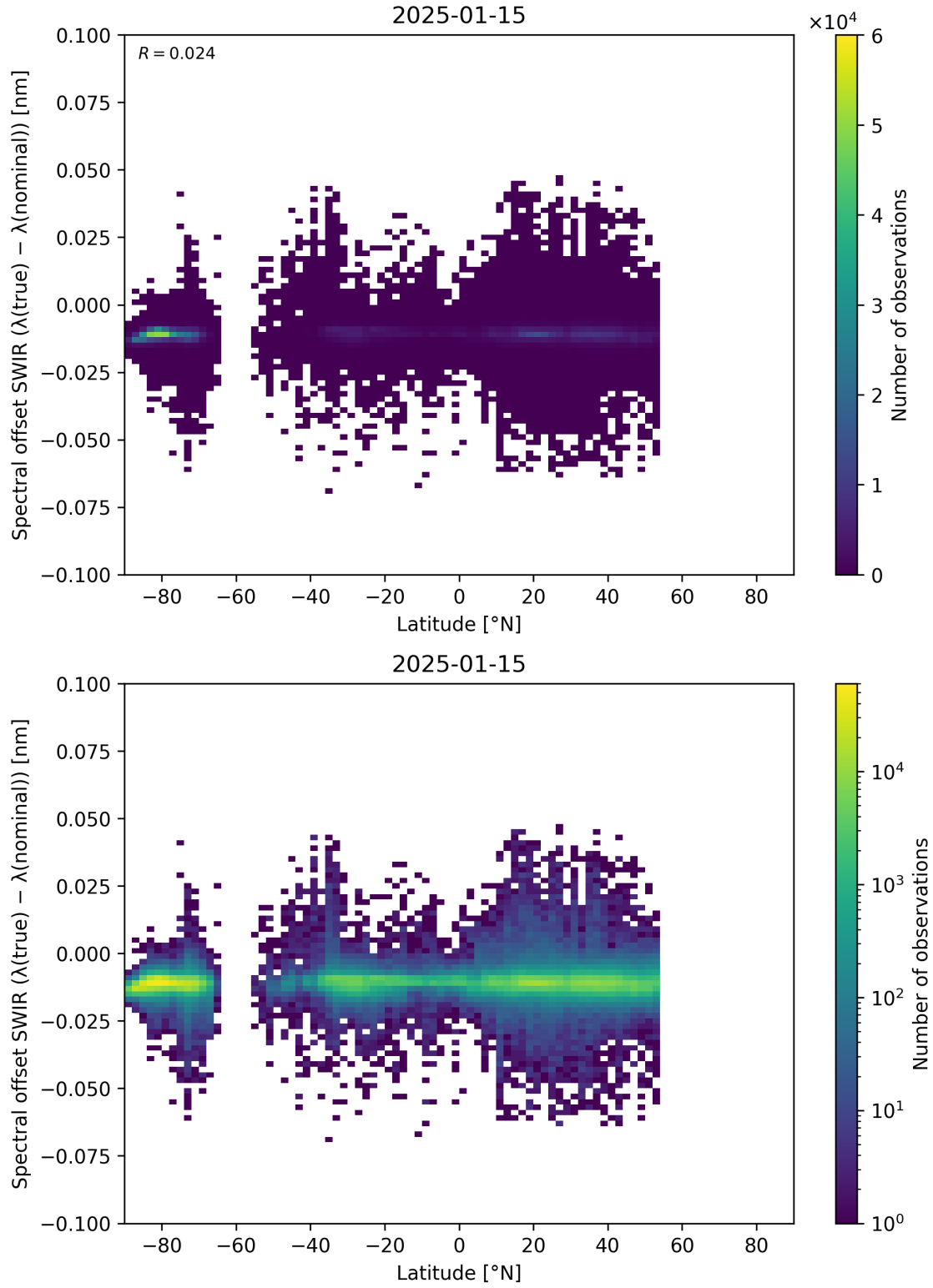
Figure 62: Scatter density plot of “Latitude” against “Spectral offset SWIR ( \lambda_{\text{true}} - \lambda_{\text{nominal}} )” for 2025-01-14 to 2025-01-16.
