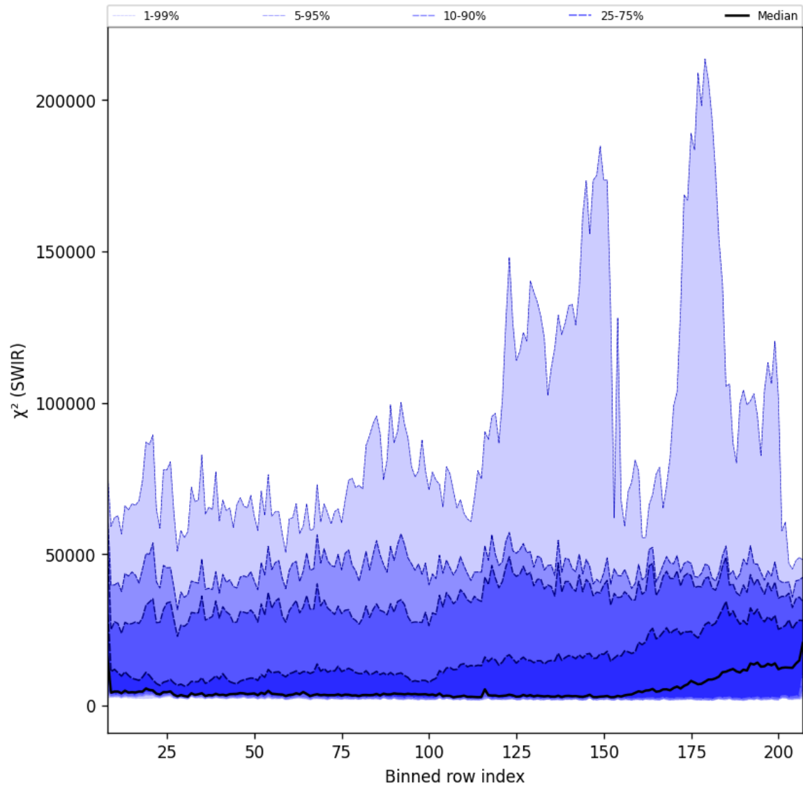
Figure 39: Along track statistics of “ \chi^2 (SWIR)” for 2025-01-14 to 2025-01-16
