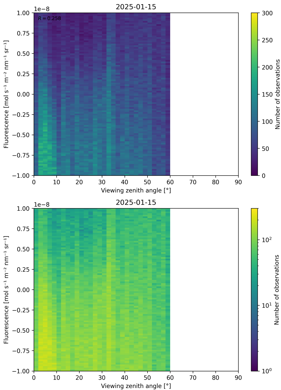
Figure 108: Scatter density plot of “Viewing zenith angle” against “Fluorescence” for 2025-01-14 to 2025-01-16.
