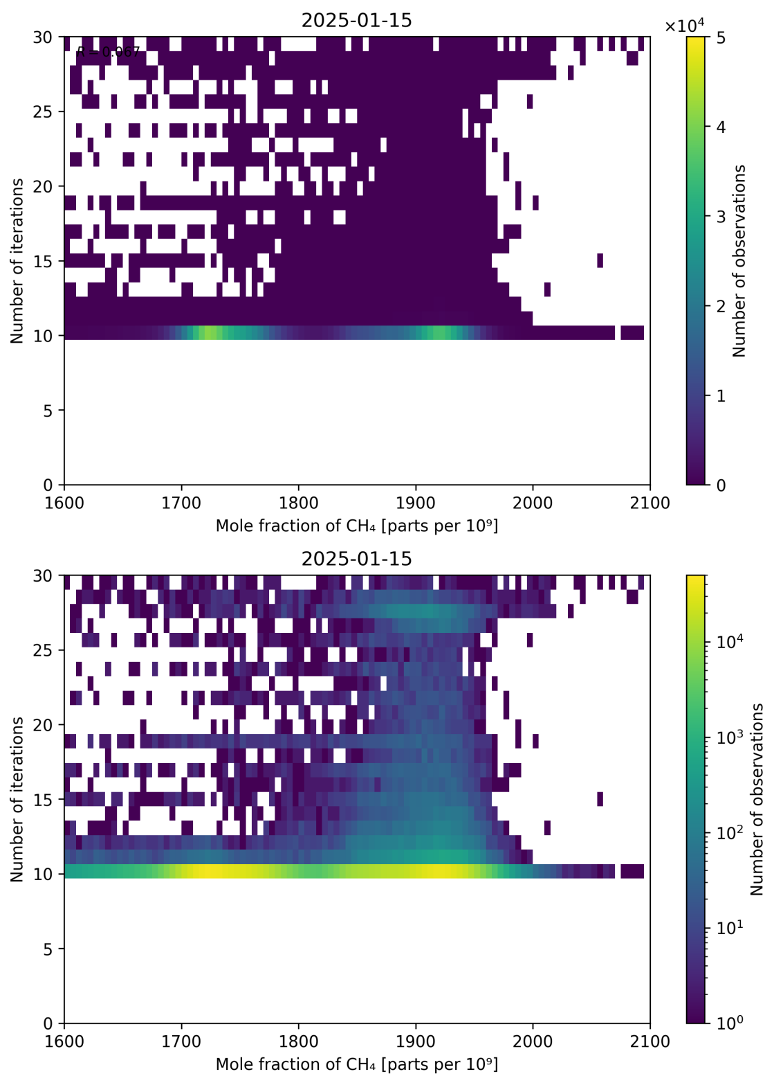
Figure 76: Scatter density plot of “Mole fraction of CH 4 ” against “Number of iterations” for 2025-01-14 to 2025-01-16.
