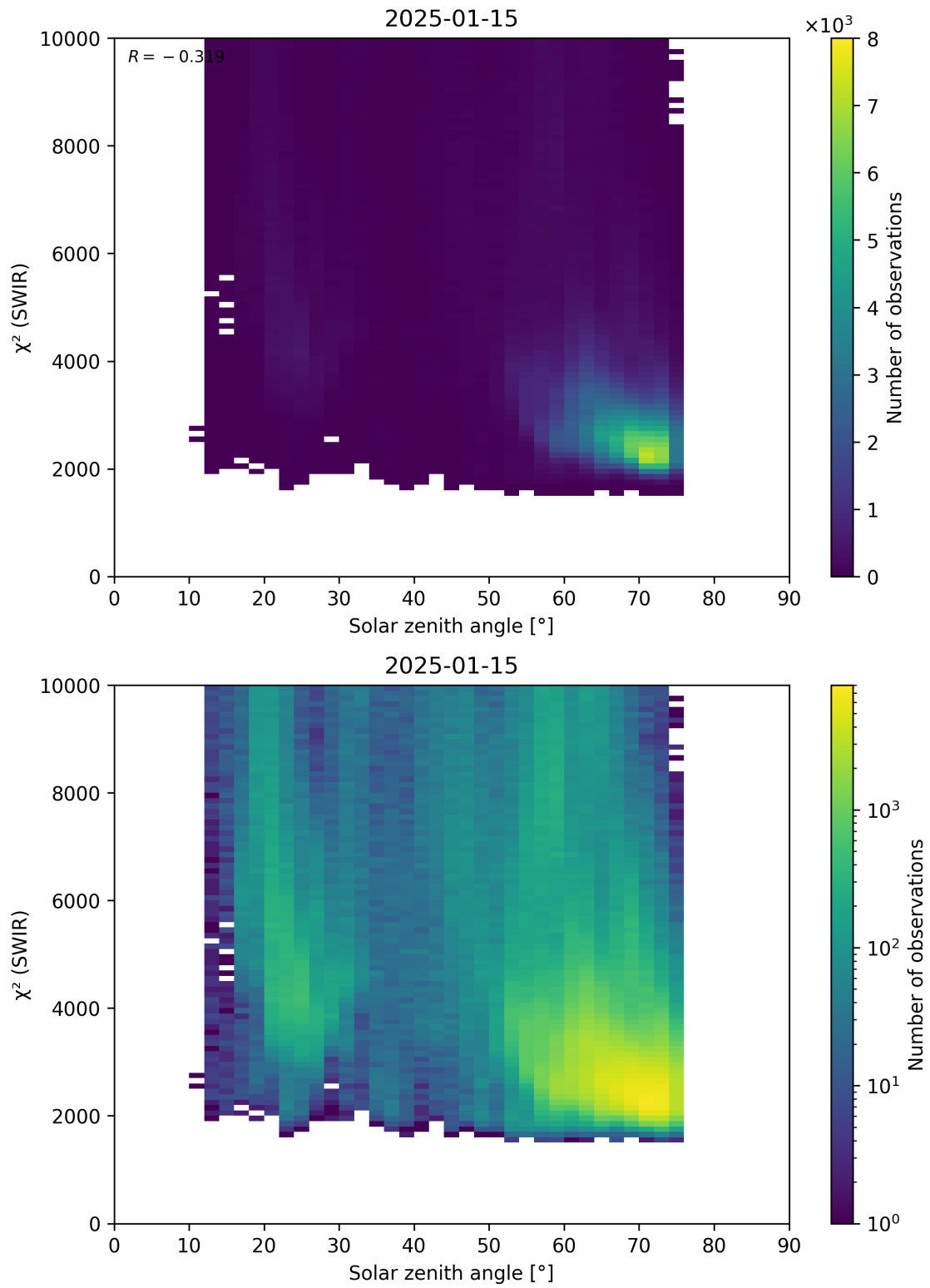
Figure 95: Scatter density plot of “Solar zenith angle” against “ \chi^2 (SWIR)” for 2025-01-14 to 2025-01-16.
