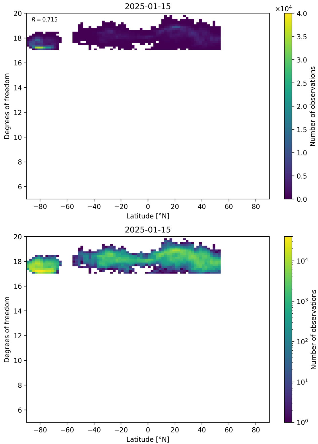
Figure 55: Scatter density plot of “Latitude” against “Degrees of freedom” for 2025-01-14 to 2025-01-16.
