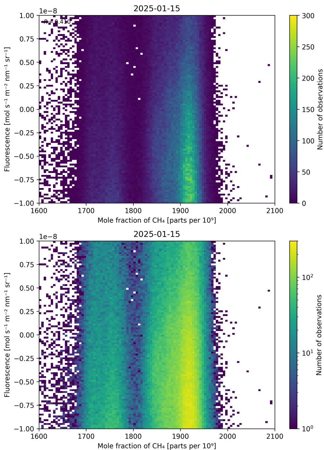
Figure 73: Scatter density plot of “Mole fraction of \text{CH}_4 ” against “Fluorescence” for 2025-01-14 to 2025-01-16.
