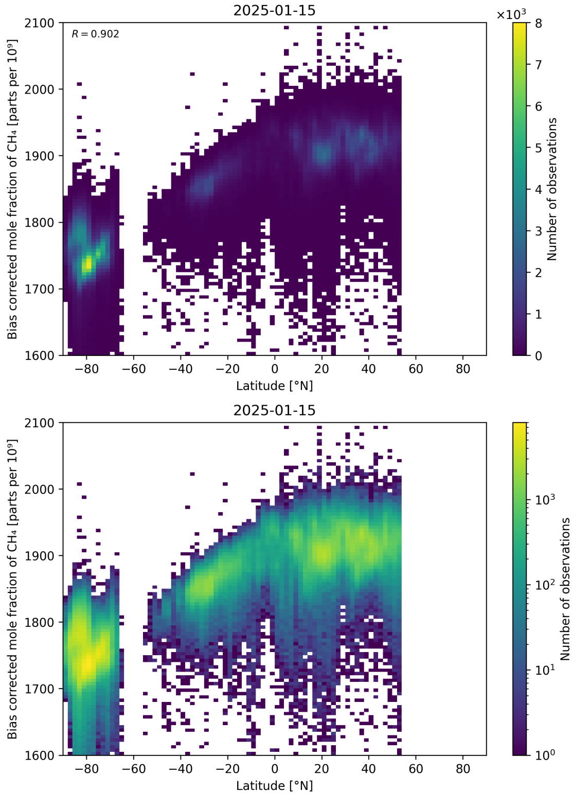
Figure 58: Scatter density plot of “Latitude” against “Bias corrected mole fraction of \text{CH}_4 ” for 2025-01-14 to 2025-01-16.
