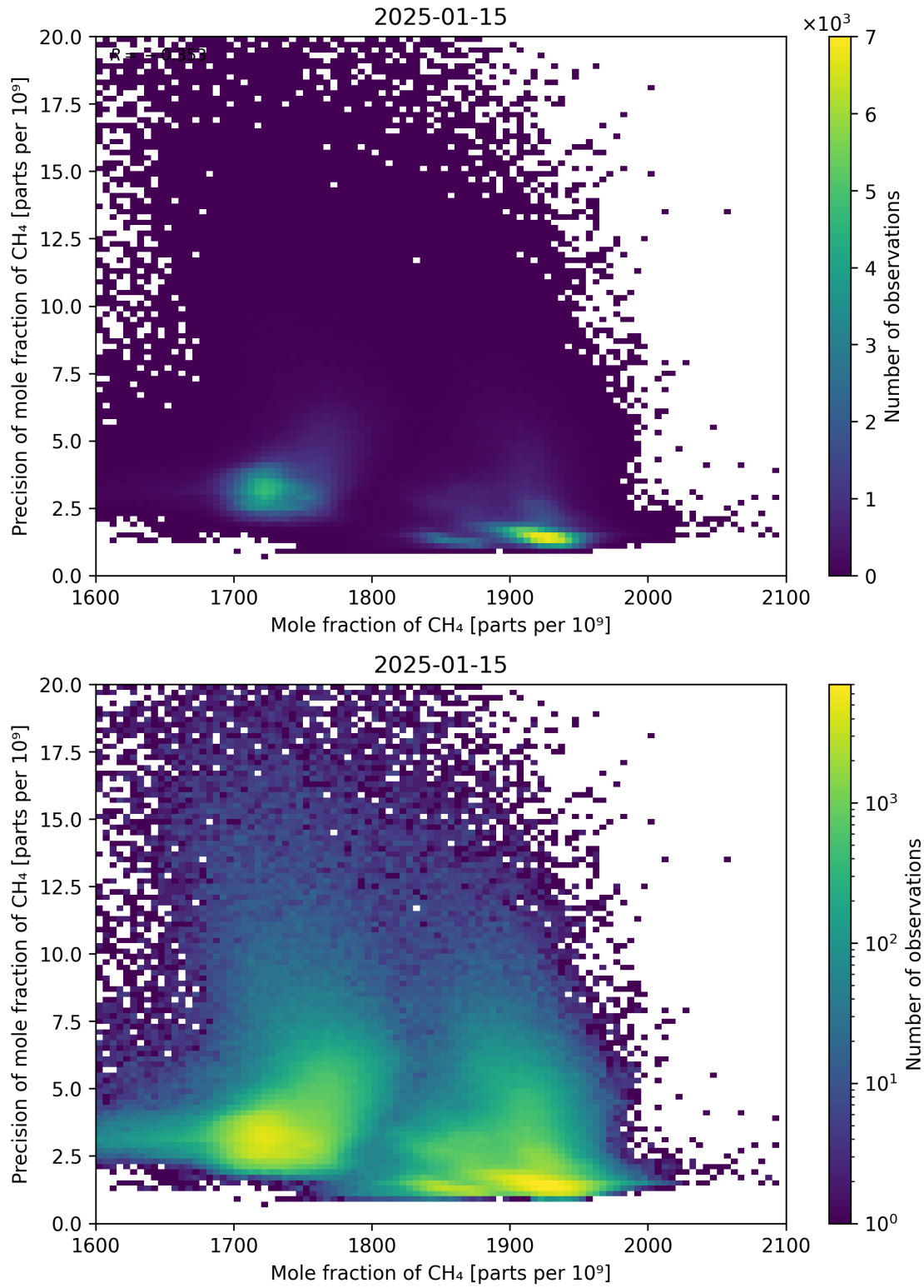
Figure 75: Scatter density plot of “Mole fraction of CH 4 ” against “Precision of mole fraction of CH 4 ” for 2025-01-14 to 2025-01-16.
