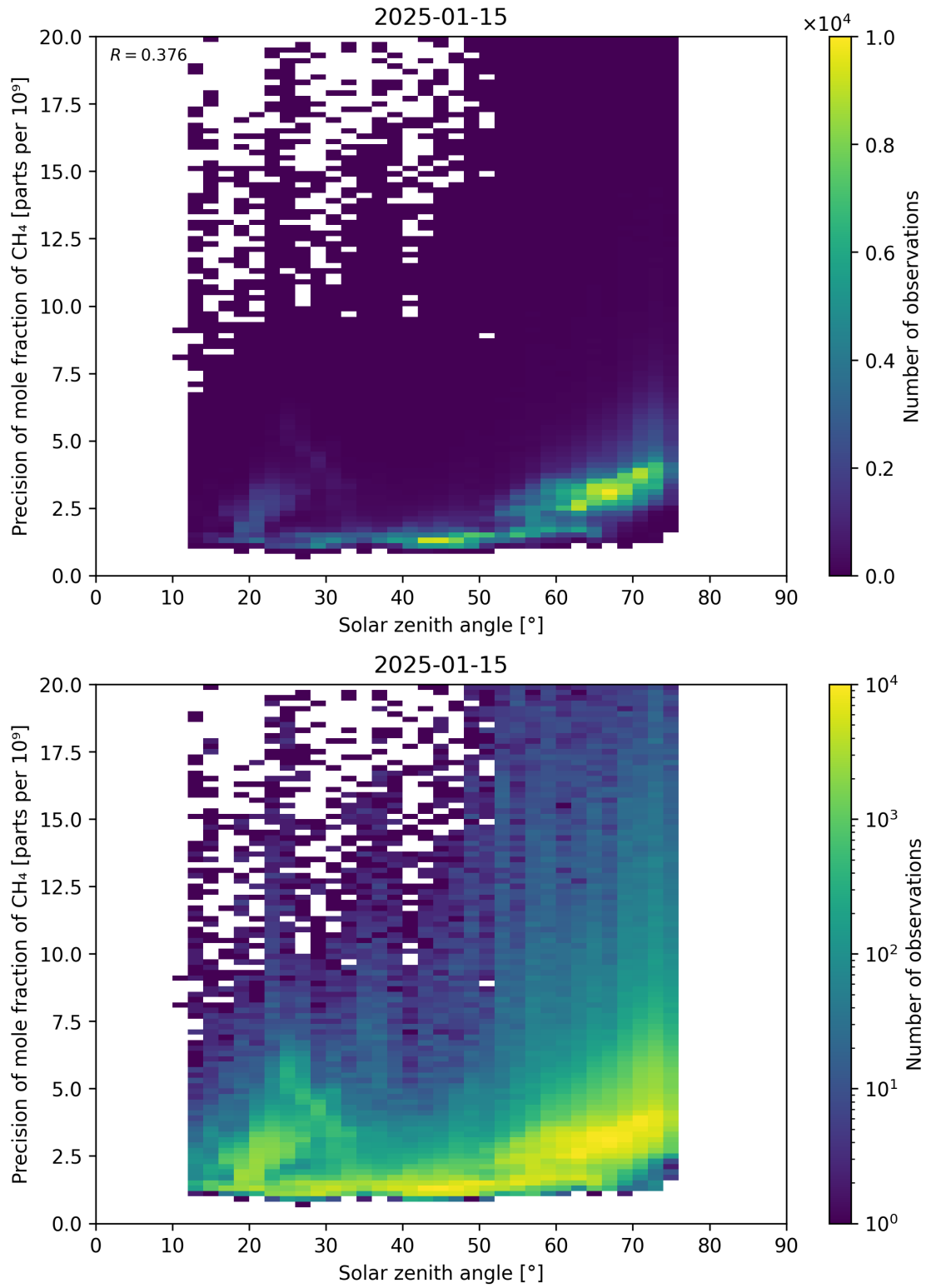
Figure 101: Scatter density plot of “Solar zenith angle” against “Precision of mole fraction of \text{CH}_4 ” for 2025-01-14 to 2025-01-16.
