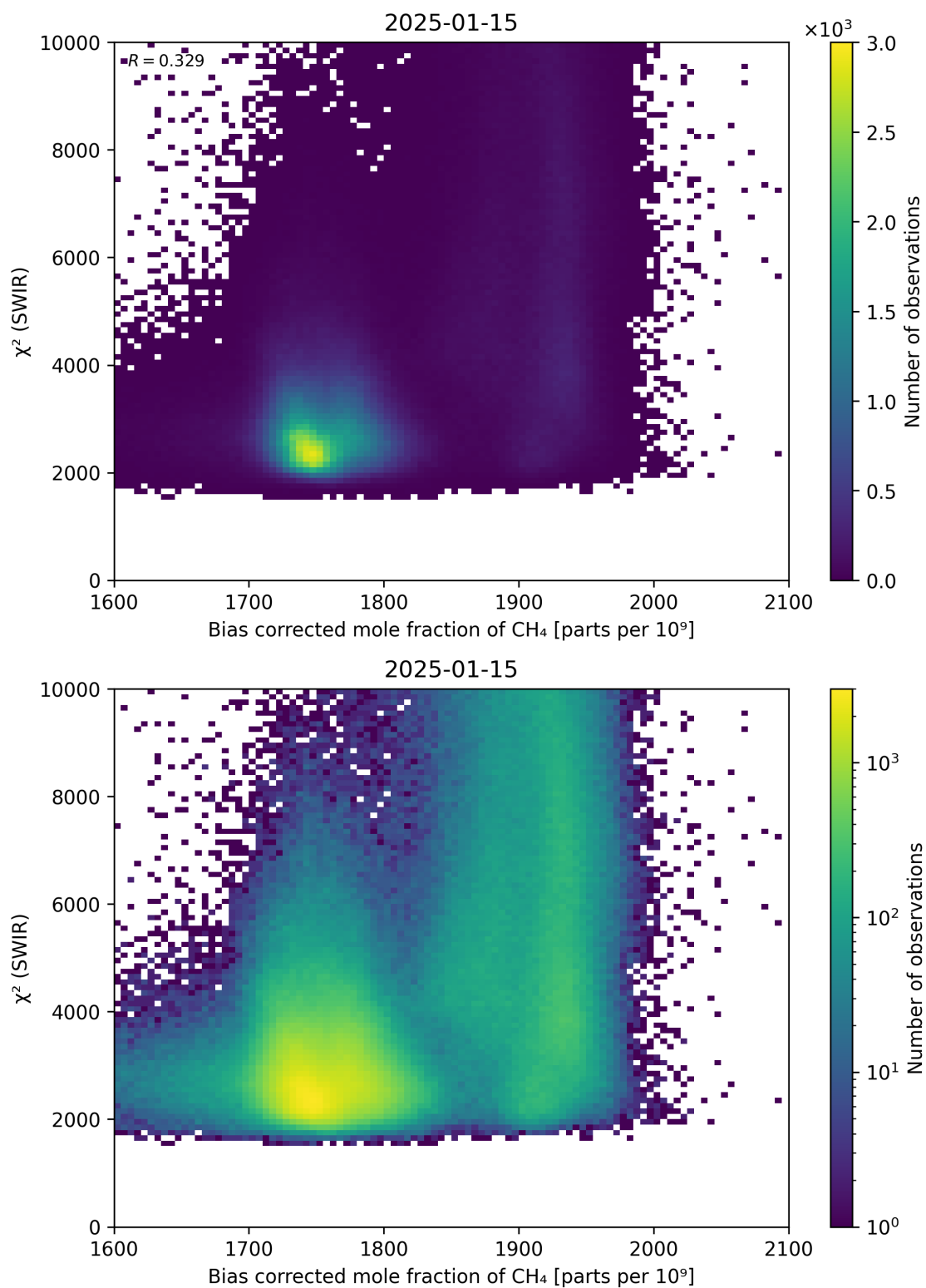
Figure 64: Scatter density plot of “Bias corrected mole fraction of \text{CH}_4 ” against “ \chi^2 (SWIR)” for 2025-01-14 to 2025-01-16.
