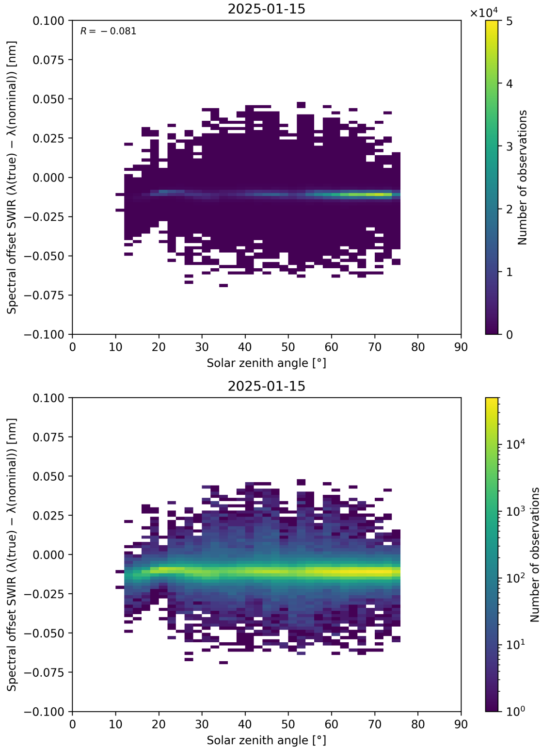
Figure 104: Scatter density plot of “Solar zenith angle” against “Spectral offset SWIR ( \lambda_{\text{true}} - \lambda_{\text{nominal}} )” for 2025-01-14 to 2025-01-16.
