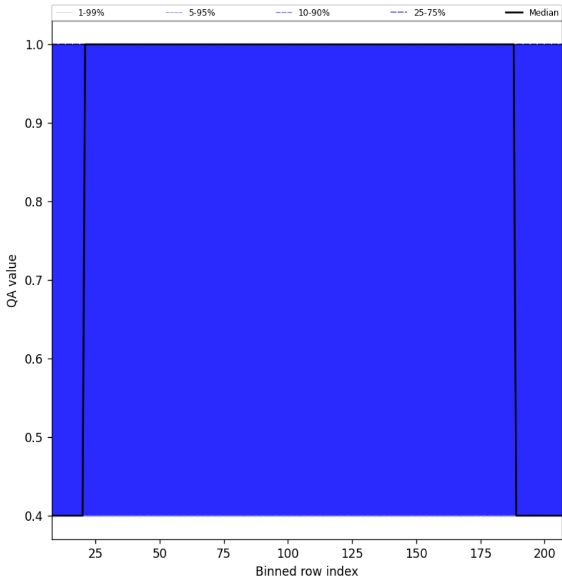
Figure 33: Along track statistics of “QA value” for 2025-01-14 to 2025-01-16
