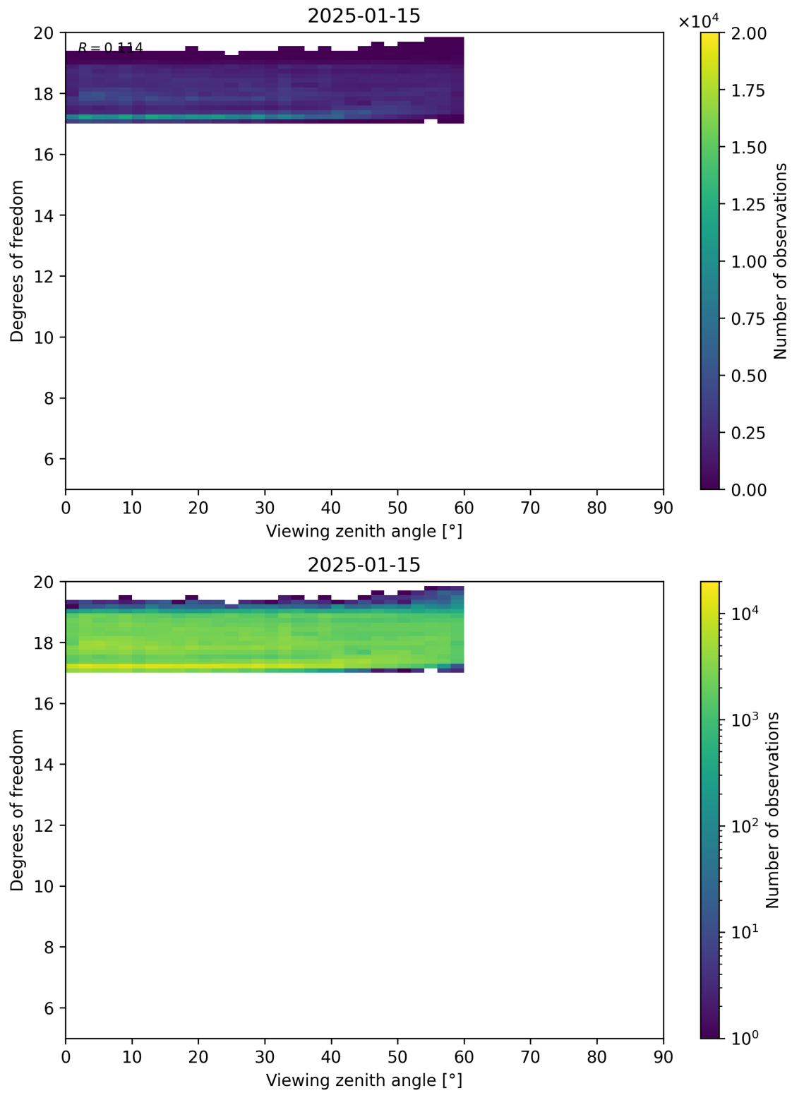
Figure 107: Scatter density plot of “Viewing zenith angle” against “Degrees of freedom” for 2025-01-14 to 2025-01-16.
