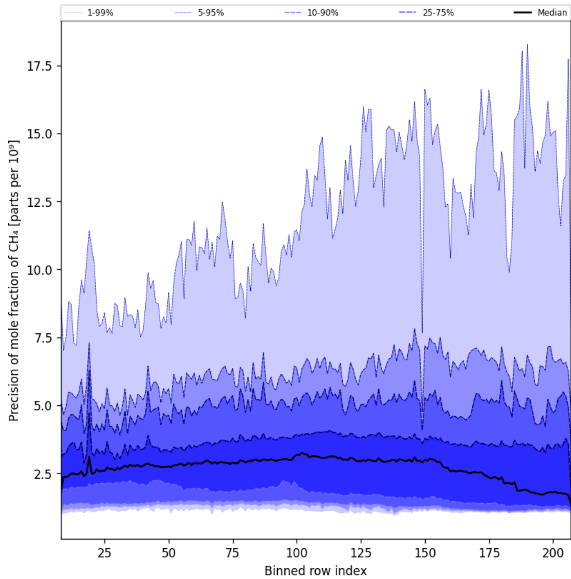
Figure 35: Along track statistics of “Precision of mole fraction of CH 4 ” for 2025-01-14 to 2025-01-16
