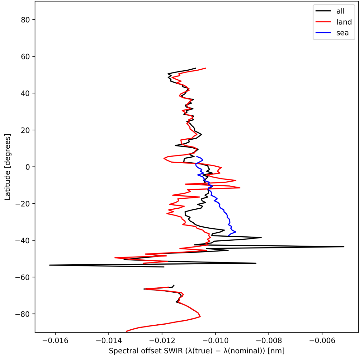
Figure 16: Zonal average of “Spectral offset SWIR ( \lambda_{\text{true}} - \lambda_{\text{nominal}} )” for 2025-01-14 to 2025-01-16.
