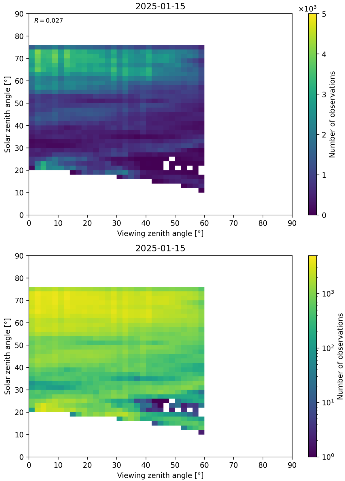
Figure 115: Scatter density plot of “Viewing zenith angle” against “Solar zenith angle” for 2025-01-14 to 2025-01-16.
