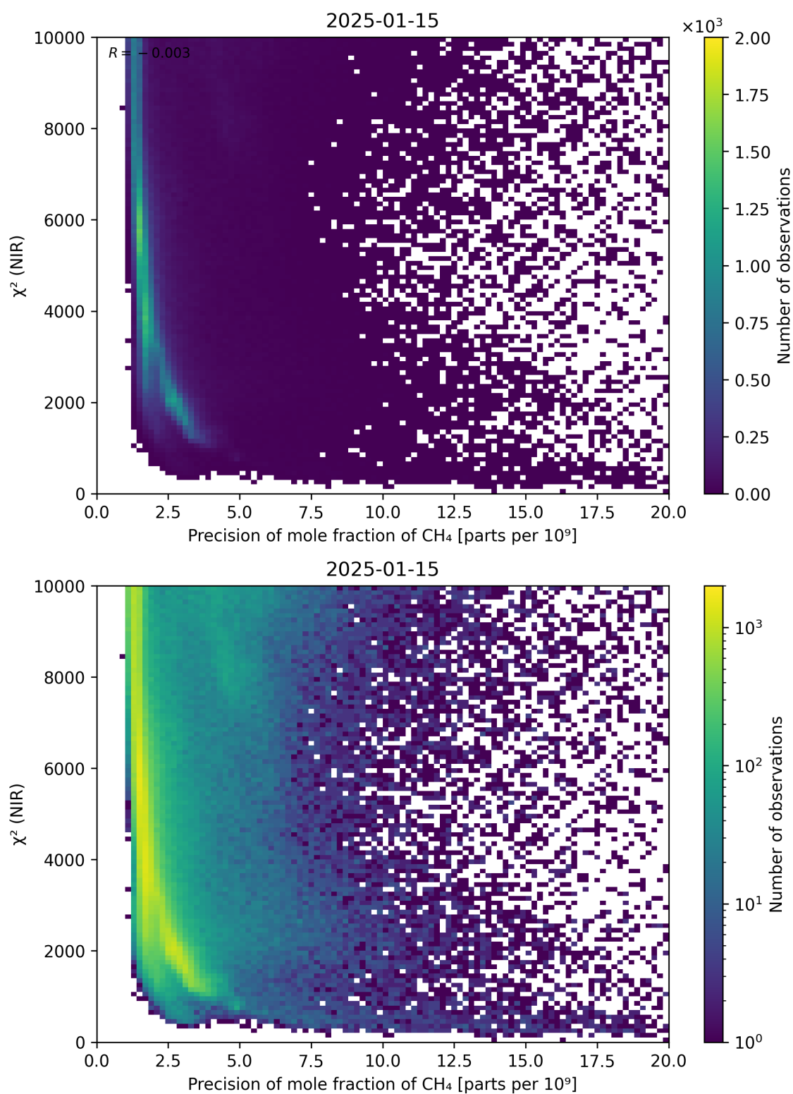
Figure 78: Scatter density plot of “Precision of mole fraction of CH 4 ” against “ \chi^2 (NIR)” for 2025-01-14 to 2025-01-16.
