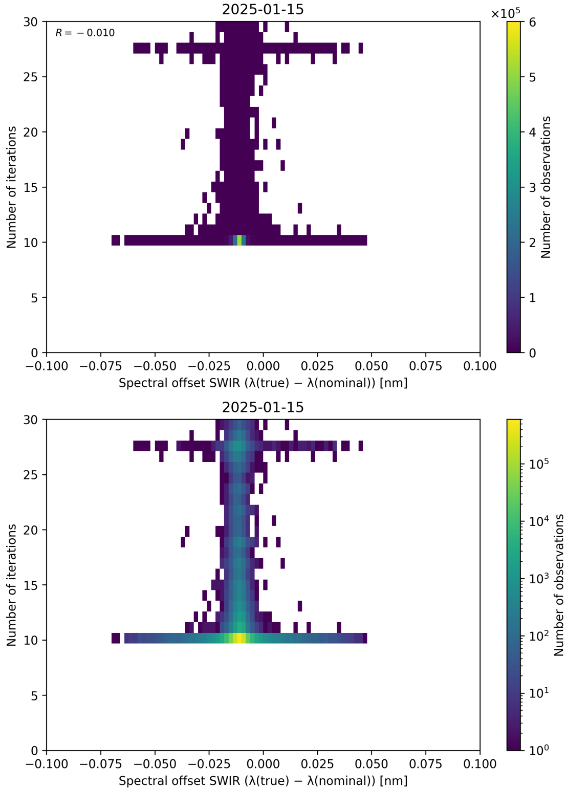
Figure 121: Scatter density plot of “Spectral offset SWIR ( \lambda_{\text{true}} - \lambda_{\text{nominal}} )” against “Number of iterations” for 2025-01-14 to 2025-01-16.
