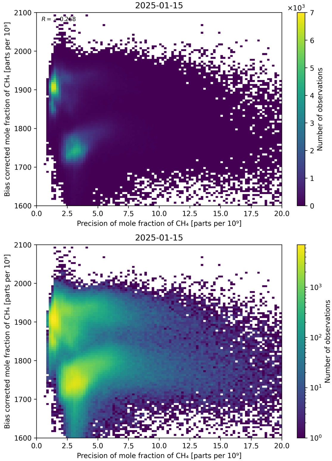
Figure 82: Scatter density plot of “Precision of mole fraction of CH 4 ” against “Bias corrected mole fraction of CH 4 ” for 2025-01-14 to 2025-01-16.
