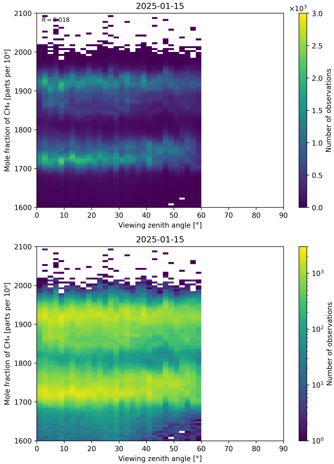
Figure 110: Scatter density plot of “Viewing zenith angle” against “Mole fraction of CH 4 ” for 2025-01-14 to 2025-01-16.
