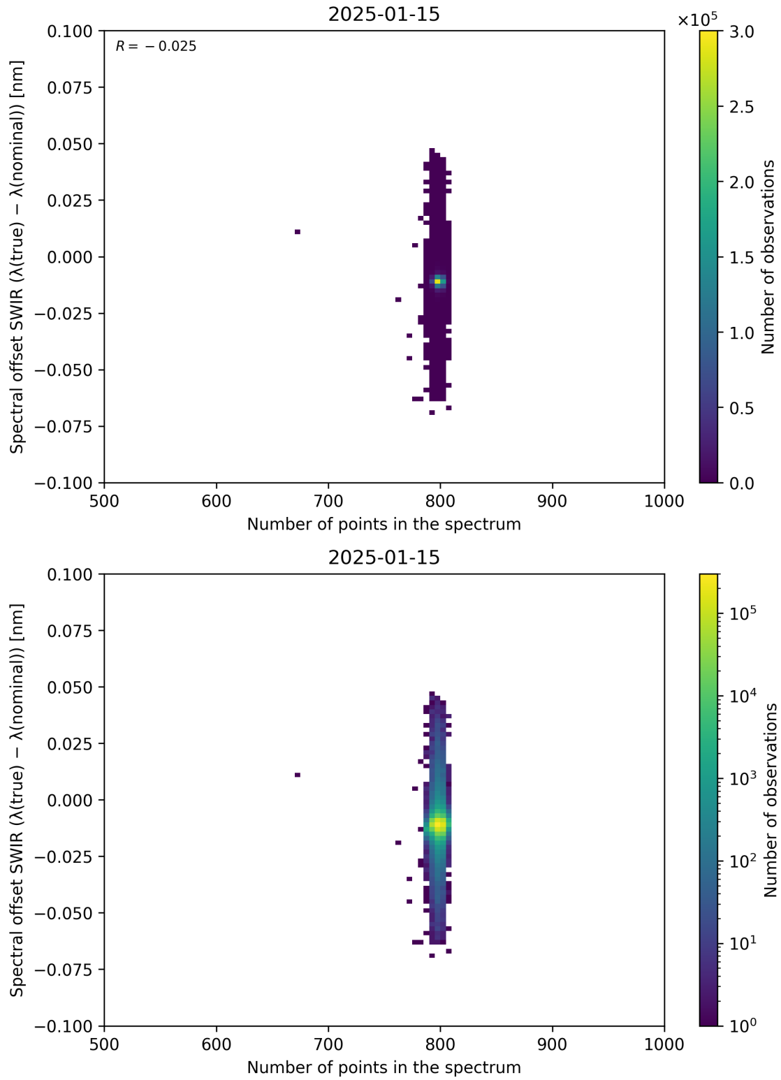
Figure 93: Scatter density plot of “Number of points in the spectrum” against “Spectral offset SWIR ( \lambda_{\text{true}} - \lambda_{\text{nominal}} )” for 2025-01-14 to 2025-01-16.
