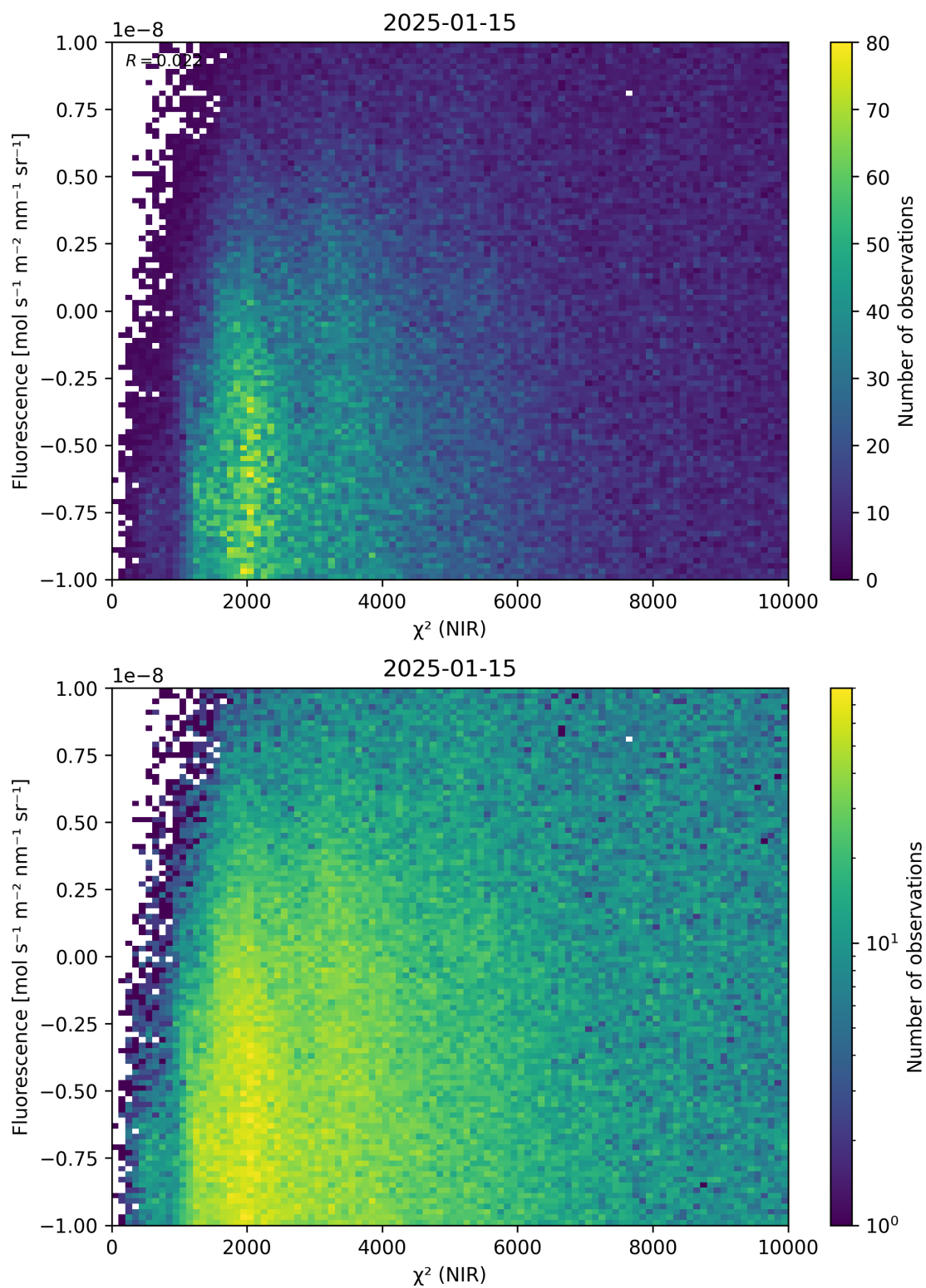
Figure 45: Scatter density plot of “ \chi^2 (NIR)” against “Fluorescence” for 2025-01-14 to 2025-01-16.
