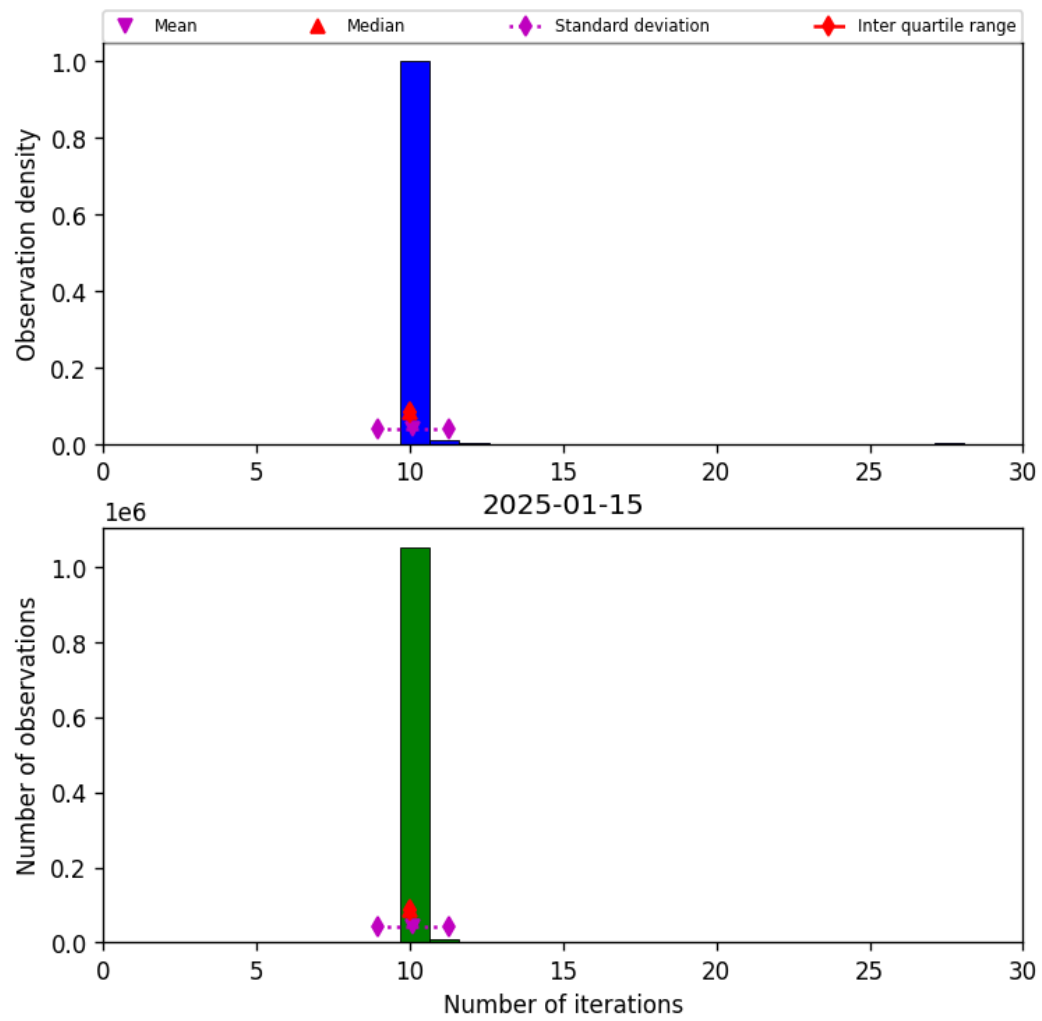
Figure 31: Histogram of “Number of iterations” for 2025-01-14 to 2025-01-16
