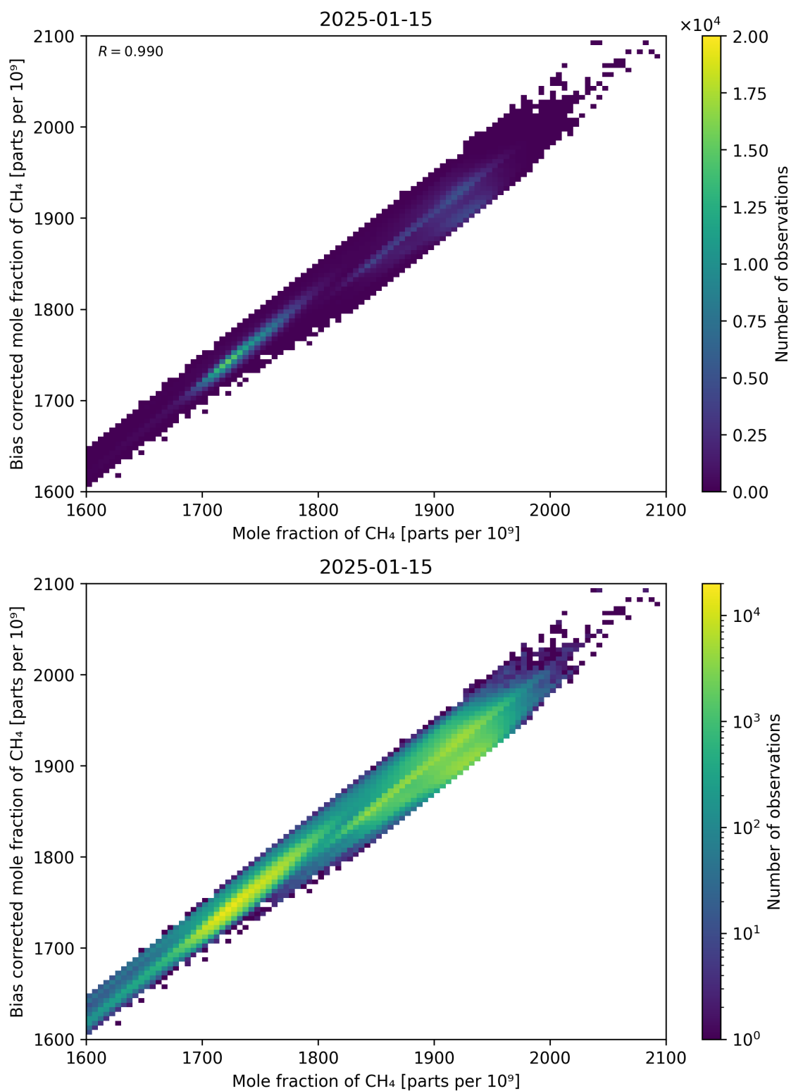
Figure 74: Scatter density plot of “Mole fraction of CH 4 ” against “Bias corrected mole fraction of CH 4 ” for 2025-01-14 to 2025-01-16.
