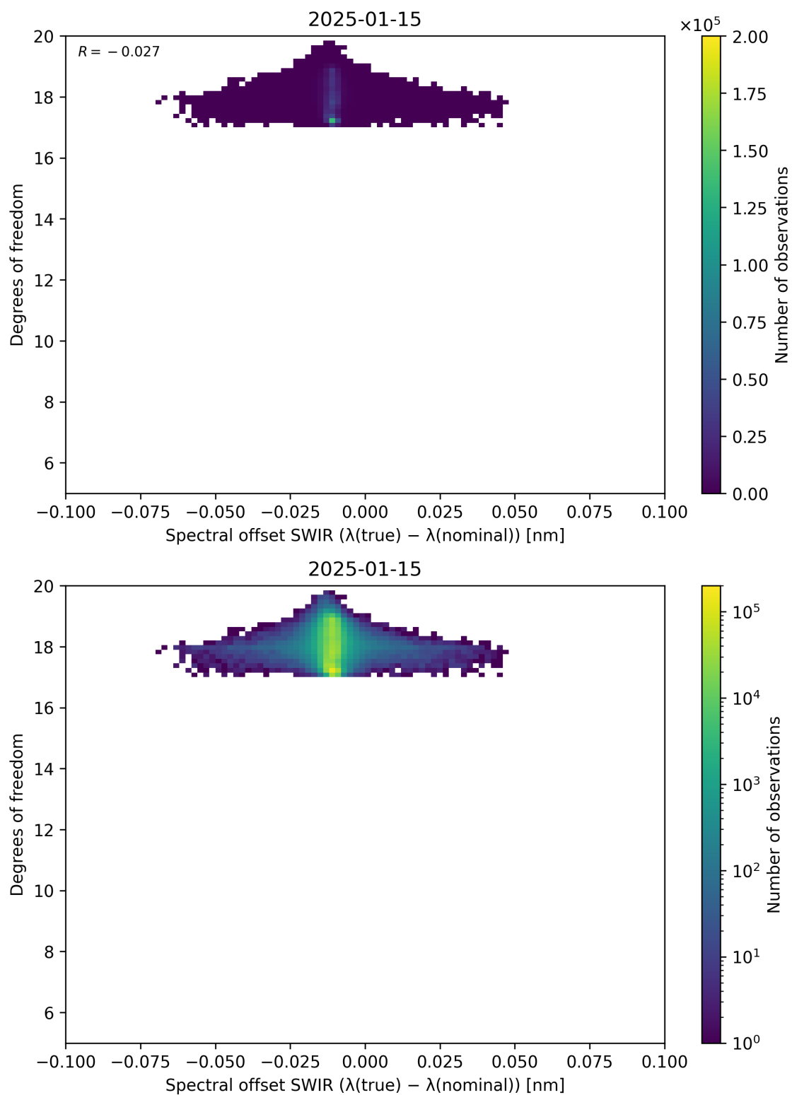
Figure 119: Scatter density plot of “Spectral offset SWIR ( \lambda_{\text{true}} - \lambda_{\text{nominal}} )” against “Degrees of freedom” for 2025-01-14 to 2025-01-16.
