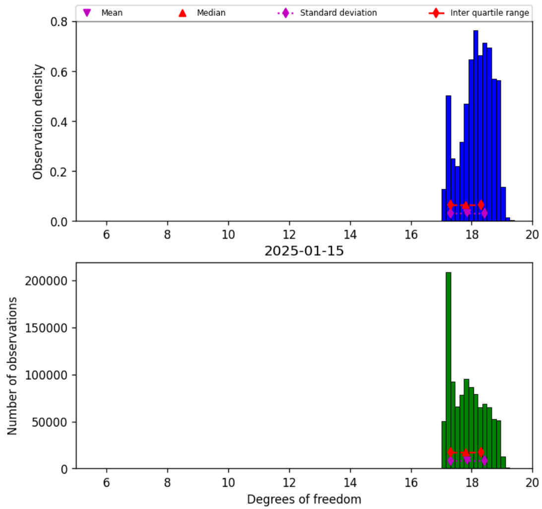
Figure 30: Histogram of “Degrees of freedom” for 2025-01-14 to 2025-01-16
