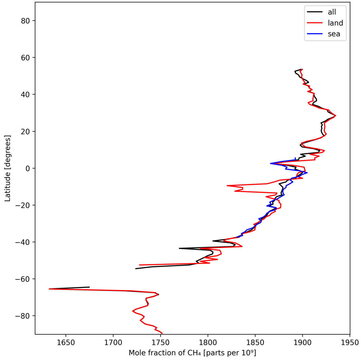
Figure 12: Zonal average of “Mole fraction of CH 4 ” for 2025-01-14 to 2025-01-16.
