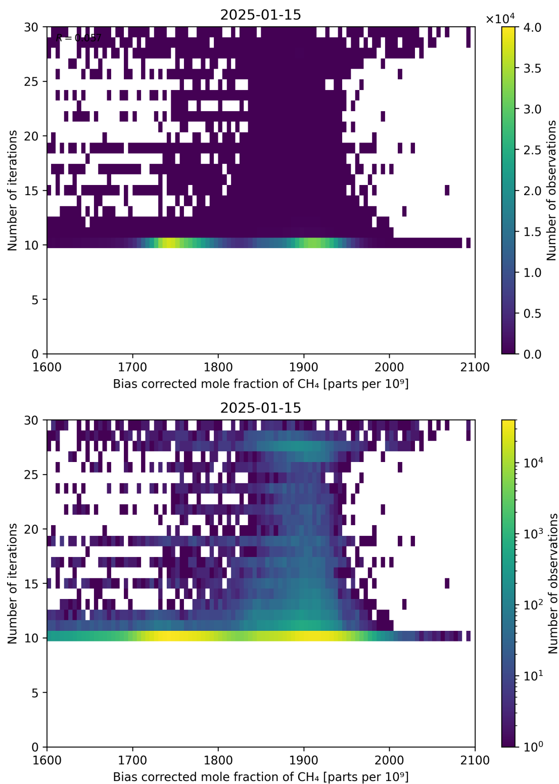
Figure 67: Scatter density plot of “Bias corrected mole fraction of \text{CH}_4 ” against “Number of iterations” for 2025-01-14 to 2025-01-16.
