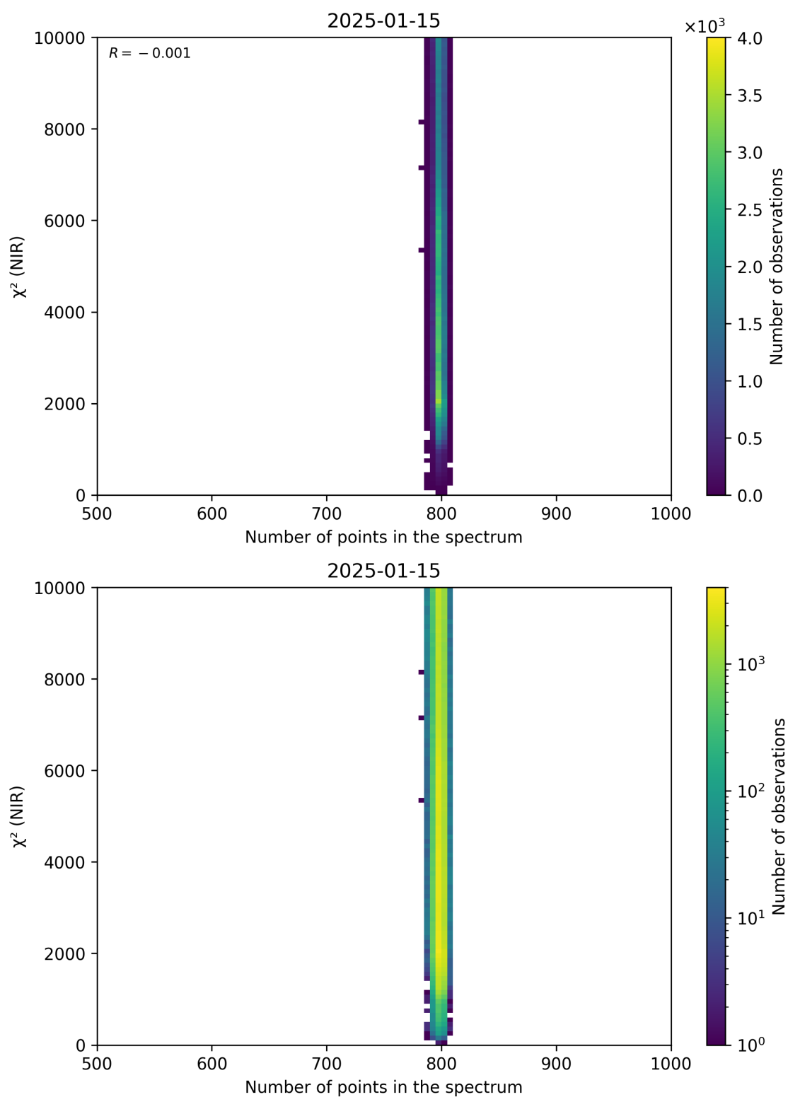
Figure 88: Scatter density plot of “Number of points in the spectrum” against “ \chi^2 (NIR)” for 2025-01-14 to 2025-01-16.
