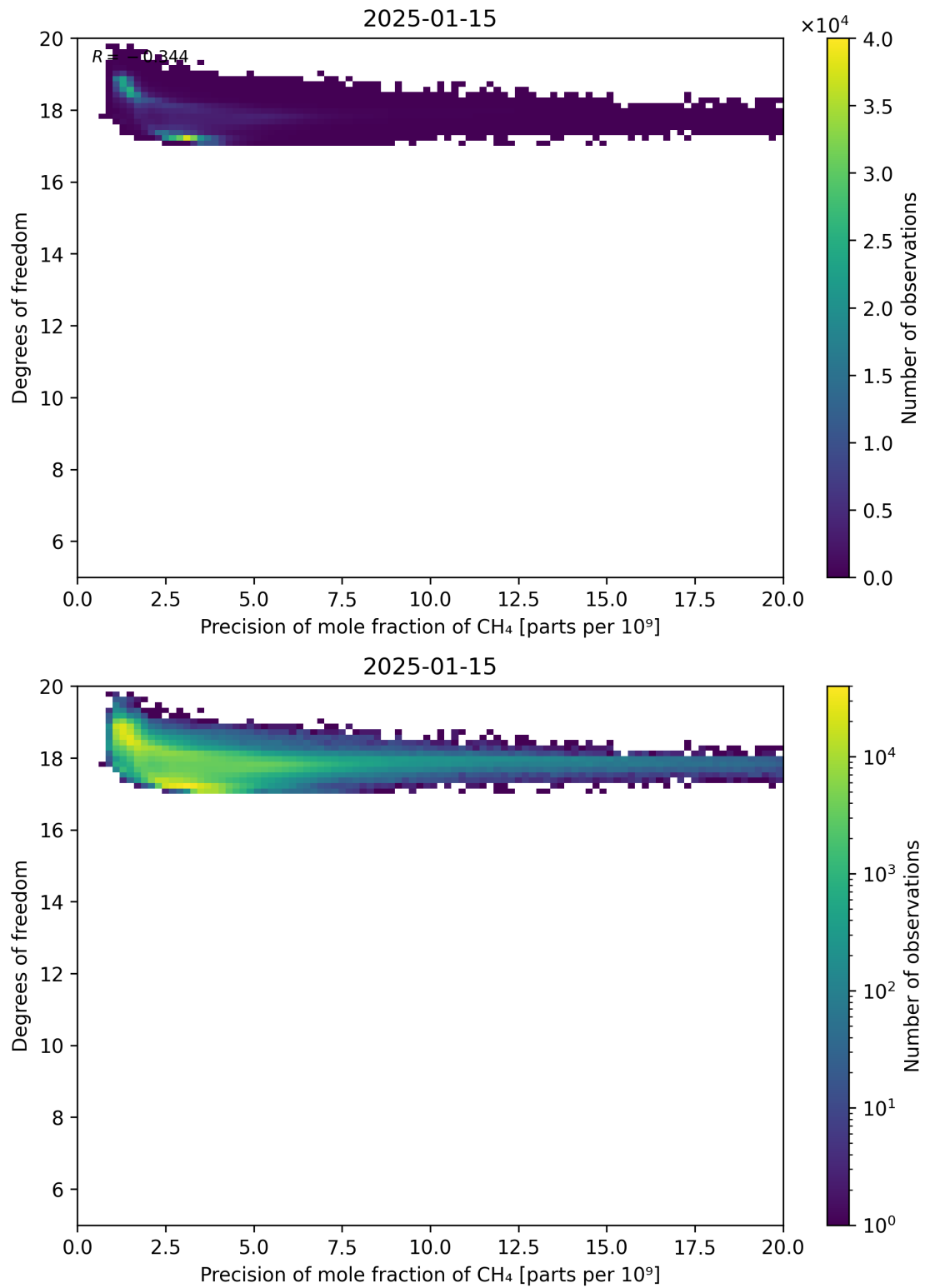
Figure 80: Scatter density plot of “Precision of mole fraction of CH 4 ” against “Degrees of freedom” for 2025-01-14 to 2025-01-16.
