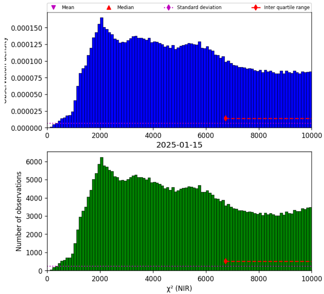
Figure 29: Histogram of “ \chi^2 (NIR)” for 2025-01-14 to 2025-01-16
