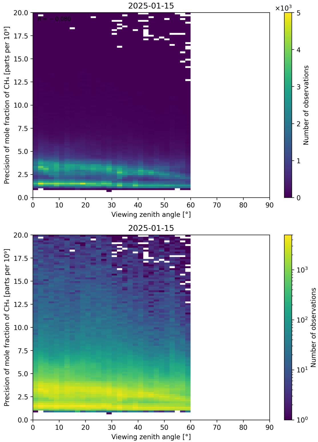
Figure 112: Scatter density plot of “Viewing zenith angle” against “Precision of mole fraction of CH 4 ” for 2025-01-14 to 2025-01-16.
