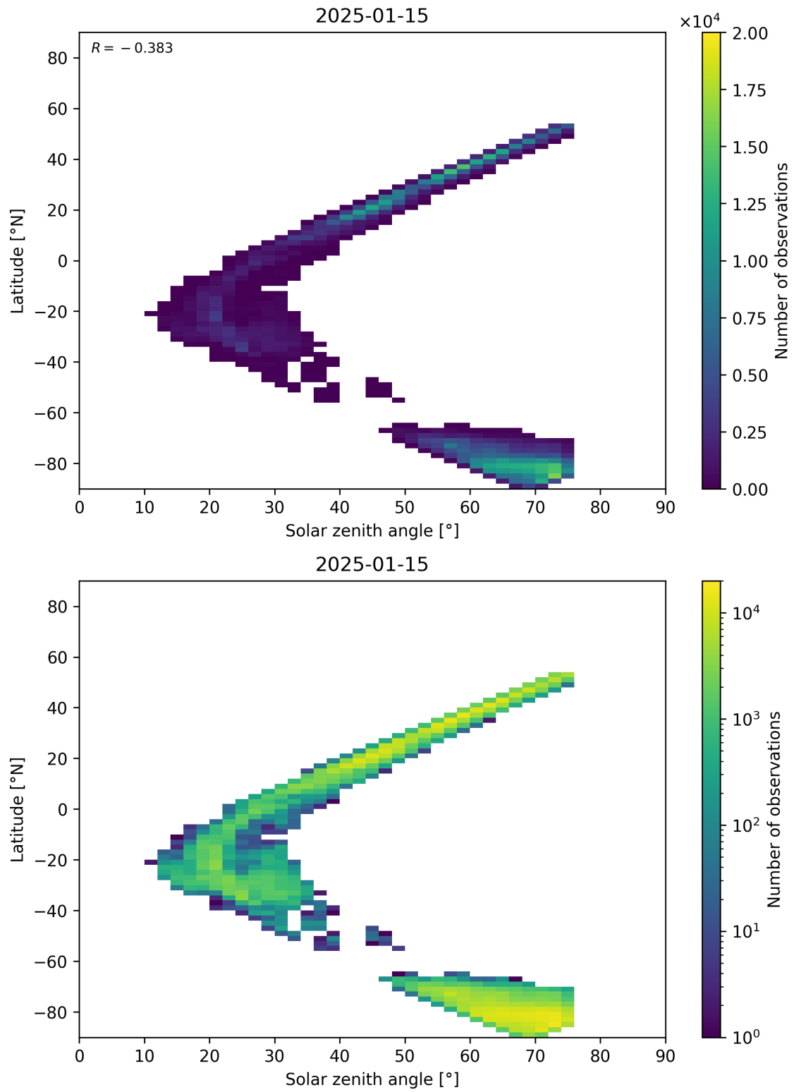
Figure 98: Scatter density plot of “Solar zenith angle” against “Latitude” for 2025-01-14 to 2025-01-16.
