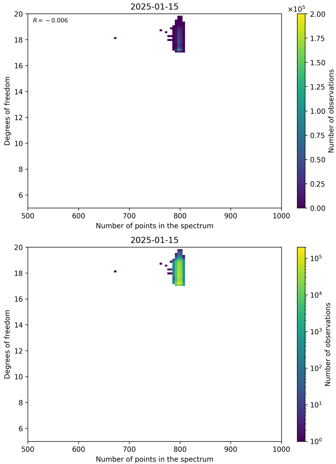
Figure 90: Scatter density plot of “Number of points in the spectrum” against “Degrees of freedom” for 2025-01-14 to 2025-01-16.
