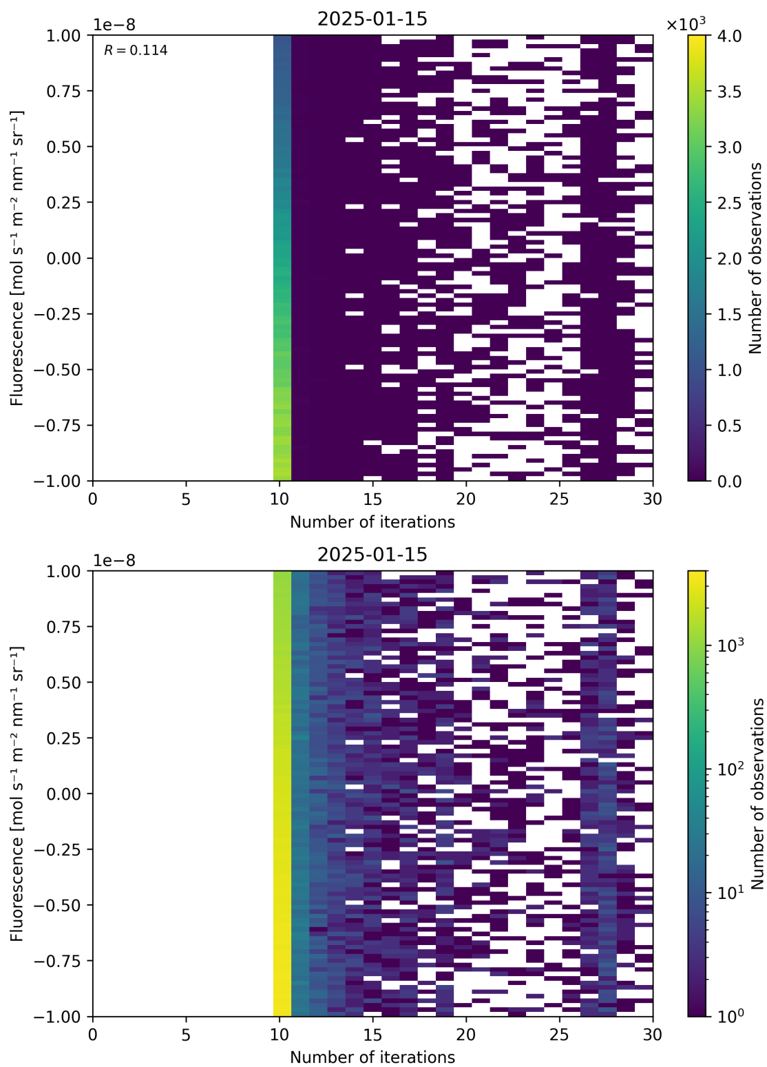
Figure 87: Scatter density plot of “Number of iterations” against “Fluorescence” for 2025-01-14 to 2025-01-16.
