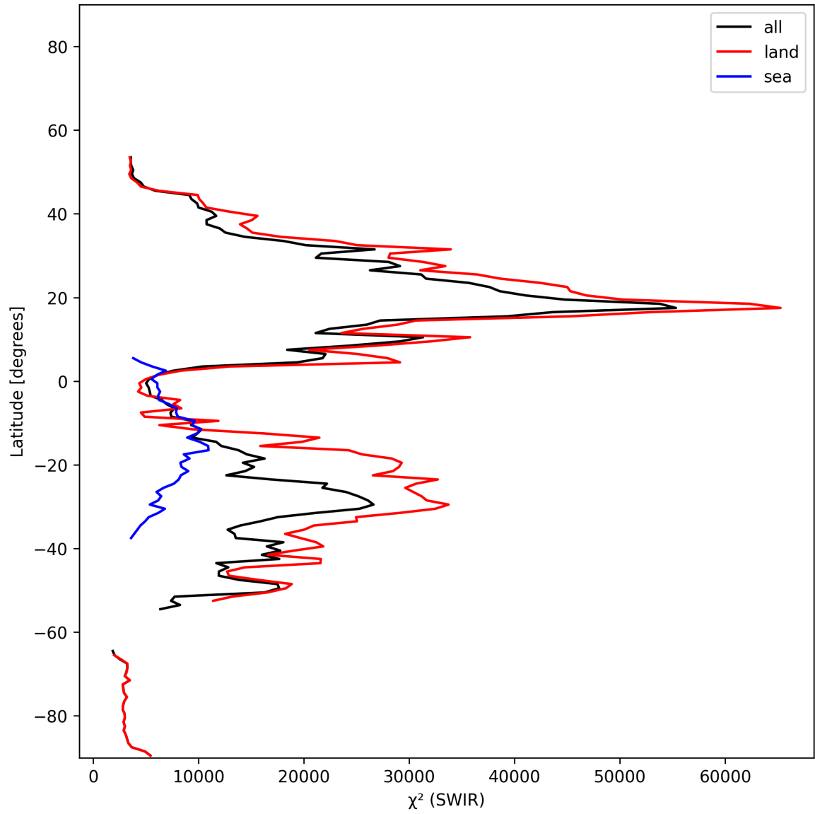
Figure 17: Zonal average of “ \chi^2 (SWIR)” for 2025-01-14 to 2025-01-16.
