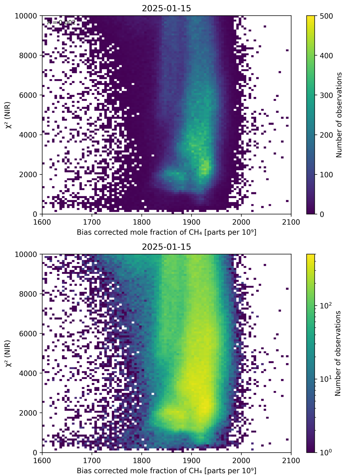
Figure 63: Scatter density plot of “Bias corrected mole fraction of \text{CH}_4 ” against “ \chi^2 (NIR)” for 2025-01-14 to 2025-01-16.
