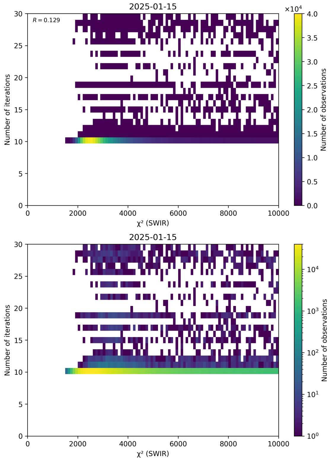
Figure 50: Scatter density plot of “ \chi^2 (SWIR)” against “Number of iterations” for 2025-01-14 to 2025-01-16.
