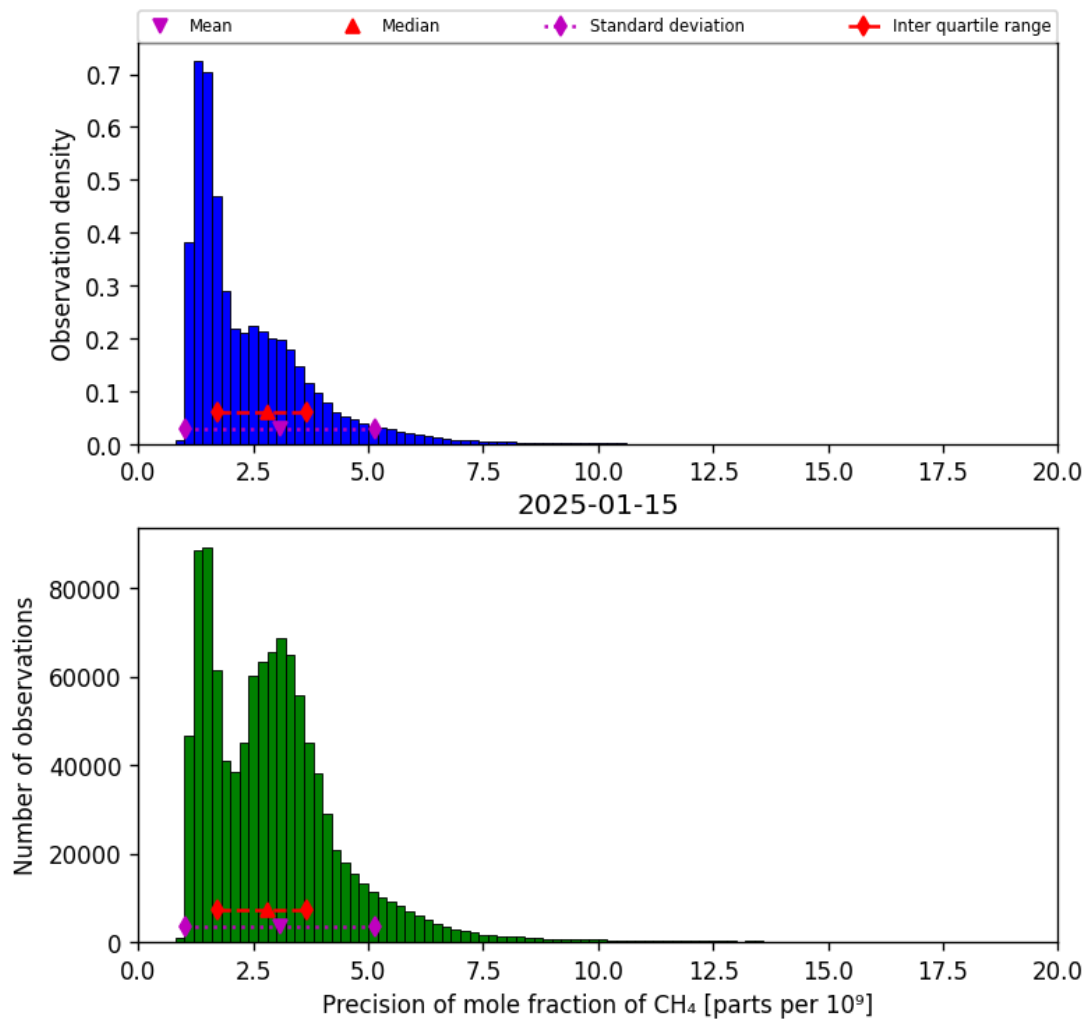
Figure 24: Histogram of “Precision of mole fraction of CH 4 ” for 2025-01-14 to 2025-01-16
