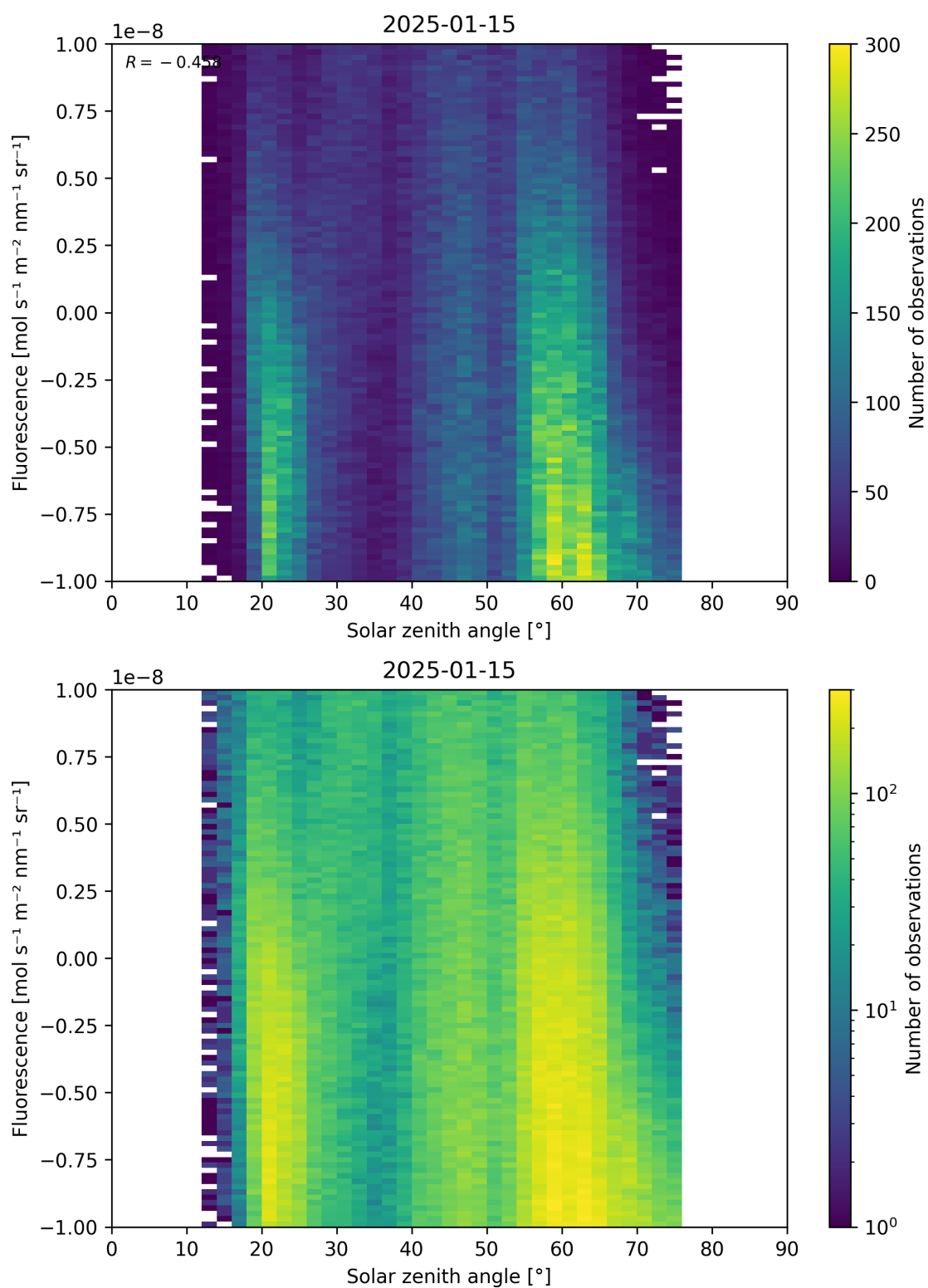
Figure 97: Scatter density plot of “Solar zenith angle” against “Fluorescence” for 2025-01-14 to 2025-01-16.
