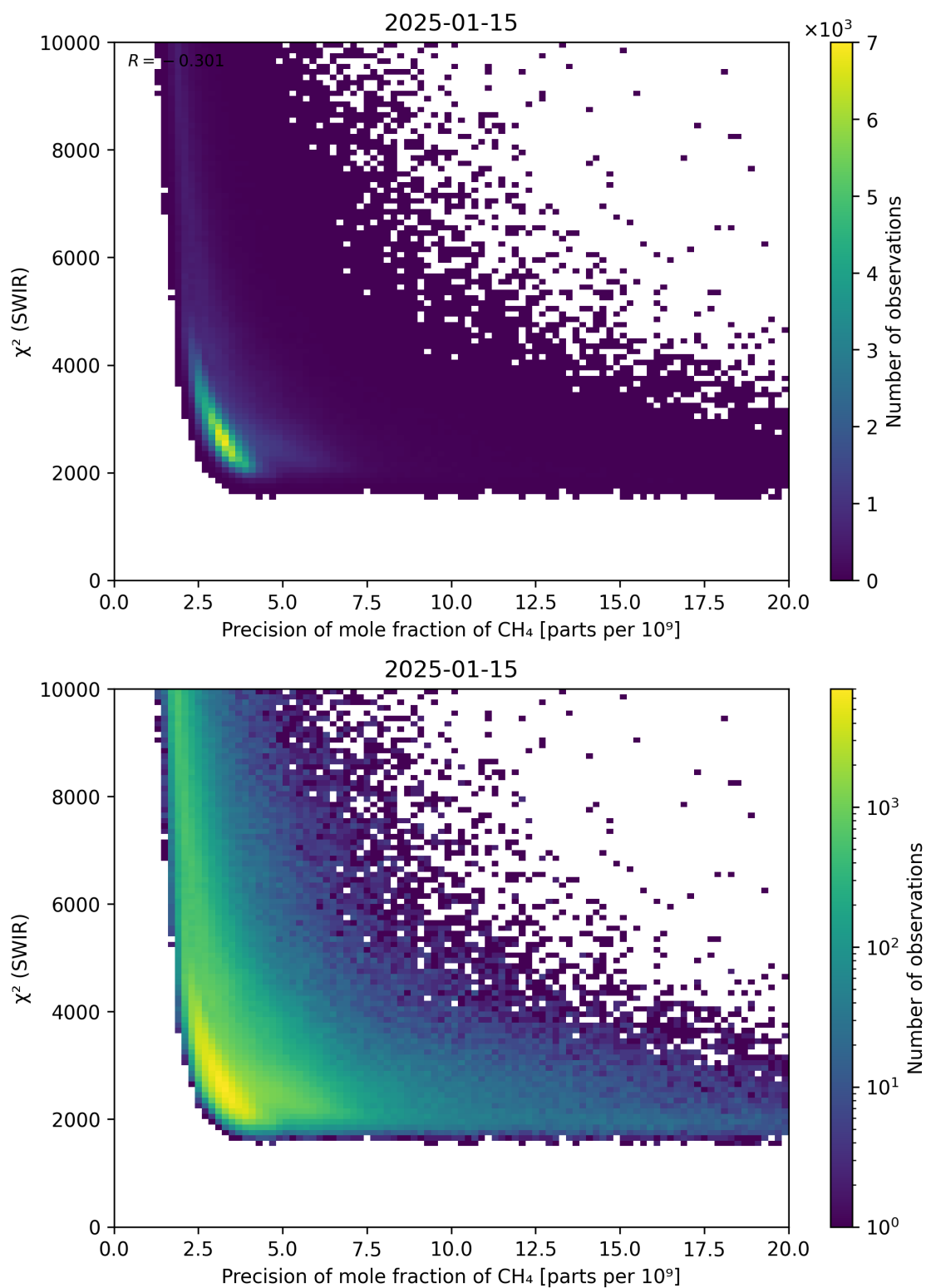
Figure 79: Scatter density plot of “Precision of mole fraction of \text{CH}_4 ” against “ \chi^2 (SWIR)” for 2025-01-14 to 2025-01-16.
