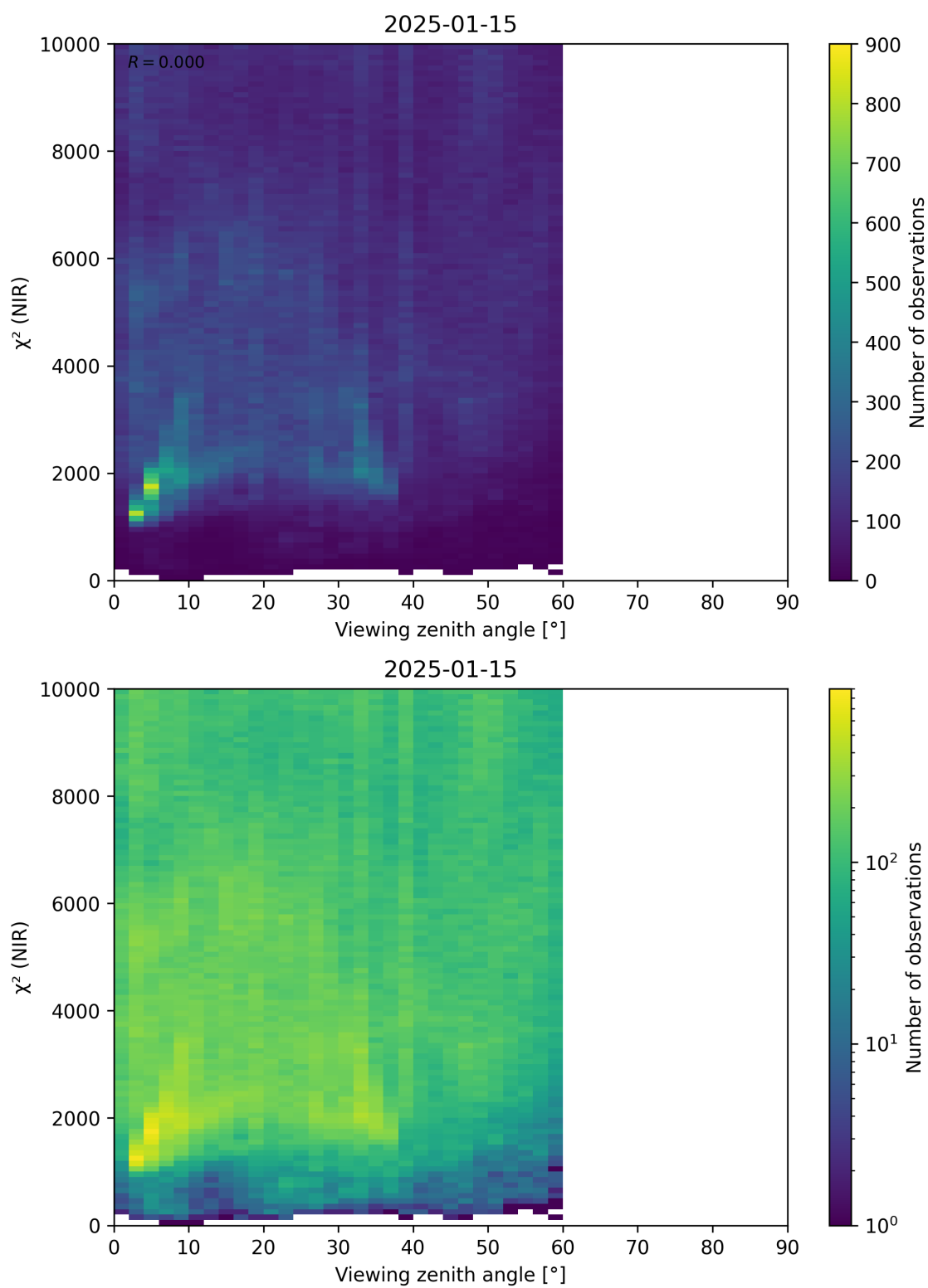
Figure 105: Scatter density plot of “Viewing zenith angle” against “ \chi^2 (NIR)” for 2025-01-14 to 2025-01-16.
