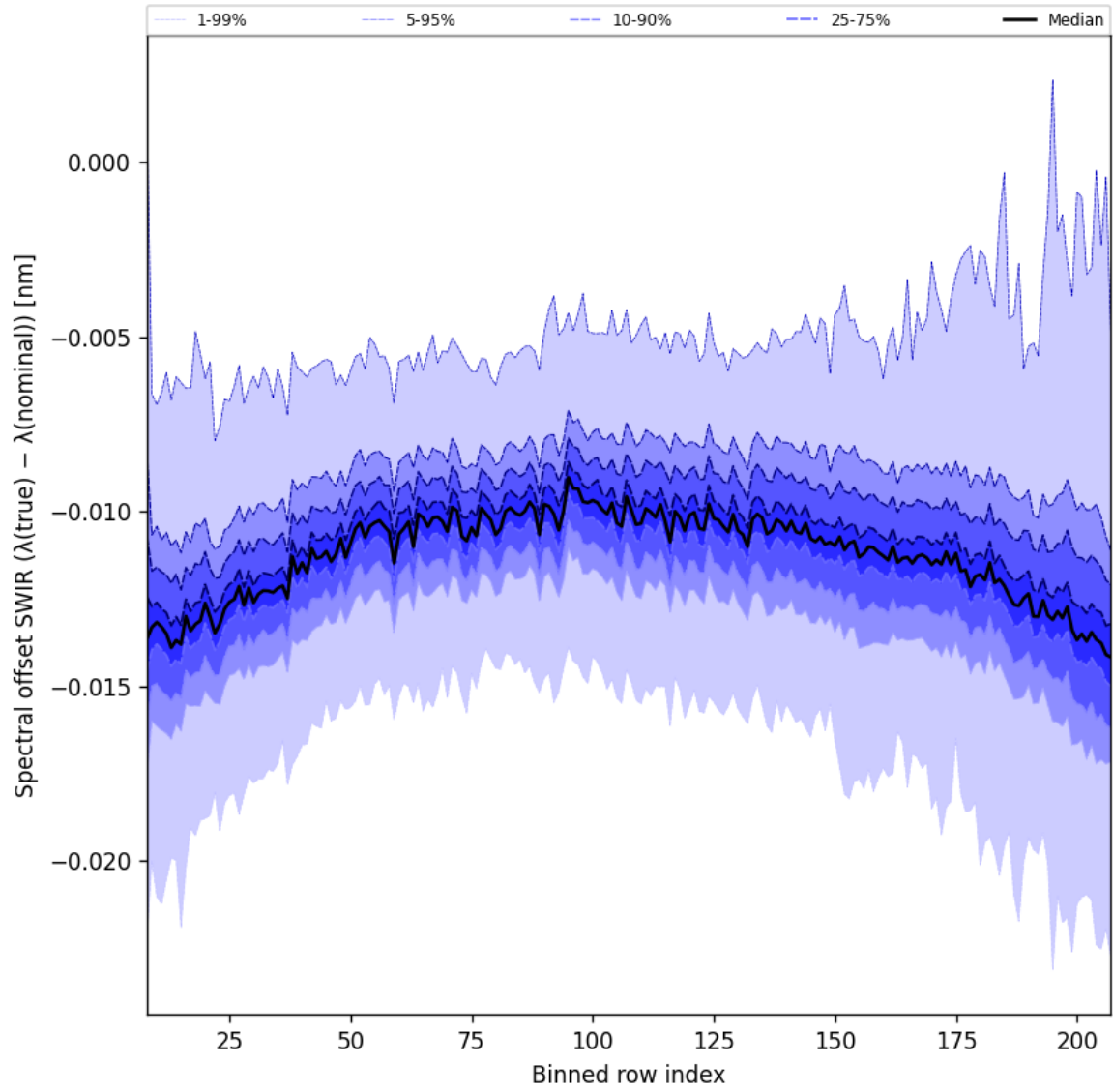
Figure 38: Along track statistics of “Spectral offset SWIR ( \lambda_{\text{true}} - \lambda_{\text{nominal}} )” for 2025-01-14 to 2025-01-16
