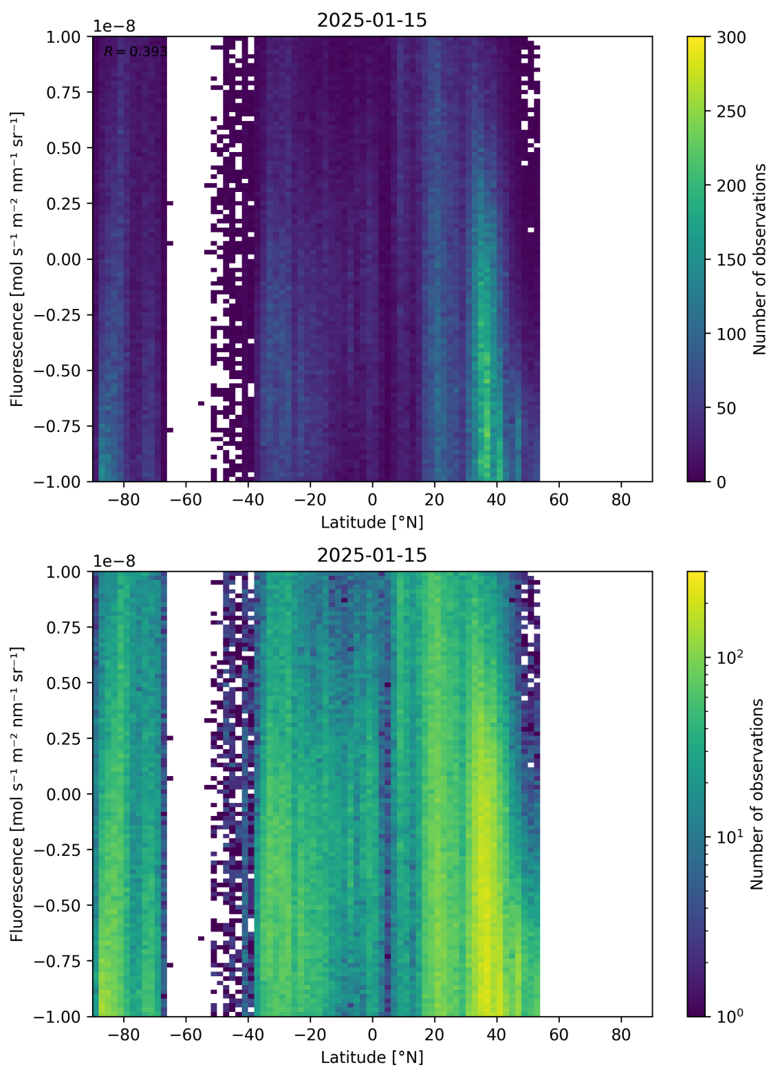
Figure 56: Scatter density plot of “Latitude” against “Fluorescence” for 2025-01-14 to 2025-01-16.
