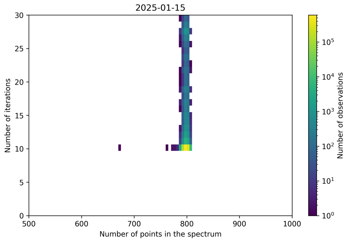
Figure 92: Scatter density plot of “Number of points in the spectrum” against “Number of iterations” for 2025-01-14 to 2025-01-16.
