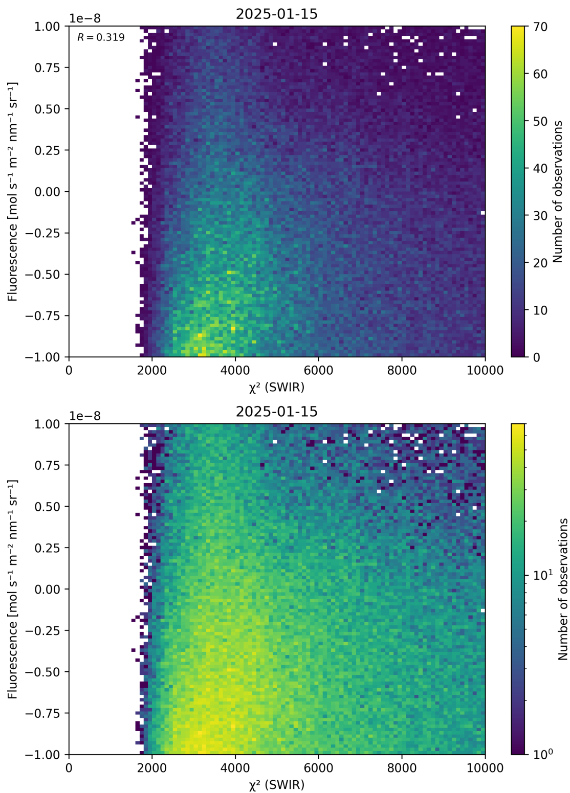
Figure 49: Scatter density plot of “ \chi^2 (SWIR)” against “Fluorescence” for 2025-01-14 to 2025-01-16.
