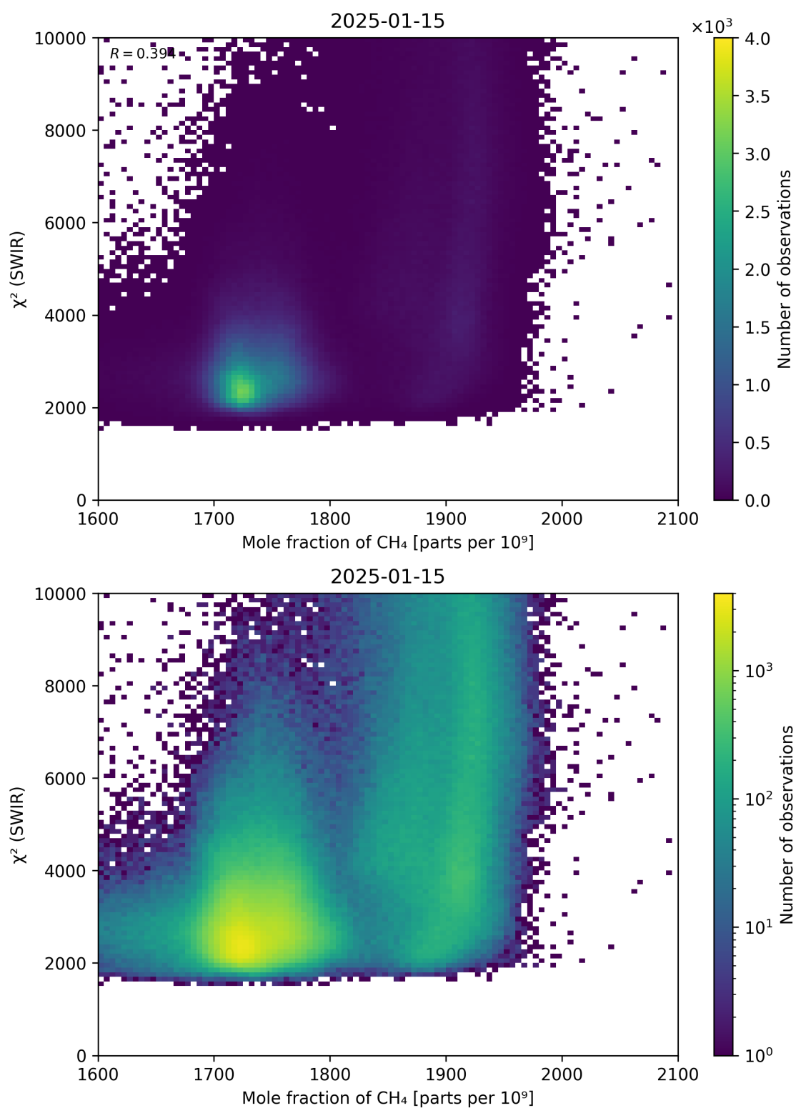
Figure 71: Scatter density plot of “Mole fraction of \text{CH}_4 ” against “ \chi^2 (SWIR)” for 2025-01-14 to 2025-01-16.
