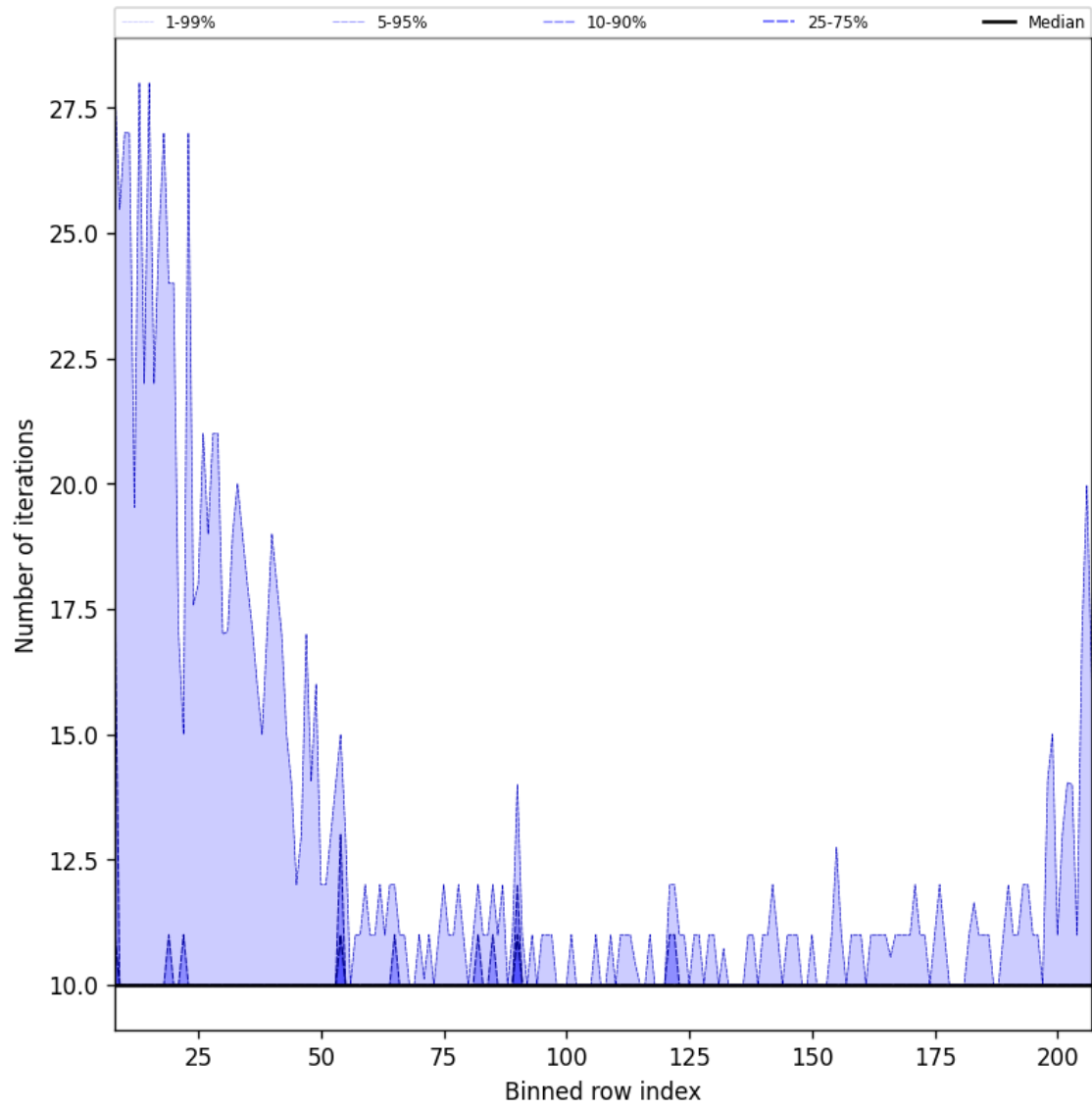
Figure 42: Along track statistics of “Number of iterations” for 2025-01-14 to 2025-01-16
