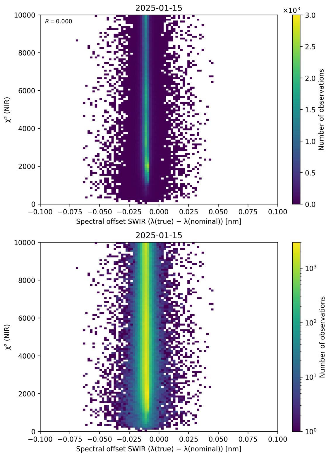
Figure 117: Scatter density plot of “Spectral offset SWIR ( \lambda_{\text{true}} - \lambda_{\text{nominal}} )” against “ \chi^2 (NIR)” for 2025-01-14 to 2025-01-16.
