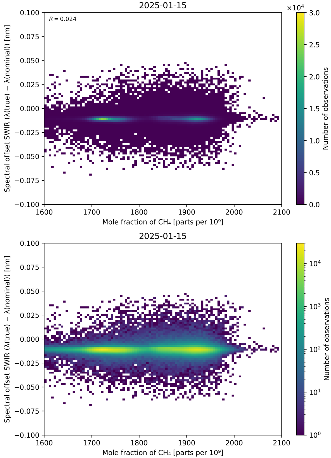
Figure 86: Scatter density plot of “Mole fraction of CH 4 ” against “Spectral offset SWIR ( \lambda_{\text{true}} - \lambda_{\text{nominal}} )” for 2025-01-14 to 2025-01-16.
