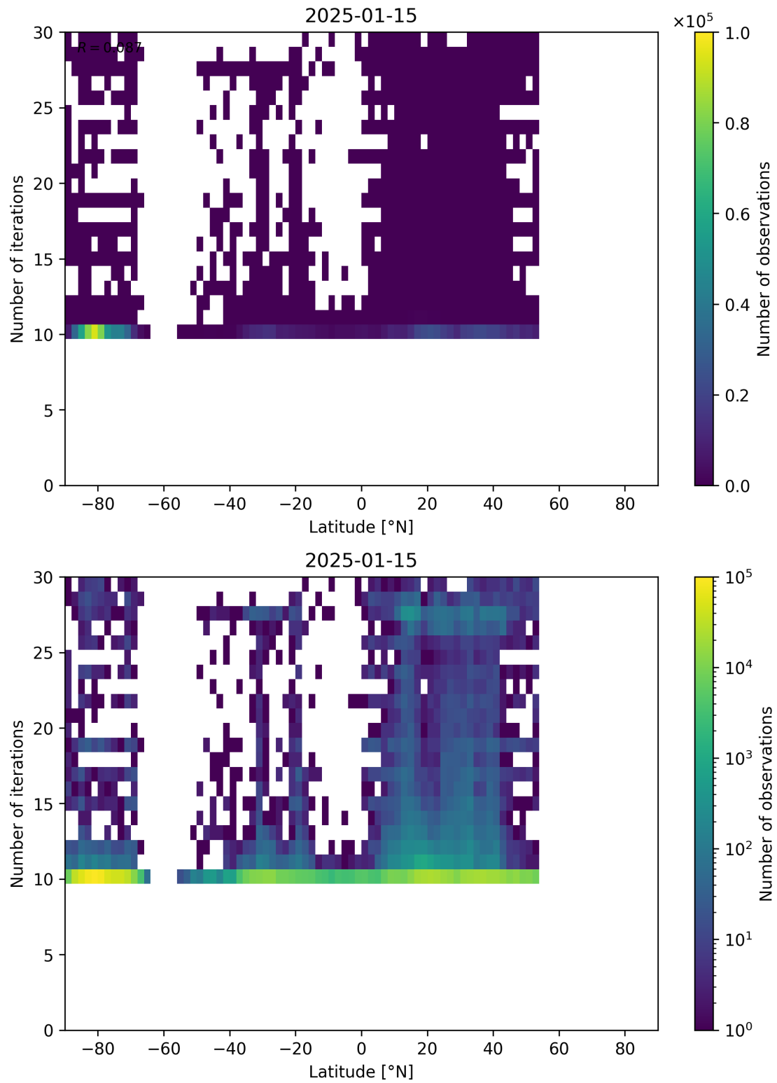
Figure 60: Scatter density plot of “Latitude” against “Number of iterations” for 2025-01-14 to 2025-01-16.
