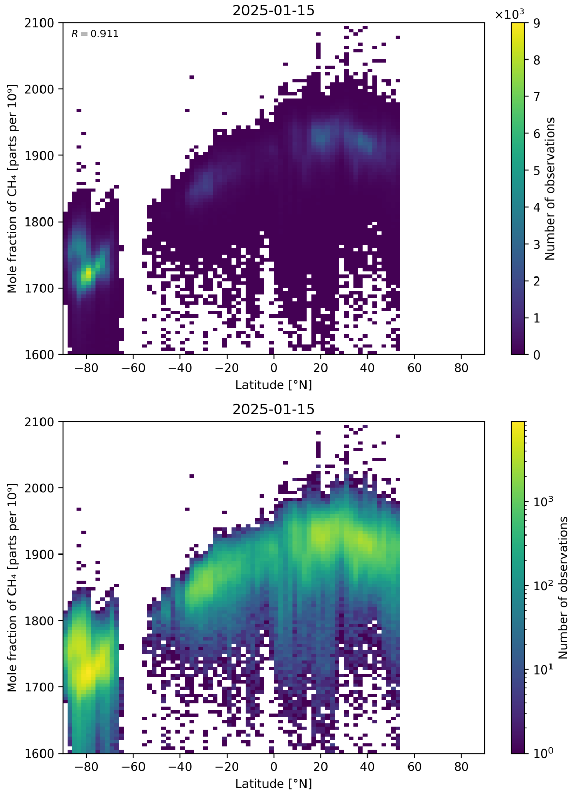
Figure 57: Scatter density plot of “Latitude” against “Mole fraction of CH 4 ” for 2025-01-14 to 2025-01-16.
