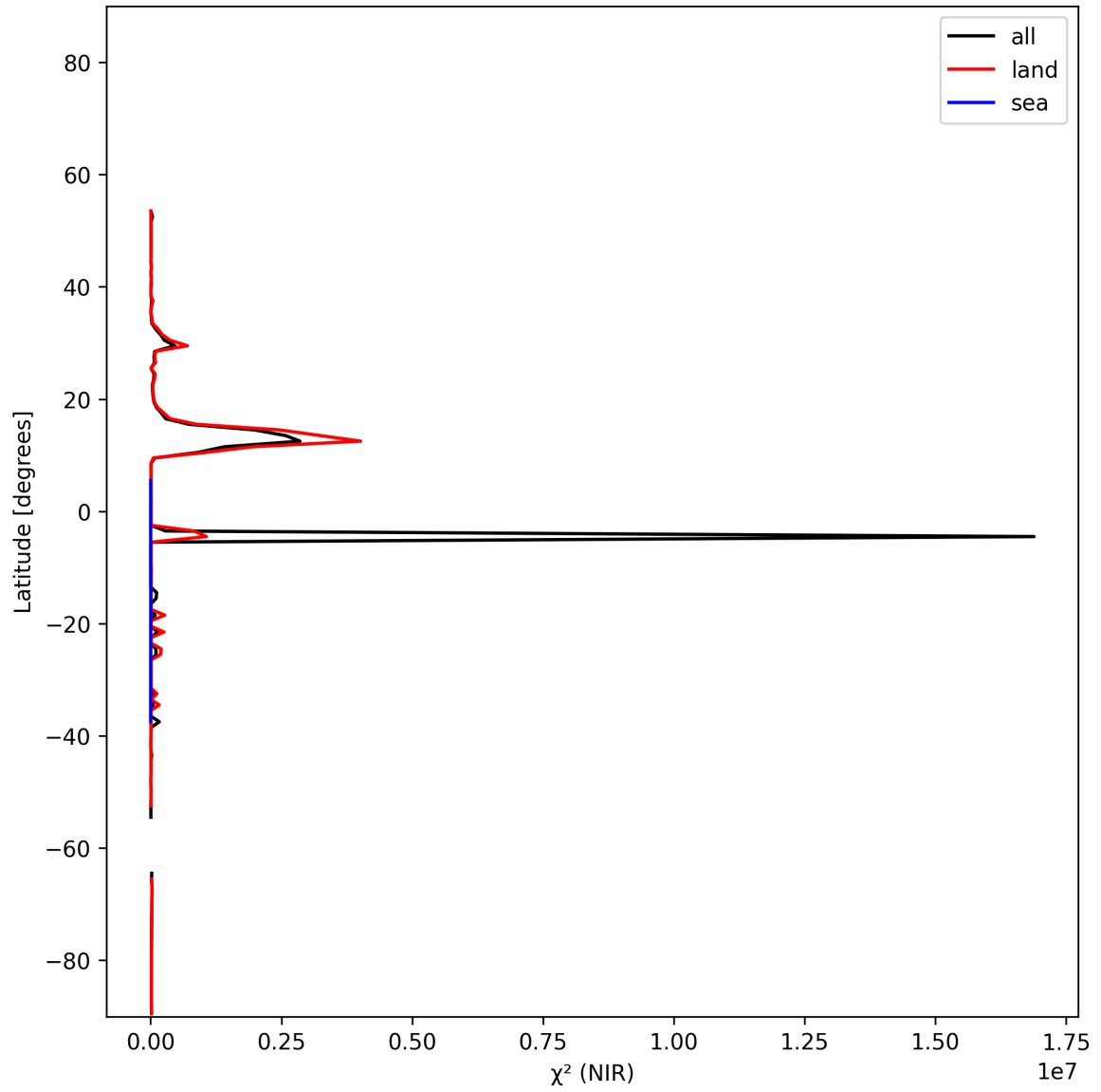
Figure 18: Zonal average of “ \chi^2 (NIR)” for 2025-01-14 to 2025-01-16.
