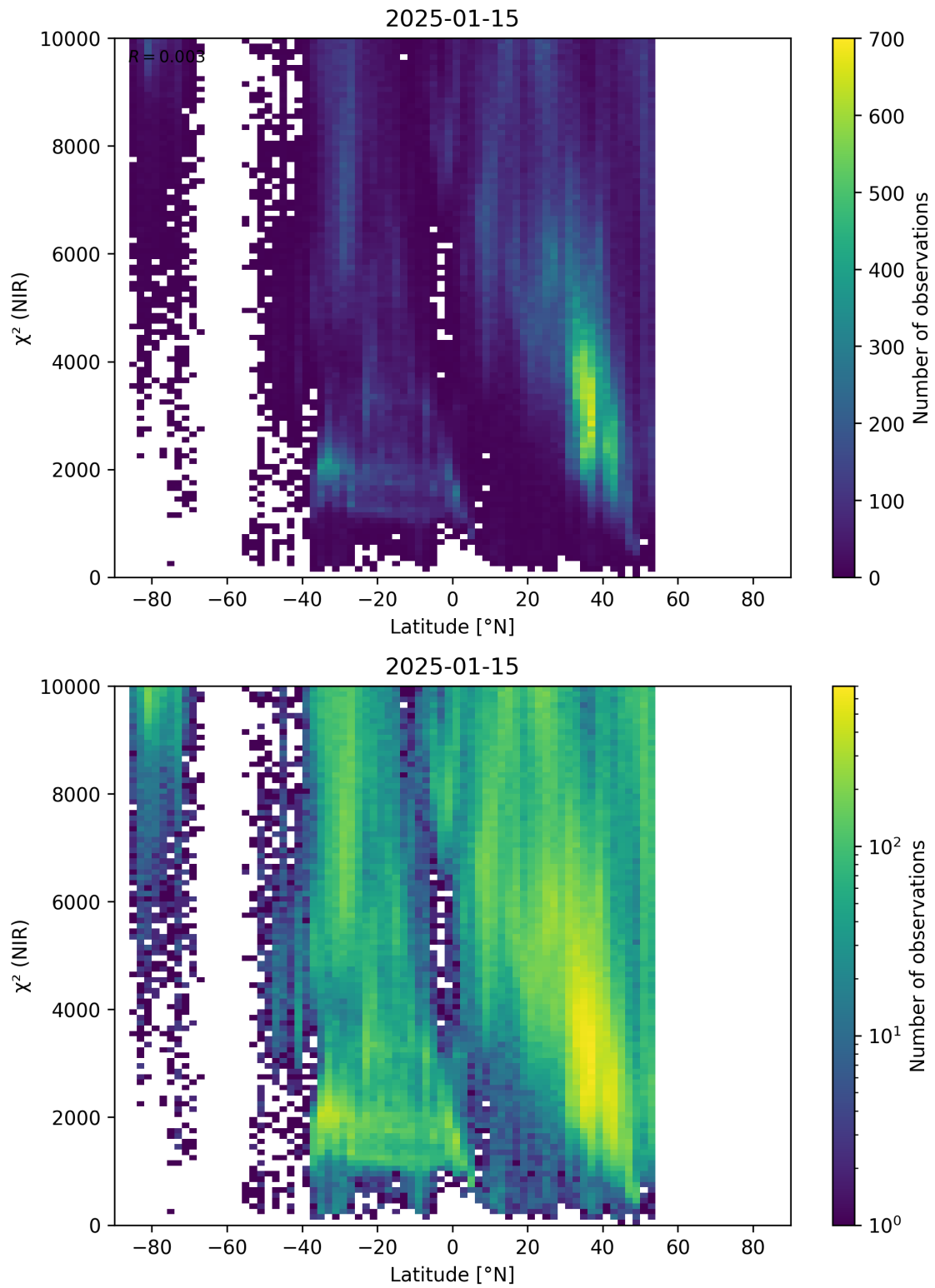
Figure 53: Scatter density plot of “Latitude” against “ \chi^2 (NIR)” for 2025-01-14 to 2025-01-16.
