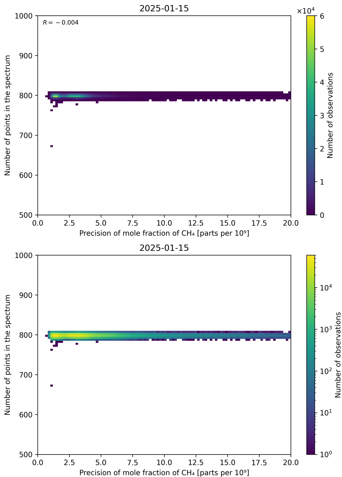
Figure 84: Scatter density plot of “Precision of mole fraction of CH 4 ” against “Number of points in the spectrum” for 2025-01-14 to 2025-01-16.
