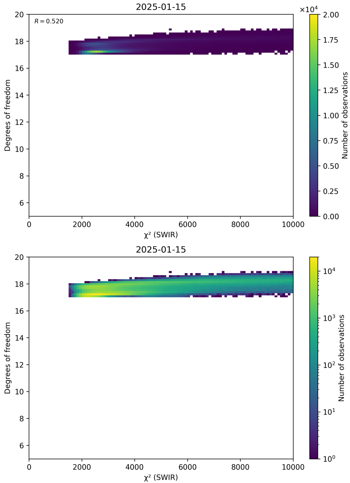
Figure 48: Scatter density plot of “ \chi^2 (SWIR)” against “Degrees of freedom” for 2025-01-14 to 2025-01-16.
