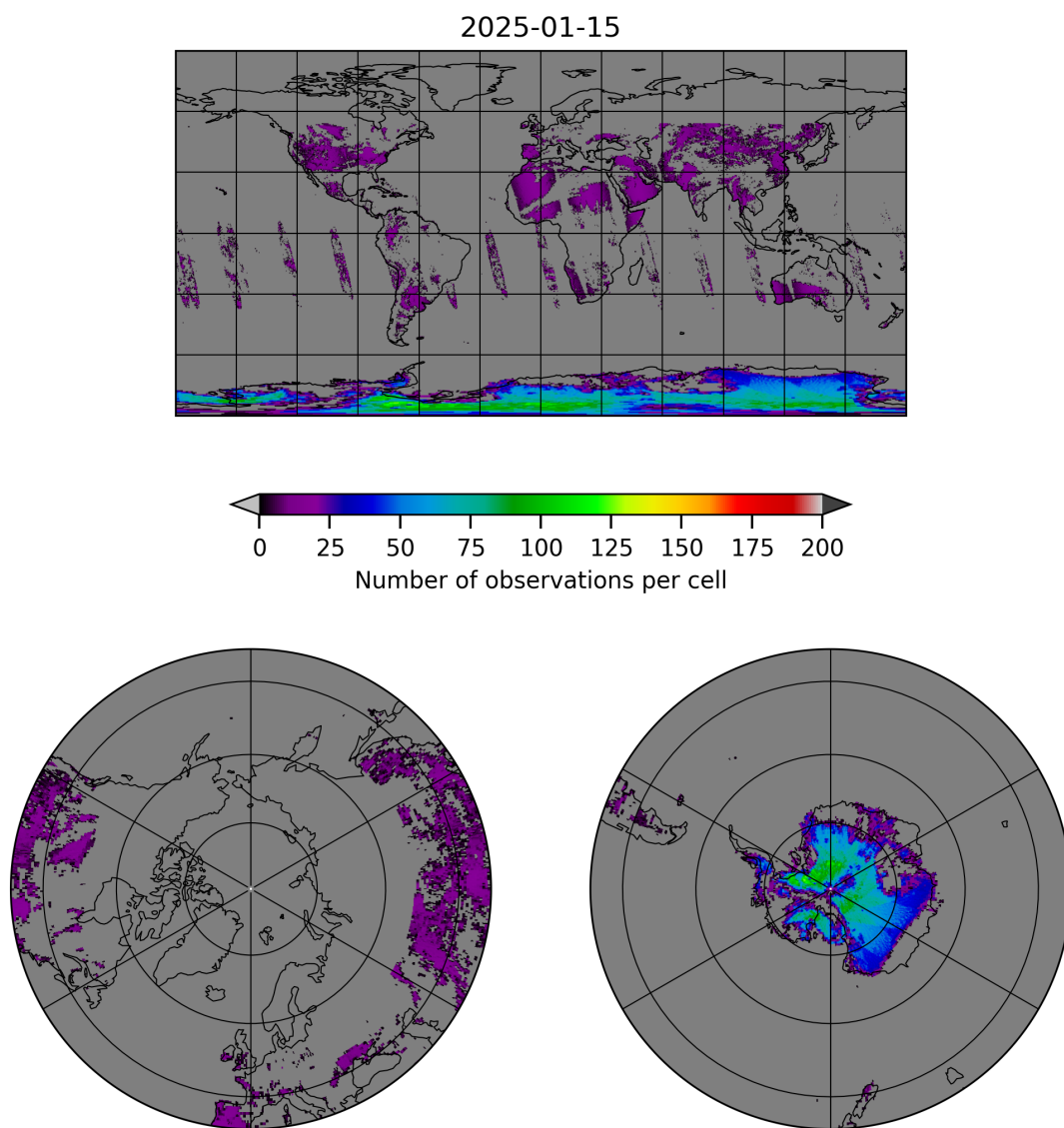
Figure 10: Map of the number of observations for 2025-01-14 to 2025-01-16
