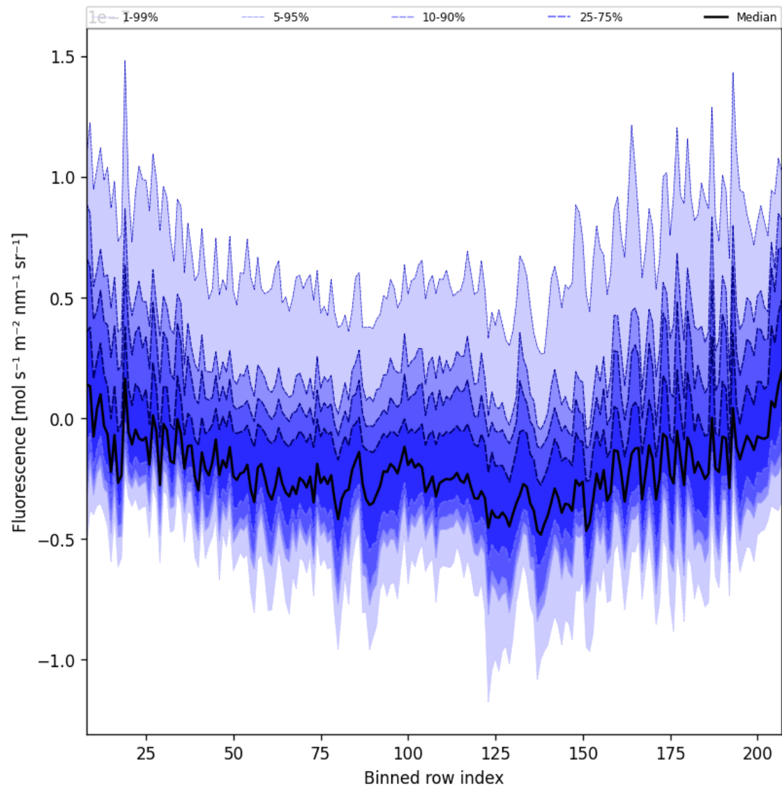
Figure 43: Along track statistics of “Fluorescence” for 2025-01-14 to 2025-01-16
