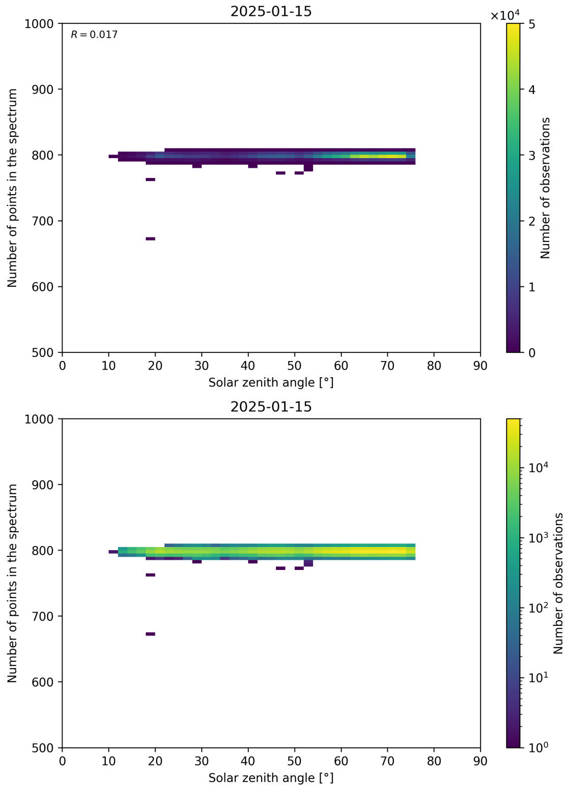
Figure 103: Scatter density plot of “Solar zenith angle” against “Number of points in the spectrum” for 2025-01-14 to 2025-01-16.
