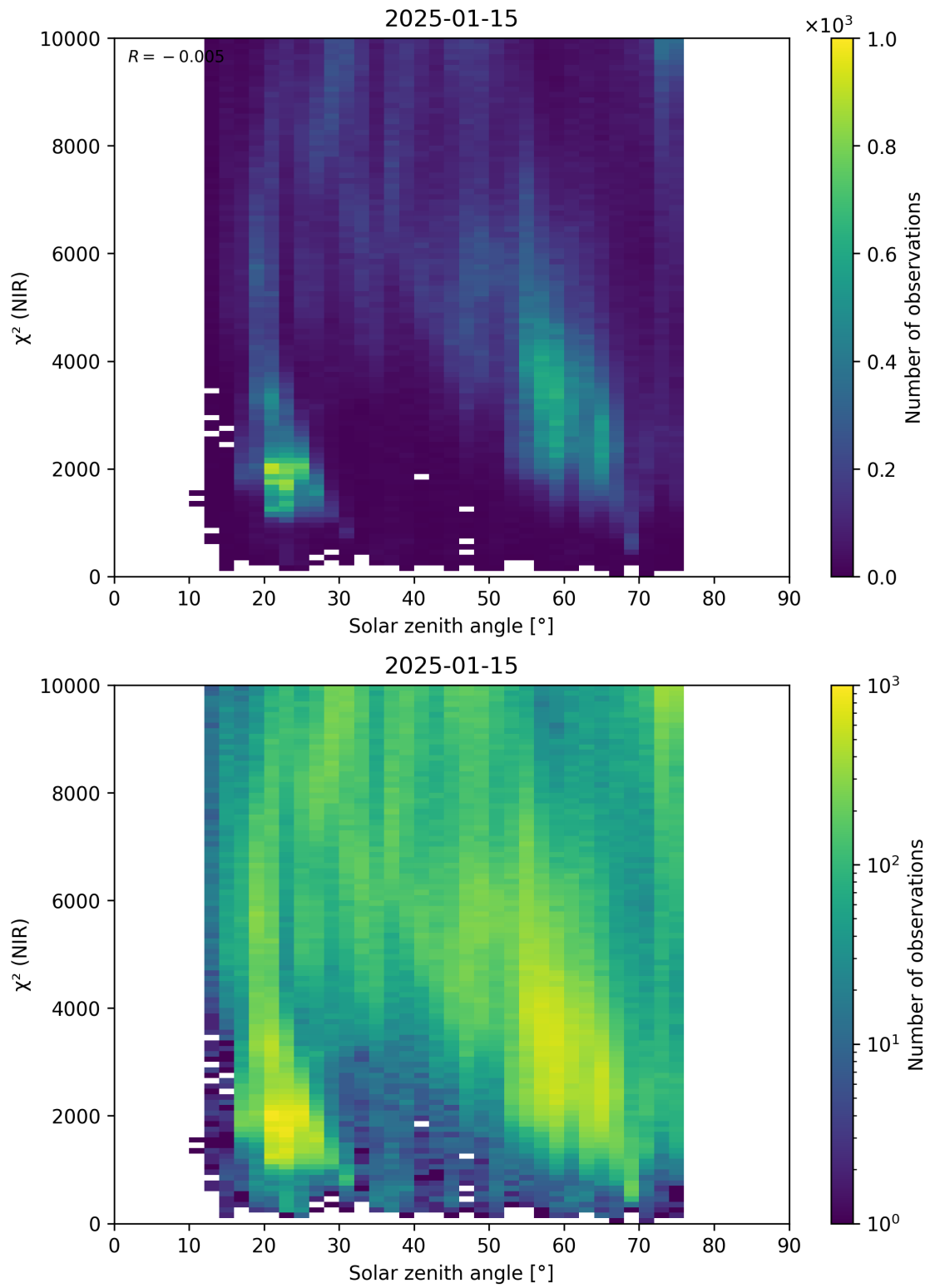
Figure 94: Scatter density plot of “Solar zenith angle” against “ \chi^2 (NIR)” for 2025-01-14 to 2025-01-16.
