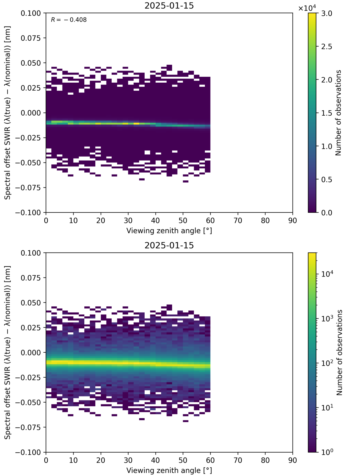
Figure 116: Scatter density plot of “Viewing zenith angle” against “Spectral offset SWIR ( \lambda_{\text{true}} - \lambda_{\text{nominal}} )” for 2025-01-14 to 2025-01-16.
