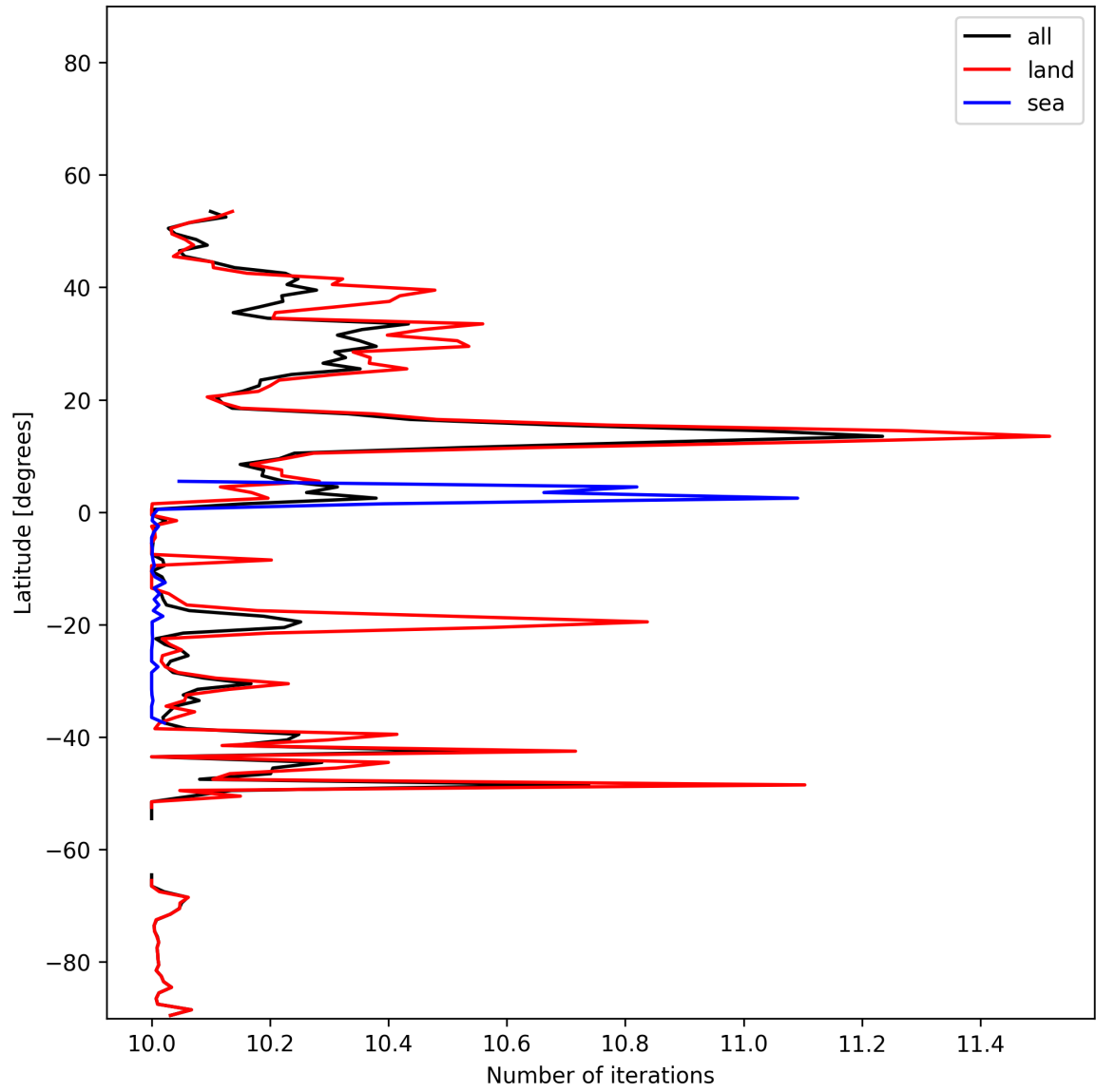
Figure 20: Zonal average of “Number of iterations” for 2025-01-14 to 2025-01-16.
