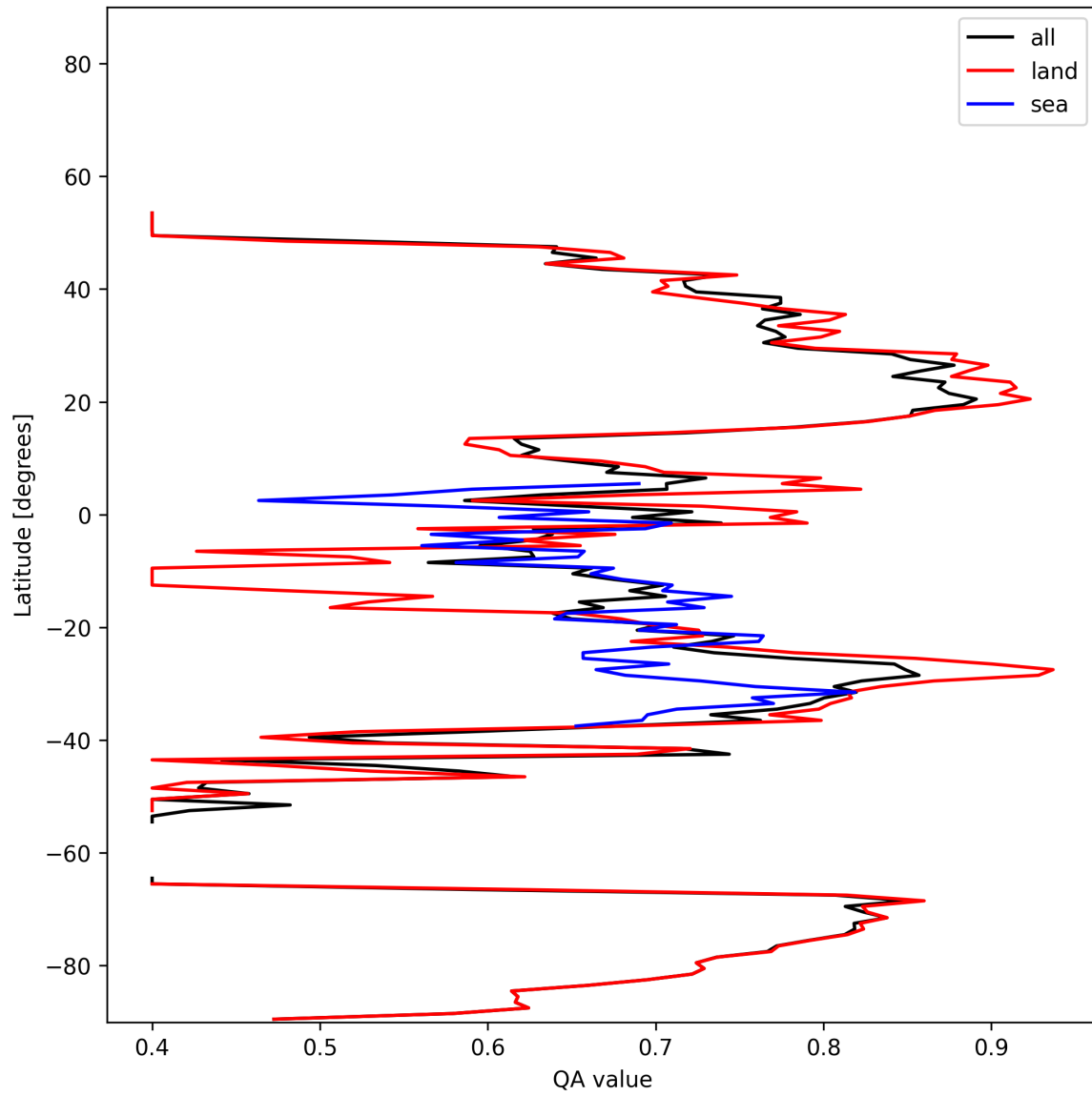
Figure 11: Zonal average of “QA value” for 2025-01-14 to 2025-01-16.
