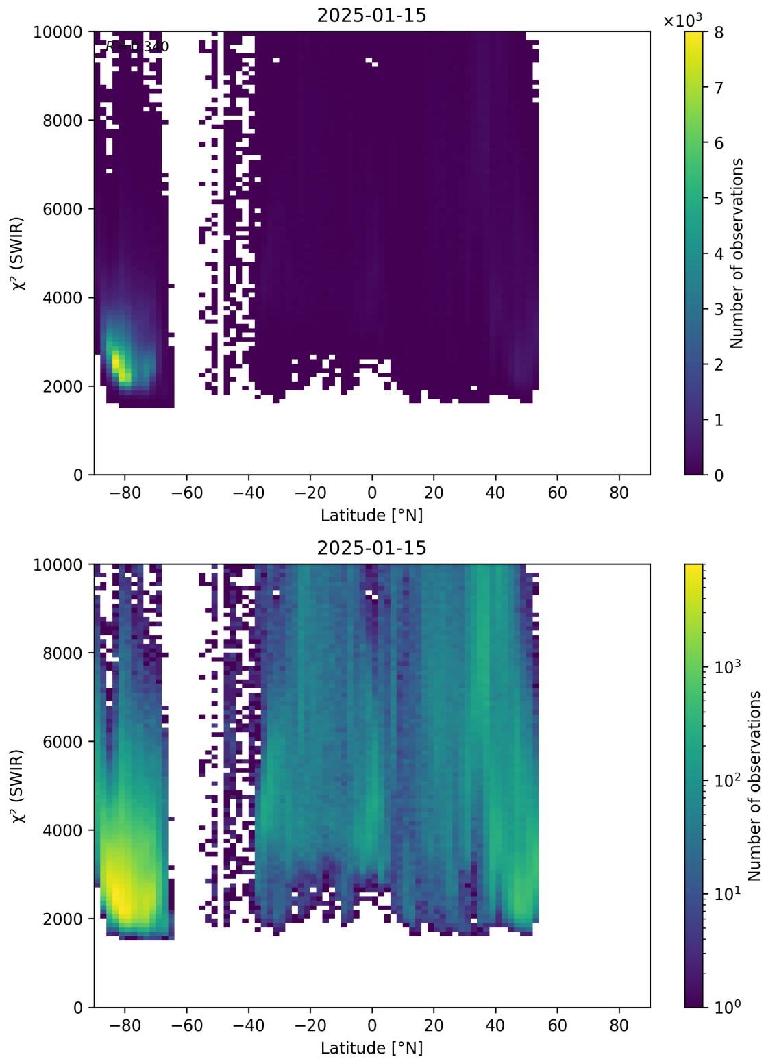
Figure 54: Scatter density plot of “Latitude” against “ \chi^2 (SWIR)” for 2025-01-14 to 2025-01-16.
