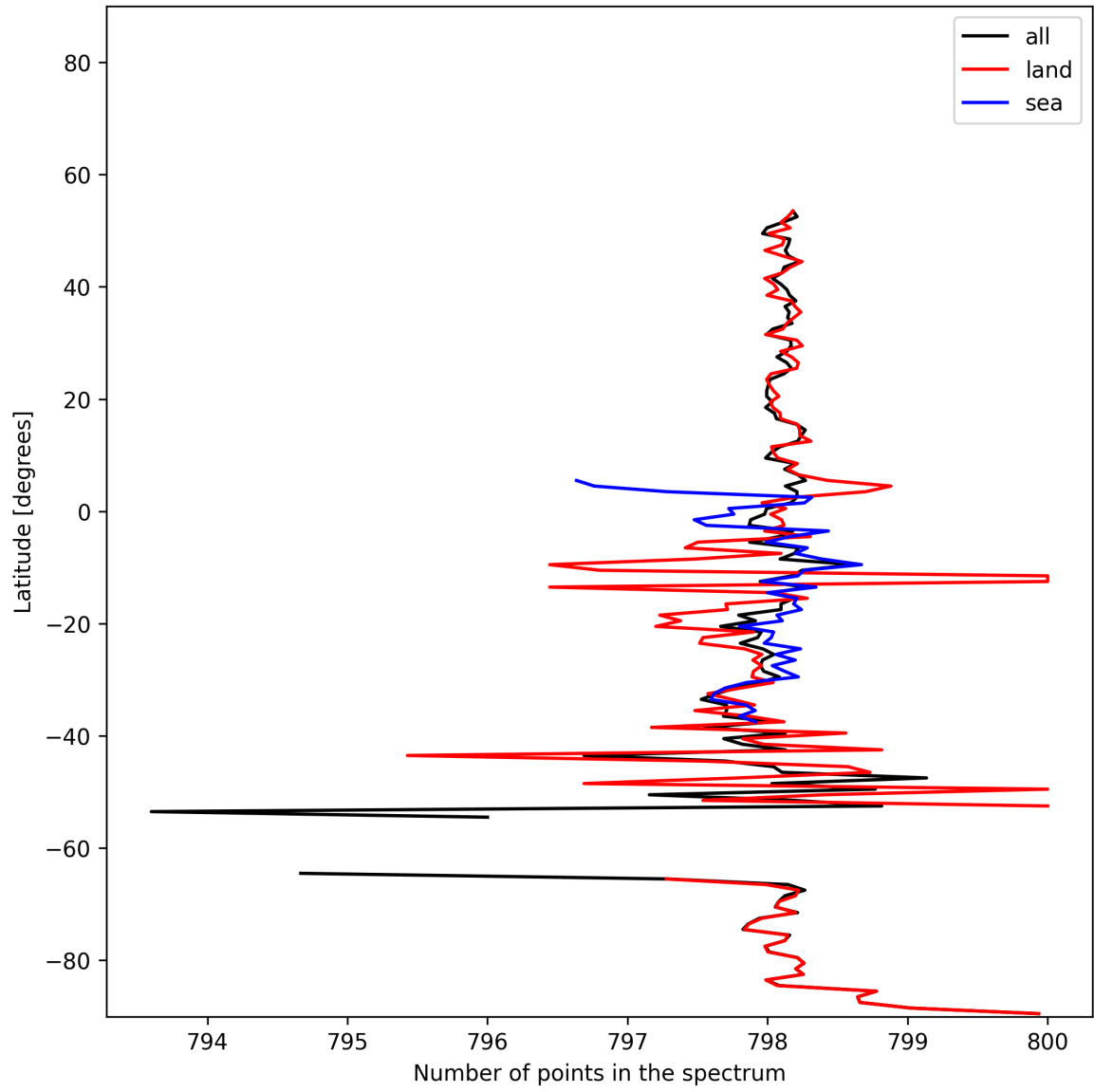
Figure 15: Zonal average of “Number of points in the spectrum” for 2025-01-14 to 2025-01-16.
