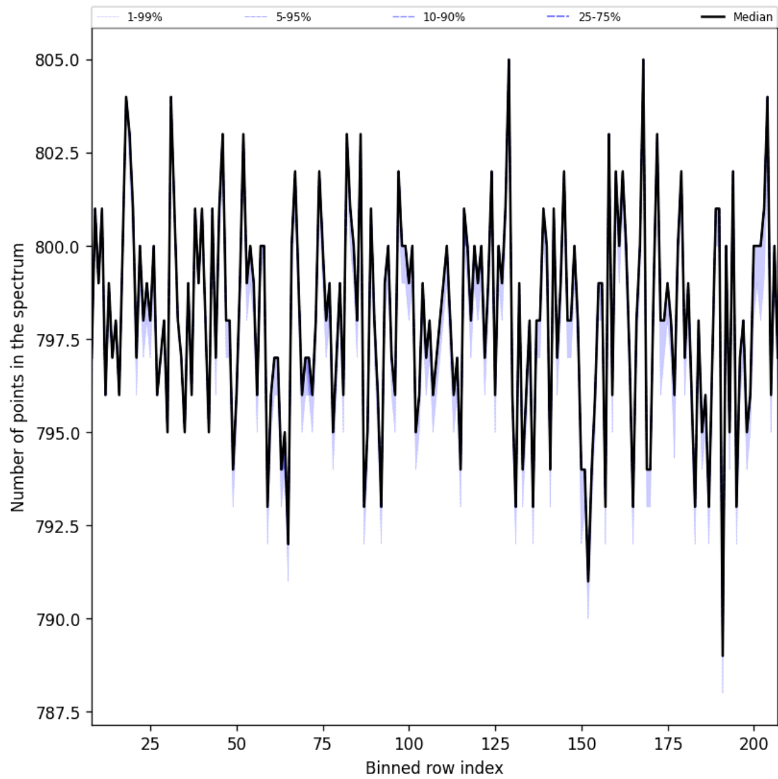
Figure 37: Along track statistics of “Number of points in the spectrum” for 2025-01-14 to 2025-01-16
