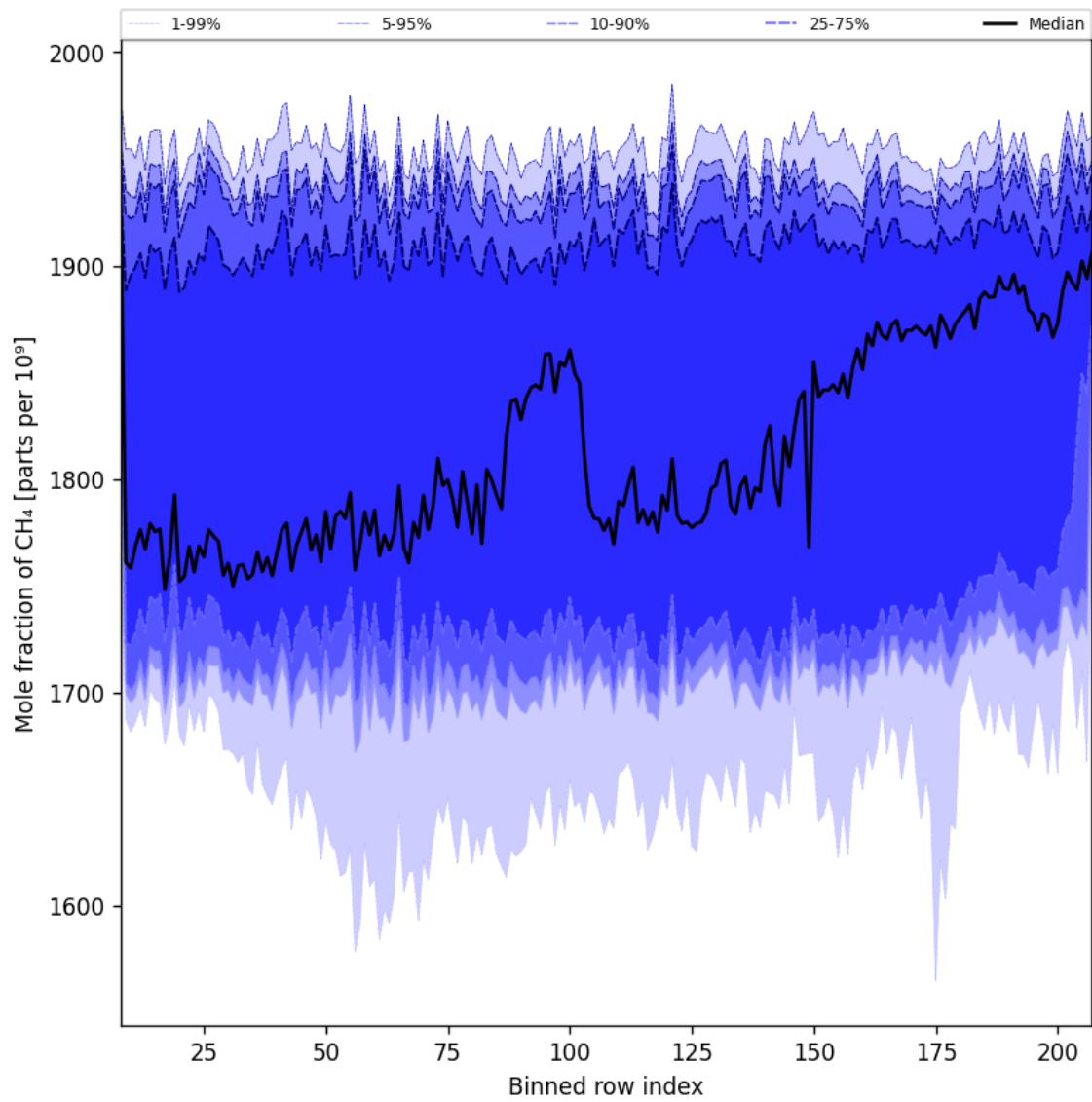
Figure 34: Along track statistics of “Mole fraction of CH 4 ” for 2025-01-14 to 2025-01-16
