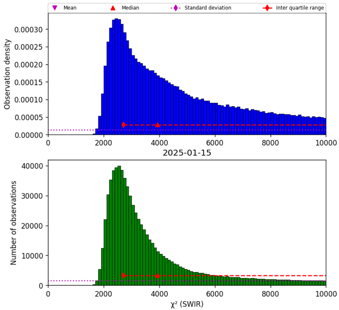
Figure 28: Histogram of “ \chi^2 (SWIR)” for 2025-01-14 to 2025-01-16
