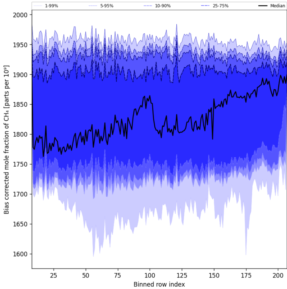
Figure 36: Along track statistics of “Bias corrected mole fraction of CH 4 ” for 2025-01-14 to 2025-01-16
