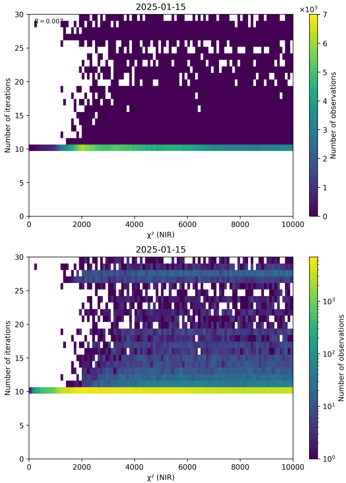
Figure 46: Scatter density plot of “ \chi^2 (NIR)” against “Number of iterations” for 2025-01-14 to 2025-01-16.
