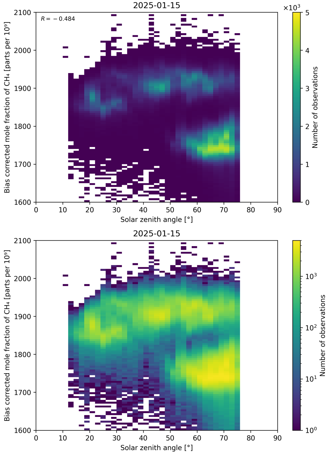
Figure 100: Scatter density plot of “Solar zenith angle” against “Bias corrected mole fraction of CH 4 ” for 2025-01-14 to 2025-01-16.
