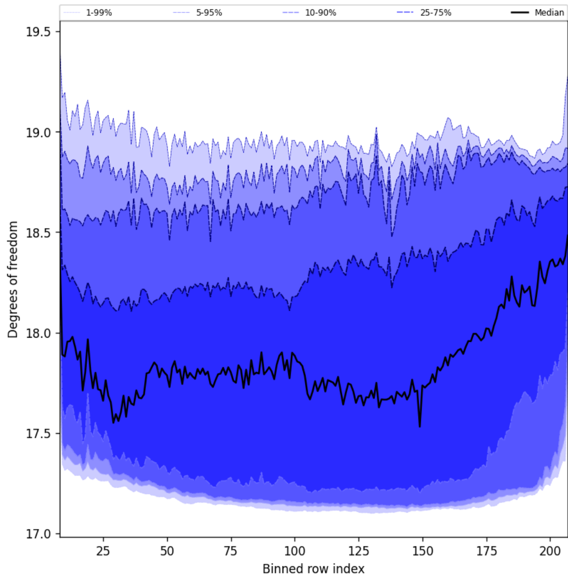
Figure 41: Along track statistics of “Degrees of freedom” for 2025-01-14 to 2025-01-16
