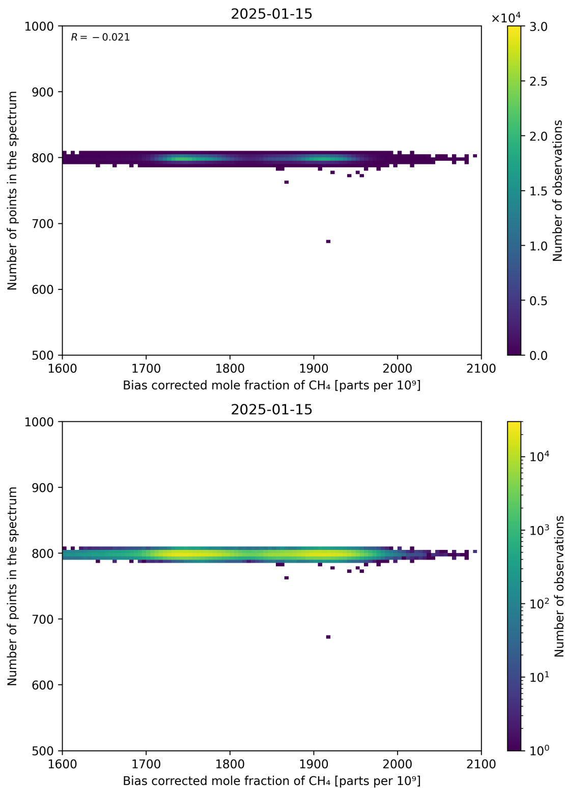
Figure 68: Scatter density plot of “Bias corrected mole fraction of CH 4 ” against “Number of points in the spectrum” for 2025-01-14 to 2025-01-16.
