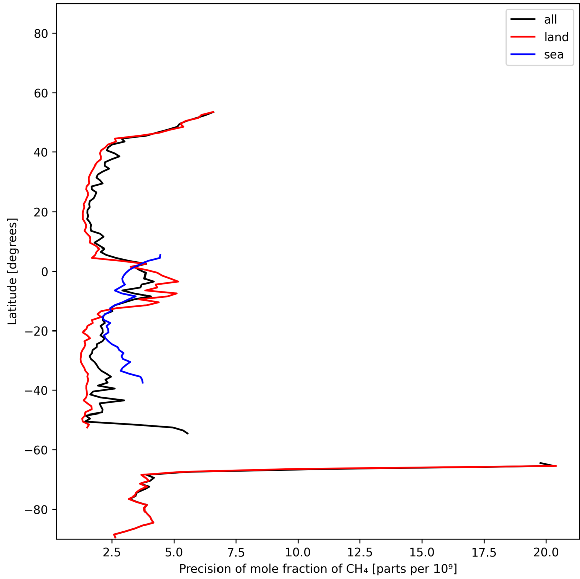
Figure 13: Zonal average of “Precision of mole fraction of CH 4 ” for 2025-01-14 to 2025-01-16.
