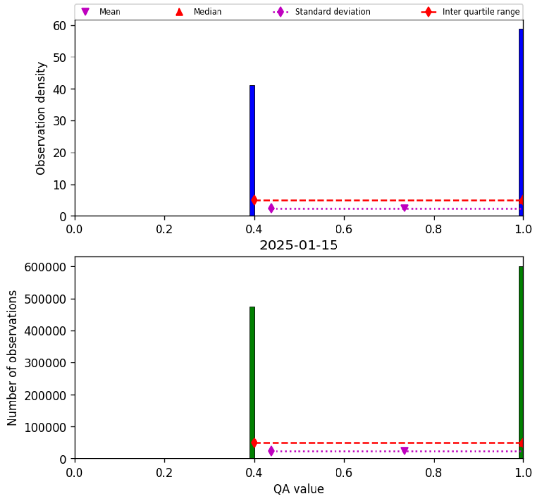
Figure 22: Histogram of “QA value” for 2025-01-14 to 2025-01-16
