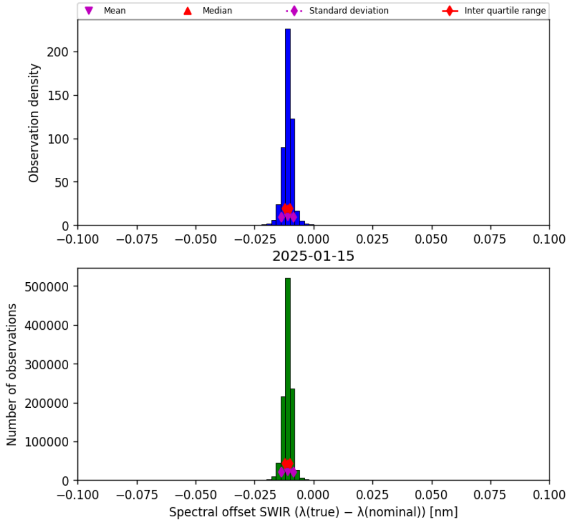
Figure 27: Histogram of “Spectral offset SWIR ( \lambda_{\text{true}} - \lambda_{\text{nominal}} )” for 2025-01-14 to 2025-01-16
