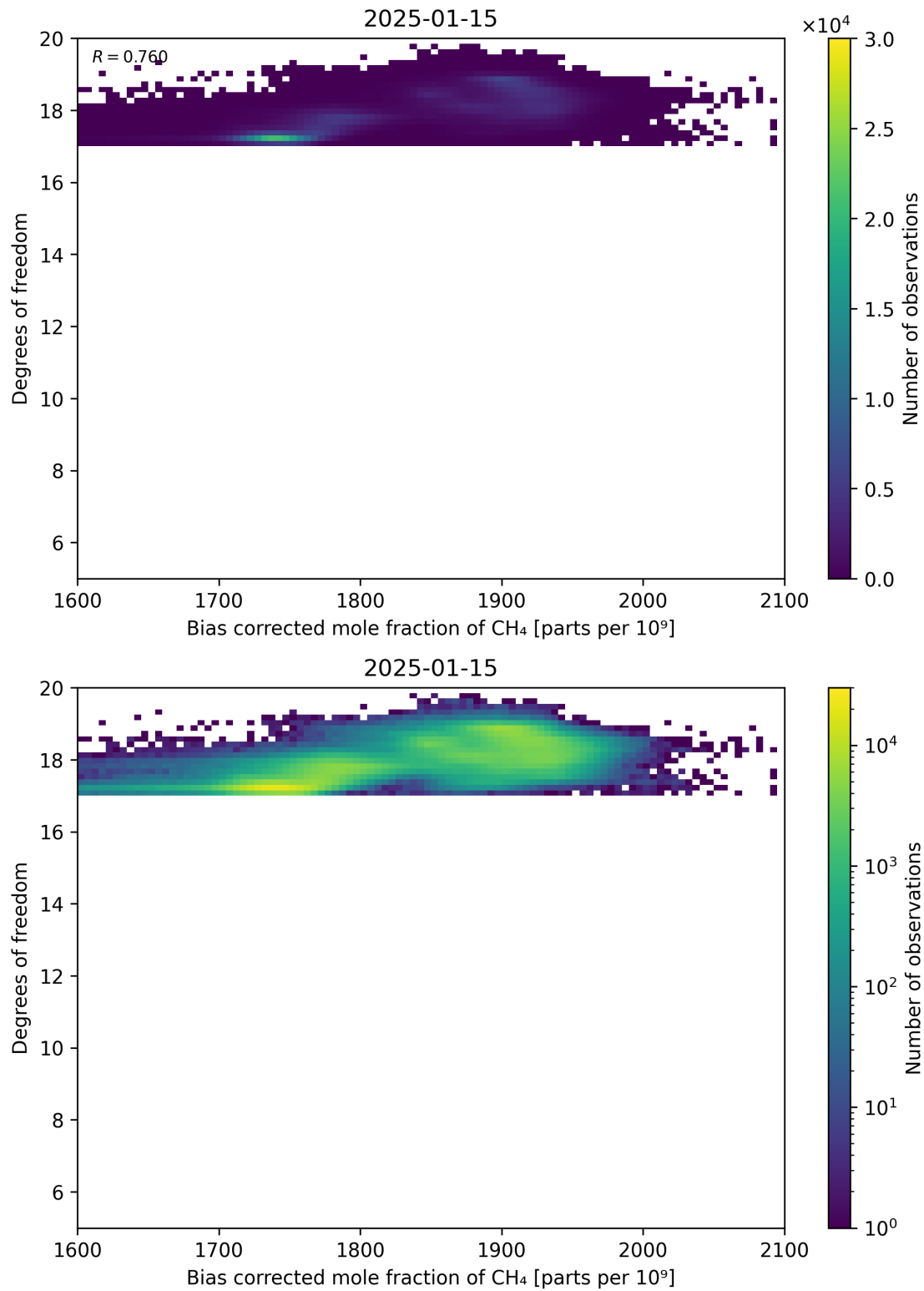
Figure 65: Scatter density plot of “Bias corrected mole fraction of CH 4 ” against “Degrees of freedom” for 2025-01-14 to 2025-01-16.
