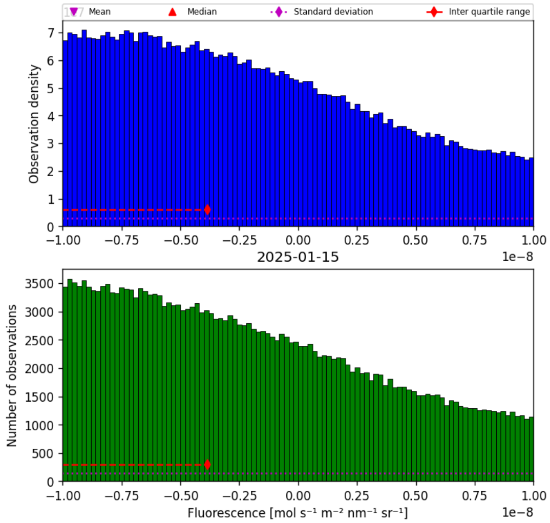
Figure 32: Histogram of “Fluorescence” for 2025-01-14 to 2025-01-16
