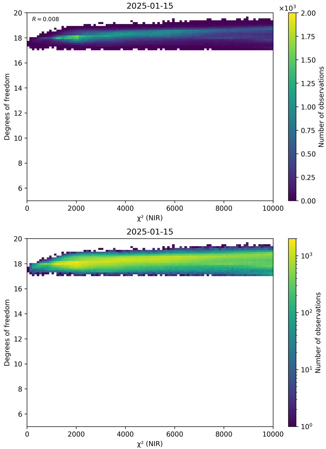
Figure 44: Scatter density plot of “ \chi^2 (NIR)” against “Degrees of freedom” for 2025-01-14 to 2025-01-16.
