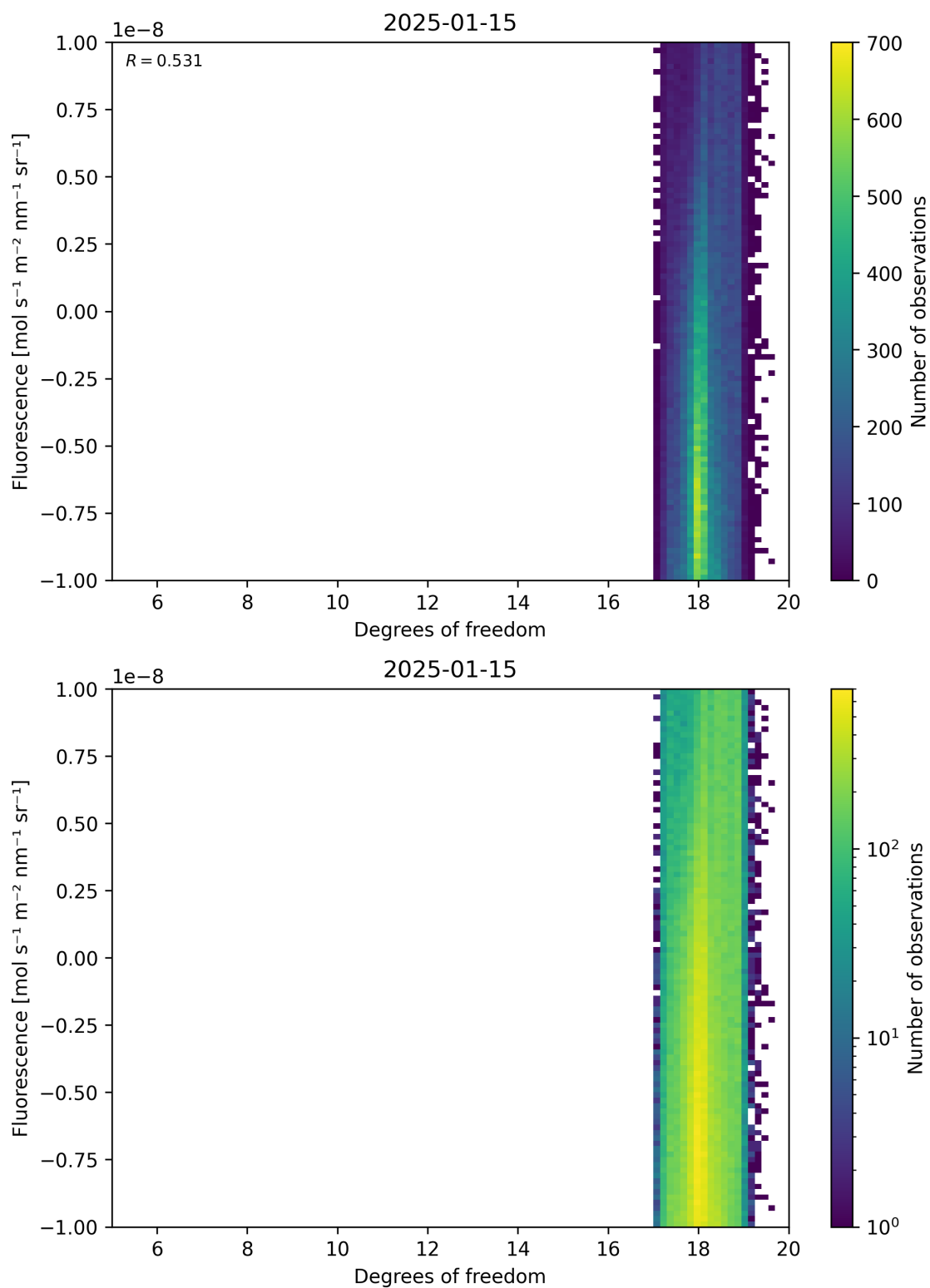
Figure 51: Scatter density plot of “Degrees of freedom” against “Fluorescence” for 2025-01-14 to 2025-01-16.
