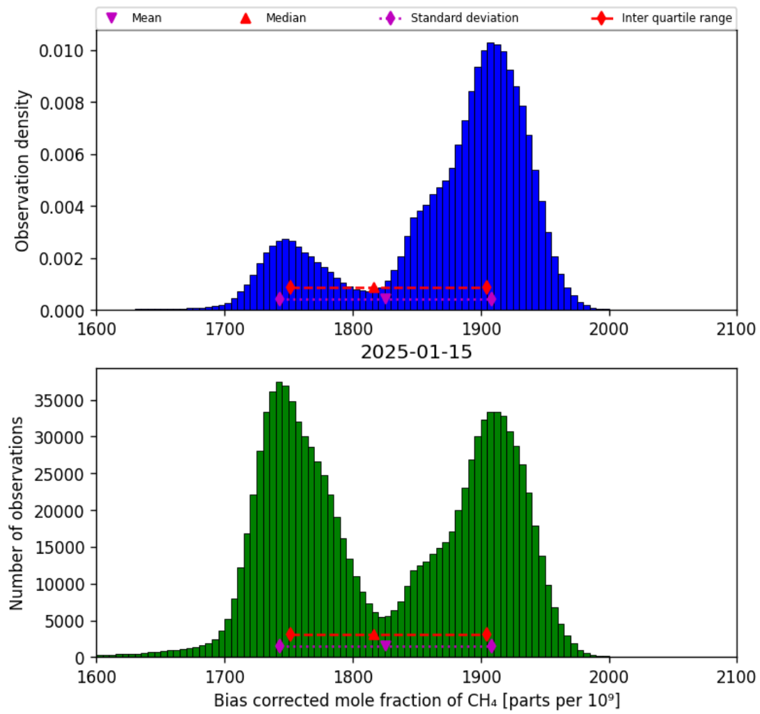
Figure 25: Histogram of “Bias corrected mole fraction of CH 4 ” for 2025-01-14 to 2025-01-16
