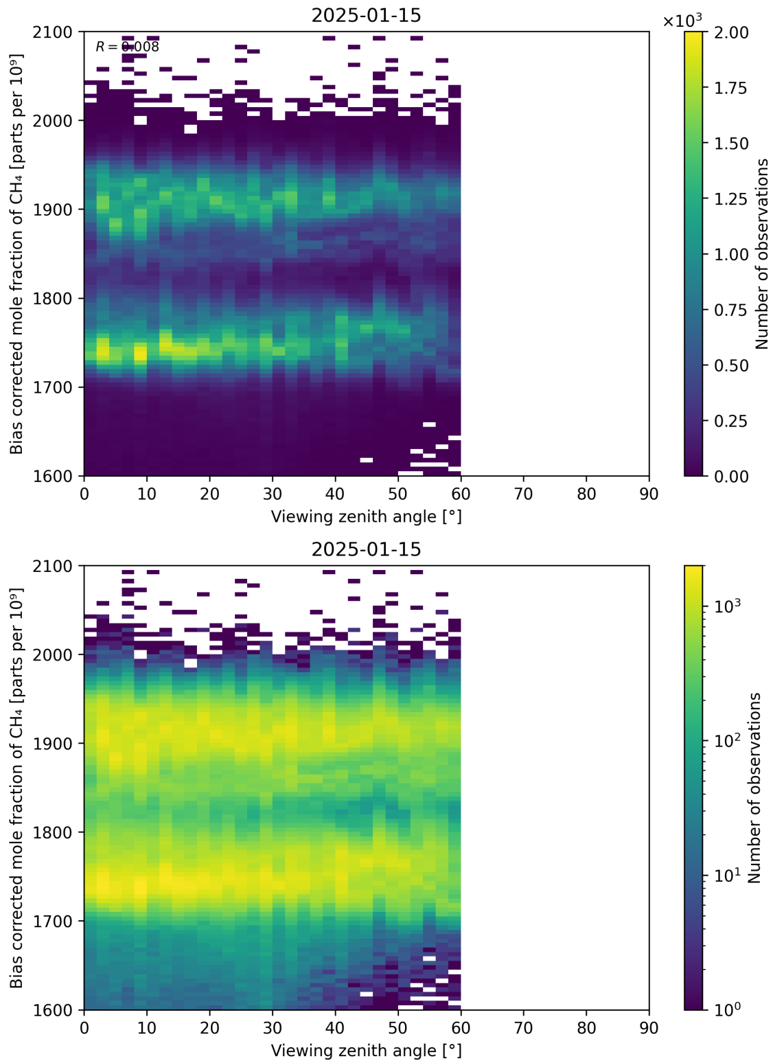
Figure 111: Scatter density plot of “Viewing zenith angle” against “Bias corrected mole fraction of \text{CH}_4 ” for 2025-01-14 to 2025-01-16.
