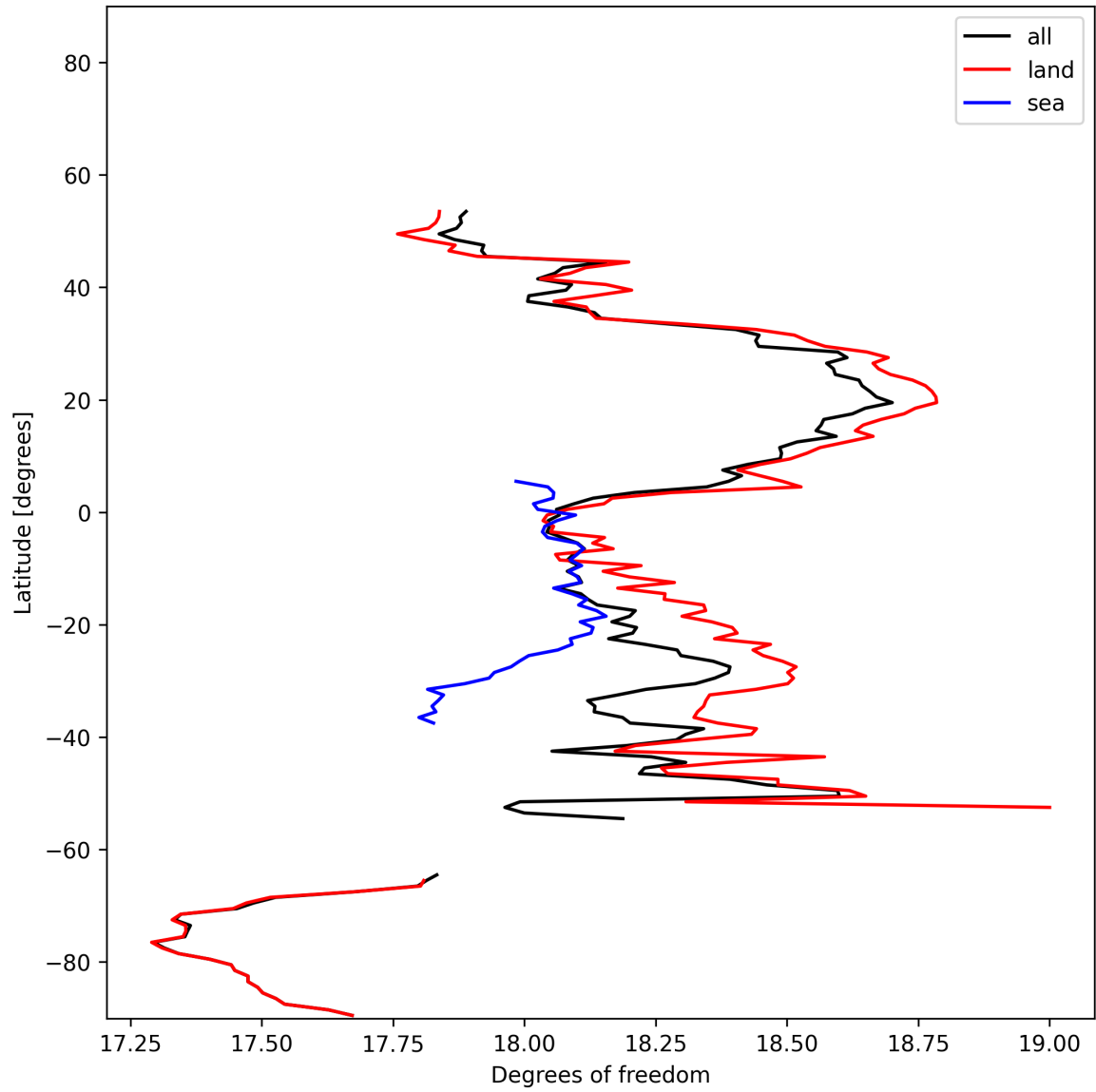
Figure 19: Zonal average of “Degrees of freedom” for 2025-01-14 to 2025-01-16.
