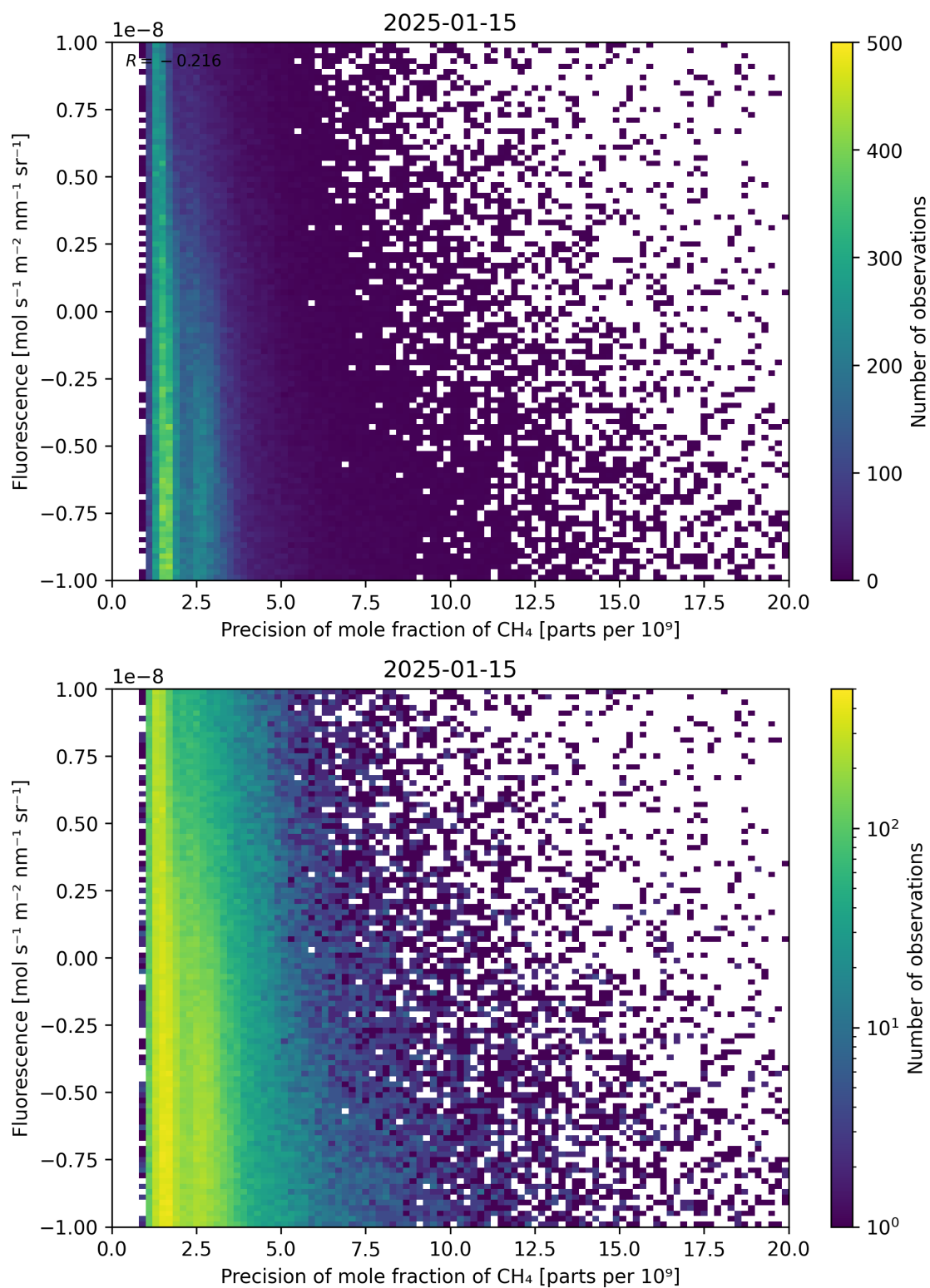
Figure 81: Scatter density plot of “Precision of mole fraction of \text{CH}_4 ” against “Fluorescence” for 2025-01-14 to 2025-01-16.
