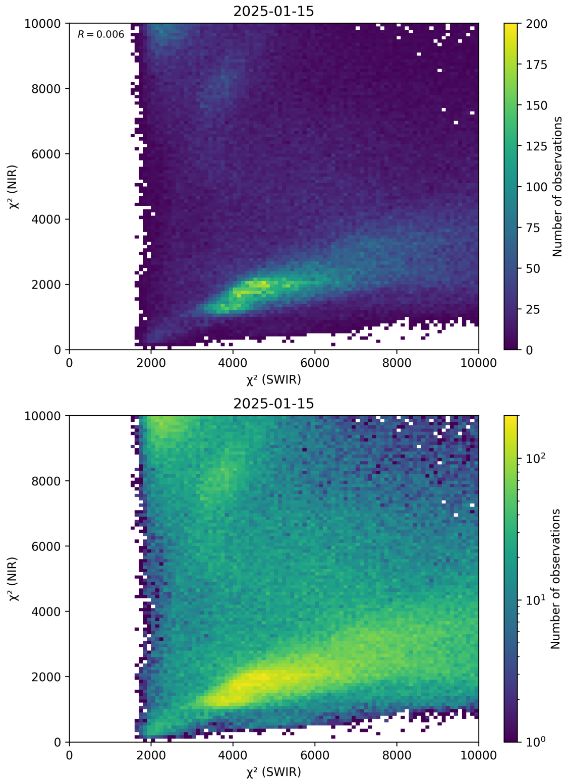
Figure 47: Scatter density plot of “ \chi^2 (SWIR)” against “ \chi^2 (NIR)” for 2025-01-14 to 2025-01-16.
