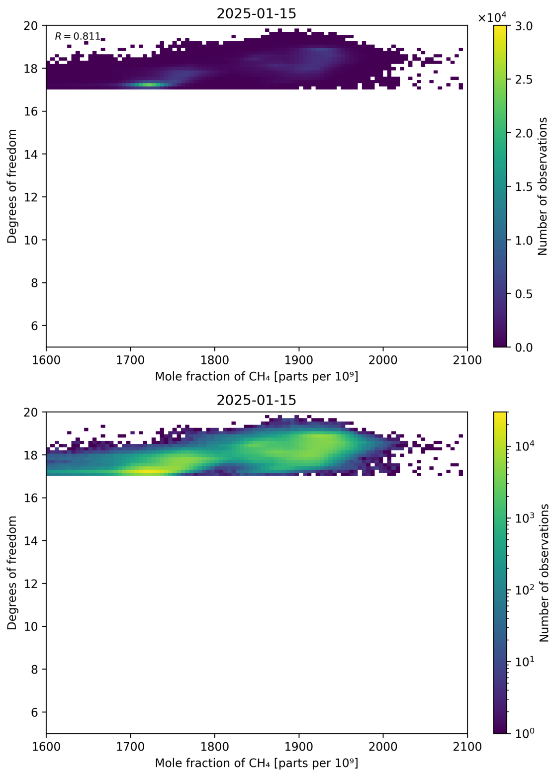
Figure 72: Scatter density plot of “Mole fraction of CH 4 ” against “Degrees of freedom” for 2025-01-14 to 2025-01-16.
