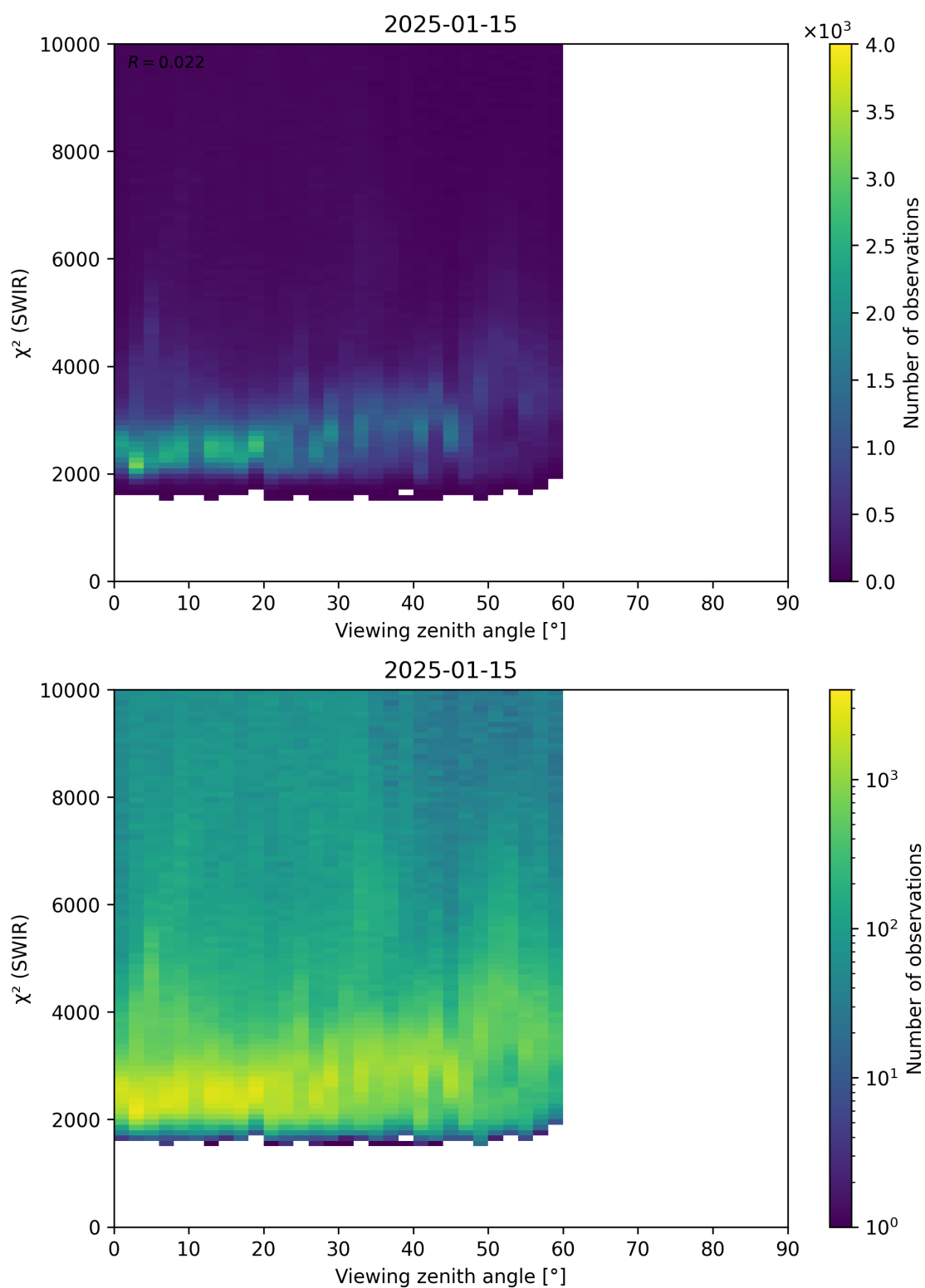
Figure 106: Scatter density plot of “Viewing zenith angle” against “ \chi^2 (SWIR)” for 2025-01-14 to 2025-01-16.
