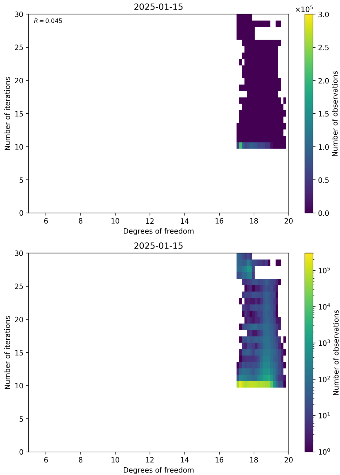
Figure 52: Scatter density plot of “Degrees of freedom” against “Number of iterations” for 2025-01-14 to 2025-01-16.
