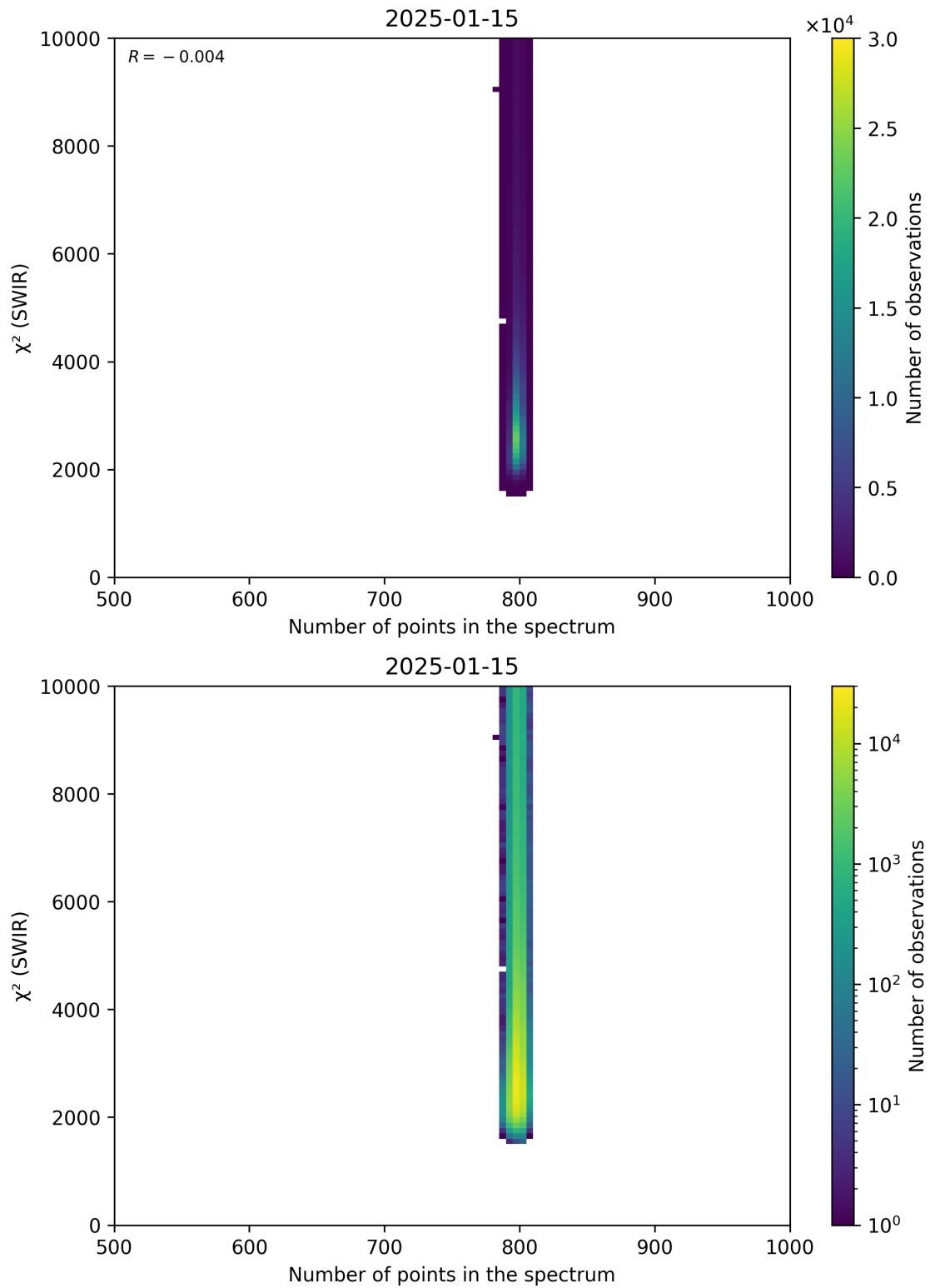
Figure 89: Scatter density plot of “Number of points in the spectrum” against “ \chi^2 (SWIR)” for 2025-01-14 to 2025-01-16.
