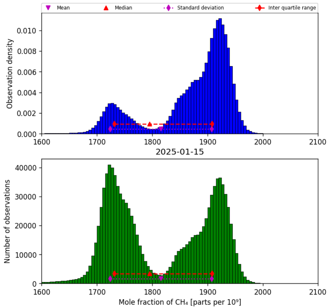
Figure 23: Histogram of “Mole fraction of CH 4 ” for 2025-01-14 to 2025-01-16
