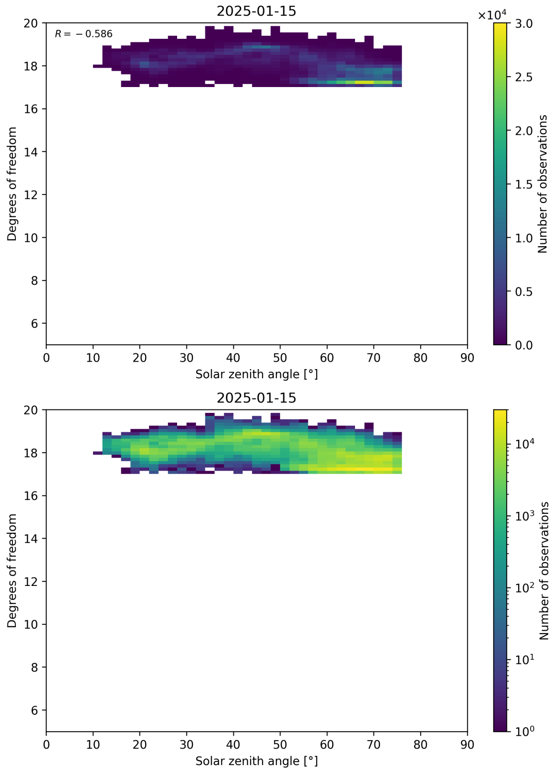
Figure 96: Scatter density plot of “Solar zenith angle” against “Degrees of freedom” for 2025-01-14 to 2025-01-16.
