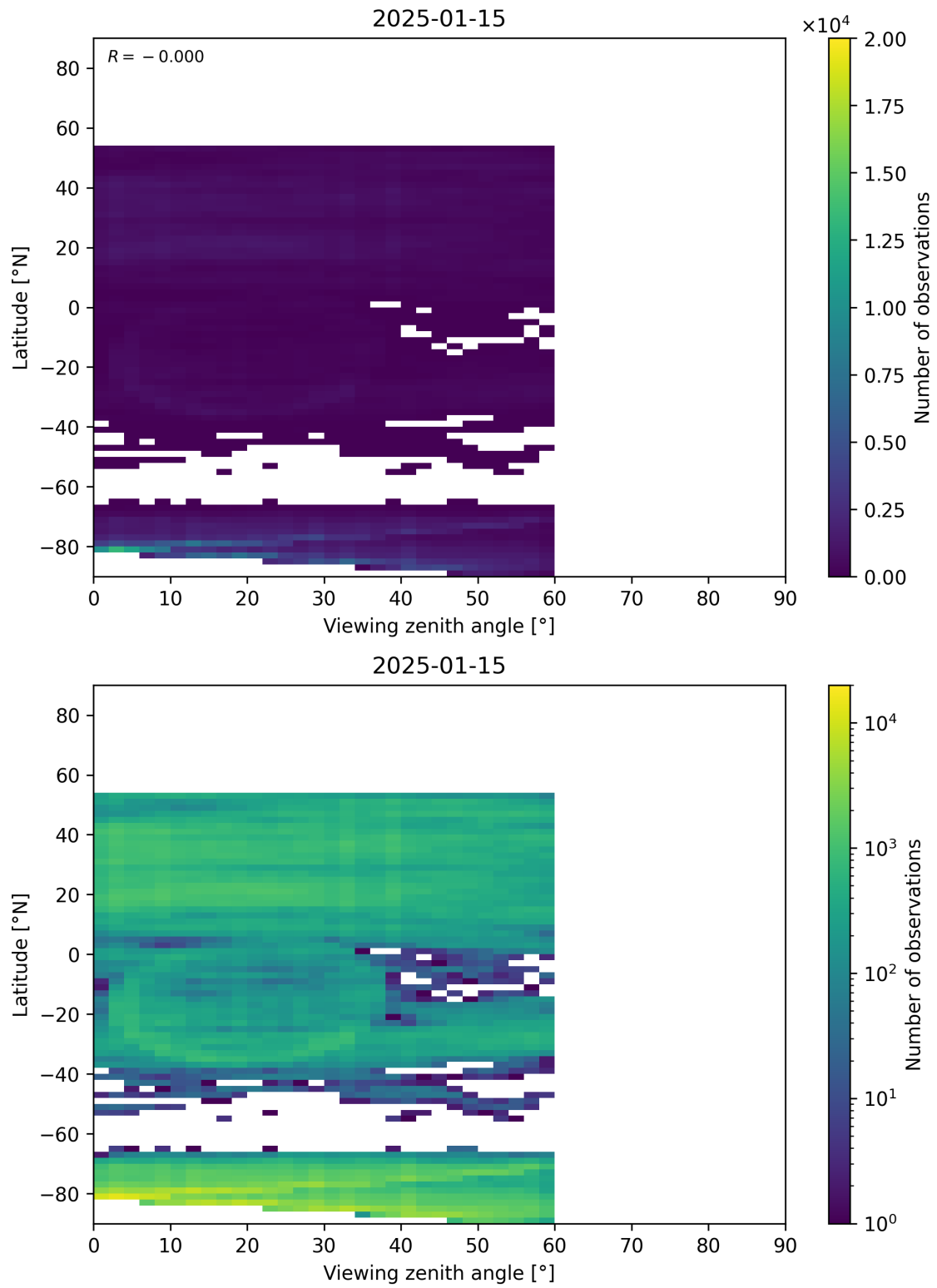
Figure 109: Scatter density plot of “Viewing zenith angle” against “Latitude” for 2025-01-14 to 2025-01-16.
