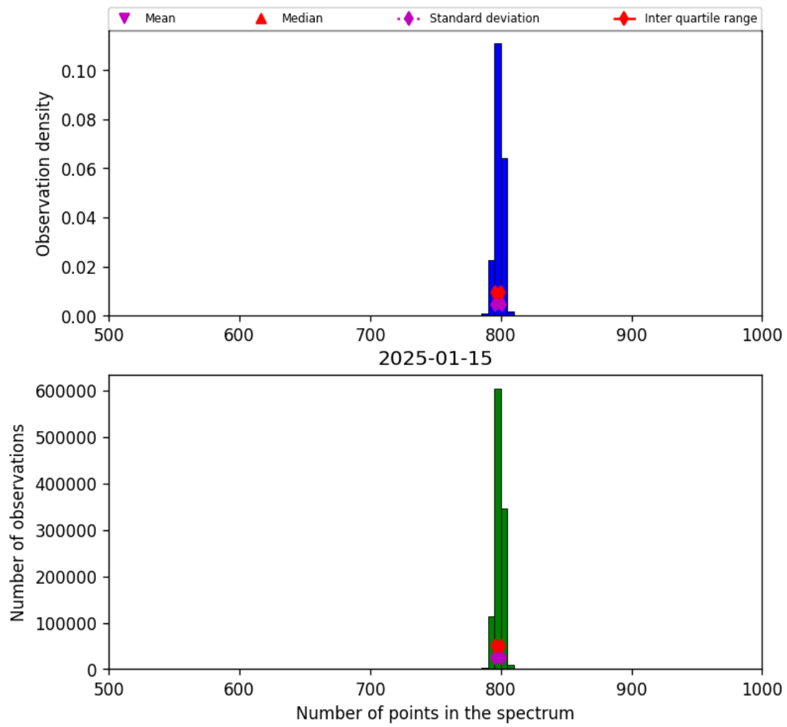
Figure 26: Histogram of “Number of points in the spectrum” for 2025-01-14 to 2025-01-16
