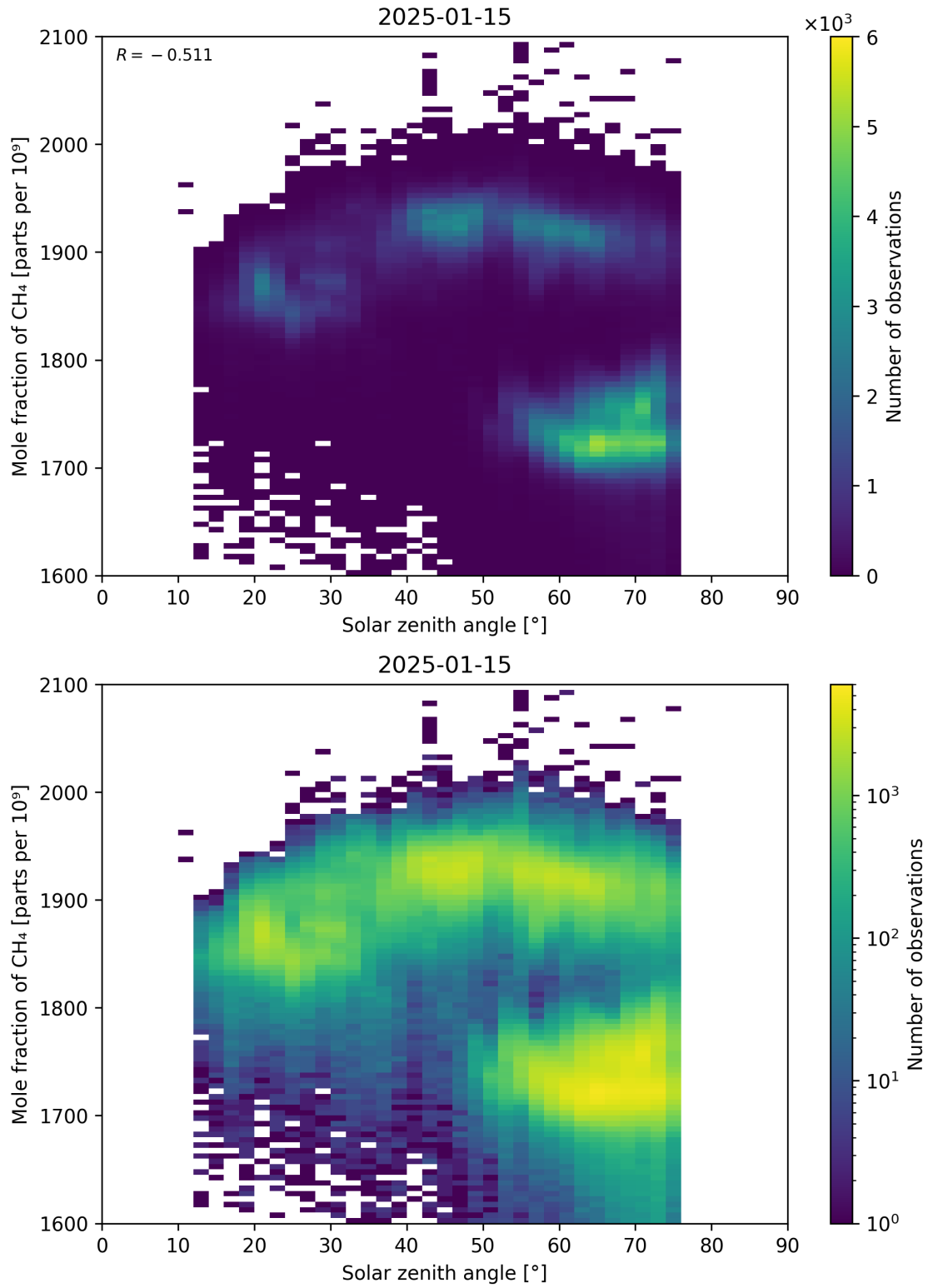
Figure 99: Scatter density plot of “Solar zenith angle” against “Mole fraction of CH 4 ” for 2025-01-14 to 2025-01-16.
