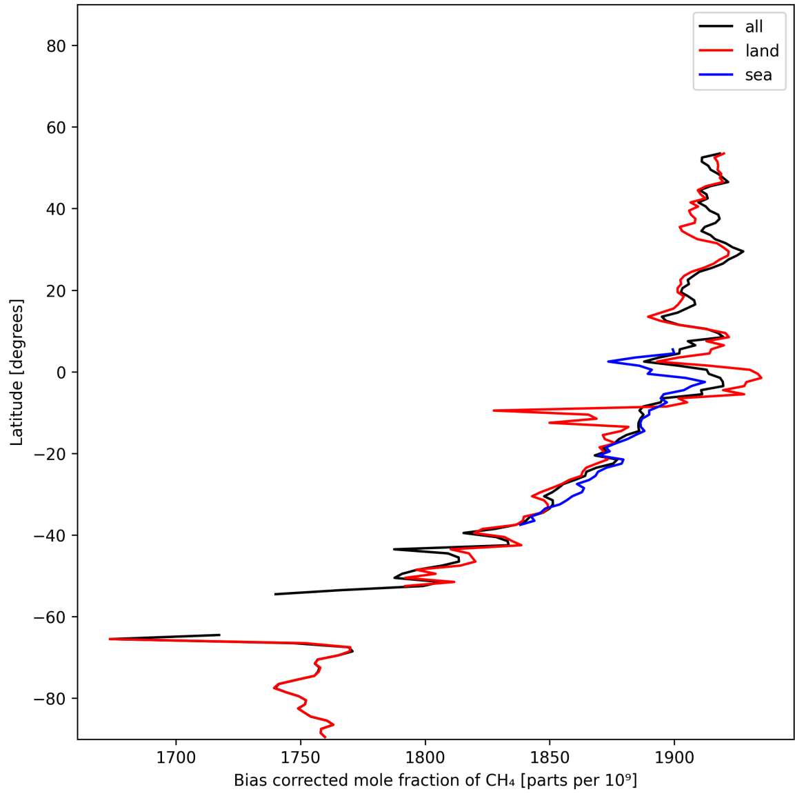
Figure 14: Zonal average of “Bias corrected mole fraction of CH 4 ” for 2025-01-14 to 2025-01-16.
