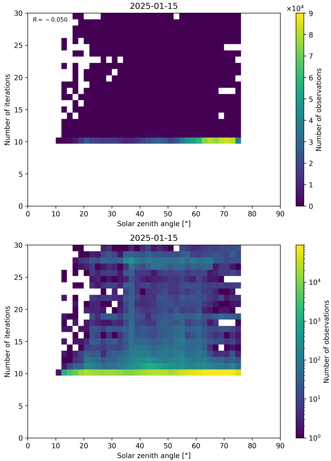
Figure 102: Scatter density plot of “Solar zenith angle” against “Number of iterations” for 2025-01-14 to 2025-01-16.
