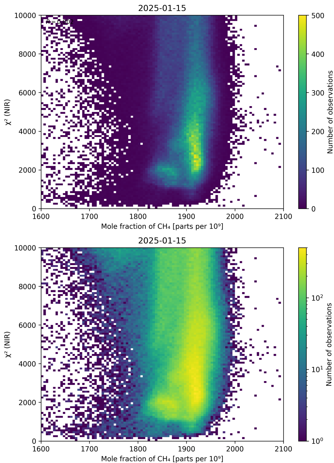
Figure 70: Scatter density plot of “Mole fraction of CH 4 ” against “ \chi^2 (NIR)” for 2025-01-14 to 2025-01-16.
