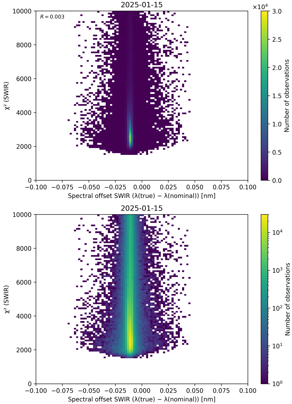
Figure 118: Scatter density plot of “Spectral offset SWIR ( \lambda_{\text{true}} - \lambda_{\text{nominal}} )” against “ \chi^2 (SWIR)” for 2025-01-14 to 2025-01-16.
