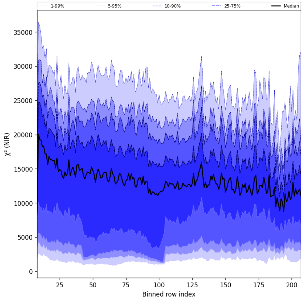
Figure 40: Along track statistics of “ \chi^2 (NIR)” for 2025-01-14 to 2025-01-16
