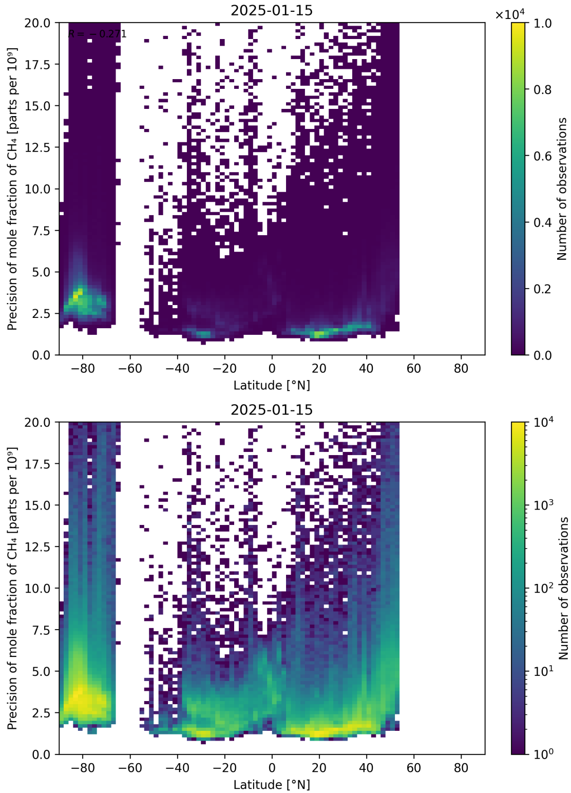
Figure 59: Scatter density plot of “Latitude” against “Precision of mole fraction of \text{CH}_4 ” for 2025-01-14 to 2025-01-16.
