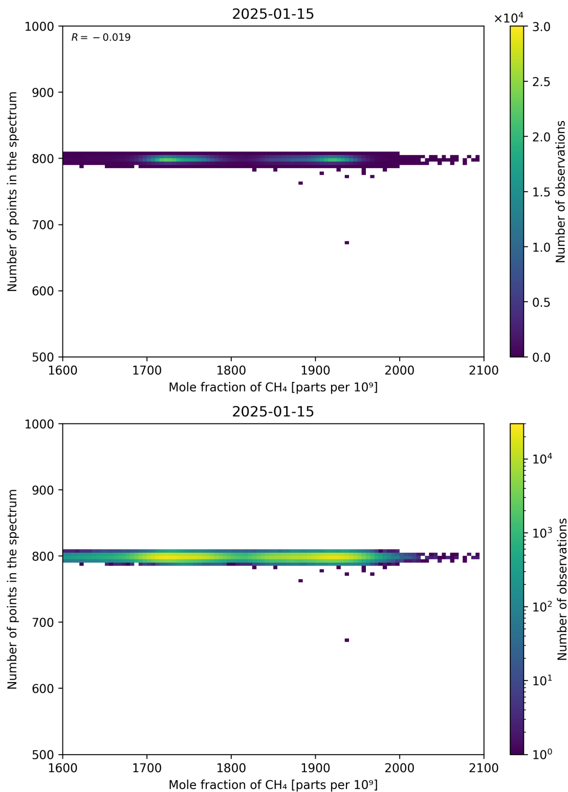
Figure 77: Scatter density plot of “Mole fraction of CH 4 ” against “Number of points in the spectrum” for 2025-01-14 to 2025-01-16.
