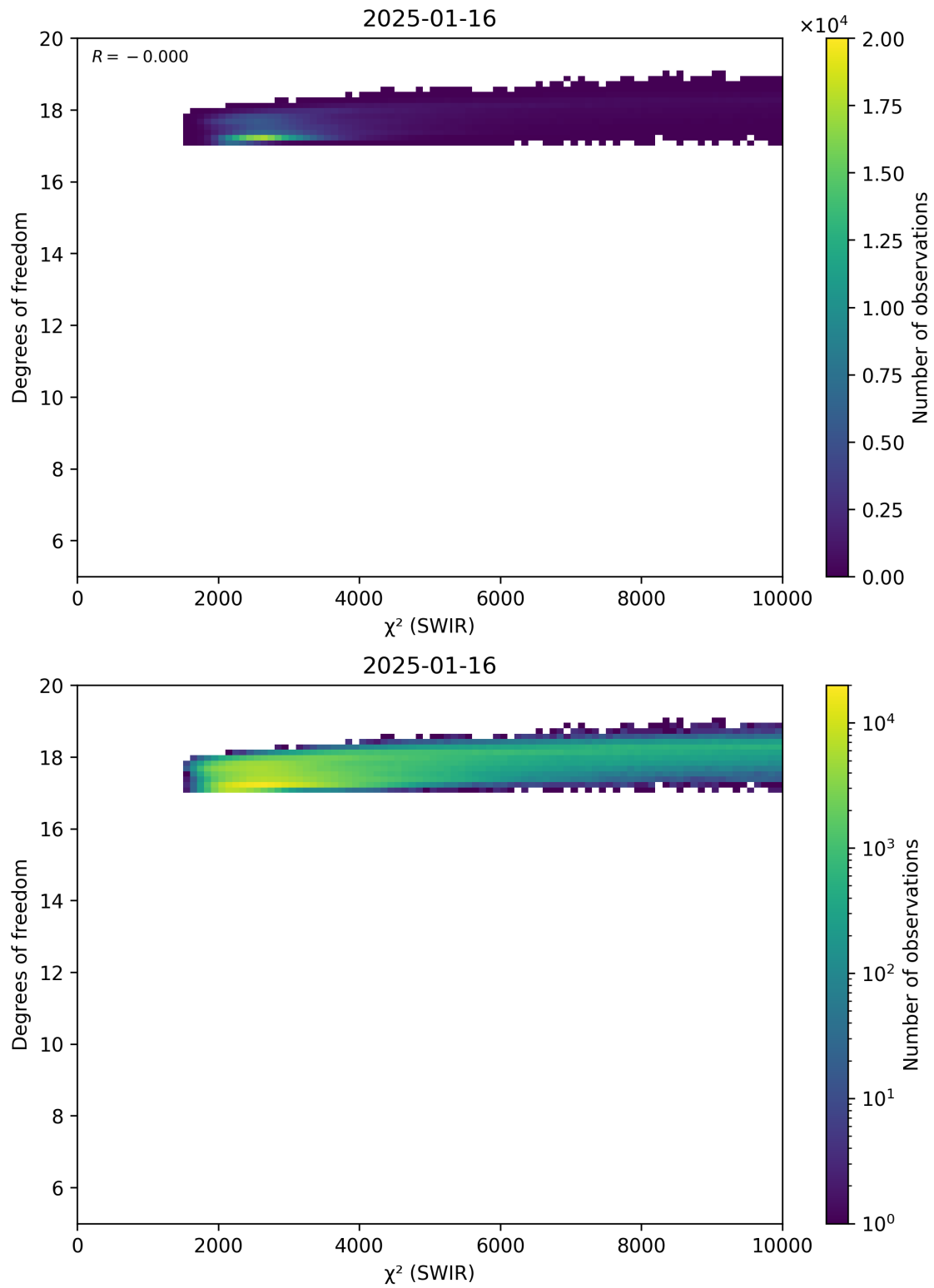
Figure 48: Scatter density plot of “ \chi^2 (SWIR)” against “Degrees of freedom” for 2025-01-15 to 2025-01-17.
