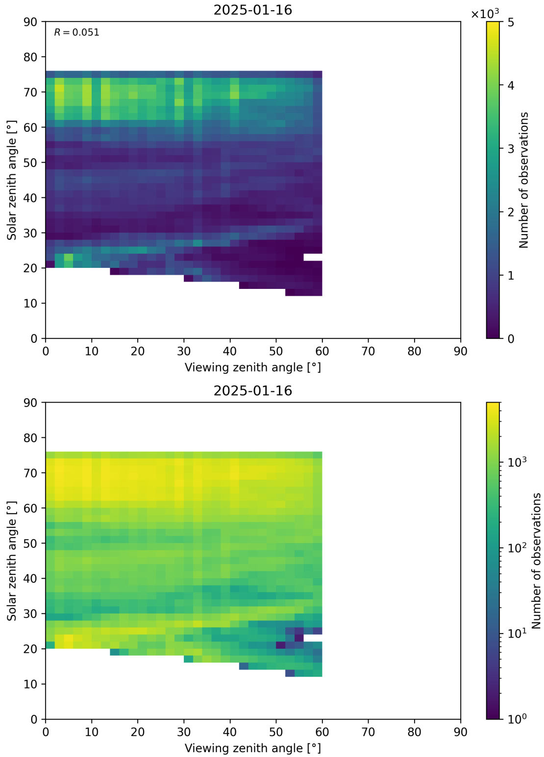
Figure 115: Scatter density plot of “Viewing zenith angle” against “Solar zenith angle” for 2025-01-15 to 2025-01-17.
