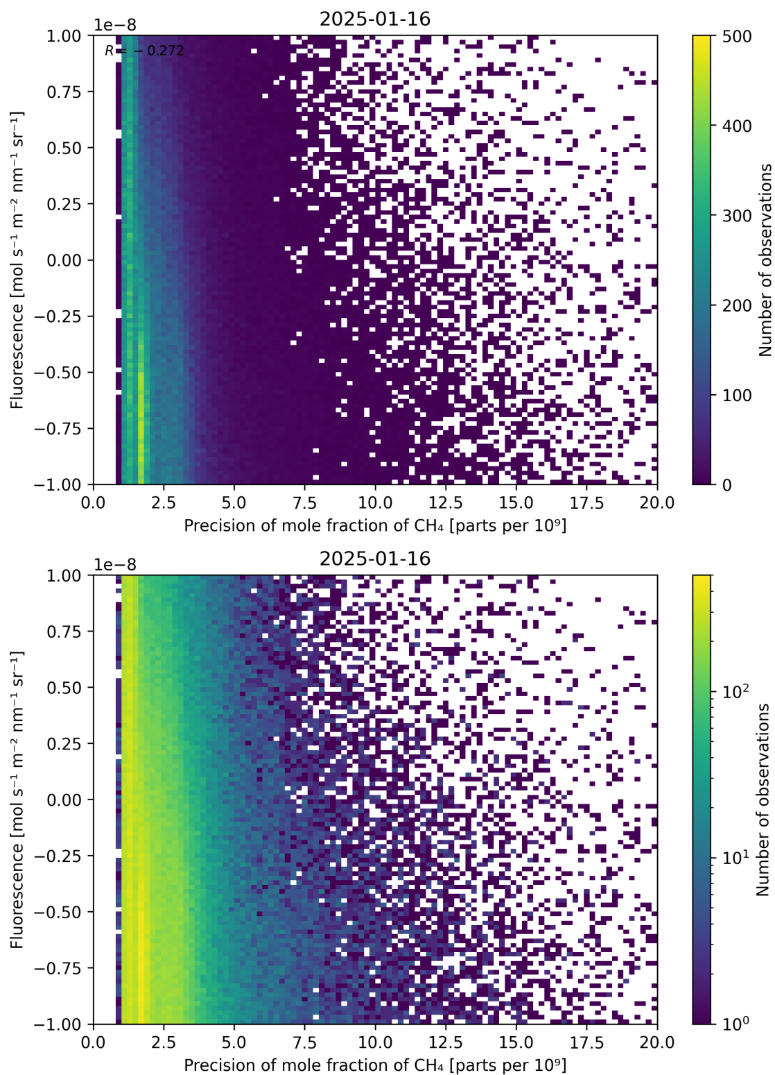
Figure 81: Scatter density plot of “Precision of mole fraction of \text{CH}_4 ” against “Fluorescence” for 2025-01-15 to 2025-01-17.
