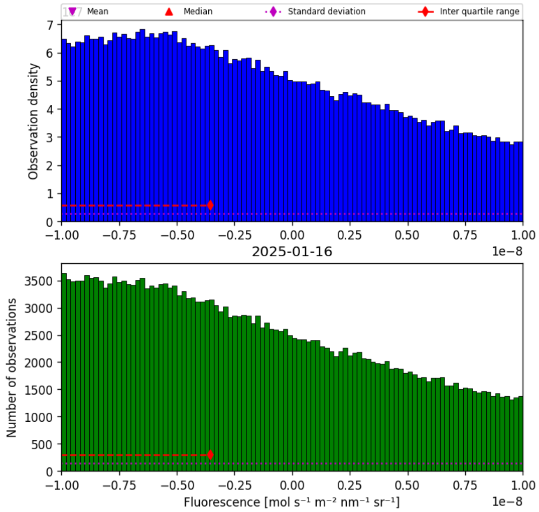
Figure 32: Histogram of “Fluorescence” for 2025-01-15 to 2025-01-17
