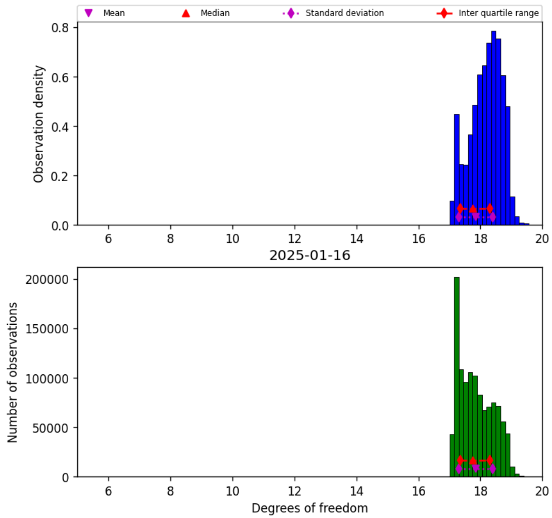
Figure 30: Histogram of “Degrees of freedom” for 2025-01-15 to 2025-01-17
