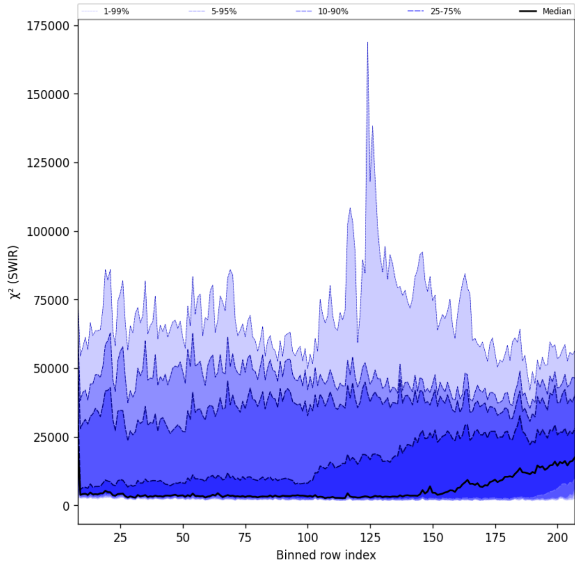
Figure 39: Along track statistics of “ \chi^2 (SWIR)” for 2025-01-15 to 2025-01-17
