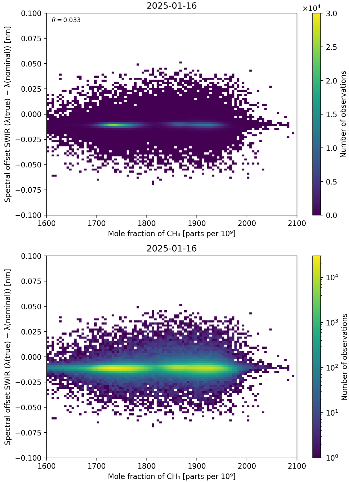
Figure 86: Scatter density plot of “Mole fraction of CH 4 ” against “Spectral offset SWIR ( \lambda_{\text{true}} - \lambda_{\text{nominal}} )” for 2025-01-15 to 2025-01-17.
