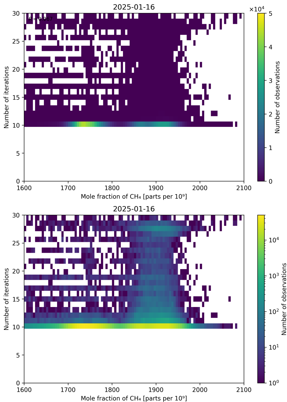
Figure 76: Scatter density plot of “Mole fraction of CH 4 ” against “Number of iterations” for 2025-01-15 to 2025-01-17.
