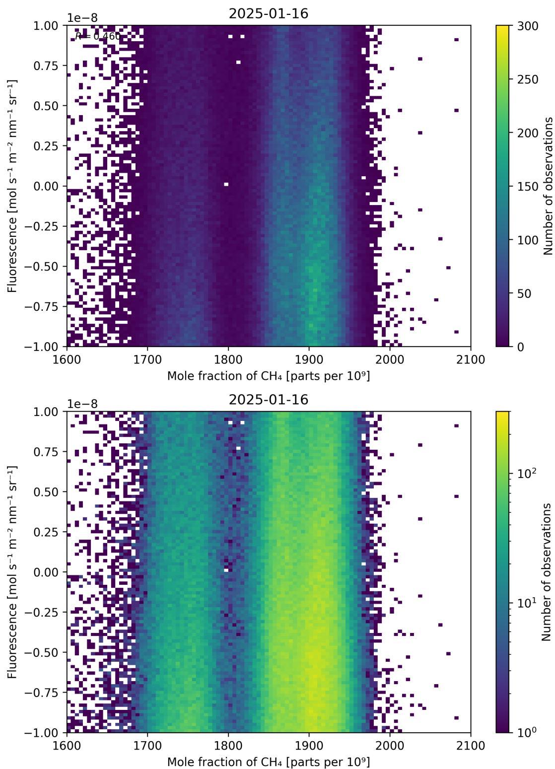
Figure 73: Scatter density plot of “Mole fraction of \text{CH}_4 ” against “Fluorescence” for 2025-01-15 to 2025-01-17.
