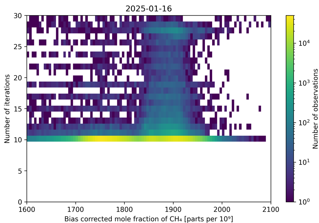
Figure 67: Scatter density plot of “Bias corrected mole fraction of CH 4 ” against “Number of iterations” for 2025-01-15 to 2025-01-17.
