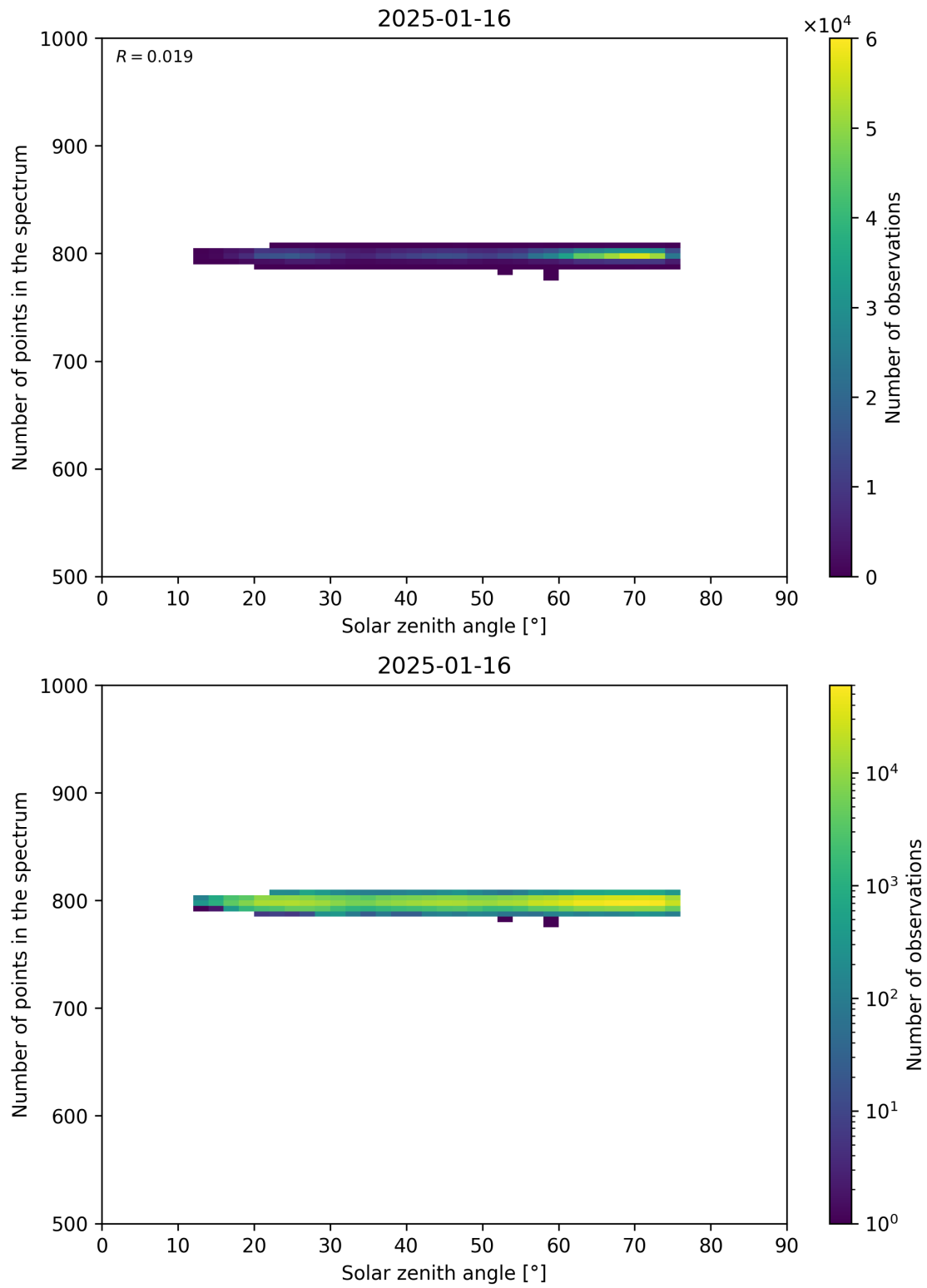
Figure 103: Scatter density plot of “Solar zenith angle” against “Number of points in the spectrum” for 2025-01-15 to 2025-01-17.
