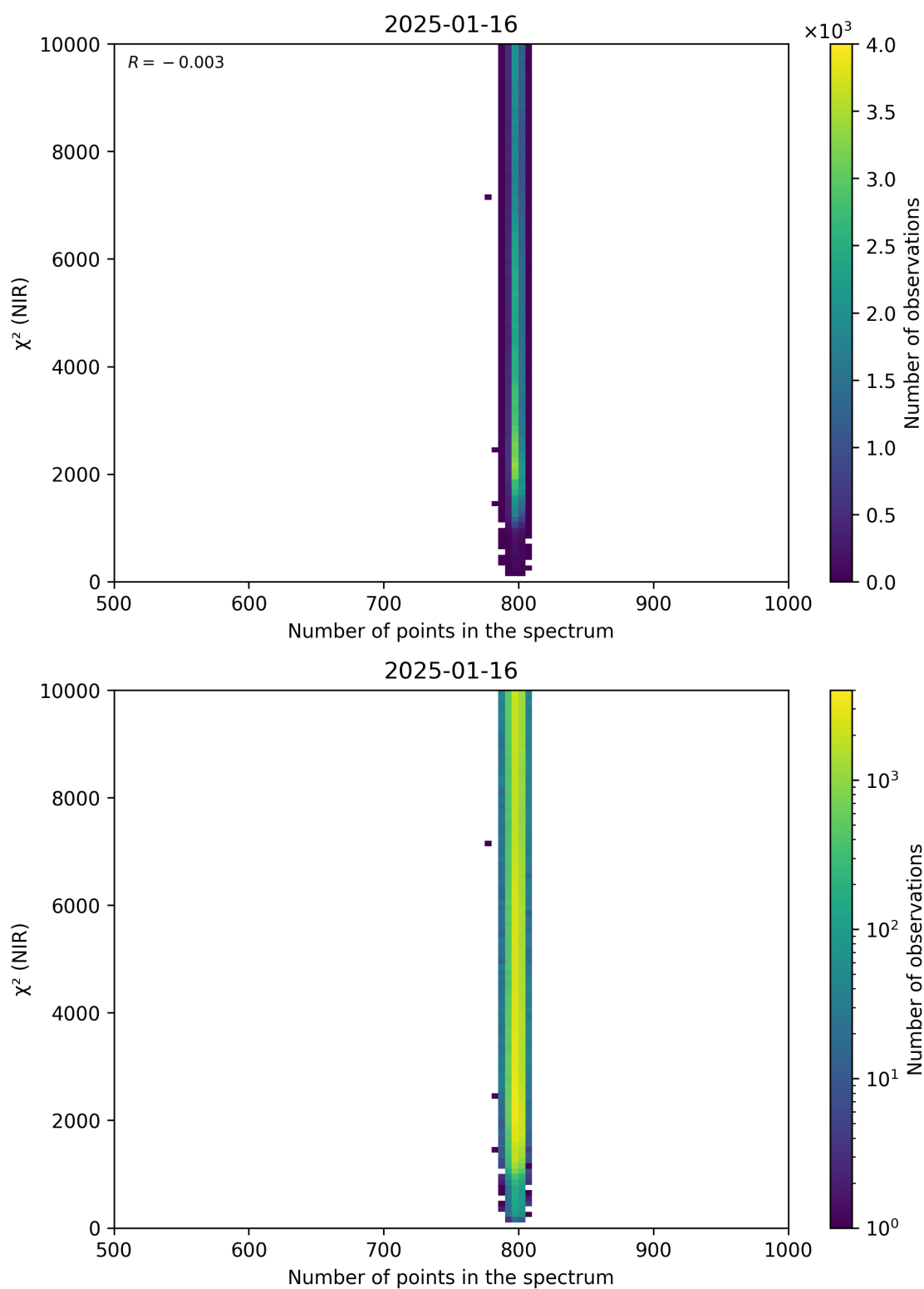
Figure 88: Scatter density plot of “Number of points in the spectrum” against “ \chi^2 (NIR)” for 2025-01-15 to 2025-01-17.
