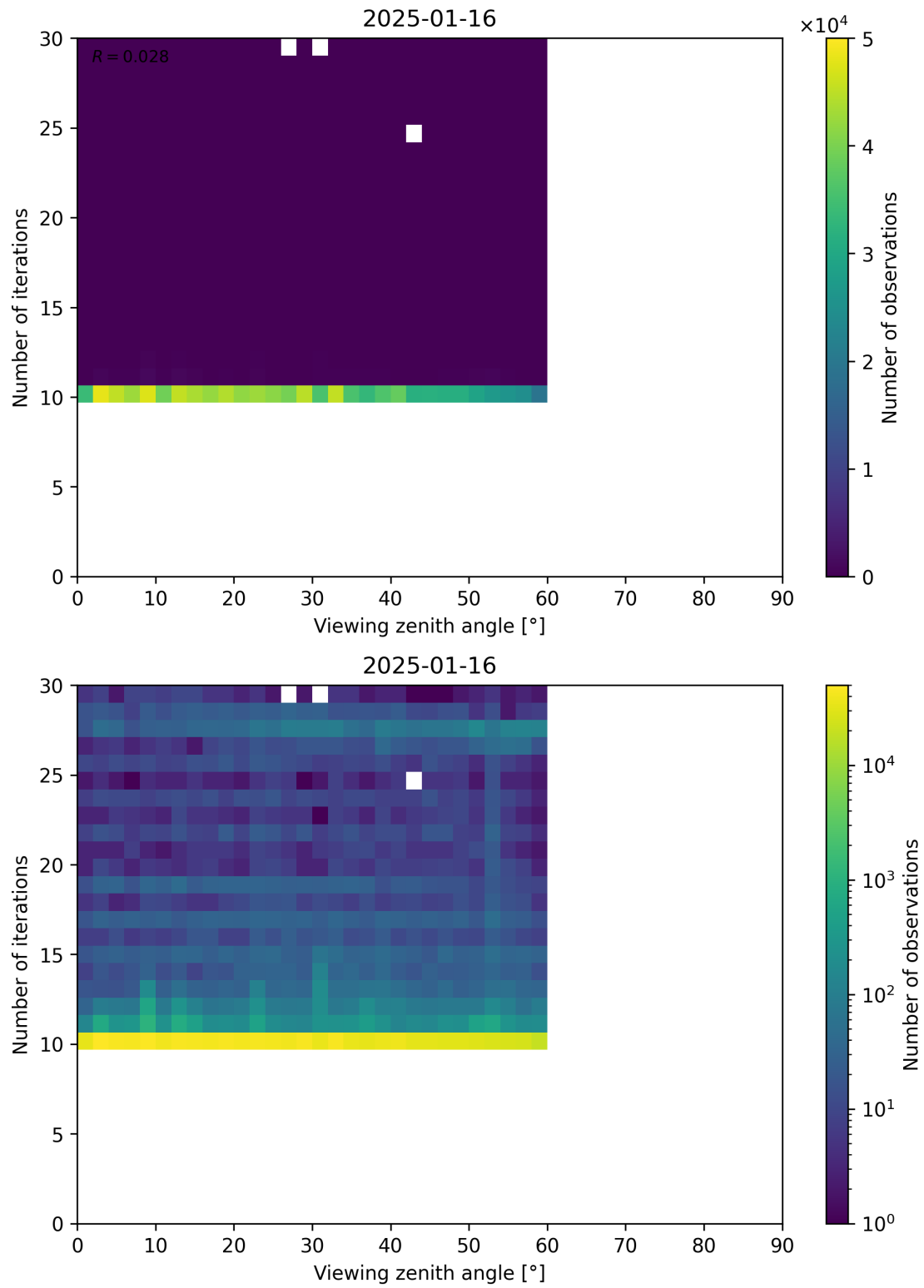
Figure 113: Scatter density plot of “Viewing zenith angle” against “Number of iterations” for 2025-01-15 to 2025-01-17.
