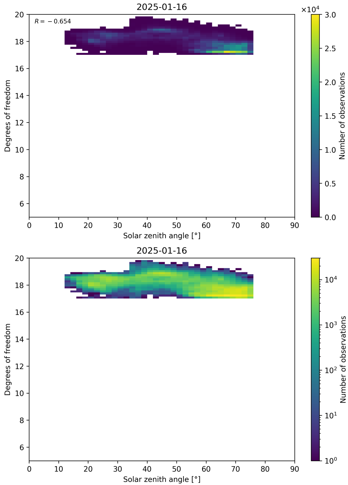
Figure 96: Scatter density plot of “Solar zenith angle” against “Degrees of freedom” for 2025-01-15 to 2025-01-17.
