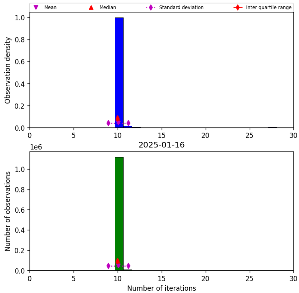
Figure 31: Histogram of “Number of iterations” for 2025-01-15 to 2025-01-17
