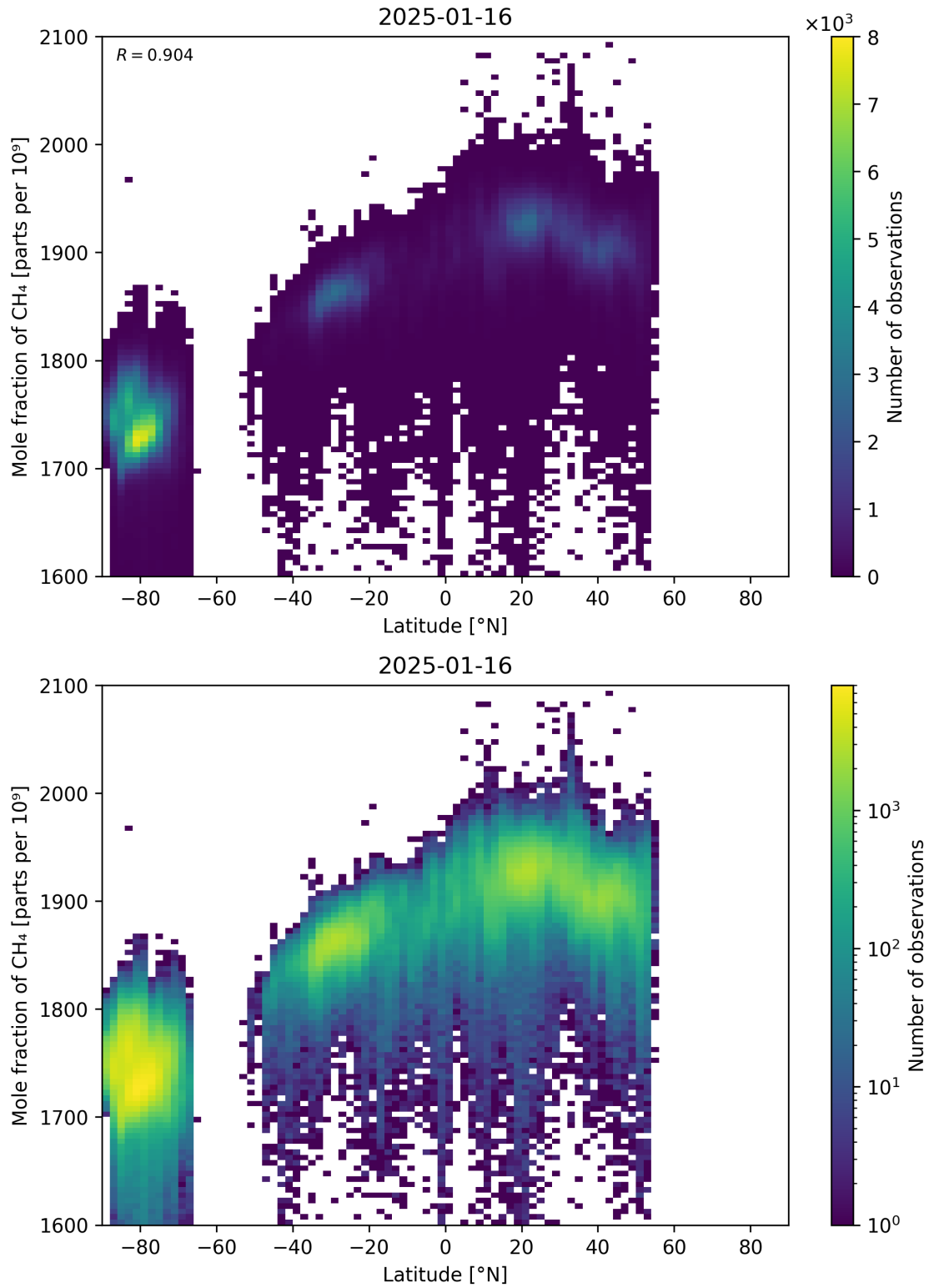
Figure 57: Scatter density plot of “Latitude” against “Mole fraction of CH 4 ” for 2025-01-15 to 2025-01-17.
