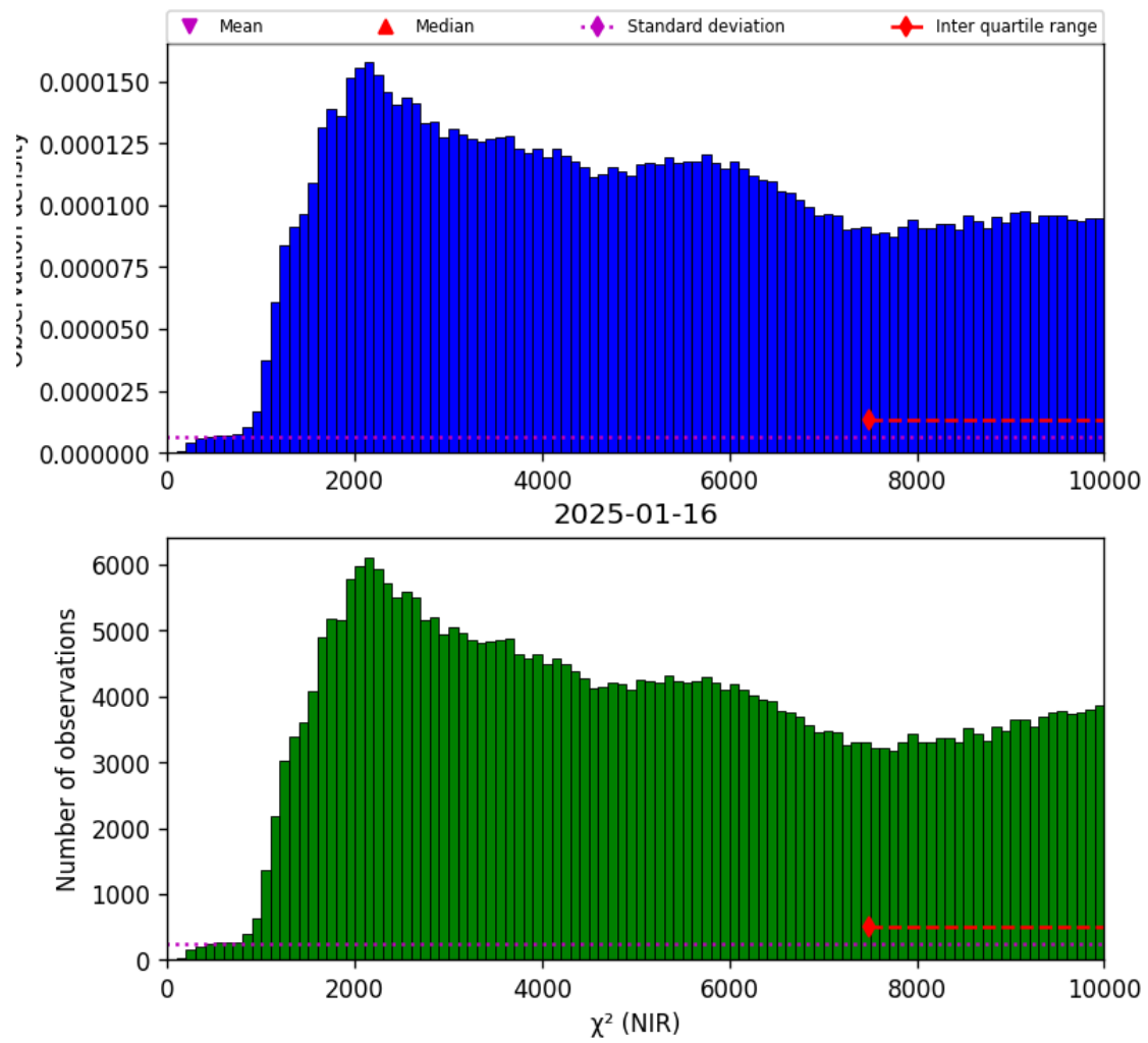
Figure 29: Histogram of “ \chi^2 (NIR)” for 2025-01-15 to 2025-01-17
