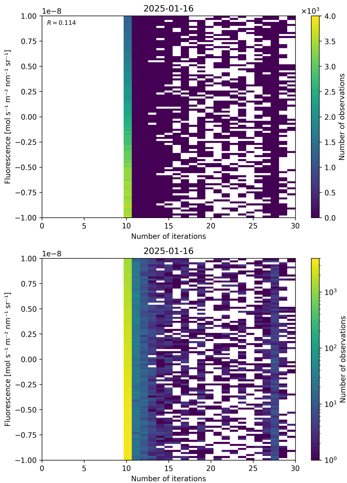
Figure 87: Scatter density plot of “Number of iterations” against “Fluorescence” for 2025-01-15 to 2025-01-17.
