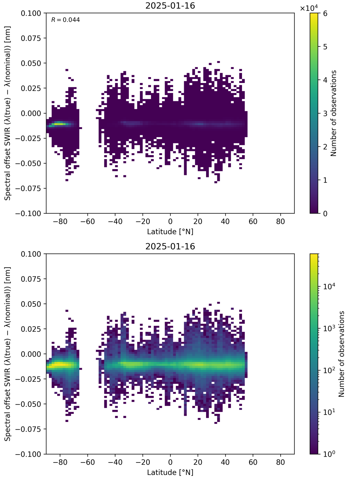
Figure 62: Scatter density plot of “Latitude” against “Spectral offset SWIR ( \lambda_{\text{true}} - \lambda_{\text{nominal}} )” for 2025-01-15 to 2025-01-17.
