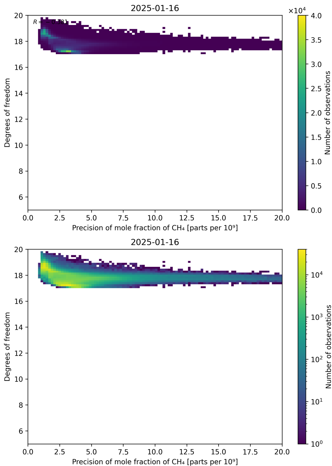
Figure 80: Scatter density plot of “Precision of mole fraction of CH 4 ” against “Degrees of freedom” for 2025-01-15 to 2025-01-17.
