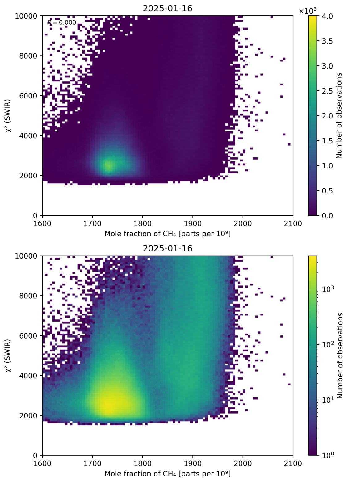
Figure 71: Scatter density plot of “Mole fraction of CH 4 ” against “ \chi^2 (SWIR)” for 2025-01-15 to 2025-01-17.
