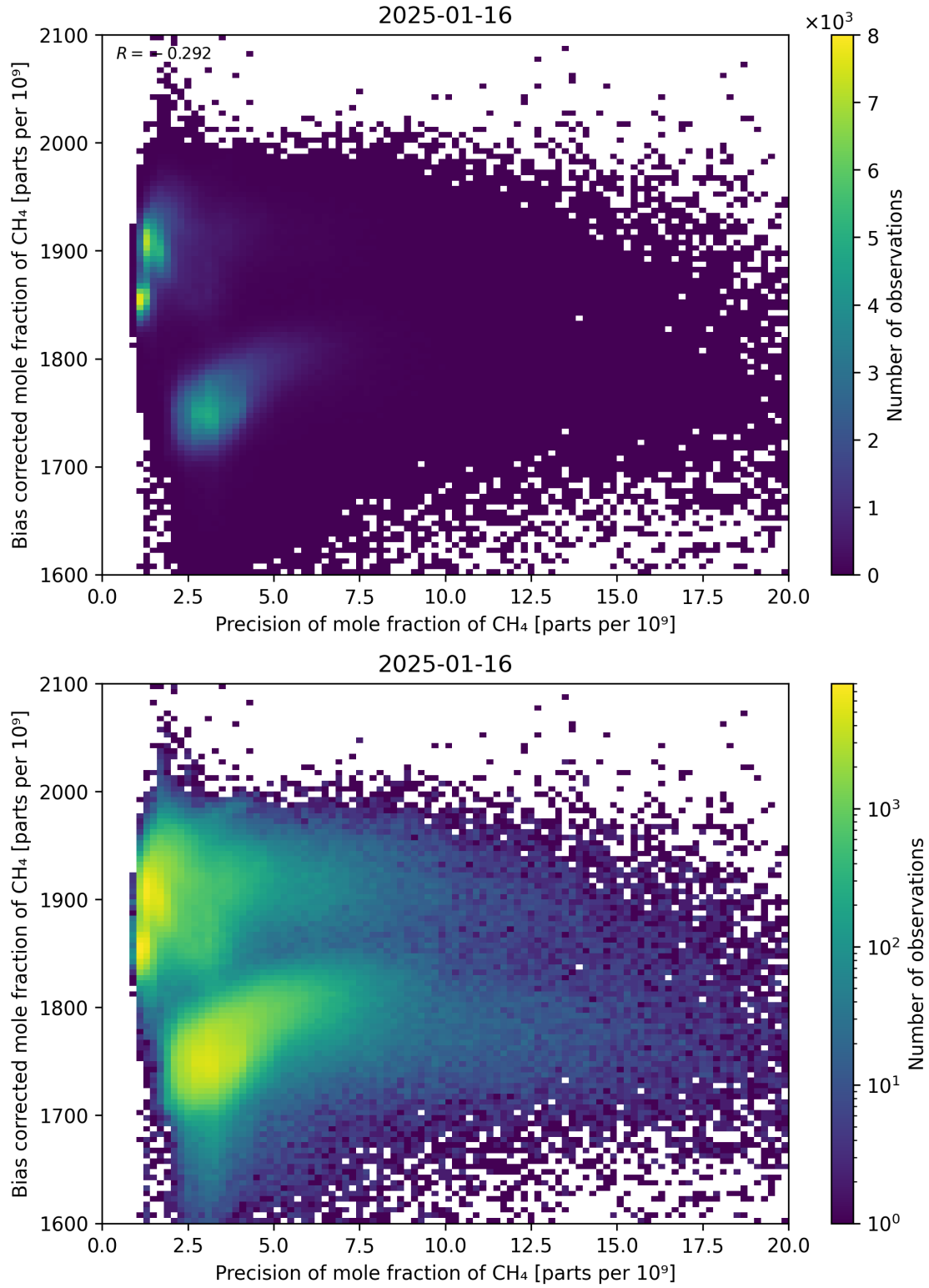
Figure 82: Scatter density plot of “Precision of mole fraction of CH 4 ” against “Bias corrected mole fraction of CH 4 ” for 2025-01-15 to 2025-01-17.
