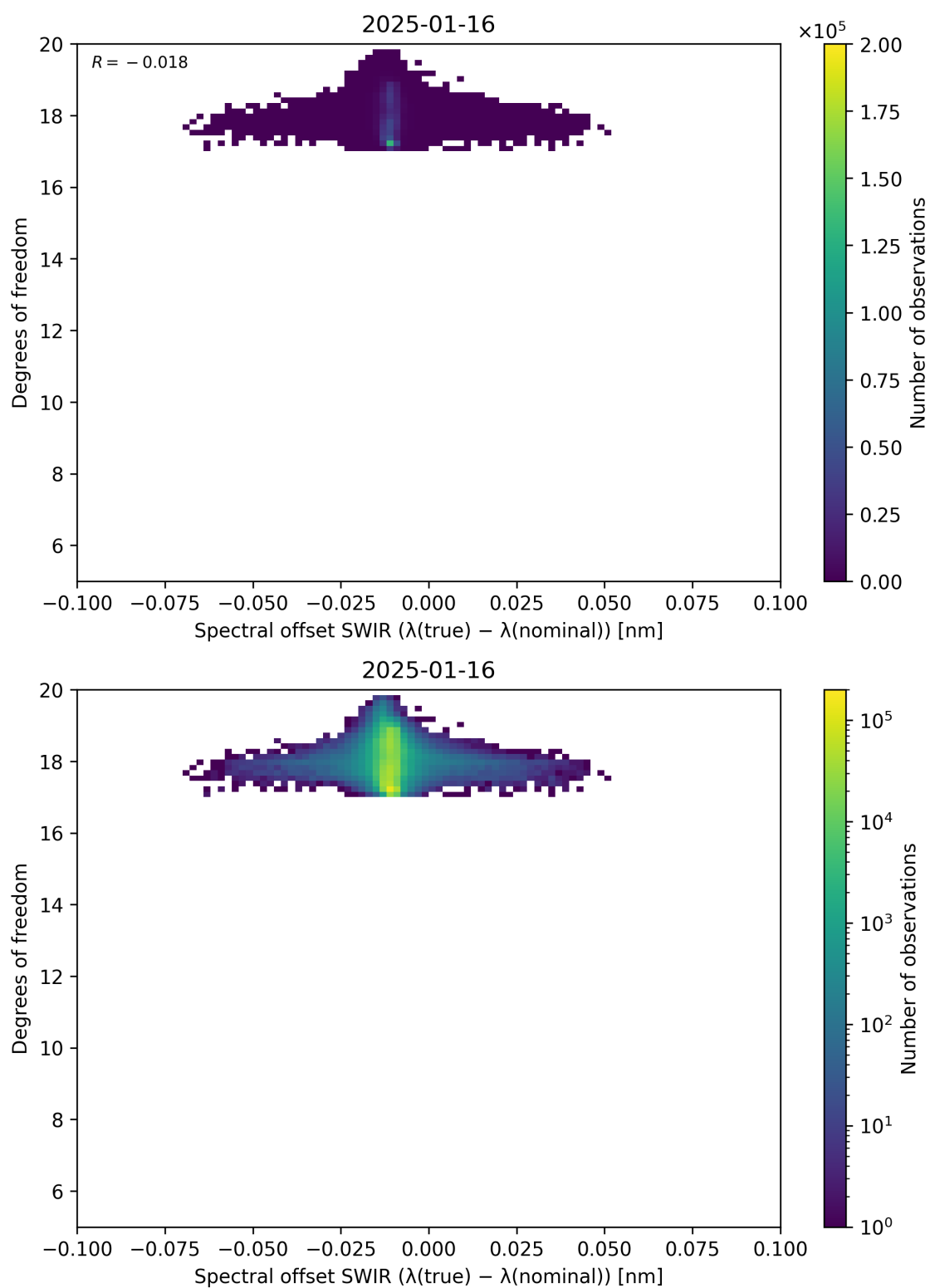
Figure 119: Scatter density plot of “Spectral offset SWIR ( \lambda_{\text{true}} - \lambda_{\text{nominal}} )” against “Degrees of freedom” for 2025-01-15 to 2025-01-17.
