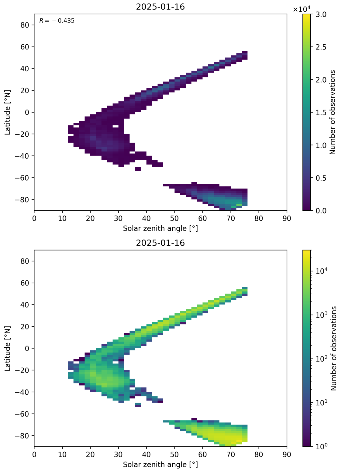
Figure 98: Scatter density plot of “Solar zenith angle” against “Latitude” for 2025-01-15 to 2025-01-17.
