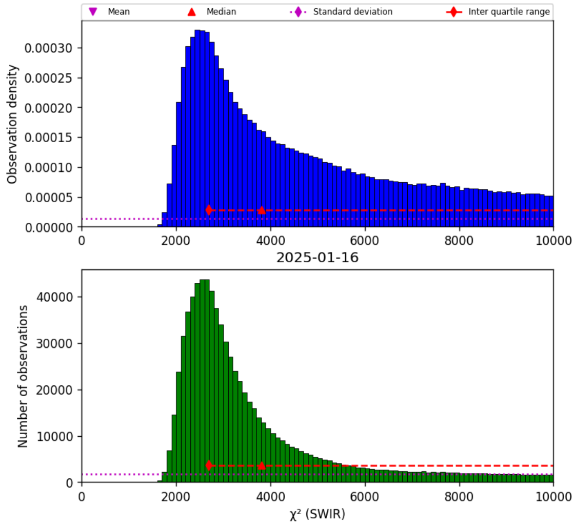
Figure 28: Histogram of “ \chi^2 (SWIR)” for 2025-01-15 to 2025-01-17
