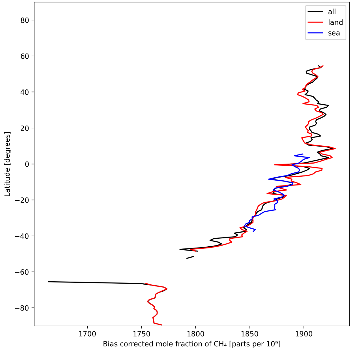
Figure 14: Zonal average of “Bias corrected mole fraction of CH 4 ” for 2025-01-15 to 2025-01-17.
