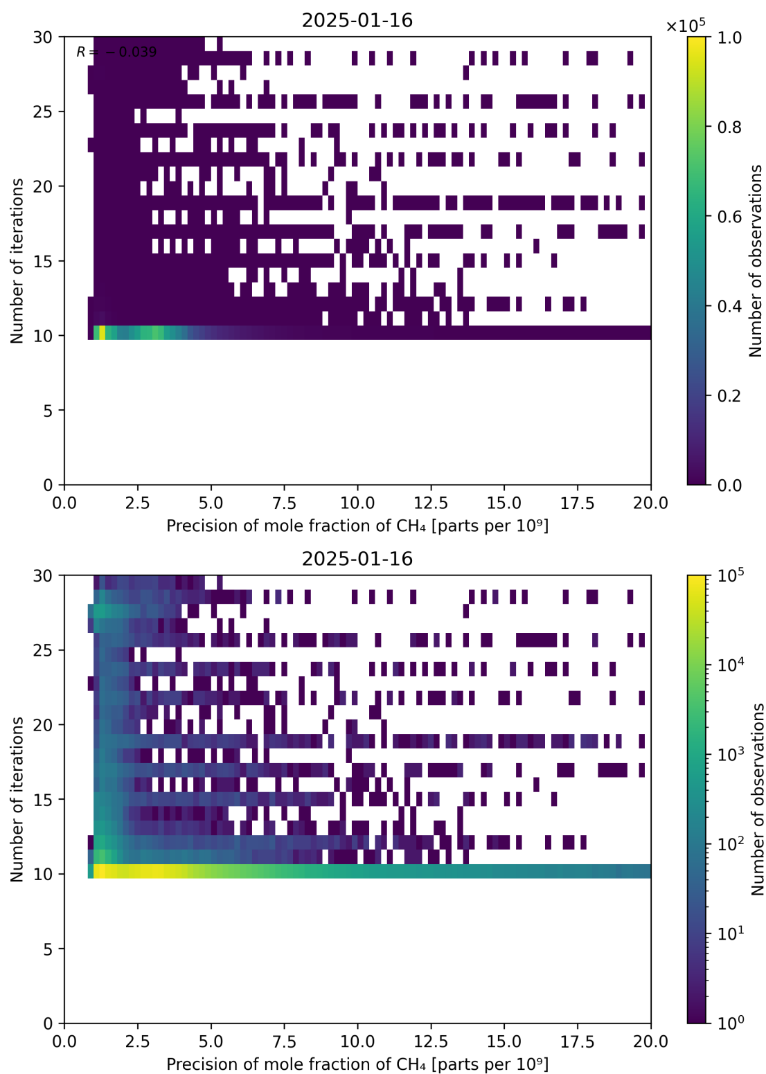
Figure 83: Scatter density plot of “Precision of mole fraction of CH 4 ” against “Number of iterations” for 2025-01-15 to 2025-01-17.
