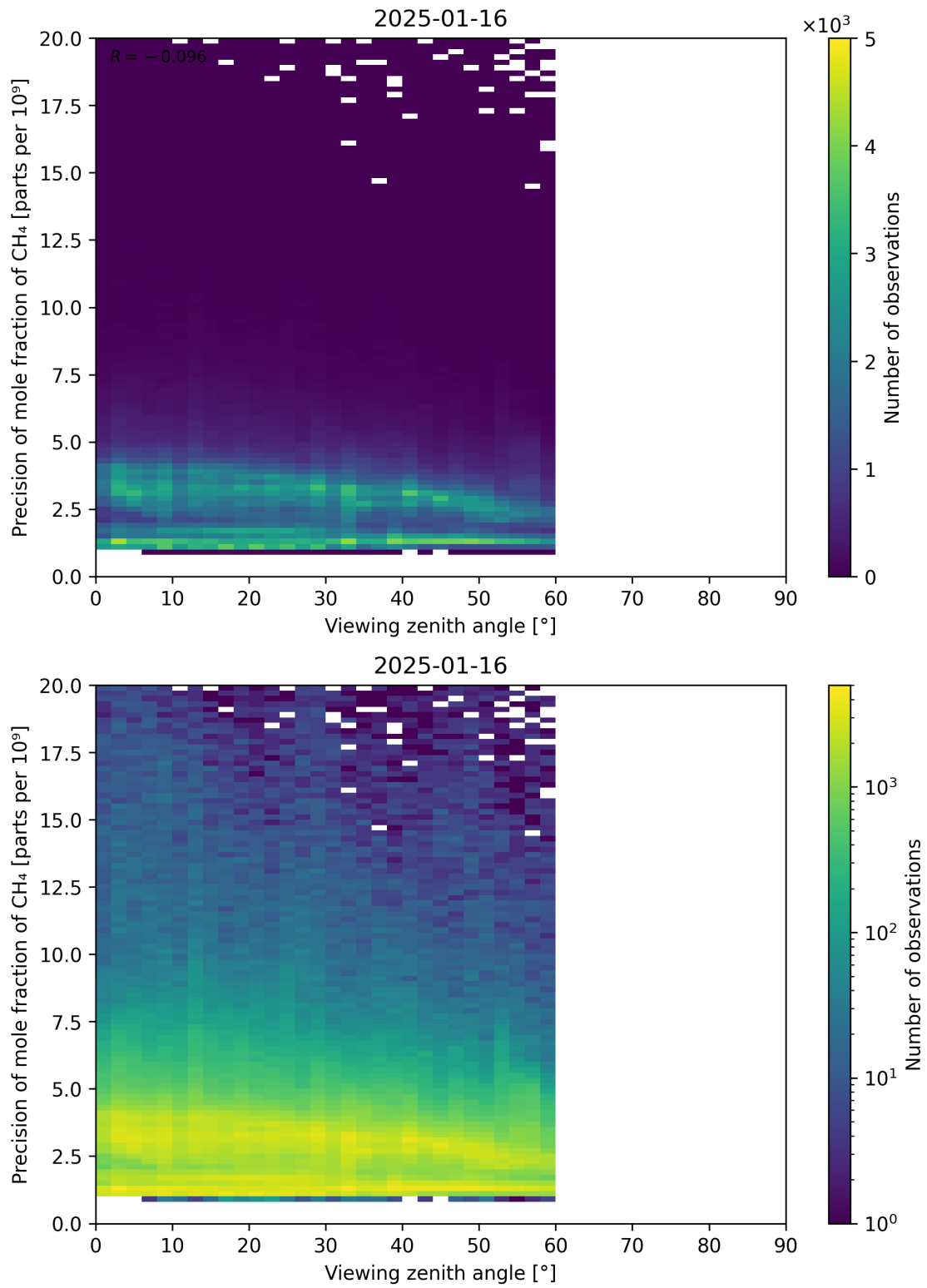
Figure 112: Scatter density plot of “Viewing zenith angle” against “Precision of mole fraction of CH 4 ” for 2025-01-15 to 2025-01-17.
