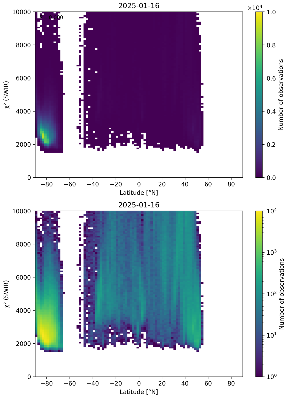
Figure 54: Scatter density plot of “Latitude” against “ \chi^2 (SWIR)” for 2025-01-15 to 2025-01-17.
