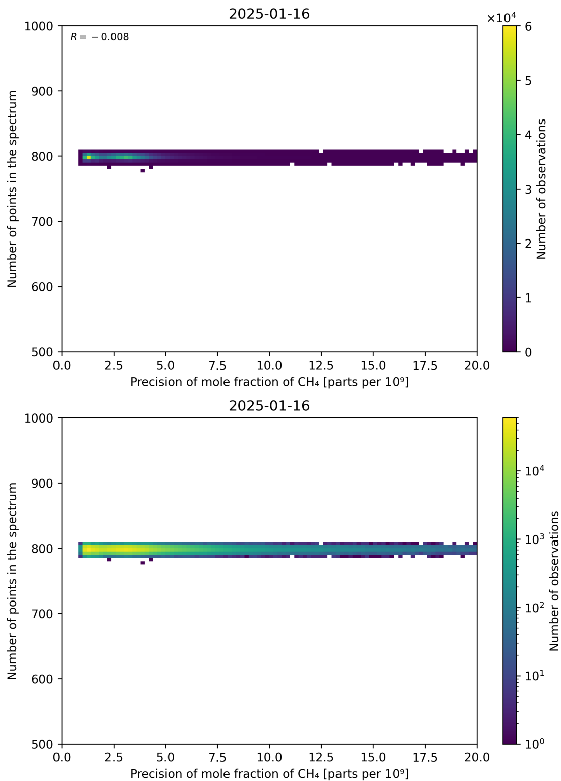
Figure 84: Scatter density plot of “Precision of mole fraction of CH 4 ” against “Number of points in the spectrum” for 2025-01-15 to 2025-01-17.
