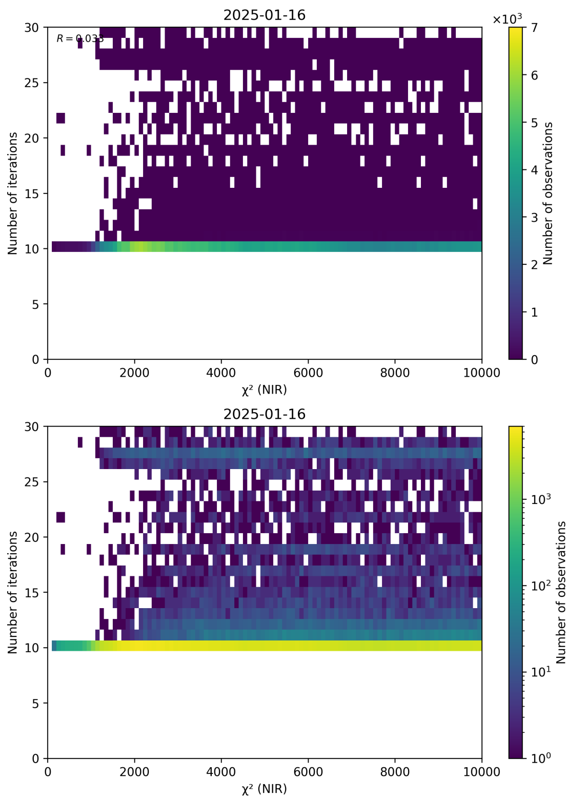
Figure 46: Scatter density plot of “ \chi^2 (NIR)” against “Number of iterations” for 2025-01-15 to 2025-01-17.
