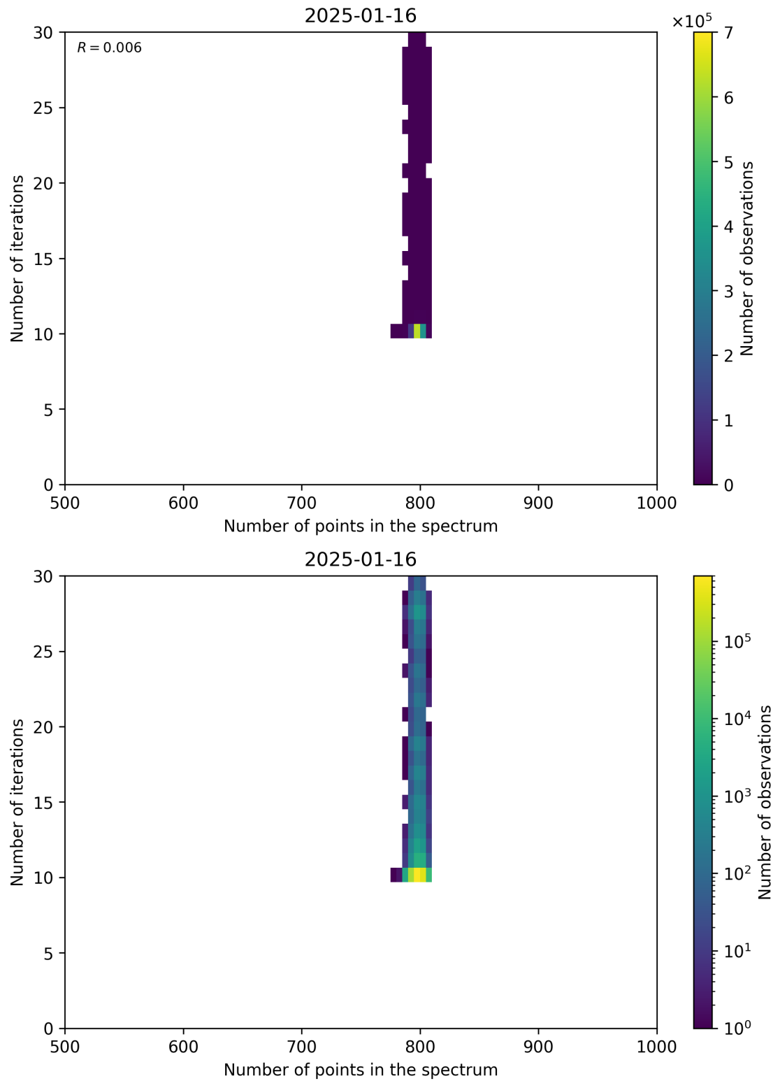
Figure 92: Scatter density plot of “Number of points in the spectrum” against “Number of iterations” for 2025-01-15 to 2025-01-17.
