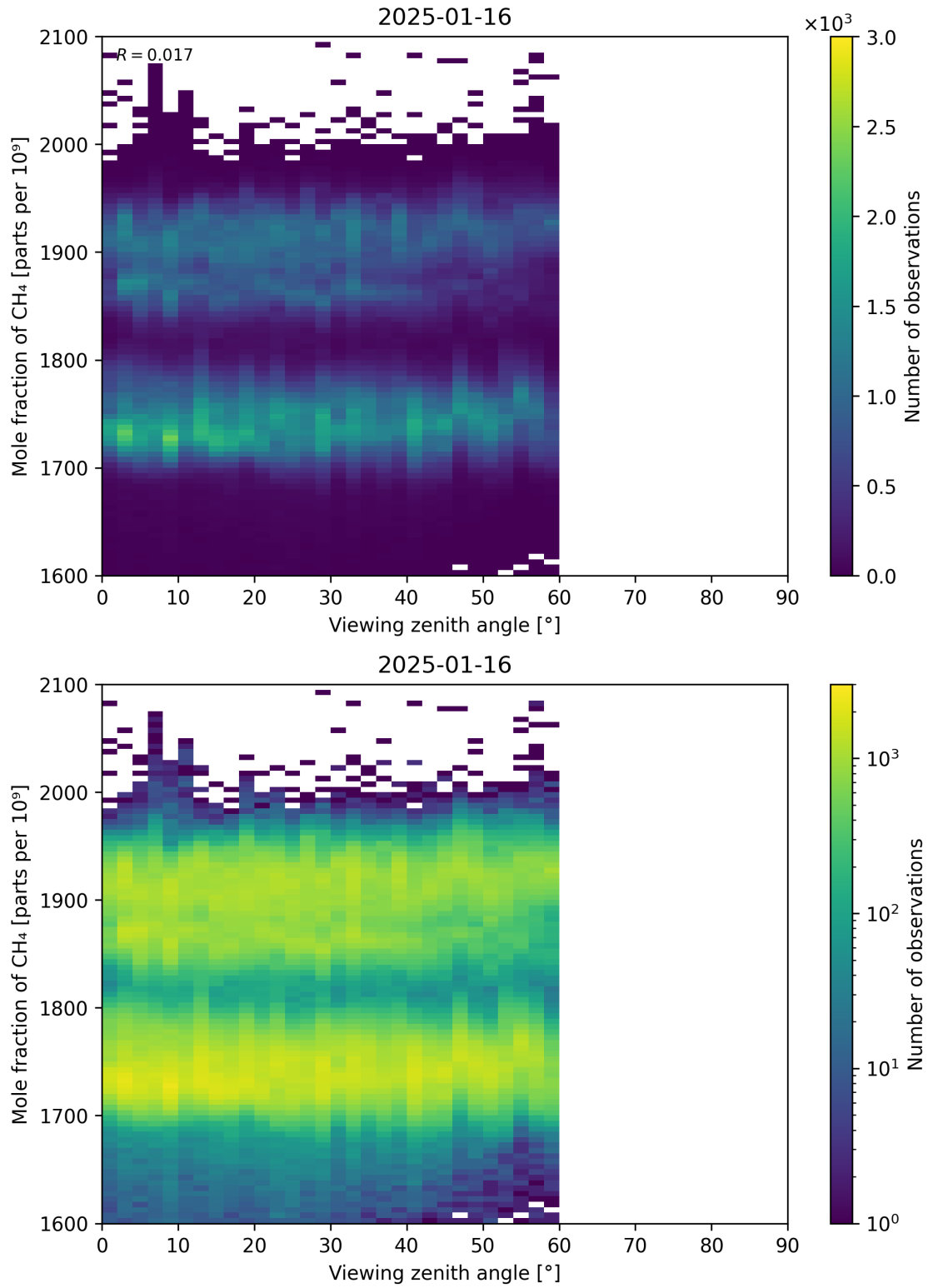
Figure 110: Scatter density plot of “Viewing zenith angle” against “Mole fraction of CH 4 ” for 2025-01-15 to 2025-01-17.
