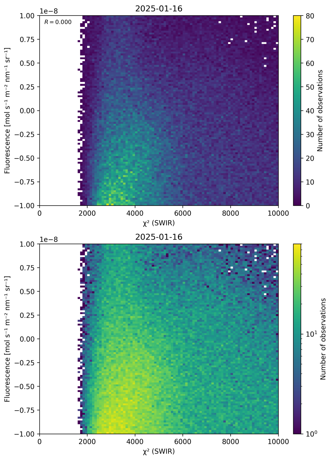
Figure 49: Scatter density plot of “ \chi^2 (SWIR)” against “Fluorescence” for 2025-01-15 to 2025-01-17.
