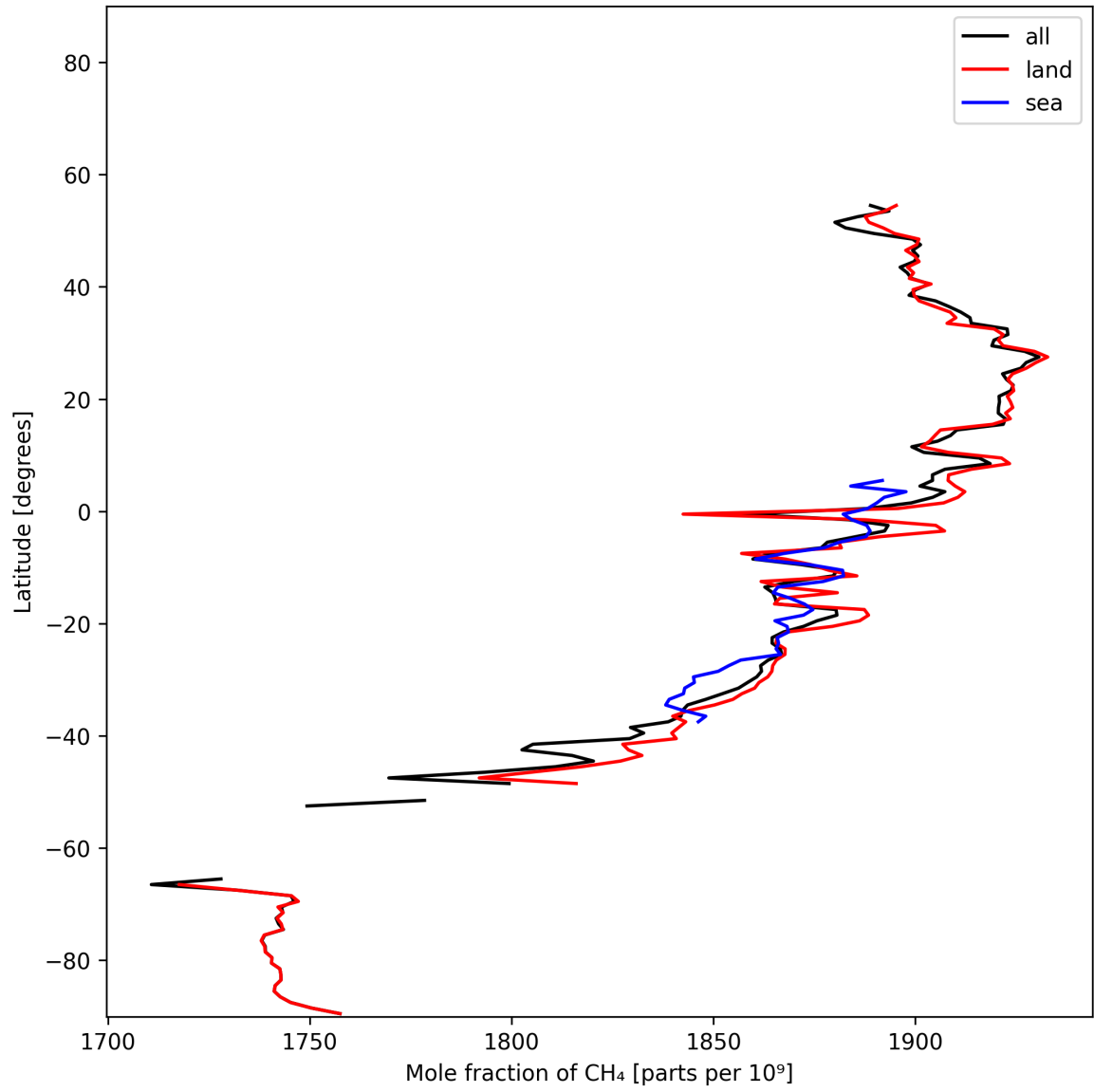
Figure 12: Zonal average of “Mole fraction of CH 4 ” for 2025-01-15 to 2025-01-17.
