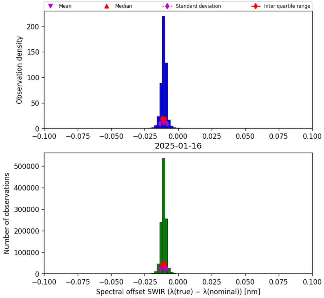
Figure 27: Histogram of “Spectral offset SWIR ( \lambda_{\text{true}} - \lambda_{\text{nominal}} )” for 2025-01-15 to 2025-01-17
