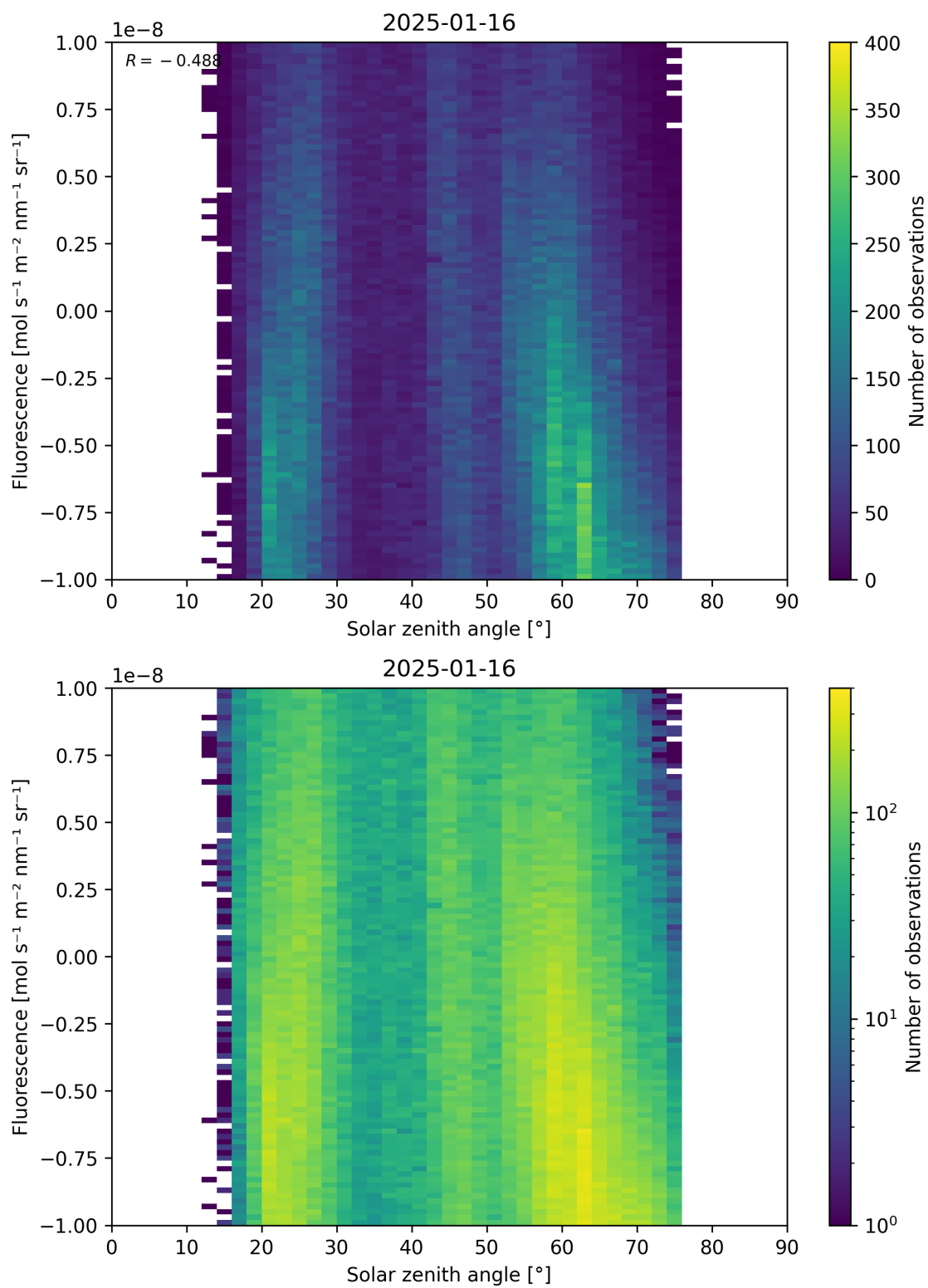
Figure 97: Scatter density plot of “Solar zenith angle” against “Fluorescence” for 2025-01-15 to 2025-01-17.
