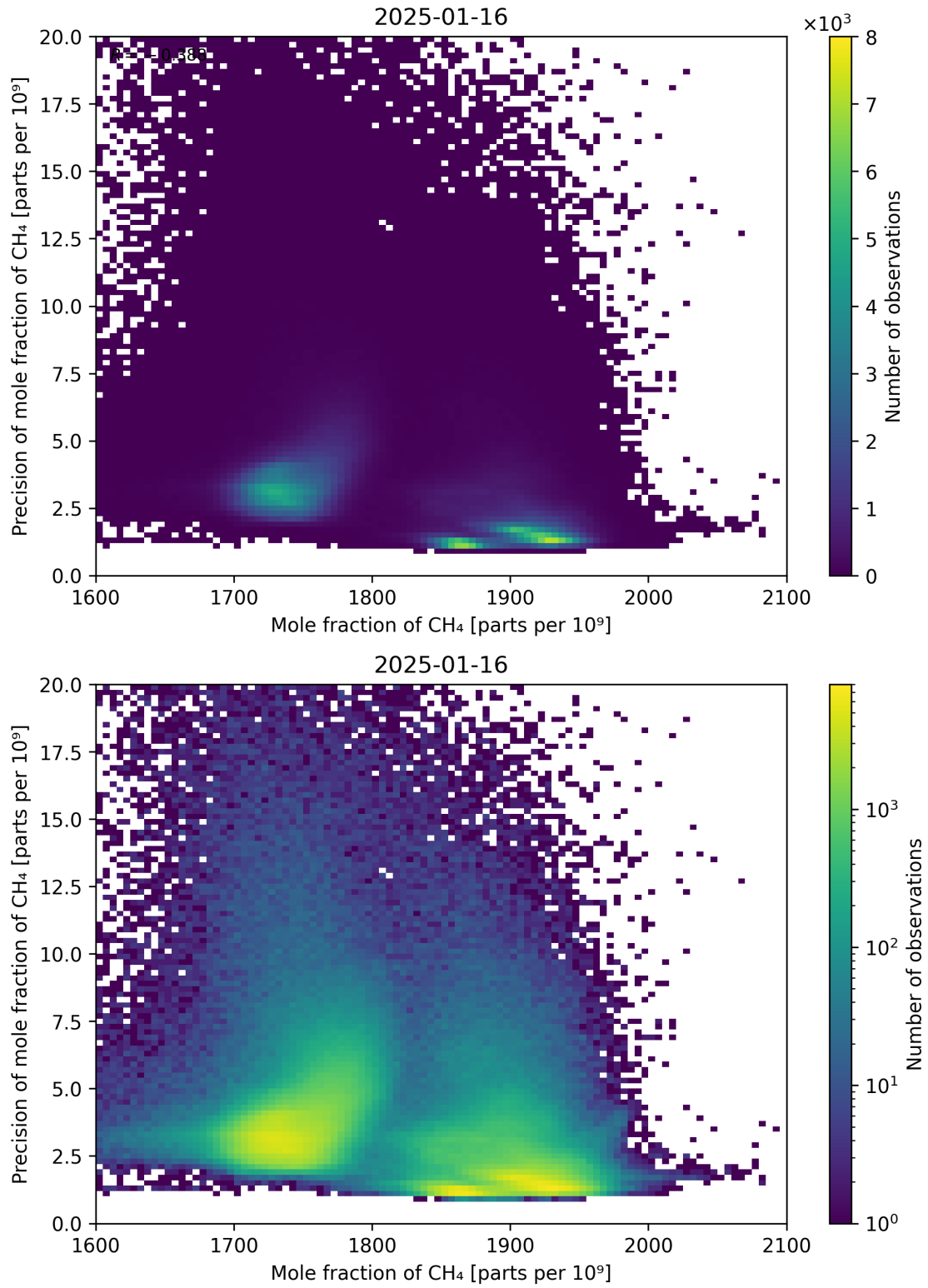
Figure 75: Scatter density plot of “Mole fraction of CH 4 ” against “Precision of mole fraction of CH 4 ” for 2025-01-15 to 2025-01-17.
