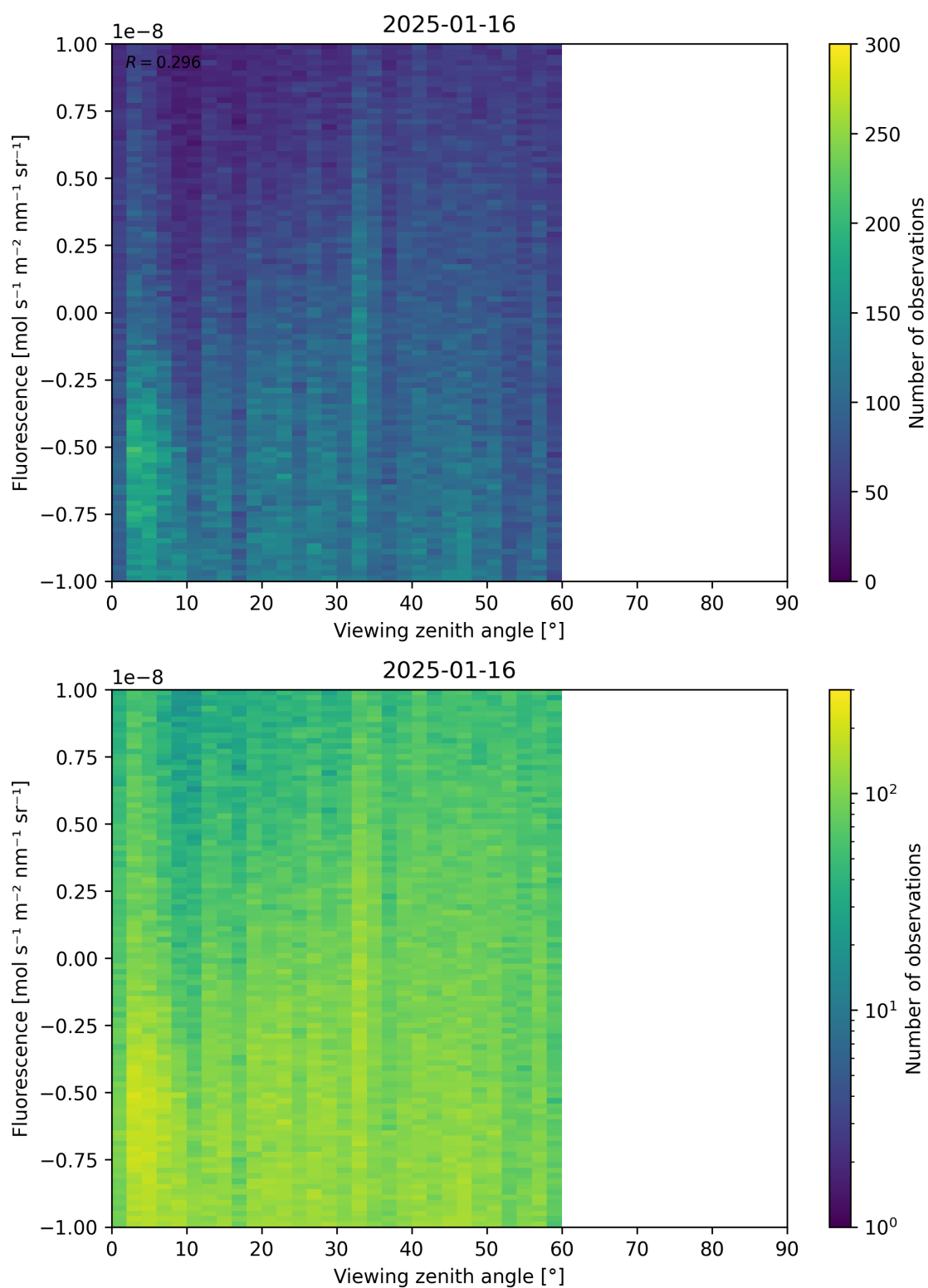
Figure 108: Scatter density plot of “Viewing zenith angle” against “Fluorescence” for 2025-01-15 to 2025-01-17.
