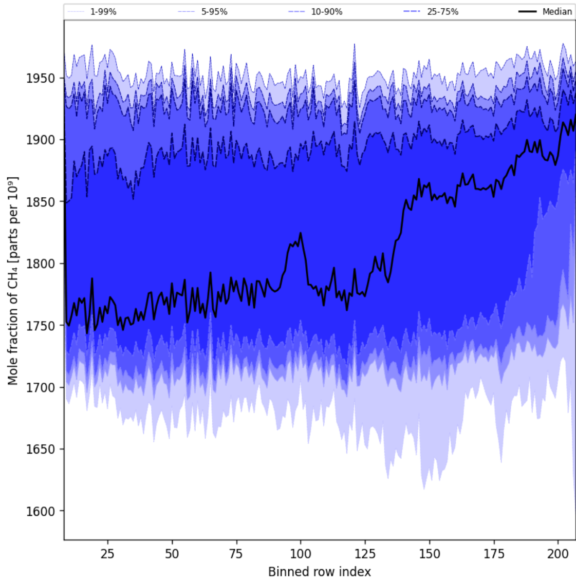
Figure 34: Along track statistics of “Mole fraction of CH 4 ” for 2025-01-15 to 2025-01-17
