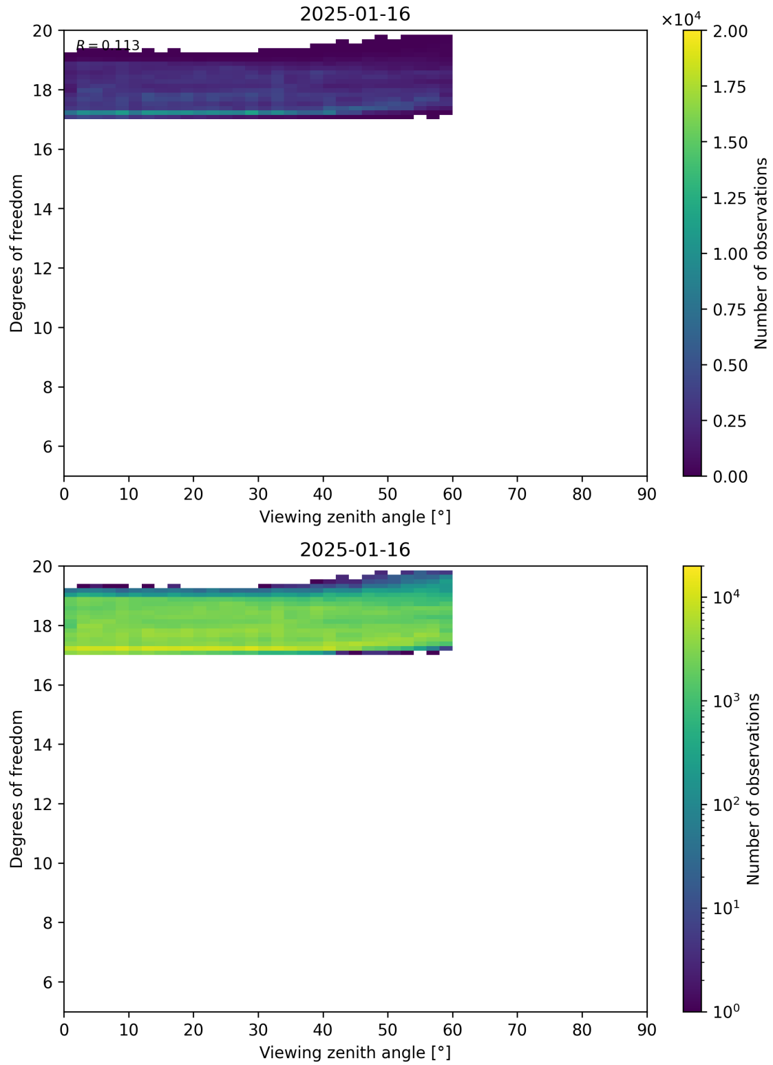
Figure 107: Scatter density plot of “Viewing zenith angle” against “Degrees of freedom” for 2025-01-15 to 2025-01-17.
