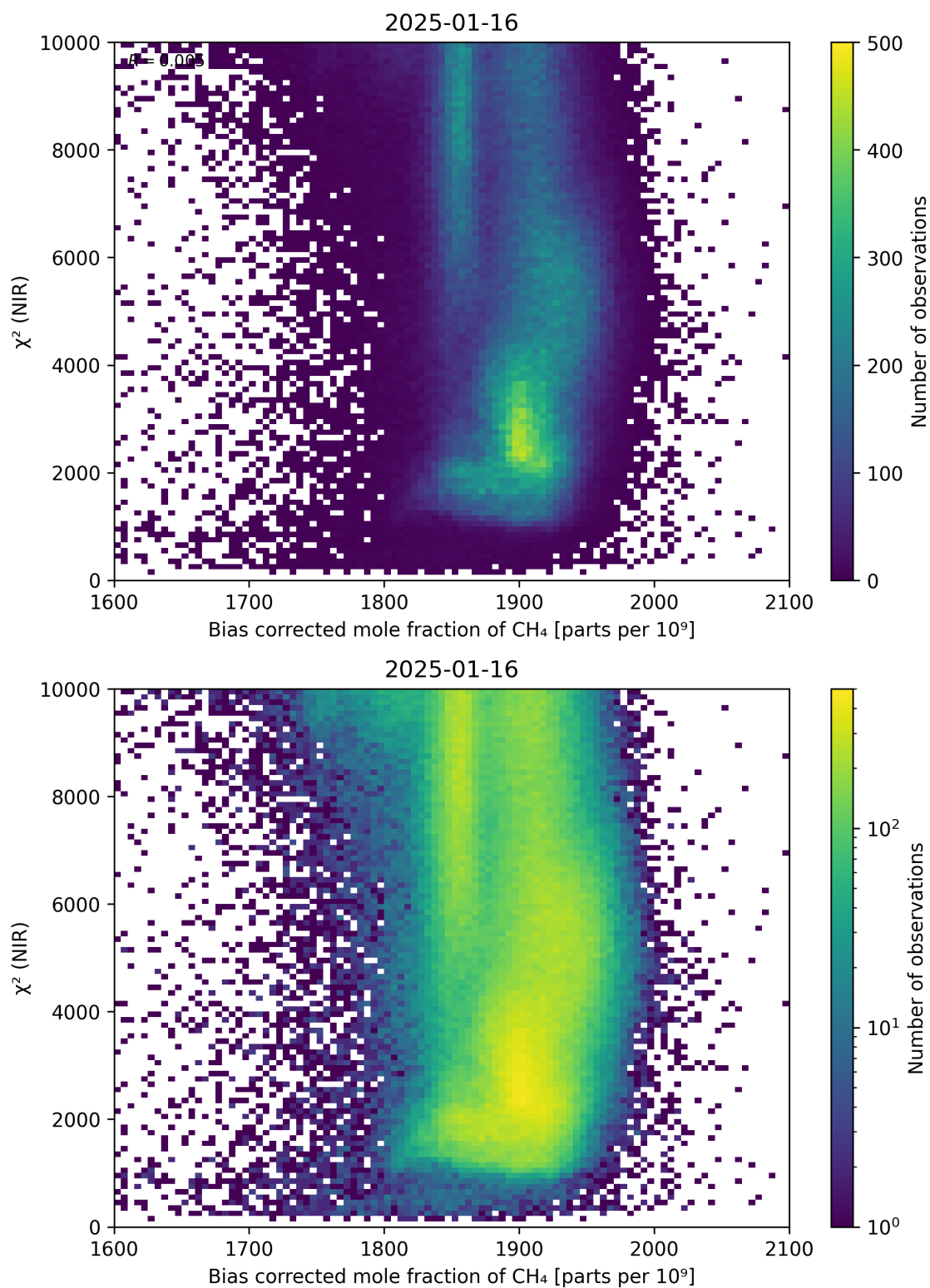
Figure 63: Scatter density plot of “Bias corrected mole fraction of \text{CH}_4 ” against “ \chi^2 (NIR)” for 2025-01-15 to 2025-01-17.
