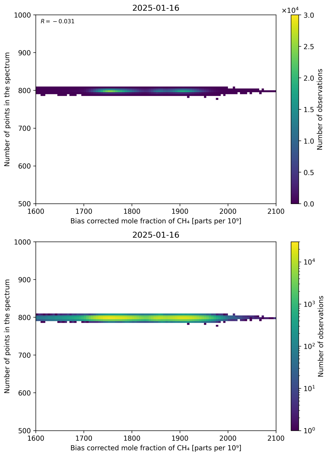
Figure 68: Scatter density plot of “Bias corrected mole fraction of CH 4 ” against “Number of points in the spectrum” for 2025-01-15 to 2025-01-17.
