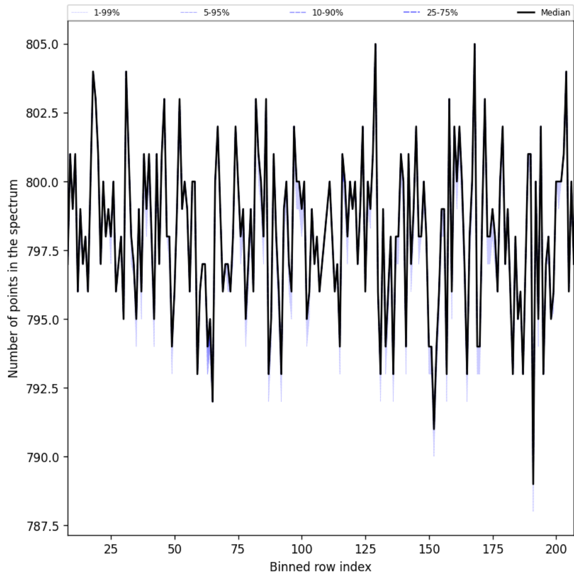
Figure 37: Along track statistics of “Number of points in the spectrum” for 2025-01-15 to 2025-01-17
