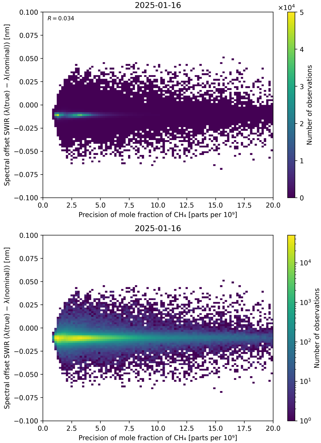
Figure 85: Scatter density plot of “Precision of mole fraction of CH 4 ” against “Spectral offset SWIR ( \lambda_{\text{true}} - \lambda_{\text{nominal}} )” for 2025-01-15 to 2025-01-17.
