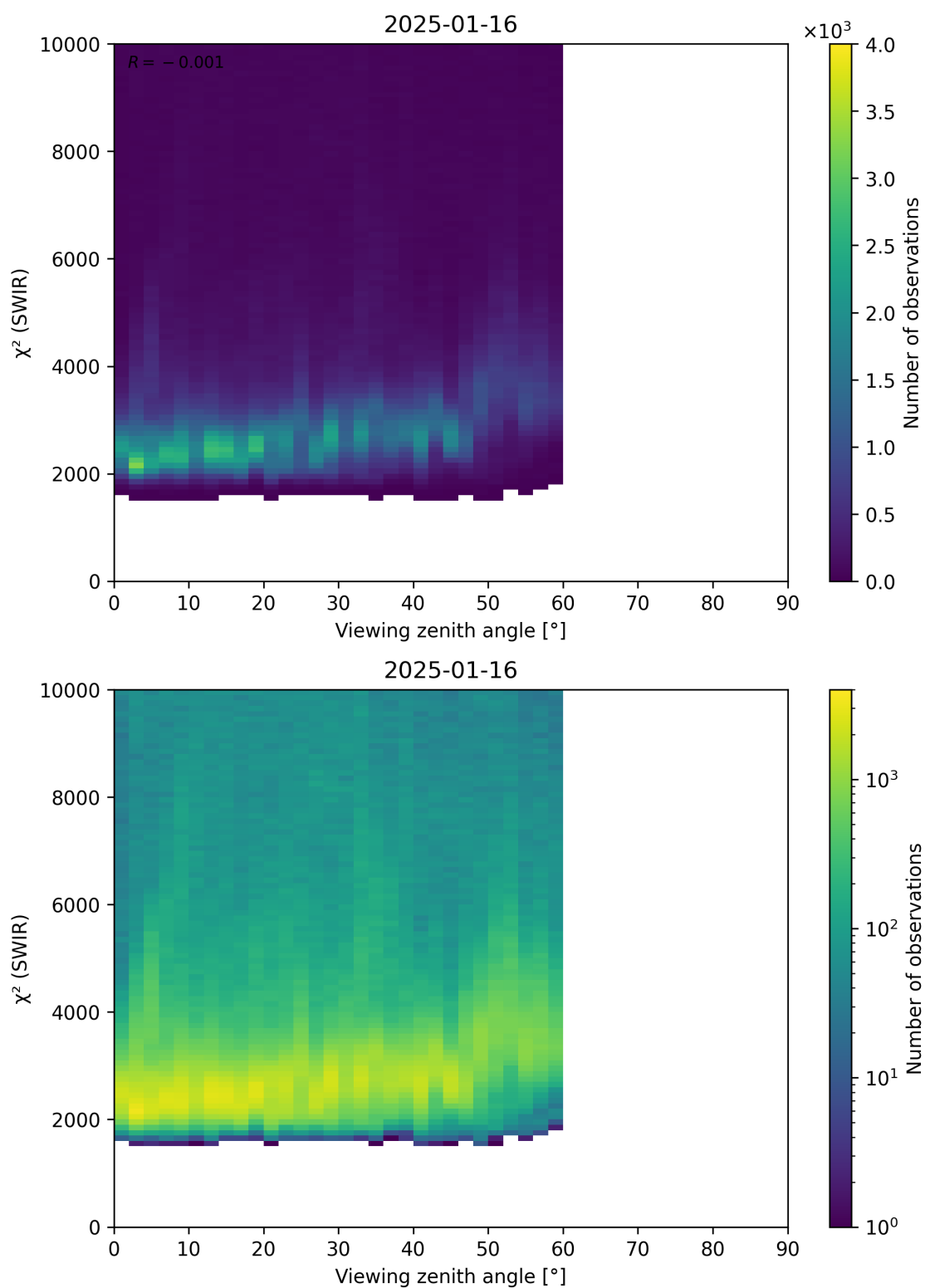
Figure 106: Scatter density plot of “Viewing zenith angle” against “ \chi^2 (SWIR)” for 2025-01-15 to 2025-01-17.
