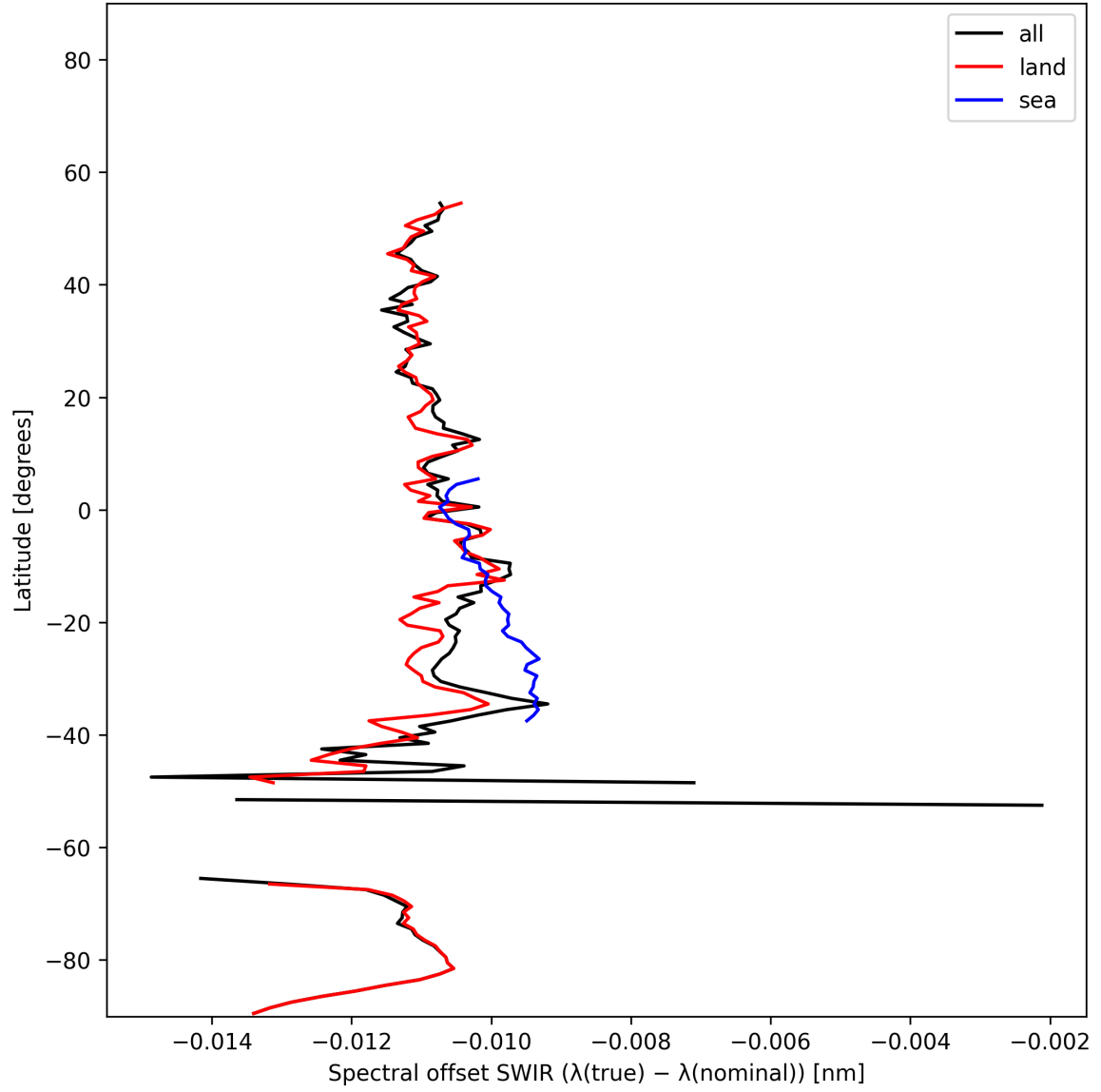
Figure 16: Zonal average of “Spectral offset SWIR ( \lambda_{\text{true}} - \lambda_{\text{nominal}} )” for 2025-01-15 to 2025-01-17.
