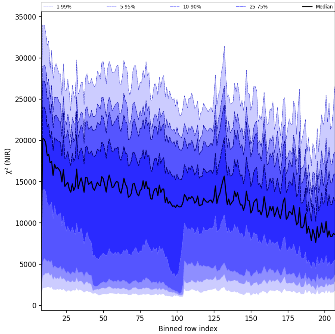
Figure 40: Along track statistics of “ \chi^2 (NIR)” for 2025-01-15 to 2025-01-17
