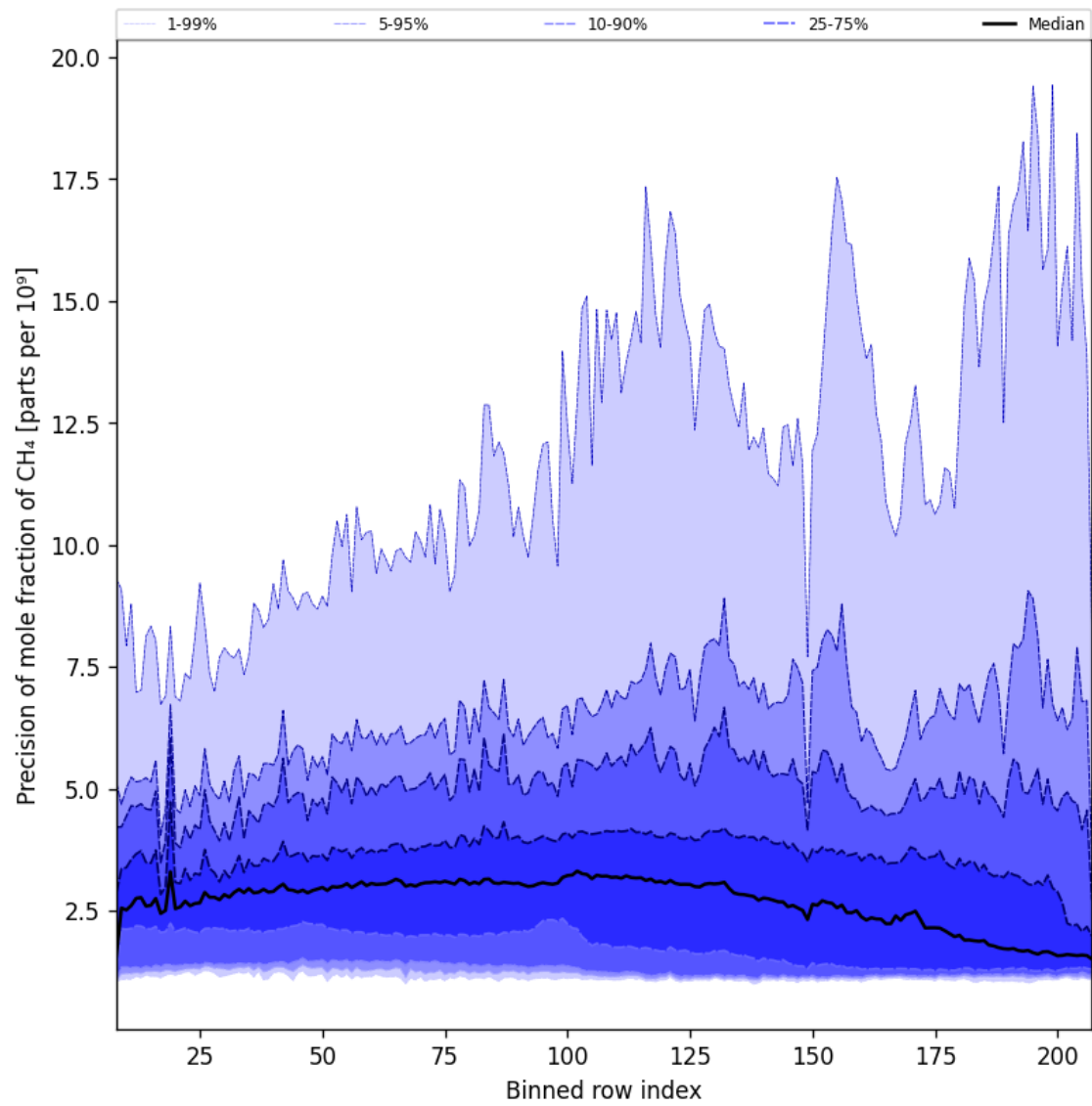
Figure 35: Along track statistics of “Precision of mole fraction of CH 4 ” for 2025-01-15 to 2025-01-17
