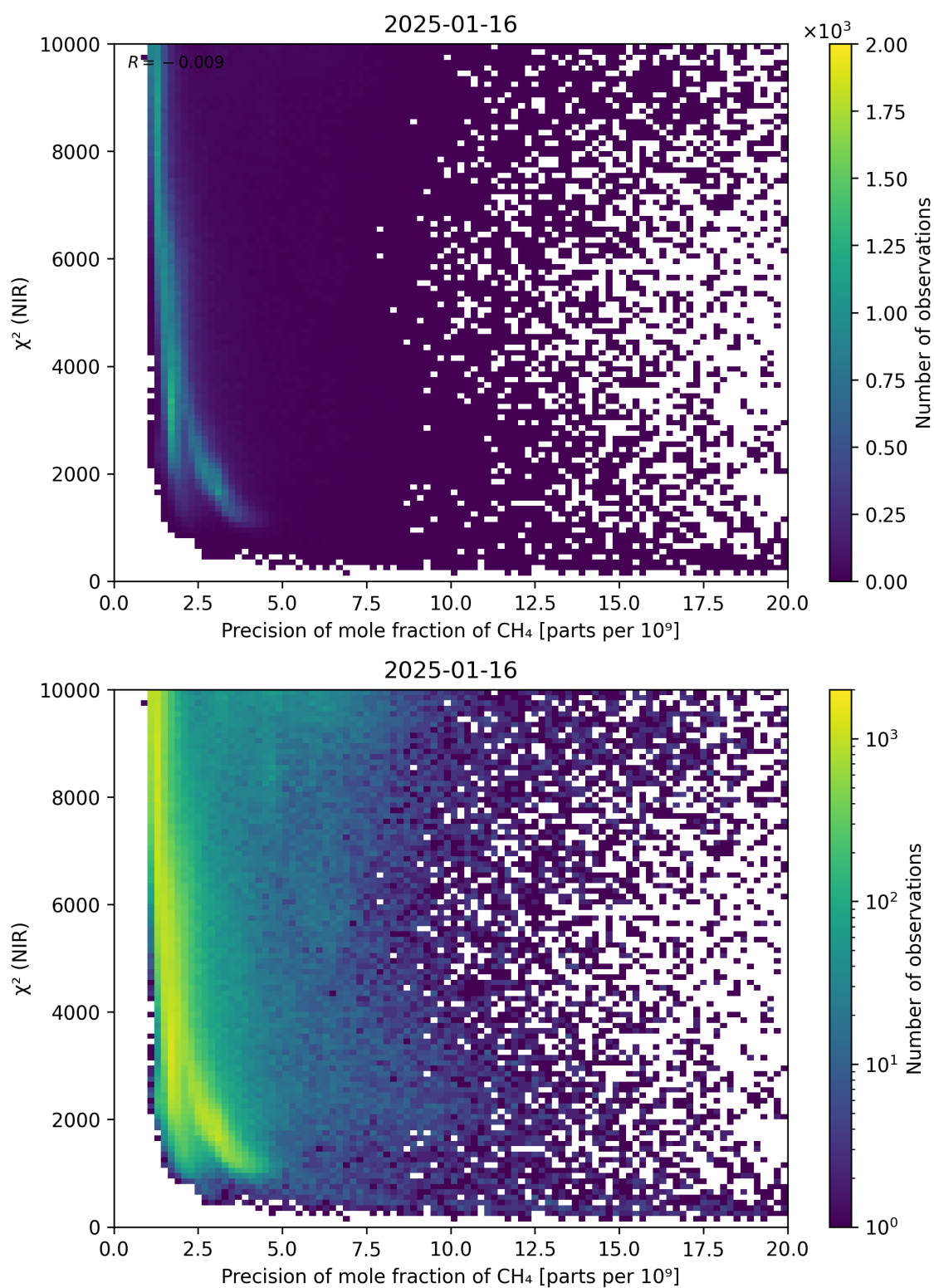
Figure 78: Scatter density plot of “Precision of mole fraction of CH 4 ” against “ \chi^2 (NIR)” for 2025-01-15 to 2025-01-17.
