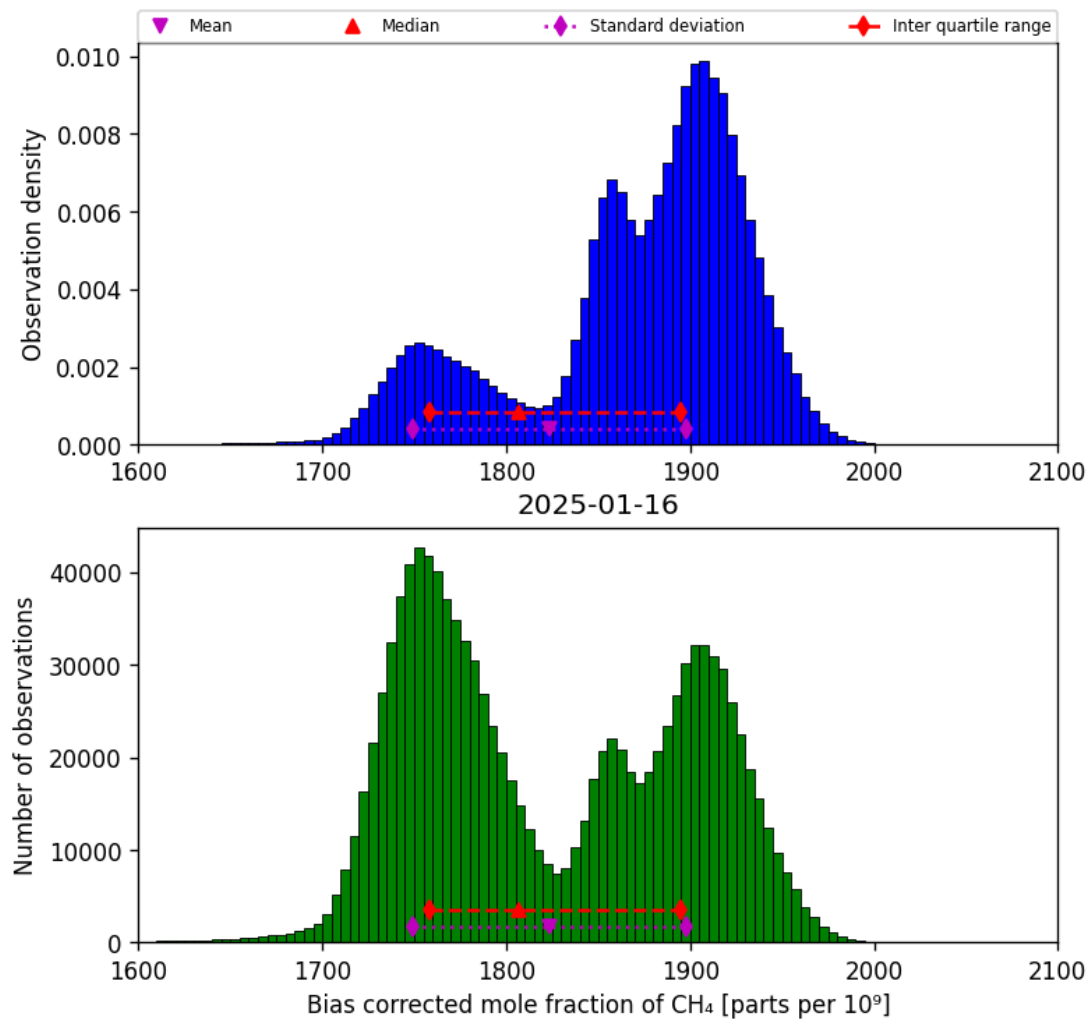
Figure 25: Histogram of “Bias corrected mole fraction of CH 4 ” for 2025-01-15 to 2025-01-17
