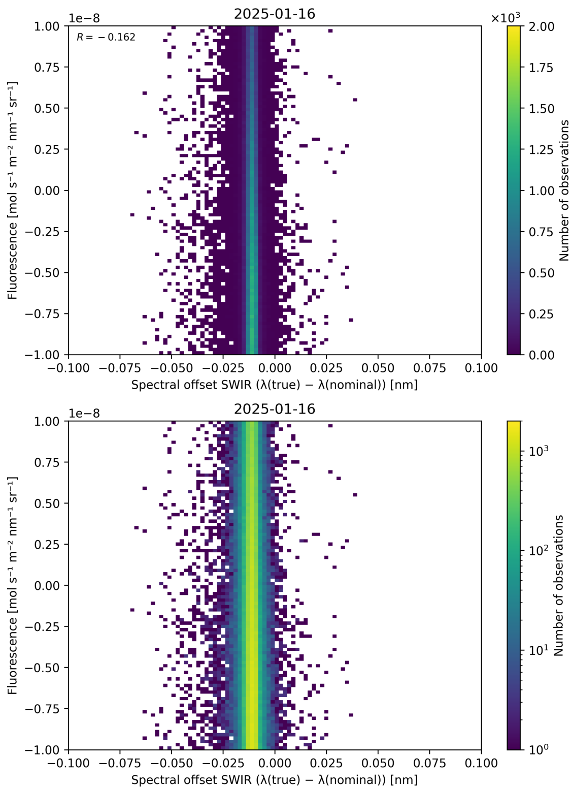
Figure 120: Scatter density plot of “Spectral offset SWIR ( \lambda_{\text{true}} - \lambda_{\text{nominal}} )” against “Fluorescence” for 2025-01-15 to 2025-01-17.
