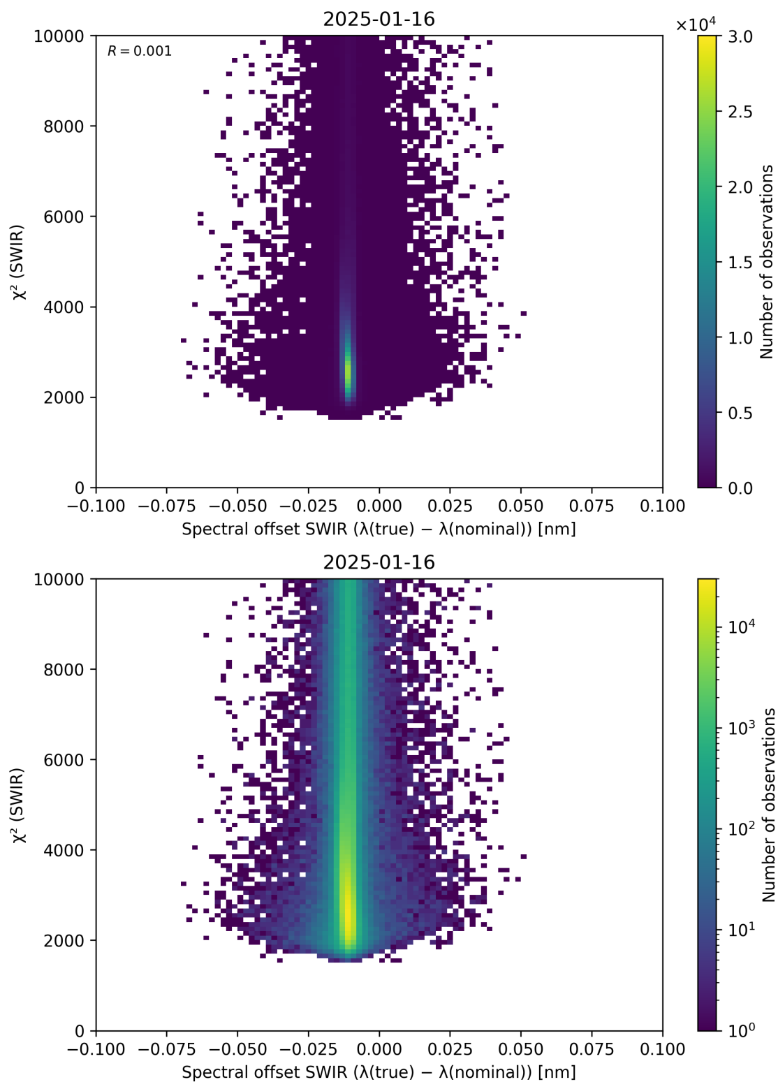
Figure 118: Scatter density plot of “Spectral offset SWIR ( \lambda_{\text{true}} - \lambda_{\text{nominal}} )” against “ \chi^2 (SWIR)” for 2025-01-15 to 2025-01-17.
