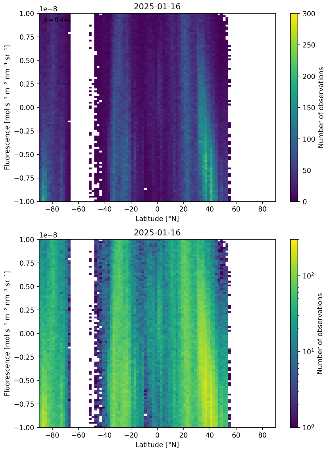
Figure 56: Scatter density plot of “Latitude” against “Fluorescence” for 2025-01-15 to 2025-01-17.
