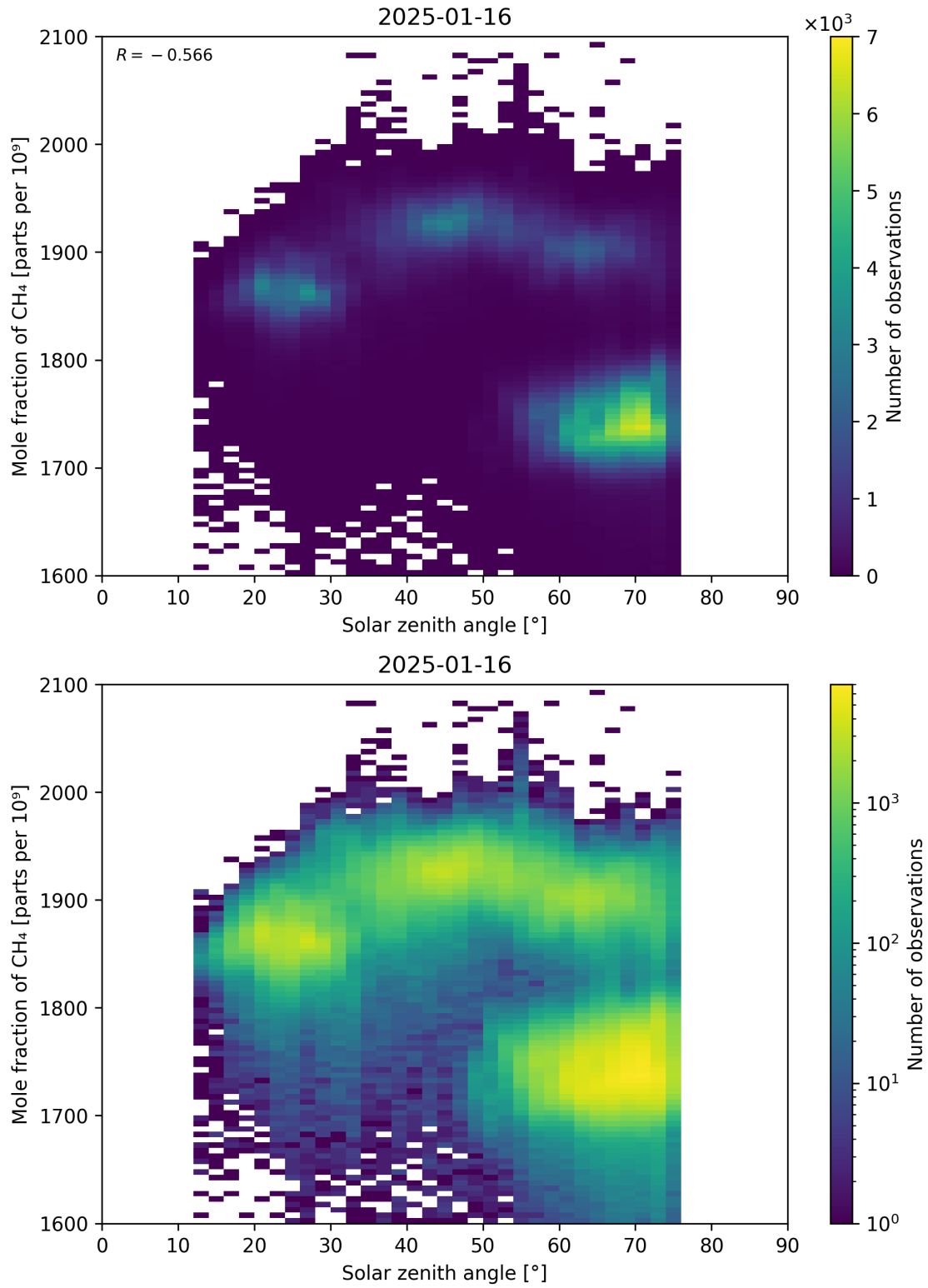
Figure 99: Scatter density plot of “Solar zenith angle” against “Mole fraction of CH 4 ” for 2025-01-15 to 2025-01-17.
