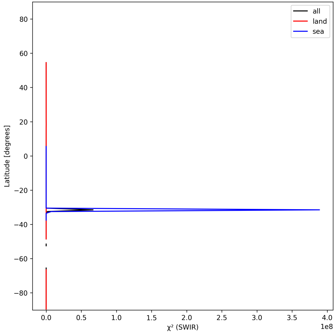
Figure 17: Zonal average of “ \chi^2 (SWIR)” for 2025-01-15 to 2025-01-17.
