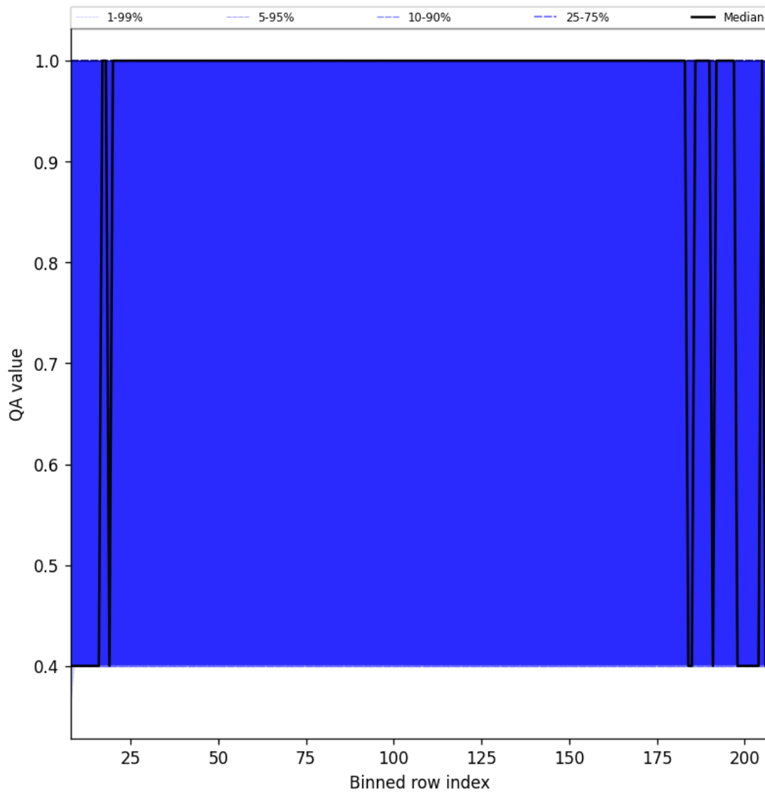
Figure 33: Along track statistics of “QA value” for 2025-01-15 to 2025-01-17
