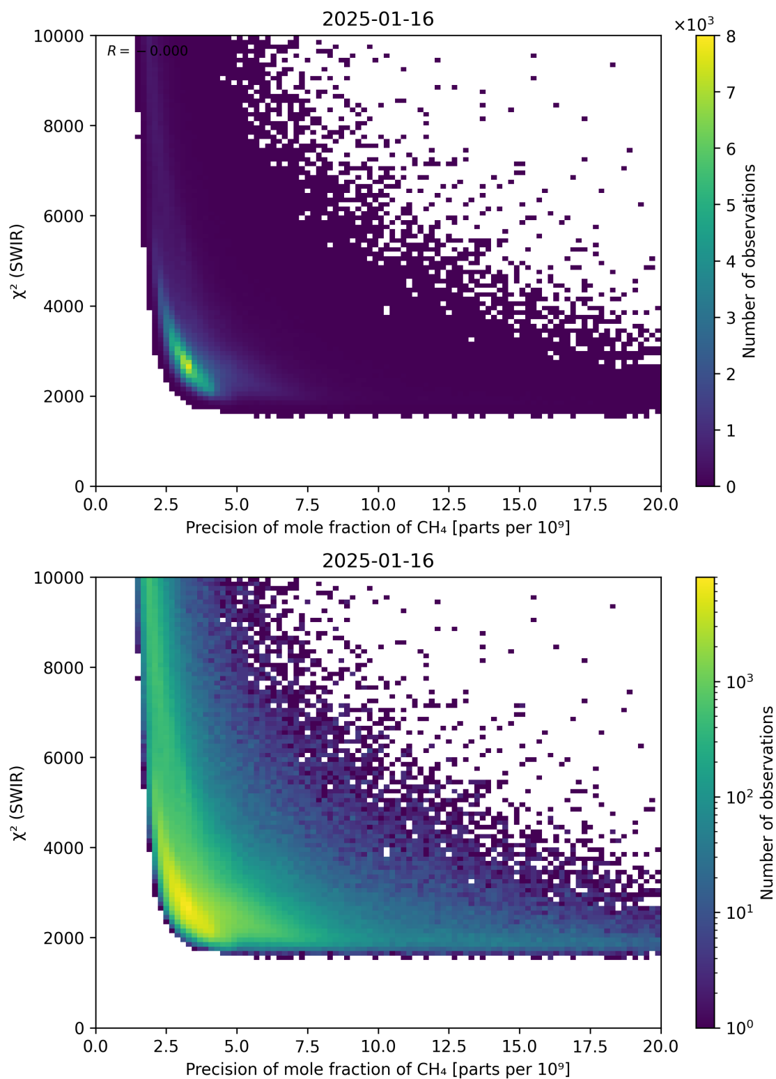
Figure 79: Scatter density plot of “Precision of mole fraction of CH 4 ” against “ \chi^2 (SWIR)” for 2025-01-15 to 2025-01-17.
