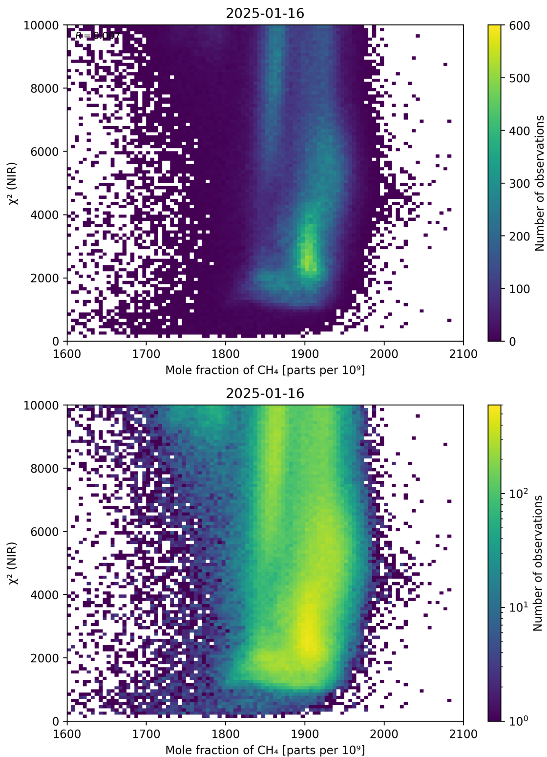
Figure 70: Scatter density plot of “Mole fraction of CH 4 ” against “ \chi^2 (NIR)” for 2025-01-15 to 2025-01-17.
