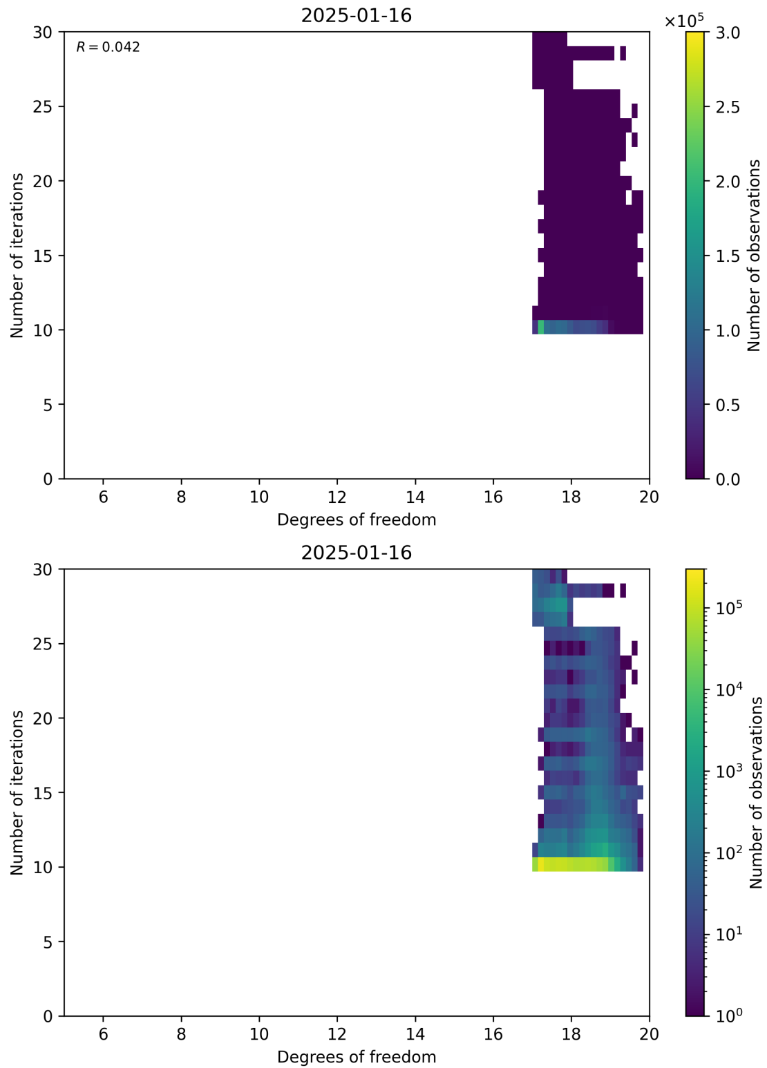
Figure 52: Scatter density plot of “Degrees of freedom” against “Number of iterations” for 2025-01-15 to 2025-01-17.
