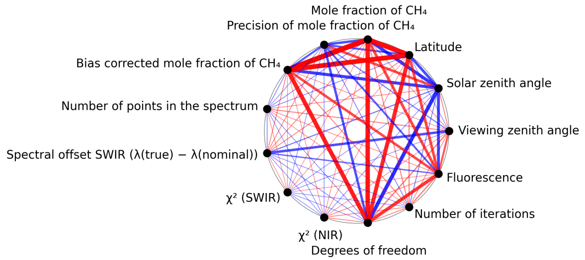
Figure 1: Map of correlation graph for 2025-01-15 to 2025-01-17.
