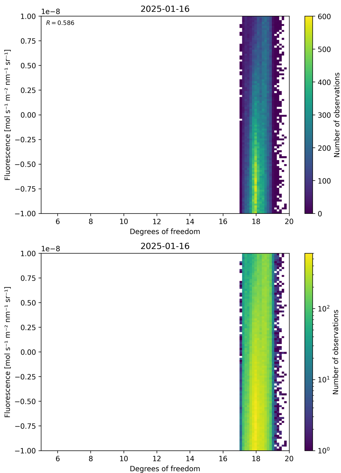
Figure 51: Scatter density plot of “Degrees of freedom” against “Fluorescence” for 2025-01-15 to 2025-01-17.
