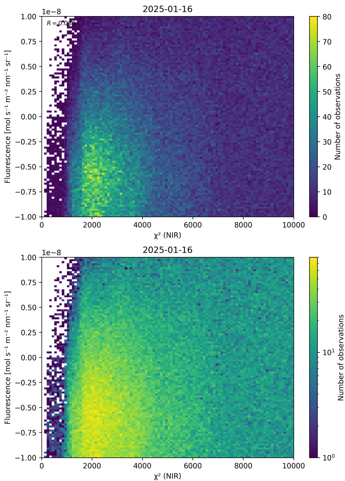
Figure 45: Scatter density plot of “ \chi^2 (NIR)” against “Fluorescence” for 2025-01-15 to 2025-01-17.
