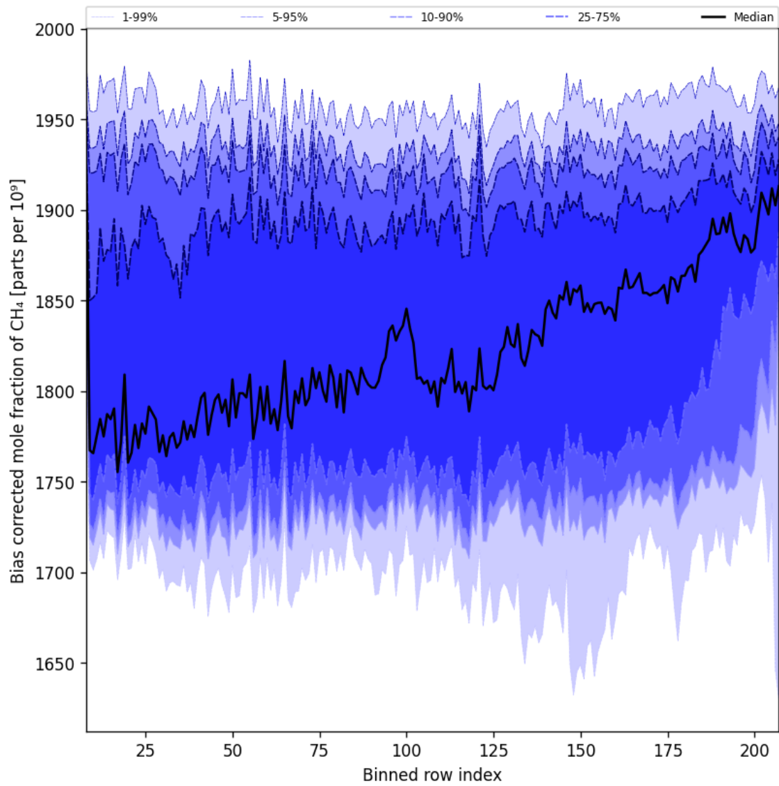
Figure 36: Along track statistics of “Bias corrected mole fraction of CH 4 ” for 2025-01-15 to 2025-01-17
