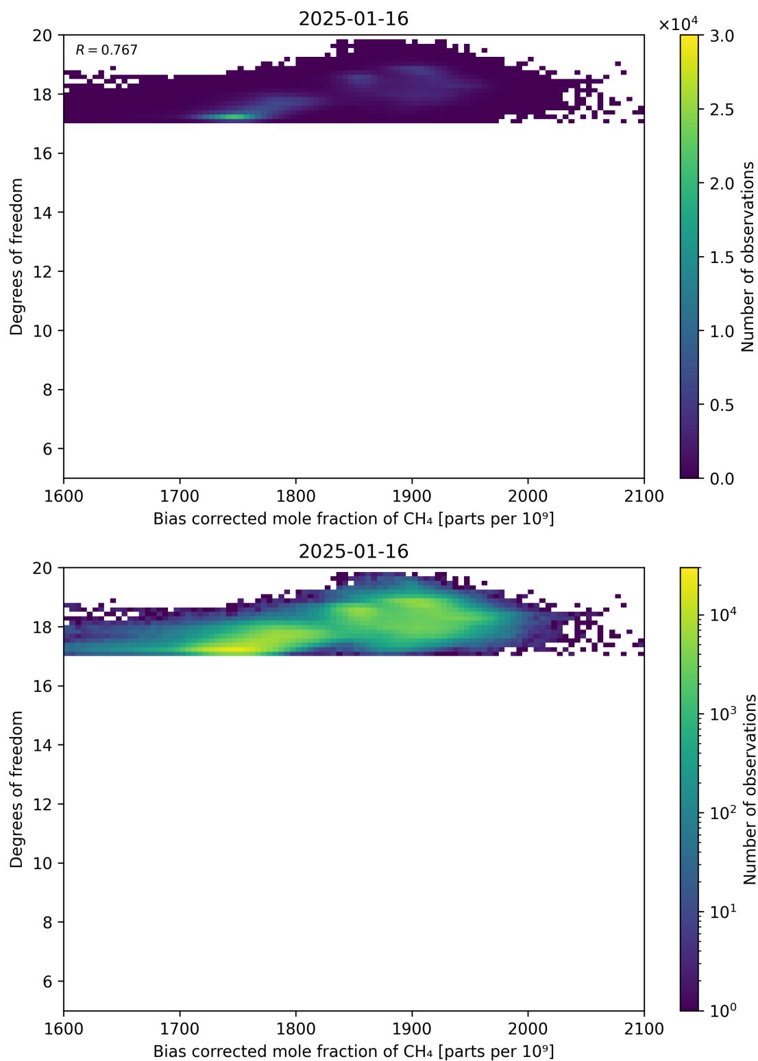
Figure 65: Scatter density plot of “Bias corrected mole fraction of CH 4 ” against “Degrees of freedom” for 2025-01-15 to 2025-01-17.
