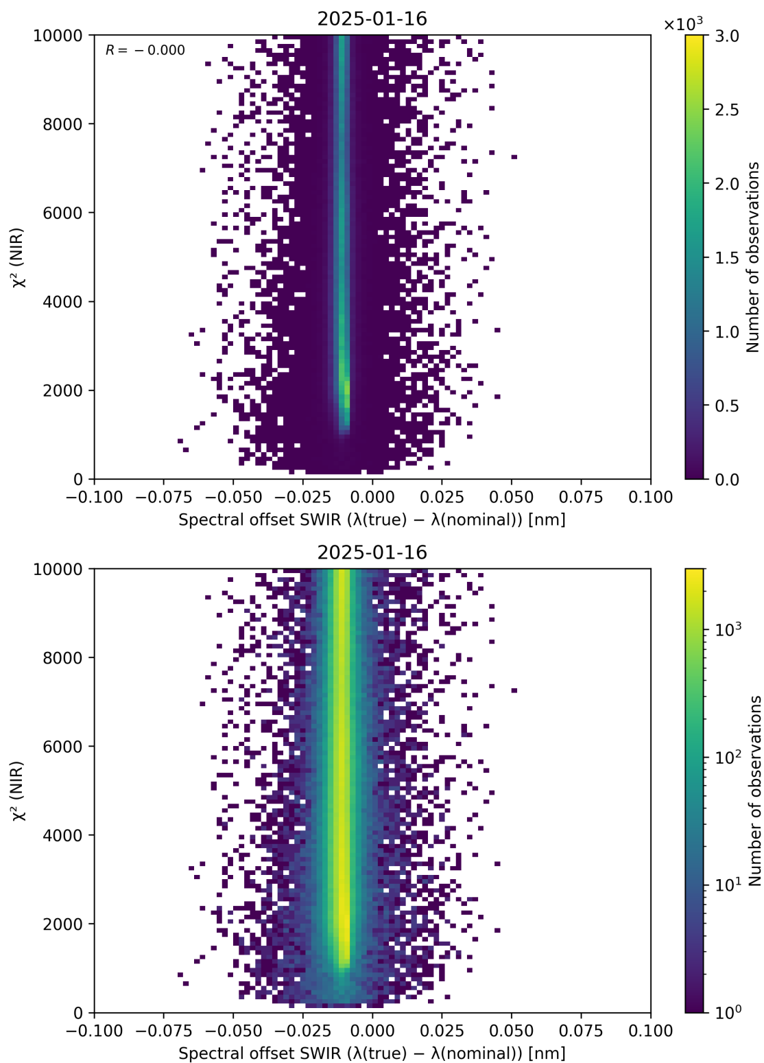
Figure 117: Scatter density plot of “Spectral offset SWIR ( \lambda_{\text{true}} - \lambda_{\text{nominal}} )” against “ \chi^2 (NIR)” for 2025-01-15 to 2025-01-17.
