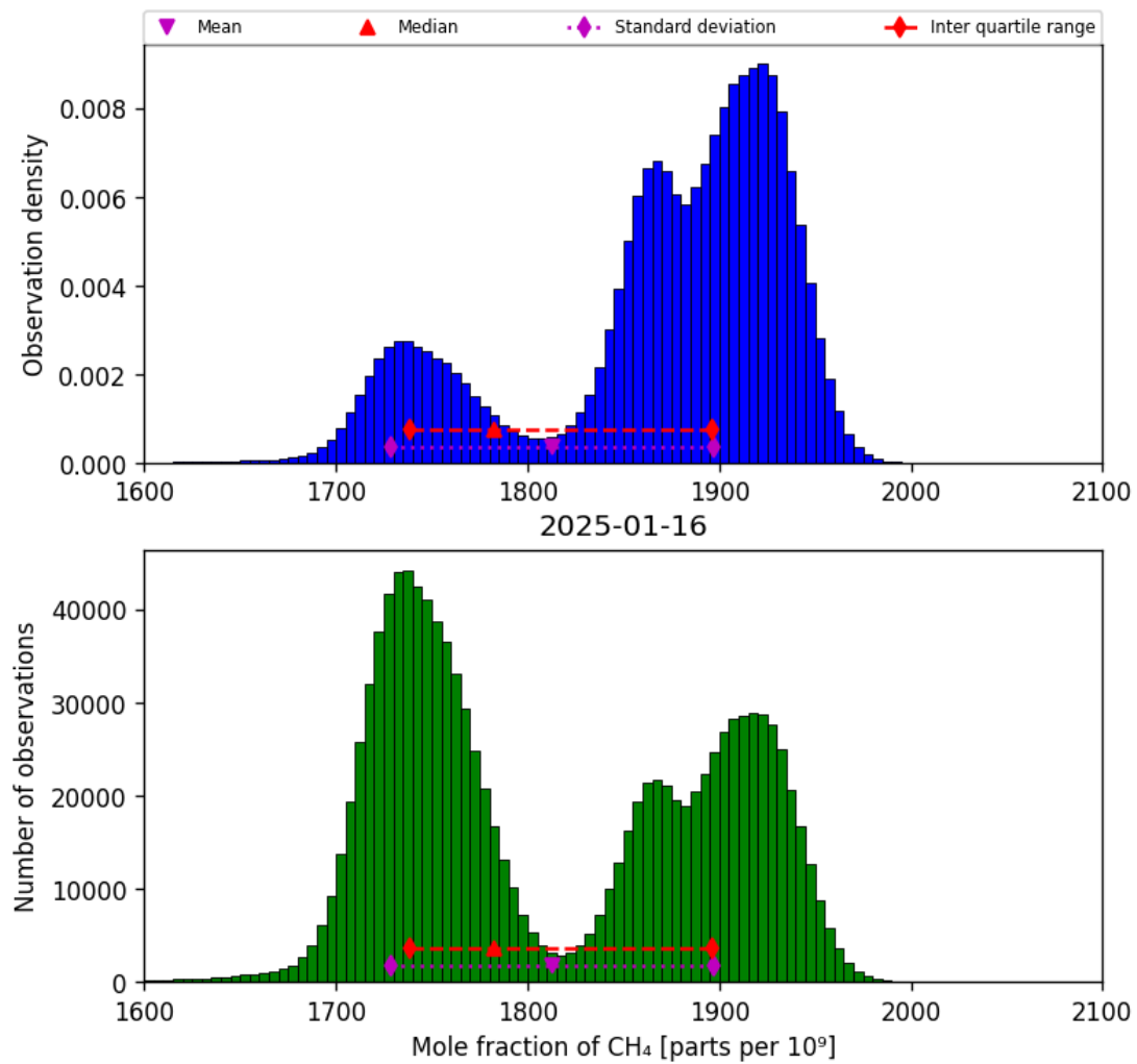
Figure 23: Histogram of “Mole fraction of CH 4 ” for 2025-01-15 to 2025-01-17
