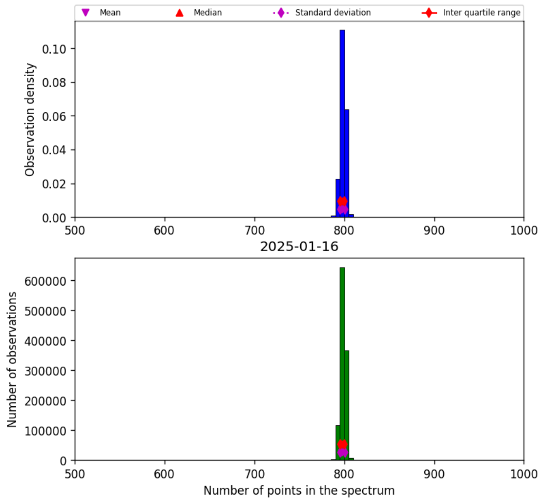
Figure 26: Histogram of “Number of points in the spectrum” for 2025-01-15 to 2025-01-17
