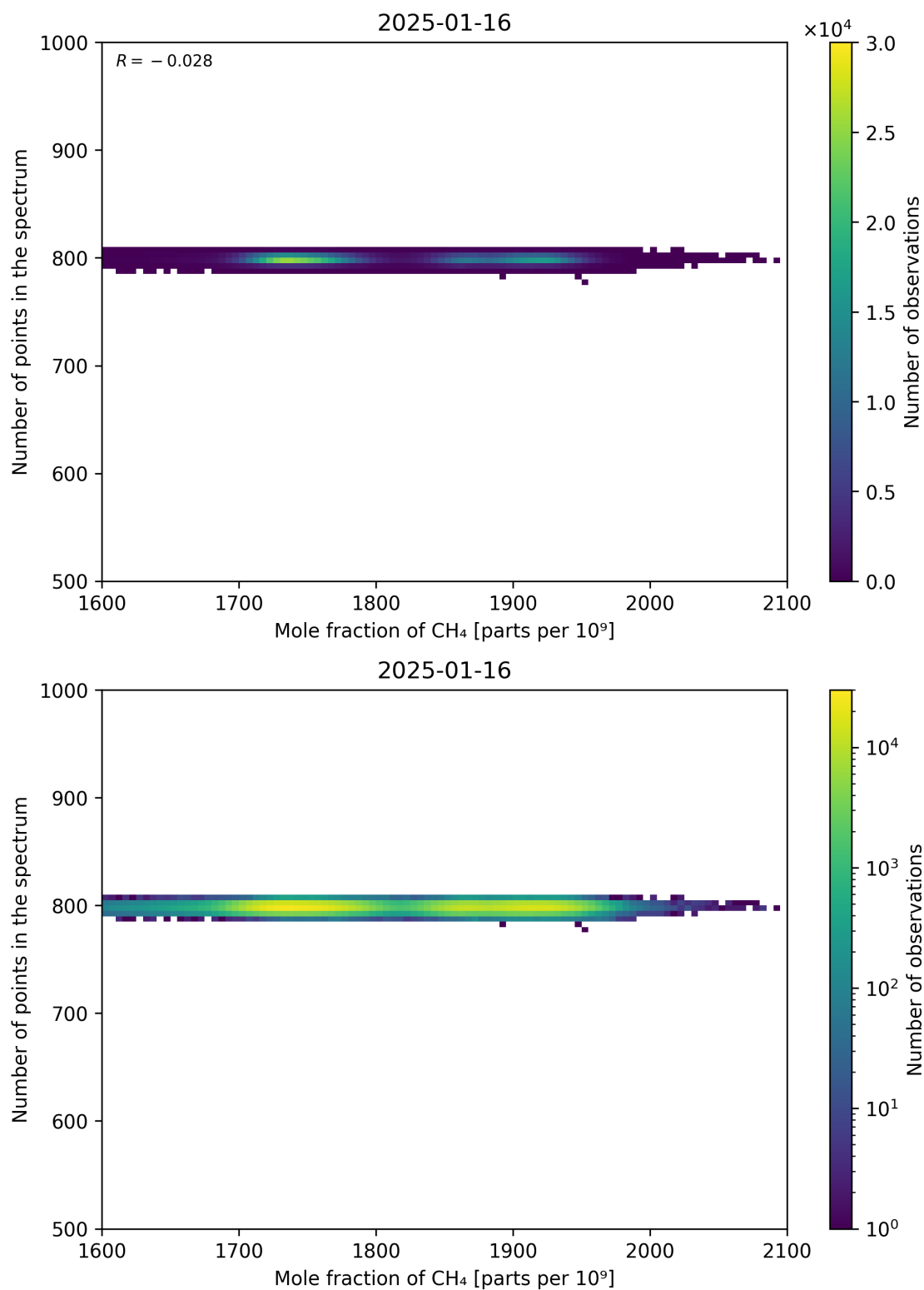
Figure 77: Scatter density plot of “Mole fraction of CH 4 ” against “Number of points in the spectrum” for 2025-01-15 to 2025-01-17.
