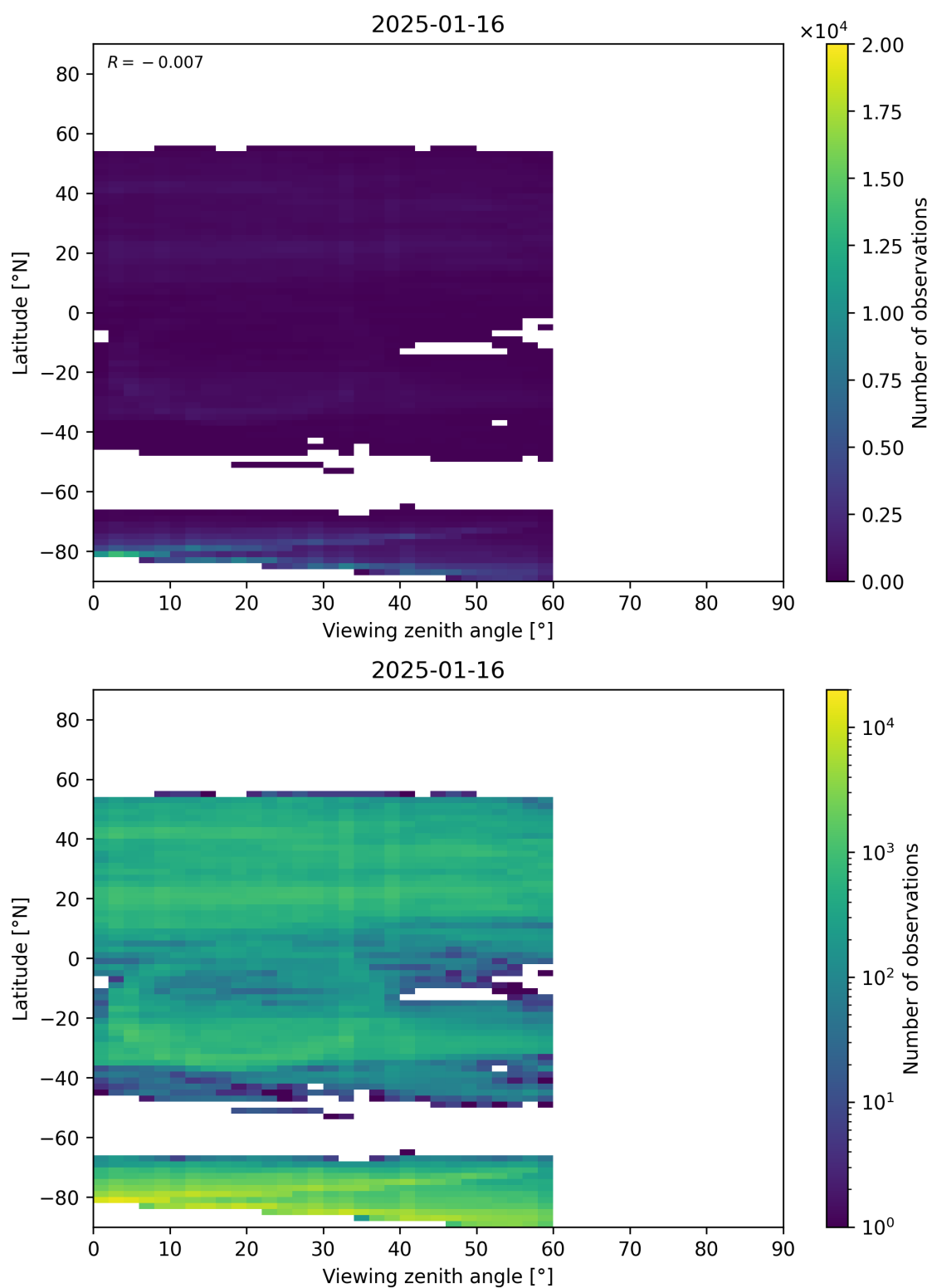
Figure 109: Scatter density plot of “Viewing zenith angle” against “Latitude” for 2025-01-15 to 2025-01-17.
