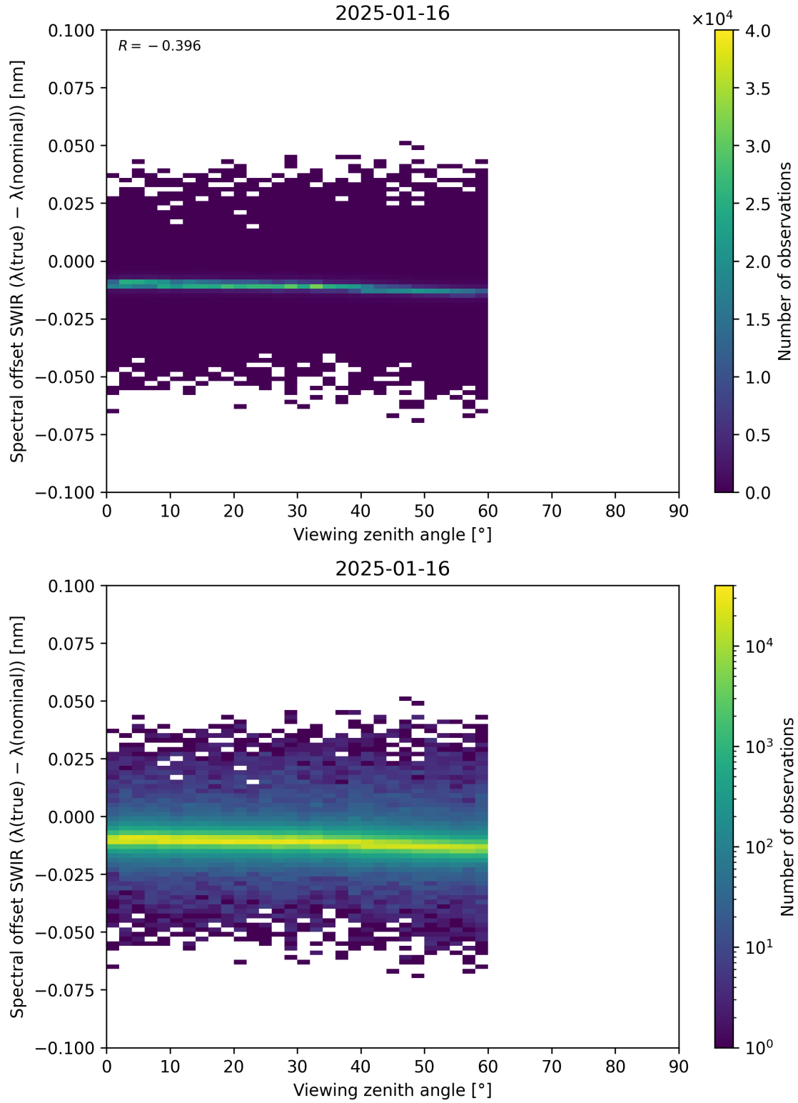
Figure 116: Scatter density plot of “Viewing zenith angle” against “Spectral offset SWIR ( \lambda_{\text{true}} - \lambda_{\text{nominal}} )” for 2025-01-15 to 2025-01-17.
