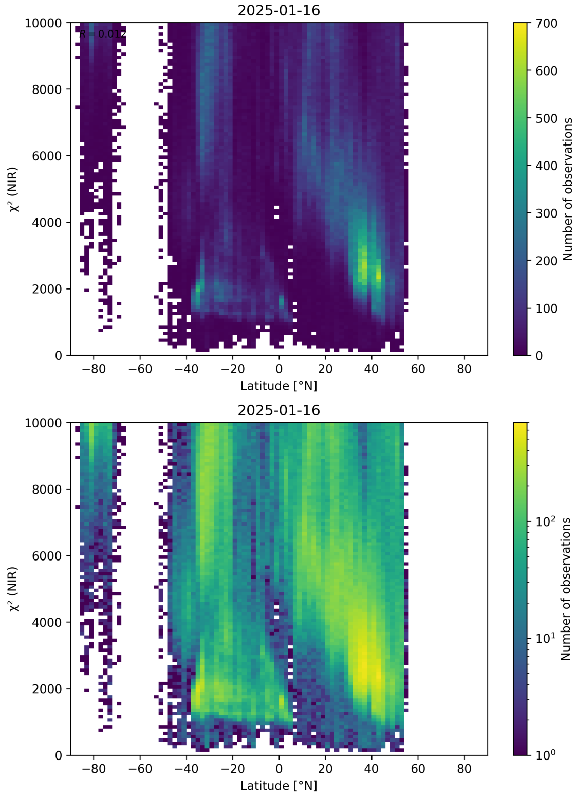
Figure 53: Scatter density plot of “Latitude” against “ \chi^2 (NIR)” for 2025-01-15 to 2025-01-17.
