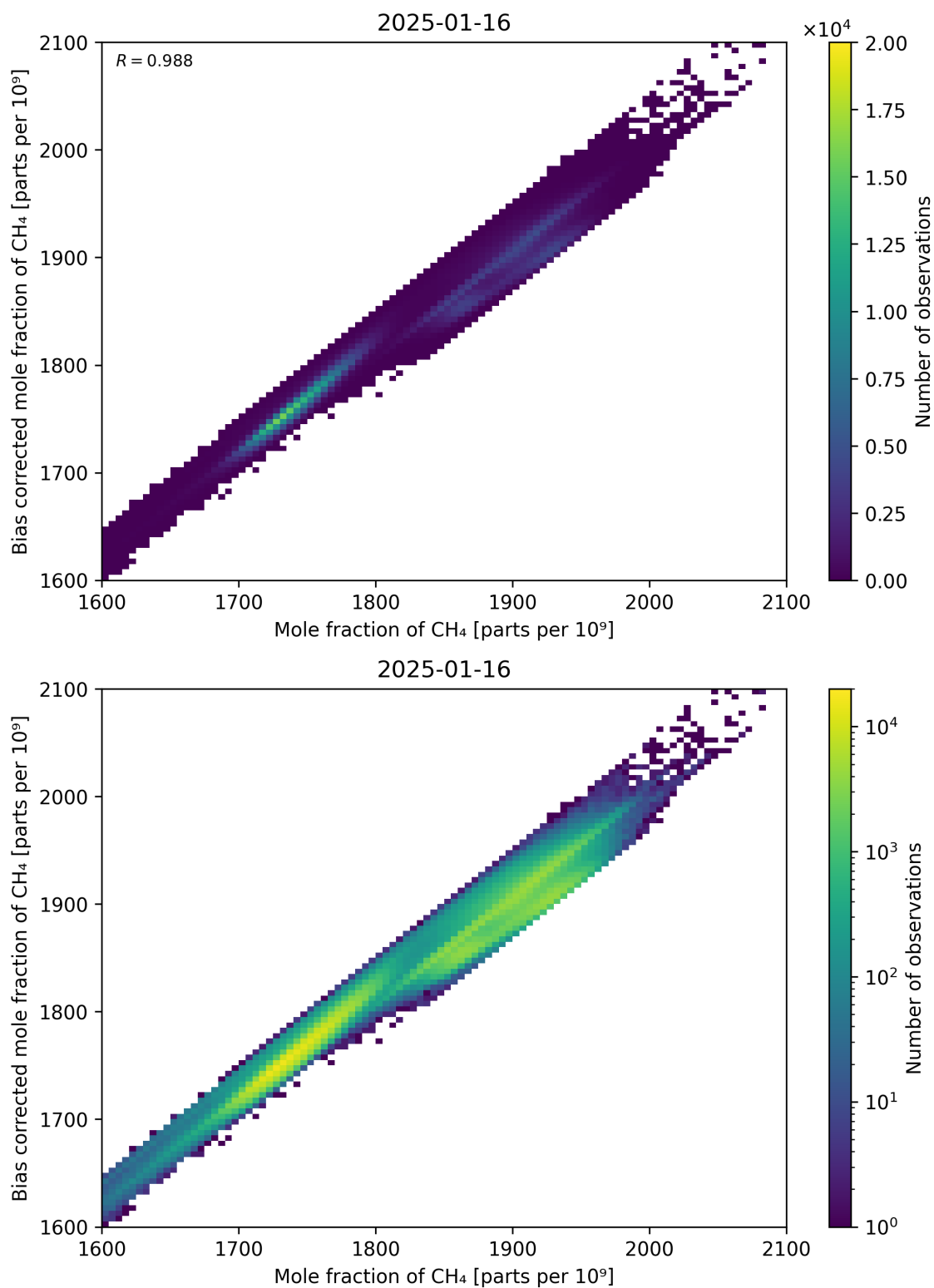
Figure 74: Scatter density plot of “Mole fraction of CH 4 ” against “Bias corrected mole fraction of CH 4 ” for 2025-01-15 to 2025-01-17.
