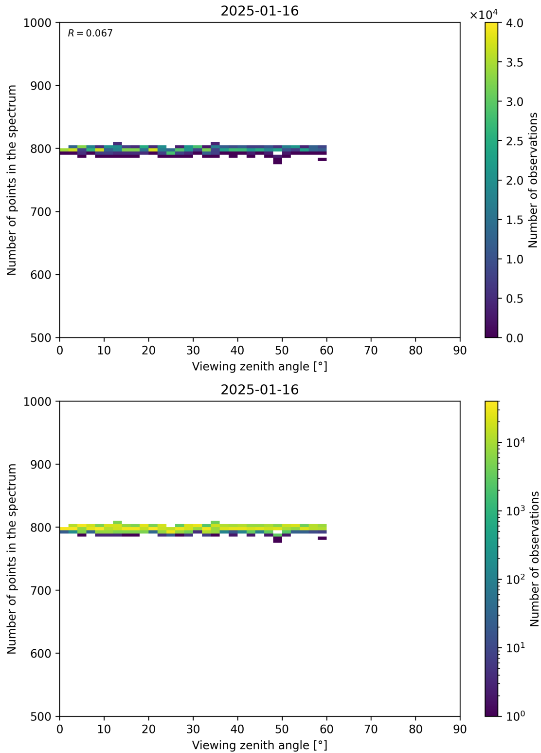
Figure 114: Scatter density plot of “Viewing zenith angle” against “Number of points in the spectrum” for 2025-01-15 to 2025-01-17.
