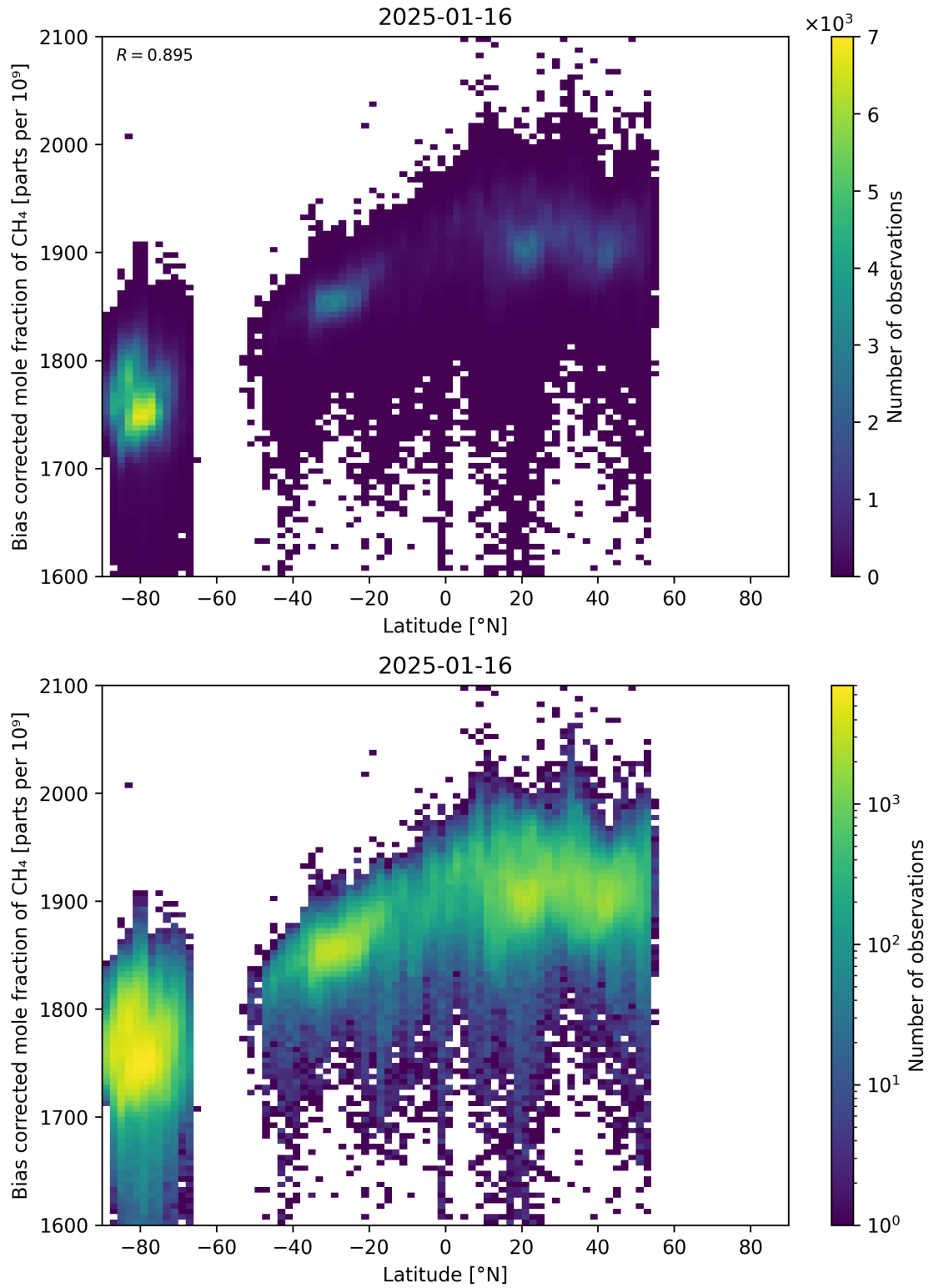
Figure 58: Scatter density plot of “Latitude” against “Bias corrected mole fraction of CH 4 ” for 2025-01-15 to 2025-01-17.
