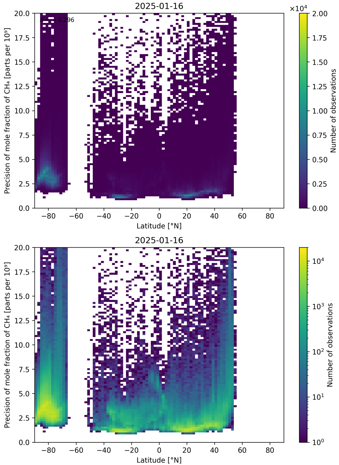
Figure 59: Scatter density plot of “Latitude” against “Precision of mole fraction of CH 4 ” for 2025-01-15 to 2025-01-17.
