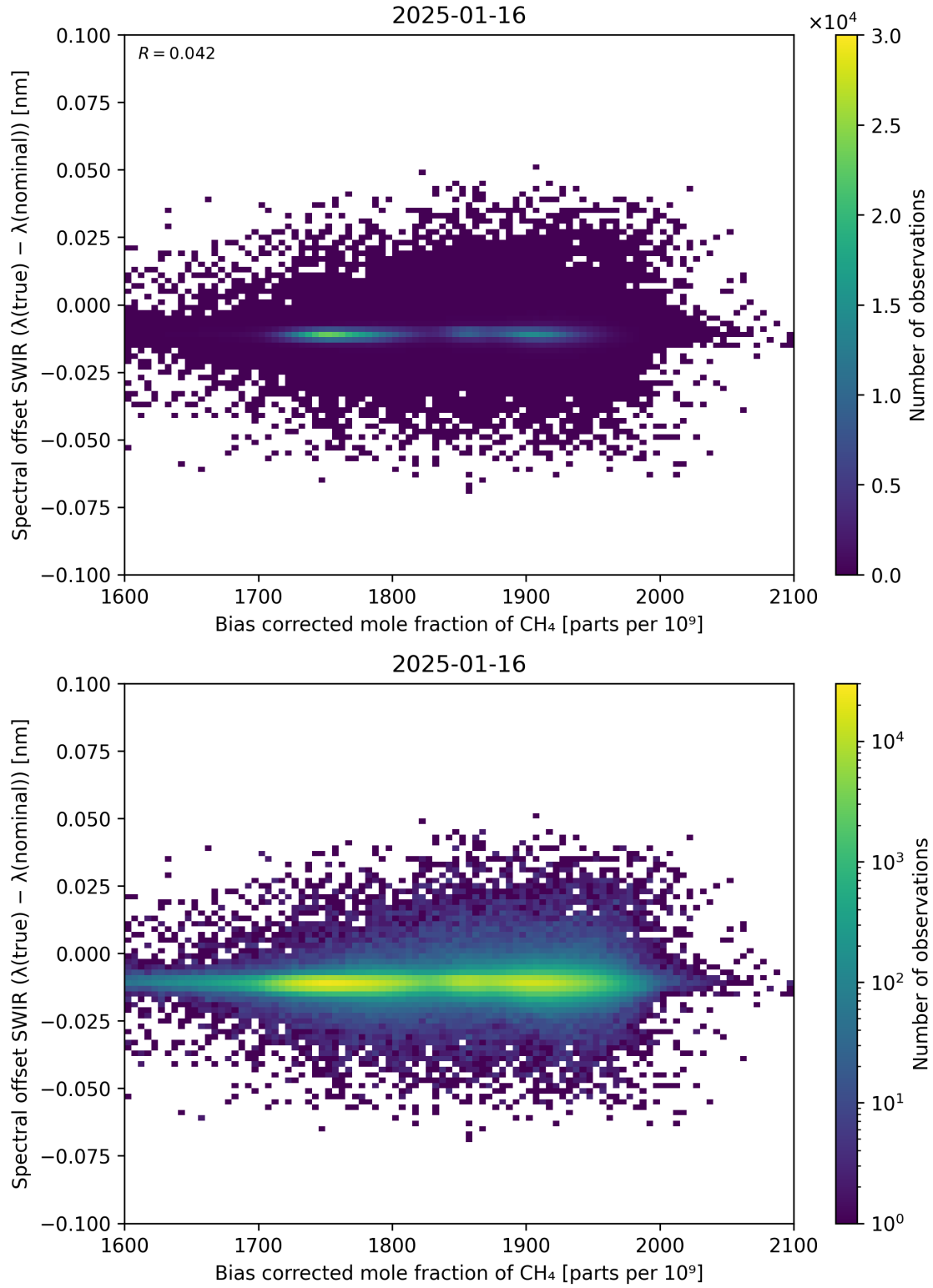
Figure 69: Scatter density plot of “Bias corrected mole fraction of \text{CH}_4 ” against “Spectral offset SWIR ( \lambda_{\text{true}} - \lambda_{\text{nominal}} )” for 2025-01-15 to 2025-01-17.
