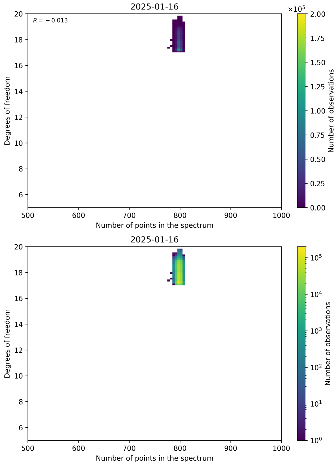
Figure 90: Scatter density plot of “Number of points in the spectrum” against “Degrees of freedom” for 2025-01-15 to 2025-01-17.
