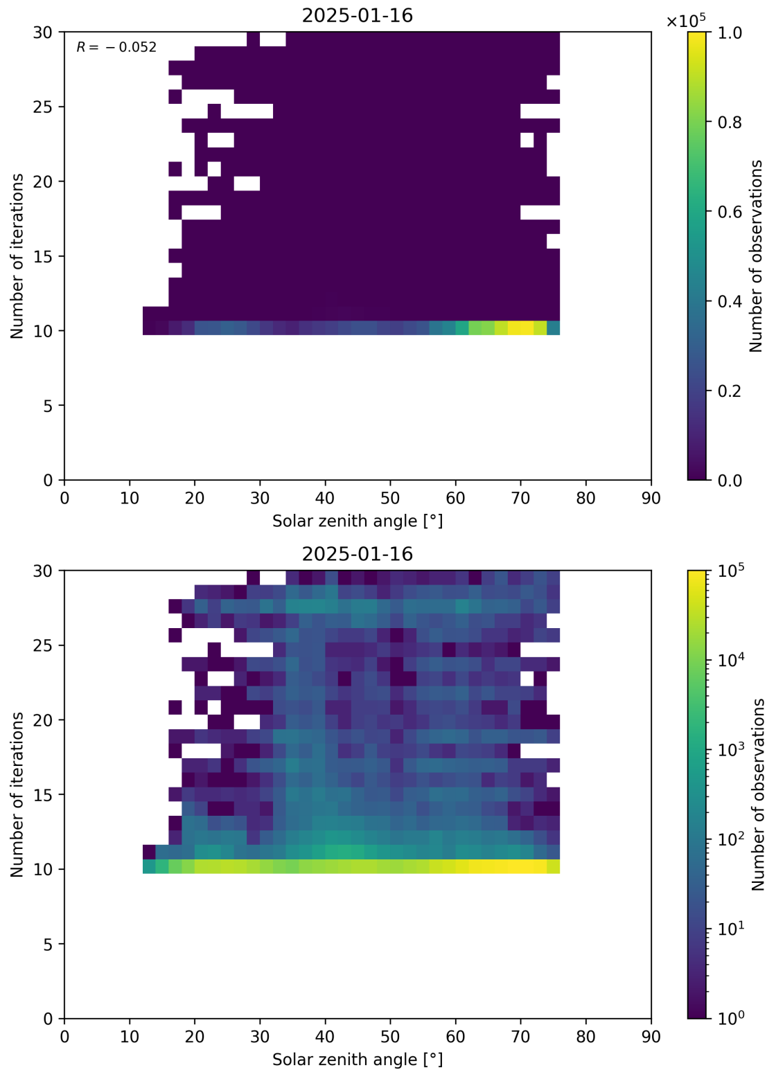
Figure 102: Scatter density plot of “Solar zenith angle” against “Number of iterations” for 2025-01-15 to 2025-01-17.
