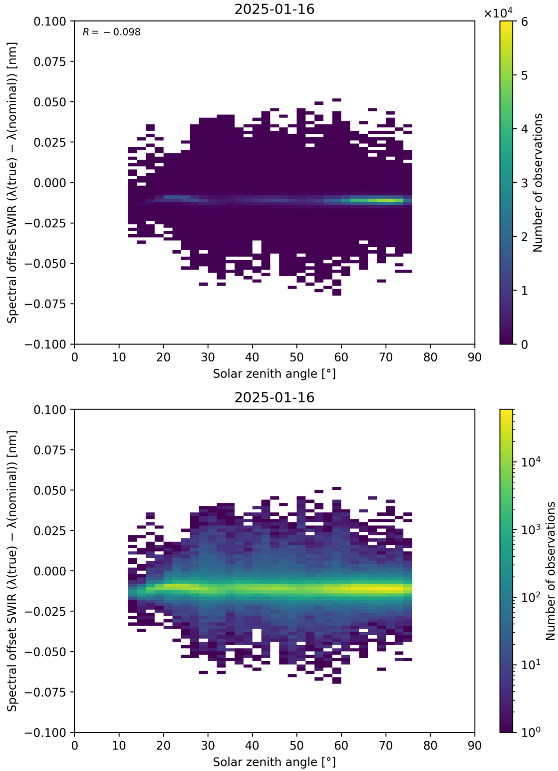
Figure 104: Scatter density plot of “Solar zenith angle” against “Spectral offset SWIR ( \lambda_{\text{true}} - \lambda_{\text{nominal}} )” for 2025-01-15 to 2025-01-17.
