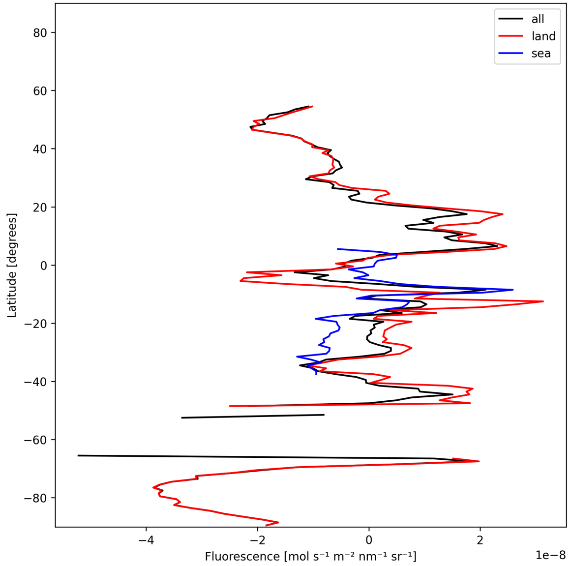
Figure 21: Zonal average of “Fluorescence” for 2025-01-15 to 2025-01-17.
