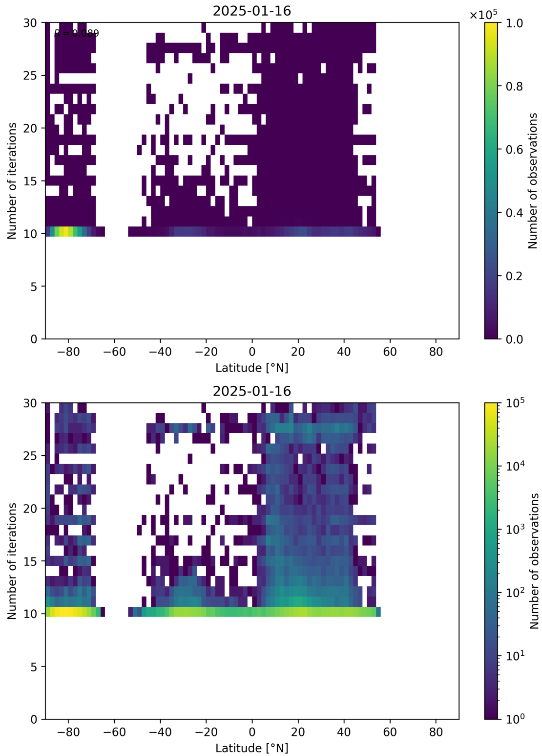
Figure 60: Scatter density plot of “Latitude” against “Number of iterations” for 2025-01-15 to 2025-01-17.
