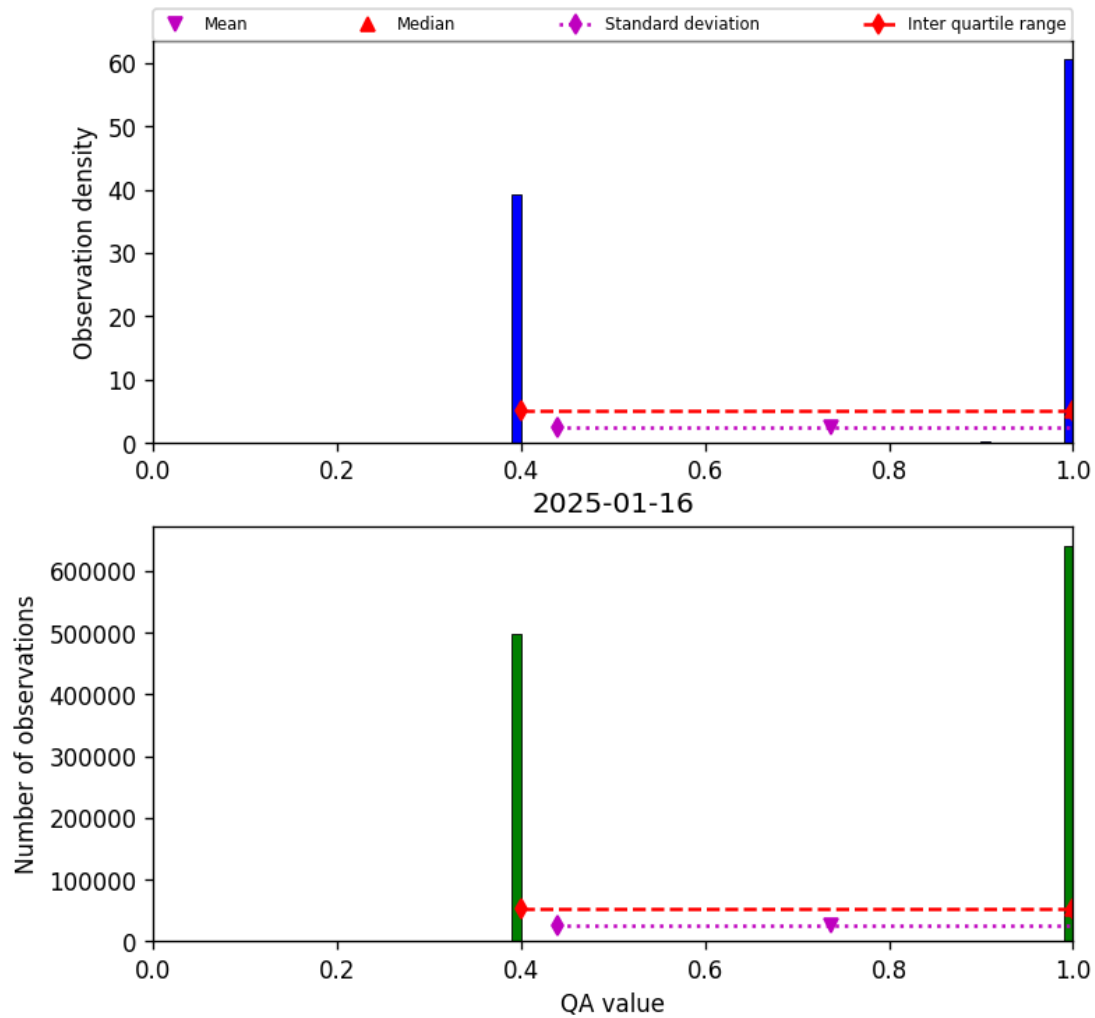
Figure 22: Histogram of “QA value” for 2025-01-15 to 2025-01-17
