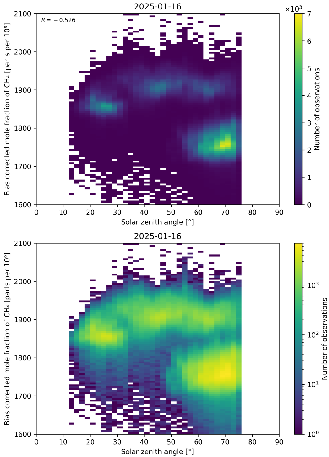
Figure 100: Scatter density plot of “Solar zenith angle” against “Bias corrected mole fraction of CH 4 ” for 2025-01-15 to 2025-01-17.
