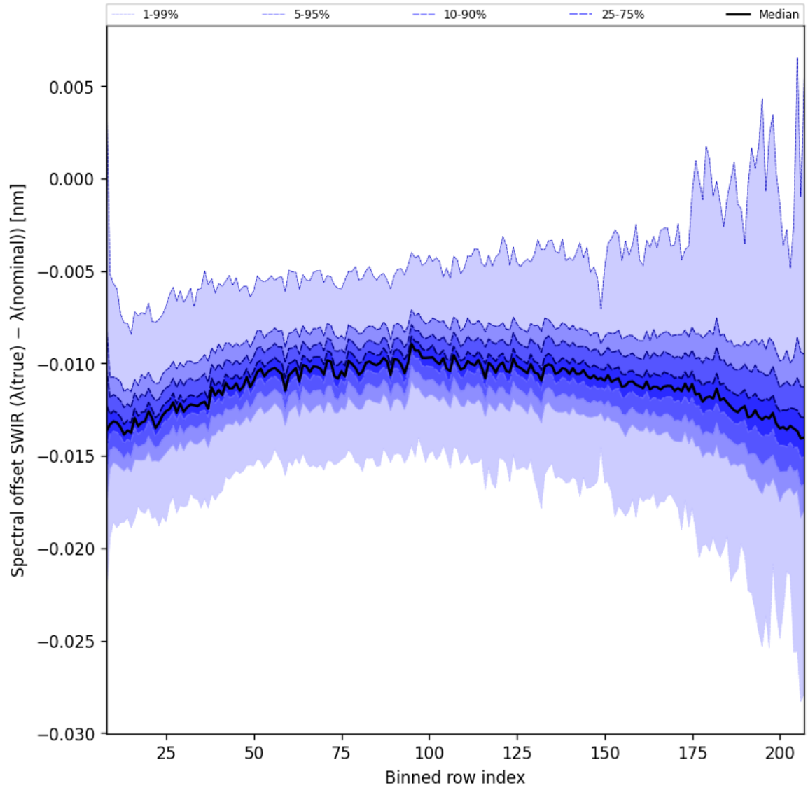
Figure 38: Along track statistics of “Spectral offset SWIR ( \lambda_{\text{true}} - \lambda_{\text{nominal}} )” for 2025-01-15 to 2025-01-17
