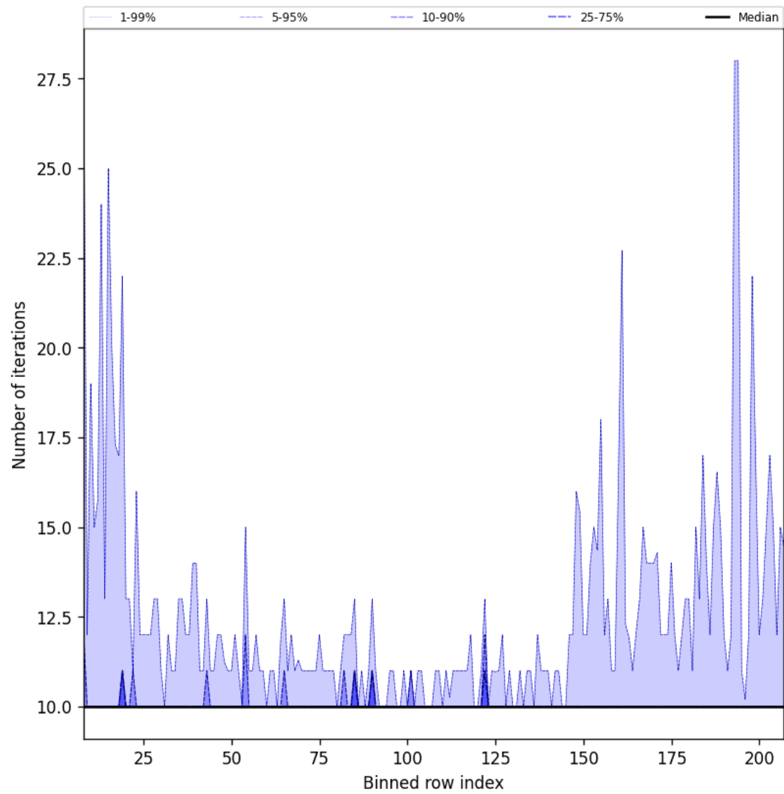
Figure 42: Along track statistics of “Number of iterations” for 2025-01-15 to 2025-01-17
