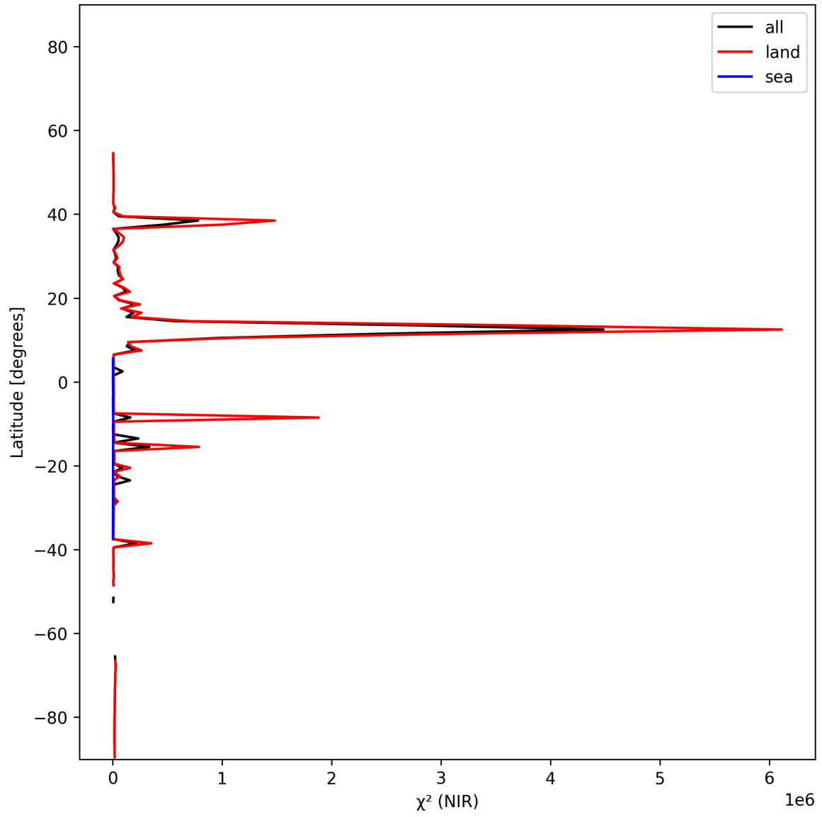
Figure 18: Zonal average of “ \chi^2 (NIR)” for 2025-01-15 to 2025-01-17.
