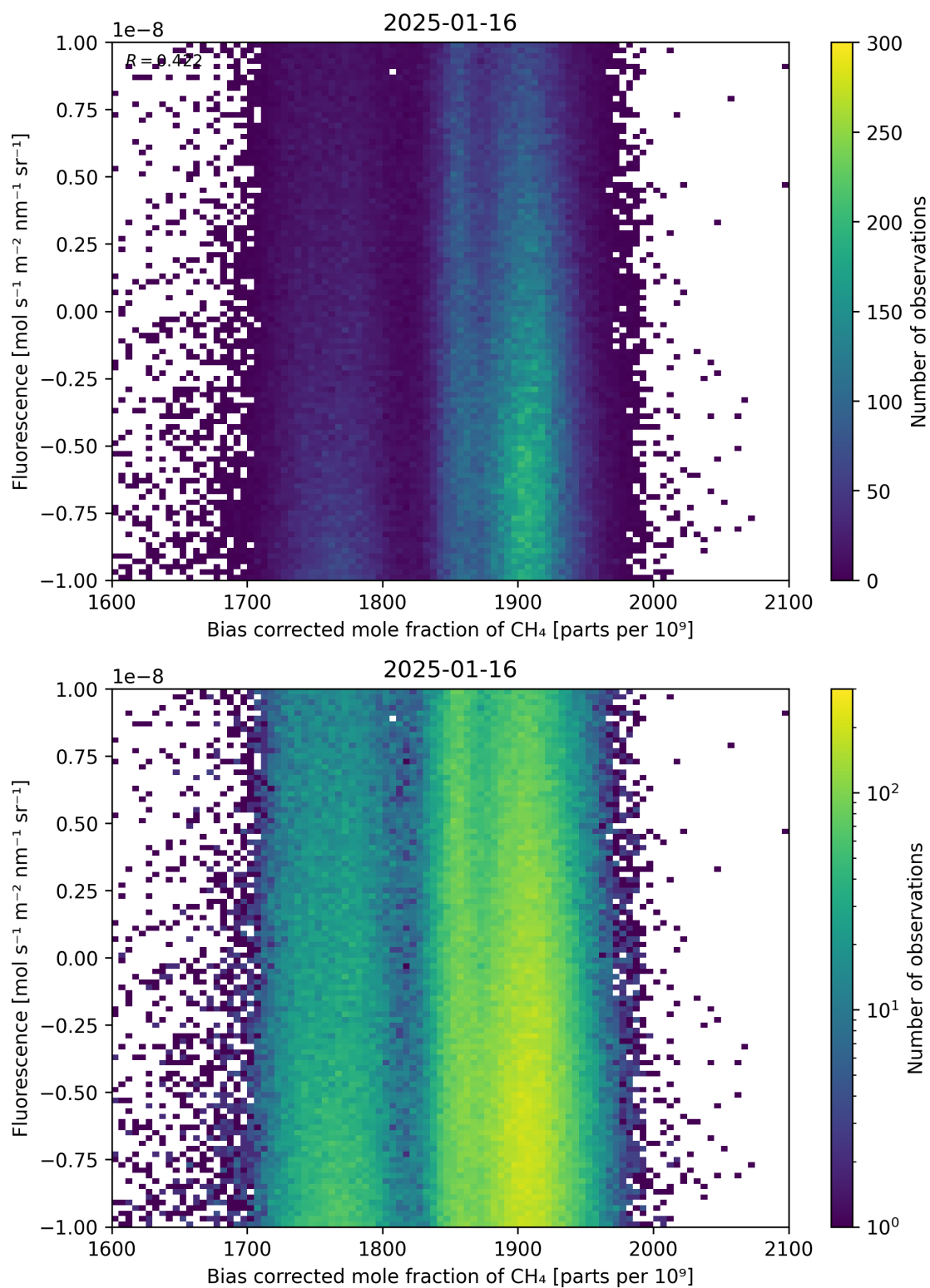
Figure 66: Scatter density plot of “Bias corrected mole fraction of \text{CH}_4 ” against “Fluorescence” for 2025-01-15 to 2025-01-17.
