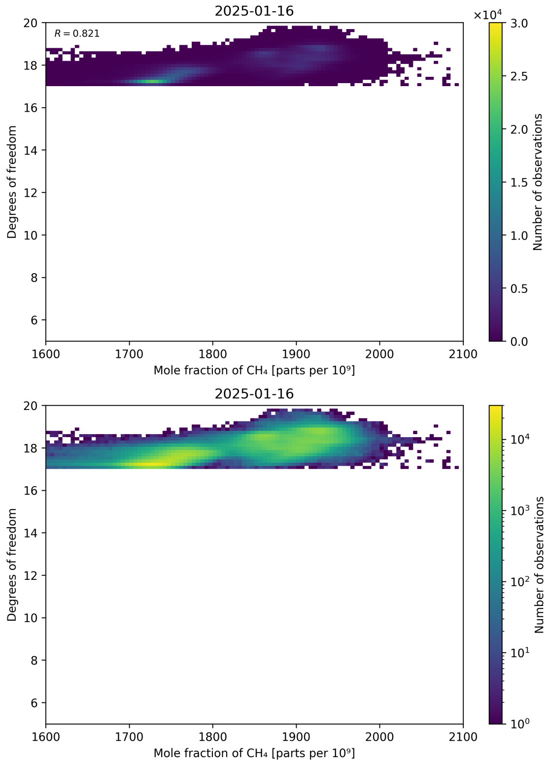
Figure 72: Scatter density plot of “Mole fraction of CH 4 ” against “Degrees of freedom” for 2025-01-15 to 2025-01-17.
