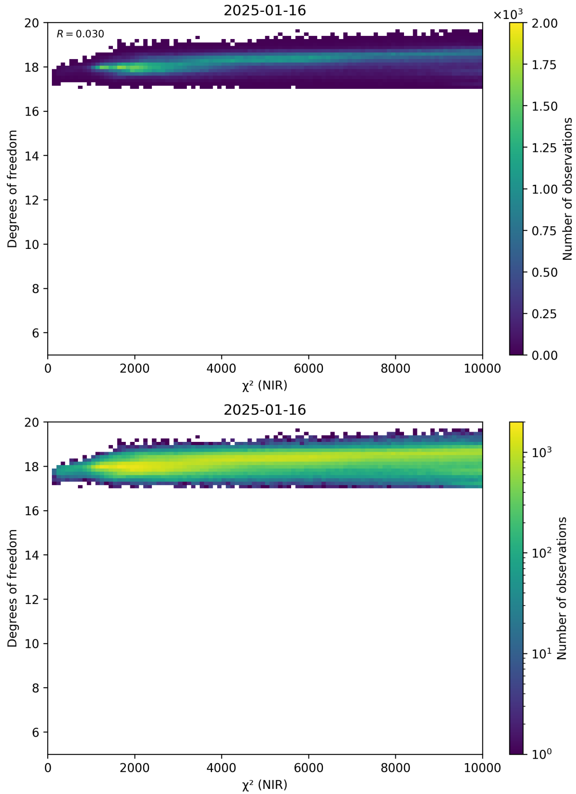
Figure 44: Scatter density plot of “ \chi^2 (NIR)” against “Degrees of freedom” for 2025-01-15 to 2025-01-17.
