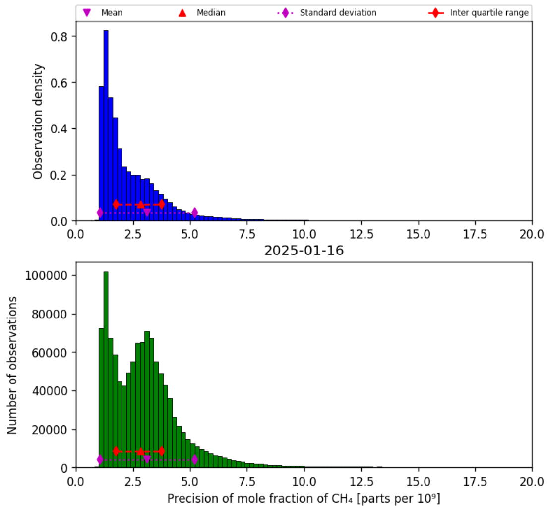
Figure 24: Histogram of “Precision of mole fraction of CH 4 ” for 2025-01-15 to 2025-01-17
