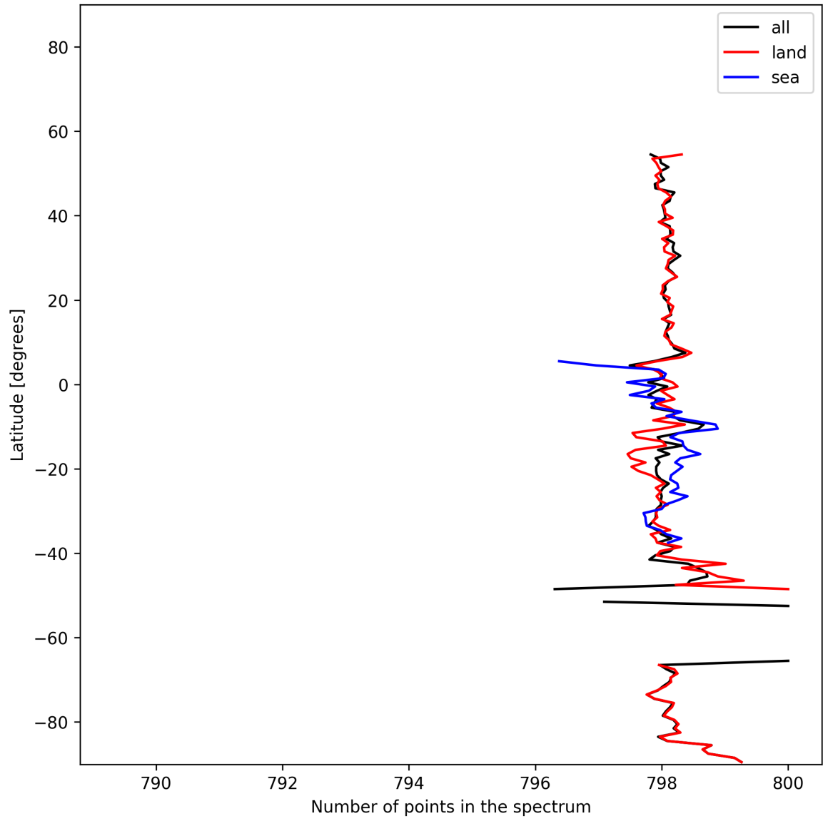
Figure 15: Zonal average of “Number of points in the spectrum” for 2025-01-15 to 2025-01-17.
