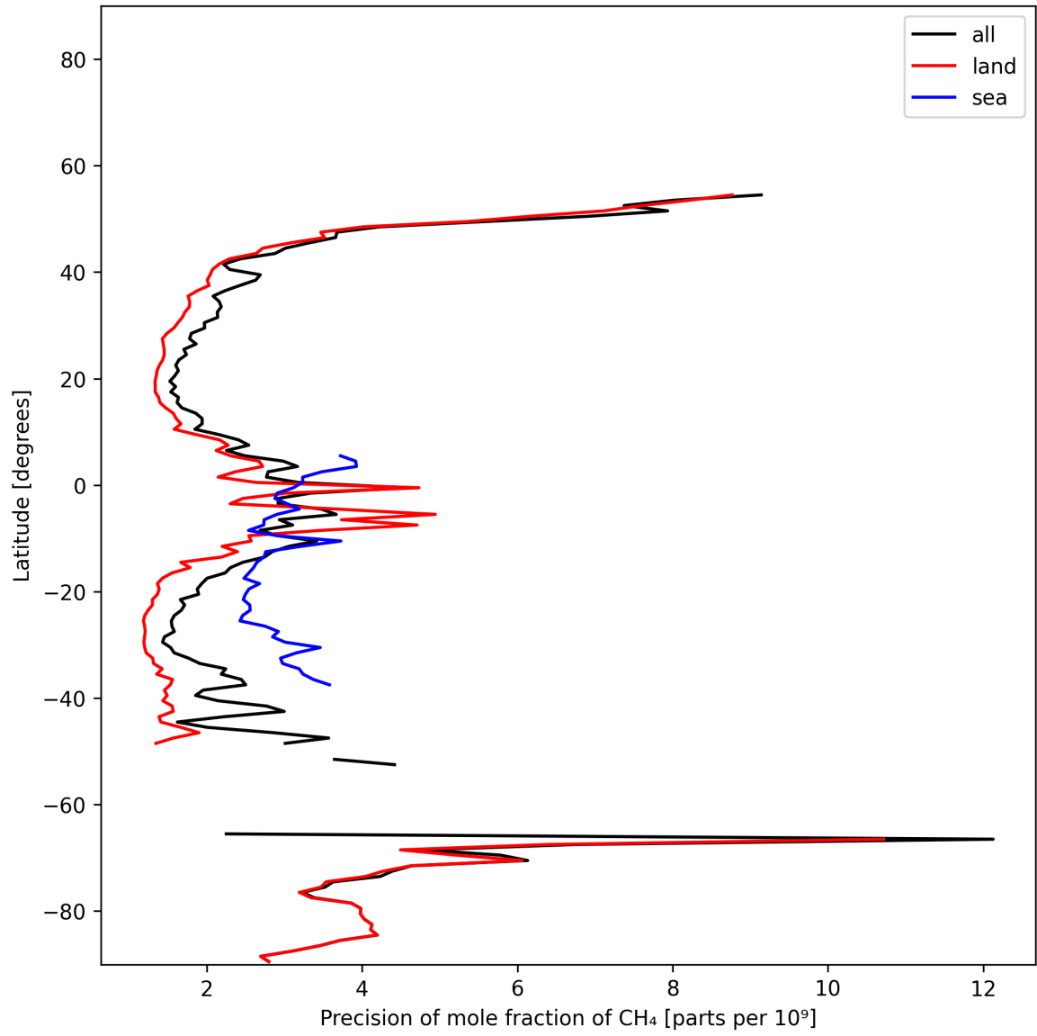
Figure 13: Zonal average of “Precision of mole fraction of CH 4 ” for 2025-01-15 to 2025-01-17.
