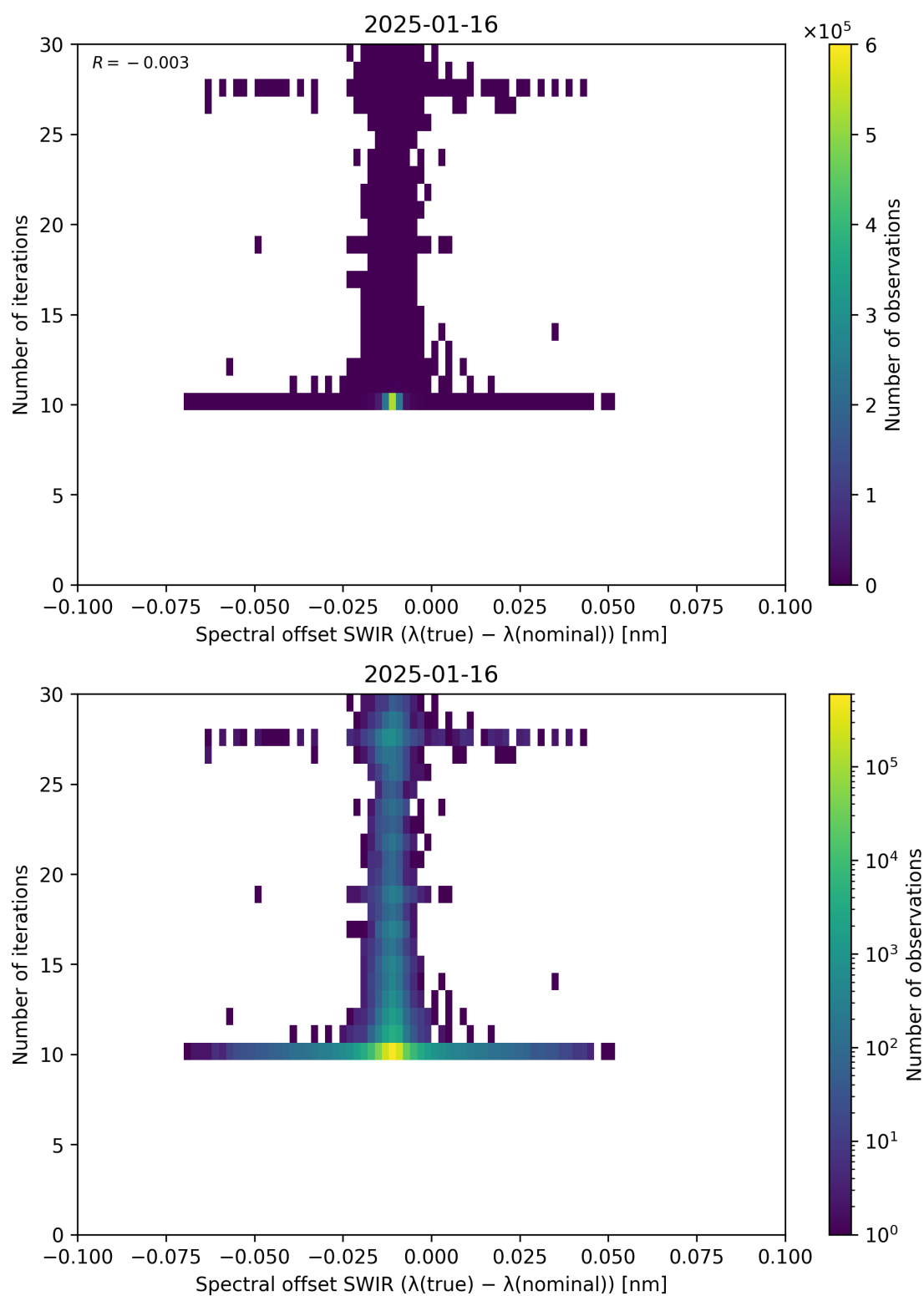
Figure 121: Scatter density plot of “Spectral offset SWIR ( \lambda_{\text{true}} - \lambda_{\text{nominal}} )” against “Number of iterations” for 2025-01-15 to 2025-01-17.
