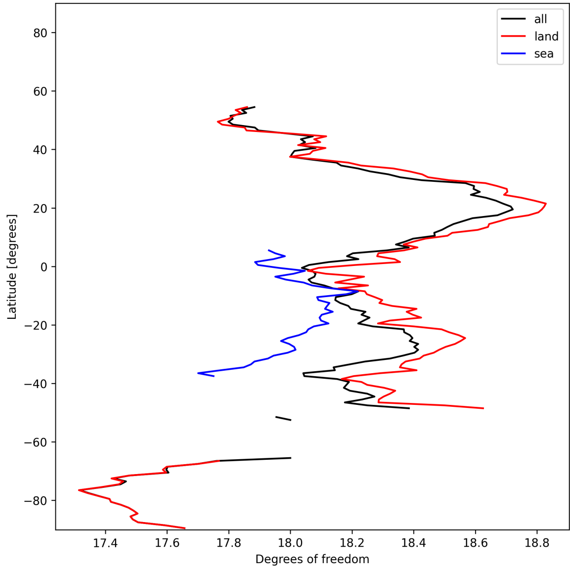
Figure 19: Zonal average of “Degrees of freedom” for 2025-01-15 to 2025-01-17.
