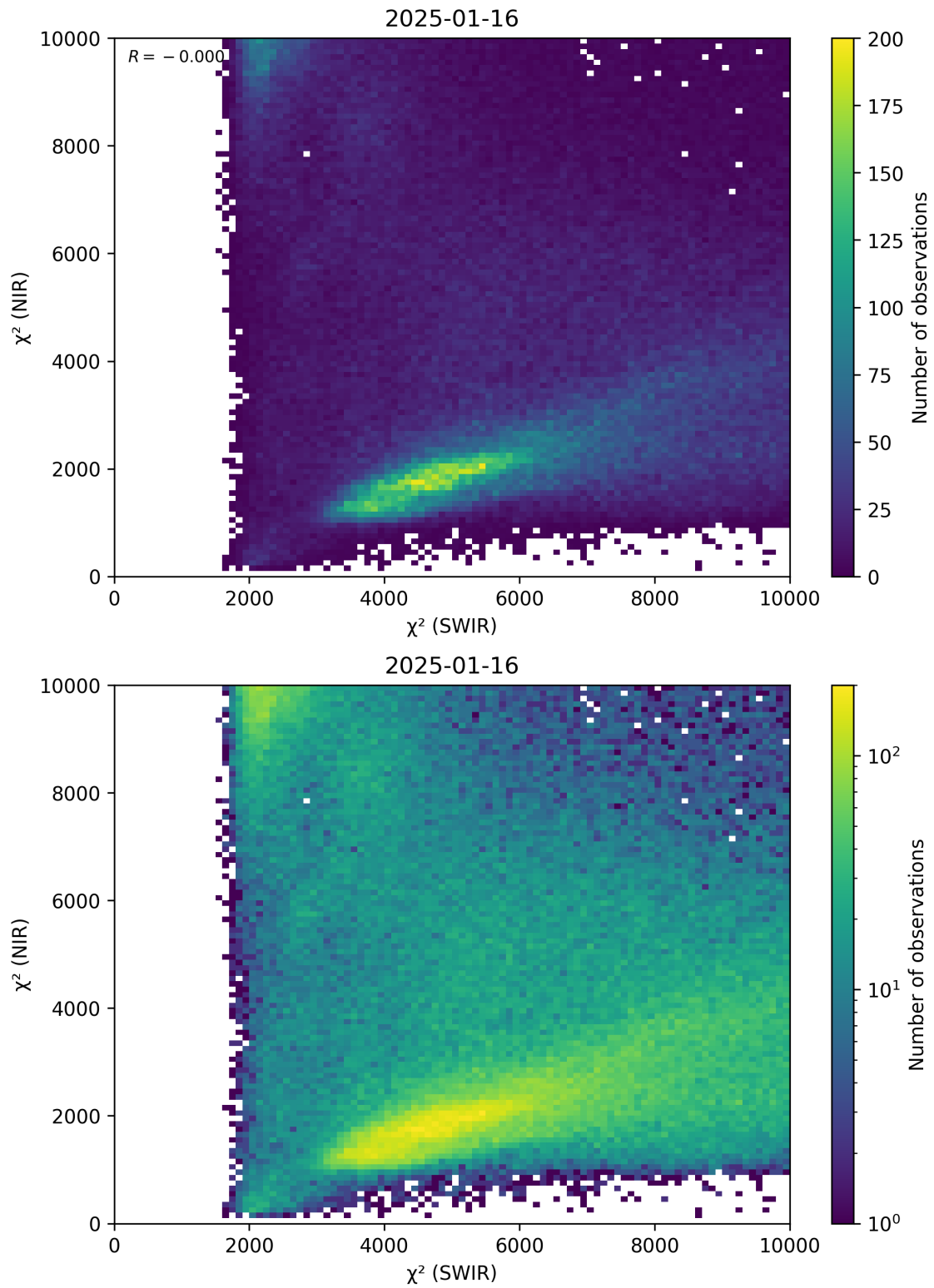
Figure 47: Scatter density plot of “ \chi^2 (SWIR)” against “ \chi^2 (NIR)” for 2025-01-15 to 2025-01-17.
