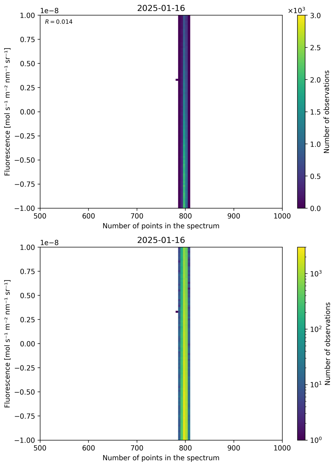
Figure 91: Scatter density plot of “Number of points in the spectrum” against “Fluorescence” for 2025-01-15 to 2025-01-17.
