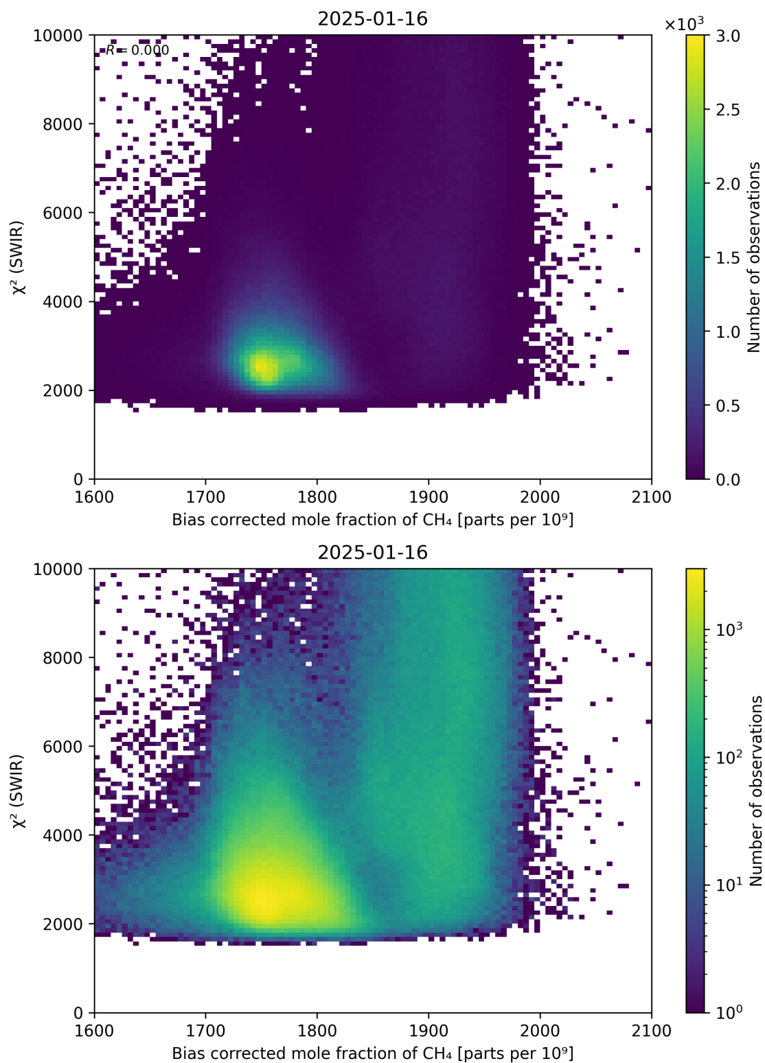
Figure 64: Scatter density plot of “Bias corrected mole fraction of CH 4 ” against “ \chi^2 (SWIR)” for 2025-01-15 to 2025-01-17.
