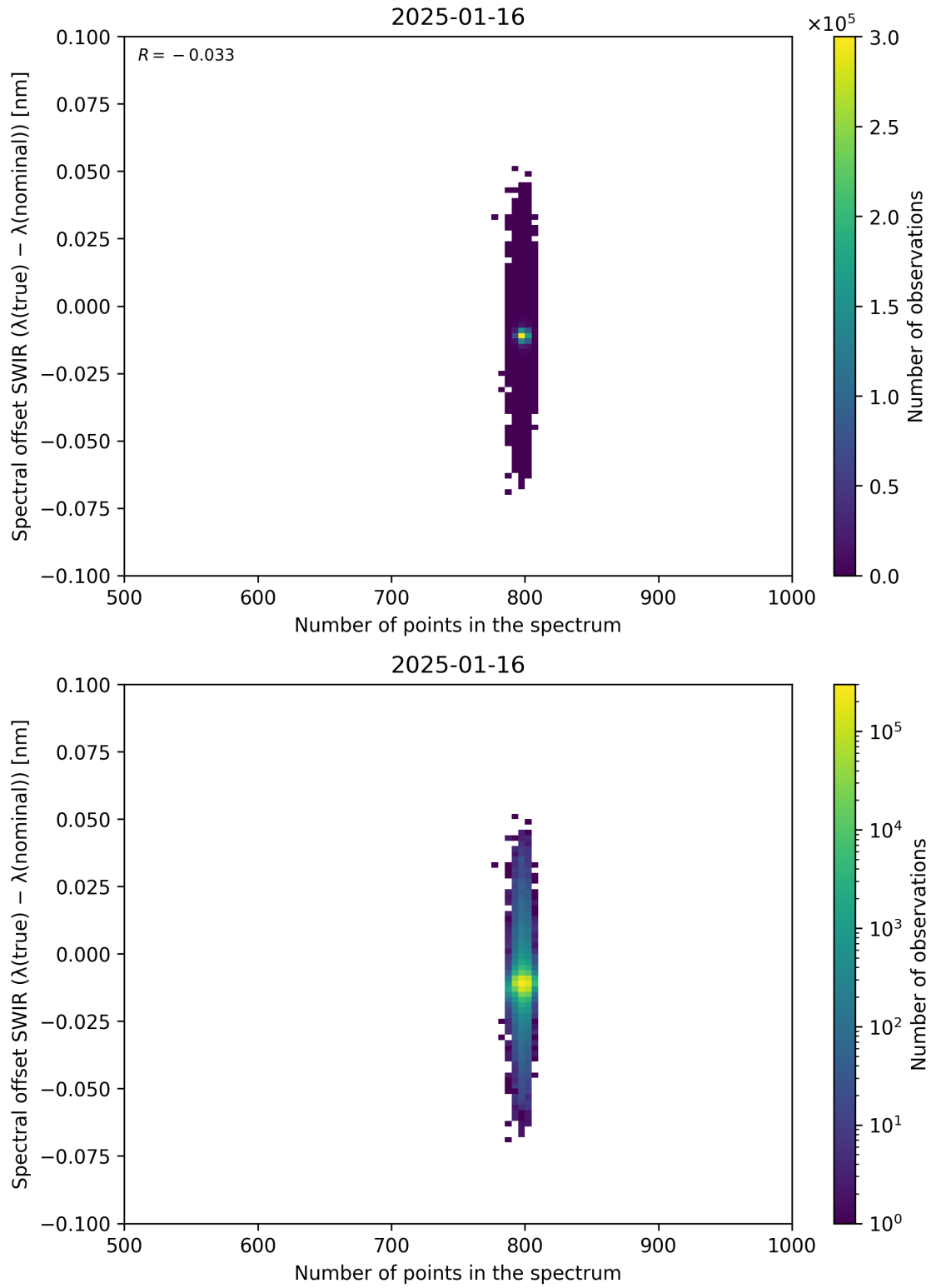
Figure 93: Scatter density plot of “Number of points in the spectrum” against “Spectral offset SWIR ( \lambda_{\text{true}} - \lambda_{\text{nominal}} )” for 2025-01-15 to 2025-01-17.
