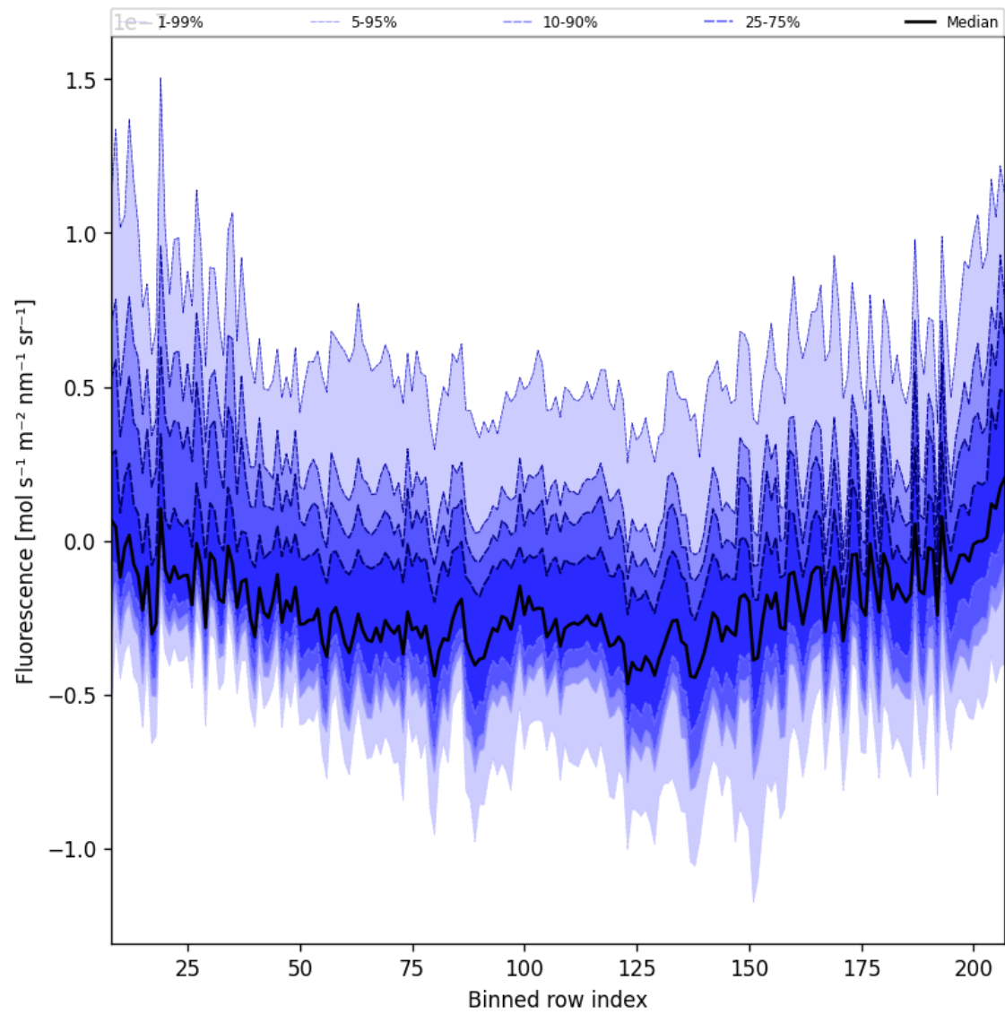
Figure 43: Along track statistics of “Fluorescence” for 2025-01-15 to 2025-01-17
