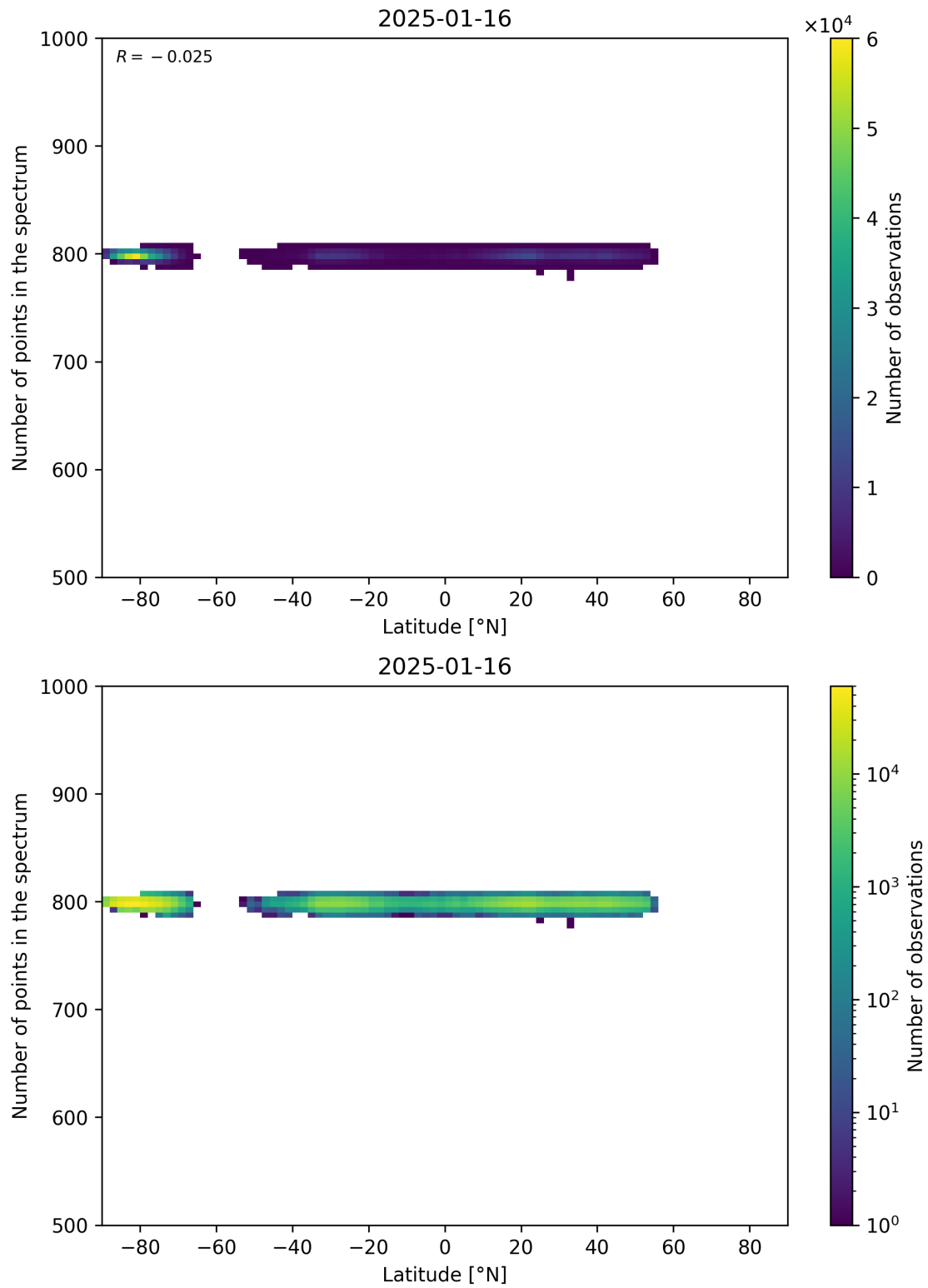
Figure 61: Scatter density plot of “Latitude” against “Number of points in the spectrum” for 2025-01-15 to 2025-01-17.
