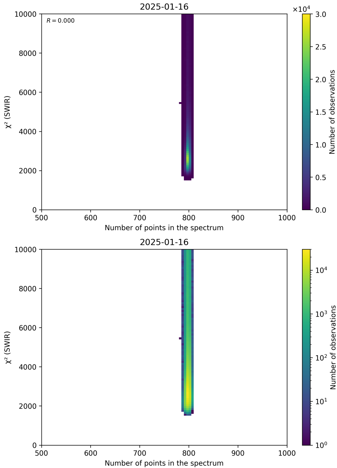
Figure 89: Scatter density plot of “Number of points in the spectrum” against “ \chi^2 (SWIR)” for 2025-01-15 to 2025-01-17.
