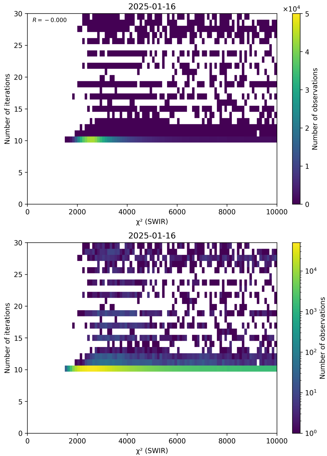
Figure 50: Scatter density plot of “ \chi^2 (SWIR)” against “Number of iterations” for 2025-01-15 to 2025-01-17.
