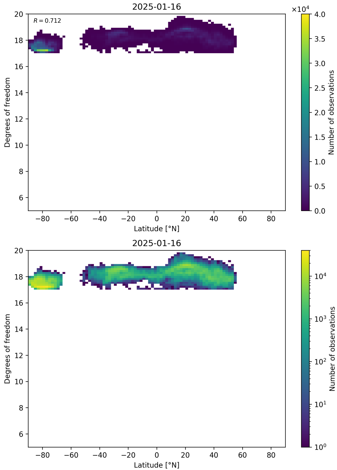
Figure 55: Scatter density plot of “Latitude” against “Degrees of freedom” for 2025-01-15 to 2025-01-17.
