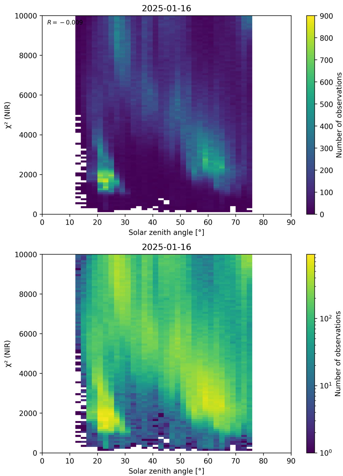
Figure 94: Scatter density plot of “Solar zenith angle” against “ \chi^2 (NIR)” for 2025-01-15 to 2025-01-17.
