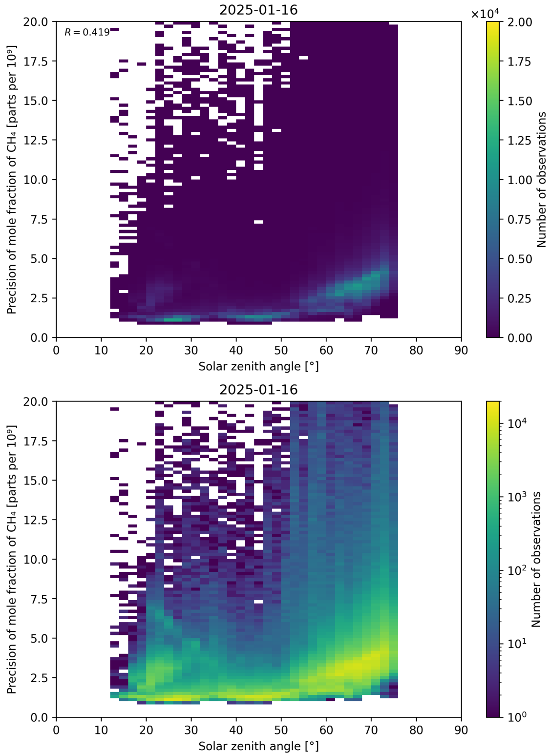
Figure 101: Scatter density plot of “Solar zenith angle” against “Precision of mole fraction of CH 4 ” for 2025-01-15 to 2025-01-17.
