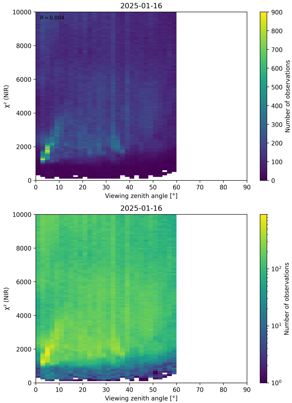
Figure 105: Scatter density plot of “Viewing zenith angle” against “ \chi^2 (NIR)” for 2025-01-15 to 2025-01-17.
