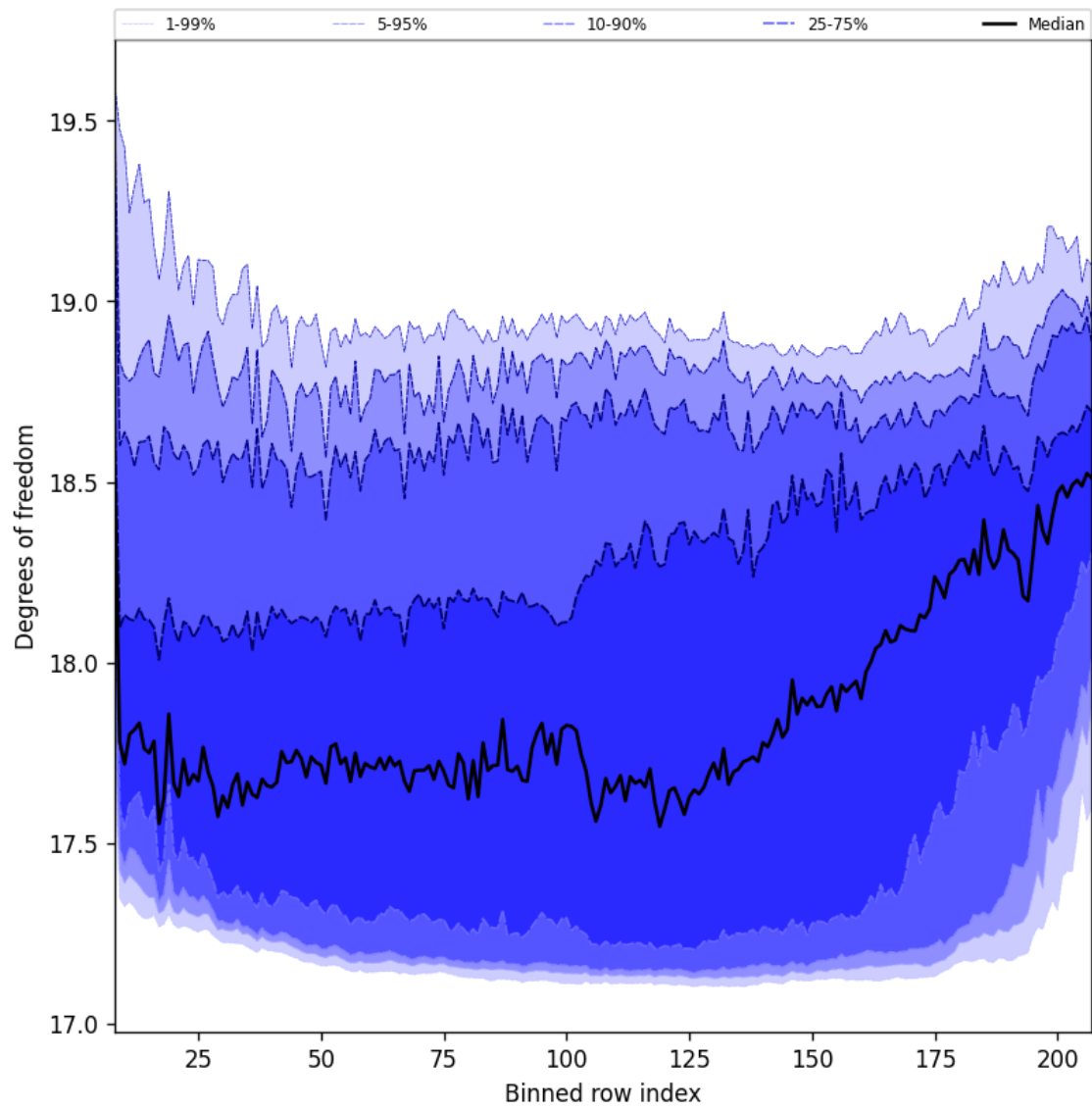
Figure 41: Along track statistics of “Degrees of freedom” for 2025-01-15 to 2025-01-17
