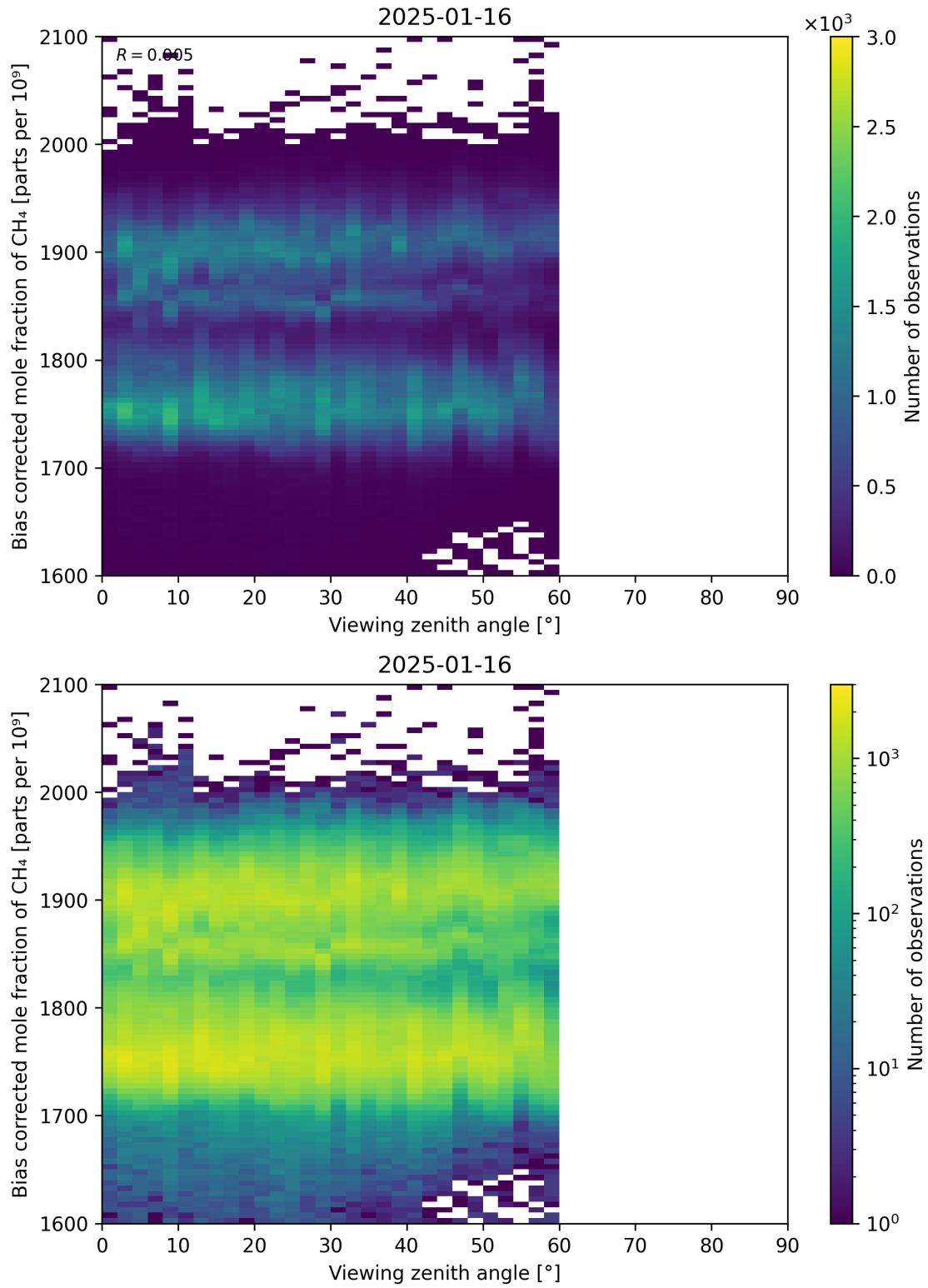
Figure 111: Scatter density plot of “Viewing zenith angle” against “Bias corrected mole fraction of CH 4 ” for 2025-01-15 to 2025-01-17.
