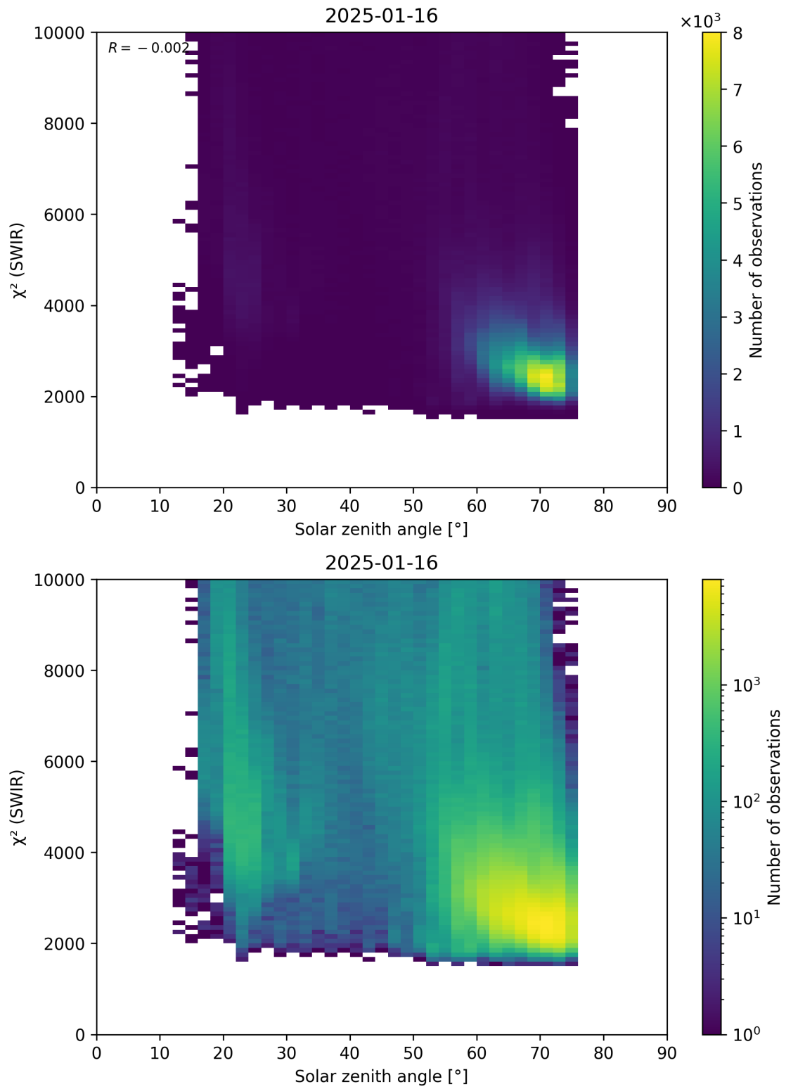
Figure 95: Scatter density plot of “Solar zenith angle” against “ \chi^2 (SWIR)” for 2025-01-15 to 2025-01-17.
