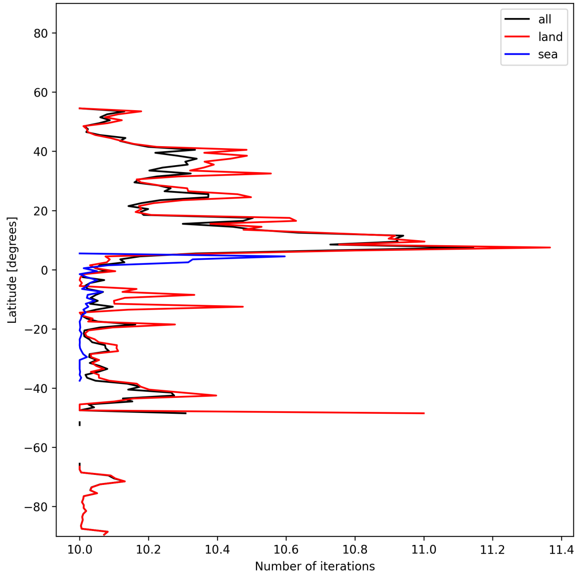
Figure 20: Zonal average of “Number of iterations” for 2025-01-15 to 2025-01-17.
