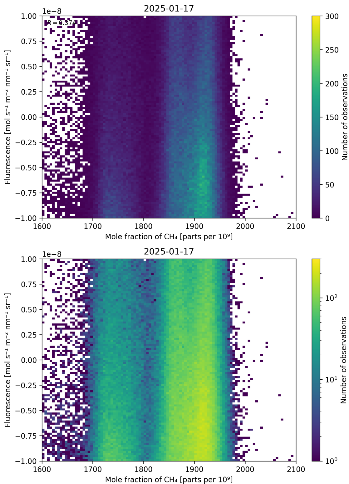
Figure 73: Scatter density plot of “Mole fraction of \text{CH}_4 ” against “Fluorescence” for 2025-01-17 to 2025-01-18.
