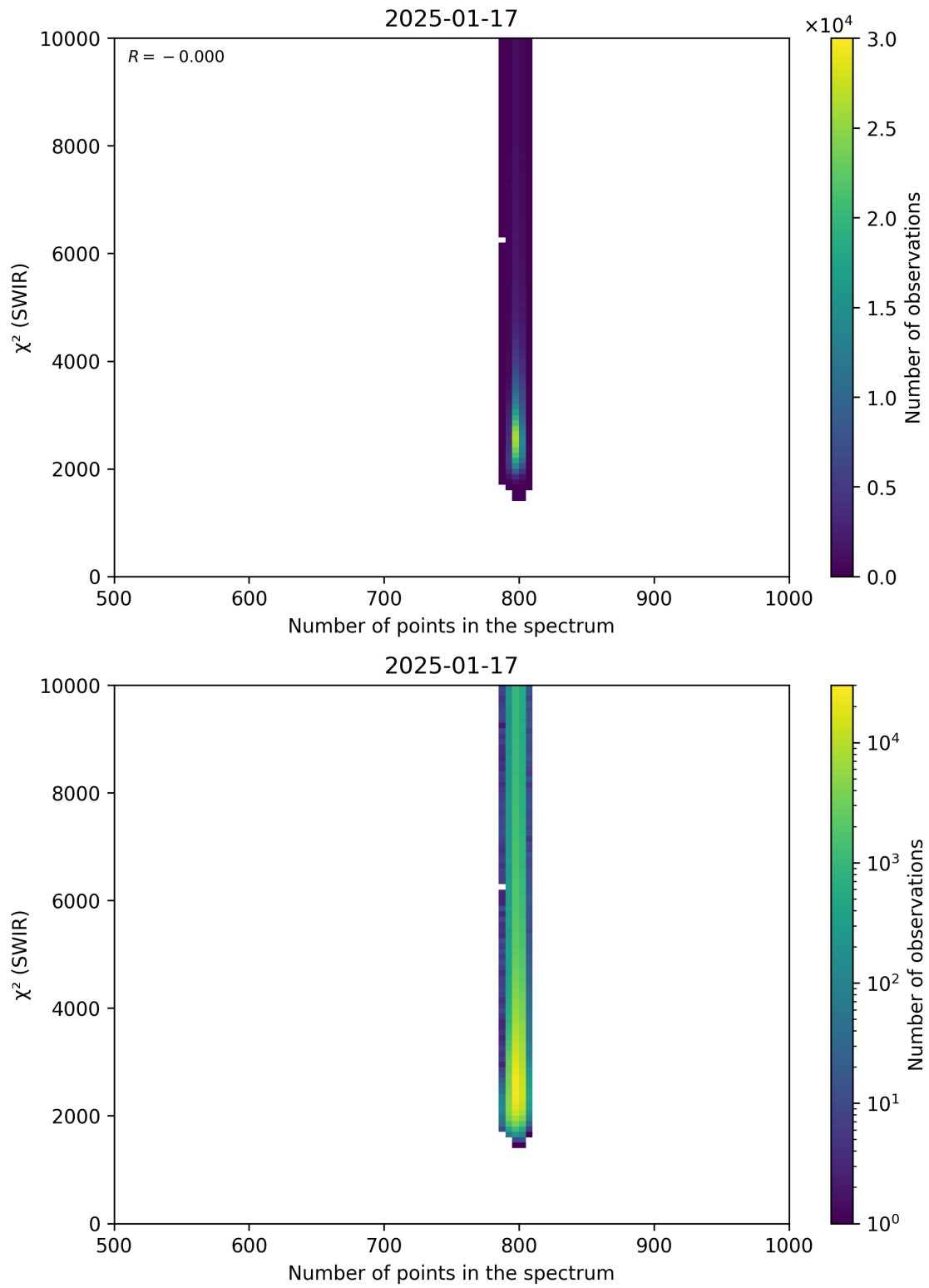
Figure 89: Scatter density plot of “Number of points in the spectrum” against “ \chi^2 (SWIR)” for 2025-01-17 to 2025-01-18.
