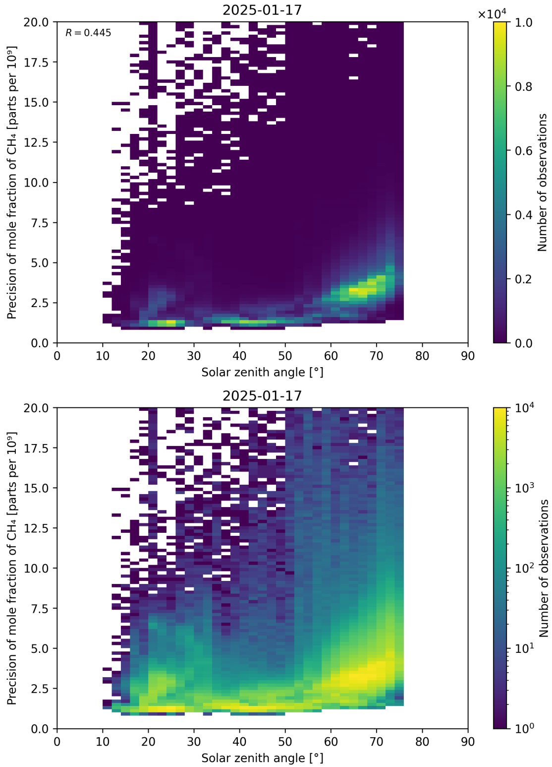
Figure 101: Scatter density plot of “Solar zenith angle” against “Precision of mole fraction of \text{CH}_4 ” for 2025-01-17 to 2025-01-18.
