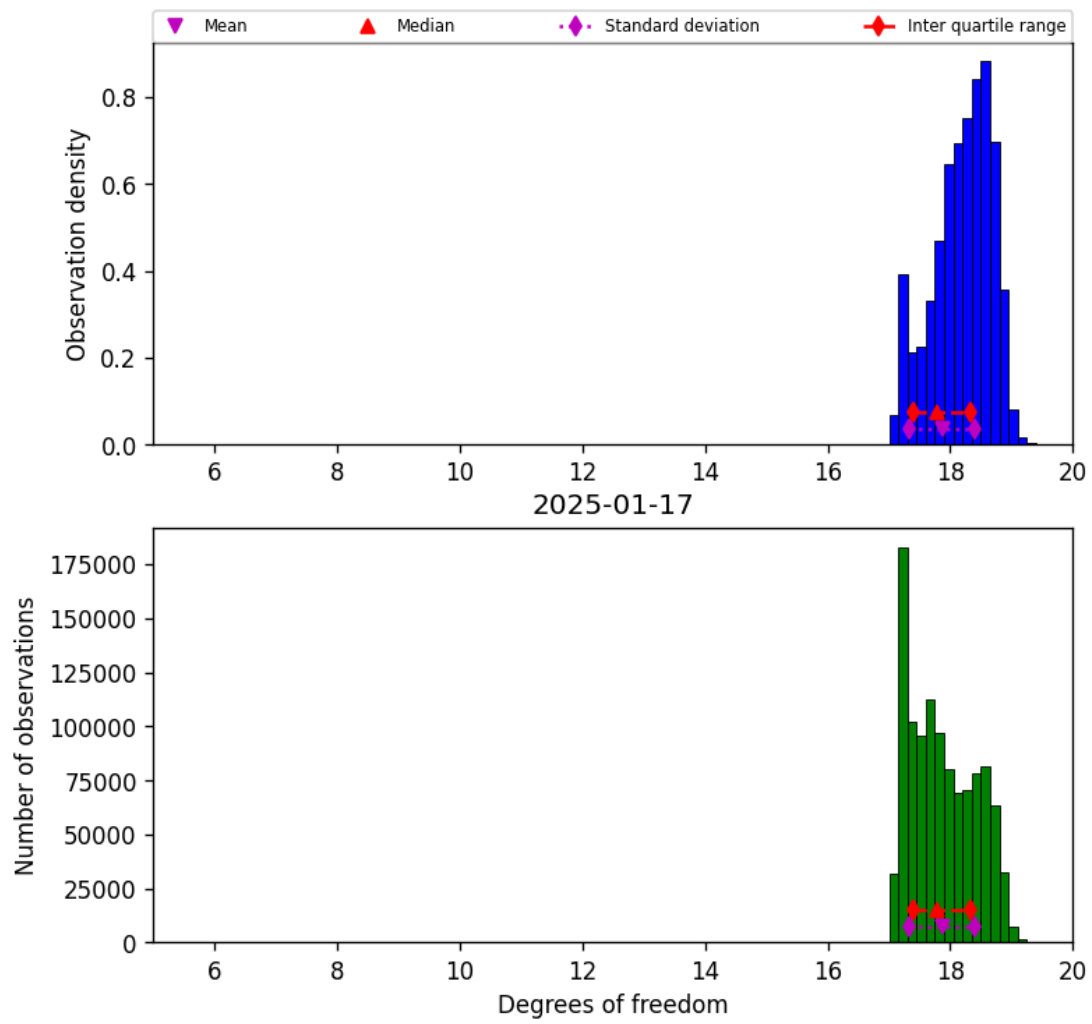
Figure 30: Histogram of “Degrees of freedom” for 2025-01-17 to 2025-01-18
