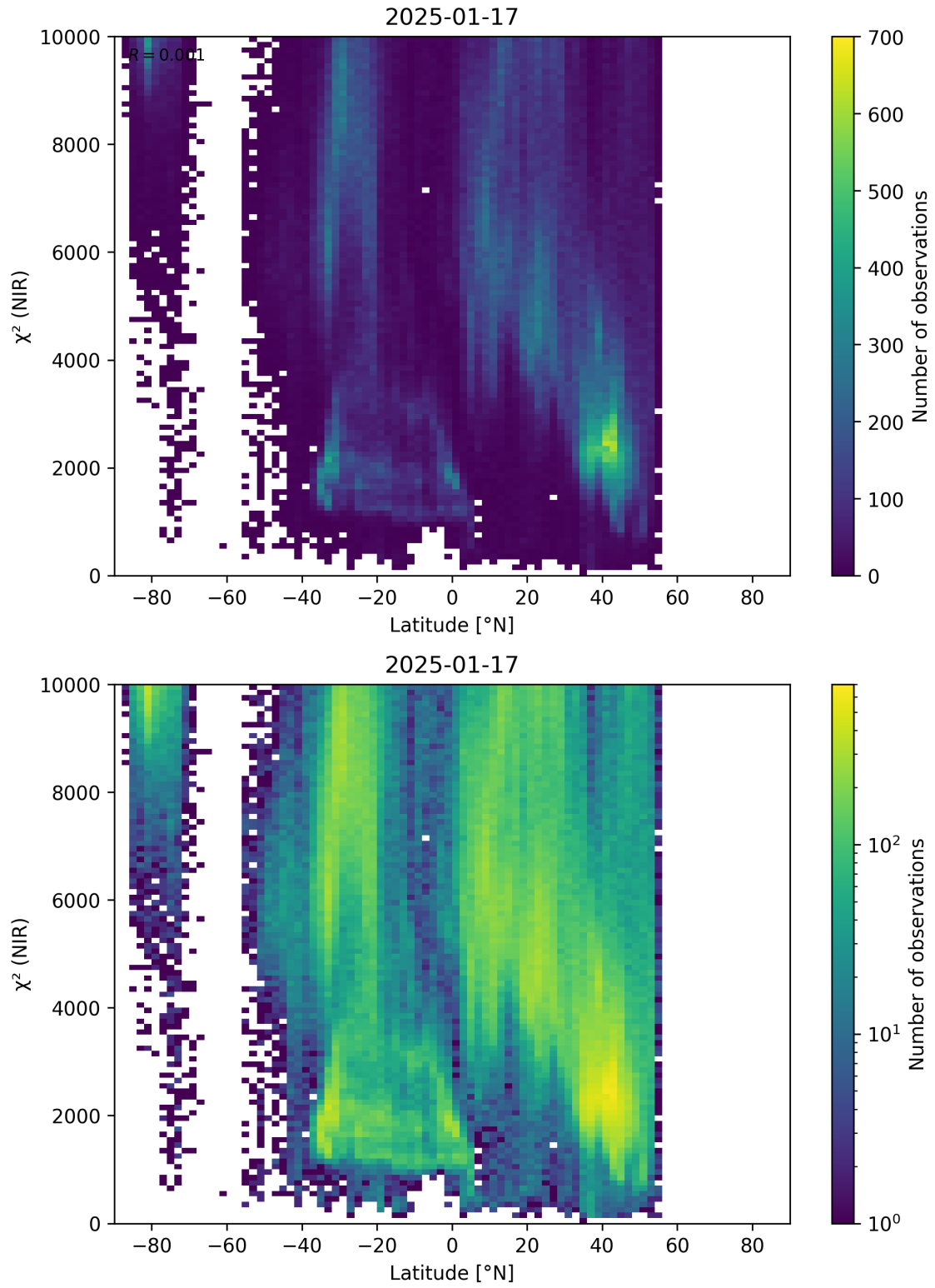
Figure 53: Scatter density plot of “Latitude” against “ \chi^2 (NIR)” for 2025-01-17 to 2025-01-18.
