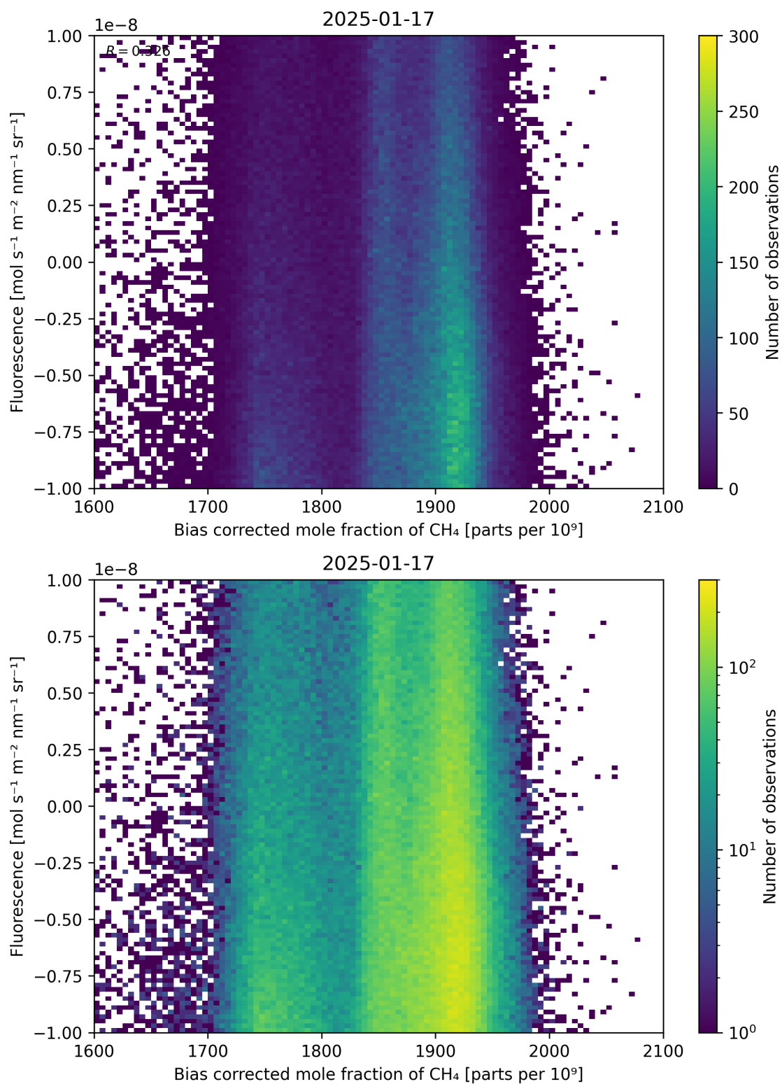
Figure 66: Scatter density plot of “Bias corrected mole fraction of \text{CH}_4 ” against “Fluorescence” for 2025-01-17 to 2025-01-18.
