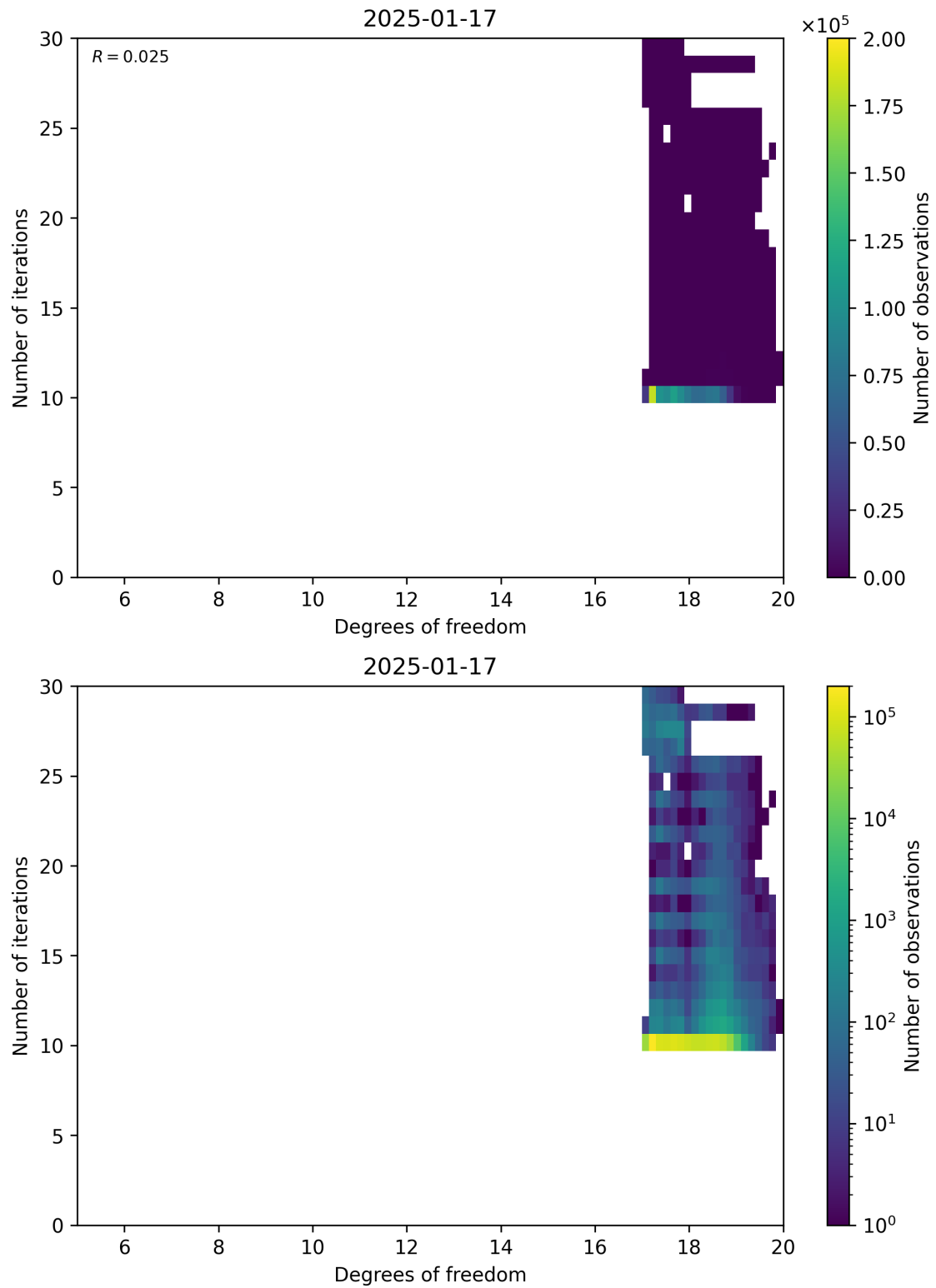
Figure 52: Scatter density plot of “Degrees of freedom” against “Number of iterations” for 2025-01-17 to 2025-01-18.
