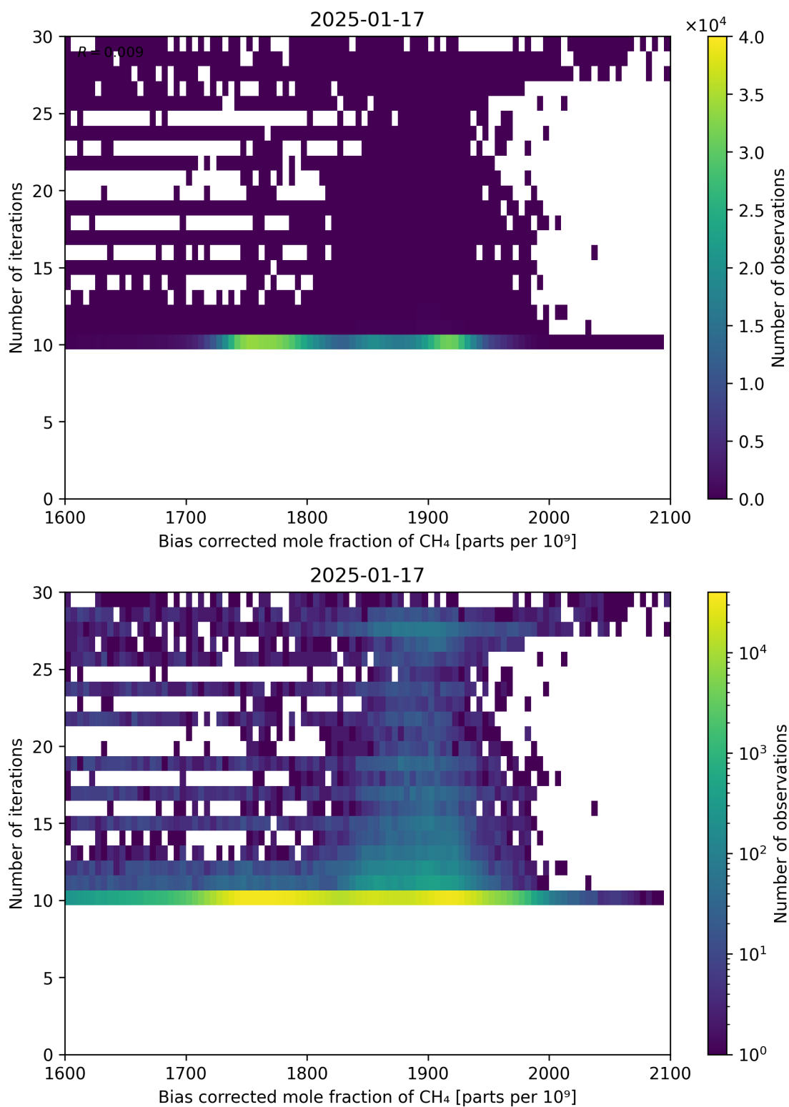
Figure 67: Scatter density plot of “Bias corrected mole fraction of CH 4 ” against “Number of iterations” for 2025-01-17 to 2025-01-18.
