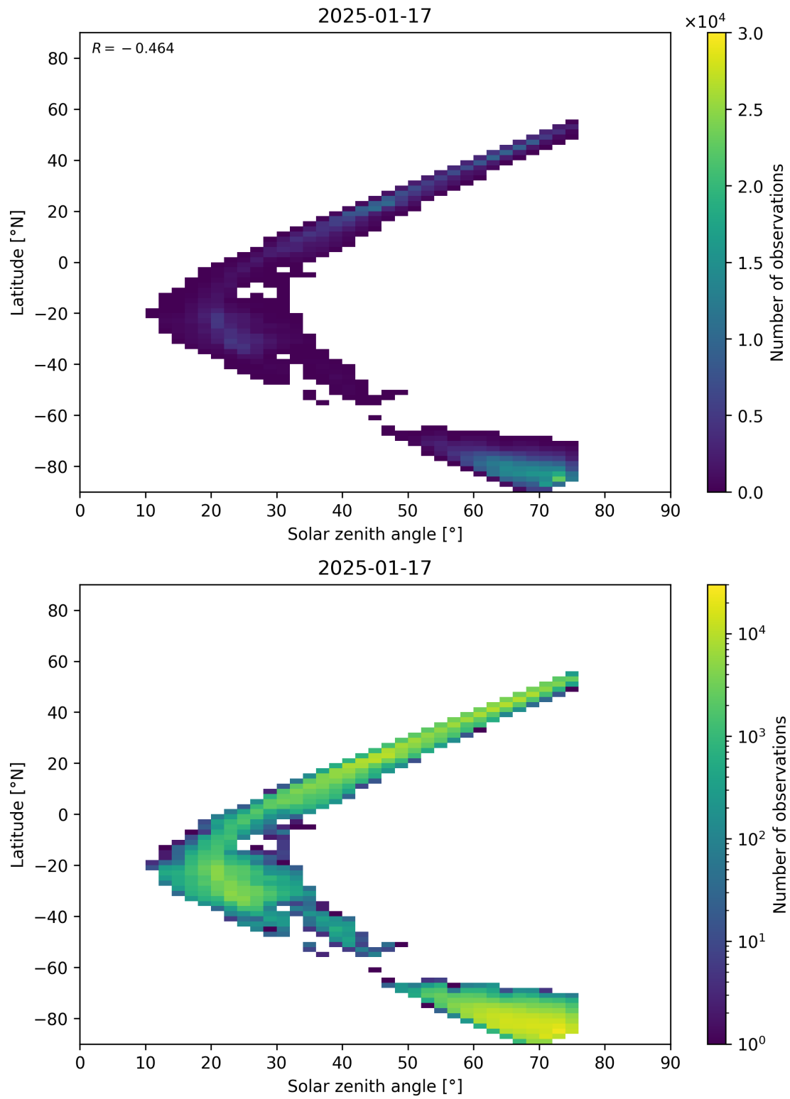
Figure 98: Scatter density plot of “Solar zenith angle” against “Latitude” for 2025-01-17 to 2025-01-18.
