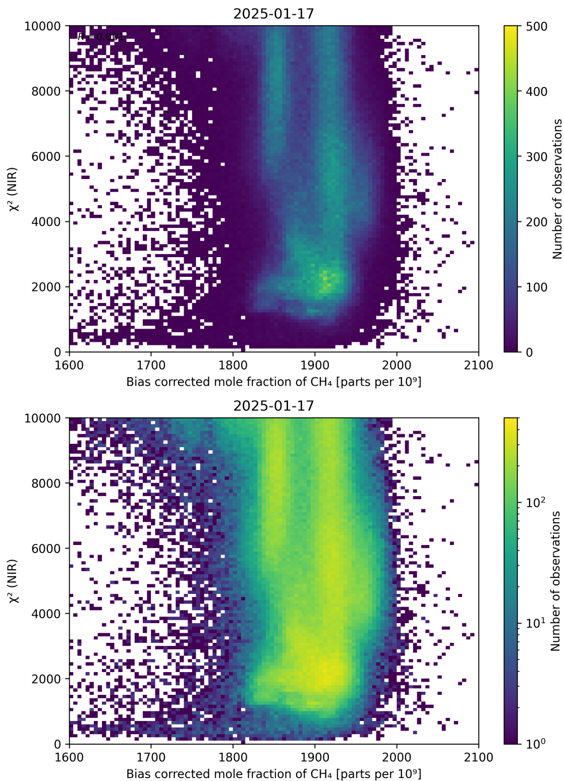
Figure 63: Scatter density plot of “Bias corrected mole fraction of \text{CH}_4 ” against “ \chi^2 (NIR)” for 2025-01-17 to 2025-01-18.
