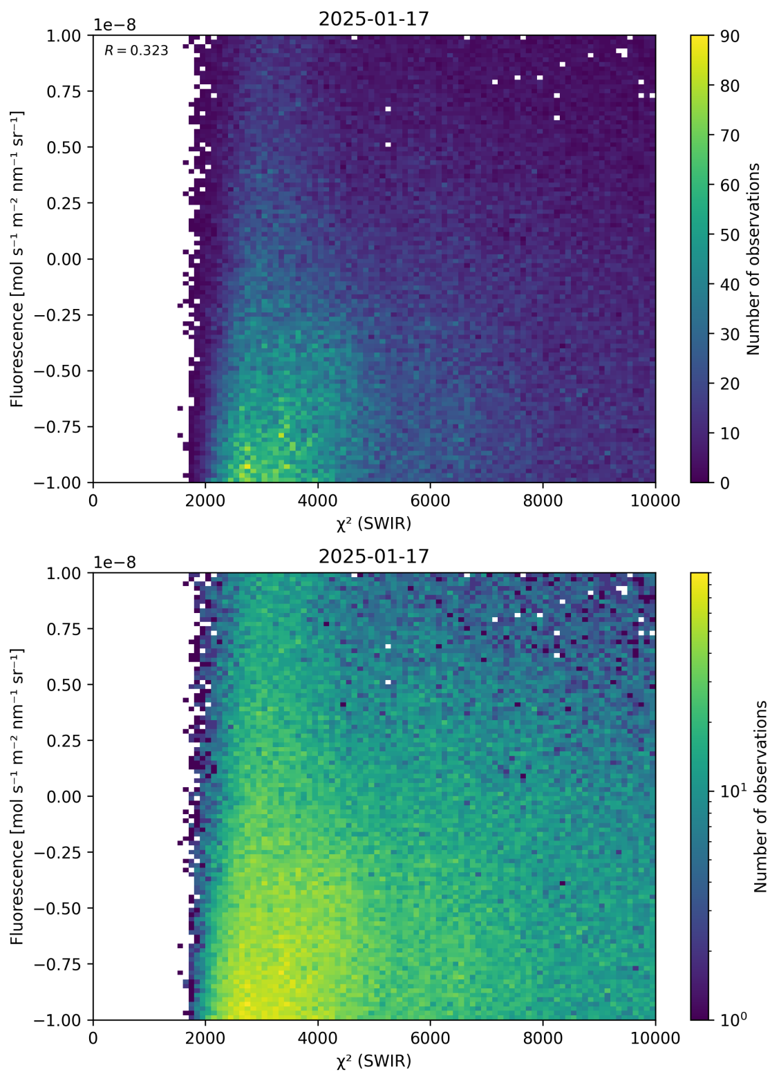
Figure 49: Scatter density plot of “ \chi^2 (SWIR)” against “Fluorescence” for 2025-01-17 to 2025-01-18.
