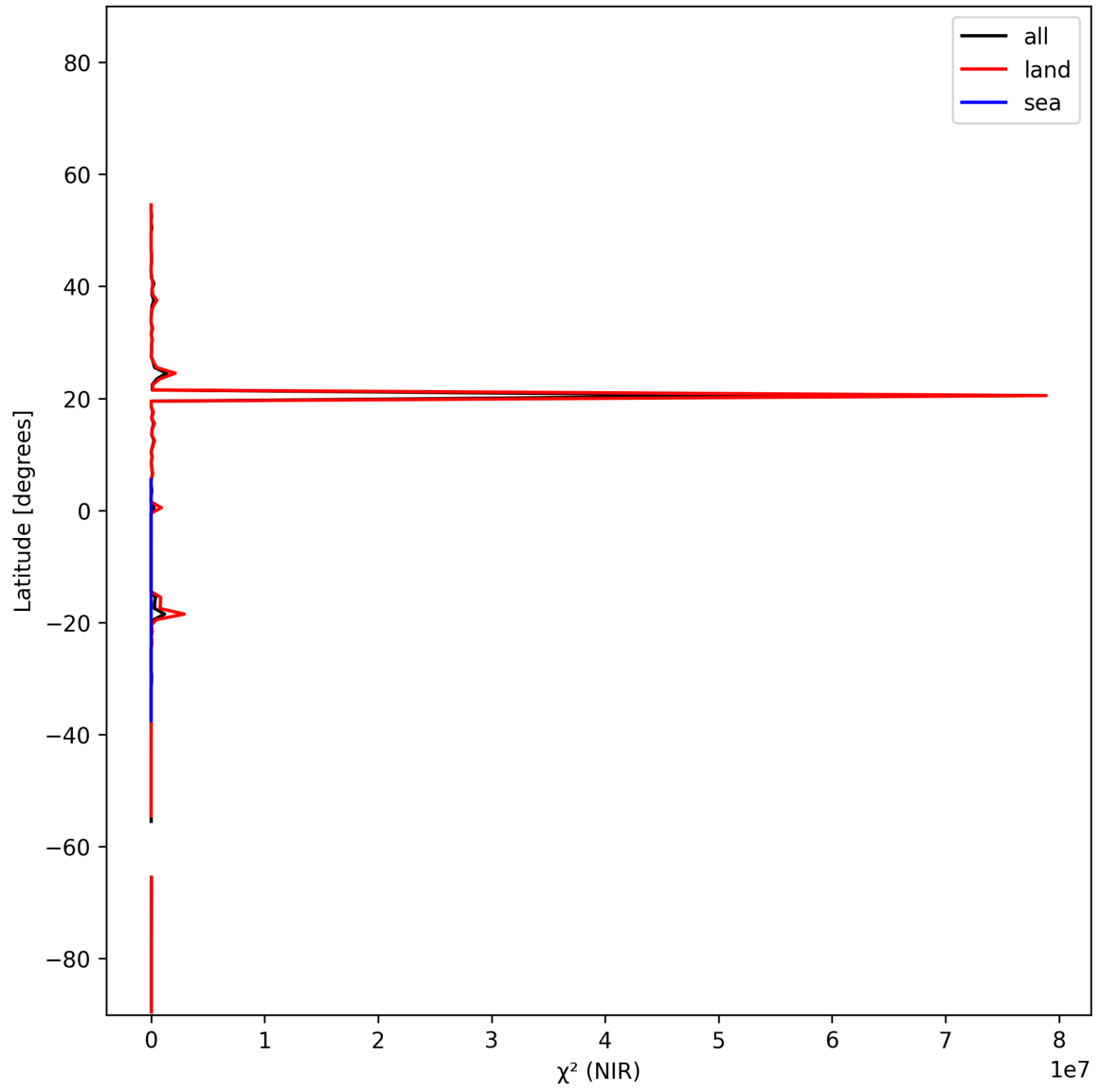
Figure 18: Zonal average of “ \chi^2 (NIR)” for 2025-01-17 to 2025-01-18.
