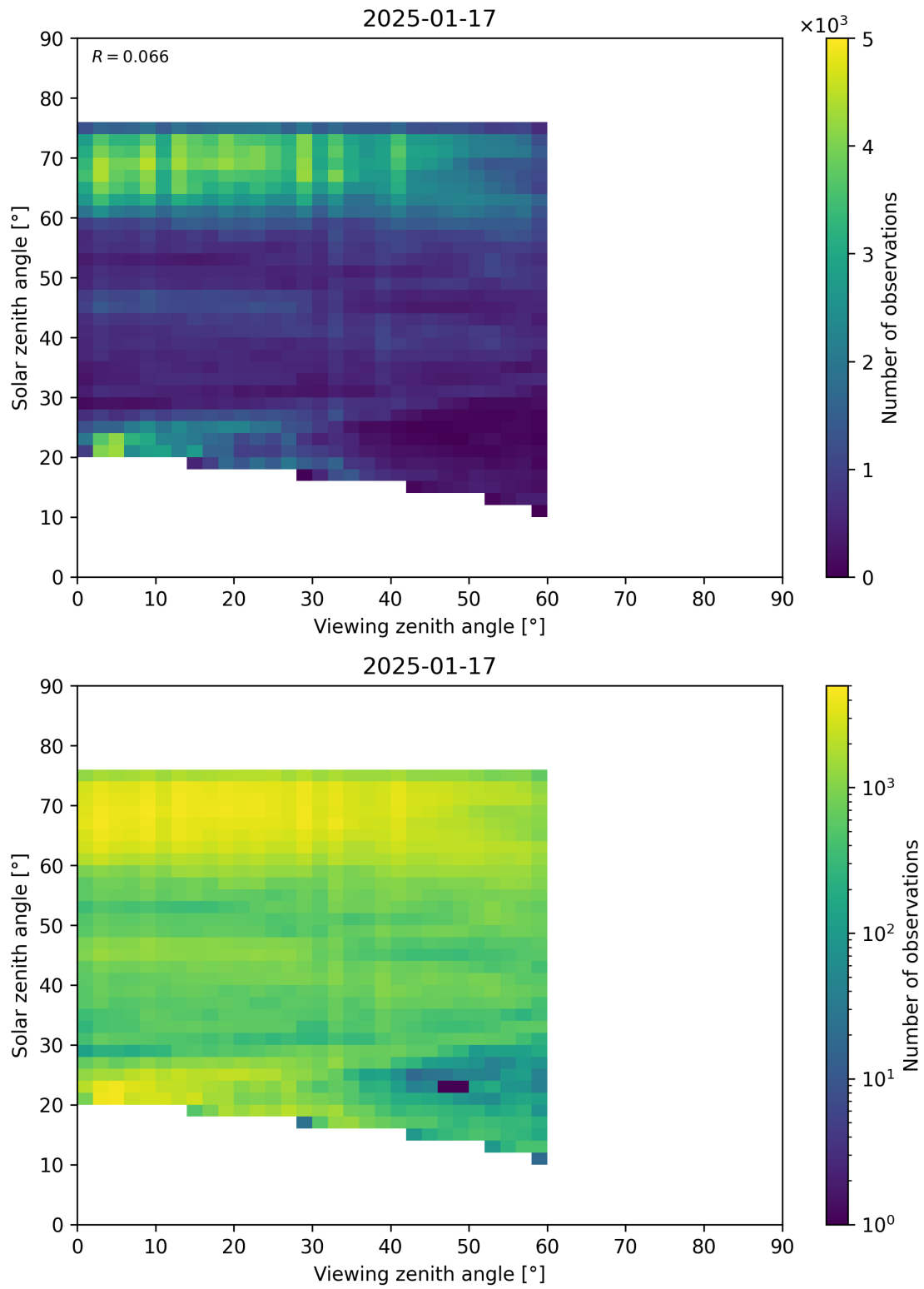
Figure 115: Scatter density plot of “Viewing zenith angle” against “Solar zenith angle” for 2025-01-17 to 2025-01-18.
