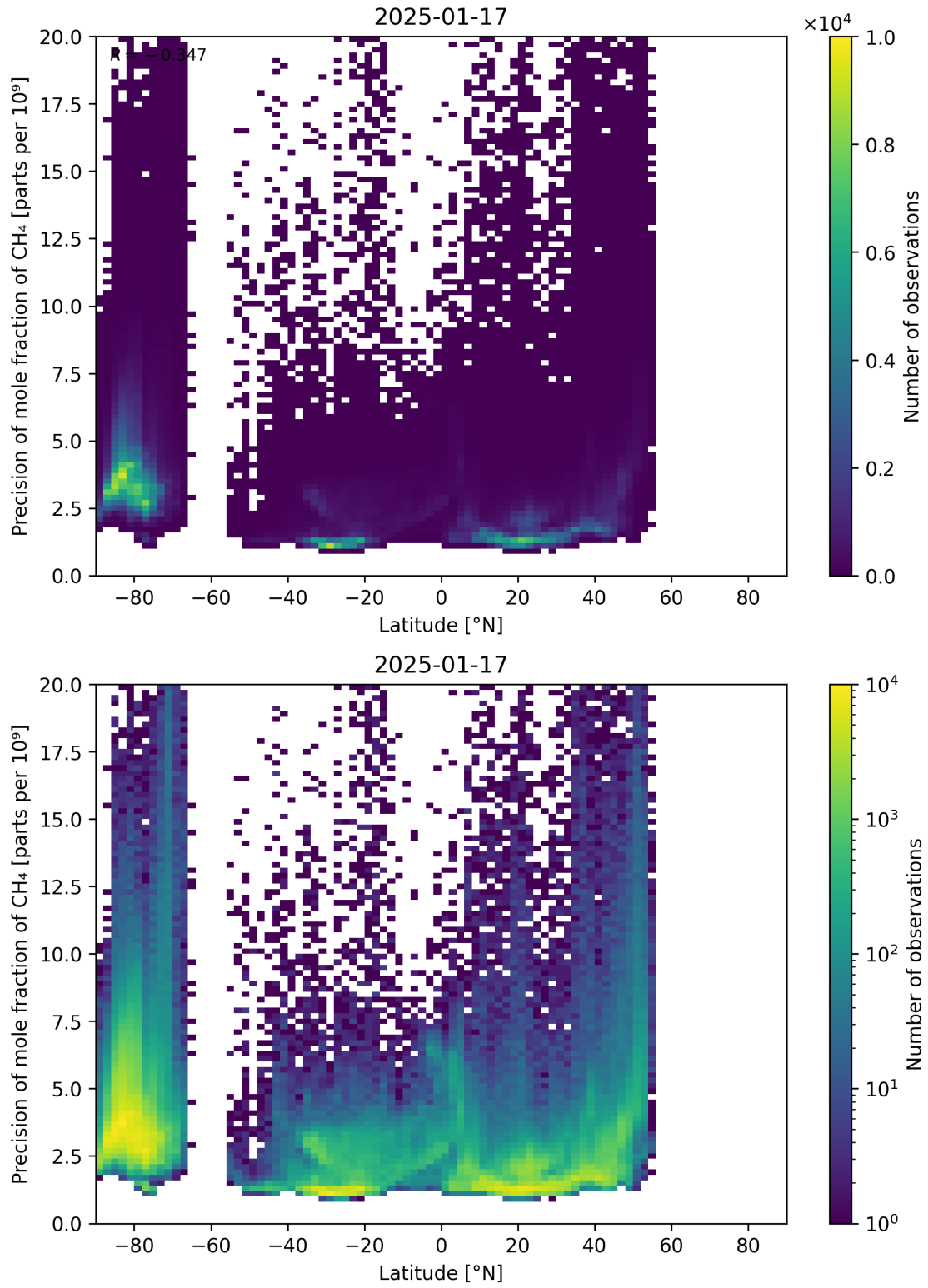
Figure 59: Scatter density plot of “Latitude” against “Precision of mole fraction of CH 4 ” for 2025-01-17 to 2025-01-18.
