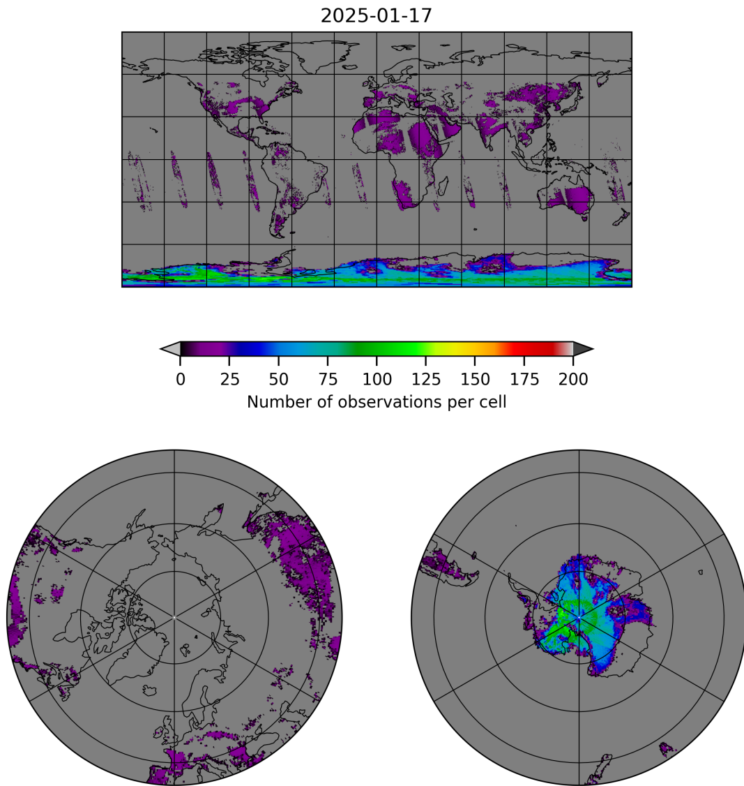
Figure 10: Map of the number of observations for 2025-01-17 to 2025-01-18
