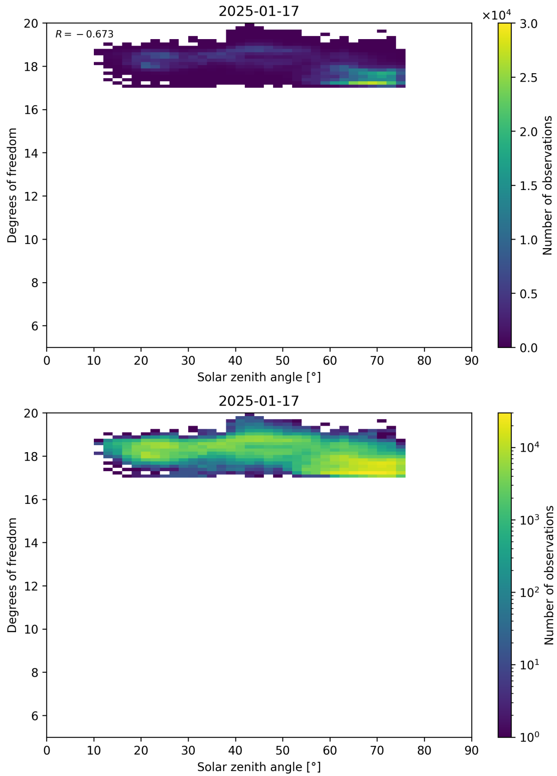
Figure 96: Scatter density plot of “Solar zenith angle” against “Degrees of freedom” for 2025-01-17 to 2025-01-18.
