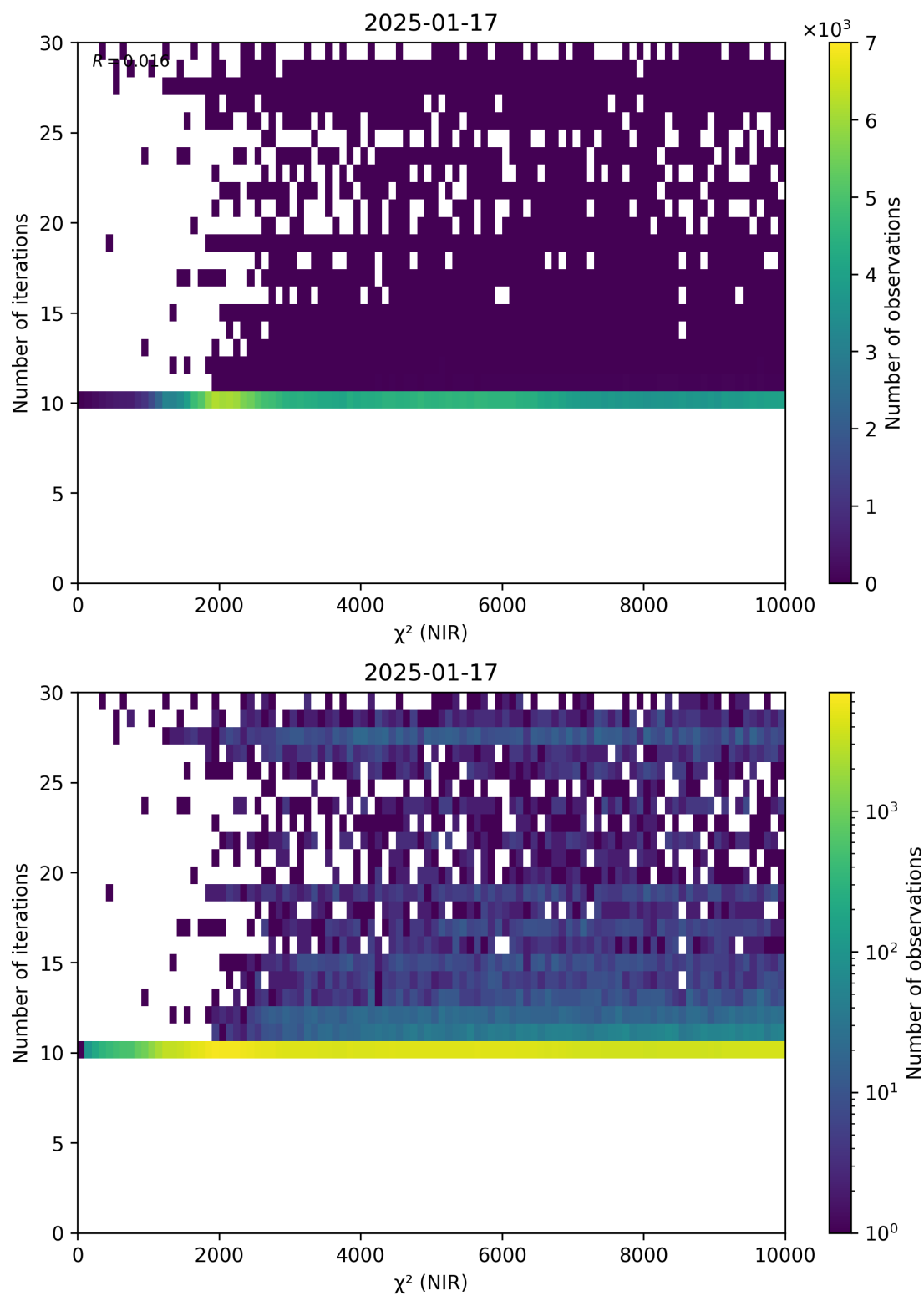
Figure 46: Scatter density plot of “ \chi^2 (NIR)” against “Number of iterations” for 2025-01-17 to 2025-01-18.
