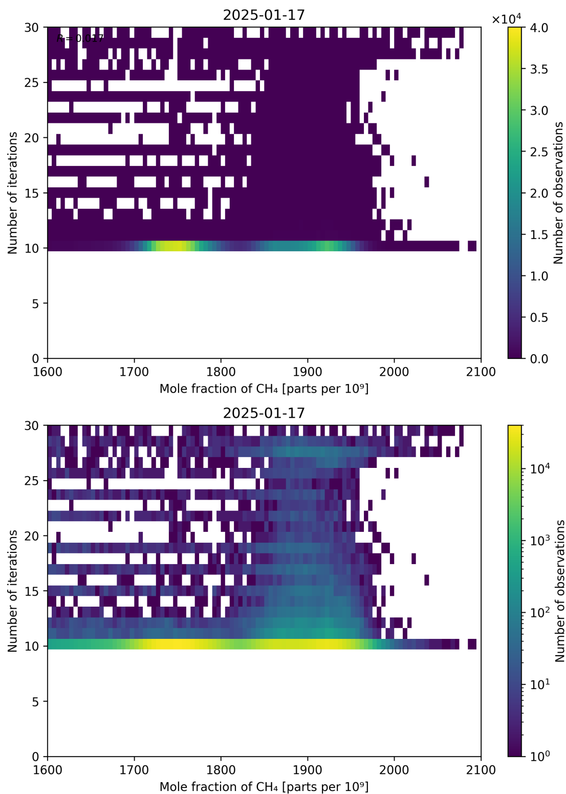
Figure 76: Scatter density plot of “Mole fraction of CH 4 ” against “Number of iterations” for 2025-01-17 to 2025-01-18.
