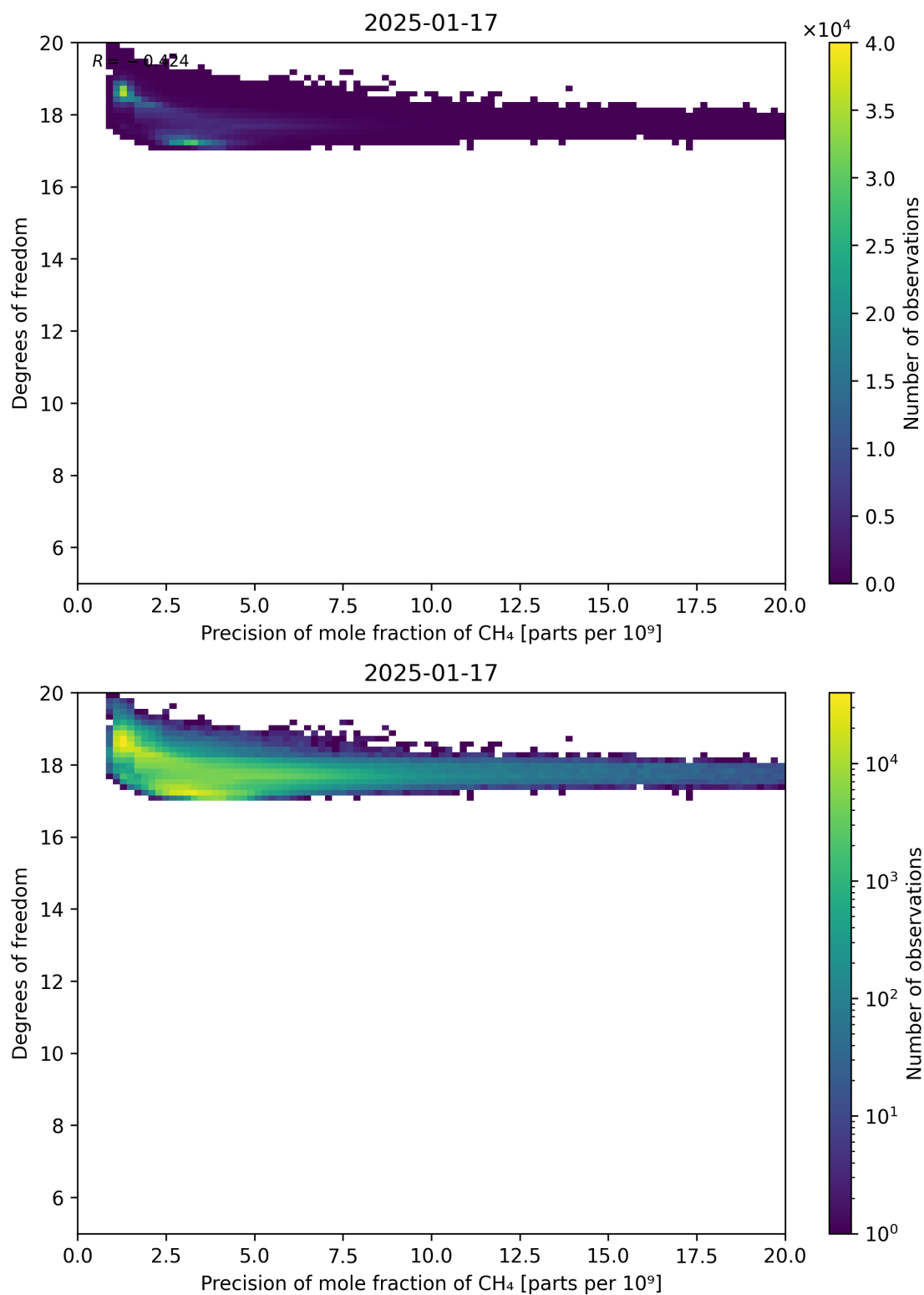
Figure 80: Scatter density plot of “Precision of mole fraction of CH 4 ” against “Degrees of freedom” for 2025-01-17 to 2025-01-18.
