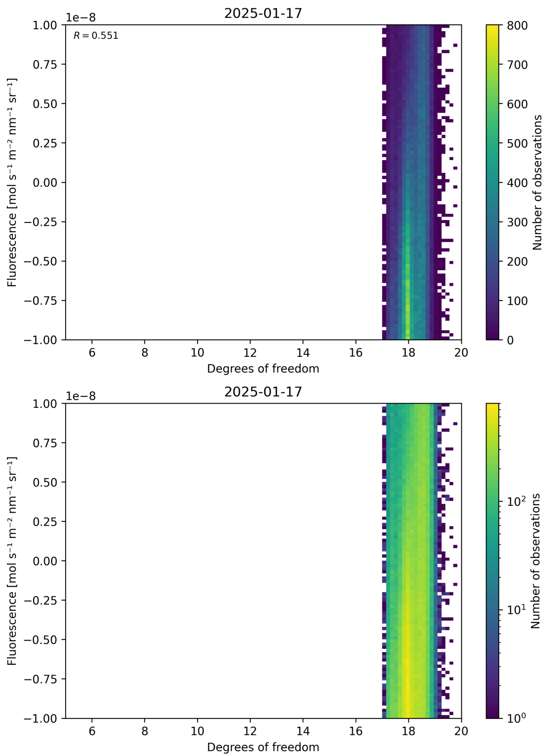
Figure 51: Scatter density plot of “Degrees of freedom” against “Fluorescence” for 2025-01-17 to 2025-01-18.
