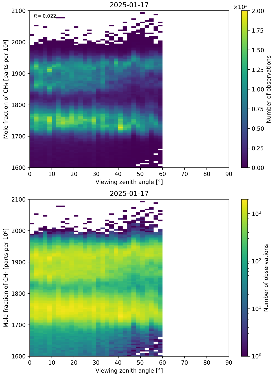
Figure 110: Scatter density plot of “Viewing zenith angle” against “Mole fraction of CH 4 ” for 2025-01-17 to 2025-01-18.
