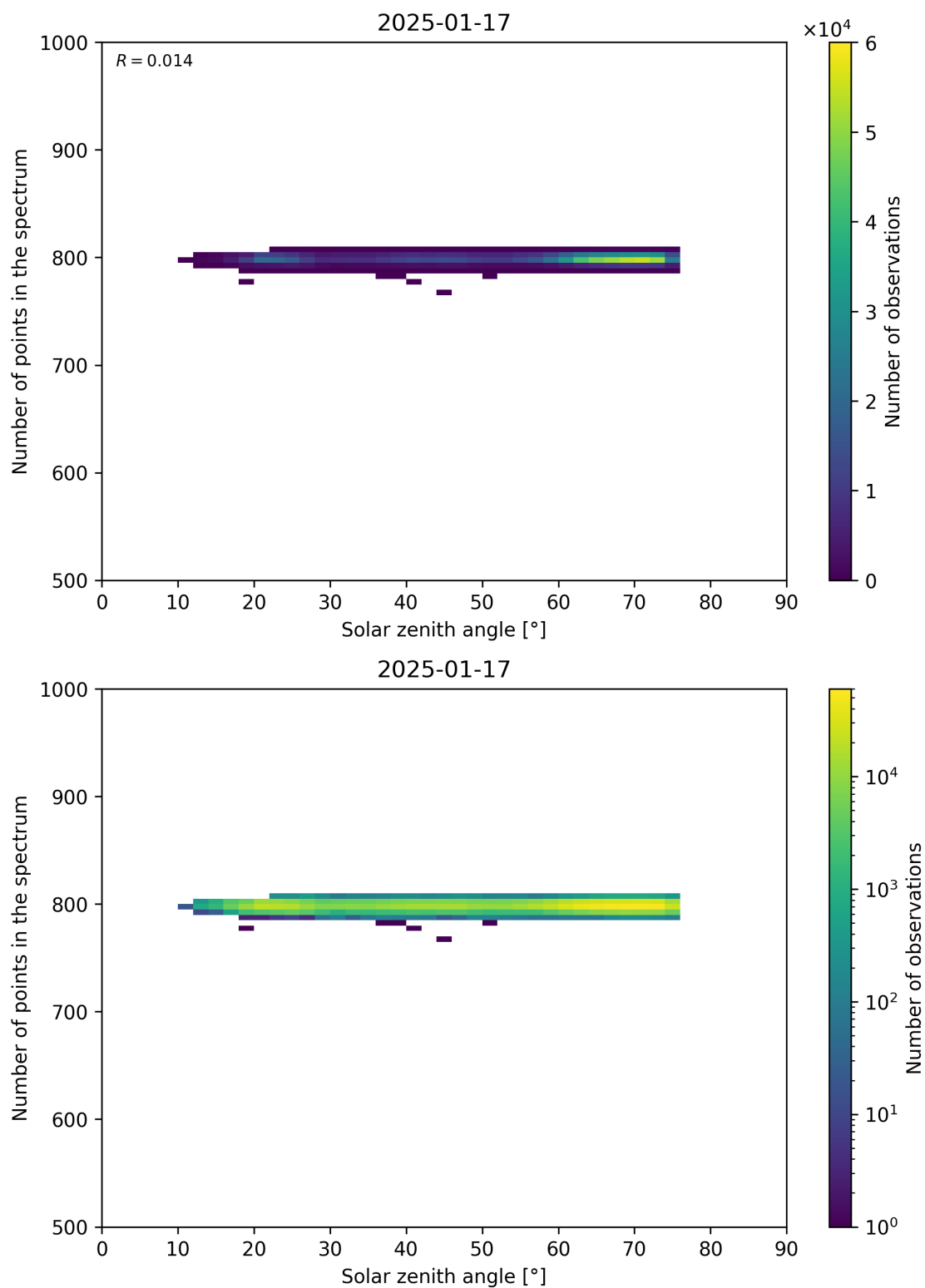
Figure 103: Scatter density plot of “Solar zenith angle” against “Number of points in the spectrum” for 2025-01-17 to 2025-01-18.
