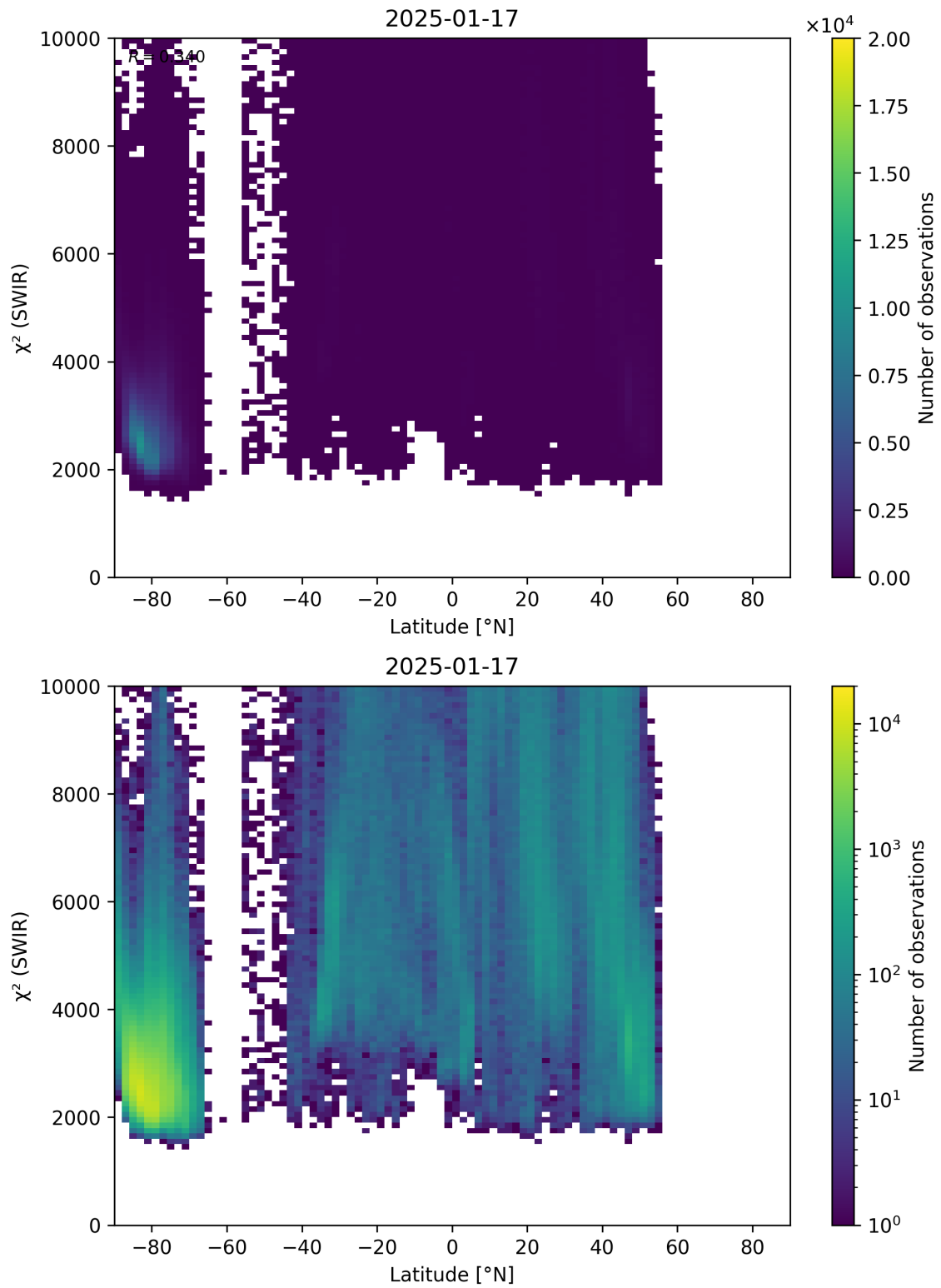
Figure 54: Scatter density plot of “Latitude” against “ \chi^2 (SWIR)” for 2025-01-17 to 2025-01-18.
