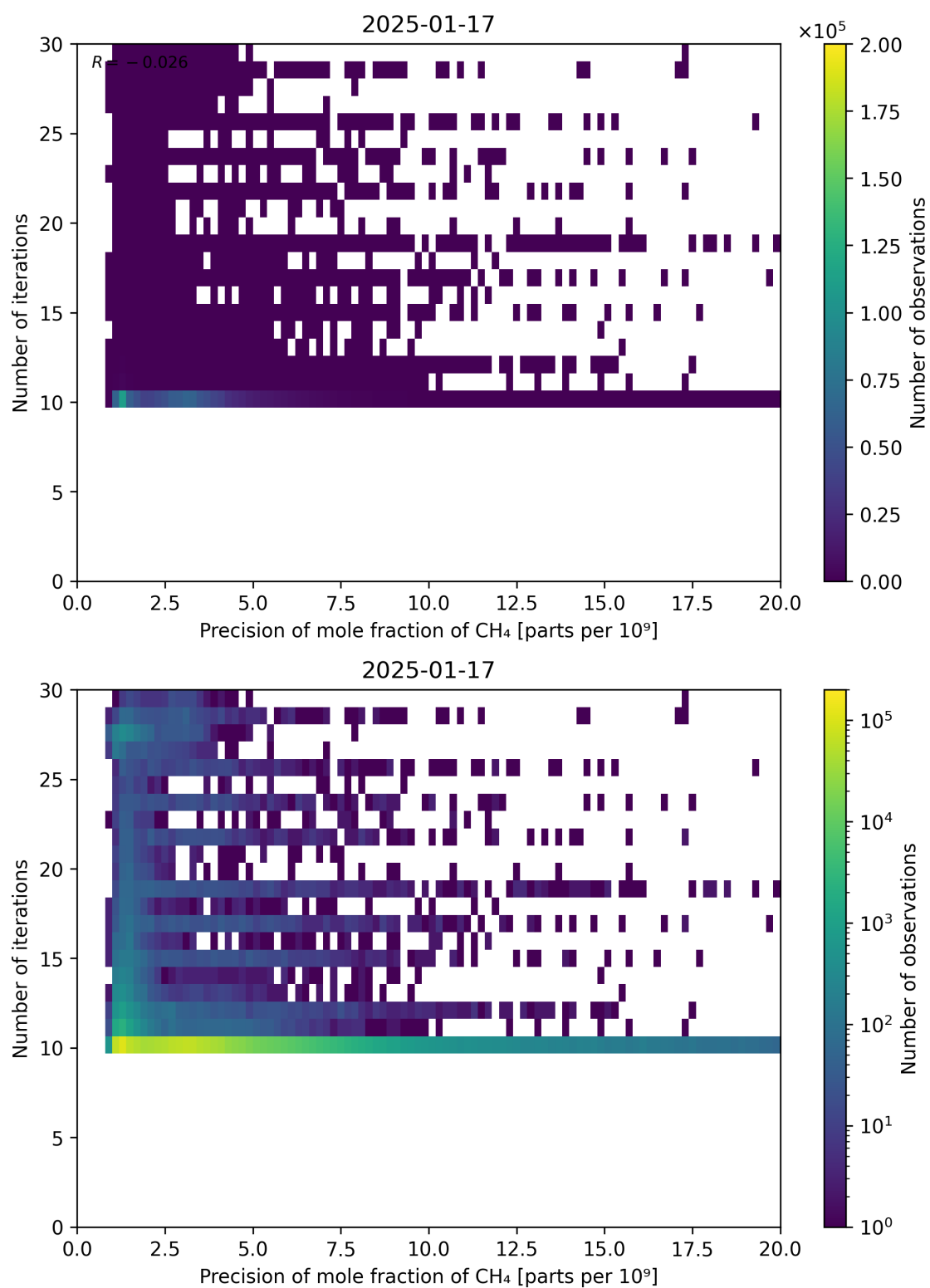
Figure 83: Scatter density plot of “Precision of mole fraction of CH 4 ” against “Number of iterations” for 2025-01-17 to 2025-01-18.
