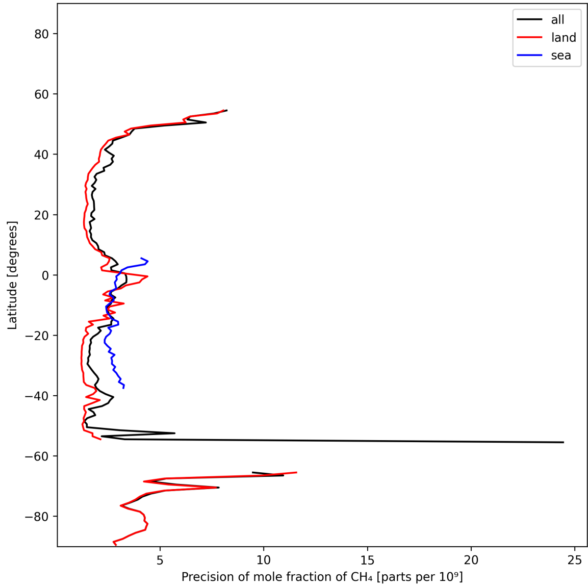
Figure 13: Zonal average of “Precision of mole fraction of CH 4 ” for 2025-01-17 to 2025-01-18.
