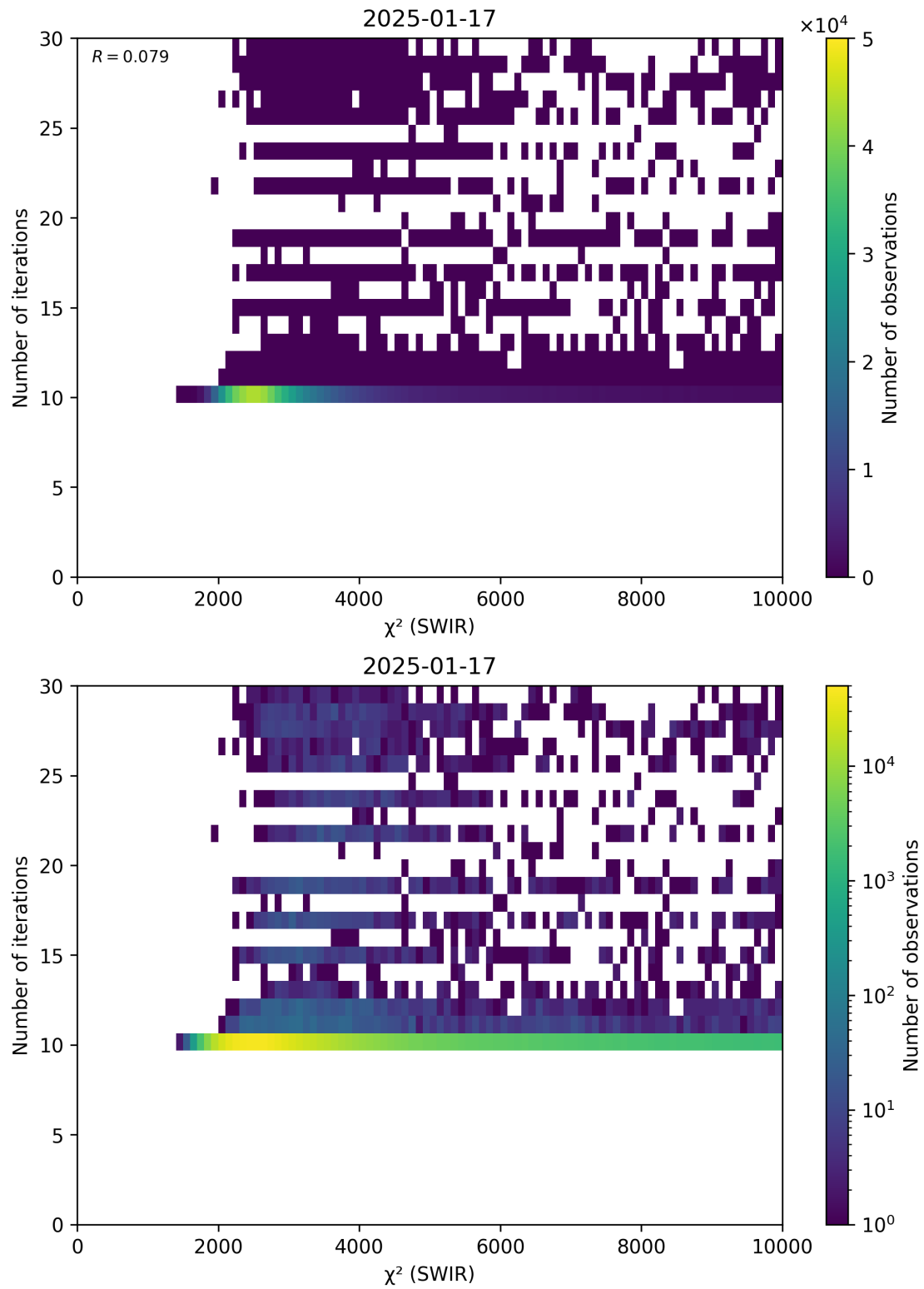
Figure 50: Scatter density plot of “ \chi^2 (SWIR)” against “Number of iterations” for 2025-01-17 to 2025-01-18.
