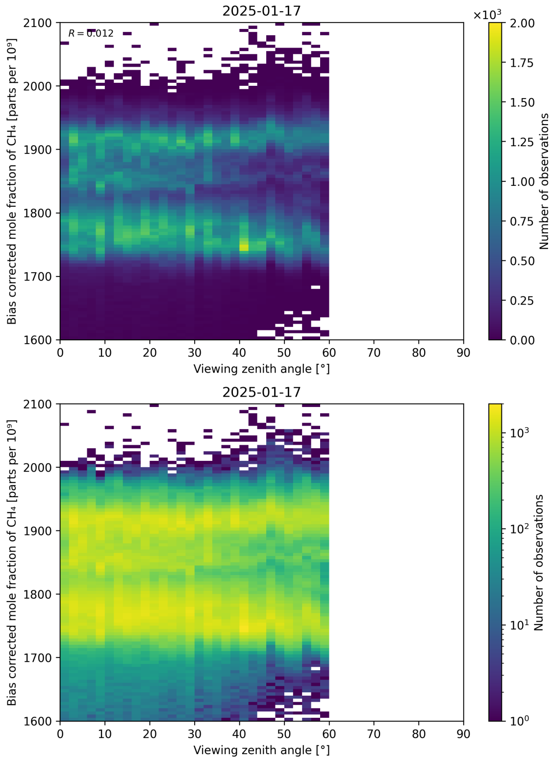
Figure 111: Scatter density plot of “Viewing zenith angle” against “Bias corrected mole fraction of CH 4 ” for 2025-01-17 to 2025-01-18.
