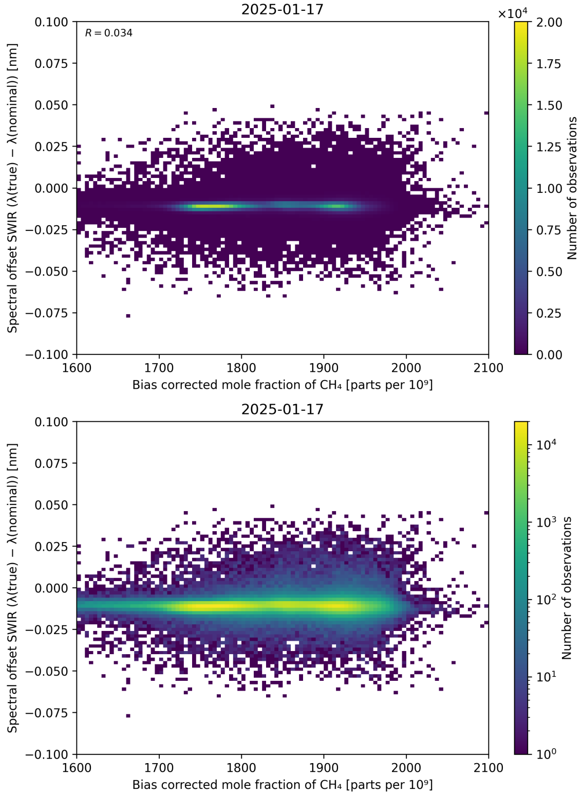
Figure 69: Scatter density plot of “Bias corrected mole fraction of \text{CH}_4 ” against “Spectral offset SWIR ( \lambda_{\text{true}} - \lambda_{\text{nominal}} )” for 2025-01-17 to 2025-01-18.
