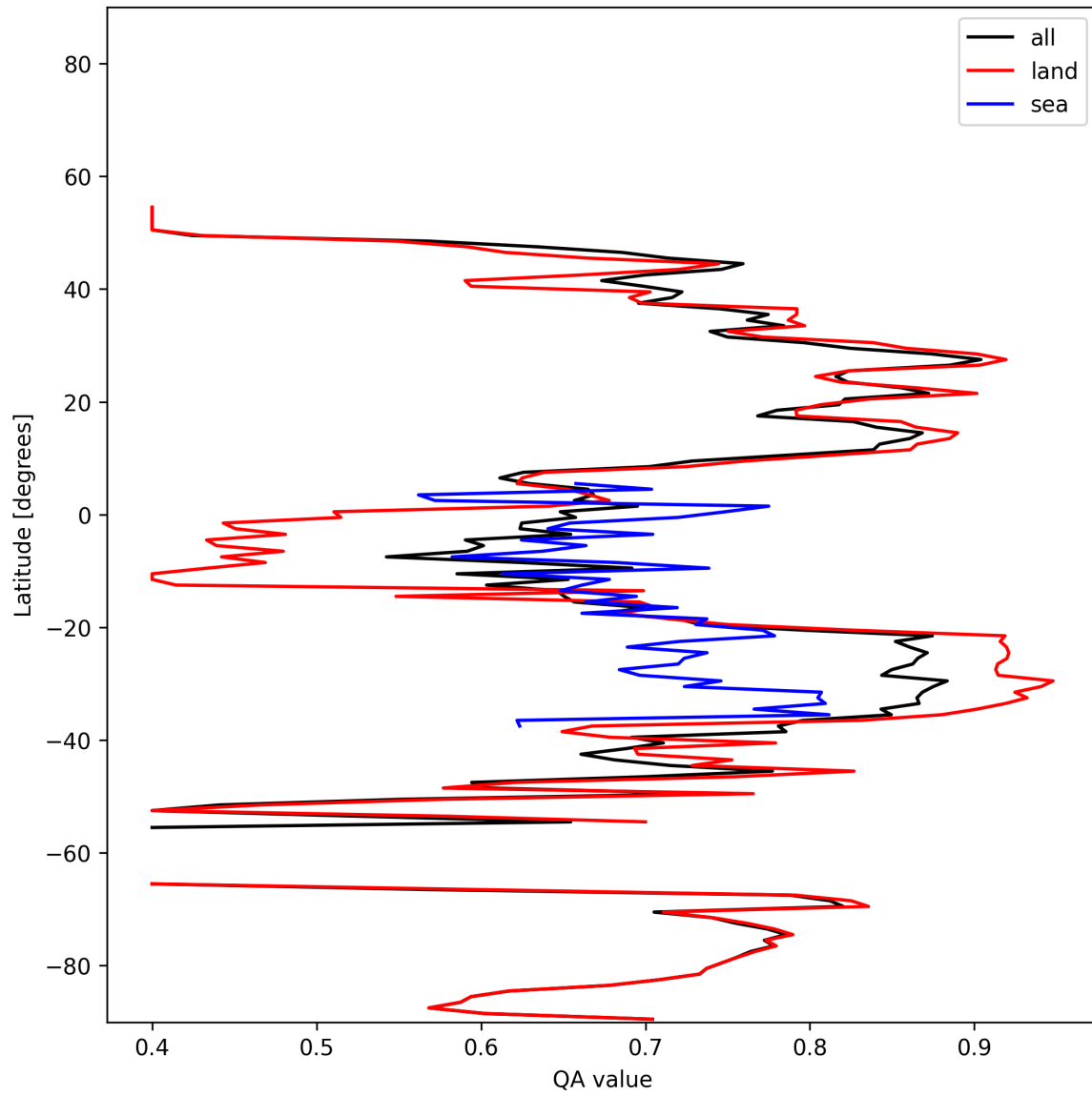
Figure 11: Zonal average of “QA value” for 2025-01-17 to 2025-01-18.
