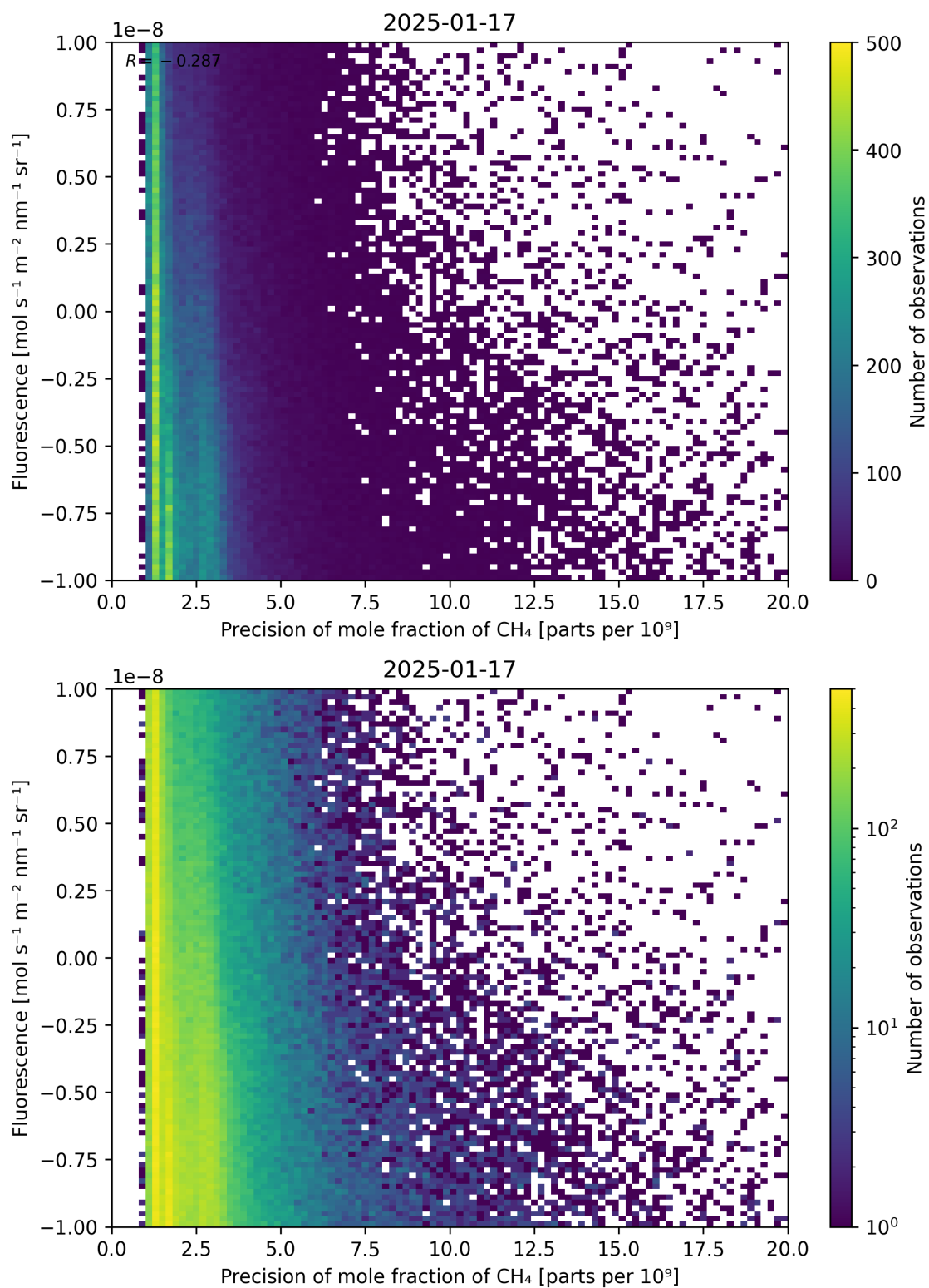
Figure 81: Scatter density plot of “Precision of mole fraction of CH 4 ” against “Fluorescence” for 2025-01-17 to 2025-01-18.
