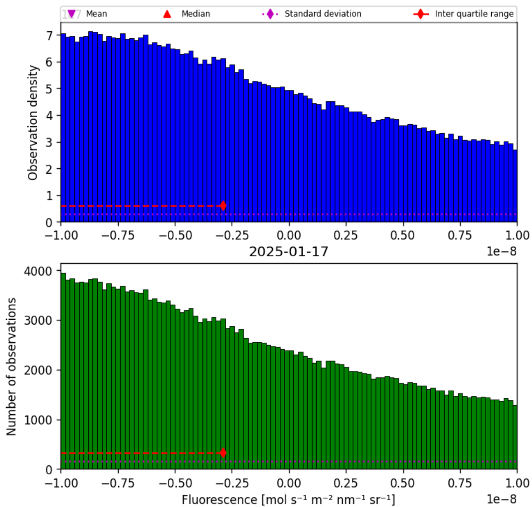
Figure 32: Histogram of “Fluorescence” for 2025-01-17 to 2025-01-18
