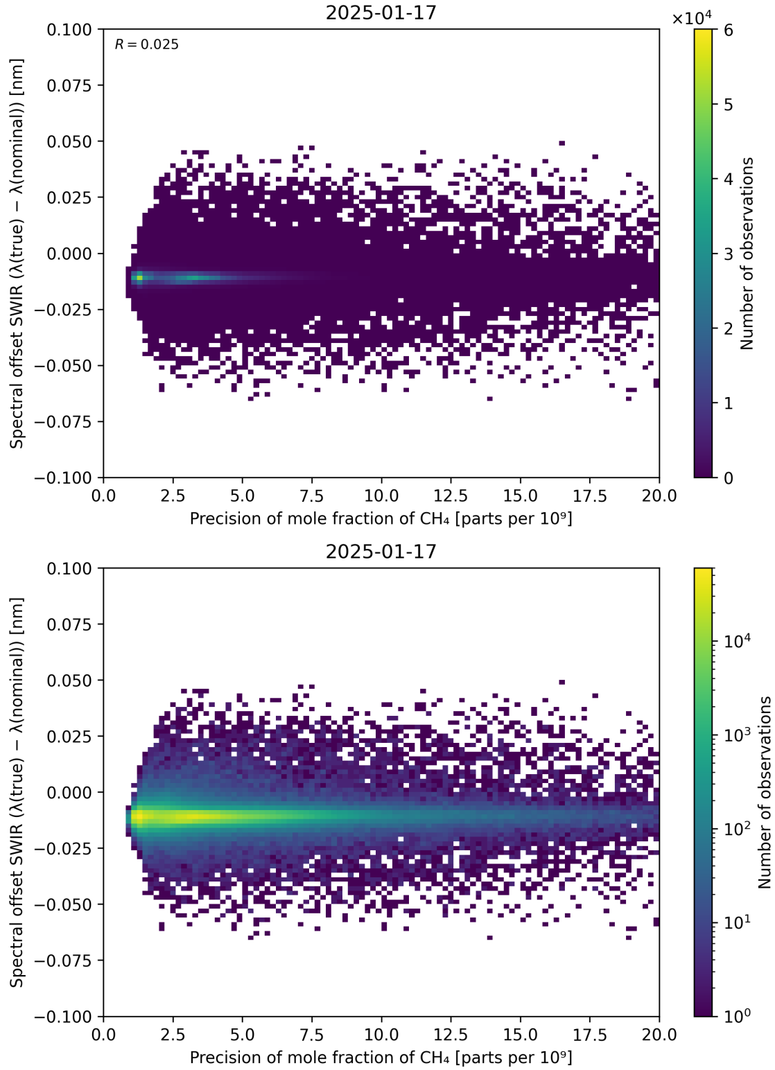
Figure 85: Scatter density plot of “Precision of mole fraction of \text{CH}_4 ” against “Spectral offset SWIR ( \lambda_{\text{true}} - \lambda_{\text{nominal}} )” for 2025-01-17 to 2025-01-18.
