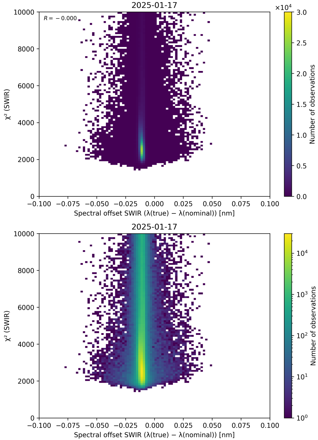
Figure 118: Scatter density plot of “Spectral offset SWIR ( \lambda_{\text{true}} - \lambda_{\text{nominal}} )” against “ \chi^2 (SWIR)” for 2025-01-17 to 2025-01-18.
