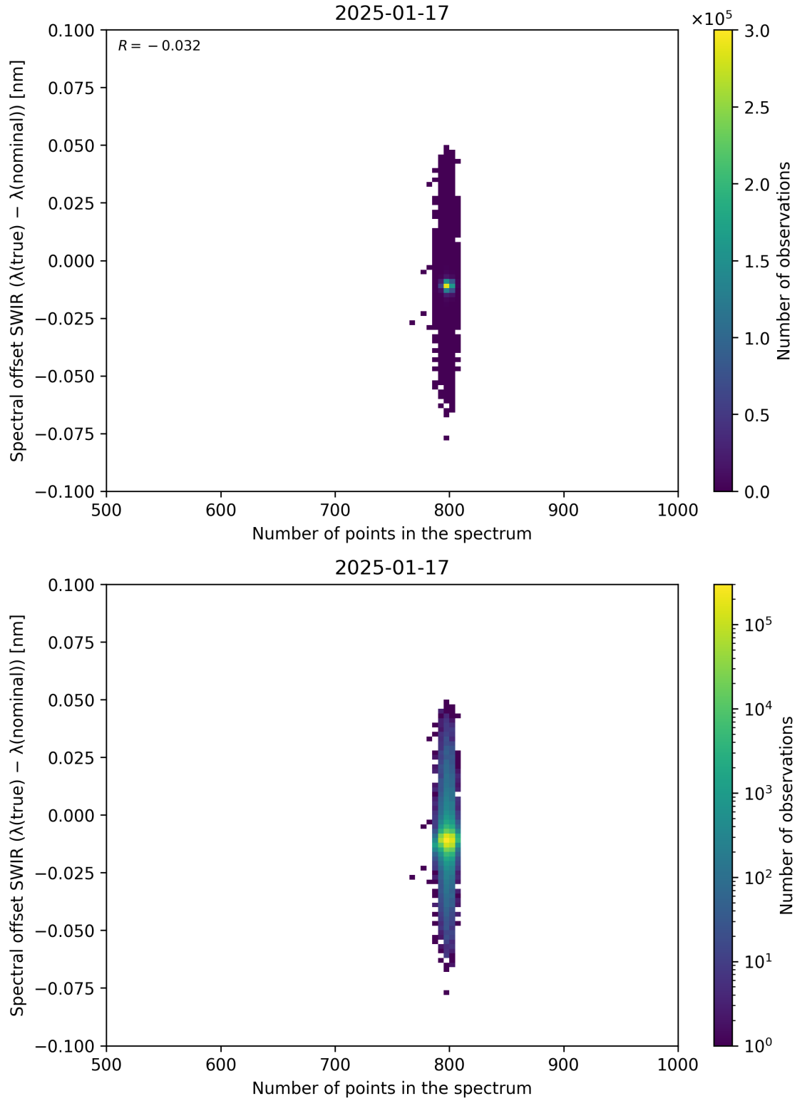
Figure 93: Scatter density plot of “Number of points in the spectrum” against “Spectral offset SWIR ( \lambda_{\text{true}} - \lambda_{\text{nominal}} )” for 2025-01-17 to 2025-01-18.
