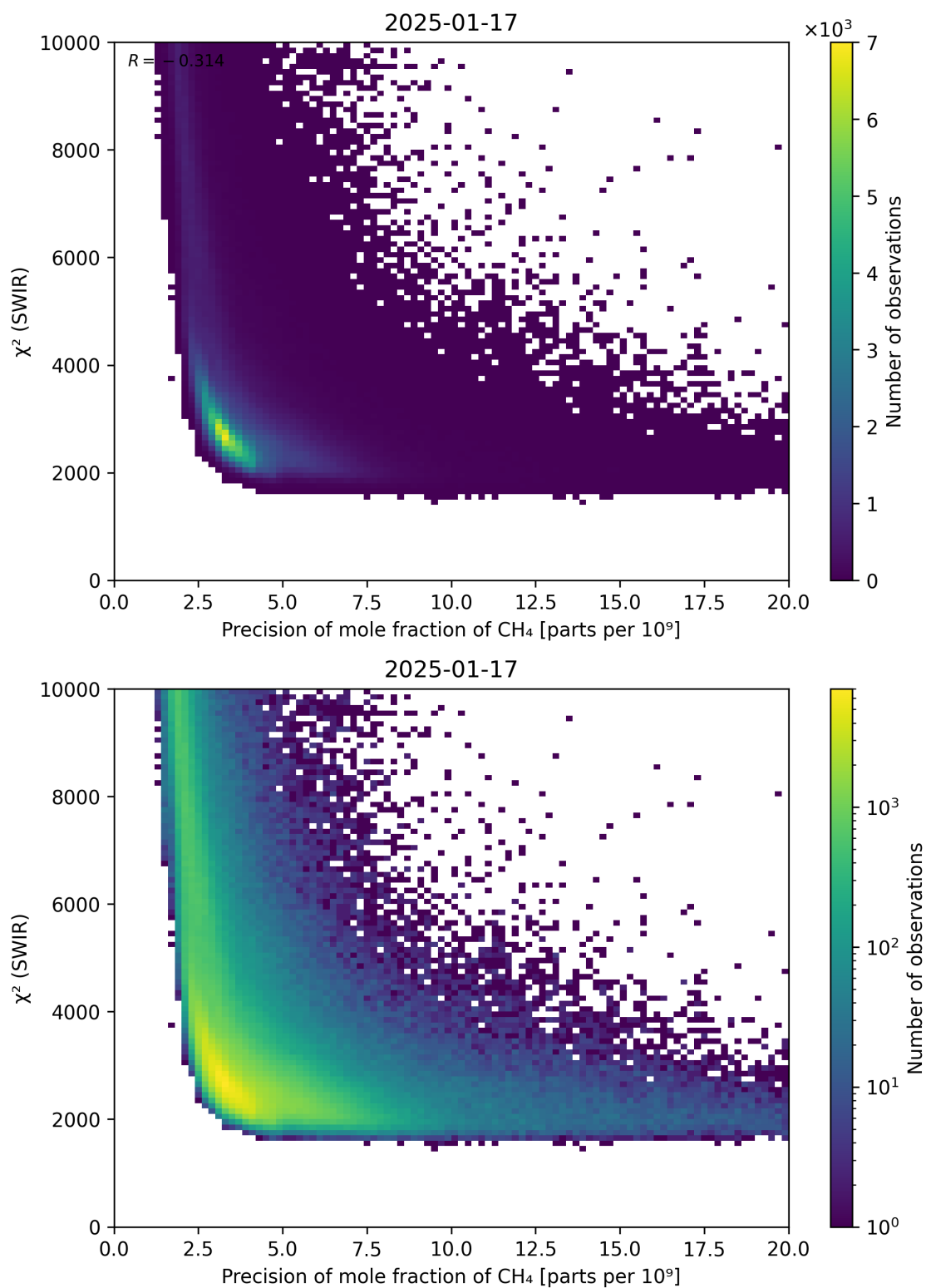
Figure 79: Scatter density plot of “Precision of mole fraction of \text{CH}_4 ” against “ \chi^2 (SWIR)” for 2025-01-17 to 2025-01-18.
