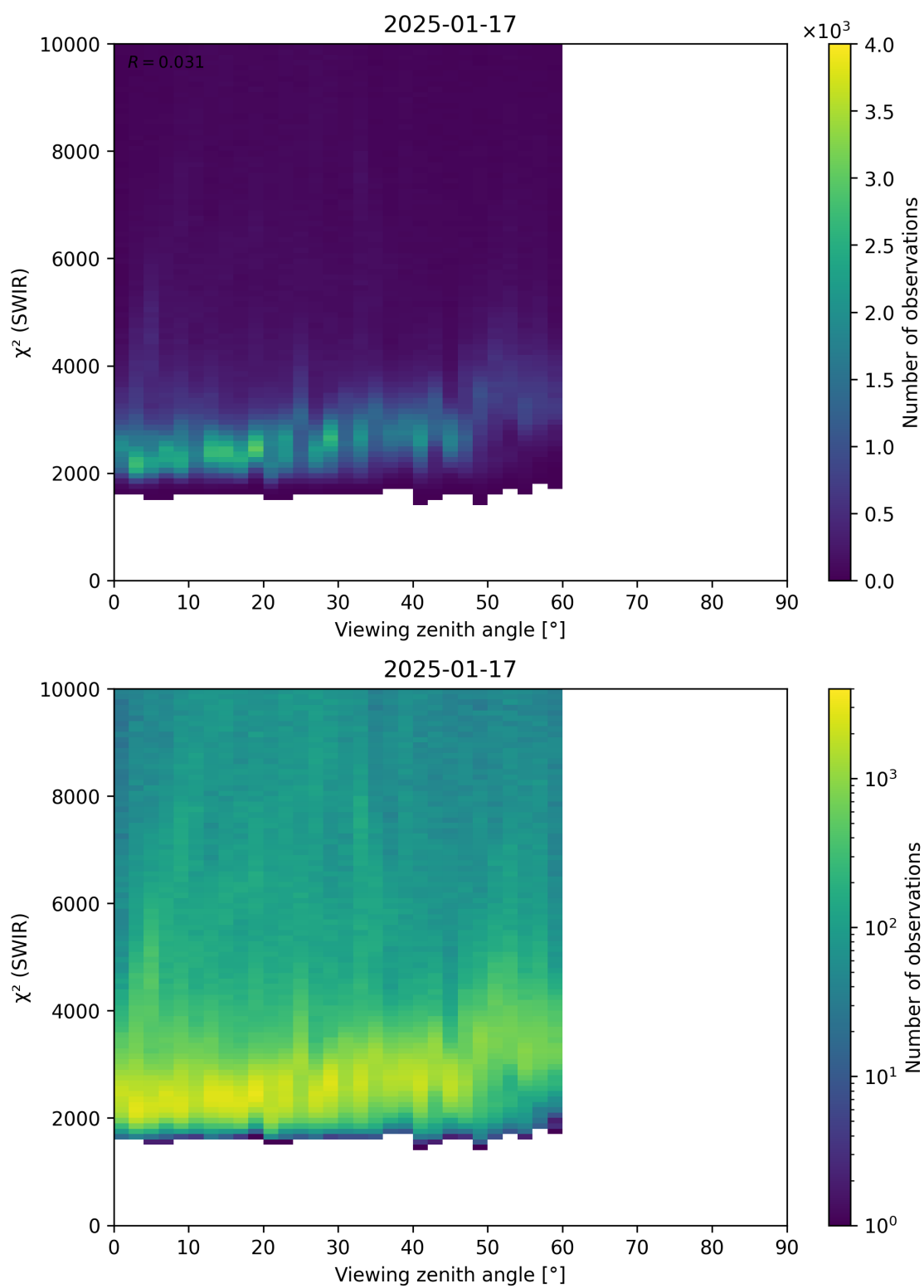
Figure 106: Scatter density plot of “Viewing zenith angle” against “ \chi^2 (SWIR)” for 2025-01-17 to 2025-01-18.
