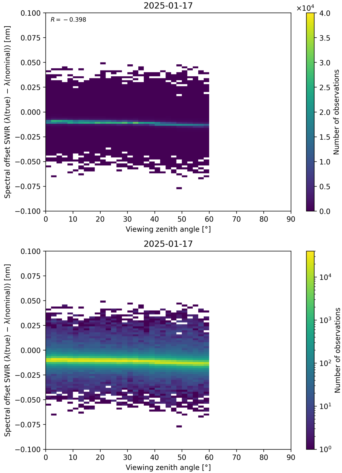
Figure 116: Scatter density plot of “Viewing zenith angle” against “Spectral offset SWIR ( \lambda_{\text{true}} - \lambda_{\text{nominal}} )” for 2025-01-17 to 2025-01-18.
