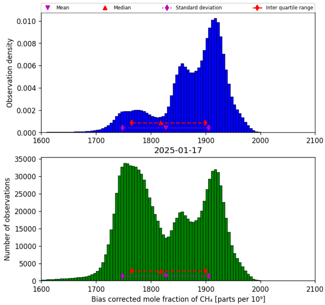
Figure 25: Histogram of “Bias corrected mole fraction of CH 4 ” for 2025-01-17 to 2025-01-18
