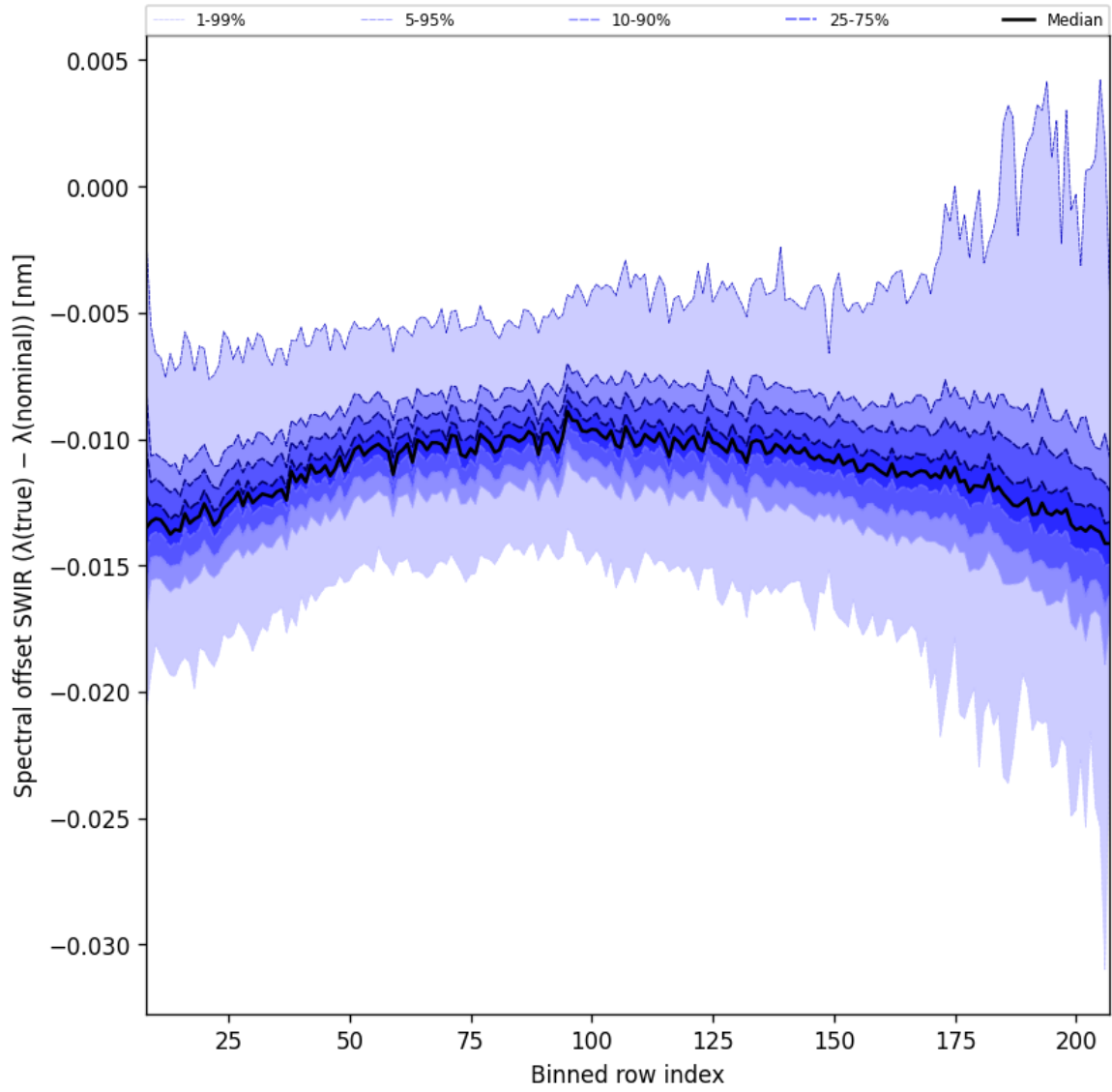
Figure 38: Along track statistics of “Spectral offset SWIR ( \lambda_{\text{true}} - \lambda_{\text{nominal}} )” for 2025-01-17 to 2025-01-18
