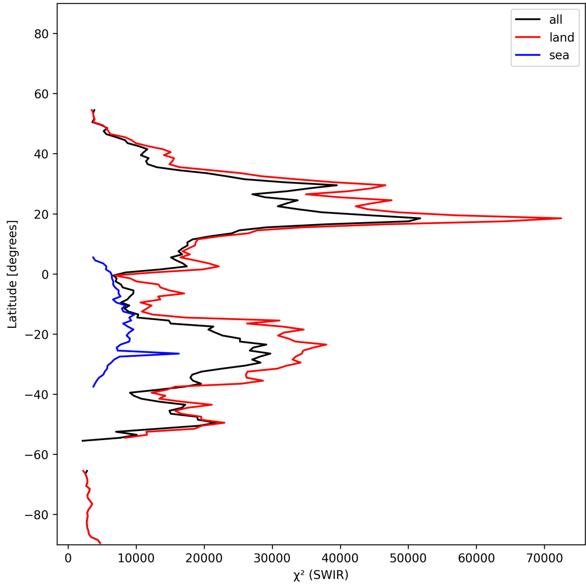
Figure 17: Zonal average of “ \chi^2 (SWIR)” for 2025-01-17 to 2025-01-18.
