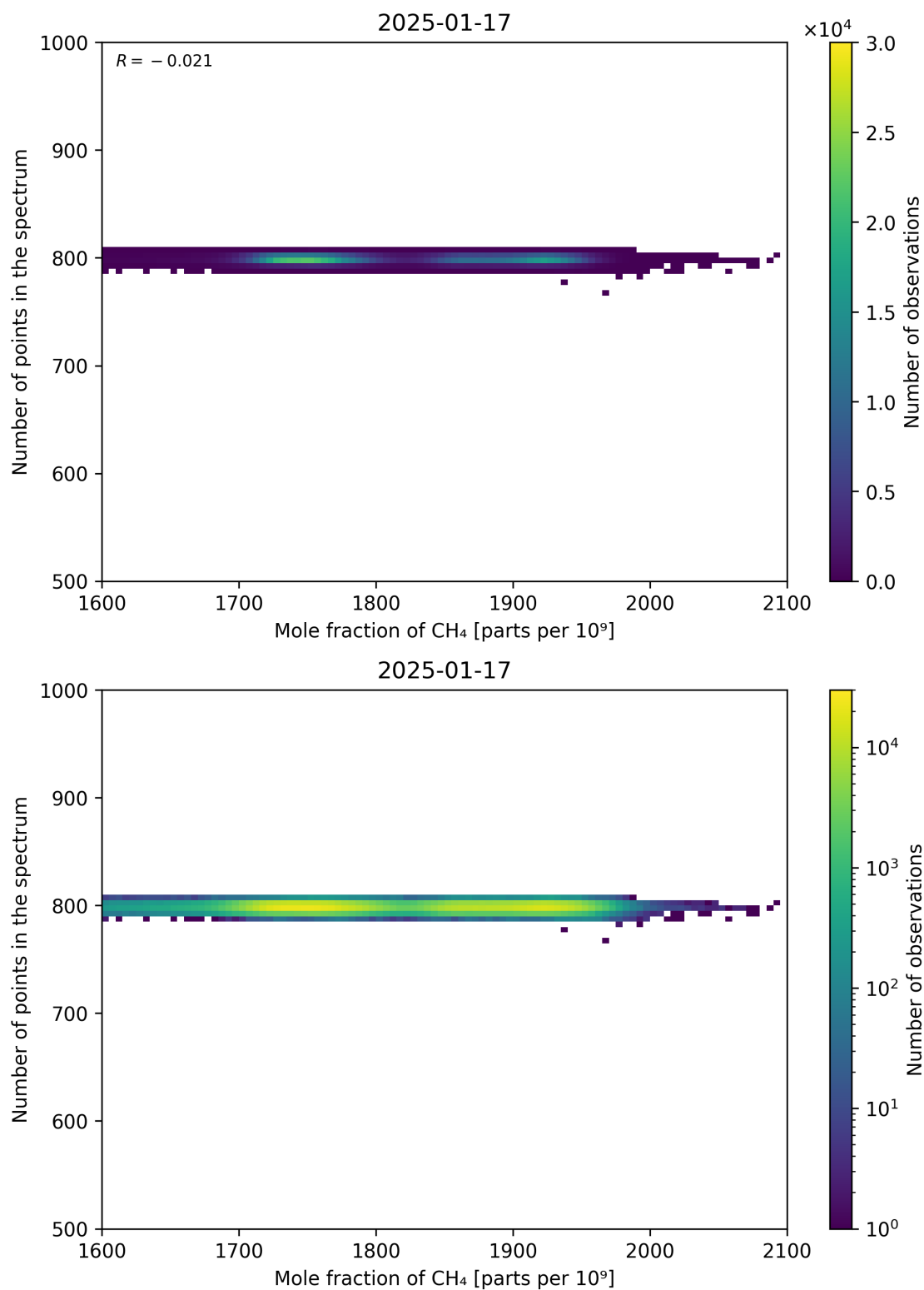
Figure 77: Scatter density plot of “Mole fraction of CH 4 ” against “Number of points in the spectrum” for 2025-01-17 to 2025-01-18.
