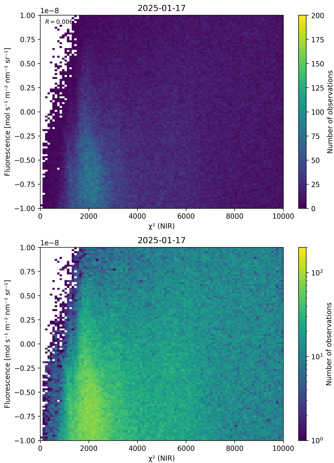
Figure 45: Scatter density plot of “ \chi^2 (NIR)” against “Fluorescence” for 2025-01-17 to 2025-01-18.
