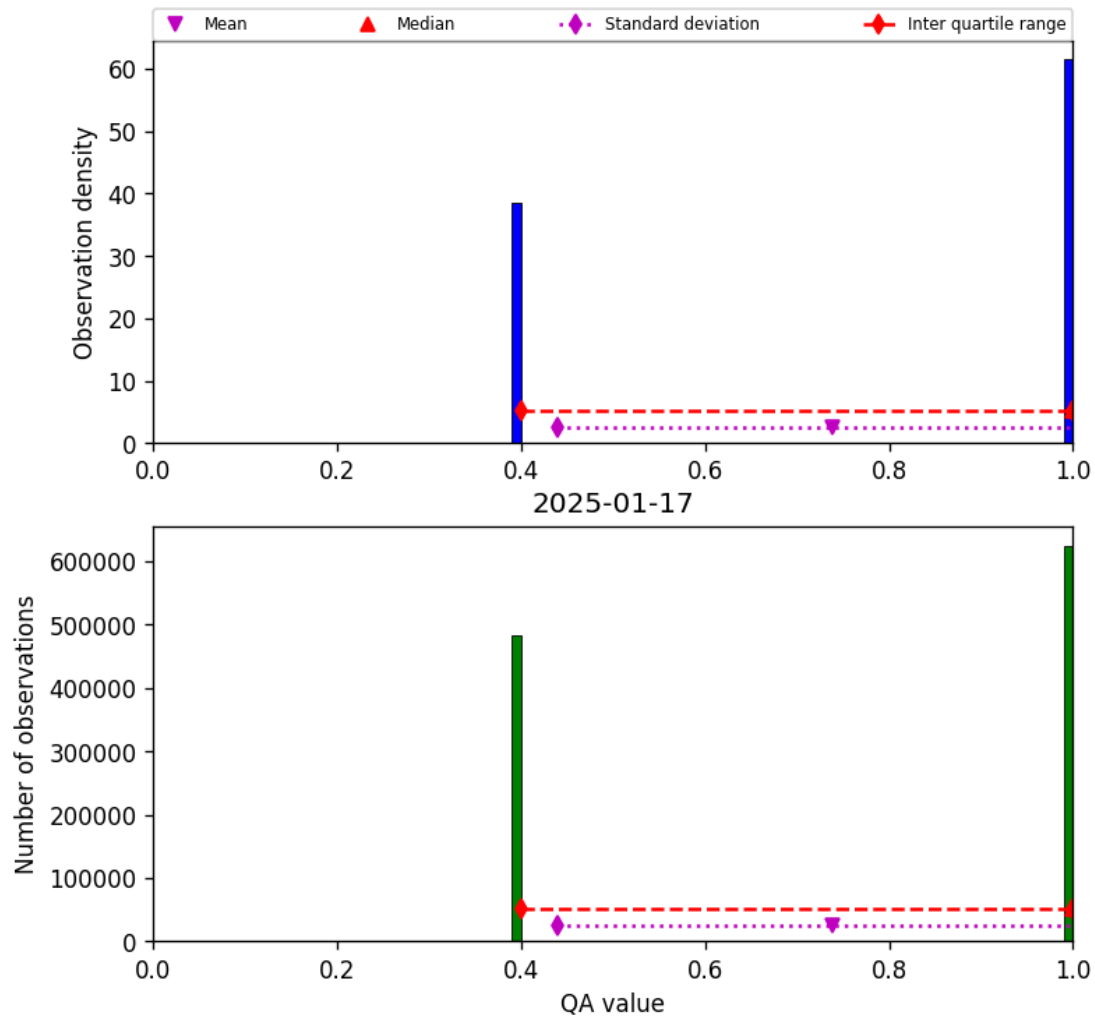
Figure 22: Histogram of “QA value” for 2025-01-17 to 2025-01-18
