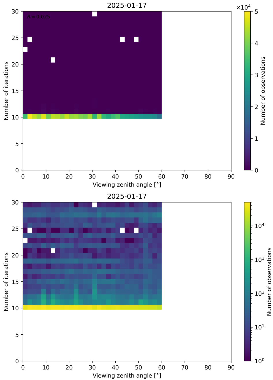
Figure 113: Scatter density plot of “Viewing zenith angle” against “Number of iterations” for 2025-01-17 to 2025-01-18.
