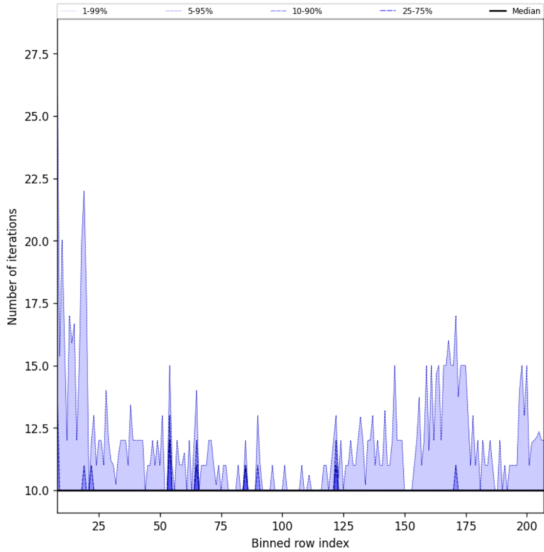
Figure 42: Along track statistics of “Number of iterations” for 2025-01-17 to 2025-01-18
