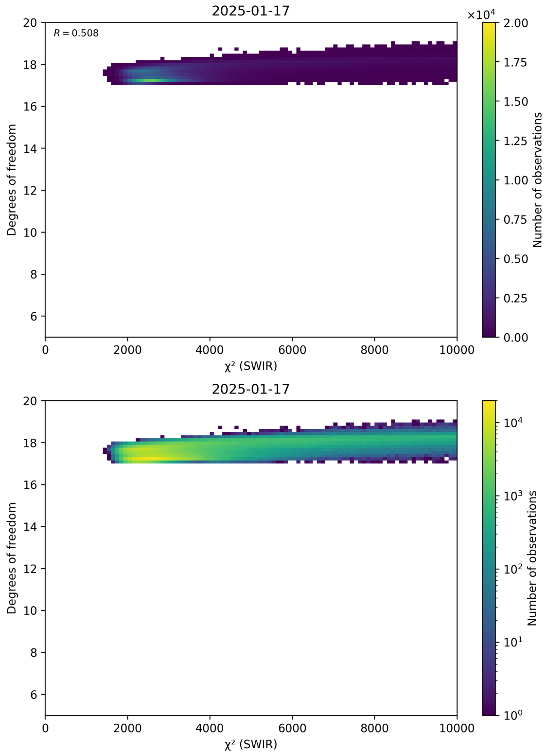
Figure 48: Scatter density plot of “ \chi^2 (SWIR)” against “Degrees of freedom” for 2025-01-17 to 2025-01-18.
