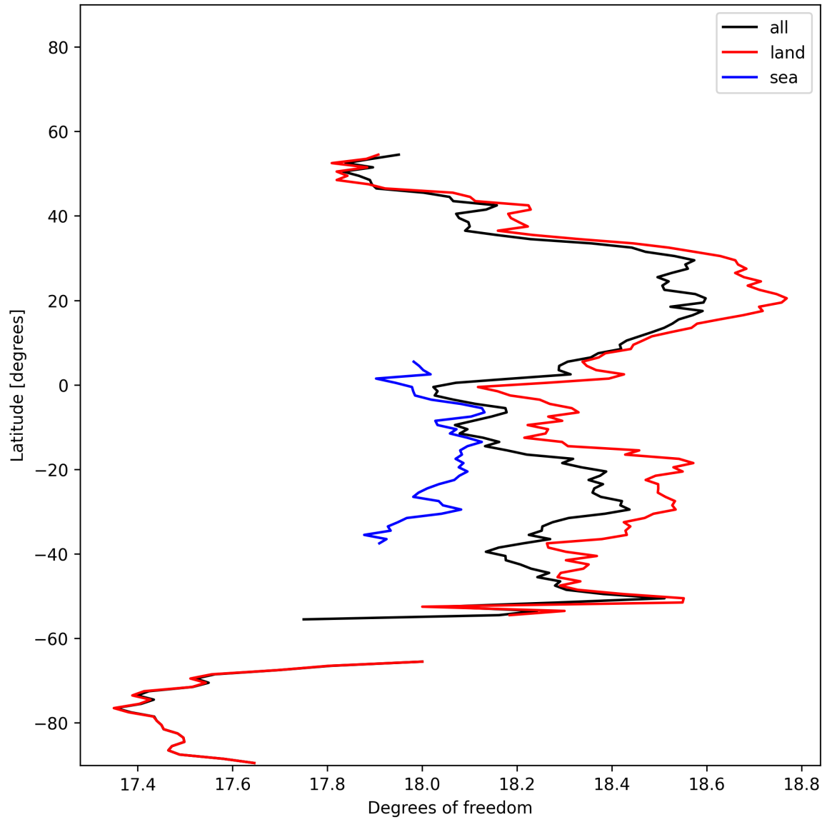
Figure 19: Zonal average of “Degrees of freedom” for 2025-01-17 to 2025-01-18.
