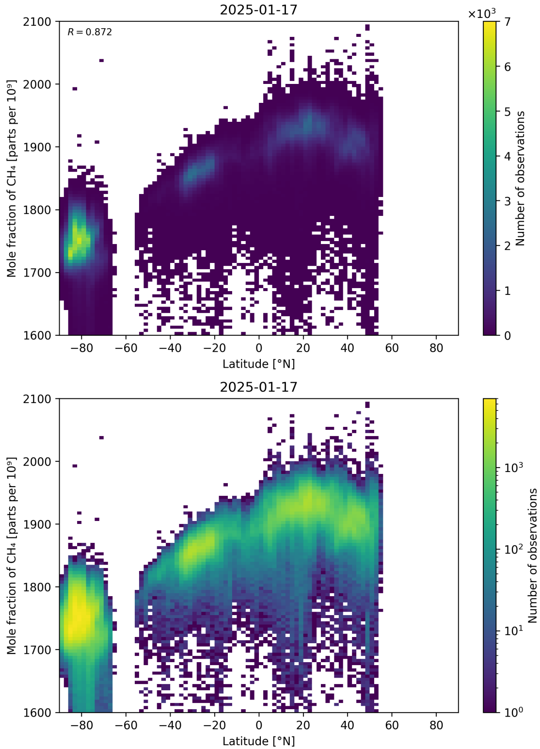
Figure 57: Scatter density plot of “Latitude” against “Mole fraction of CH 4 ” for 2025-01-17 to 2025-01-18.
