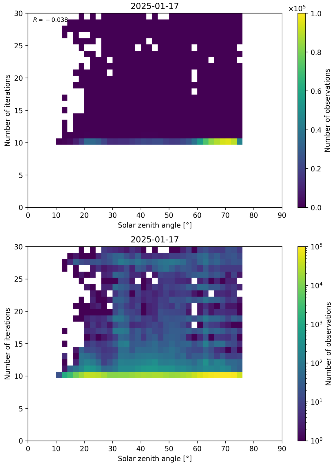
Figure 102: Scatter density plot of “Solar zenith angle” against “Number of iterations” for 2025-01-17 to 2025-01-18.
