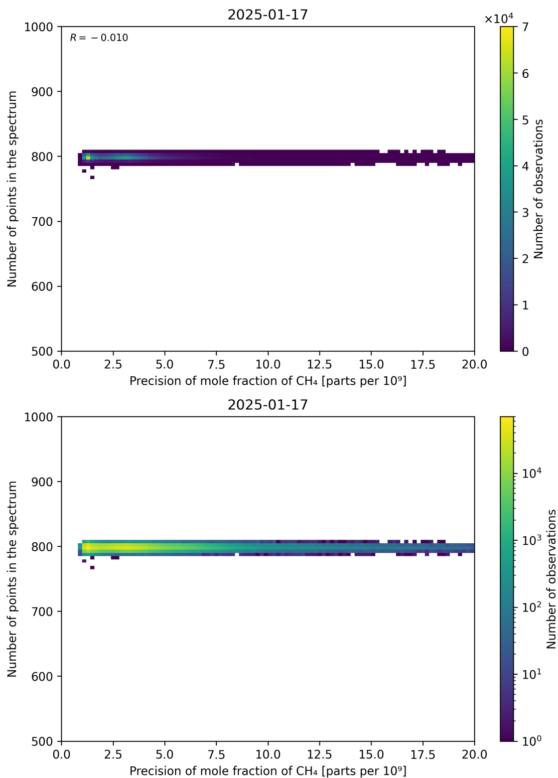
Figure 84: Scatter density plot of “Precision of mole fraction of CH 4 ” against “Number of points in the spectrum” for 2025-01-17 to 2025-01-18.
