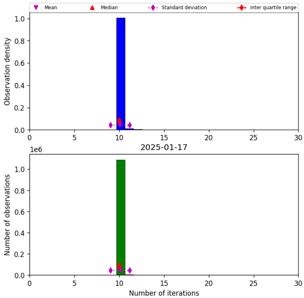
Figure 31: Histogram of “Number of iterations” for 2025-01-17 to 2025-01-18
