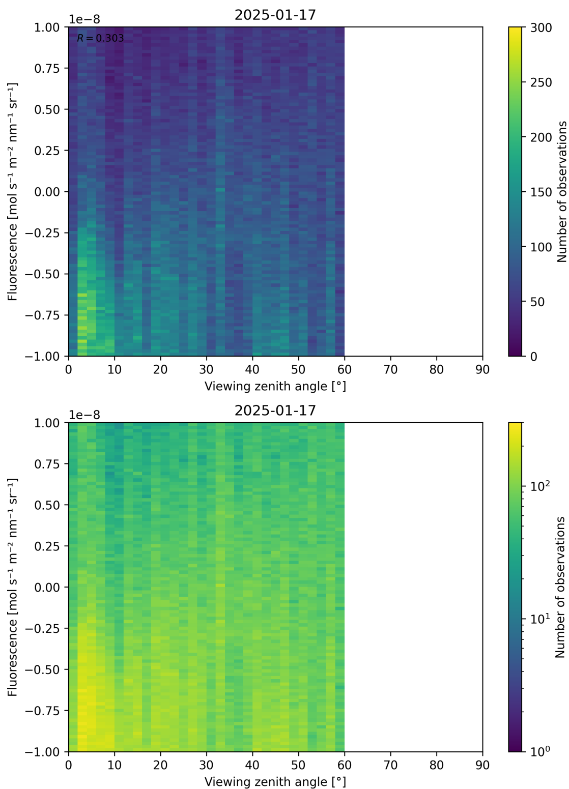
Figure 108: Scatter density plot of “Viewing zenith angle” against “Fluorescence” for 2025-01-17 to 2025-01-18.
