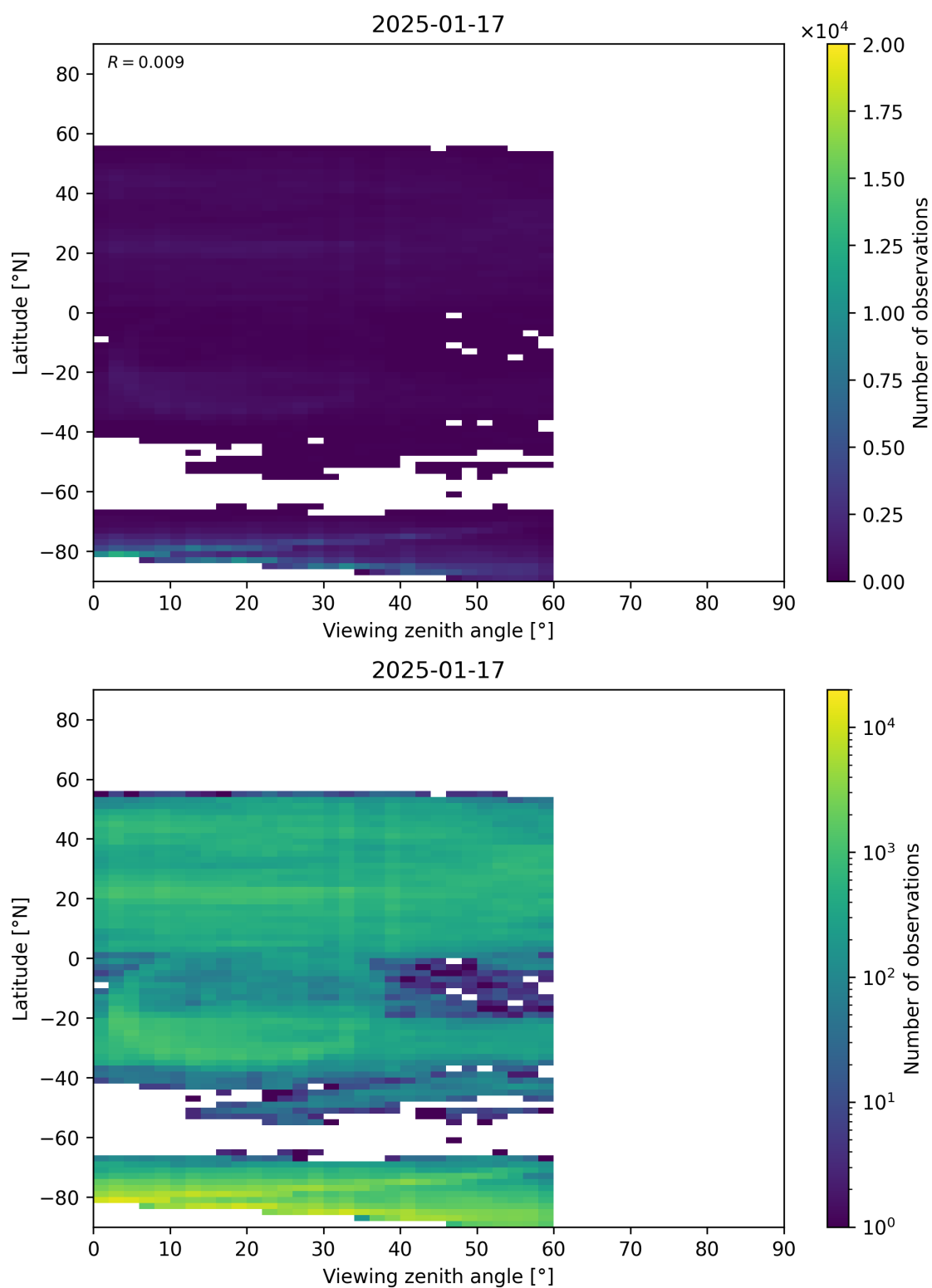
Figure 109: Scatter density plot of “Viewing zenith angle” against “Latitude” for 2025-01-17 to 2025-01-18.
