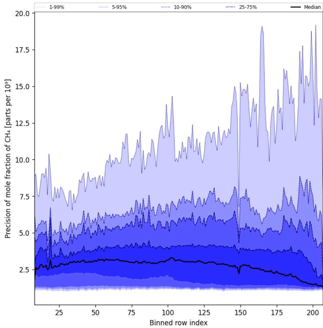
Figure 35: Along track statistics of “Precision of mole fraction of CH 4 ” for 2025-01-17 to 2025-01-18
