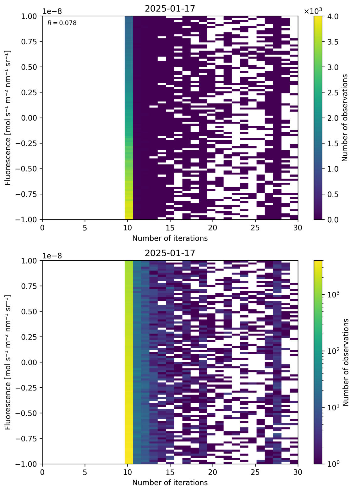
Figure 87: Scatter density plot of “Number of iterations” against “Fluorescence” for 2025-01-17 to 2025-01-18.
