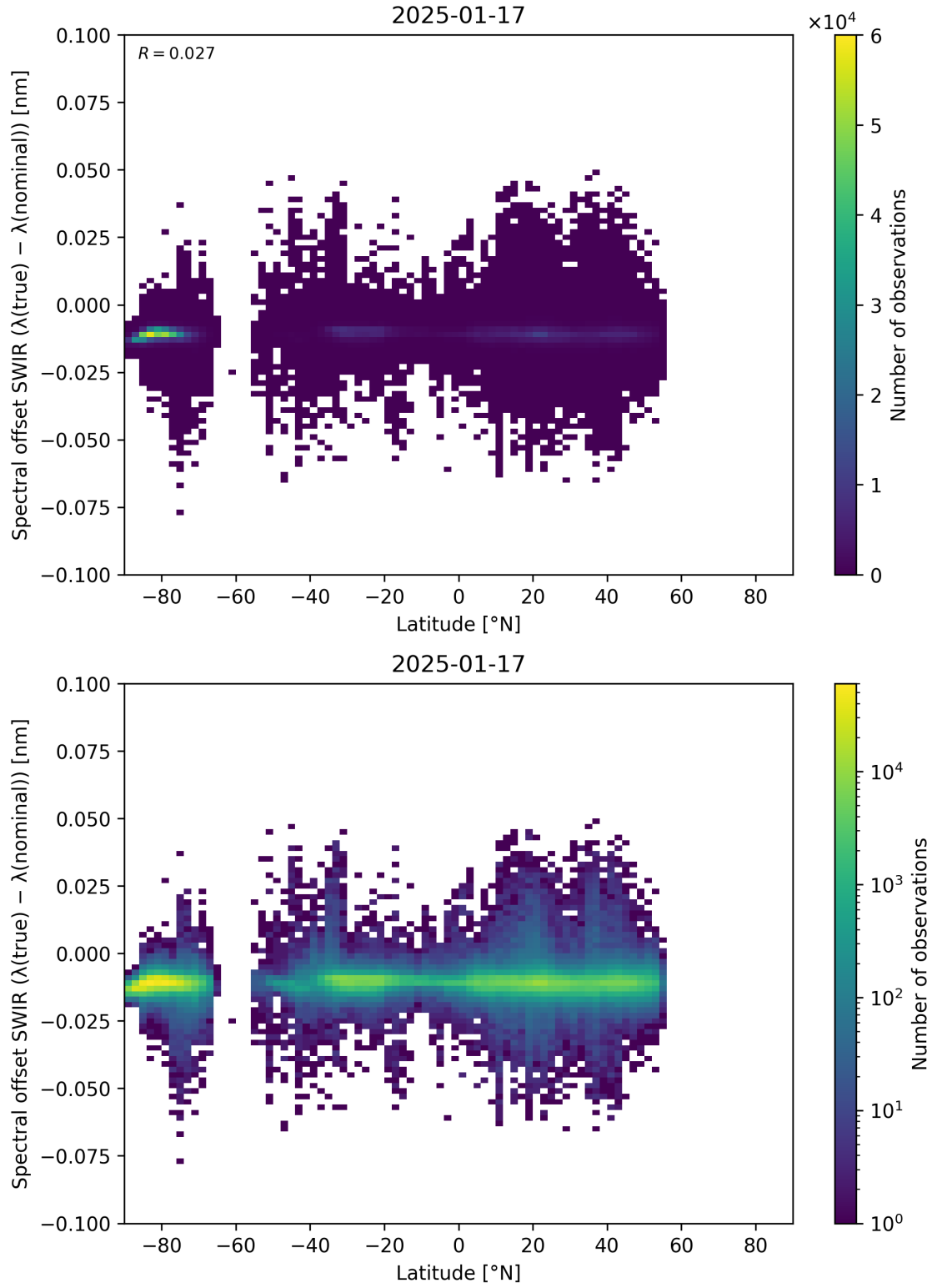
Figure 62: Scatter density plot of “Latitude” against “Spectral offset SWIR ( \lambda_{\text{true}} - \lambda_{\text{nominal}} )” for 2025-01-17 to 2025-01-18.
