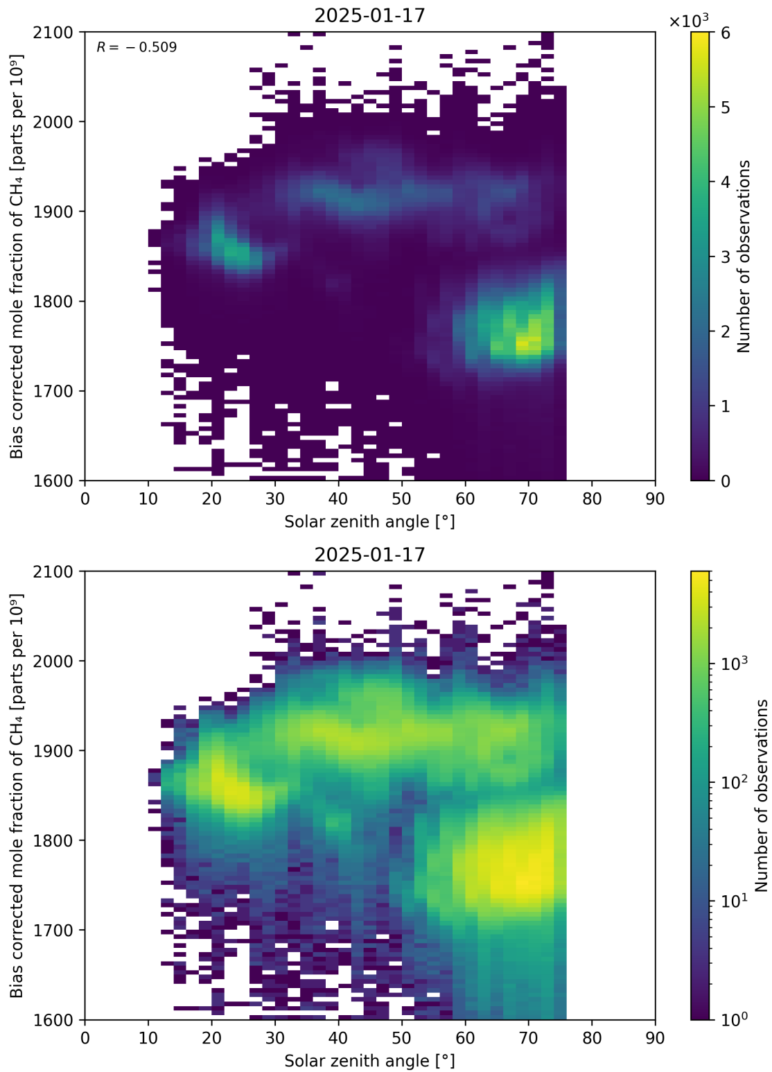
Figure 100: Scatter density plot of “Solar zenith angle” against “Bias corrected mole fraction of CH 4 ” for 2025-01-17 to 2025-01-18.
