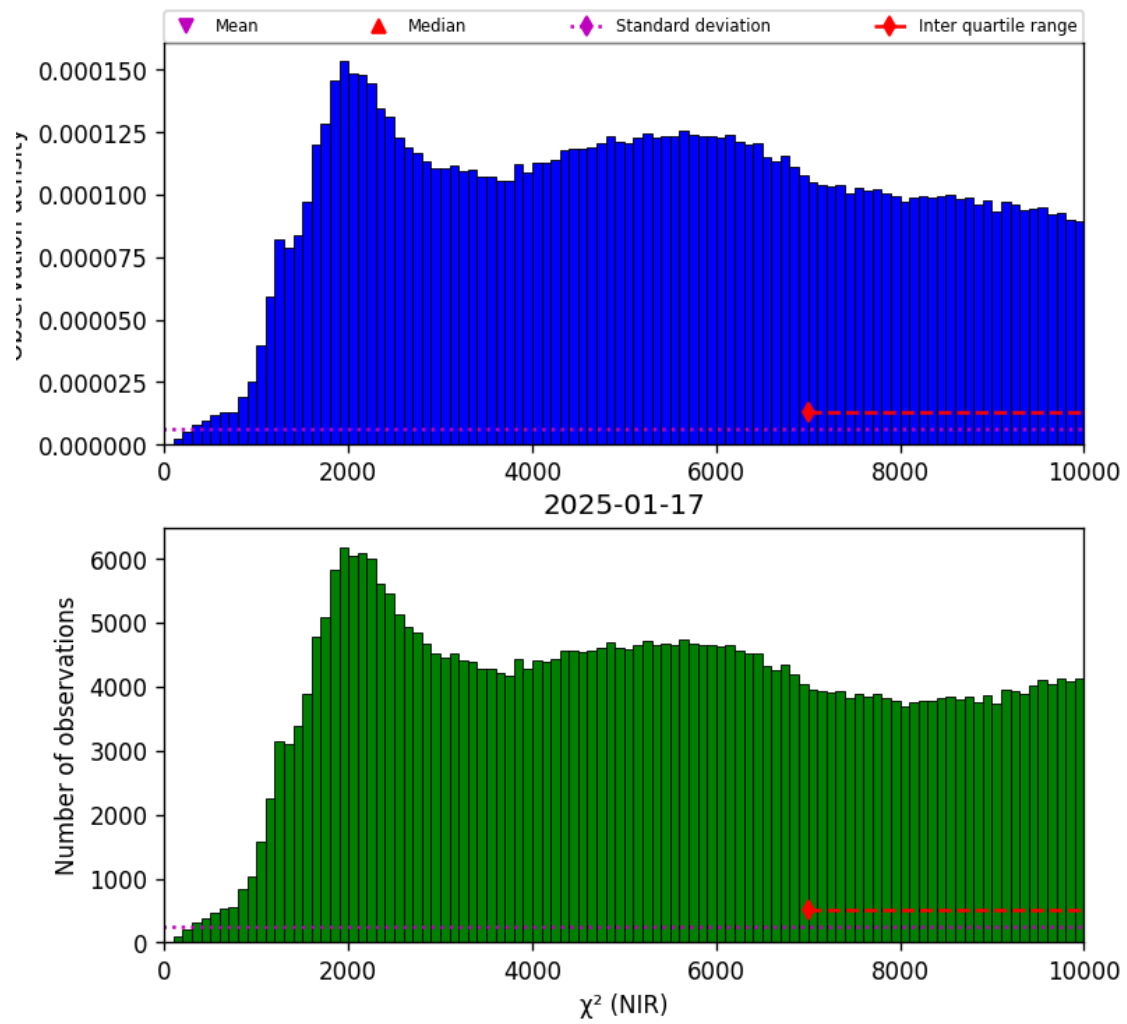
Figure 29: Histogram of “ \chi^2 (NIR)” for 2025-01-17 to 2025-01-18
