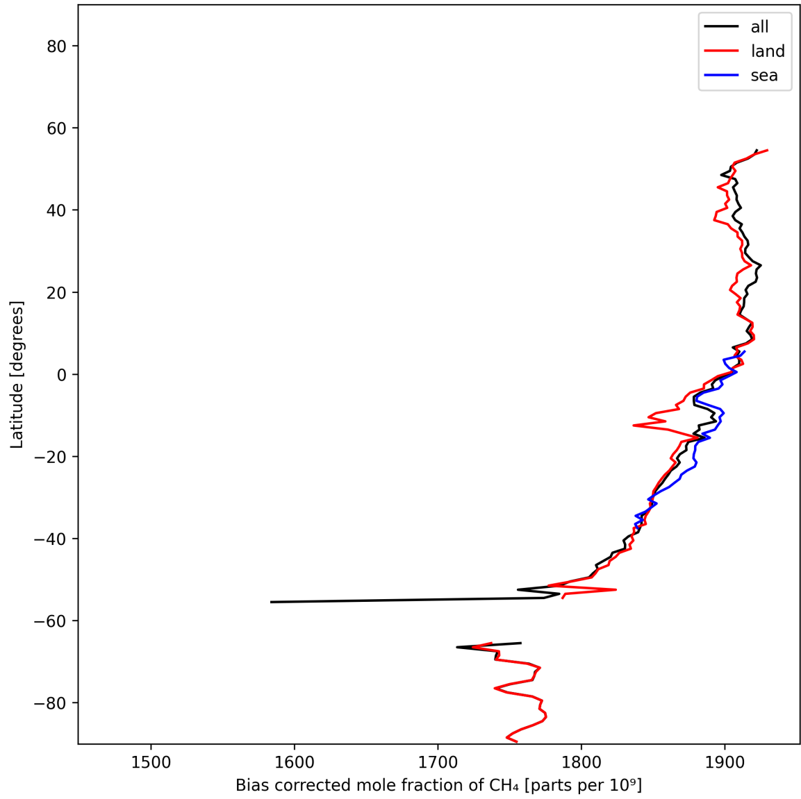
Figure 14: Zonal average of “Bias corrected mole fraction of CH 4 ” for 2025-01-17 to 2025-01-18.
