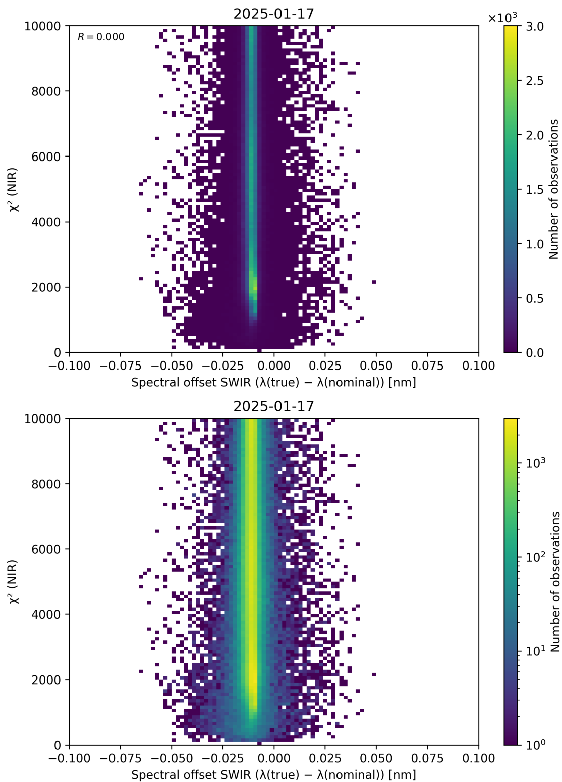
Figure 117: Scatter density plot of “Spectral offset SWIR ( \lambda_{\text{true}} - \lambda_{\text{nominal}} )” against “ \chi^2 (NIR)” for 2025-01-17 to 2025-01-18.
