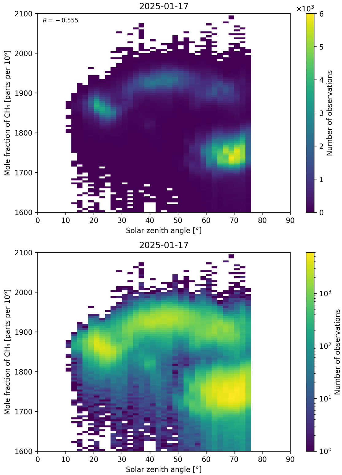
Figure 99: Scatter density plot of “Solar zenith angle” against “Mole fraction of CH 4 ” for 2025-01-17 to 2025-01-18.
