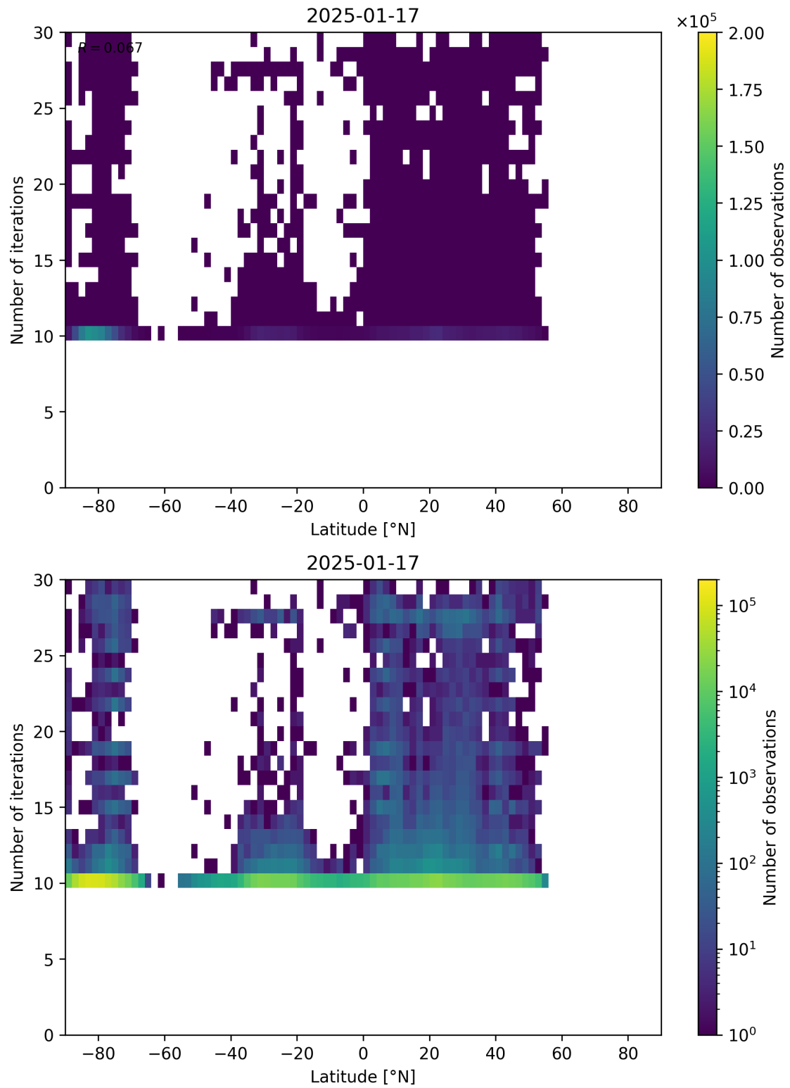
Figure 60: Scatter density plot of “Latitude” against “Number of iterations” for 2025-01-17 to 2025-01-18.
