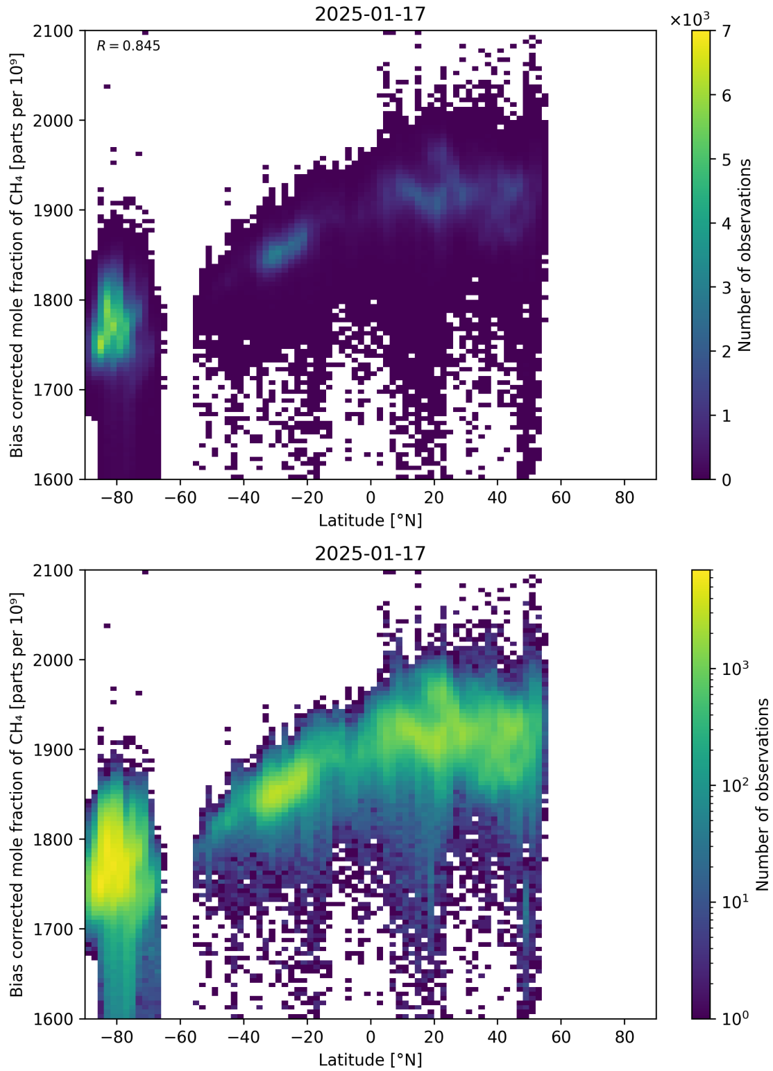
Figure 58: Scatter density plot of “Latitude” against “Bias corrected mole fraction of CH 4 ” for 2025-01-17 to 2025-01-18.
