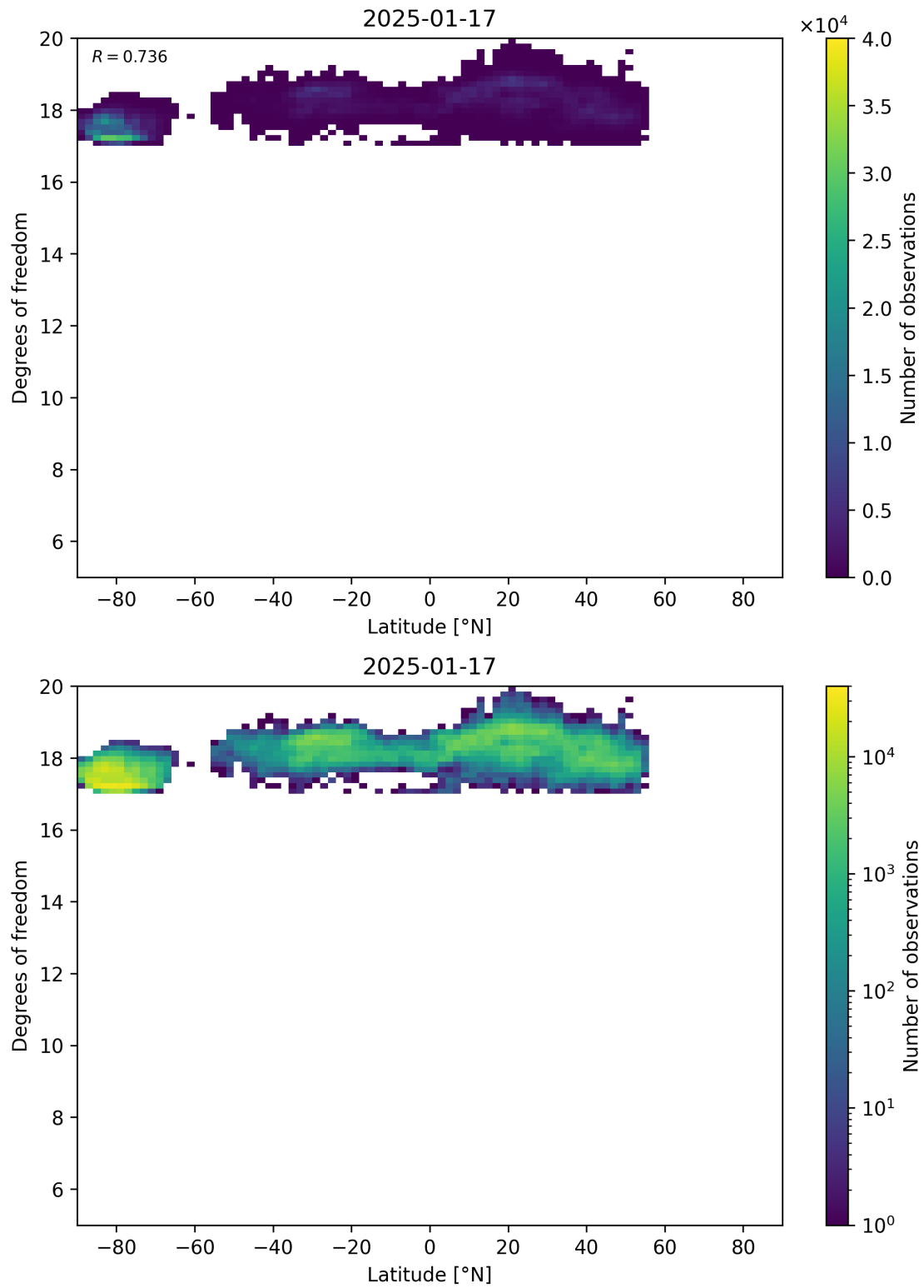
Figure 55: Scatter density plot of “Latitude” against “Degrees of freedom” for 2025-01-17 to 2025-01-18.
