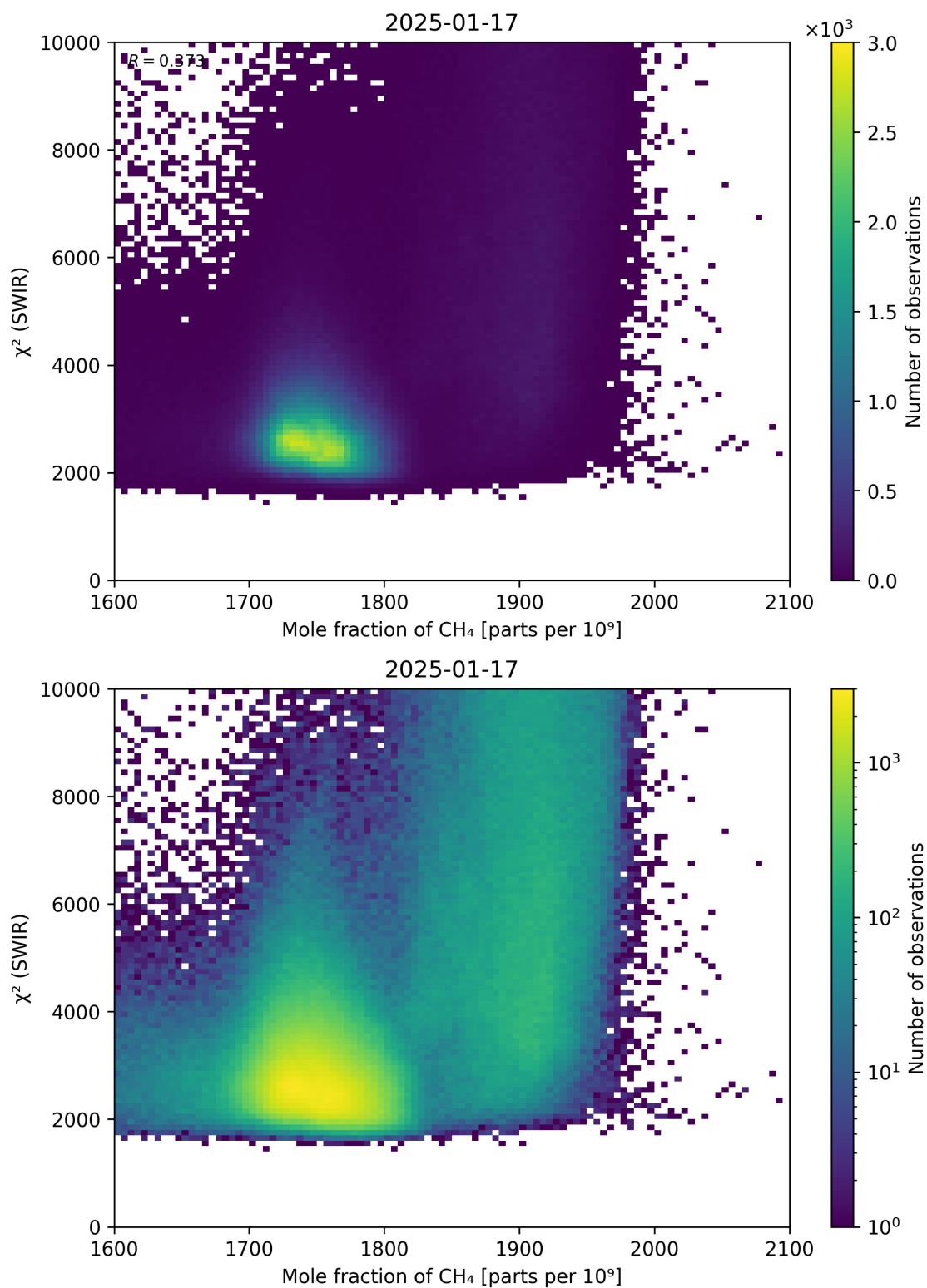
Figure 71: Scatter density plot of “Mole fraction of \text{CH}_4 ” against “ \chi^2 (SWIR)” for 2025-01-17 to 2025-01-18.
