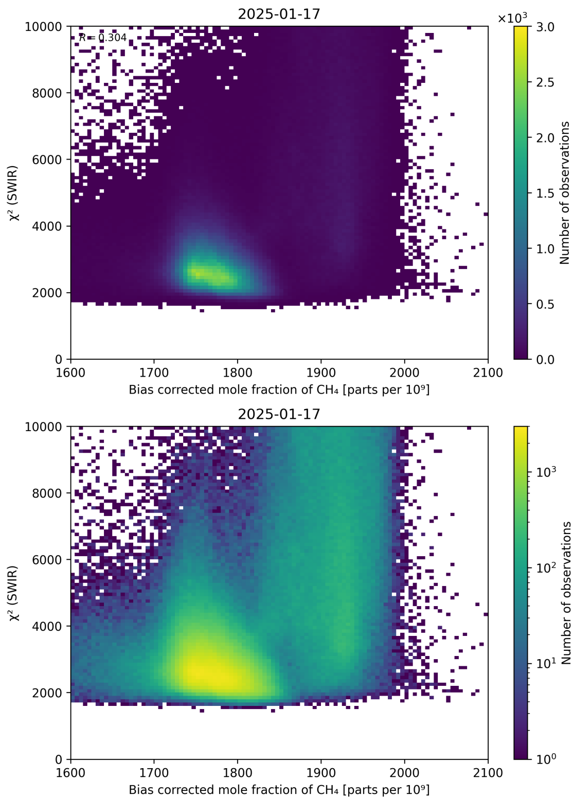
Figure 64: Scatter density plot of “Bias corrected mole fraction of \text{CH}_4 ” against “ \chi^2 (SWIR)” for 2025-01-17 to 2025-01-18.
