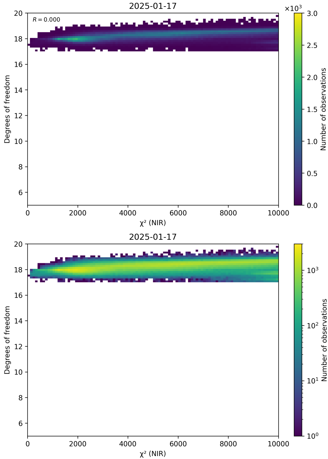
Figure 44: Scatter density plot of “ \chi^2 (NIR)” against “Degrees of freedom” for 2025-01-17 to 2025-01-18.
