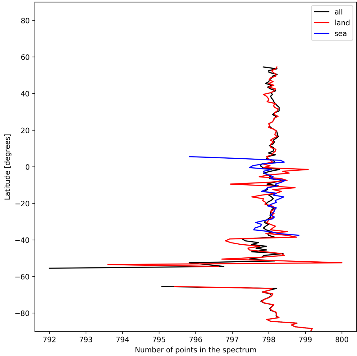
Figure 15: Zonal average of “Number of points in the spectrum” for 2025-01-17 to 2025-01-18.
