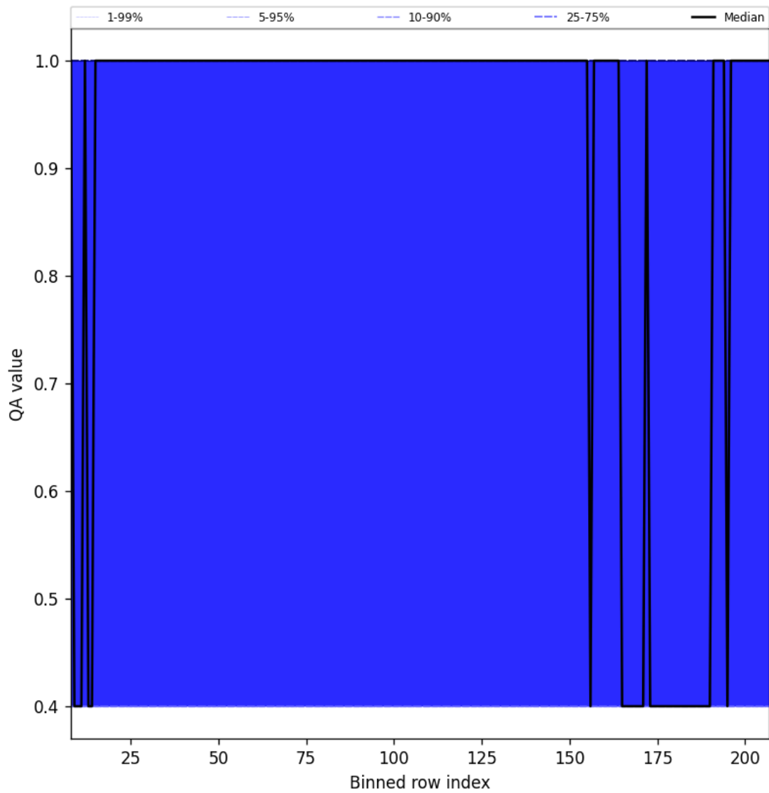
Figure 33: Along track statistics of “QA value” for 2025-01-17 to 2025-01-18
