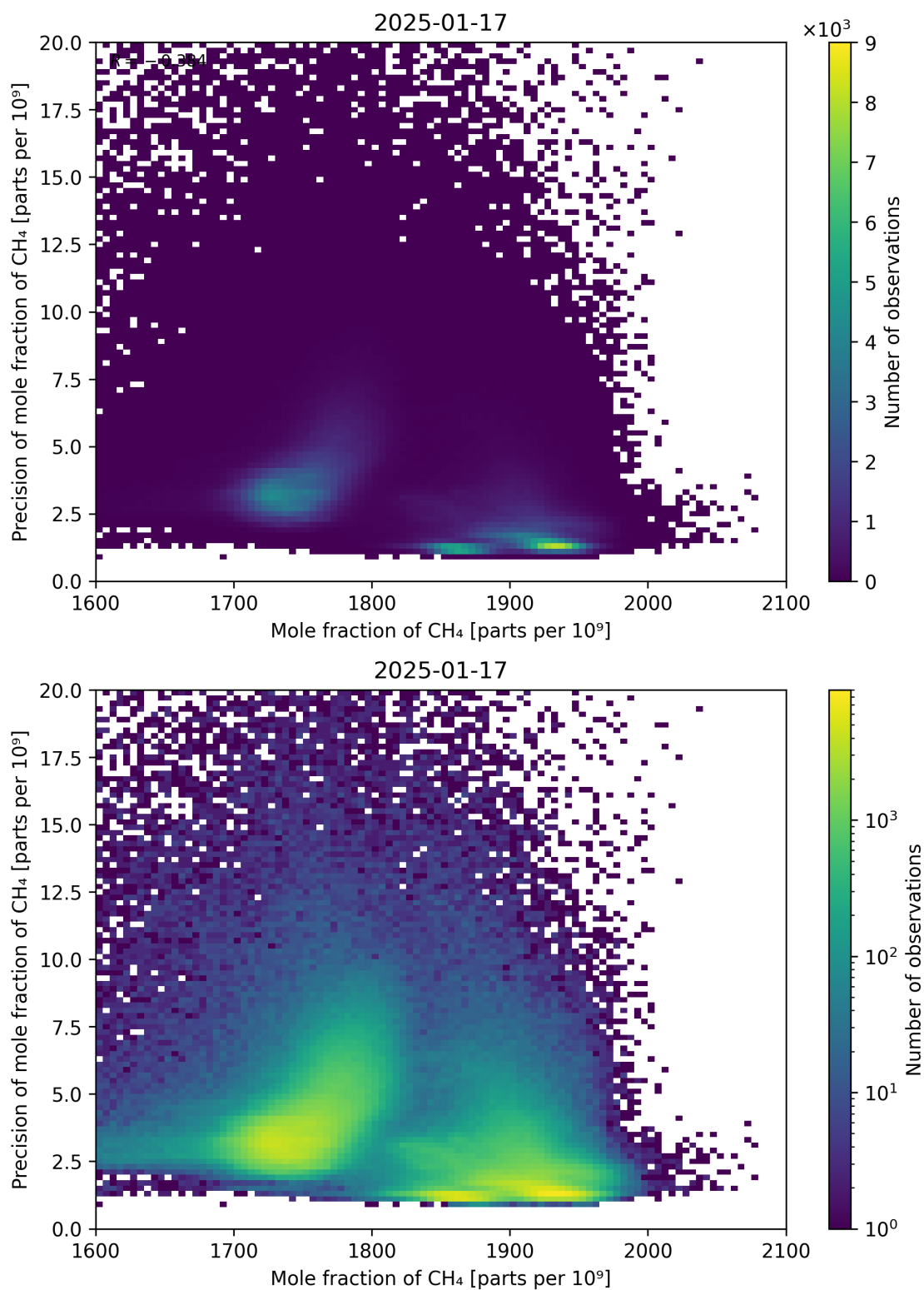
Figure 75: Scatter density plot of “Mole fraction of CH 4 ” against “Precision of mole fraction of CH 4 ” for 2025-01-17 to 2025-01-18.
