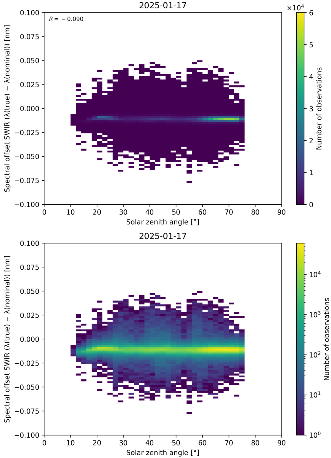
Figure 104: Scatter density plot of “Solar zenith angle” against “Spectral offset SWIR ( \lambda_{\text{true}} - \lambda_{\text{nominal}} )” for 2025-01-17 to 2025-01-18.
