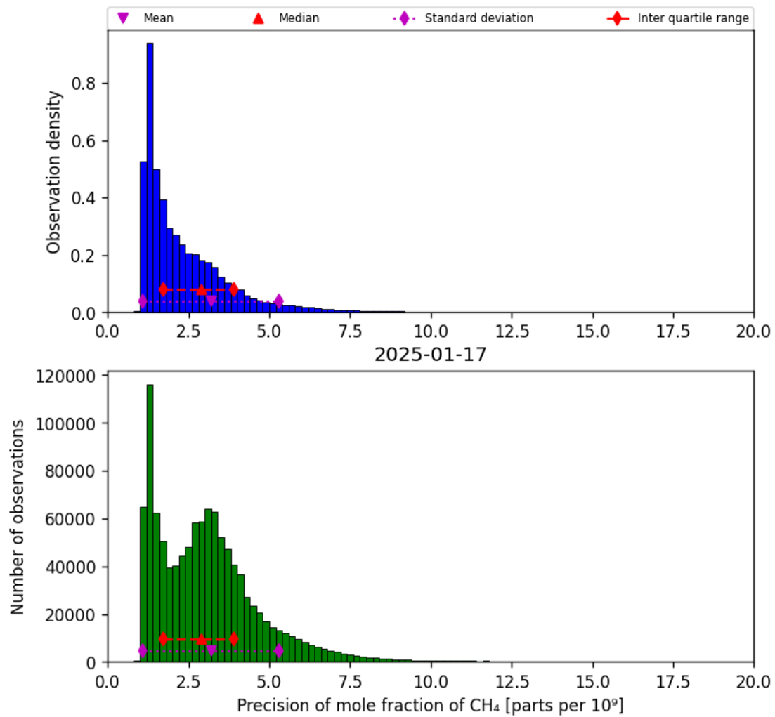
Figure 24: Histogram of “Precision of mole fraction of CH 4 ” for 2025-01-17 to 2025-01-18
