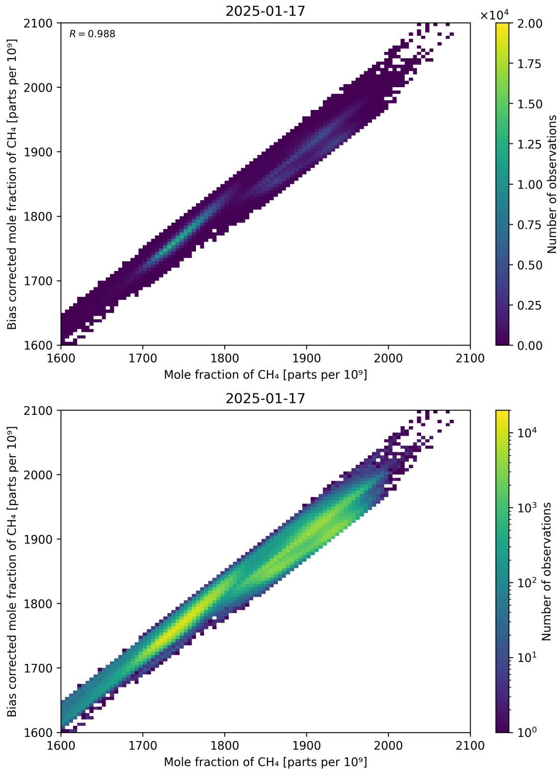
Figure 74: Scatter density plot of “Mole fraction of CH 4 ” against “Bias corrected mole fraction of CH 4 ” for 2025-01-17 to 2025-01-18.
