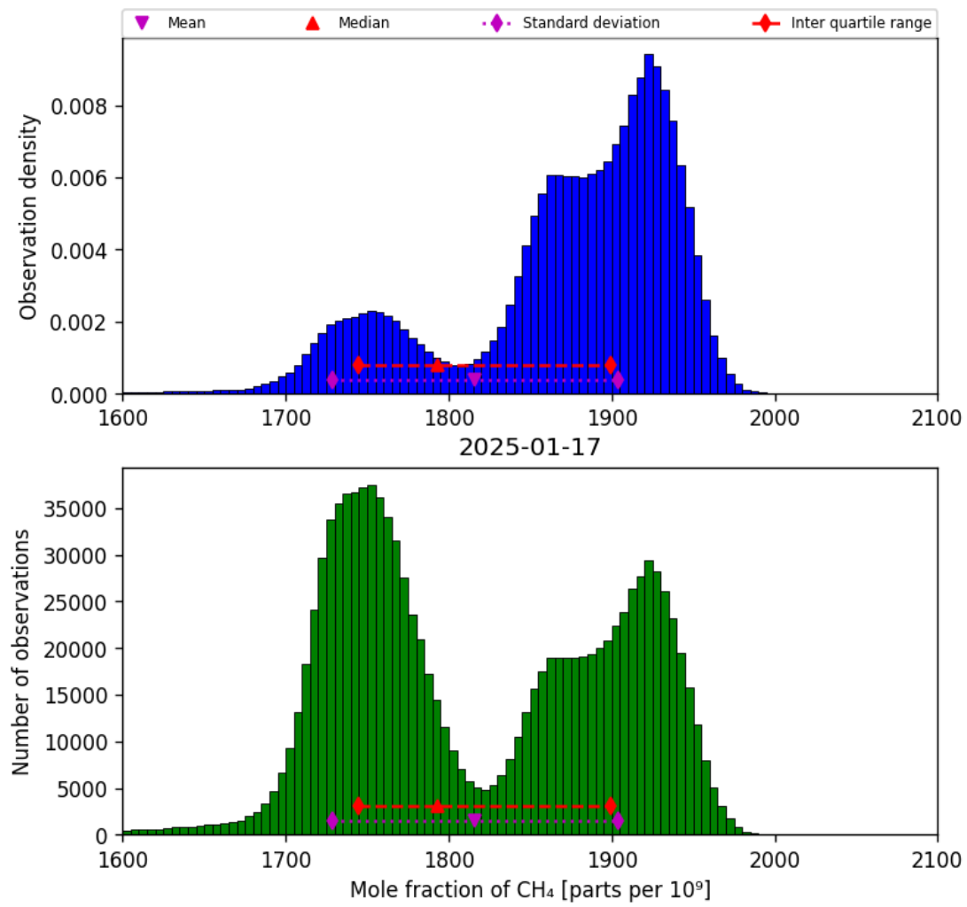
Figure 23: Histogram of “Mole fraction of CH 4 ” for 2025-01-17 to 2025-01-18
