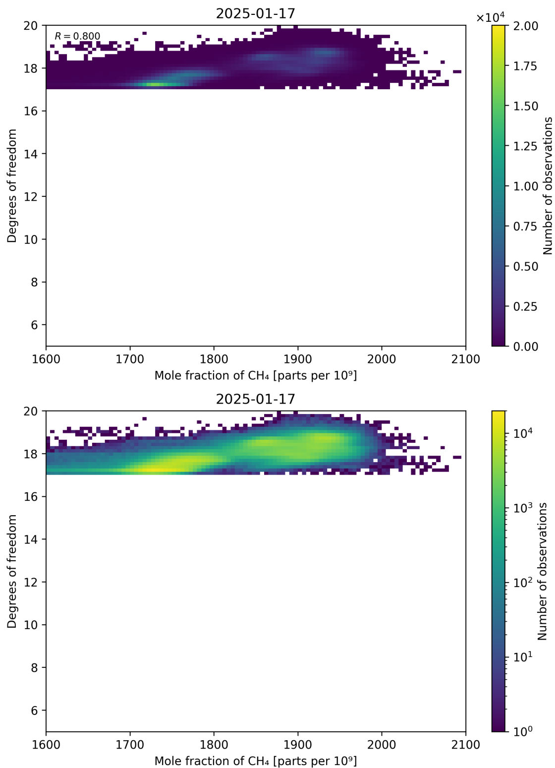
Figure 72: Scatter density plot of “Mole fraction of CH 4 ” against “Degrees of freedom” for 2025-01-17 to 2025-01-18.
