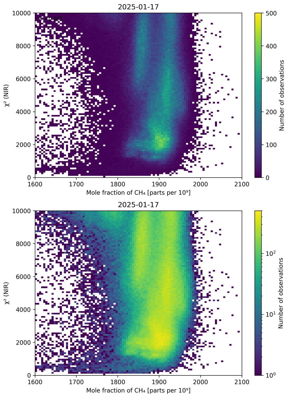
Figure 70: Scatter density plot of “Mole fraction of \text{CH}_4 ” against “ \chi^2 (NIR)” for 2025-01-17 to 2025-01-18.
