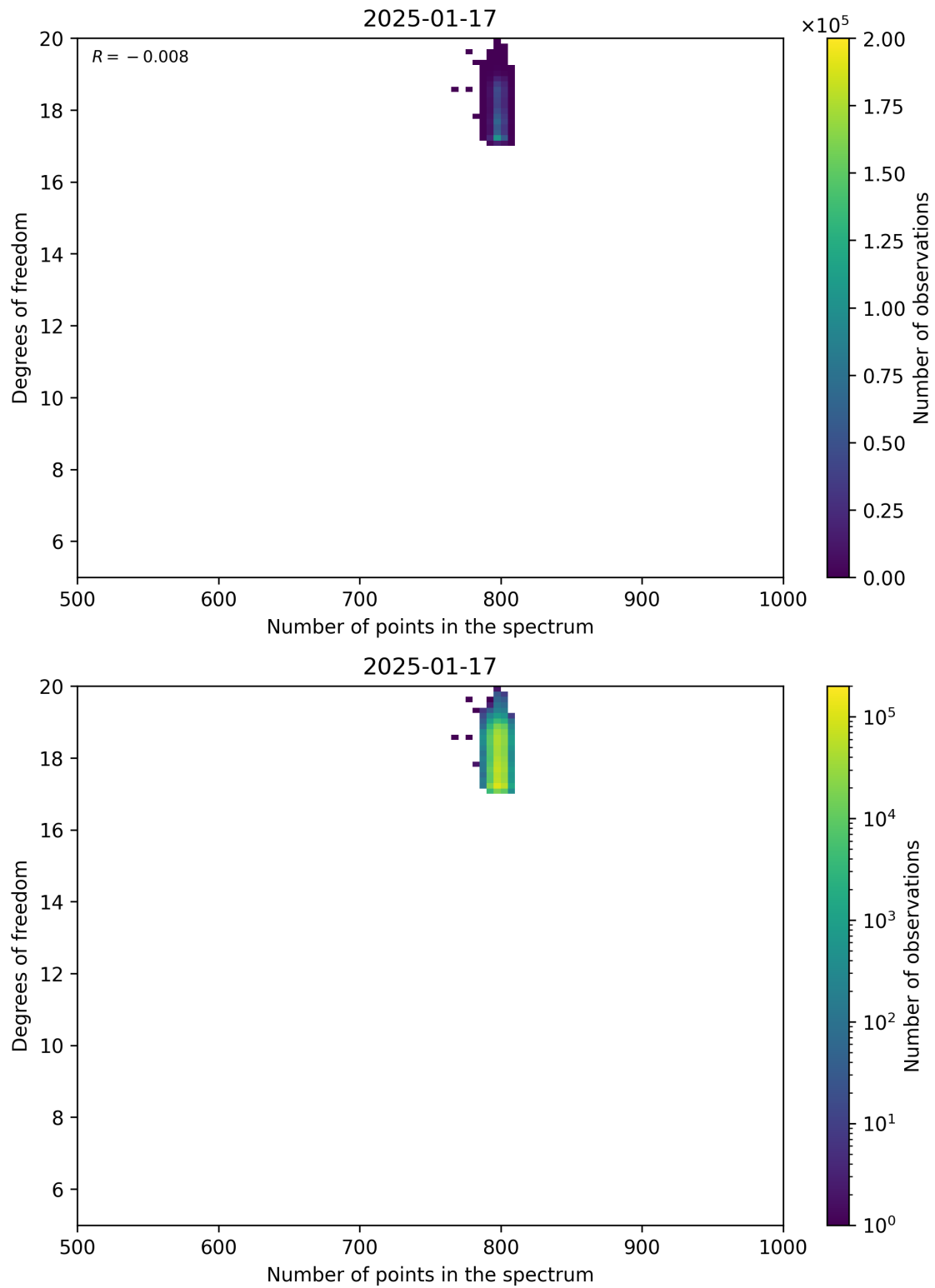
Figure 90: Scatter density plot of “Number of points in the spectrum” against “Degrees of freedom” for 2025-01-17 to 2025-01-18.
