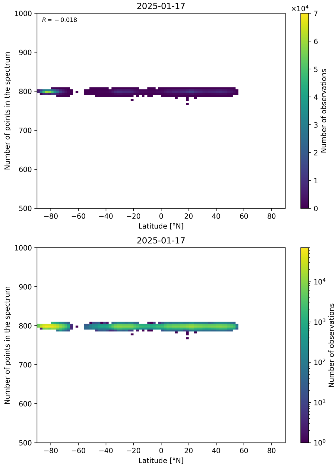
Figure 61: Scatter density plot of “Latitude” against “Number of points in the spectrum” for 2025-01-17 to 2025-01-18.
