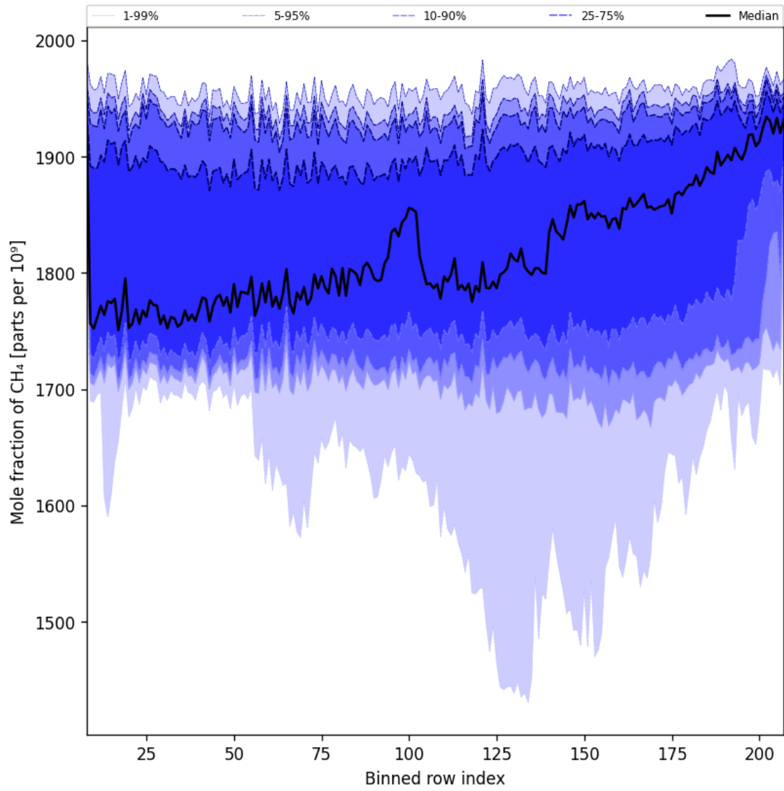
Figure 34: Along track statistics of “Mole fraction of CH 4 ” for 2025-01-17 to 2025-01-18
