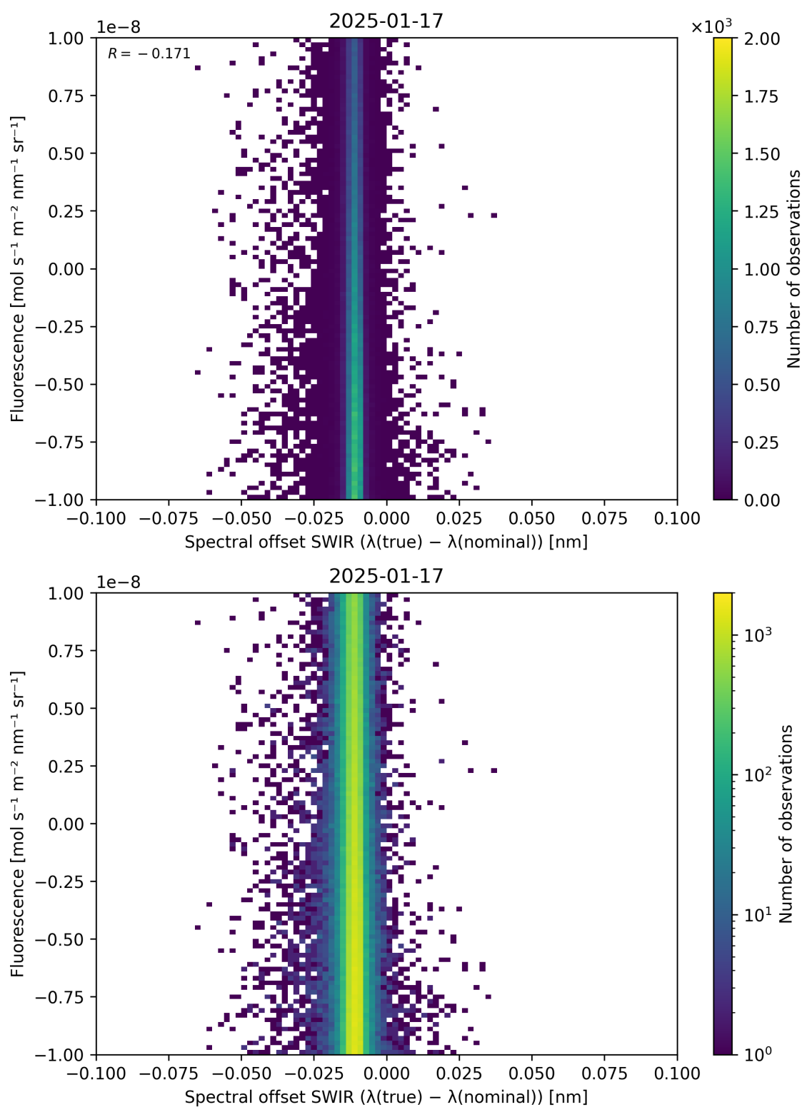
Figure 120: Scatter density plot of “Spectral offset SWIR ( \lambda_{\text{true}} - \lambda_{\text{nominal}} )” against “Fluorescence” for 2025-01-17 to 2025-01-18.
