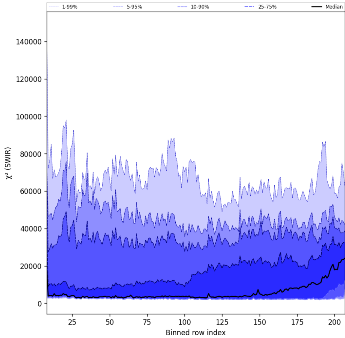
Figure 39: Along track statistics of “ \chi^2 (SWIR)” for 2025-01-17 to 2025-01-18
