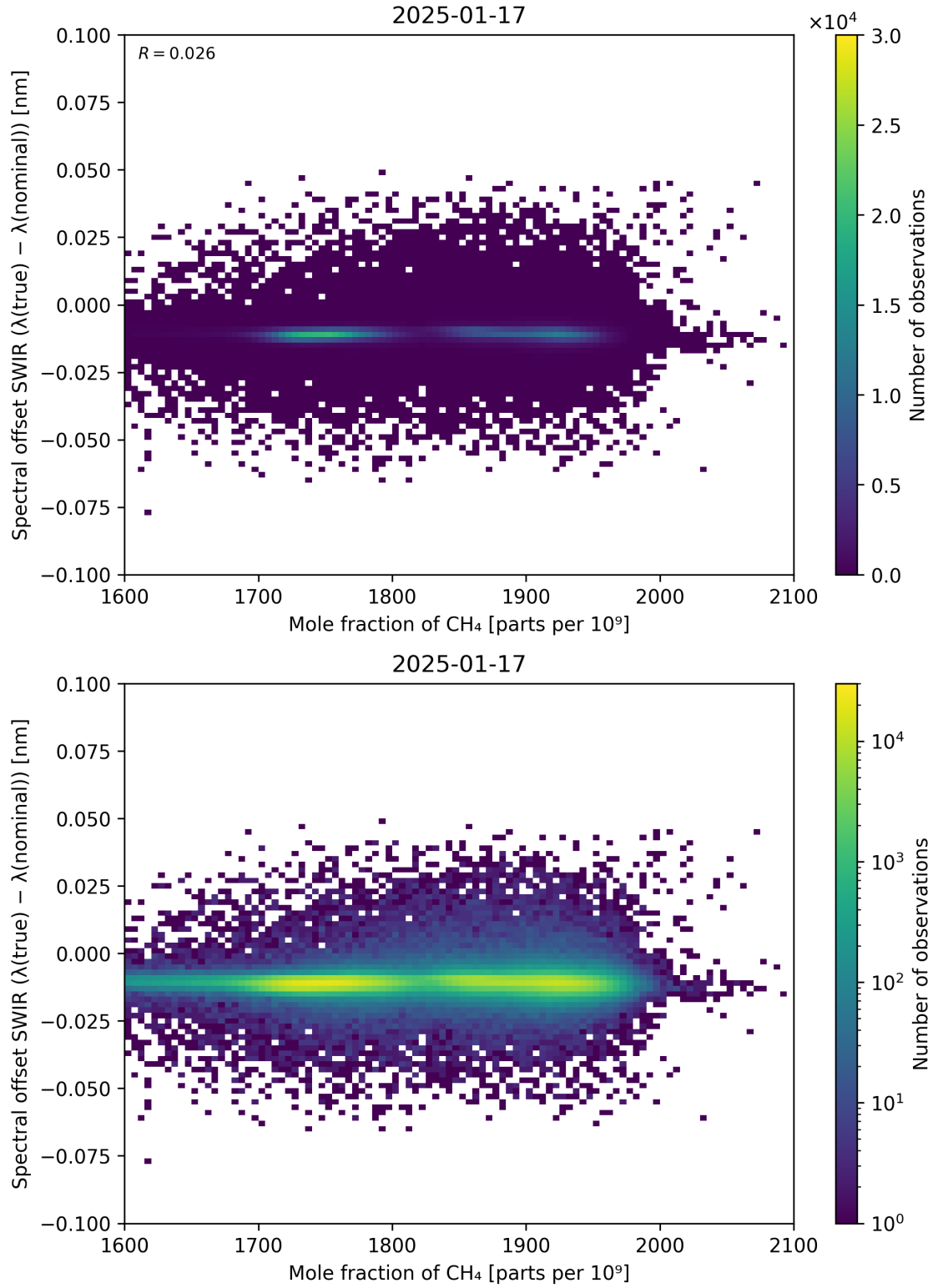
Figure 86: Scatter density plot of “Mole fraction of CH 4 ” against “Spectral offset SWIR ( \lambda_{\text{true}} - \lambda_{\text{nominal}} )” for 2025-01-17 to 2025-01-18.
