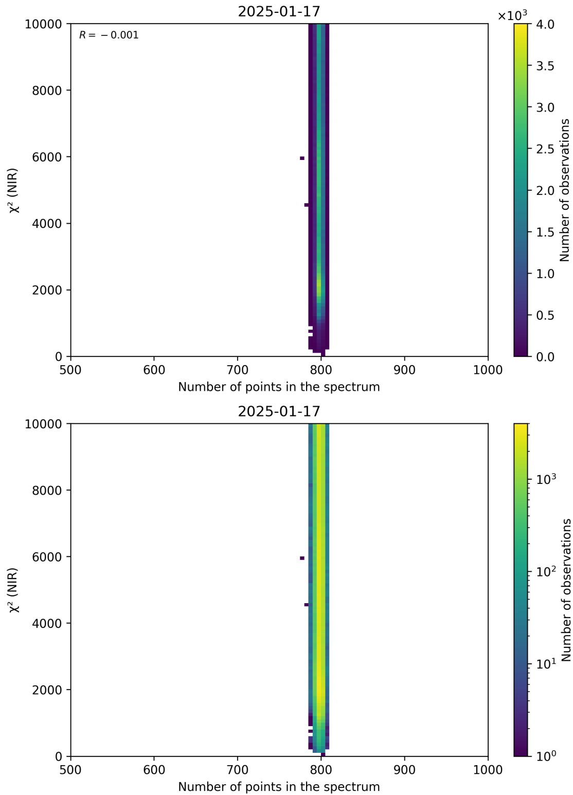
Figure 88: Scatter density plot of “Number of points in the spectrum” against “ \chi^2 (NIR)” for 2025-01-17 to 2025-01-18.
