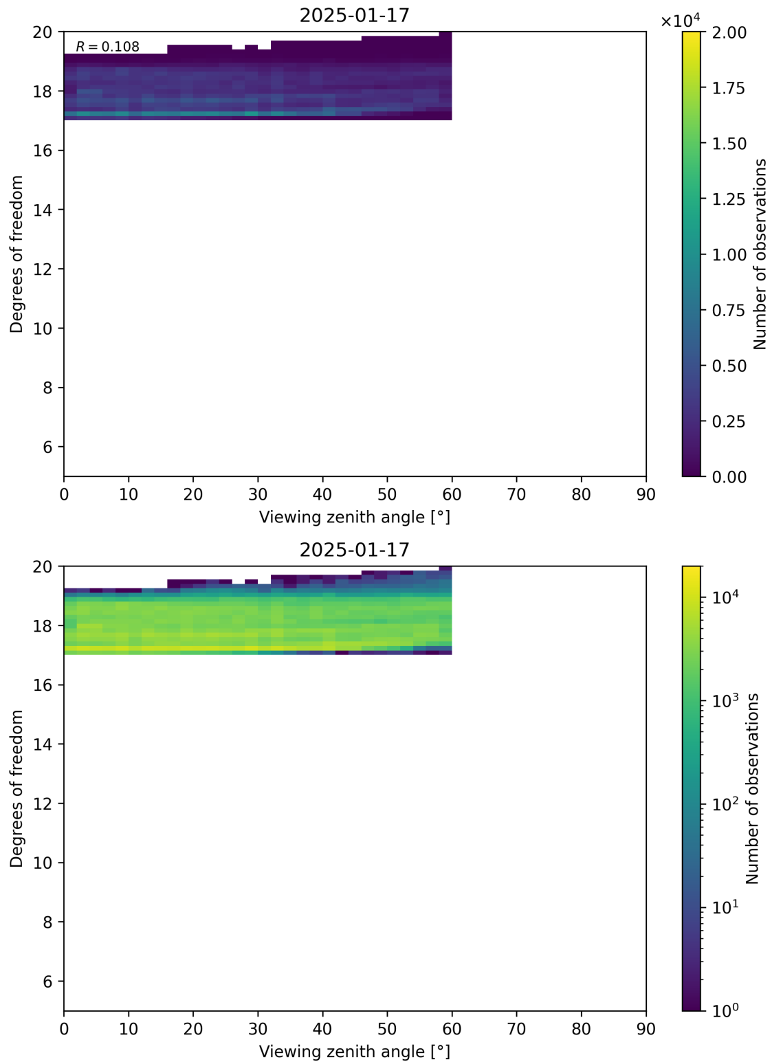
Figure 107: Scatter density plot of “Viewing zenith angle” against “Degrees of freedom” for 2025-01-17 to 2025-01-18.
