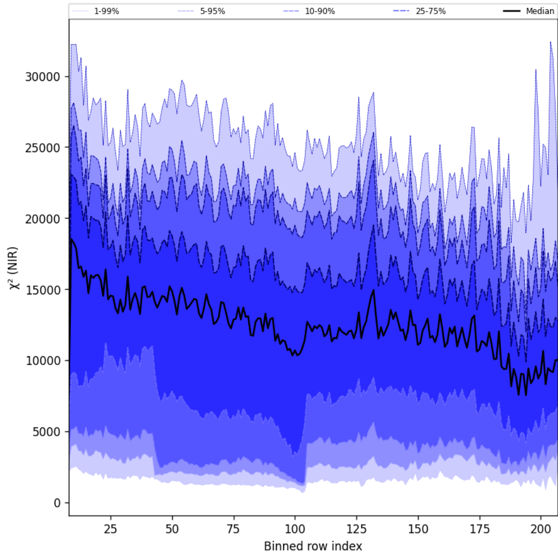
Figure 40: Along track statistics of “ \chi^2 (NIR)” for 2025-01-17 to 2025-01-18
