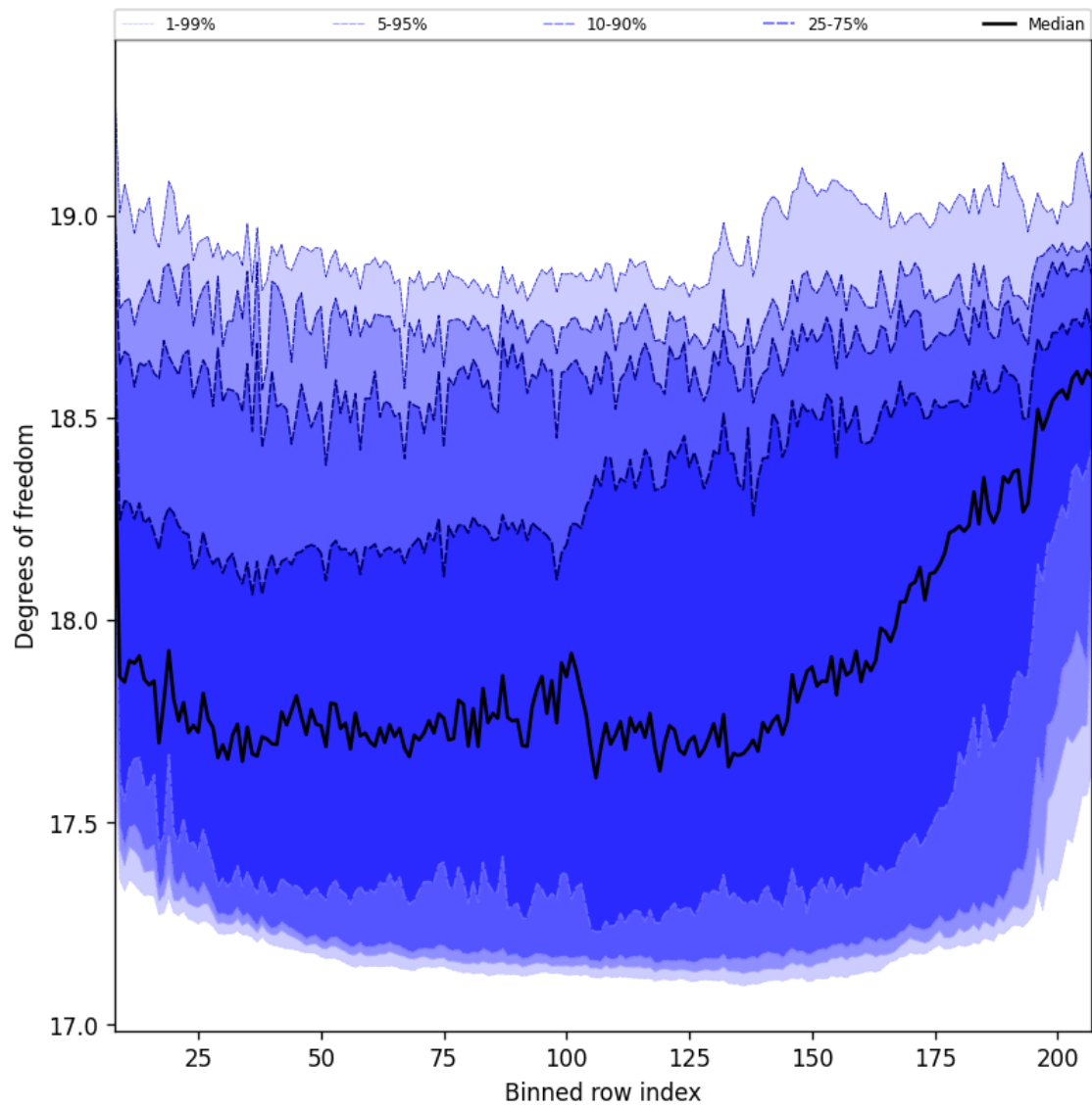
Figure 41: Along track statistics of “Degrees of freedom” for 2025-01-17 to 2025-01-18
