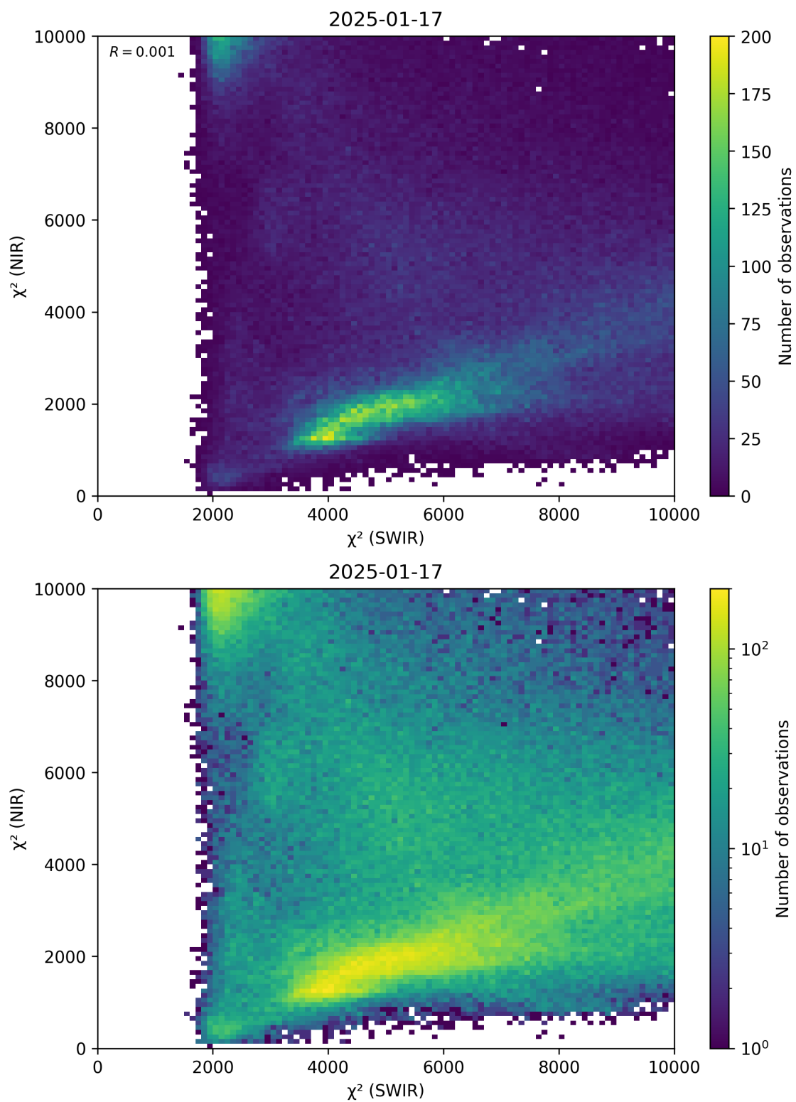
Figure 47: Scatter density plot of “ \chi^2 (SWIR)” against “ \chi^2 (NIR)” for 2025-01-17 to 2025-01-18.
