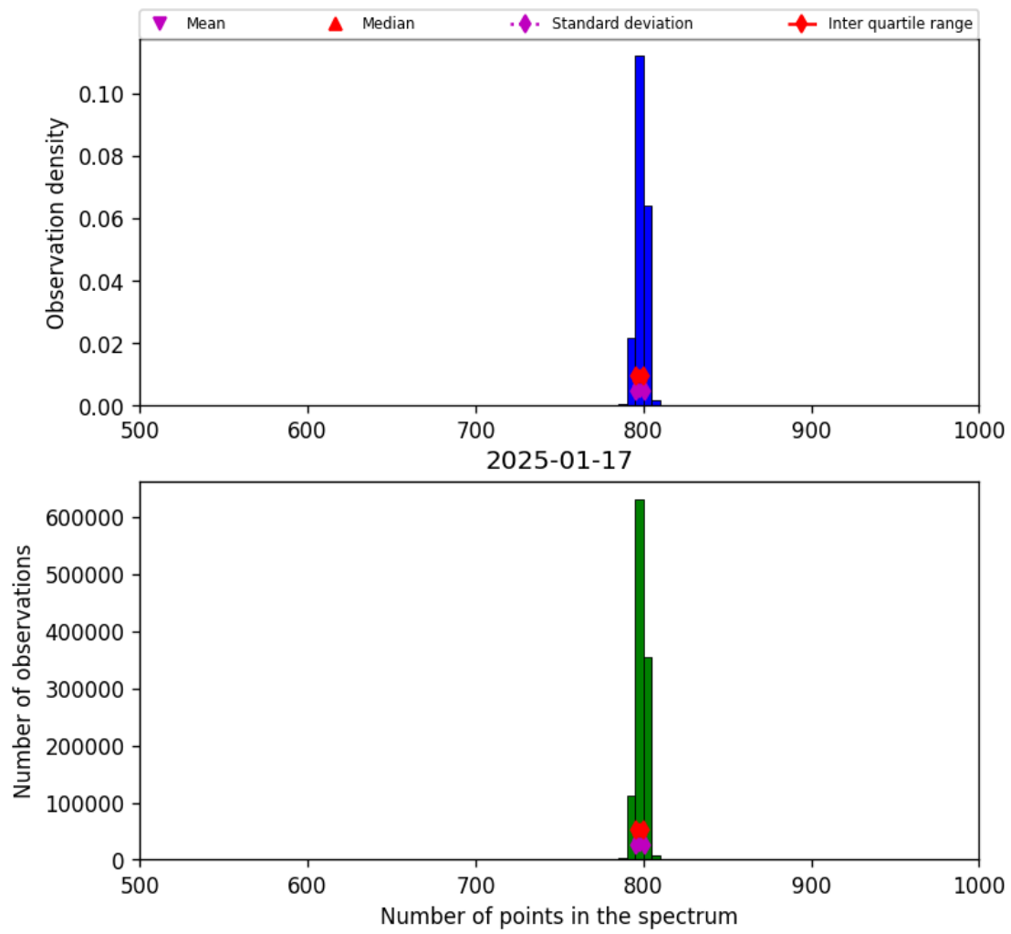
Figure 26: Histogram of “Number of points in the spectrum” for 2025-01-17 to 2025-01-18
