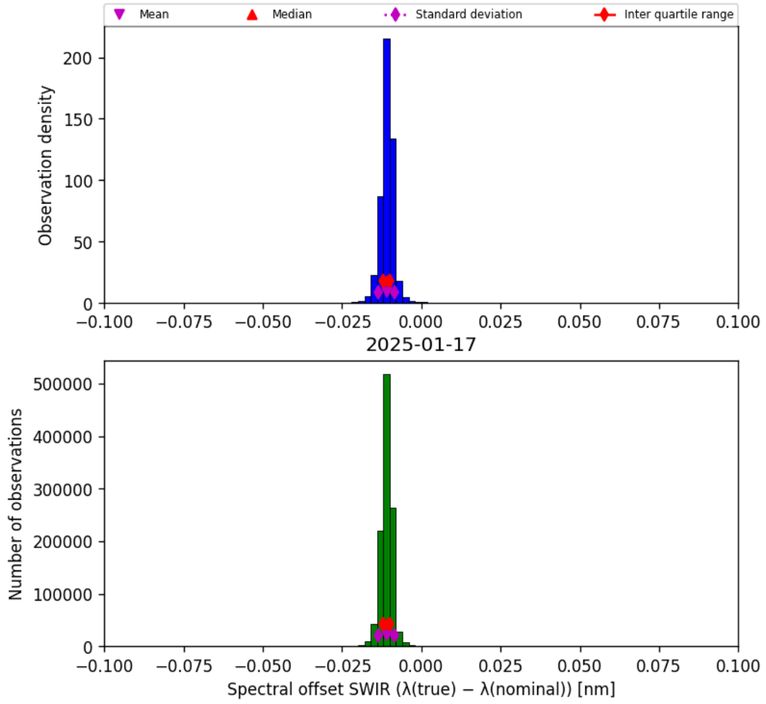
Figure 27: Histogram of “Spectral offset SWIR ( \lambda_{\text{true}} - \lambda_{\text{nominal}} )” for 2025-01-17 to 2025-01-18
