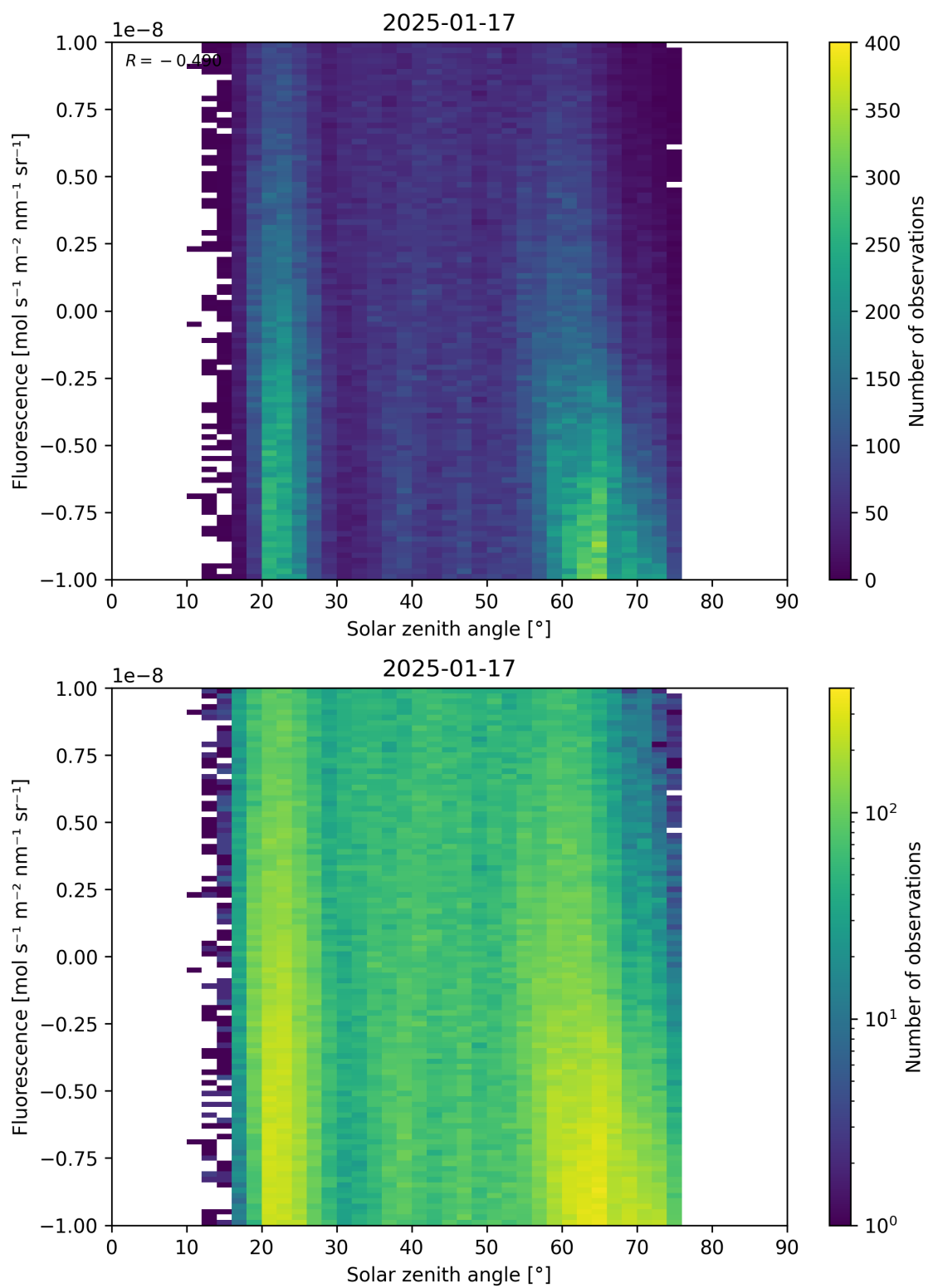
Figure 97: Scatter density plot of “Solar zenith angle” against “Fluorescence” for 2025-01-17 to 2025-01-18.
