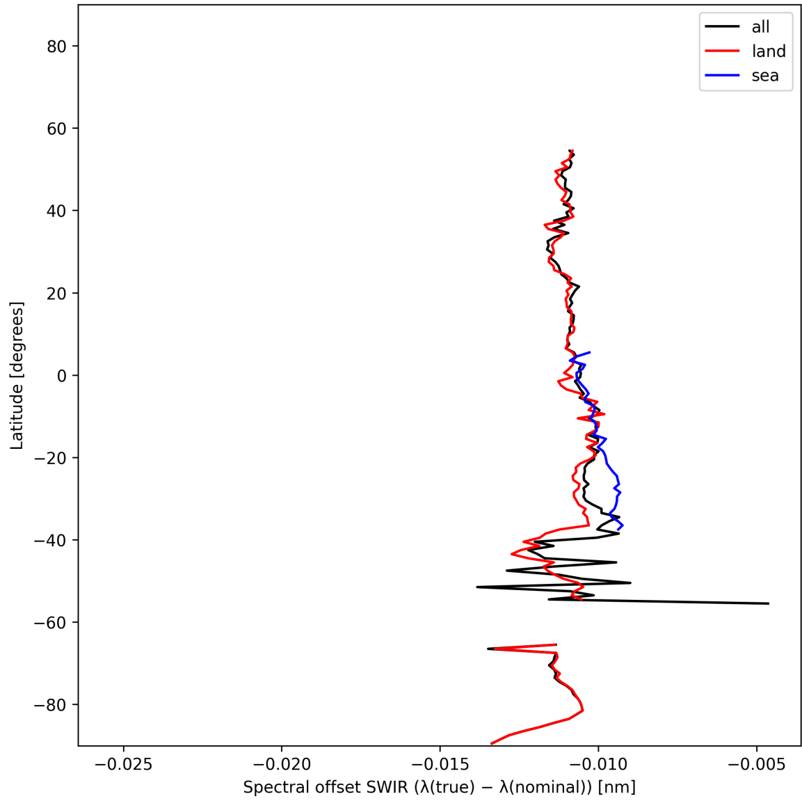
Figure 16: Zonal average of “Spectral offset SWIR ( \lambda_{\text{true}} - \lambda_{\text{nominal}} )” for 2025-01-17 to 2025-01-18.
