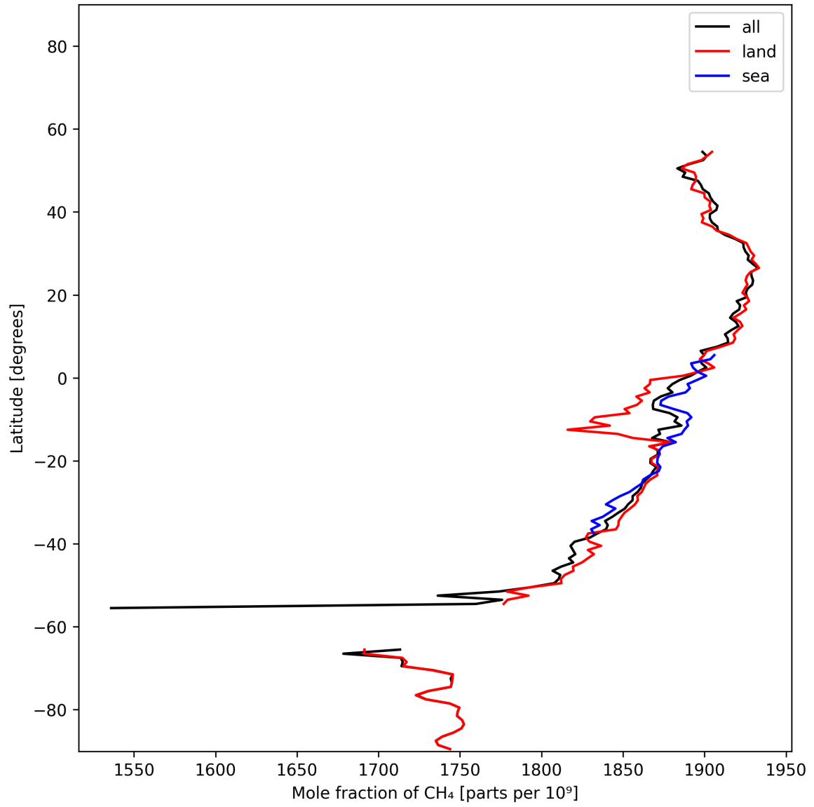
Figure 12: Zonal average of “Mole fraction of \text{CH}_4 ” for 2025-01-17 to 2025-01-18.
