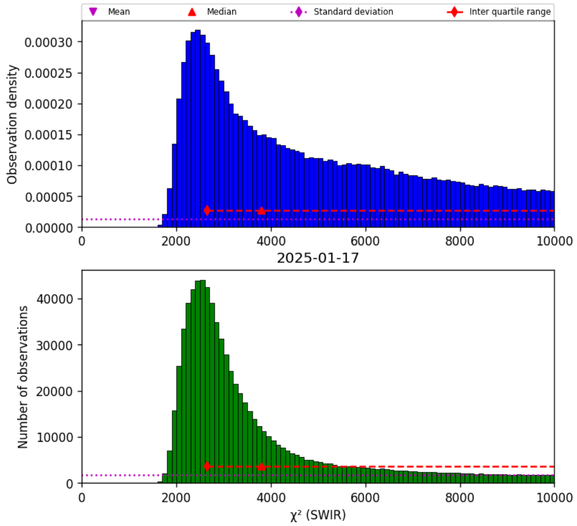
Figure 28: Histogram of “ \chi^2 (SWIR)” for 2025-01-17 to 2025-01-18
