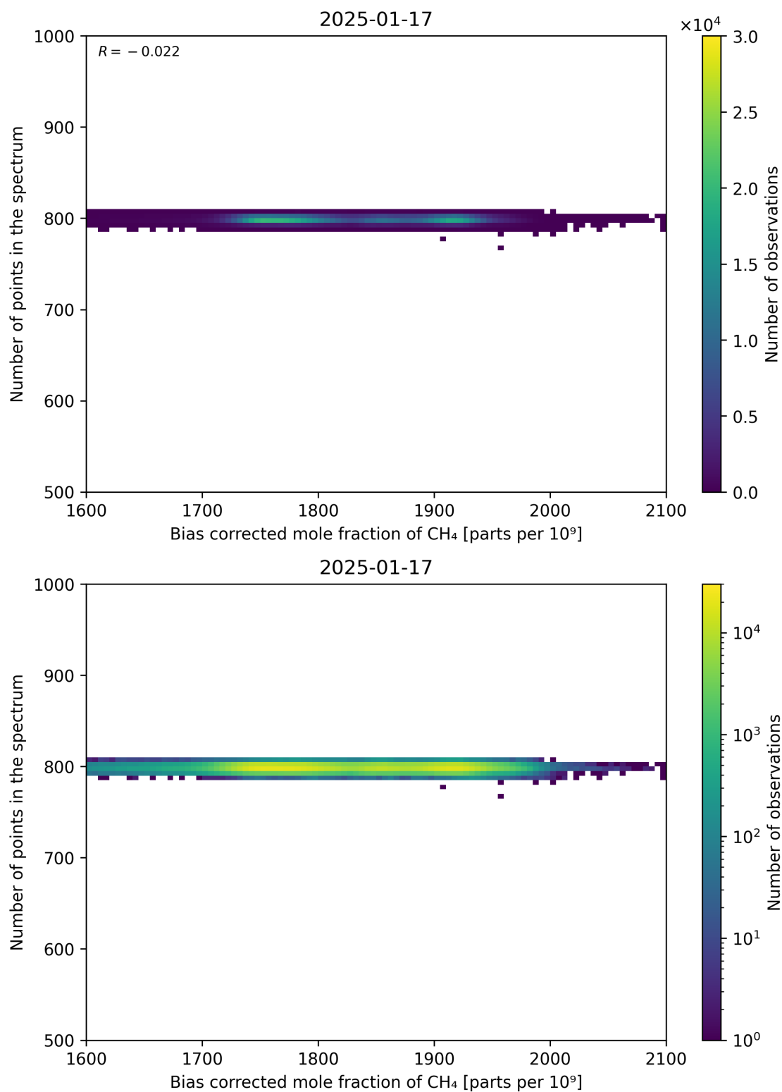
Figure 68: Scatter density plot of “Bias corrected mole fraction of CH 4 ” against “Number of points in the spectrum” for 2025-01-17 to 2025-01-18.
