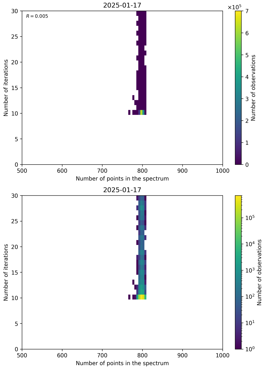
Figure 92: Scatter density plot of “Number of points in the spectrum” against “Number of iterations” for 2025-01-17 to 2025-01-18.
