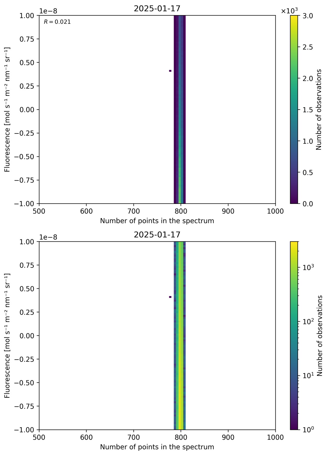
Figure 91: Scatter density plot of “Number of points in the spectrum” against “Fluorescence” for 2025-01-17 to 2025-01-18.
