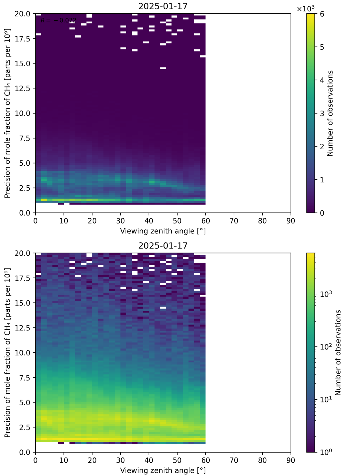
Figure 112: Scatter density plot of “Viewing zenith angle” against “Precision of mole fraction of CH 4 ” for 2025-01-17 to 2025-01-18.
