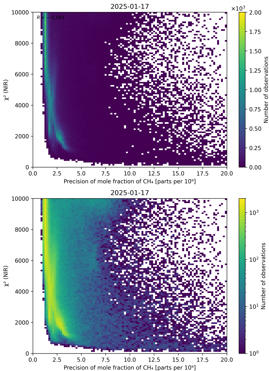
Figure 78: Scatter density plot of “Precision of mole fraction of CH 4 ” against “ \chi^2 (NIR)” for 2025-01-17 to 2025-01-18.
