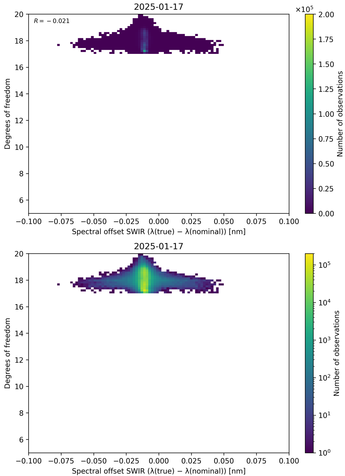
Figure 119: Scatter density plot of “Spectral offset SWIR ( \lambda_{\text{true}} - \lambda_{\text{nominal}} )” against “Degrees of freedom” for 2025-01-17 to 2025-01-18.
