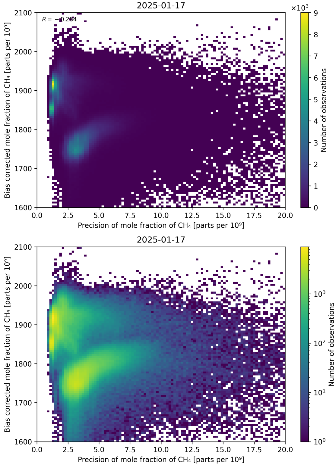
Figure 82: Scatter density plot of “Precision of mole fraction of CH 4 ” against “Bias corrected mole fraction of CH 4 ” for 2025-01-17 to 2025-01-18.
