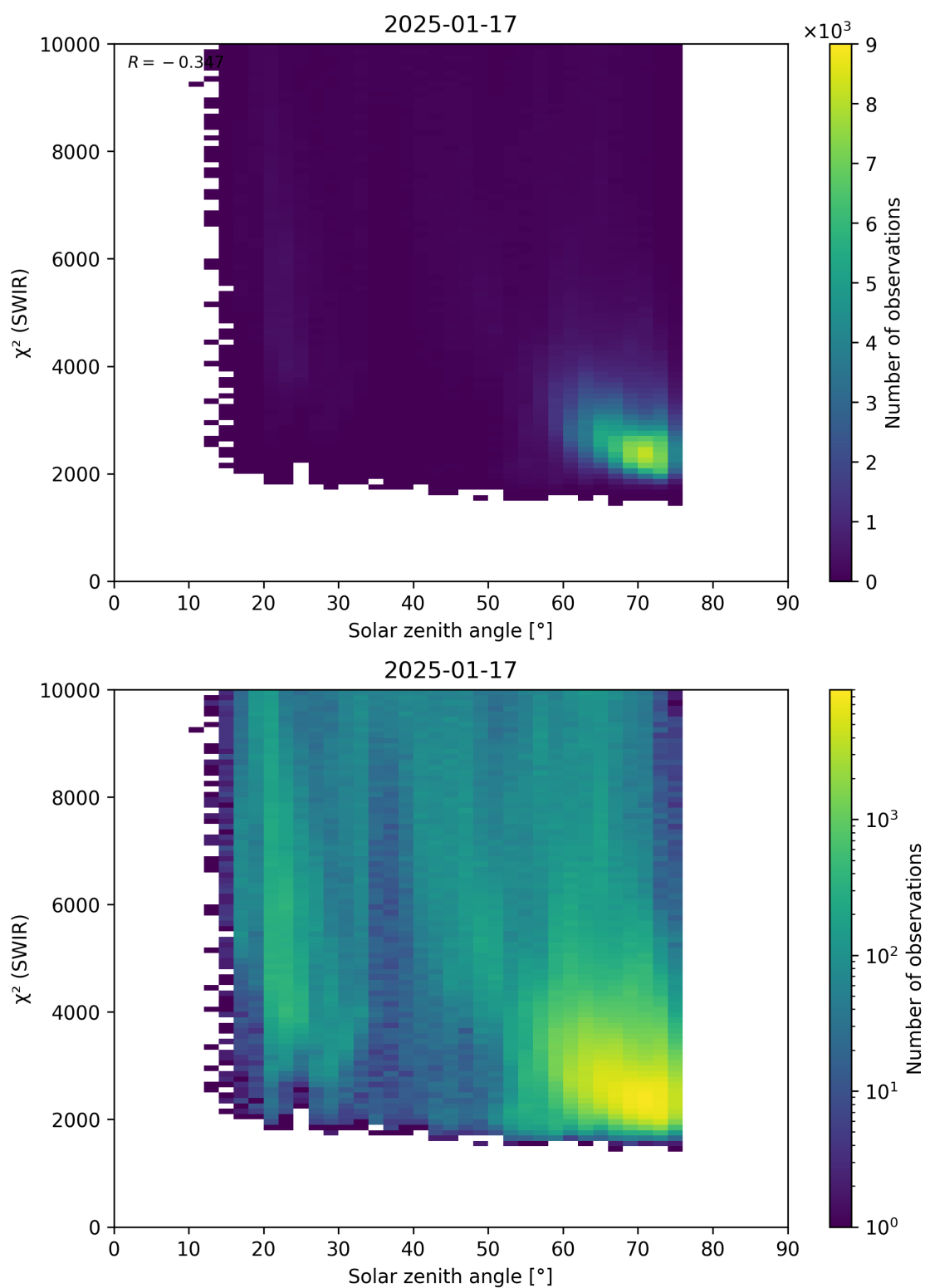
Figure 95: Scatter density plot of “Solar zenith angle” against “ \chi^2 (SWIR)” for 2025-01-17 to 2025-01-18.
