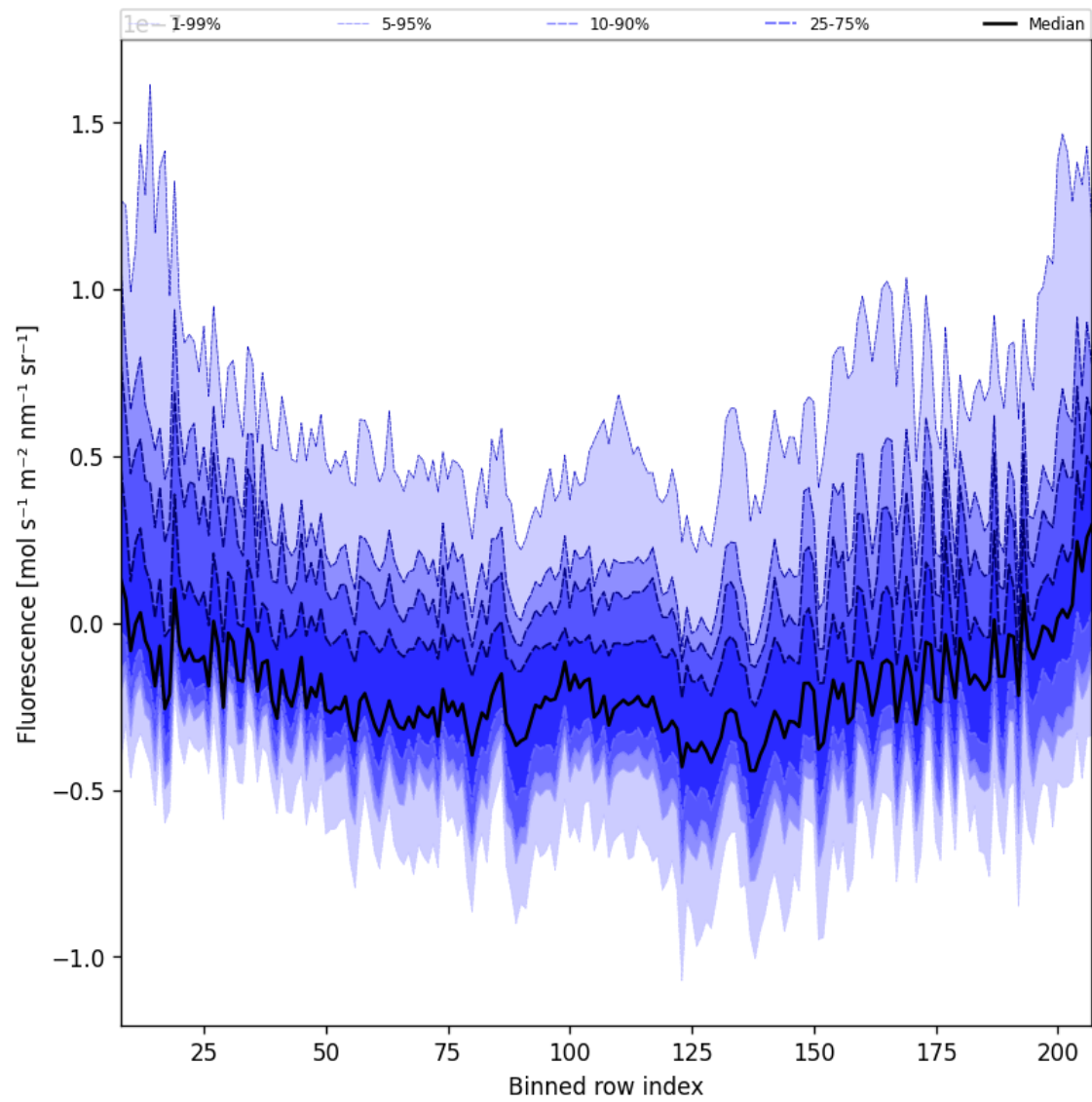
Figure 43: Along track statistics of “Fluorescence” for 2025-01-17 to 2025-01-18
