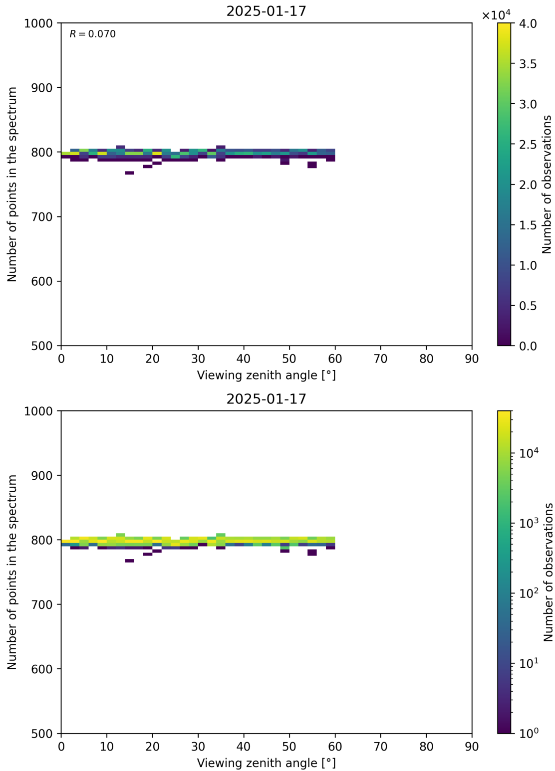
Figure 114: Scatter density plot of “Viewing zenith angle” against “Number of points in the spectrum” for 2025-01-17 to 2025-01-18.
