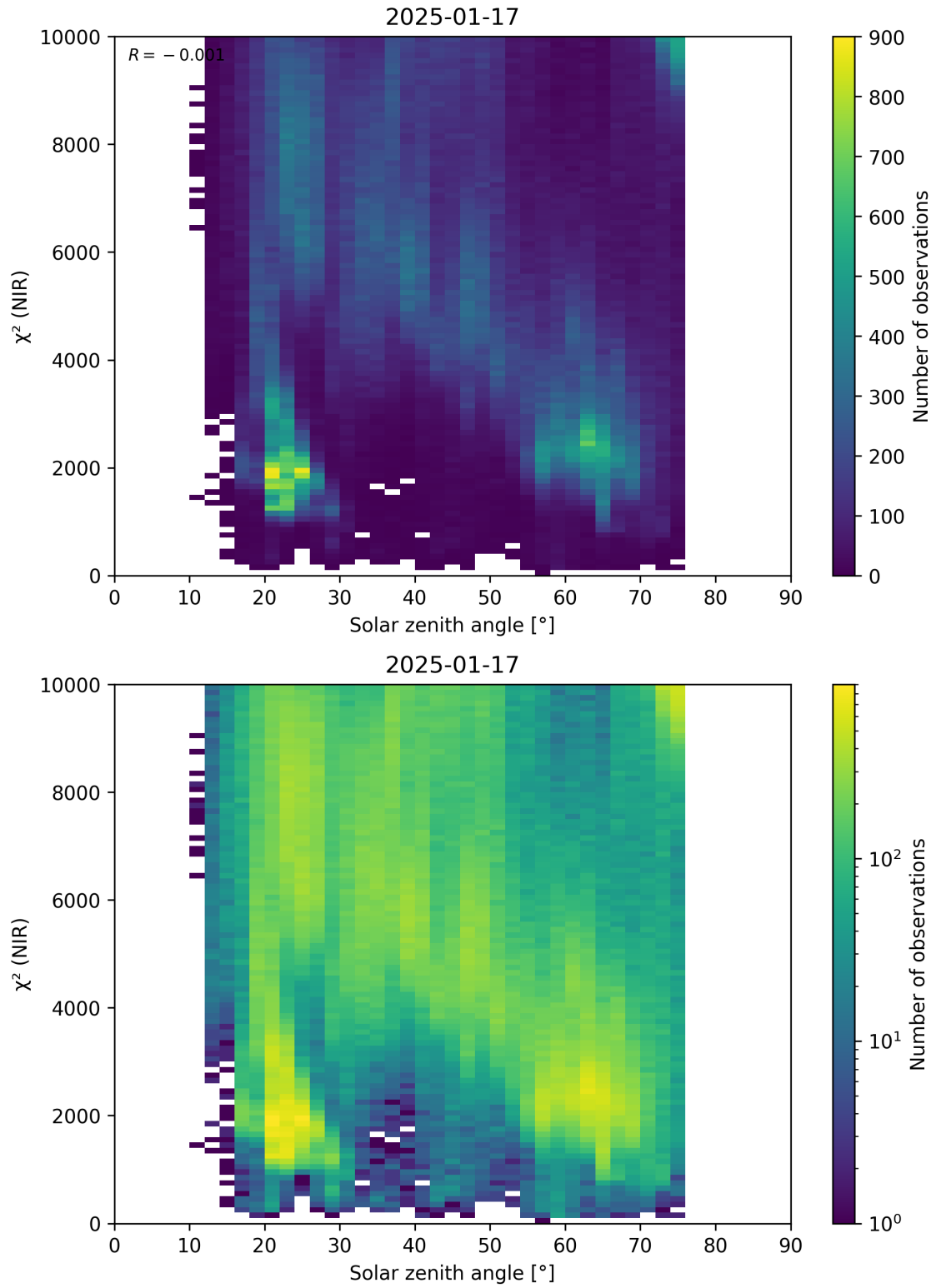
Figure 94: Scatter density plot of “Solar zenith angle” against “ \chi^2 (NIR)” for 2025-01-17 to 2025-01-18.
