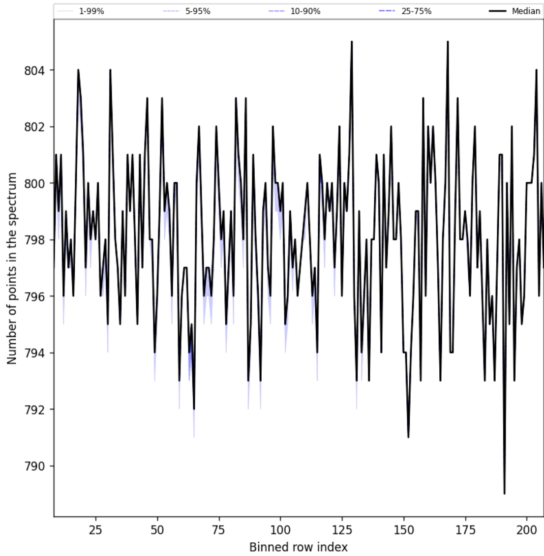
Figure 37: Along track statistics of “Number of points in the spectrum” for 2025-01-17 to 2025-01-18
