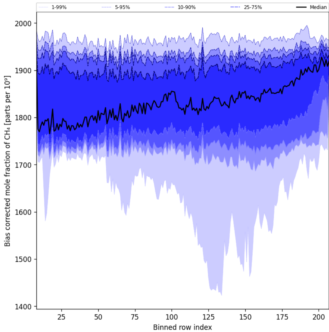
Figure 36: Along track statistics of “Bias corrected mole fraction of CH 4 ” for 2025-01-17 to 2025-01-18
