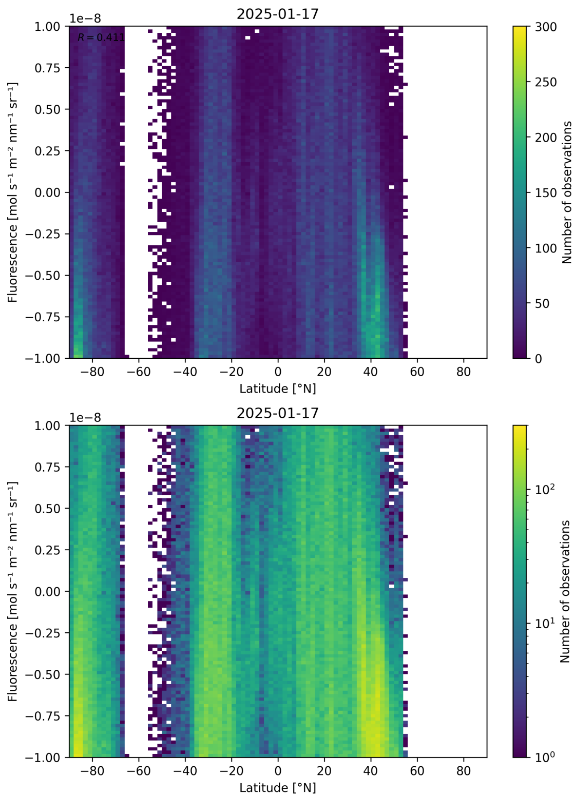
Figure 56: Scatter density plot of “Latitude” against “Fluorescence” for 2025-01-17 to 2025-01-18.
