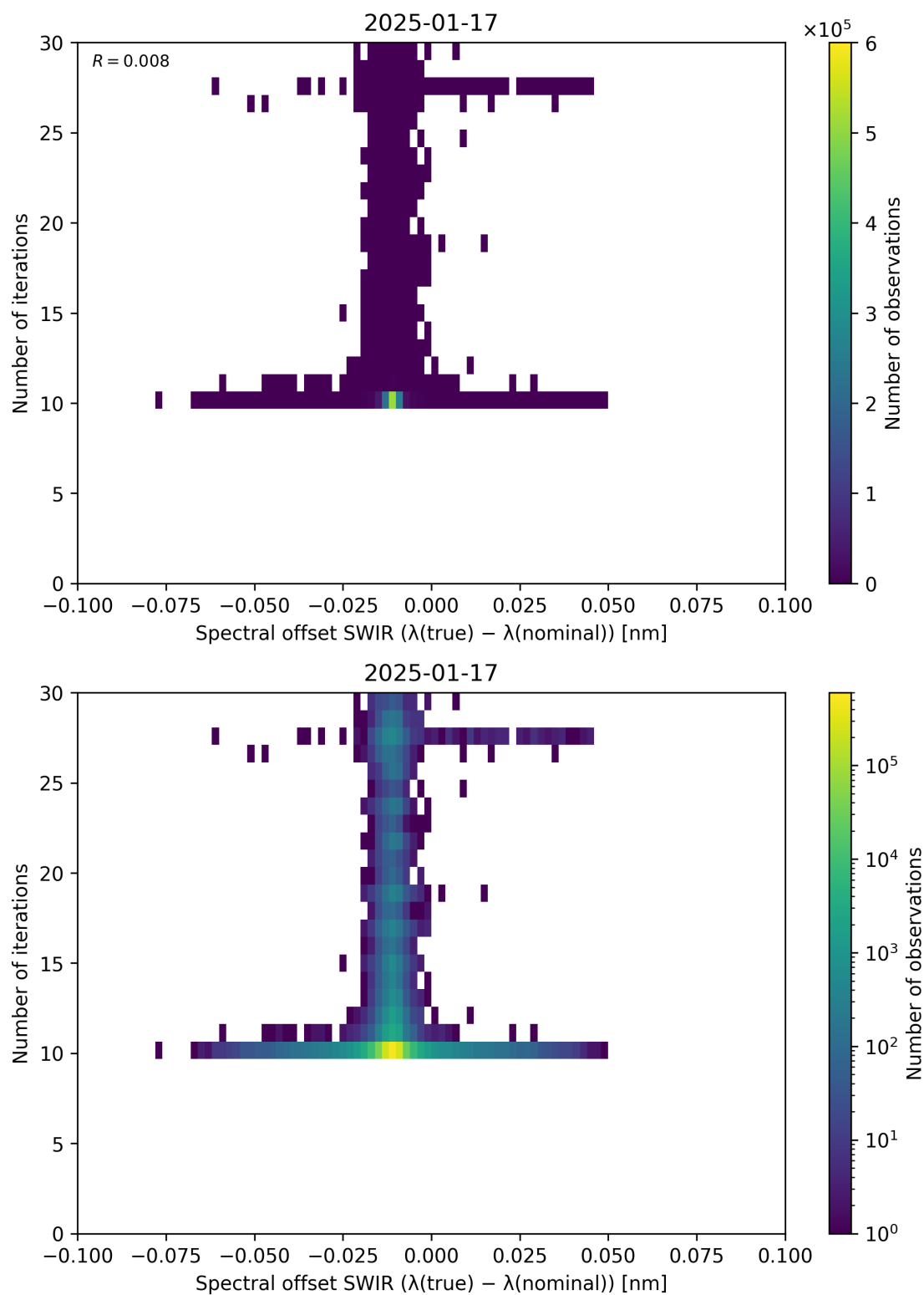
Figure 121: Scatter density plot of “Spectral offset SWIR ( \lambda_{\text{true}} - \lambda_{\text{nominal}} )” against “Number of iterations” for 2025-01-17 to 2025-01-18.
