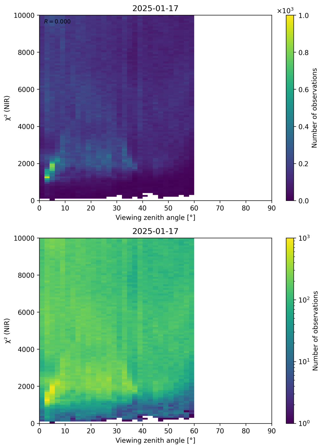
Figure 105: Scatter density plot of “Viewing zenith angle” against “ \chi^2 (NIR)” for 2025-01-17 to 2025-01-18.
