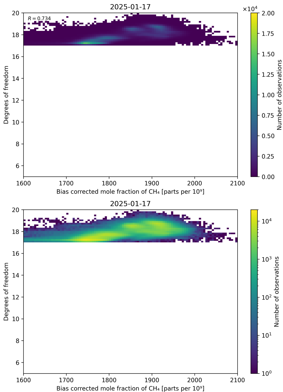
Figure 65: Scatter density plot of “Bias corrected mole fraction of CH 4 ” against “Degrees of freedom” for 2025-01-17 to 2025-01-18.
