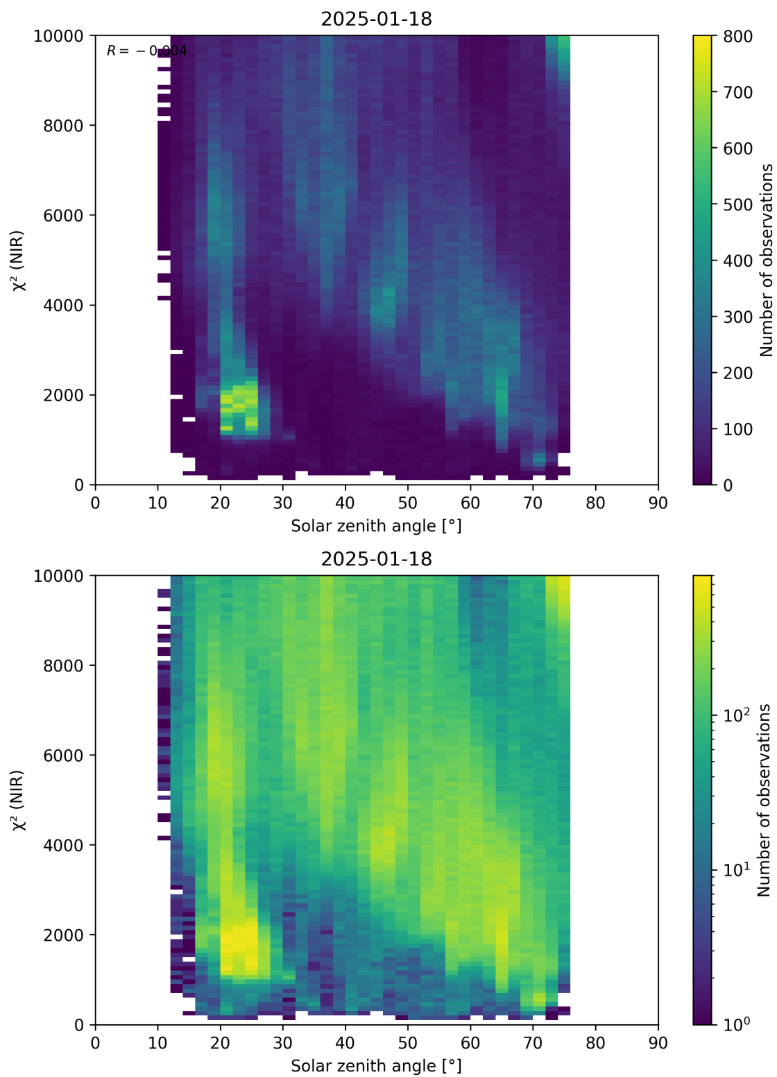
Figure 94: Scatter density plot of “Solar zenith angle” against “ \chi^2 (NIR)” for 2025-01-17 to 2025-01-19.
