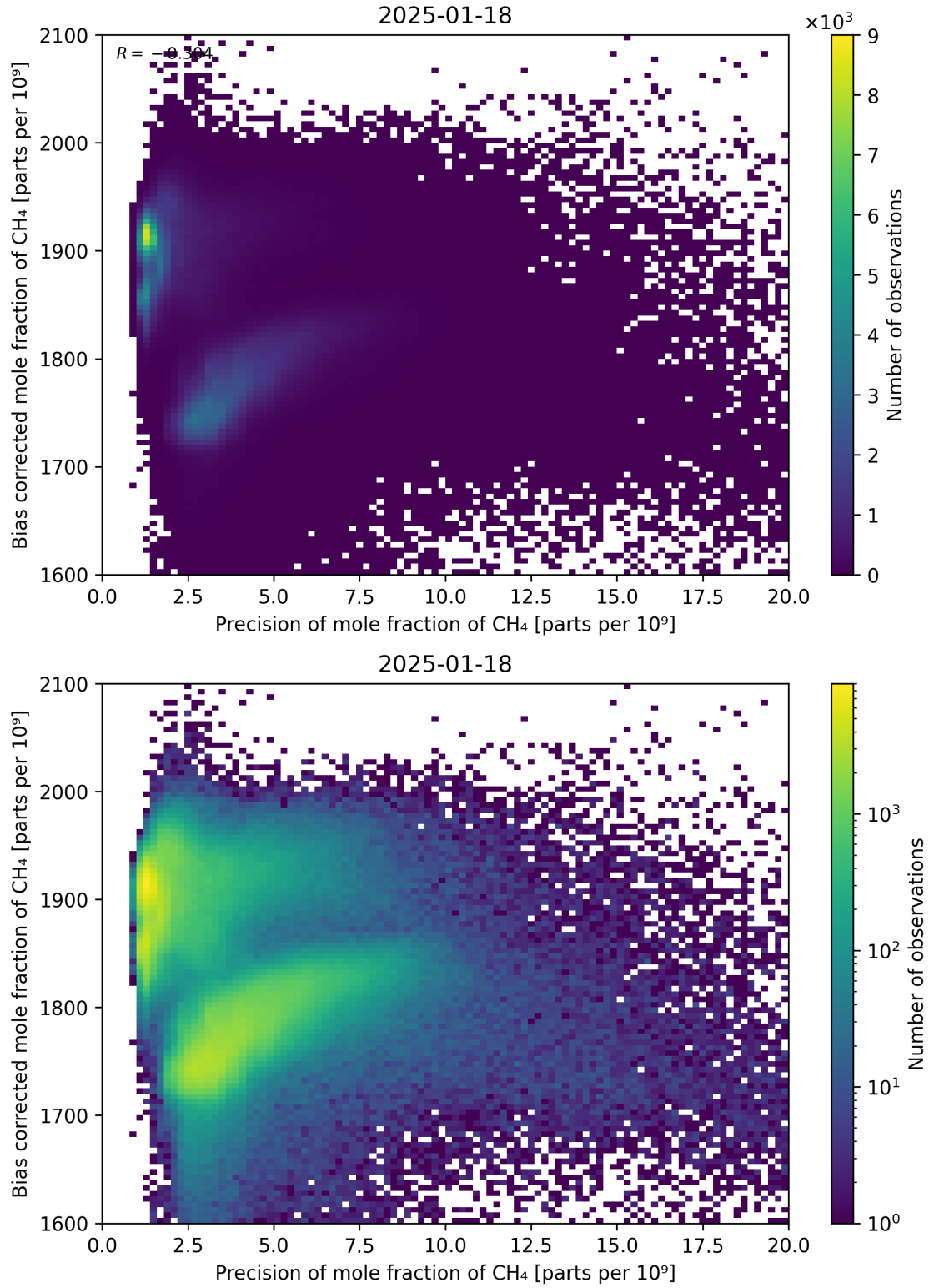
Figure 82: Scatter density plot of “Precision of mole fraction of CH 4 ” against “Bias corrected mole fraction of CH 4 ” for 2025-01-17 to 2025-01-19.
