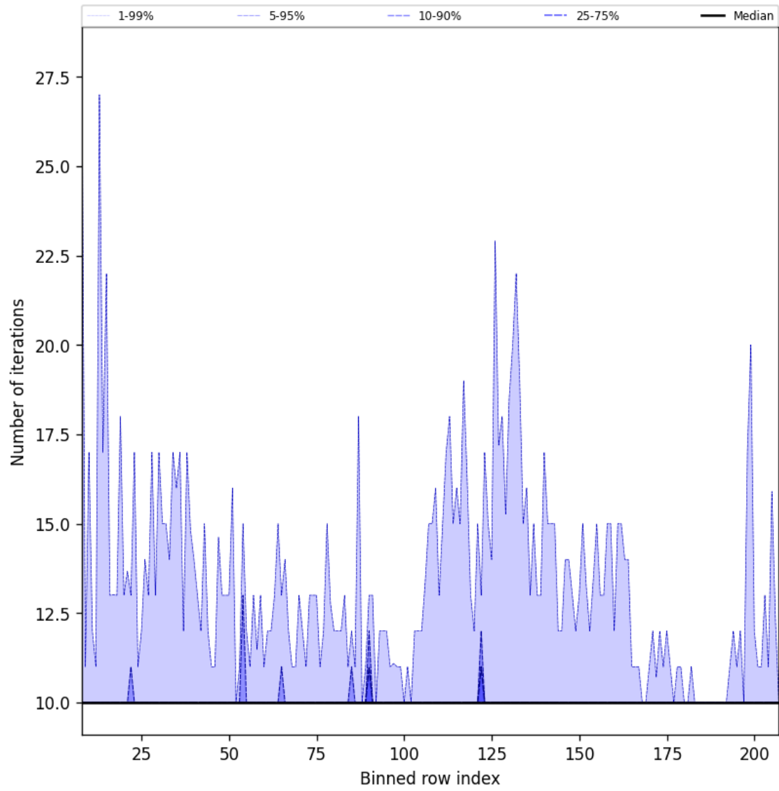
Figure 42: Along track statistics of “Number of iterations” for 2025-01-17 to 2025-01-19
