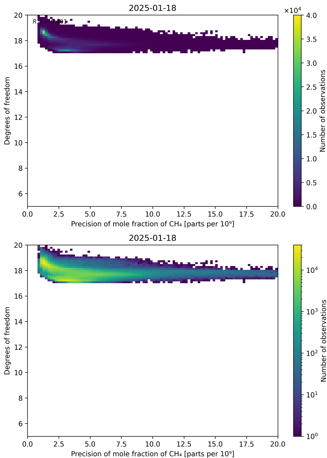
Figure 80: Scatter density plot of “Precision of mole fraction of CH 4 ” against “Degrees of freedom” for 2025-01-17 to 2025-01-19.
