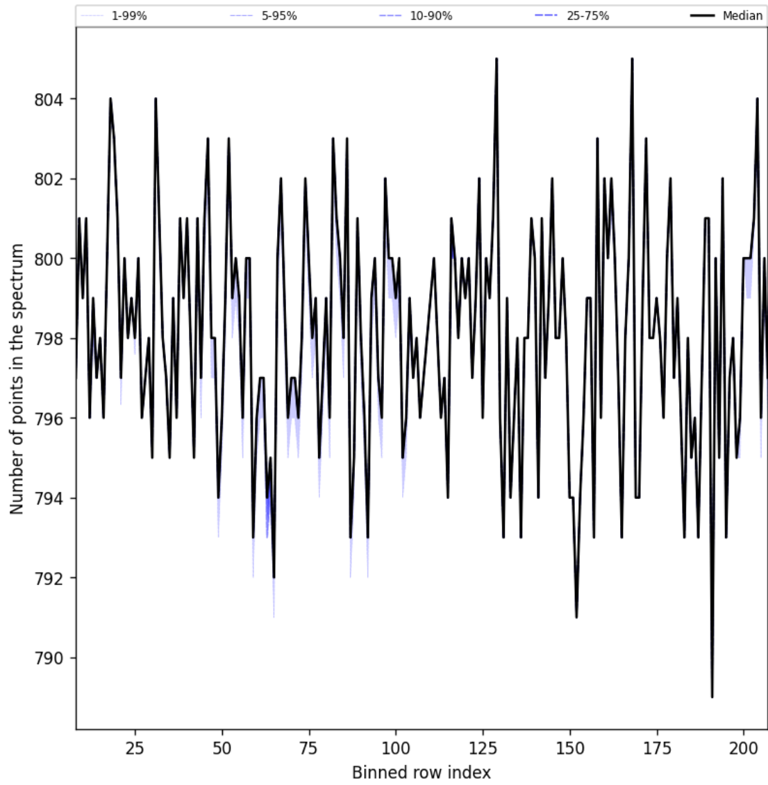
Figure 37: Along track statistics of “Number of points in the spectrum” for 2025-01-17 to 2025-01-19
