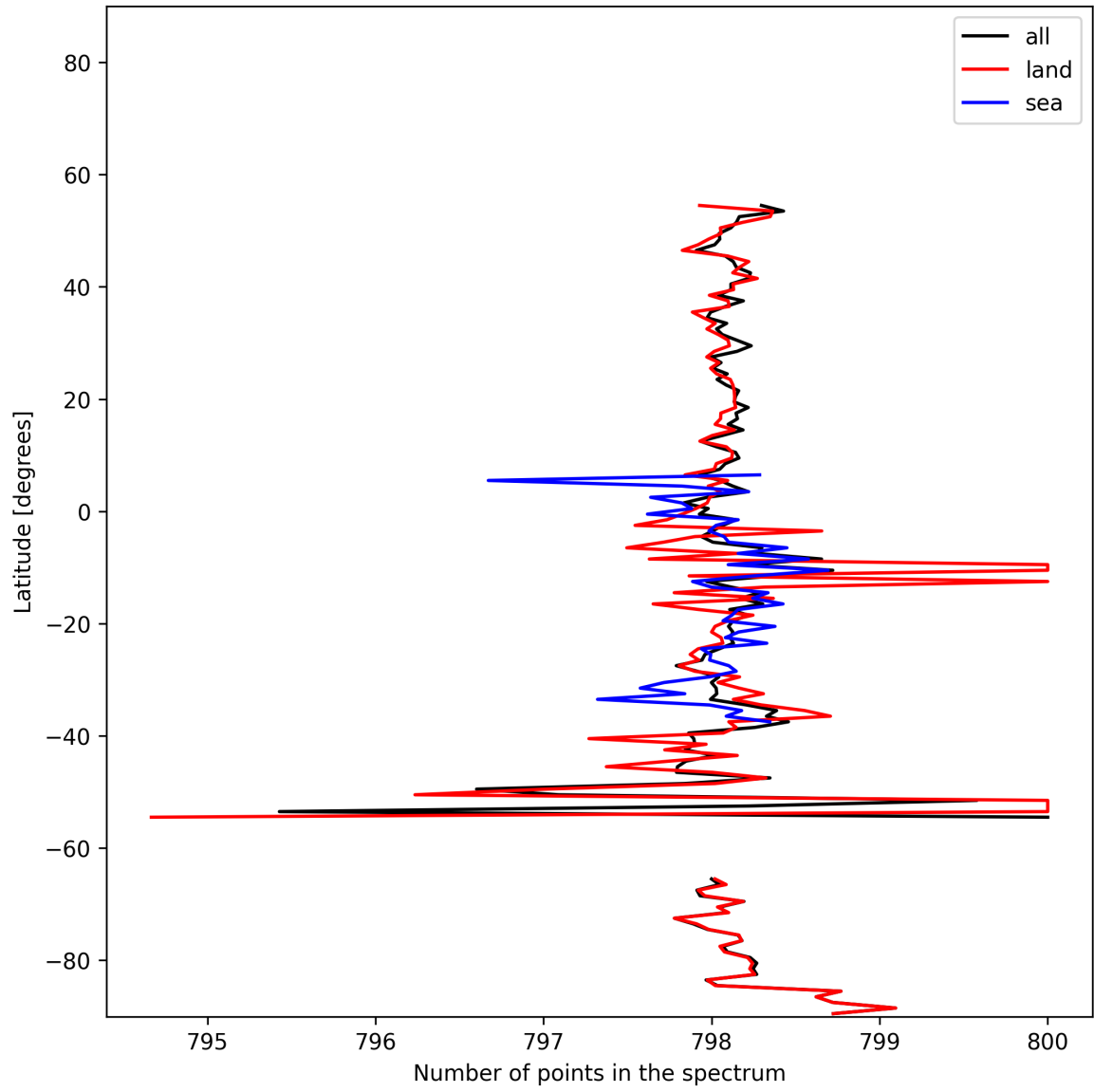
Figure 15: Zonal average of “Number of points in the spectrum” for 2025-01-17 to 2025-01-19.
