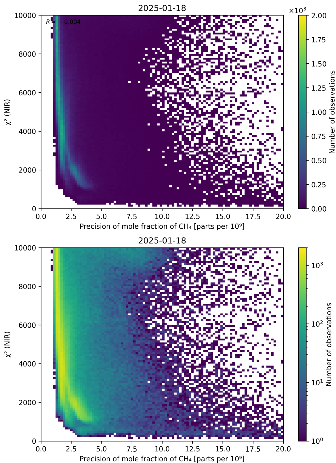
Figure 78: Scatter density plot of “Precision of mole fraction of \text{CH}_4 ” against “ \chi^2 (NIR)” for 2025-01-17 to 2025-01-19.
