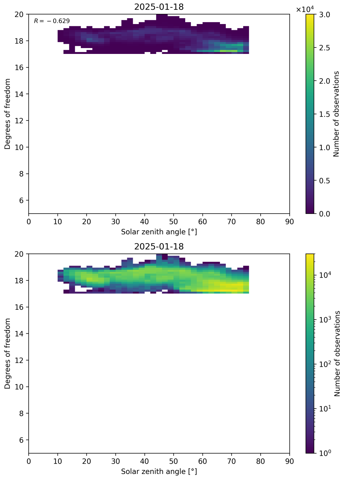
Figure 96: Scatter density plot of “Solar zenith angle” against “Degrees of freedom” for 2025-01-17 to 2025-01-19.
