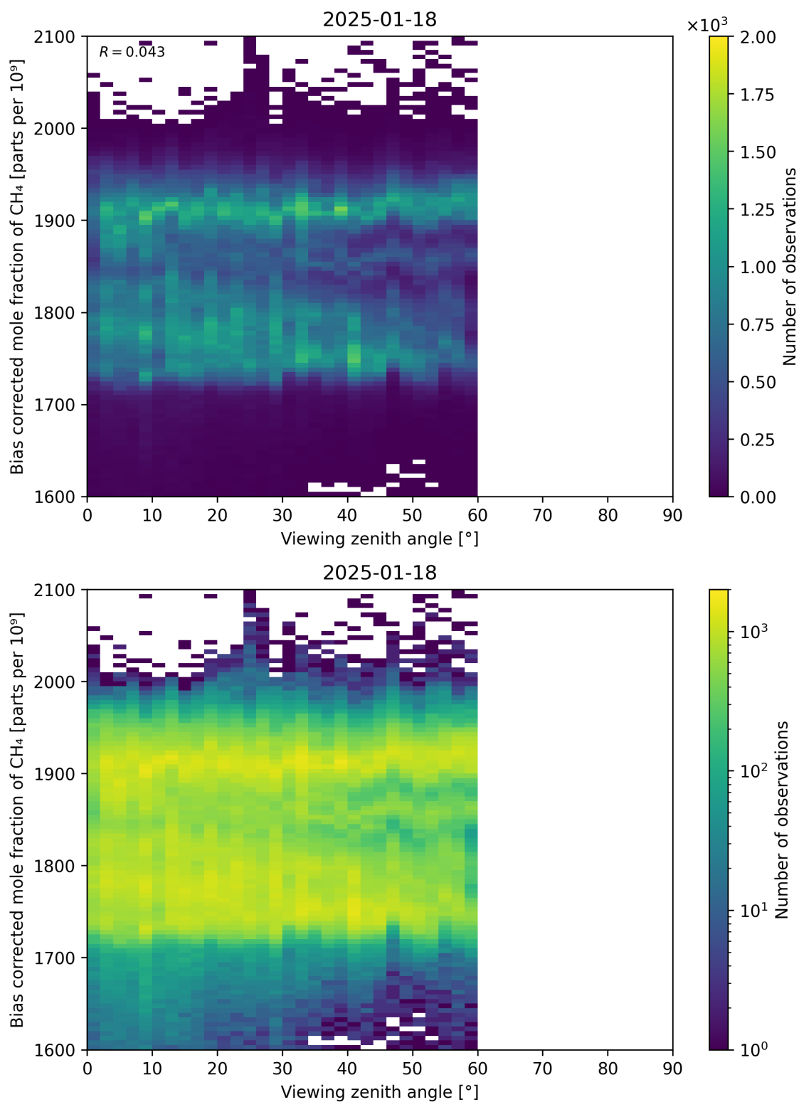
Figure 111: Scatter density plot of “Viewing zenith angle” against “Bias corrected mole fraction of CH 4 ” for 2025-01-17 to 2025-01-19.
