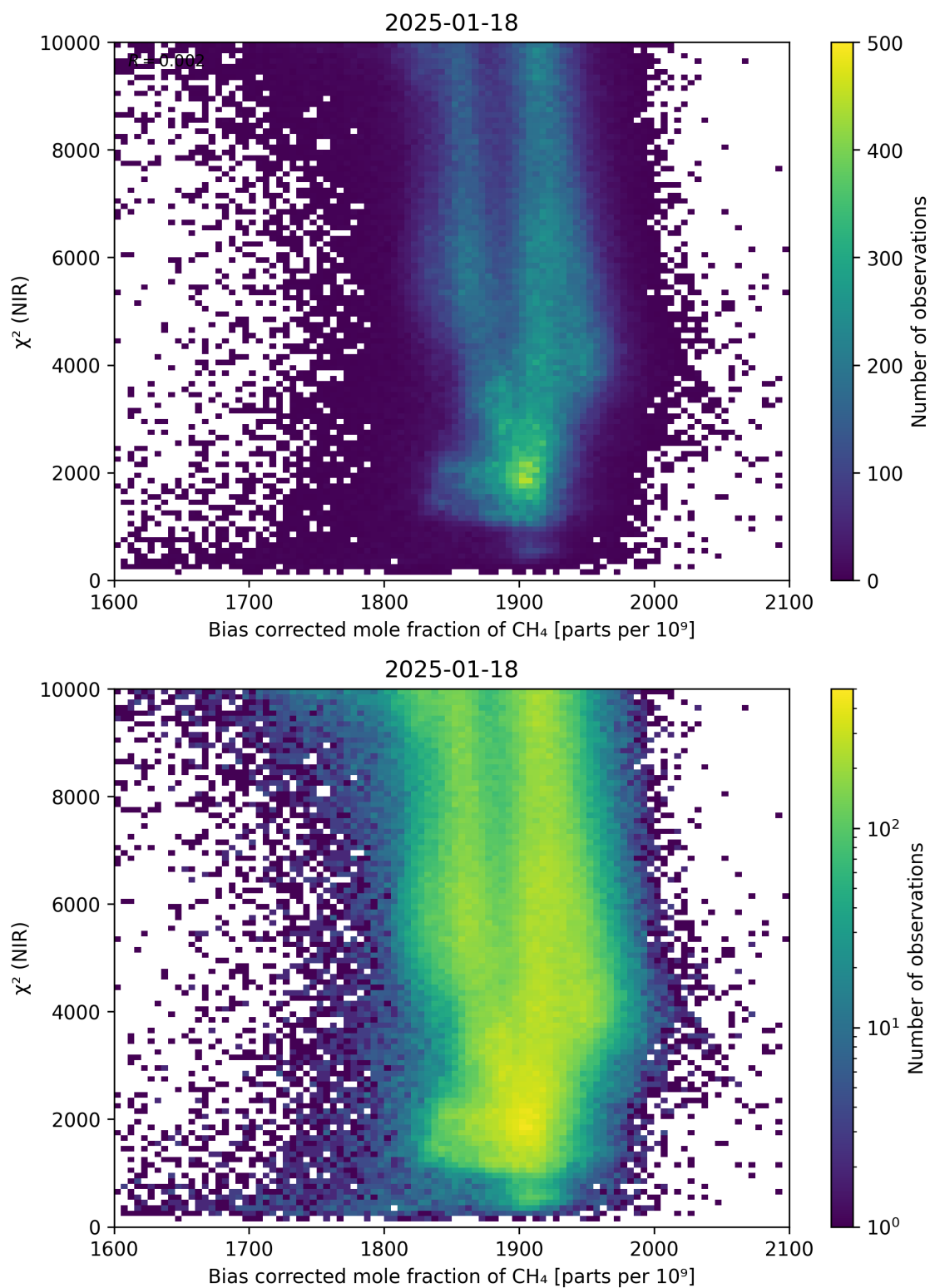
Figure 63: Scatter density plot of “Bias corrected mole fraction of \text{CH}_4 ” against “ \chi^2 (NIR)” for 2025-01-17 to 2025-01-19.
