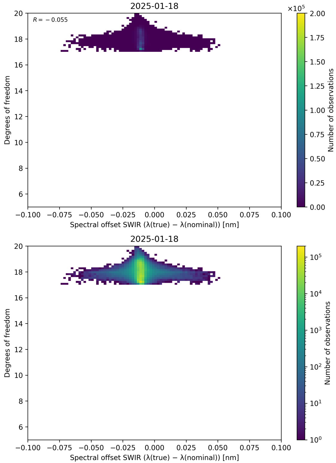
Figure 119: Scatter density plot of “Spectral offset SWIR ( \lambda_{\text{true}} - \lambda_{\text{nominal}} )” against “Degrees of freedom” for 2025-01-17 to 2025-01-19.
