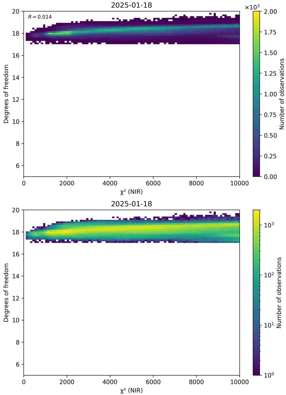
Figure 44: Scatter density plot of “ \chi^2 (NIR)” against “Degrees of freedom” for 2025-01-17 to 2025-01-19.
