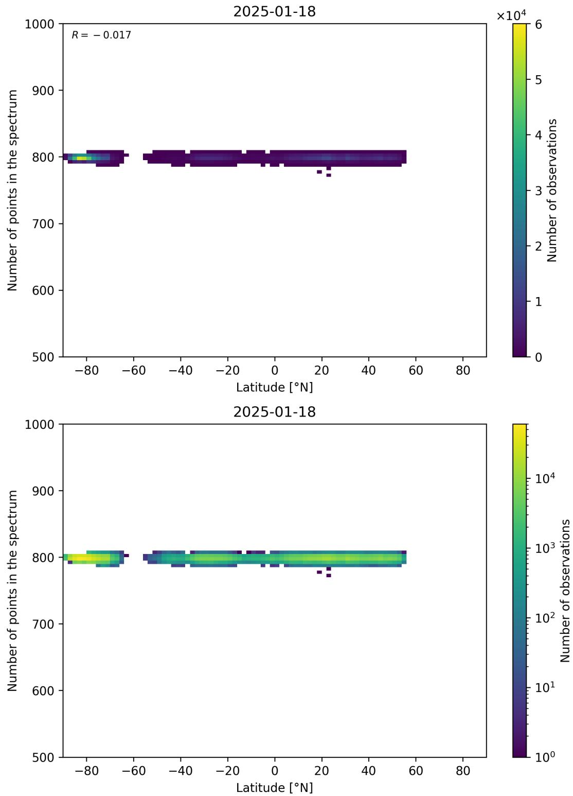
Figure 61: Scatter density plot of “Latitude” against “Number of points in the spectrum” for 2025-01-17 to 2025-01-19.
