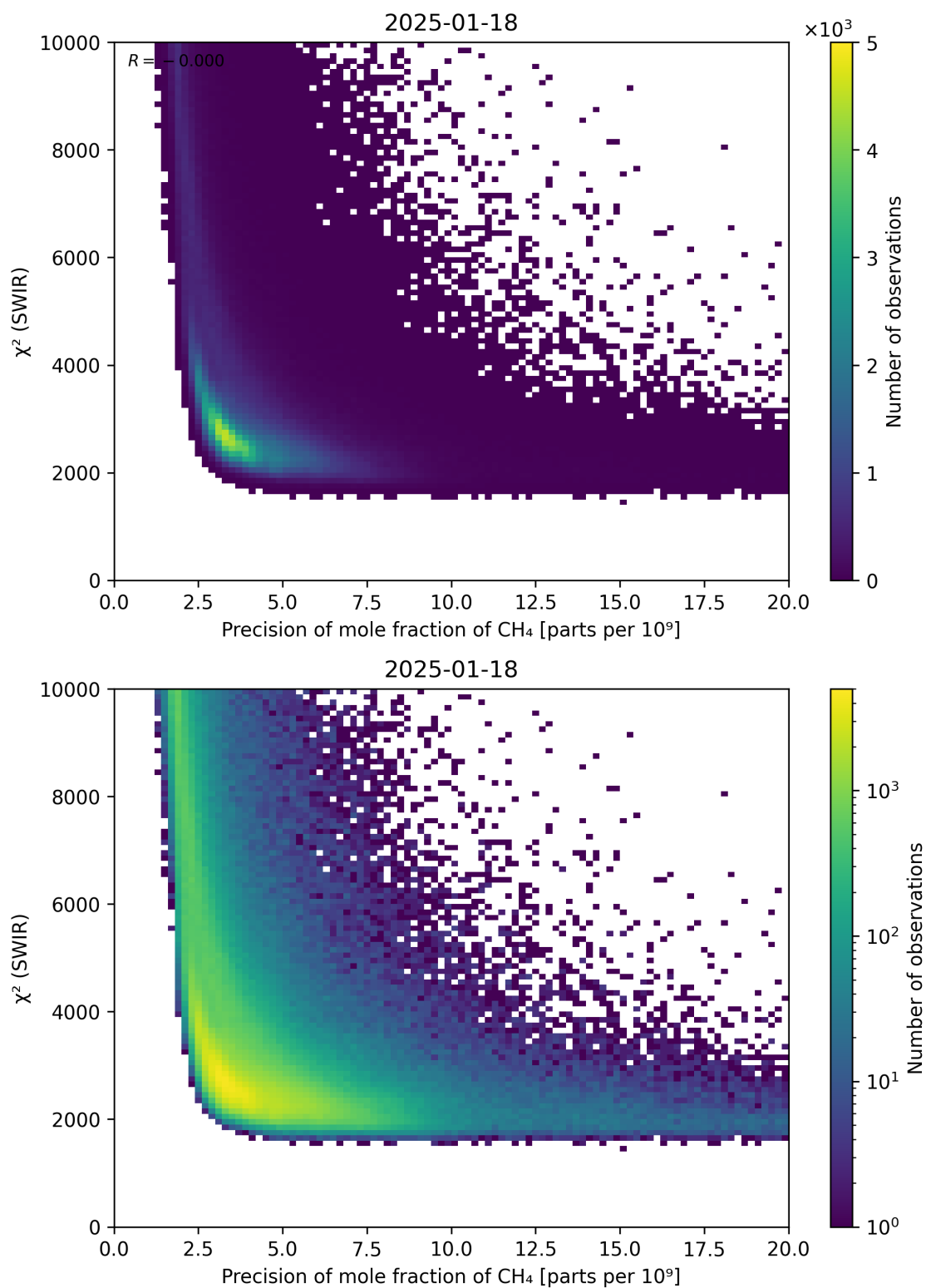
Figure 79: Scatter density plot of “Precision of mole fraction of CH 4 ” against “ \chi^2 (SWIR)” for 2025-01-17 to 2025-01-19.
