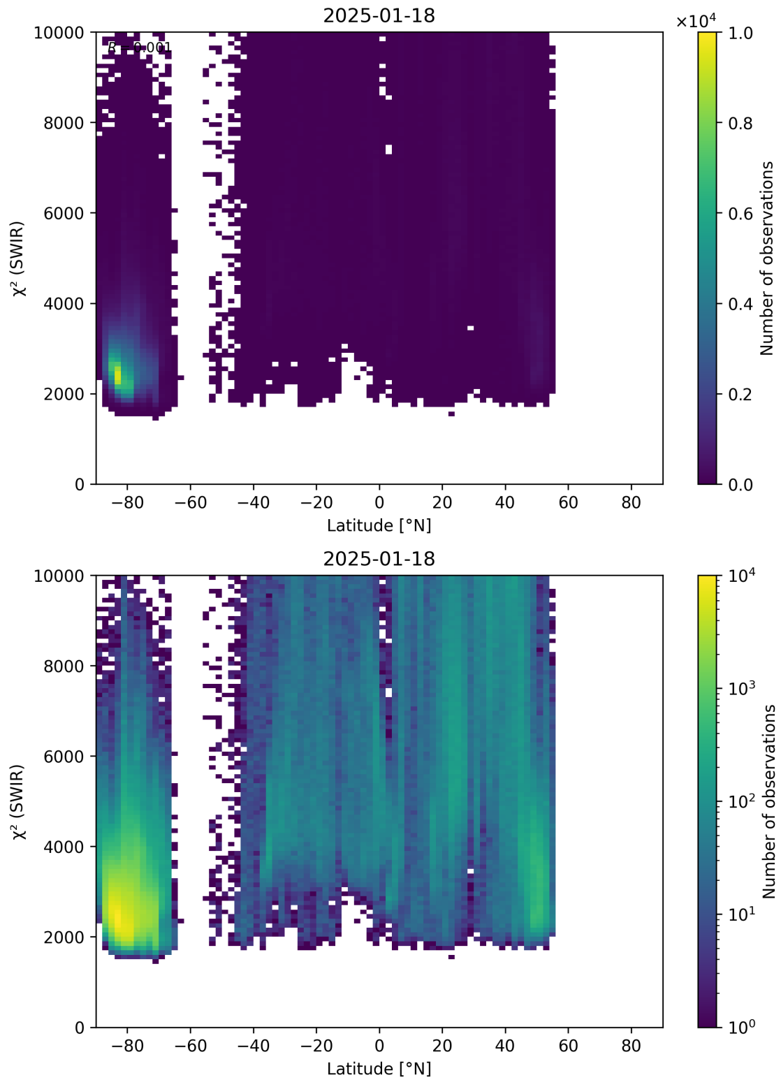
Figure 54: Scatter density plot of “Latitude” against “ \chi^2 (SWIR)” for 2025-01-17 to 2025-01-19.
