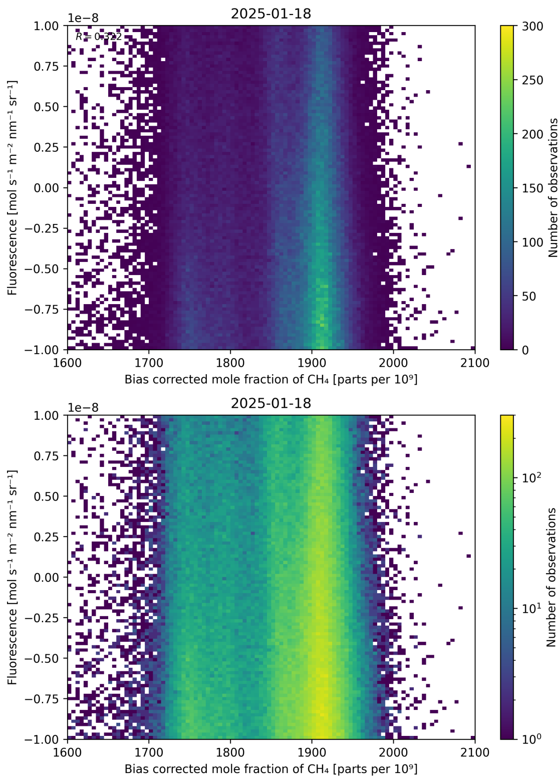
Figure 66: Scatter density plot of “Bias corrected mole fraction of \text{CH}_4 ” against “Fluorescence” for 2025-01-17 to 2025-01-19.
