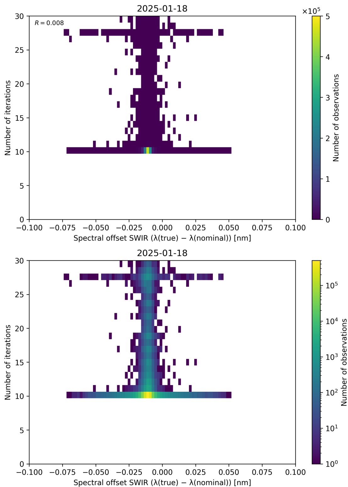
Figure 121: Scatter density plot of “Spectral offset SWIR ( \lambda_{\text{true}} - \lambda_{\text{nominal}} )” against “Number of iterations” for 2025-01-17 to 2025-01-19.
