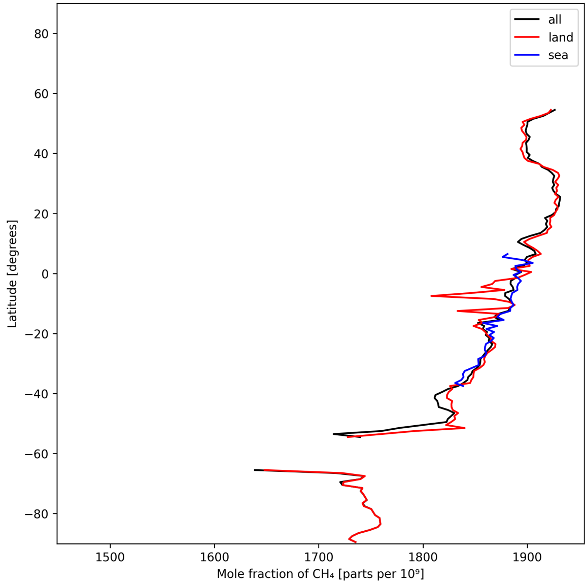
Figure 12: Zonal average of “Mole fraction of \text{CH}_4 ” for 2025-01-17 to 2025-01-19.
