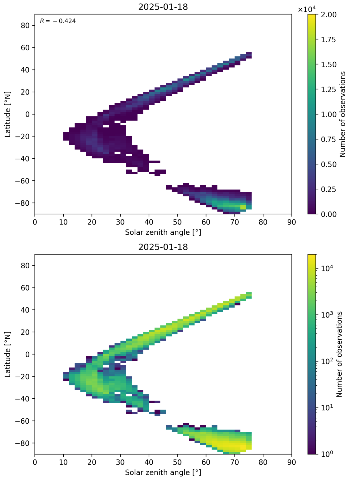
Figure 98: Scatter density plot of “Solar zenith angle” against “Latitude” for 2025-01-17 to 2025-01-19.
