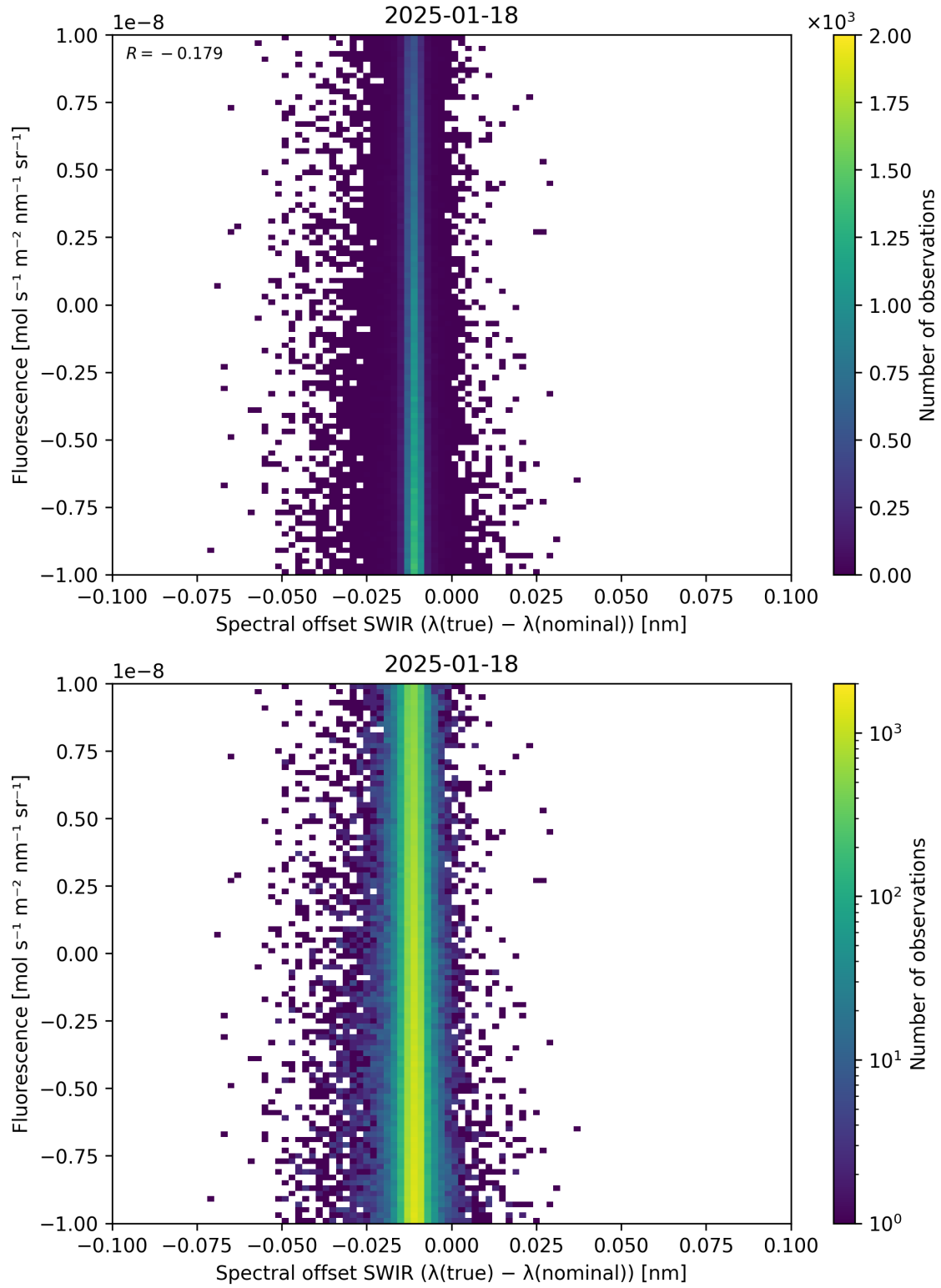
Figure 120: Scatter density plot of “Spectral offset SWIR ( \lambda_{\text{true}} - \lambda_{\text{nominal}} )” against “Fluorescence” for 2025-01-17 to 2025-01-19.
