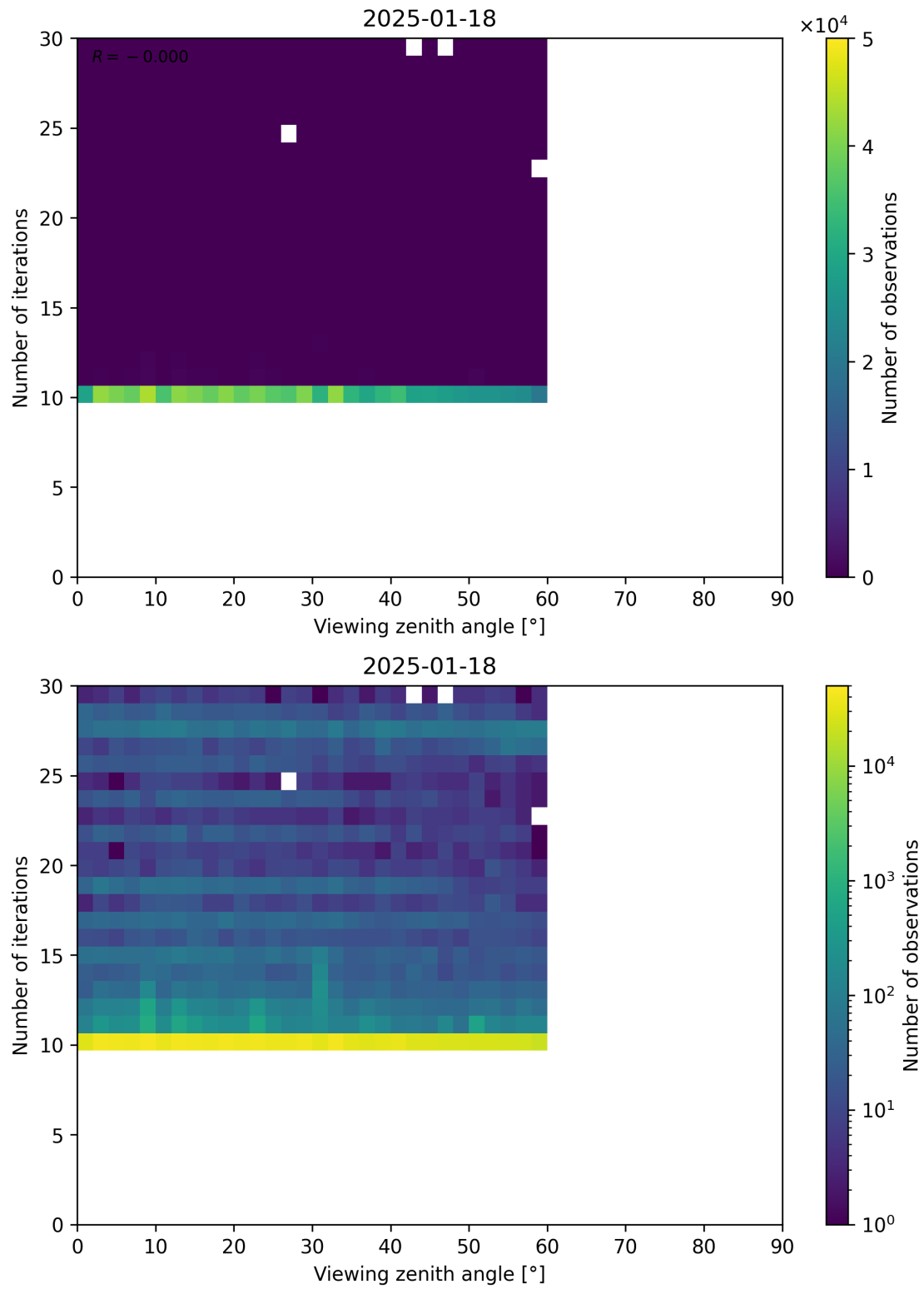
Figure 113: Scatter density plot of “Viewing zenith angle” against “Number of iterations” for 2025-01-17 to 2025-01-19.
