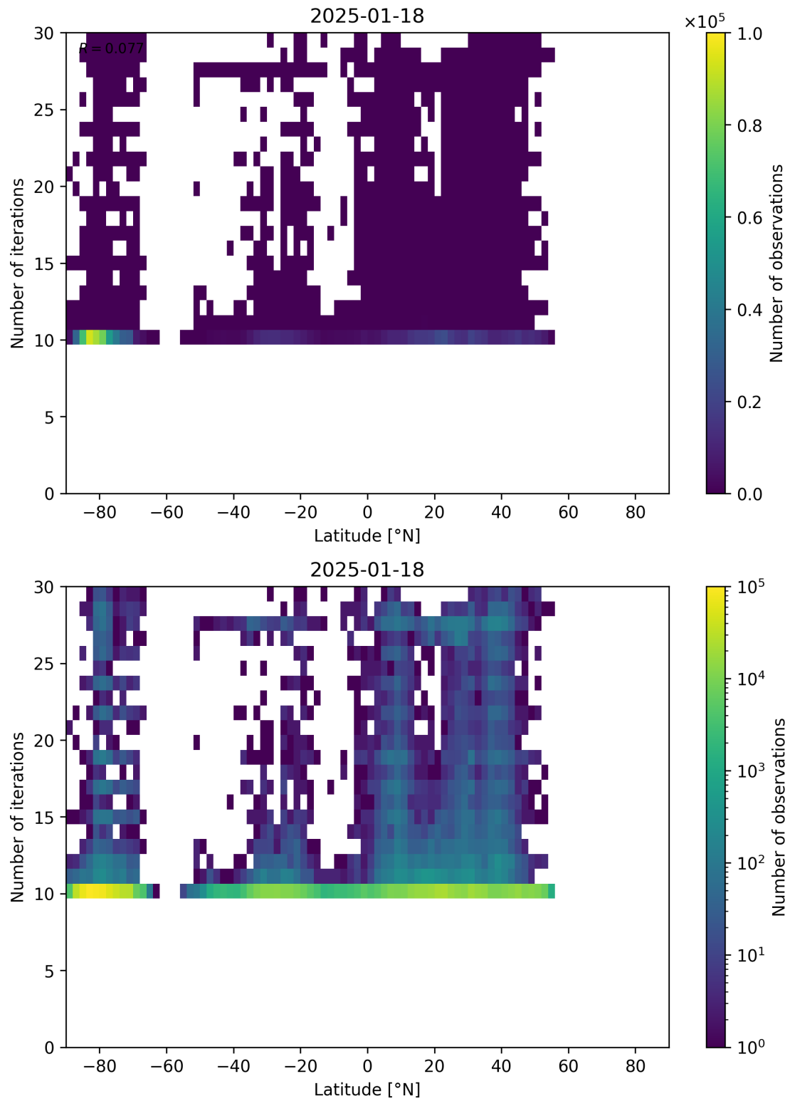
Figure 60: Scatter density plot of “Latitude” against “Number of iterations” for 2025-01-17 to 2025-01-19.
