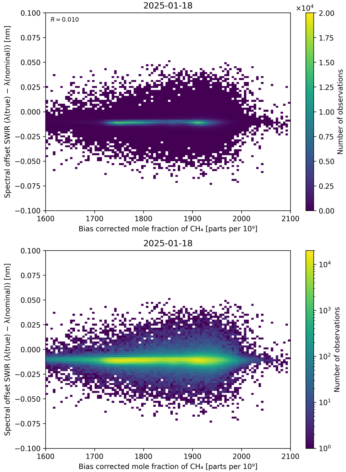
Figure 69: Scatter density plot of “Bias corrected mole fraction of \text{CH}_4 ” against “Spectral offset SWIR ( \lambda_{\text{true}} - \lambda_{\text{nominal}} )” for 2025-01-17 to 2025-01-19.
