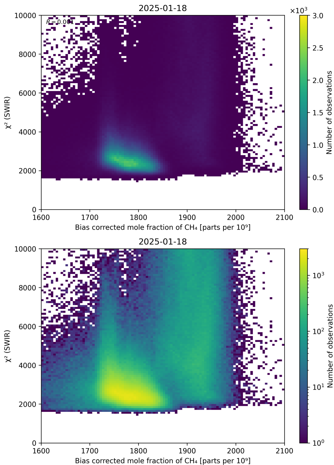
Figure 64: Scatter density plot of “Bias corrected mole fraction of CH 4 ” against “ \chi^2 (SWIR)” for 2025-01-17 to 2025-01-19.
