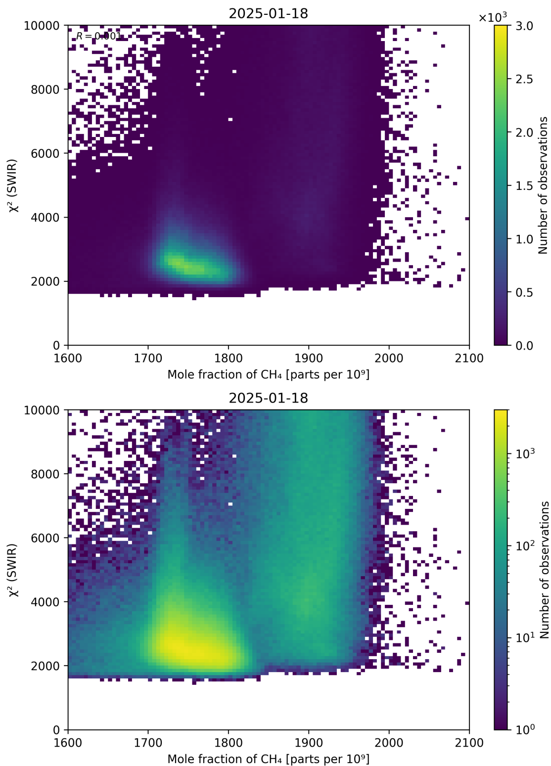
Figure 71: Scatter density plot of “Mole fraction of \text{CH}_4 ” against “ \chi^2 (SWIR)” for 2025-01-17 to 2025-01-19.
