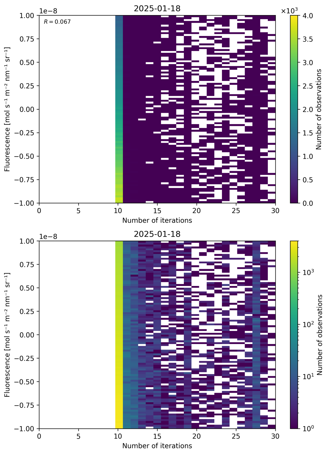
Figure 87: Scatter density plot of “Number of iterations” against “Fluorescence” for 2025-01-17 to 2025-01-19.
