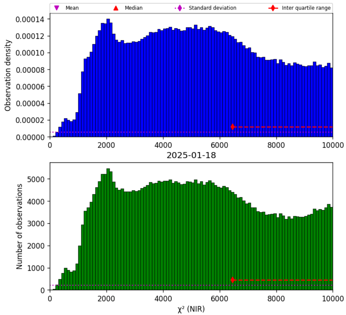
Figure 29: Histogram of " \chi^2 (NIR)" for 2025-01-17 to 2025-01-19
