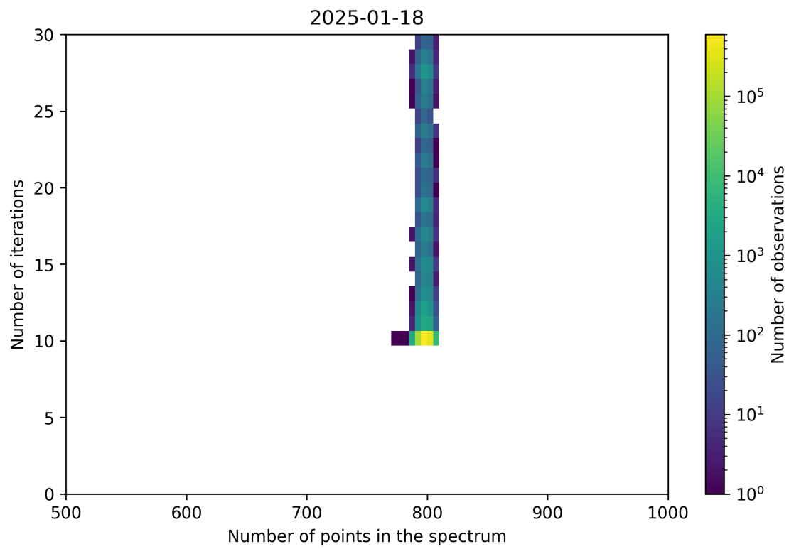
Figure 92: Scatter density plot of “Number of points in the spectrum” against “Number of iterations” for 2025-01-17 to 2025-01-19.
