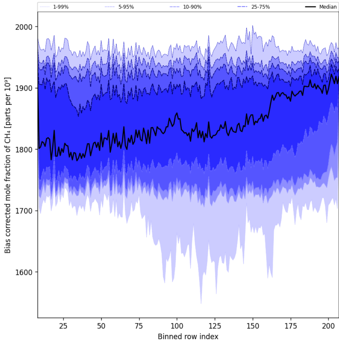
Figure 36: Along track statistics of “Bias corrected mole fraction of CH 4 ” for 2025-01-17 to 2025-01-19
