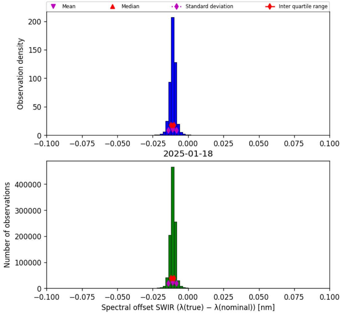
Figure 27: Histogram of “Spectral offset SWIR ( \lambda_{\text{true}} - \lambda_{\text{nominal}} )” for 2025-01-17 to 2025-01-19
