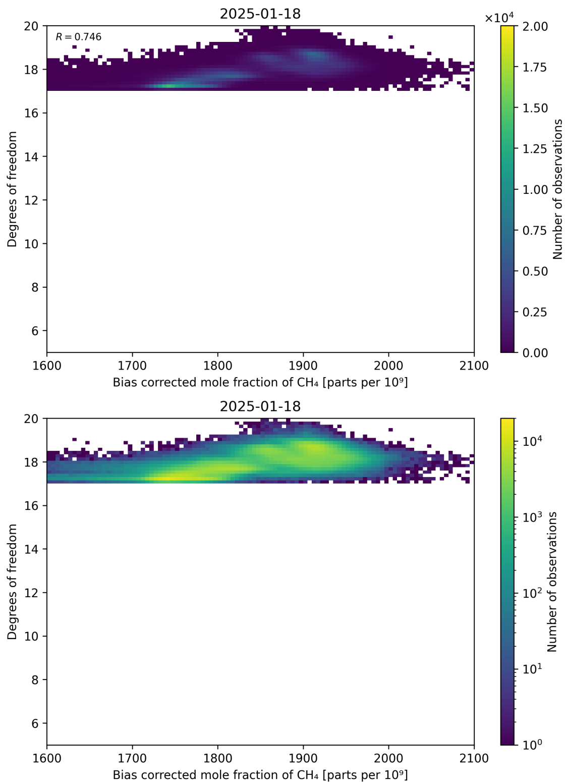
Figure 65: Scatter density plot of “Bias corrected mole fraction of CH 4 ” against “Degrees of freedom” for 2025-01-17 to 2025-01-19.
