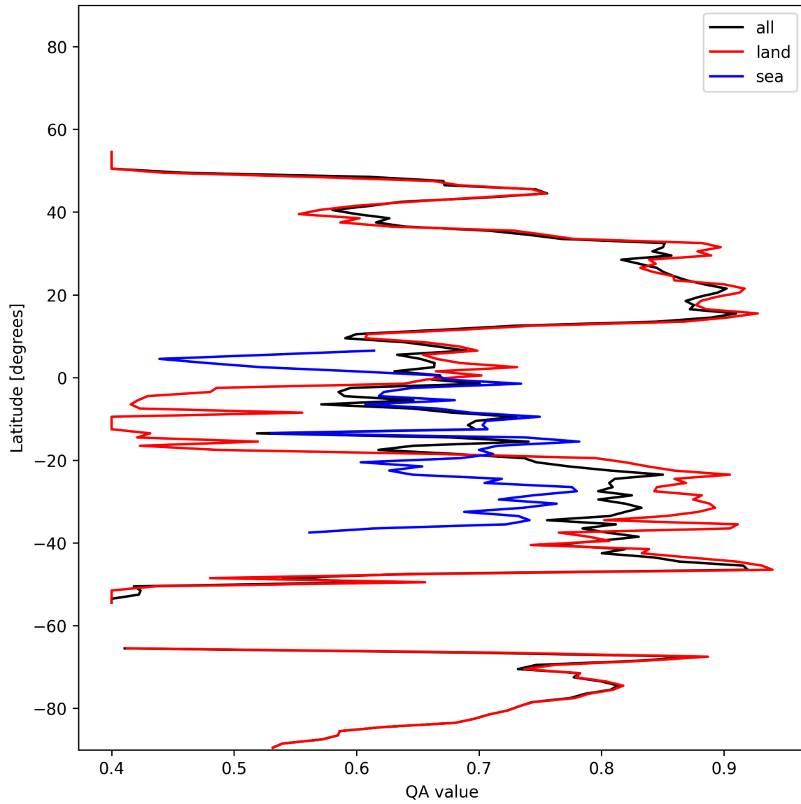
Figure 11: Zonal average of “QA value” for 2025-01-17 to 2025-01-19.
