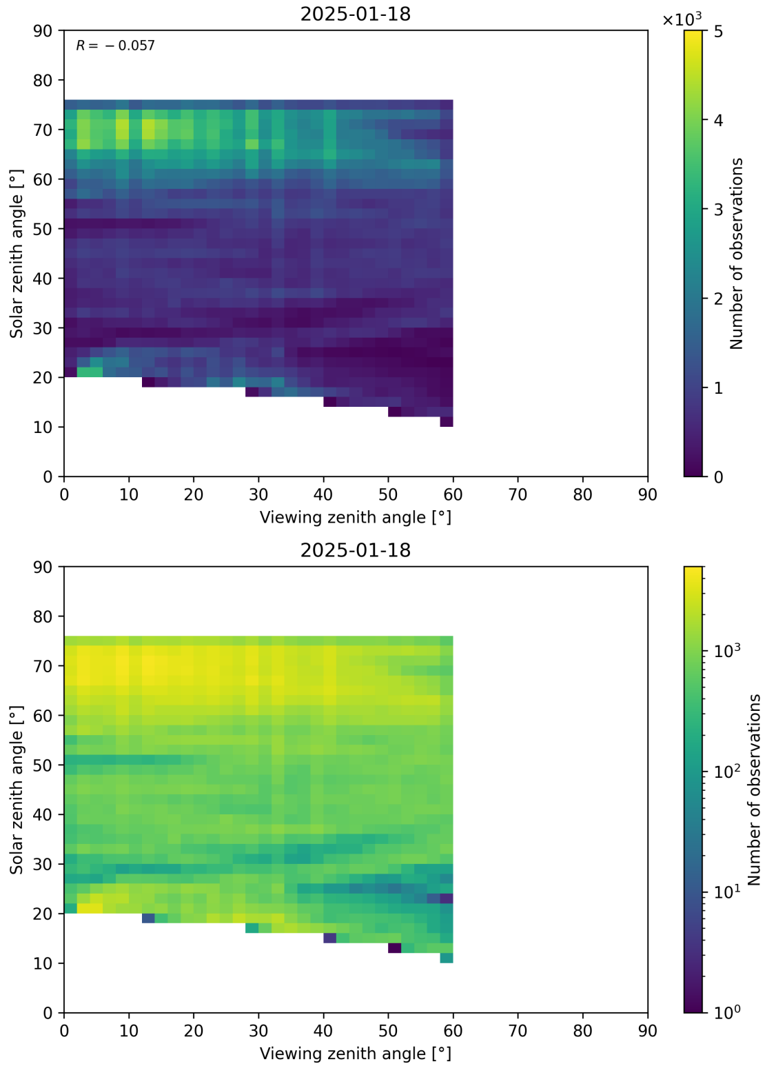
Figure 115: Scatter density plot of “Viewing zenith angle” against “Solar zenith angle” for 2025-01-17 to 2025-01-19.
