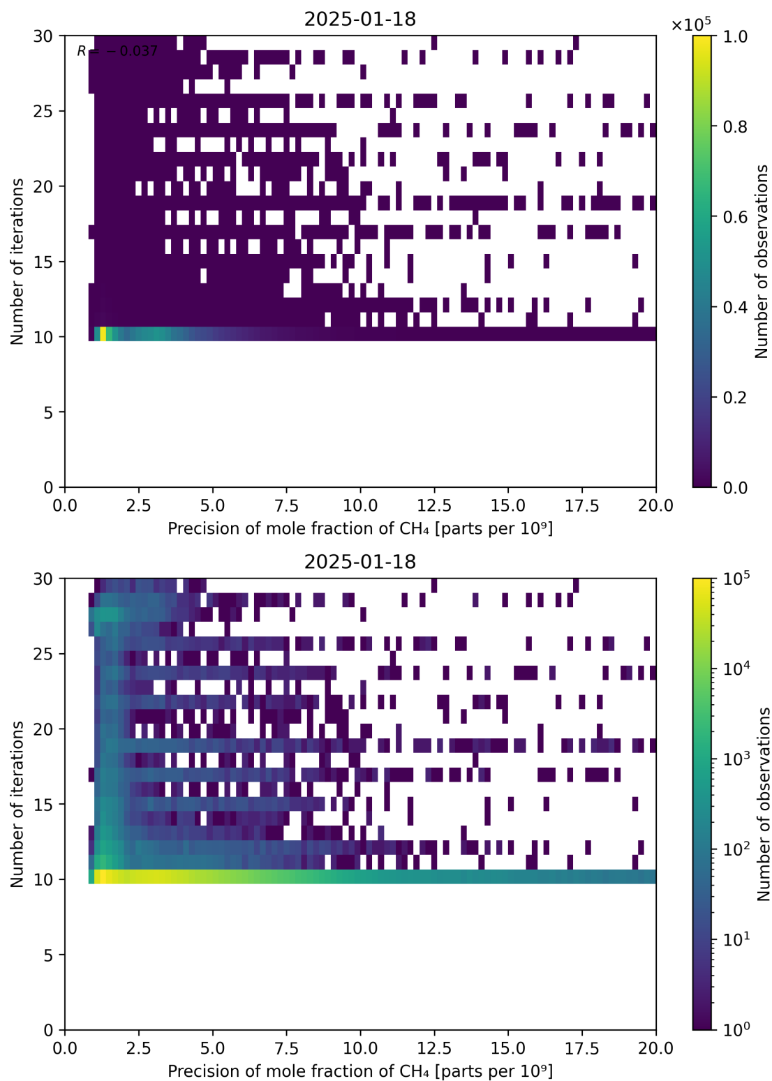
Figure 83: Scatter density plot of “Precision of mole fraction of CH 4 ” against “Number of iterations” for 2025-01-17 to 2025-01-19.
