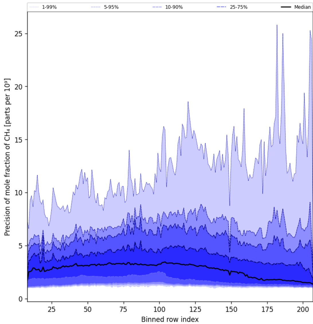
Figure 35: Along track statistics of “Precision of mole fraction of CH 4 ” for 2025-01-17 to 2025-01-19
