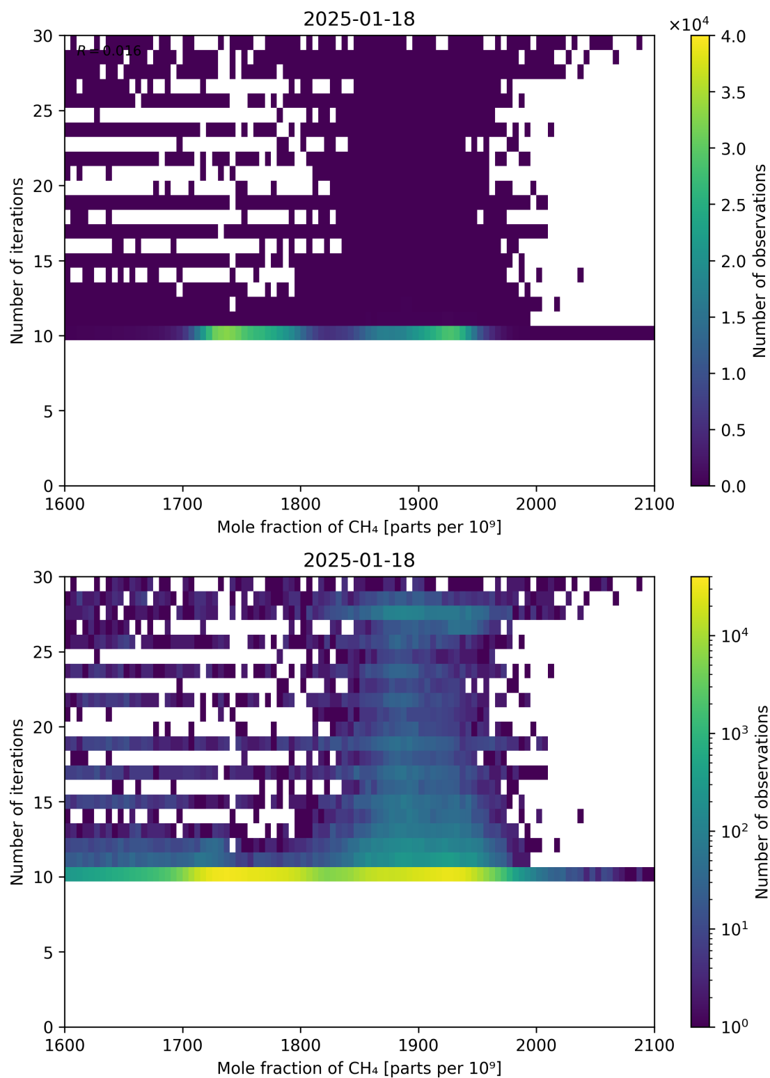
Figure 76: Scatter density plot of “Mole fraction of CH 4 ” against “Number of iterations” for 2025-01-17 to 2025-01-19.
