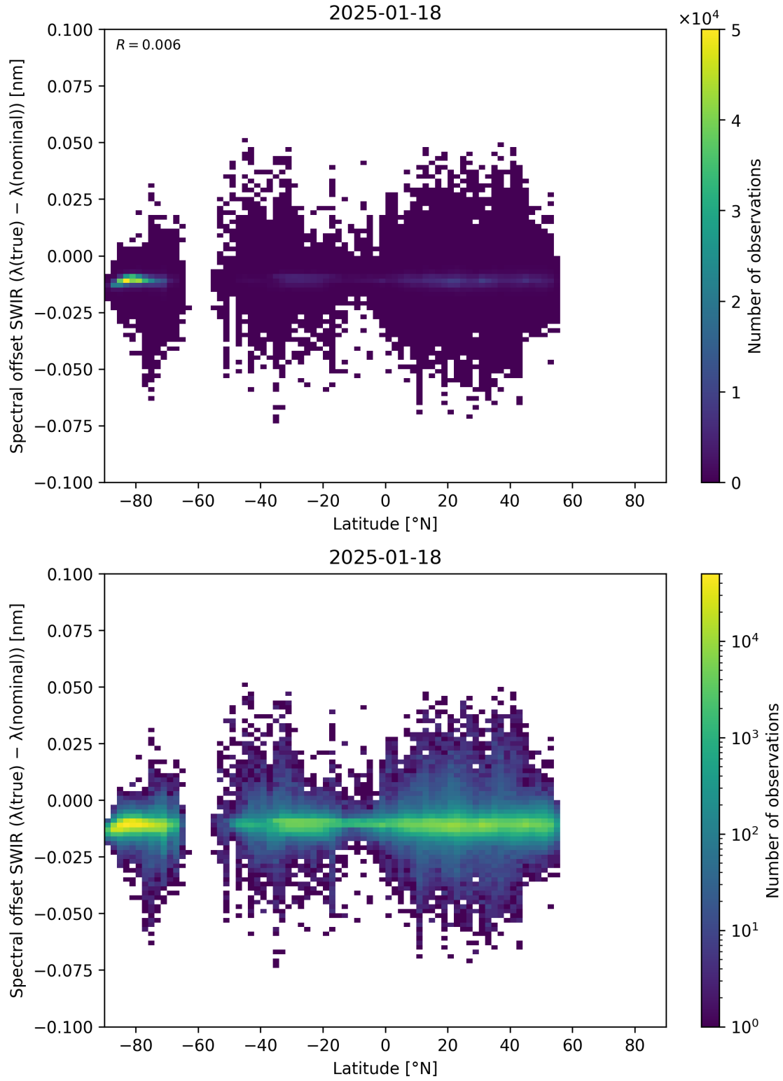
Figure 62: Scatter density plot of “Latitude” against “Spectral offset SWIR ( \lambda_{\text{true}} - \lambda_{\text{nominal}} )” for 2025-01-17 to 2025-01-19.
