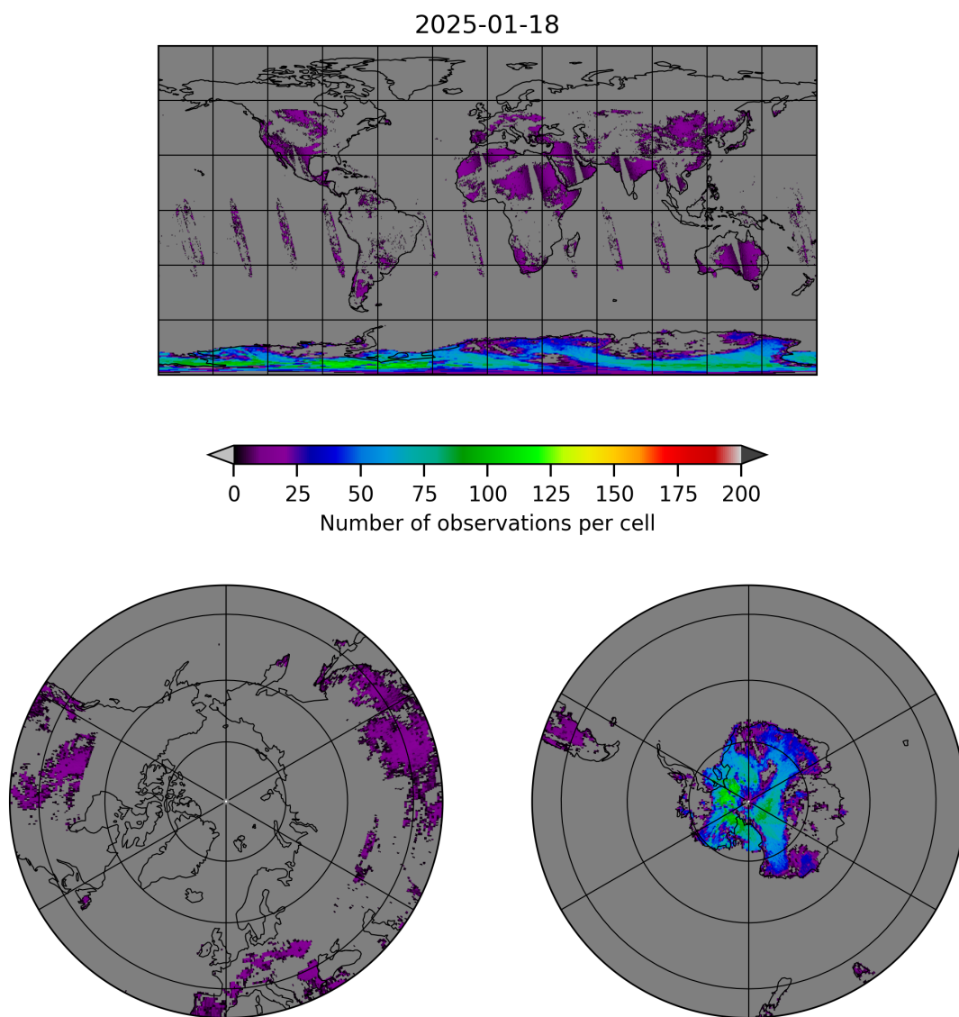
Figure 10: Map of the number of observations for 2025-01-17 to 2025-01-19
