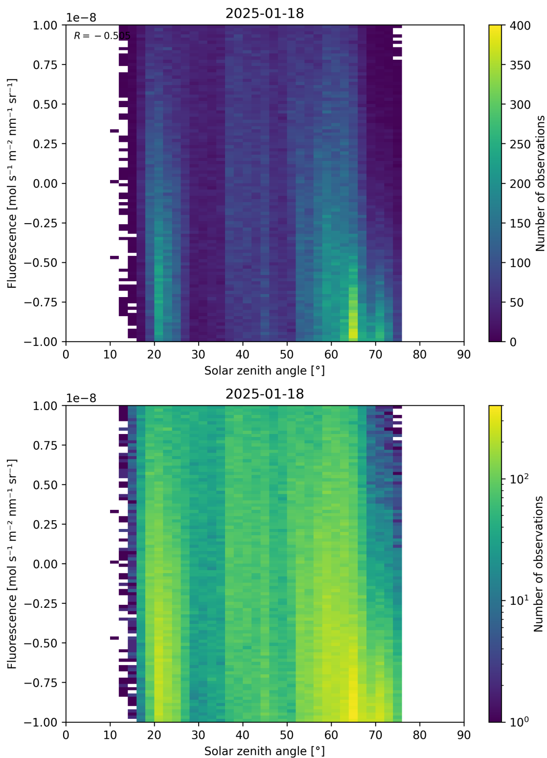
Figure 97: Scatter density plot of “Solar zenith angle” against “Fluorescence” for 2025-01-17 to 2025-01-19.
