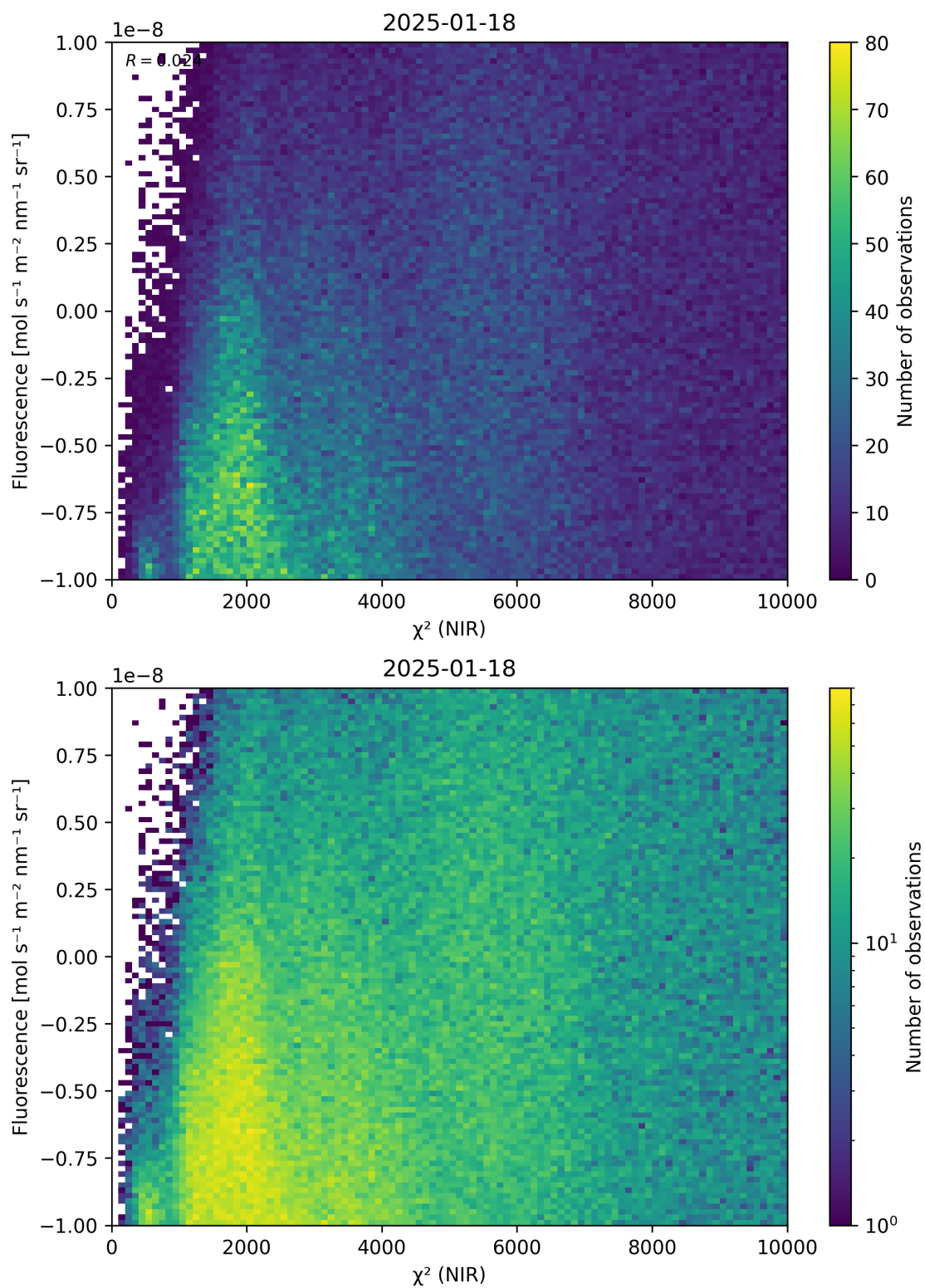
Figure 45: Scatter density plot of “ \chi^2 (NIR)” against “Fluorescence” for 2025-01-17 to 2025-01-19.
