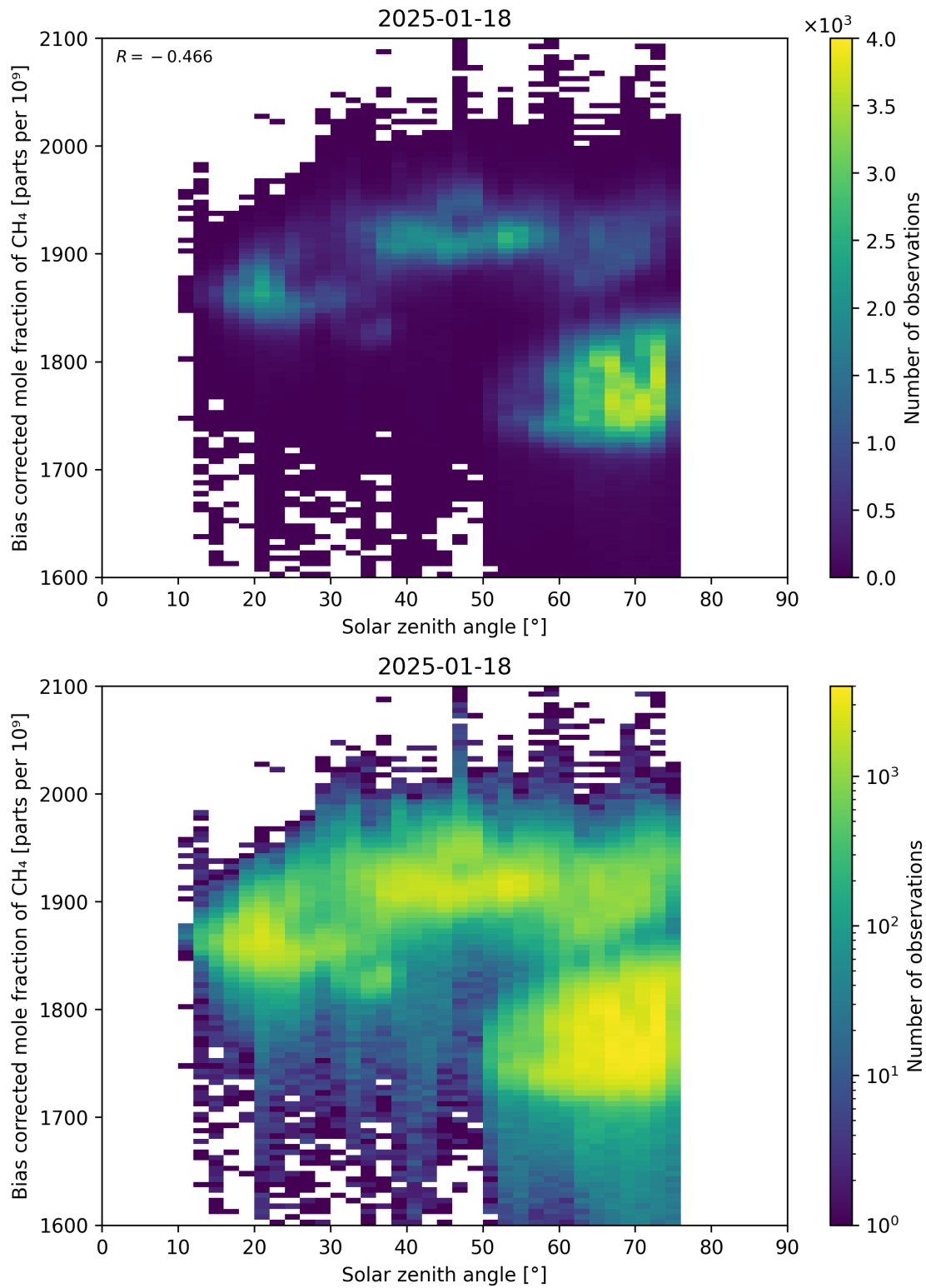
Figure 100: Scatter density plot of “Solar zenith angle” against “Bias corrected mole fraction of CH 4 ” for 2025-01-17 to 2025-01-19.
