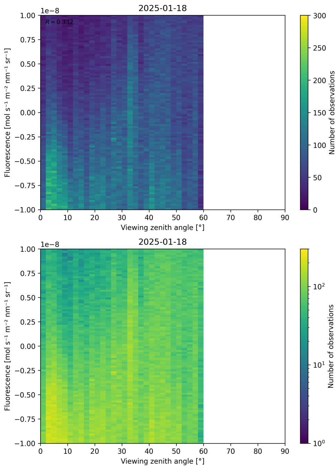
Figure 108: Scatter density plot of “Viewing zenith angle” against “Fluorescence” for 2025-01-17 to 2025-01-19.
