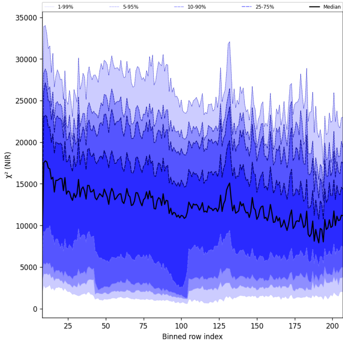
Figure 40: Along track statistics of “ \chi^2 (NIR)” for 2025-01-17 to 2025-01-19
