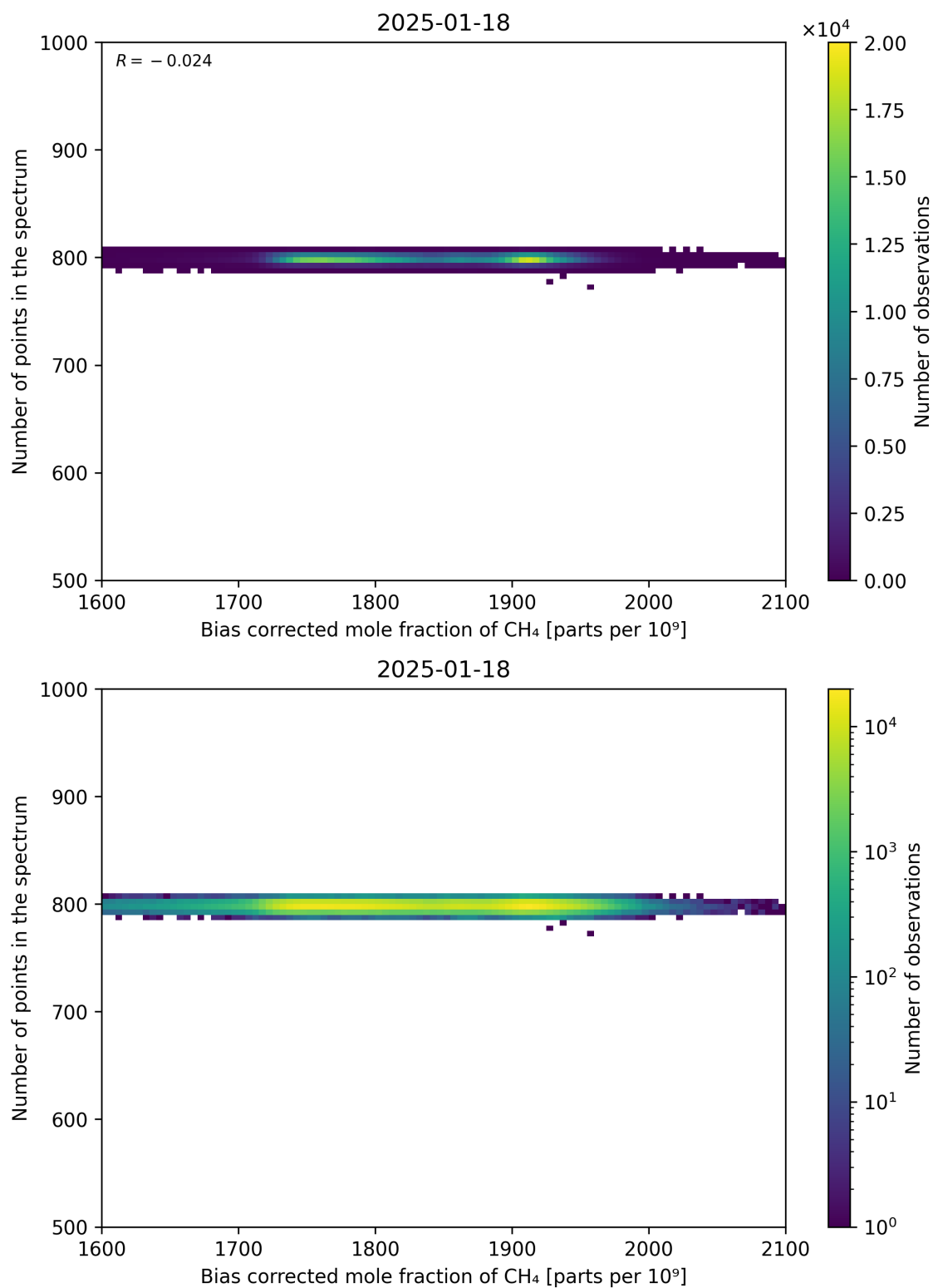
Figure 68: Scatter density plot of “Bias corrected mole fraction of CH 4 ” against “Number of points in the spectrum” for 2025-01-17 to 2025-01-19.
