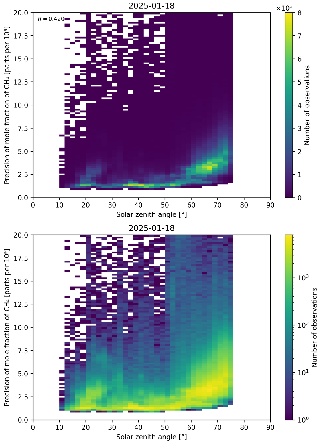
Figure 101: Scatter density plot of “Solar zenith angle” against “Precision of mole fraction of \text{CH}_4 ” for 2025-01-17 to 2025-01-19.
