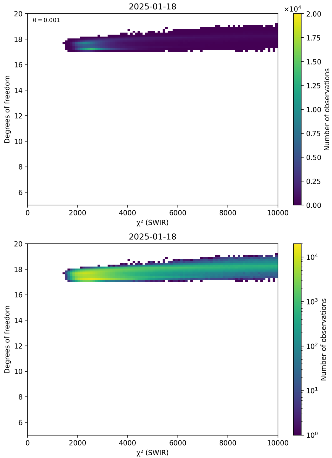
Figure 48: Scatter density plot of “ \chi^2 (SWIR)” against “Degrees of freedom” for 2025-01-17 to 2025-01-19.
