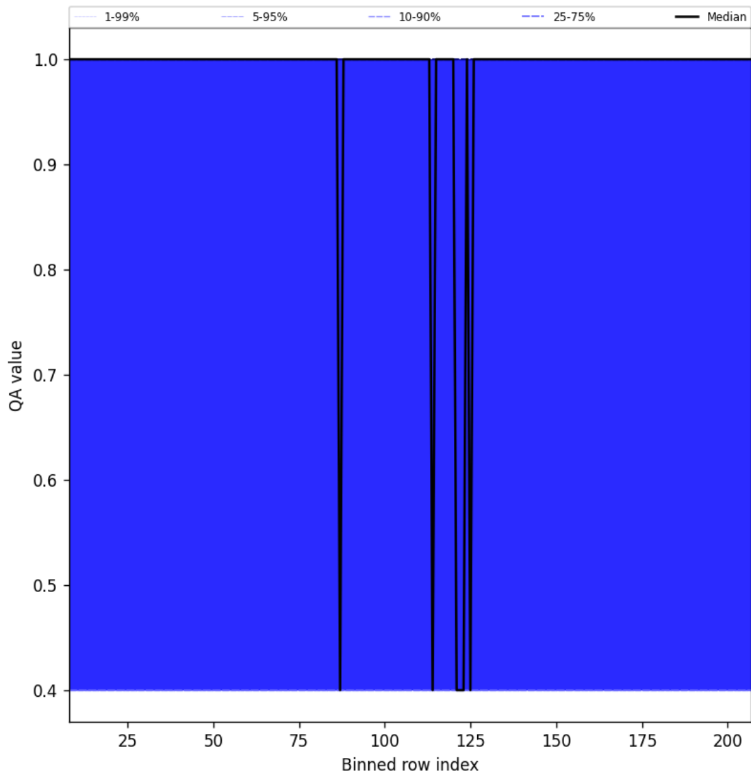
Figure 33: Along track statistics of “QA value” for 2025-01-17 to 2025-01-19
