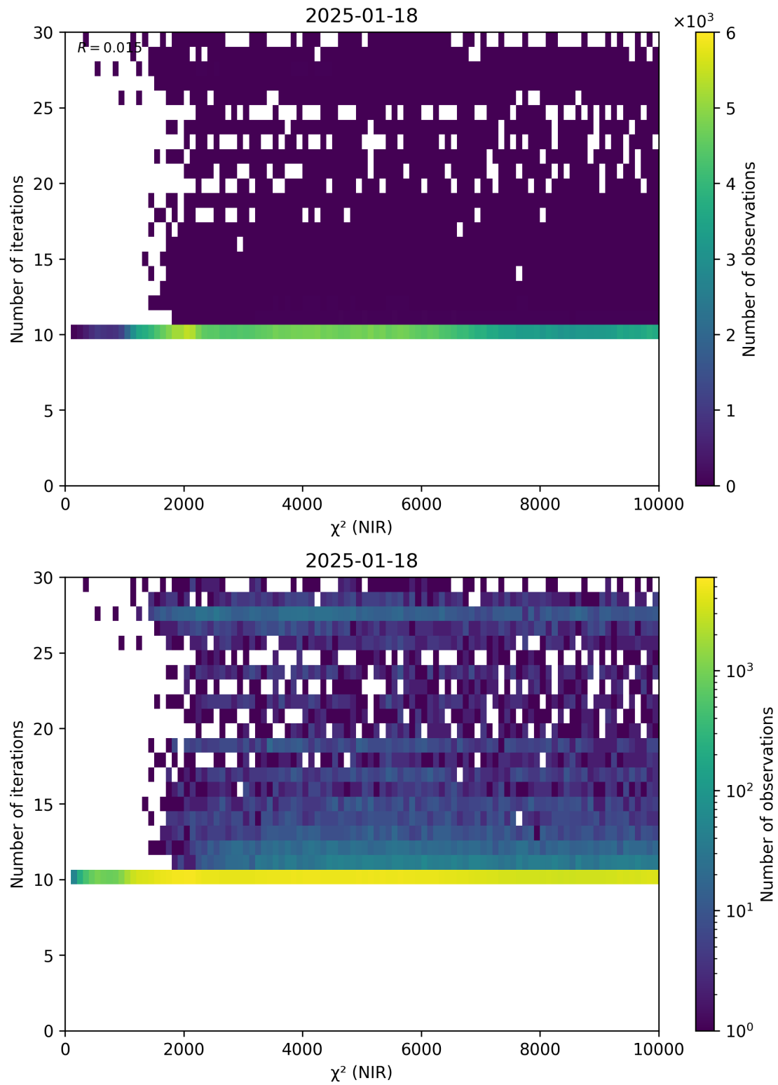
Figure 46: Scatter density plot of “ \chi^2 (NIR)” against “Number of iterations” for 2025-01-17 to 2025-01-19.
