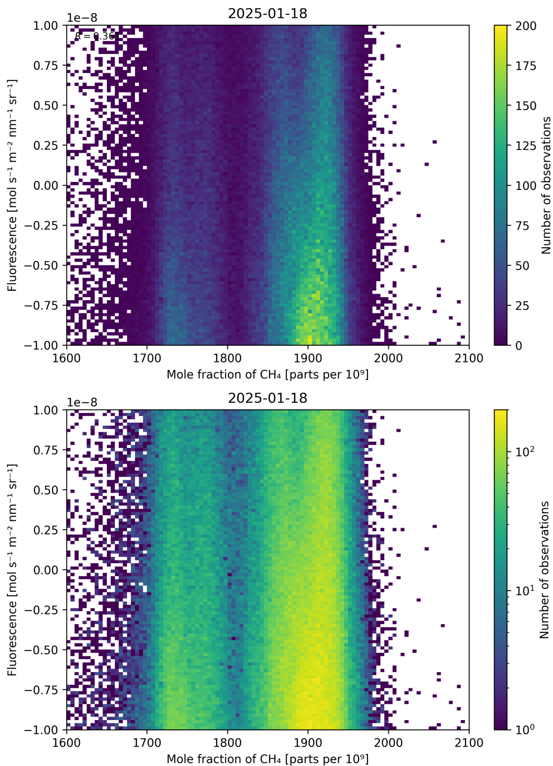
Figure 73: Scatter density plot of “Mole fraction of \text{CH}_4 ” against “Fluorescence” for 2025-01-17 to 2025-01-19.
