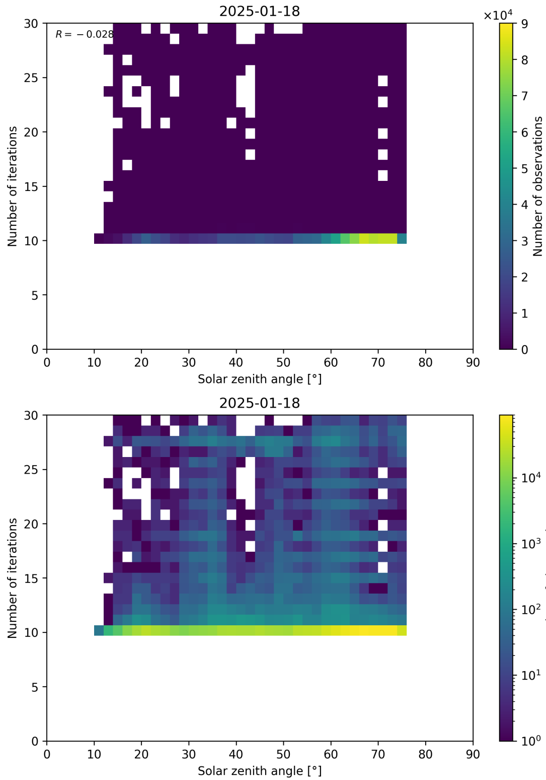
Figure 102: Scatter density plot of “Solar zenith angle” against “Number of iterations” for 2025-01-17 to 2025-01-19.
