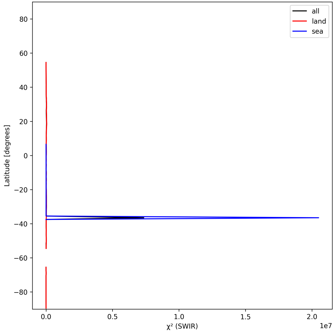
Figure 17: Zonal average of “ \chi^2 (SWIR)” for 2025-01-17 to 2025-01-19.
