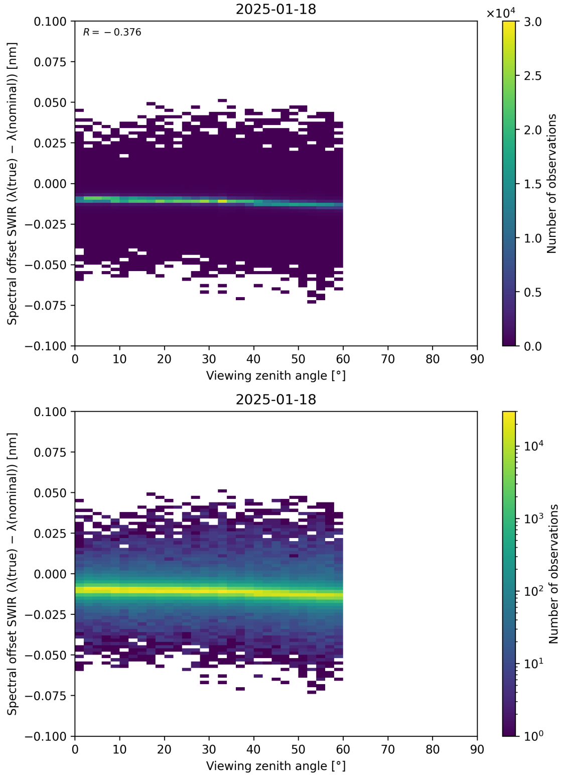
Figure 116: Scatter density plot of “Viewing zenith angle” against “Spectral offset SWIR ( \lambda_{\text{true}} - \lambda_{\text{nominal}} )” for 2025-01-17 to 2025-01-19.
