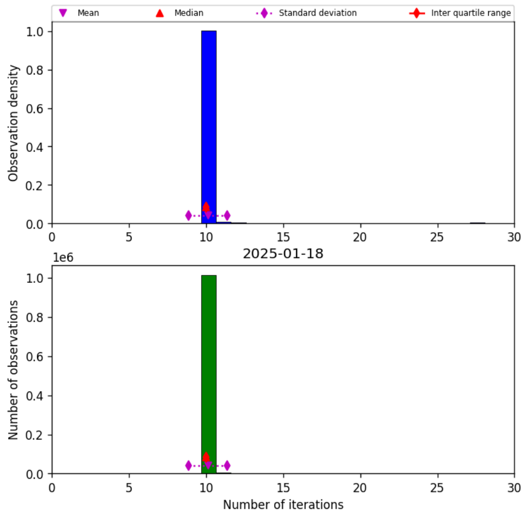
Figure 31: Histogram of “Number of iterations” for 2025-01-17 to 2025-01-19
