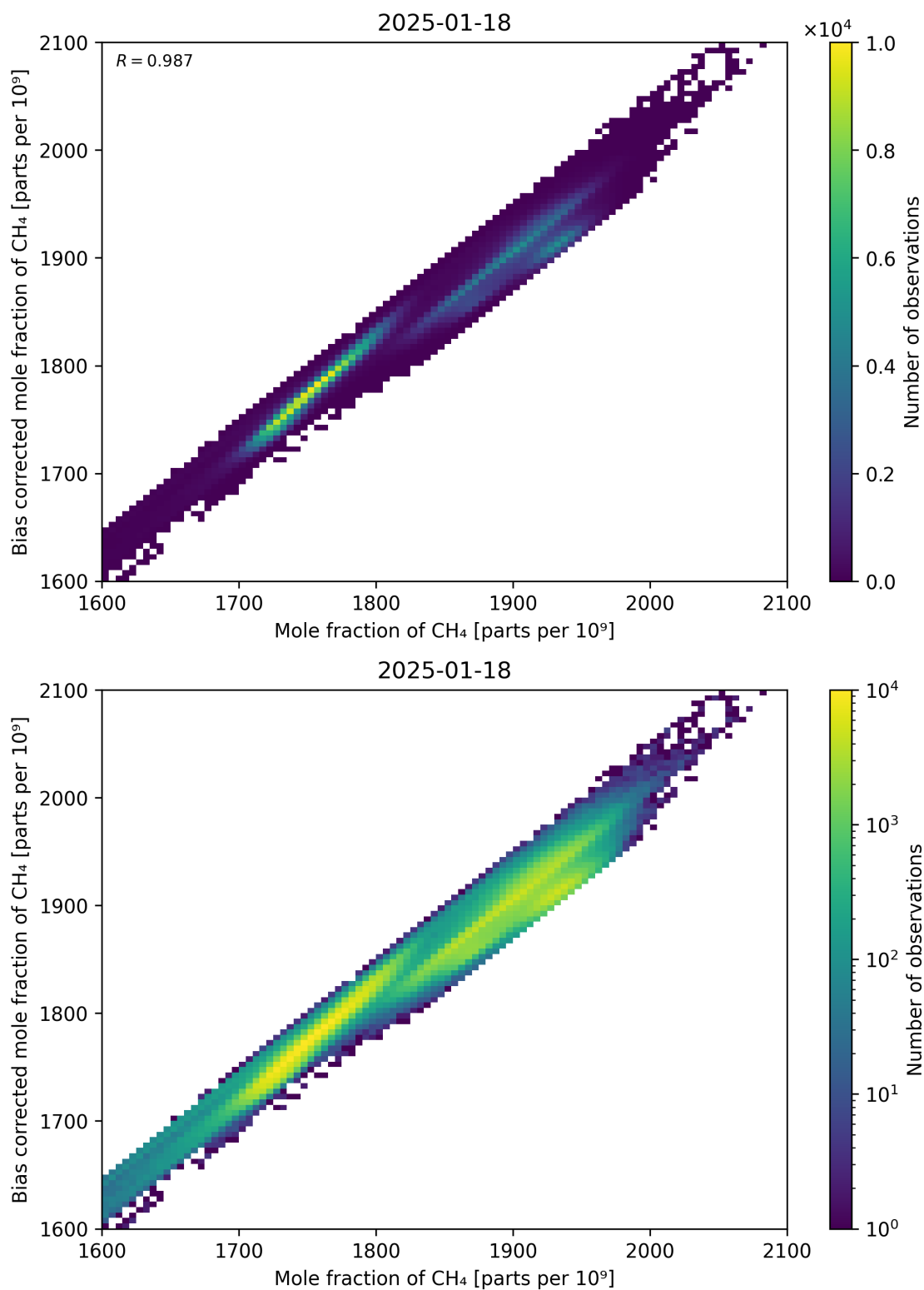
Figure 74: Scatter density plot of “Mole fraction of CH 4 ” against “Bias corrected mole fraction of CH 4 ” for 2025-01-17 to 2025-01-19.
