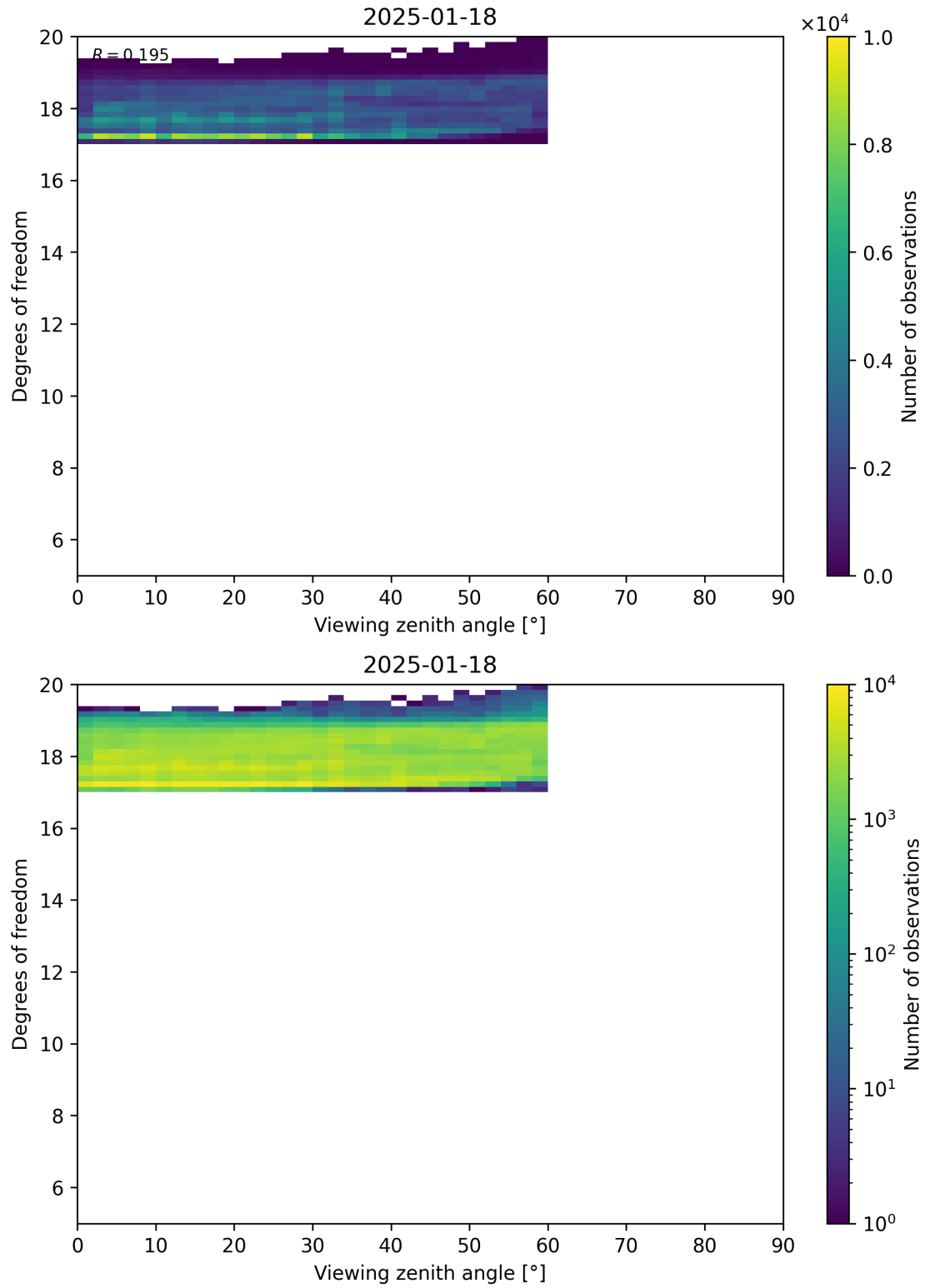
Figure 107: Scatter density plot of “Viewing zenith angle” against “Degrees of freedom” for 2025-01-17 to 2025-01-19.
