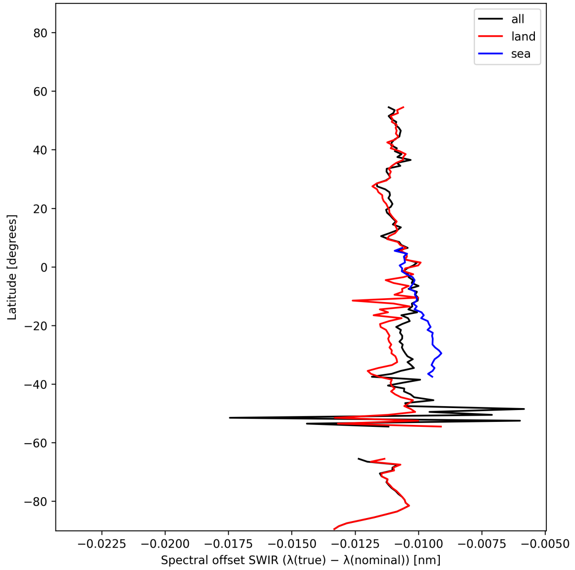
Figure 16: Zonal average of “Spectral offset SWIR ( \lambda_{\text{true}} - \lambda_{\text{nominal}} )” for 2025-01-17 to 2025-01-19.
