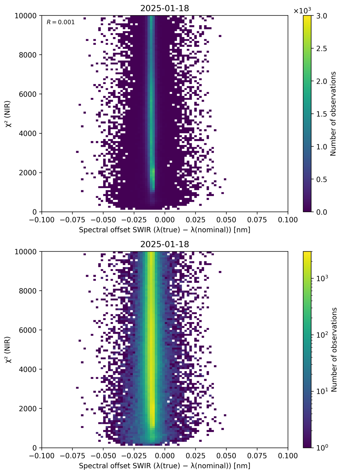
Figure 117: Scatter density plot of “Spectral offset SWIR ( \lambda_{\text{true}} - \lambda_{\text{nominal}} )” against “ \chi^2 (NIR)” for 2025-01-17 to 2025-01-19.
