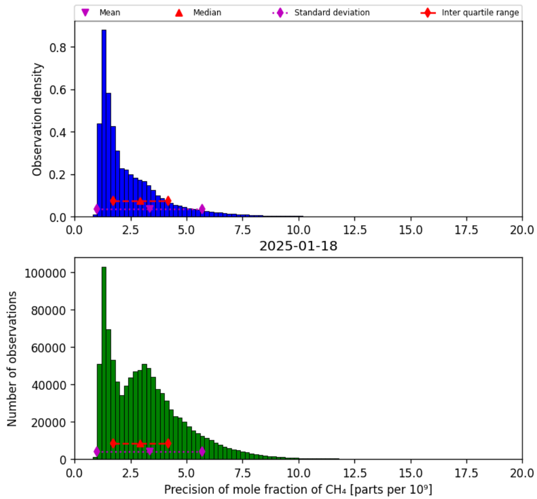
Figure 24: Histogram of “Precision of mole fraction of CH 4 ” for 2025-01-17 to 2025-01-19
