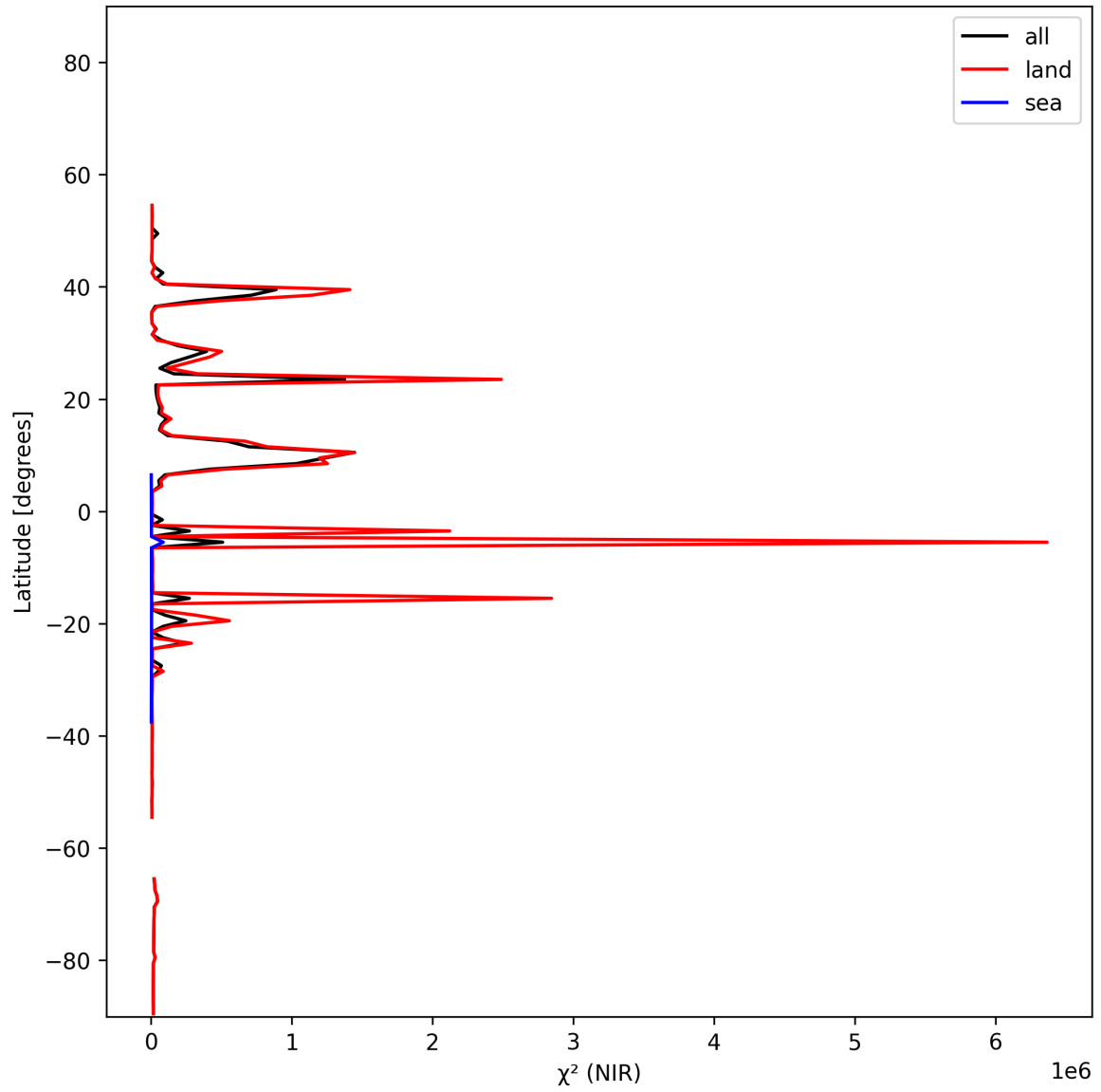
Figure 18: Zonal average of “ \chi^2 (NIR)” for 2025-01-17 to 2025-01-19.
