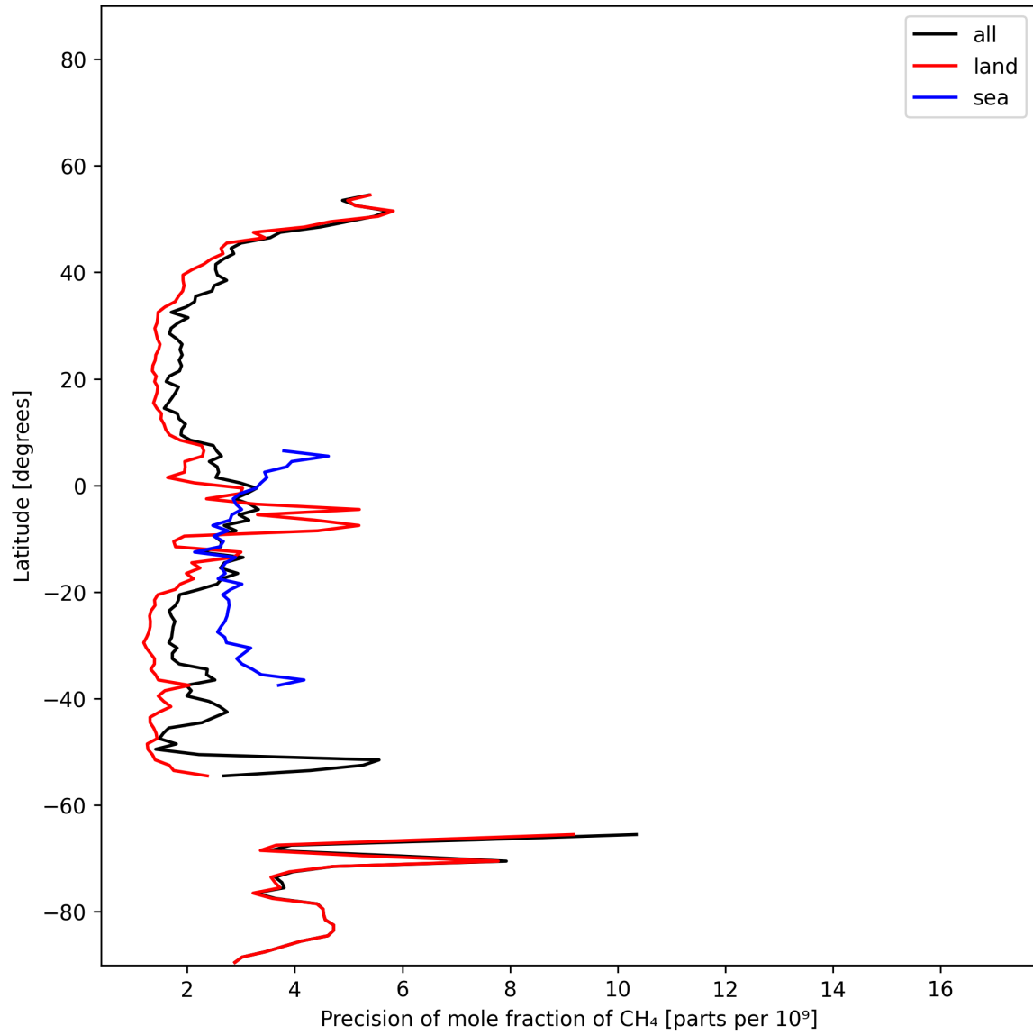
Figure 13: Zonal average of “Precision of mole fraction of CH 4 ” for 2025-01-17 to 2025-01-19.
