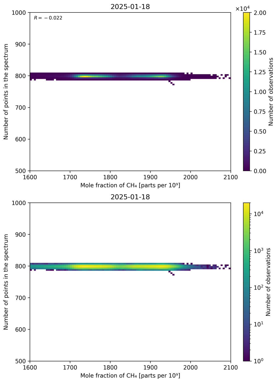
Figure 77: Scatter density plot of “Mole fraction of CH 4 ” against “Number of points in the spectrum” for 2025-01-17 to 2025-01-19.
