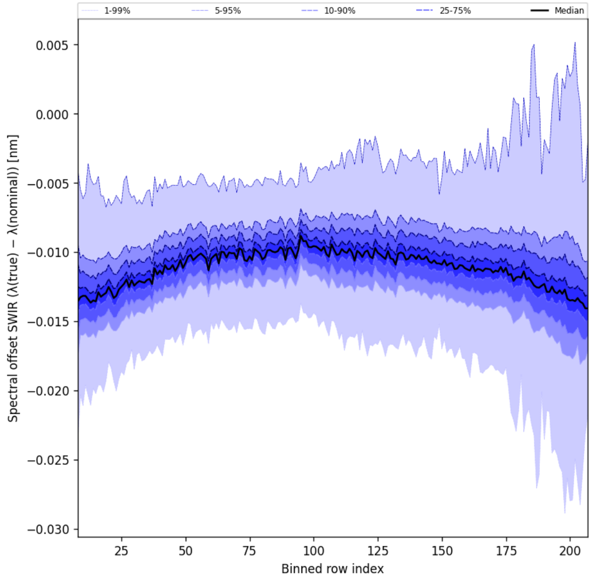
Figure 38: Along track statistics of “Spectral offset SWIR ( \lambda_{\text{true}} - \lambda_{\text{nominal}} )” for 2025-01-17 to 2025-01-19
