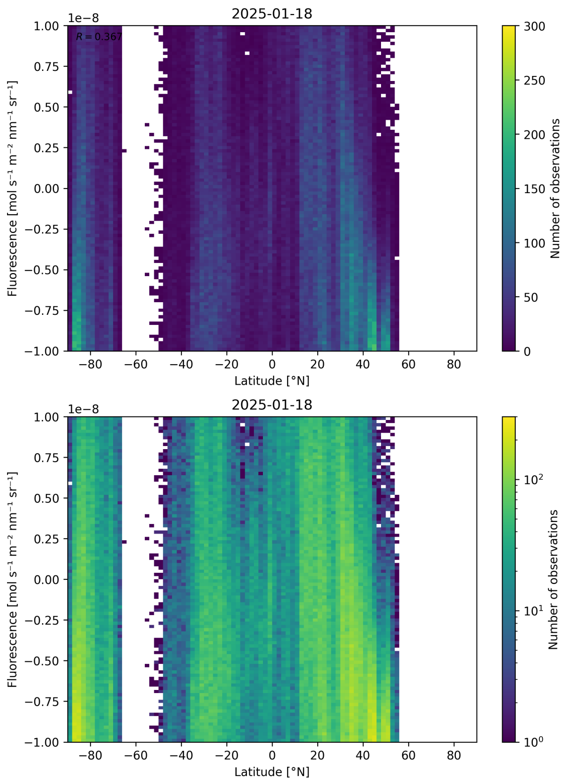
Figure 56: Scatter density plot of “Latitude” against “Fluorescence” for 2025-01-17 to 2025-01-19.
