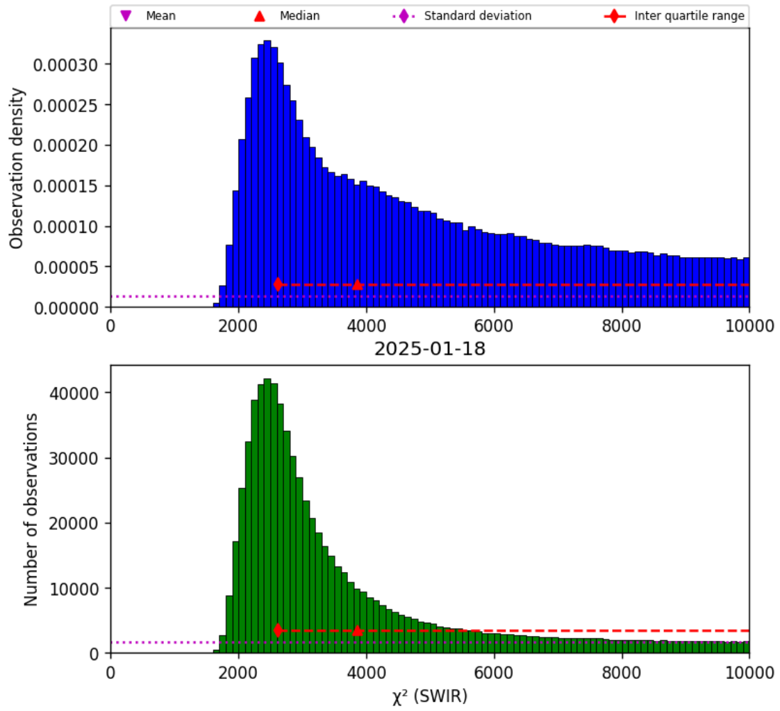
Figure 28: Histogram of “ \chi^2 (SWIR)” for 2025-01-17 to 2025-01-19
