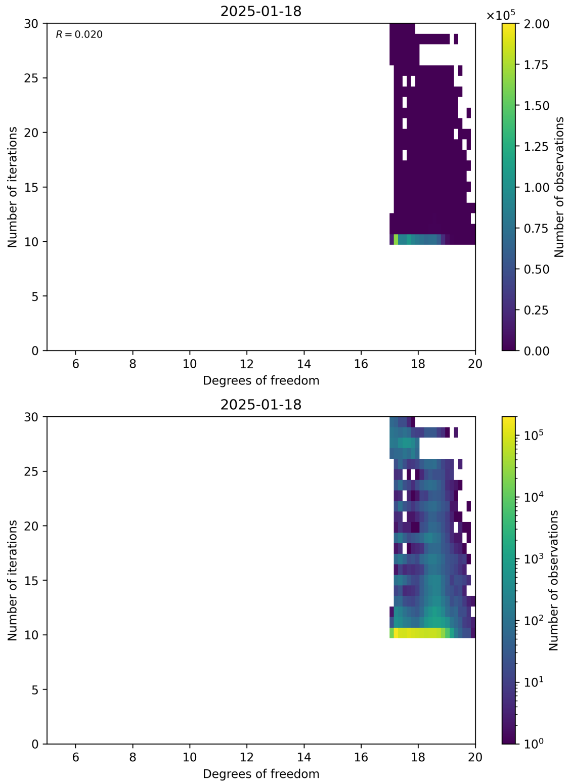
Figure 52: Scatter density plot of “Degrees of freedom” against “Number of iterations” for 2025-01-17 to 2025-01-19.
