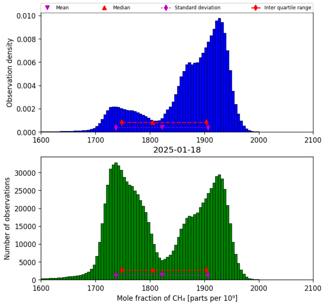
Figure 23: Histogram of “Mole fraction of CH 4 ” for 2025-01-17 to 2025-01-19
