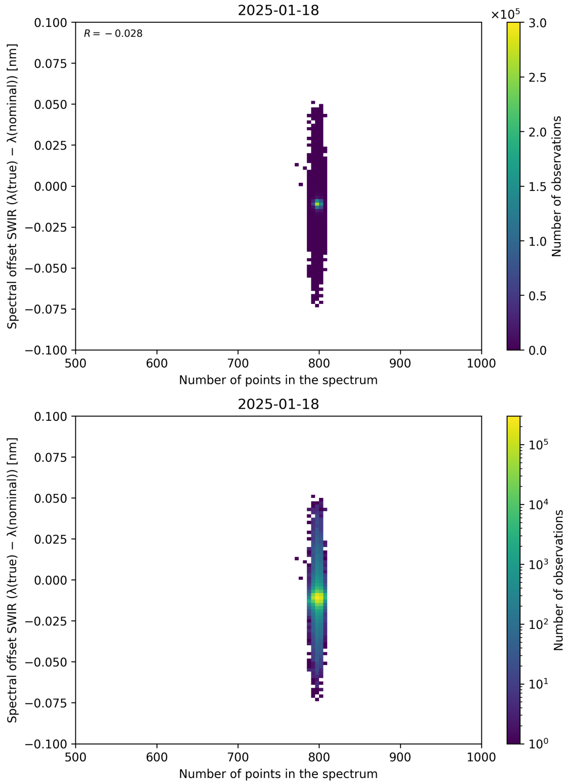
Figure 93: Scatter density plot of “Number of points in the spectrum” against “Spectral offset SWIR ( \lambda_{\text{true}} - \lambda_{\text{nominal}} )” for 2025-01-17 to 2025-01-19.
