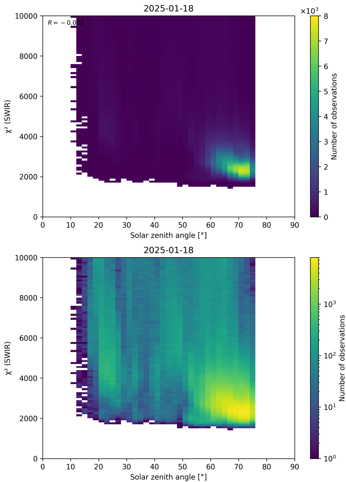
Figure 95: Scatter density plot of “Solar zenith angle” against “ \chi^2 (SWIR)” for 2025-01-17 to 2025-01-19.
