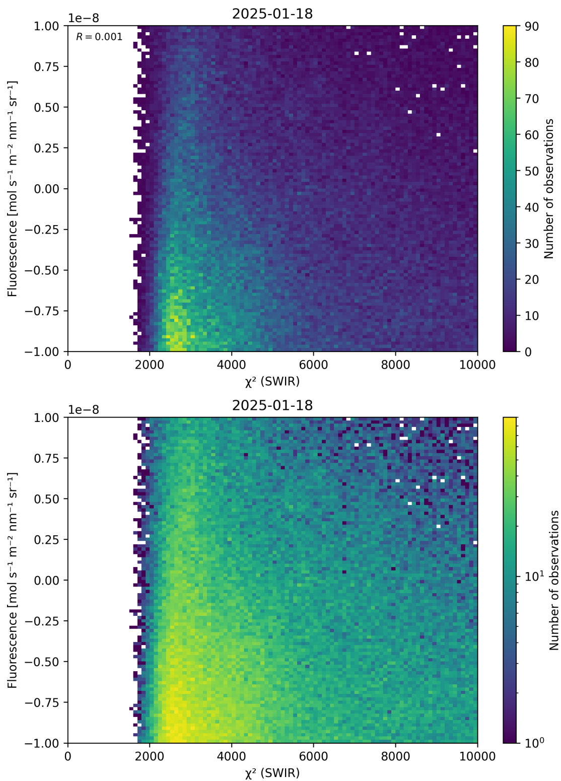
Figure 49: Scatter density plot of “ \chi^2 (SWIR)” against “Fluorescence” for 2025-01-17 to 2025-01-19.
