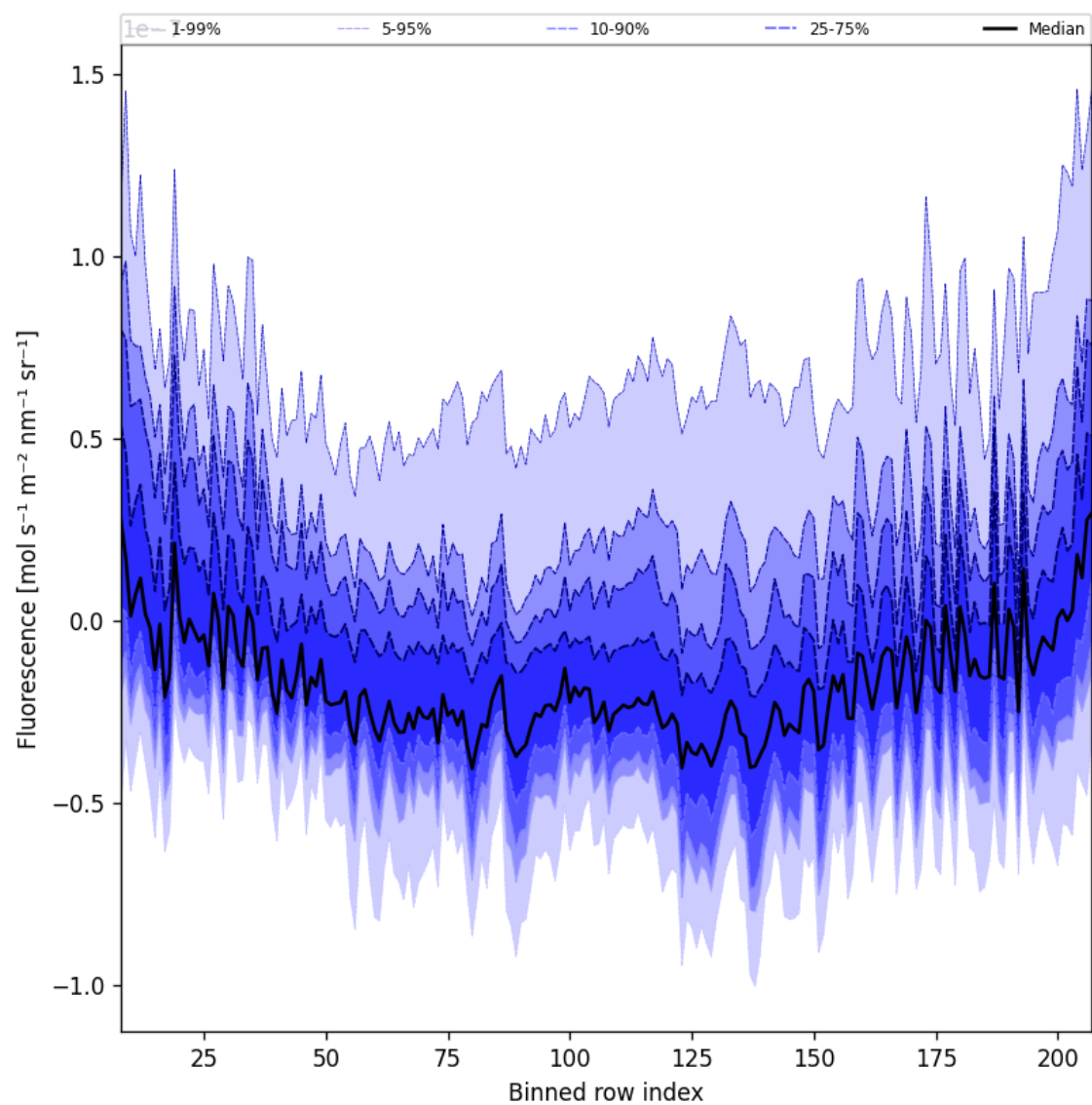
Figure 43: Along track statistics of “Fluorescence” for 2025-01-17 to 2025-01-19
