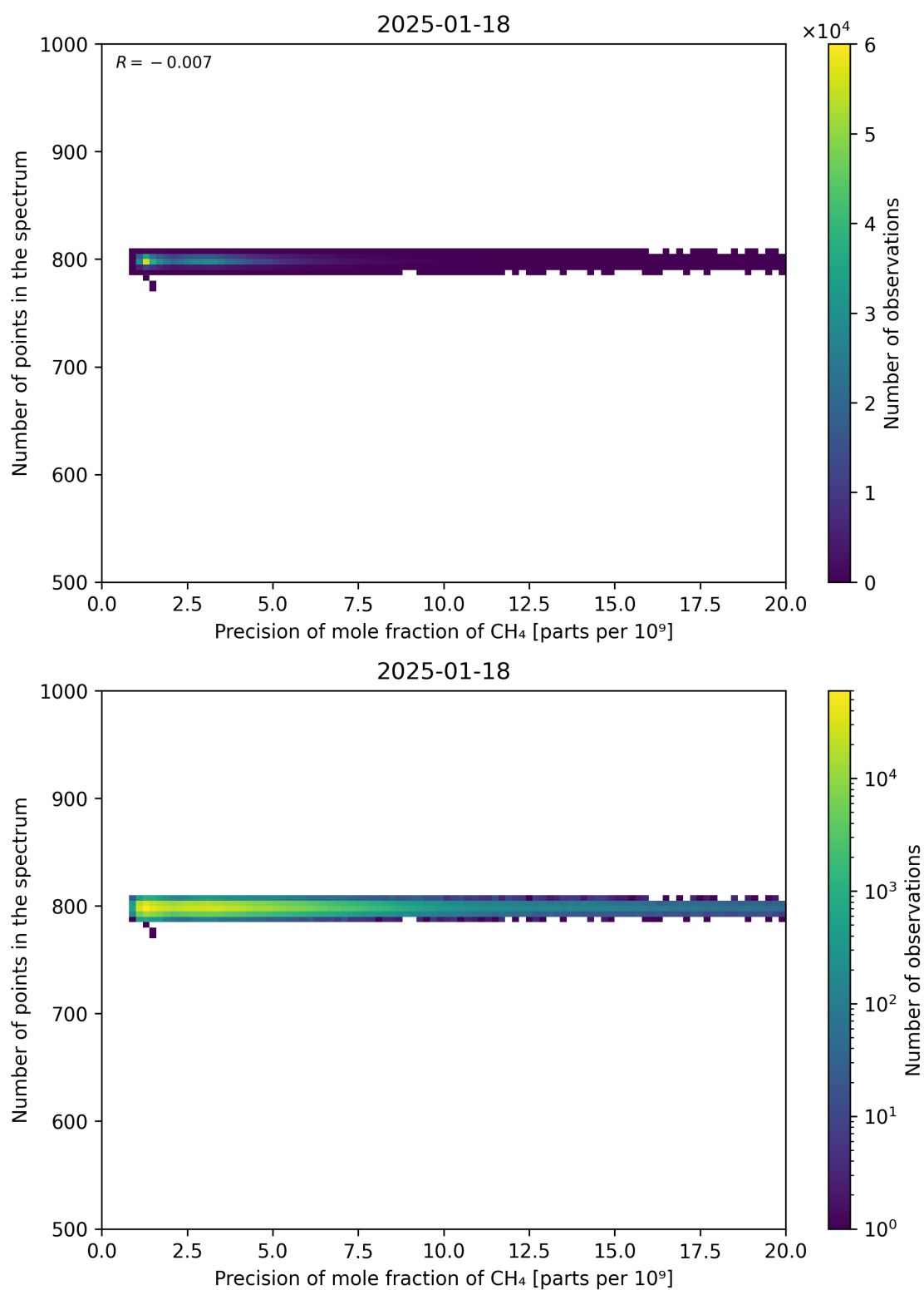
Figure 84: Scatter density plot of “Precision of mole fraction of CH 4 ” against “Number of points in the spectrum” for 2025-01-17 to 2025-01-19.
