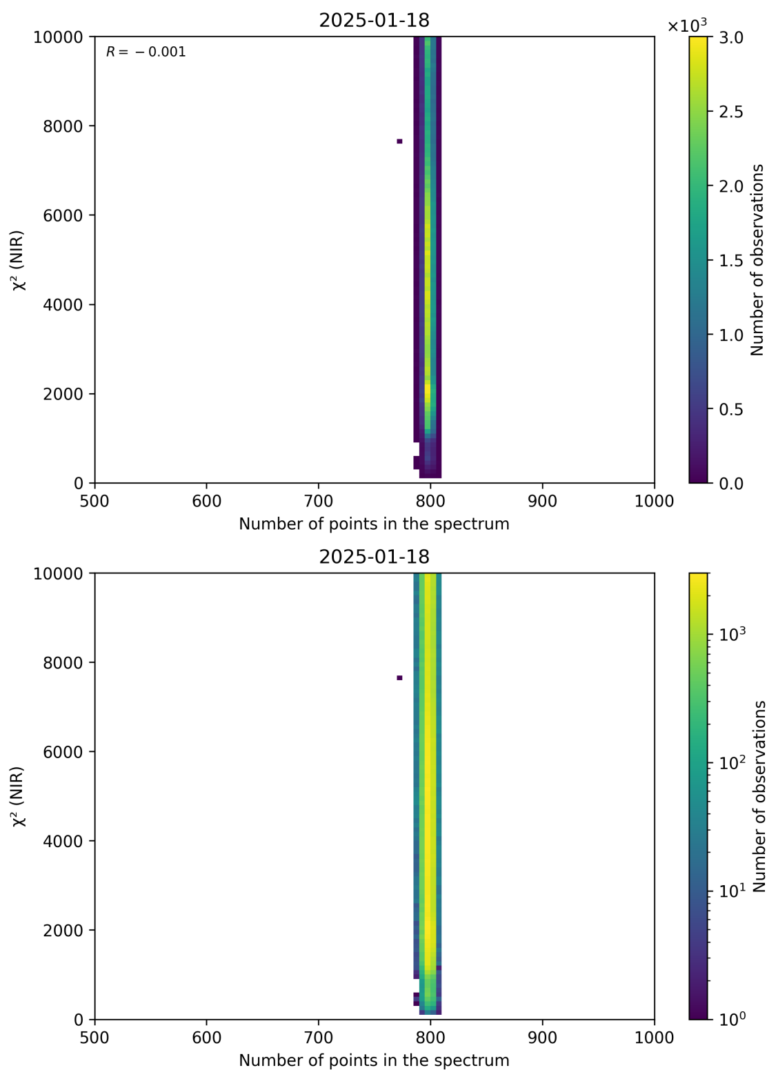
Figure 88: Scatter density plot of “Number of points in the spectrum” against “ \chi^2 (NIR)” for 2025-01-17 to 2025-01-19.
