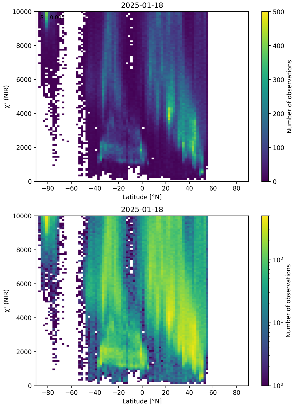
Figure 53: Scatter density plot of “Latitude” against “ \chi^2 (NIR)” for 2025-01-17 to 2025-01-19.
