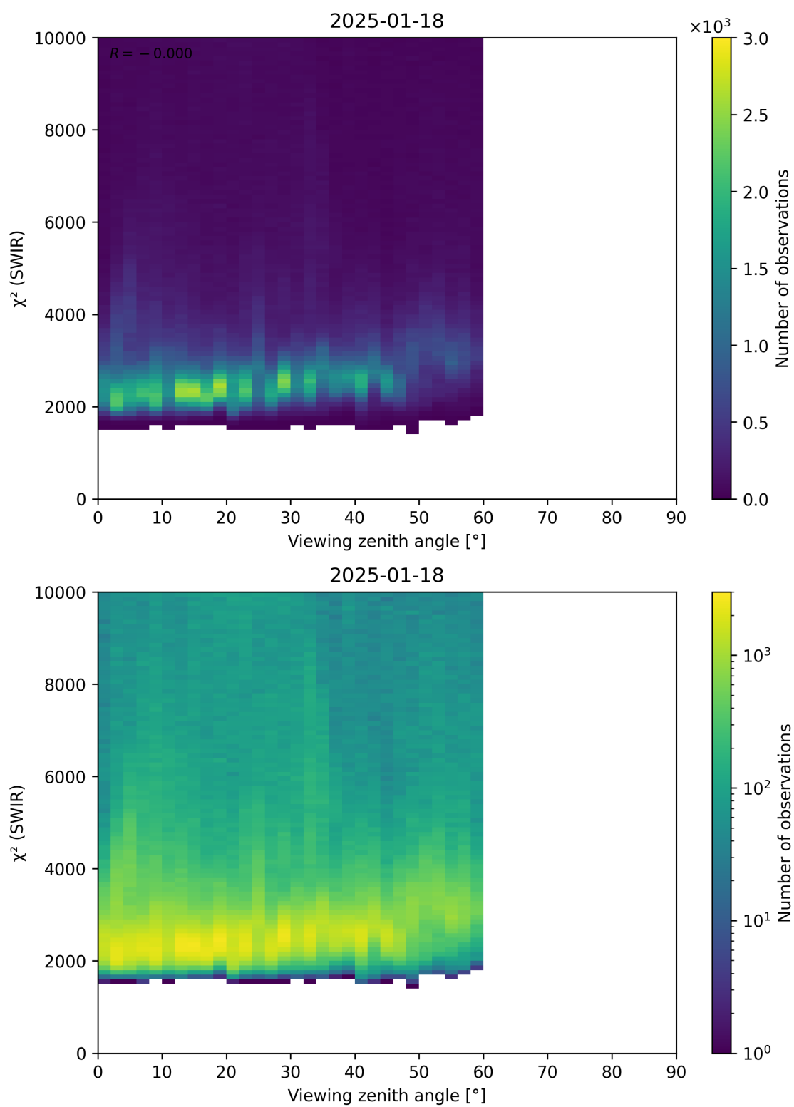
Figure 106: Scatter density plot of “Viewing zenith angle” against “ \chi^2 (SWIR)” for 2025-01-17 to 2025-01-19.
