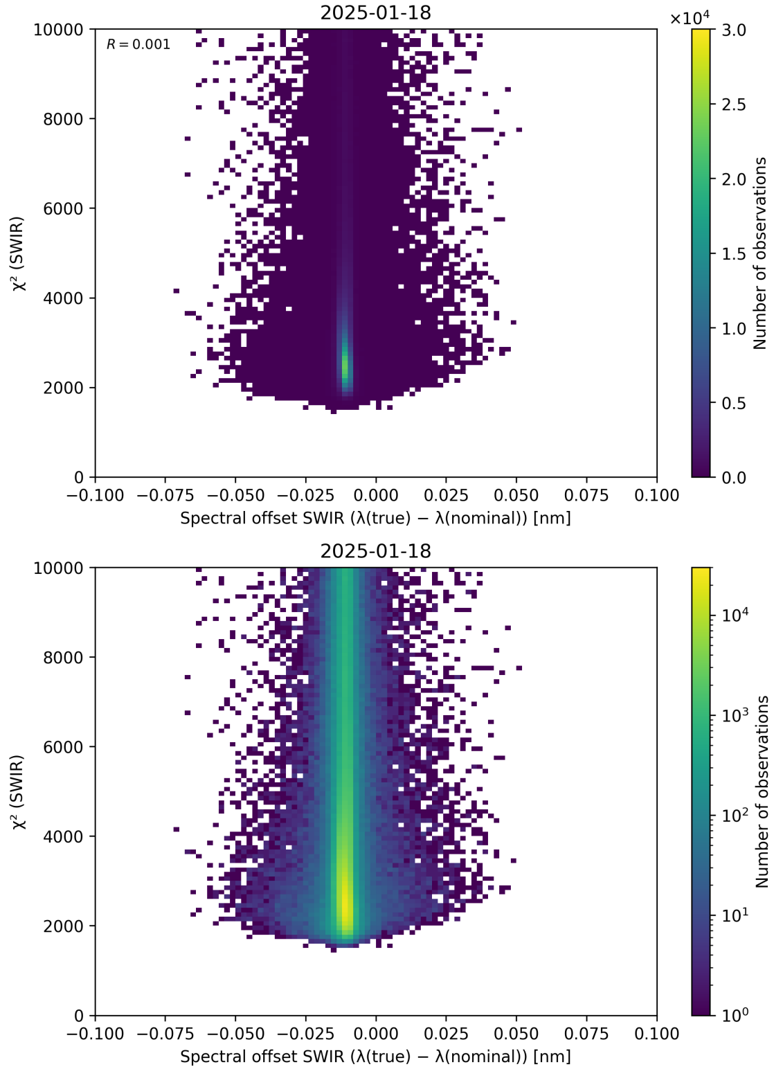
Figure 118: Scatter density plot of “Spectral offset SWIR ( \lambda_{\text{true}} - \lambda_{\text{nominal}} )” against “ \chi^2 (SWIR)” for 2025-01-17 to 2025-01-19.
