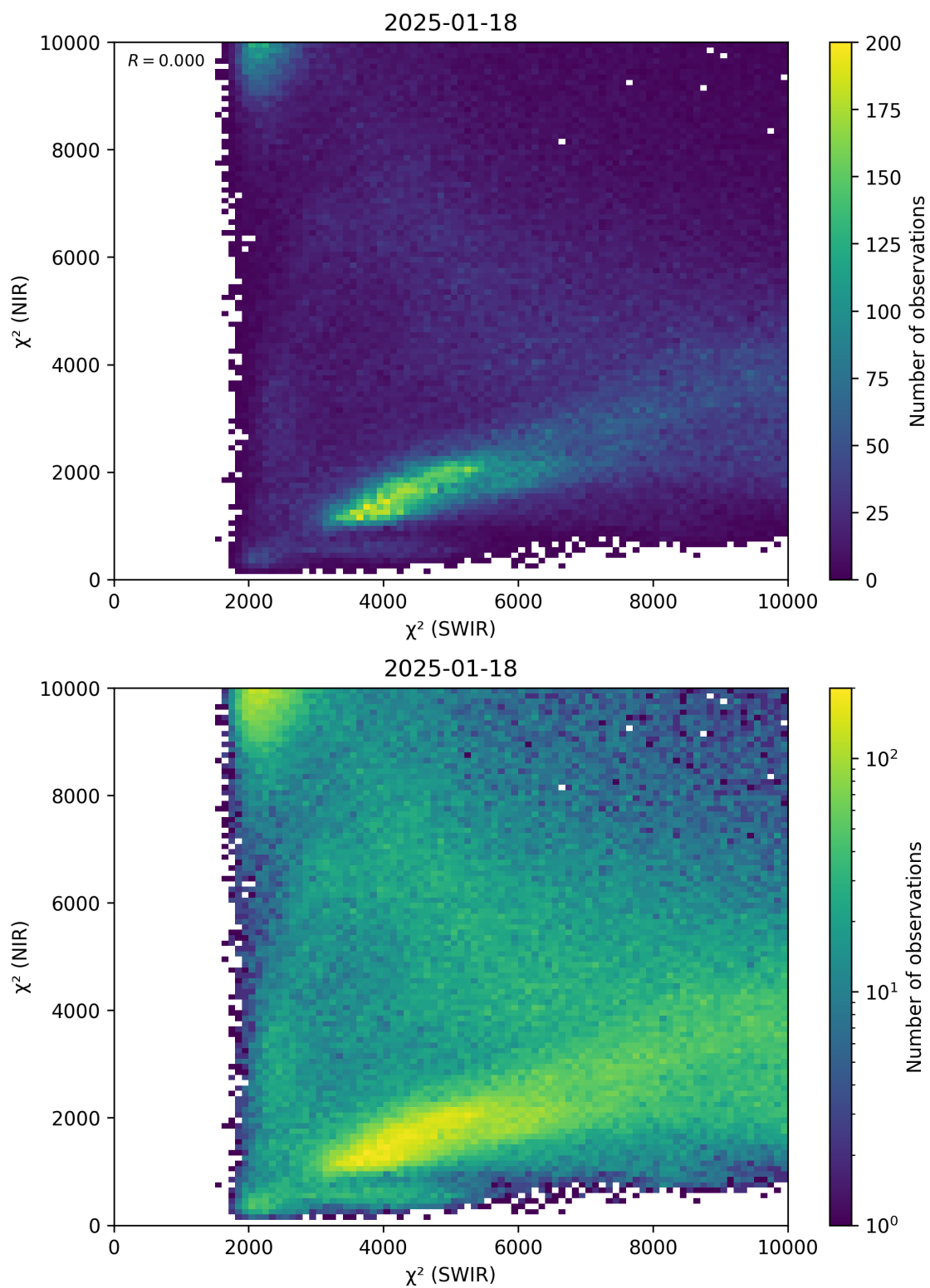
Figure 47: Scatter density plot of “ \chi^2 (SWIR)” against “ \chi^2 (NIR)” for 2025-01-17 to 2025-01-19.
