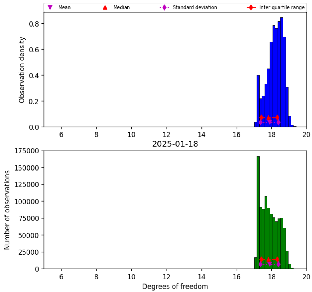
Figure 30: Histogram of “Degrees of freedom” for 2025-01-17 to 2025-01-19
