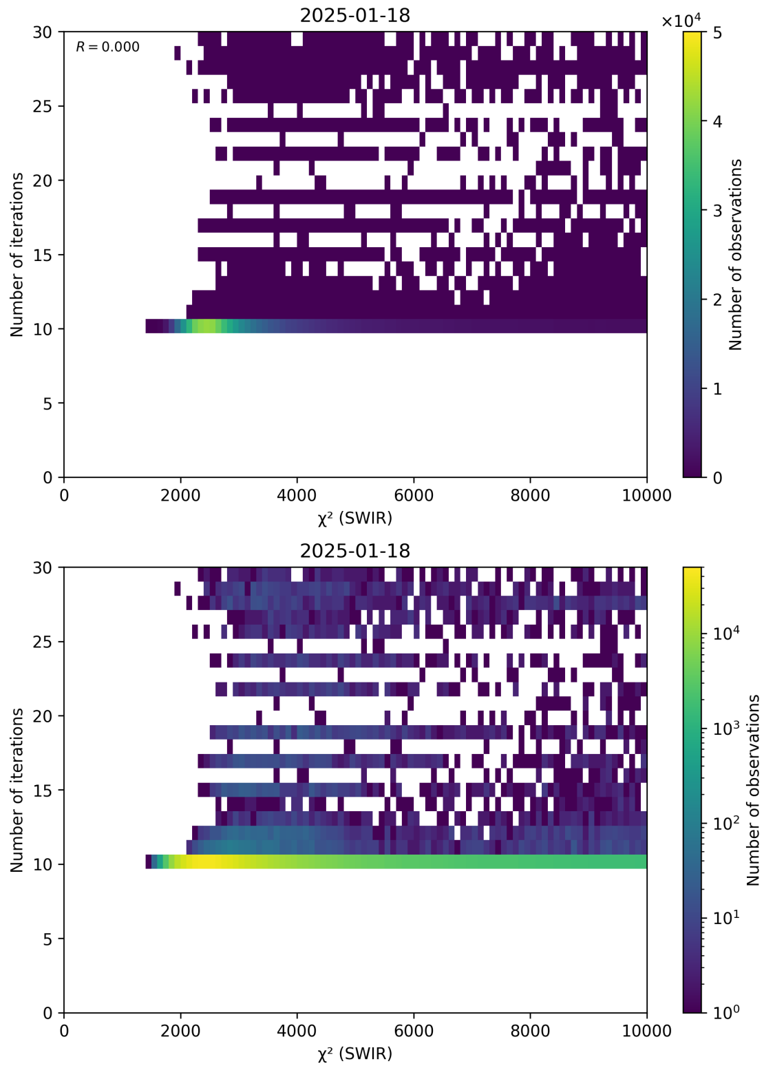
Figure 50: Scatter density plot of “ \chi^2 (SWIR)” against “Number of iterations” for 2025-01-17 to 2025-01-19.
