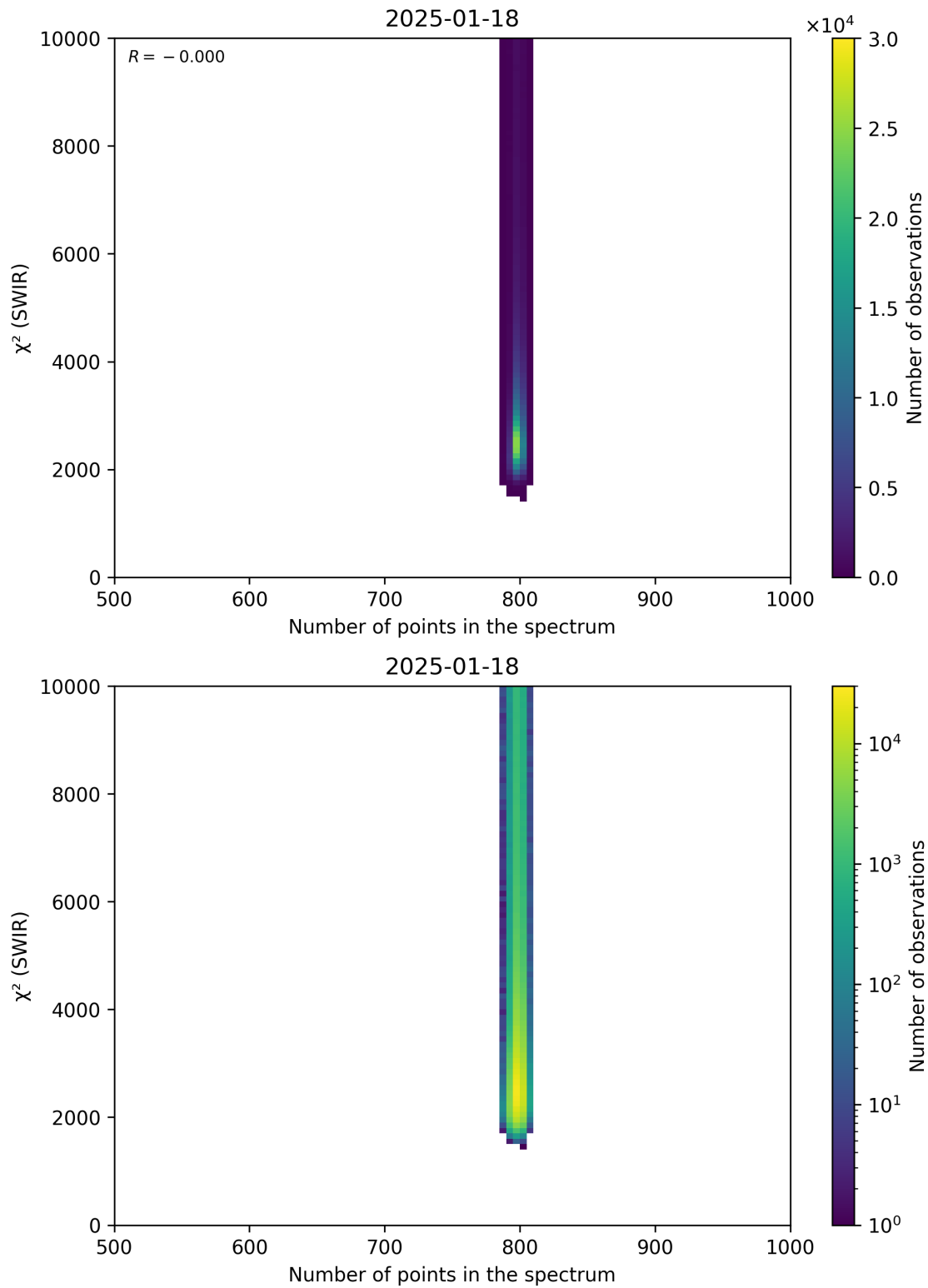
Figure 89: Scatter density plot of “Number of points in the spectrum” against “ \chi^2 (SWIR)” for 2025-01-17 to 2025-01-19.
