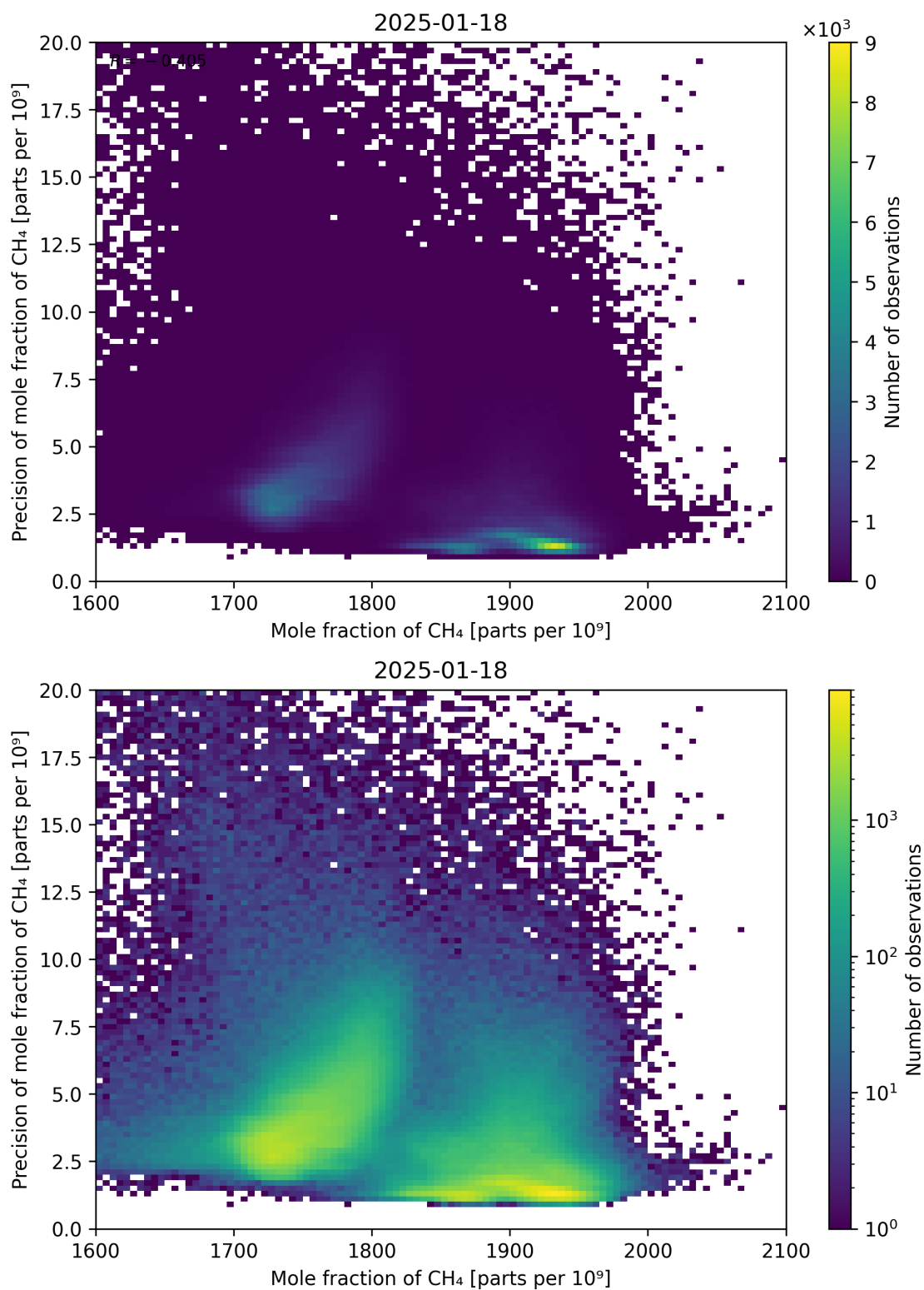
Figure 75: Scatter density plot of “Mole fraction of CH 4 ” against “Precision of mole fraction of CH 4 ” for 2025-01-17 to 2025-01-19.
