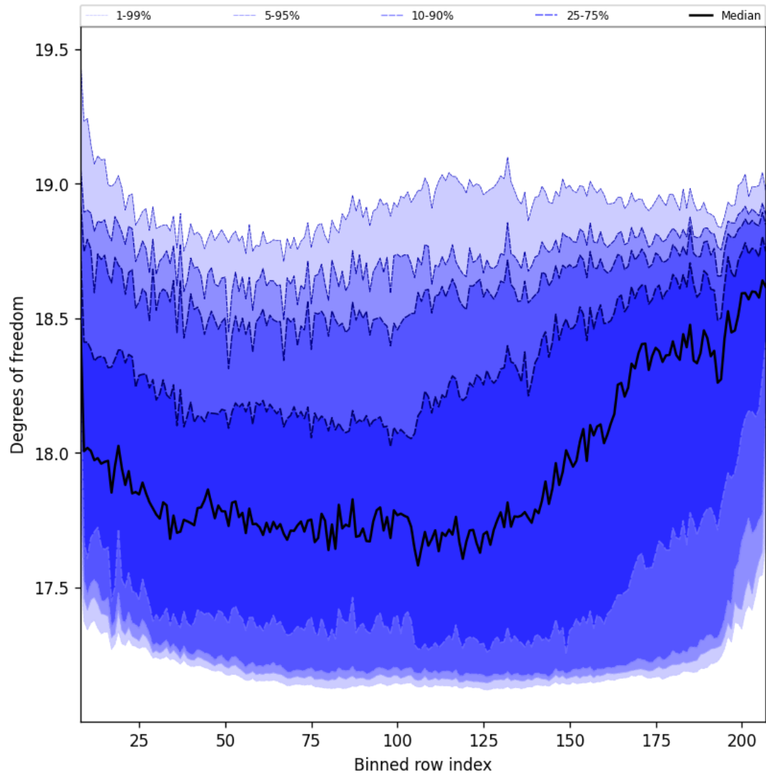
Figure 41: Along track statistics of “Degrees of freedom” for 2025-01-17 to 2025-01-19
