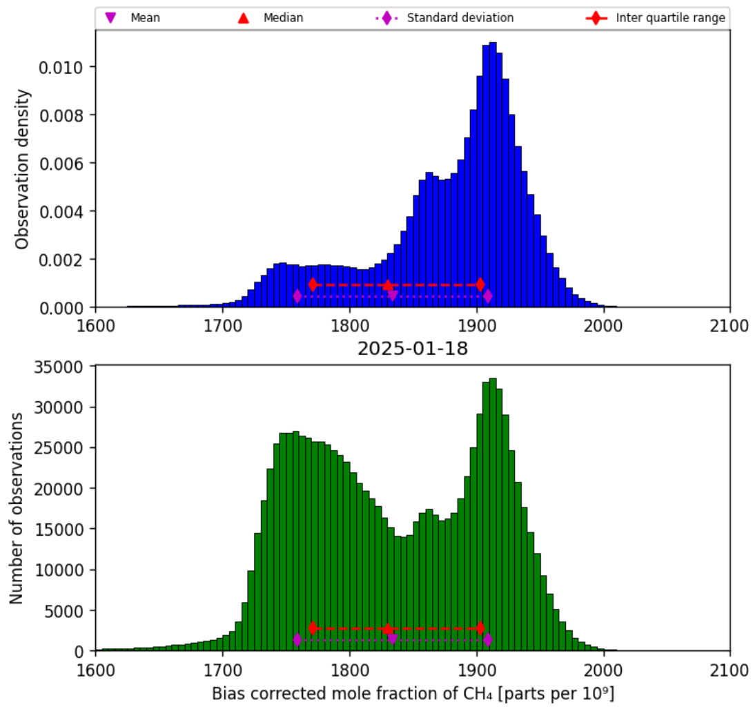
Figure 25: Histogram of “Bias corrected mole fraction of CH 4 ” for 2025-01-17 to 2025-01-19
