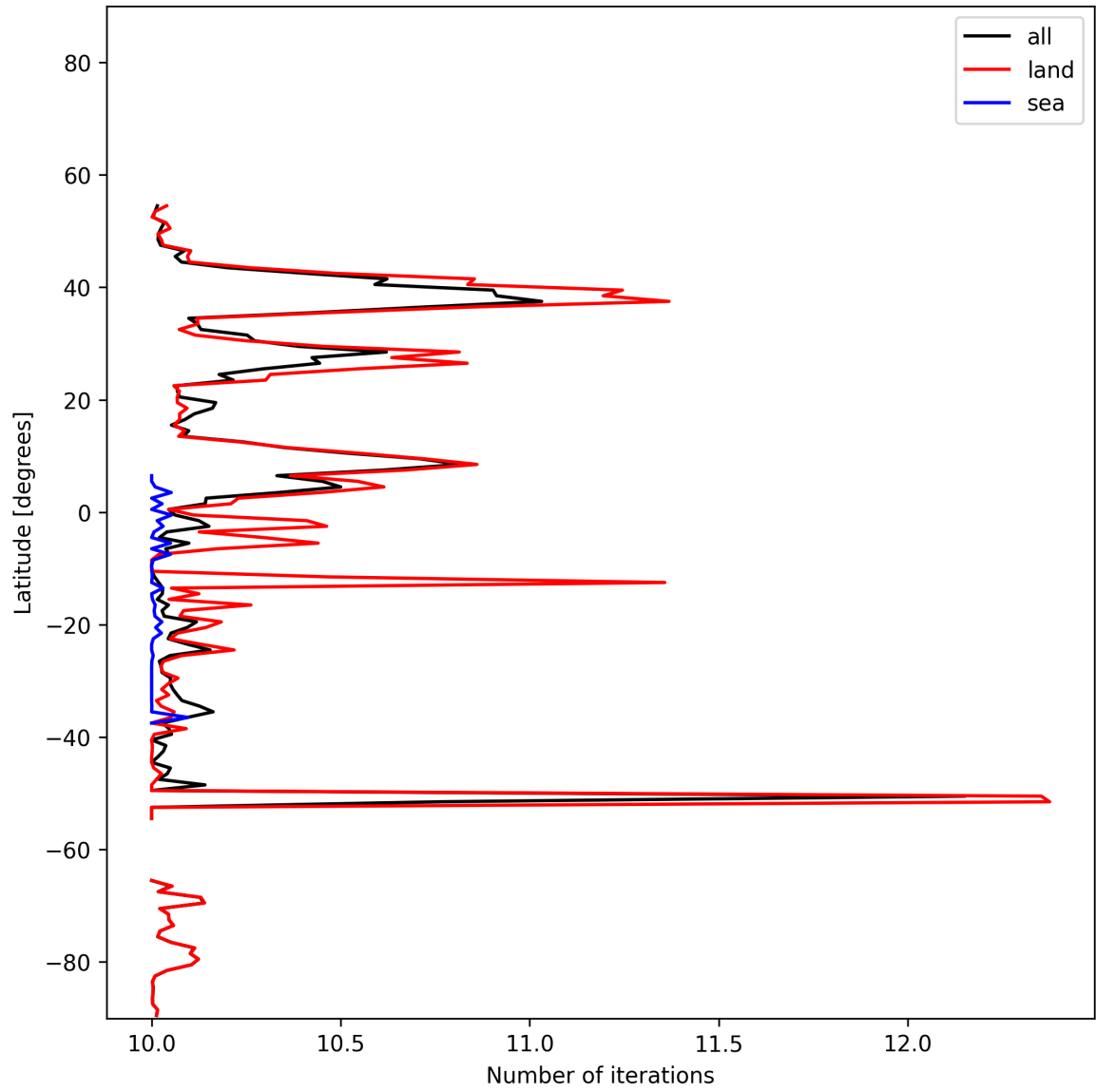
Figure 20: Zonal average of “Number of iterations” for 2025-01-17 to 2025-01-19.
