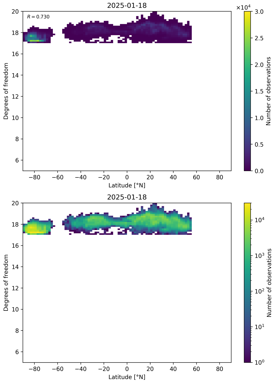
Figure 55: Scatter density plot of “Latitude” against “Degrees of freedom” for 2025-01-17 to 2025-01-19.
