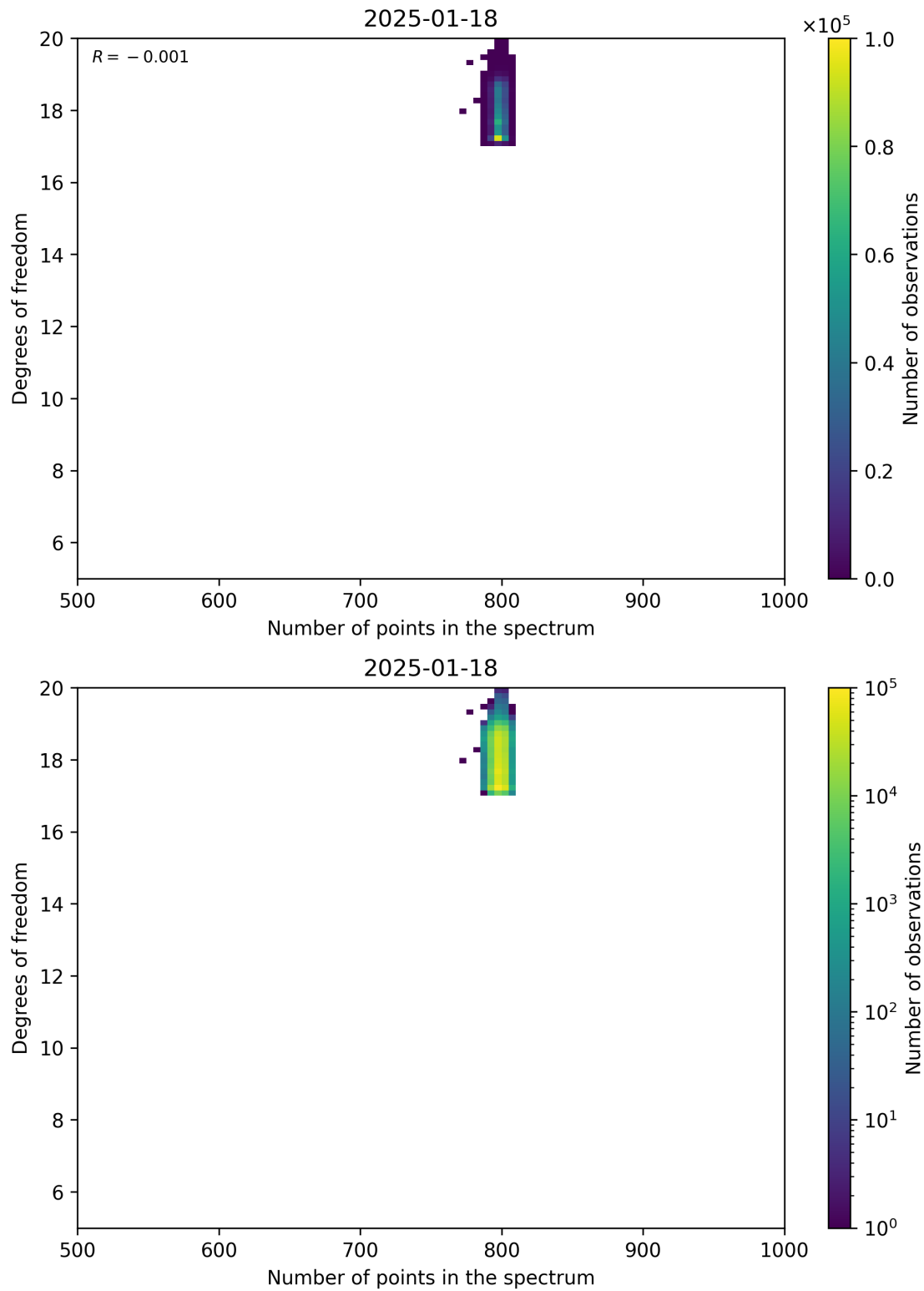
Figure 90: Scatter density plot of “Number of points in the spectrum” against “Degrees of freedom” for 2025-01-17 to 2025-01-19.
