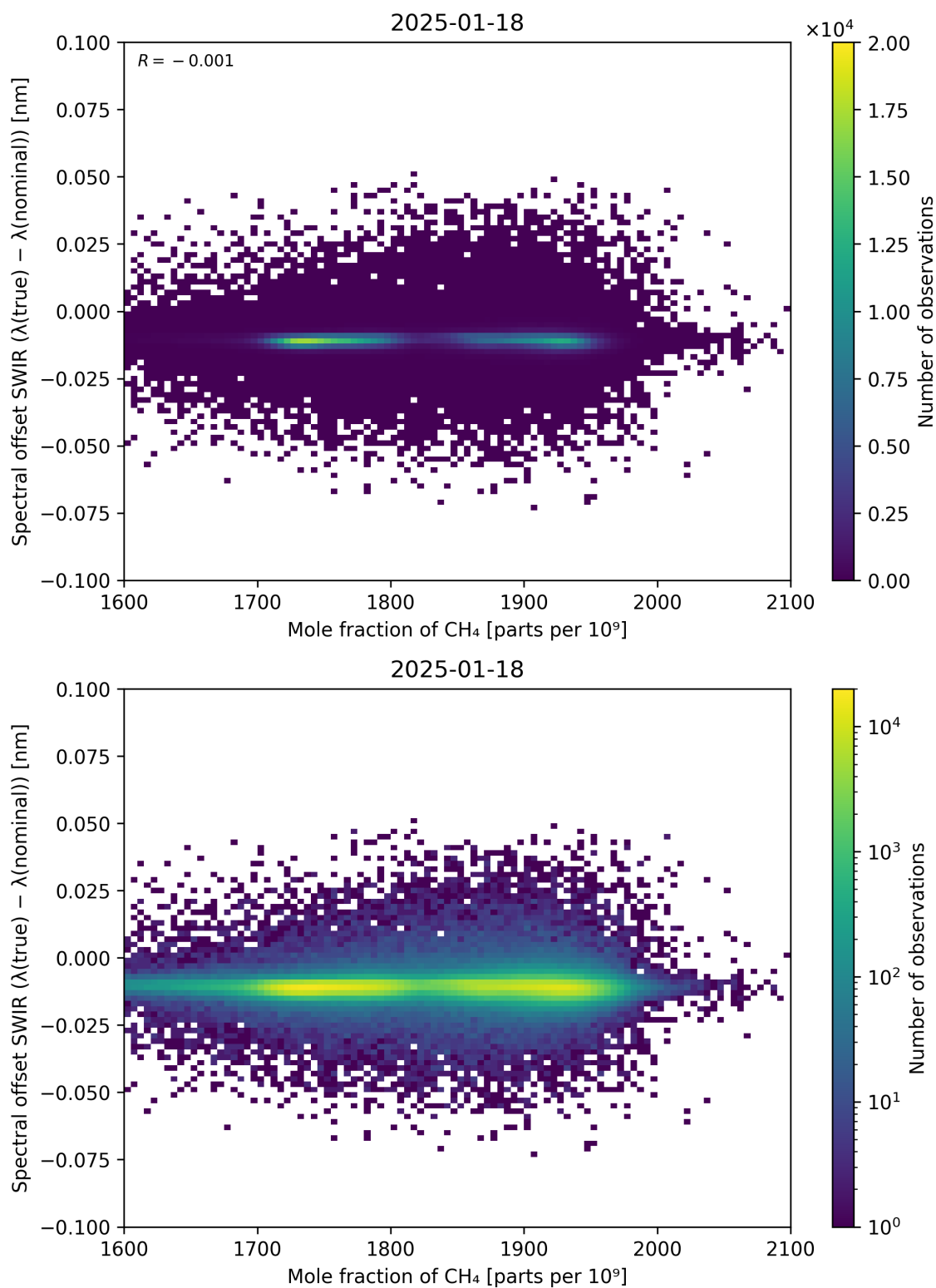
Figure 86: Scatter density plot of “Mole fraction of CH 4 ” against “Spectral offset SWIR ( \lambda_{\text{true}} - \lambda_{\text{nominal}} )” for 2025-01-17 to 2025-01-19.
