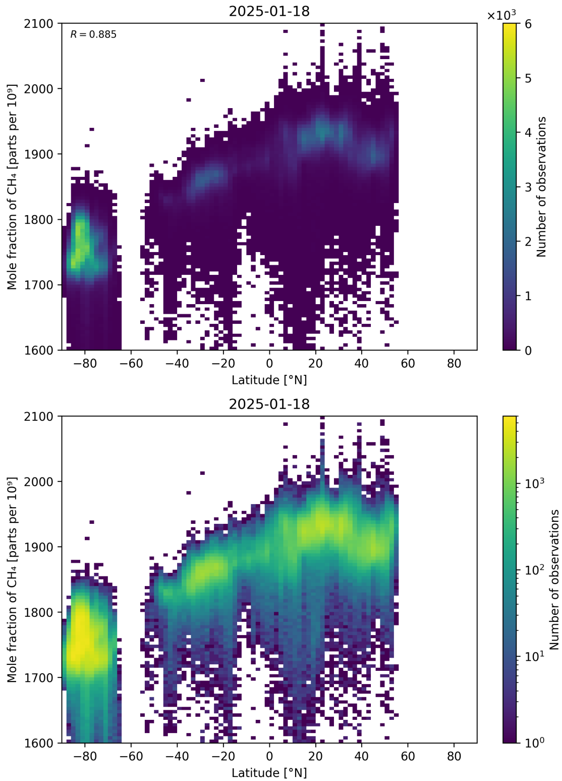
Figure 57: Scatter density plot of “Latitude” against “Mole fraction of CH 4 ” for 2025-01-17 to 2025-01-19.
