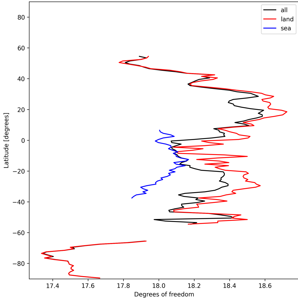
Figure 19: Zonal average of “Degrees of freedom” for 2025-01-17 to 2025-01-19.
