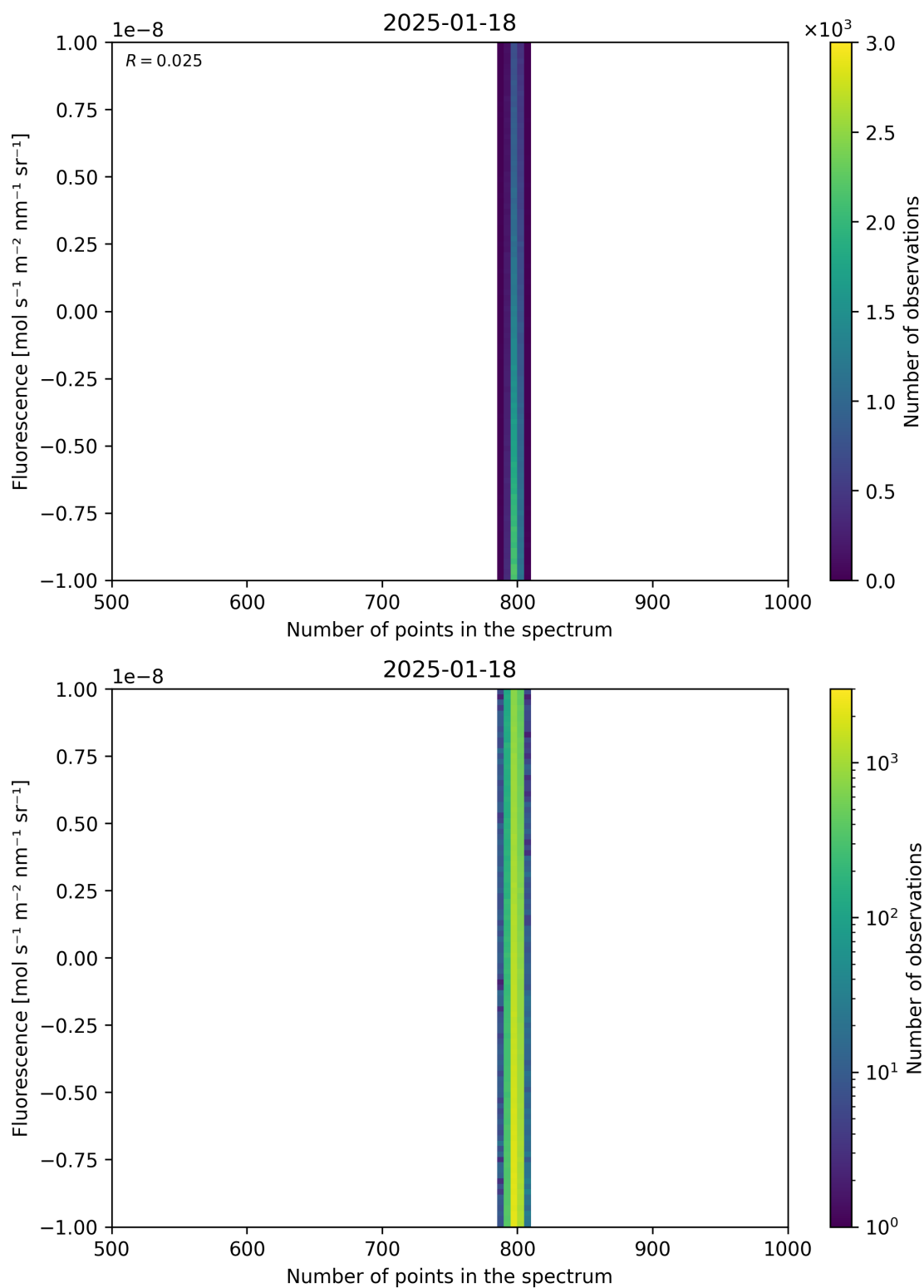
Figure 91: Scatter density plot of “Number of points in the spectrum” against “Fluorescence” for 2025-01-17 to 2025-01-19.
