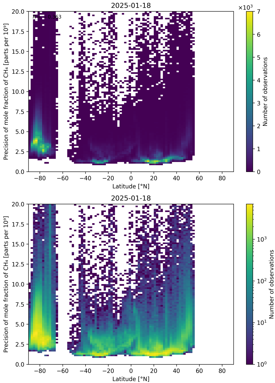
Figure 59: Scatter density plot of “Latitude” against “Precision of mole fraction of CH 4 ” for 2025-01-17 to 2025-01-19.
