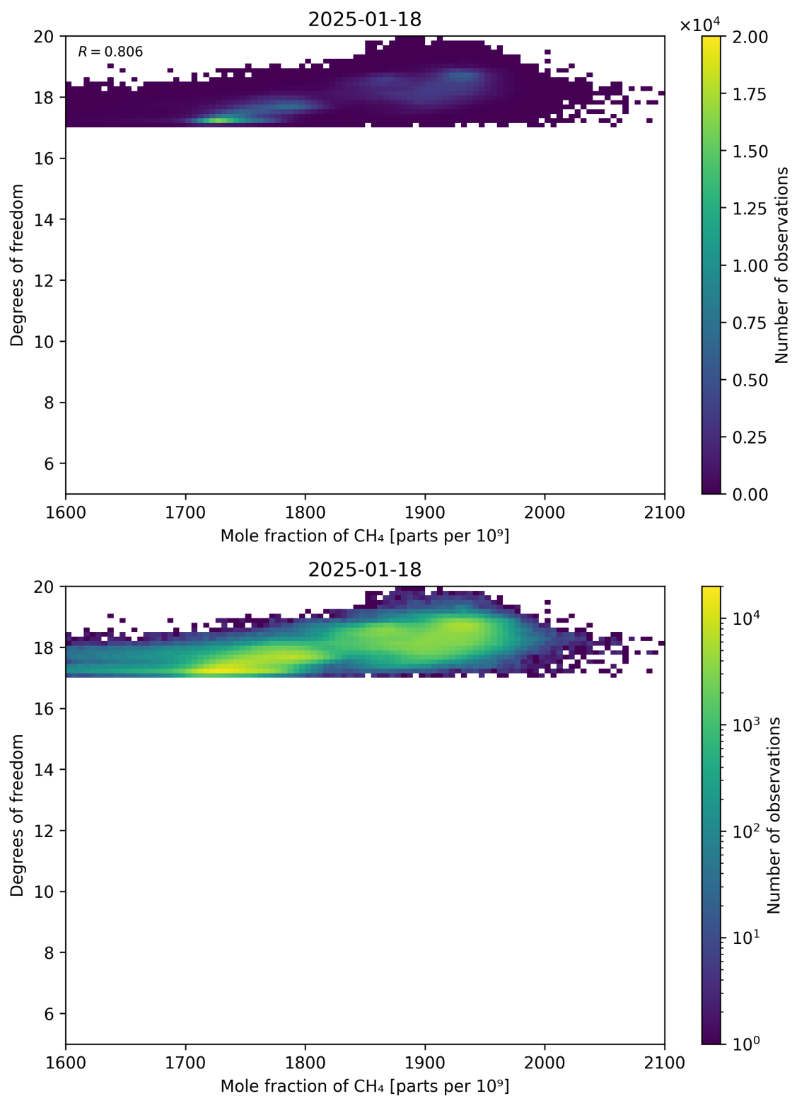
Figure 72: Scatter density plot of “Mole fraction of CH 4 ” against “Degrees of freedom” for 2025-01-17 to 2025-01-19.
