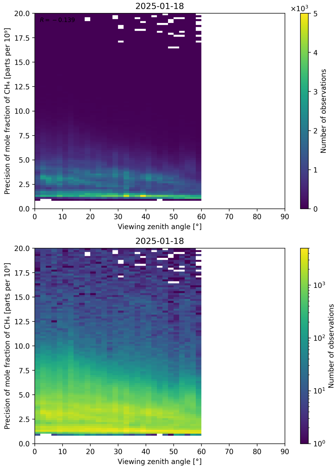
Figure 112: Scatter density plot of “Viewing zenith angle” against “Precision of mole fraction of CH 4 ” for 2025-01-17 to 2025-01-19.
