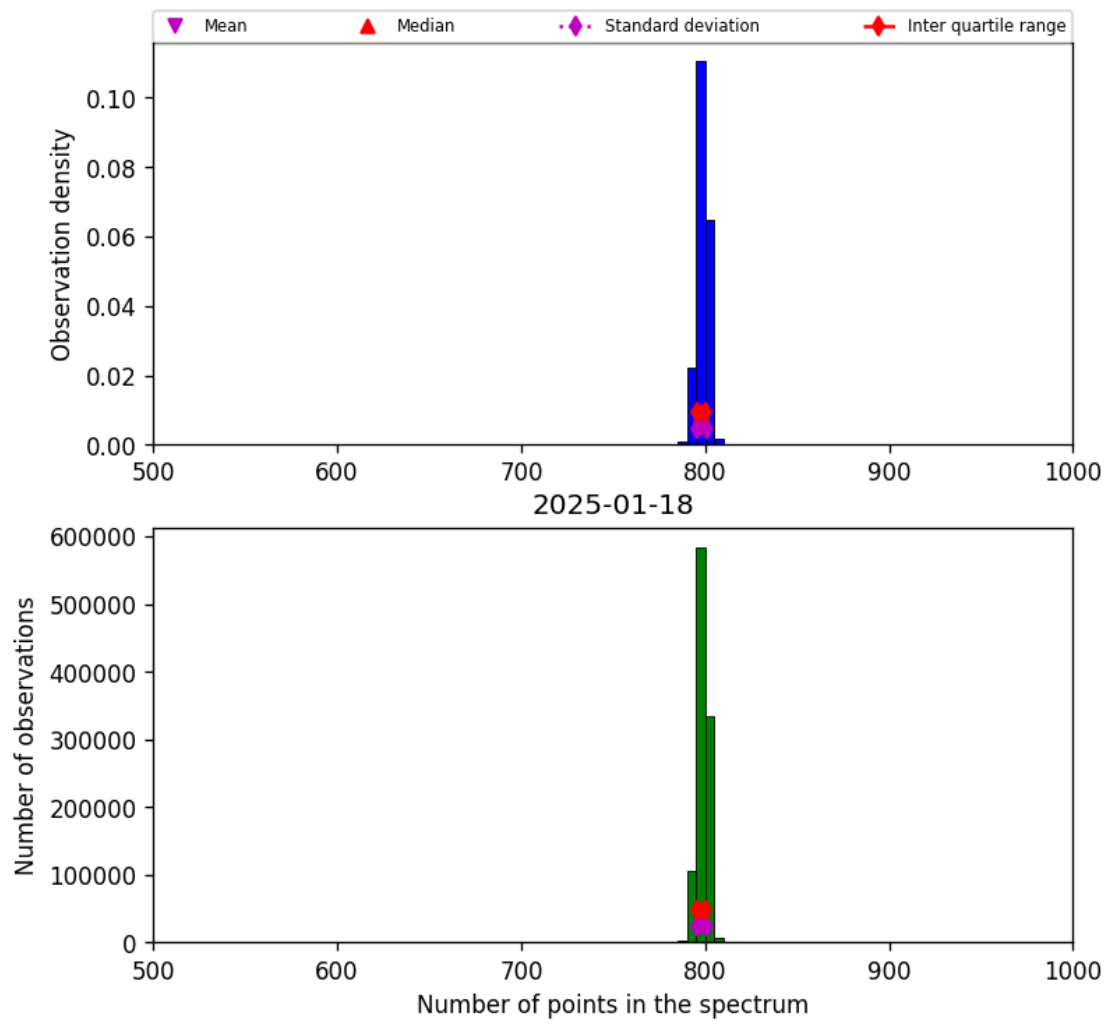
Figure 26: Histogram of “Number of points in the spectrum” for 2025-01-17 to 2025-01-19
