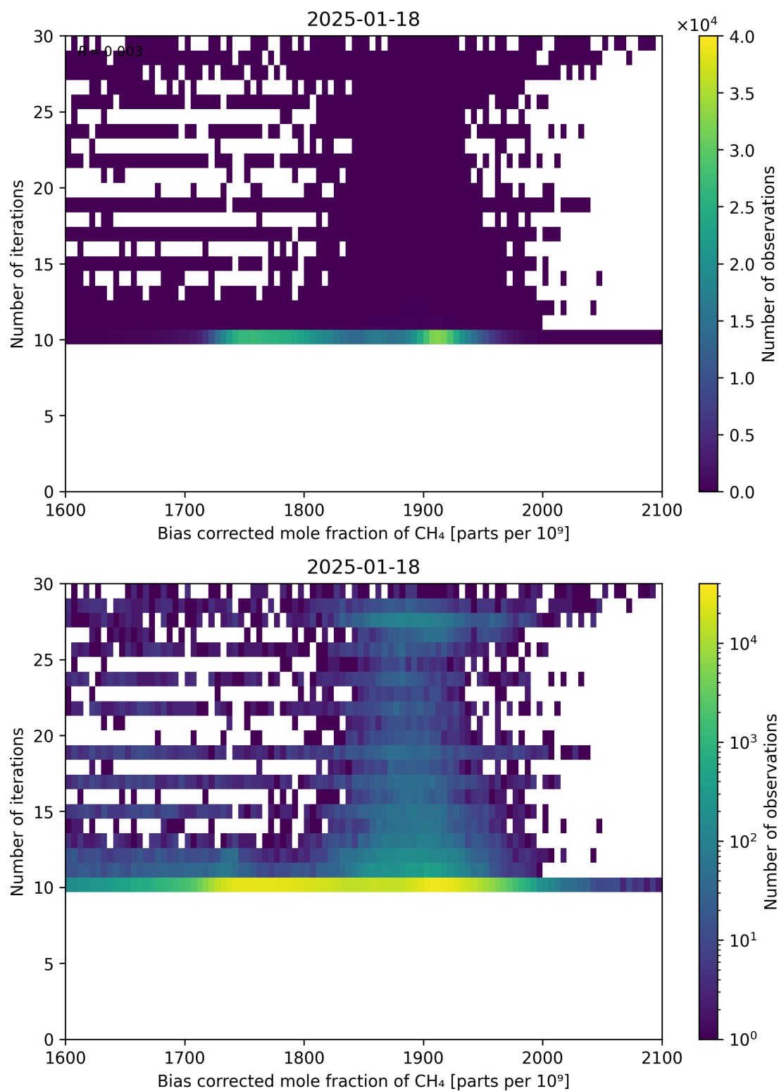
Figure 67: Scatter density plot of “Bias corrected mole fraction of \text{CH}_4 ” against “Number of iterations” for 2025-01-17 to 2025-01-19.
