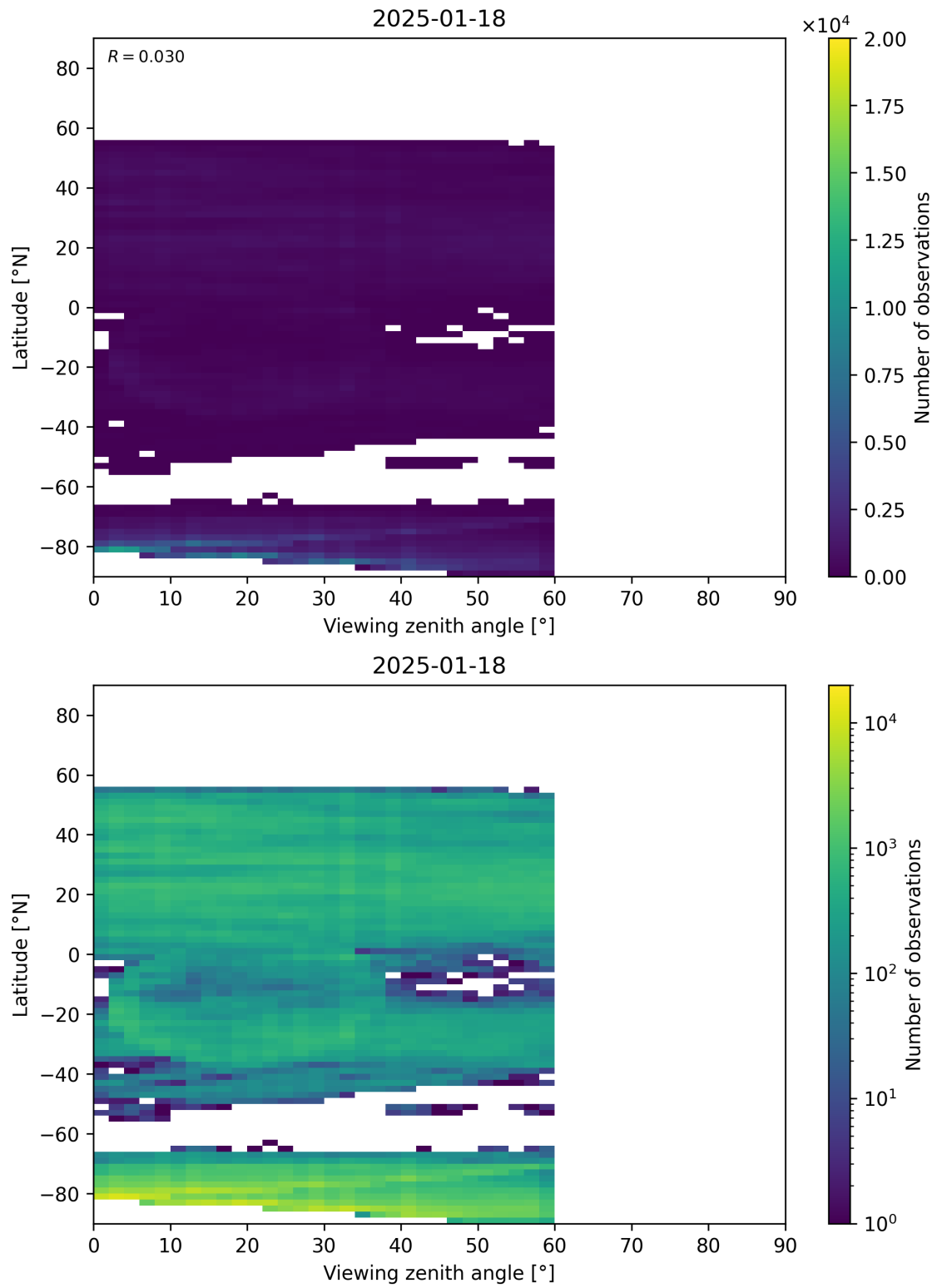
Figure 109: Scatter density plot of “Viewing zenith angle” against “Latitude” for 2025-01-17 to 2025-01-19.
