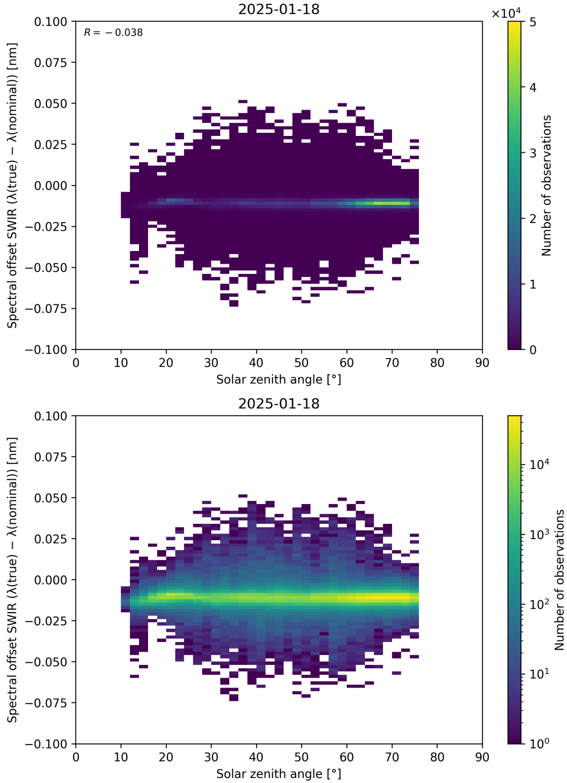
Figure 104: Scatter density plot of “Solar zenith angle” against “Spectral offset SWIR ( \lambda_{\text{true}} - \lambda_{\text{nominal}} )” for 2025-01-17 to 2025-01-19.
