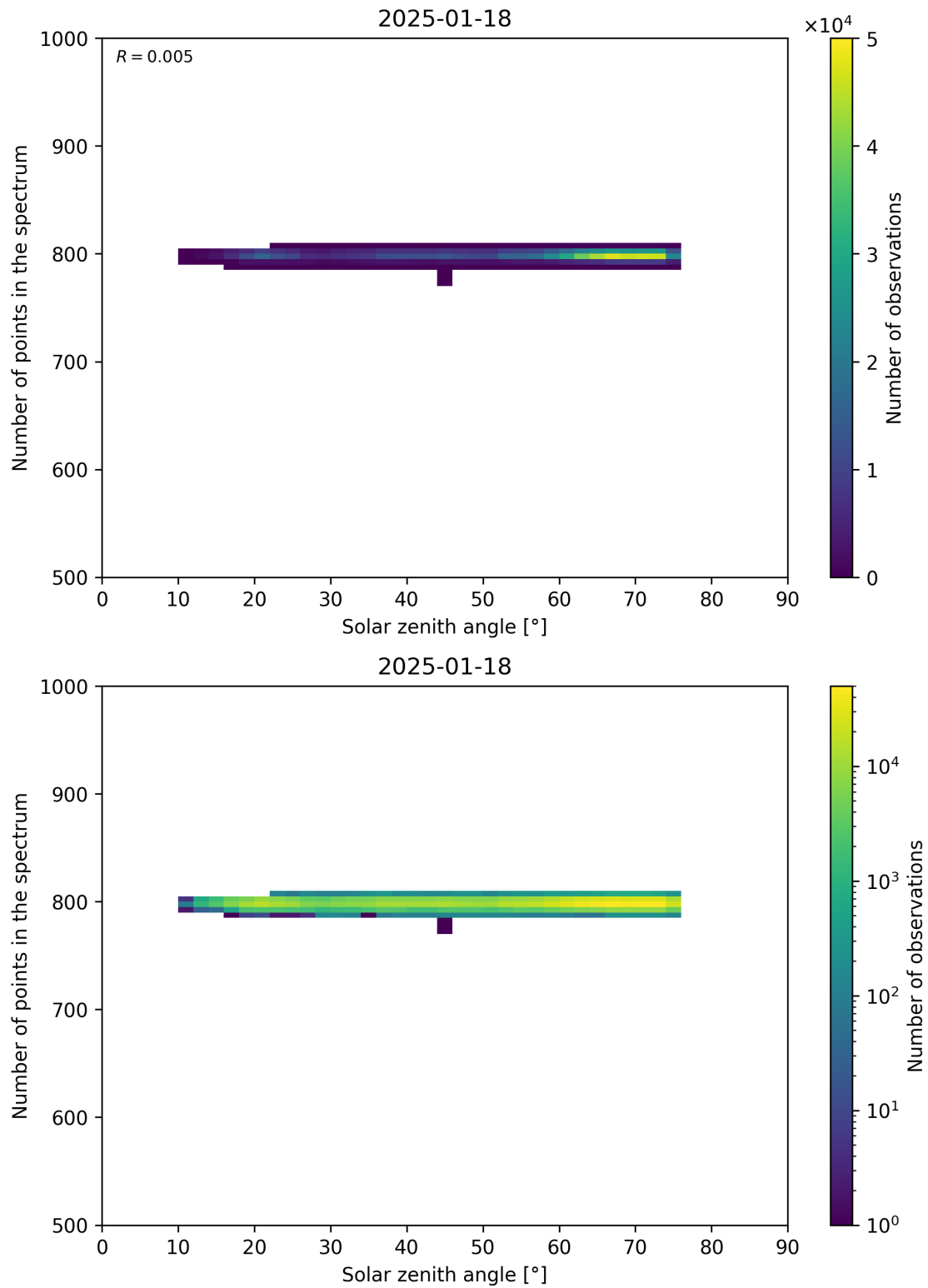
Figure 103: Scatter density plot of “Solar zenith angle” against “Number of points in the spectrum” for 2025-01-17 to 2025-01-19.
