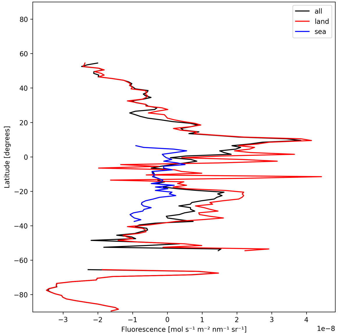
Figure 21: Zonal average of “Fluorescence” for 2025-01-17 to 2025-01-19.
