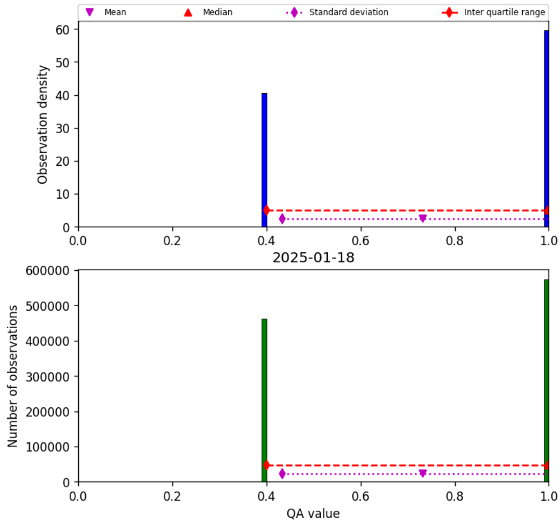
Figure 22: Histogram of “QA value” for 2025-01-17 to 2025-01-19
