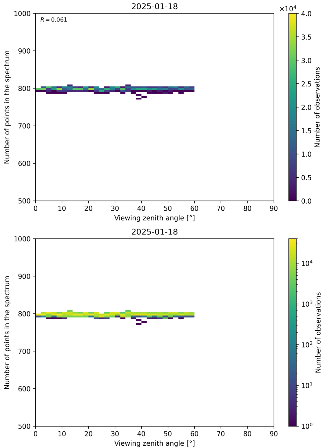
Figure 114: Scatter density plot of “Viewing zenith angle” against “Number of points in the spectrum” for 2025-01-17 to 2025-01-19.
