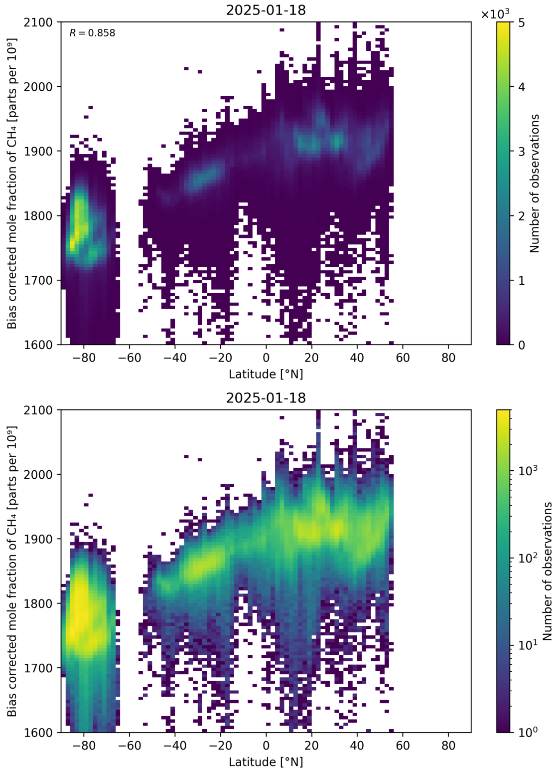
Figure 58: Scatter density plot of “Latitude” against “Bias corrected mole fraction of CH 4 ” for 2025-01-17 to 2025-01-19.
