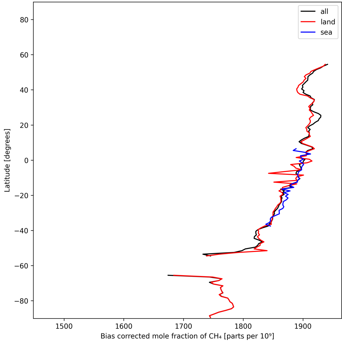
Figure 14: Zonal average of “Bias corrected mole fraction of CH 4 ” for 2025-01-17 to 2025-01-19.
