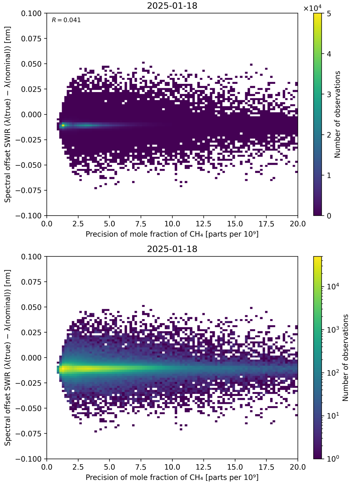
Figure 85: Scatter density plot of “Precision of mole fraction of CH 4 ” against “Spectral offset SWIR ( \lambda_{\text{true}} - \lambda_{\text{nominal}} )” for 2025-01-17 to 2025-01-19.
