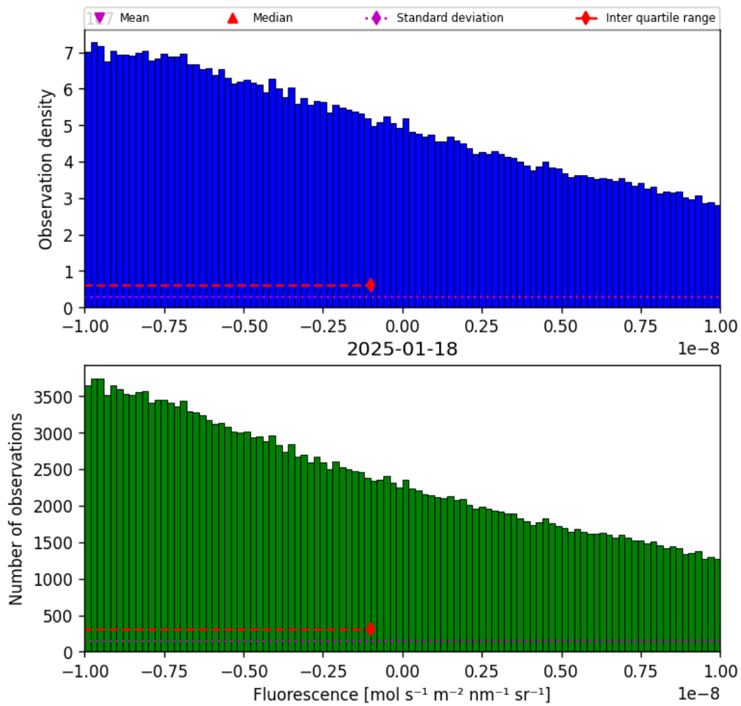
Figure 32: Histogram of “Fluorescence” for 2025-01-17 to 2025-01-19
