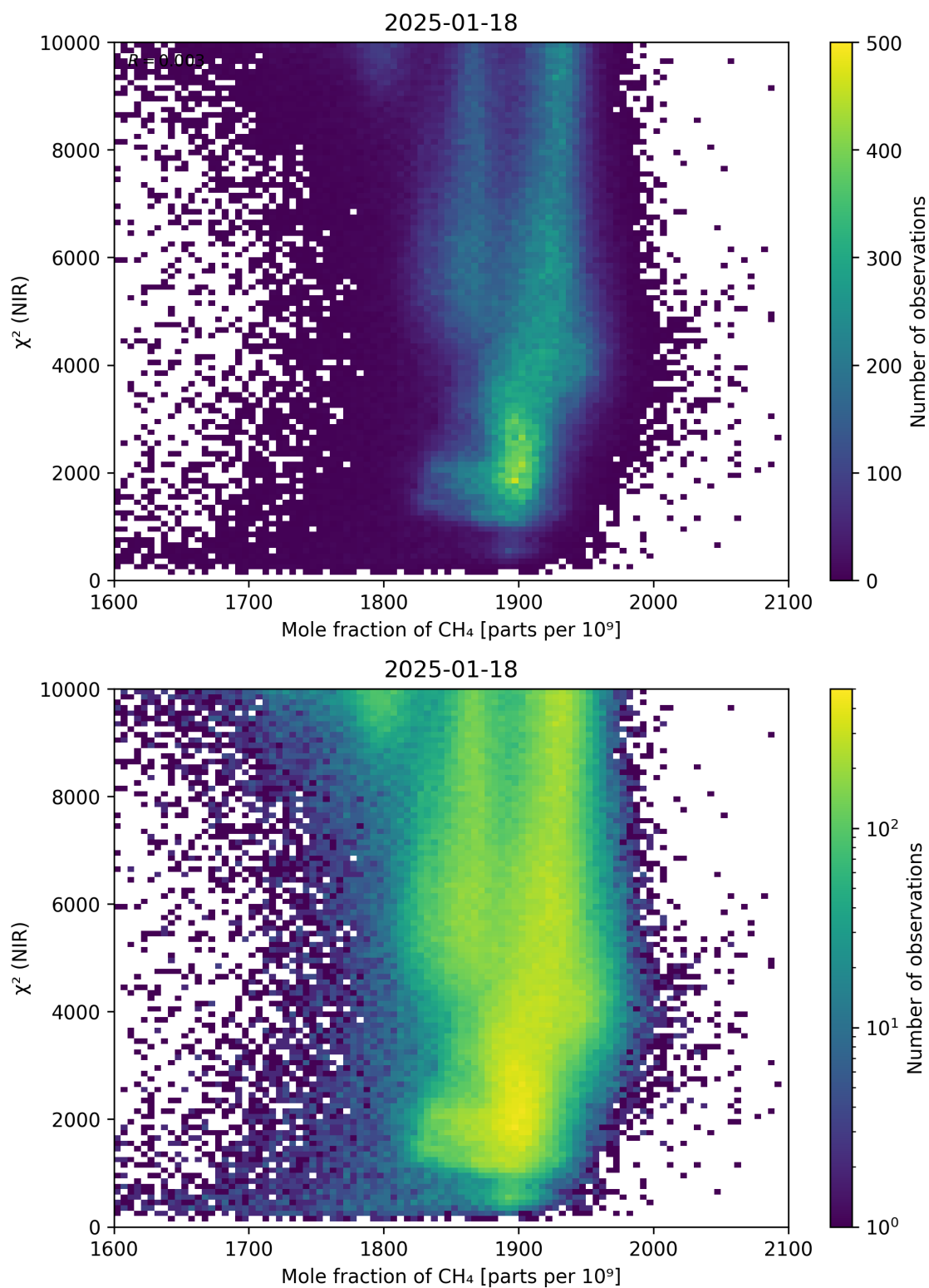
Figure 70: Scatter density plot of “Mole fraction of CH 4 ” against “ \chi^2 (NIR)” for 2025-01-17 to 2025-01-19.
