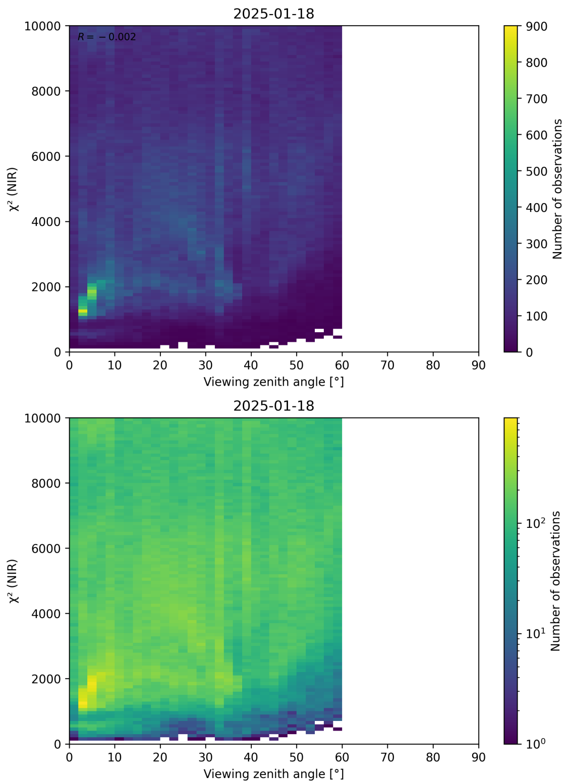
Figure 105: Scatter density plot of “Viewing zenith angle” against “ \chi^2 (NIR)” for 2025-01-17 to 2025-01-19.
