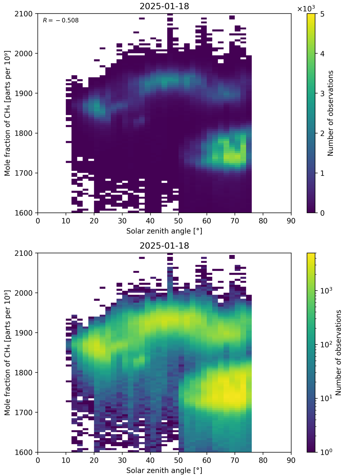
Figure 99: Scatter density plot of “Solar zenith angle” against “Mole fraction of \text{CH}_4 ” for 2025-01-17 to 2025-01-19.
