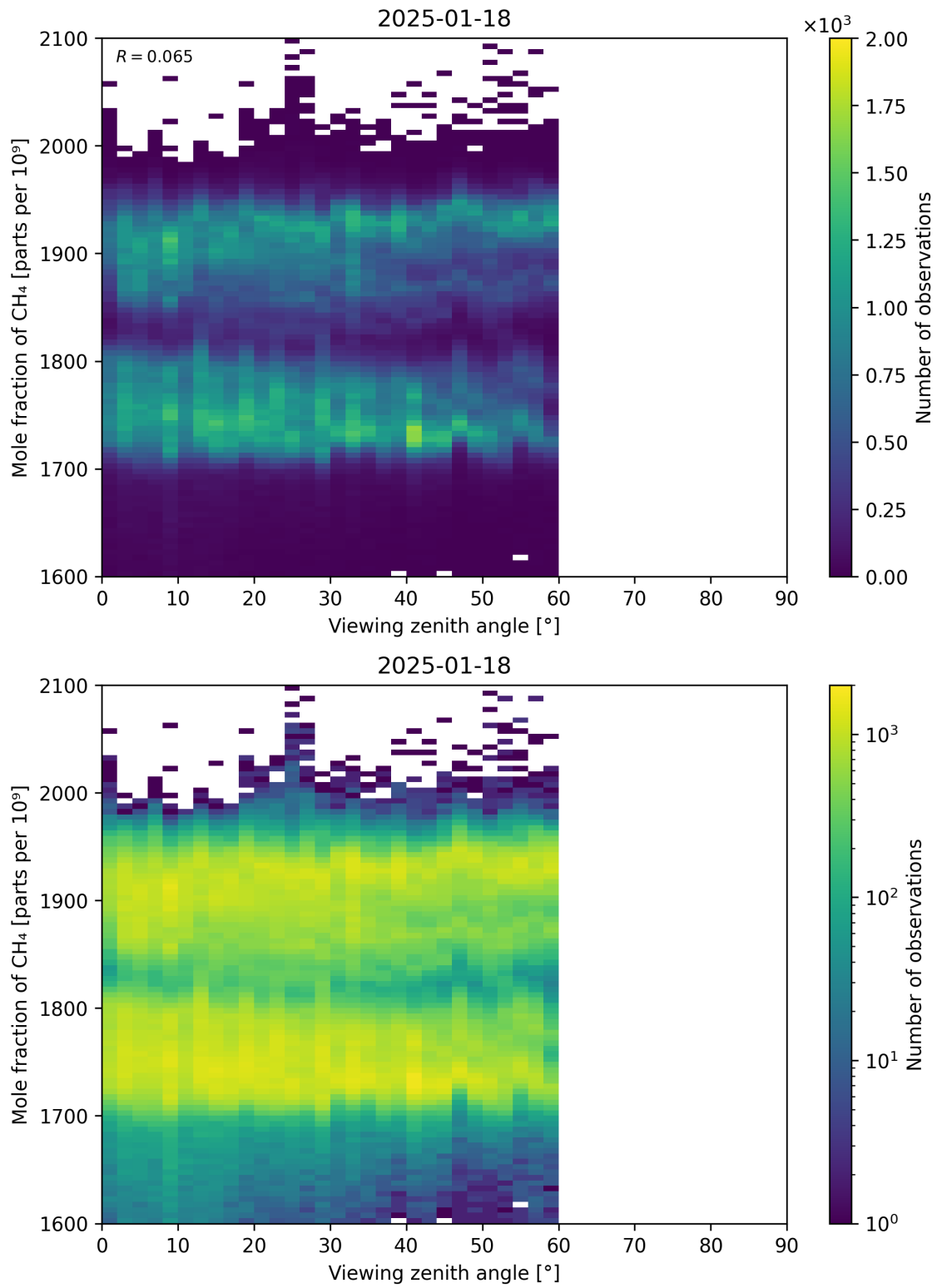
Figure 110: Scatter density plot of “Viewing zenith angle” against “Mole fraction of \text{CH}_4 ” for 2025-01-17 to 2025-01-19.
