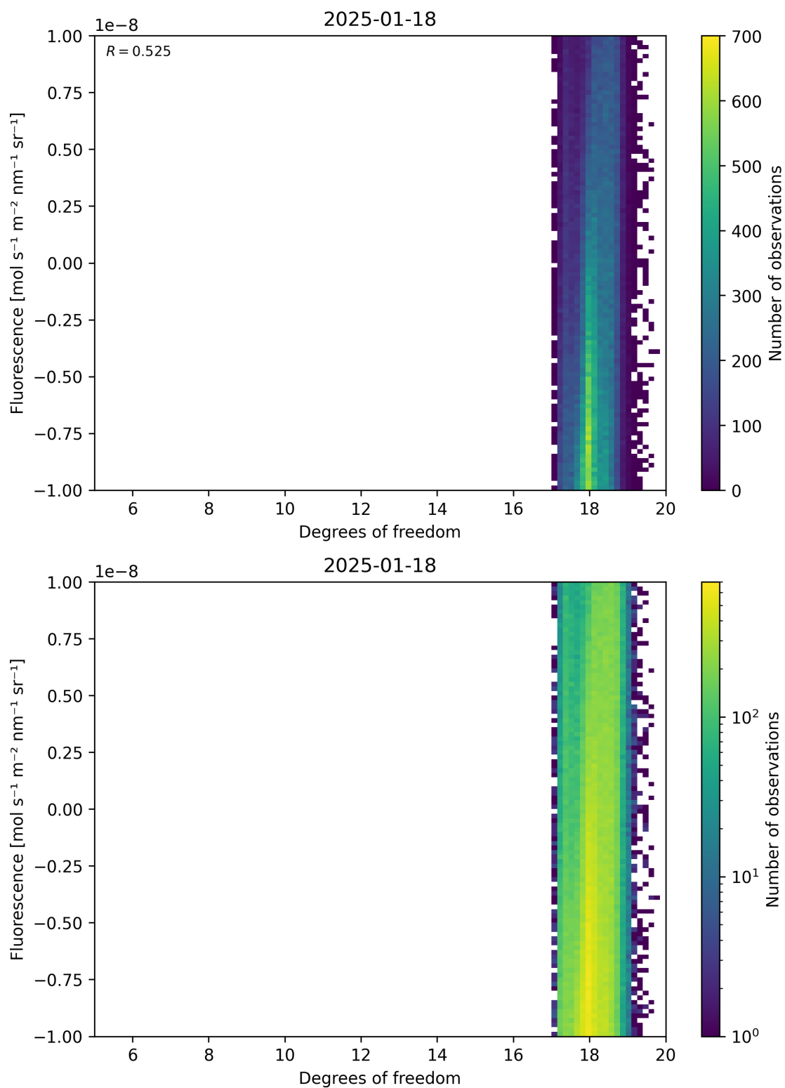
Figure 51: Scatter density plot of “Degrees of freedom” against “Fluorescence” for 2025-01-17 to 2025-01-19.
