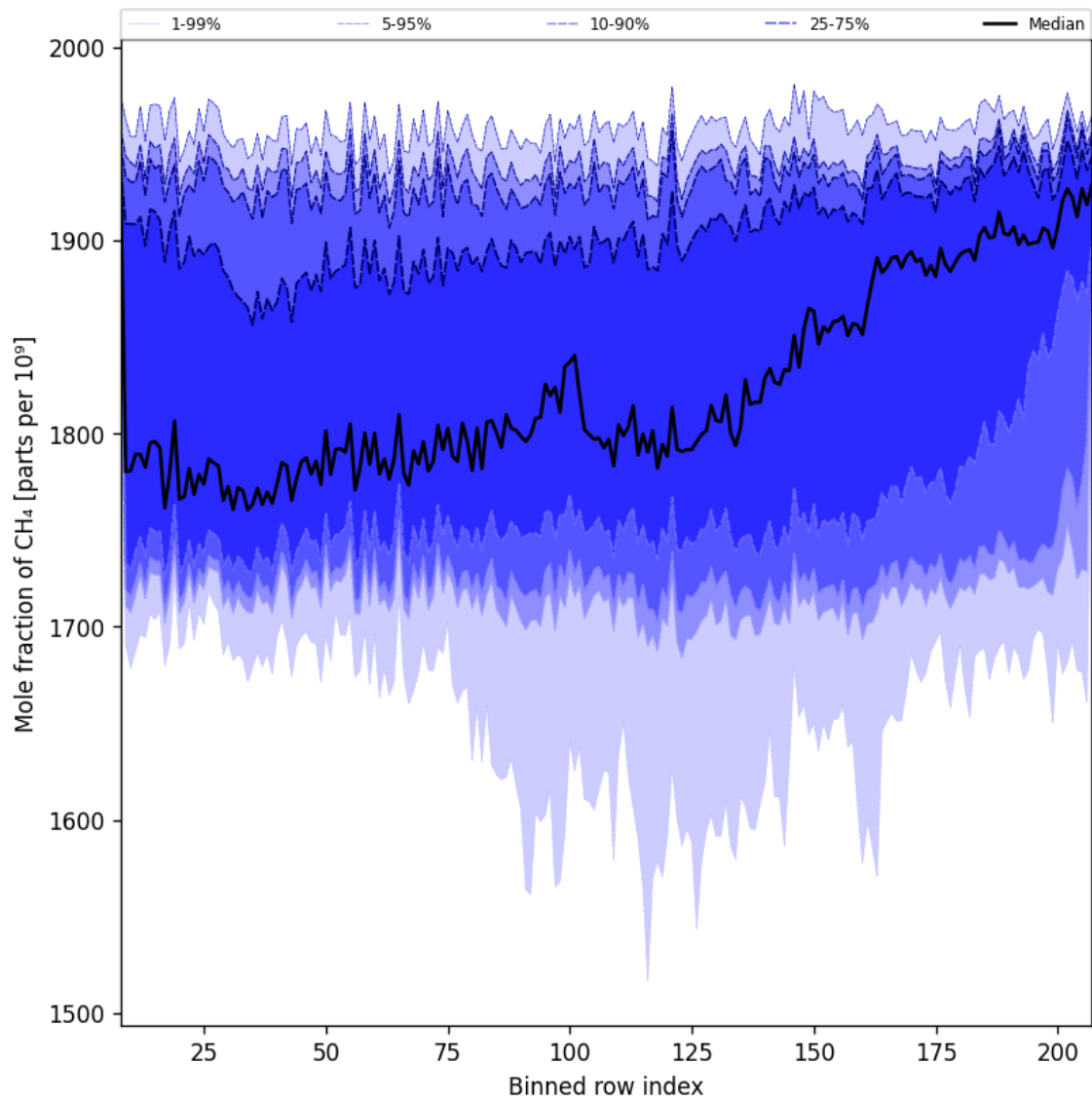
Figure 34: Along track statistics of “Mole fraction of CH 4 ” for 2025-01-17 to 2025-01-19
