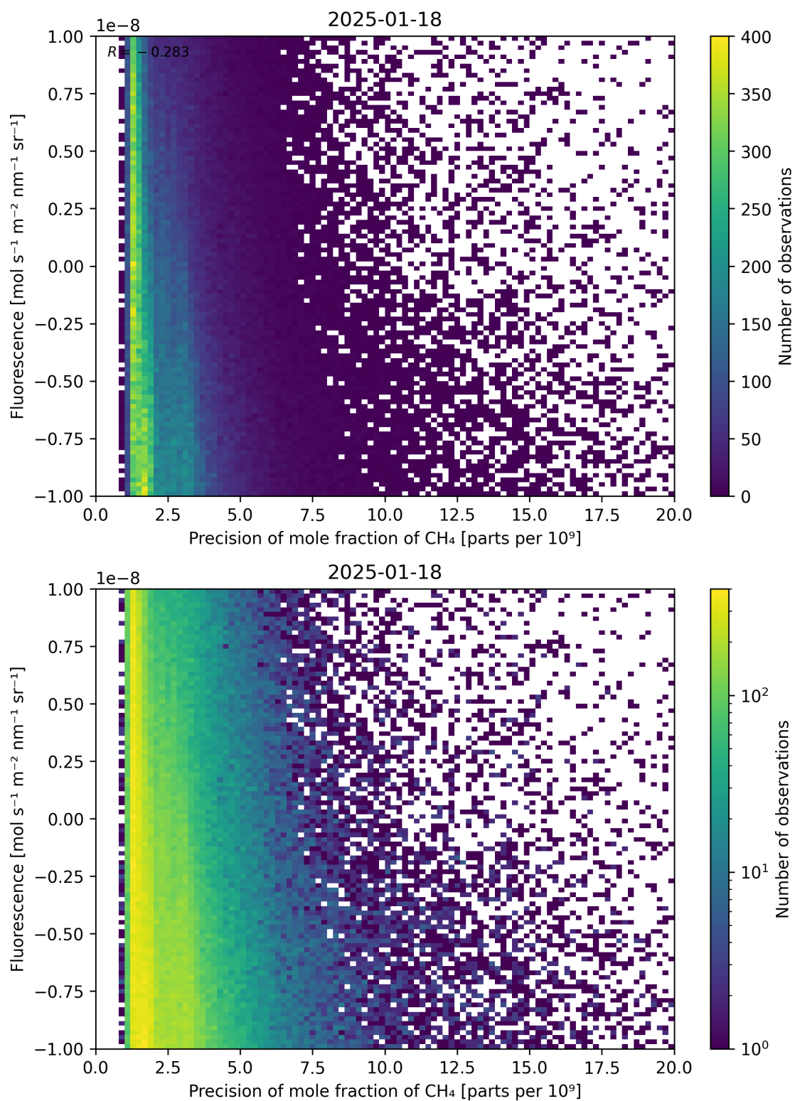
Figure 81: Scatter density plot of “Precision of mole fraction of \text{CH}_4 ” against “Fluorescence” for 2025-01-17 to 2025-01-19.
