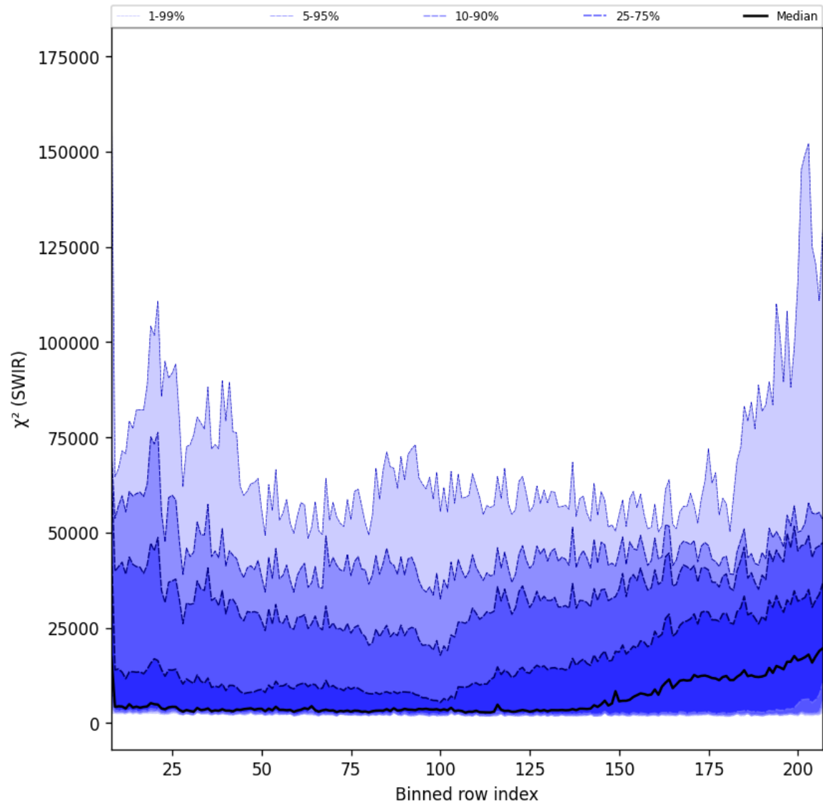
Figure 39: Along track statistics of “ \chi^2 (SWIR)” for 2025-01-17 to 2025-01-19
