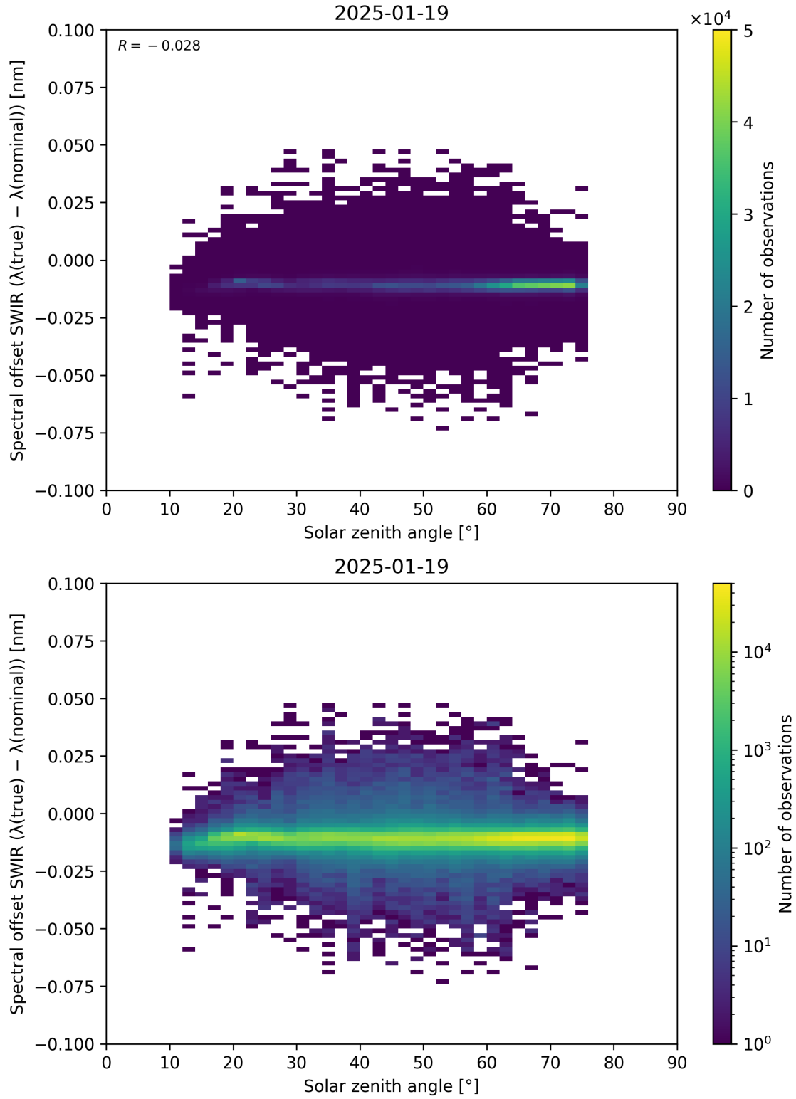
Figure 104: Scatter density plot of “Solar zenith angle” against “Spectral offset SWIR ( \lambda_{\text{true}} - \lambda_{\text{nominal}} )” for 2025-01-18 to 2025-01-20.
