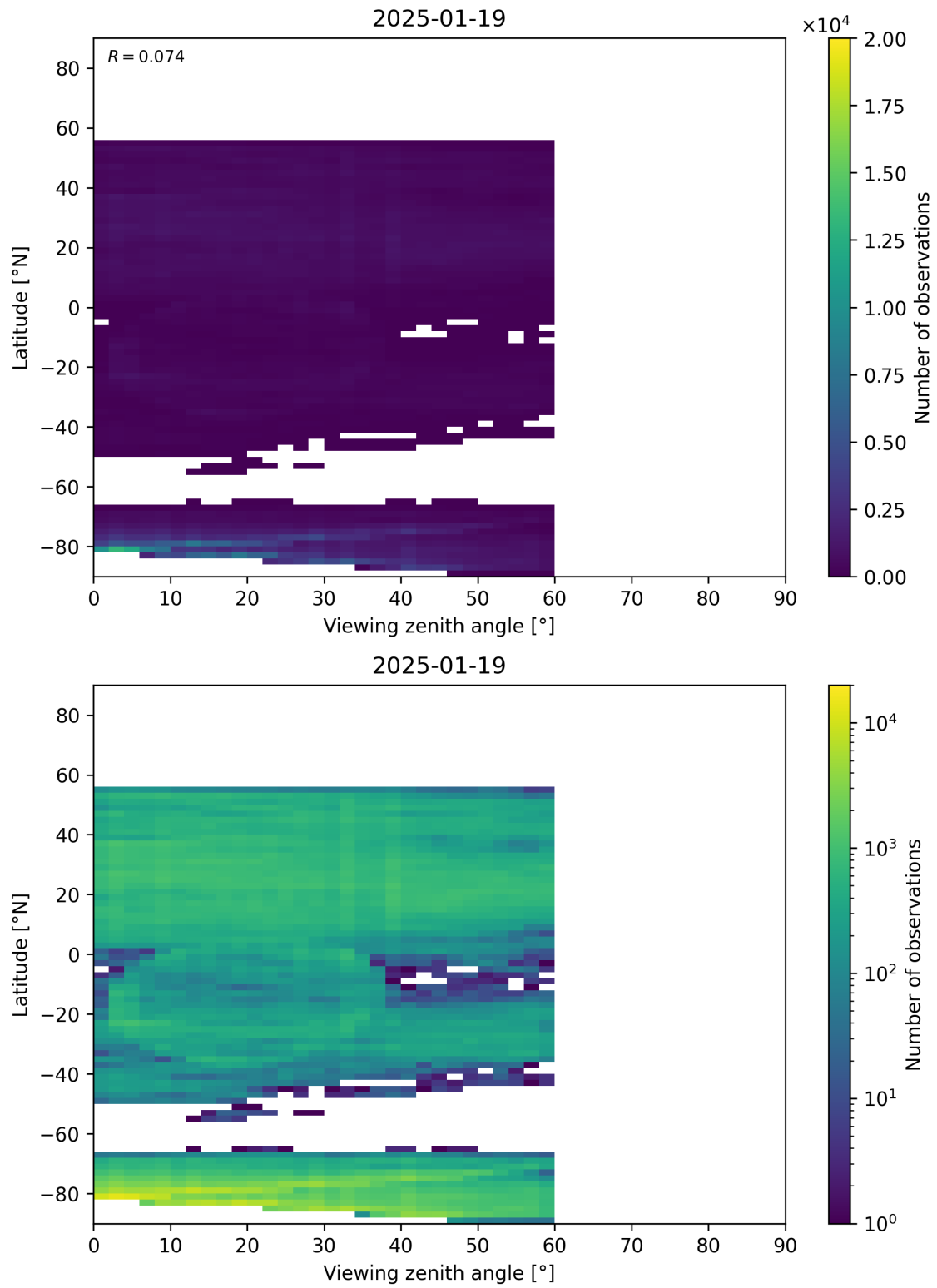
Figure 109: Scatter density plot of “Viewing zenith angle” against “Latitude” for 2025-01-18 to 2025-01-20.
