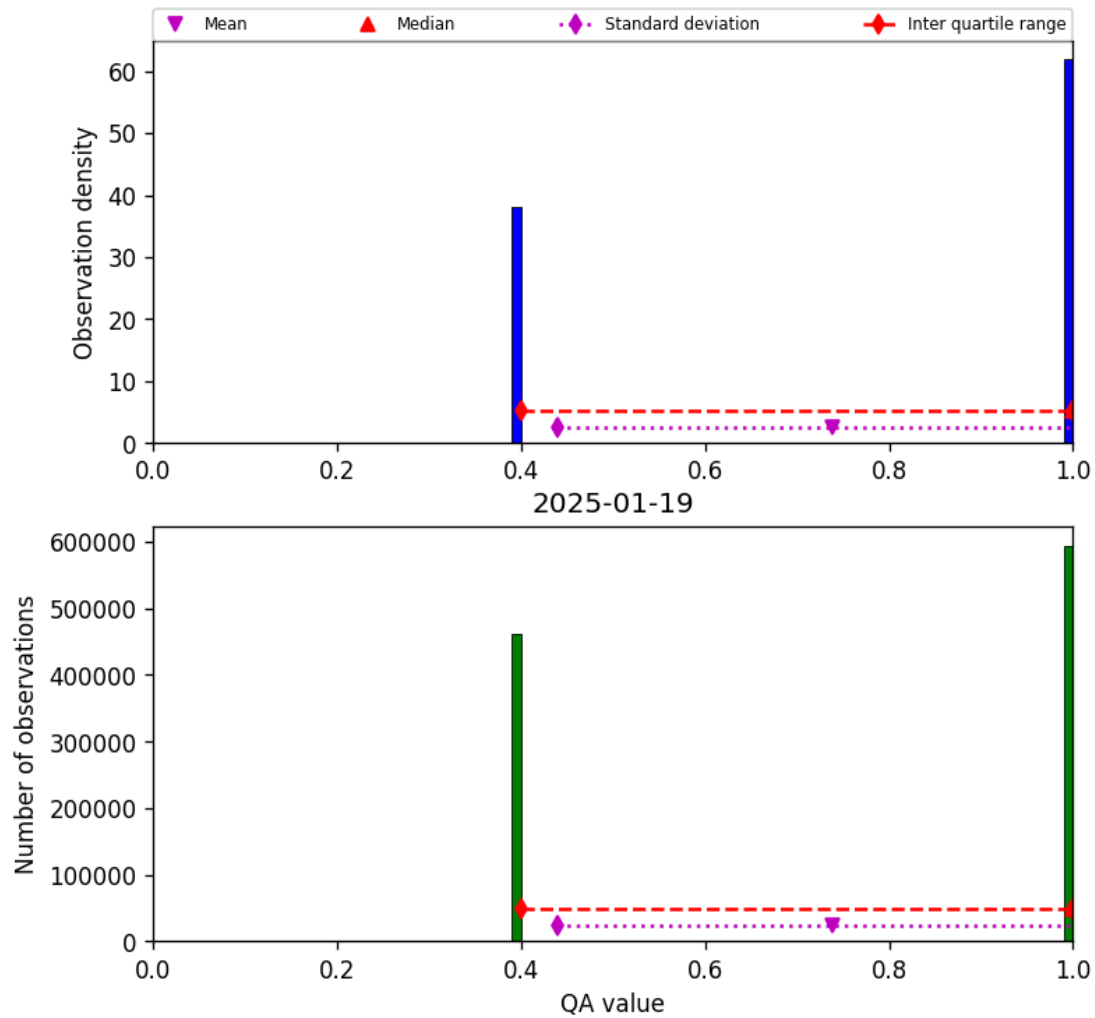
Figure 22: Histogram of “QA value” for 2025-01-18 to 2025-01-20
