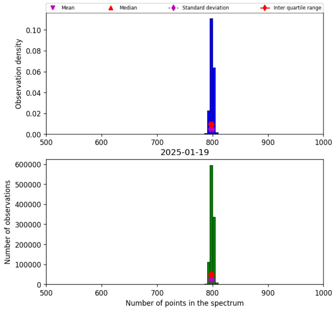
Figure 26: Histogram of “Number of points in the spectrum” for 2025-01-18 to 2025-01-20
