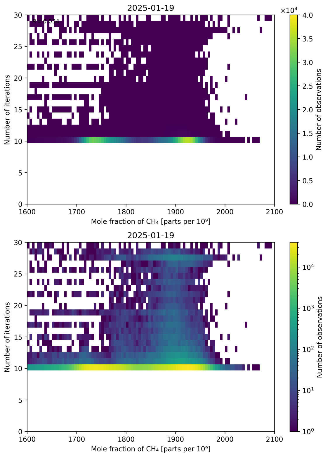
Figure 76: Scatter density plot of “Mole fraction of CH 4 ” against “Number of iterations” for 2025-01-18 to 2025-01-20.
