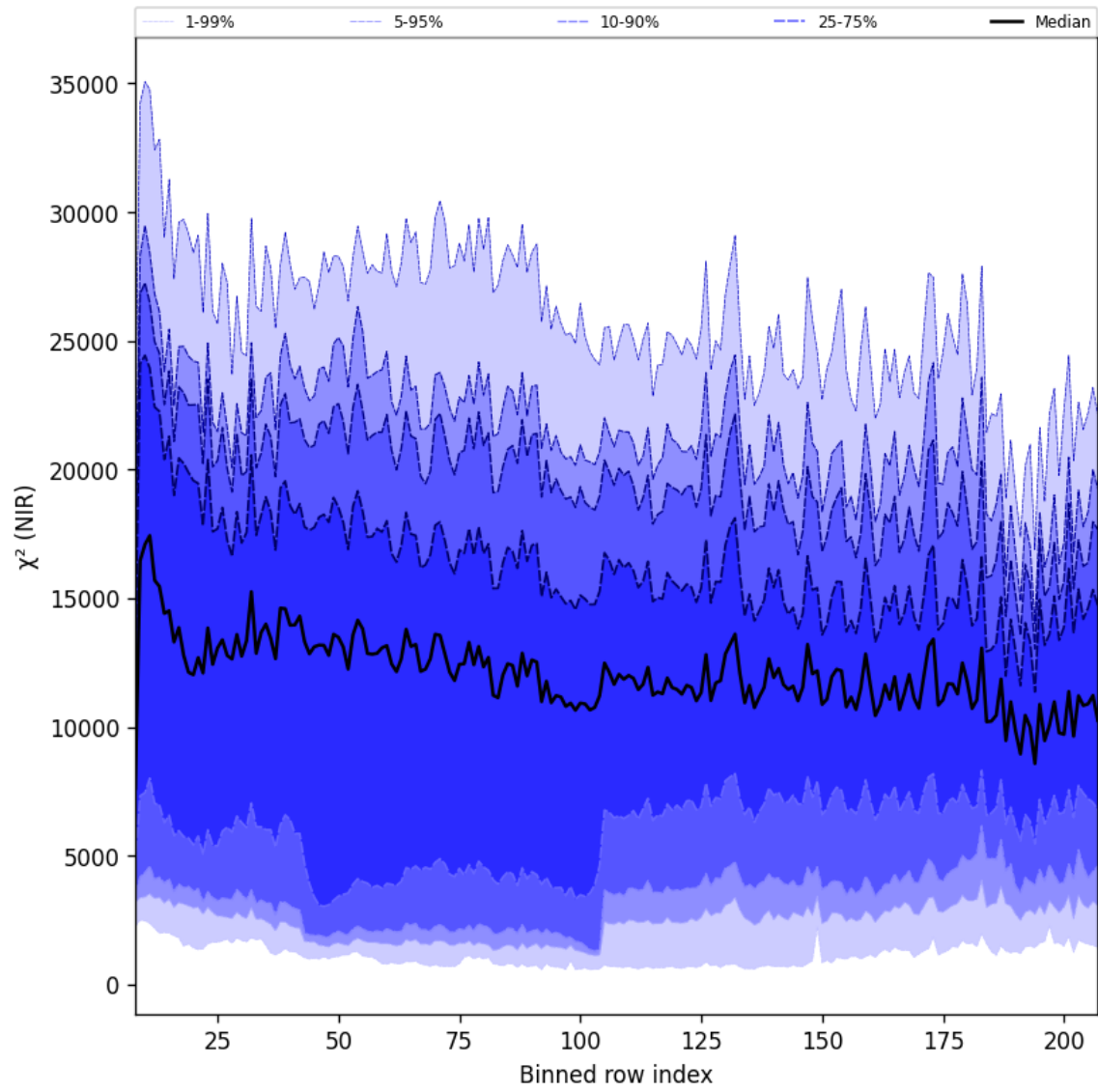
Figure 40: Along track statistics of “ \chi^2 (NIR)” for 2025-01-18 to 2025-01-20
