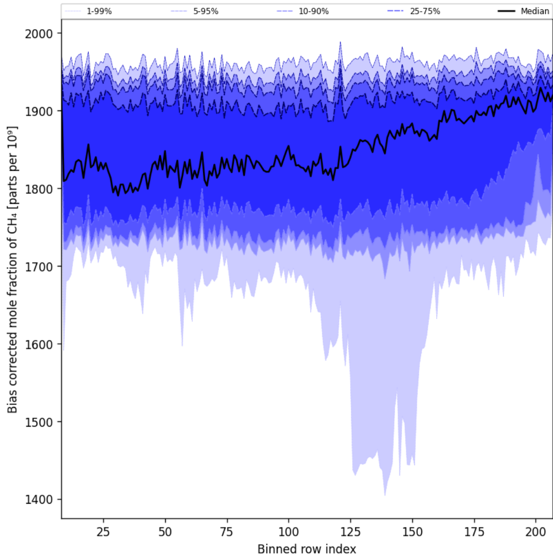
Figure 36: Along track statistics of “Bias corrected mole fraction of CH 4 ” for 2025-01-18 to 2025-01-20
