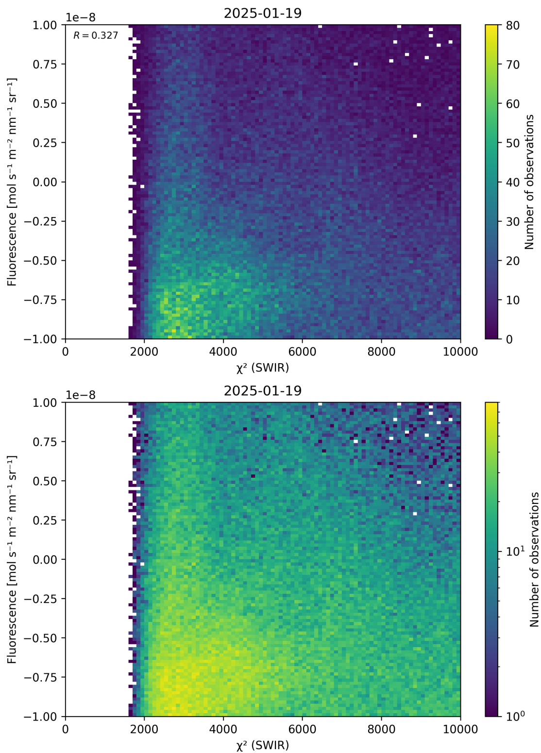
Figure 49: Scatter density plot of “ \chi^2 (SWIR)” against “Fluorescence” for 2025-01-18 to 2025-01-20.
