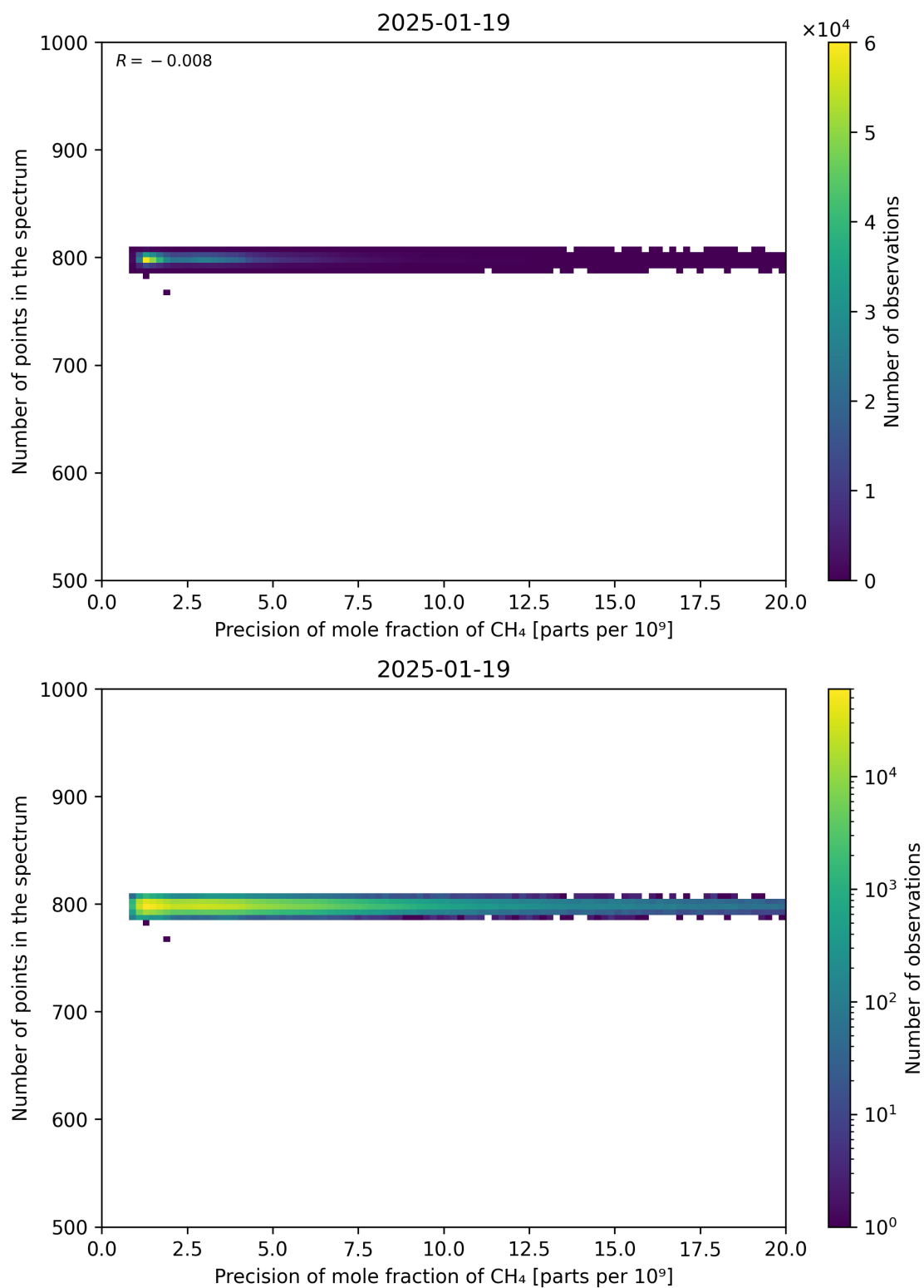
Figure 84: Scatter density plot of “Precision of mole fraction of CH 4 ” against “Number of points in the spectrum” for 2025-01-18 to 2025-01-20.
