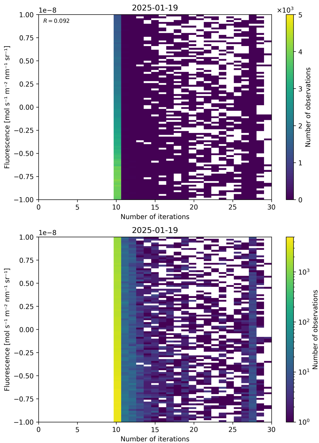
Figure 87: Scatter density plot of “Number of iterations” against “Fluorescence” for 2025-01-18 to 2025-01-20.
