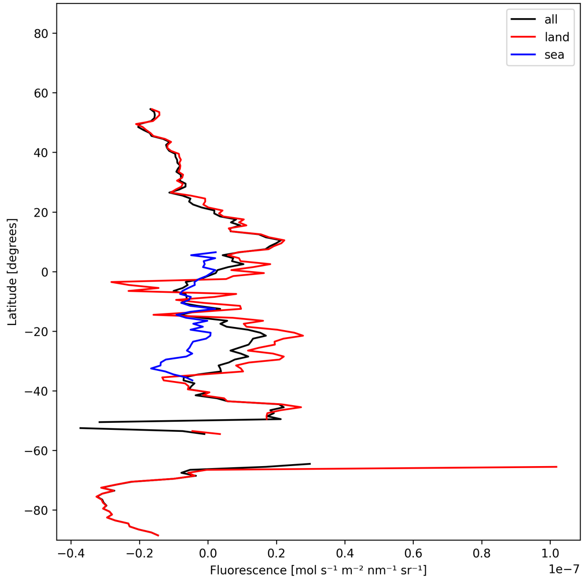
Figure 21: Zonal average of “Fluorescence” for 2025-01-18 to 2025-01-20.
