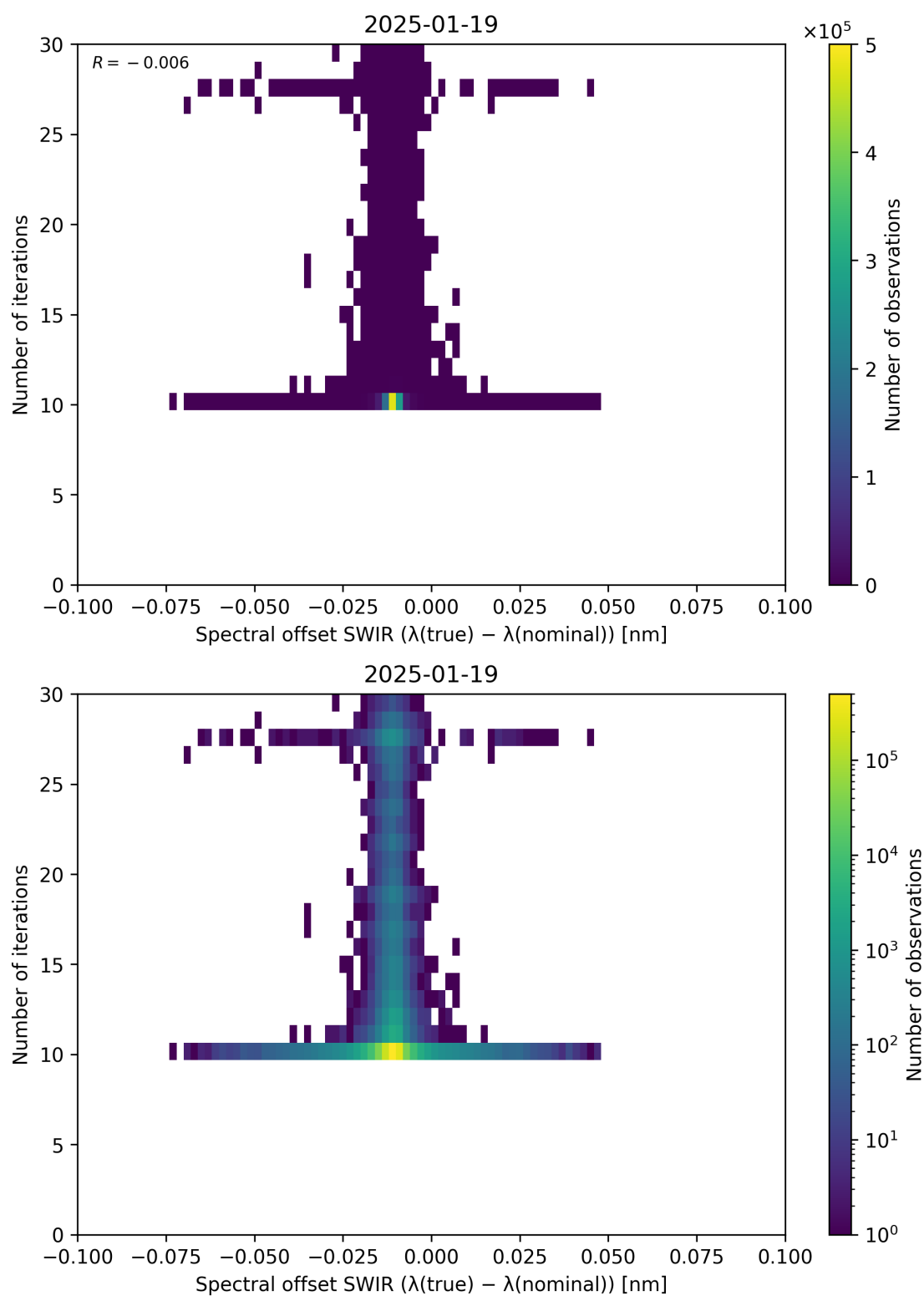
Figure 121: Scatter density plot of “Spectral offset SWIR ( \lambda_{\text{true}} - \lambda_{\text{nominal}} )” against “Number of iterations” for 2025-01-18 to 2025-01-20.
