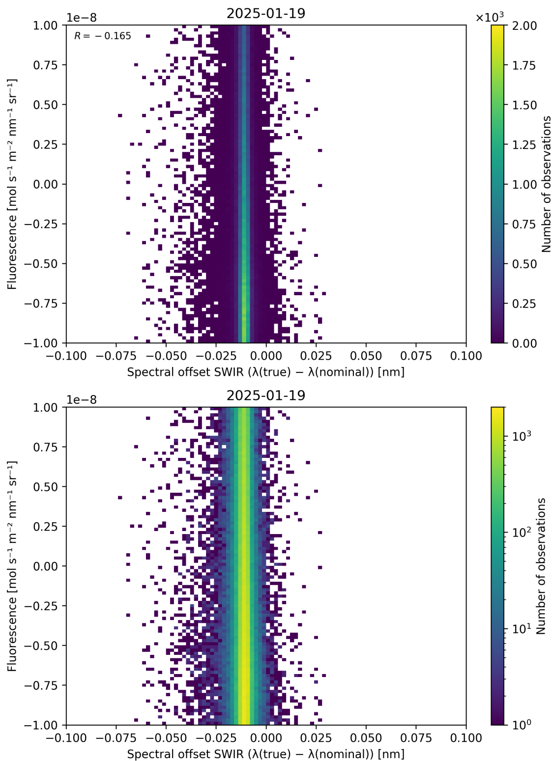
Figure 120: Scatter density plot of “Spectral offset SWIR ( \lambda_{\text{true}} - \lambda_{\text{nominal}} )” against “Fluorescence” for 2025-01-18 to 2025-01-20.
