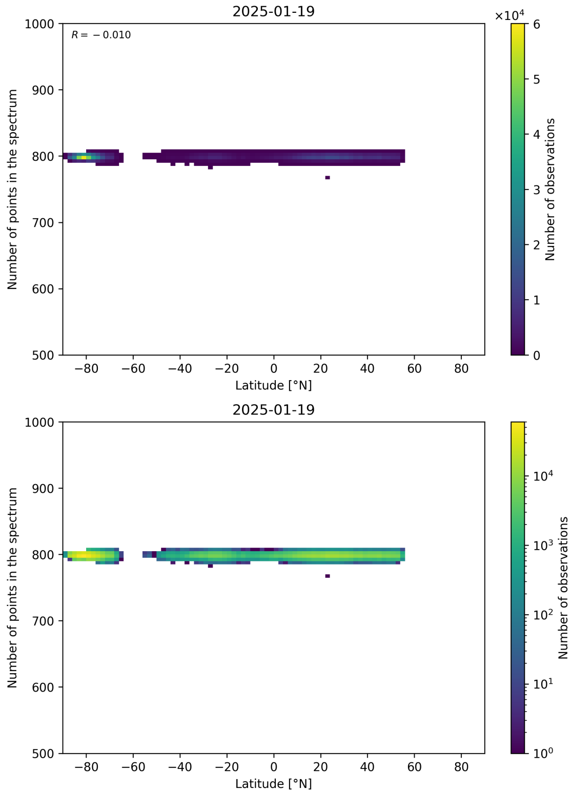
Figure 61: Scatter density plot of “Latitude” against “Number of points in the spectrum” for 2025-01-18 to 2025-01-20.
