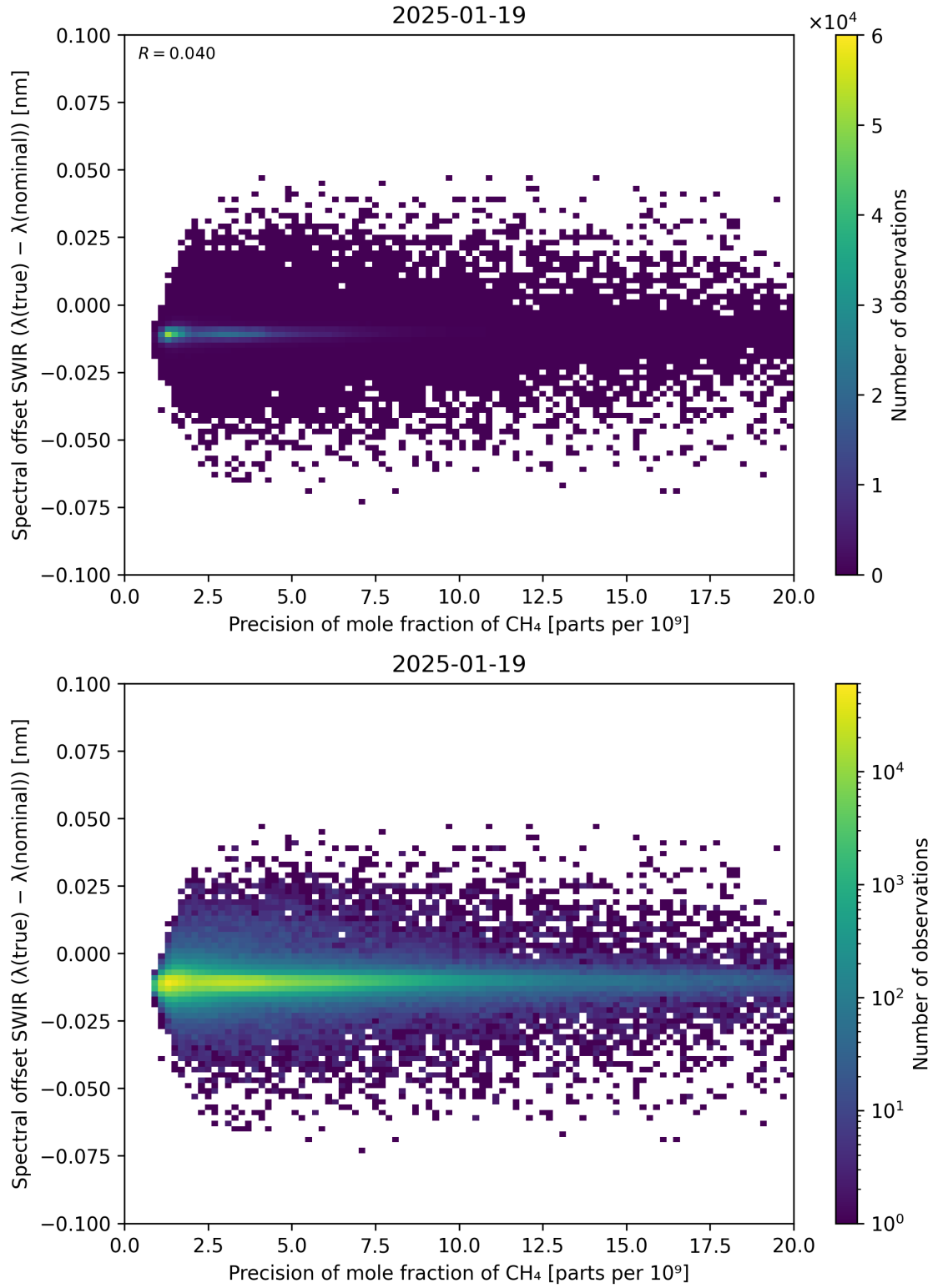
Figure 85: Scatter density plot of “Precision of mole fraction of \text{CH}_4 ” against “Spectral offset SWIR ( \lambda_{\text{true}} - \lambda_{\text{nominal}} )” for 2025-01-18 to 2025-01-20.
