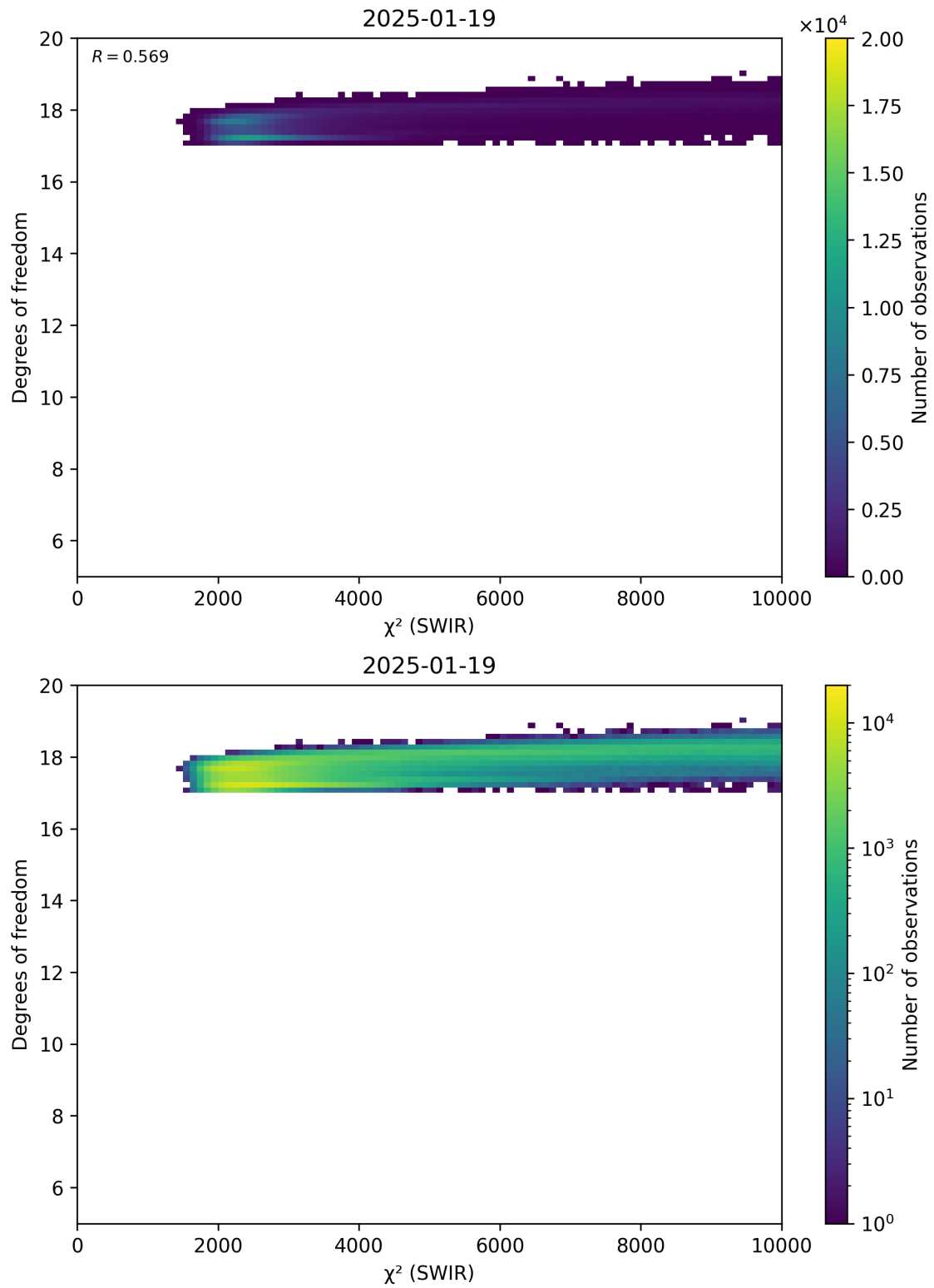
Figure 48: Scatter density plot of “ \chi^2 (SWIR)” against “Degrees of freedom” for 2025-01-18 to 2025-01-20.
