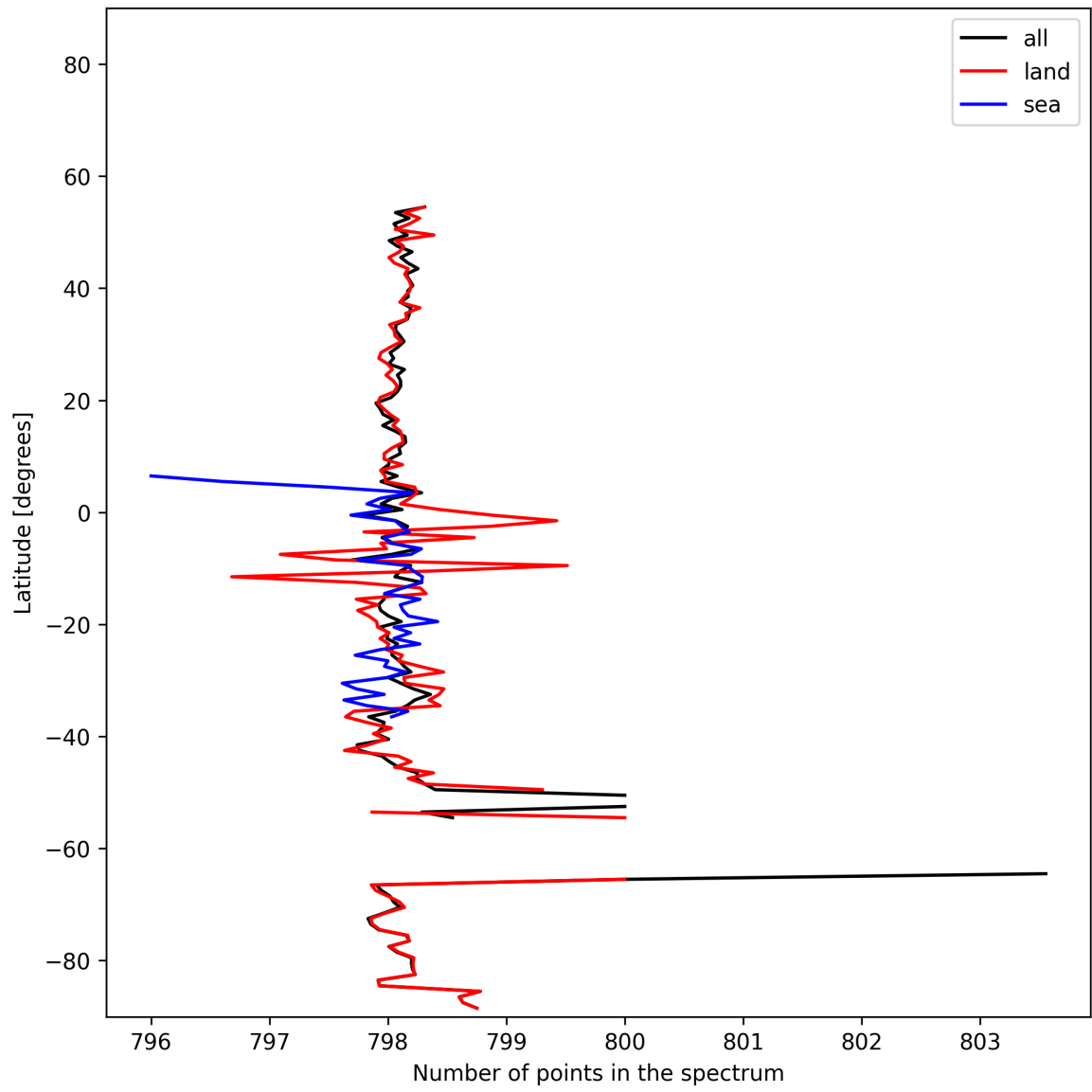
Figure 15: Zonal average of “Number of points in the spectrum” for 2025-01-18 to 2025-01-20.
