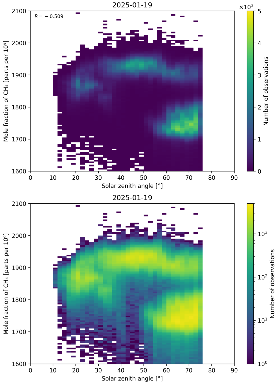
Figure 99: Scatter density plot of “Solar zenith angle” against “Mole fraction of CH 4 ” for 2025-01-18 to 2025-01-20.
