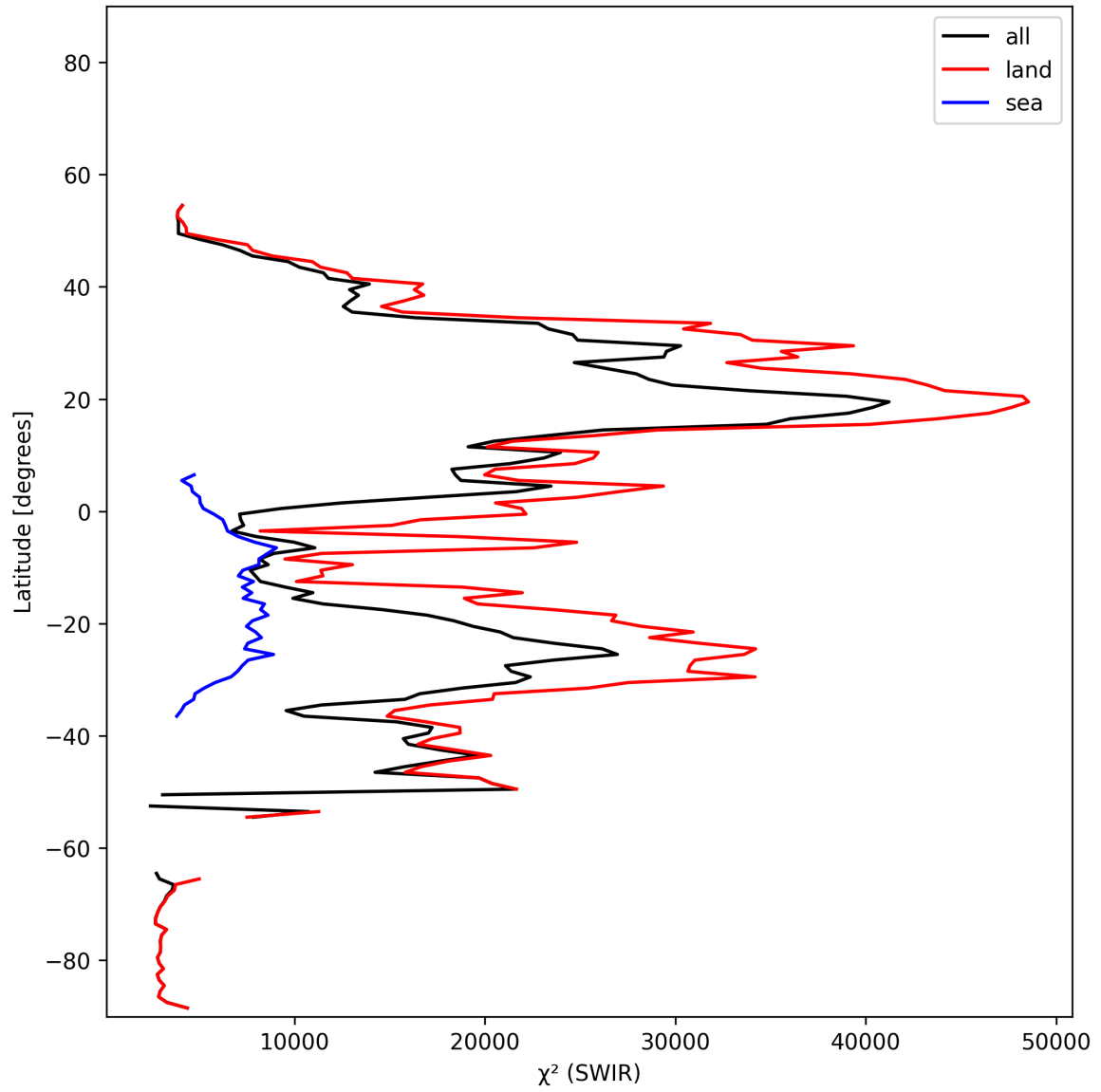
Figure 17: Zonal average of “ \chi^2 (SWIR)” for 2025-01-18 to 2025-01-20.
