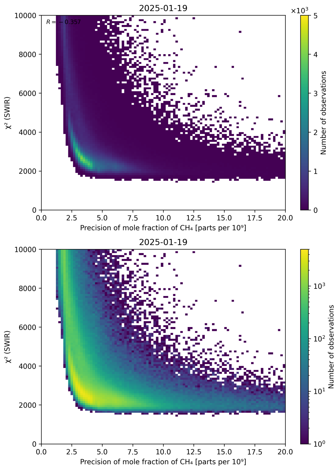
Figure 79: Scatter density plot of “Precision of mole fraction of CH 4 ” against “ \chi^2 (SWIR)” for 2025-01-18 to 2025-01-20.
