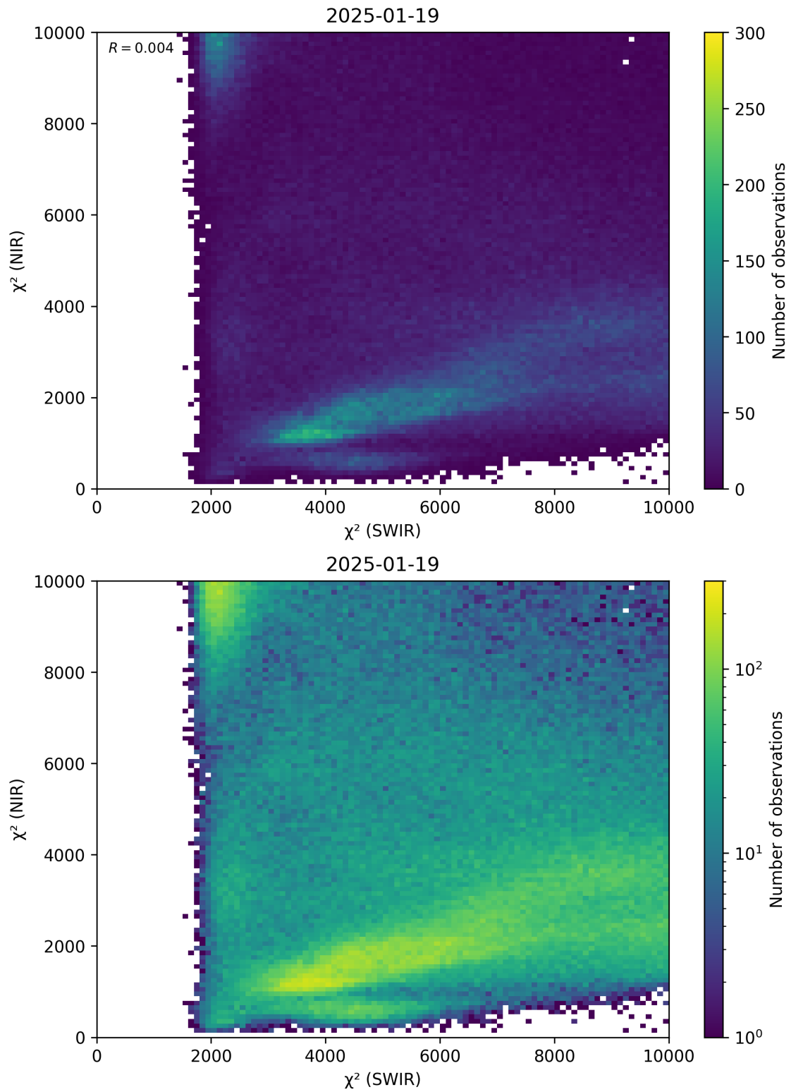
Figure 47: Scatter density plot of “ \chi^2 (SWIR)” against “ \chi^2 (NIR)” for 2025-01-18 to 2025-01-20.
