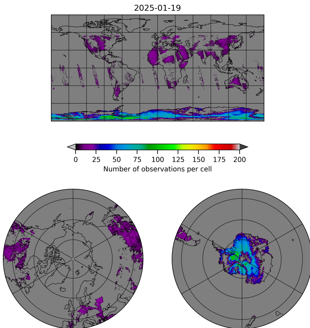
Figure 10: Map of the number of observations for 2025-01-18 to 2025-01-20
