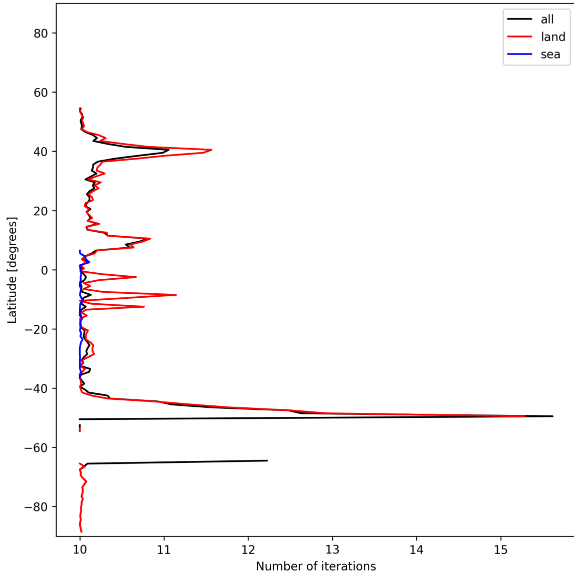
Figure 20: Zonal average of “Number of iterations” for 2025-01-18 to 2025-01-20.
