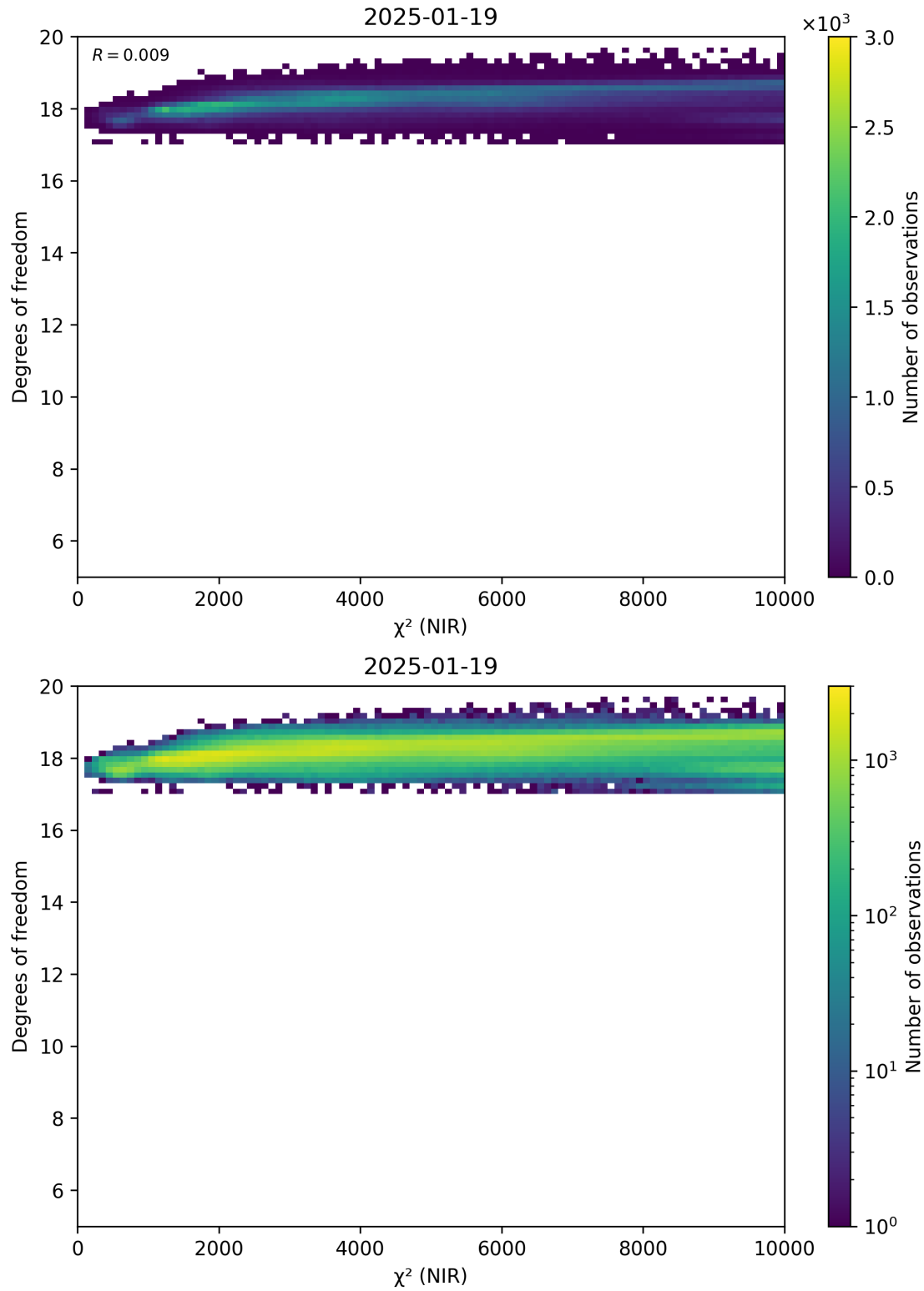
Figure 44: Scatter density plot of “ \chi^2 (NIR)” against “Degrees of freedom” for 2025-01-18 to 2025-01-20.
