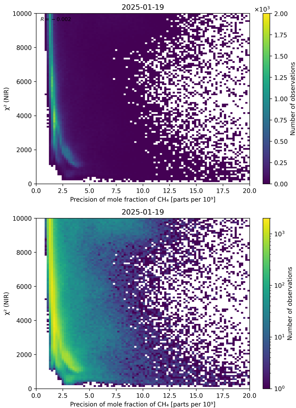
Figure 78: Scatter density plot of “Precision of mole fraction of CH 4 ” against “ \chi^2 (NIR)” for 2025-01-18 to 2025-01-20.
