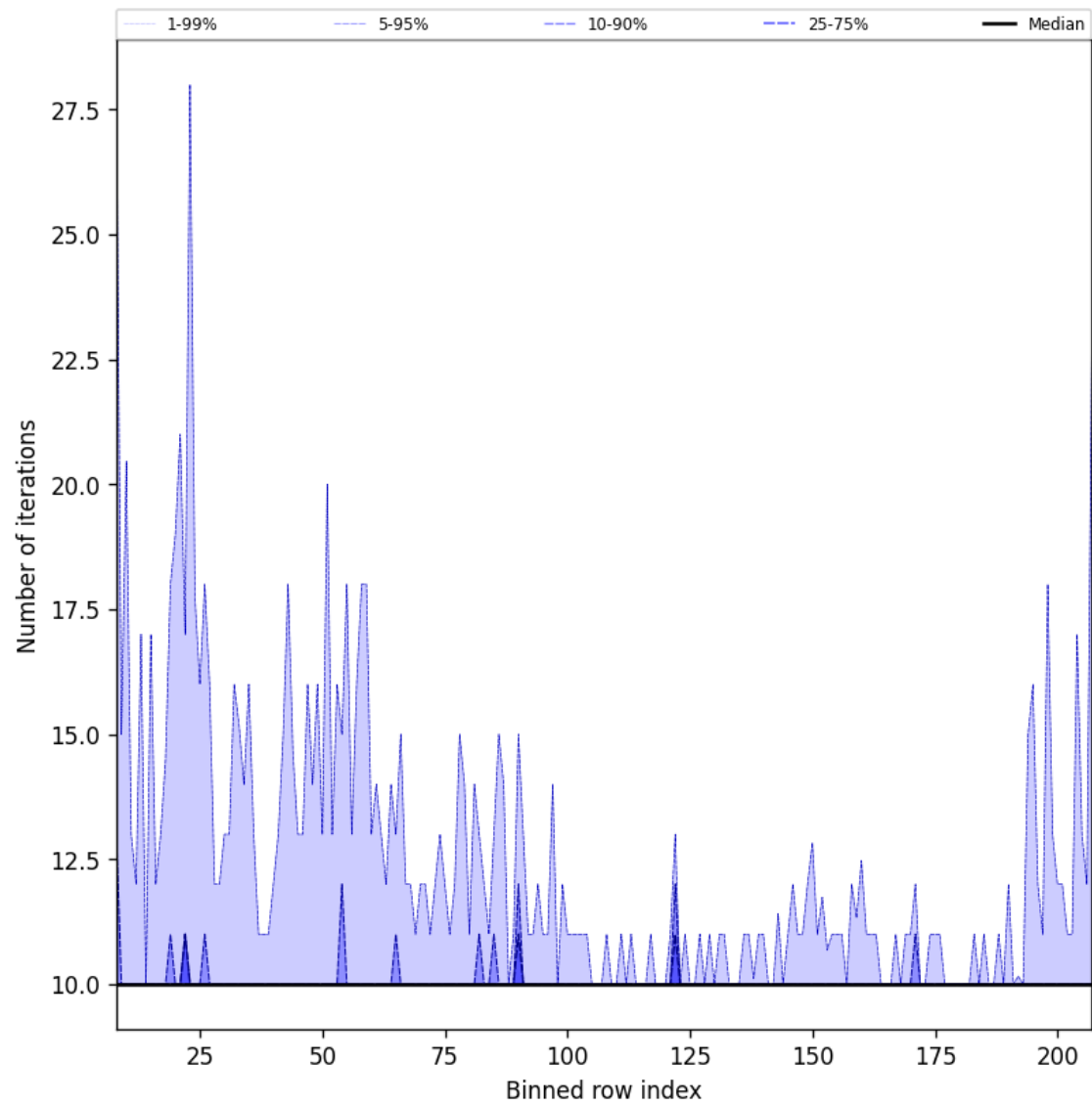
Figure 42: Along track statistics of “Number of iterations” for 2025-01-18 to 2025-01-20
