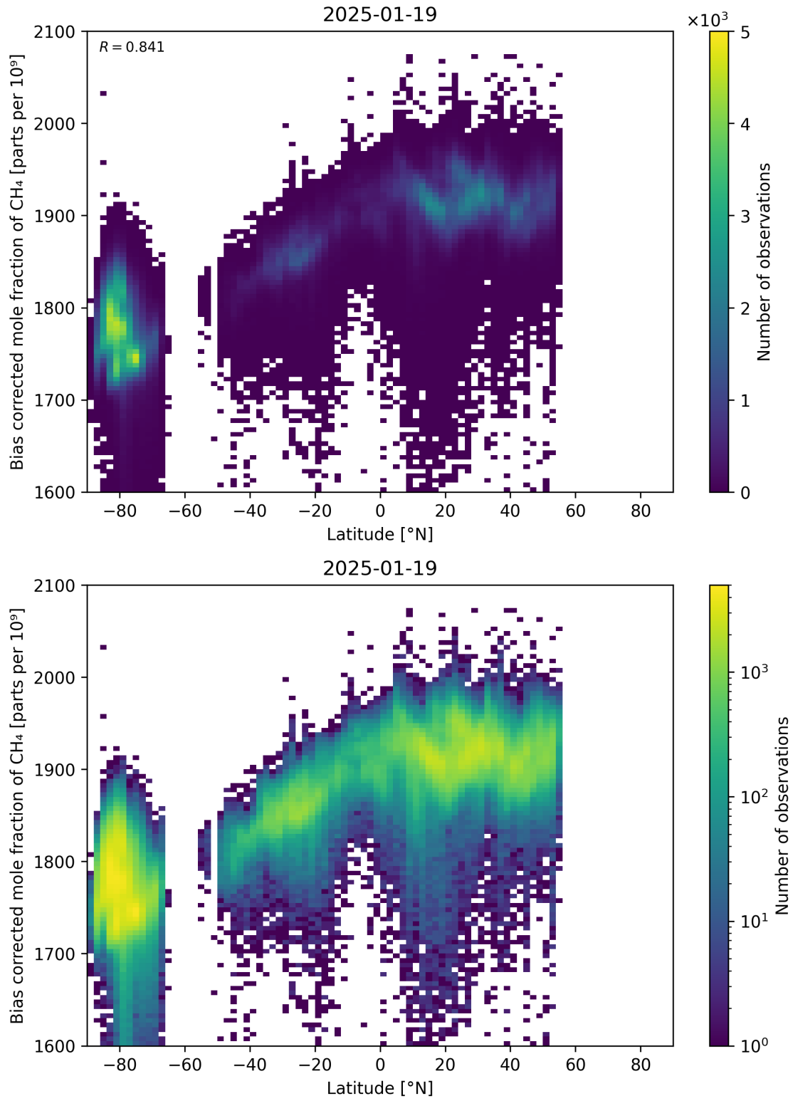
Figure 58: Scatter density plot of “Latitude” against “Bias corrected mole fraction of \text{CH}_4 ” for 2025-01-18 to 2025-01-20.
