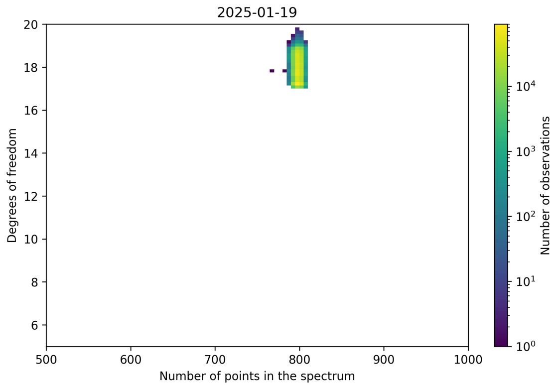
Figure 90: Scatter density plot of “Number of points in the spectrum” against “Degrees of freedom” for 2025-01-18 to 2025-01-20.
