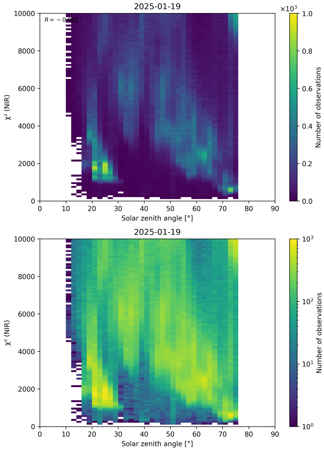
Figure 94: Scatter density plot of “Solar zenith angle” against “ \chi^2 (NIR)” for 2025-01-18 to 2025-01-20.
