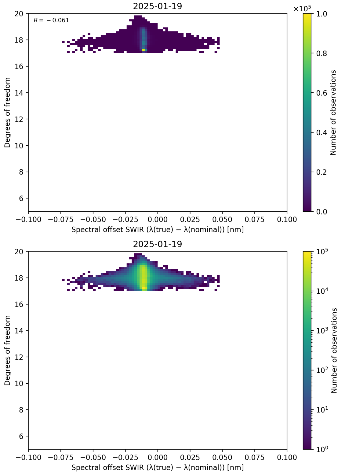
Figure 119: Scatter density plot of “Spectral offset SWIR ( \lambda_{\text{true}} - \lambda_{\text{nominal}} )” against “Degrees of freedom” for 2025-01-18 to 2025-01-20.
