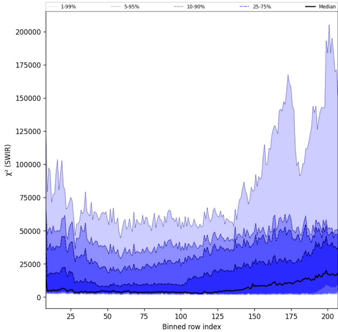
Figure 39: Along track statistics of “ \chi^2 (SWIR)” for 2025-01-18 to 2025-01-20
