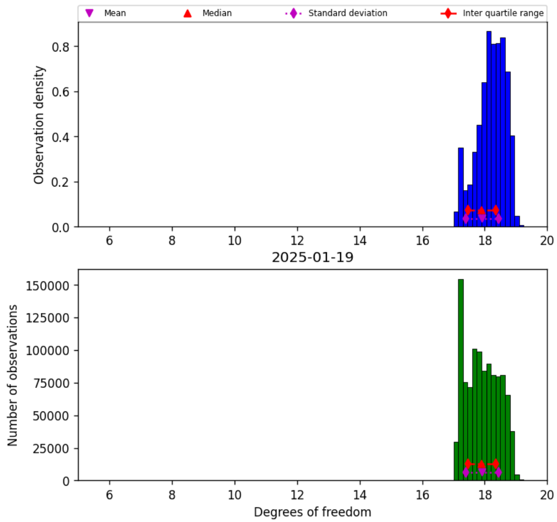
Figure 30: Histogram of “Degrees of freedom” for 2025-01-18 to 2025-01-20
