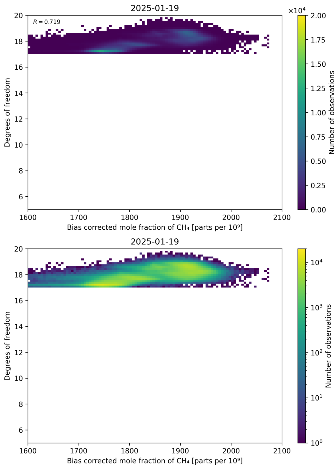
Figure 65: Scatter density plot of “Bias corrected mole fraction of CH 4 ” against “Degrees of freedom” for 2025-01-18 to 2025-01-20.
