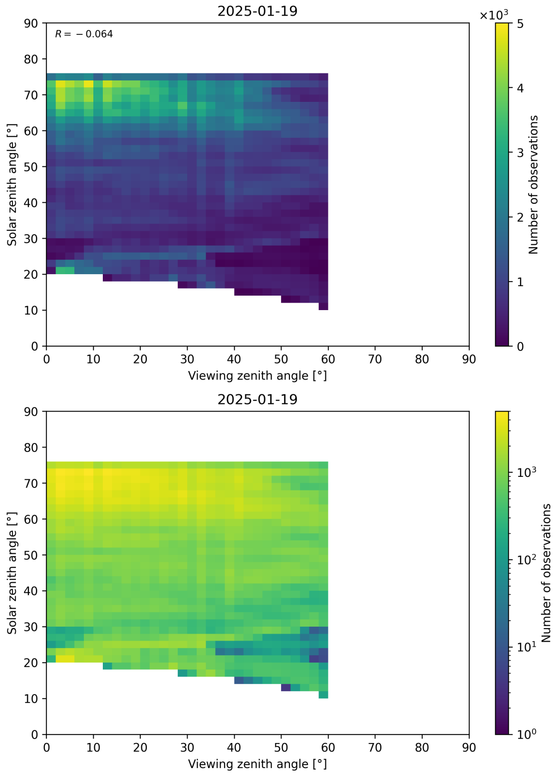
Figure 115: Scatter density plot of “Viewing zenith angle” against “Solar zenith angle” for 2025-01-18 to 2025-01-20.
