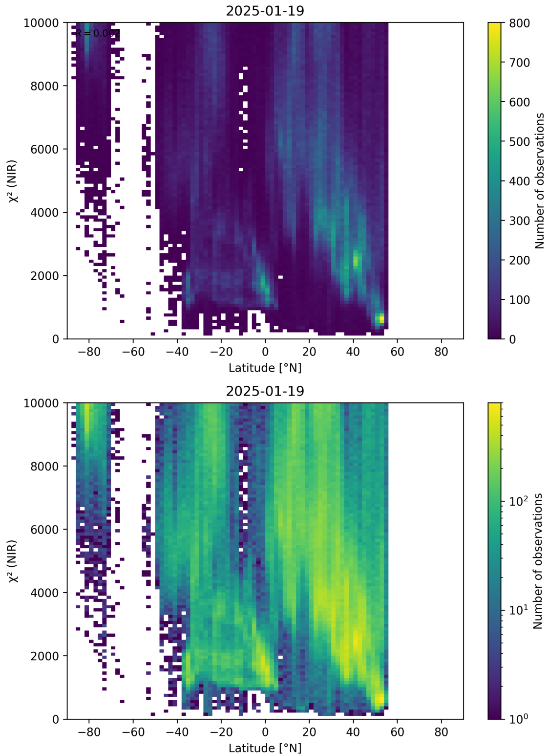
Figure 53: Scatter density plot of “Latitude” against “ \chi^2 (NIR)” for 2025-01-18 to 2025-01-20.
