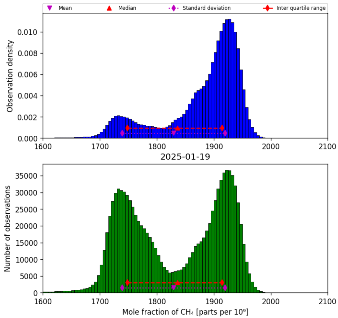
Figure 23: Histogram of “Mole fraction of CH 4 ” for 2025-01-18 to 2025-01-20
