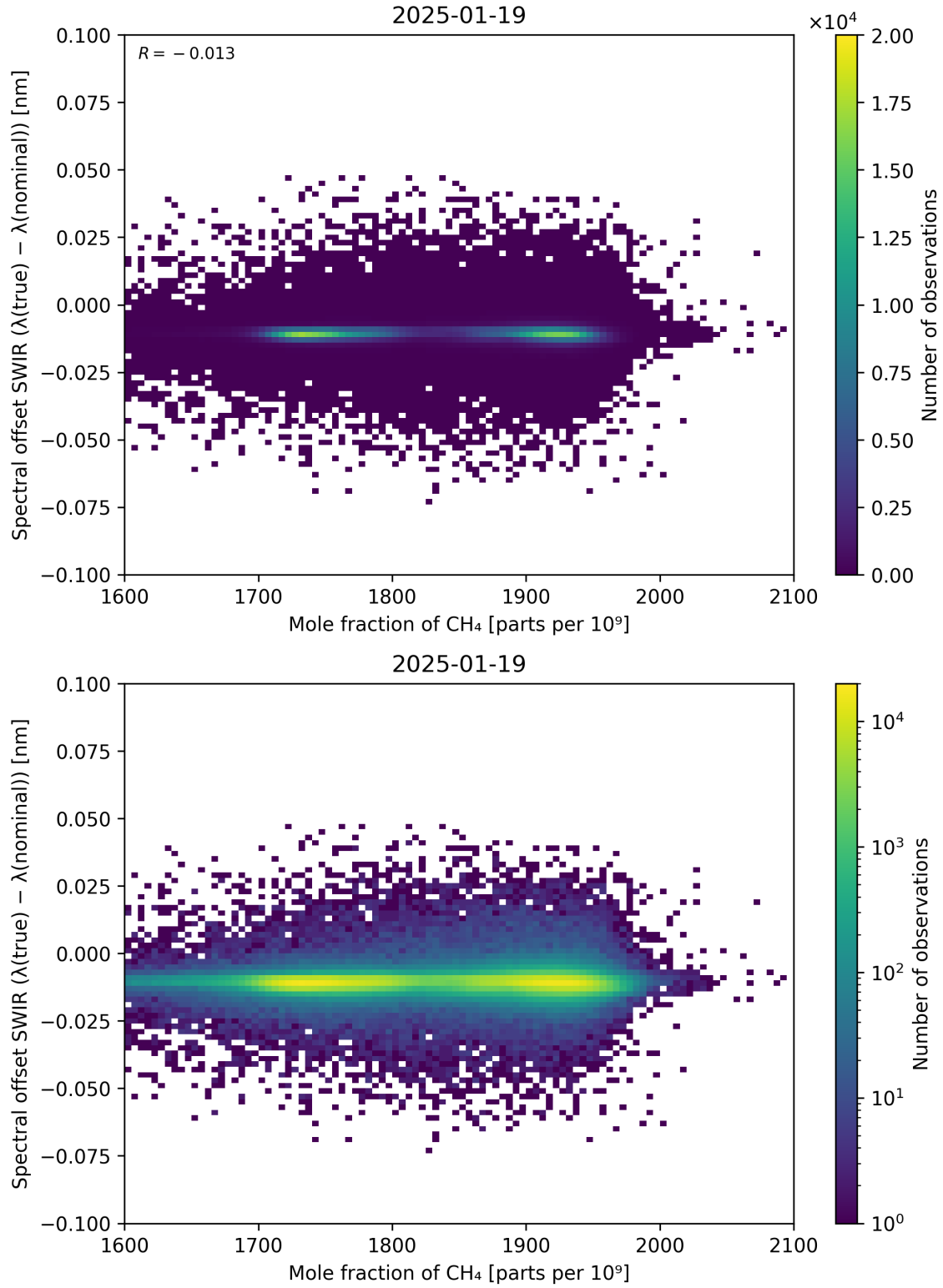
Figure 86: Scatter density plot of “Mole fraction of CH 4 ” against “Spectral offset SWIR ( \lambda_{\text{true}} - \lambda_{\text{nominal}} )” for 2025-01-18 to 2025-01-20.
