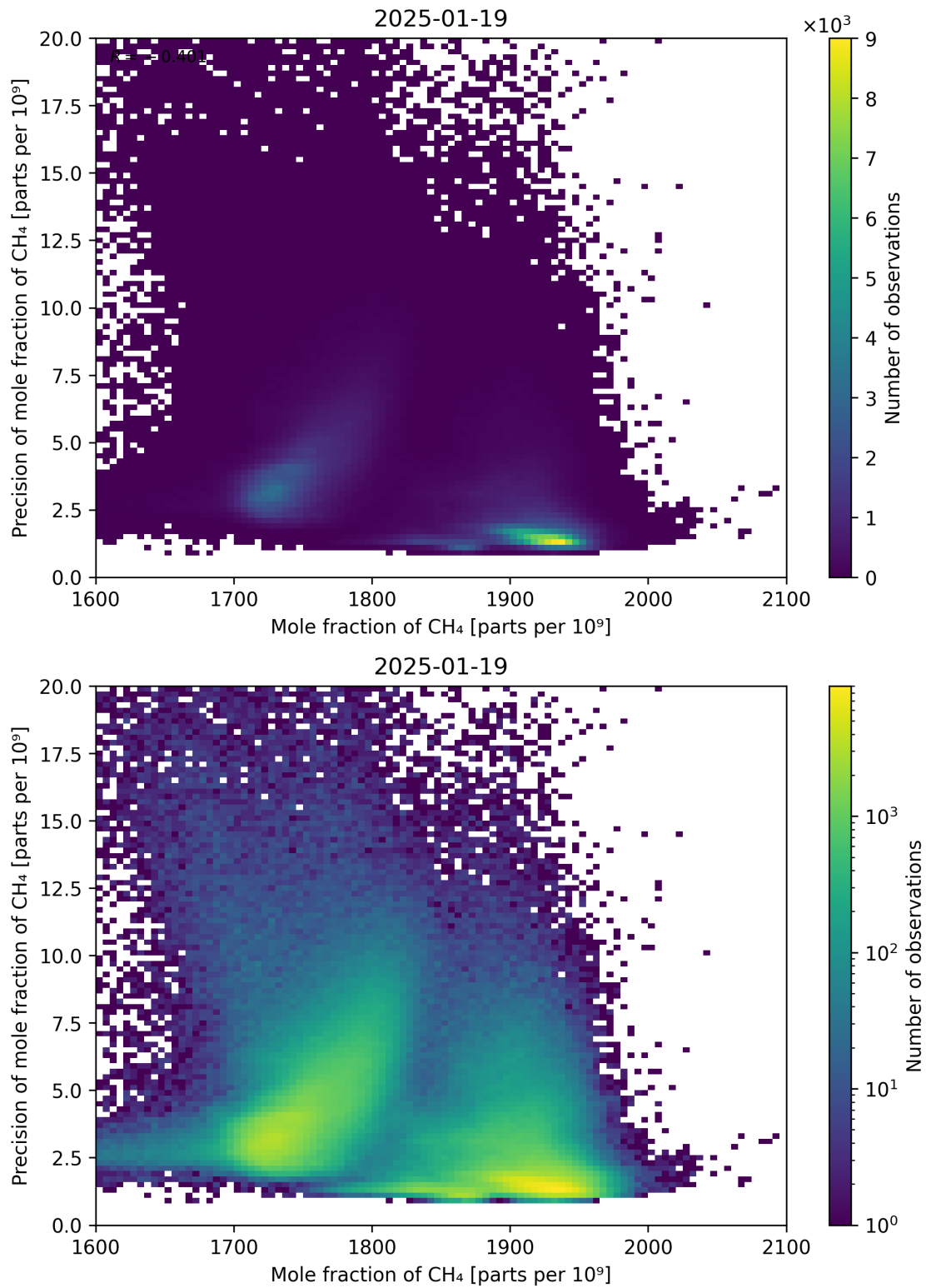
Figure 75: Scatter density plot of “Mole fraction of CH 4 ” against “Precision of mole fraction of CH 4 ” for 2025-01-18 to 2025-01-20.
