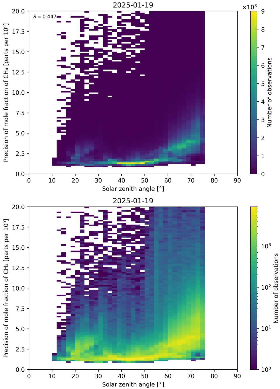
Figure 101: Scatter density plot of “Solar zenith angle” against “Precision of mole fraction of CH 4 ” for 2025-01-18 to 2025-01-20.
