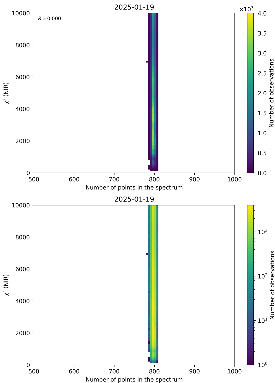
Figure 88: Scatter density plot of “Number of points in the spectrum” against “ \chi^2 (NIR)” for 2025-01-18 to 2025-01-20.
