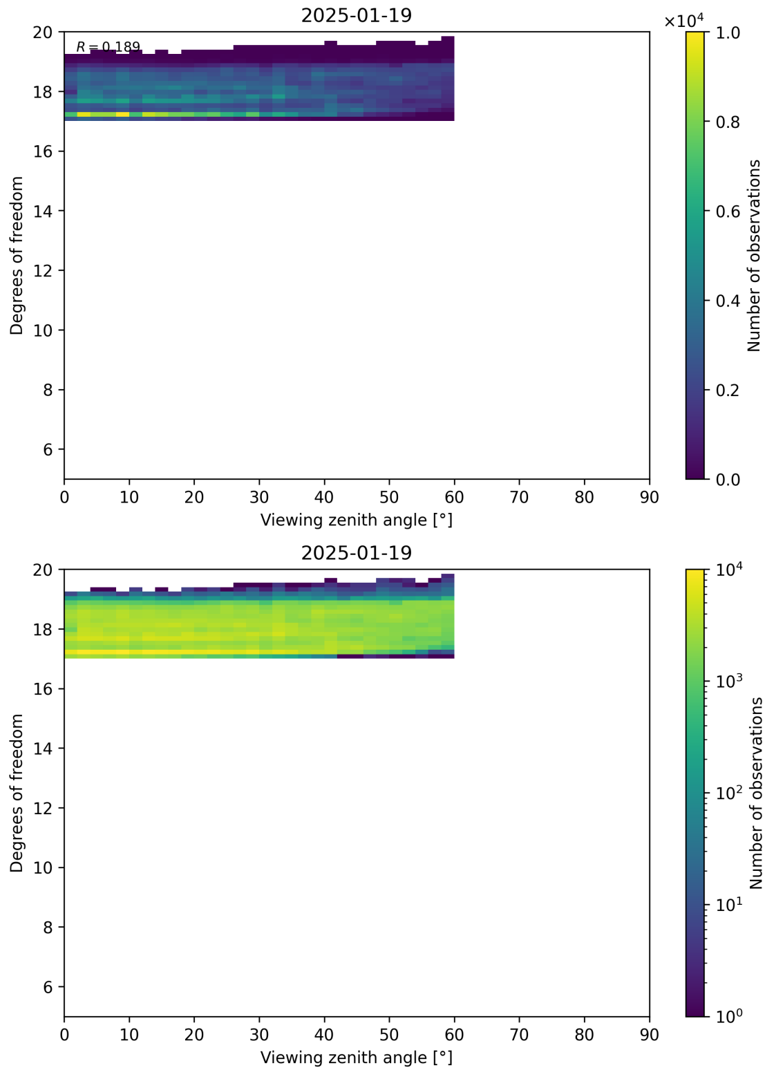
Figure 107: Scatter density plot of “Viewing zenith angle” against “Degrees of freedom” for 2025-01-18 to 2025-01-20.
