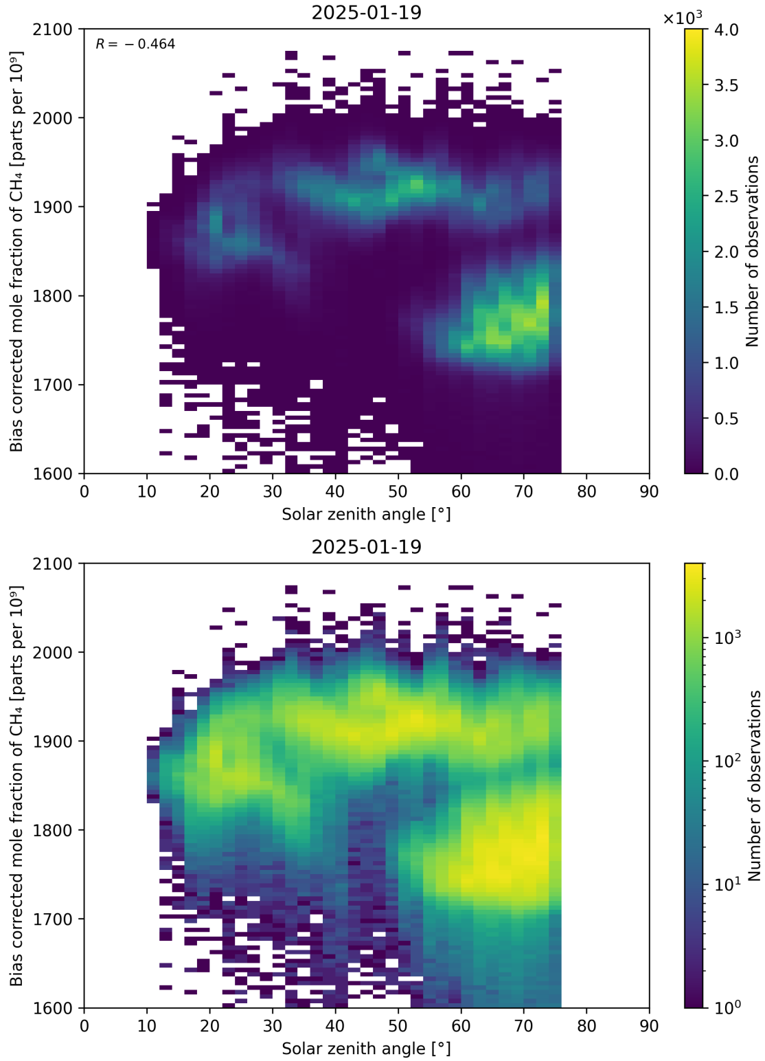
Figure 100: Scatter density plot of “Solar zenith angle” against “Bias corrected mole fraction of CH 4 ” for 2025-01-18 to 2025-01-20.
