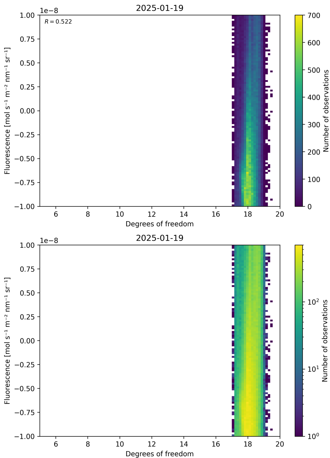
Figure 51: Scatter density plot of “Degrees of freedom” against “Fluorescence” for 2025-01-18 to 2025-01-20.
