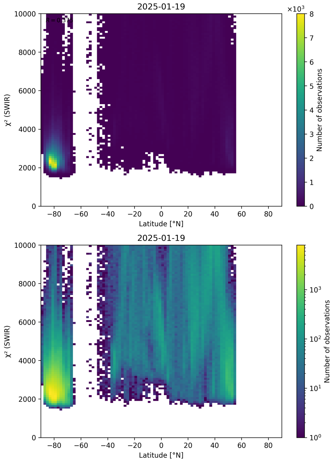
Figure 54: Scatter density plot of “Latitude” against “ \chi^2 (SWIR)” for 2025-01-18 to 2025-01-20.
