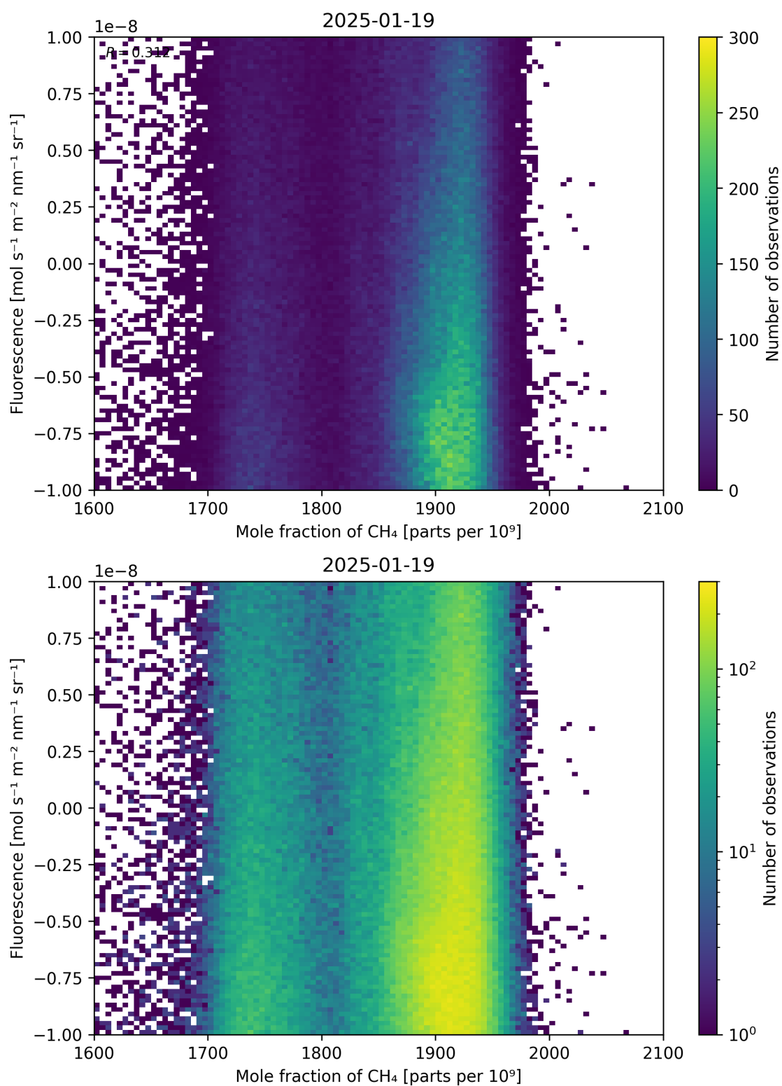
Figure 73: Scatter density plot of “Mole fraction of CH 4 ” against “Fluorescence” for 2025-01-18 to 2025-01-20.
