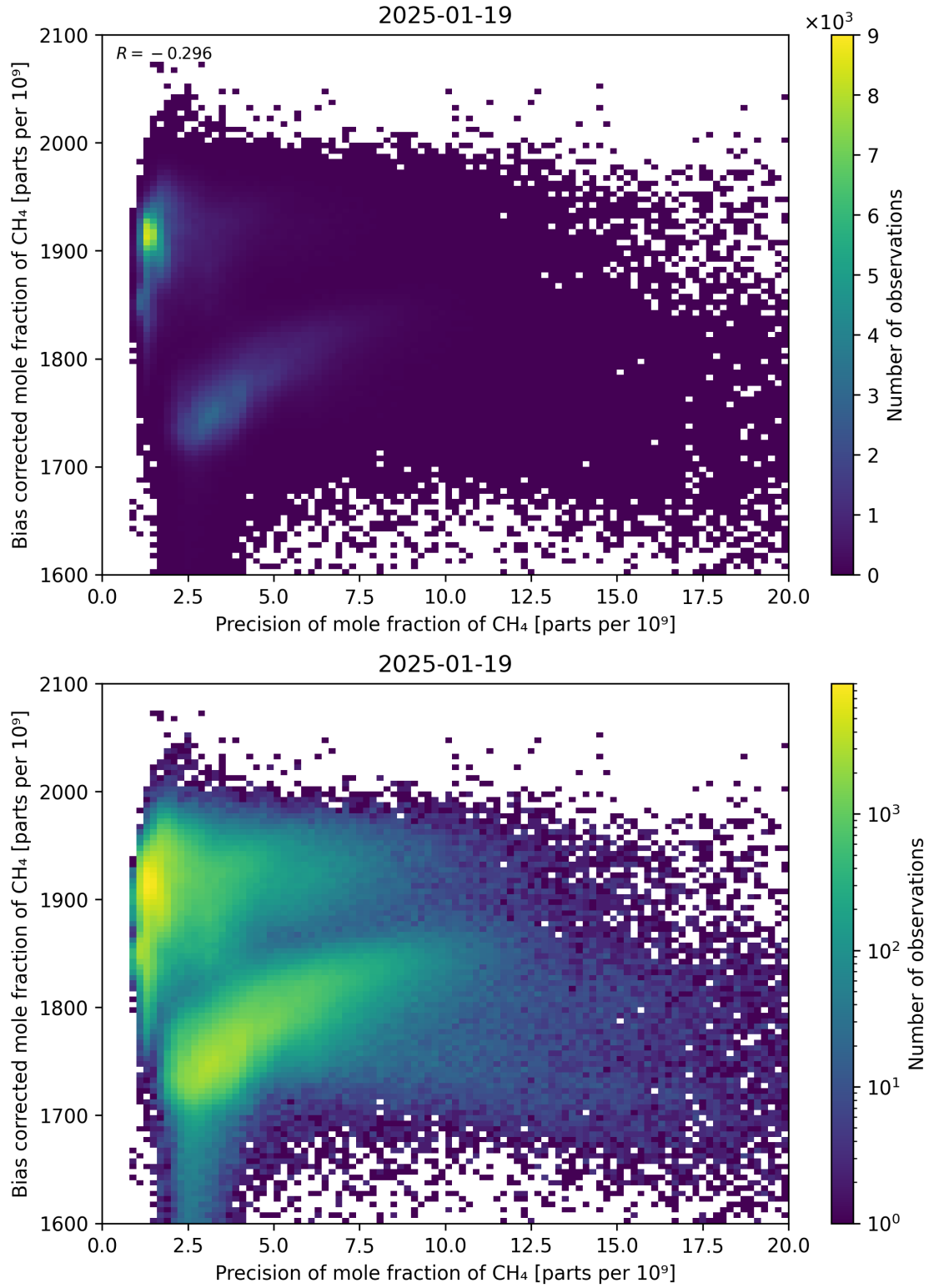
Figure 82: Scatter density plot of “Precision of mole fraction of CH 4 ” against “Bias corrected mole fraction of CH 4 ” for 2025-01-18 to 2025-01-20.
