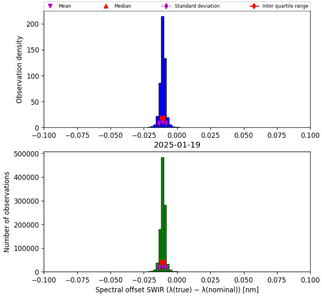
Figure 27: Histogram of “Spectral offset SWIR ( \lambda_{\text{true}} - \lambda_{\text{nominal}} )” for 2025-01-18 to 2025-01-20
