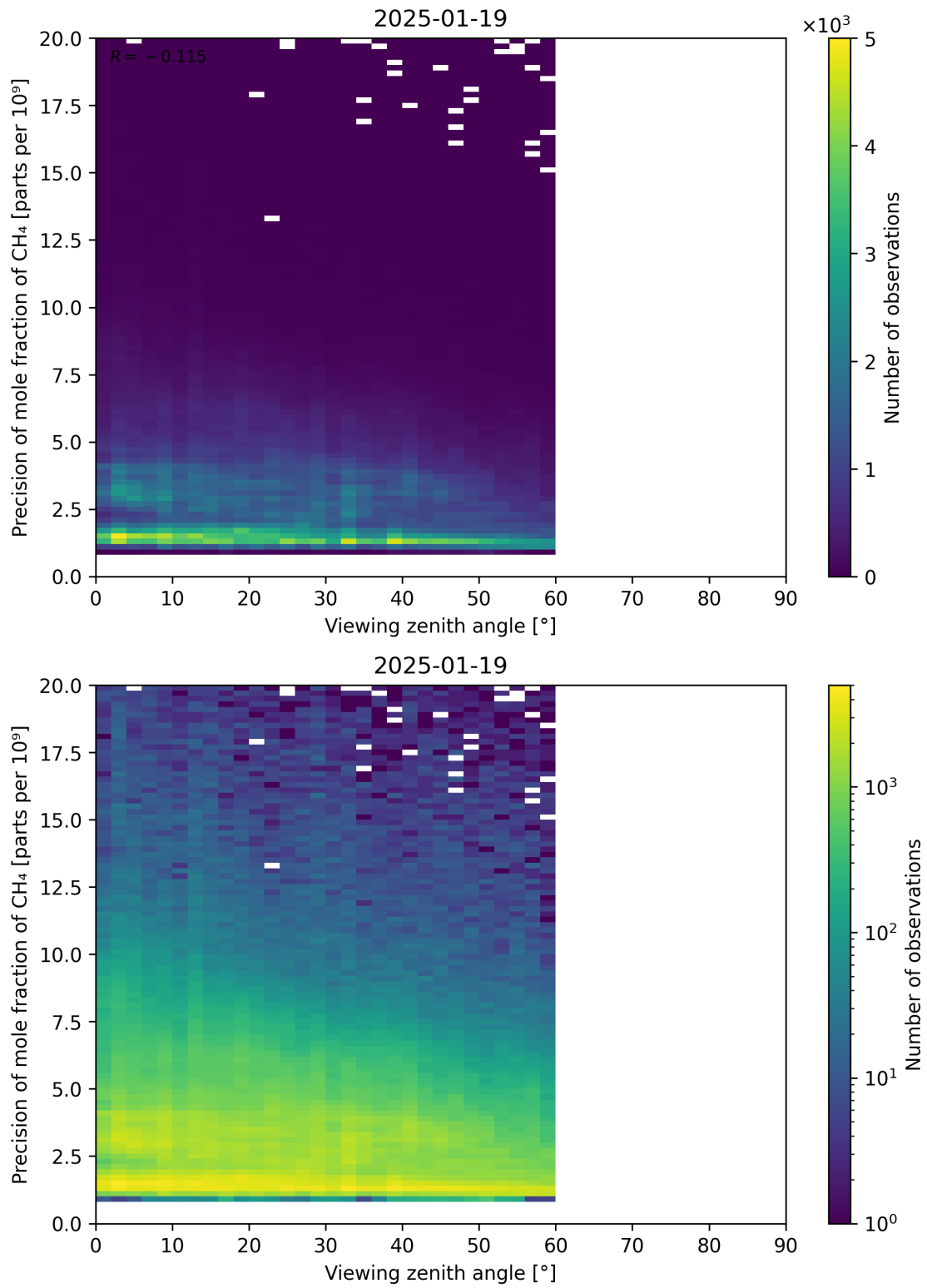
Figure 112: Scatter density plot of “Viewing zenith angle” against “Precision of mole fraction of CH 4 ” for 2025-01-18 to 2025-01-20.
