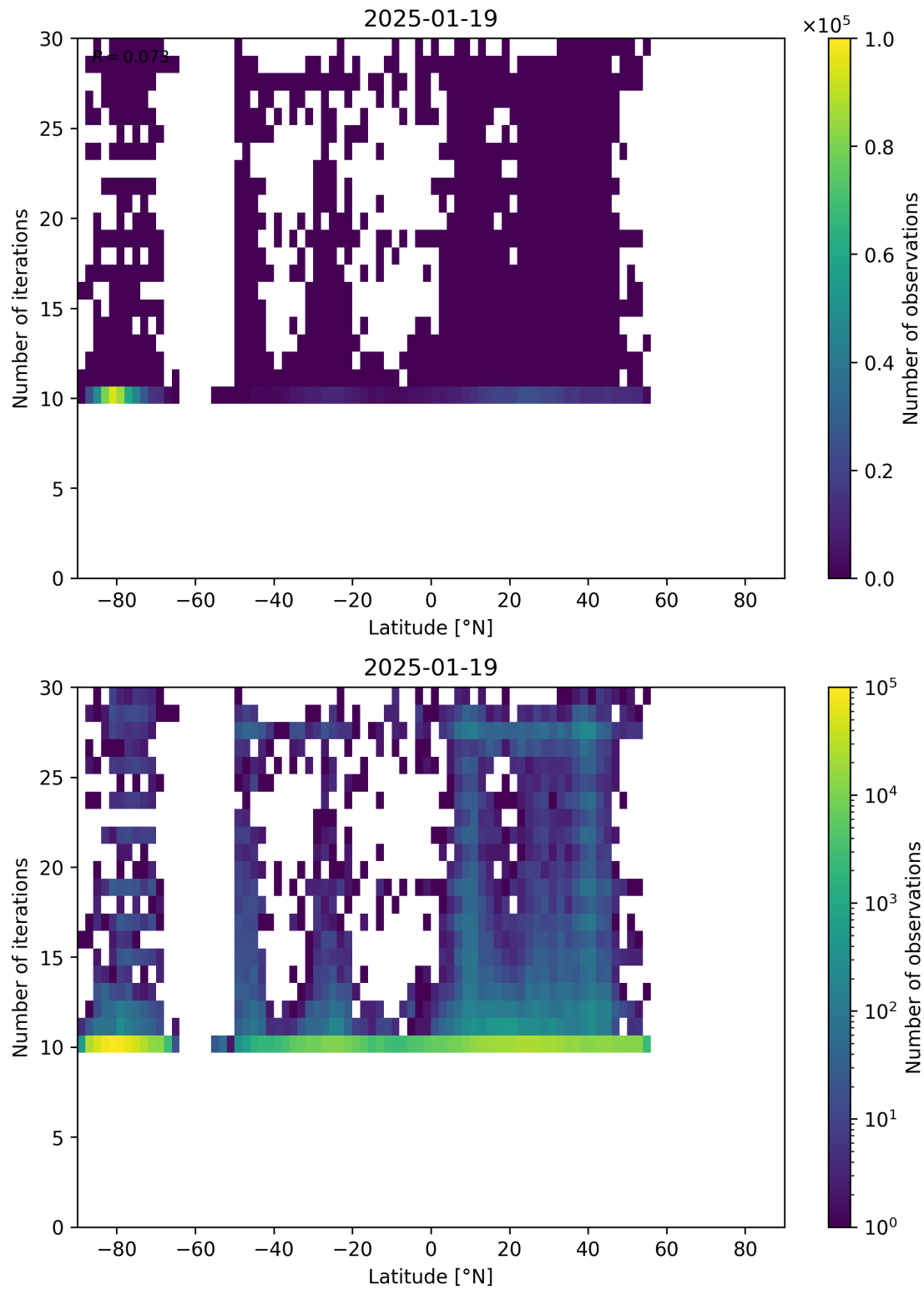
Figure 60: Scatter density plot of “Latitude” against “Number of iterations” for 2025-01-18 to 2025-01-20.
