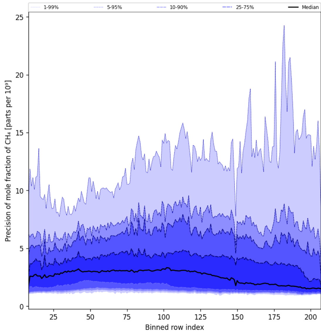
Figure 35: Along track statistics of “Precision of mole fraction of CH 4 ” for 2025-01-18 to 2025-01-20
