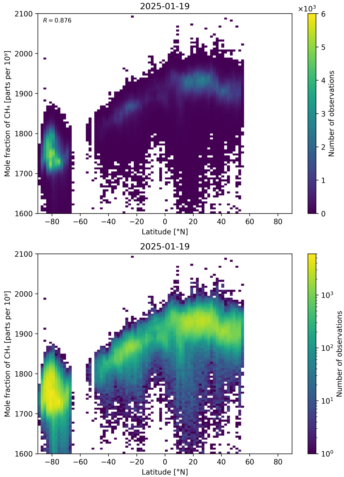
Figure 57: Scatter density plot of “Latitude” against “Mole fraction of CH 4 ” for 2025-01-18 to 2025-01-20.
