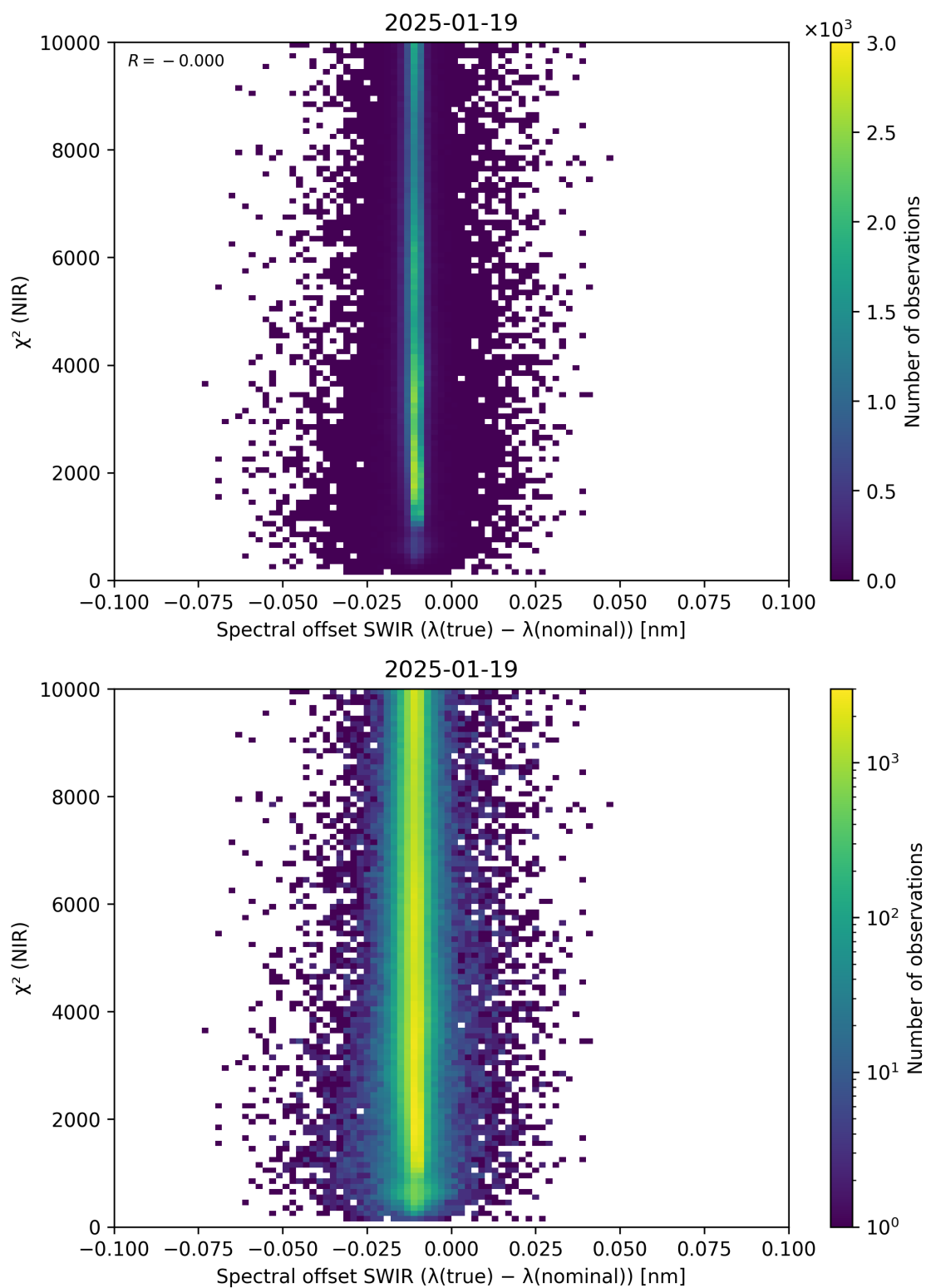
Figure 117: Scatter density plot of “Spectral offset SWIR ( \lambda_{\text{true}} - \lambda_{\text{nominal}} )” against “ \chi^2 (NIR)” for 2025-01-18 to 2025-01-20.
