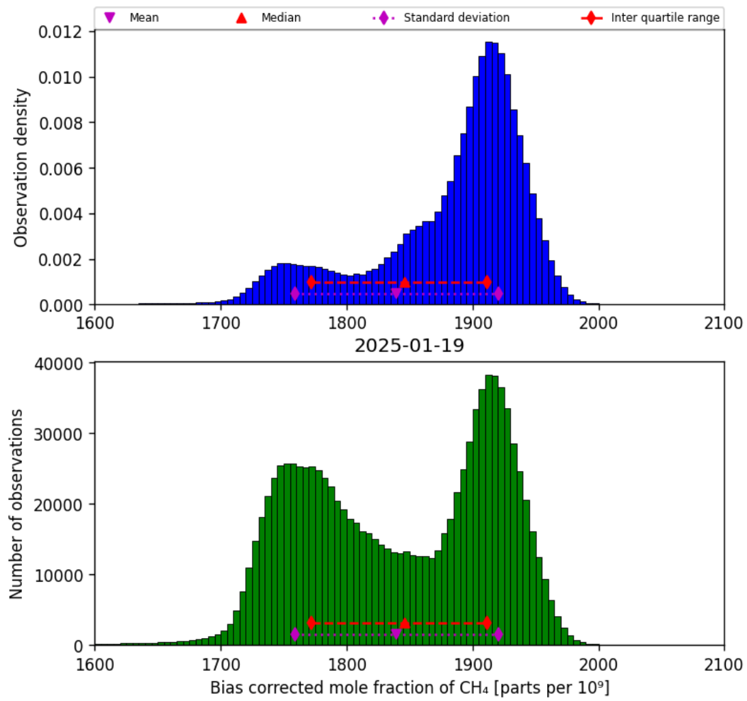
Figure 25: Histogram of “Bias corrected mole fraction of CH 4 ” for 2025-01-18 to 2025-01-20
