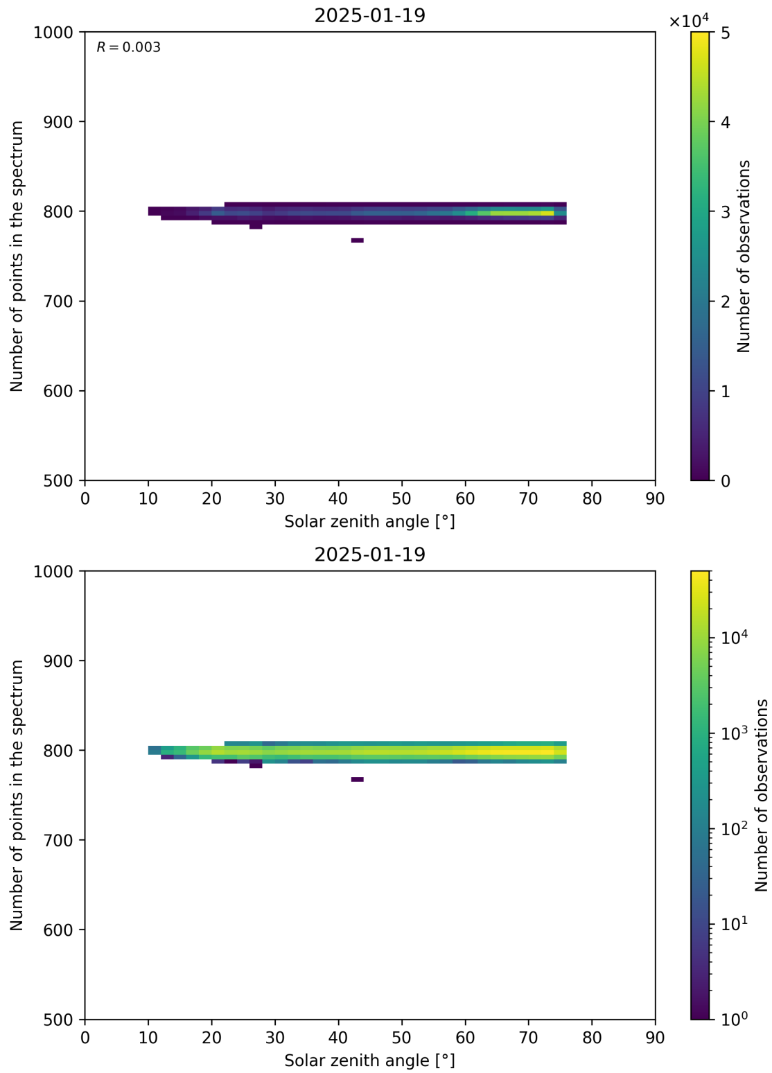
Figure 103: Scatter density plot of “Solar zenith angle” against “Number of points in the spectrum” for 2025-01-18 to 2025-01-20.
