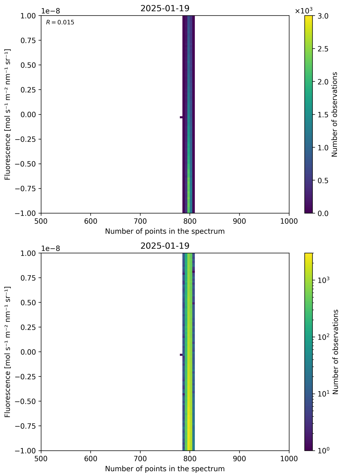
Figure 91: Scatter density plot of “Number of points in the spectrum” against “Fluorescence” for 2025-01-18 to 2025-01-20.
