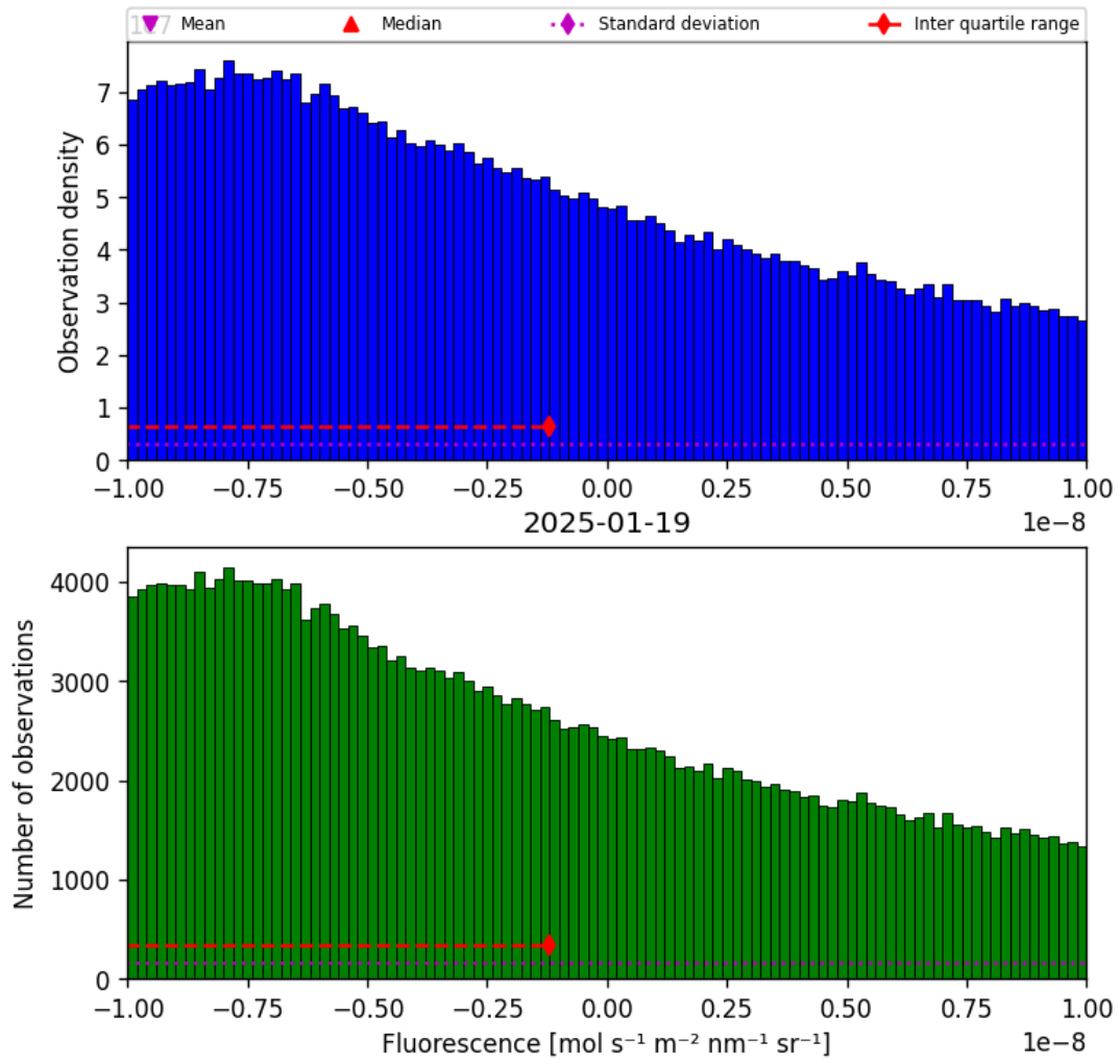
Figure 32: Histogram of “Fluorescence” for 2025-01-18 to 2025-01-20
