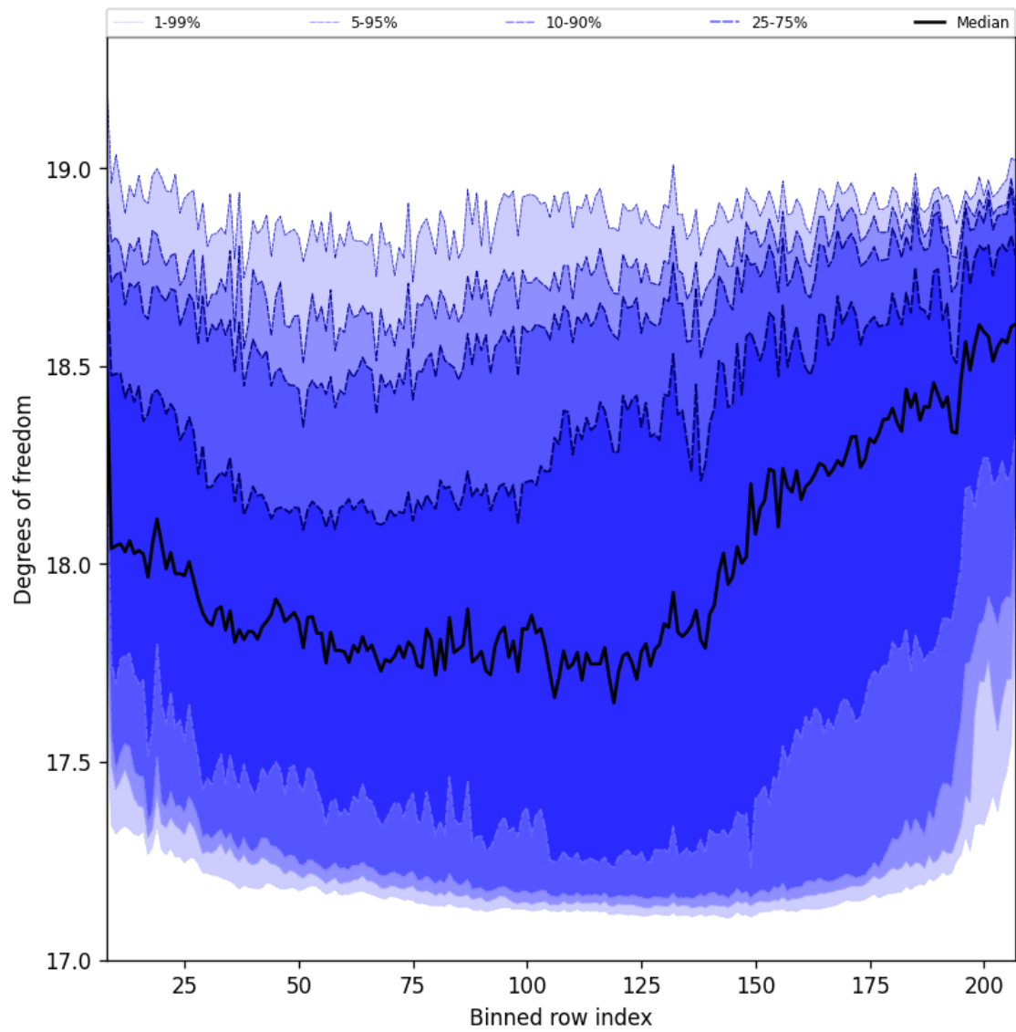
Figure 41: Along track statistics of “Degrees of freedom” for 2025-01-18 to 2025-01-20
