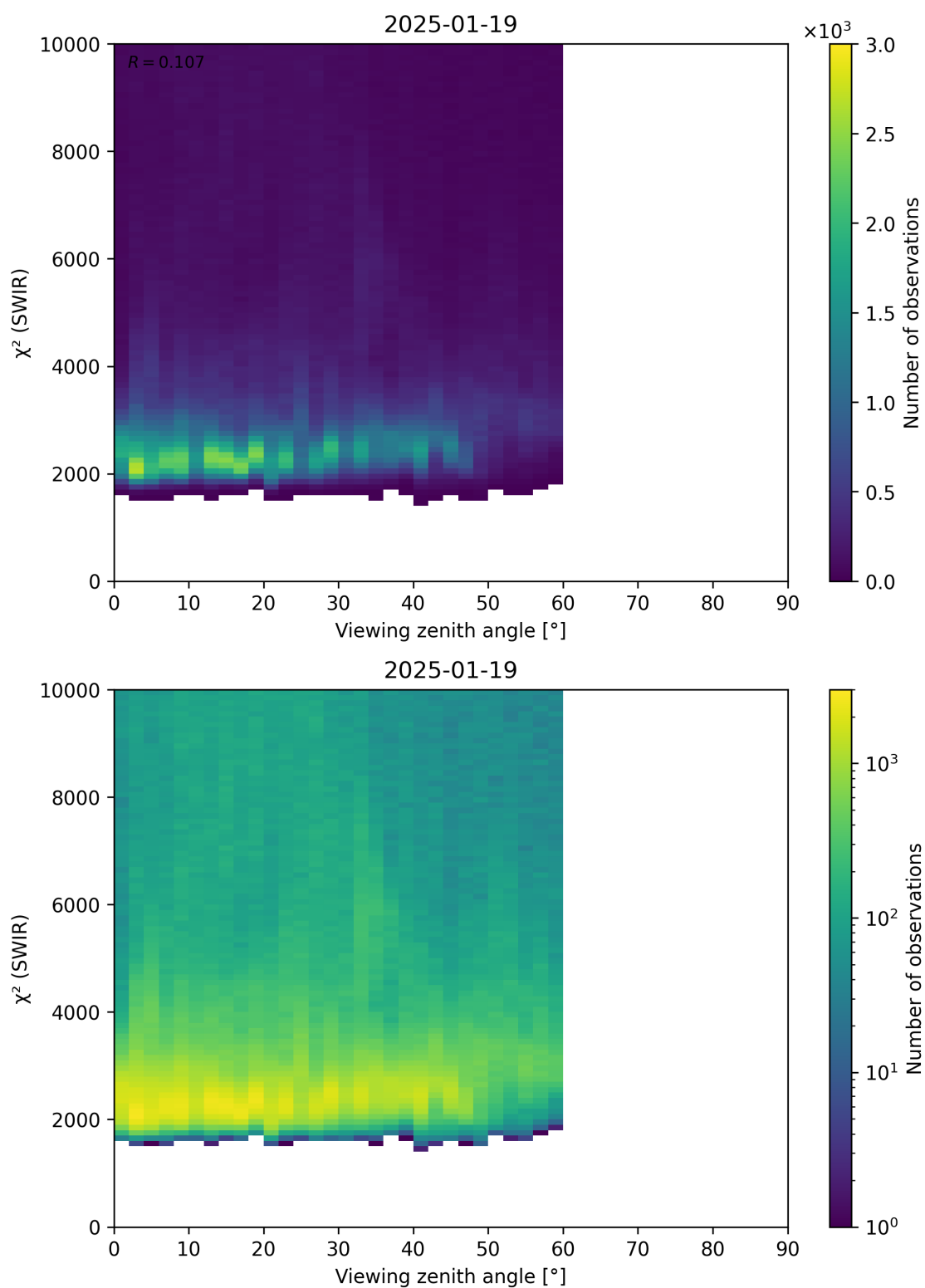
Figure 106: Scatter density plot of “Viewing zenith angle” against “ \chi^2 (SWIR)” for 2025-01-18 to 2025-01-20.
