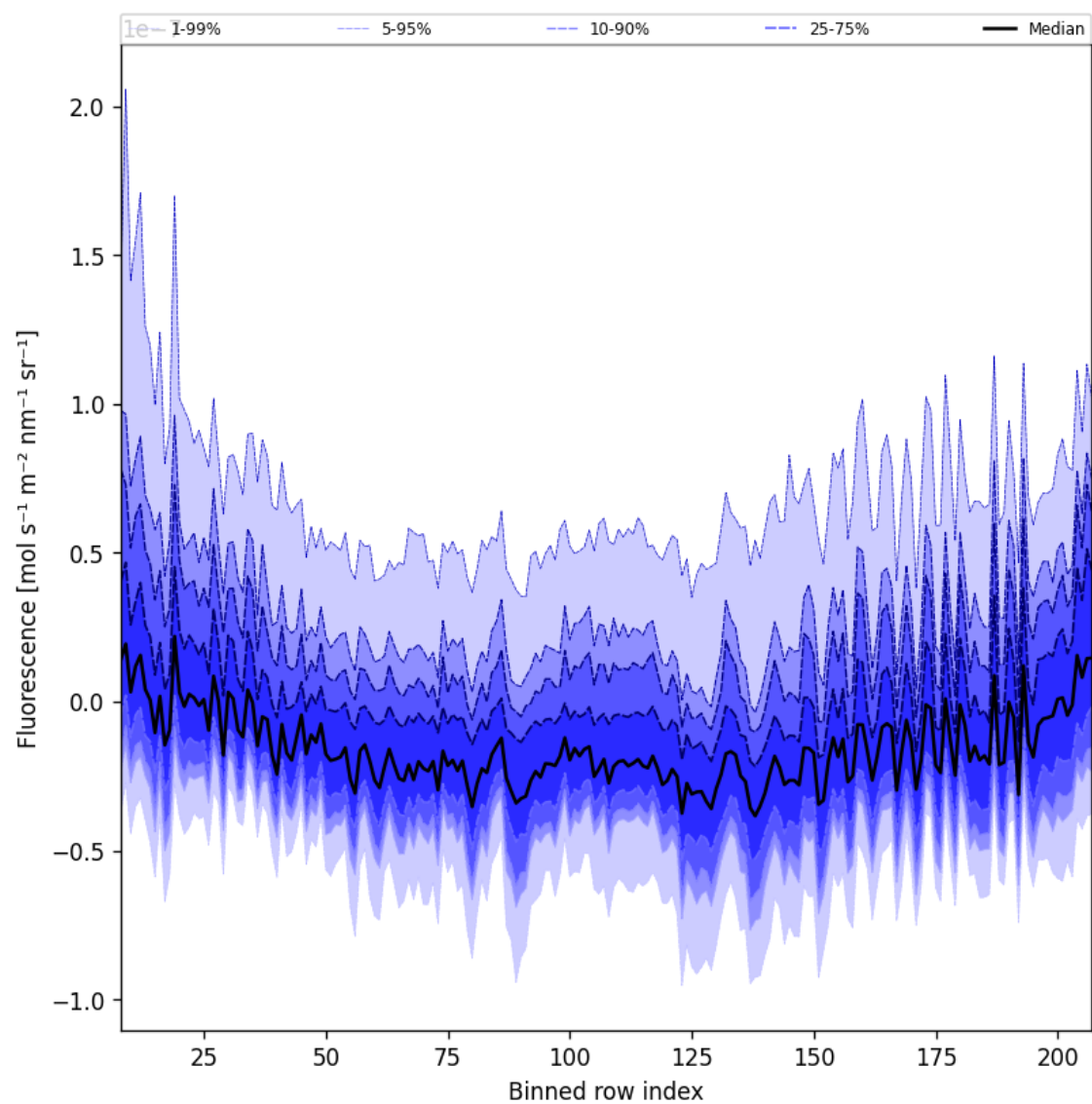
Figure 43: Along track statistics of “Fluorescence” for 2025-01-18 to 2025-01-20
