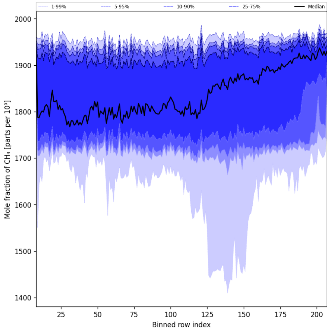
Figure 34: Along track statistics of “Mole fraction of CH 4 ” for 2025-01-18 to 2025-01-20
