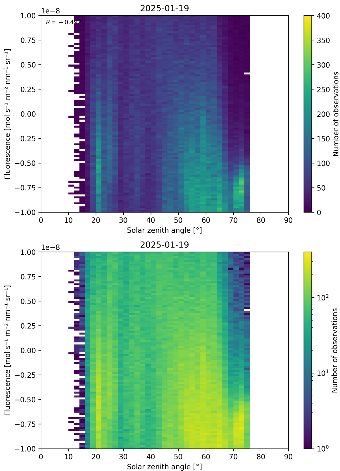
Figure 97: Scatter density plot of “Solar zenith angle” against “Fluorescence” for 2025-01-18 to 2025-01-20.
