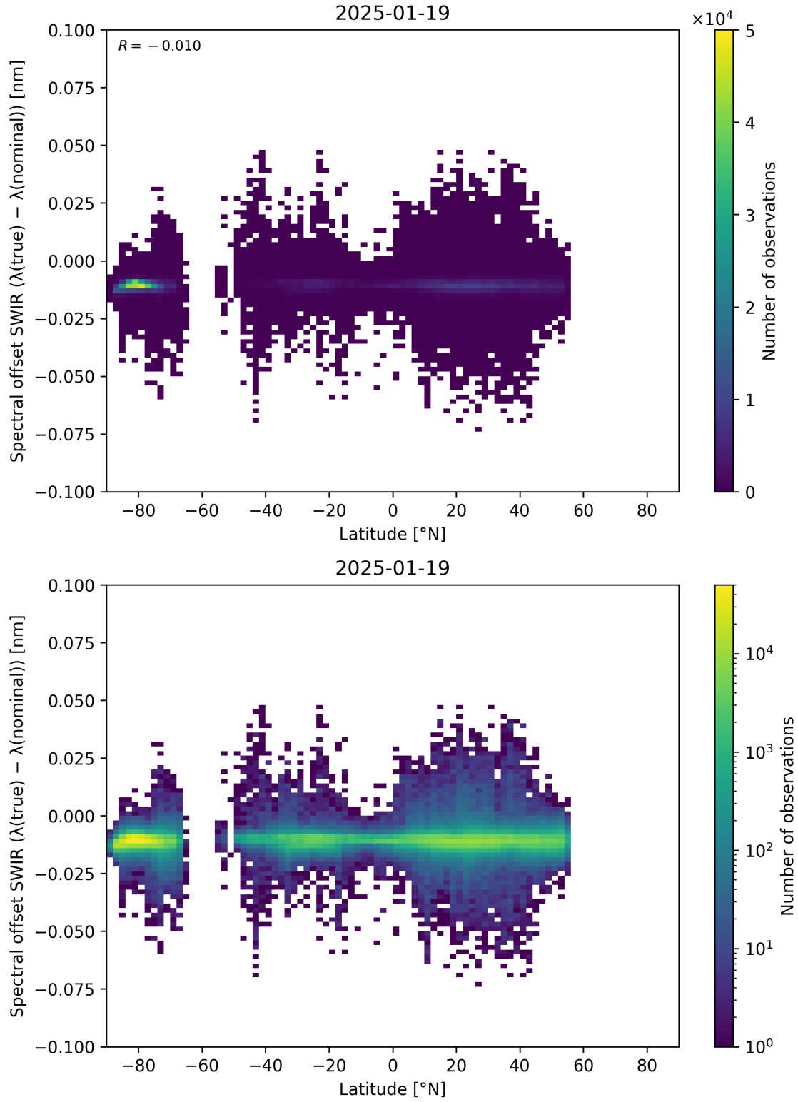
Figure 62: Scatter density plot of “Latitude” against “Spectral offset SWIR ( \lambda_{\text{true}} - \lambda_{\text{nominal}} )” for 2025-01-18 to 2025-01-20.
