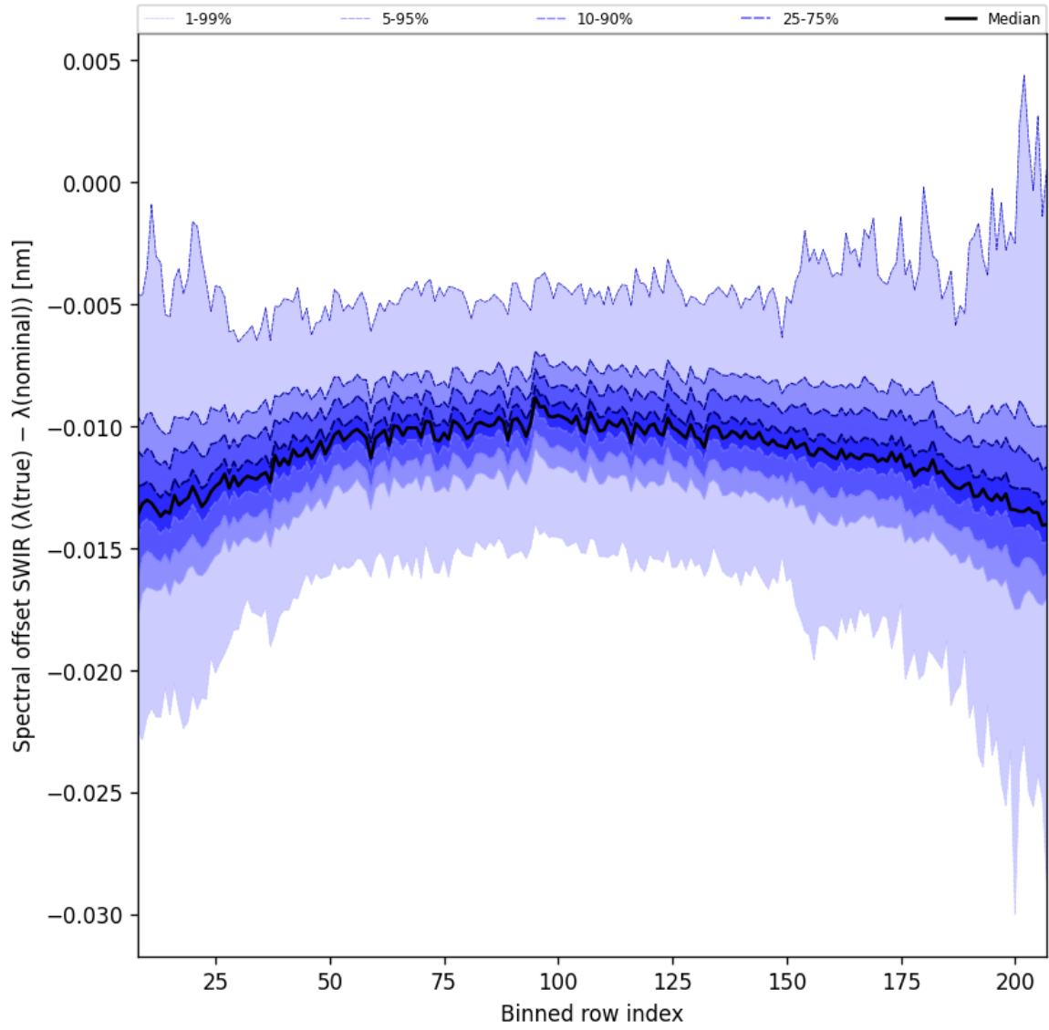
Figure 38: Along track statistics of “Spectral offset SWIR ( \lambda_{\text{true}} - \lambda_{\text{nominal}} )” for 2025-01-18 to 2025-01-20
