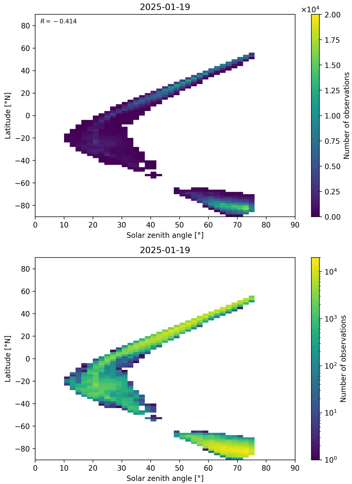
Figure 98: Scatter density plot of “Solar zenith angle” against “Latitude” for 2025-01-18 to 2025-01-20.
