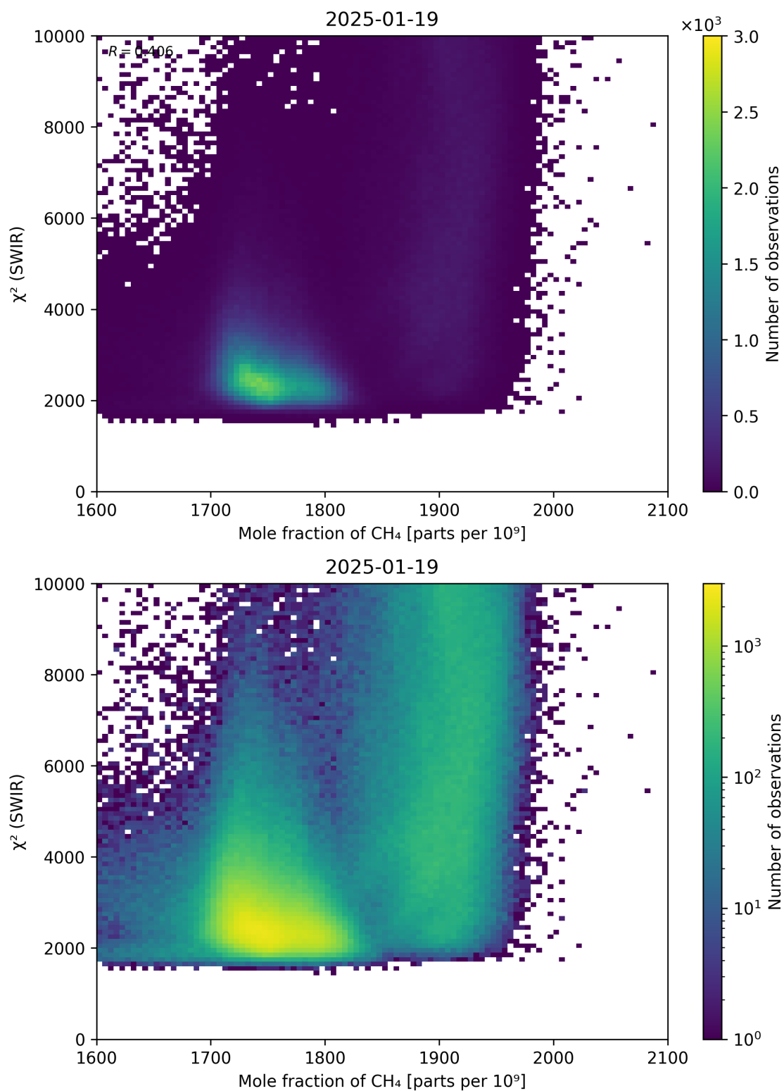
Figure 71: Scatter density plot of “Mole fraction of CH 4 ” against “ \chi^2 (SWIR)” for 2025-01-18 to 2025-01-20.
