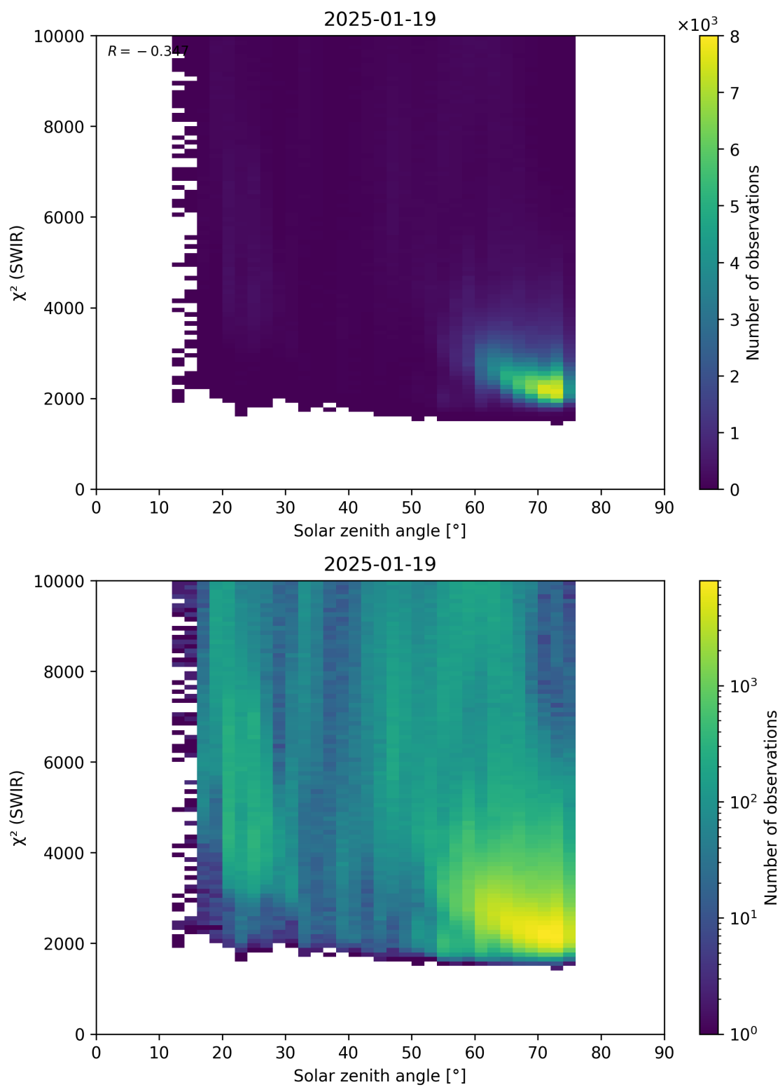
Figure 95: Scatter density plot of “Solar zenith angle” against “ \chi^2 (SWIR)” for 2025-01-18 to 2025-01-20.
