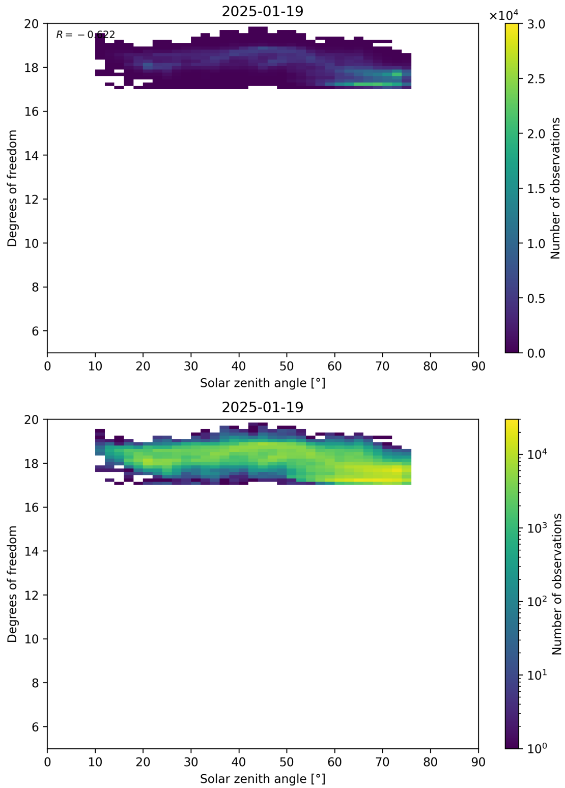
Figure 96: Scatter density plot of “Solar zenith angle” against “Degrees of freedom” for 2025-01-18 to 2025-01-20.
