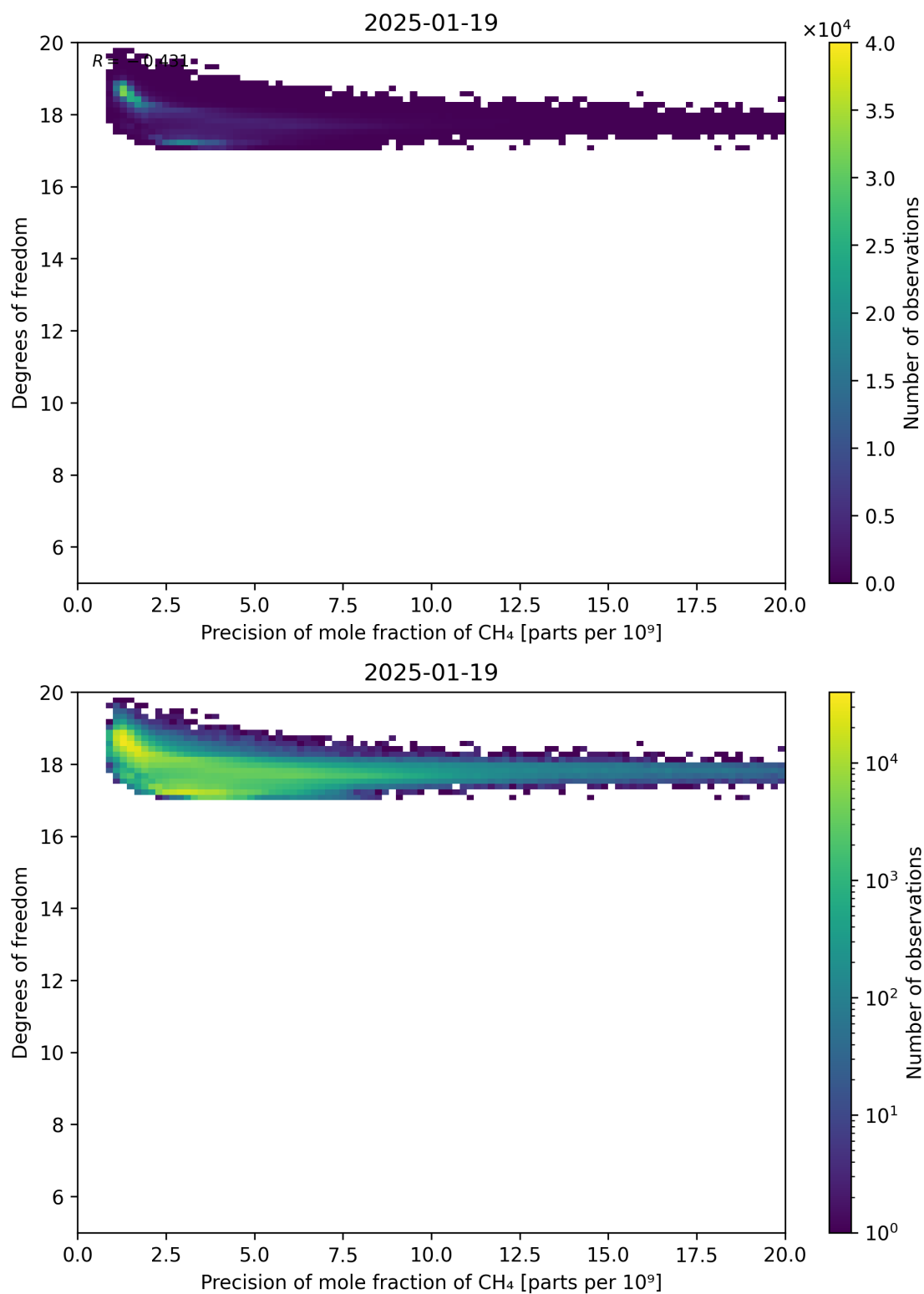
Figure 80: Scatter density plot of “Precision of mole fraction of CH 4 ” against “Degrees of freedom” for 2025-01-18 to 2025-01-20.
