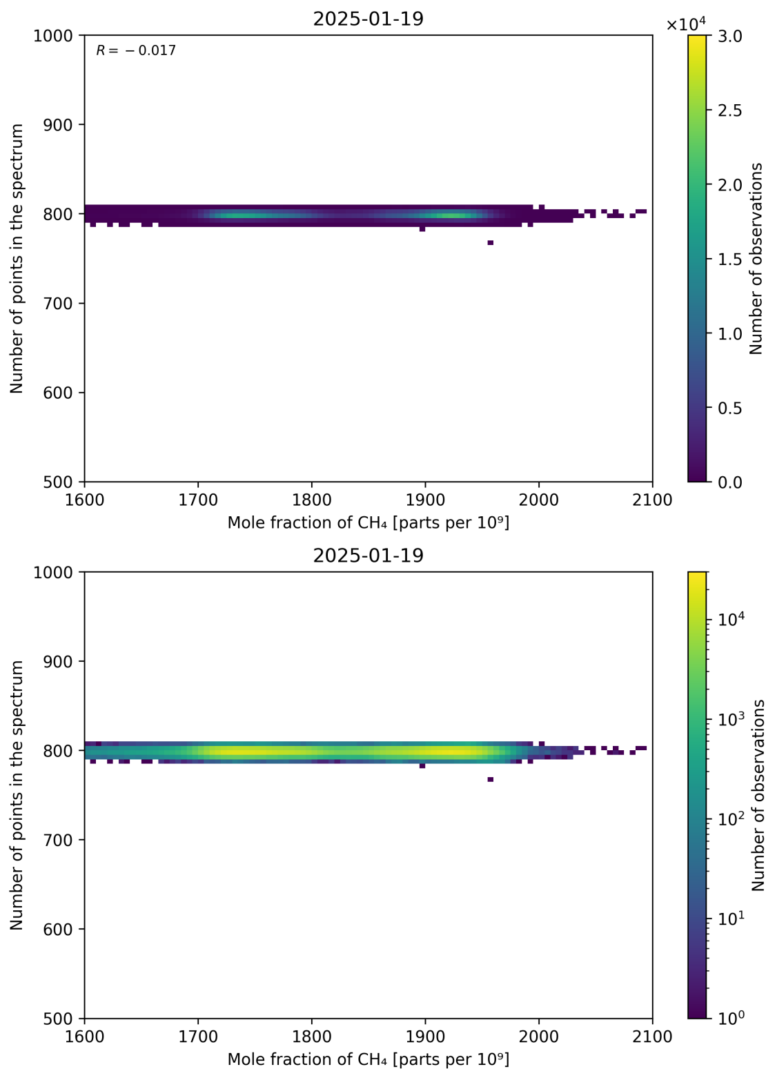
Figure 77: Scatter density plot of “Mole fraction of CH 4 ” against “Number of points in the spectrum” for 2025-01-18 to 2025-01-20.
