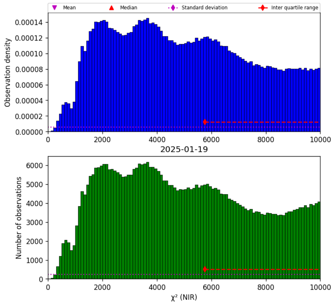
Figure 29: Histogram of " \chi^2 (NIR)" for 2025-01-18 to 2025-01-20
