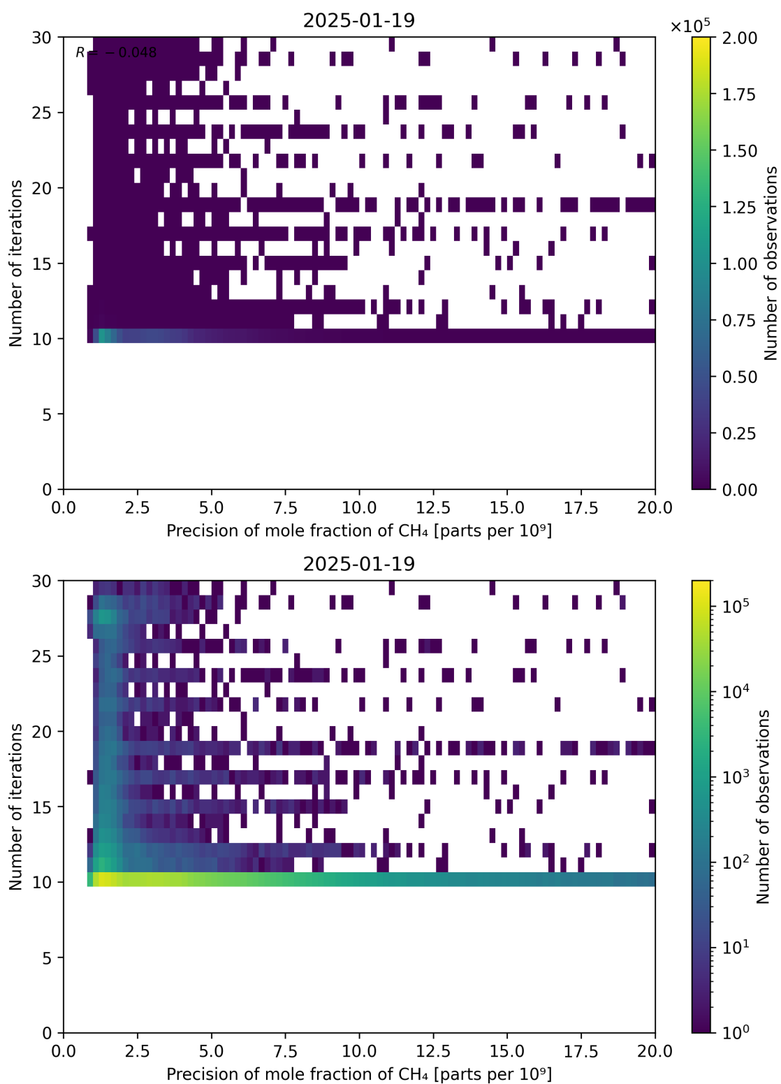
Figure 83: Scatter density plot of “Precision of mole fraction of CH 4 ” against “Number of iterations” for 2025-01-18 to 2025-01-20.
