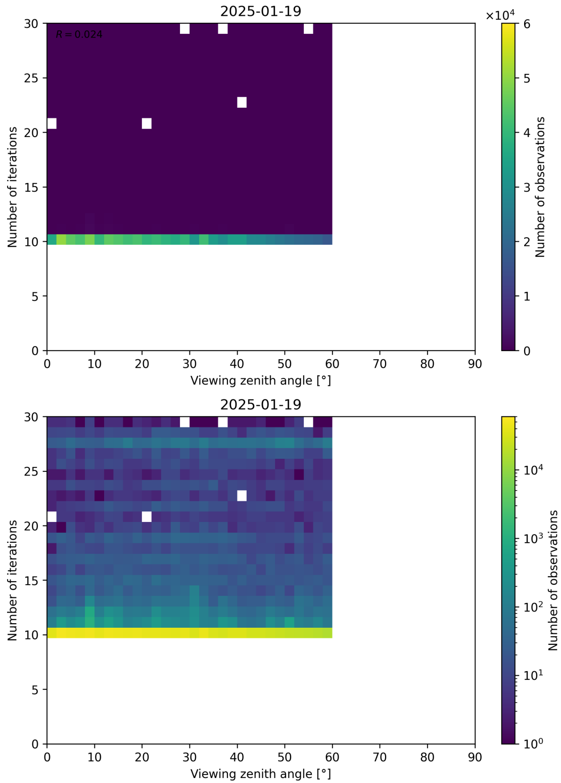
Figure 113: Scatter density plot of “Viewing zenith angle” against “Number of iterations” for 2025-01-18 to 2025-01-20.
