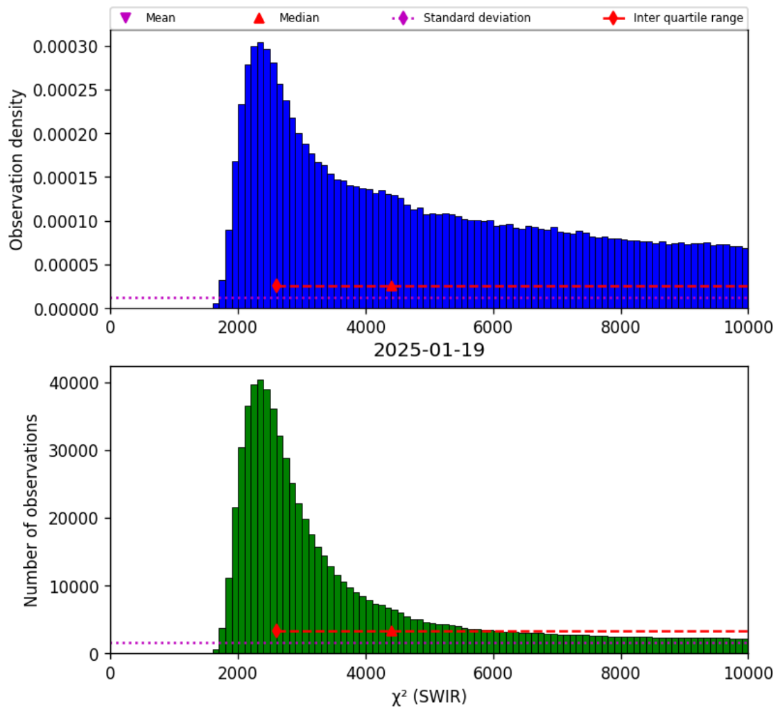
Figure 28: Histogram of “ \chi^2 (SWIR)” for 2025-01-18 to 2025-01-20
