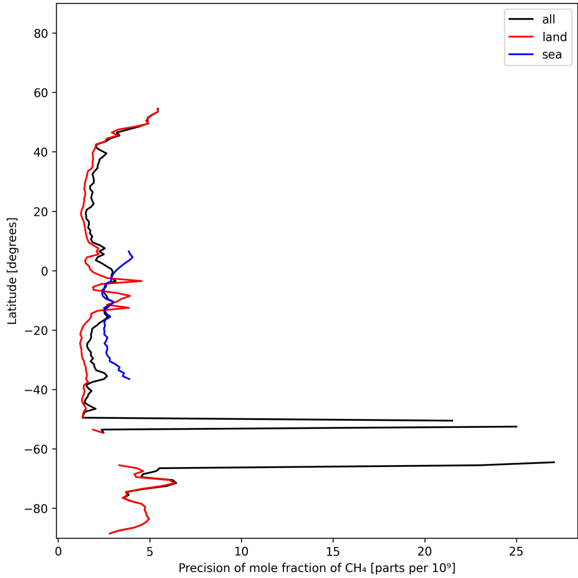
Figure 13: Zonal average of “Precision of mole fraction of CH 4 ” for 2025-01-18 to 2025-01-20.
