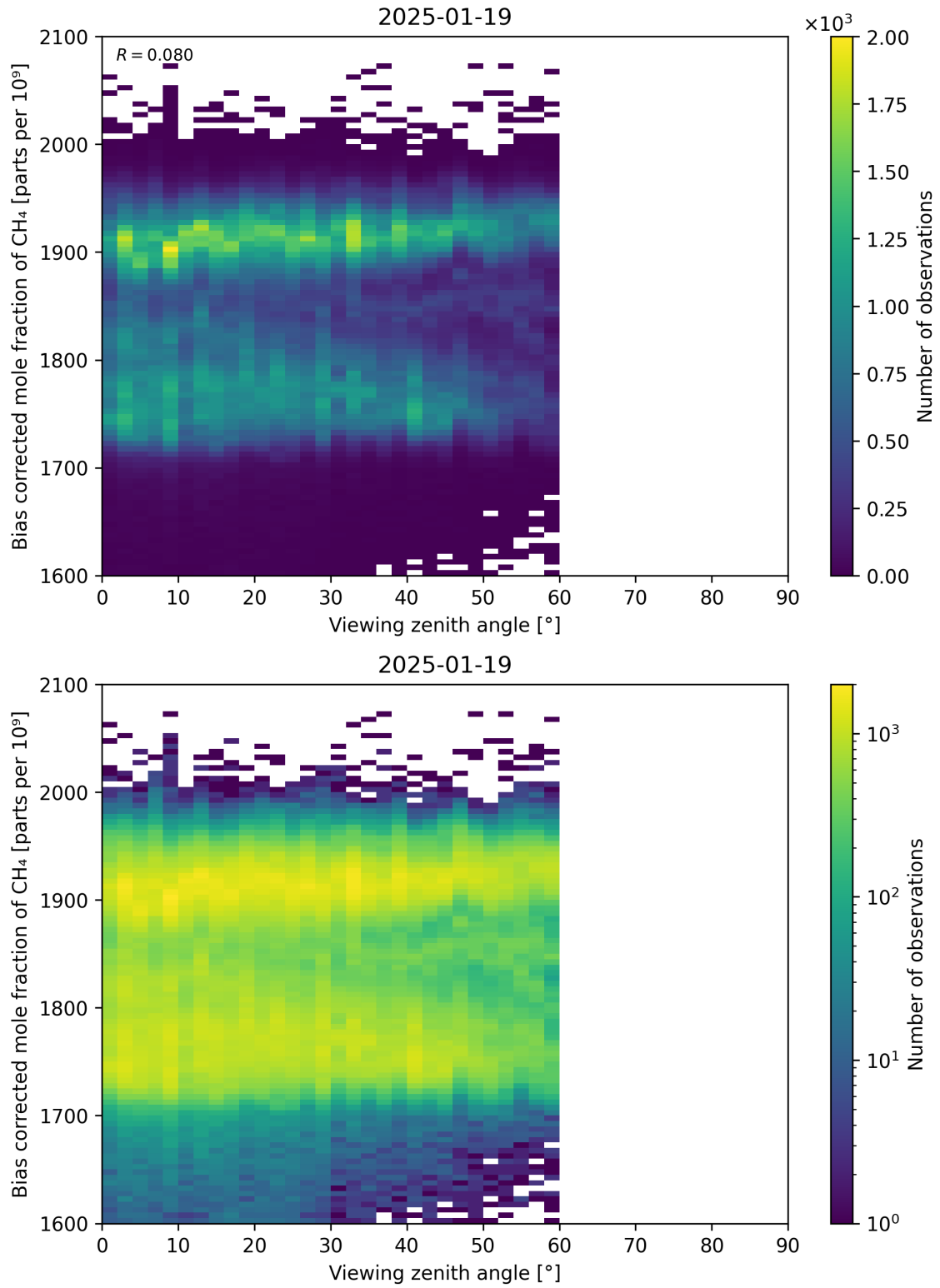
Figure 111: Scatter density plot of “Viewing zenith angle” against “Bias corrected mole fraction of CH 4 ” for 2025-01-18 to 2025-01-20.
