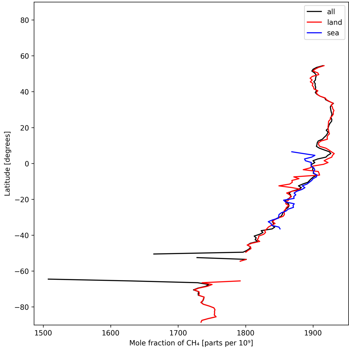
Figure 12: Zonal average of “Mole fraction of \text{CH}_4 ” for 2025-01-18 to 2025-01-20.
