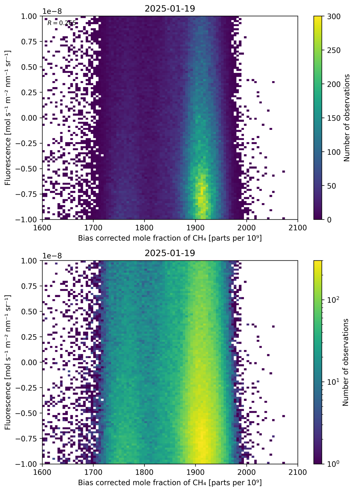
Figure 66: Scatter density plot of “Bias corrected mole fraction of \text{CH}_4 ” against “Fluorescence” for 2025-01-18 to 2025-01-20.
