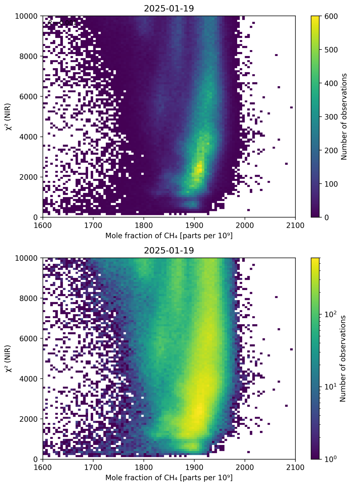
Figure 70: Scatter density plot of “Mole fraction of CH 4 ” against “ \chi^2 (NIR)” for 2025-01-18 to 2025-01-20.
