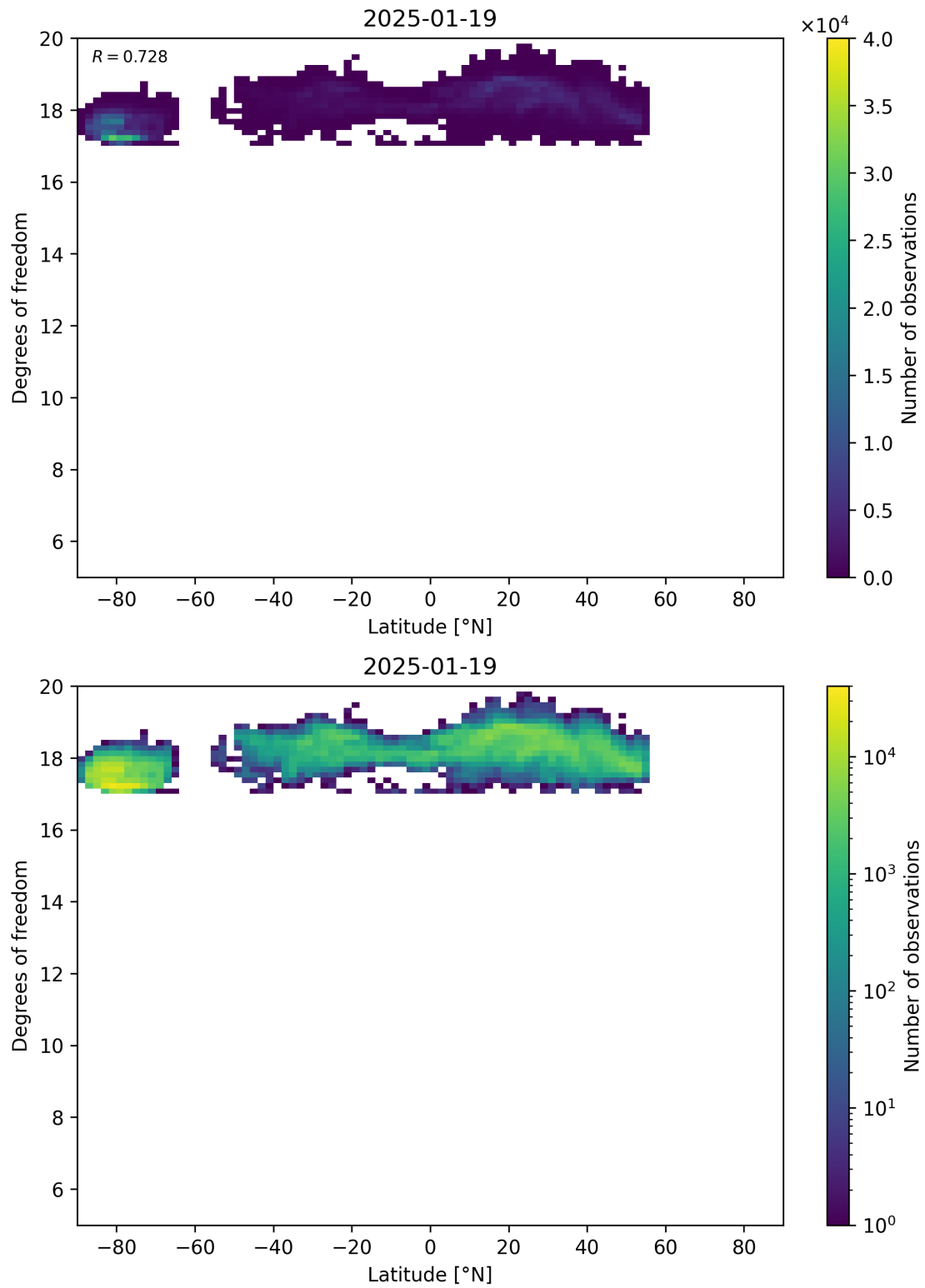
Figure 55: Scatter density plot of “Latitude” against “Degrees of freedom” for 2025-01-18 to 2025-01-20.
