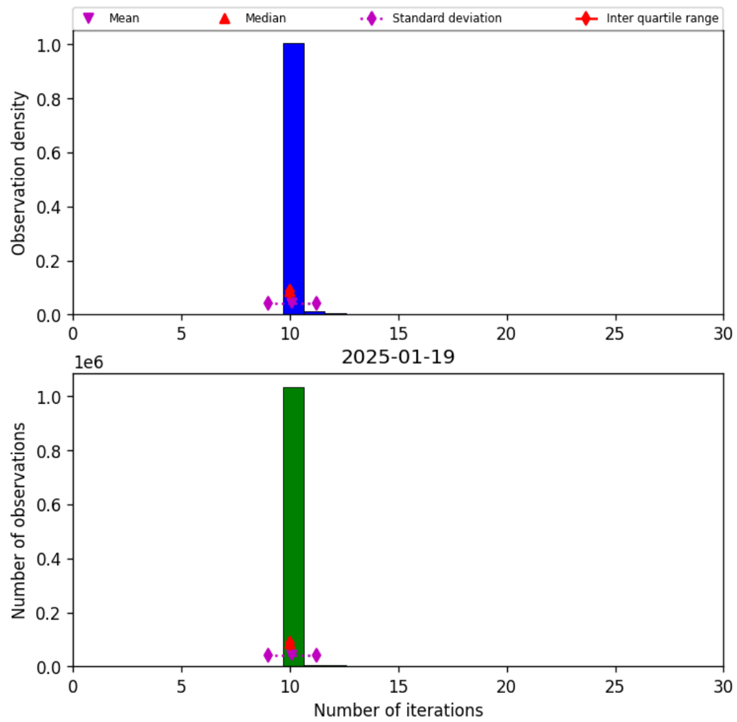
Figure 31: Histogram of "Number of iterations" for 2025-01-18 to 2025-01-20
