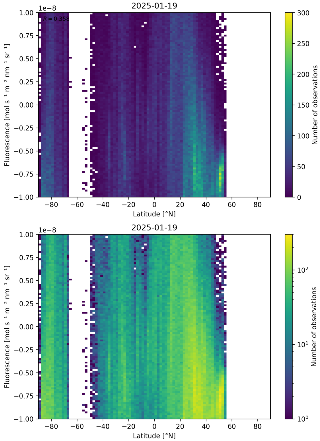
Figure 56: Scatter density plot of “Latitude” against “Fluorescence” for 2025-01-18 to 2025-01-20.
