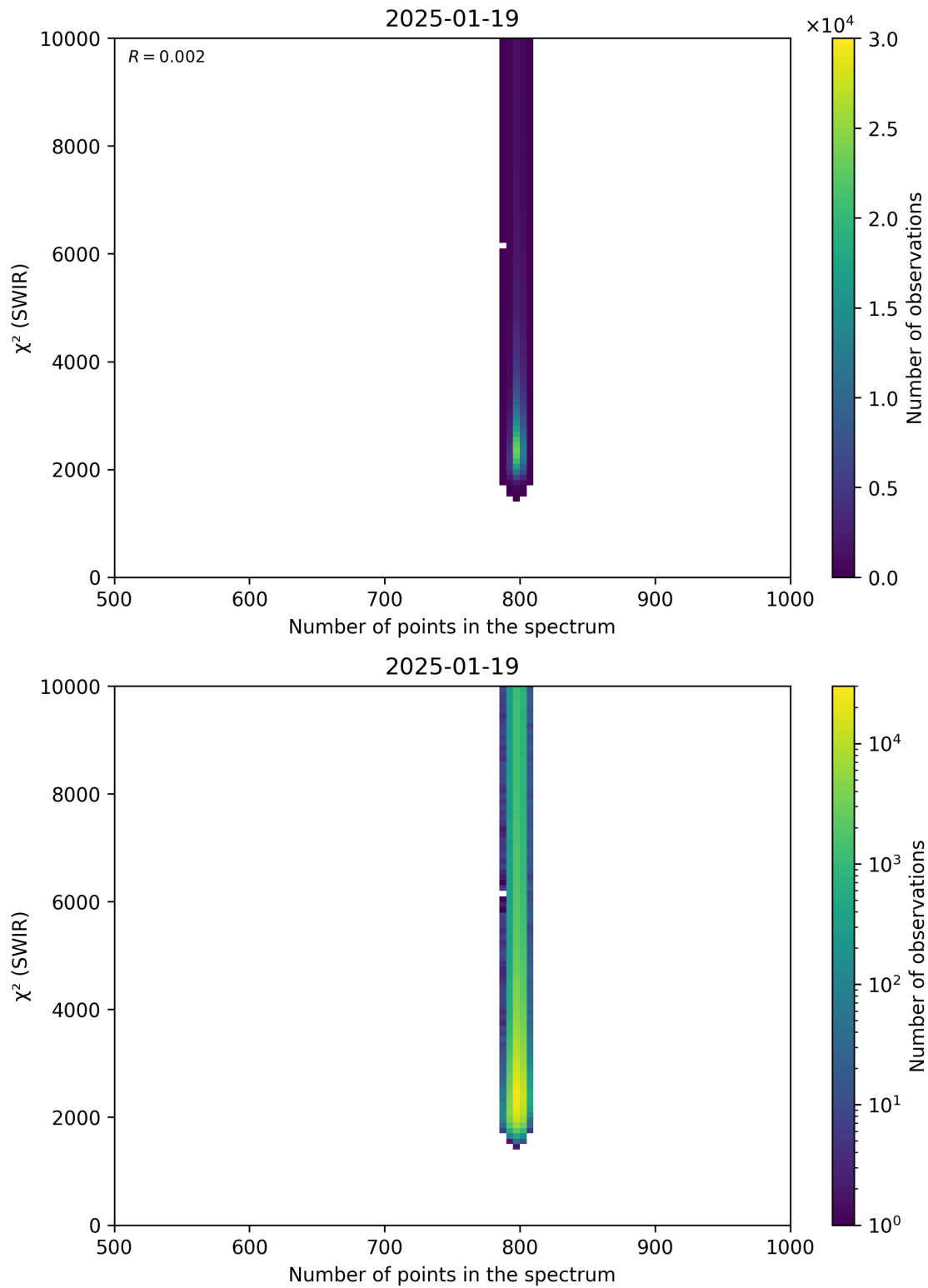
Figure 89: Scatter density plot of “Number of points in the spectrum” against “ \chi^2 (SWIR)” for 2025-01-18 to 2025-01-20.
