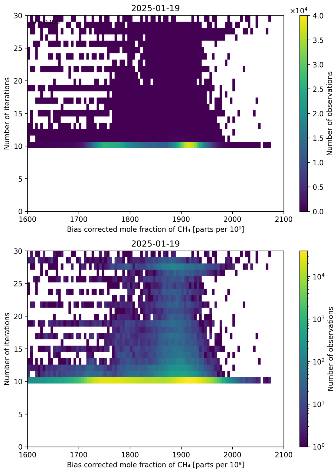
Figure 67: Scatter density plot of “Bias corrected mole fraction of \text{CH}_4 ” against “Number of iterations” for 2025-01-18 to 2025-01-20.
