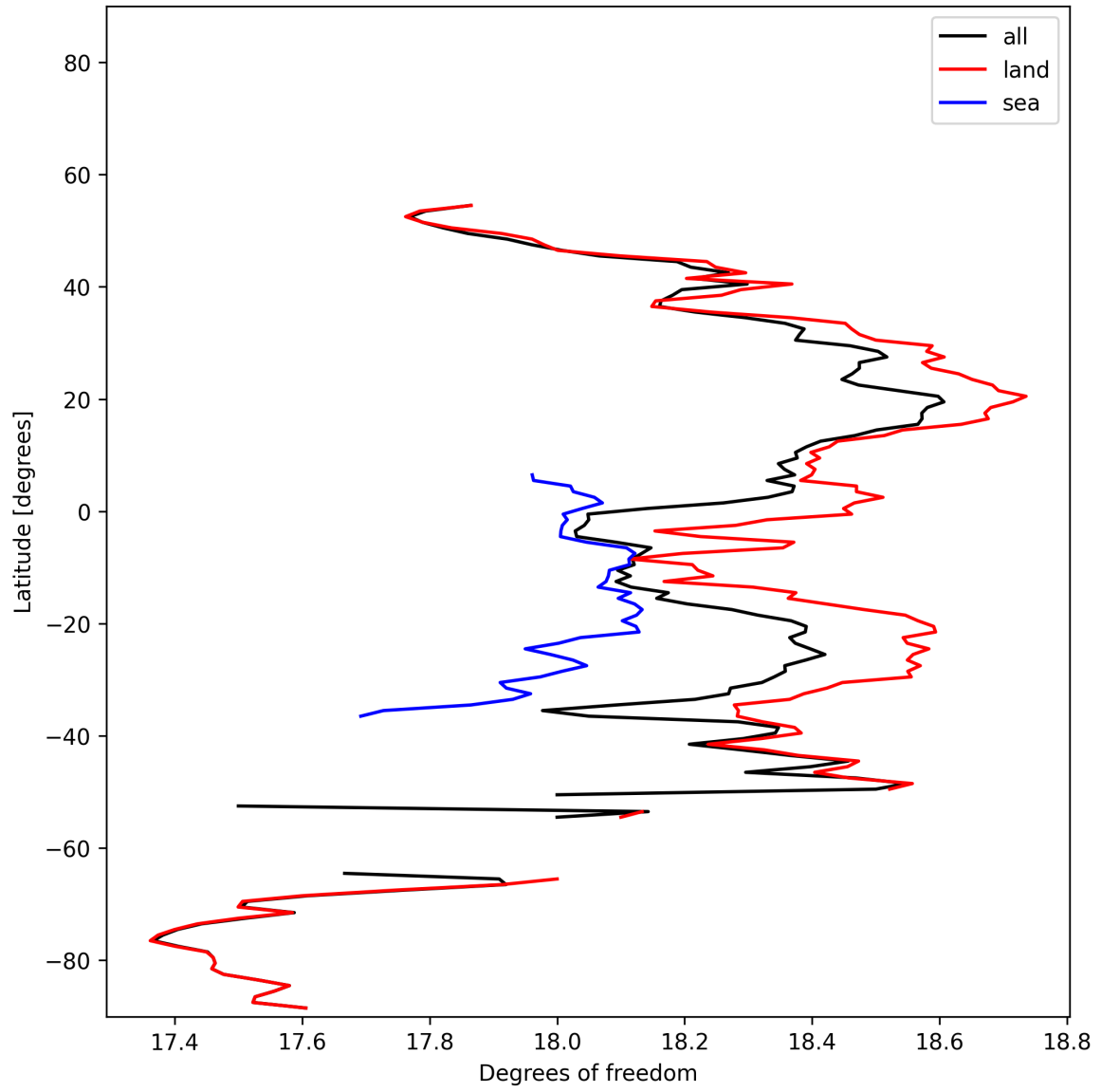
Figure 19: Zonal average of “Degrees of freedom” for 2025-01-18 to 2025-01-20.
