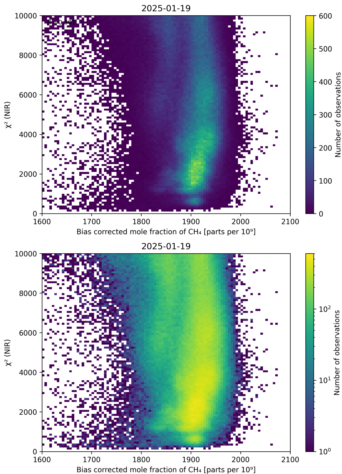
Figure 63: Scatter density plot of “Bias corrected mole fraction of \text{CH}_4 ” against “ \chi^2 (NIR)” for 2025-01-18 to 2025-01-20.
