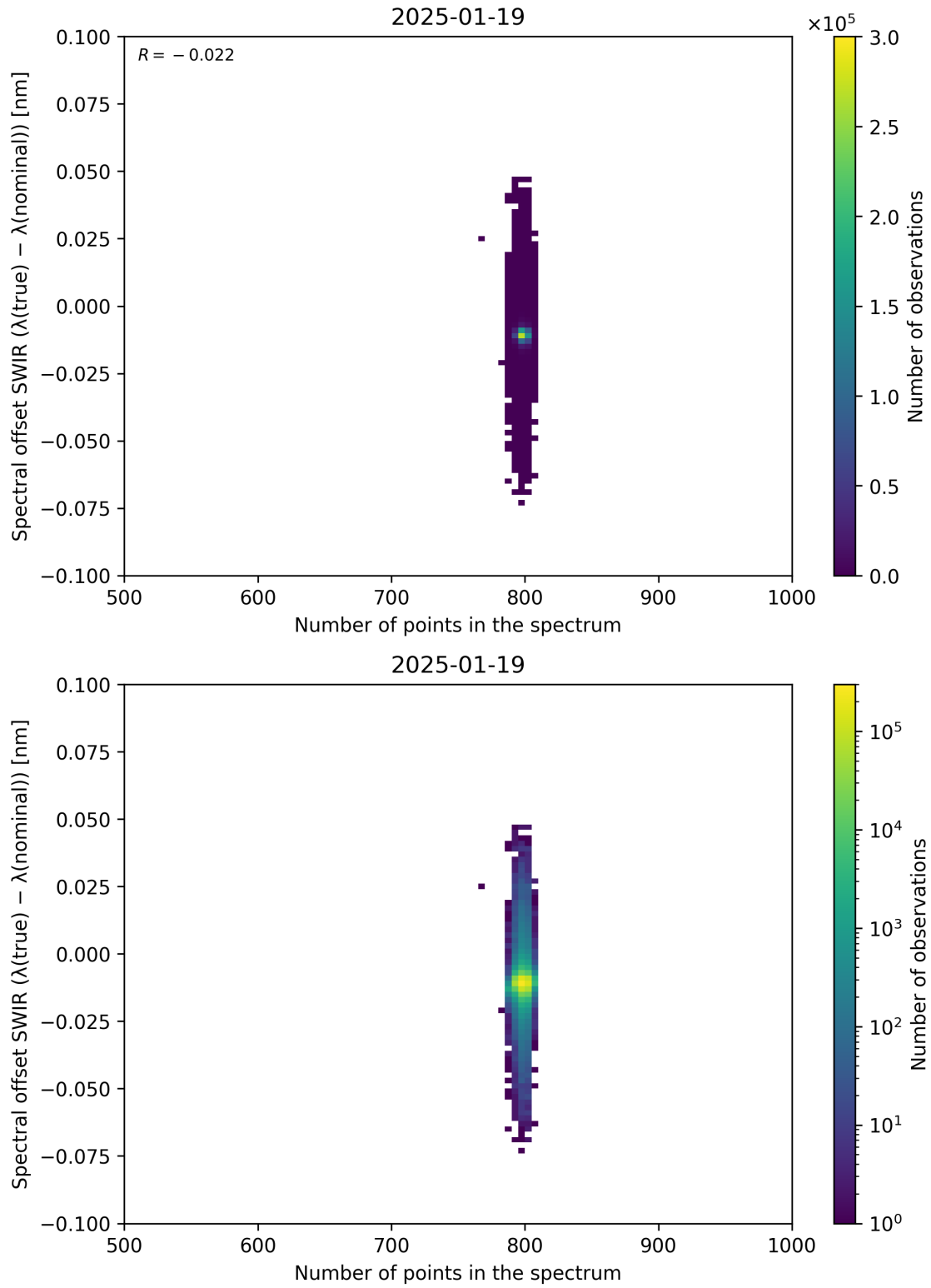
Figure 93: Scatter density plot of “Number of points in the spectrum” against “Spectral offset SWIR ( \lambda_{\text{true}} - \lambda_{\text{nominal}} )” for 2025-01-18 to 2025-01-20.
