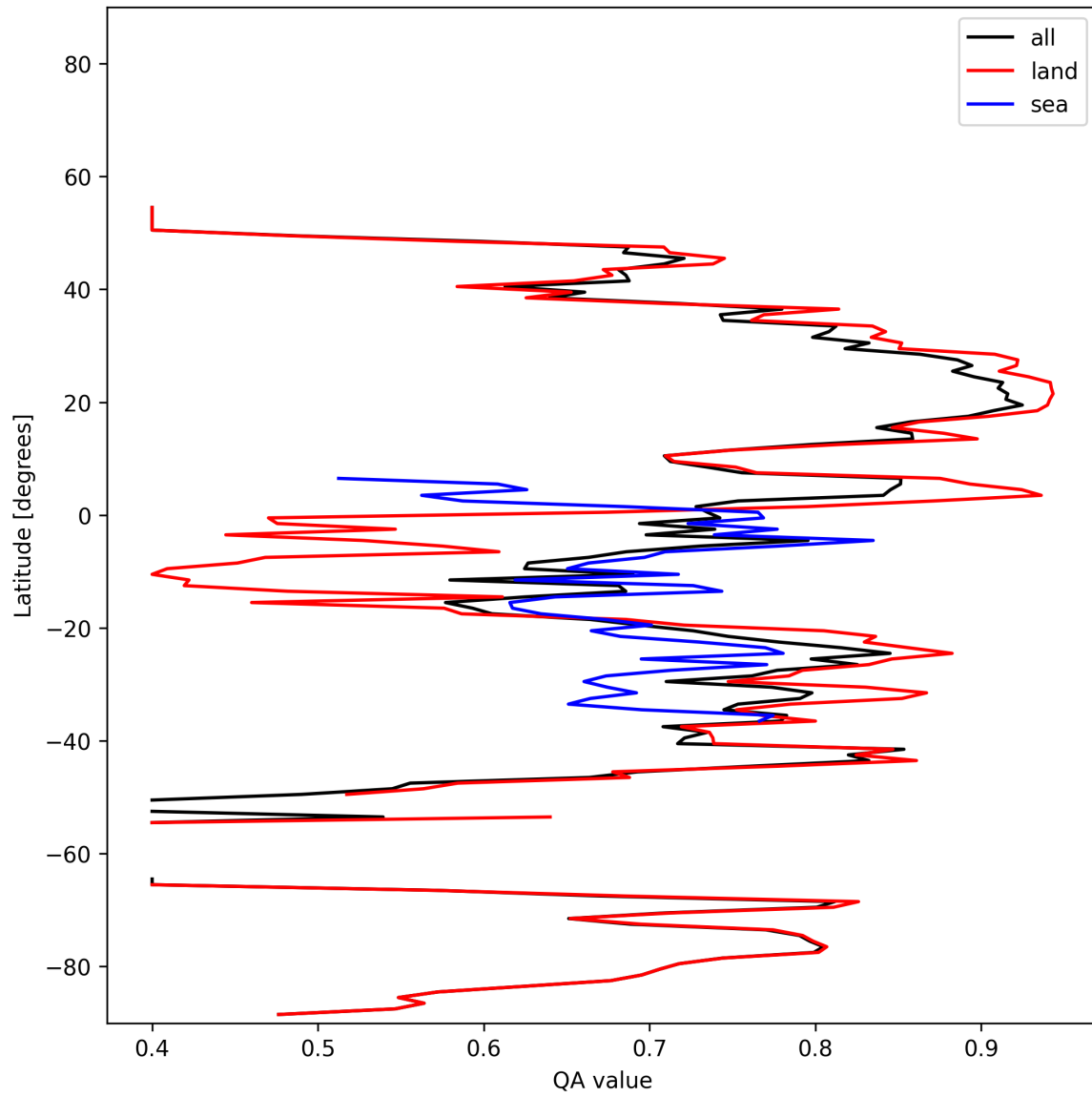
Figure 11: Zonal average of “QA value” for 2025-01-18 to 2025-01-20.
