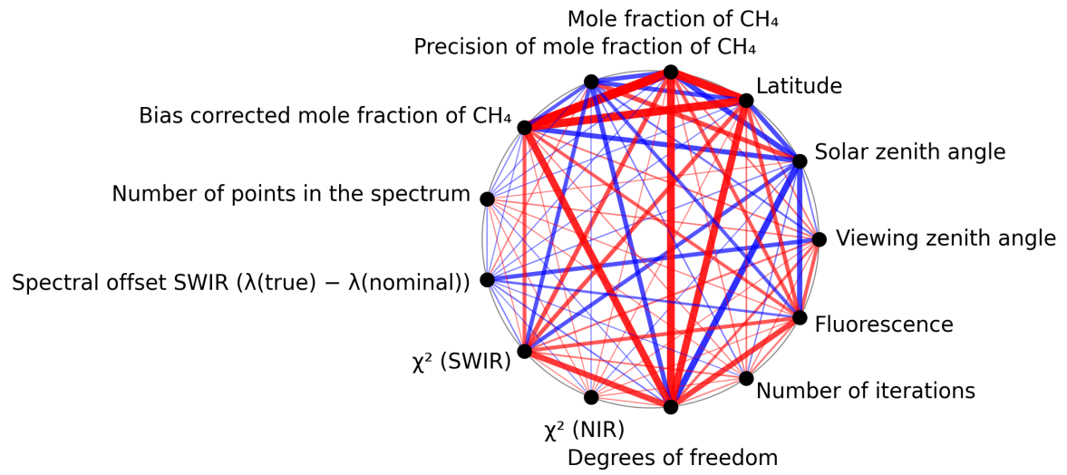
Figure 1: Map of correlation graph for 2025-01-18 to 2025-01-20.
