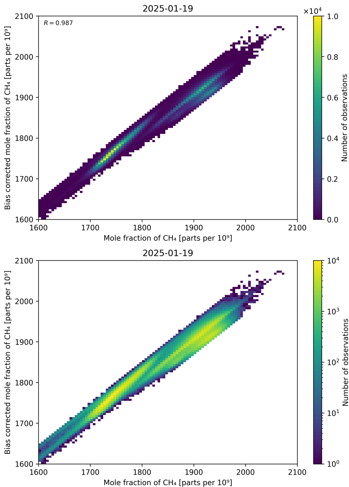
Figure 74: Scatter density plot of “Mole fraction of CH 4 ” against “Bias corrected mole fraction of CH 4 ” for 2025-01-18 to 2025-01-20.
