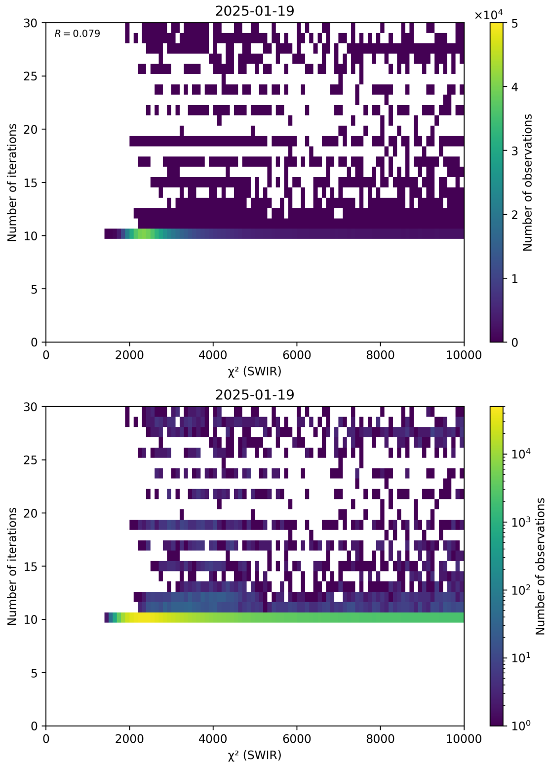
Figure 50: Scatter density plot of “ \chi^2 (SWIR)” against “Number of iterations” for 2025-01-18 to 2025-01-20.
