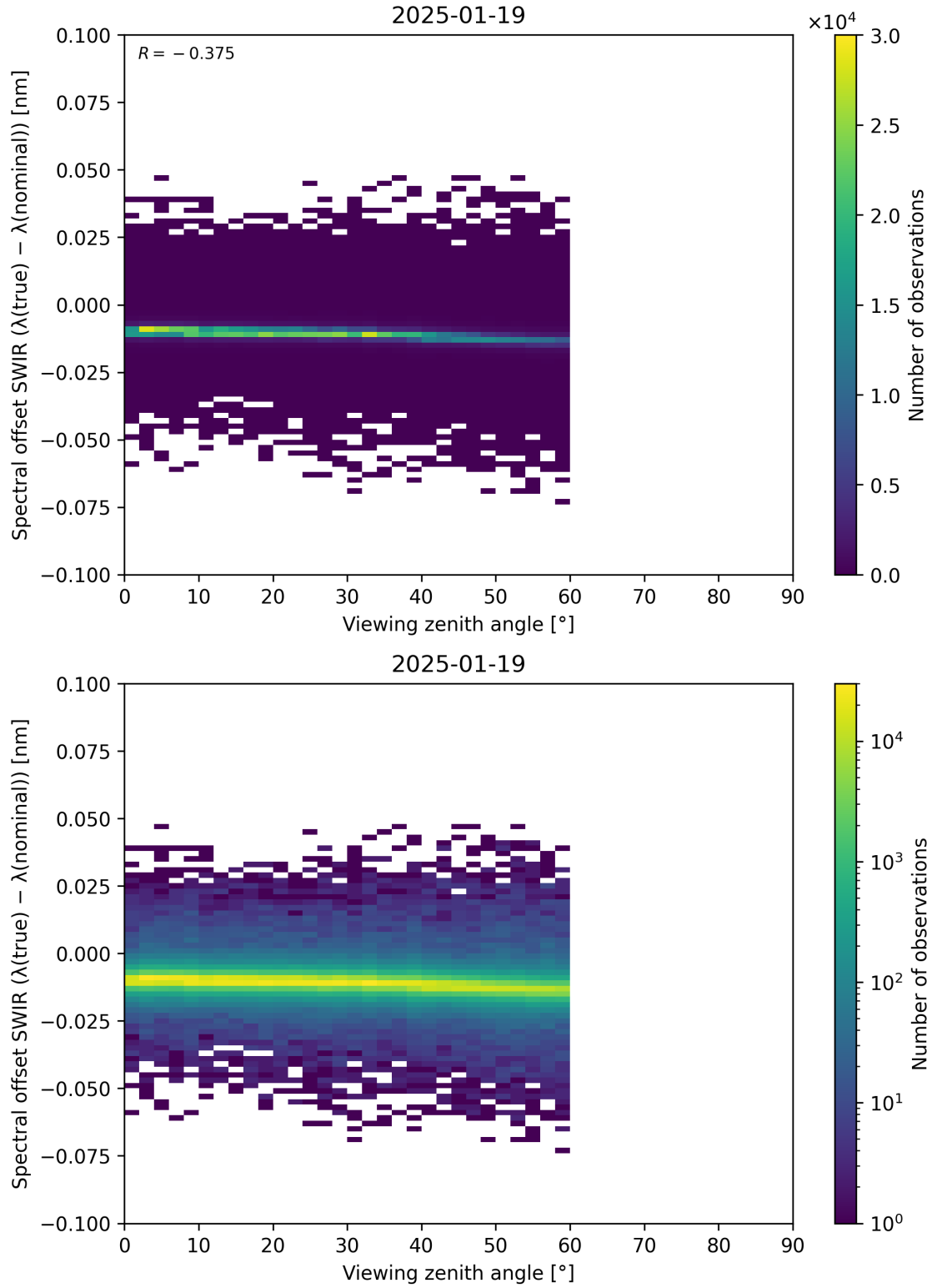
Figure 116: Scatter density plot of “Viewing zenith angle” against “Spectral offset SWIR ( \lambda_{\text{true}} - \lambda_{\text{nominal}} )” for 2025-01-18 to 2025-01-20.
