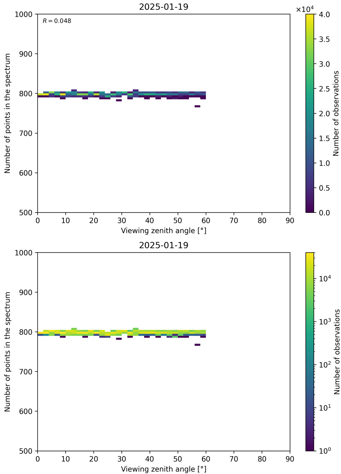
Figure 114: Scatter density plot of “Viewing zenith angle” against “Number of points in the spectrum” for 2025-01-18 to 2025-01-20.
