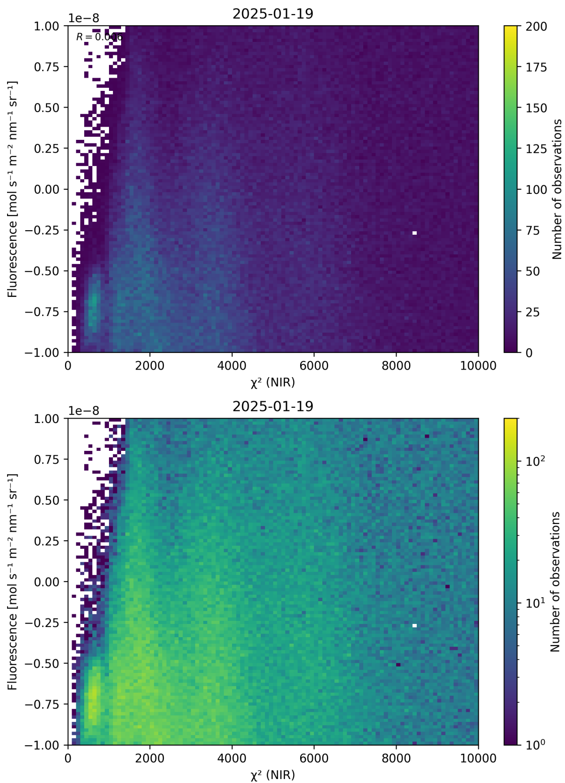
Figure 45: Scatter density plot of “ \chi^2 (NIR)” against “Fluorescence” for 2025-01-18 to 2025-01-20.
