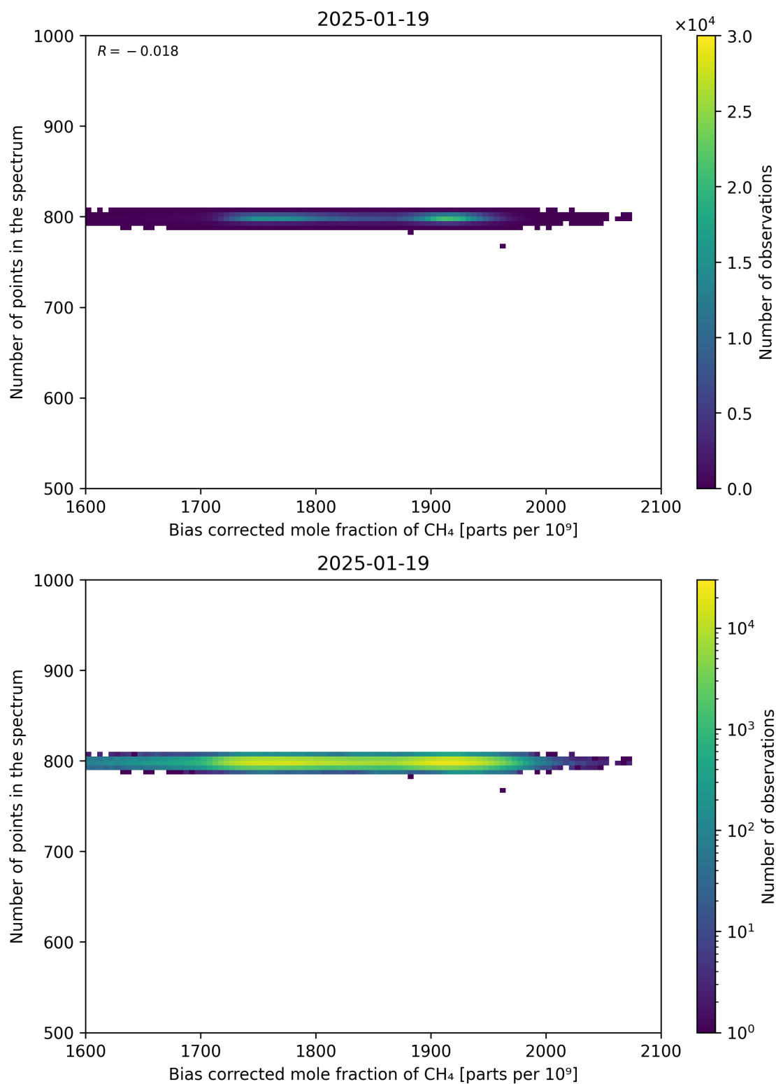
Figure 68: Scatter density plot of “Bias corrected mole fraction of CH 4 ” against “Number of points in the spectrum” for 2025-01-18 to 2025-01-20.
