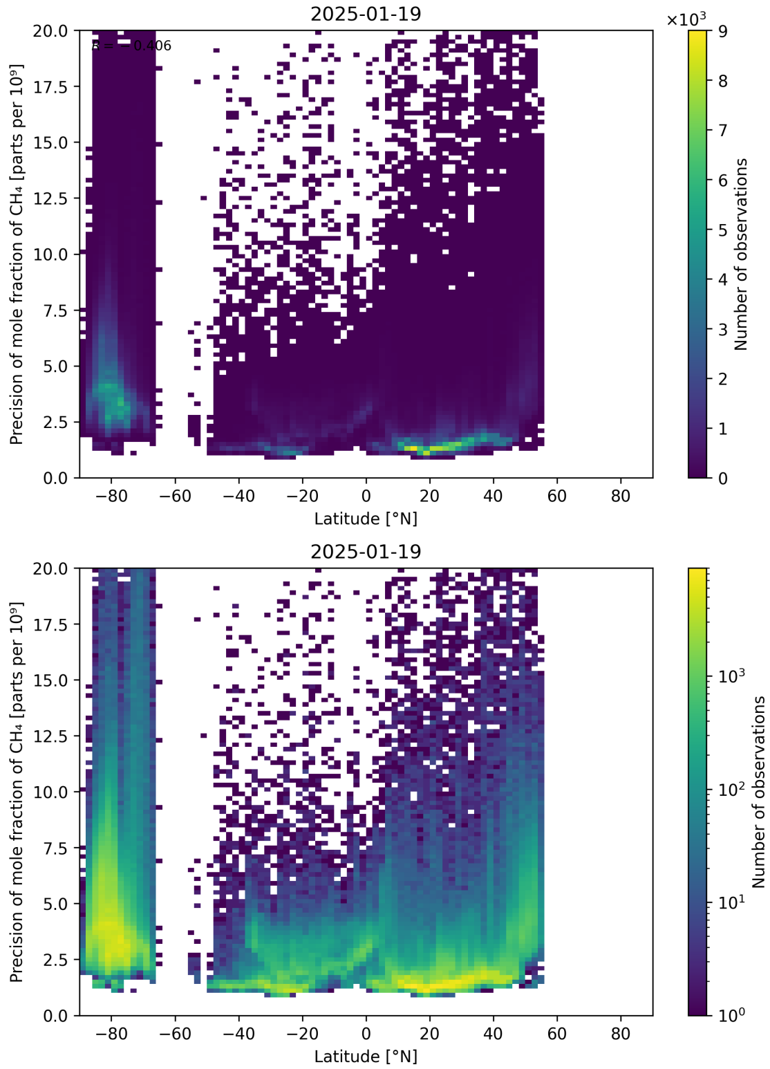
Figure 59: Scatter density plot of “Latitude” against “Precision of mole fraction of CH 4 ” for 2025-01-18 to 2025-01-20.
