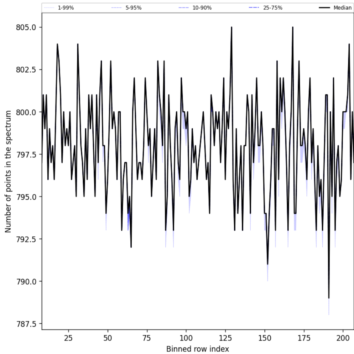
Figure 37: Along track statistics of “Number of points in the spectrum” for 2025-01-18 to 2025-01-20
