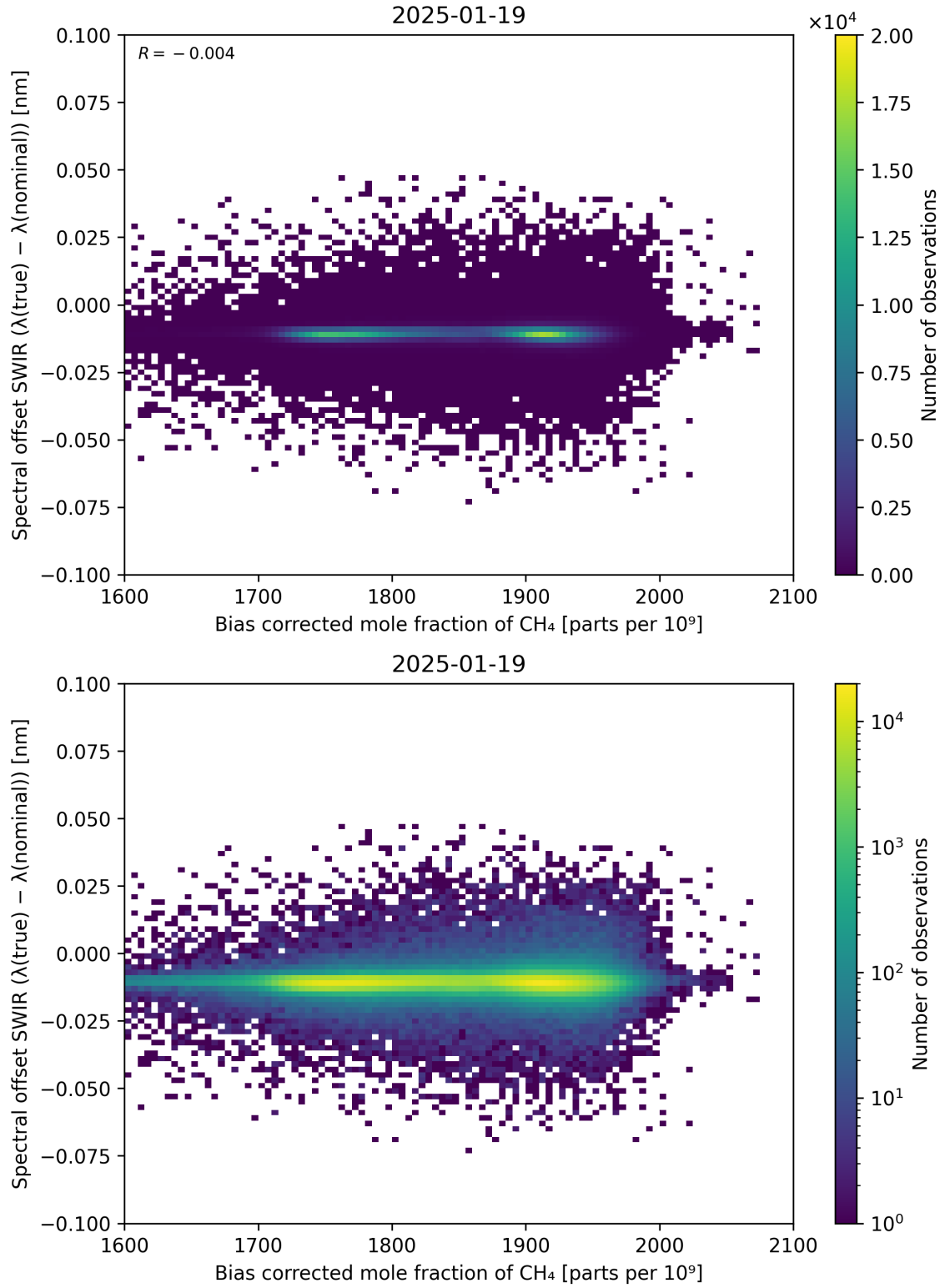
Figure 69: Scatter density plot of “Bias corrected mole fraction of \text{CH}_4 ” against “Spectral offset SWIR ( \lambda_{\text{true}} - \lambda_{\text{nominal}} )” for 2025-01-18 to 2025-01-20.
