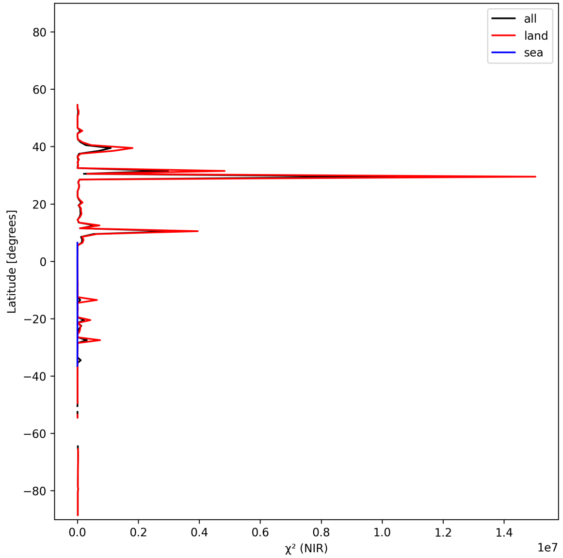
Figure 18: Zonal average of “ \chi^2 (NIR)” for 2025-01-18 to 2025-01-20.
