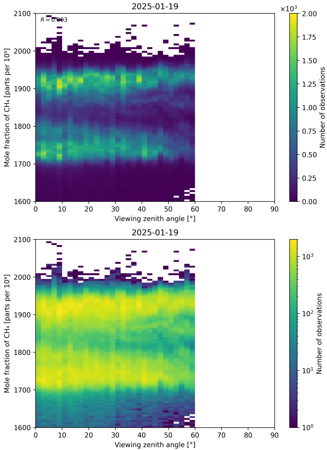
Figure 110: Scatter density plot of "Viewing zenith angle" against "Mole fraction of CH 4 " for 2025-01-18 to 2025-01-20.
