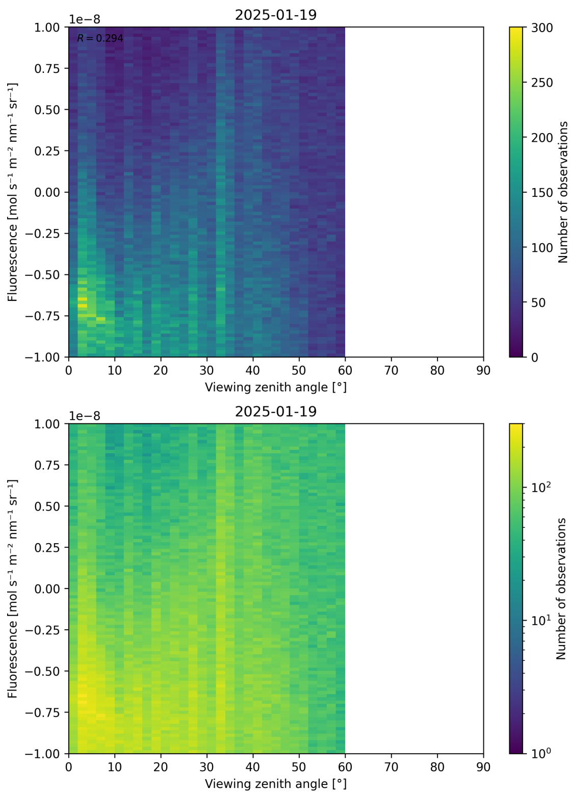
Figure 108: Scatter density plot of “Viewing zenith angle” against “Fluorescence” for 2025-01-18 to 2025-01-20.
