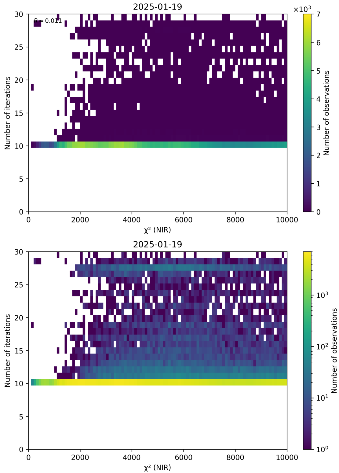
Figure 46: Scatter density plot of “ \chi^2 (NIR)” against “Number of iterations” for 2025-01-18 to 2025-01-20.
