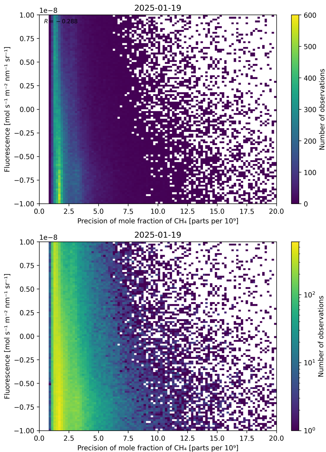
Figure 81: Scatter density plot of “Precision of mole fraction of \text{CH}_4 ” against “Fluorescence” for 2025-01-18 to 2025-01-20.
