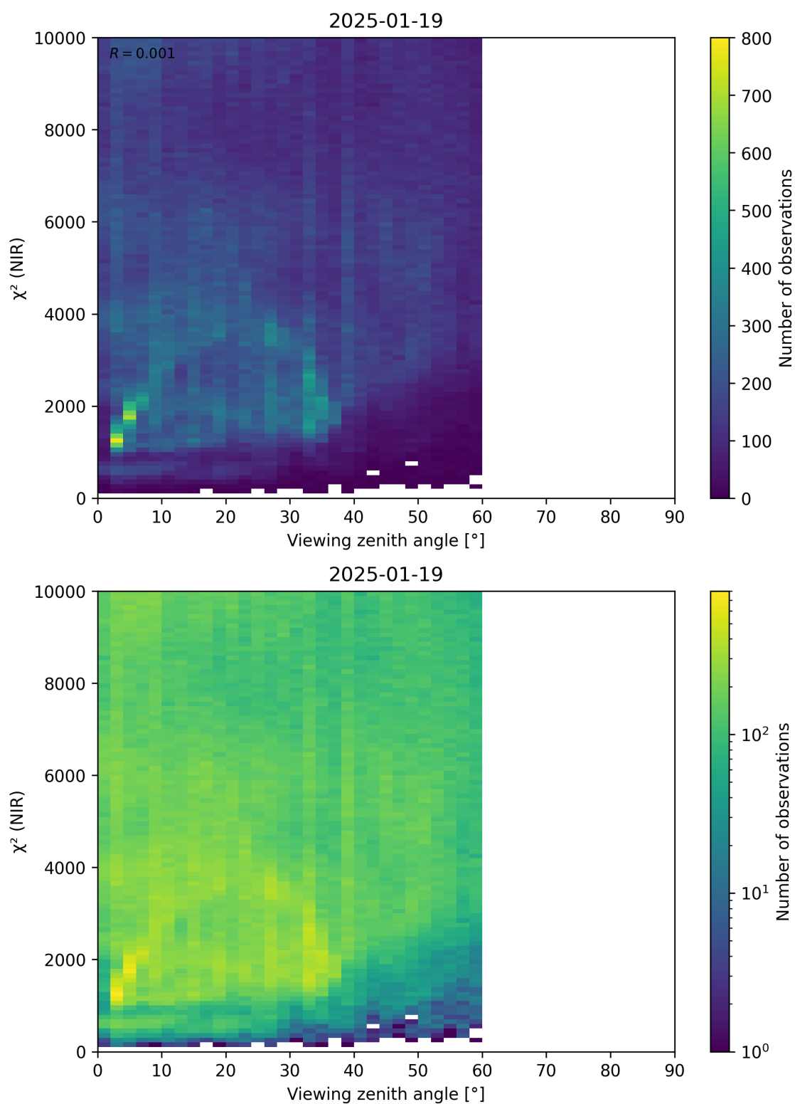
Figure 105: Scatter density plot of “Viewing zenith angle” against “ \chi^2 (NIR)” for 2025-01-18 to 2025-01-20.
