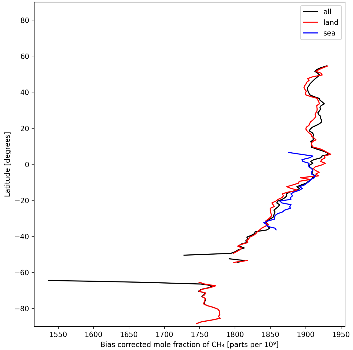
Figure 14: Zonal average of “Bias corrected mole fraction of CH 4 ” for 2025-01-18 to 2025-01-20.
