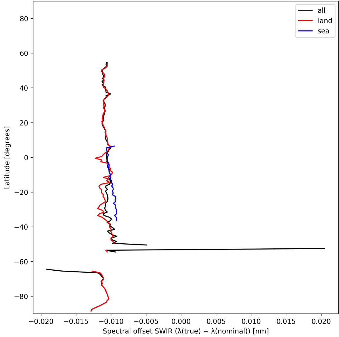
Figure 16: Zonal average of “Spectral offset SWIR ( \lambda_{\text{true}} - \lambda_{\text{nominal}} )” for 2025-01-18 to 2025-01-20.
