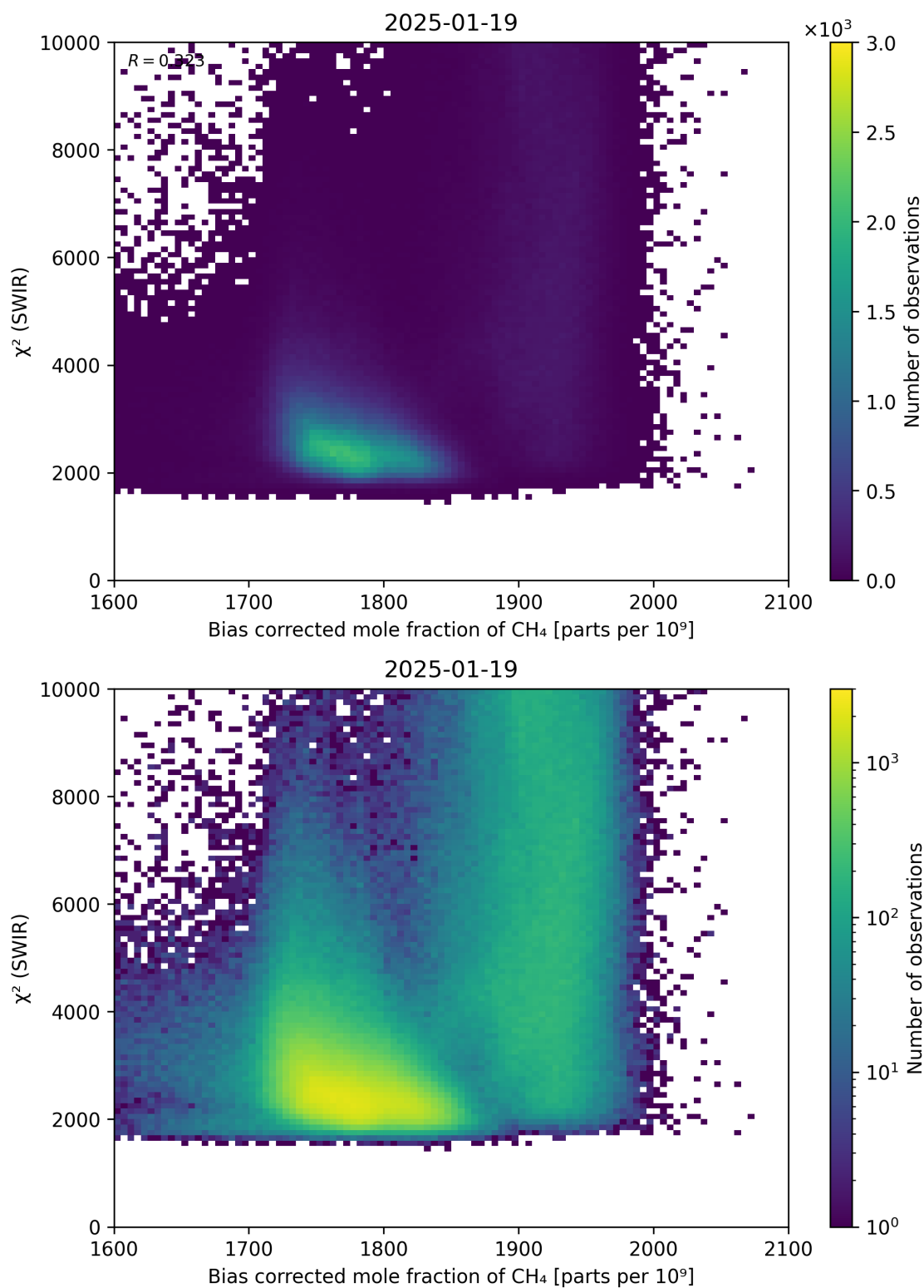
Figure 64: Scatter density plot of “Bias corrected mole fraction of \text{CH}_4 ” against “ \chi^2 (SWIR)” for 2025-01-18 to 2025-01-20.
