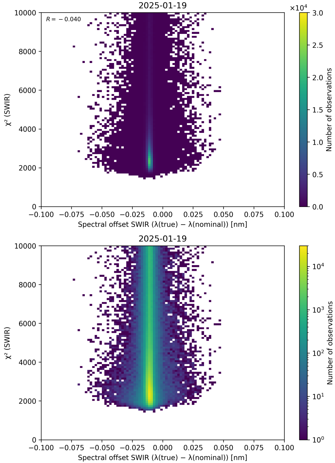
Figure 118: Scatter density plot of “Spectral offset SWIR ( \lambda_{\text{true}} - \lambda_{\text{nominal}} )” against “ \chi^2 (SWIR)” for 2025-01-18 to 2025-01-20.
