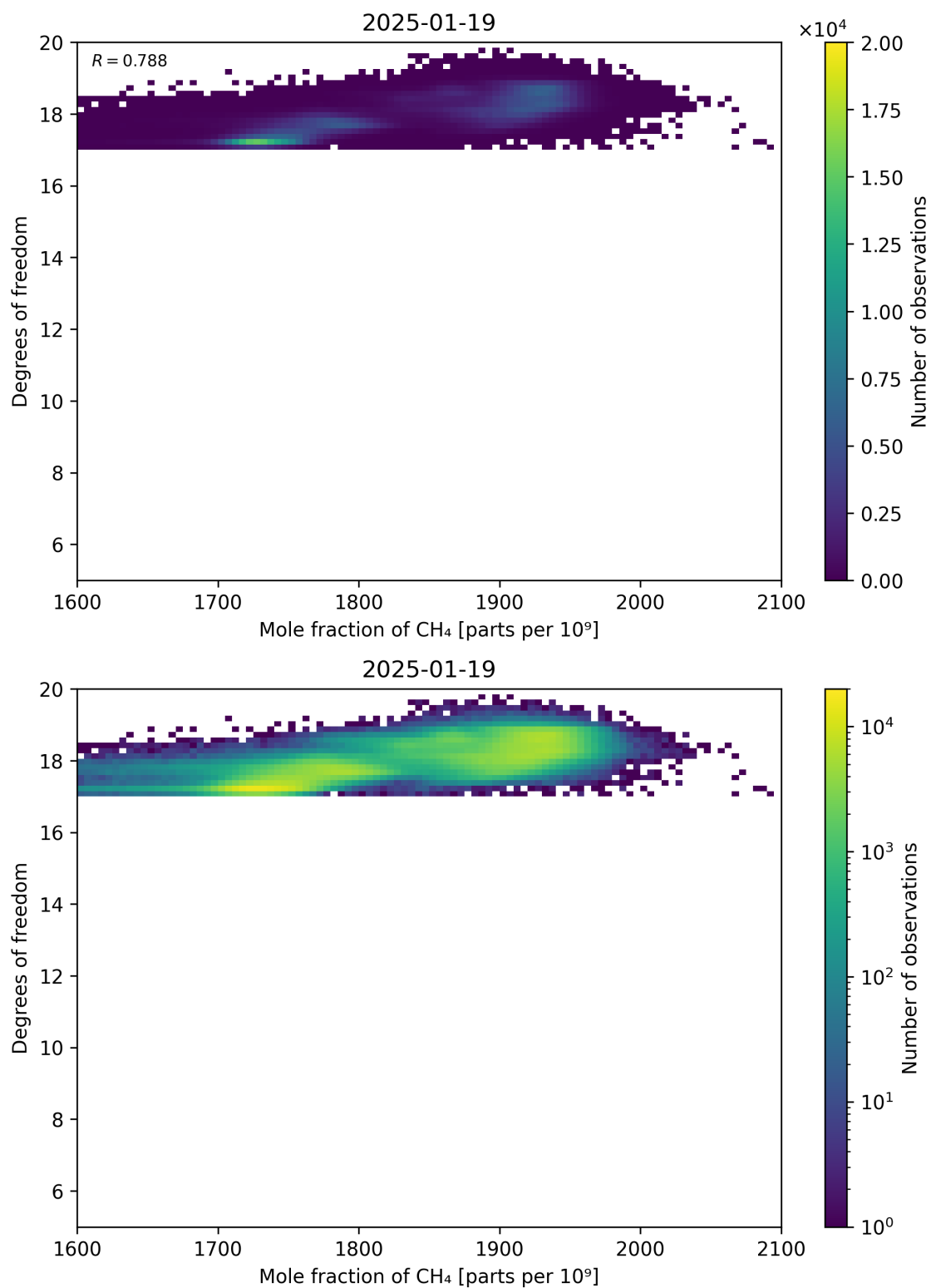
Figure 72: Scatter density plot of “Mole fraction of CH 4 ” against “Degrees of freedom” for 2025-01-18 to 2025-01-20.
