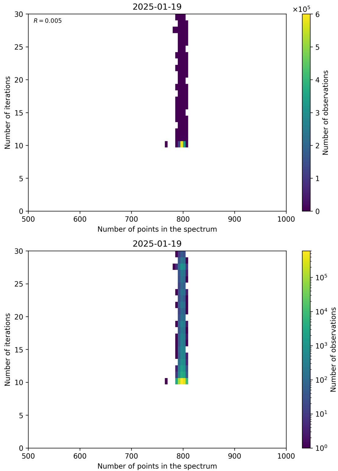
Figure 92: Scatter density plot of “Number of points in the spectrum” against “Number of iterations” for 2025-01-18 to 2025-01-20.
