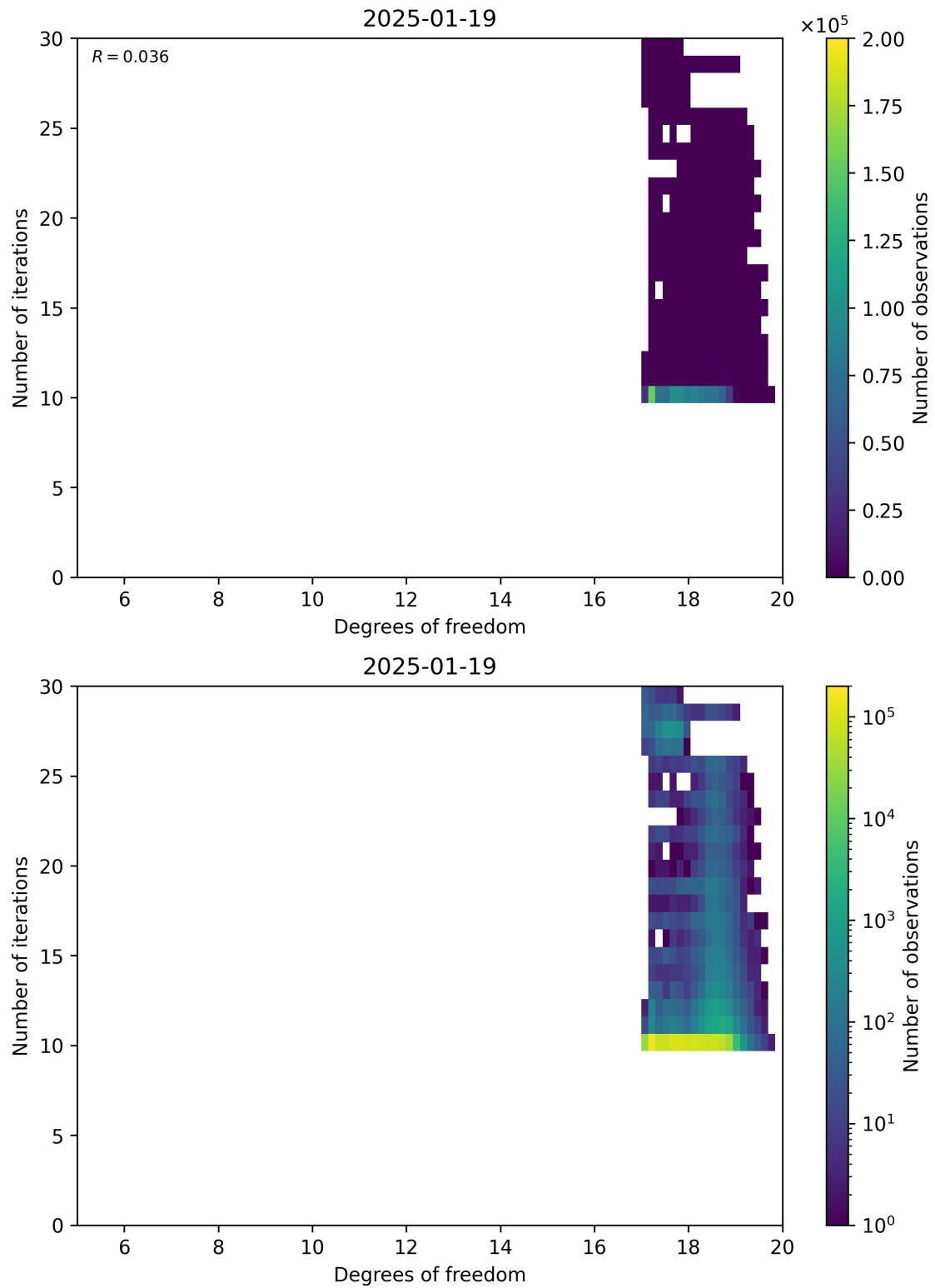
Figure 52: Scatter density plot of “Degrees of freedom” against “Number of iterations” for 2025-01-18 to 2025-01-20.
