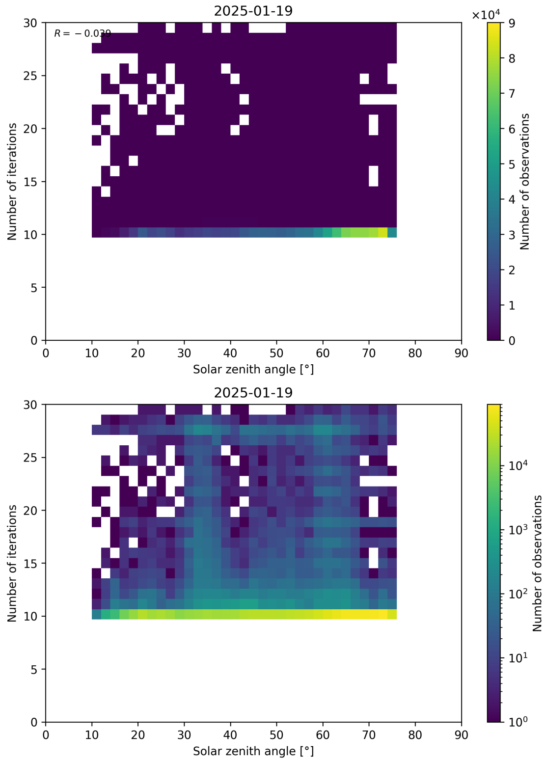
Figure 102: Scatter density plot of “Solar zenith angle” against “Number of iterations” for 2025-01-18 to 2025-01-20.
