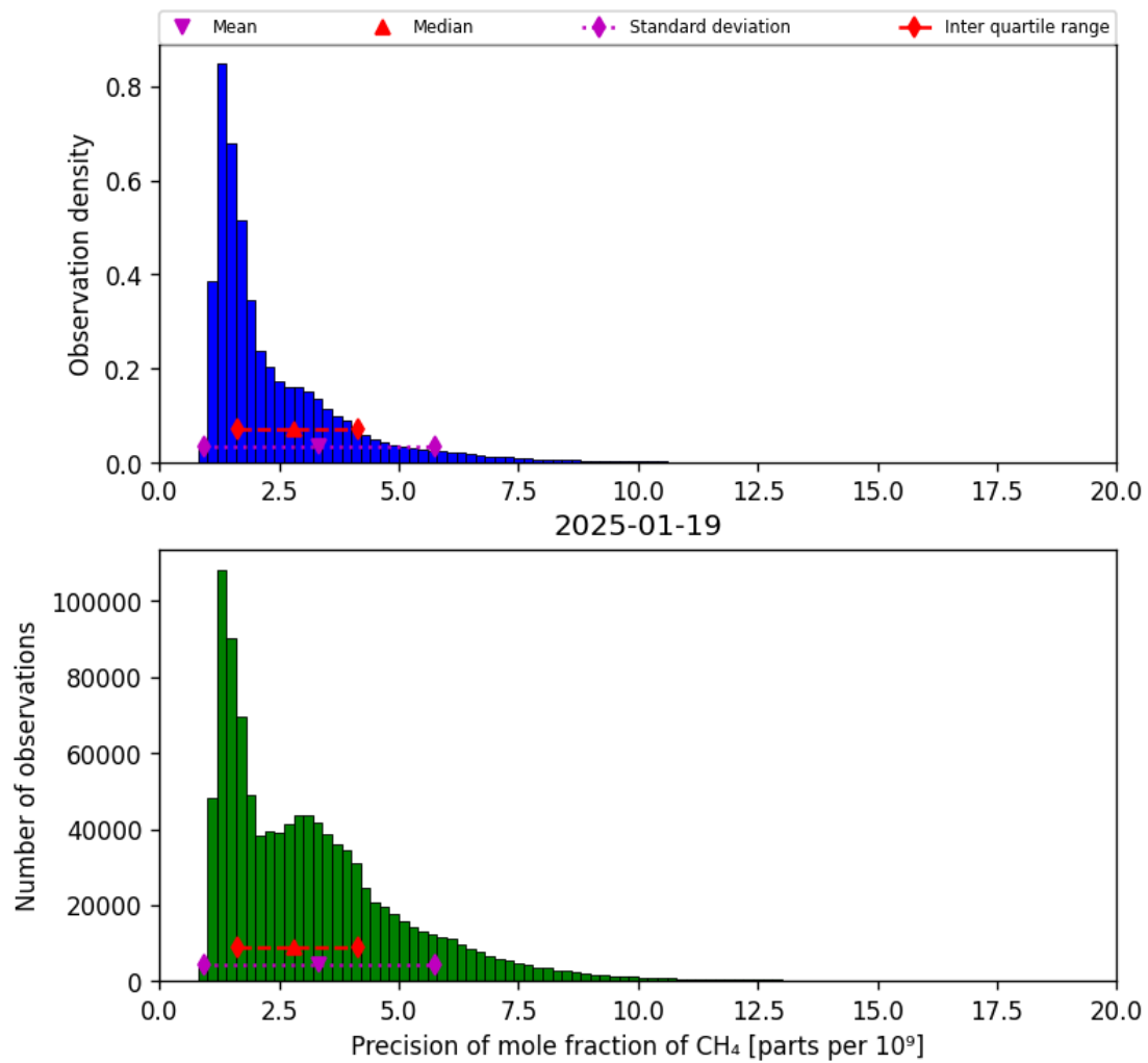
Figure 24: Histogram of “Precision of mole fraction of CH 4 ” for 2025-01-18 to 2025-01-20
