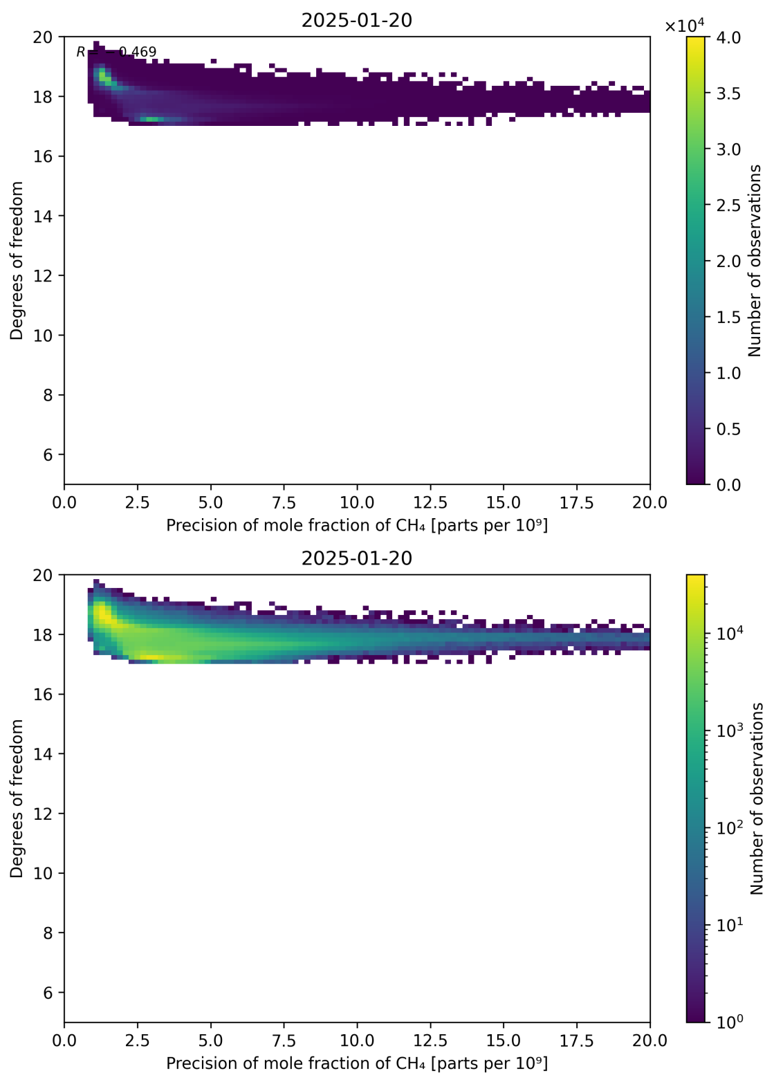
Figure 80: Scatter density plot of “Precision of mole fraction of CH 4 ” against “Degrees of freedom” for 2025-01-19 to 2025-01-21.
