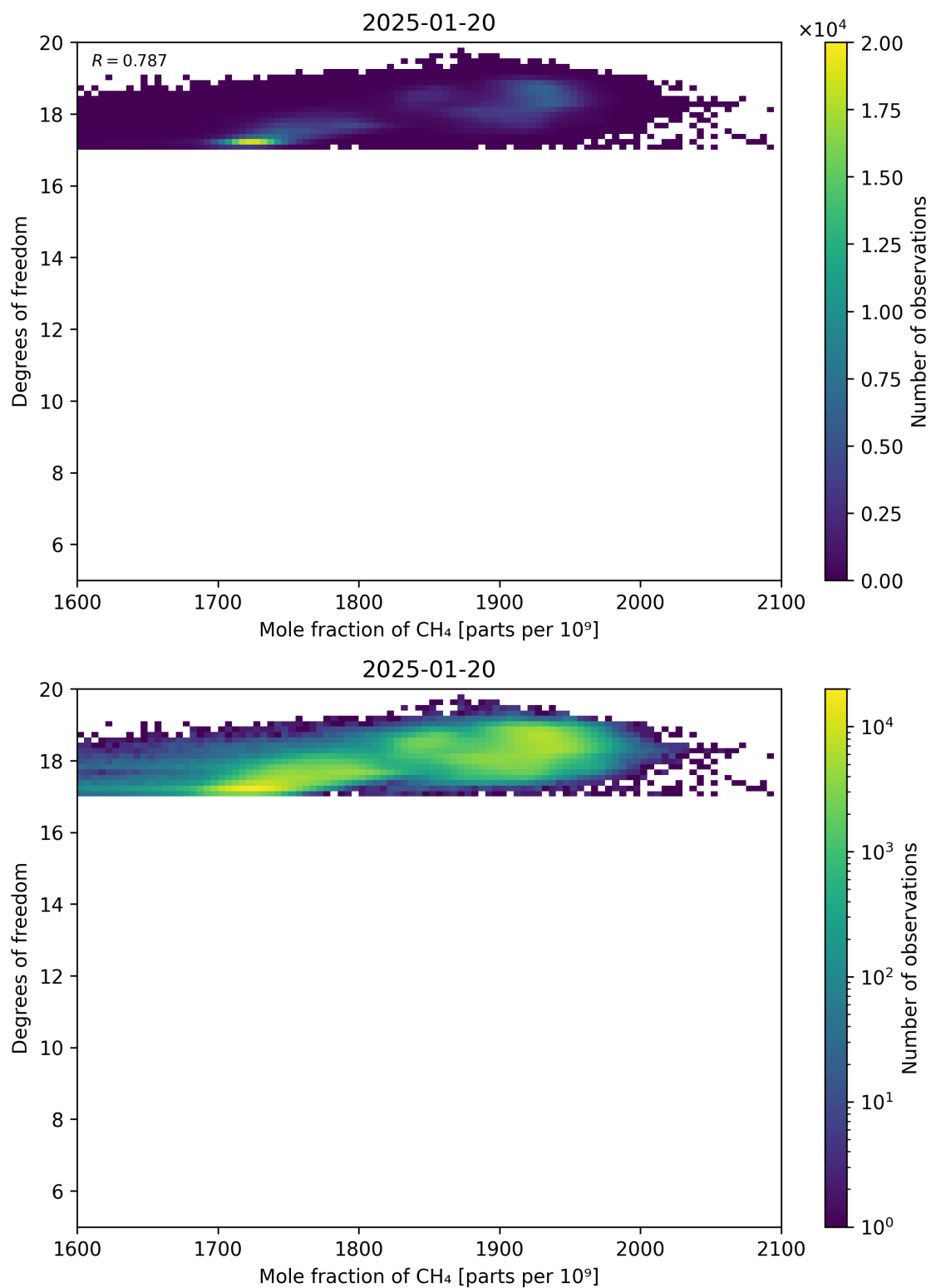
Figure 72: Scatter density plot of “Mole fraction of CH 4 ” against “Degrees of freedom” for 2025-01-19 to 2025-01-21.
