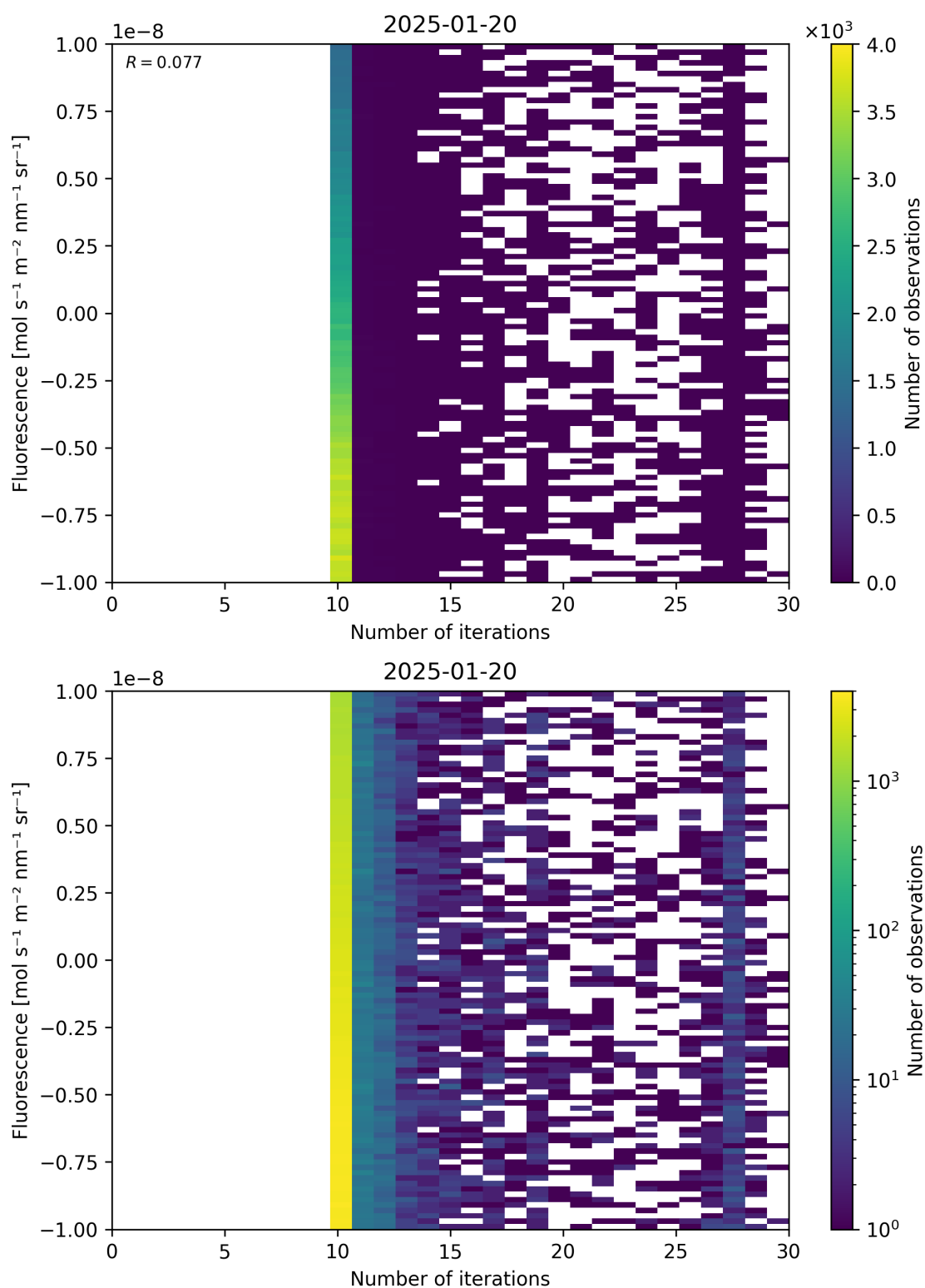
Figure 87: Scatter density plot of “Number of iterations” against “Fluorescence” for 2025-01-19 to 2025-01-21.
