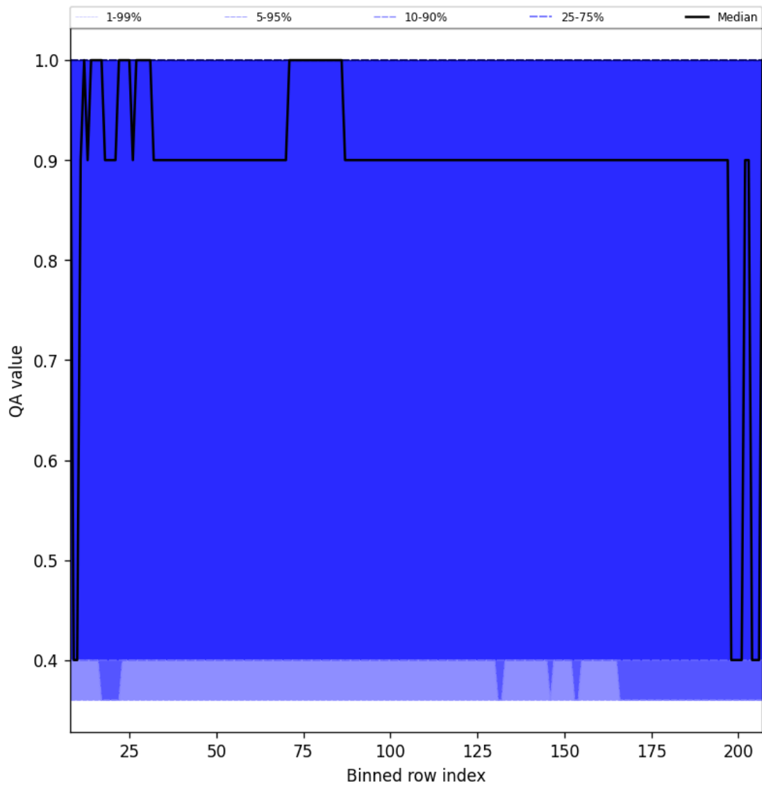
Figure 33: Along track statistics of “QA value” for 2025-01-19 to 2025-01-21
