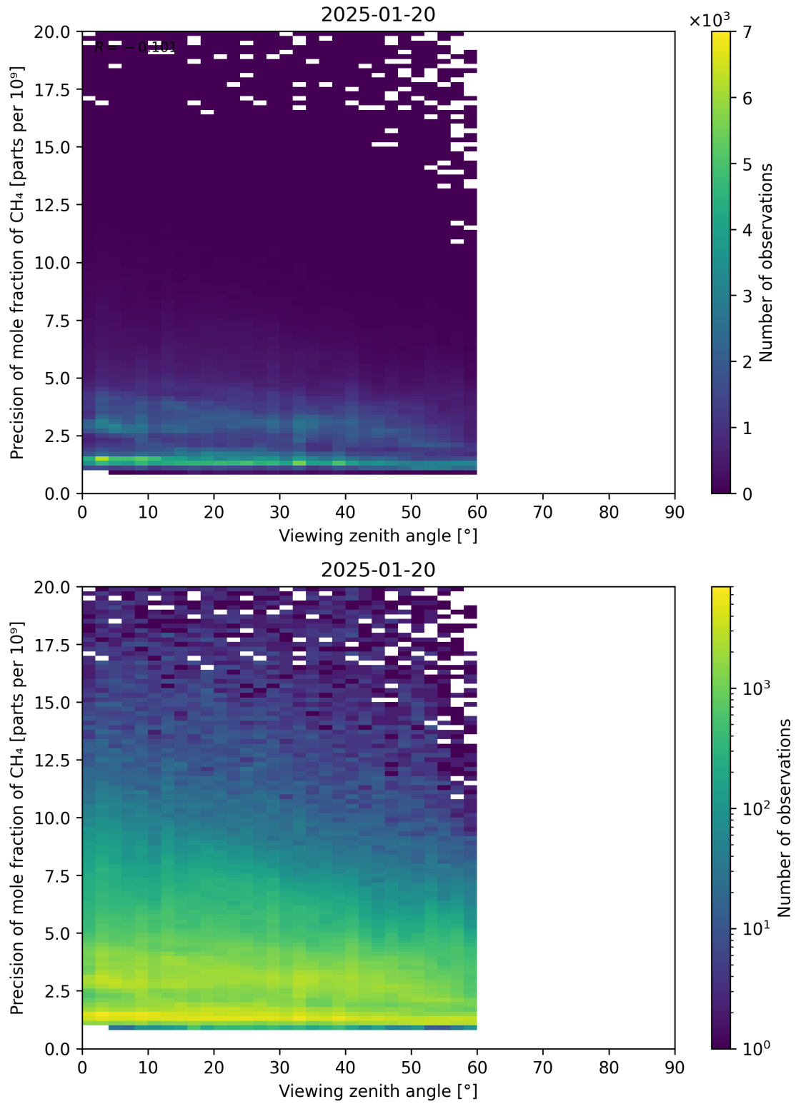
Figure 112: Scatter density plot of “Viewing zenith angle” against “Precision of mole fraction of CH 4 ” for 2025-01-19 to 2025-01-21.
