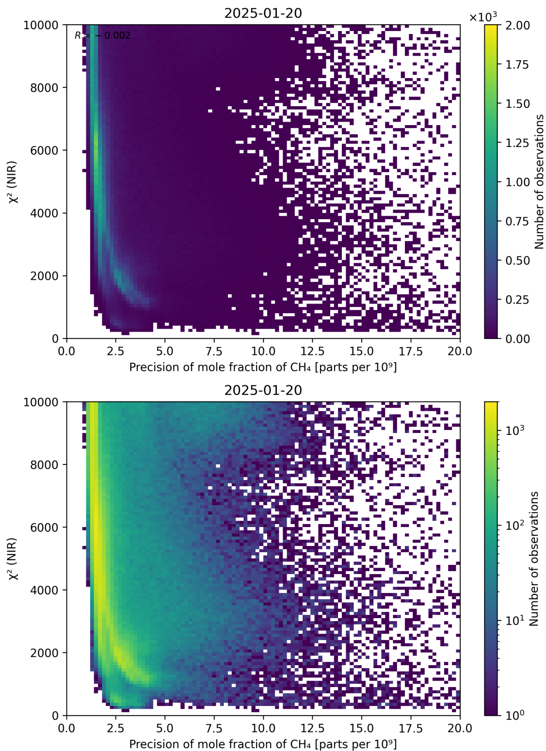
Figure 78: Scatter density plot of “Precision of mole fraction of \text{CH}_4 ” against “ \chi^2 (NIR)” for 2025-01-19 to 2025-01-21.
