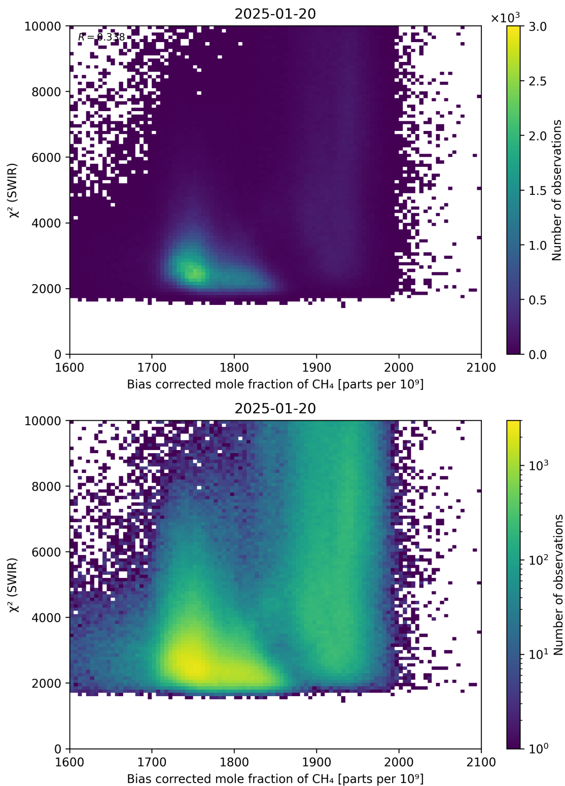
Figure 64: Scatter density plot of “Bias corrected mole fraction of \text{CH}_4 ” against “ \chi^2 (SWIR)” for 2025-01-19 to 2025-01-21.
