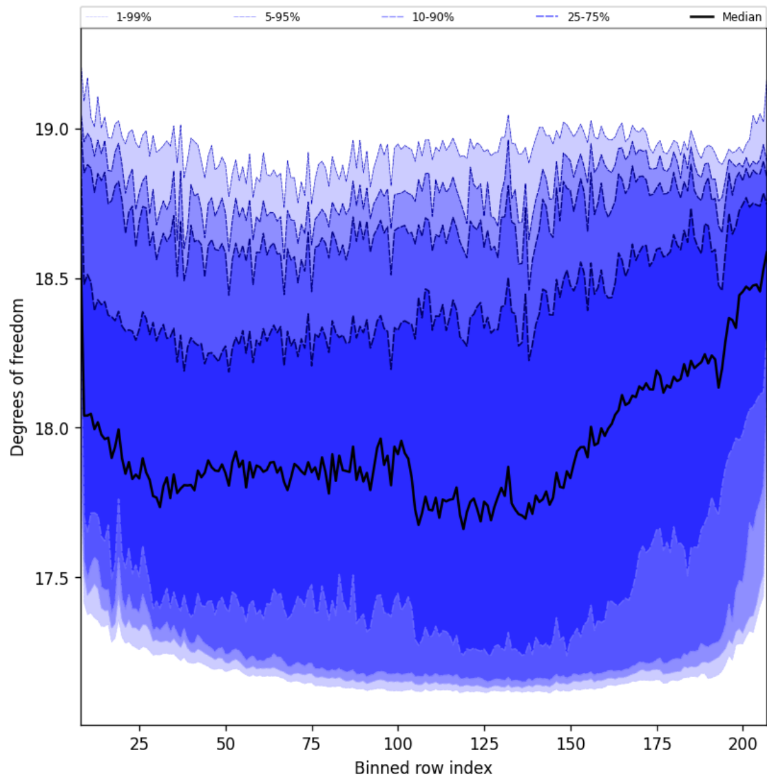
Figure 41: Along track statistics of “Degrees of freedom” for 2025-01-19 to 2025-01-21
