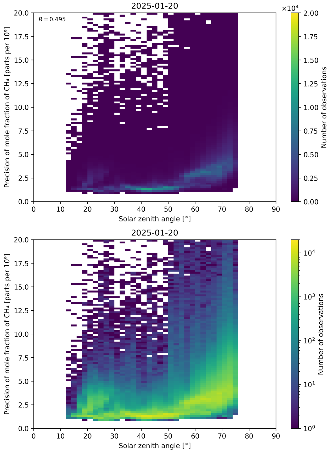
Figure 101: Scatter density plot of “Solar zenith angle” against “Precision of mole fraction of \text{CH}_4 ” for 2025-01-19 to 2025-01-21.
