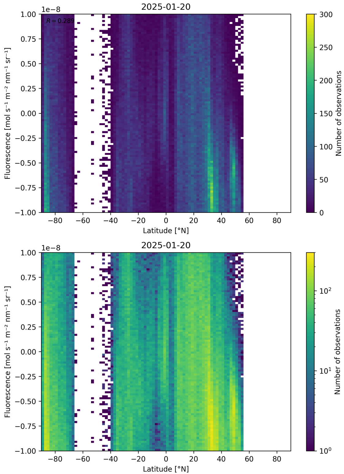
Figure 56: Scatter density plot of “Latitude” against “Fluorescence” for 2025-01-19 to 2025-01-21.
