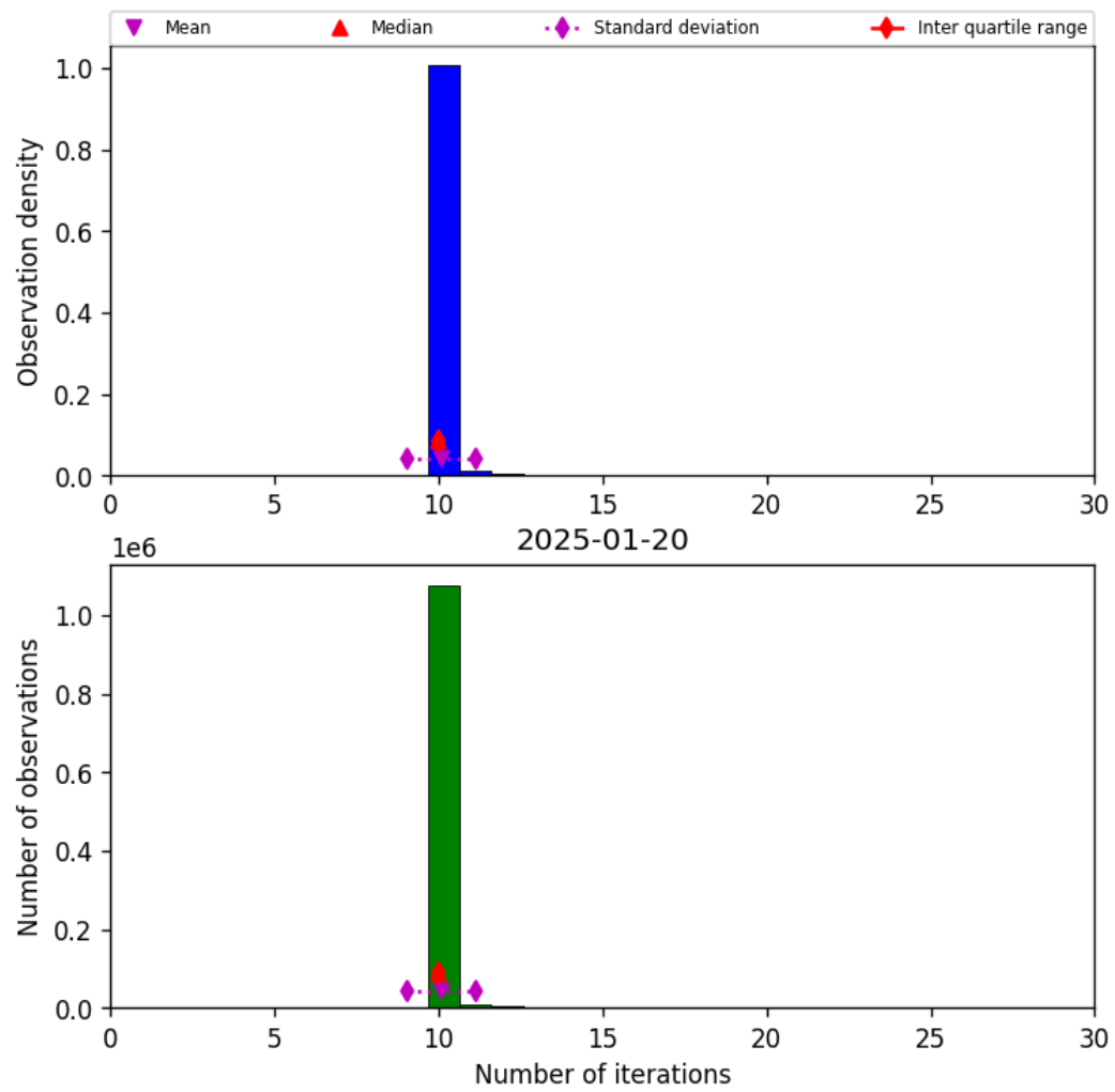
Figure 31: Histogram of "Number of iterations" for 2025-01-19 to 2025-01-21
