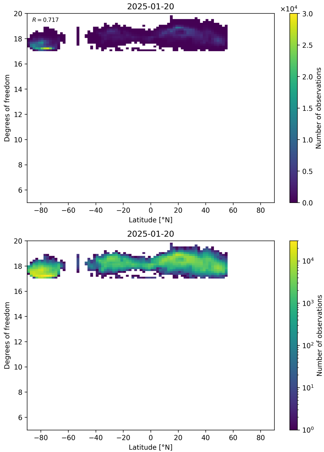
Figure 55: Scatter density plot of “Latitude” against “Degrees of freedom” for 2025-01-19 to 2025-01-21.
