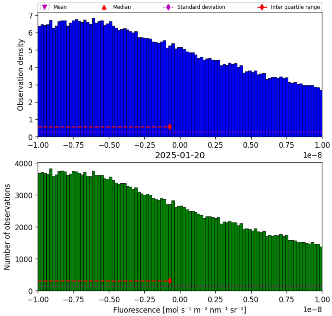
Figure 32: Histogram of “Fluorescence” for 2025-01-19 to 2025-01-21
