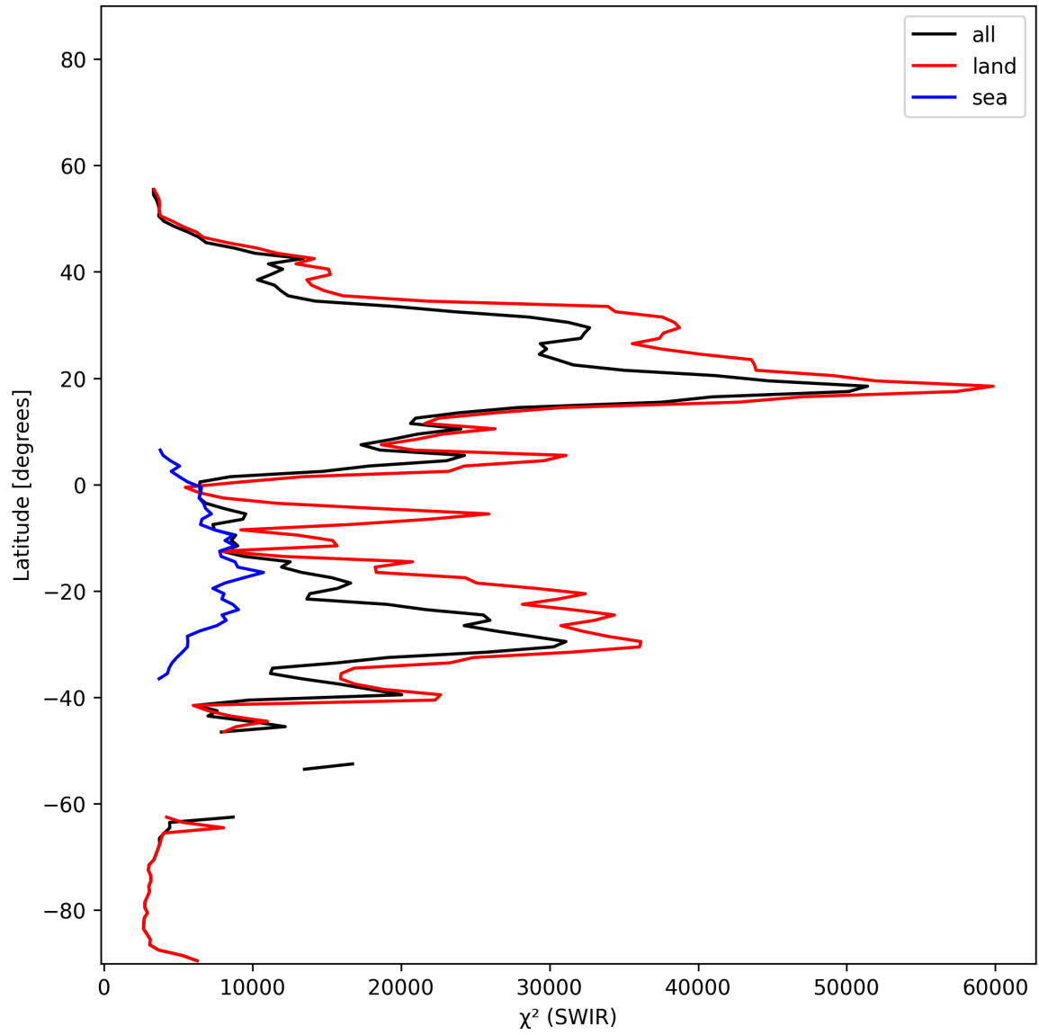
Figure 17: Zonal average of “ \chi^2 (SWIR)” for 2025-01-19 to 2025-01-21.
