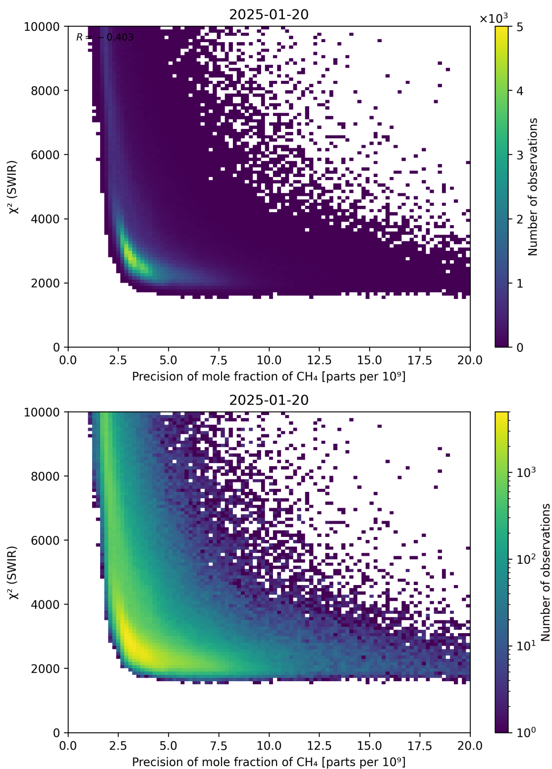
Figure 79: Scatter density plot of “Precision of mole fraction of \text{CH}_4 ” against “ \chi^2 (SWIR)” for 2025-01-19 to 2025-01-21.
