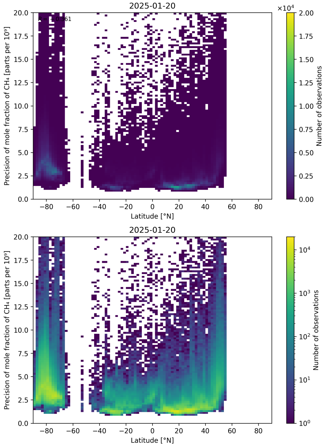
Figure 59: Scatter density plot of “Latitude” against “Precision of mole fraction of CH 4 ” for 2025-01-19 to 2025-01-21.
