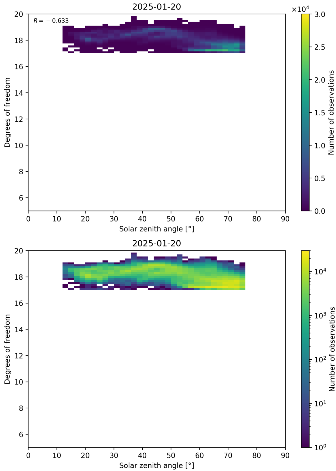
Figure 96: Scatter density plot of “Solar zenith angle” against “Degrees of freedom” for 2025-01-19 to 2025-01-21.
