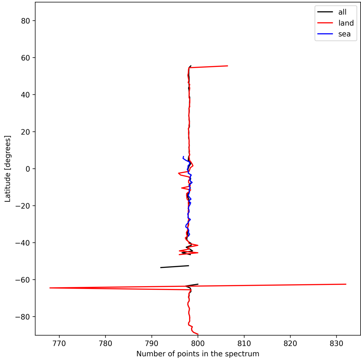
Figure 15: Zonal average of “Number of points in the spectrum” for 2025-01-19 to 2025-01-21.
