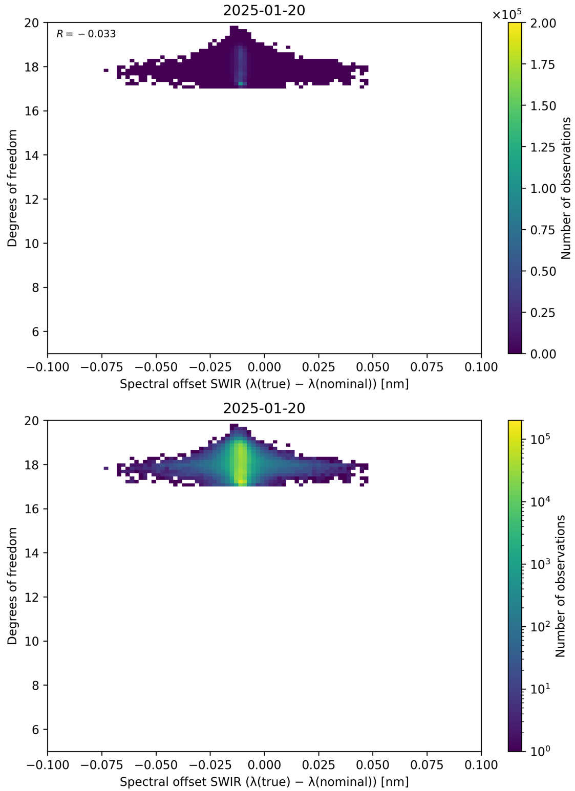
Figure 119: Scatter density plot of “Spectral offset SWIR ( \lambda_{\text{true}} - \lambda_{\text{nominal}} )” against “Degrees of freedom” for 2025-01-19 to 2025-01-21.
