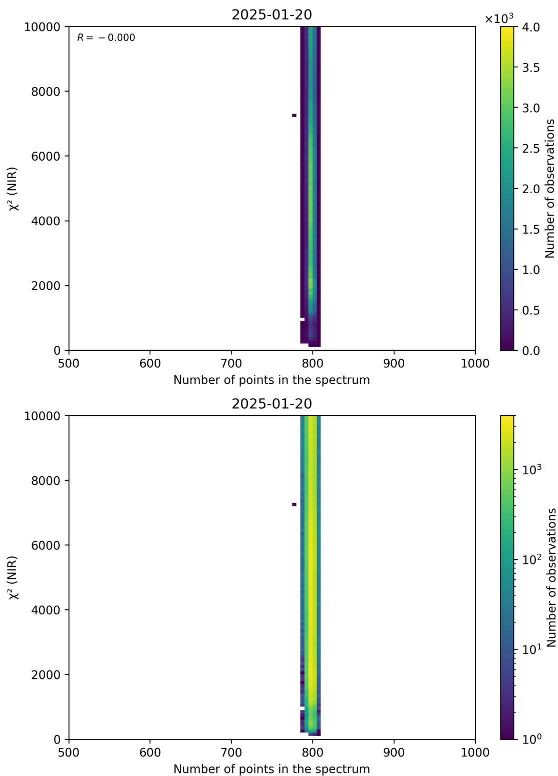
Figure 88: Scatter density plot of “Number of points in the spectrum” against “ \chi^2 (NIR)” for 2025-01-19 to 2025-01-21.
