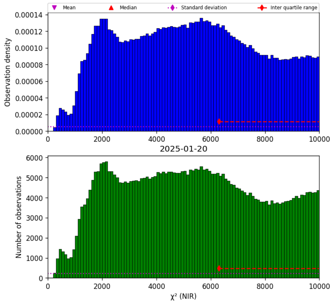
Figure 29: Histogram of " \chi^2 (NIR)" for 2025-01-19 to 2025-01-21
