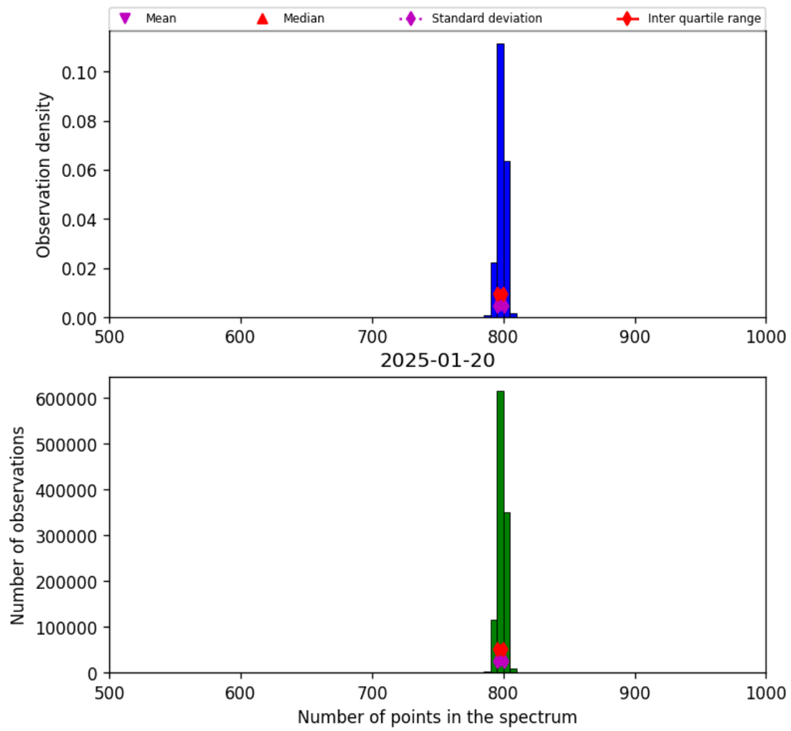
Figure 26: Histogram of “Number of points in the spectrum” for 2025-01-19 to 2025-01-21
