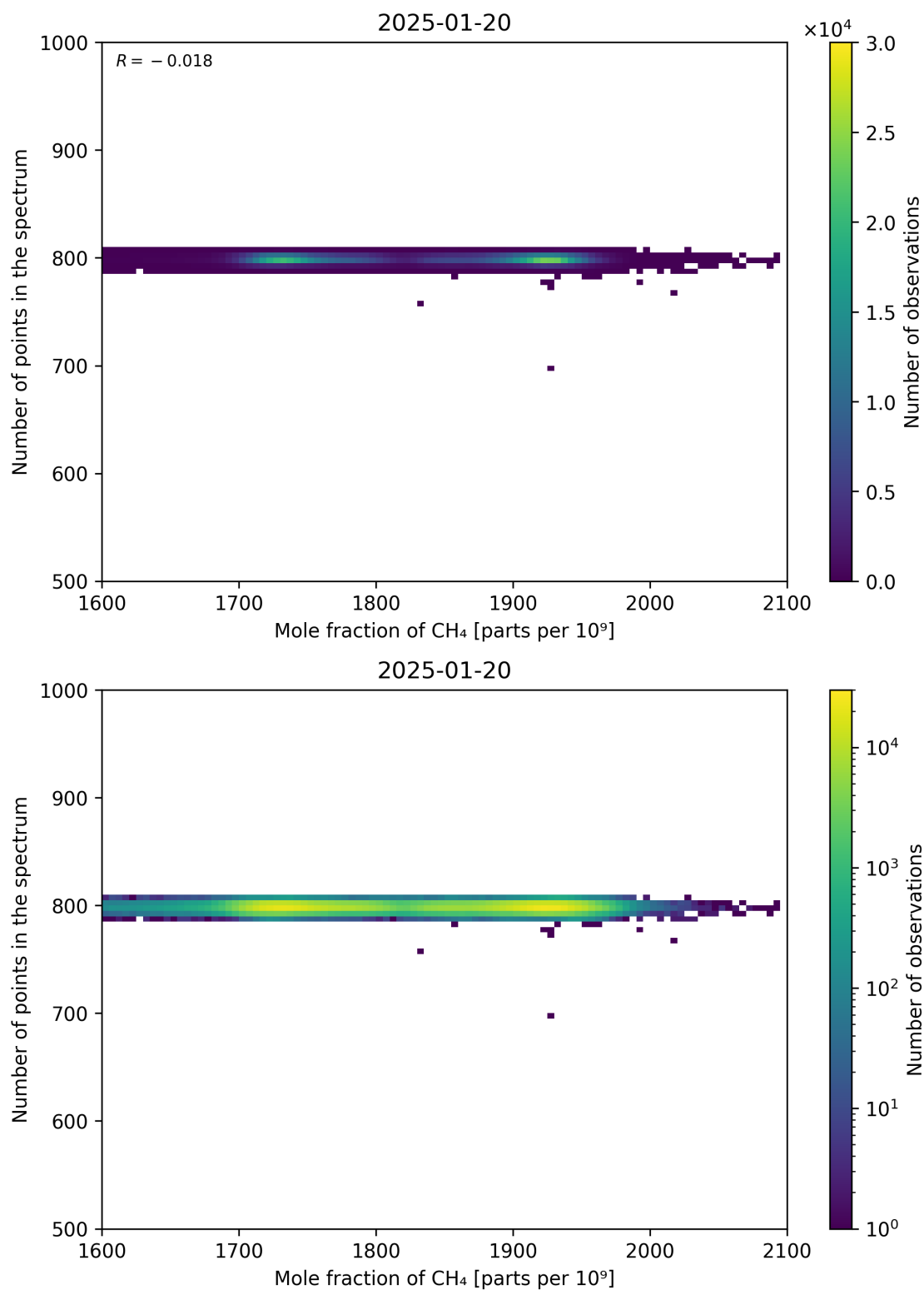
Figure 77: Scatter density plot of “Mole fraction of CH 4 ” against “Number of points in the spectrum” for 2025-01-19 to 2025-01-21.
