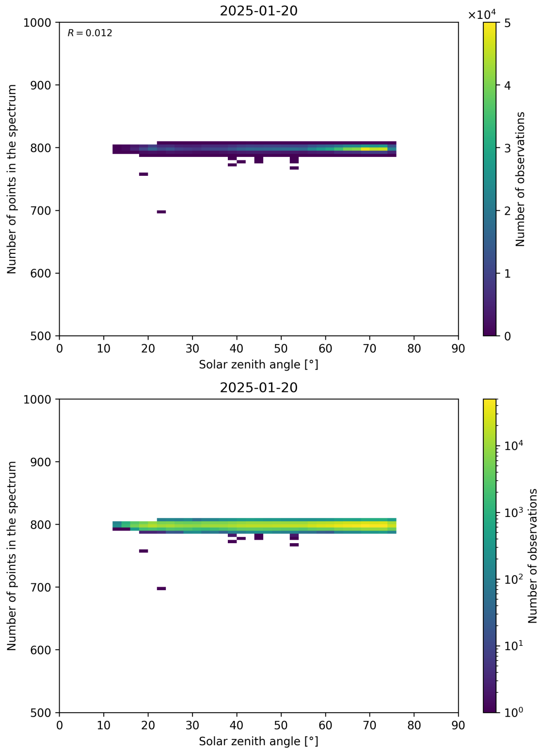
Figure 103: Scatter density plot of “Solar zenith angle” against “Number of points in the spectrum” for 2025-01-19 to 2025-01-21.
