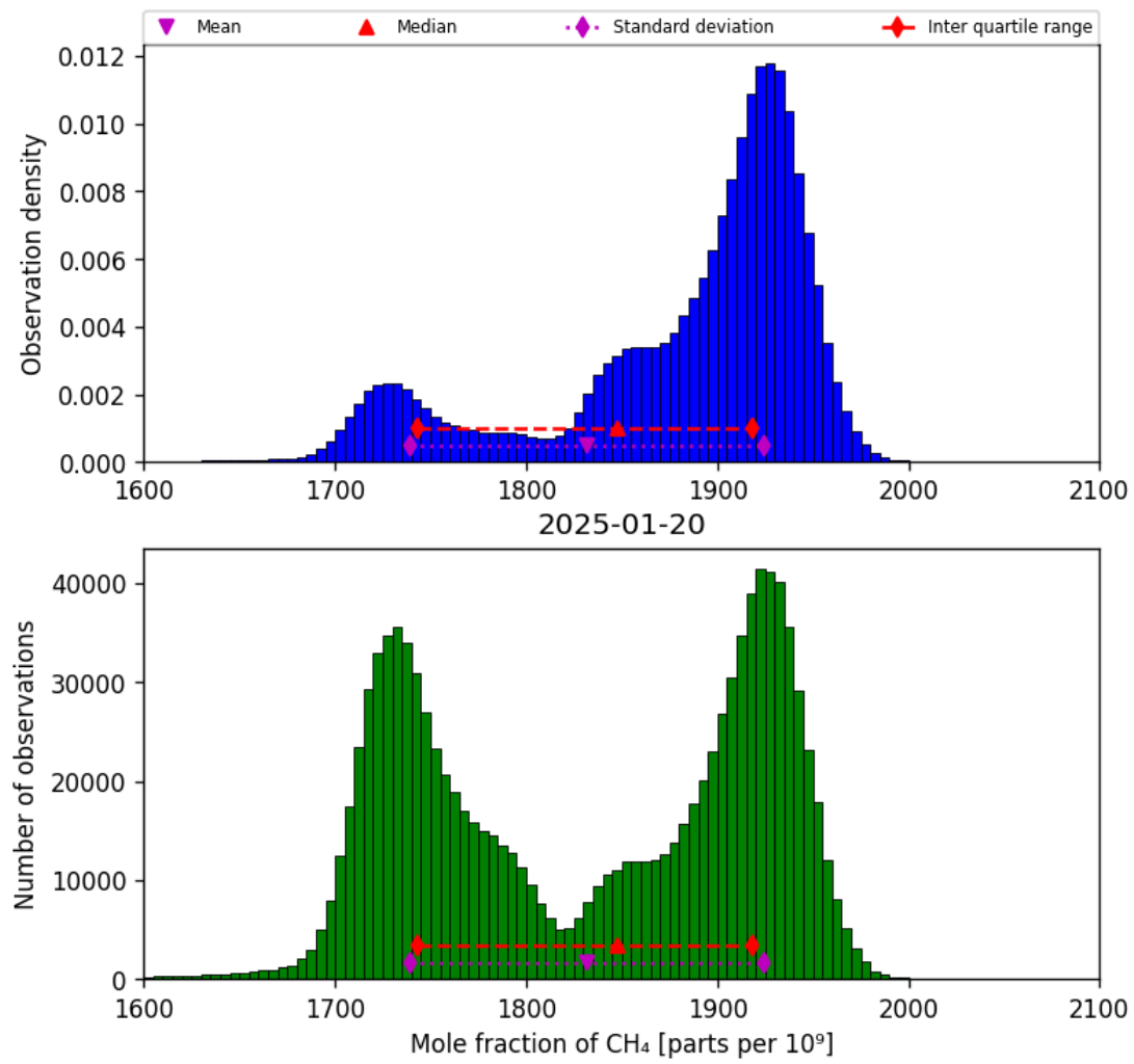
Figure 23: Histogram of “Mole fraction of CH 4 ” for 2025-01-19 to 2025-01-21
