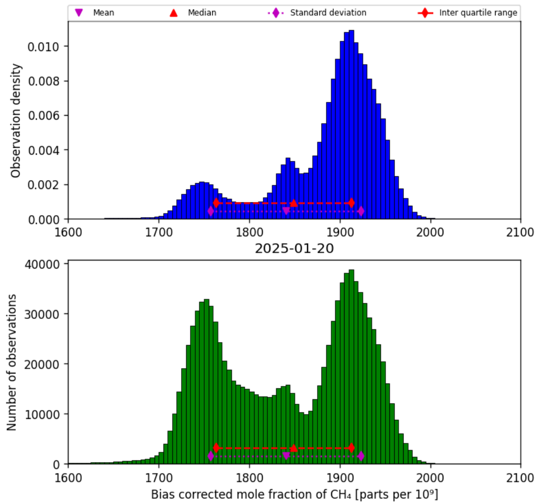
Figure 25: Histogram of “Bias corrected mole fraction of CH 4 ” for 2025-01-19 to 2025-01-21
