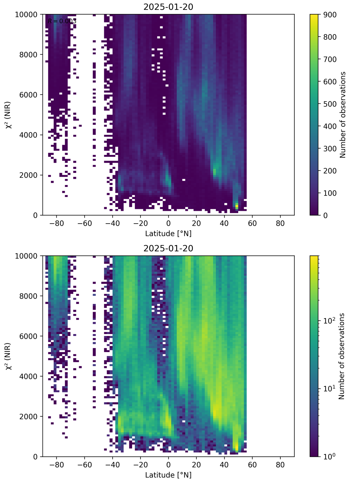
Figure 53: Scatter density plot of “Latitude” against “ \chi^2 (NIR)” for 2025-01-19 to 2025-01-21.
