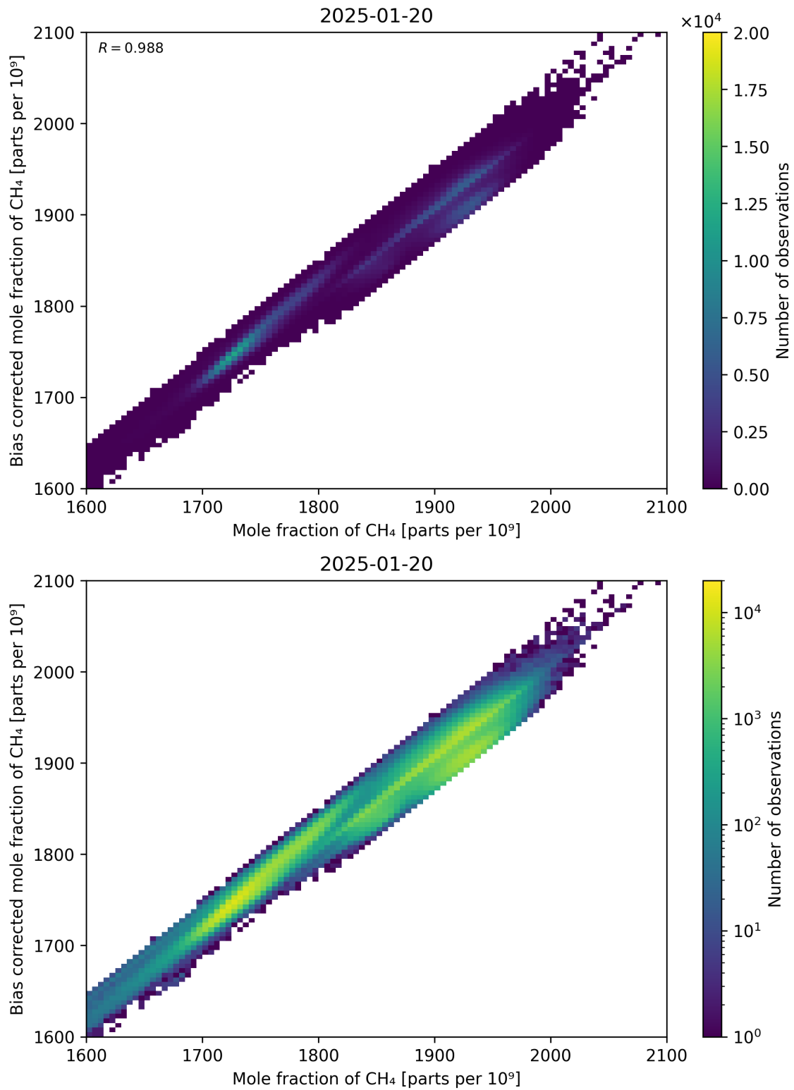
Figure 74: Scatter density plot of “Mole fraction of CH 4 ” against “Bias corrected mole fraction of CH 4 ” for 2025-01-19 to 2025-01-21.
