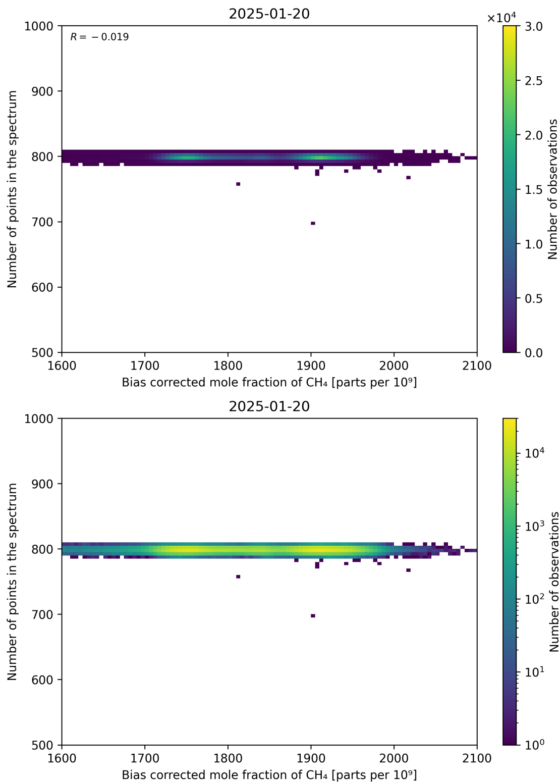
Figure 68: Scatter density plot of “Bias corrected mole fraction of CH 4 ” against “Number of points in the spectrum” for 2025-01-19 to 2025-01-21.
