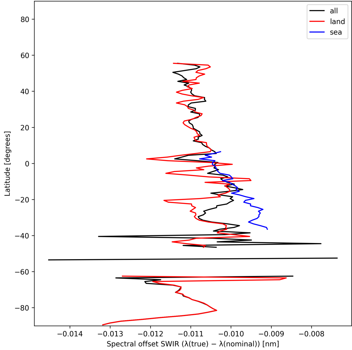
Figure 16: Zonal average of “Spectral offset SWIR ( \lambda_{\text{true}} - \lambda_{\text{nominal}} )” for 2025-01-19 to 2025-01-21.
