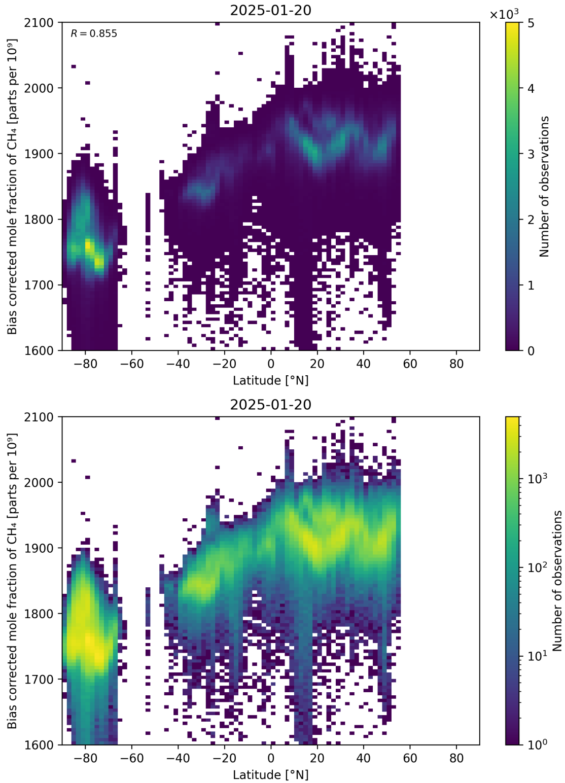
Figure 58: Scatter density plot of “Latitude” against “Bias corrected mole fraction of CH 4 ” for 2025-01-19 to 2025-01-21.
