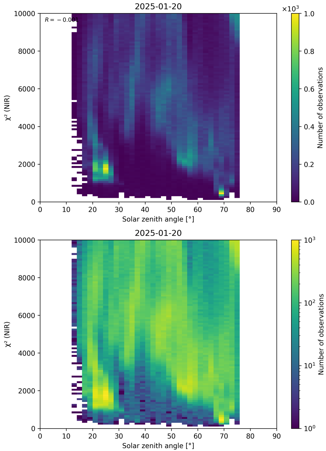
Figure 94: Scatter density plot of “Solar zenith angle” against “ \chi^2 (NIR)” for 2025-01-19 to 2025-01-21.
