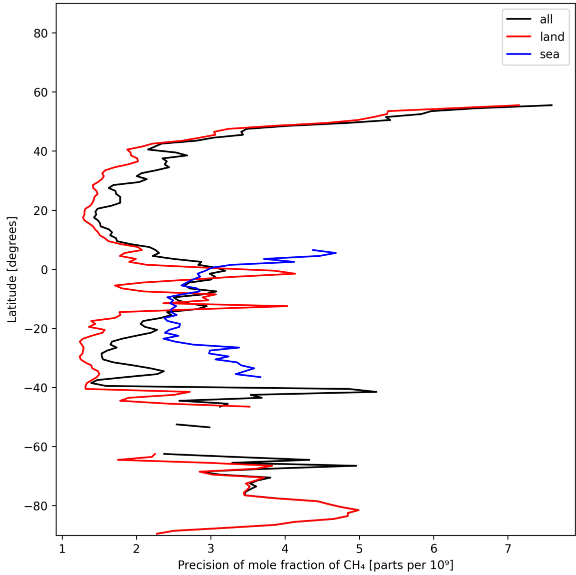
Figure 13: Zonal average of “Precision of mole fraction of CH 4 ” for 2025-01-19 to 2025-01-21.
