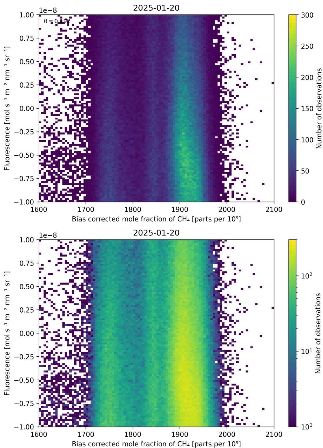
Figure 66: Scatter density plot of “Bias corrected mole fraction of \text{CH}_4 ” against “Fluorescence” for 2025-01-19 to 2025-01-21.
