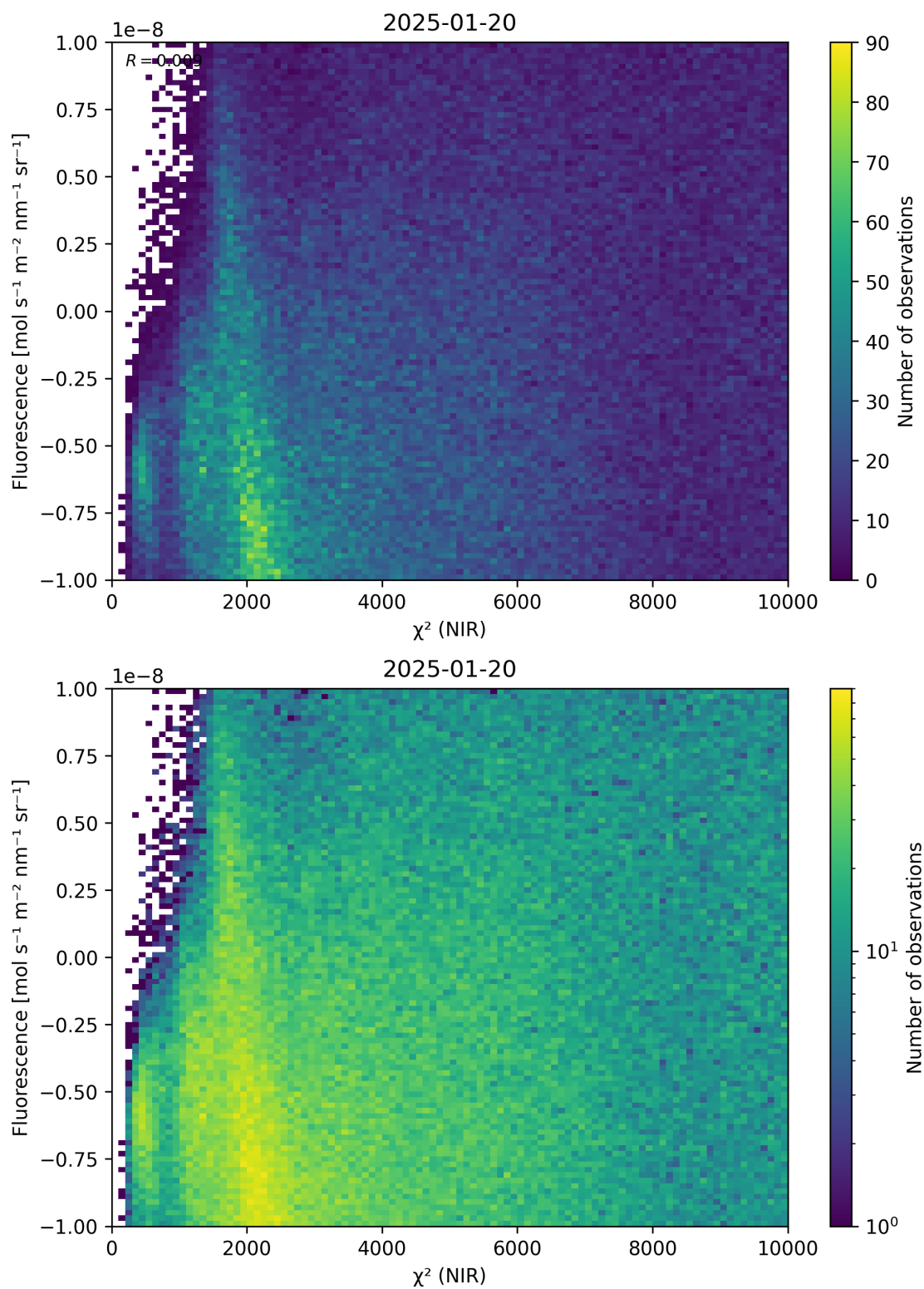
Figure 45: Scatter density plot of “ \chi^2 (NIR)” against “Fluorescence” for 2025-01-19 to 2025-01-21.
