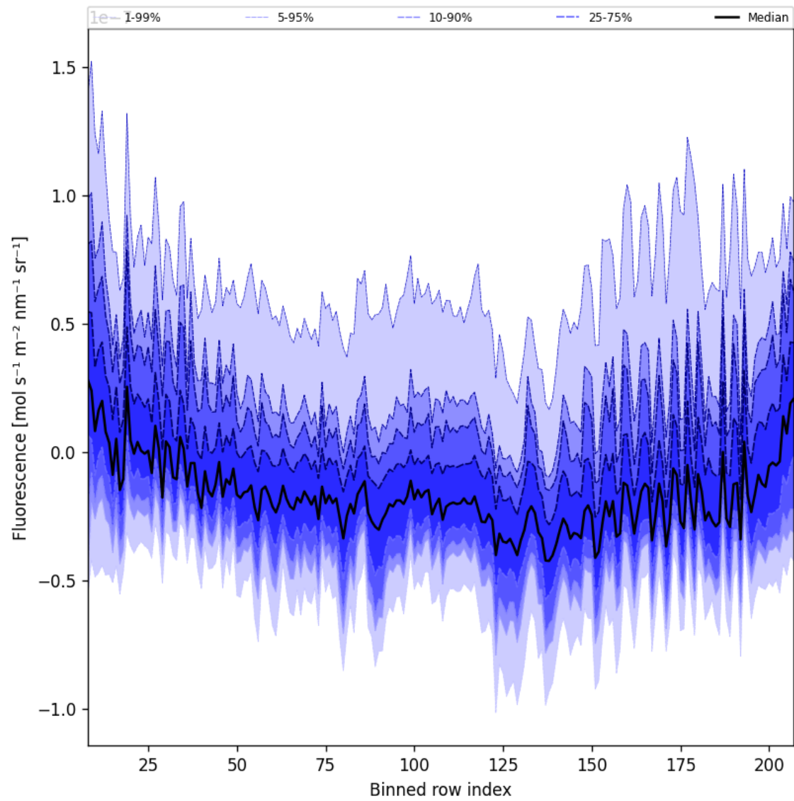
Figure 43: Along track statistics of “Fluorescence” for 2025-01-19 to 2025-01-21
