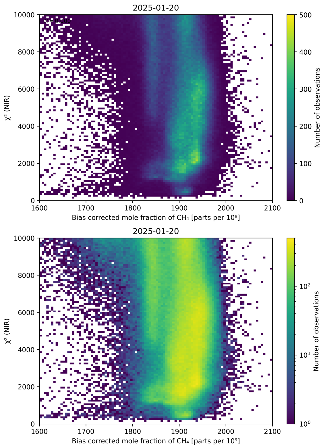
Figure 63: Scatter density plot of “Bias corrected mole fraction of \text{CH}_4 ” against “ \chi^2 (NIR)” for 2025-01-19 to 2025-01-21.
