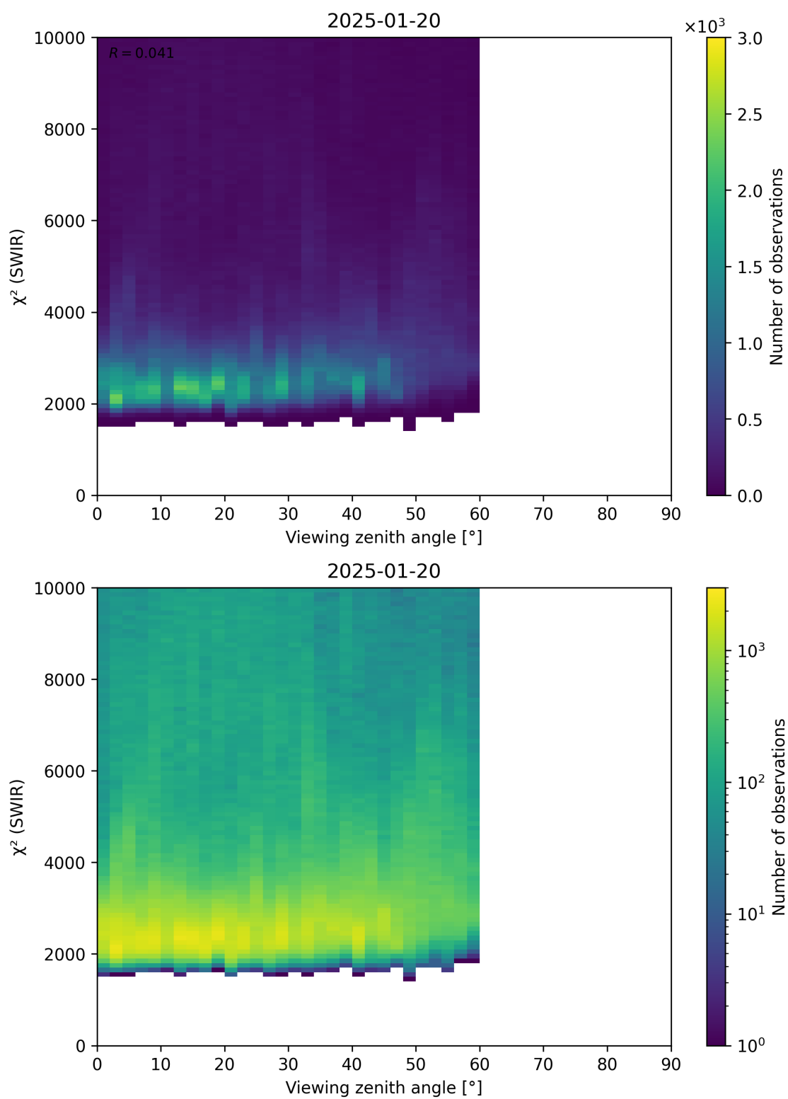
Figure 106: Scatter density plot of “Viewing zenith angle” against “ \chi^2 (SWIR)” for 2025-01-19 to 2025-01-21.
