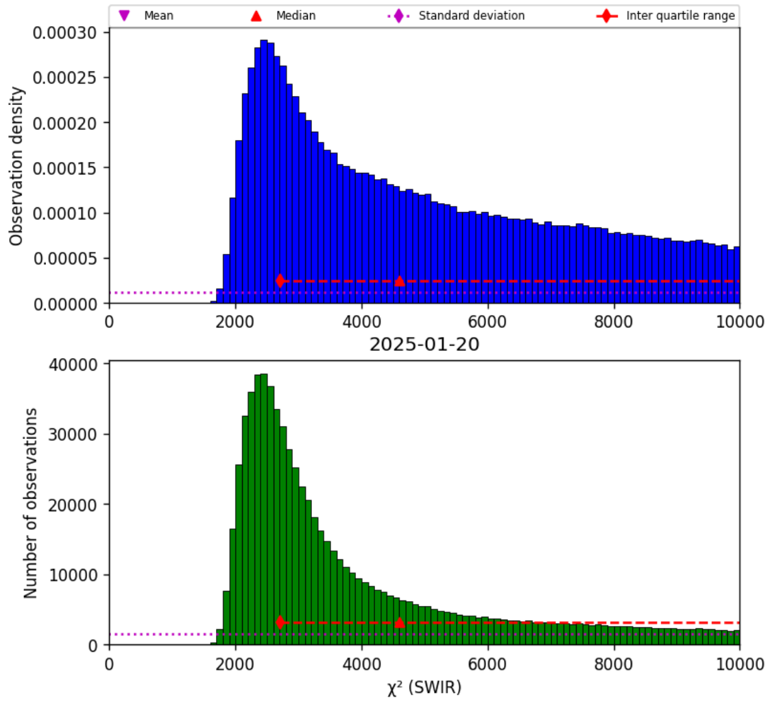
Figure 28: Histogram of " \chi^2 (SWIR)" for 2025-01-19 to 2025-01-21
