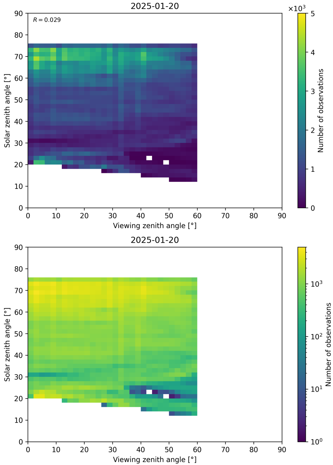
Figure 115: Scatter density plot of “Viewing zenith angle” against “Solar zenith angle” for 2025-01-19 to 2025-01-21.
