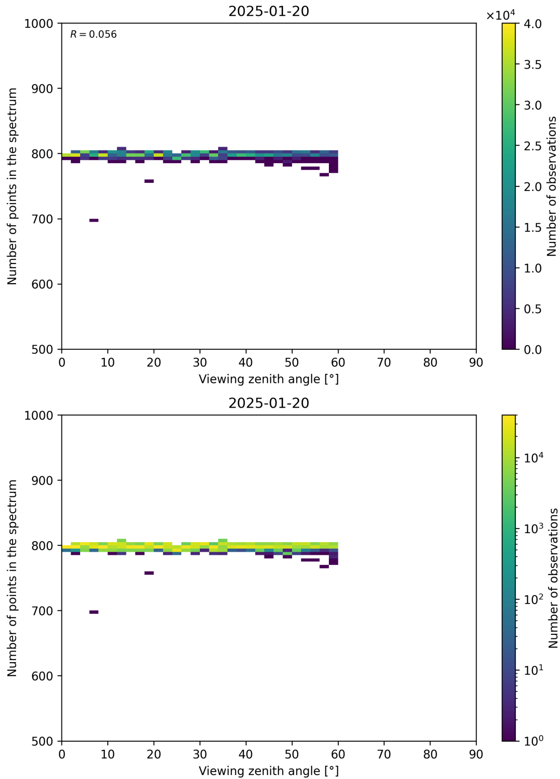
Figure 114: Scatter density plot of “Viewing zenith angle” against “Number of points in the spectrum” for 2025-01-19 to 2025-01-21.
