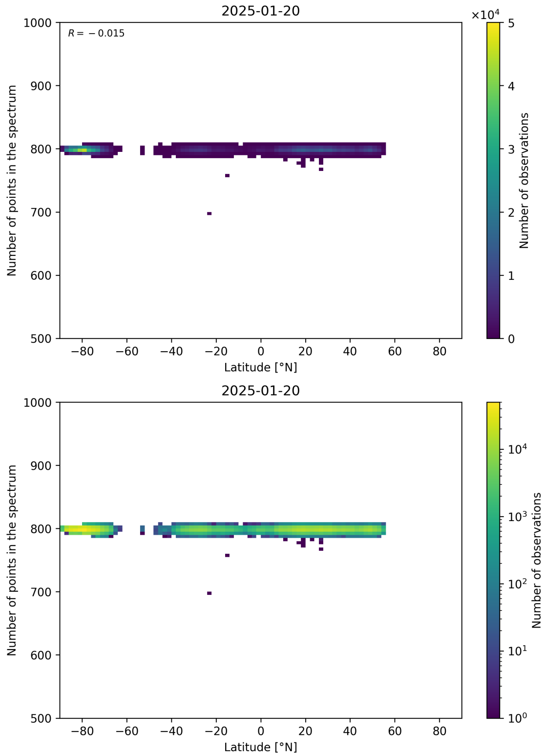
Figure 61: Scatter density plot of “Latitude” against “Number of points in the spectrum” for 2025-01-19 to 2025-01-21.
