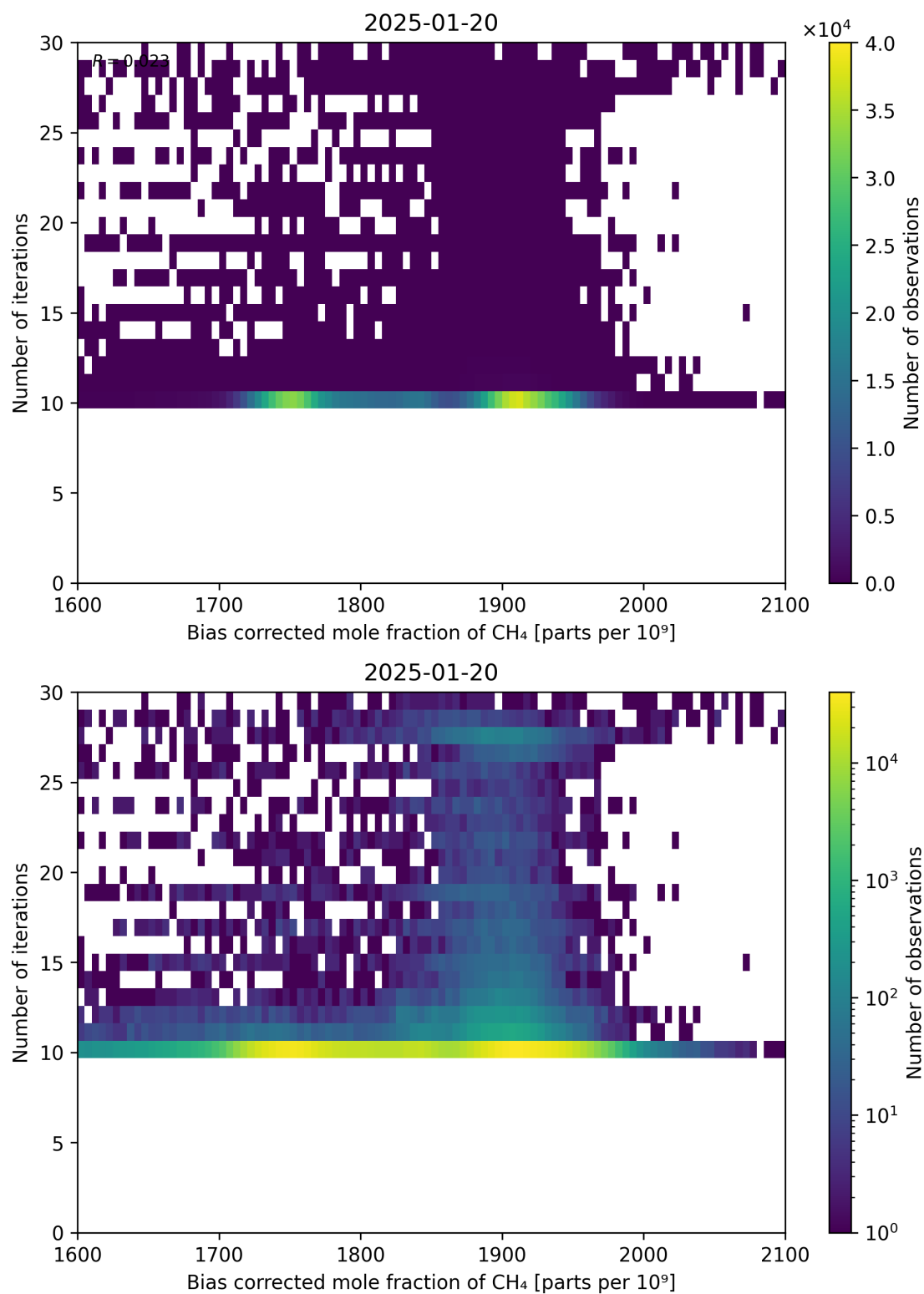
Figure 67: Scatter density plot of “Bias corrected mole fraction of \text{CH}_4 ” against “Number of iterations” for 2025-01-19 to 2025-01-21.
