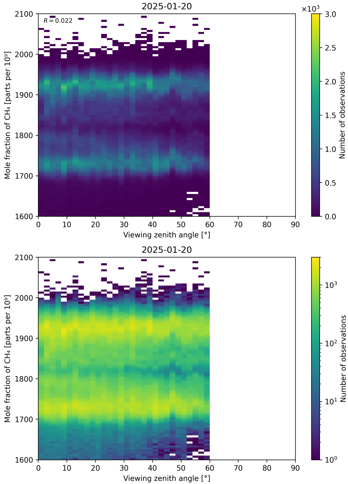
Figure 110: Scatter density plot of “Viewing zenith angle” against “Mole fraction of CH 4 ” for 2025-01-19 to 2025-01-21.
