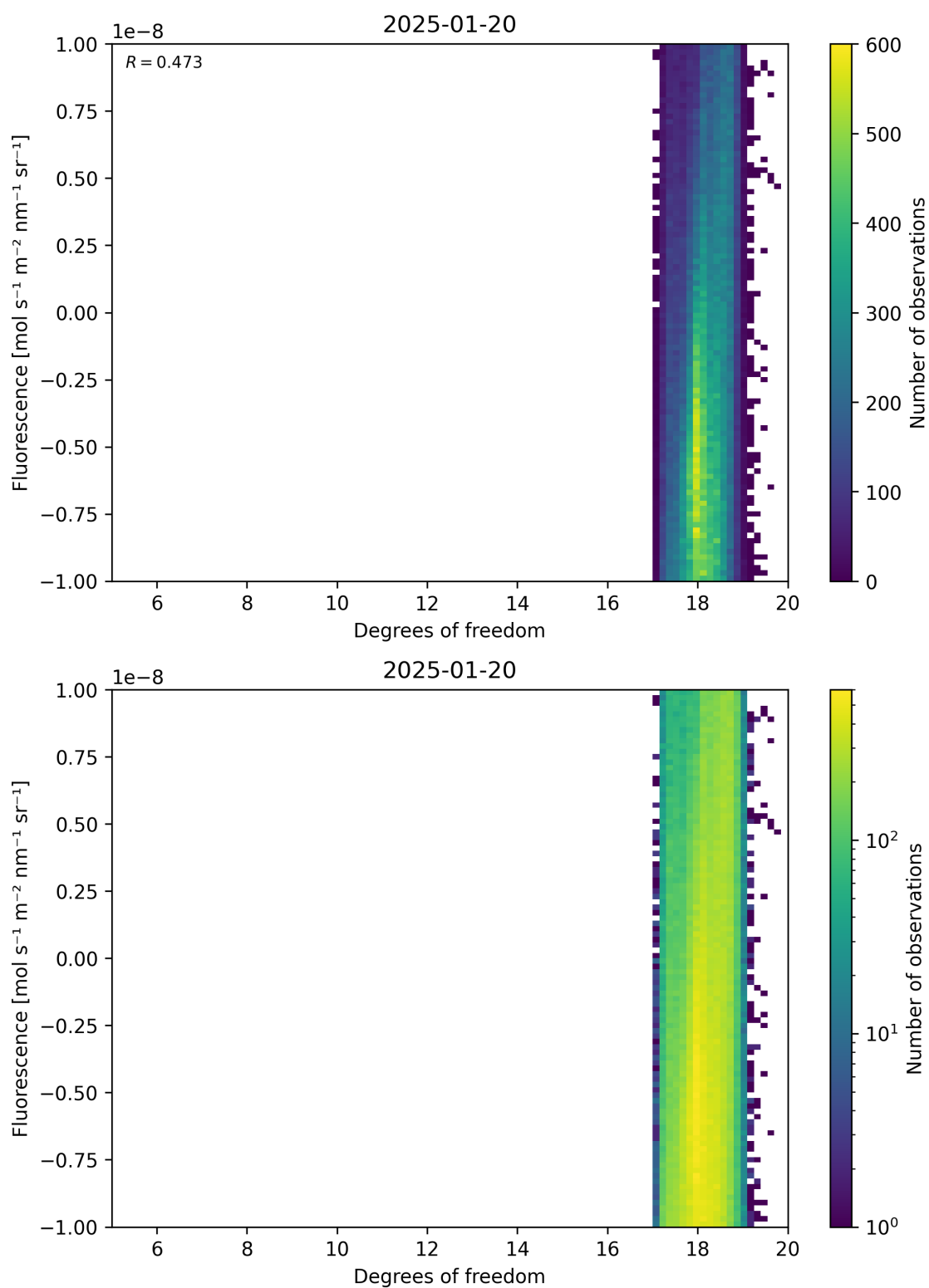
Figure 51: Scatter density plot of “Degrees of freedom” against “Fluorescence” for 2025-01-19 to 2025-01-21.
