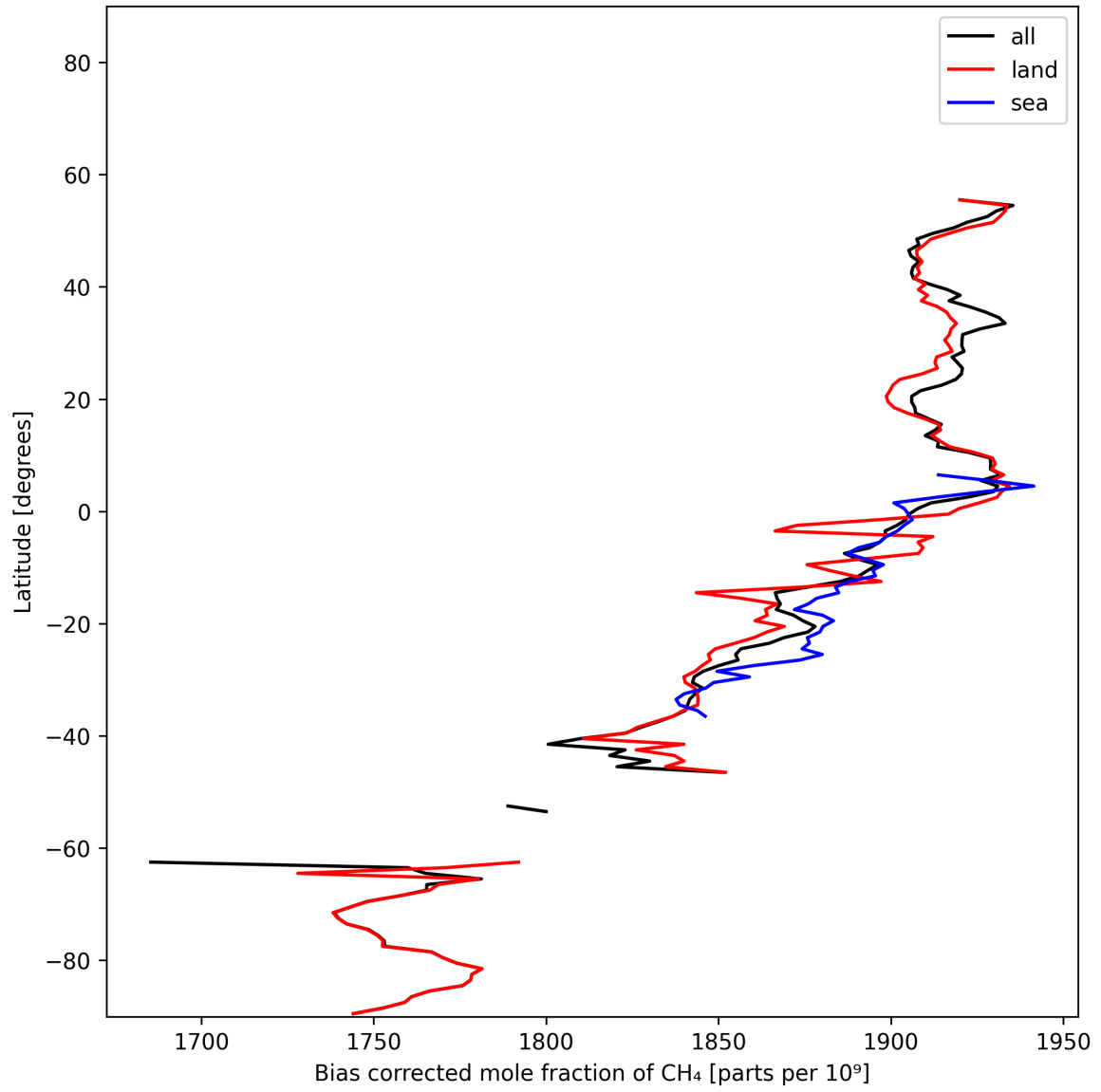
Figure 14: Zonal average of “Bias corrected mole fraction of CH 4 ” for 2025-01-19 to 2025-01-21.
