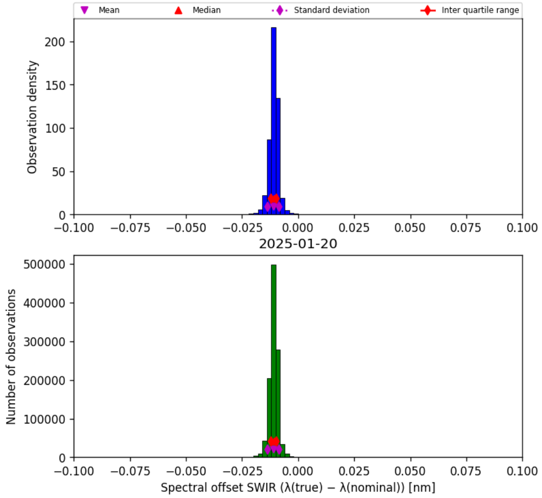
Figure 27: Histogram of “Spectral offset SWIR ( \lambda_{\text{true}} - \lambda_{\text{nominal}} )” for 2025-01-19 to 2025-01-21
