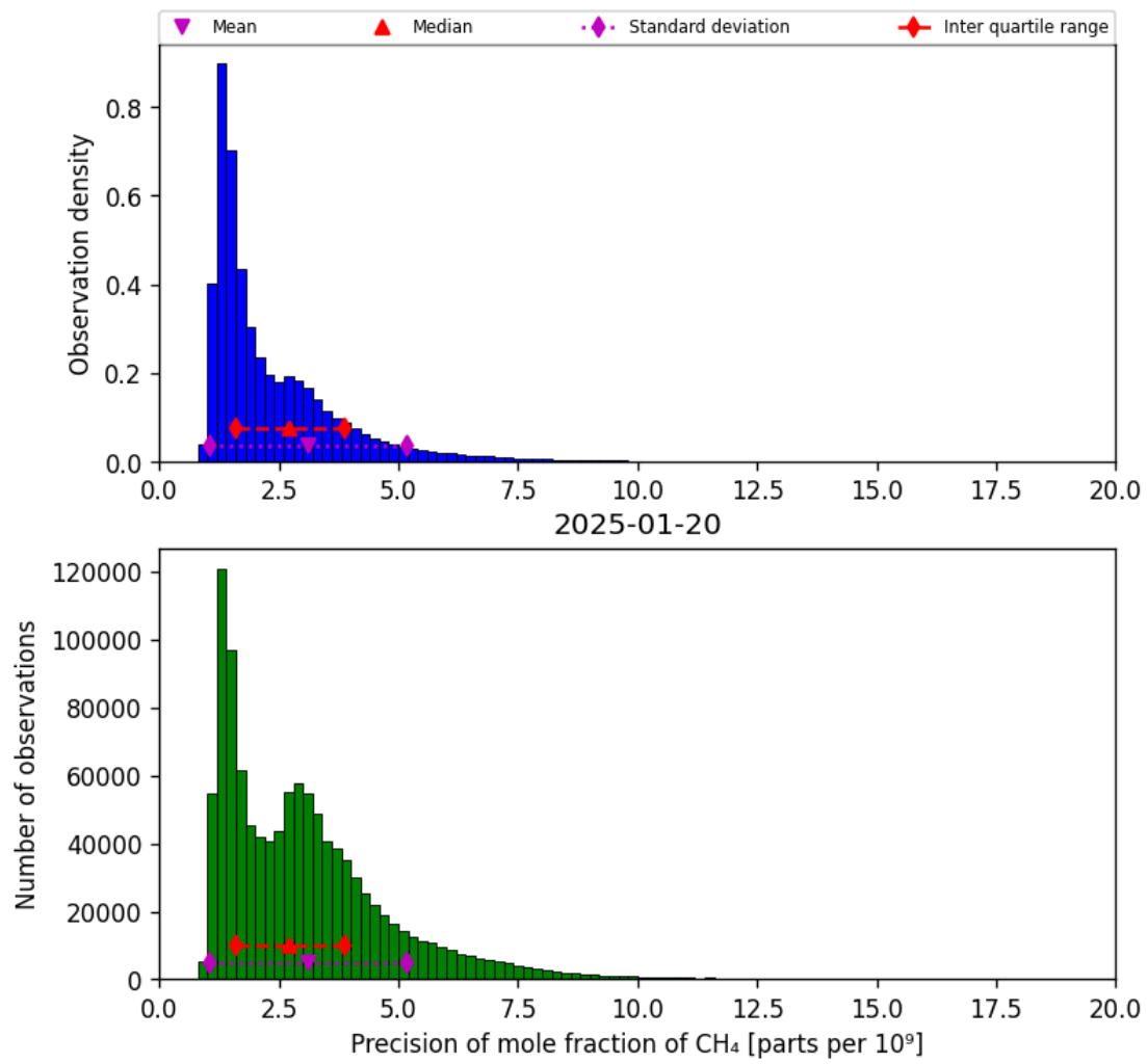
Figure 24: Histogram of “Precision of mole fraction of CH 4 ” for 2025-01-19 to 2025-01-21
