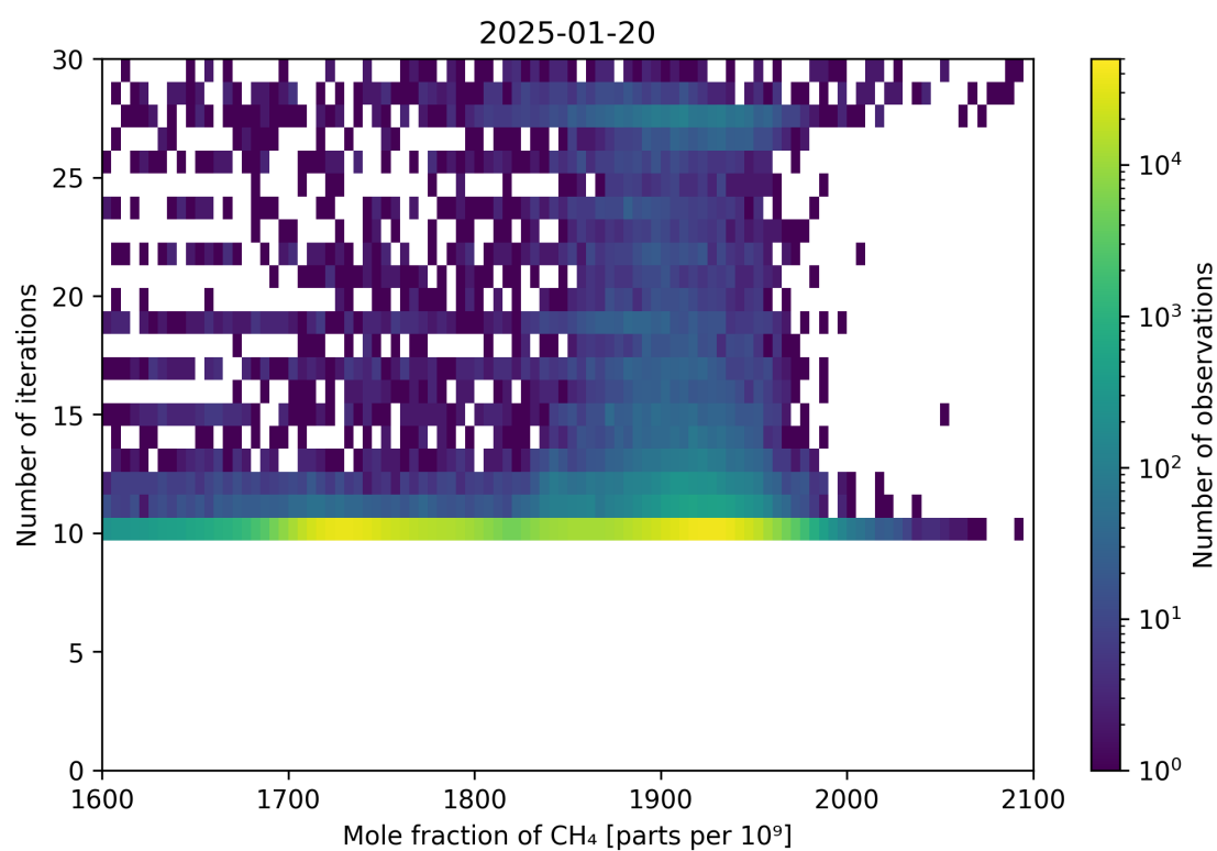
Figure 76: Scatter density plot of “Mole fraction of CH 4 ” against “Number of iterations” for 2025-01-19 to 2025-01-21.
