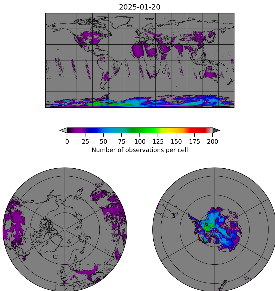
Figure 10: Map of the number of observations for 2025-01-19 to 2025-01-21
