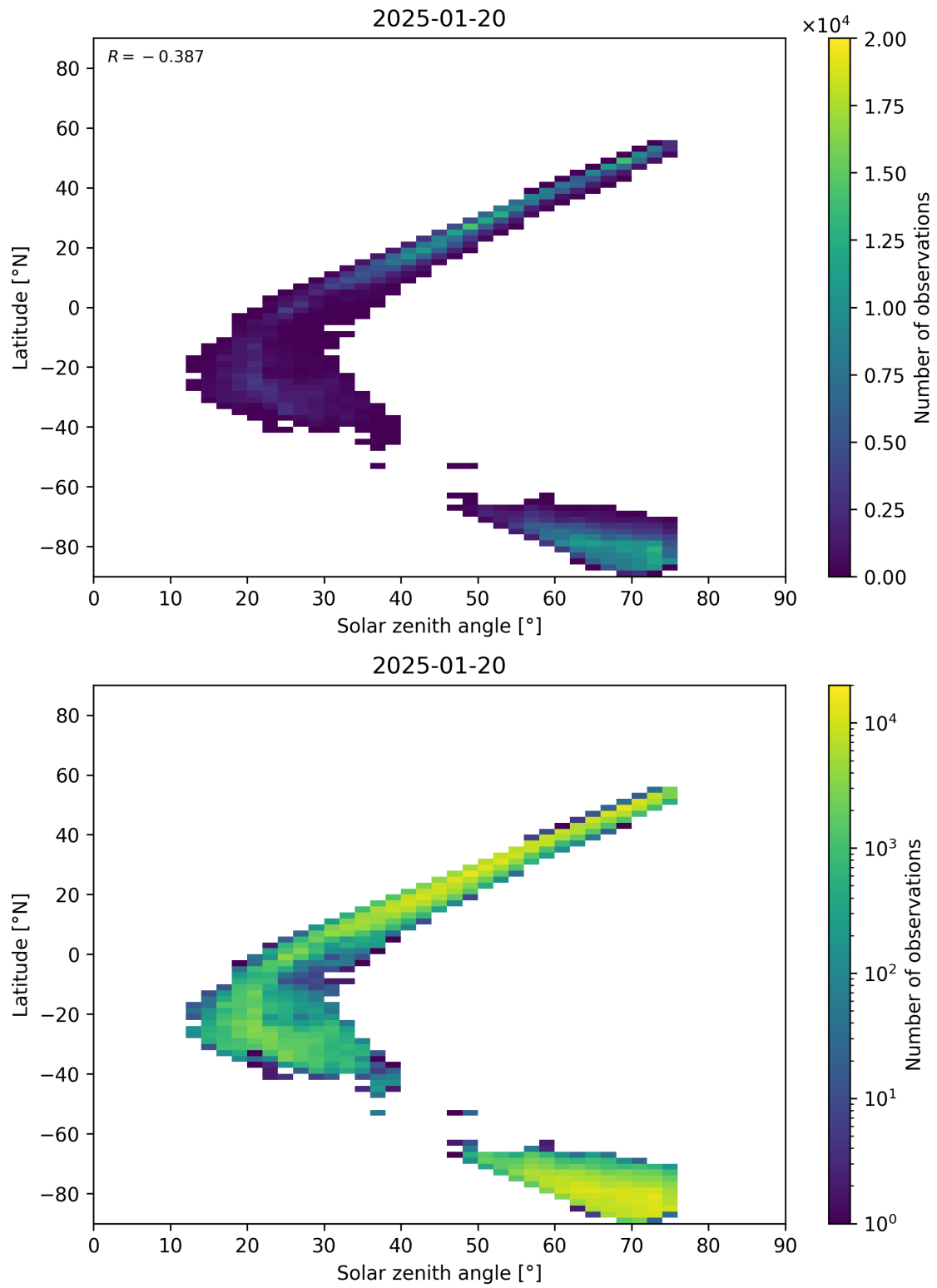
Figure 98: Scatter density plot of “Solar zenith angle” against “Latitude” for 2025-01-19 to 2025-01-21.
