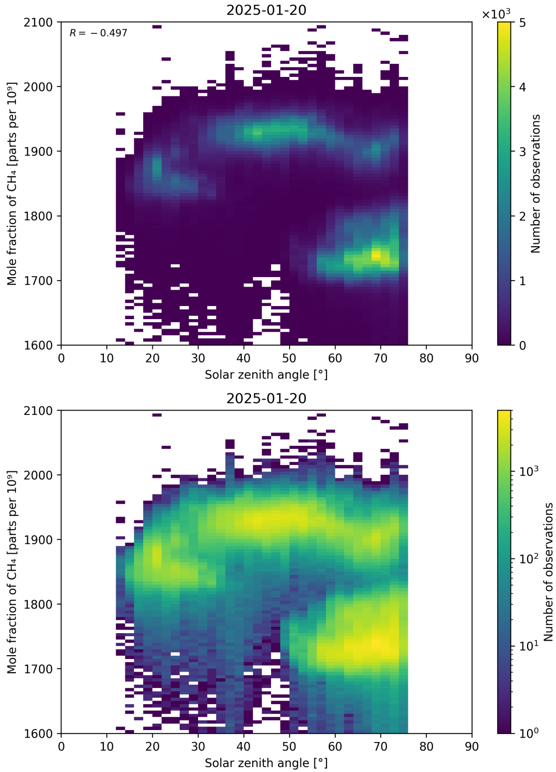
Figure 99: Scatter density plot of “Solar zenith angle” against “Mole fraction of CH 4 ” for 2025-01-19 to 2025-01-21.
