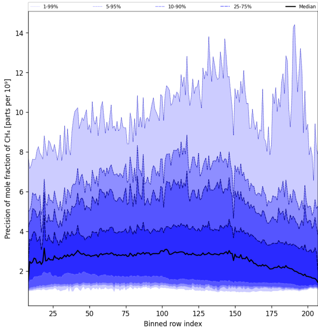
Figure 35: Along track statistics of “Precision of mole fraction of CH 4 ” for 2025-01-19 to 2025-01-21
