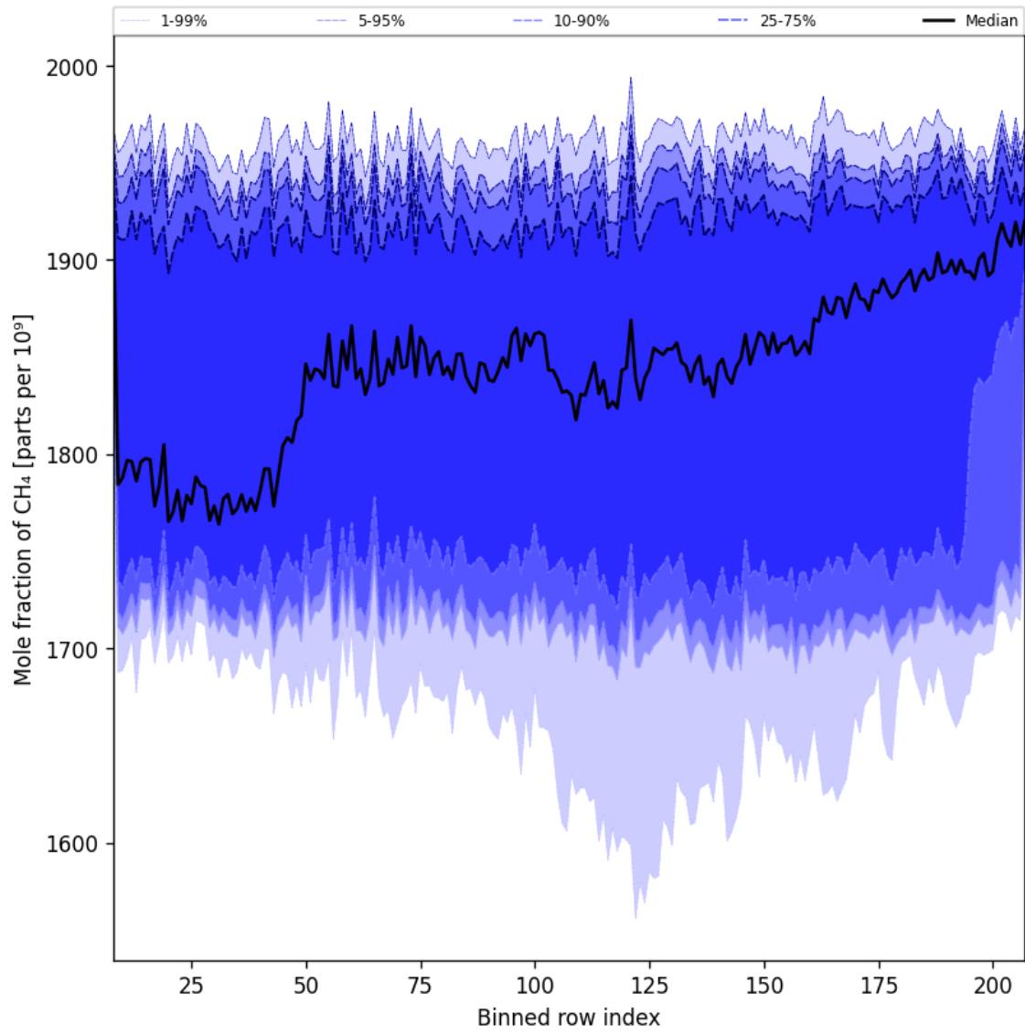
Figure 34: Along track statistics of “Mole fraction of CH 4 ” for 2025-01-19 to 2025-01-21
