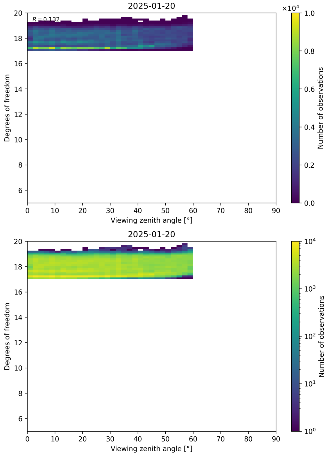
Figure 107: Scatter density plot of “Viewing zenith angle” against “Degrees of freedom” for 2025-01-19 to 2025-01-21.
