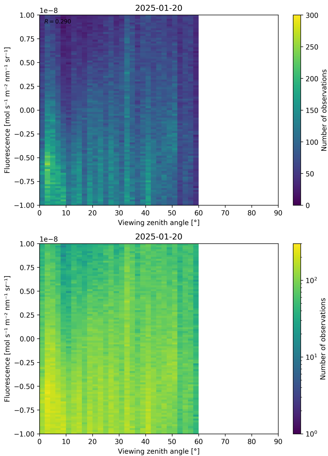
Figure 108: Scatter density plot of “Viewing zenith angle” against “Fluorescence” for 2025-01-19 to 2025-01-21.
