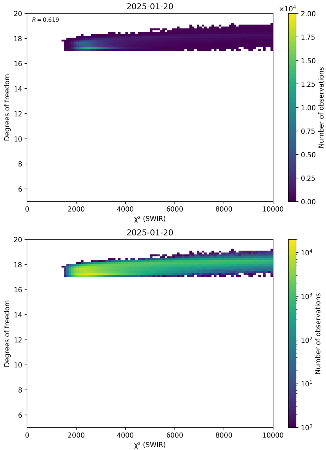
Figure 48: Scatter density plot of “ \chi^2 (SWIR)” against “Degrees of freedom” for 2025-01-19 to 2025-01-21.
