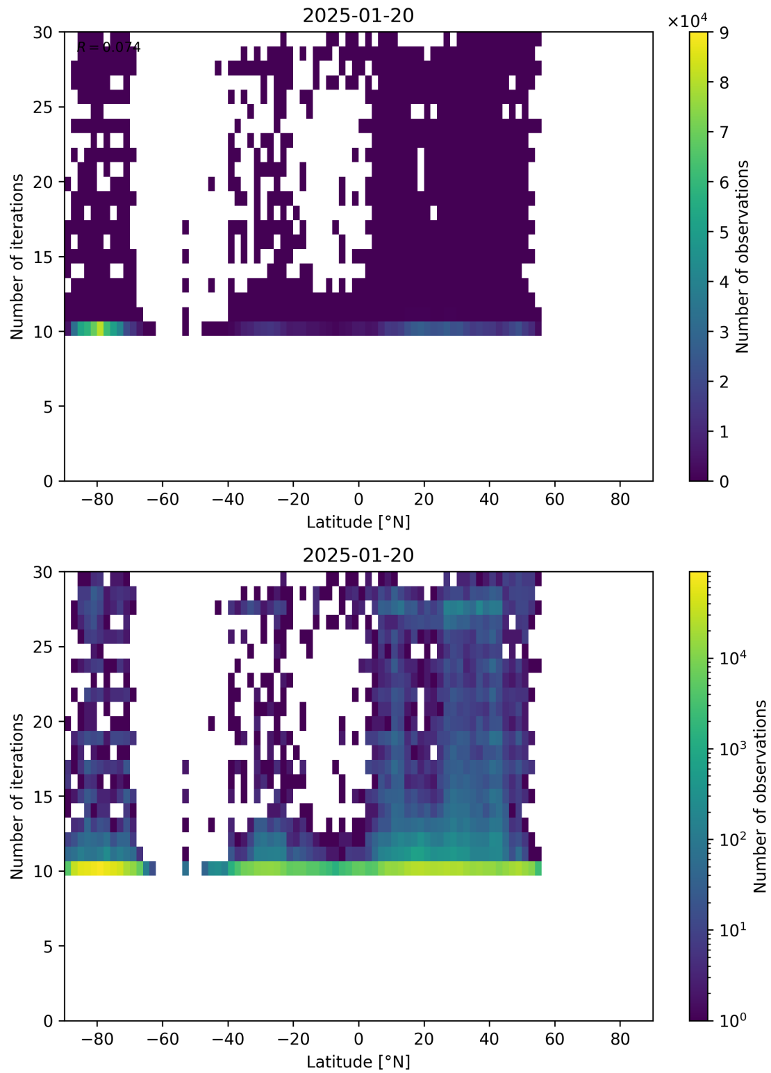
Figure 60: Scatter density plot of “Latitude” against “Number of iterations” for 2025-01-19 to 2025-01-21.
