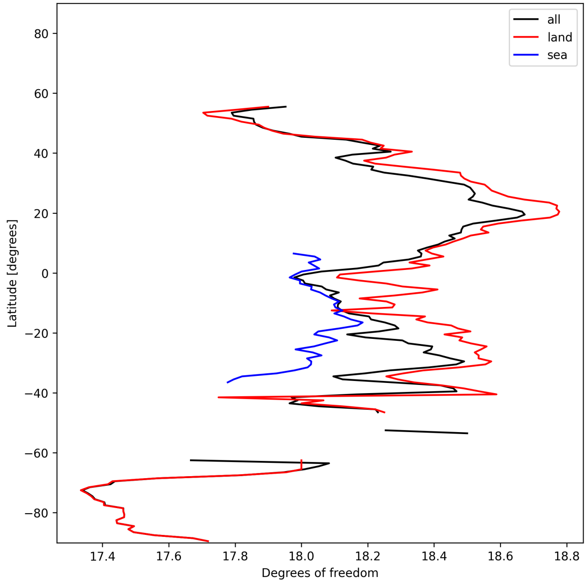
Figure 19: Zonal average of “Degrees of freedom” for 2025-01-19 to 2025-01-21.
