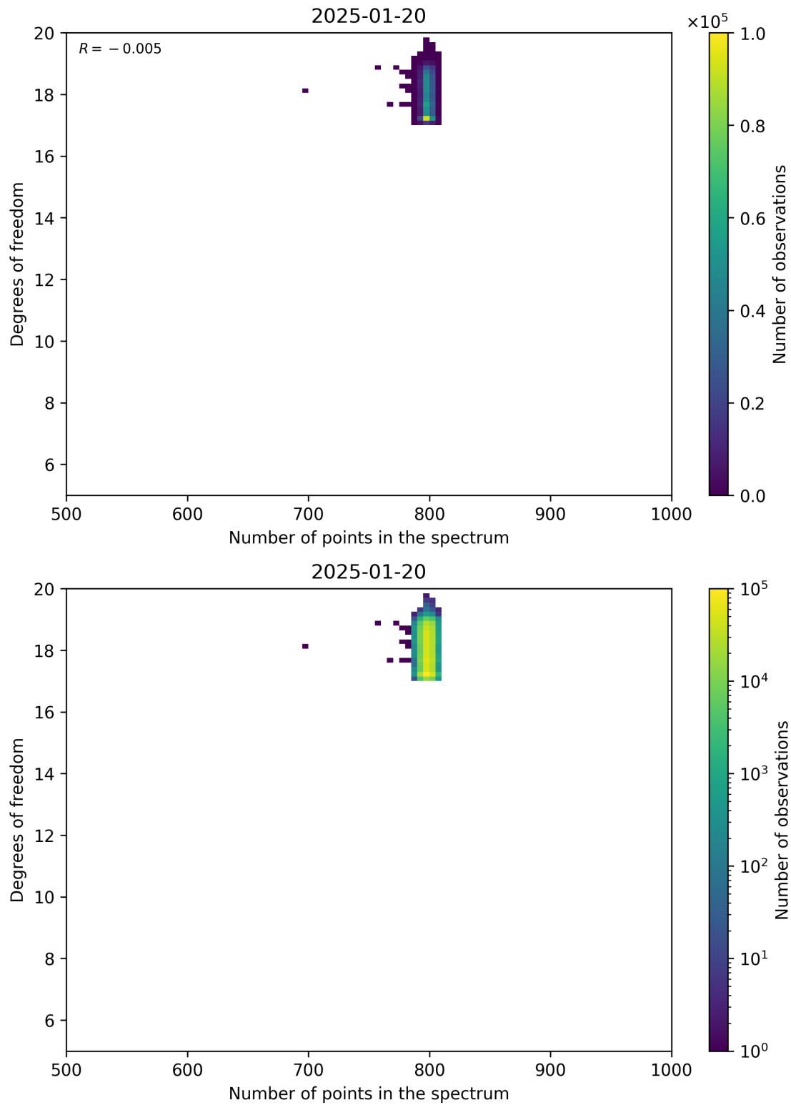
Figure 90: Scatter density plot of “Number of points in the spectrum” against “Degrees of freedom” for 2025-01-19 to 2025-01-21.
