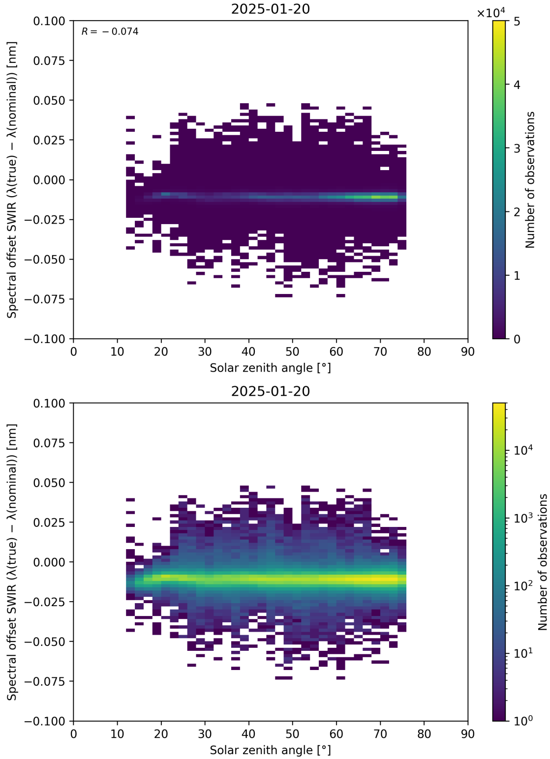
Figure 104: Scatter density plot of “Solar zenith angle” against “Spectral offset SWIR ( \lambda_{\text{true}} - \lambda_{\text{nominal}} )” for 2025-01-19 to 2025-01-21.
