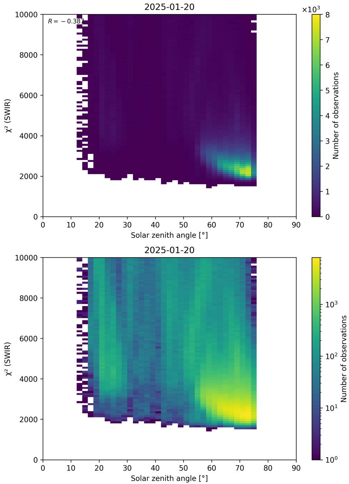
Figure 95: Scatter density plot of “Solar zenith angle” against “ \chi^2 (SWIR)” for 2025-01-19 to 2025-01-21.
