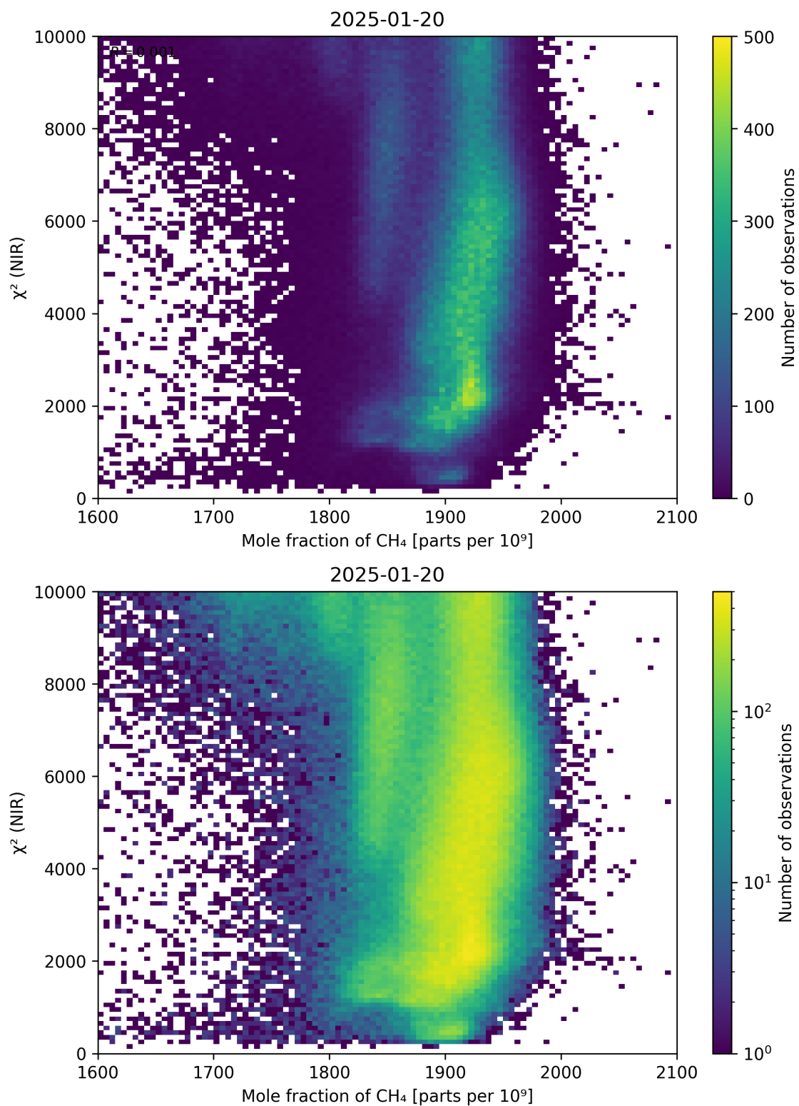
Figure 70: Scatter density plot of “Mole fraction of CH 4 ” against “ \chi^2 (NIR)” for 2025-01-19 to 2025-01-21.
