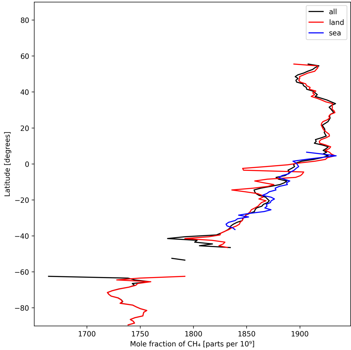
Figure 12: Zonal average of “Mole fraction of CH 4 ” for 2025-01-19 to 2025-01-21.
