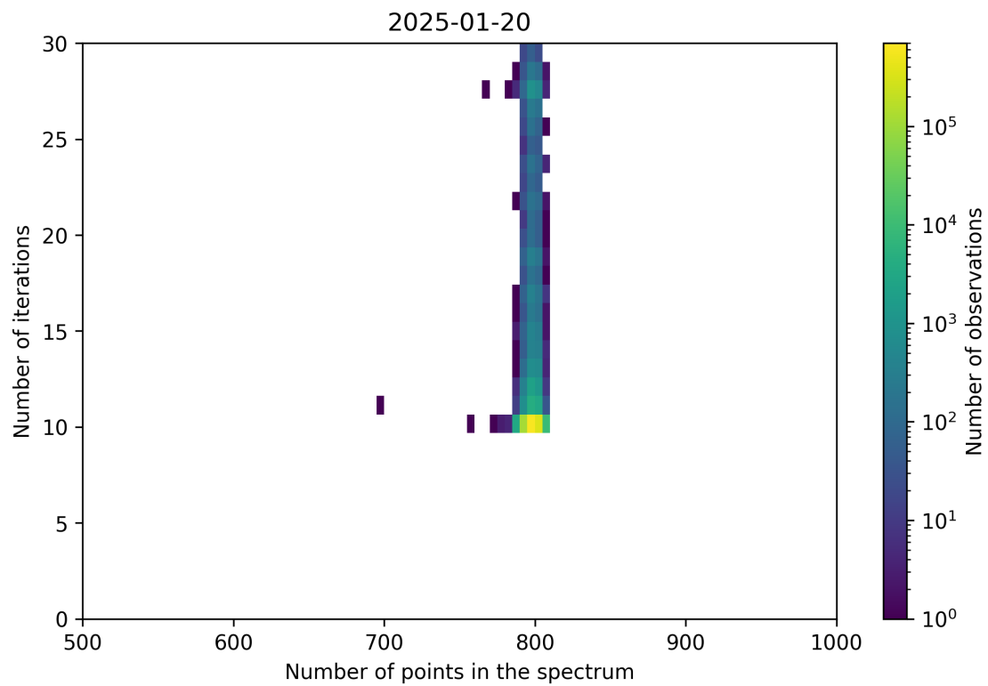
Figure 92: Scatter density plot of “Number of points in the spectrum” against “Number of iterations” for 2025-01-19 to 2025-01-21.
