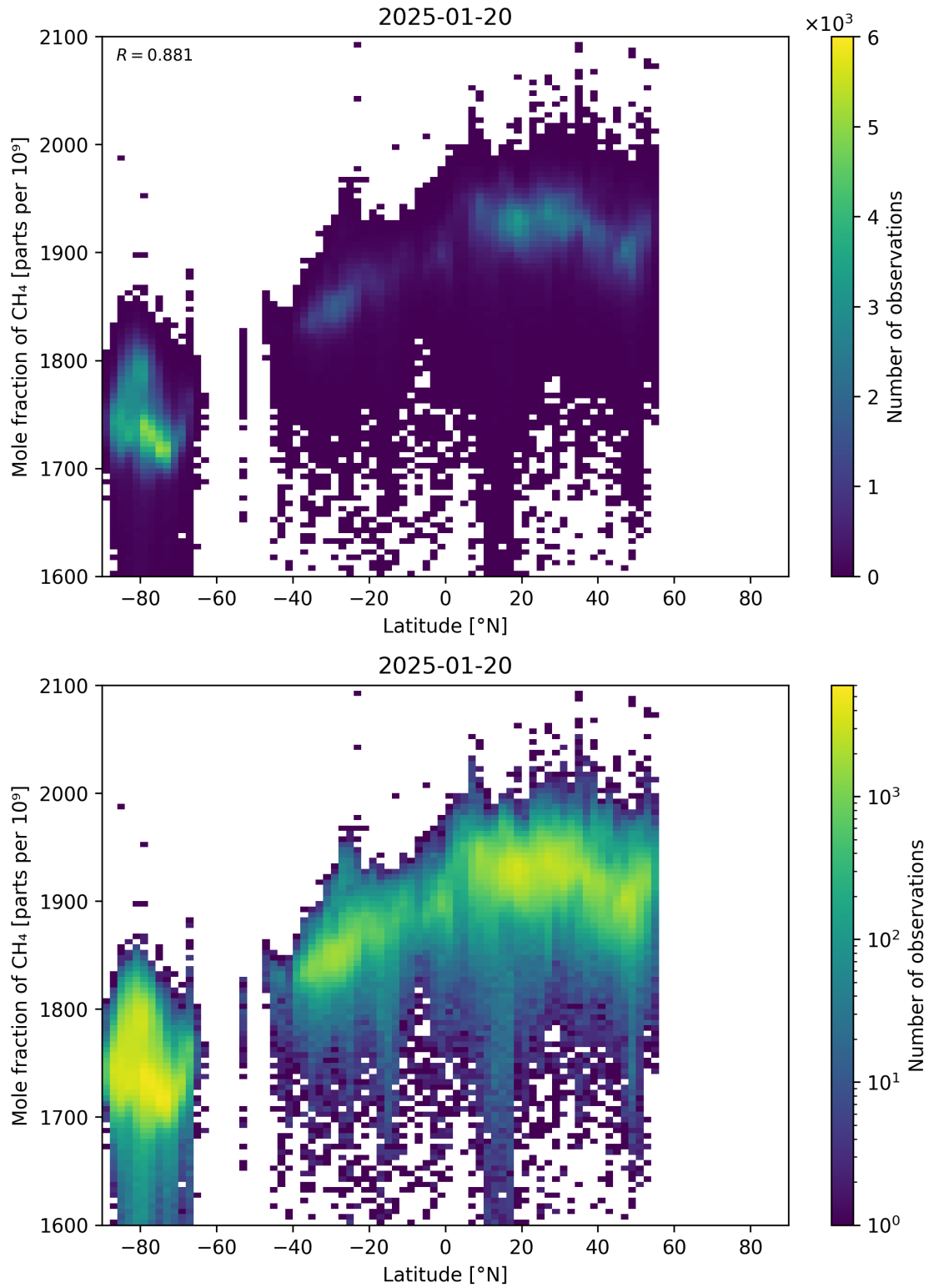
Figure 57: Scatter density plot of “Latitude” against “Mole fraction of CH 4 ” for 2025-01-19 to 2025-01-21.
