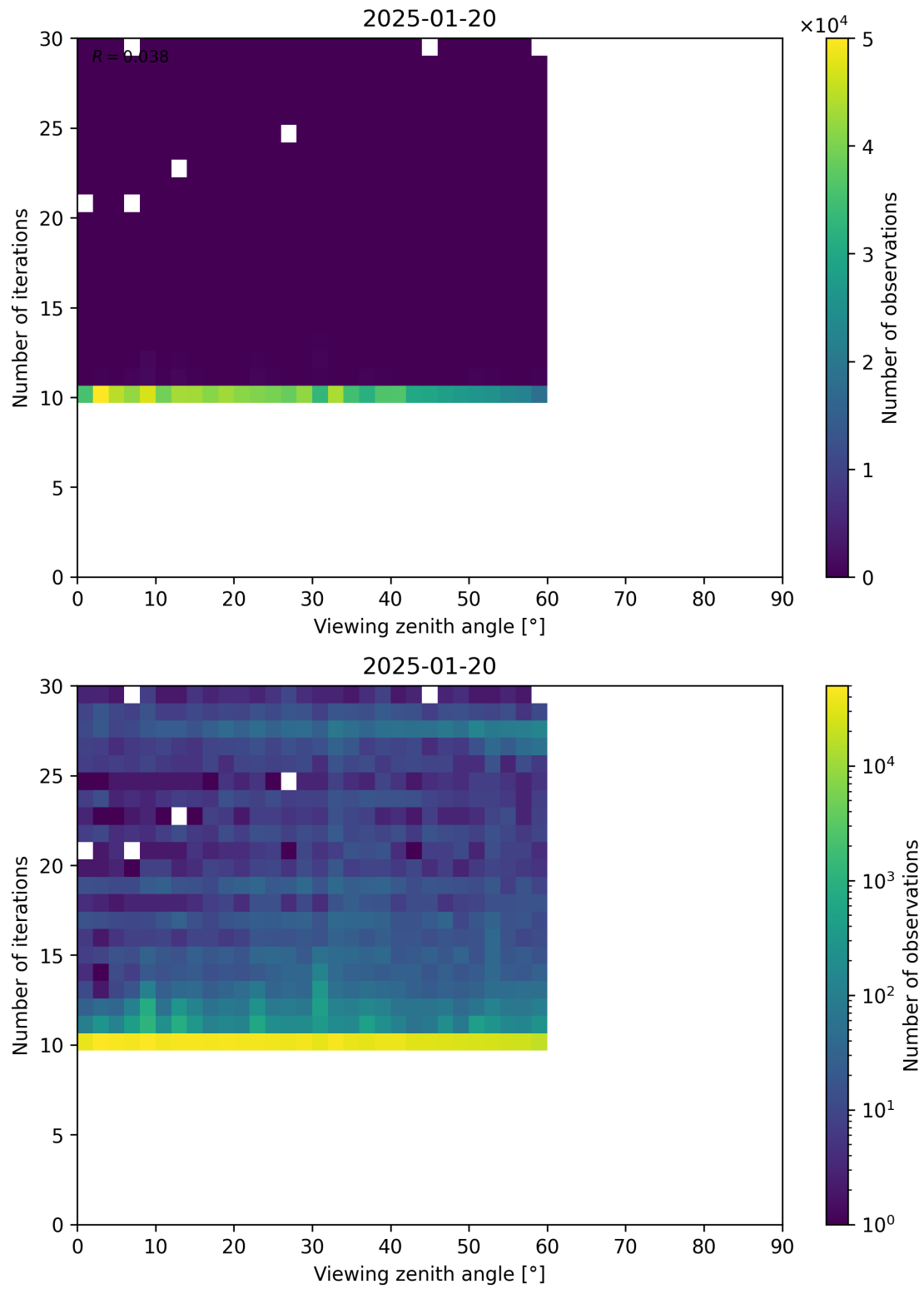
Figure 113: Scatter density plot of “Viewing zenith angle” against “Number of iterations” for 2025-01-19 to 2025-01-21.
