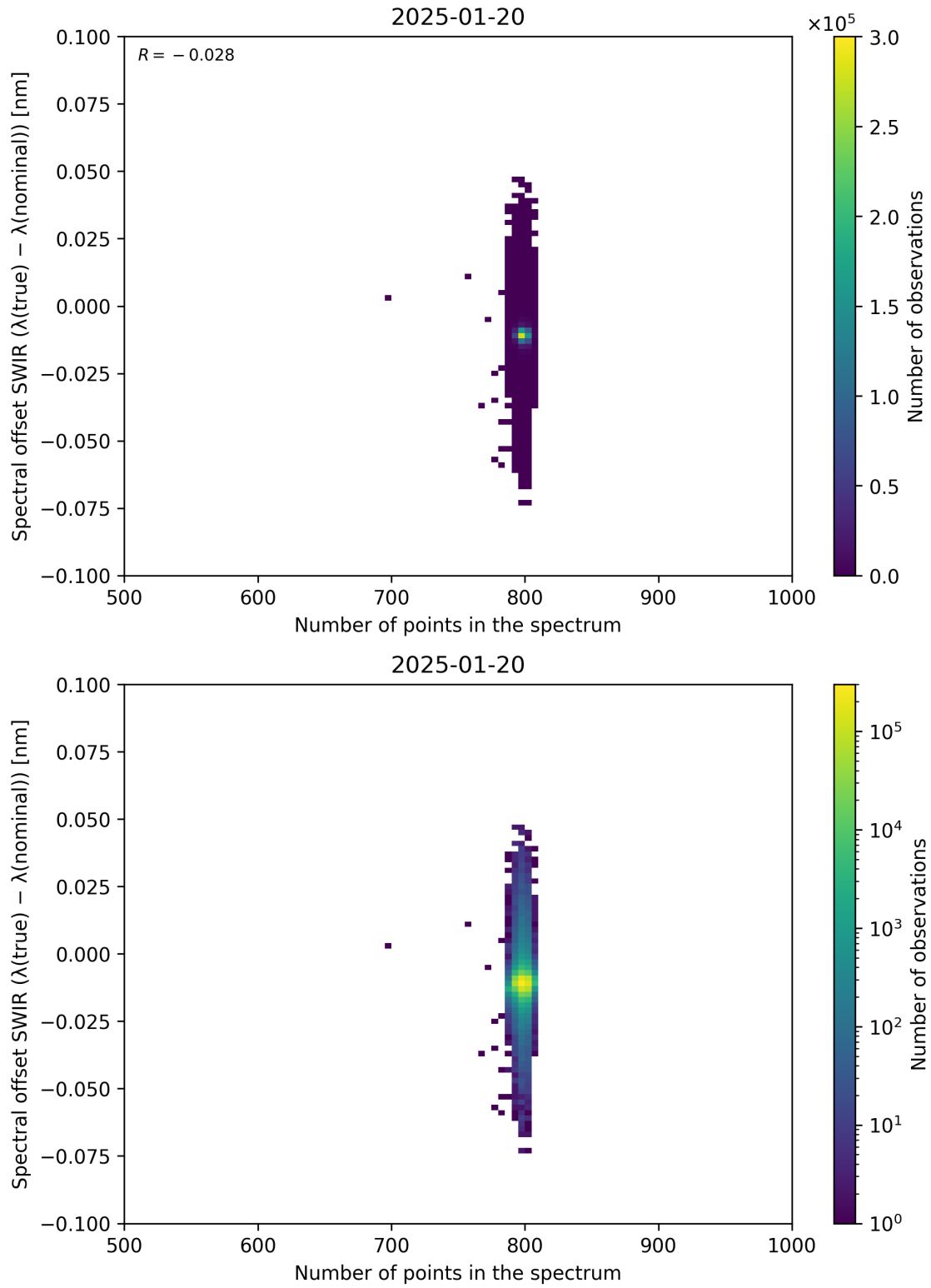
Figure 93: Scatter density plot of “Number of points in the spectrum” against “Spectral offset SWIR ( \lambda_{\text{true}} - \lambda_{\text{nominal}} )” for 2025-01-19 to 2025-01-21.
