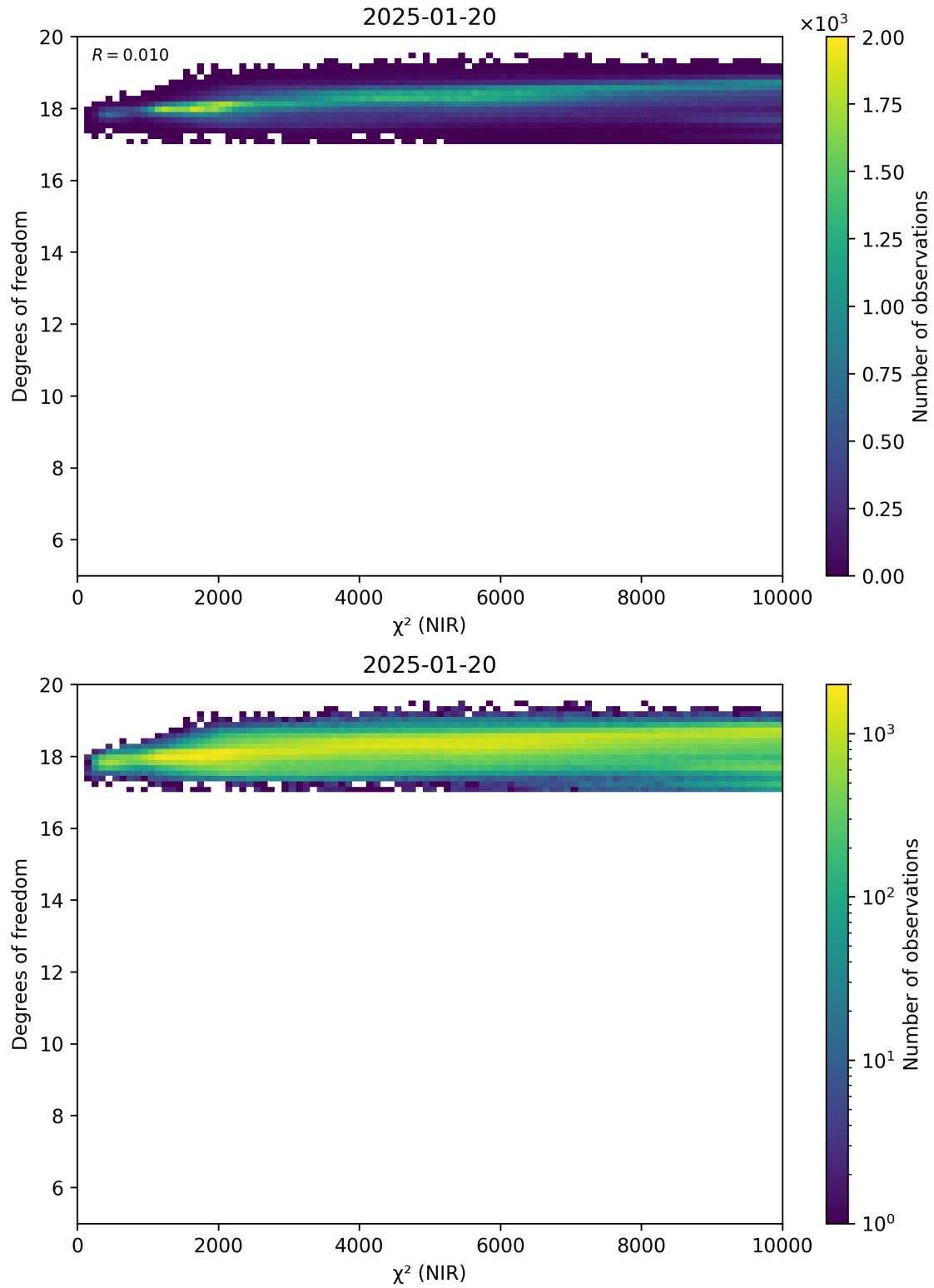
Figure 44: Scatter density plot of “ \chi^2 (NIR)” against “Degrees of freedom” for 2025-01-19 to 2025-01-21.
