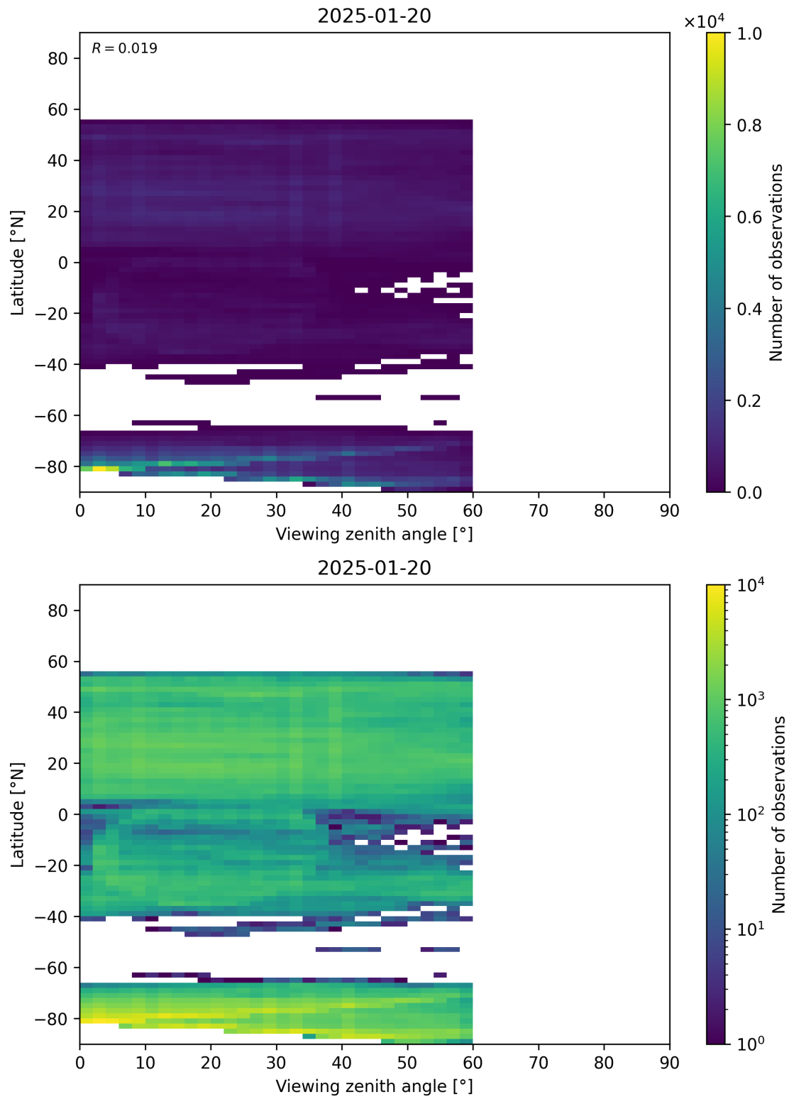
Figure 109: Scatter density plot of “Viewing zenith angle” against “Latitude” for 2025-01-19 to 2025-01-21.
