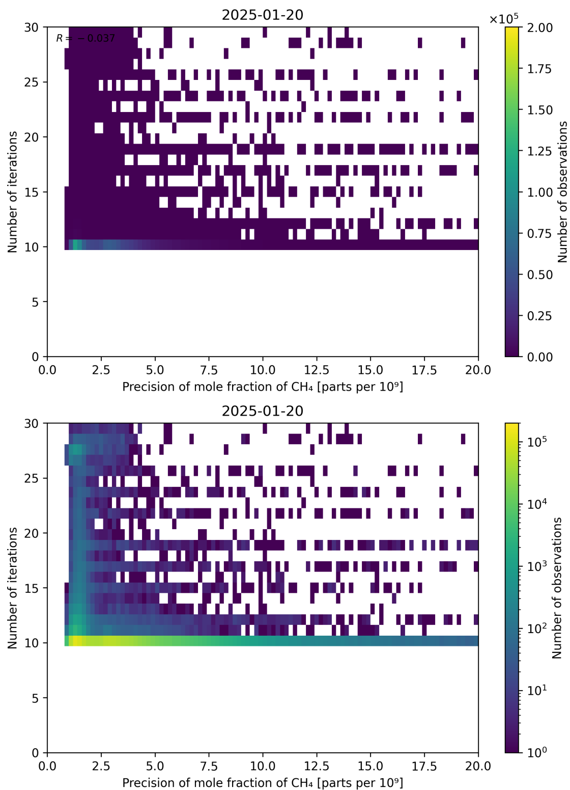
Figure 83: Scatter density plot of “Precision of mole fraction of CH 4 ” against “Number of iterations” for 2025-01-19 to 2025-01-21.
