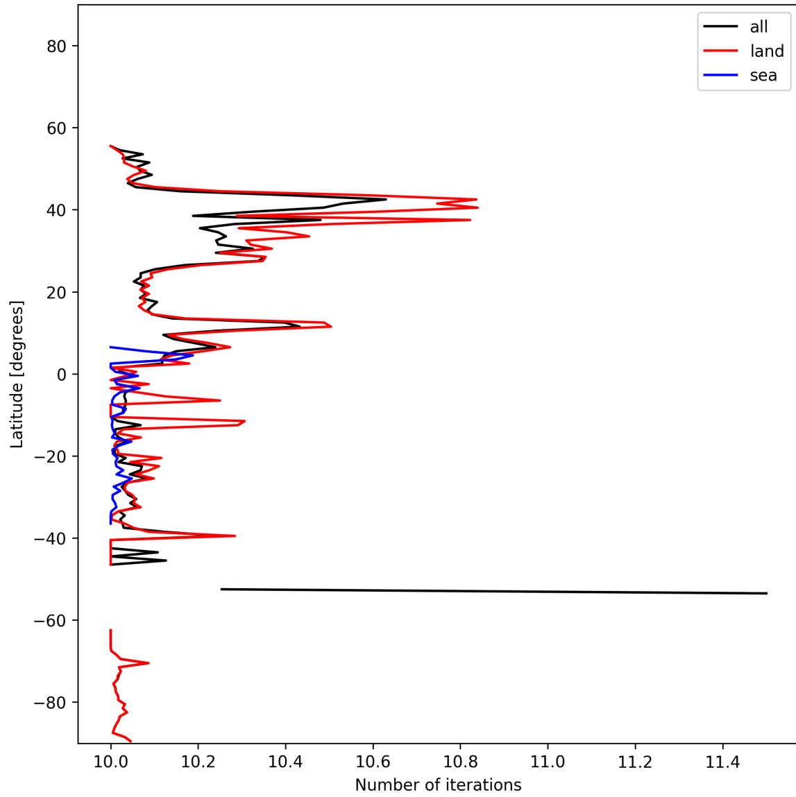
Figure 20: Zonal average of “Number of iterations” for 2025-01-19 to 2025-01-21.
