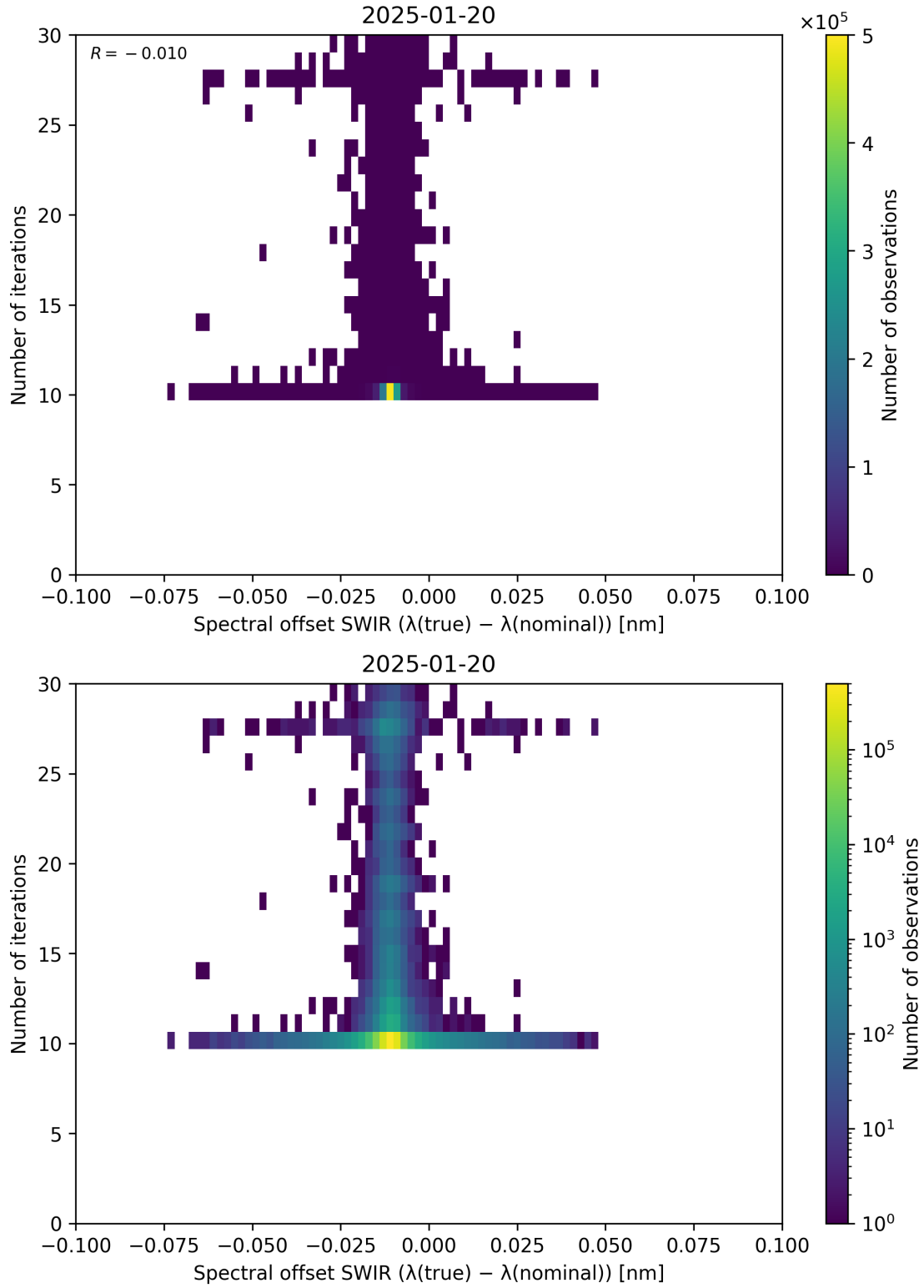
Figure 121: Scatter density plot of “Spectral offset SWIR ( \lambda_{\text{true}} - \lambda_{\text{nominal}} )” against “Number of iterations” for 2025-01-19 to 2025-01-21.
