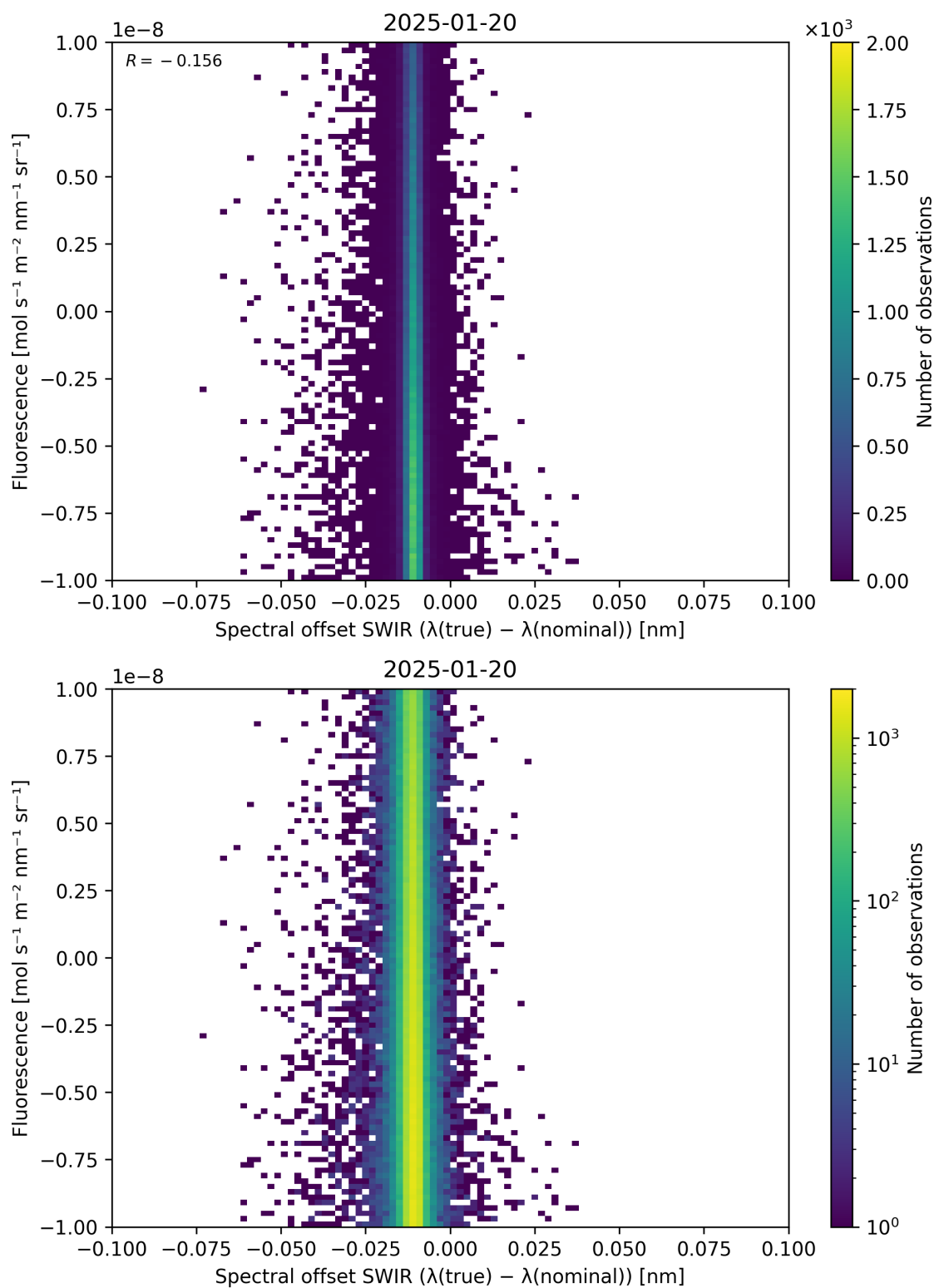
Figure 120: Scatter density plot of “Spectral offset SWIR ( \lambda_{\text{true}} - \lambda_{\text{nominal}} )” against “Fluorescence” for 2025-01-19 to 2025-01-21.
