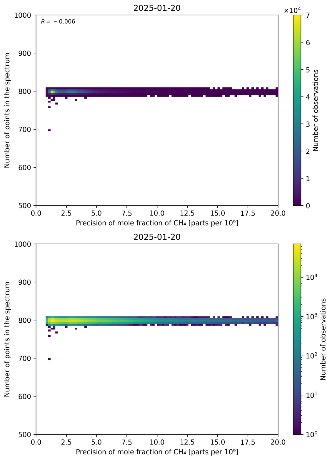
Figure 84: Scatter density plot of “Precision of mole fraction of CH 4 ” against “Number of points in the spectrum” for 2025-01-19 to 2025-01-21.
