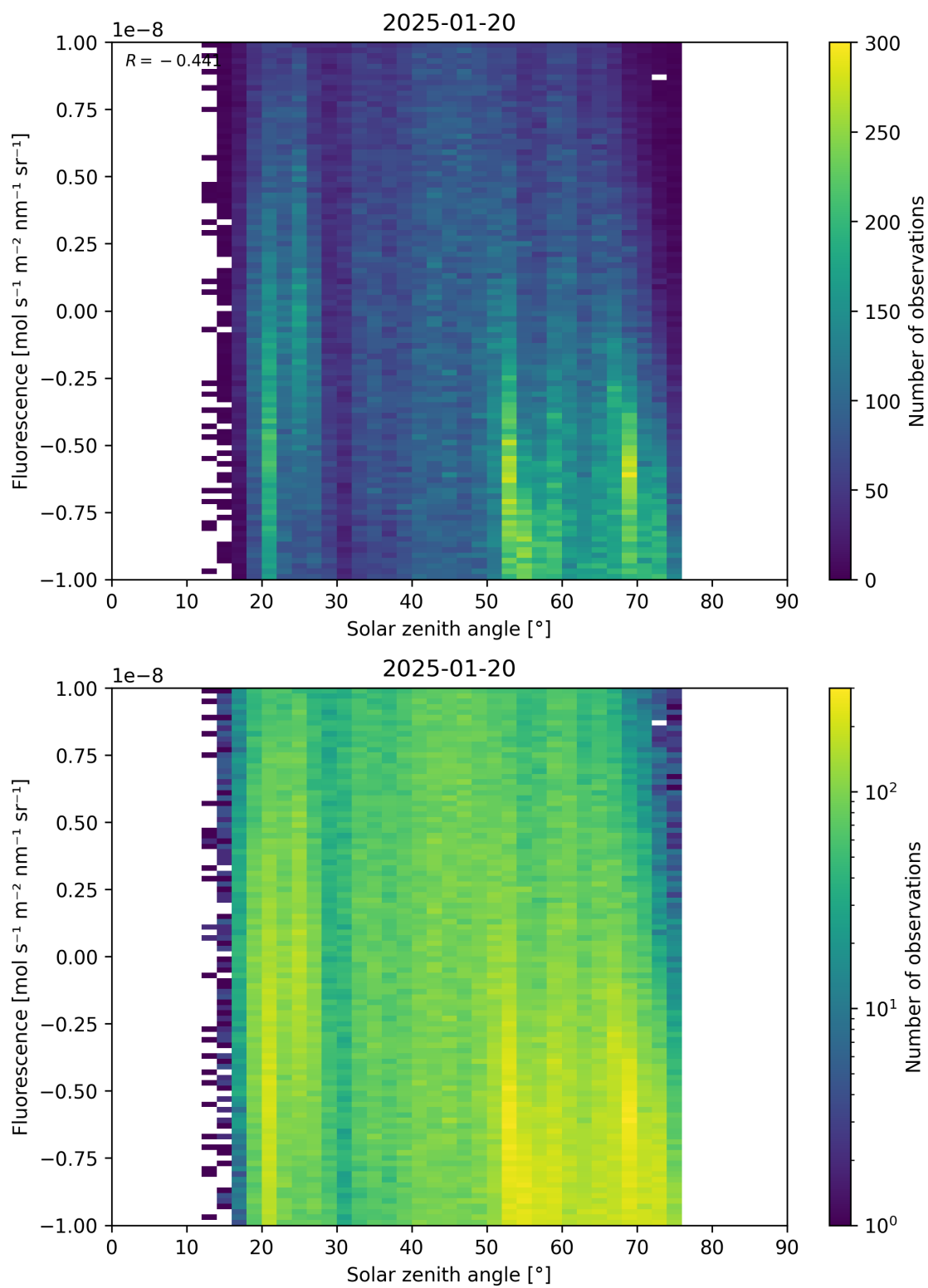
Figure 97: Scatter density plot of “Solar zenith angle” against “Fluorescence” for 2025-01-19 to 2025-01-21.
