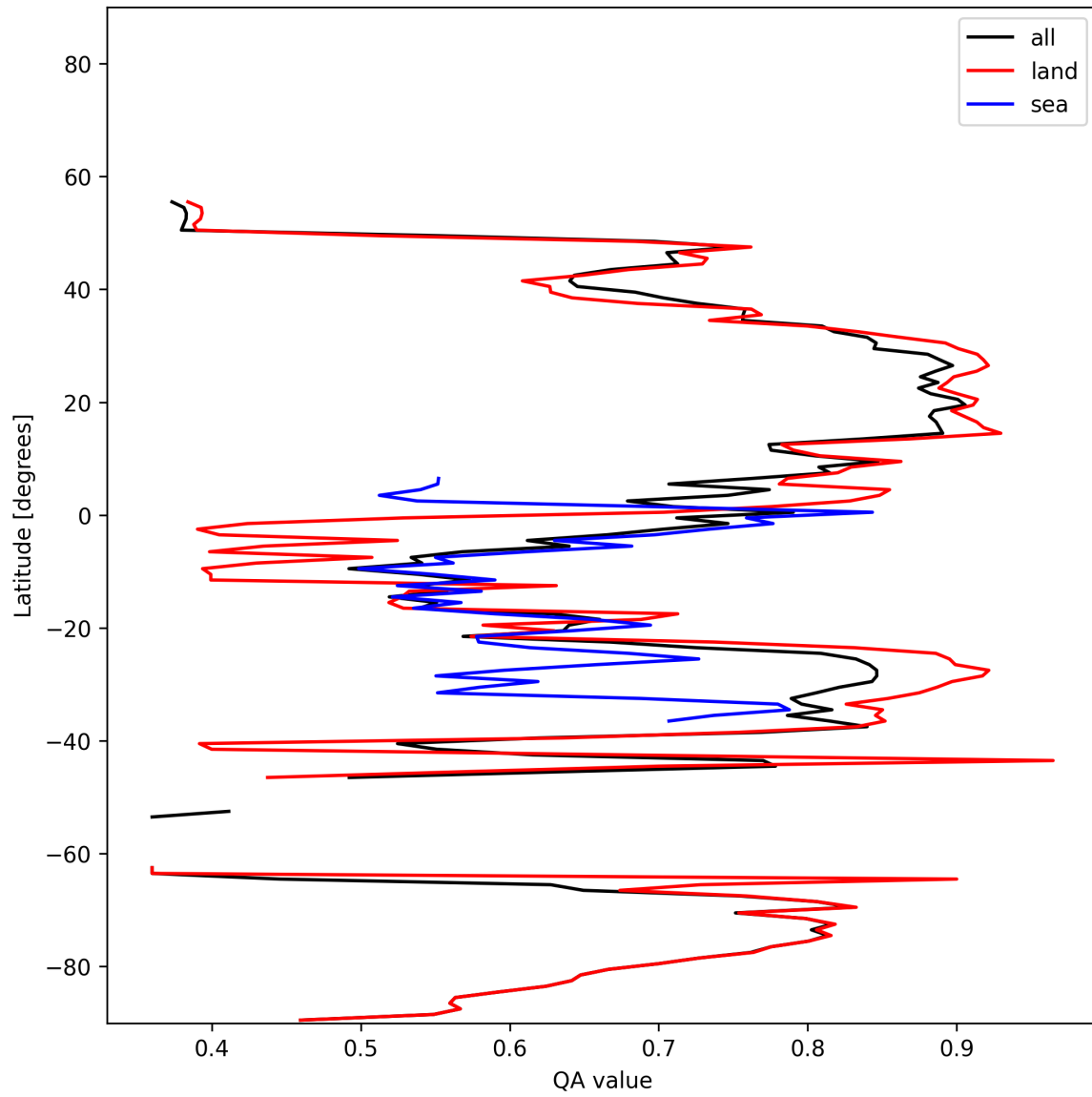
Figure 11: Zonal average of “QA value” for 2025-01-19 to 2025-01-21.
