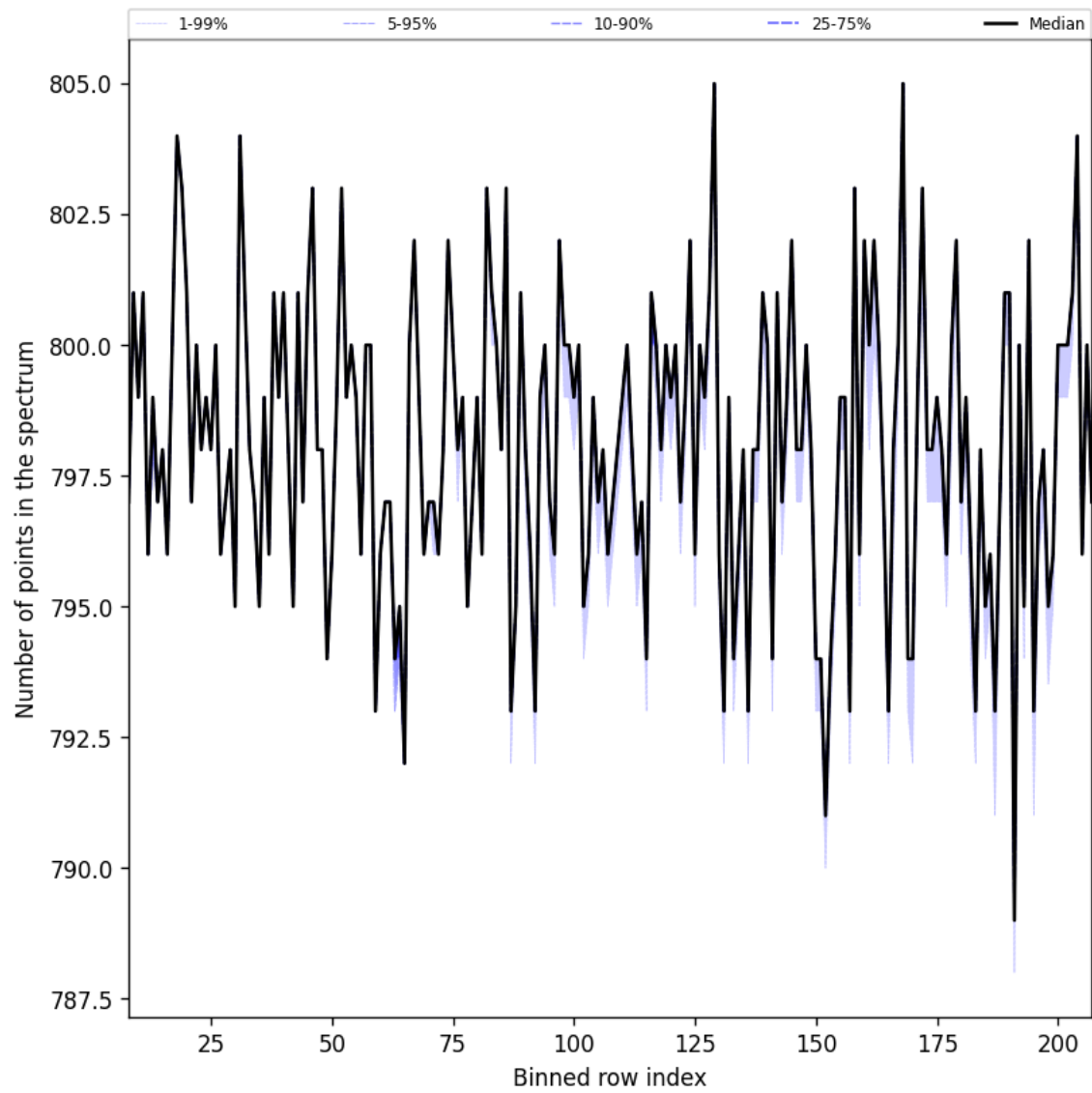
Figure 37: Along track statistics of “Number of points in the spectrum” for 2025-01-19 to 2025-01-21
