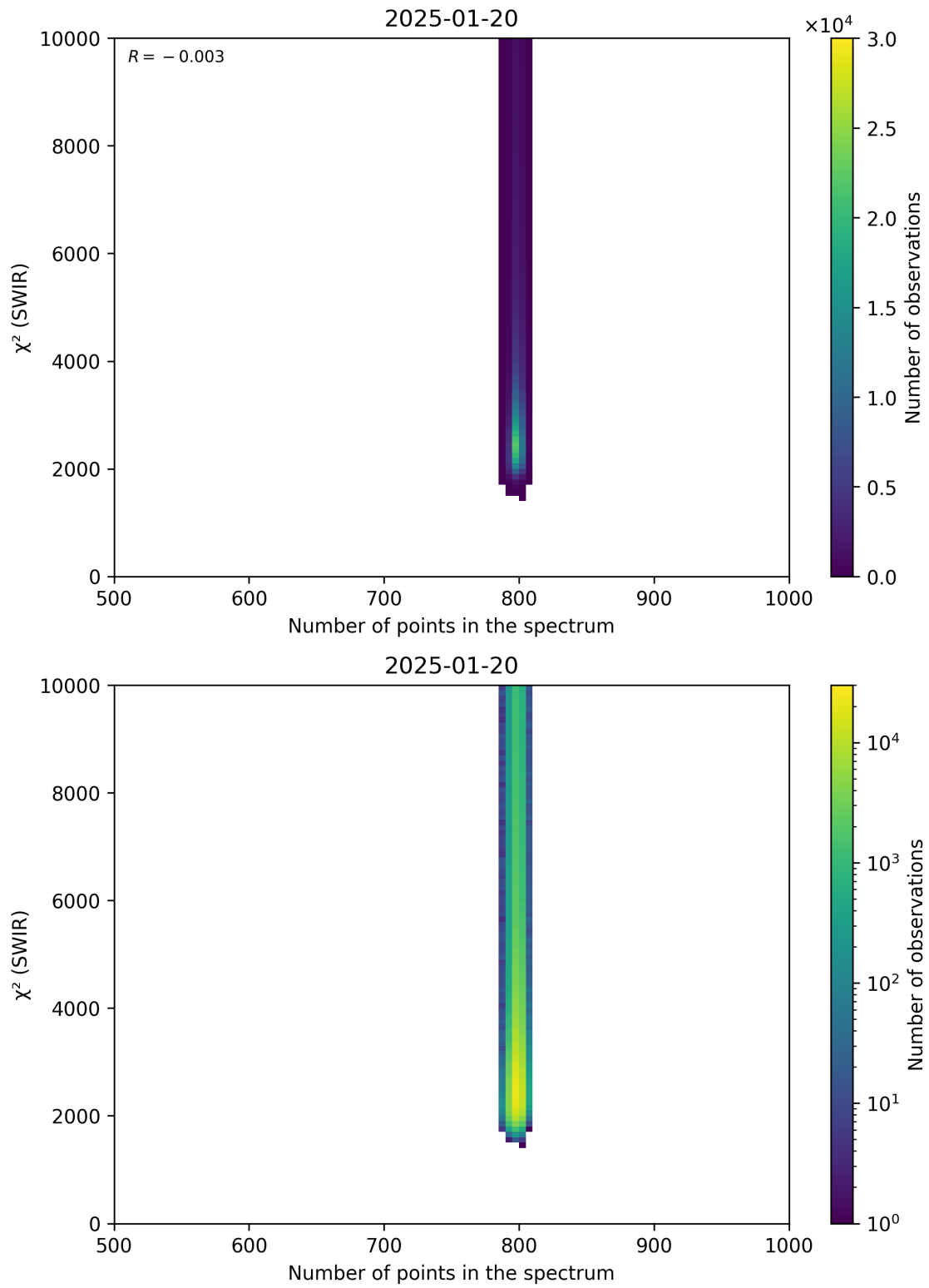
Figure 89: Scatter density plot of “Number of points in the spectrum” against “ \chi^2 (SWIR)” for 2025-01-19 to 2025-01-21.
