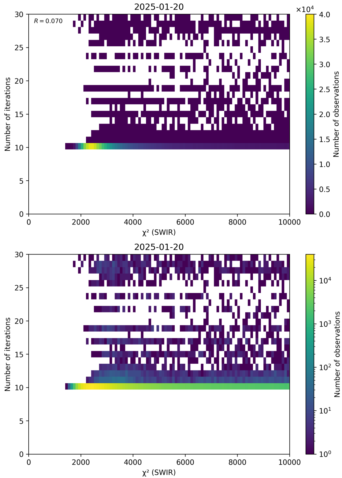
Figure 50: Scatter density plot of “ \chi^2 (SWIR)” against “Number of iterations” for 2025-01-19 to 2025-01-21.
