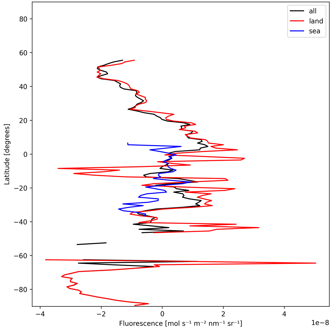
Figure 21: Zonal average of “Fluorescence” for 2025-01-19 to 2025-01-21.
