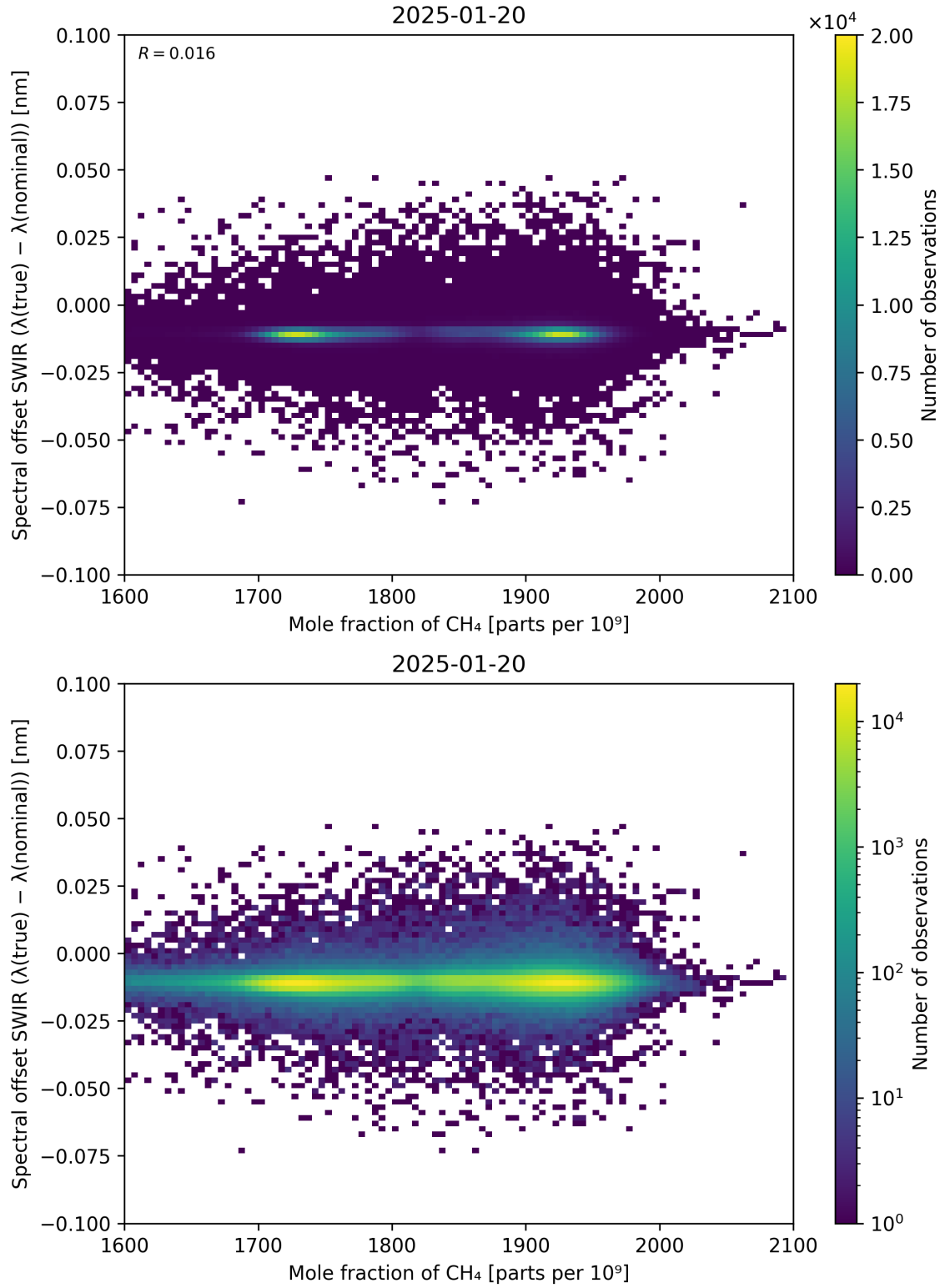
Figure 86: Scatter density plot of “Mole fraction of CH 4 ” against “Spectral offset SWIR ( \lambda_{\text{true}} - \lambda_{\text{nominal}} )” for 2025-01-19 to 2025-01-21.
