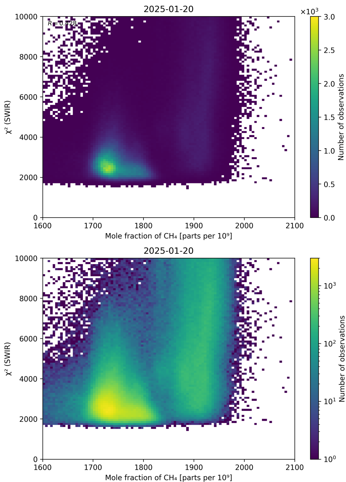
Figure 71: Scatter density plot of “Mole fraction of \text{CH}_4 ” against “ \chi^2 (SWIR)” for 2025-01-19 to 2025-01-21.
