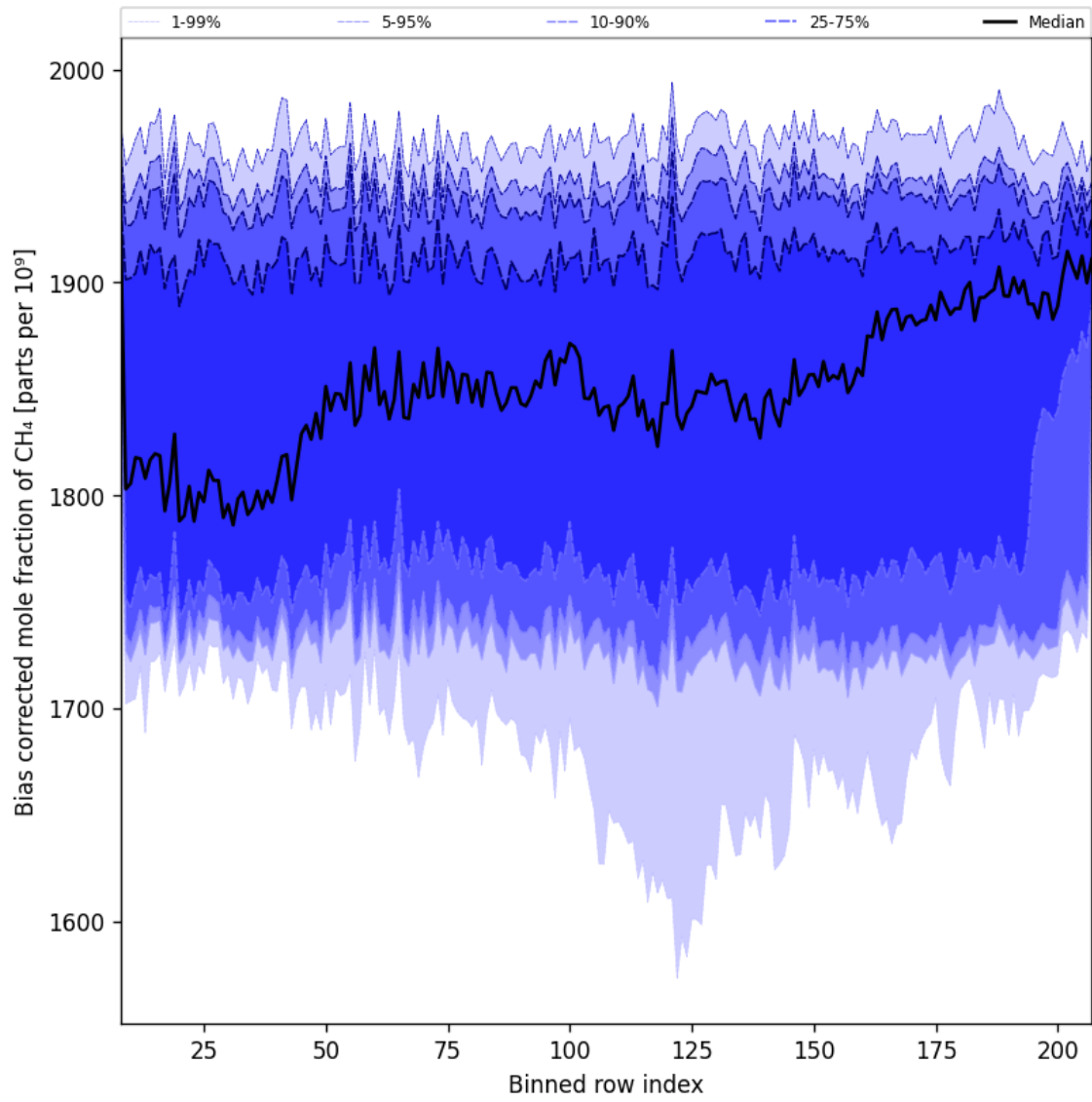
Figure 36: Along track statistics of “Bias corrected mole fraction of CH 4 ” for 2025-01-19 to 2025-01-21
