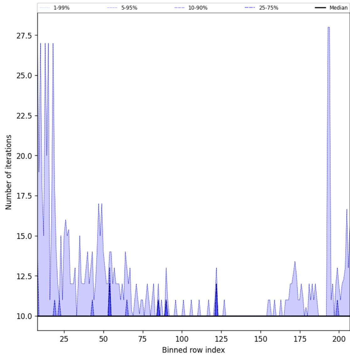
Figure 42: Along track statistics of “Number of iterations” for 2025-01-19 to 2025-01-21
