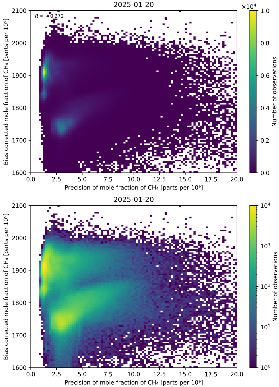
Figure 82: Scatter density plot of “Precision of mole fraction of \text{CH}_4 ” against “Bias corrected mole fraction of \text{CH}_4 ” for 2025-01-19 to 2025-01-21.
