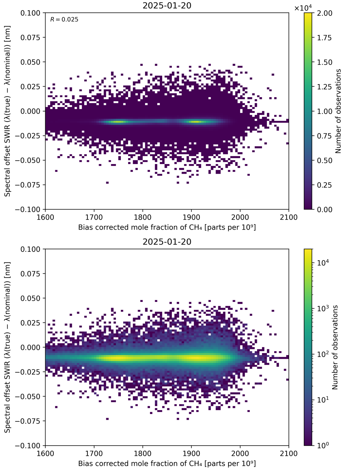
Figure 69: Scatter density plot of “Bias corrected mole fraction of \text{CH}_4 ” against “Spectral offset SWIR ( \lambda_{\text{true}} - \lambda_{\text{nominal}} )” for 2025-01-19 to 2025-01-21.
