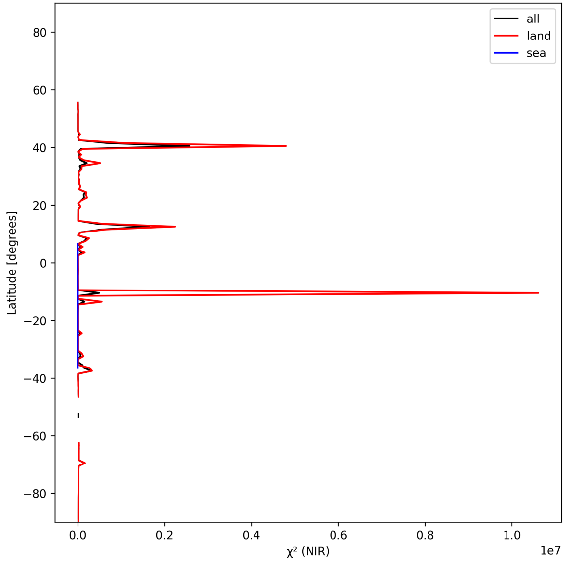
Figure 18: Zonal average of “ \chi^2 (NIR)” for 2025-01-19 to 2025-01-21.
