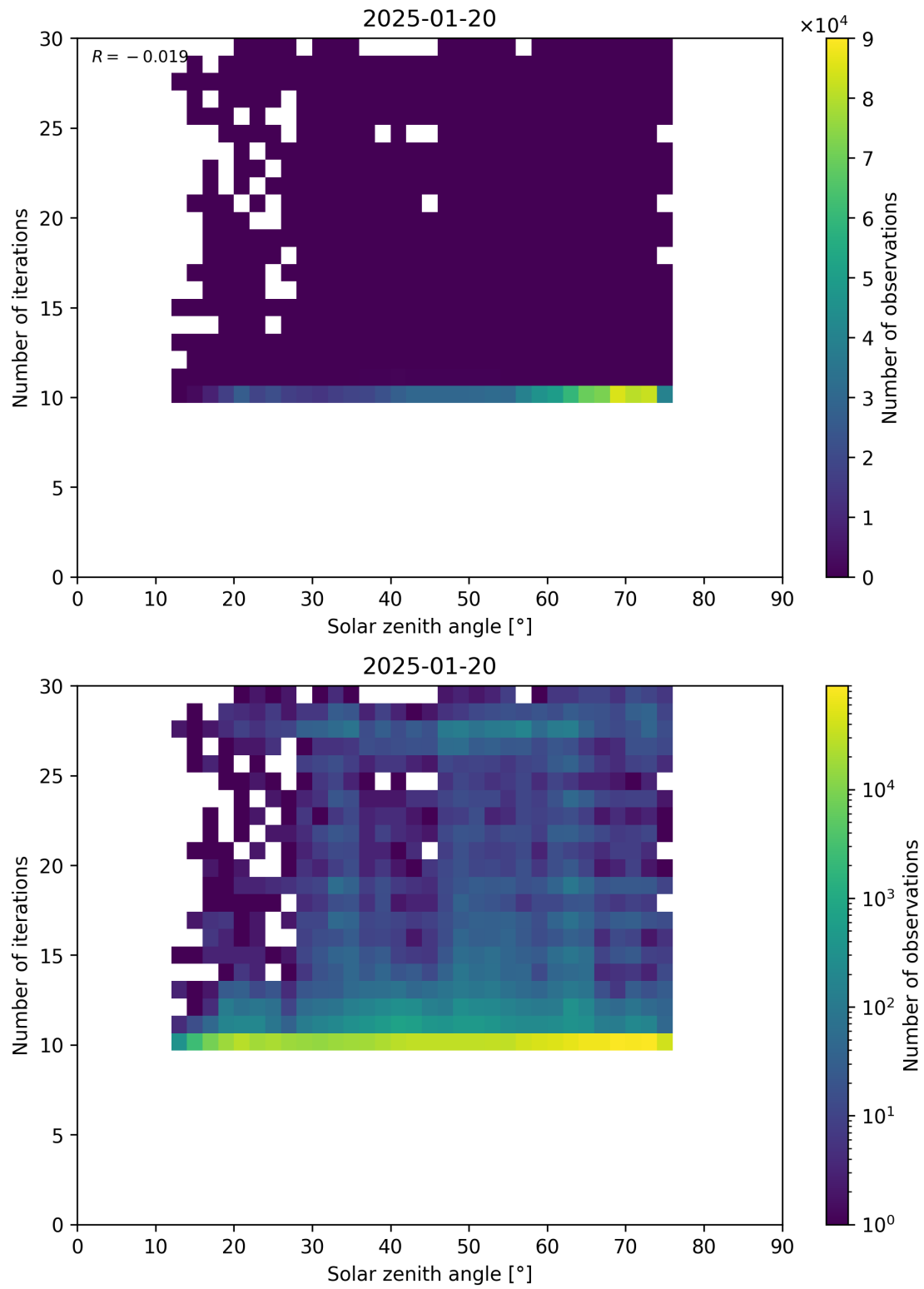
Figure 102: Scatter density plot of “Solar zenith angle” against “Number of iterations” for 2025-01-19 to 2025-01-21.
