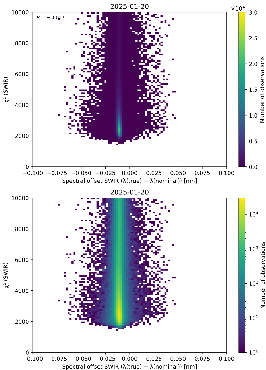
Figure 118: Scatter density plot of “Spectral offset SWIR ( \lambda_{\text{true}} - \lambda_{\text{nominal}} )” against “ \chi^2 (SWIR)” for 2025-01-19 to 2025-01-21.
