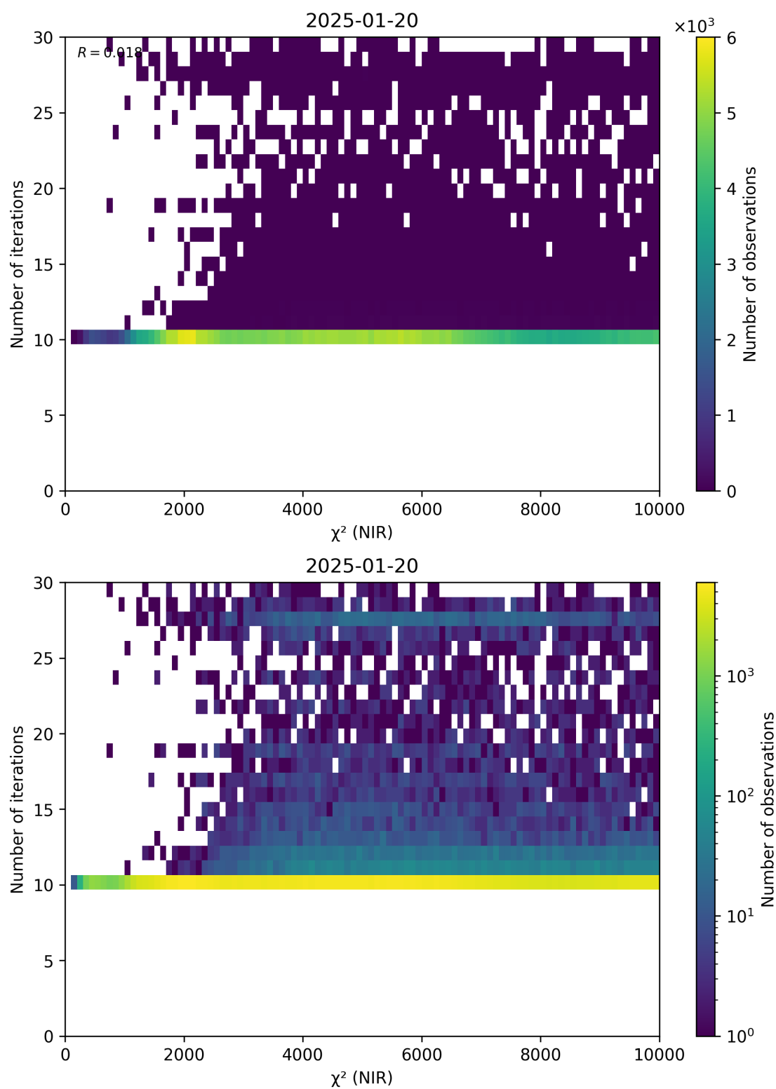
Figure 46: Scatter density plot of “ \chi^2 (NIR)” against “Number of iterations” for 2025-01-19 to 2025-01-21.
