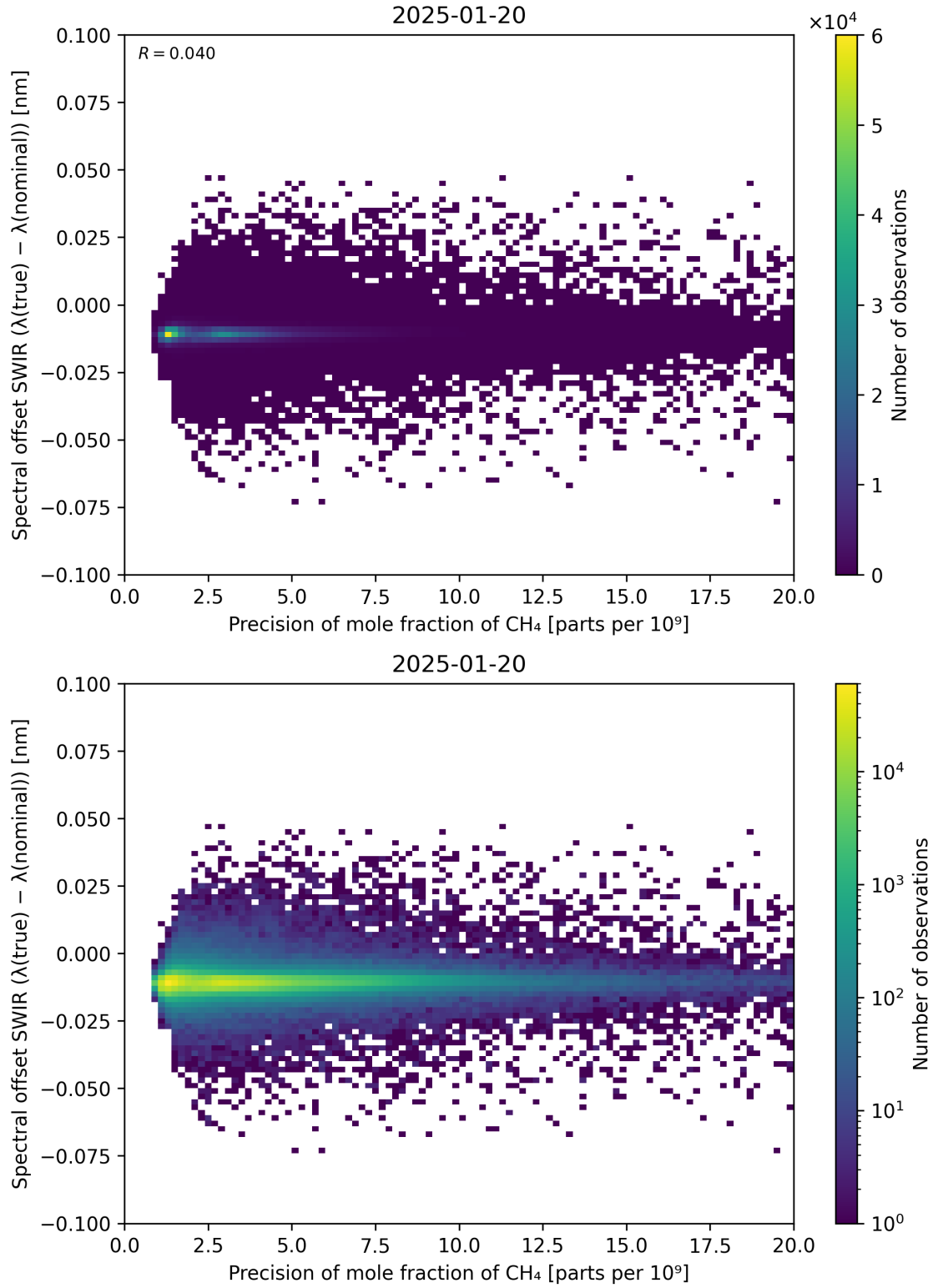
Figure 85: Scatter density plot of “Precision of mole fraction of \text{CH}_4 ” against “Spectral offset SWIR ( \lambda_{\text{true}} - \lambda_{\text{nominal}} )” for 2025-01-19 to 2025-01-21.
