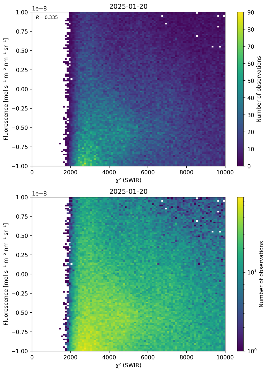
Figure 49: Scatter density plot of “ \chi^2 (SWIR)” against “Fluorescence” for 2025-01-19 to 2025-01-21.
