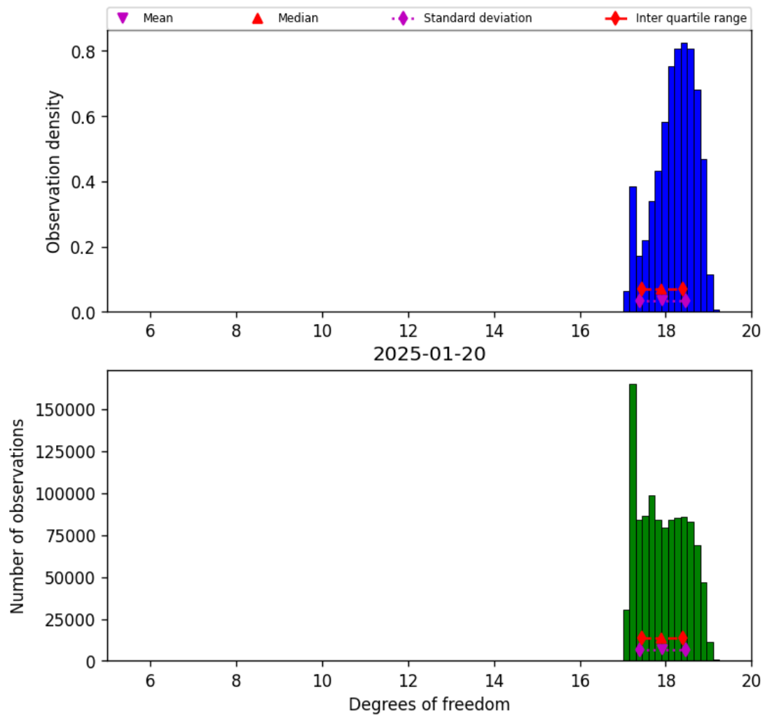
Figure 30: Histogram of “Degrees of freedom” for 2025-01-19 to 2025-01-21
