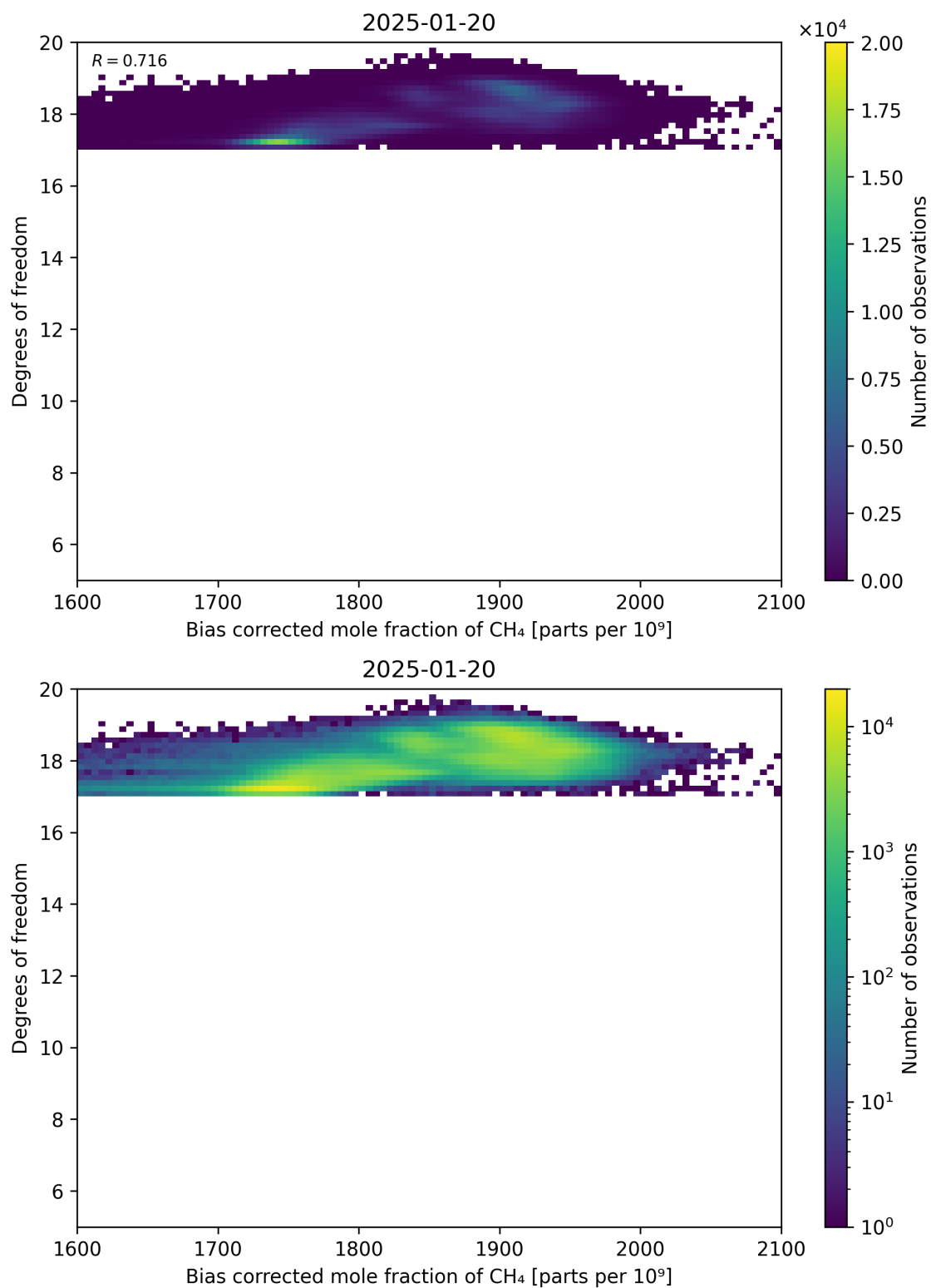
Figure 65: Scatter density plot of “Bias corrected mole fraction of CH 4 ” against “Degrees of freedom” for 2025-01-19 to 2025-01-21.
