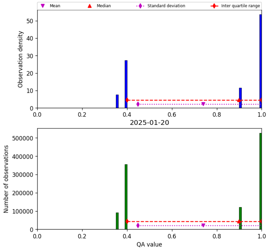
Figure 22: Histogram of “QA value” for 2025-01-19 to 2025-01-21
