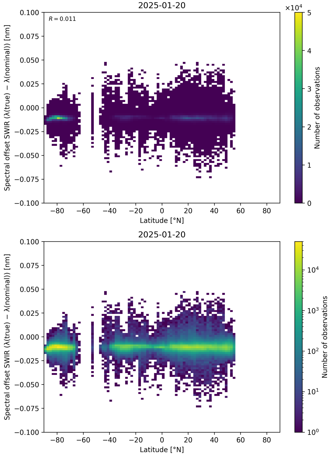
Figure 62: Scatter density plot of “Latitude” against “Spectral offset SWIR ( \lambda_{\text{true}} - \lambda_{\text{nominal}} )” for 2025-01-19 to 2025-01-21.
