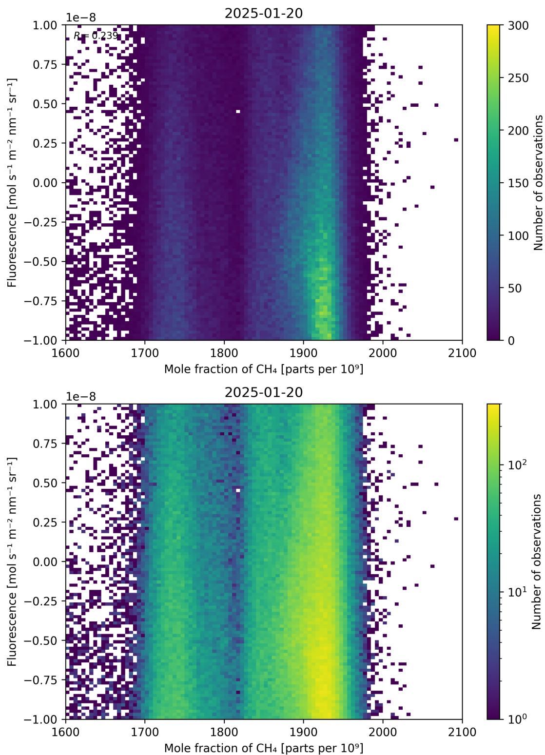
Figure 73: Scatter density plot of “Mole fraction of \text{CH}_4 ” against “Fluorescence” for 2025-01-19 to 2025-01-21.
