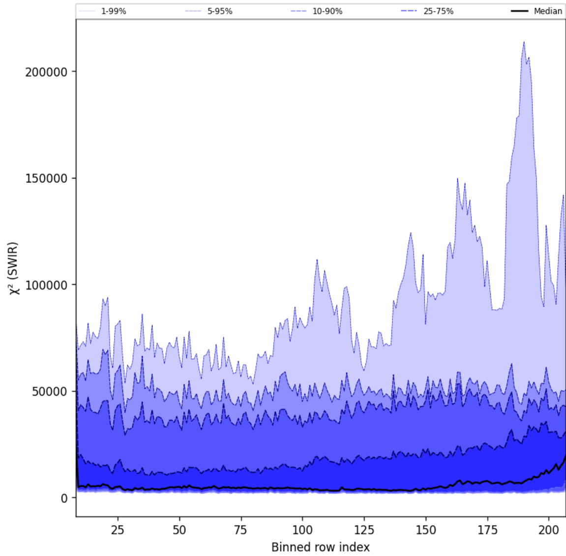
Figure 39: Along track statistics of “ \chi^2 (SWIR)” for 2025-01-19 to 2025-01-21
