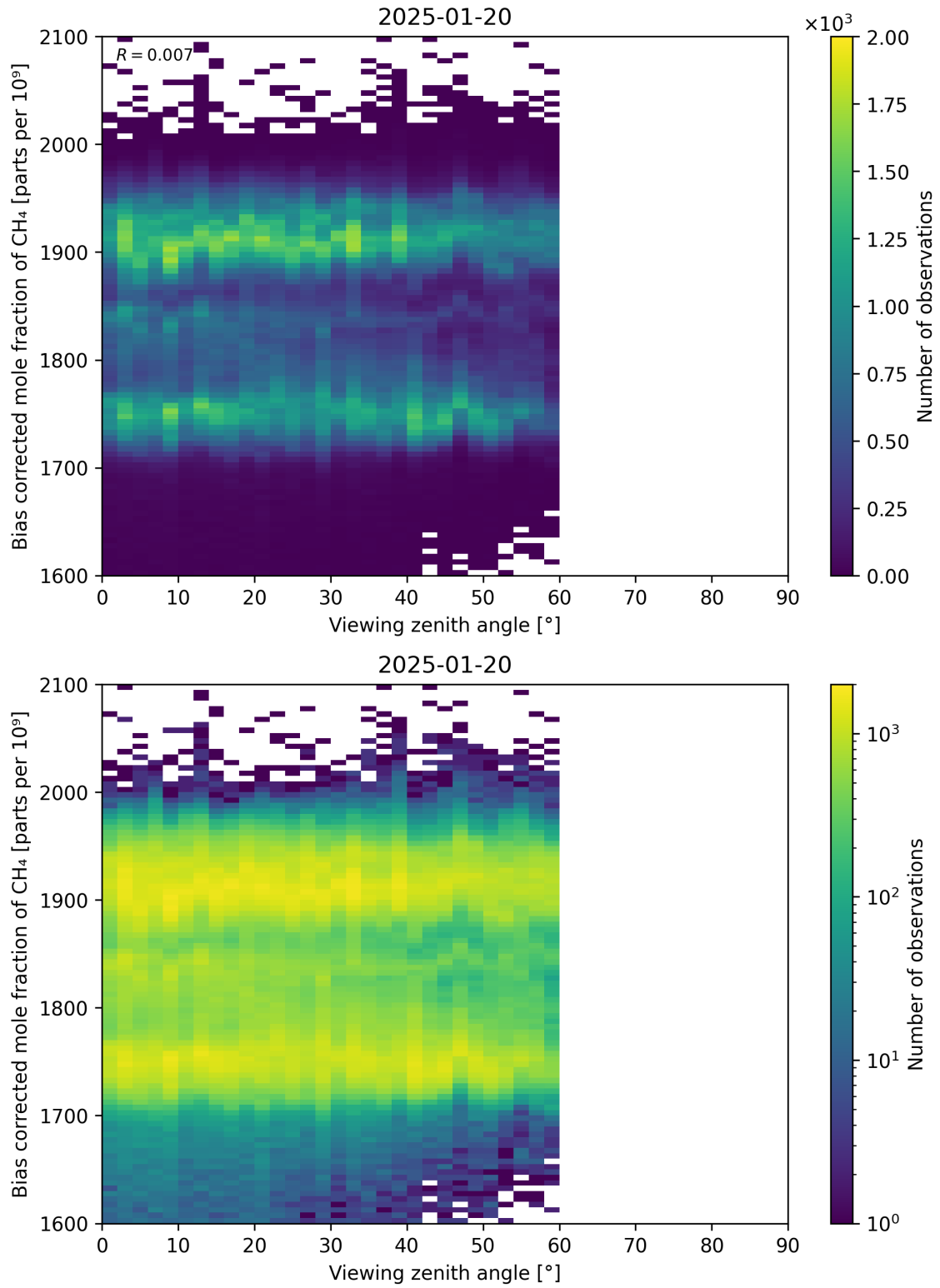
Figure 111: Scatter density plot of “Viewing zenith angle” against “Bias corrected mole fraction of CH 4 ” for 2025-01-19 to 2025-01-21.
