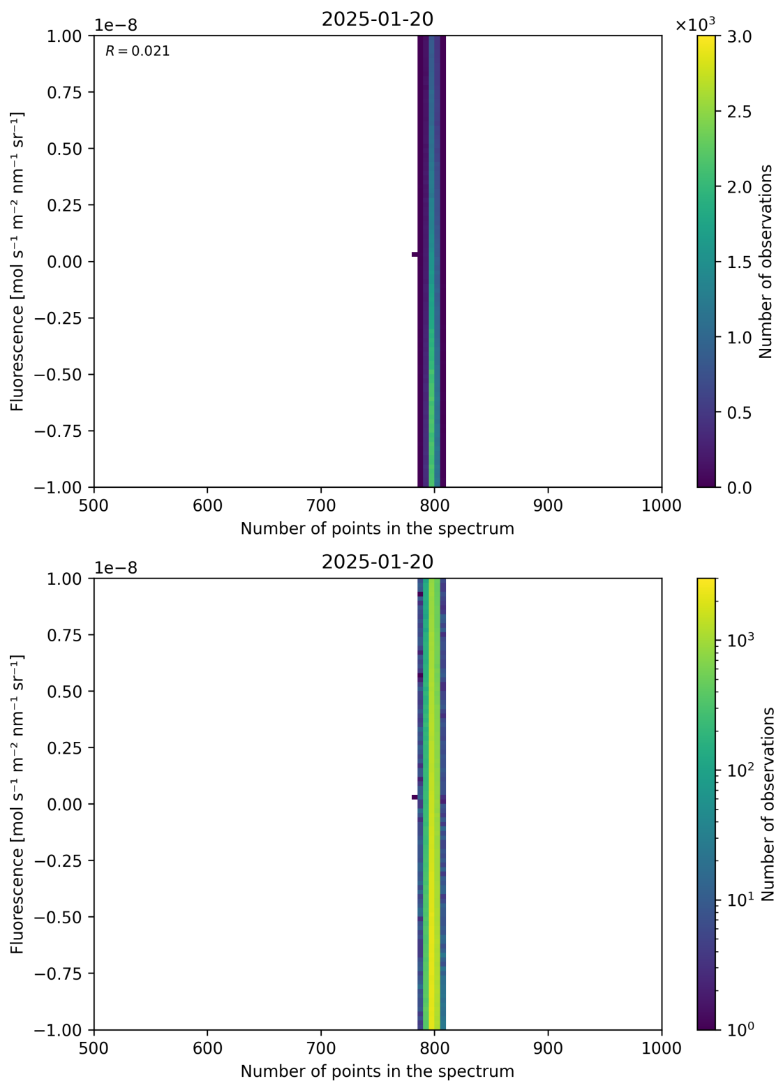
Figure 91: Scatter density plot of “Number of points in the spectrum” against “Fluorescence” for 2025-01-19 to 2025-01-21.
