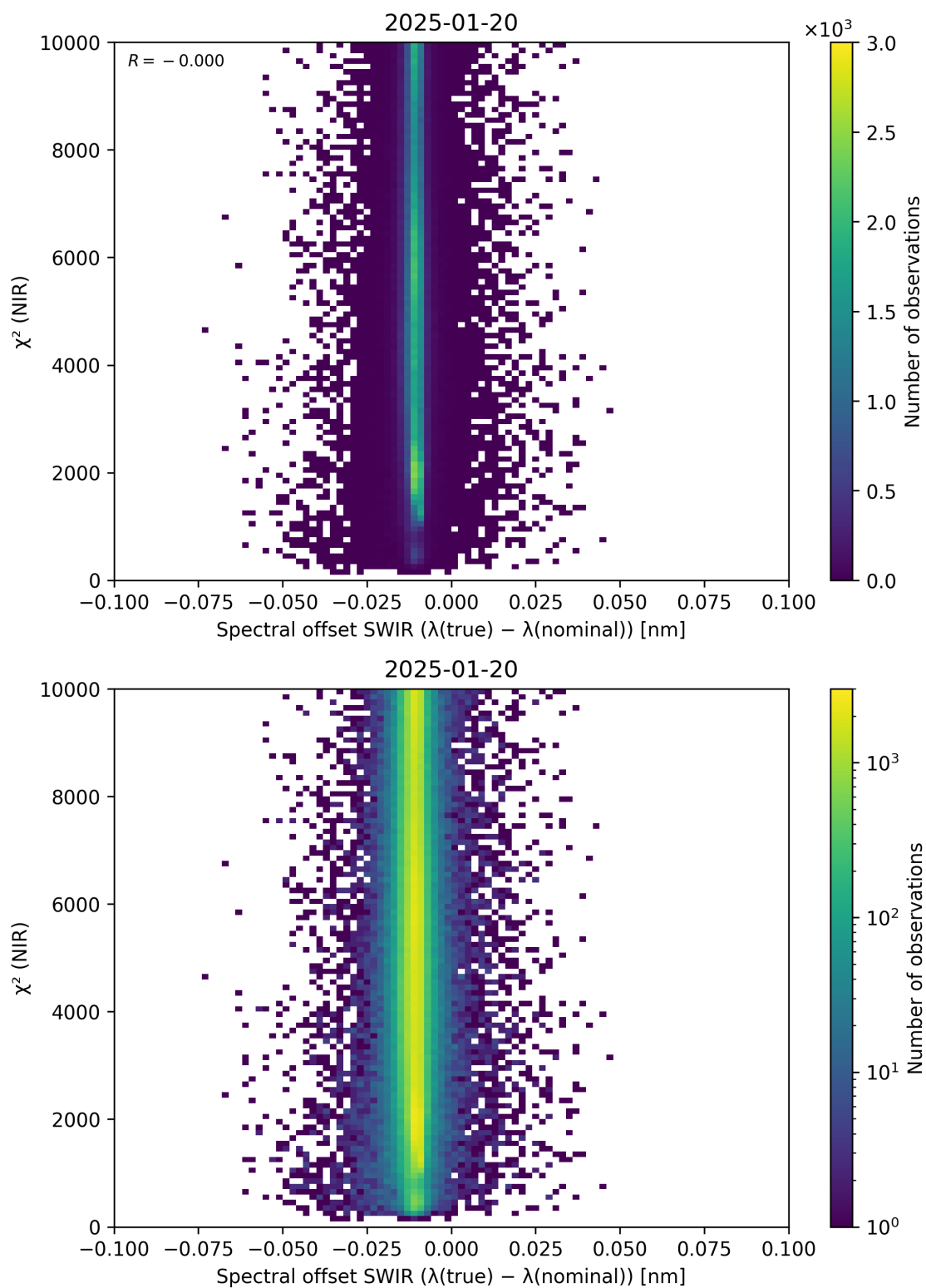
Figure 117: Scatter density plot of “Spectral offset SWIR ( \lambda_{\text{true}} - \lambda_{\text{nominal}} )” against “ \chi^2 (NIR)” for 2025-01-19 to 2025-01-21.
