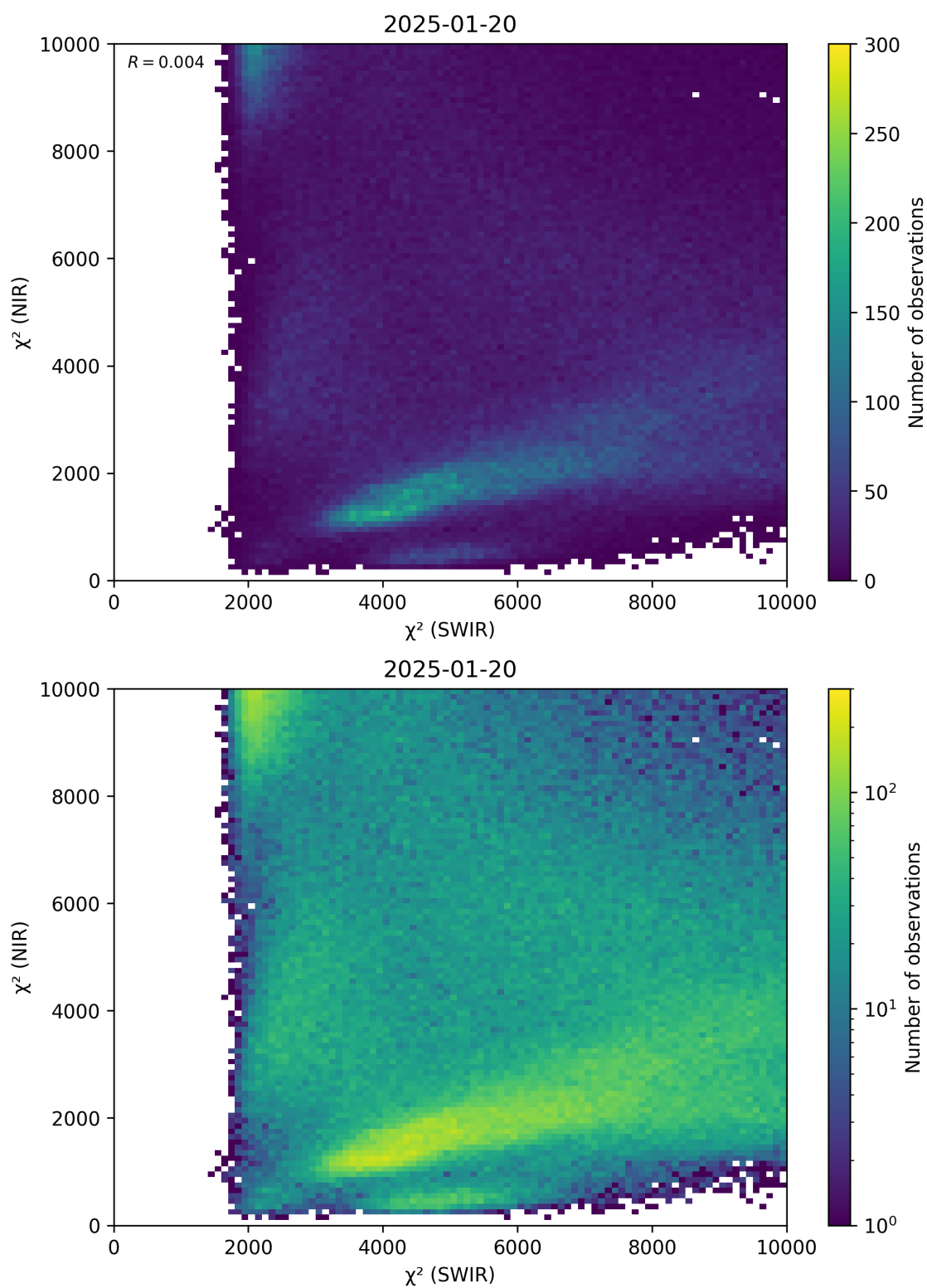
Figure 47: Scatter density plot of “ \chi^2 (SWIR)” against “ \chi^2 (NIR)” for 2025-01-19 to 2025-01-21.
