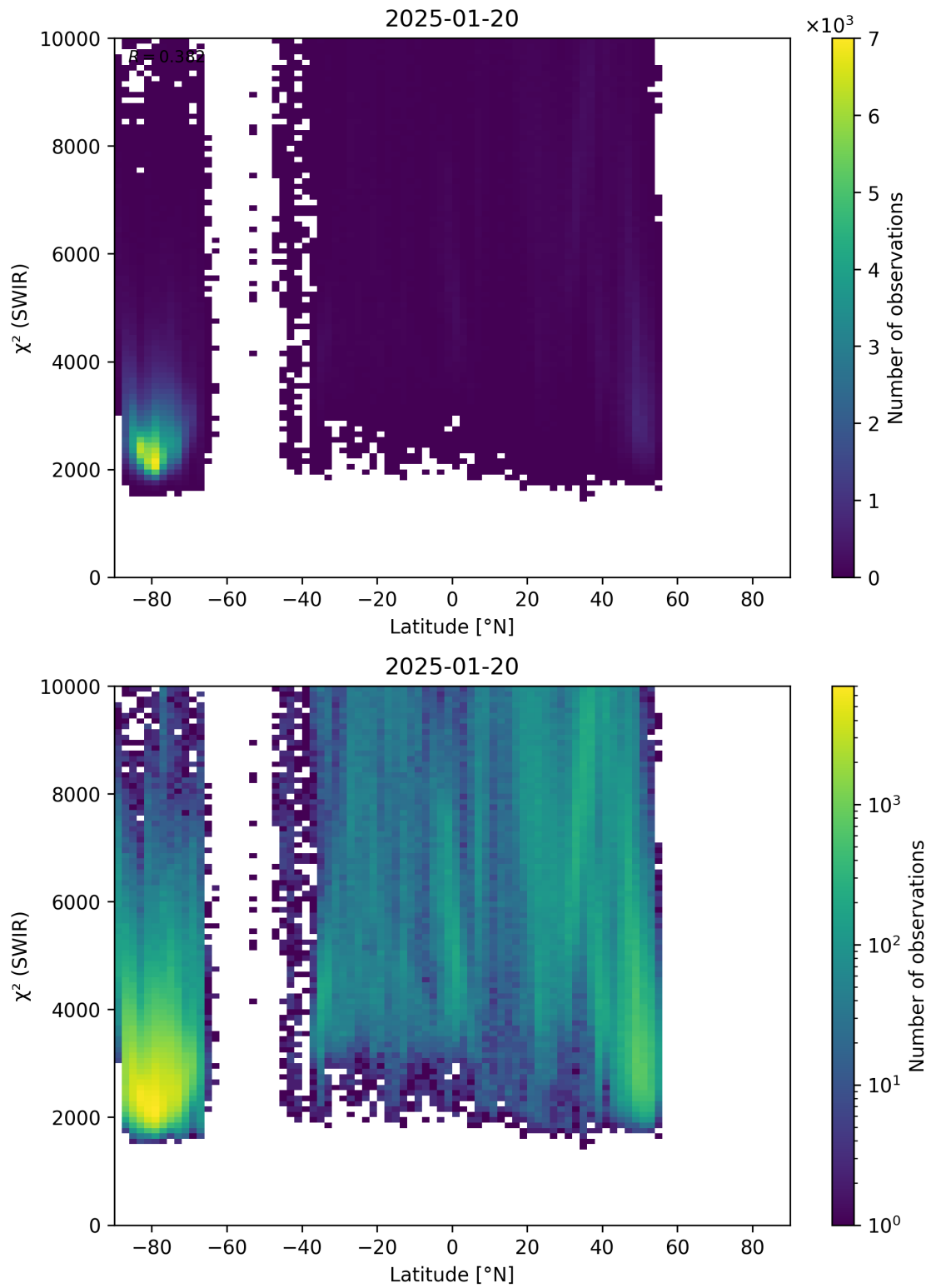
Figure 54: Scatter density plot of “Latitude” against “ \chi^2 (SWIR)” for 2025-01-19 to 2025-01-21.
