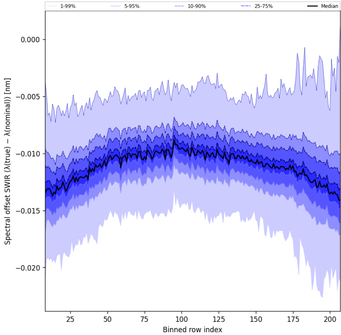
Figure 38: Along track statistics of “Spectral offset SWIR ( \lambda_{\text{true}} - \lambda_{\text{nominal}} )” for 2025-01-19 to 2025-01-21
