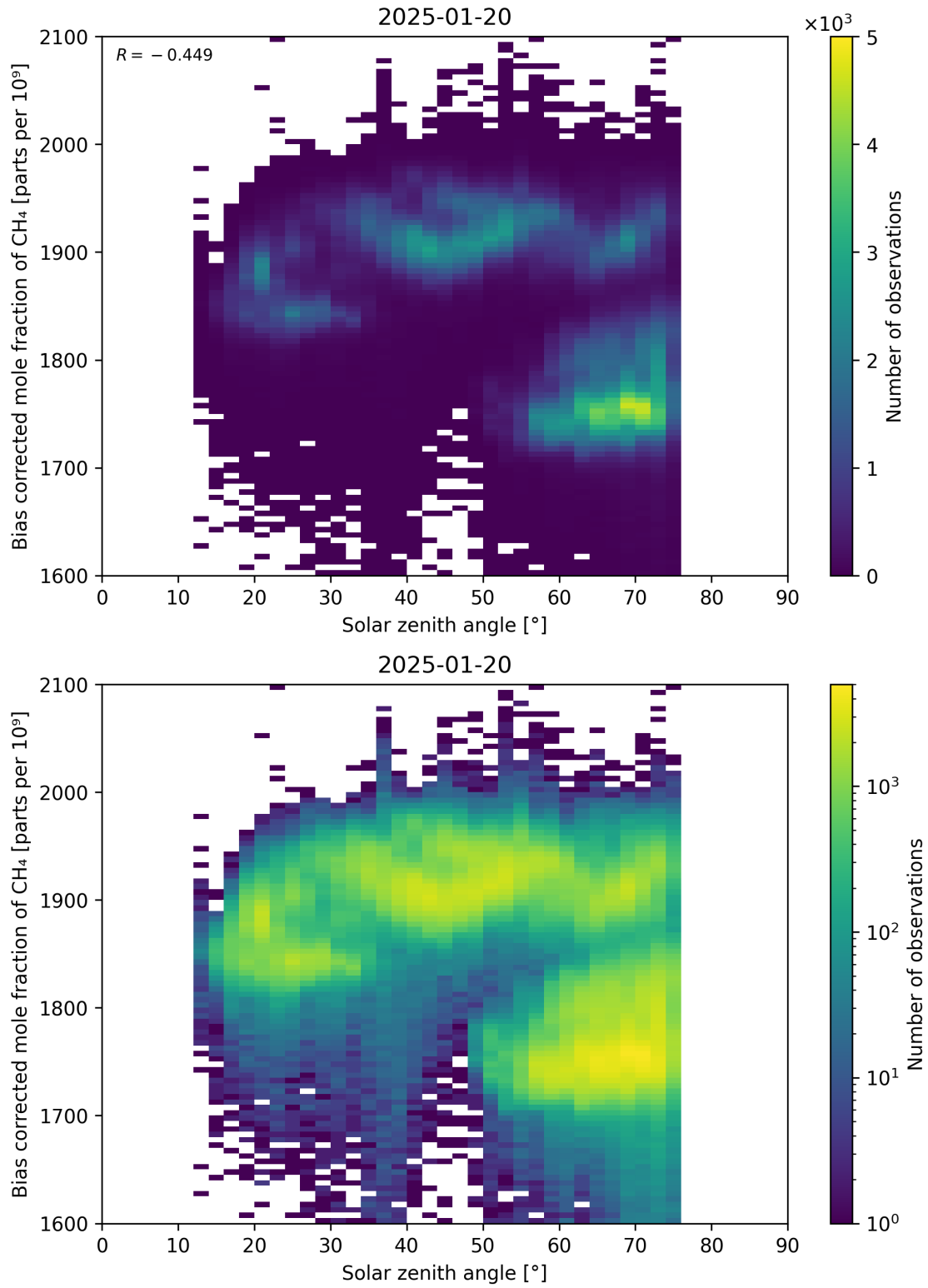
Figure 100: Scatter density plot of “Solar zenith angle” against “Bias corrected mole fraction of \text{CH}_4 ” for 2025-01-19 to 2025-01-21.
