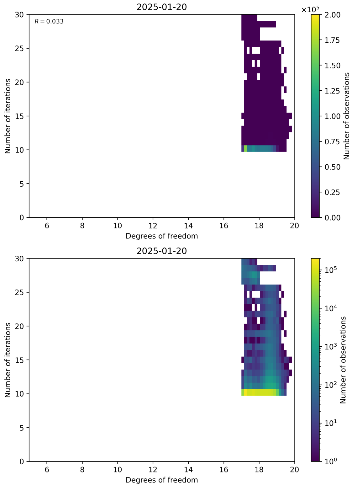
Figure 52: Scatter density plot of “Degrees of freedom” against “Number of iterations” for 2025-01-19 to 2025-01-21.
