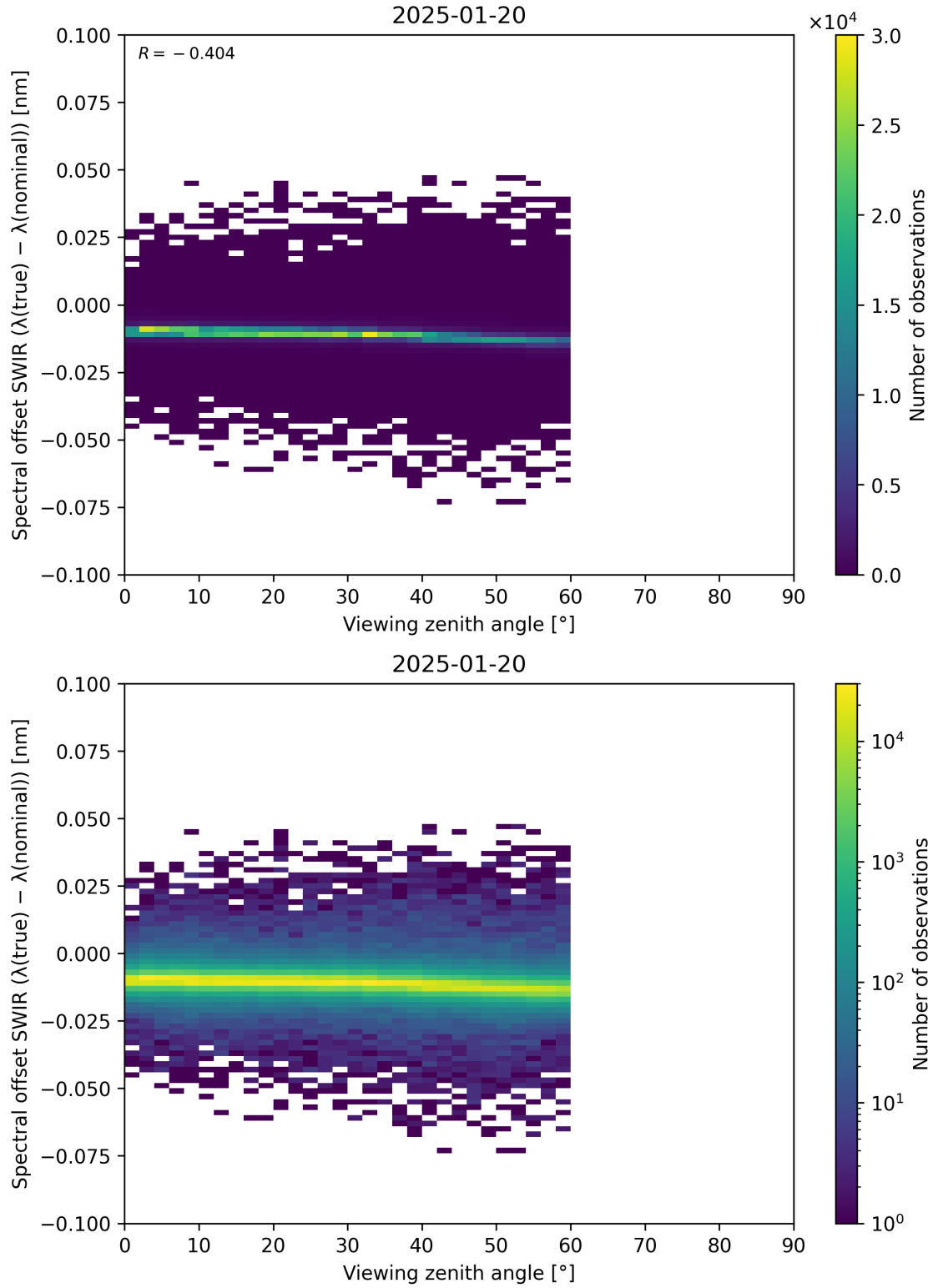
Figure 116: Scatter density plot of “Viewing zenith angle” against “Spectral offset SWIR ( \lambda_{\text{true}} - \lambda_{\text{nominal}} )” for 2025-01-19 to 2025-01-21.
