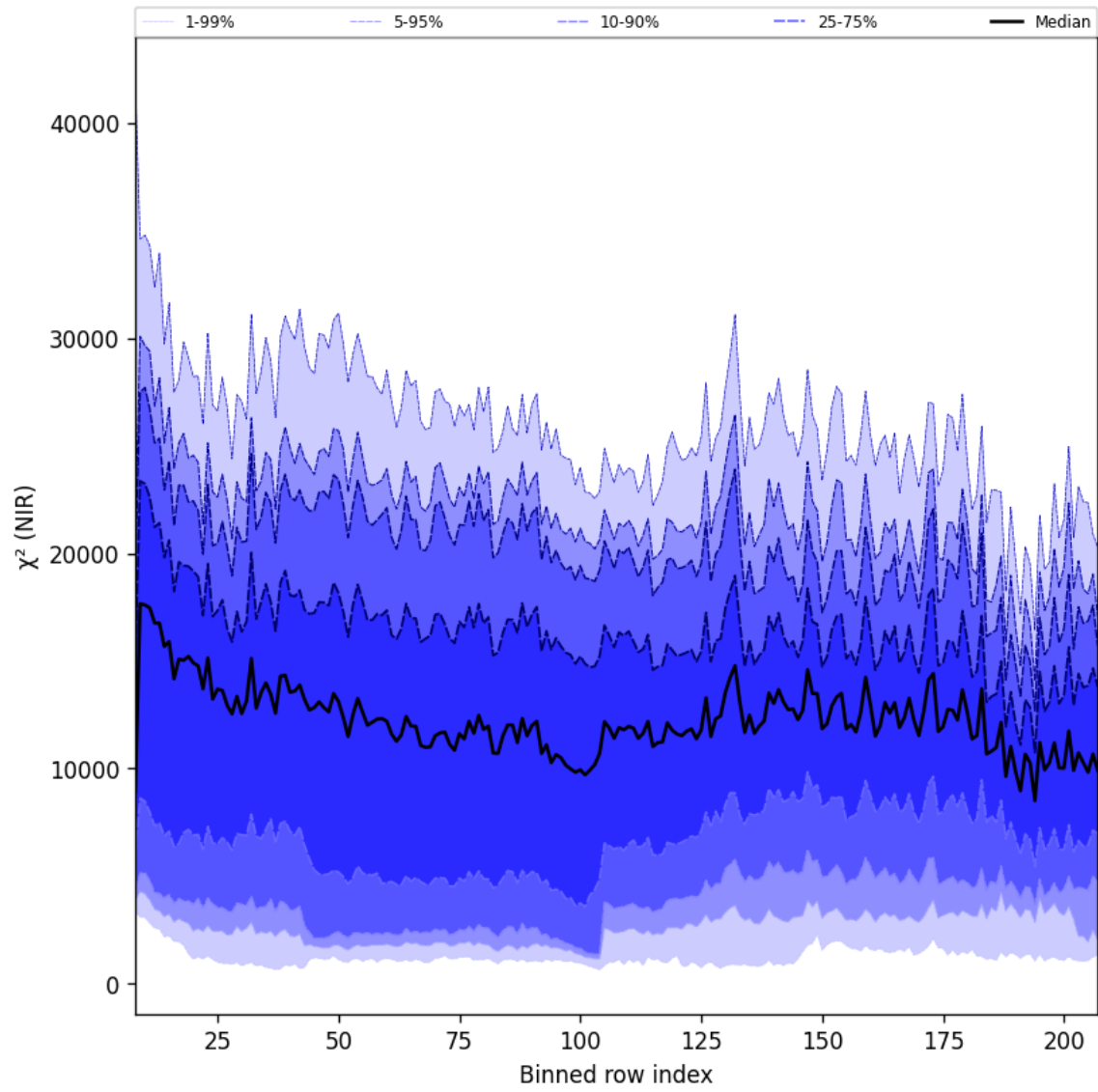
Figure 40: Along track statistics of " \chi^2 (NIR)" for 2025-01-19 to 2025-01-21
