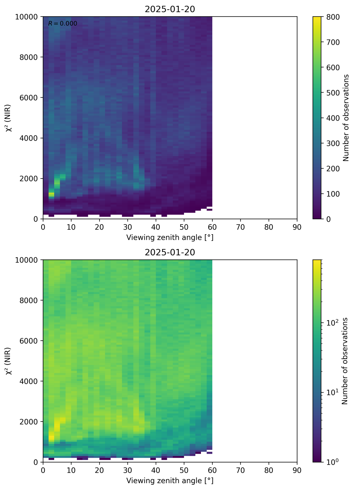
Figure 105: Scatter density plot of “Viewing zenith angle” against “ \chi^2 (NIR)” for 2025-01-19 to 2025-01-21.
