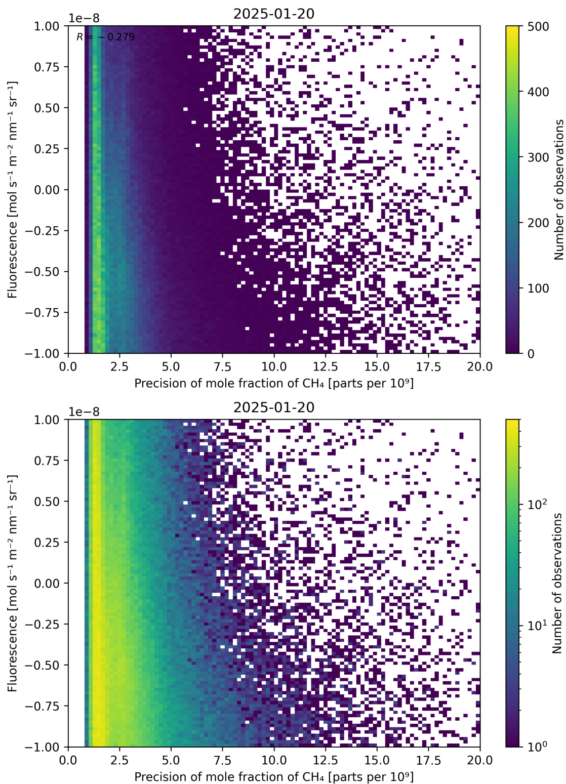
Figure 81: Scatter density plot of “Precision of mole fraction of CH 4 ” against “Fluorescence” for 2025-01-19 to 2025-01-21.
