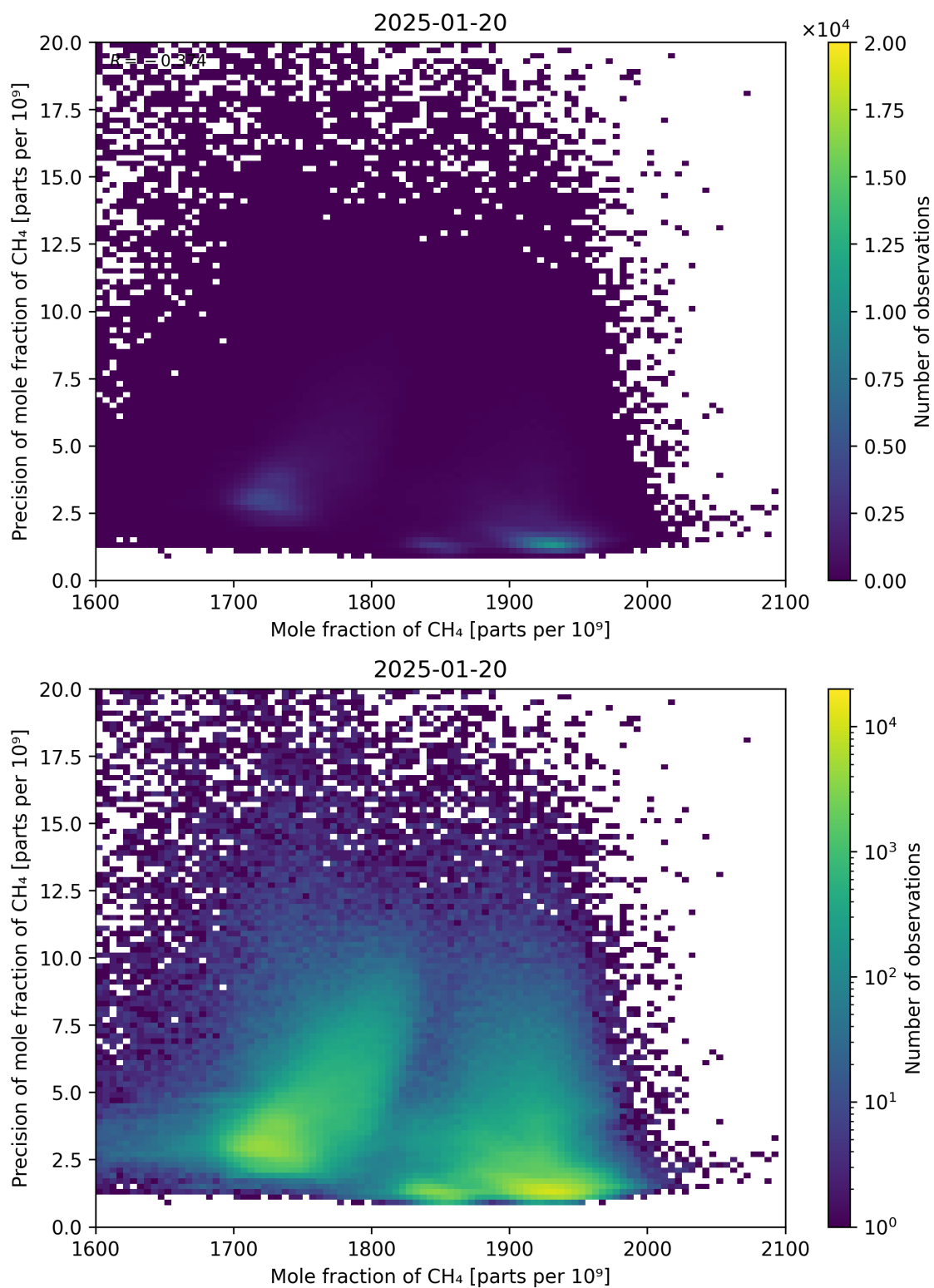
Figure 75: Scatter density plot of “Mole fraction of CH 4 ” against “Precision of mole fraction of CH 4 ” for 2025-01-19 to 2025-01-21.
