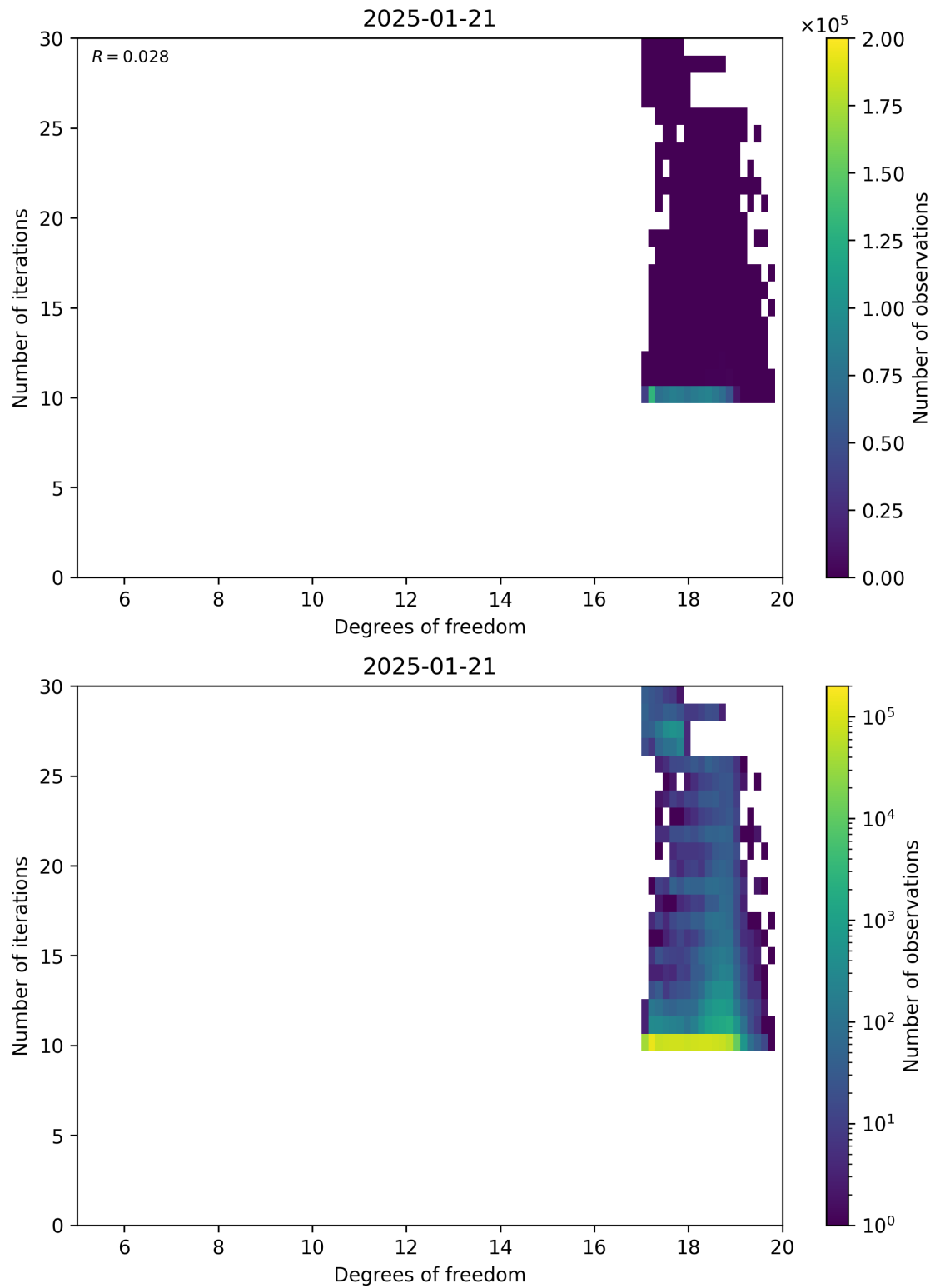
Figure 52: Scatter density plot of “Degrees of freedom” against “Number of iterations” for 2025-01-20 to 2025-01-22.
