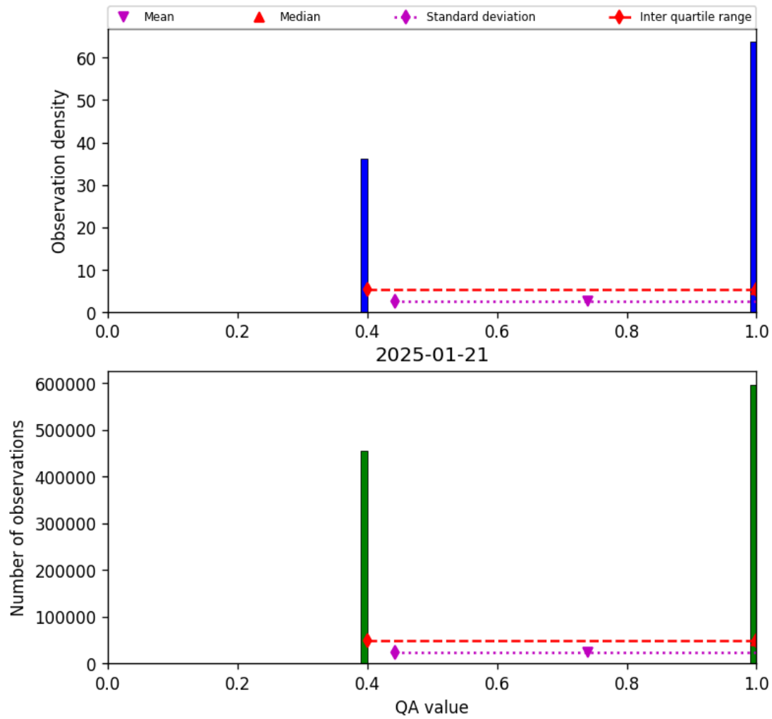
Figure 22: Histogram of “QA value” for 2025-01-20 to 2025-01-22
