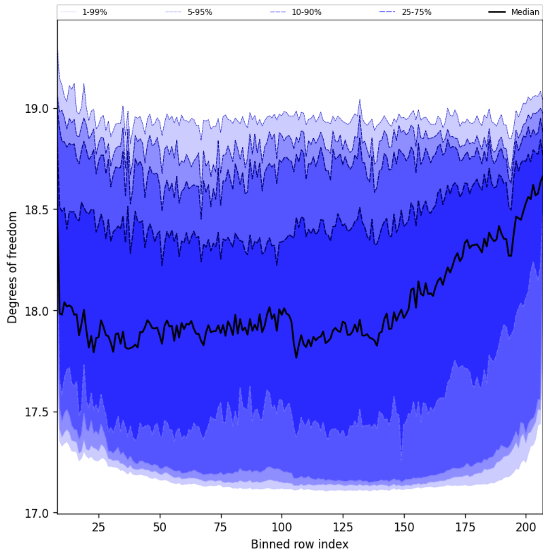
Figure 41: Along track statistics of “Degrees of freedom” for 2025-01-20 to 2025-01-22
