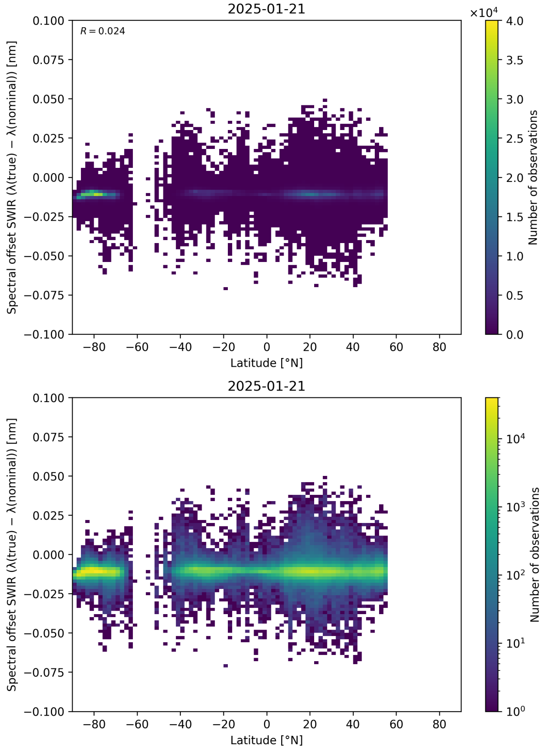
Figure 62: Scatter density plot of “Latitude” against “Spectral offset SWIR ( \lambda_{\text{true}} - \lambda_{\text{nominal}} )” for 2025-01-20 to 2025-01-22.
