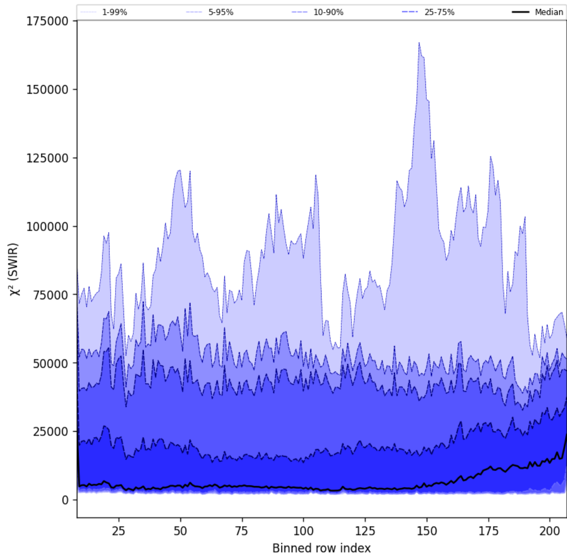
Figure 39: Along track statistics of “ \chi^2 (SWIR)” for 2025-01-20 to 2025-01-22
