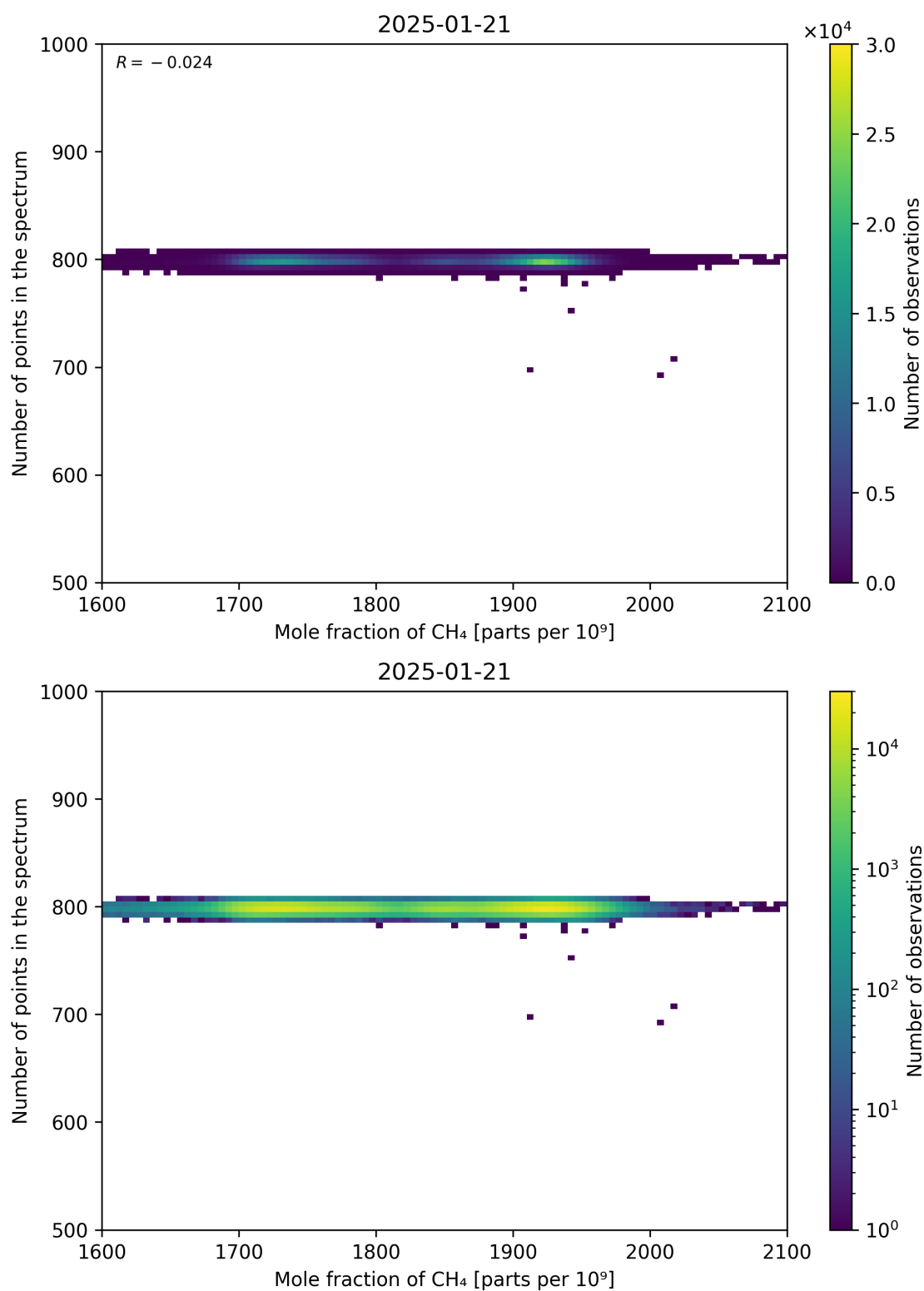
Figure 77: Scatter density plot of “Mole fraction of CH 4 ” against “Number of points in the spectrum” for 2025-01-20 to 2025-01-22.
