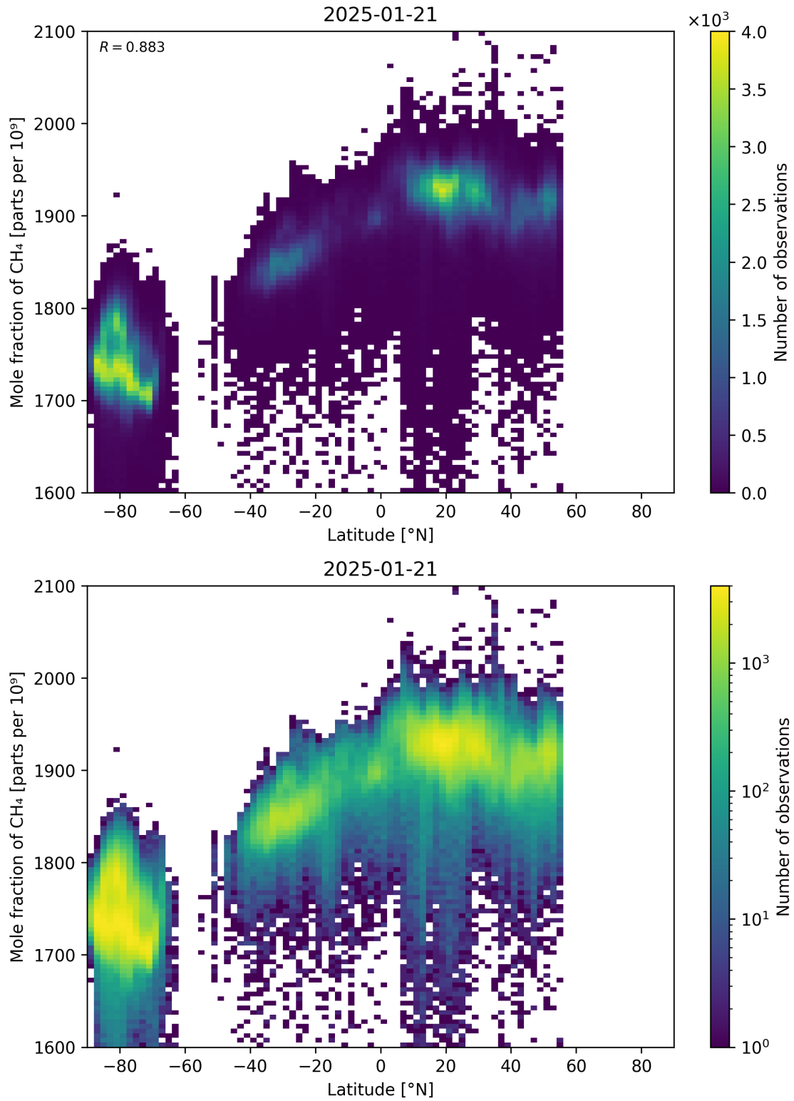
Figure 57: Scatter density plot of “Latitude” against “Mole fraction of CH 4 ” for 2025-01-20 to 2025-01-22.
