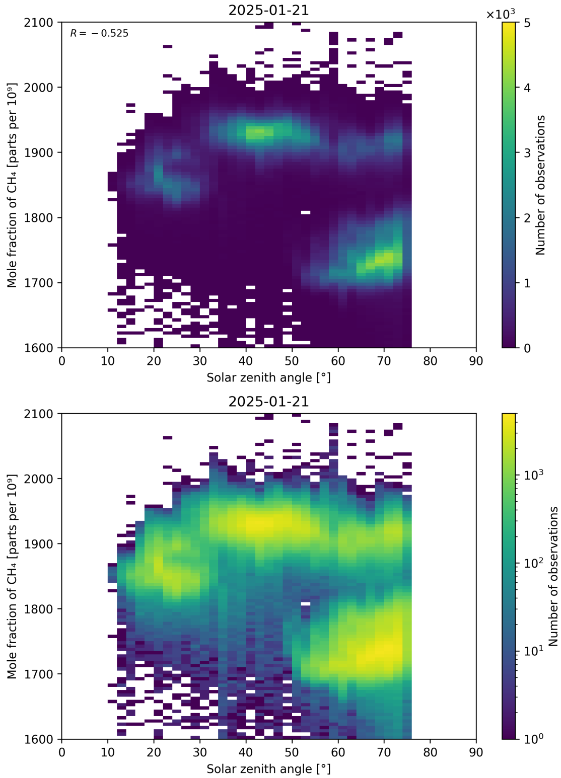
Figure 99: Scatter density plot of “Solar zenith angle” against “Mole fraction of CH 4 ” for 2025-01-20 to 2025-01-22.
