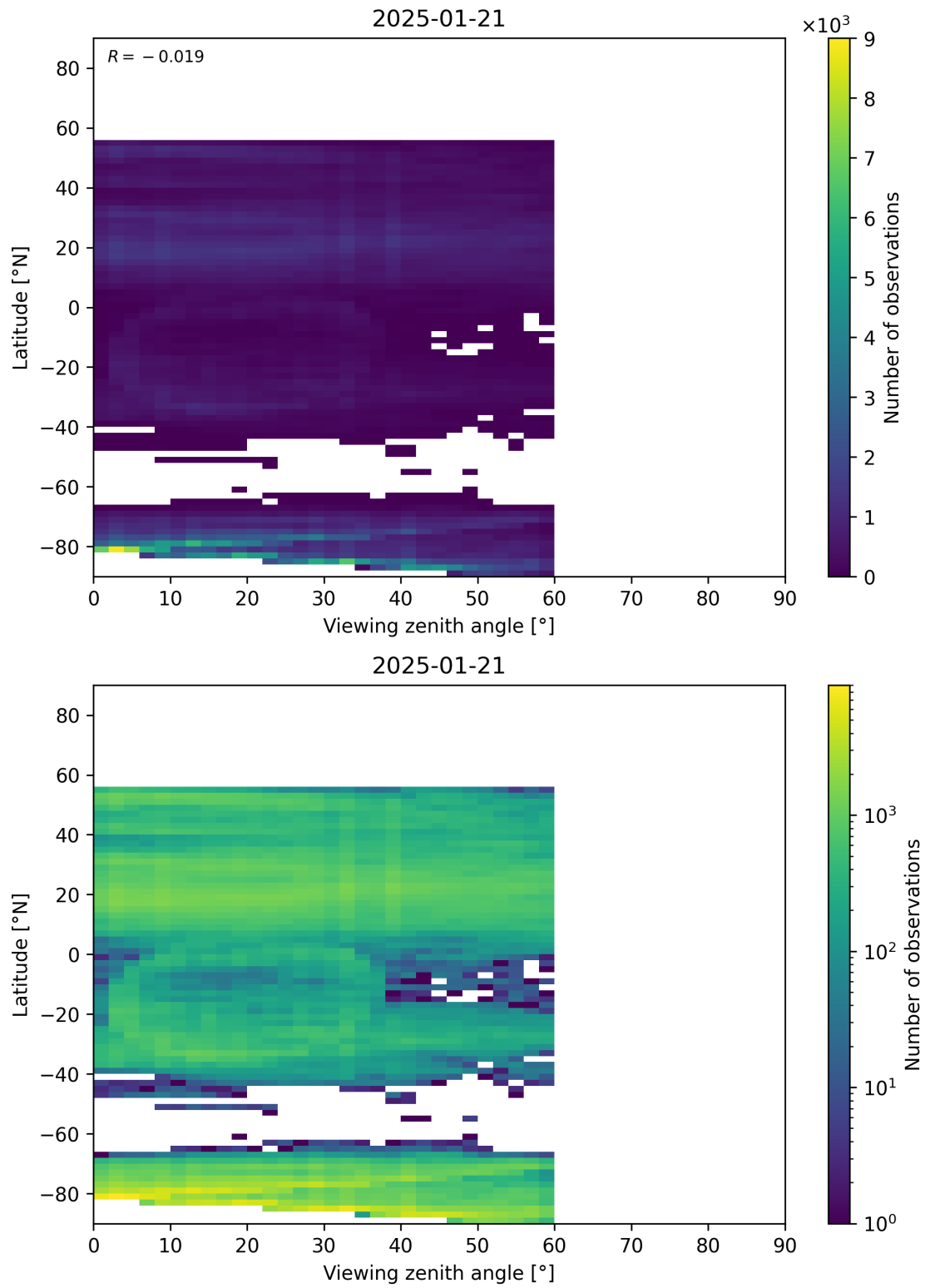
Figure 109: Scatter density plot of “Viewing zenith angle” against “Latitude” for 2025-01-20 to 2025-01-22.
