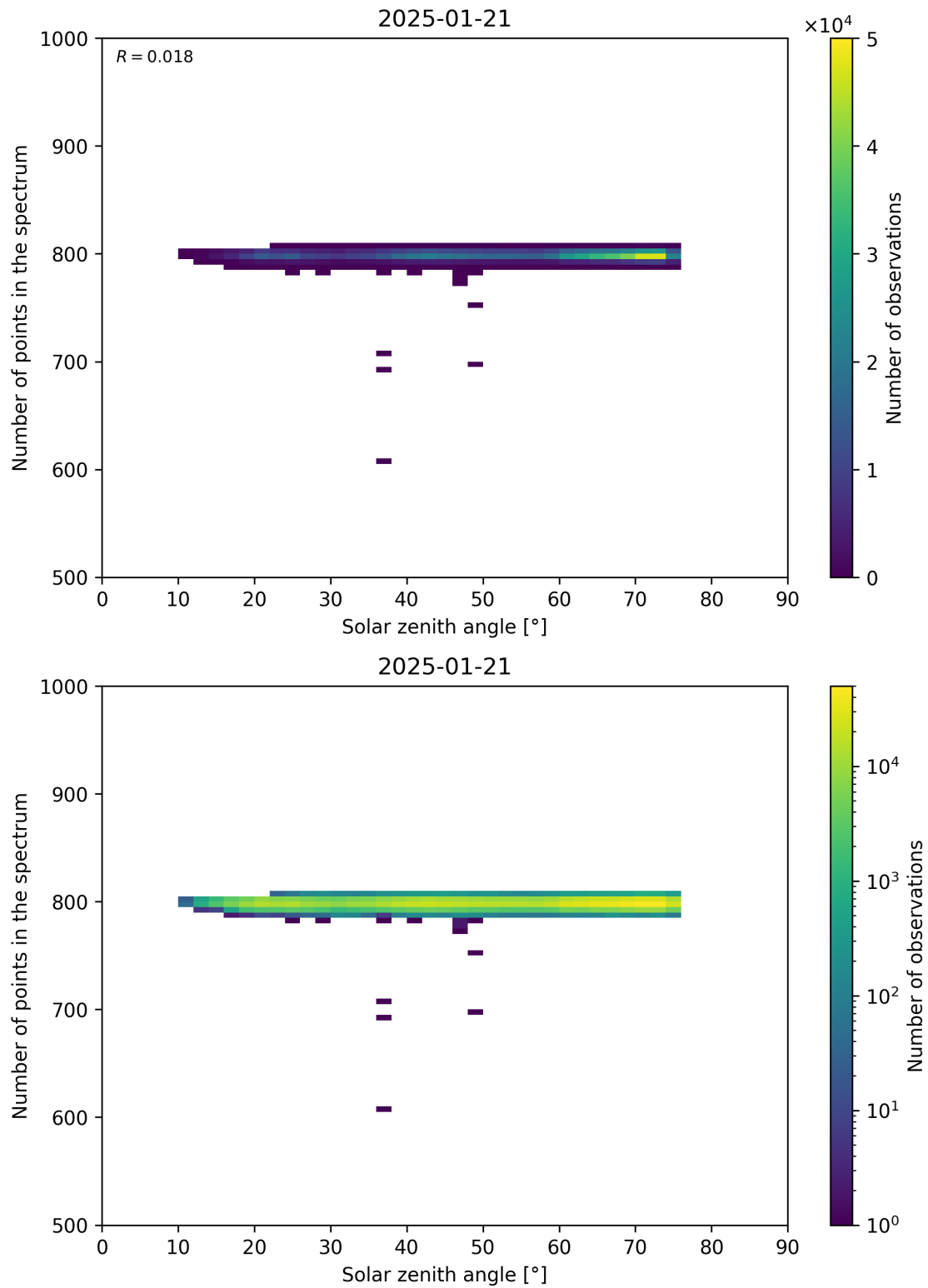
Figure 103: Scatter density plot of “Solar zenith angle” against “Number of points in the spectrum” for 2025-01-20 to 2025-01-22.
