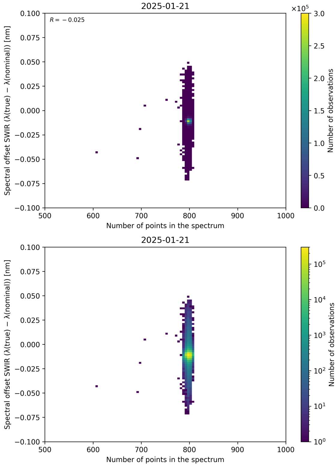
Figure 93: Scatter density plot of “Number of points in the spectrum” against “Spectral offset SWIR ( \lambda_{\text{true}} - \lambda_{\text{nominal}} )” for 2025-01-20 to 2025-01-22.
