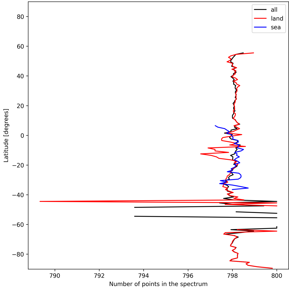
Figure 15: Zonal average of “Number of points in the spectrum” for 2025-01-20 to 2025-01-22.
