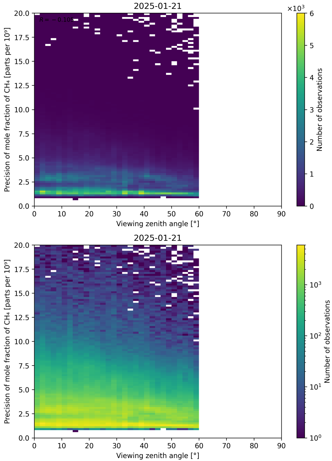
Figure 112: Scatter density plot of “Viewing zenith angle” against “Precision of mole fraction of \text{CH}_4 ” for 2025-01-20 to 2025-01-22.
