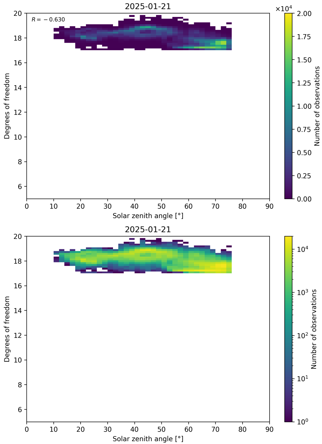
Figure 96: Scatter density plot of “Solar zenith angle” against “Degrees of freedom” for 2025-01-20 to 2025-01-22.
