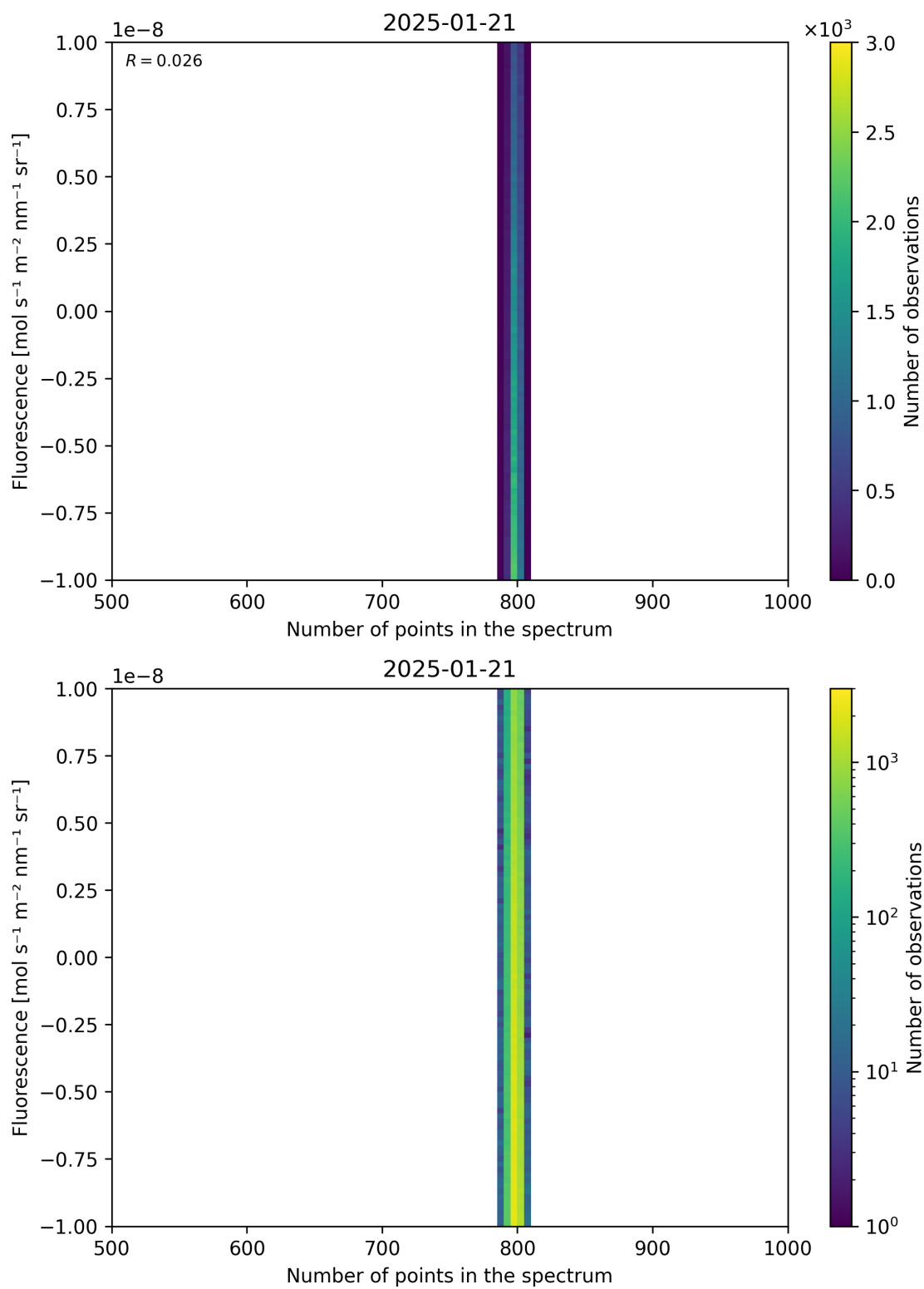
Figure 91: Scatter density plot of “Number of points in the spectrum” against “Fluorescence” for 2025-01-20 to 2025-01-22.
