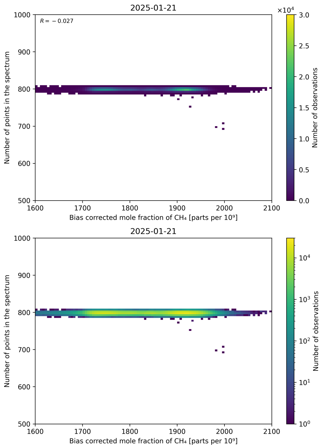
Figure 68: Scatter density plot of “Bias corrected mole fraction of CH 4 ” against “Number of points in the spectrum” for 2025-01-20 to 2025-01-22.
