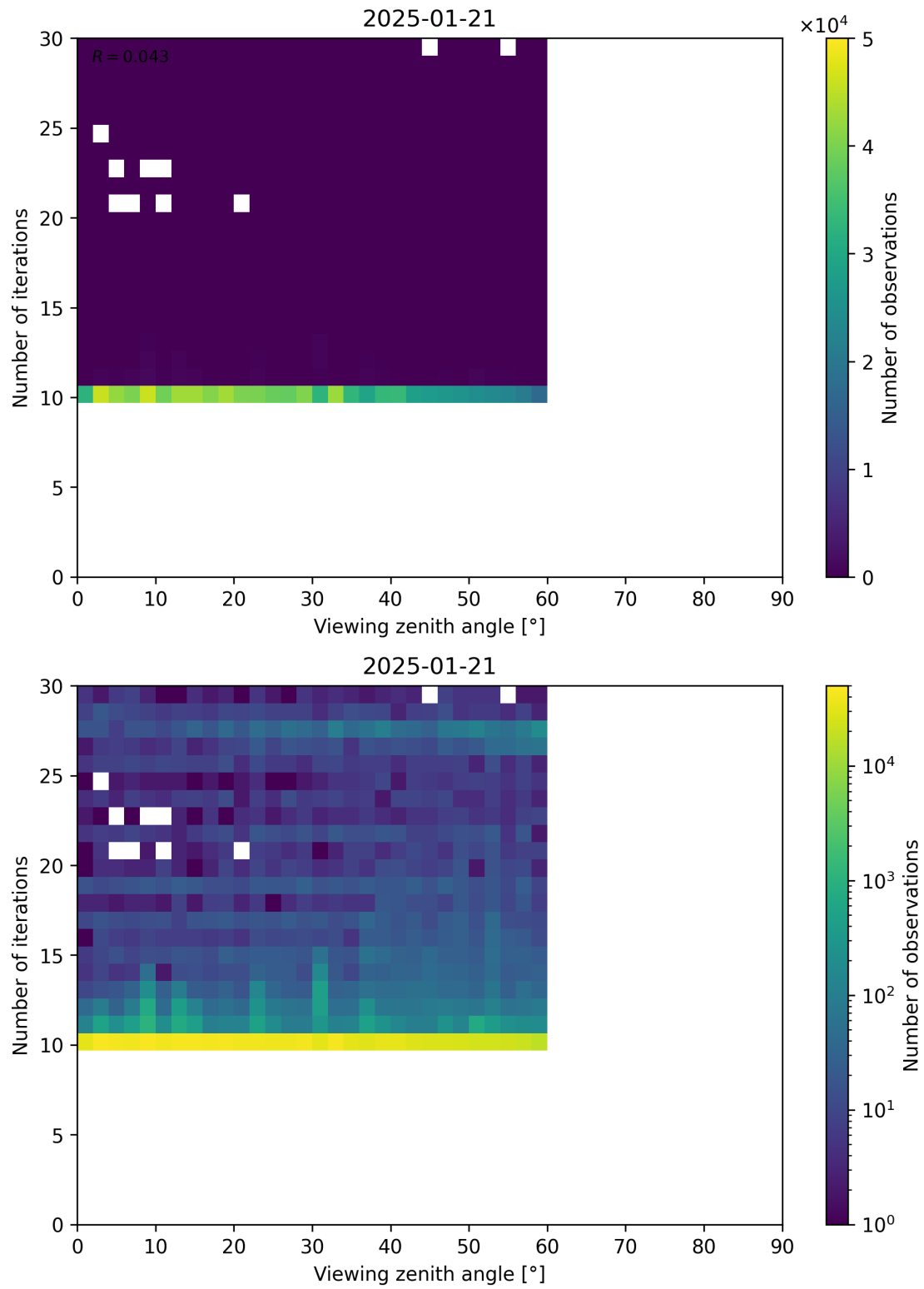
Figure 113: Scatter density plot of “Viewing zenith angle” against “Number of iterations” for 2025-01-20 to 2025-01-22.
