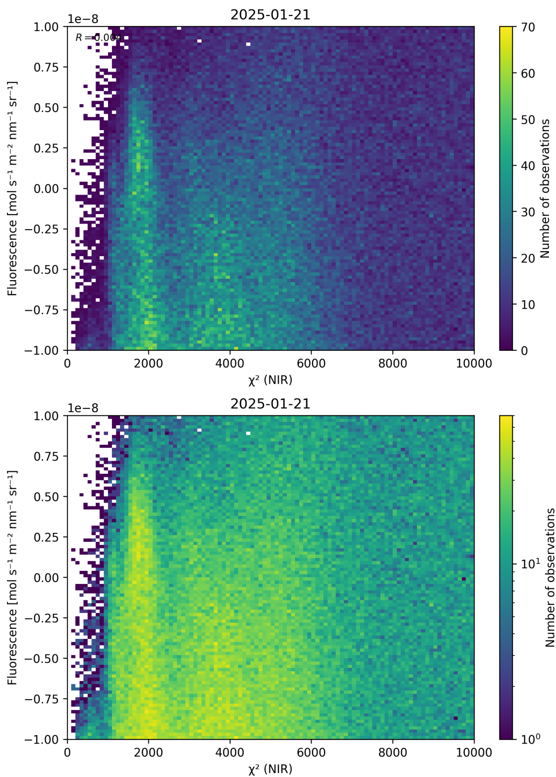
Figure 45: Scatter density plot of “ \chi^2 (NIR)” against “Fluorescence” for 2025-01-20 to 2025-01-22.
