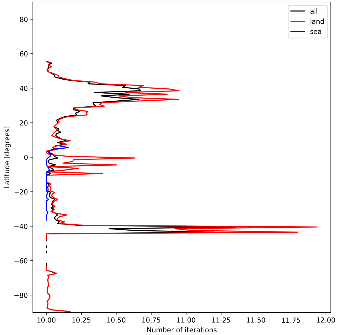
Figure 20: Zonal average of “Number of iterations” for 2025-01-20 to 2025-01-22.
