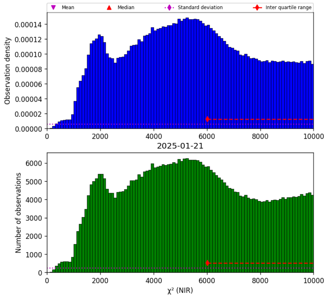
Figure 29: Histogram of " \chi^2 (NIR)" for 2025-01-20 to 2025-01-22
