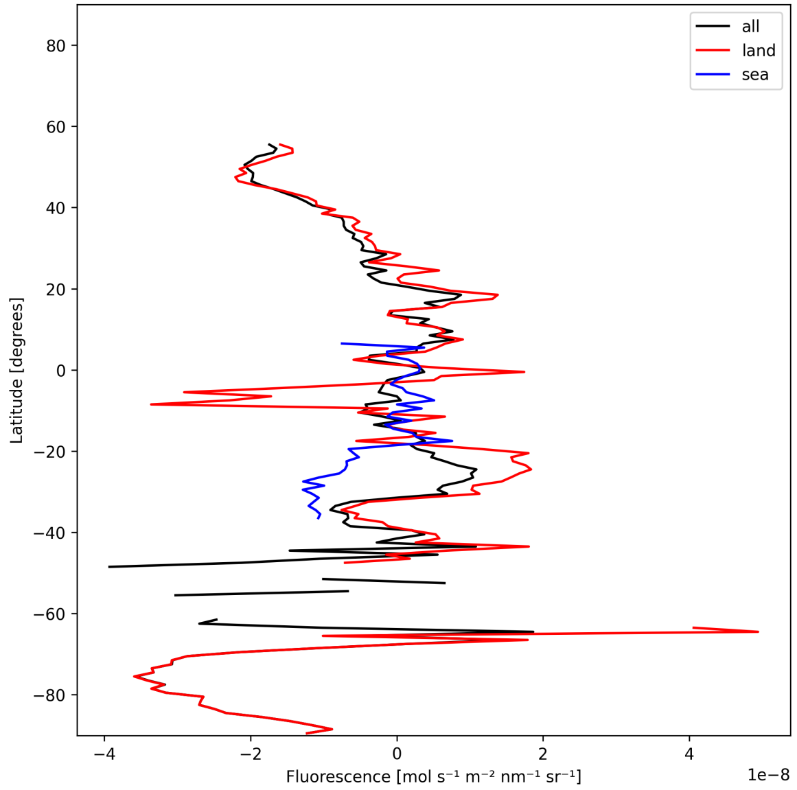
Figure 21: Zonal average of “Fluorescence” for 2025-01-20 to 2025-01-22.
