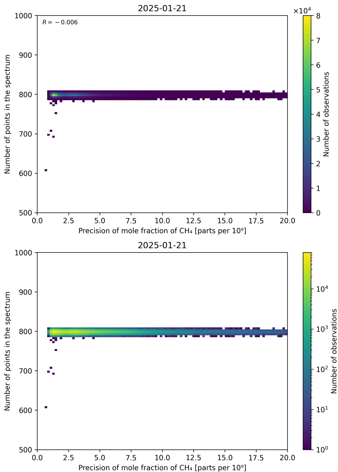
Figure 84: Scatter density plot of “Precision of mole fraction of CH 4 ” against “Number of points in the spectrum” for 2025-01-20 to 2025-01-22.
