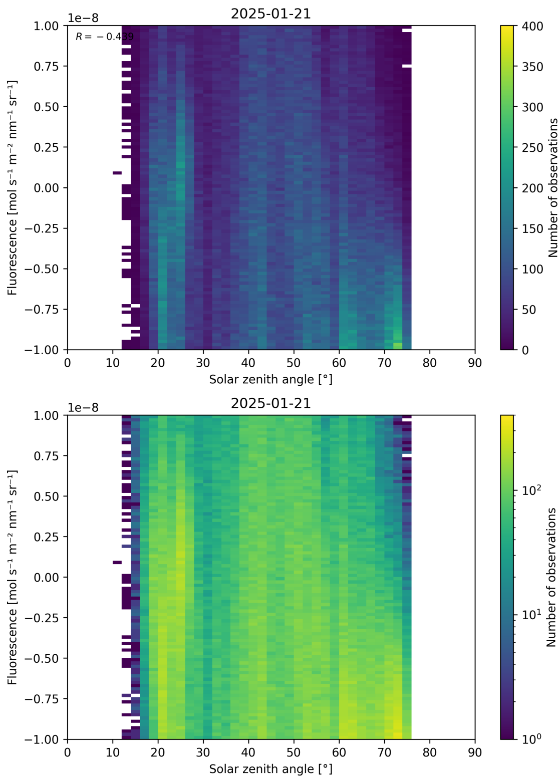
Figure 97: Scatter density plot of “Solar zenith angle” against “Fluorescence” for 2025-01-20 to 2025-01-22.
