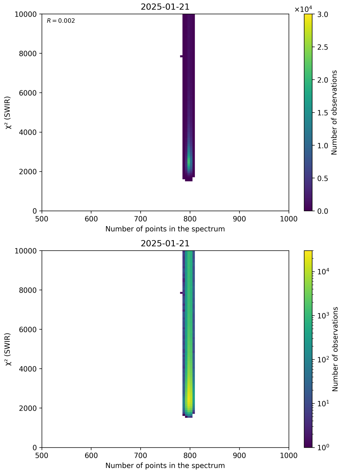
Figure 89: Scatter density plot of “Number of points in the spectrum” against “ \chi^2 (SWIR)” for 2025-01-20 to 2025-01-22.
