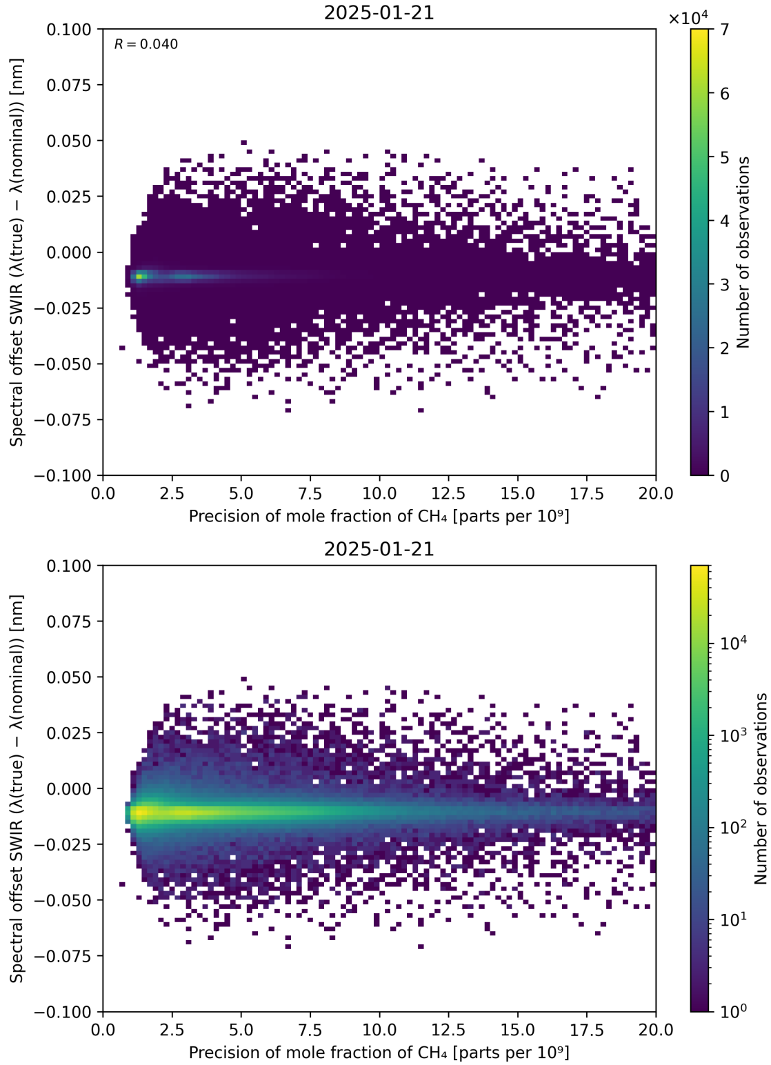
Figure 85: Scatter density plot of “Precision of mole fraction of CH 4 ” against “Spectral offset SWIR ( \lambda_{\text{true}} - \lambda_{\text{nominal}} )” for 2025-01-20 to 2025-01-22.
