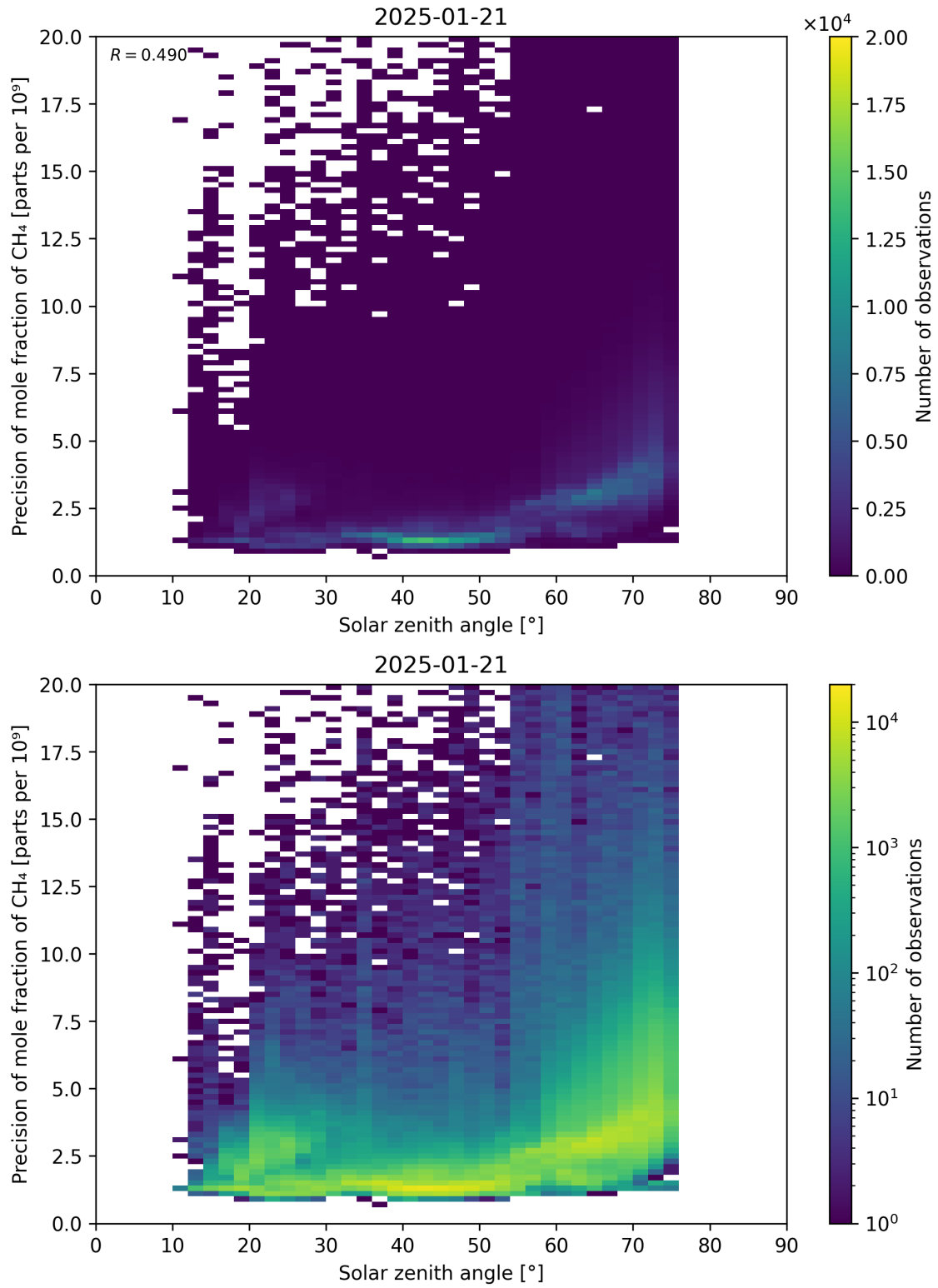
Figure 101: Scatter density plot of “Solar zenith angle” against “Precision of mole fraction of CH 4 ” for 2025-01-20 to 2025-01-22.
