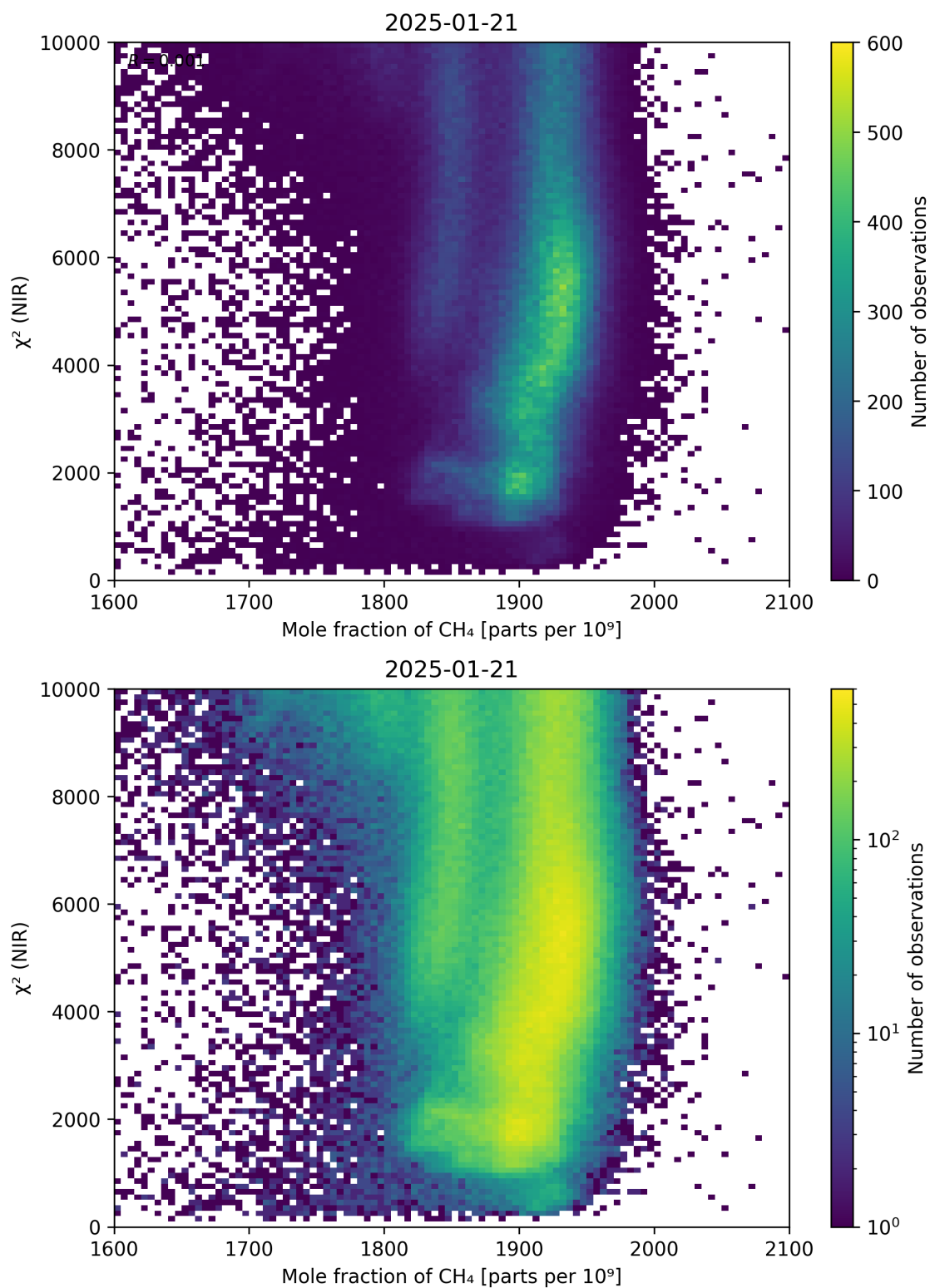
Figure 70: Scatter density plot of “Mole fraction of CH 4 ” against “ \chi^2 (NIR)” for 2025-01-20 to 2025-01-22.
