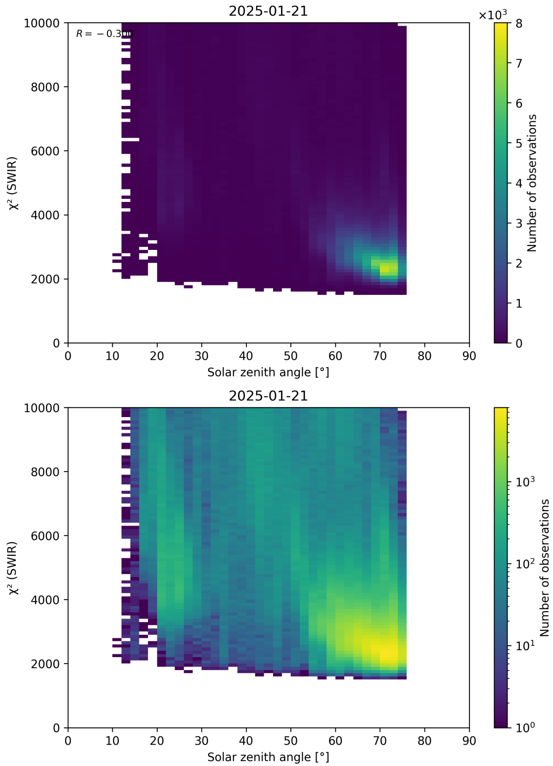
Figure 95: Scatter density plot of “Solar zenith angle” against “ \chi^2 (SWIR)” for 2025-01-20 to 2025-01-22.
