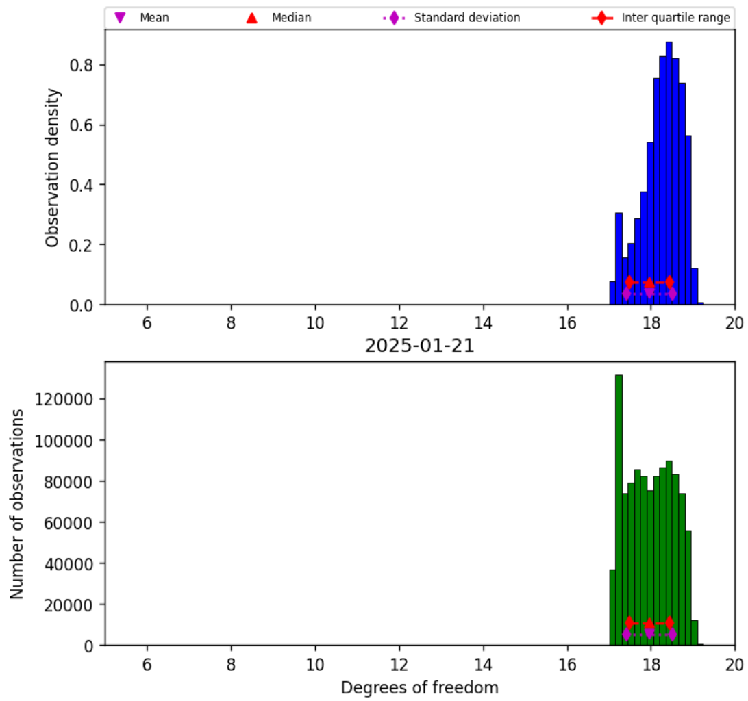
Figure 30: Histogram of "Degrees of freedom" for 2025-01-20 to 2025-01-22
