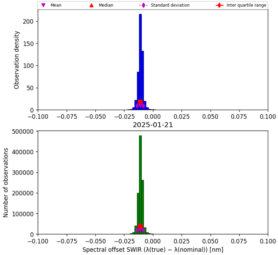
Figure 27: Histogram of “Spectral offset SWIR ( \lambda_{\text{true}} - \lambda_{\text{nominal}} )” for 2025-01-20 to 2025-01-22
