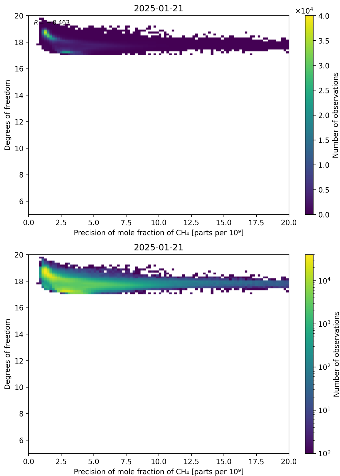
Figure 80: Scatter density plot of “Precision of mole fraction of CH 4 ” against “Degrees of freedom” for 2025-01-20 to 2025-01-22.
