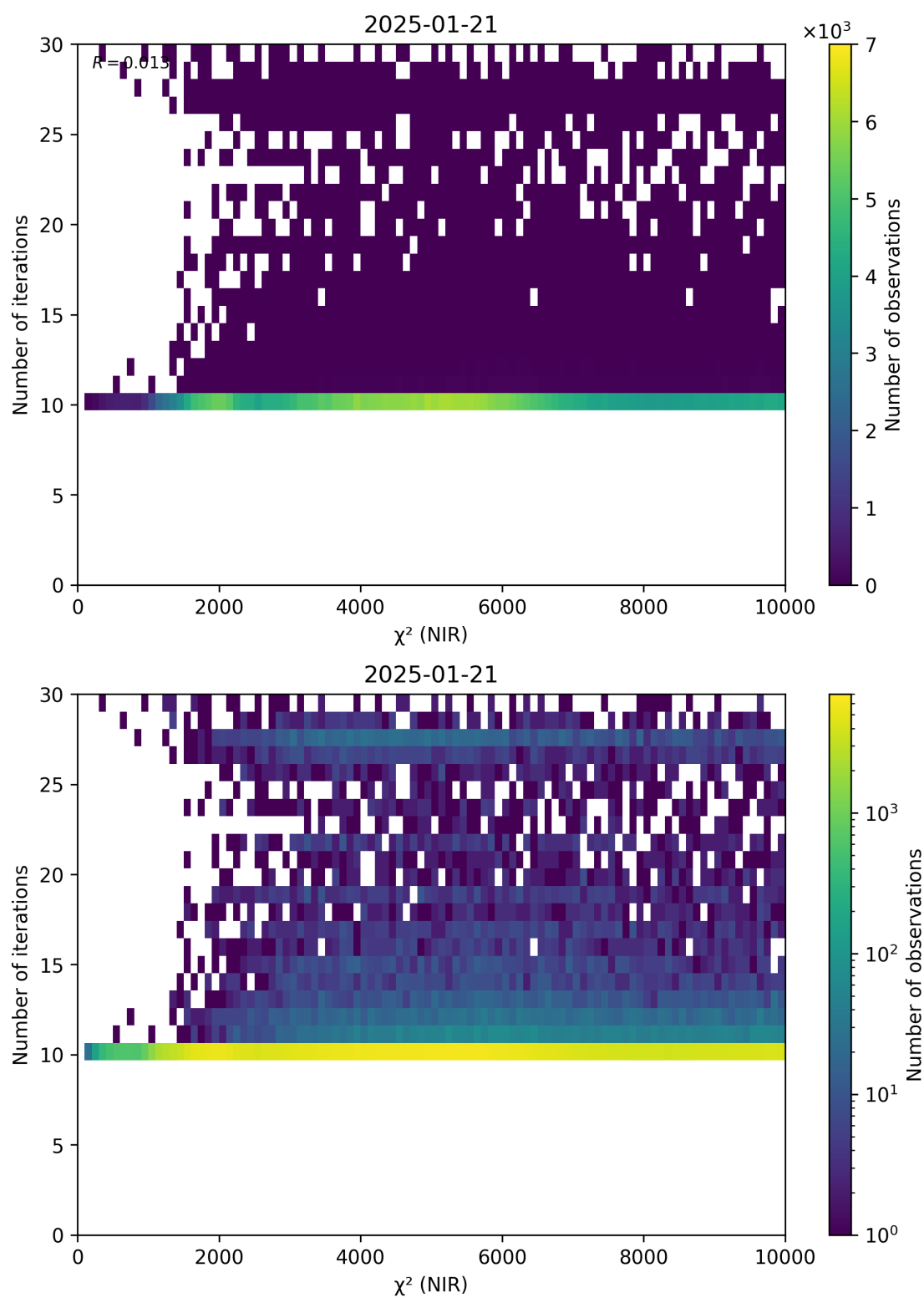
Figure 46: Scatter density plot of “ \chi^2 (NIR)” against “Number of iterations” for 2025-01-20 to 2025-01-22.
