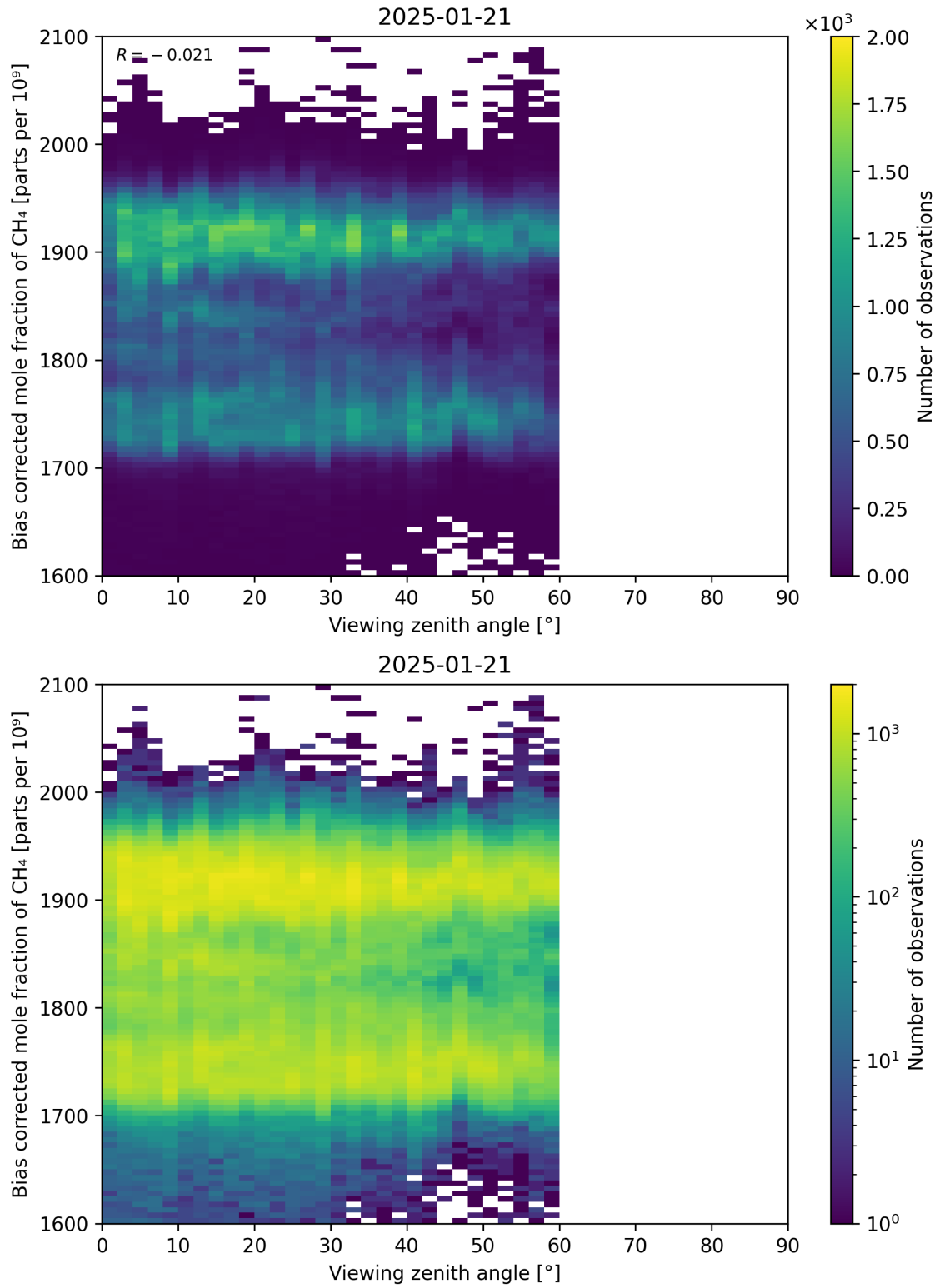
Figure 111: Scatter density plot of “Viewing zenith angle” against “Bias corrected mole fraction of CH 4 ” for 2025-01-20 to 2025-01-22.
