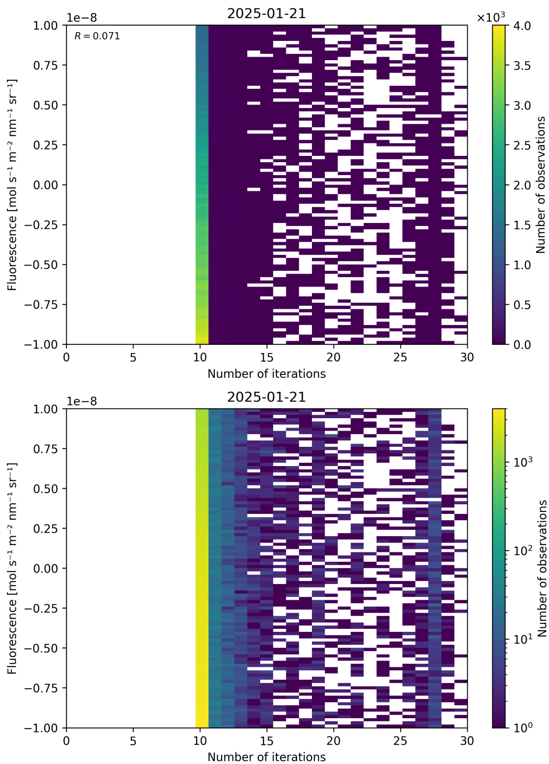
Figure 87: Scatter density plot of “Number of iterations” against “Fluorescence” for 2025-01-20 to 2025-01-22.
