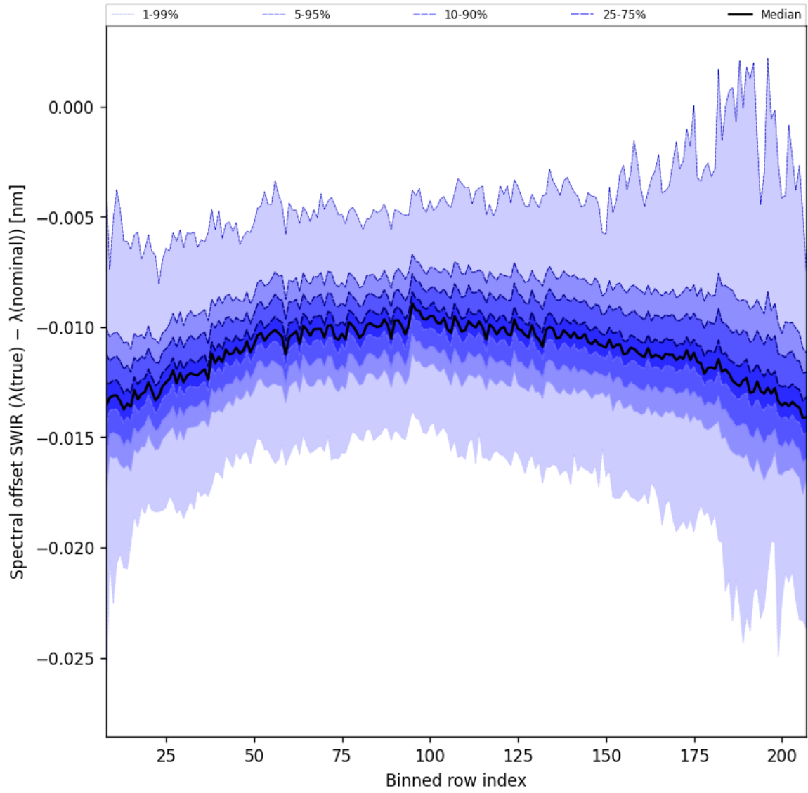
Figure 38: Along track statistics of “Spectral offset SWIR ( \lambda_{\text{true}} - \lambda_{\text{nominal}} )” for 2025-01-20 to 2025-01-22
