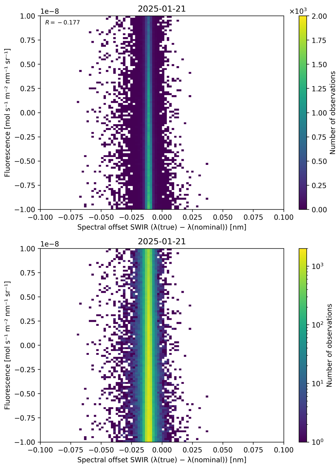
Figure 120: Scatter density plot of “Spectral offset SWIR ( \lambda_{\text{true}} - \lambda_{\text{nominal}} )” against “Fluorescence” for 2025-01-20 to 2025-01-22.
