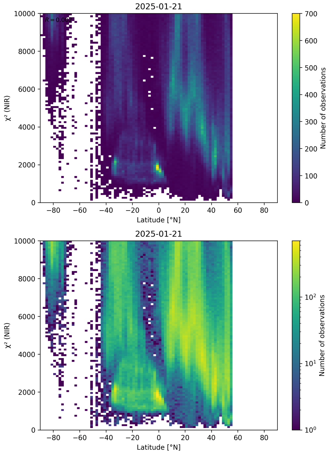
Figure 53: Scatter density plot of “Latitude” against “ \chi^2 (NIR)” for 2025-01-20 to 2025-01-22.
