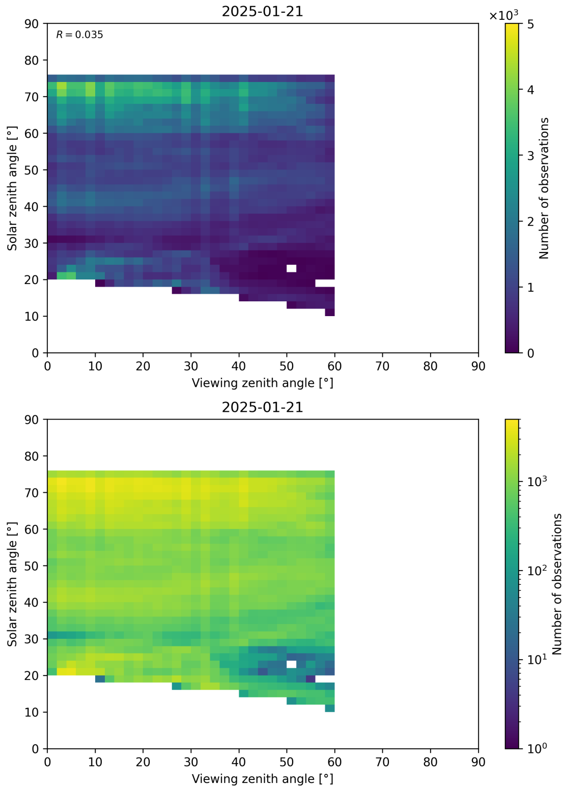
Figure 115: Scatter density plot of “Viewing zenith angle” against “Solar zenith angle” for 2025-01-20 to 2025-01-22.
