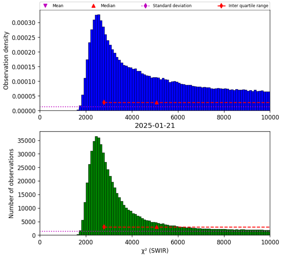
Figure 28: Histogram of “ \chi^2 (SWIR)” for 2025-01-20 to 2025-01-22
