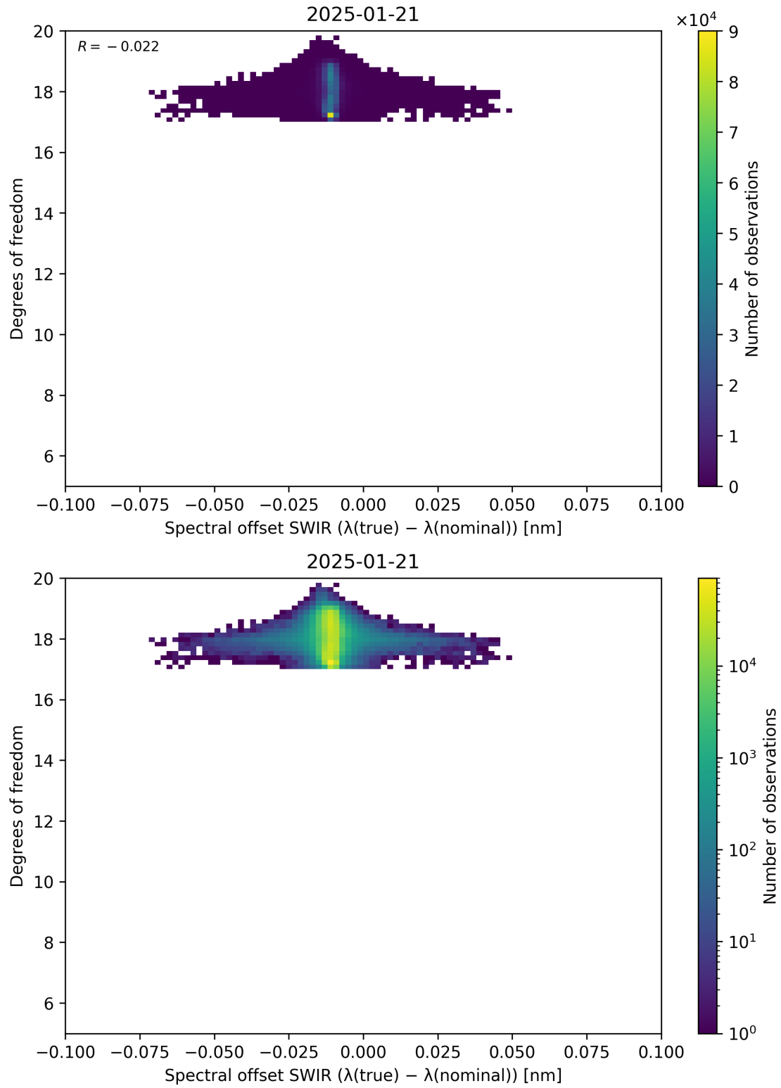
Figure 119: Scatter density plot of “Spectral offset SWIR ( \lambda_{\text{true}} - \lambda_{\text{nominal}} )” against “Degrees of freedom” for 2025-01-20 to 2025-01-22.
