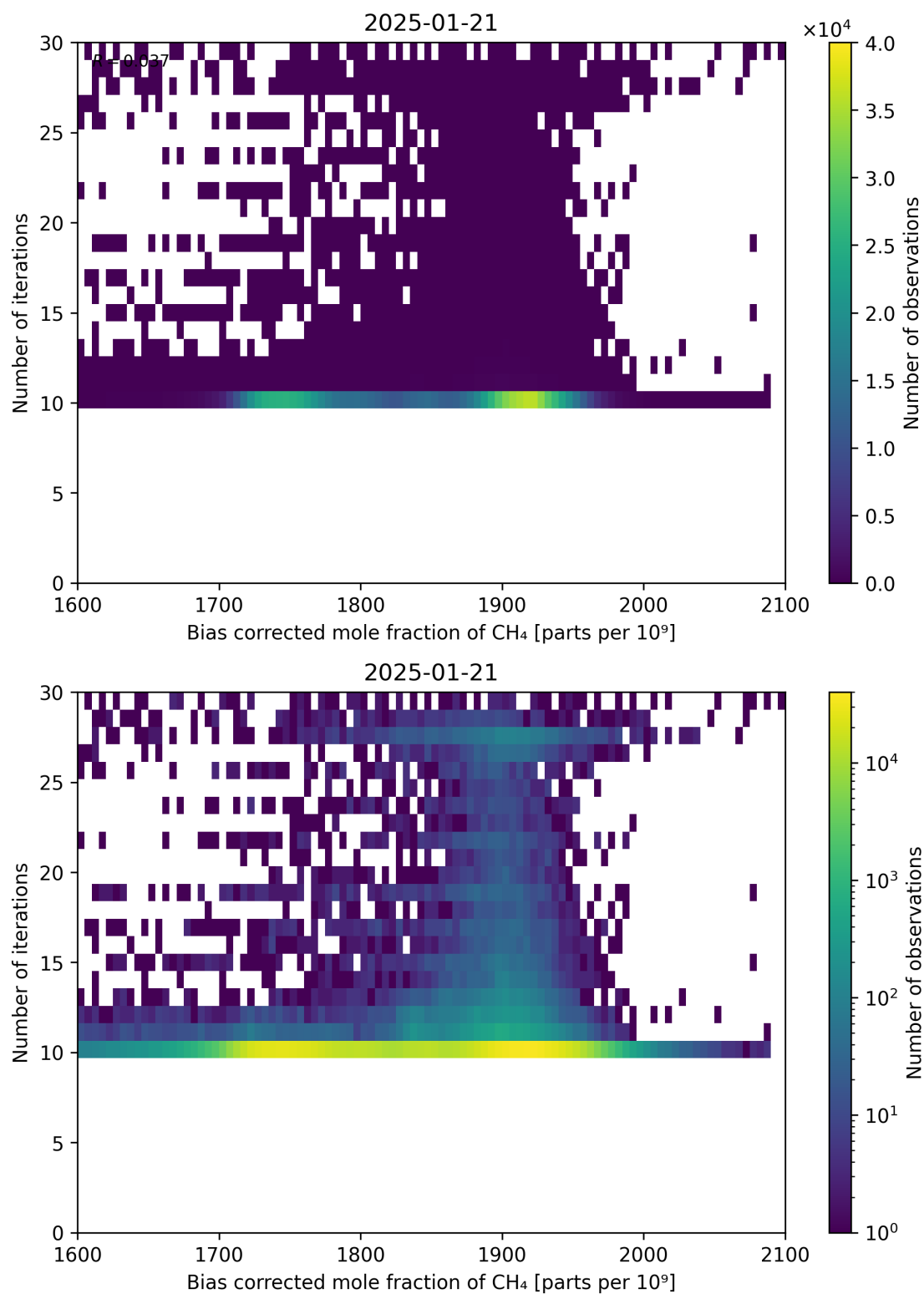
Figure 67: Scatter density plot of “Bias corrected mole fraction of \text{CH}_4 ” against “Number of iterations” for 2025-01-20 to 2025-01-22.
