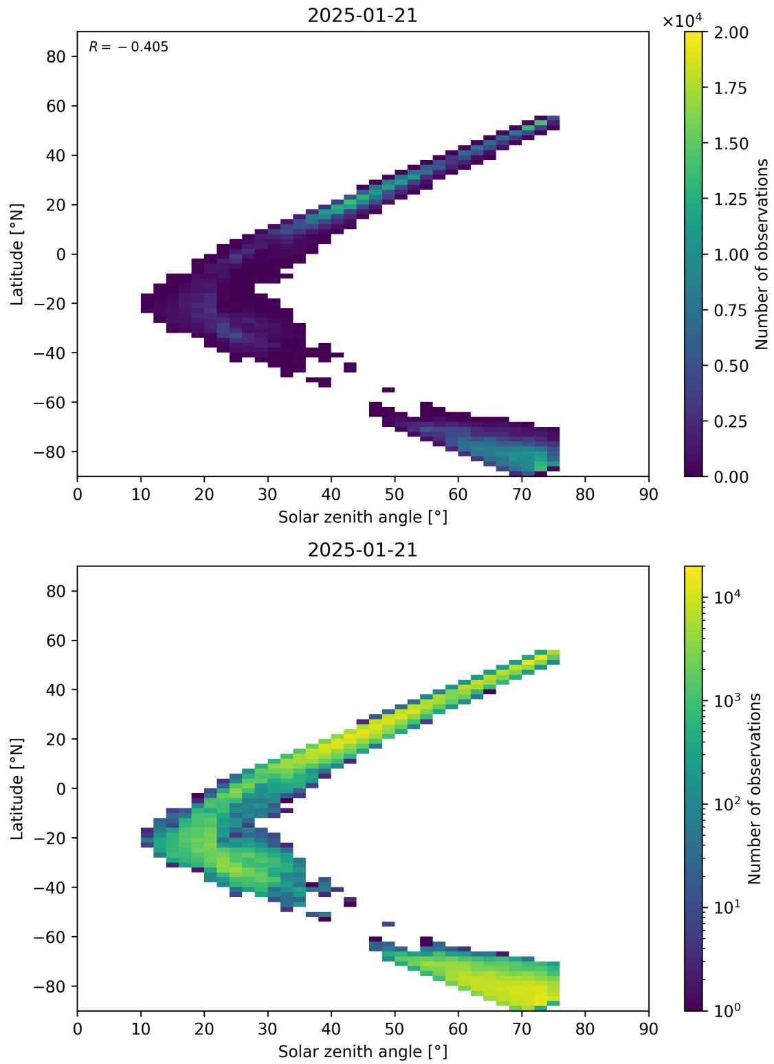
Figure 98: Scatter density plot of “Solar zenith angle” against “Latitude” for 2025-01-20 to 2025-01-22.
