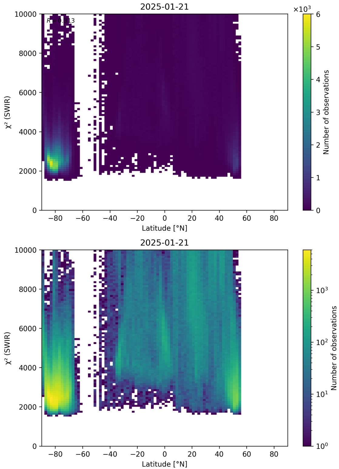
Figure 54: Scatter density plot of “Latitude” against “ \chi^2 (SWIR)” for 2025-01-20 to 2025-01-22.
