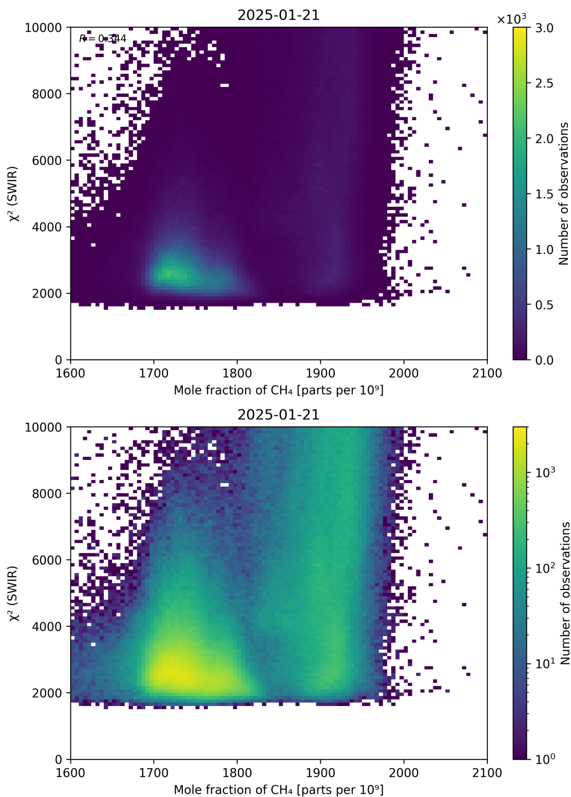
Figure 71: Scatter density plot of “Mole fraction of CH 4 ” against “ \chi^2 (SWIR)” for 2025-01-20 to 2025-01-22.
