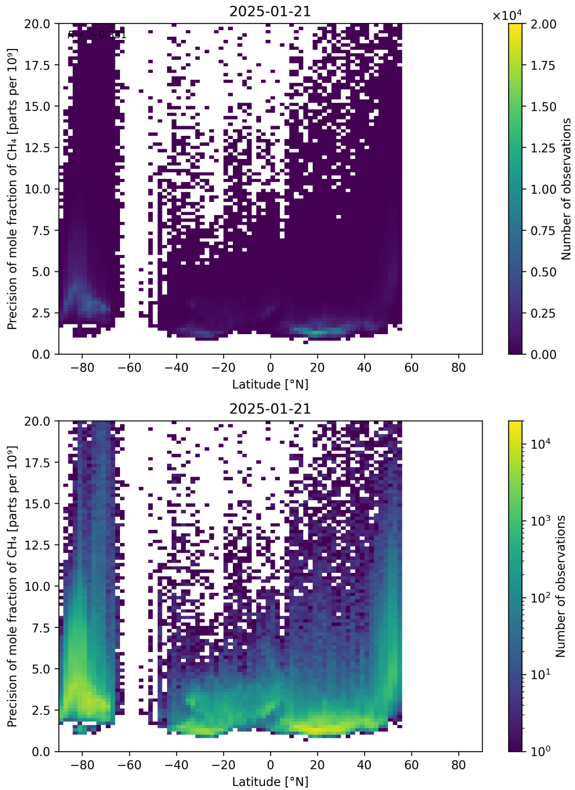
Figure 59: Scatter density plot of “Latitude” against “Precision of mole fraction of CH 4 ” for 2025-01-20 to 2025-01-22.
