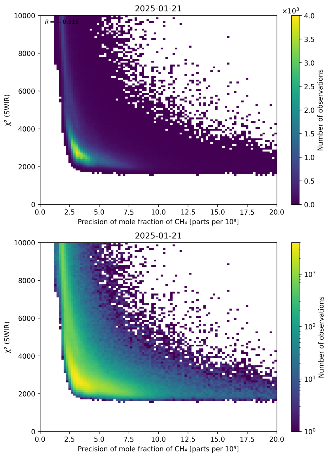
Figure 79: Scatter density plot of “Precision of mole fraction of \text{CH}_4 ” against “ \chi^2 (SWIR)” for 2025-01-20 to 2025-01-22.
