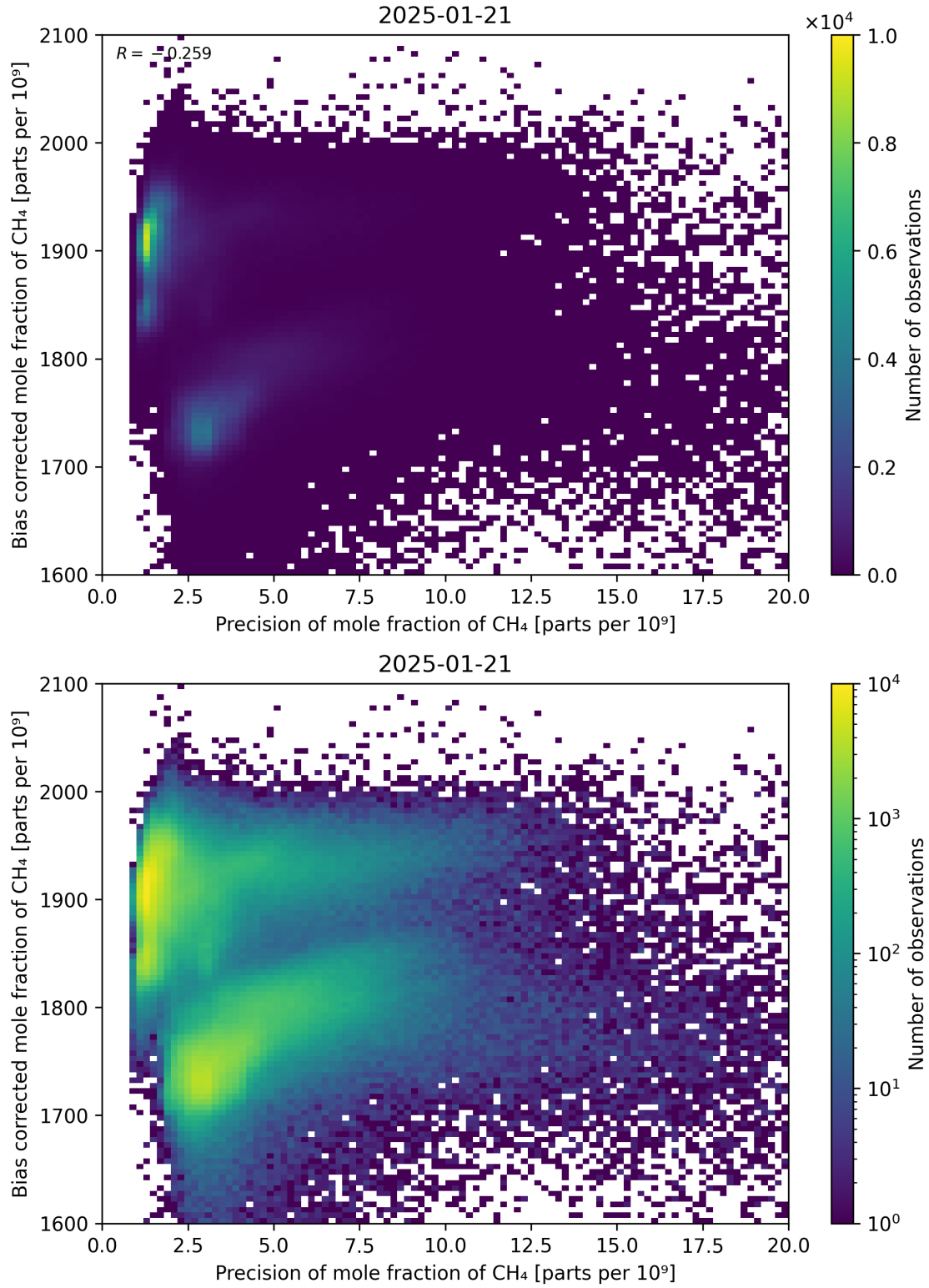
Figure 82: Scatter density plot of “Precision of mole fraction of \text{CH}_4 ” against “Bias corrected mole fraction of \text{CH}_4 ” for 2025-01-20 to 2025-01-22.
