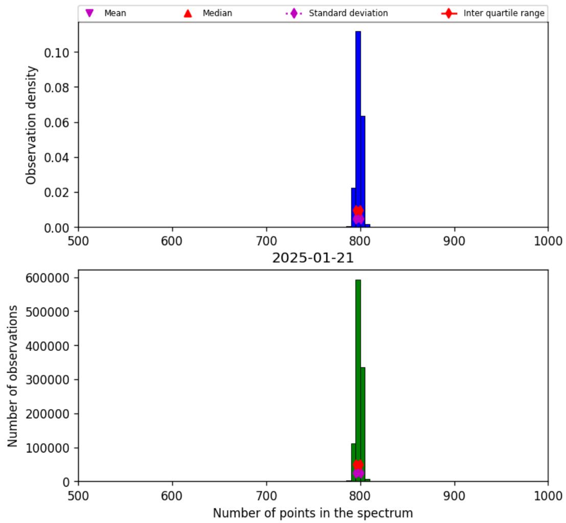
Figure 26: Histogram of “Number of points in the spectrum” for 2025-01-20 to 2025-01-22
