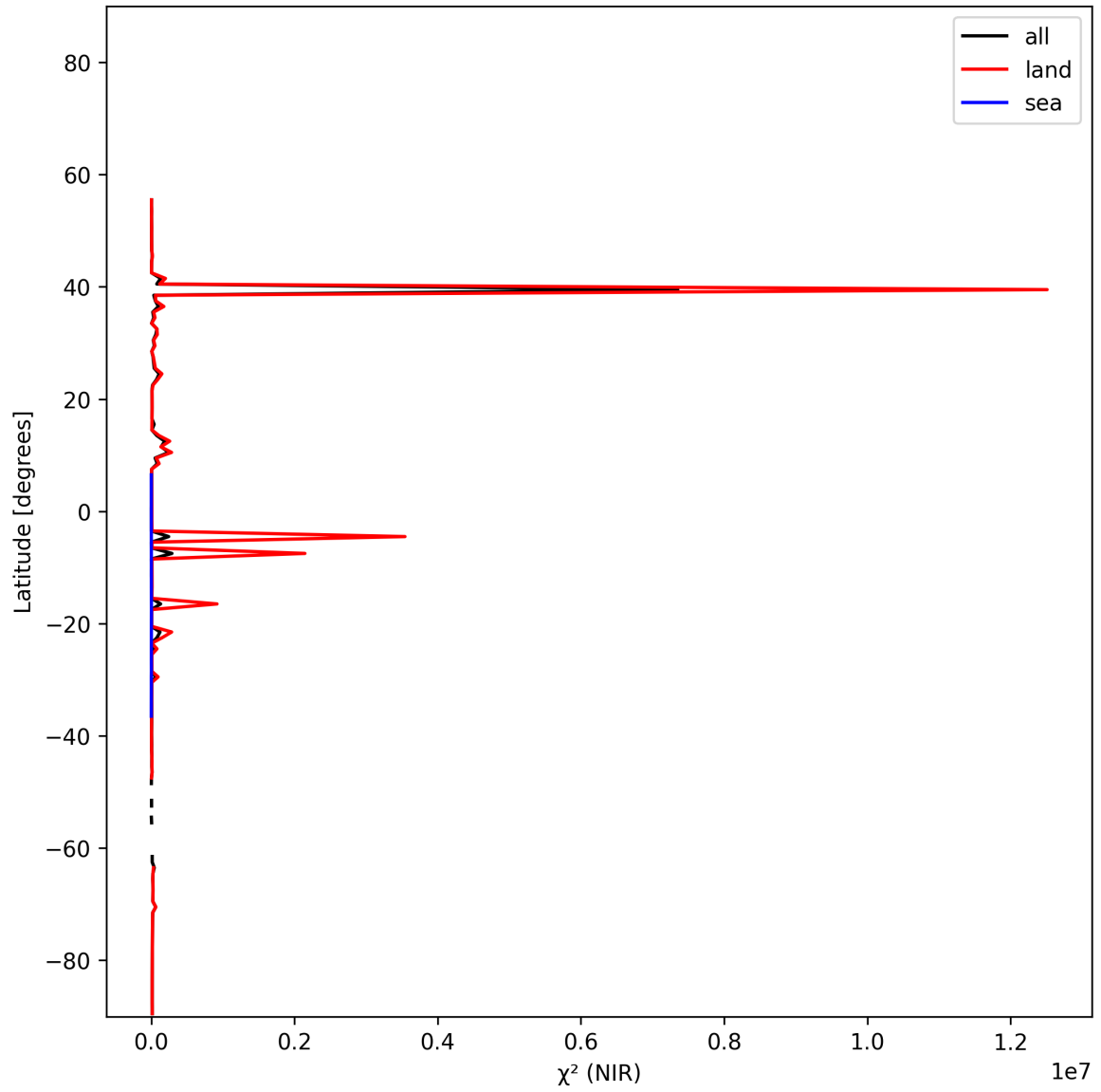
Figure 18: Zonal average of “ \chi^2 (NIR)” for 2025-01-20 to 2025-01-22.
