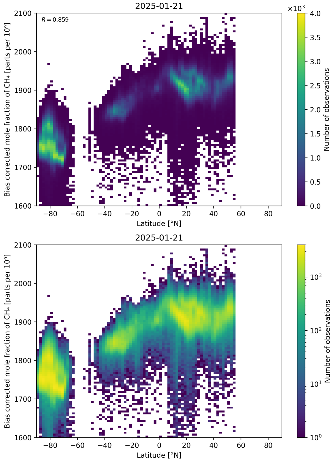
Figure 58: Scatter density plot of “Latitude” against “Bias corrected mole fraction of CH 4 ” for 2025-01-20 to 2025-01-22.
