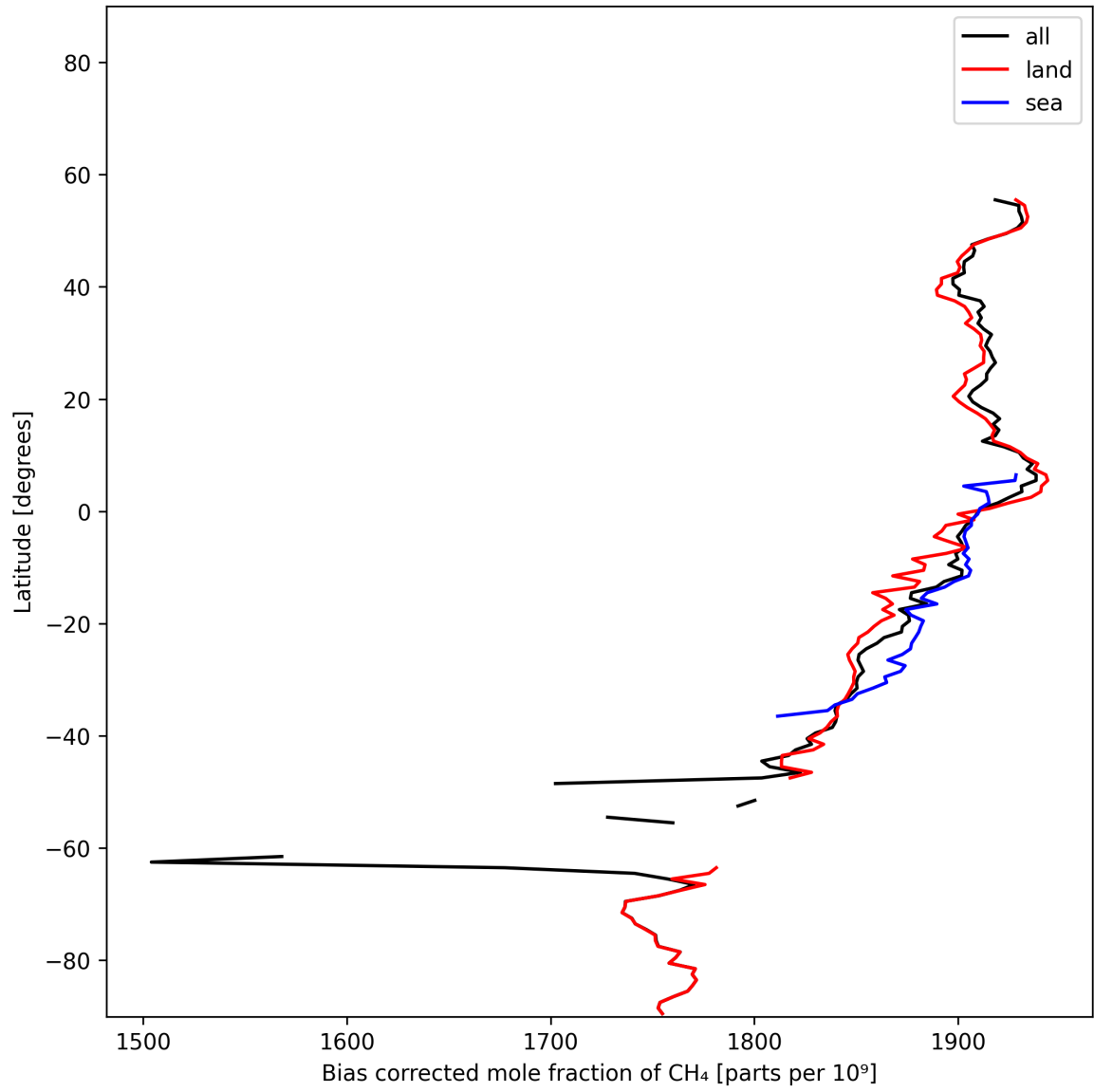
Figure 14: Zonal average of “Bias corrected mole fraction of CH 4 ” for 2025-01-20 to 2025-01-22.
