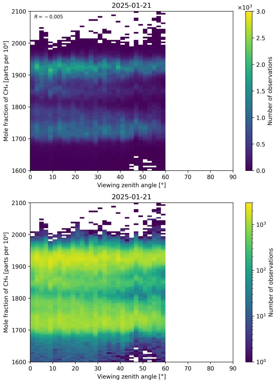
Figure 110: Scatter density plot of “Viewing zenith angle” against “Mole fraction of CH 4 ” for 2025-01-20 to 2025-01-22.
