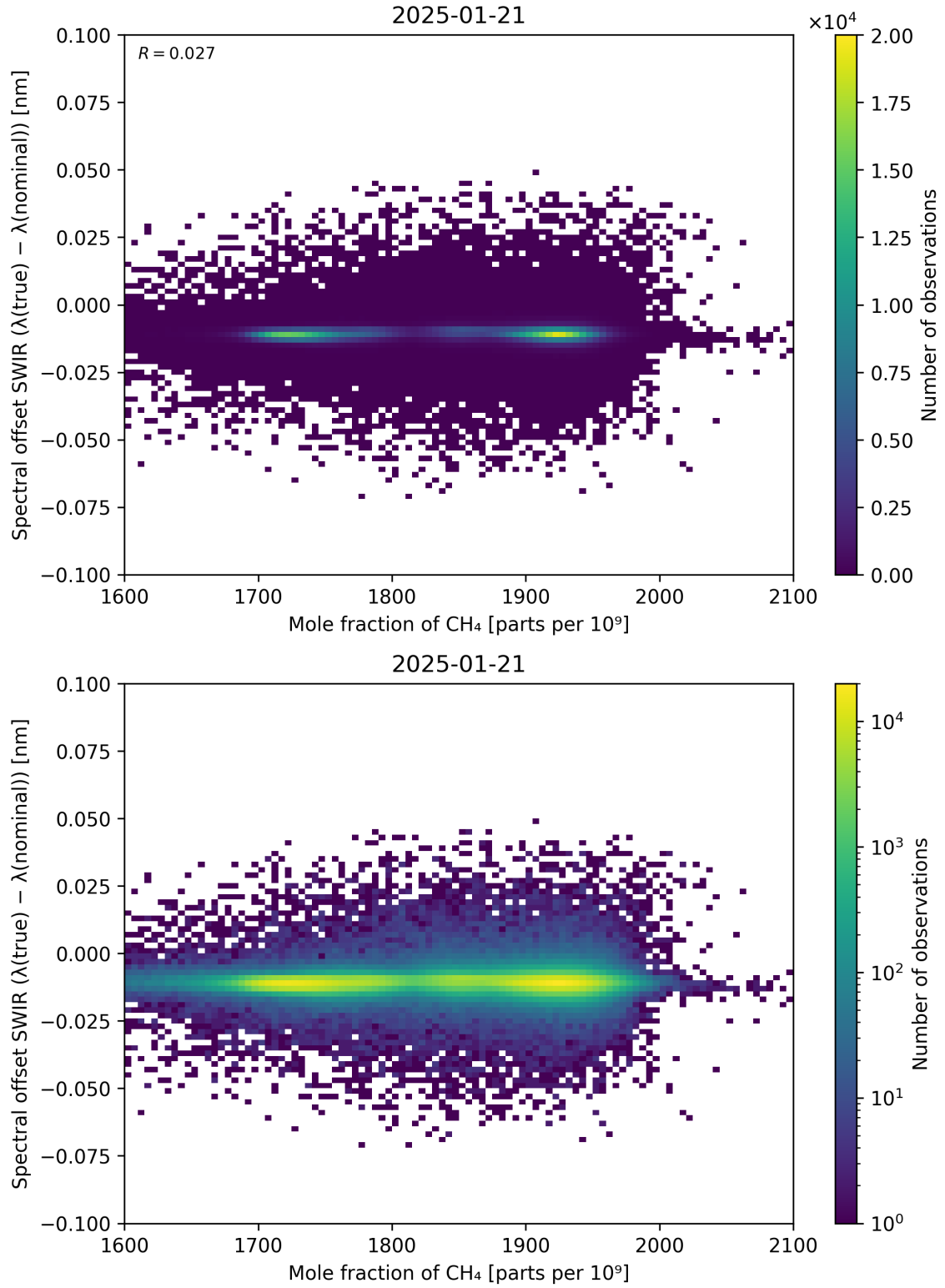
Figure 86: Scatter density plot of “Mole fraction of CH 4 ” against “Spectral offset SWIR ( \lambda_{\text{true}} - \lambda_{\text{nominal}} )” for 2025-01-20 to 2025-01-22.
