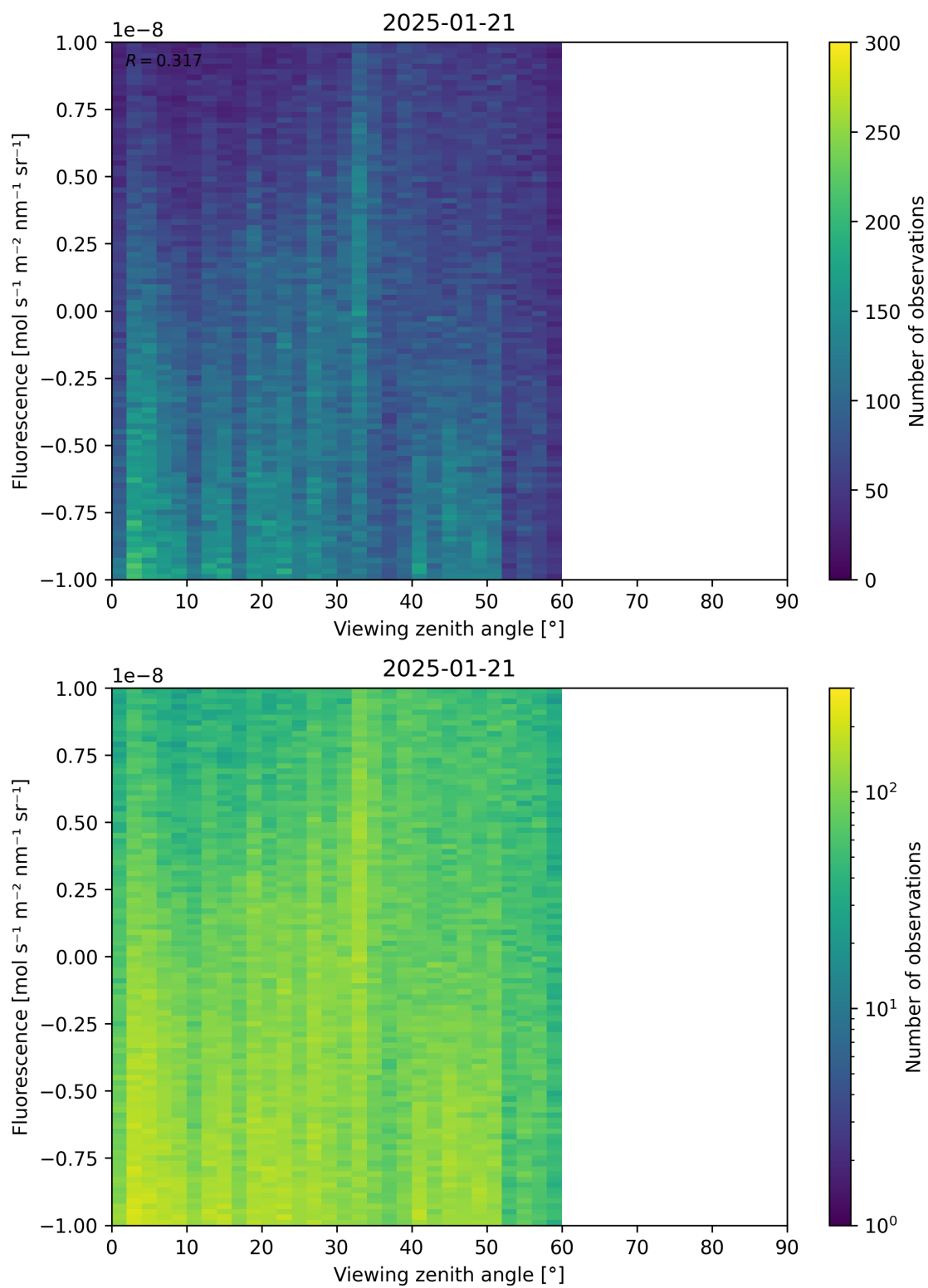
Figure 108: Scatter density plot of “Viewing zenith angle” against “Fluorescence” for 2025-01-20 to 2025-01-22.
