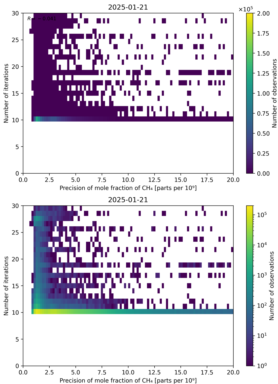
Figure 83: Scatter density plot of “Precision of mole fraction of CH 4 ” against “Number of iterations” for 2025-01-20 to 2025-01-22.
