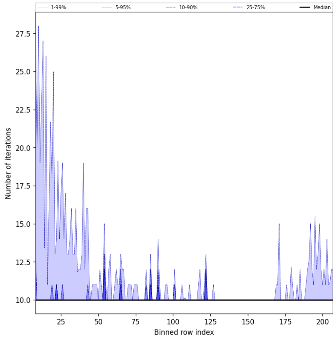
Figure 42: Along track statistics of “Number of iterations” for 2025-01-20 to 2025-01-22
