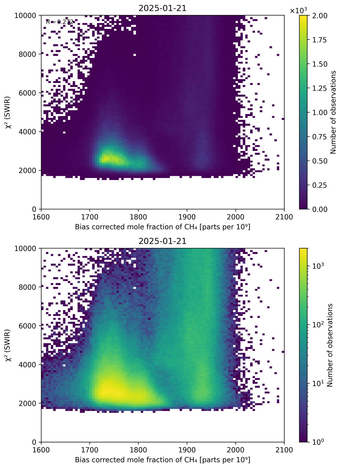
Figure 64: Scatter density plot of “Bias corrected mole fraction of \text{CH}_4 ” against “ \chi^2 (SWIR)” for 2025-01-20 to 2025-01-22.
