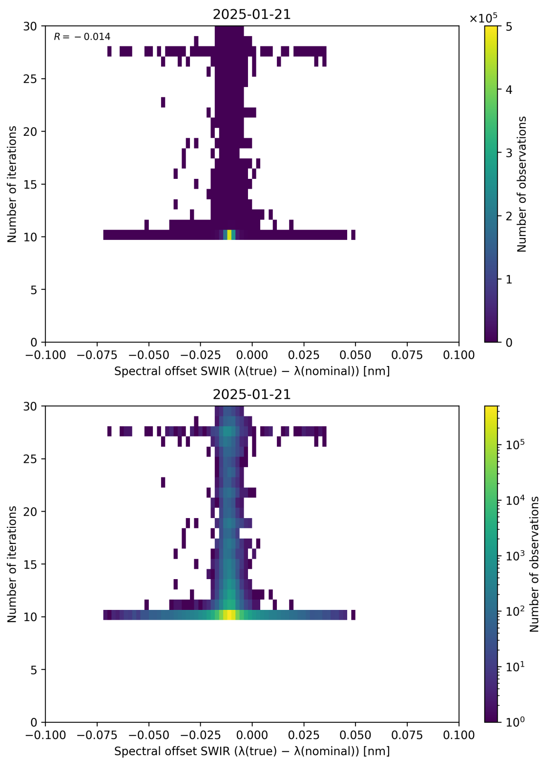
Figure 121: Scatter density plot of “Spectral offset SWIR ( \lambda_{\text{true}} - \lambda_{\text{nominal}} )” against “Number of iterations” for 2025-01-20 to 2025-01-22.
