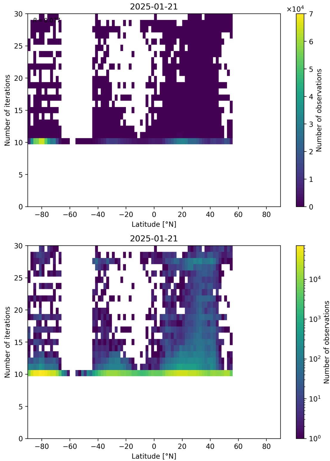
Figure 60: Scatter density plot of “Latitude” against “Number of iterations” for 2025-01-20 to 2025-01-22.
