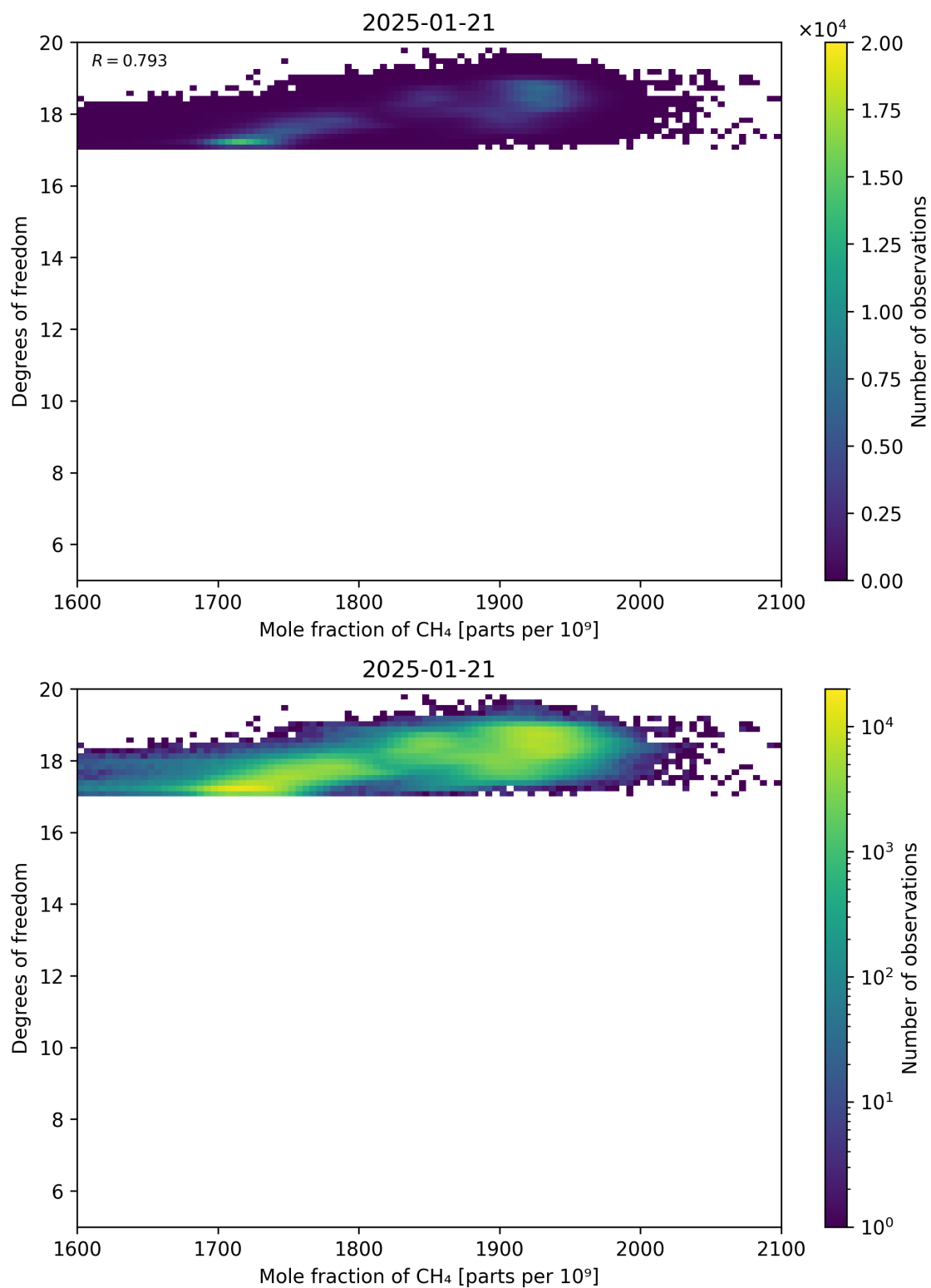
Figure 72: Scatter density plot of “Mole fraction of CH 4 ” against “Degrees of freedom” for 2025-01-20 to 2025-01-22.
