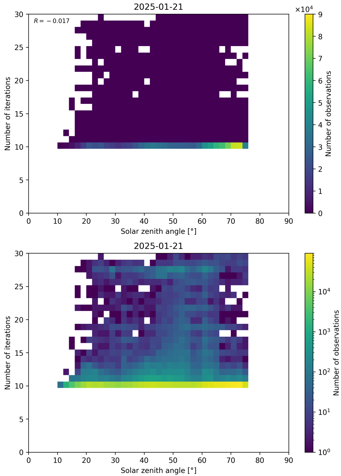
Figure 102: Scatter density plot of “Solar zenith angle” against “Number of iterations” for 2025-01-20 to 2025-01-22.
