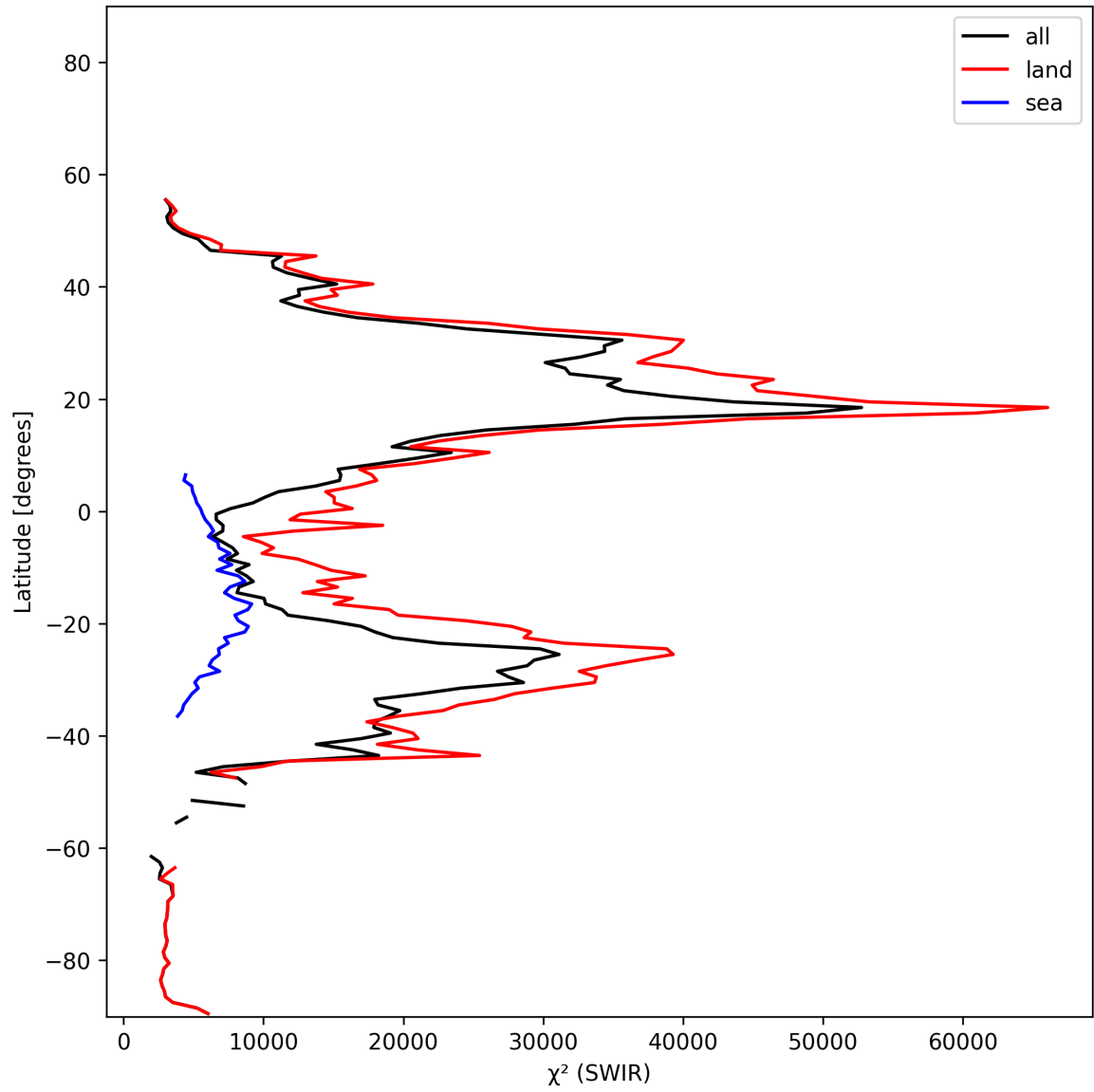
Figure 17: Zonal average of “ \chi^2 (SWIR)” for 2025-01-20 to 2025-01-22.
