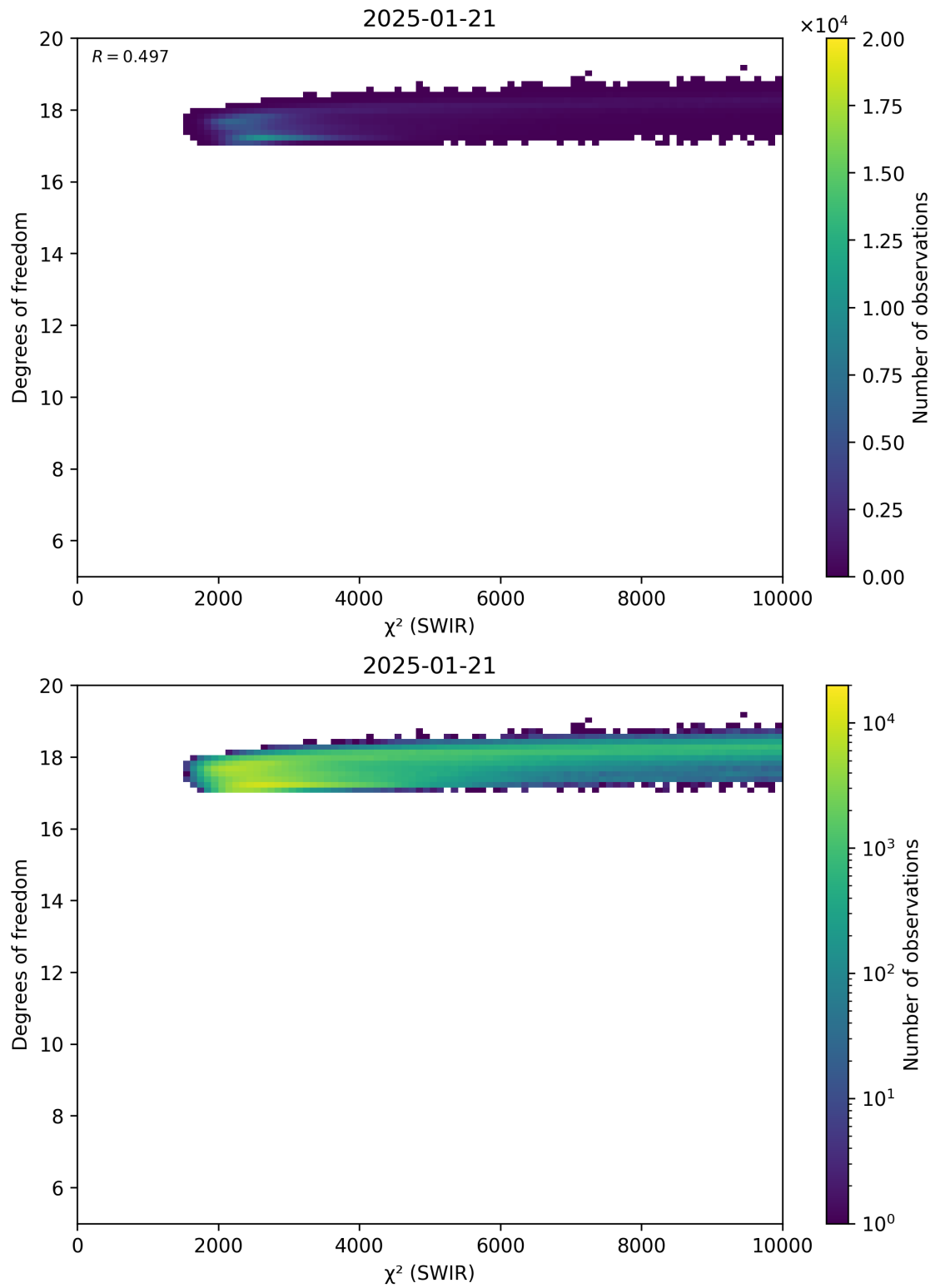
Figure 48: Scatter density plot of “ \chi^2 (SWIR)” against “Degrees of freedom” for 2025-01-20 to 2025-01-22.
