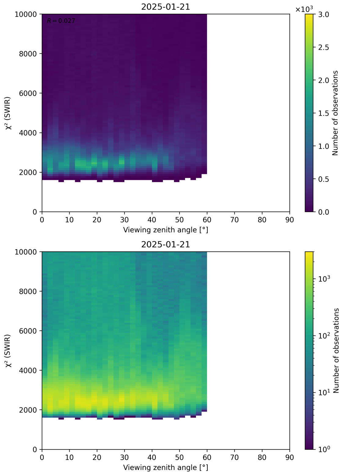
Figure 106: Scatter density plot of “Viewing zenith angle” against “ \chi^2 (SWIR)” for 2025-01-20 to 2025-01-22.
