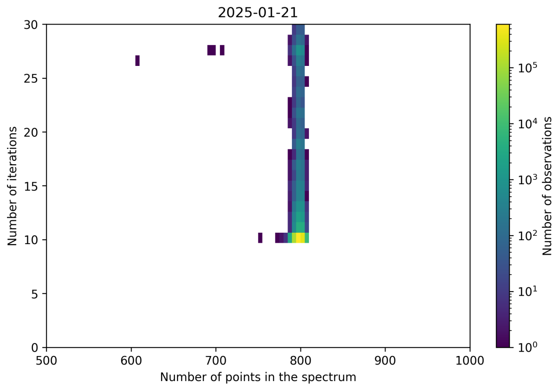
Figure 92: Scatter density plot of “Number of points in the spectrum” against “Number of iterations” for 2025-01-20 to 2025-01-22.
