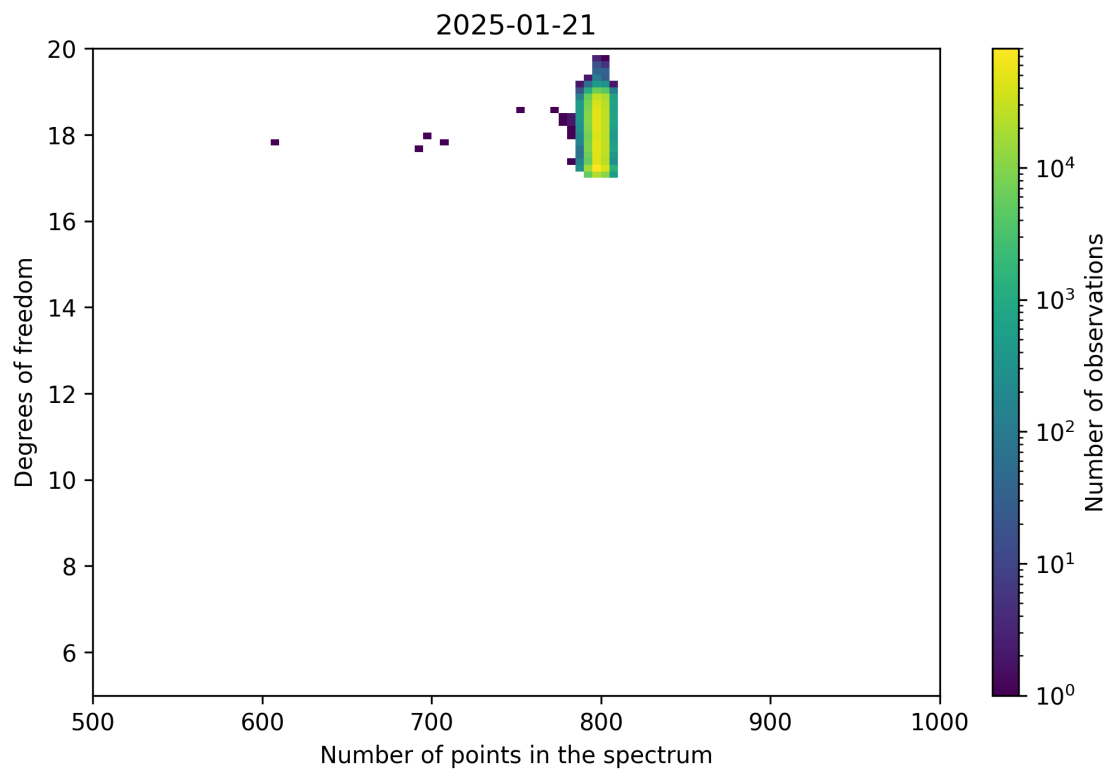
Figure 90: Scatter density plot of “Number of points in the spectrum” against “Degrees of freedom” for 2025-01-20 to 2025-01-22.
