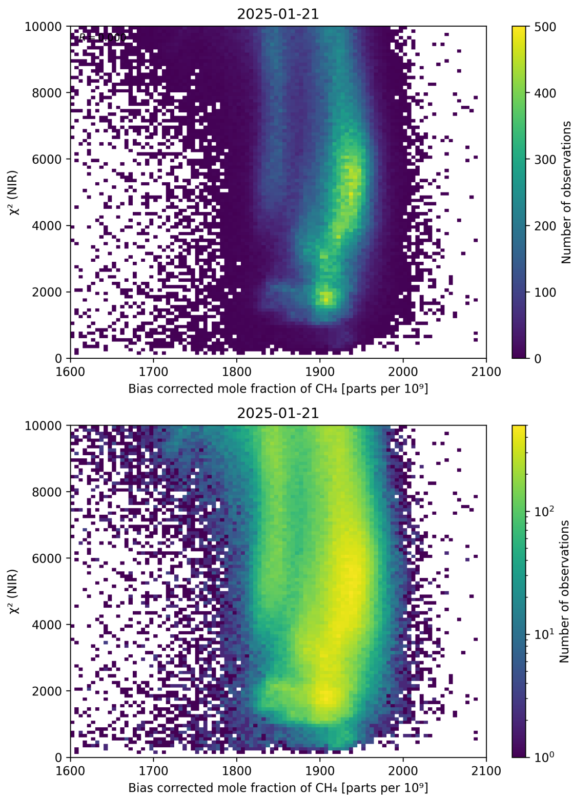
Figure 63: Scatter density plot of “Bias corrected mole fraction of CH 4 ” against “ \chi^2 (NIR)” for 2025-01-20 to 2025-01-22.
