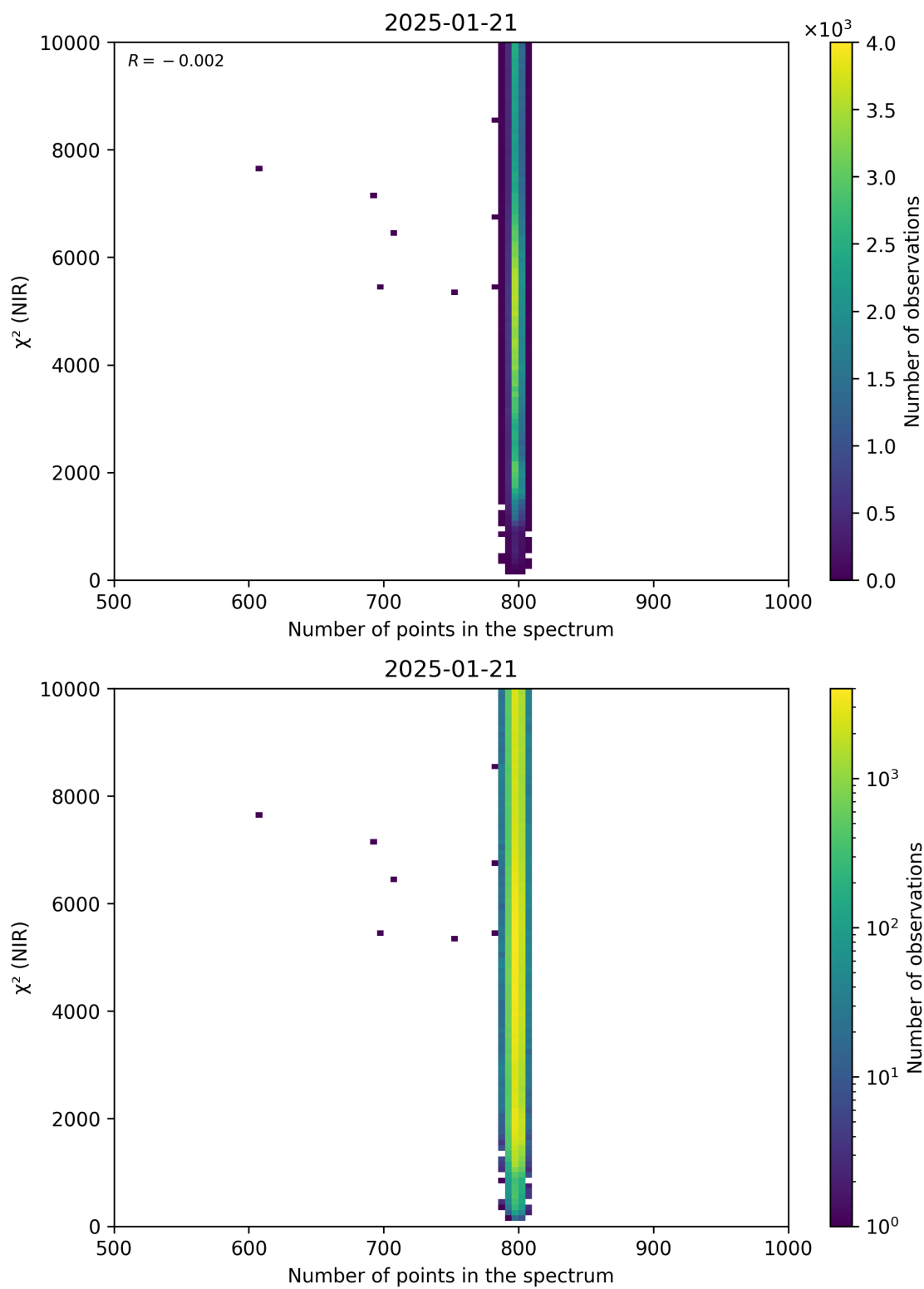
Figure 88: Scatter density plot of “Number of points in the spectrum” against “ \chi^2 (NIR)” for 2025-01-20 to 2025-01-22.
