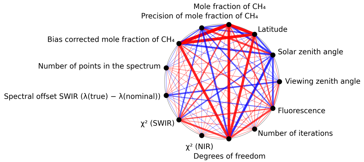
Figure 1: Map of correlation graph for 2025-01-20 to 2025-01-22.
