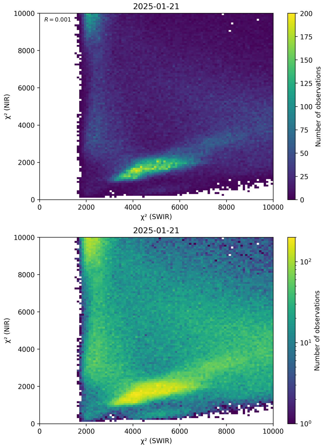
Figure 47: Scatter density plot of “ \chi^2 (SWIR)” against “ \chi^2 (NIR)” for 2025-01-20 to 2025-01-22.
