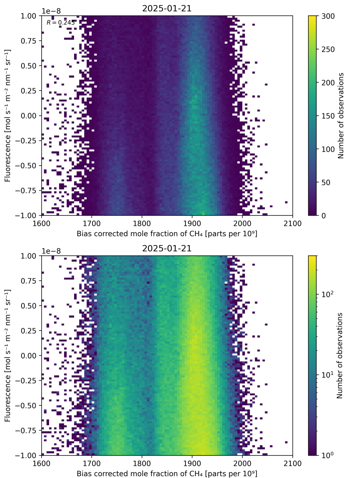
Figure 66: Scatter density plot of “Bias corrected mole fraction of \text{CH}_4 ” against “Fluorescence” for 2025-01-20 to 2025-01-22.
