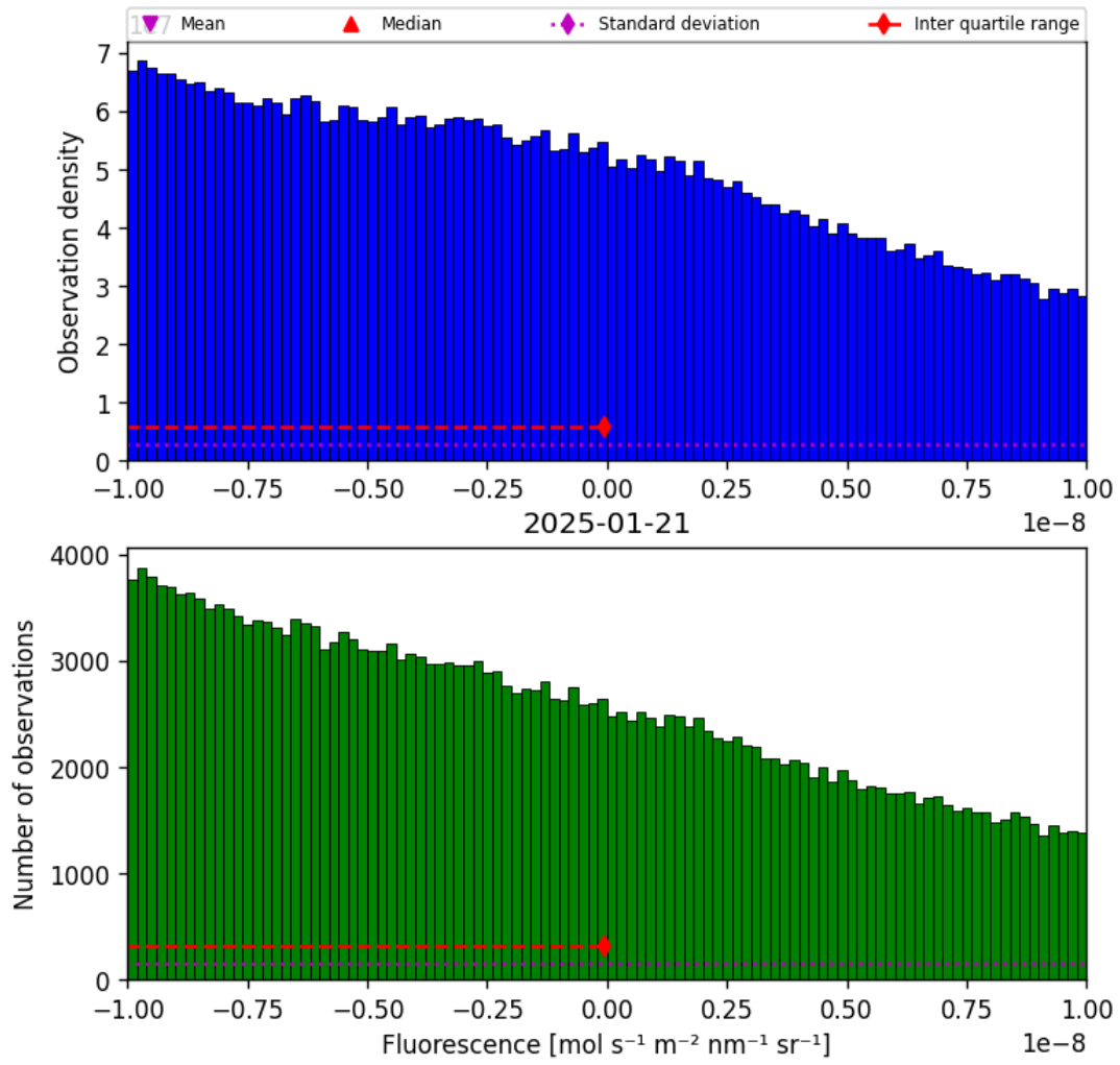
Figure 32: Histogram of “Fluorescence” for 2025-01-20 to 2025-01-22
