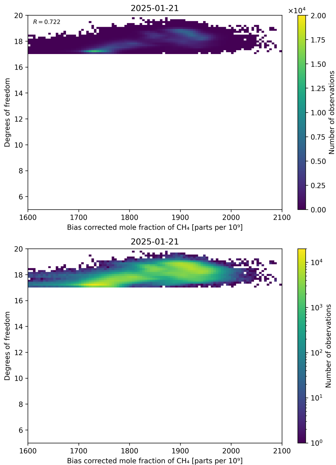
Figure 65: Scatter density plot of “Bias corrected mole fraction of CH 4 ” against “Degrees of freedom” for 2025-01-20 to 2025-01-22.
