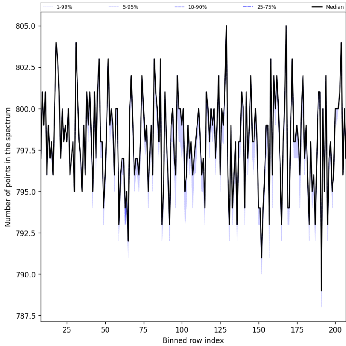
Figure 37: Along track statistics of “Number of points in the spectrum” for 2025-01-20 to 2025-01-22
