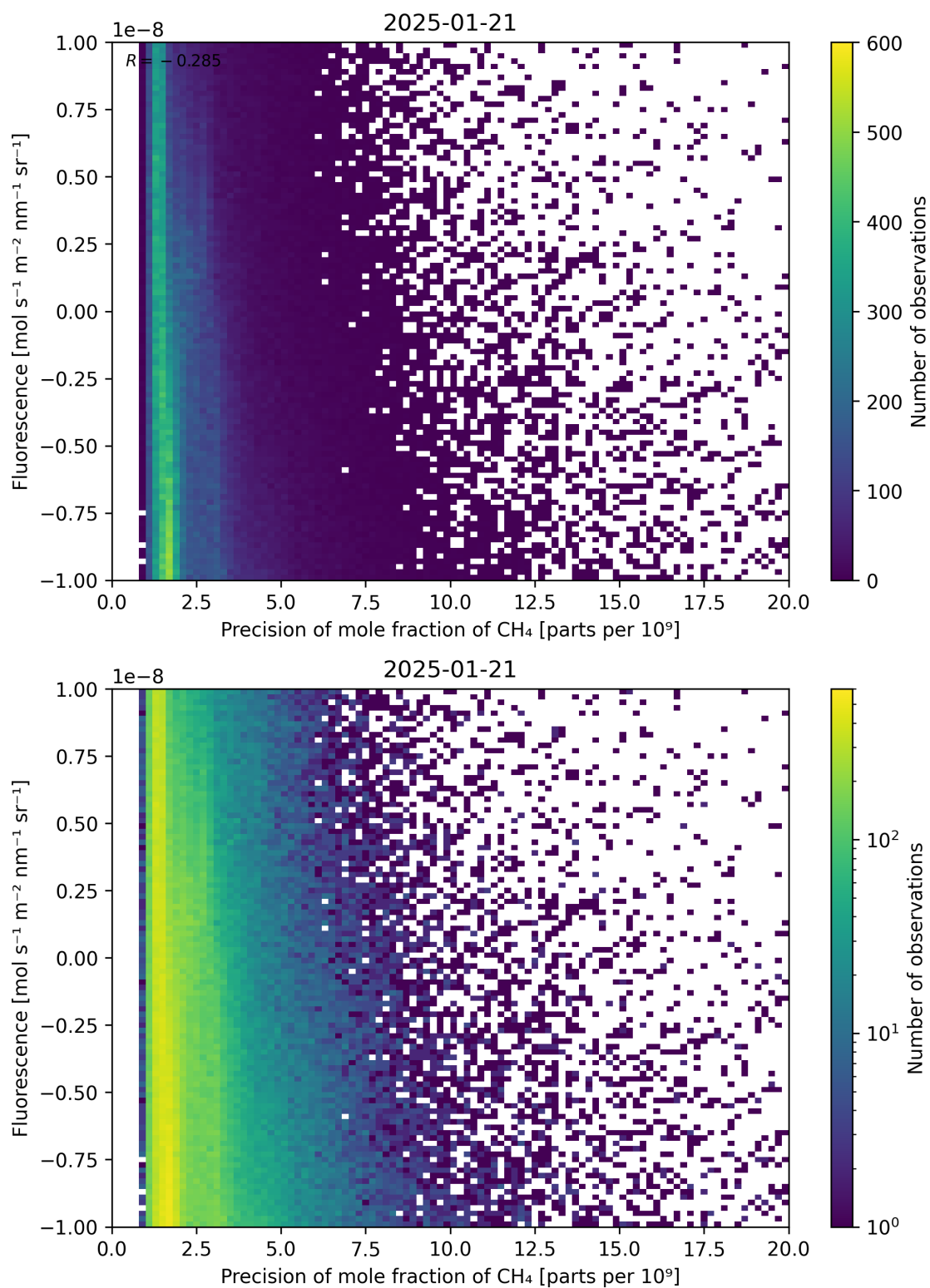
Figure 81: Scatter density plot of “Precision of mole fraction of \text{CH}_4 ” against “Fluorescence” for 2025-01-20 to 2025-01-22.
