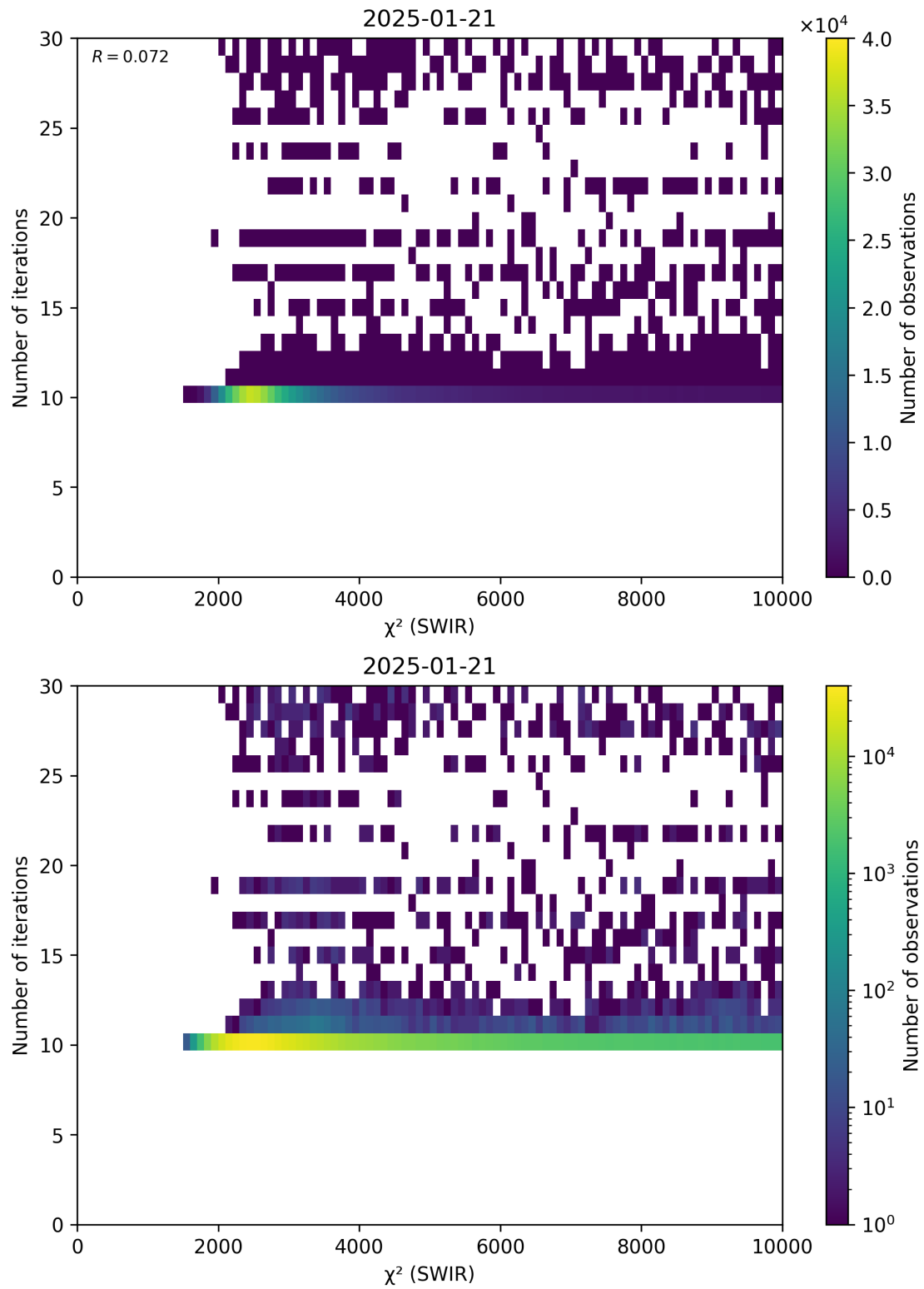
Figure 50: Scatter density plot of “ \chi^2 (SWIR)” against “Number of iterations” for 2025-01-20 to 2025-01-22.
