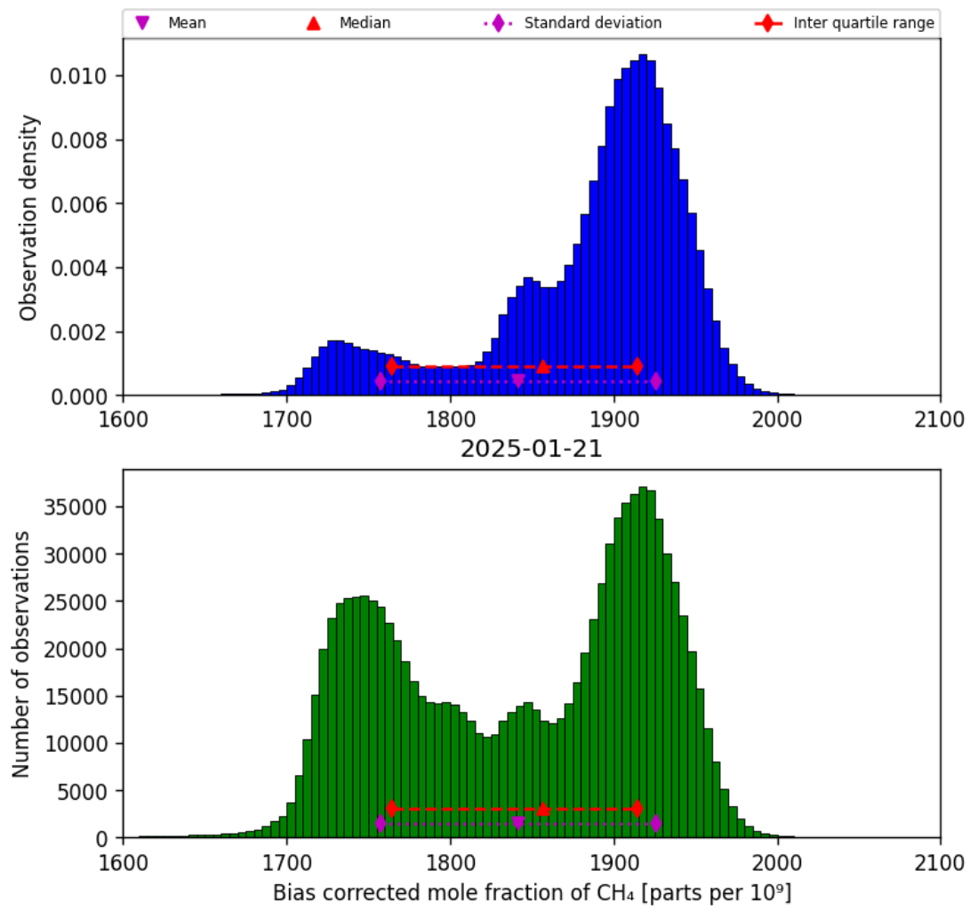
Figure 25: Histogram of “Bias corrected mole fraction of CH 4 ” for 2025-01-20 to 2025-01-22
