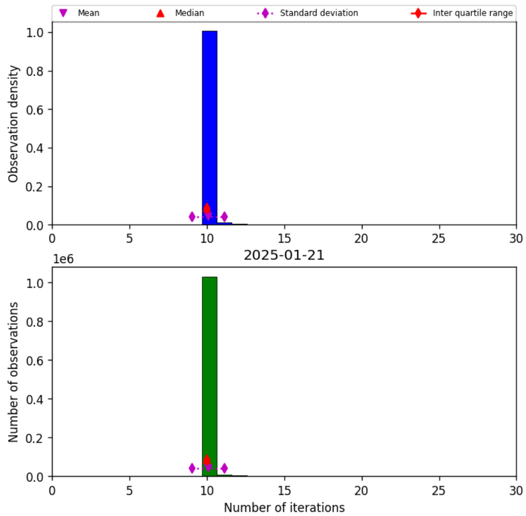
Figure 31: Histogram of “Number of iterations” for 2025-01-20 to 2025-01-22
