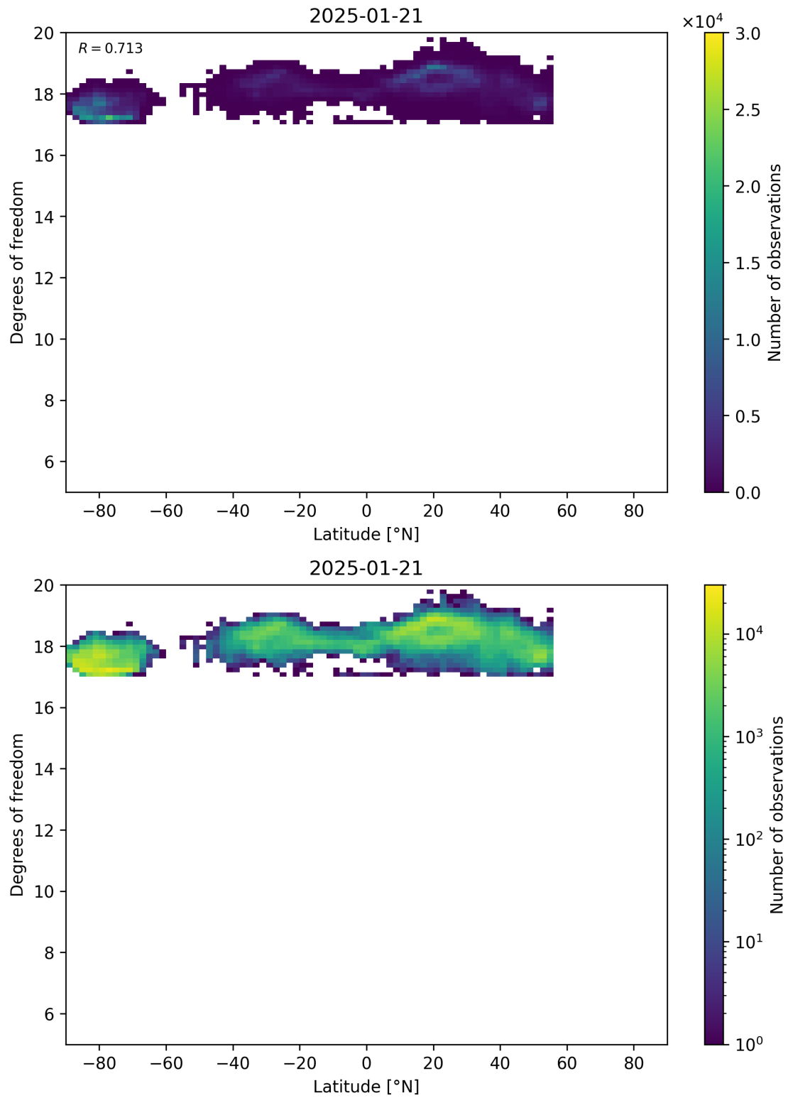
Figure 55: Scatter density plot of “Latitude” against “Degrees of freedom” for 2025-01-20 to 2025-01-22.
