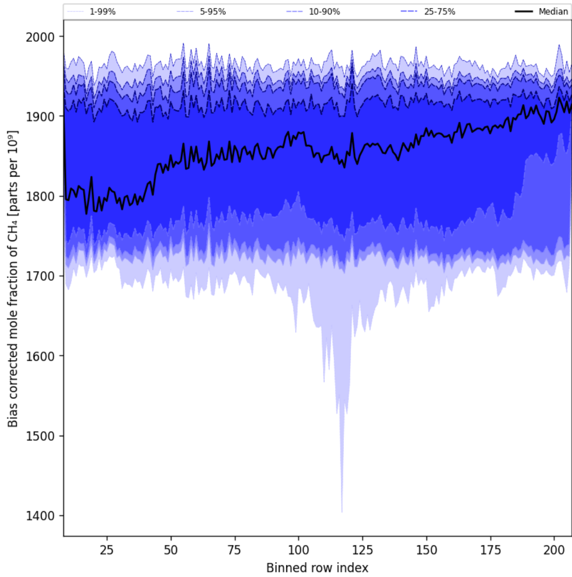
Figure 36: Along track statistics of “Bias corrected mole fraction of CH 4 ” for 2025-01-20 to 2025-01-22
