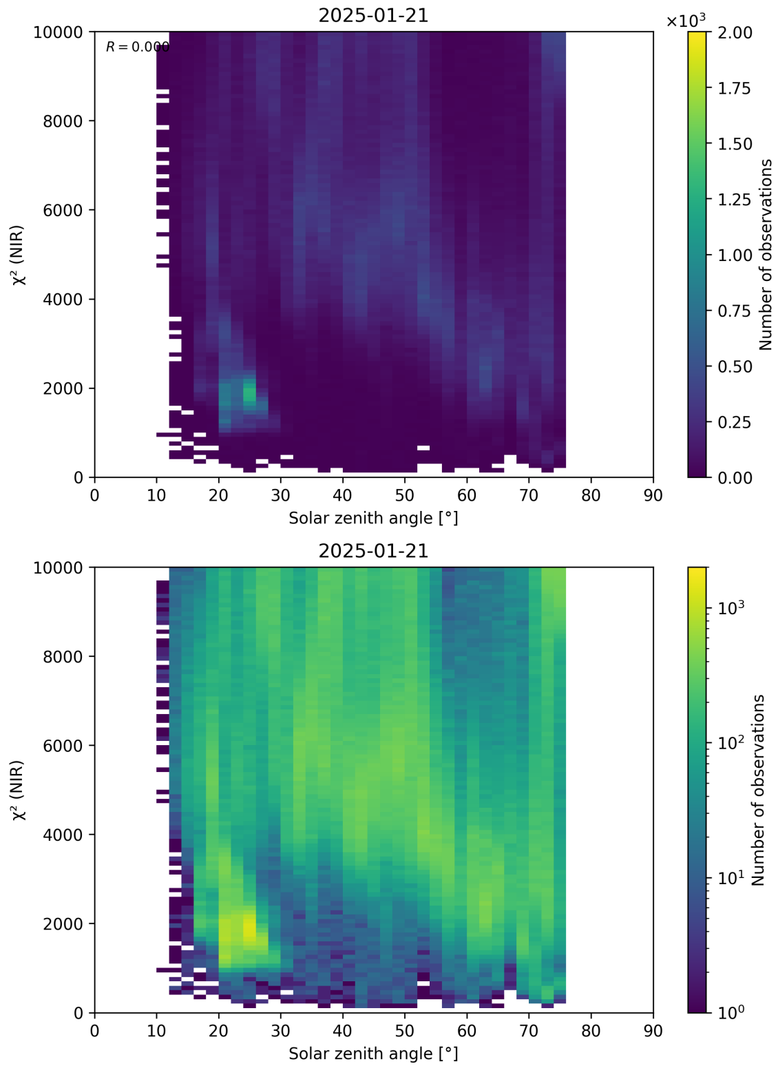
Figure 94: Scatter density plot of “Solar zenith angle” against “ \chi^2 (NIR)” for 2025-01-20 to 2025-01-22.
