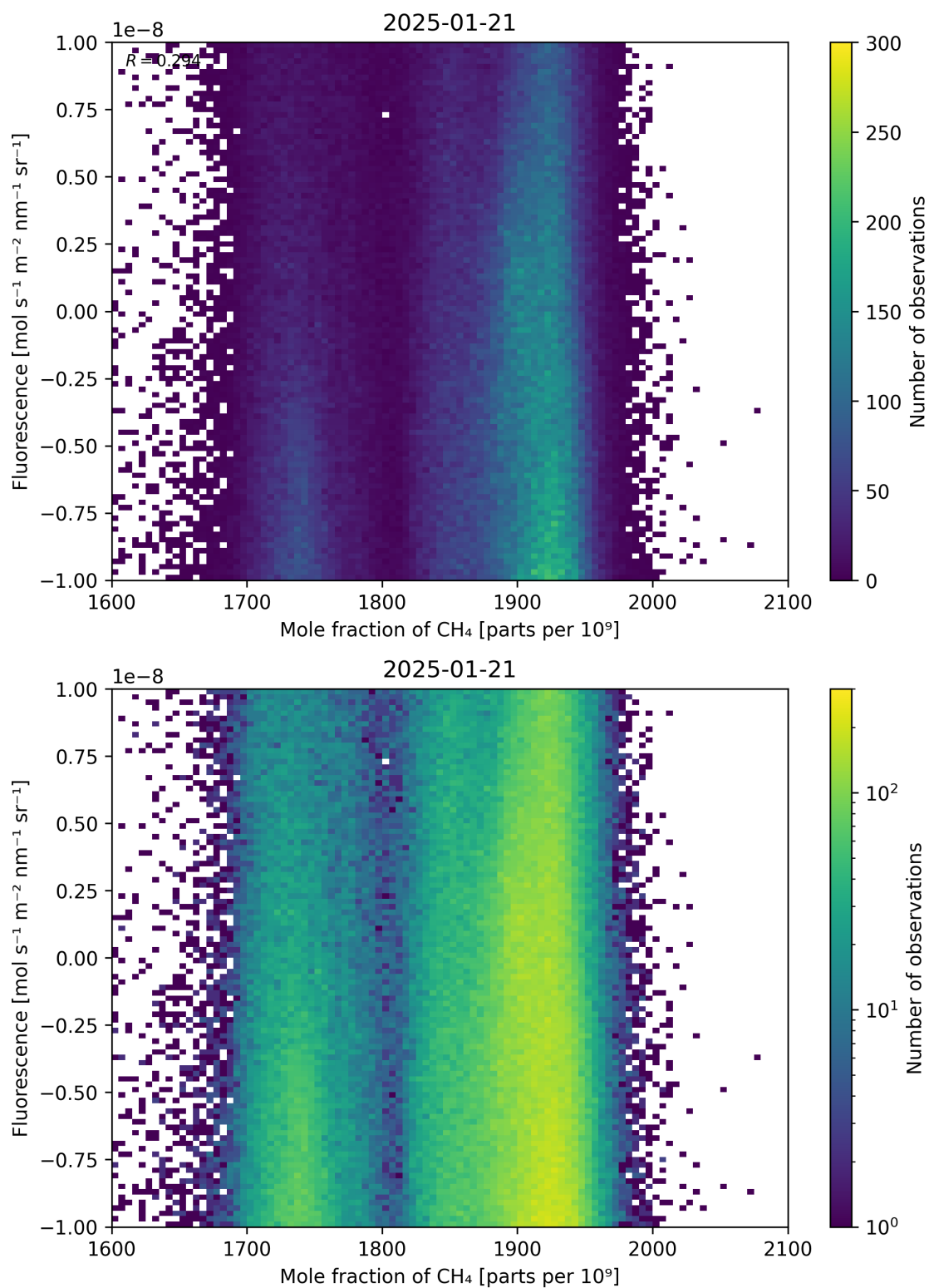
Figure 73: Scatter density plot of “Mole fraction of \text{CH}_4 ” against “Fluorescence” for 2025-01-20 to 2025-01-22.
