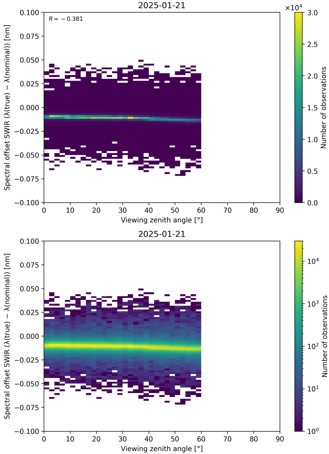
Figure 116: Scatter density plot of “Viewing zenith angle” against “Spectral offset SWIR ( \lambda_{\text{true}} - \lambda_{\text{nominal}} )” for 2025-01-20 to 2025-01-22.
