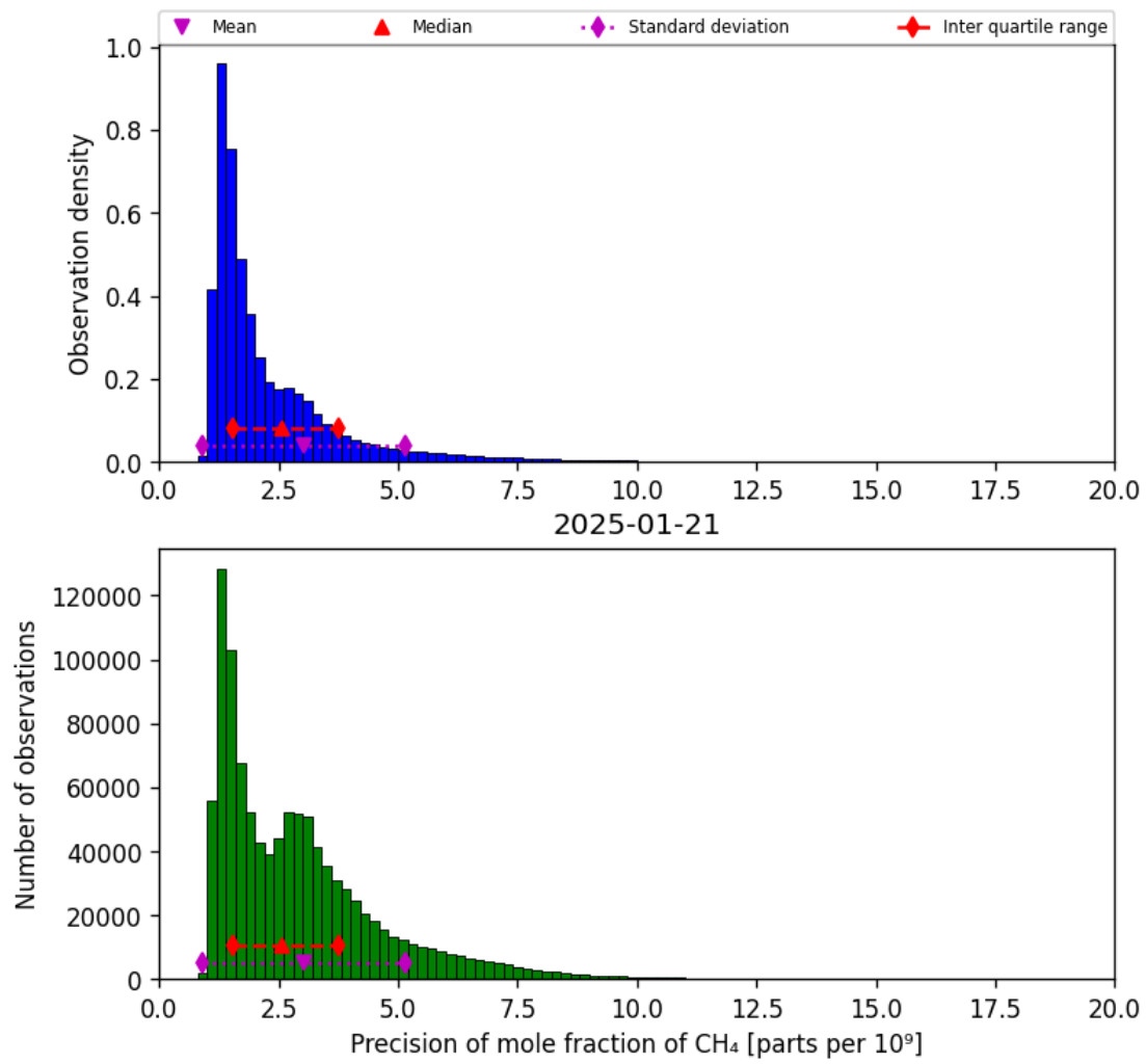
Figure 24: Histogram of “Precision of mole fraction of CH 4 ” for 2025-01-20 to 2025-01-22
