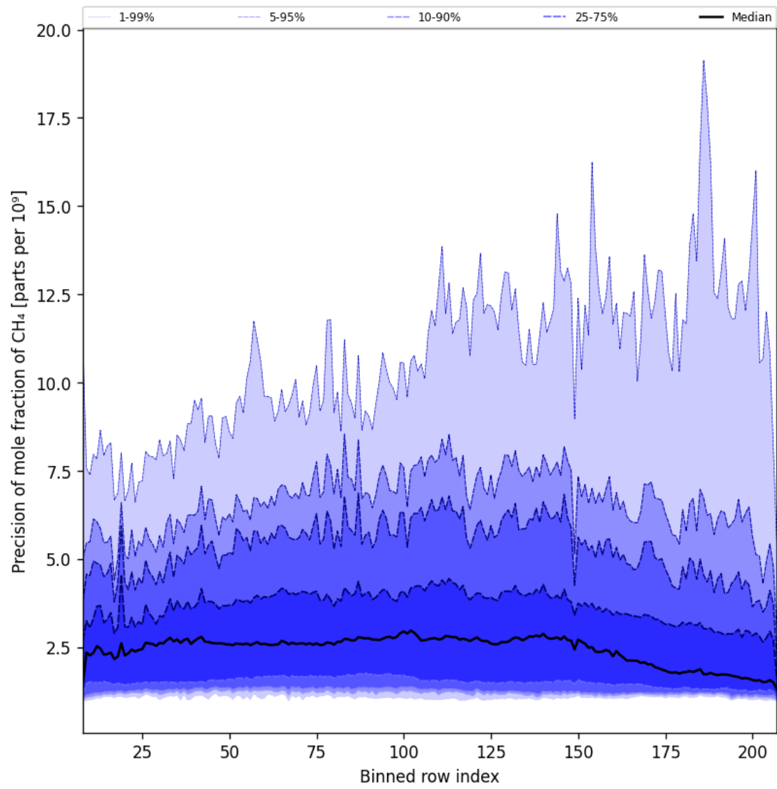
Figure 35: Along track statistics of “Precision of mole fraction of CH 4 ” for 2025-01-20 to 2025-01-22
