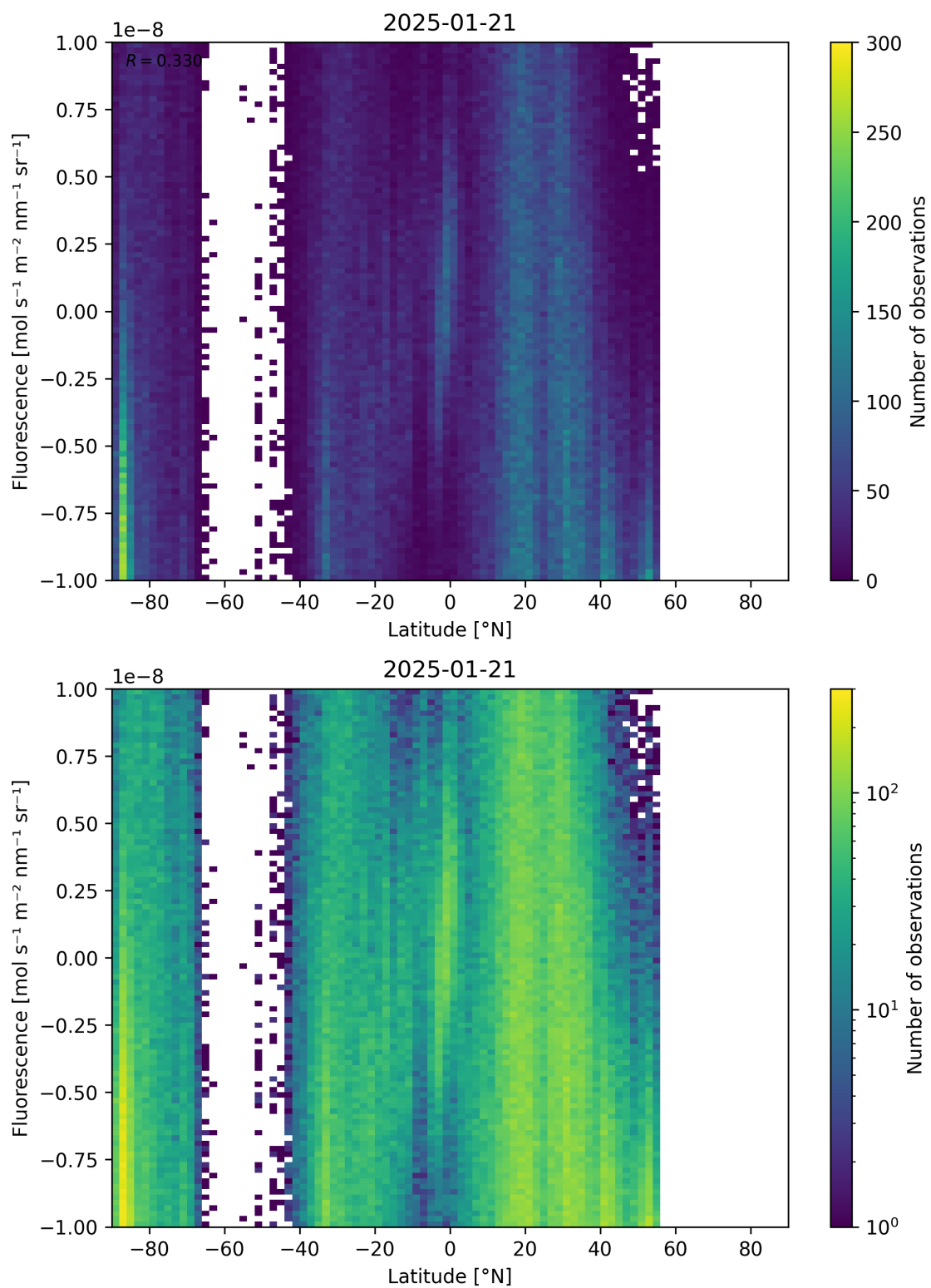
Figure 56: Scatter density plot of “Latitude” against “Fluorescence” for 2025-01-20 to 2025-01-22.
