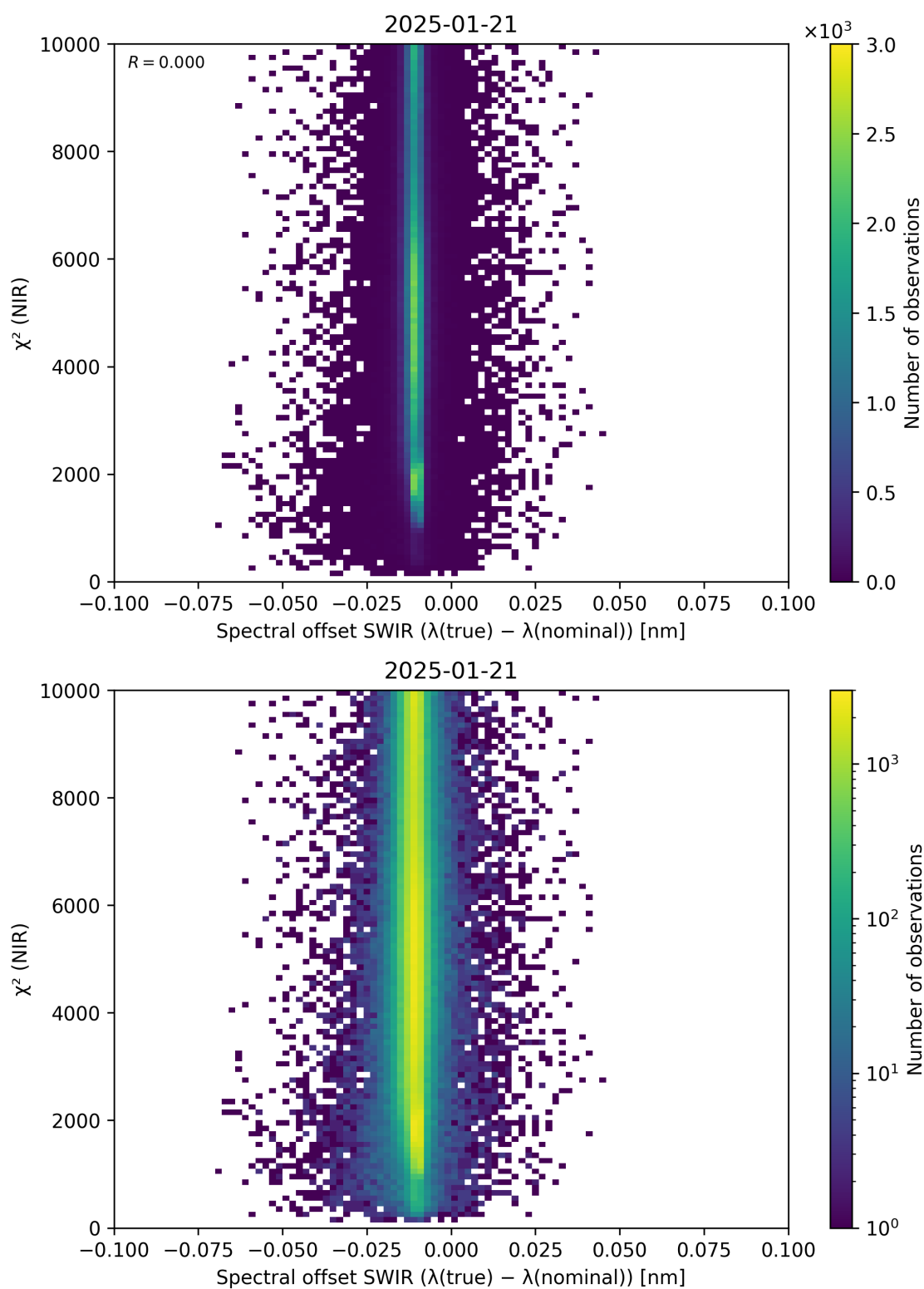
Figure 117: Scatter density plot of “Spectral offset SWIR ( \lambda_{\text{true}} - \lambda_{\text{nominal}} )” against “ \chi^2 (NIR)” for 2025-01-20 to 2025-01-22.
