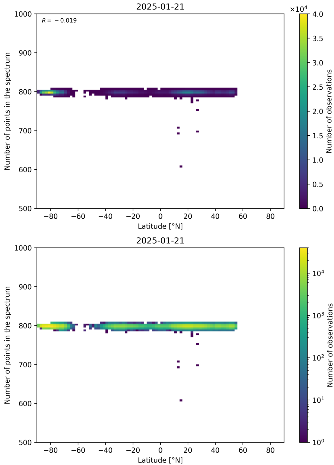
Figure 61: Scatter density plot of “Latitude” against “Number of points in the spectrum” for 2025-01-20 to 2025-01-22.
