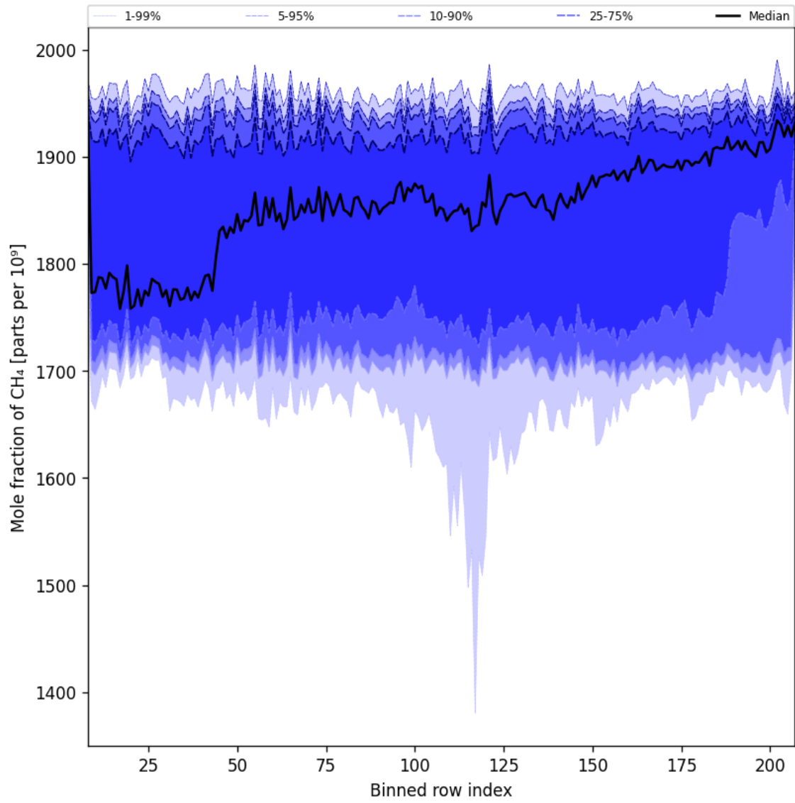
Figure 34: Along track statistics of “Mole fraction of CH 4 ” for 2025-01-20 to 2025-01-22
