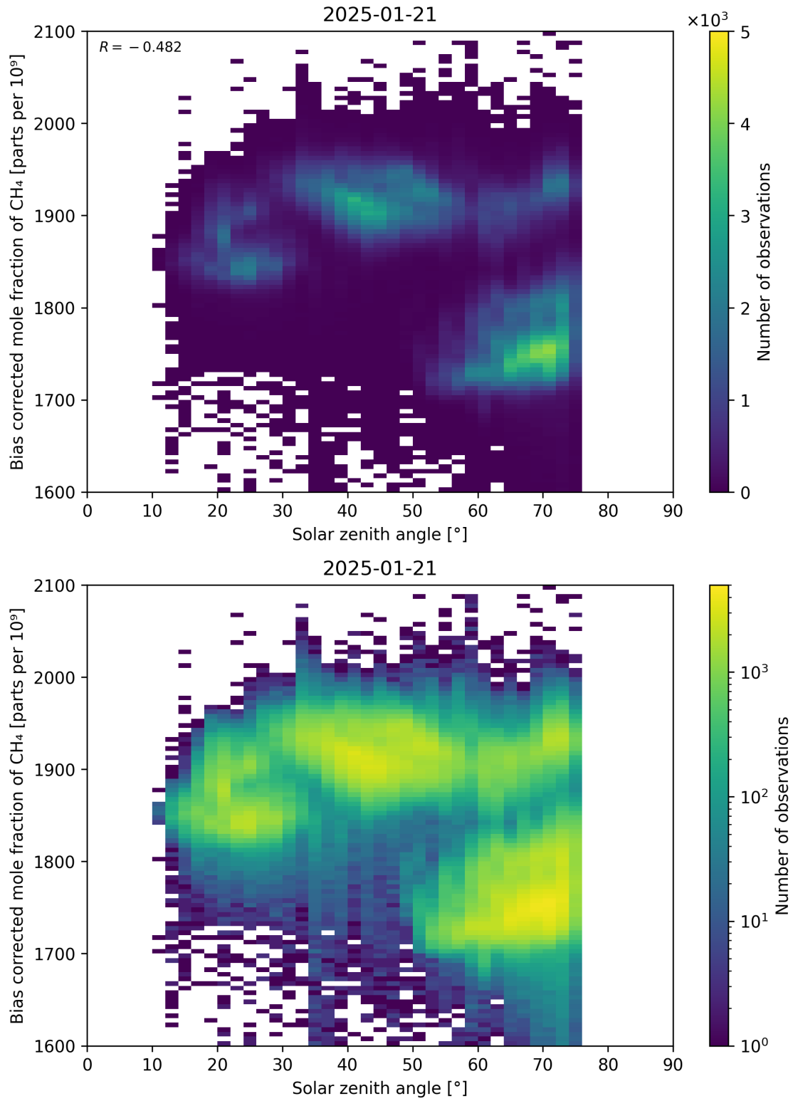
Figure 100: Scatter density plot of “Solar zenith angle” against “Bias corrected mole fraction of CH 4 ” for 2025-01-20 to 2025-01-22.
