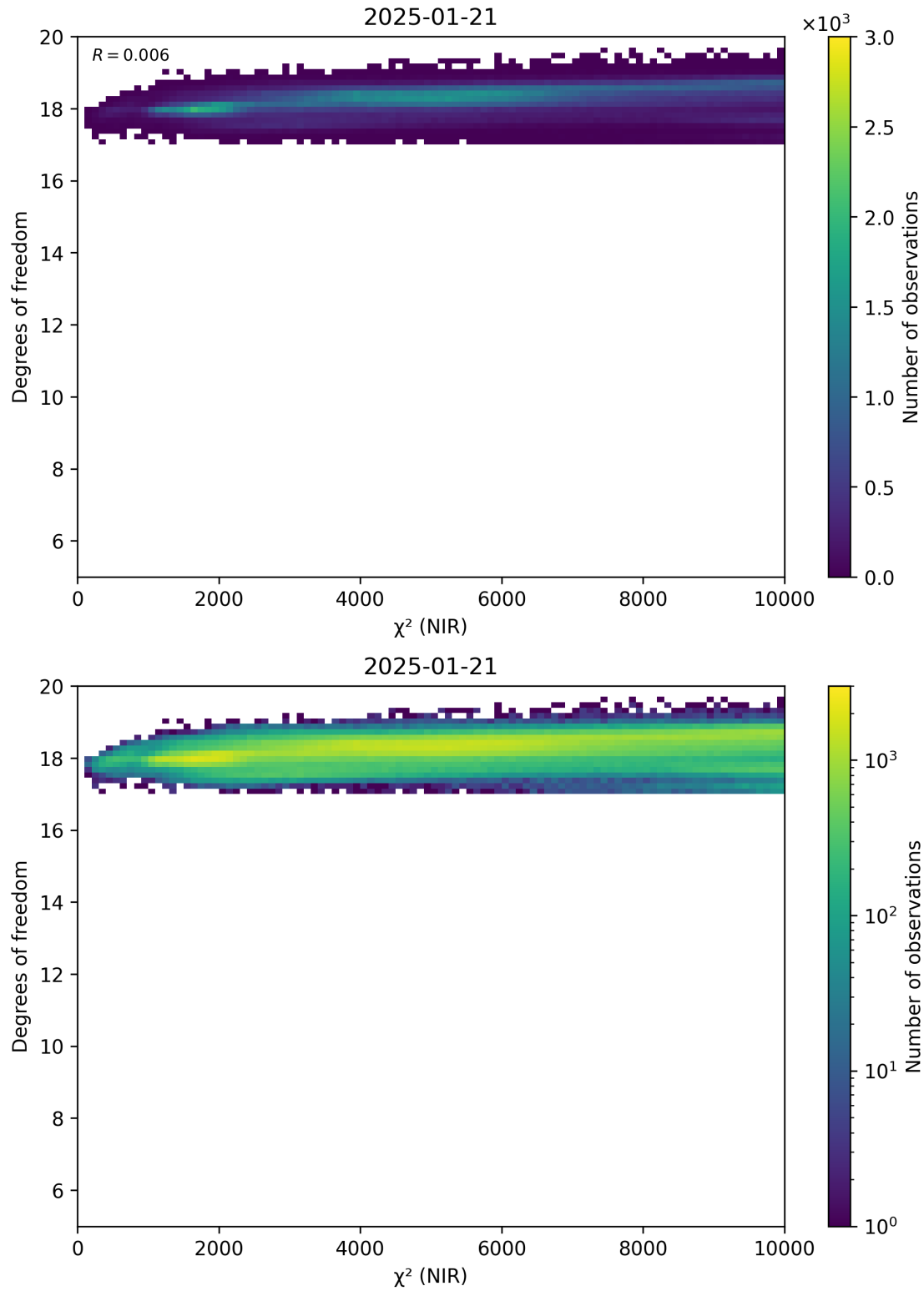
Figure 44: Scatter density plot of “ \chi^2 (NIR)” against “Degrees of freedom” for 2025-01-20 to 2025-01-22.
