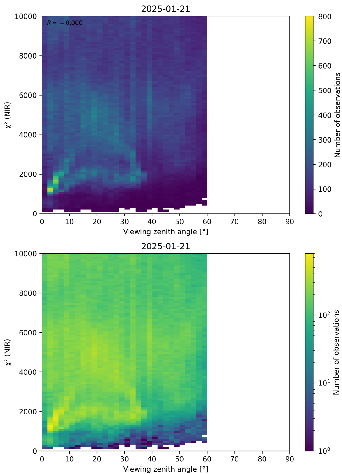
Figure 105: Scatter density plot of “Viewing zenith angle” against “ \chi^2 (NIR)” for 2025-01-20 to 2025-01-22.
