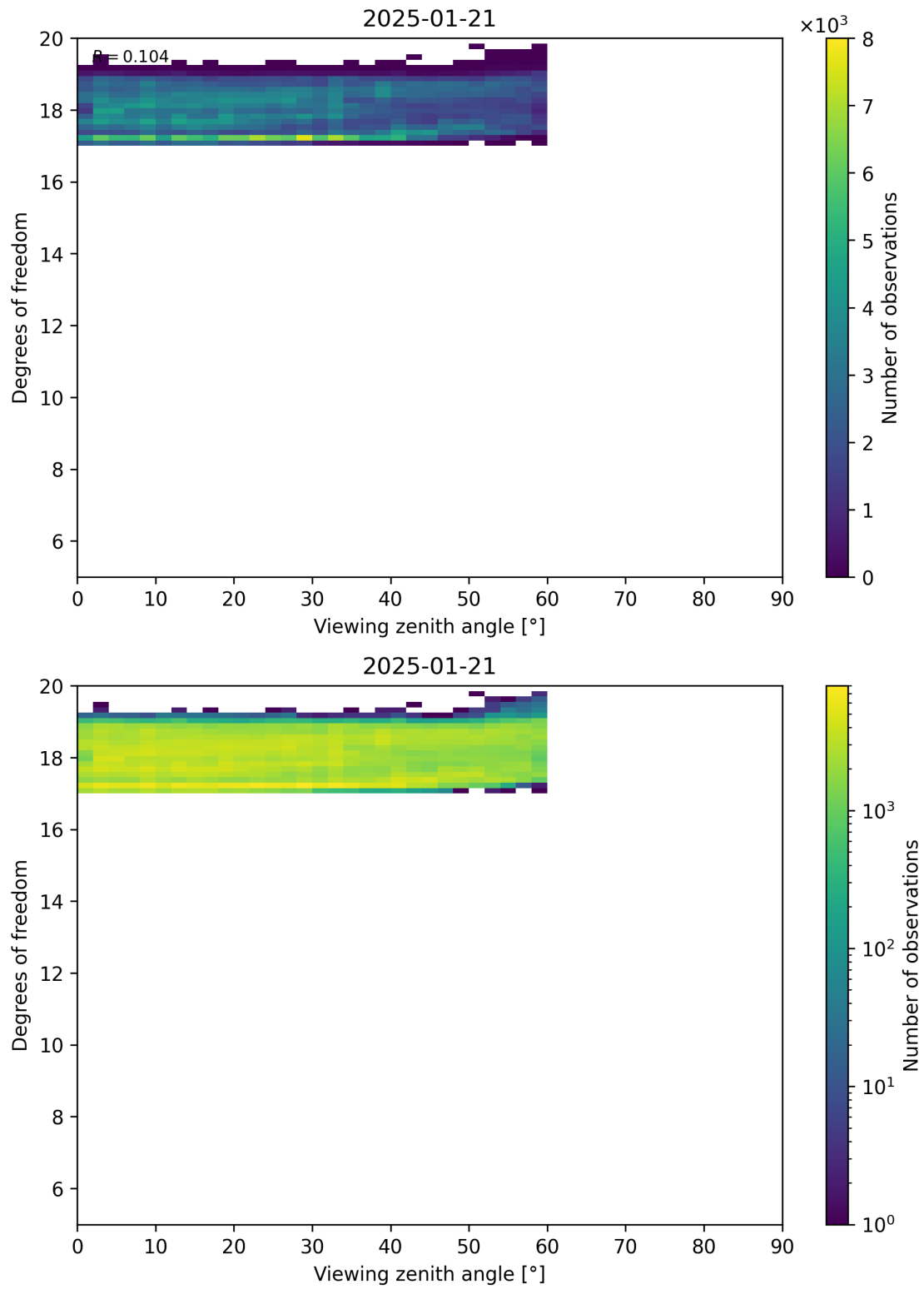
Figure 107: Scatter density plot of “Viewing zenith angle” against “Degrees of freedom” for 2025-01-20 to 2025-01-22.
