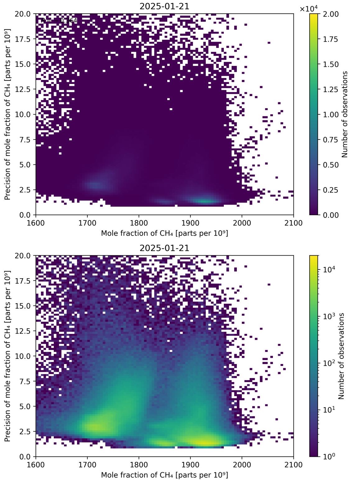
Figure 75: Scatter density plot of “Mole fraction of CH 4 ” against “Precision of mole fraction of CH 4 ” for 2025-01-20 to 2025-01-22.
