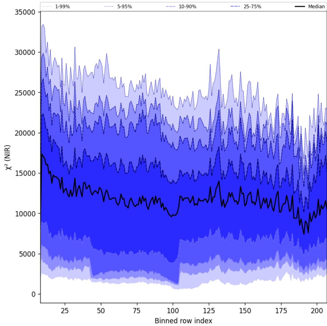
Figure 40: Along track statistics of “ \chi^2 (NIR)” for 2025-01-20 to 2025-01-22
