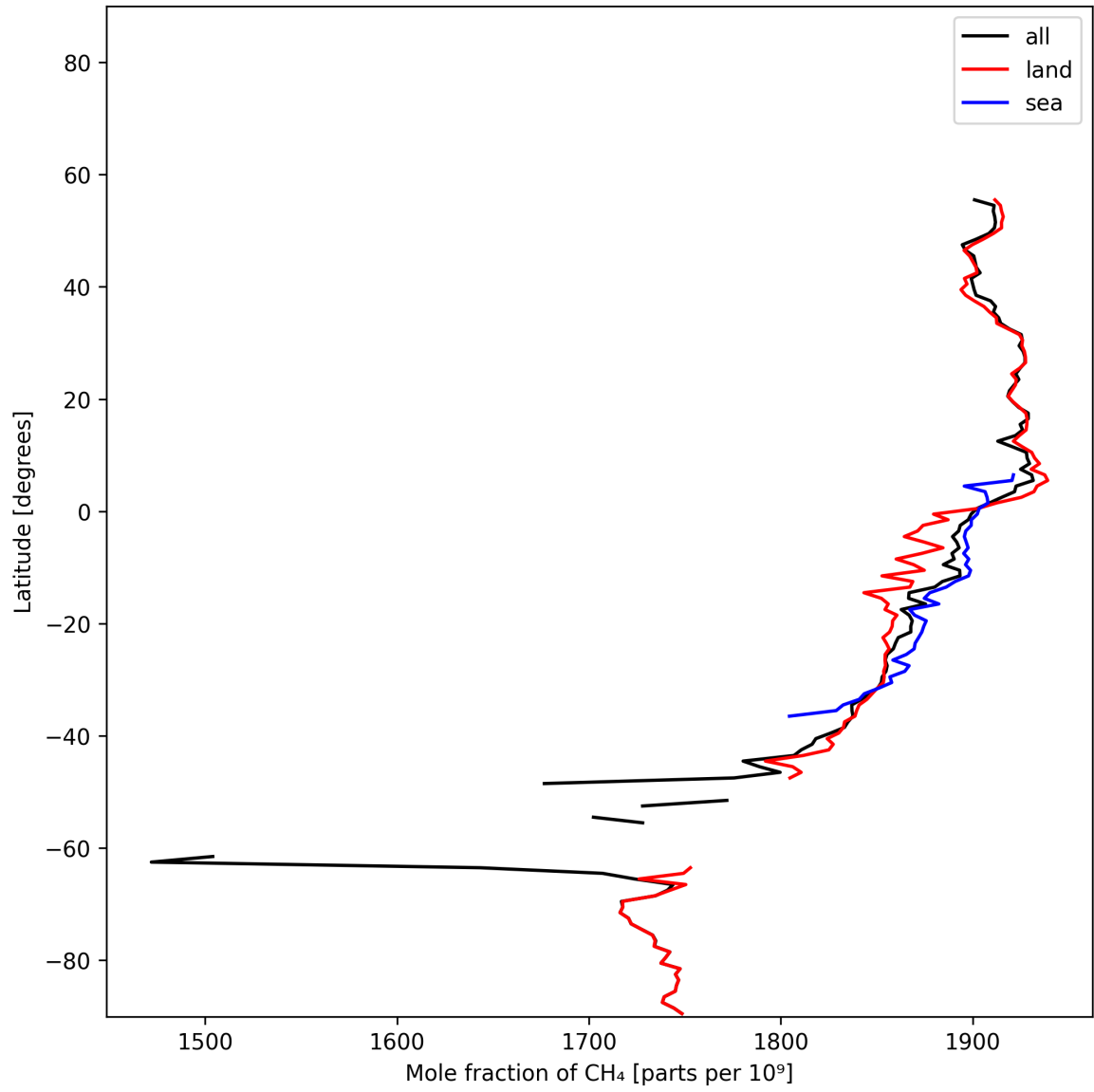
Figure 12: Zonal average of “Mole fraction of CH 4 ” for 2025-01-20 to 2025-01-22.
