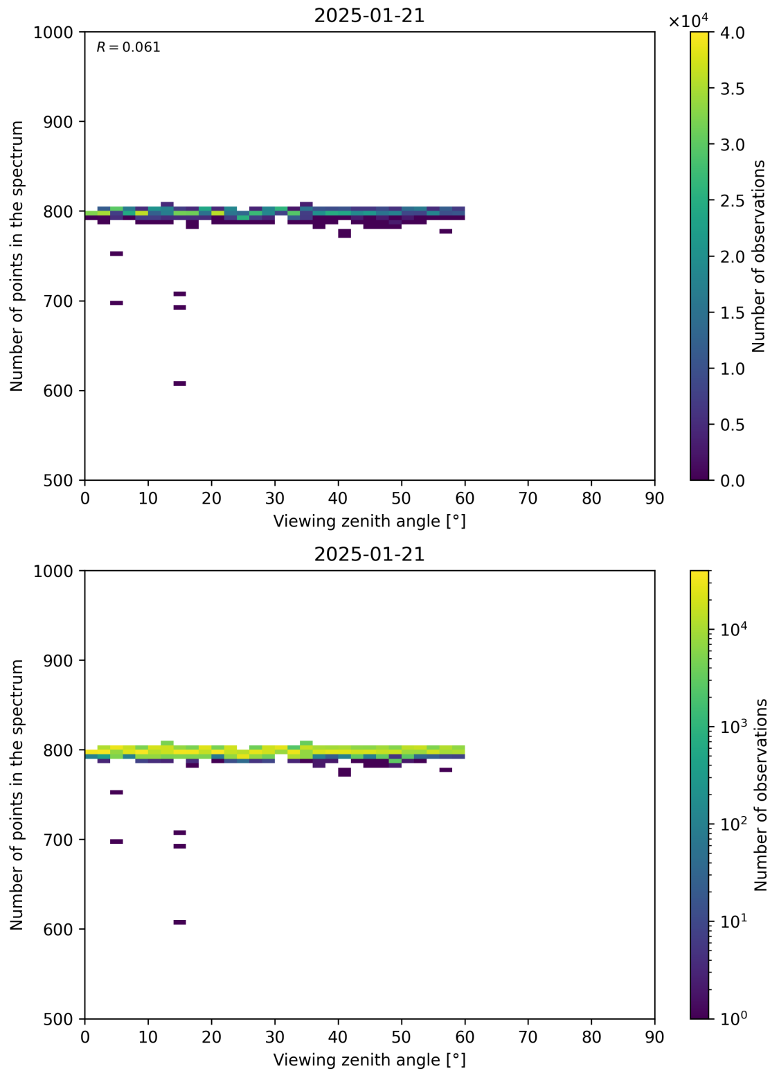
Figure 114: Scatter density plot of “Viewing zenith angle” against “Number of points in the spectrum” for 2025-01-20 to 2025-01-22.
