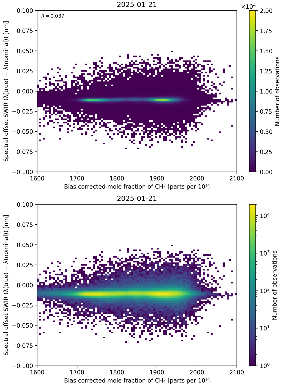
Figure 69: Scatter density plot of “Bias corrected mole fraction of \text{CH}_4 ” against “Spectral offset SWIR ( \lambda_{\text{true}} - \lambda_{\text{nominal}} )” for 2025-01-20 to 2025-01-22.
