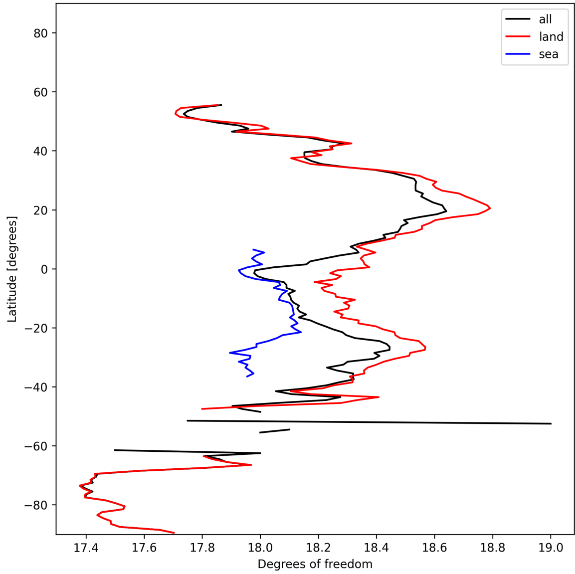
Figure 19: Zonal average of “Degrees of freedom” for 2025-01-20 to 2025-01-22.
