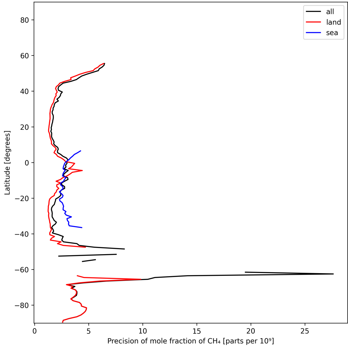
Figure 13: Zonal average of “Precision of mole fraction of CH 4 ” for 2025-01-20 to 2025-01-22.
