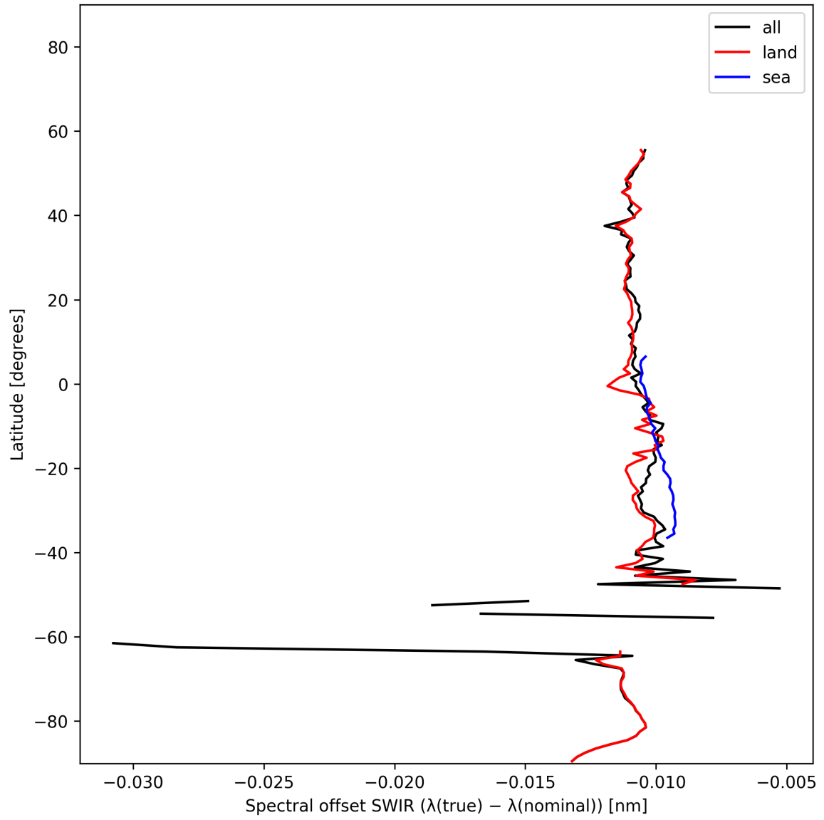
Figure 16: Zonal average of “Spectral offset SWIR ( \lambda_{\text{true}} - \lambda_{\text{nominal}} )” for 2025-01-20 to 2025-01-22.
