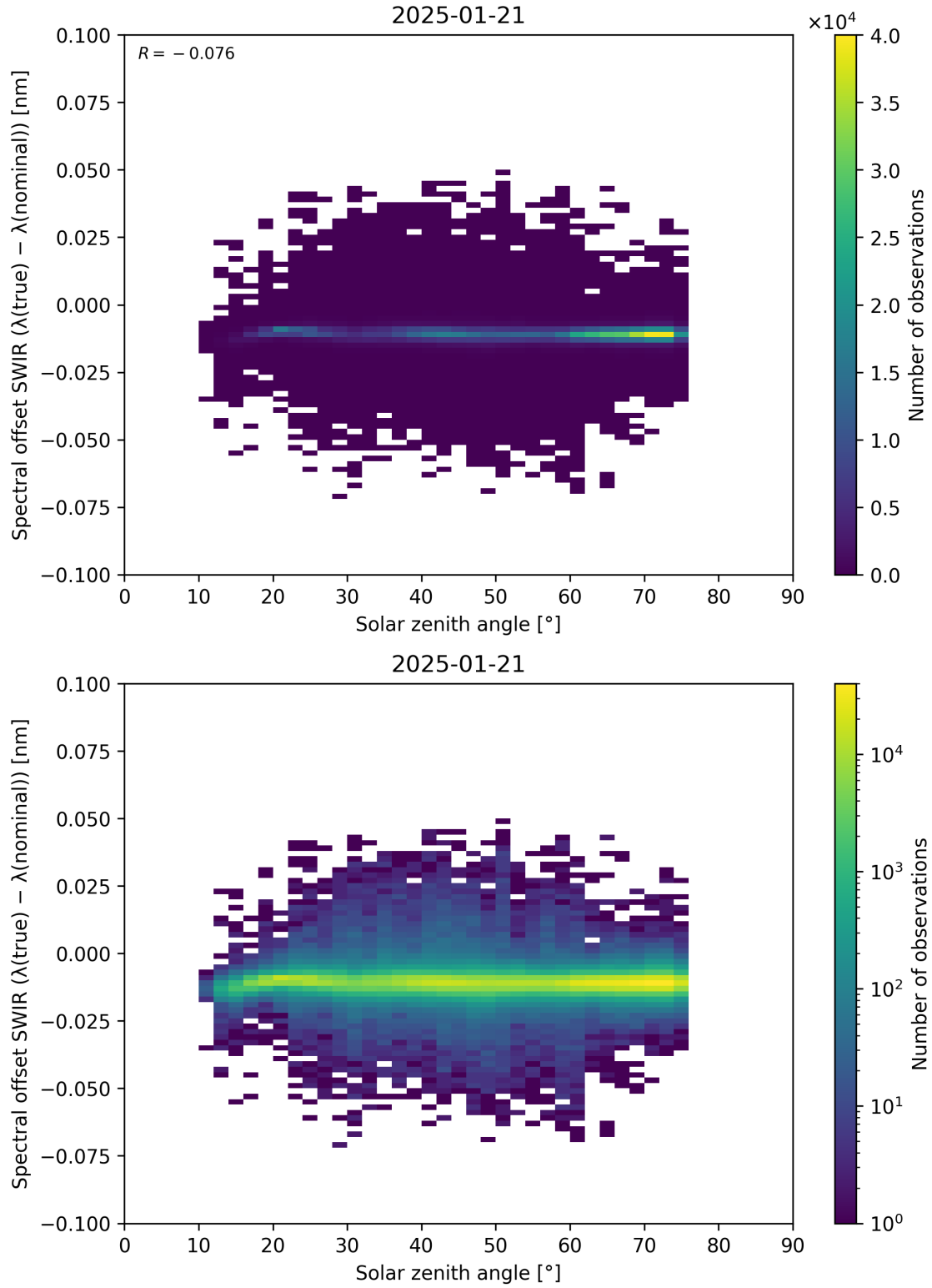
Figure 104: Scatter density plot of “Solar zenith angle” against “Spectral offset SWIR ( \lambda_{\text{true}} - \lambda_{\text{nominal}} )” for 2025-01-20 to 2025-01-22.
