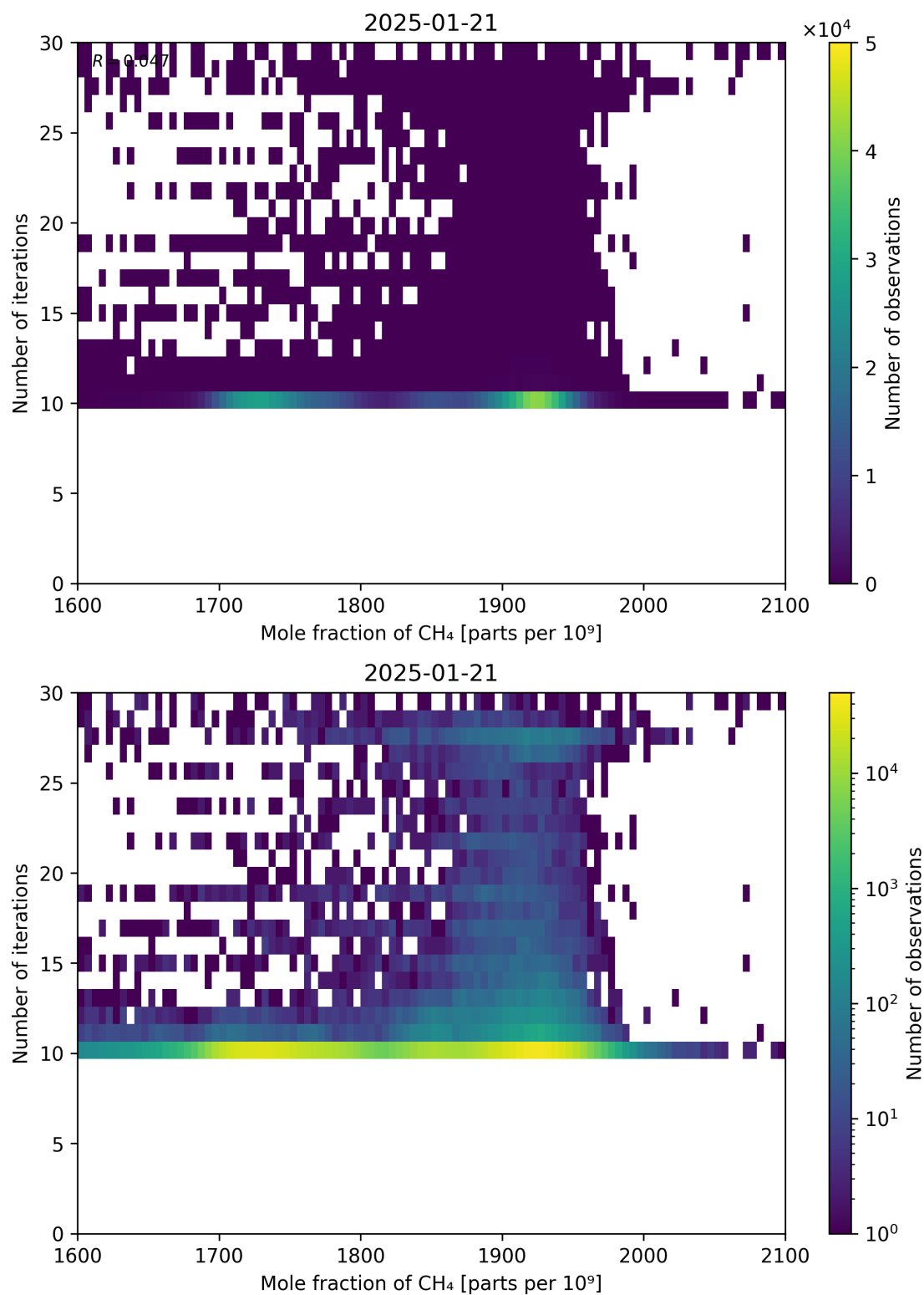
Figure 76: Scatter density plot of “Mole fraction of CH 4 ” against “Number of iterations” for 2025-01-20 to 2025-01-22.
