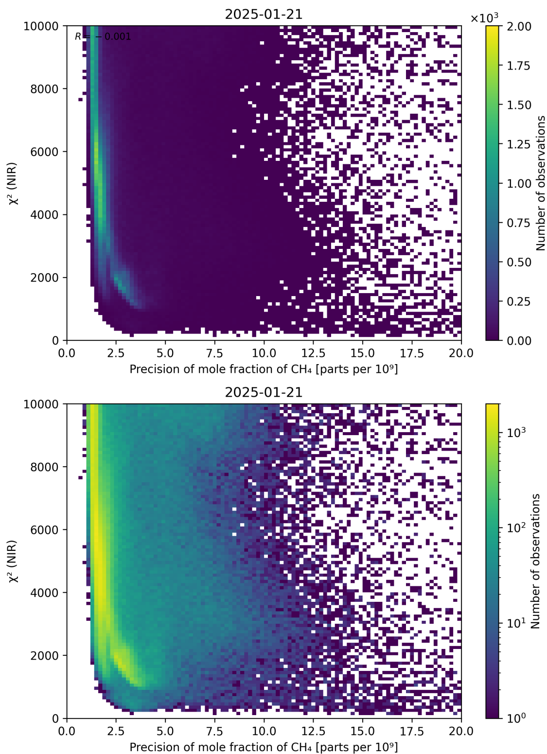
Figure 78: Scatter density plot of “Precision of mole fraction of CH 4 ” against “ \chi^2 (NIR)” for 2025-01-20 to 2025-01-22.
