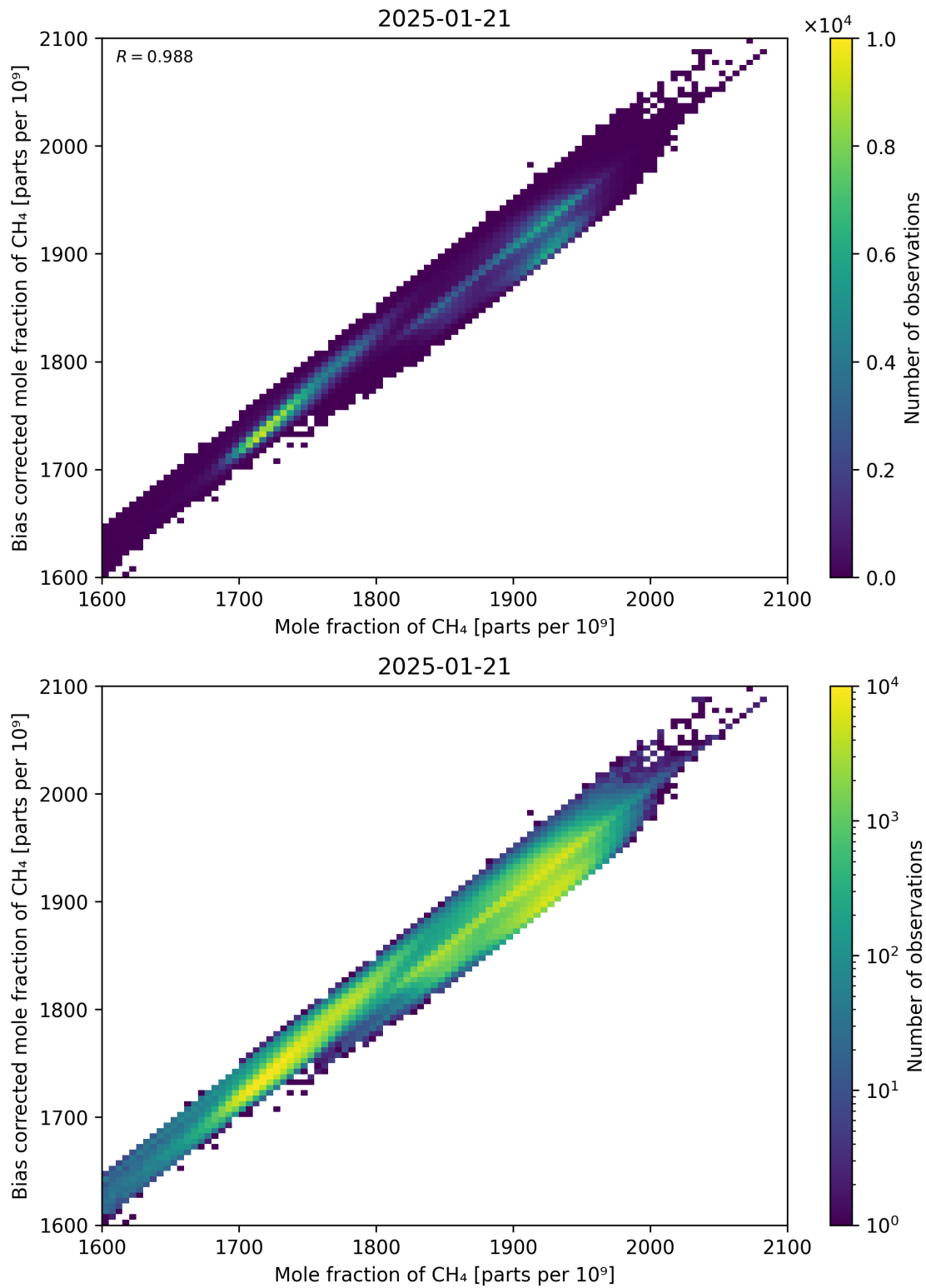
Figure 74: Scatter density plot of “Mole fraction of CH 4 ” against “Bias corrected mole fraction of CH 4 ” for 2025-01-20 to 2025-01-22.
