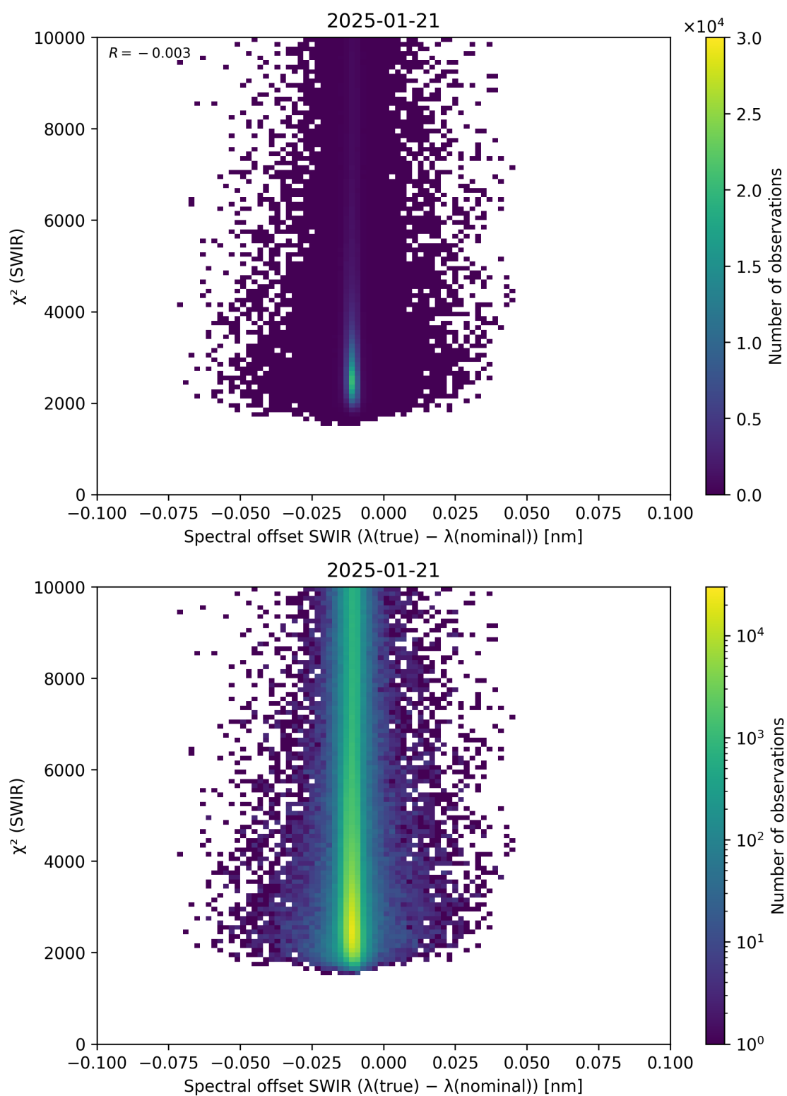
Figure 118: Scatter density plot of “Spectral offset SWIR ( \lambda_{\text{true}} - \lambda_{\text{nominal}} )” against “ \chi^2 (SWIR)” for 2025-01-20 to 2025-01-22.
