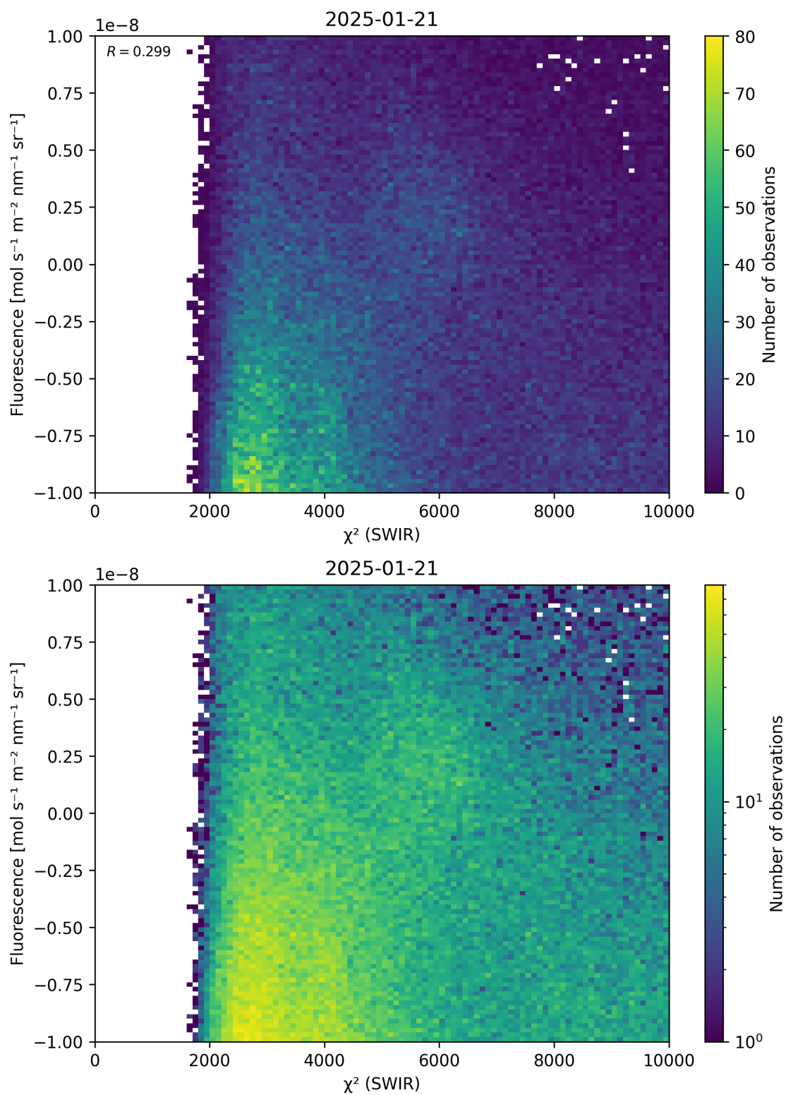
Figure 49: Scatter density plot of “ \chi^2 (SWIR)” against “Fluorescence” for 2025-01-20 to 2025-01-22.
