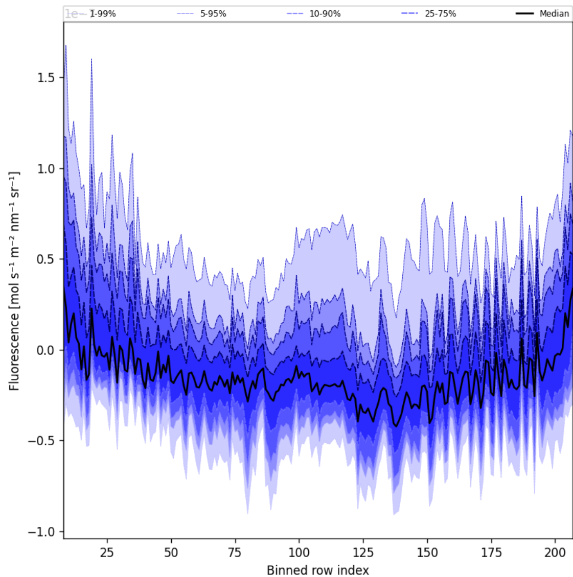
Figure 43: Along track statistics of “Fluorescence” for 2025-01-20 to 2025-01-22
