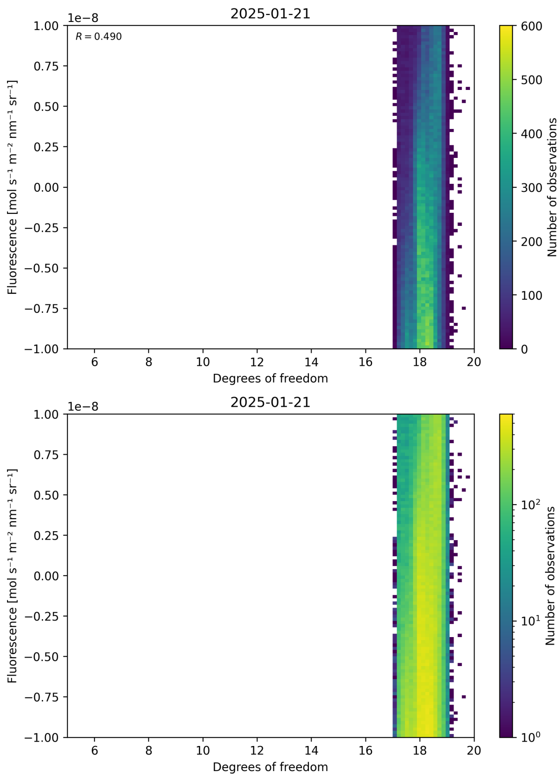
Figure 51: Scatter density plot of “Degrees of freedom” against “Fluorescence” for 2025-01-20 to 2025-01-22.
