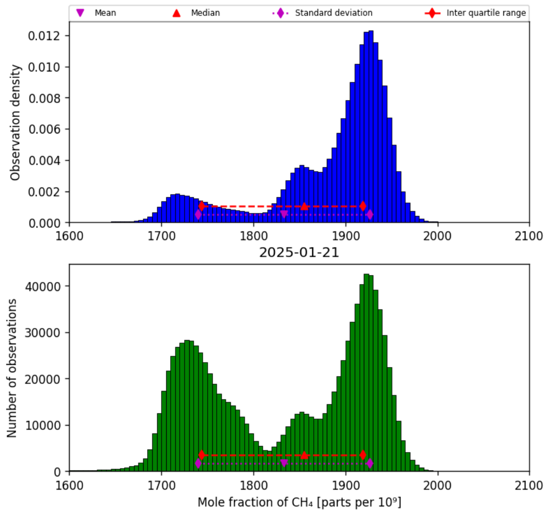
Figure 23: Histogram of “Mole fraction of CH 4 ” for 2025-01-20 to 2025-01-22
