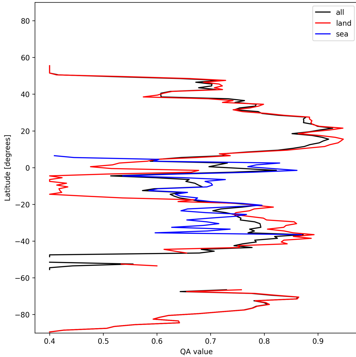
Figure 11: Zonal average of “QA value” for 2025-01-21 to 2025-01-23.
