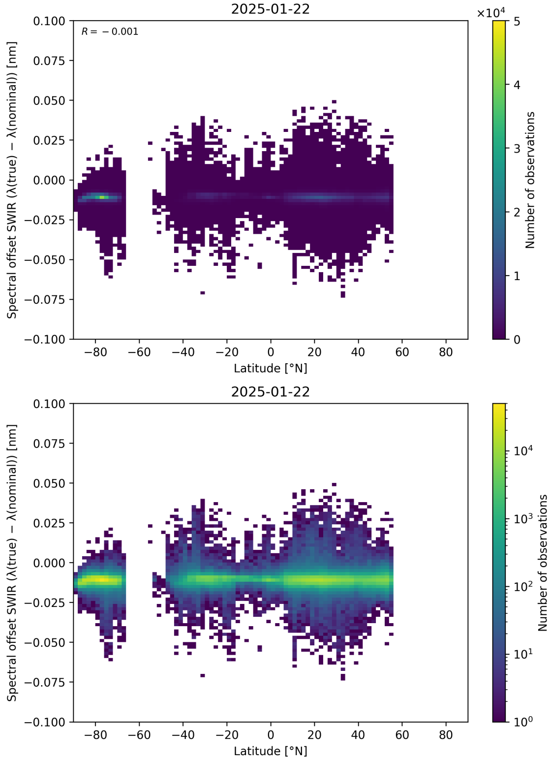
Figure 62: Scatter density plot of “Latitude” against “Spectral offset SWIR ( \lambda_{\text{true}} - \lambda_{\text{nominal}} )” for 2025-01-21 to 2025-01-23.
