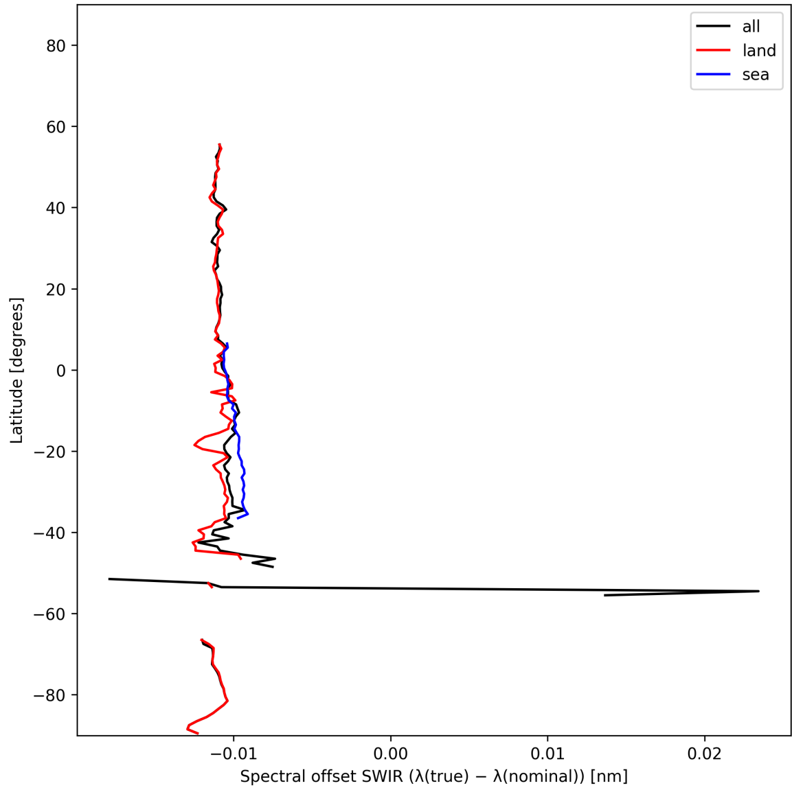
Figure 16: Zonal average of “Spectral offset SWIR ( \lambda_{\text{true}} - \lambda_{\text{nominal}} )” for 2025-01-21 to 2025-01-23.
