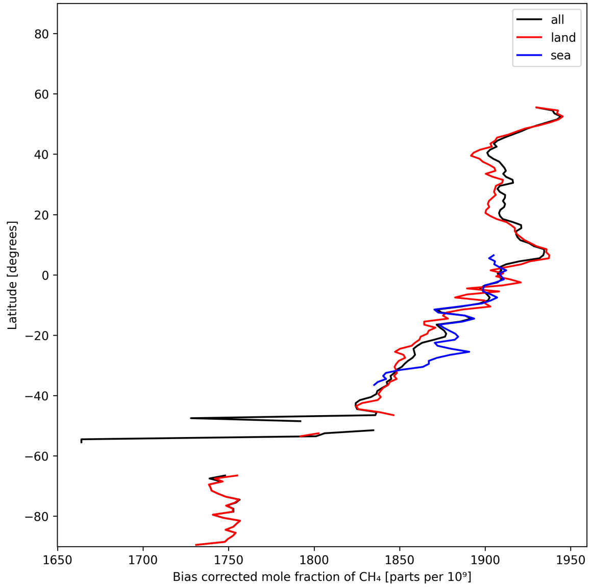
Figure 14: Zonal average of “Bias corrected mole fraction of CH 4 ” for 2025-01-21 to 2025-01-23.
