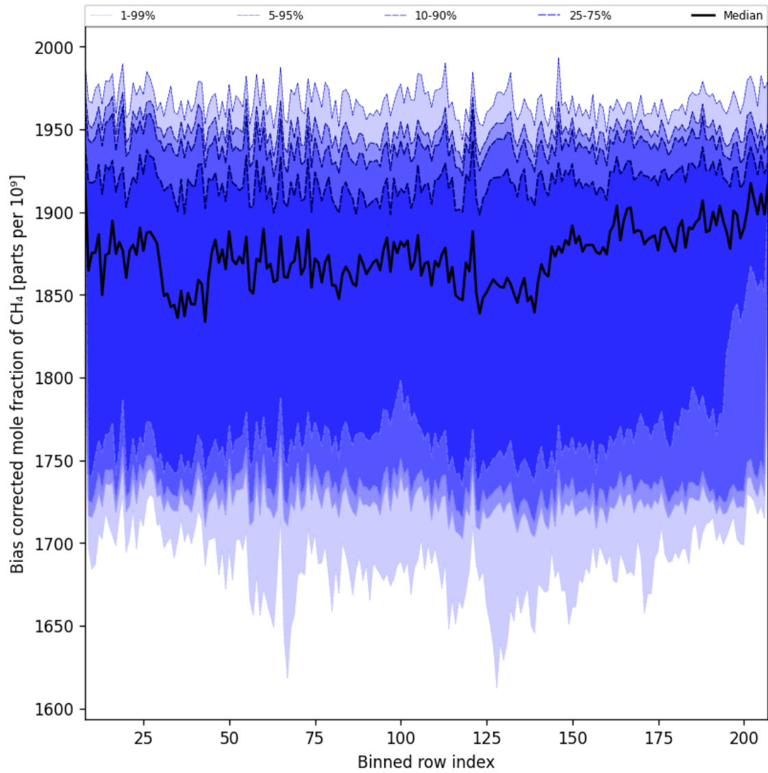
Figure 36: Along track statistics of “Bias corrected mole fraction of CH 4 ” for 2025-01-21 to 2025-01-23
