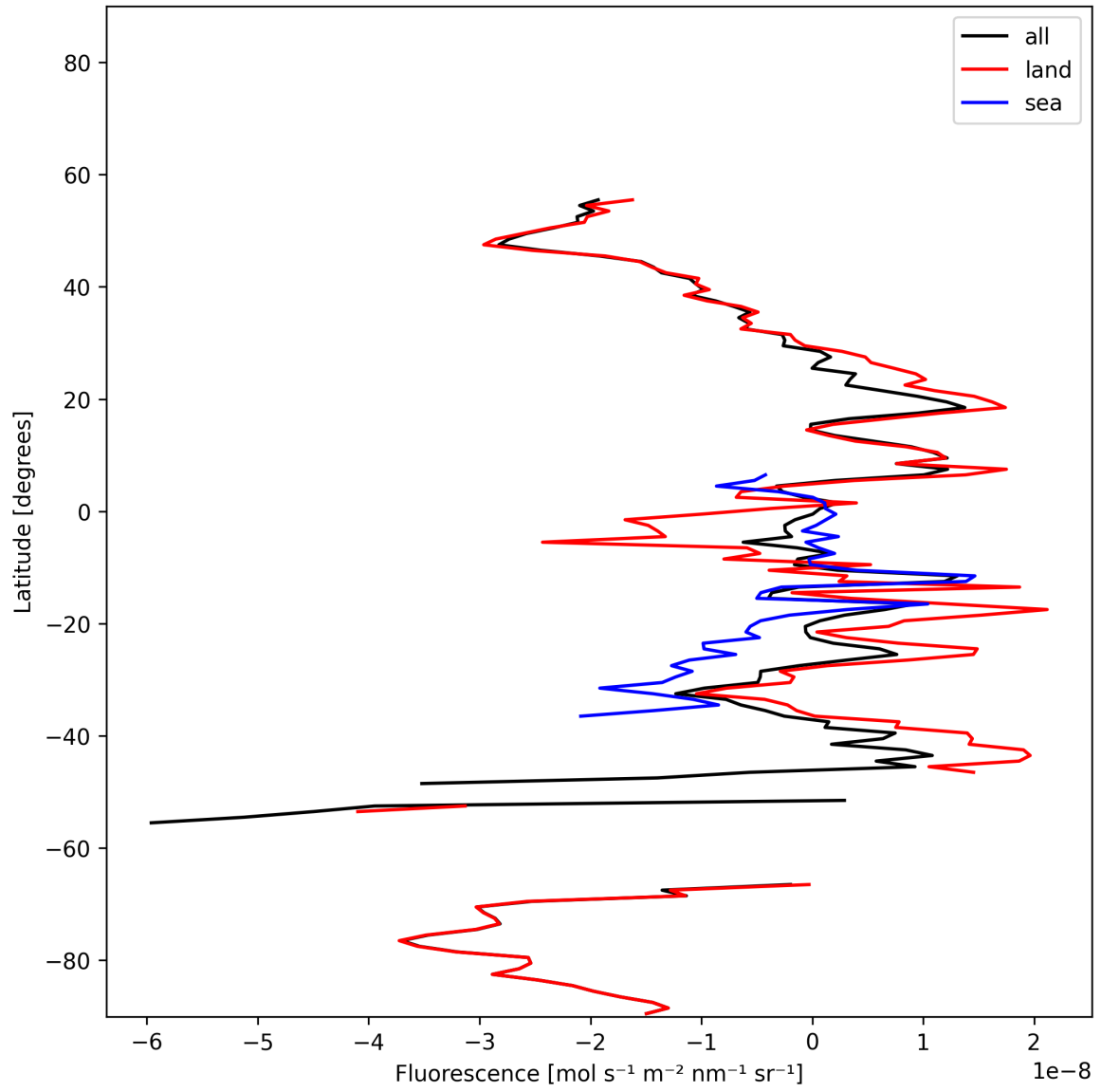
Figure 21: Zonal average of “Fluorescence” for 2025-01-21 to 2025-01-23.
