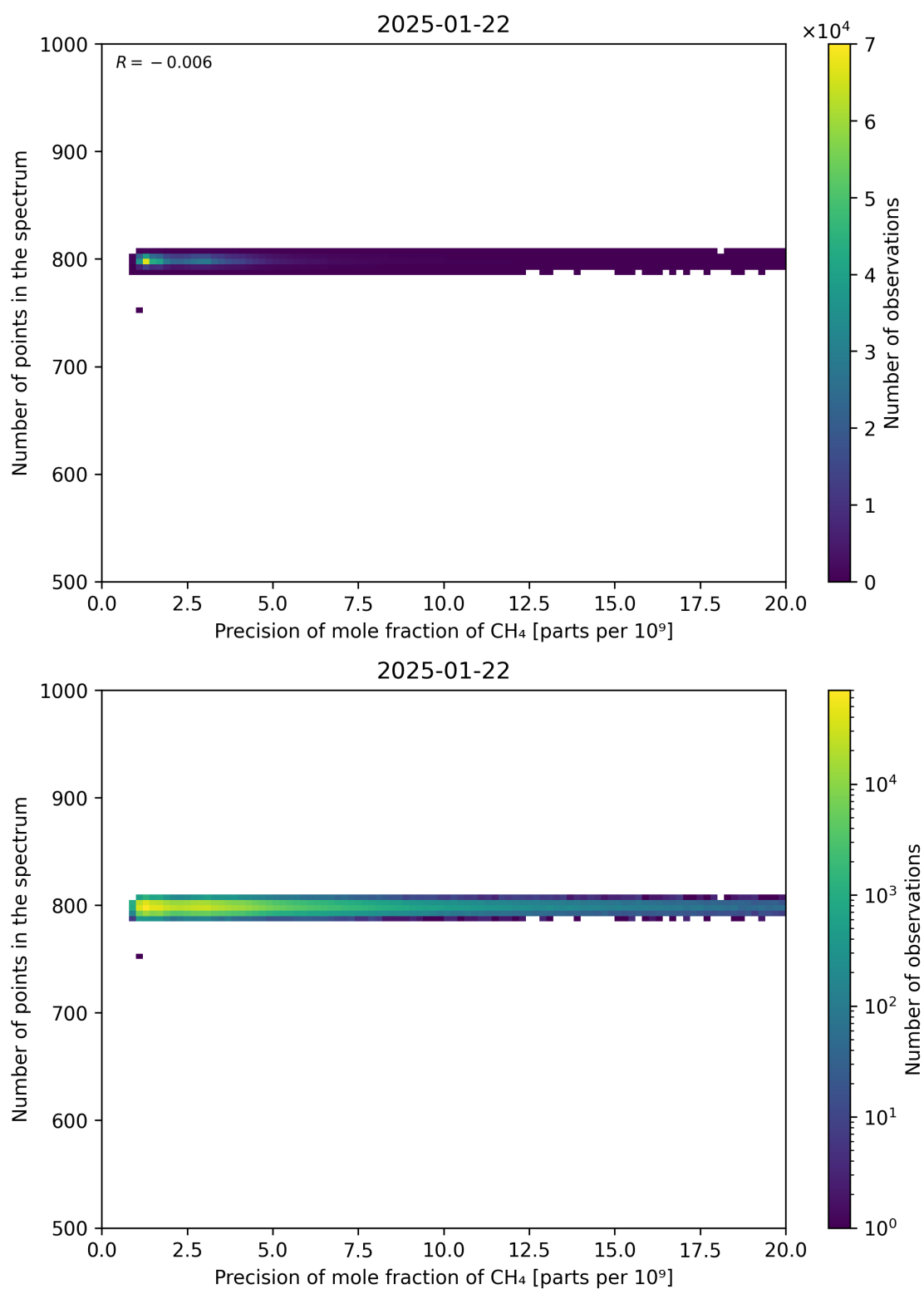
Figure 84: Scatter density plot of “Precision of mole fraction of CH 4 ” against “Number of points in the spectrum” for 2025-01-21 to 2025-01-23.
