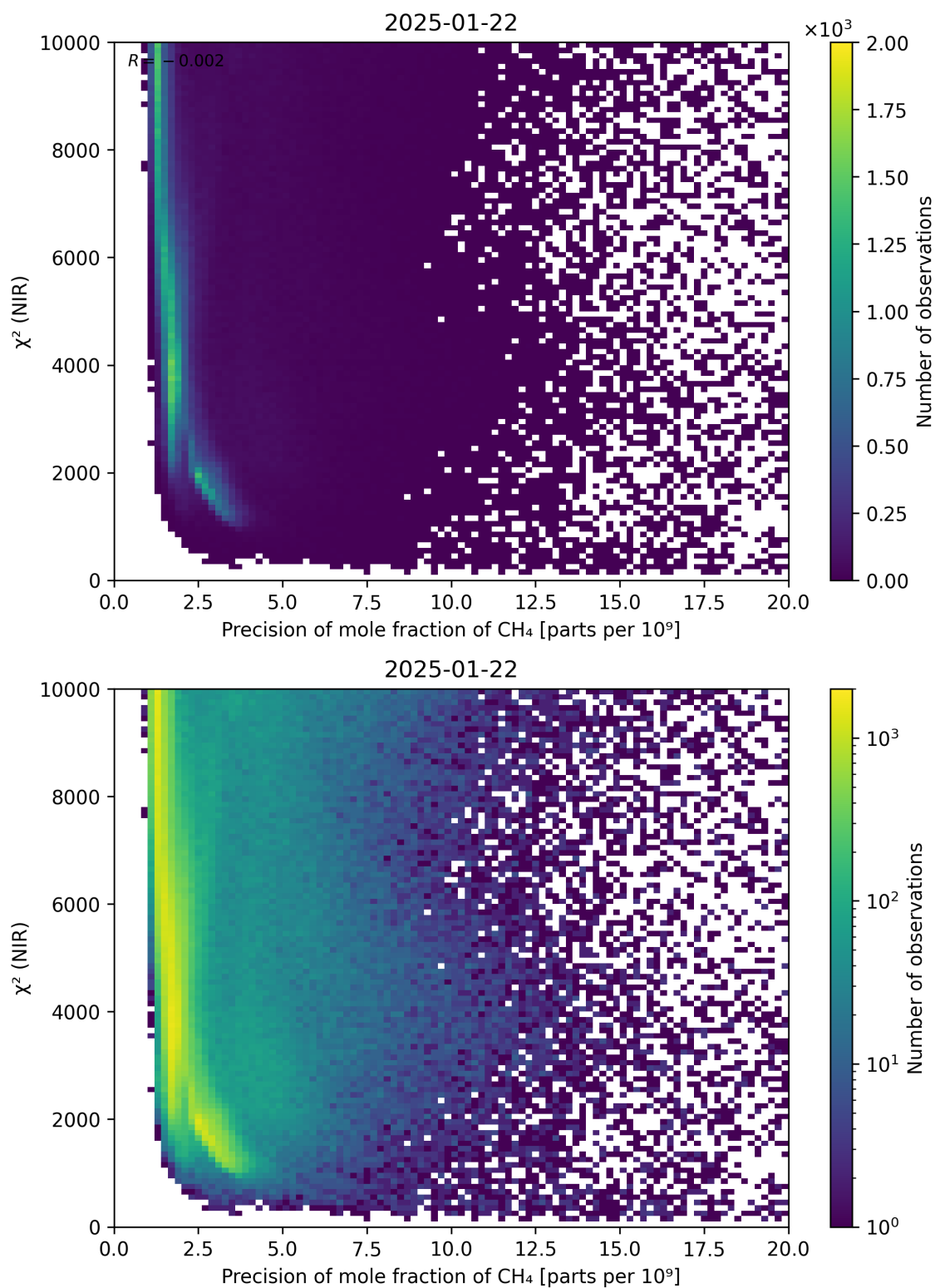
Figure 78: Scatter density plot of “Precision of mole fraction of CH 4 ” against “ \chi^2 (NIR)” for 2025-01-21 to 2025-01-23.
