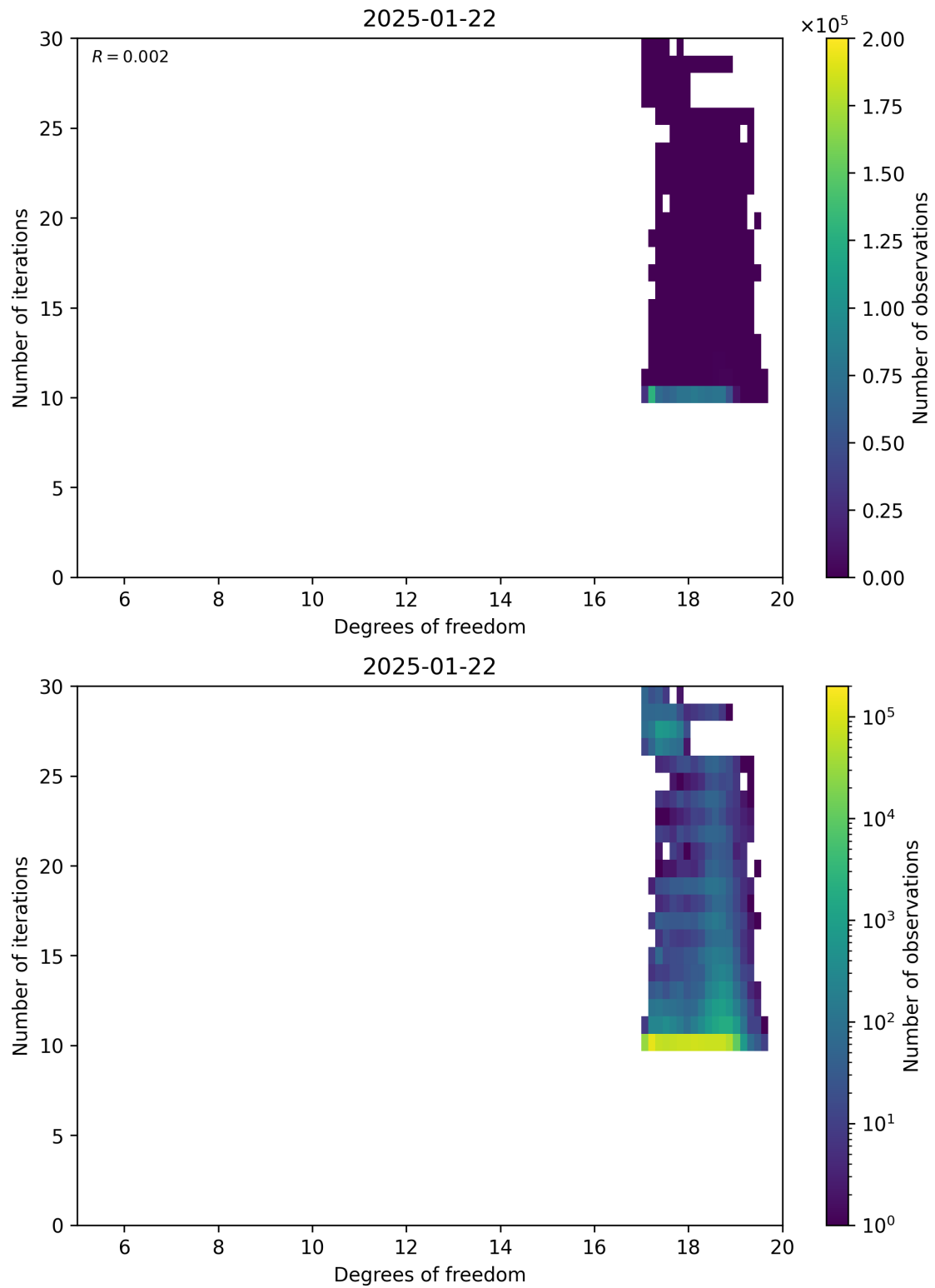
Figure 52: Scatter density plot of “Degrees of freedom” against “Number of iterations” for 2025-01-21 to 2025-01-23.
