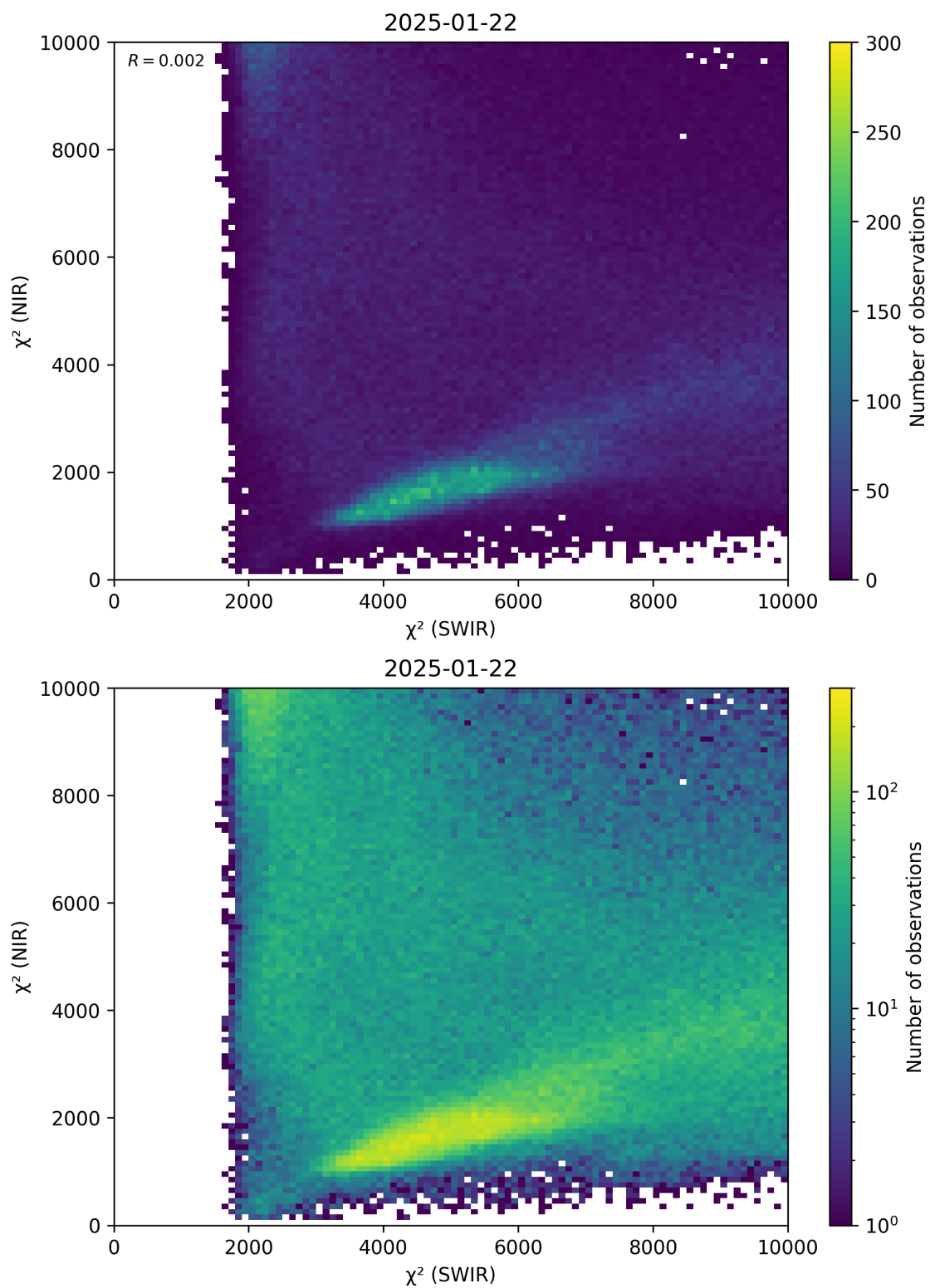
Figure 47: Scatter density plot of “ \chi^2 (SWIR)” against “ \chi^2 (NIR)” for 2025-01-21 to 2025-01-23.
