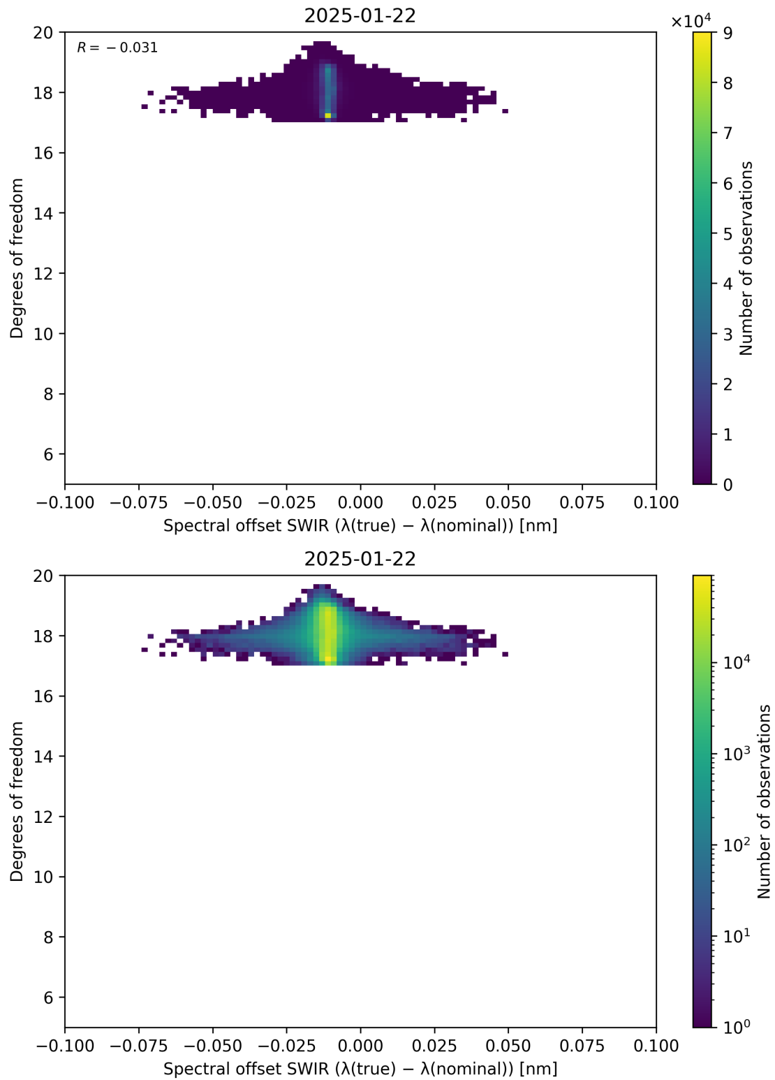
Figure 119: Scatter density plot of “Spectral offset SWIR ( \lambda_{\text{true}} - \lambda_{\text{nominal}} )” against “Degrees of freedom” for 2025-01-21 to 2025-01-23.
