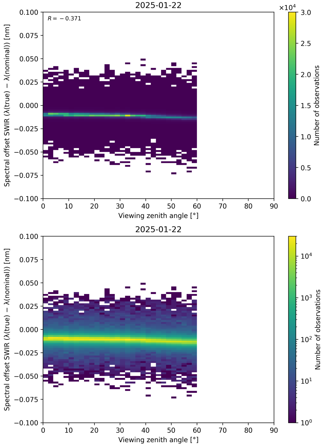
Figure 116: Scatter density plot of “Viewing zenith angle” against “Spectral offset SWIR ( \lambda_{\text{true}} - \lambda_{\text{nominal}} )” for 2025-01-21 to 2025-01-23.
