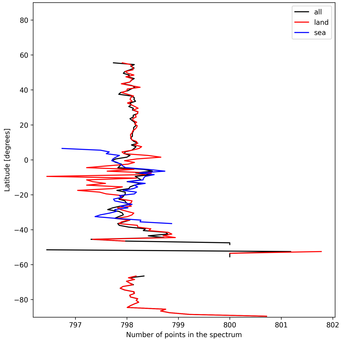
Figure 15: Zonal average of “Number of points in the spectrum” for 2025-01-21 to 2025-01-23.
