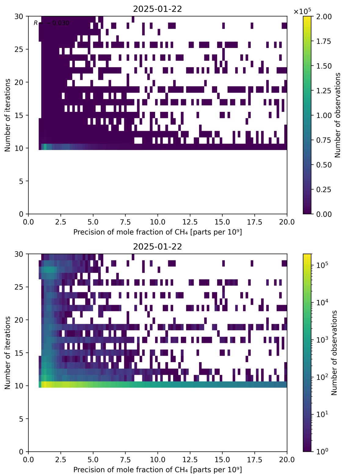
Figure 83: Scatter density plot of “Precision of mole fraction of CH 4 ” against “Number of iterations” for 2025-01-21 to 2025-01-23.
