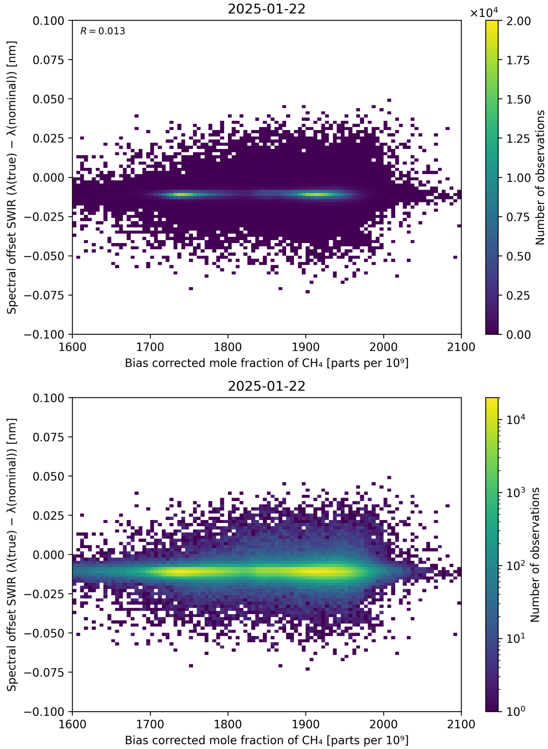
Figure 69: Scatter density plot of “Bias corrected mole fraction of \text{CH}_4 ” against “Spectral offset SWIR ( \lambda_{\text{true}} - \lambda_{\text{nominal}} )” for 2025-01-21 to 2025-01-23.
