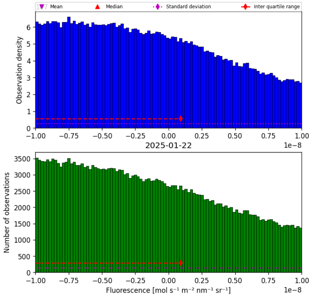
Figure 32: Histogram of “Fluorescence” for 2025-01-21 to 2025-01-23
