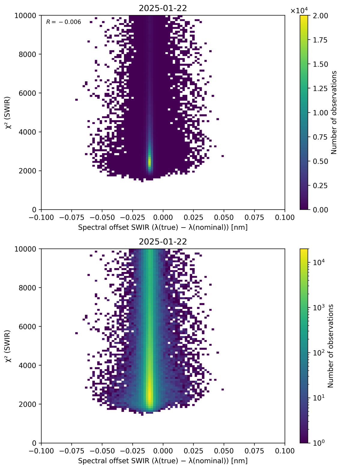
Figure 118: Scatter density plot of “Spectral offset SWIR ( \lambda_{\text{true}} - \lambda_{\text{nominal}} )” against “ \chi^2 (SWIR)” for 2025-01-21 to 2025-01-23.
