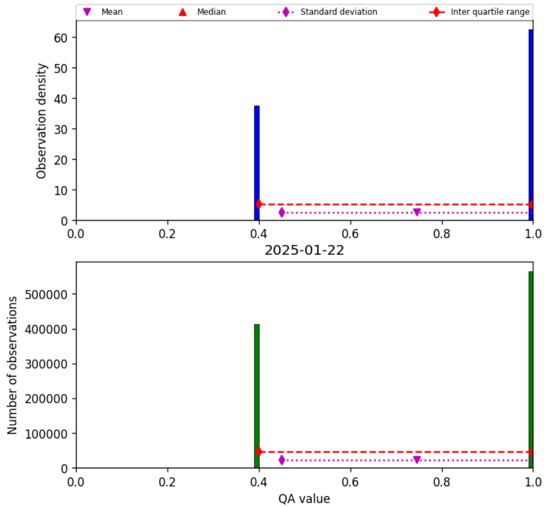
Figure 22: Histogram of “QA value” for 2025-01-21 to 2025-01-23
