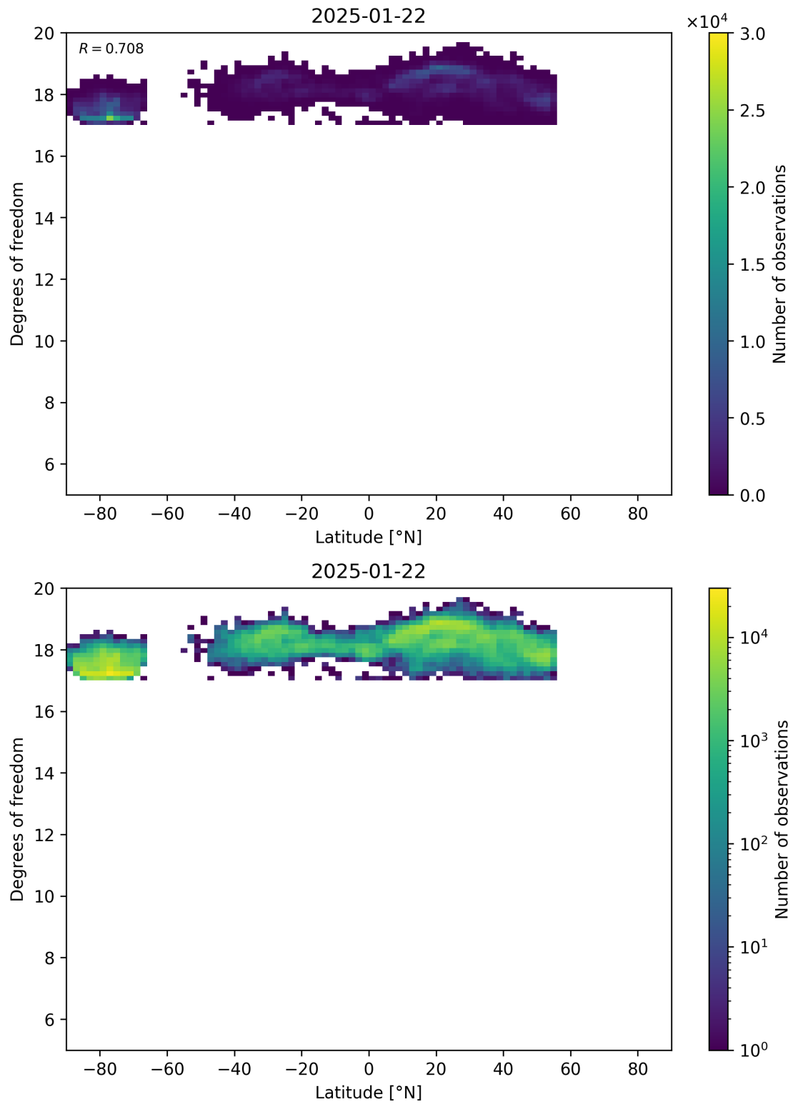
Figure 55: Scatter density plot of “Latitude” against “Degrees of freedom” for 2025-01-21 to 2025-01-23.
