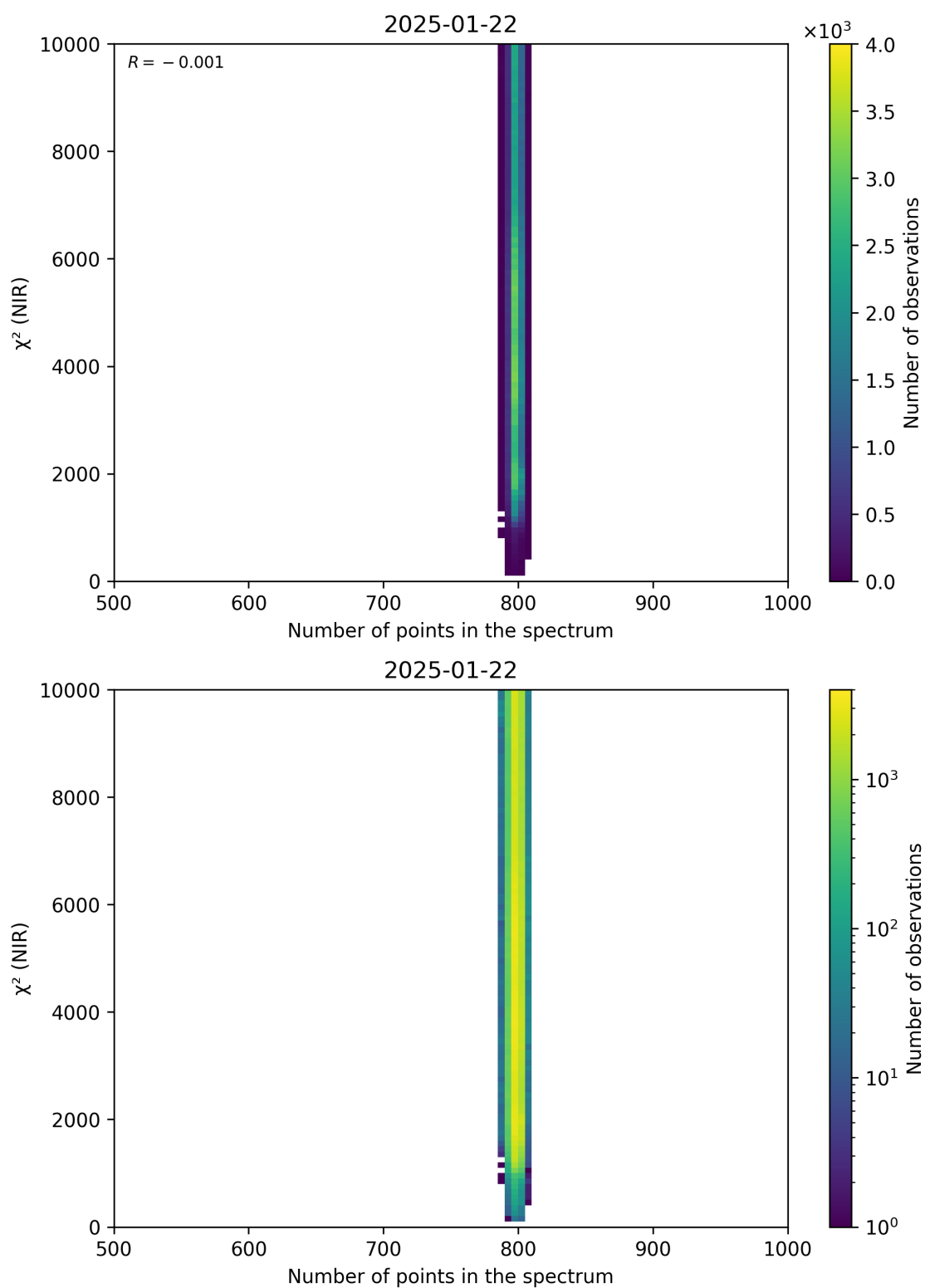
Figure 88: Scatter density plot of “Number of points in the spectrum” against “ \chi^2 (NIR)” for 2025-01-21 to 2025-01-23.
