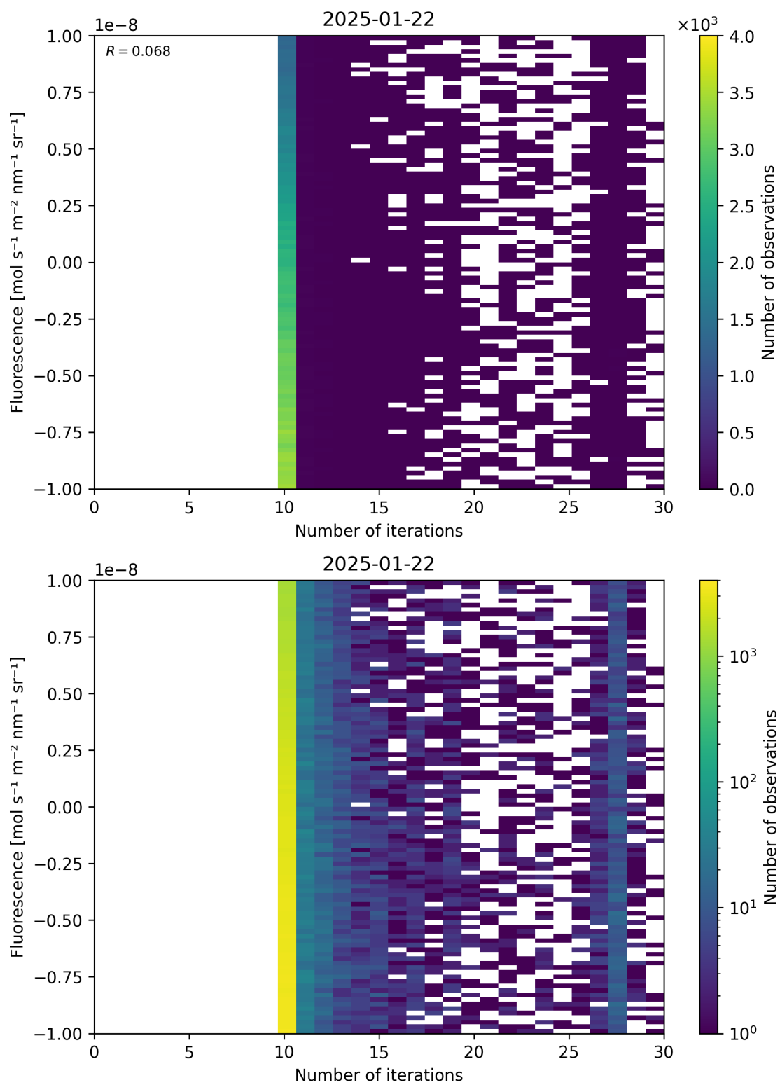
Figure 87: Scatter density plot of “Number of iterations” against “Fluorescence” for 2025-01-21 to 2025-01-23.
