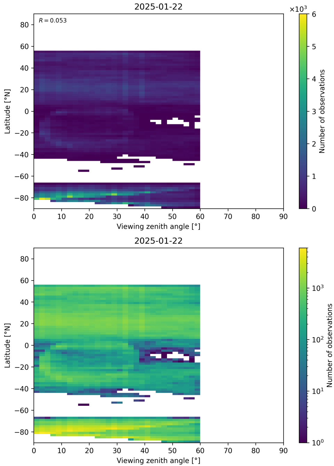
Figure 109: Scatter density plot of “Viewing zenith angle” against “Latitude” for 2025-01-21 to 2025-01-23.
