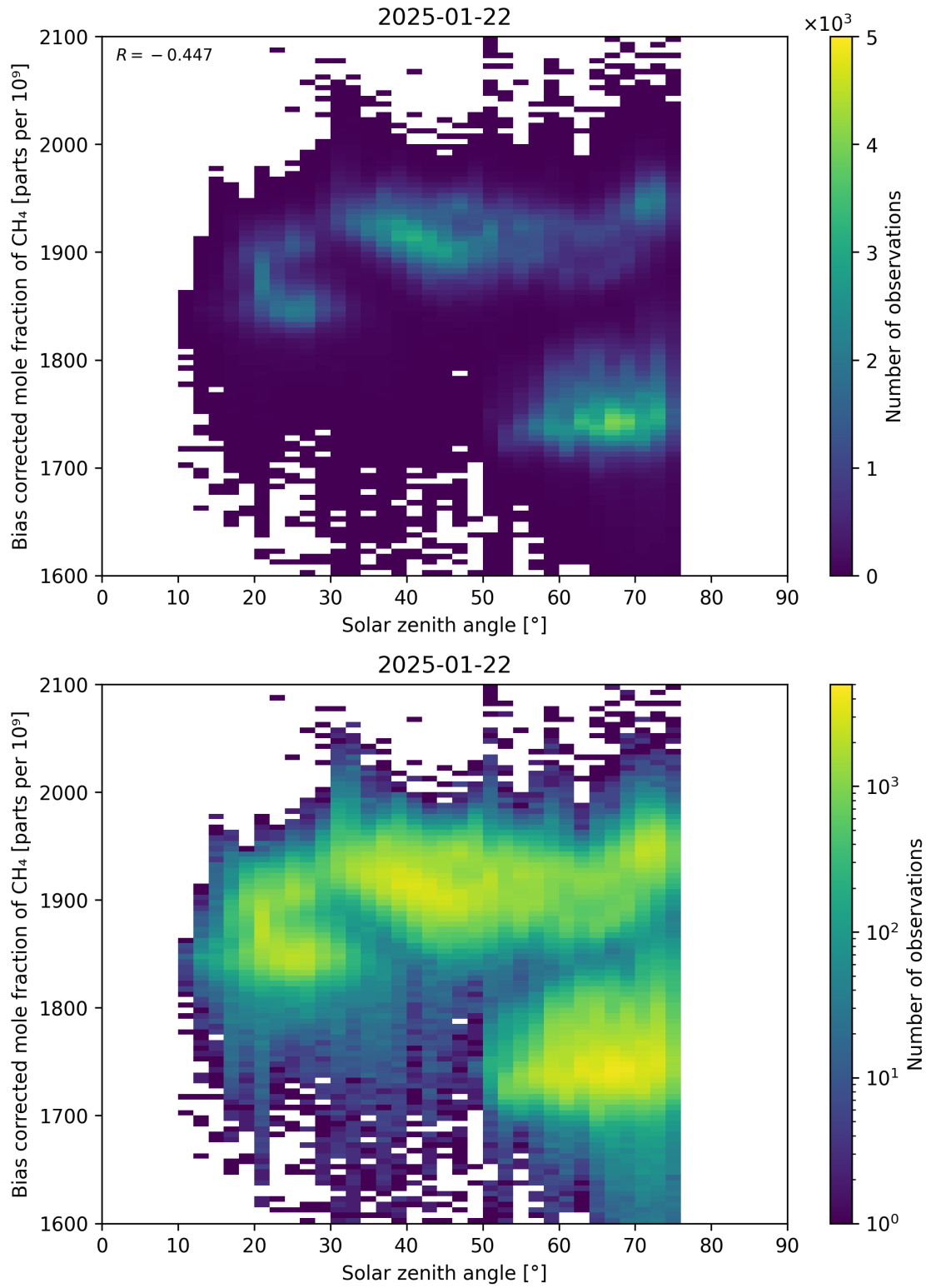
Figure 100: Scatter density plot of “Solar zenith angle” against “Bias corrected mole fraction of CH 4 ” for 2025-01-21 to 2025-01-23.
