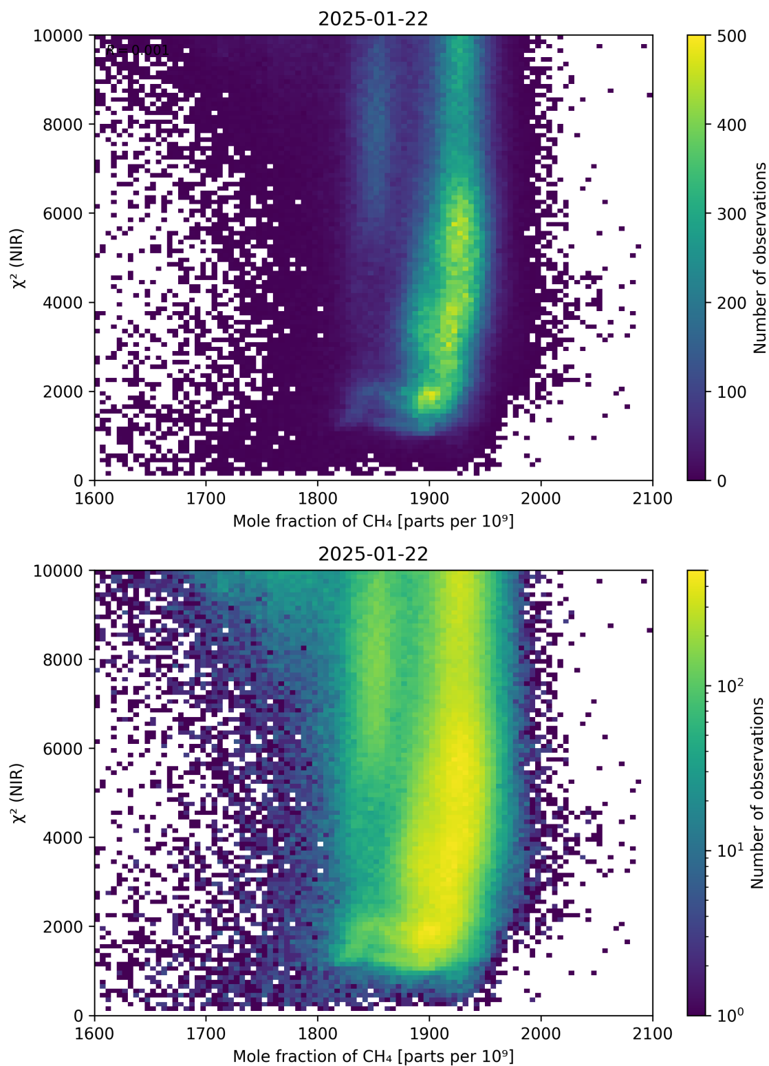
Figure 70: Scatter density plot of “Mole fraction of \text{CH}_4 ” against “ \chi^2 (NIR)” for 2025-01-21 to 2025-01-23.
