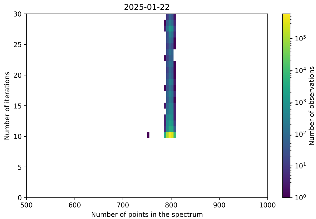
Figure 92: Scatter density plot of “Number of points in the spectrum” against “Number of iterations” for 2025-01-21 to 2025-01-23.
