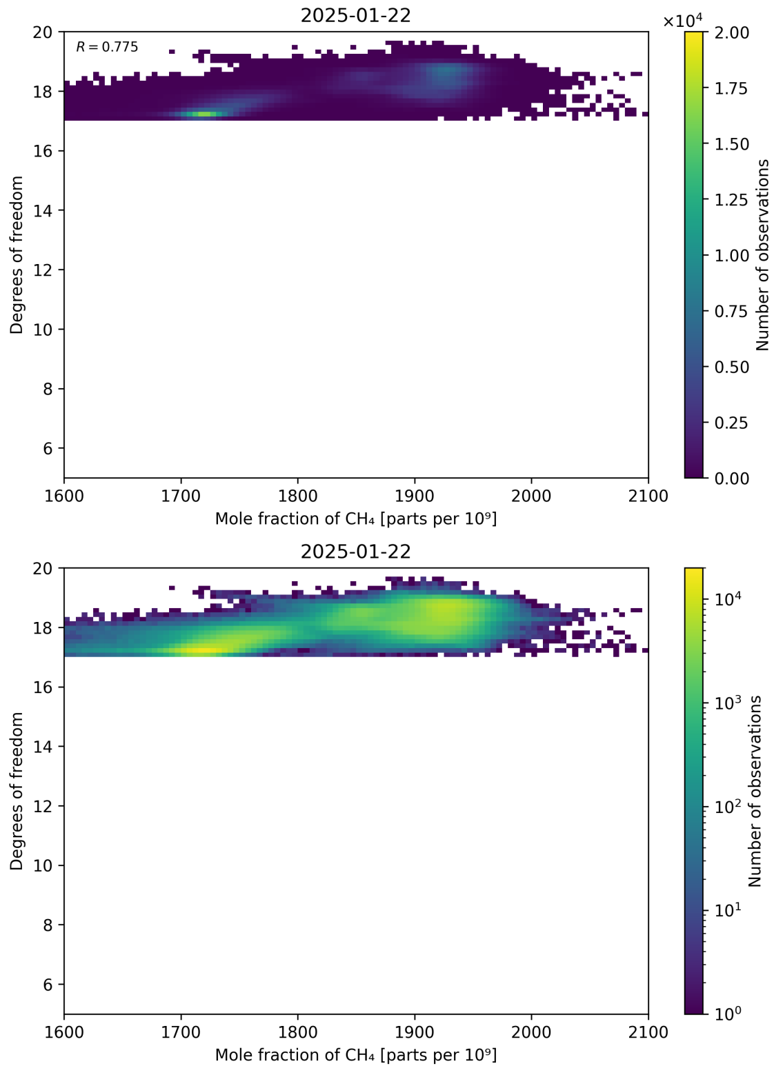
Figure 72: Scatter density plot of “Mole fraction of CH 4 ” against “Degrees of freedom” for 2025-01-21 to 2025-01-23.
