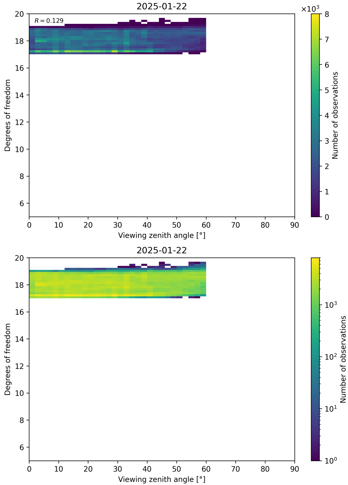
Figure 107: Scatter density plot of “Viewing zenith angle” against “Degrees of freedom” for 2025-01-21 to 2025-01-23.
