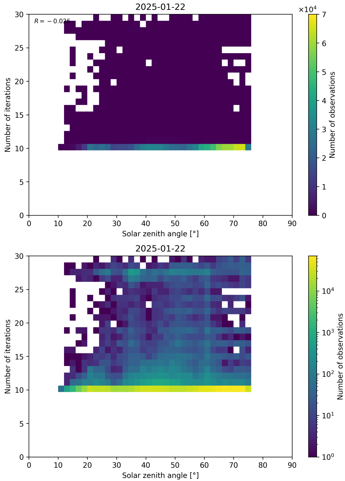
Figure 102: Scatter density plot of “Solar zenith angle” against “Number of iterations” for 2025-01-21 to 2025-01-23.
