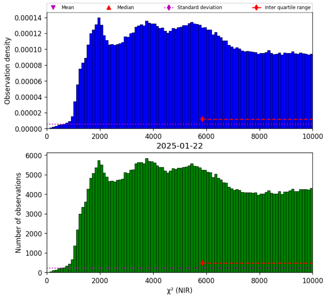
Figure 29: Histogram of “ \chi^2 (NIR)” for 2025-01-21 to 2025-01-23
