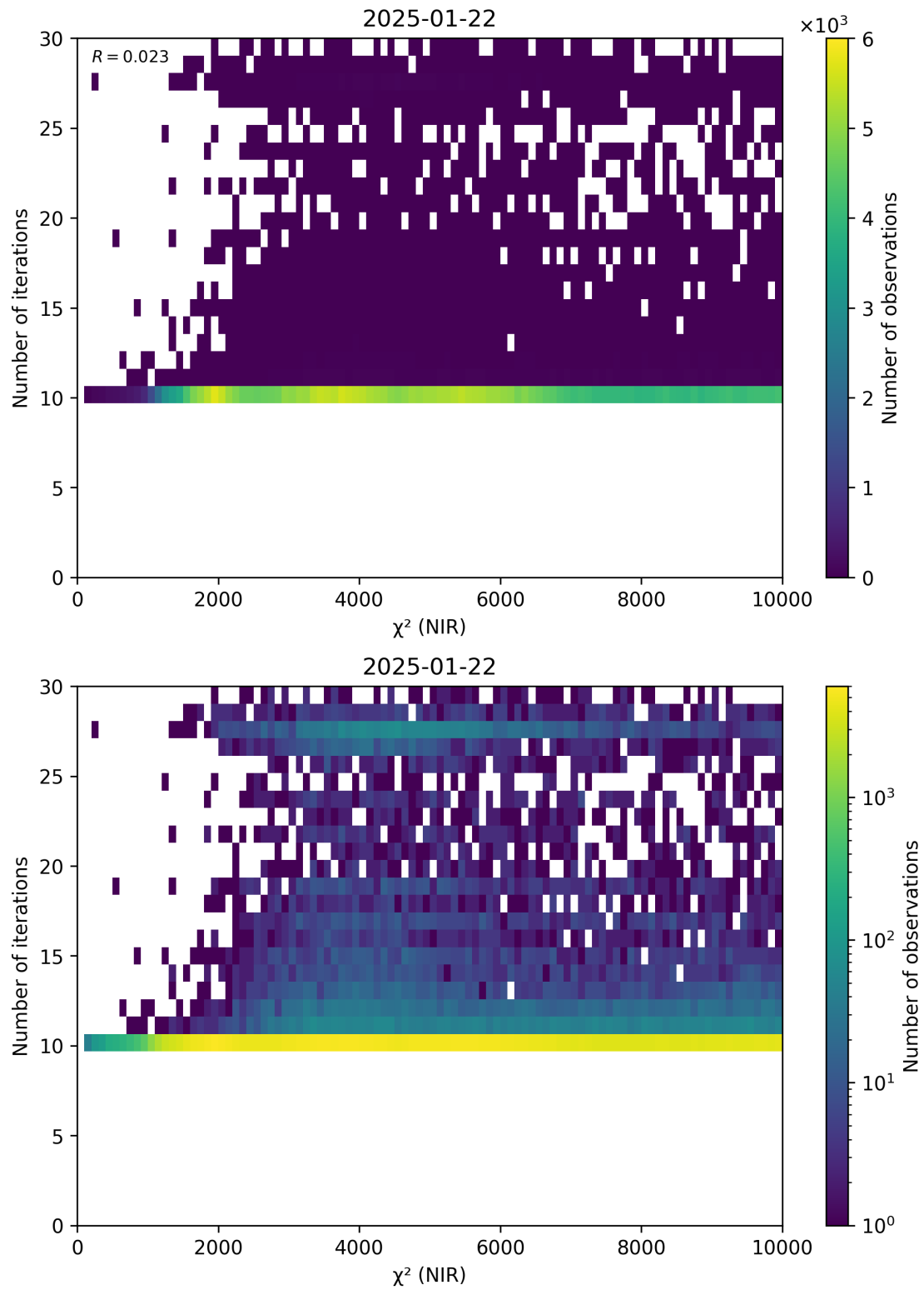
Figure 46: Scatter density plot of “ \chi^2 (NIR)” against “Number of iterations” for 2025-01-21 to 2025-01-23.
