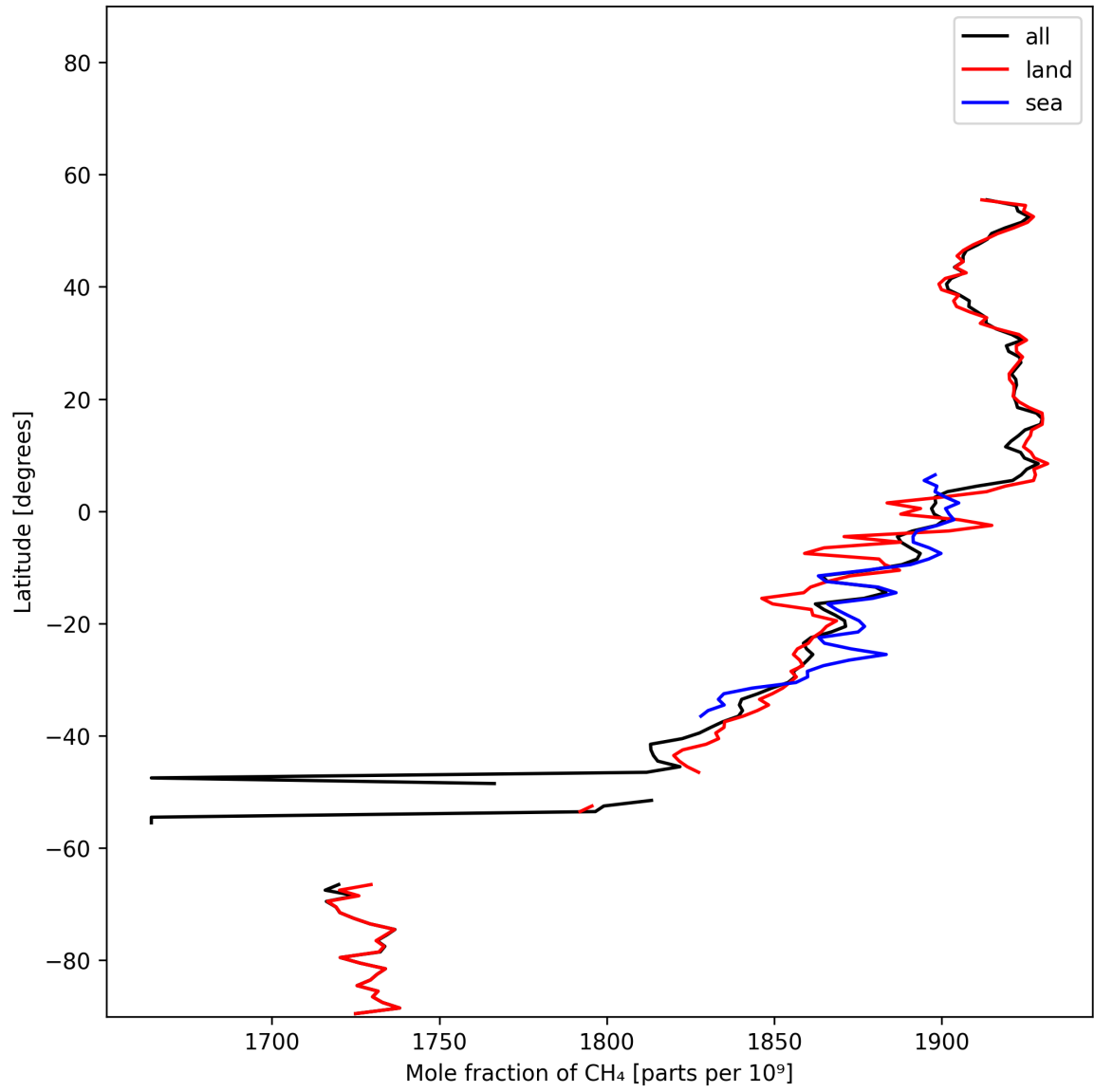
Figure 12: Zonal average of “Mole fraction of \text{CH}_4 ” for 2025-01-21 to 2025-01-23.
