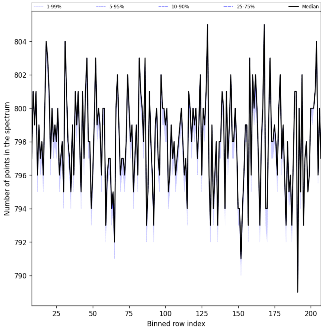
Figure 37: Along track statistics of “Number of points in the spectrum” for 2025-01-21 to 2025-01-23
