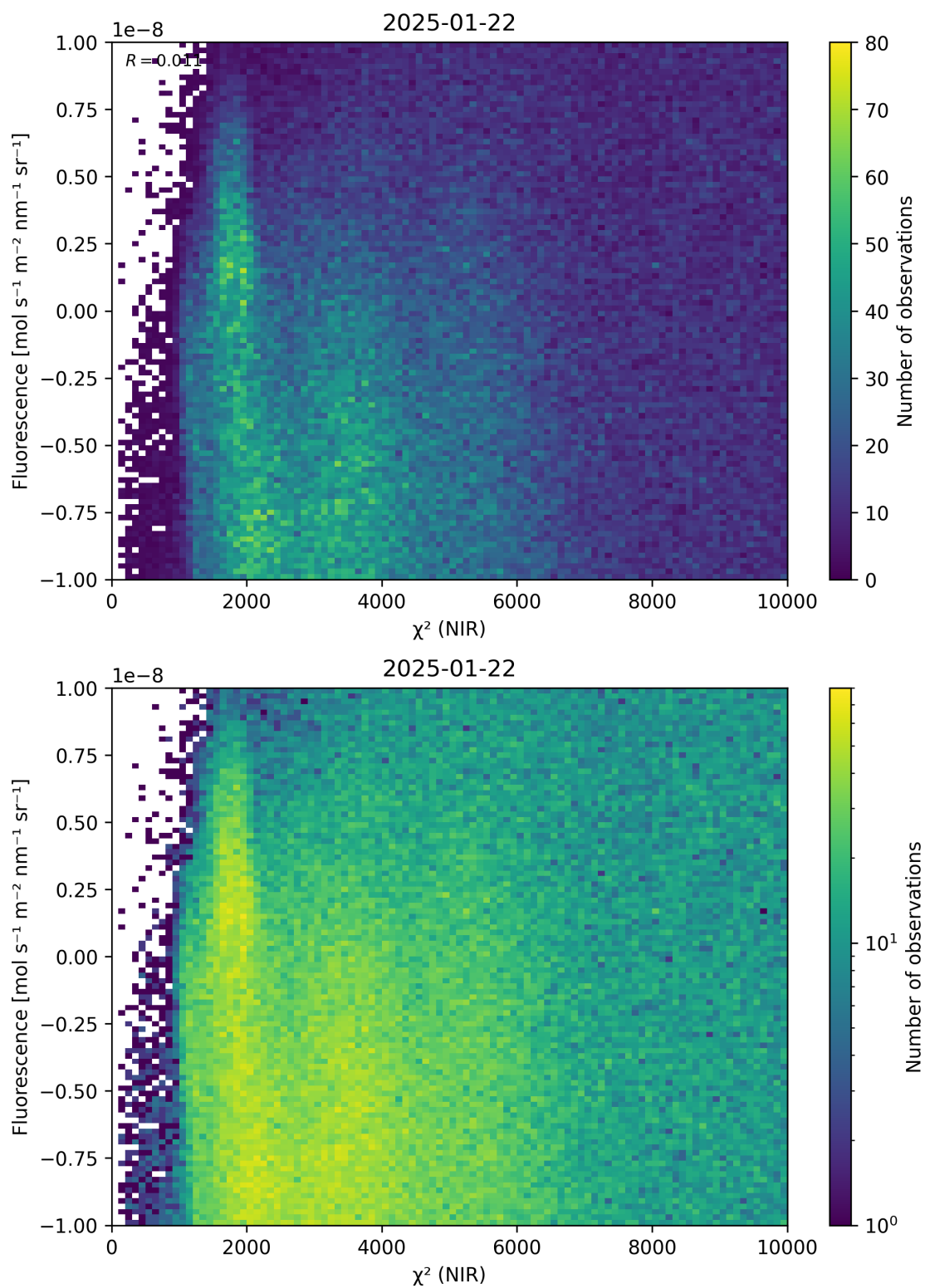
Figure 45: Scatter density plot of “ \chi^2 (NIR)” against “Fluorescence” for 2025-01-21 to 2025-01-23.
