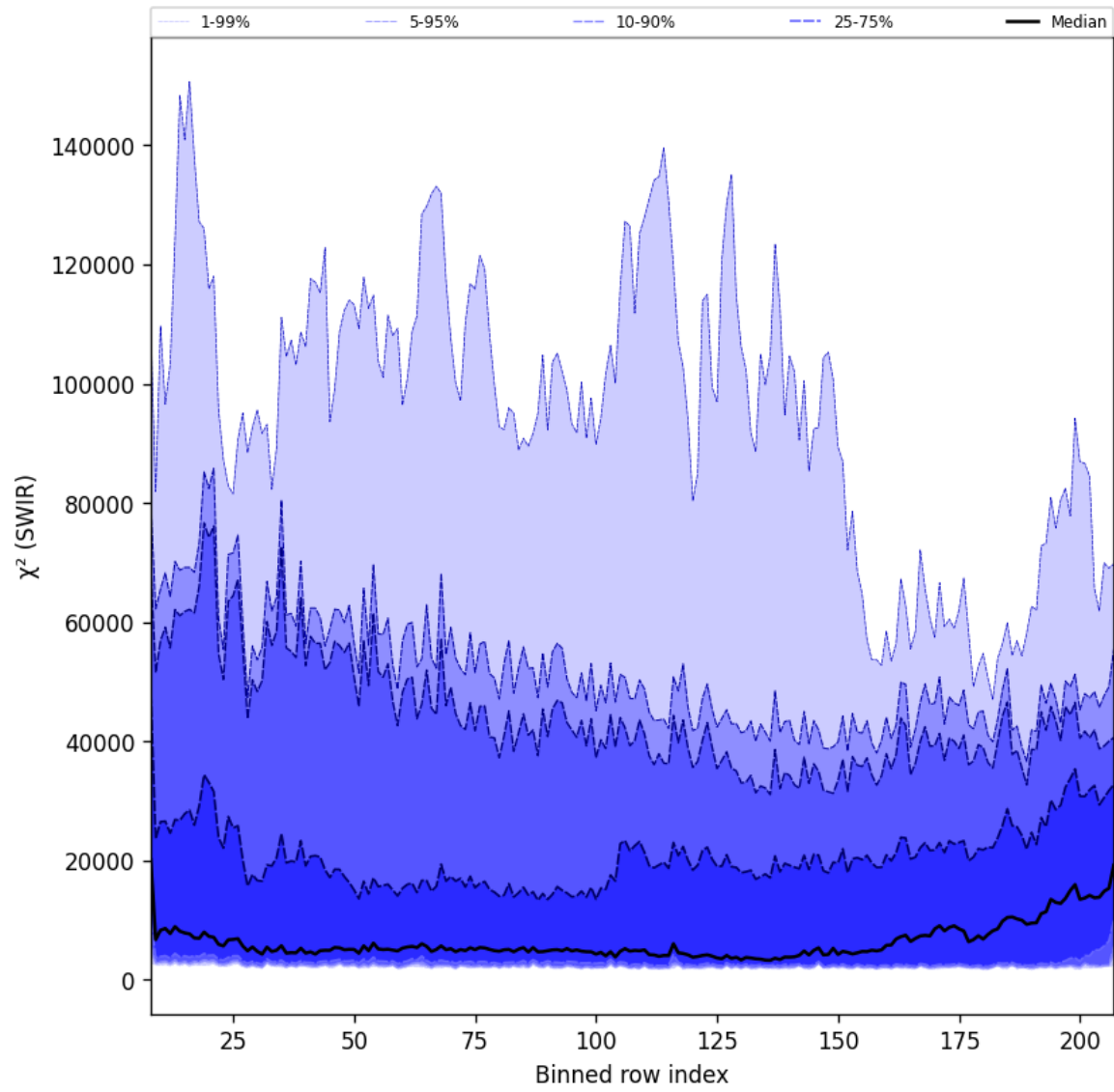
Figure 39: Along track statistics of “ \chi^2 (SWIR)” for 2025-01-21 to 2025-01-23
