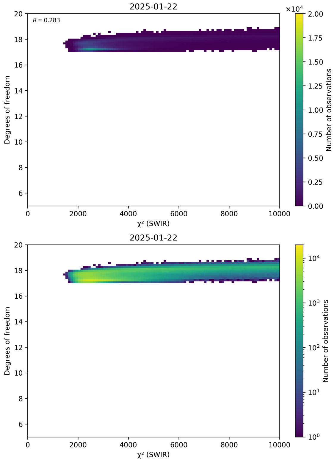
Figure 48: Scatter density plot of “ \chi^2 (SWIR)” against “Degrees of freedom” for 2025-01-21 to 2025-01-23.
