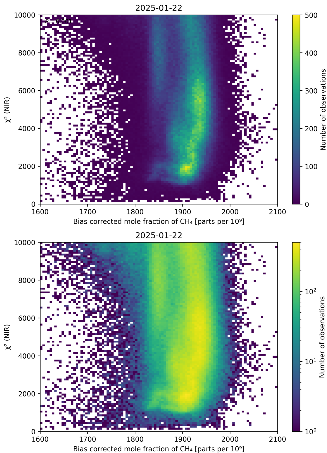
Figure 63: Scatter density plot of “Bias corrected mole fraction of \text{CH}_4 ” against “ \chi^2 (NIR)” for 2025-01-21 to 2025-01-23.
