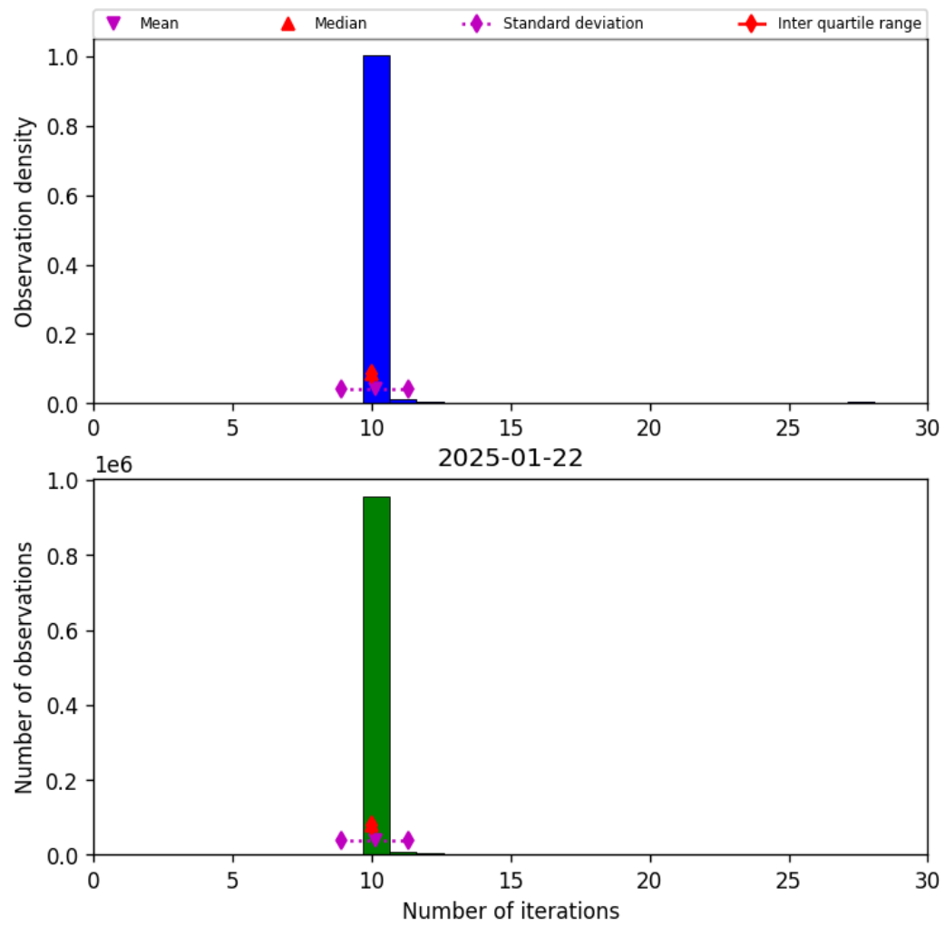
Figure 31: Histogram of "Number of iterations" for 2025-01-21 to 2025-01-23
