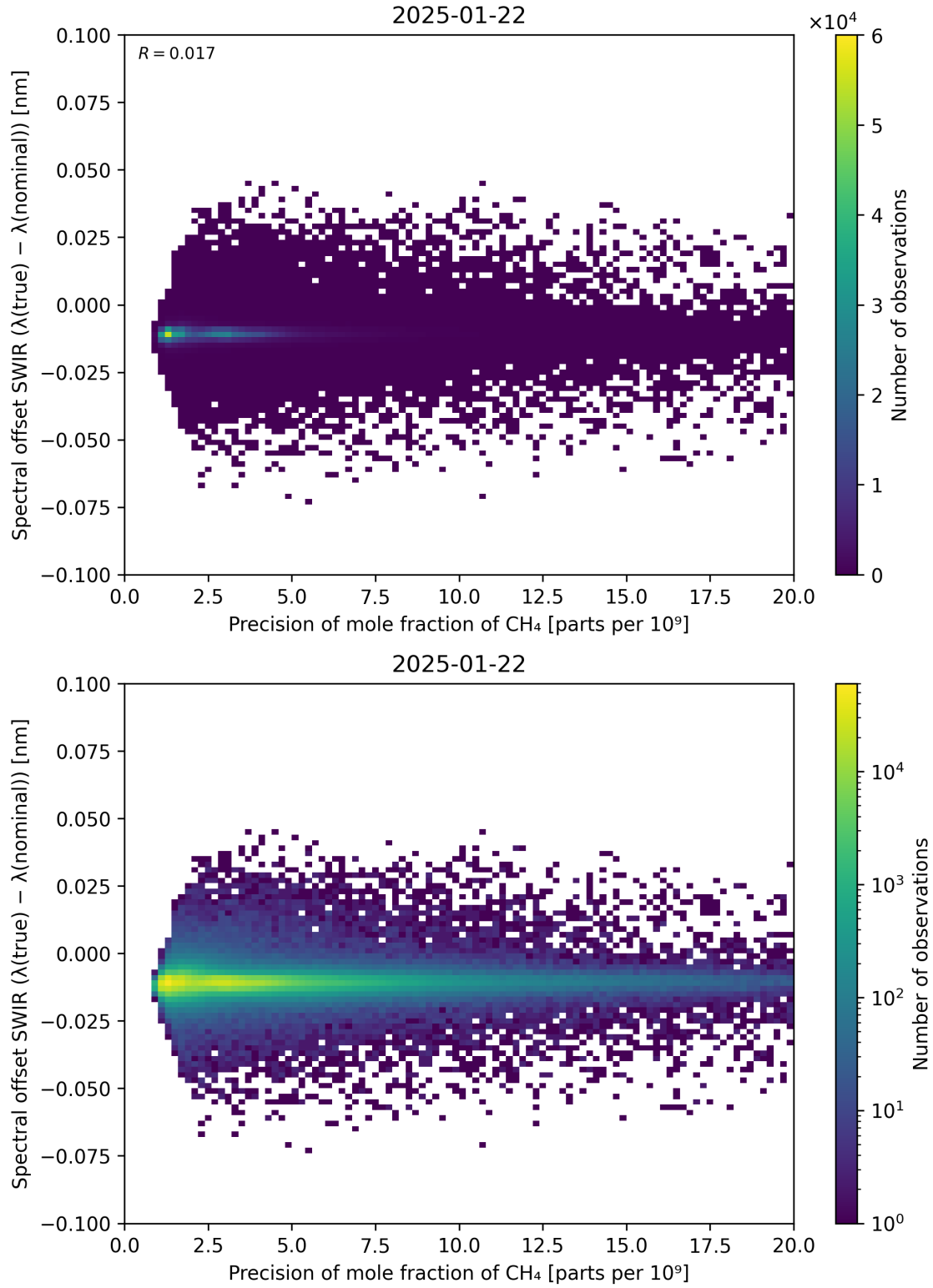
Figure 85: Scatter density plot of “Precision of mole fraction of CH 4 ” against “Spectral offset SWIR ( \lambda_{\text{true}} - \lambda_{\text{nominal}} )” for 2025-01-21 to 2025-01-23.
