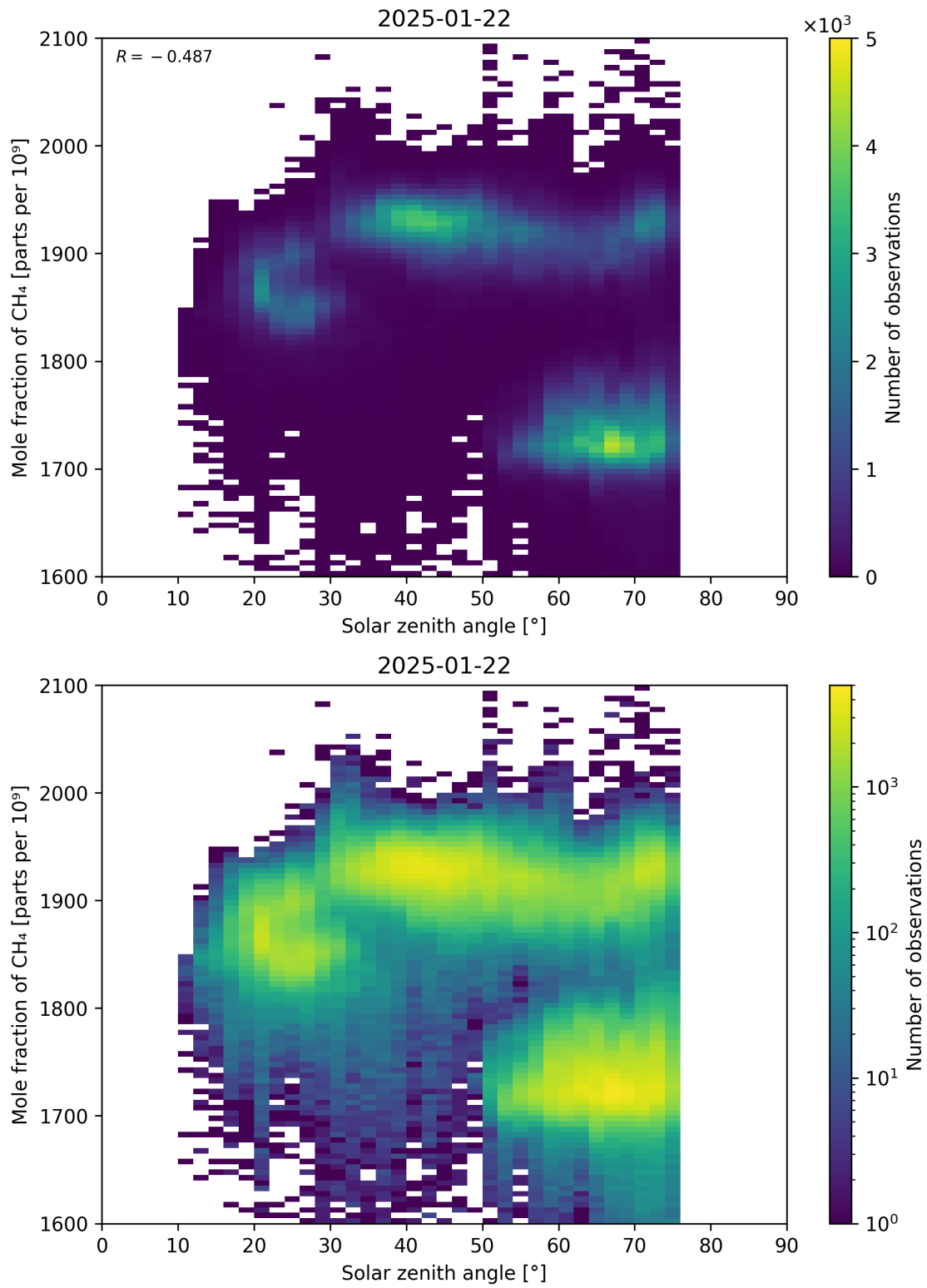
Figure 99: Scatter density plot of “Solar zenith angle” against “Mole fraction of CH 4 ” for 2025-01-21 to 2025-01-23.
