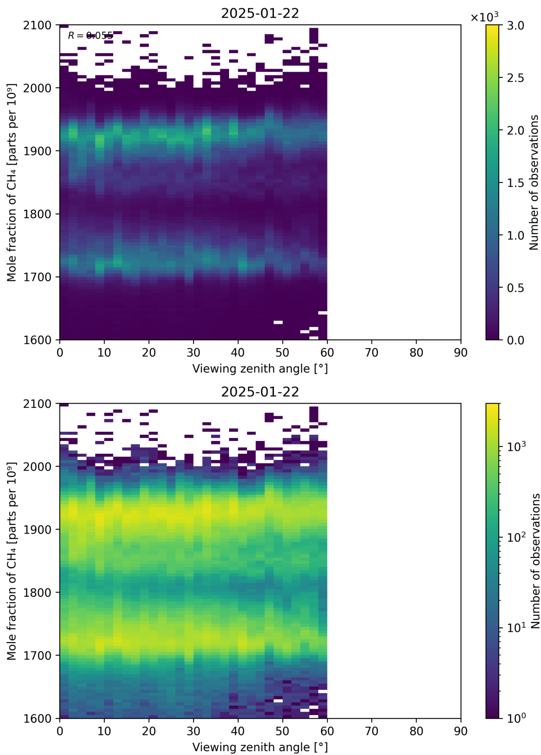
Figure 110: Scatter density plot of “Viewing zenith angle” against “Mole fraction of CH 4 ” for 2025-01-21 to 2025-01-23.
