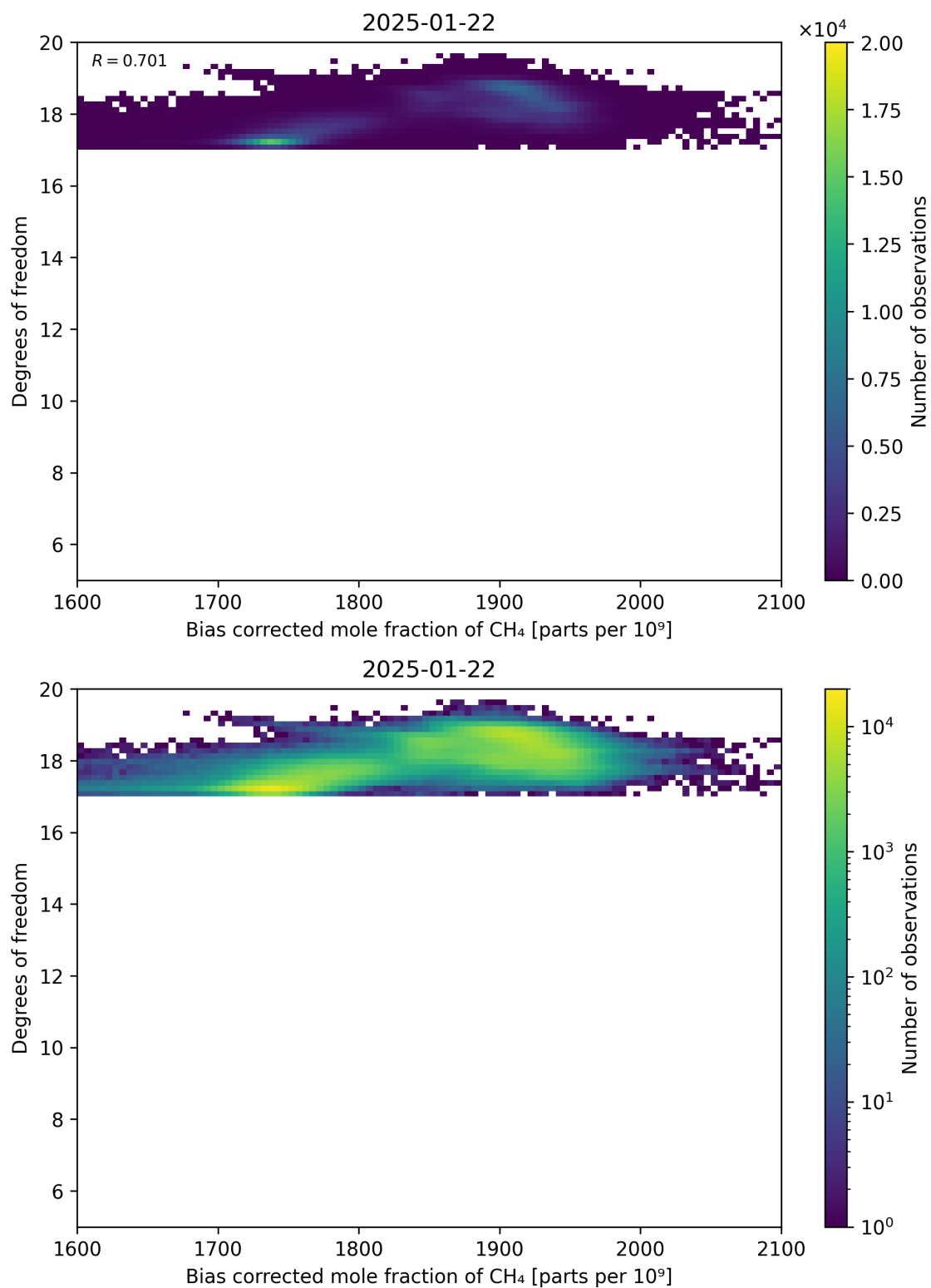
Figure 65: Scatter density plot of “Bias corrected mole fraction of CH 4 ” against “Degrees of freedom” for 2025-01-21 to 2025-01-23.
