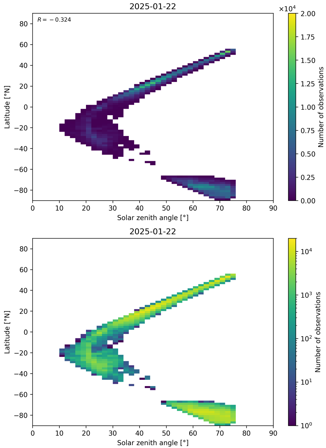
Figure 98: Scatter density plot of “Solar zenith angle” against “Latitude” for 2025-01-21 to 2025-01-23.
