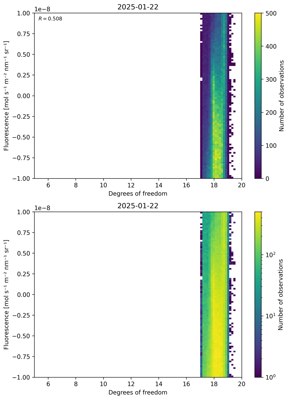
Figure 51: Scatter density plot of “Degrees of freedom” against “Fluorescence” for 2025-01-21 to 2025-01-23.
