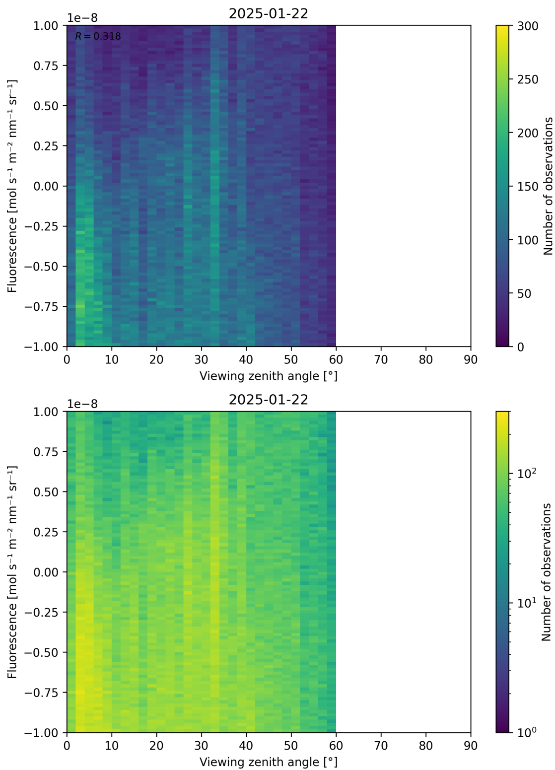
Figure 108: Scatter density plot of “Viewing zenith angle” against “Fluorescence” for 2025-01-21 to 2025-01-23.
