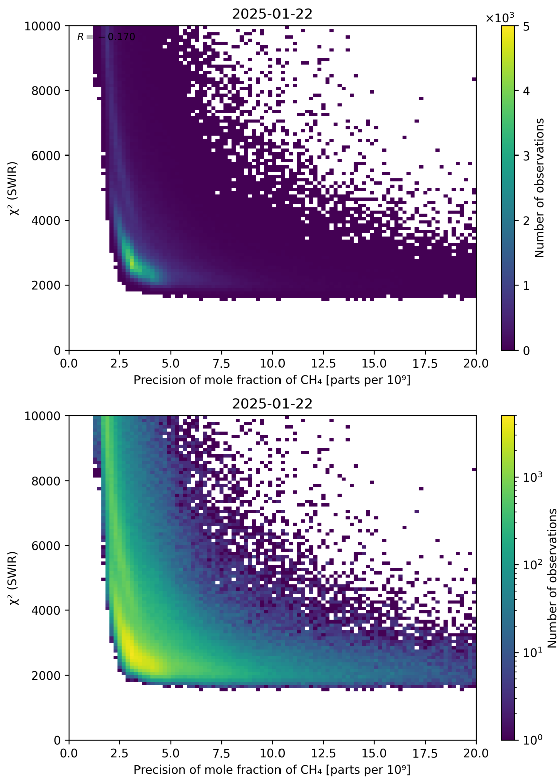
Figure 79: Scatter density plot of “Precision of mole fraction of \text{CH}_4 ” against “ \chi^2 (SWIR)” for 2025-01-21 to 2025-01-23.
