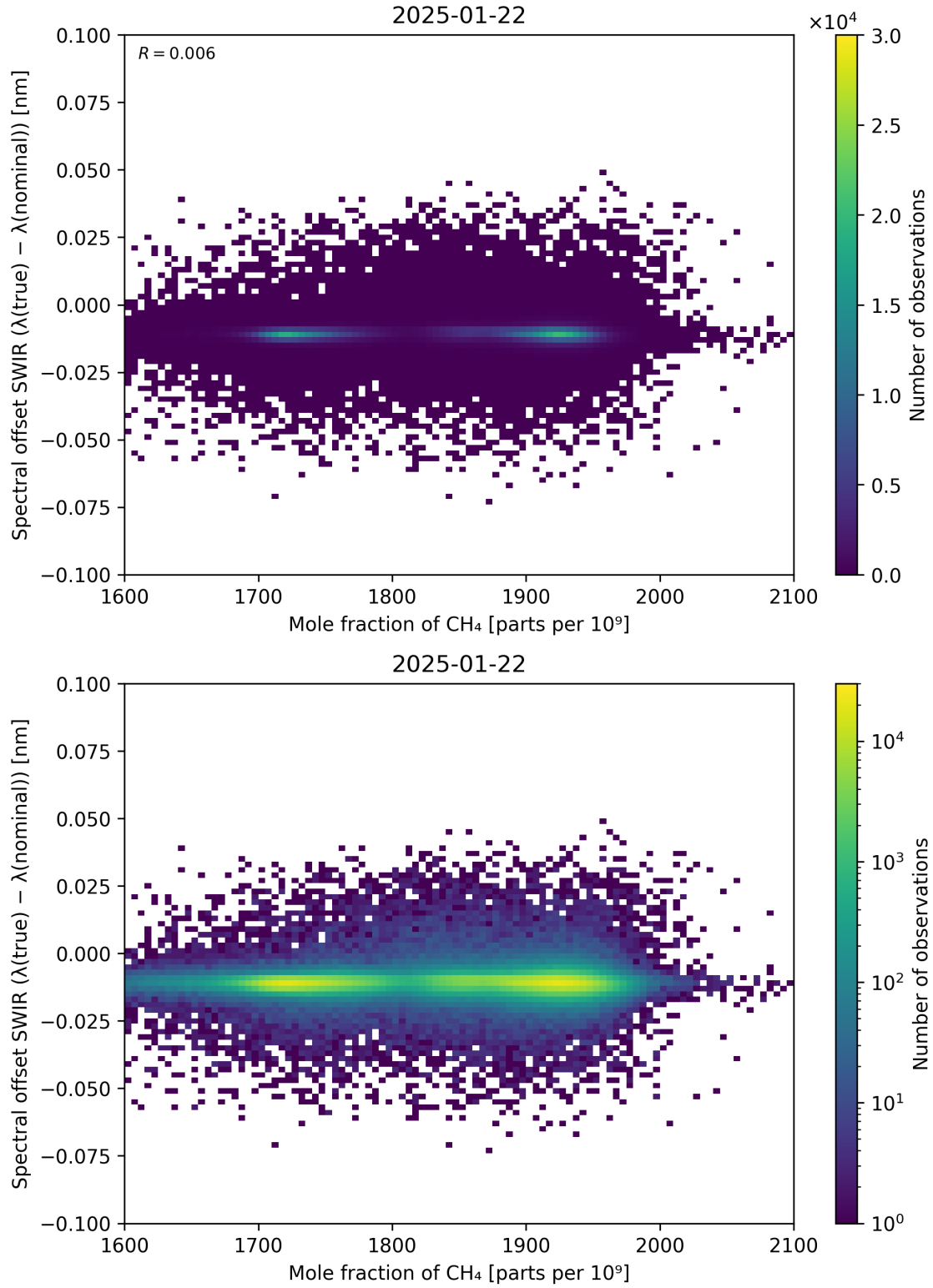
Figure 86: Scatter density plot of “Mole fraction of CH 4 ” against “Spectral offset SWIR ( \lambda_{\text{true}} - \lambda_{\text{nominal}} )” for 2025-01-21 to 2025-01-23.
