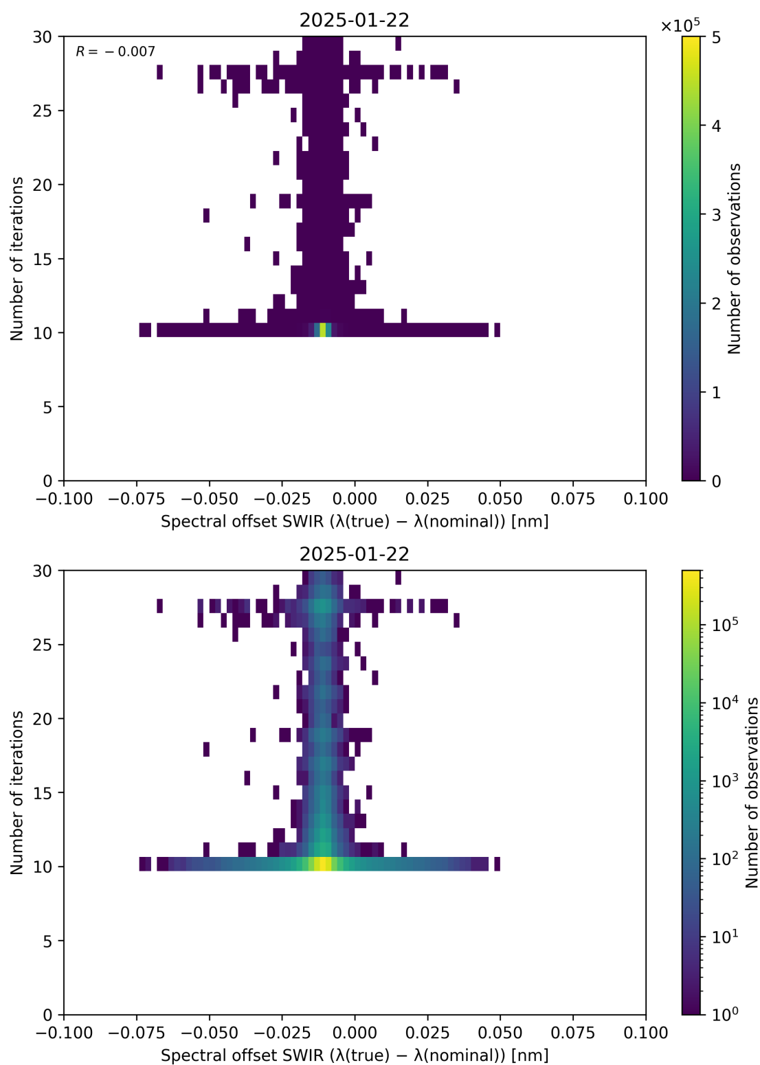
Figure 121: Scatter density plot of “Spectral offset SWIR ( \lambda_{\text{true}} - \lambda_{\text{nominal}} )” against “Number of iterations” for 2025-01-21 to 2025-01-23.
