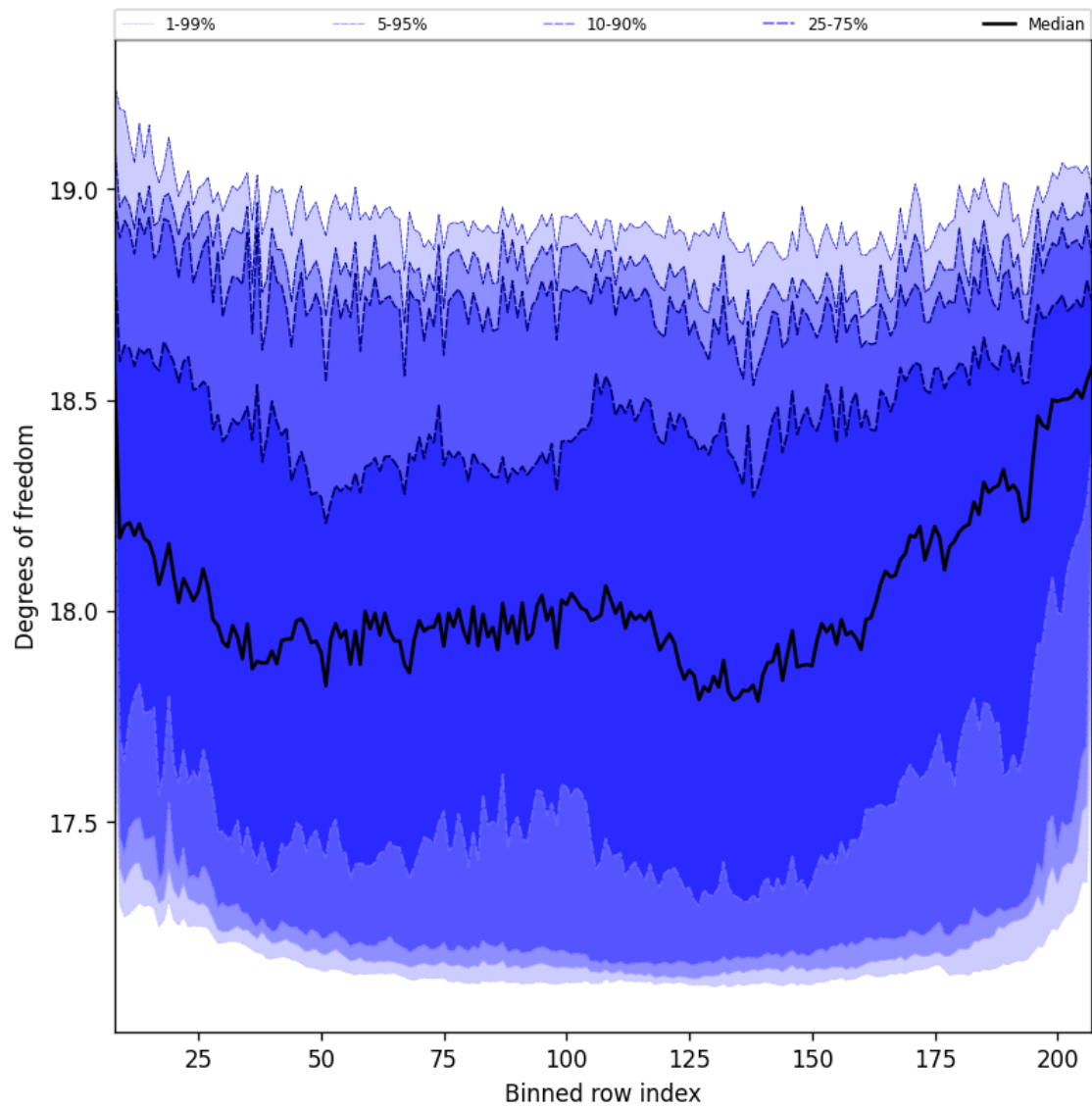
Figure 41: Along track statistics of “Degrees of freedom” for 2025-01-21 to 2025-01-23
