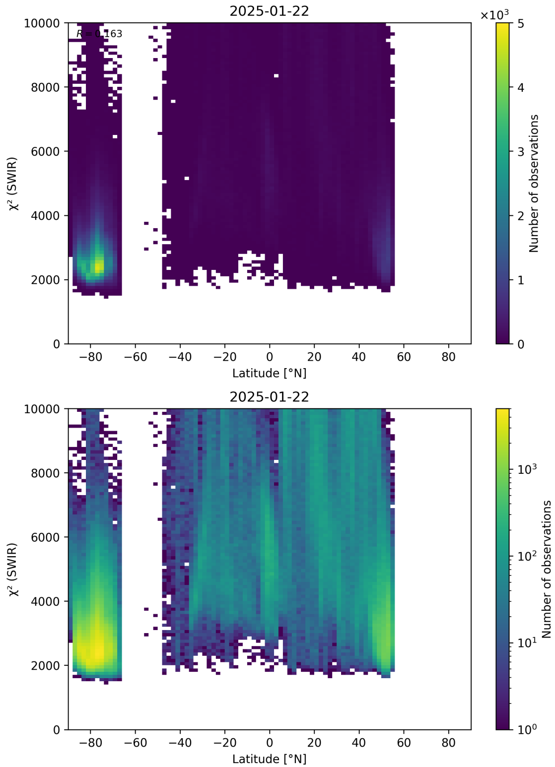
Figure 54: Scatter density plot of “Latitude” against “ \chi^2 (SWIR)” for 2025-01-21 to 2025-01-23.
