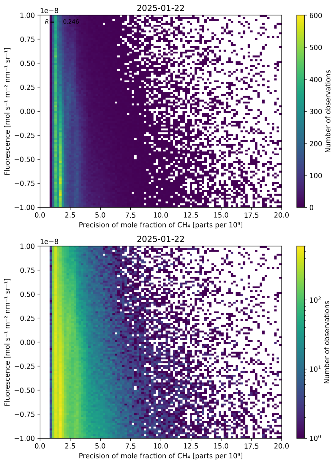
Figure 81: Scatter density plot of “Precision of mole fraction of CH 4 ” against “Fluorescence” for 2025-01-21 to 2025-01-23.
