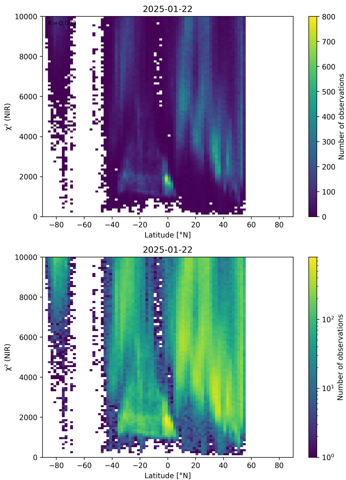
Figure 53: Scatter density plot of “Latitude” against “ \chi^2 (NIR)” for 2025-01-21 to 2025-01-23.
