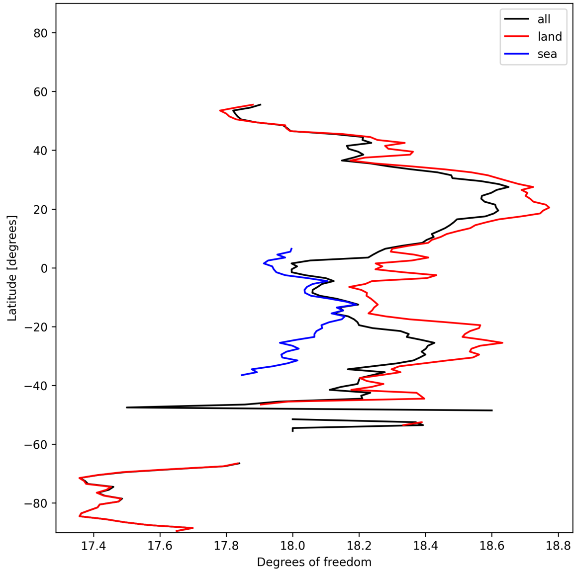
Figure 19: Zonal average of “Degrees of freedom” for 2025-01-21 to 2025-01-23.
