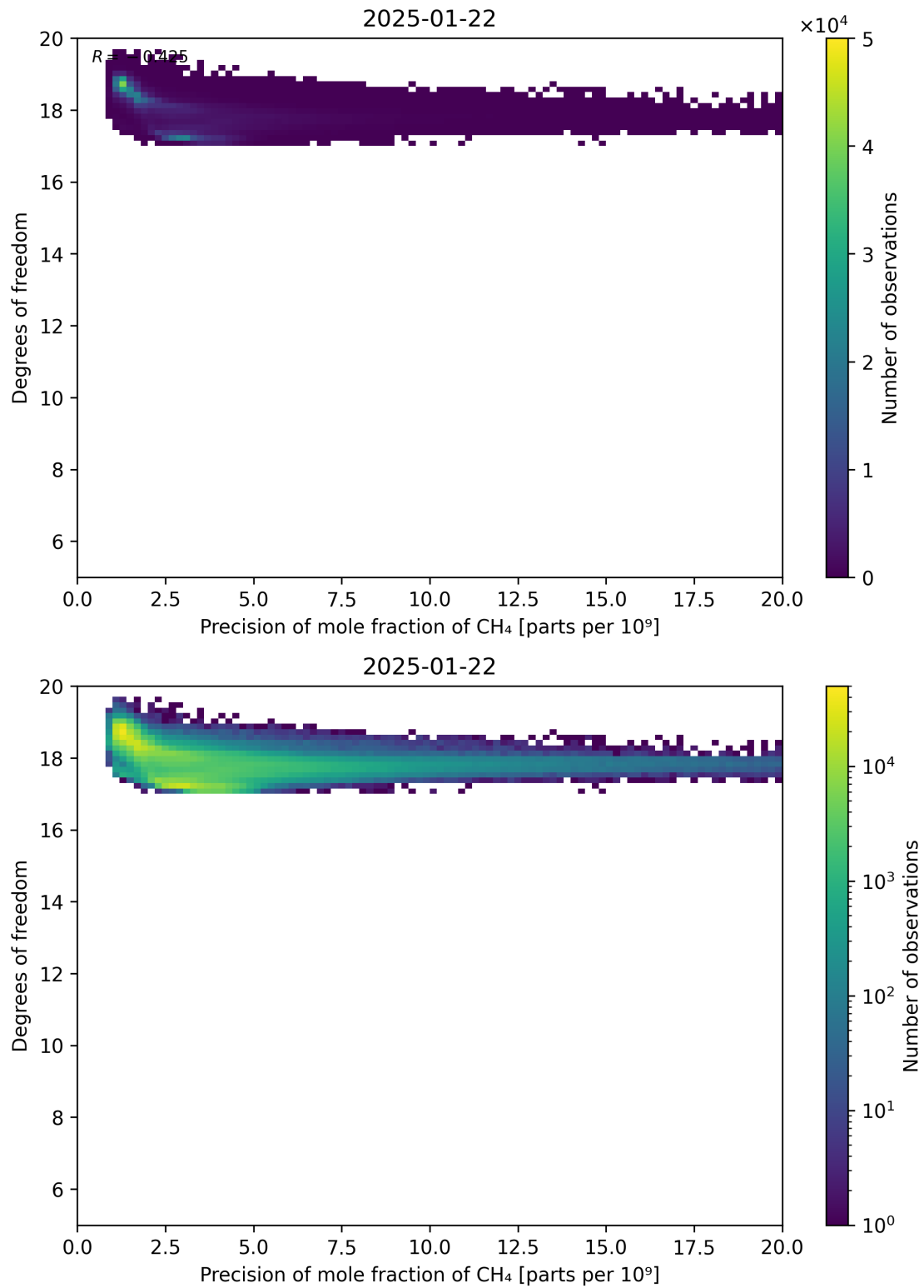
Figure 80: Scatter density plot of “Precision of mole fraction of CH 4 ” against “Degrees of freedom” for 2025-01-21 to 2025-01-23.
