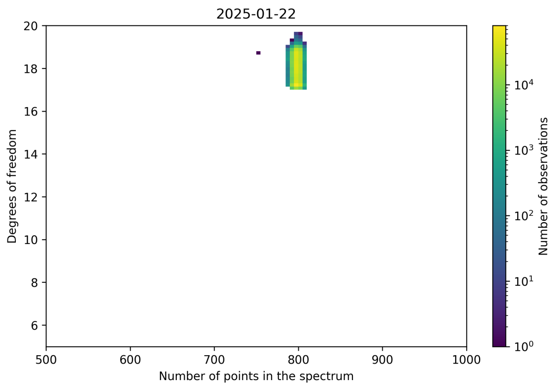
Figure 90: Scatter density plot of “Number of points in the spectrum” against “Degrees of freedom” for 2025-01-21 to 2025-01-23.
