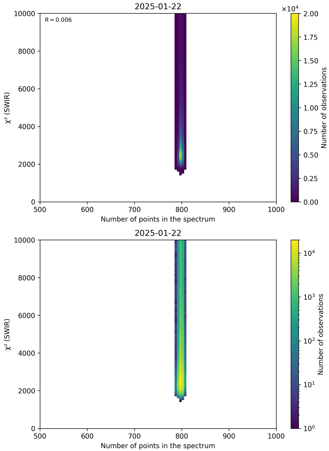
Figure 89: Scatter density plot of “Number of points in the spectrum” against “ \chi^2 (SWIR)” for 2025-01-21 to 2025-01-23.
