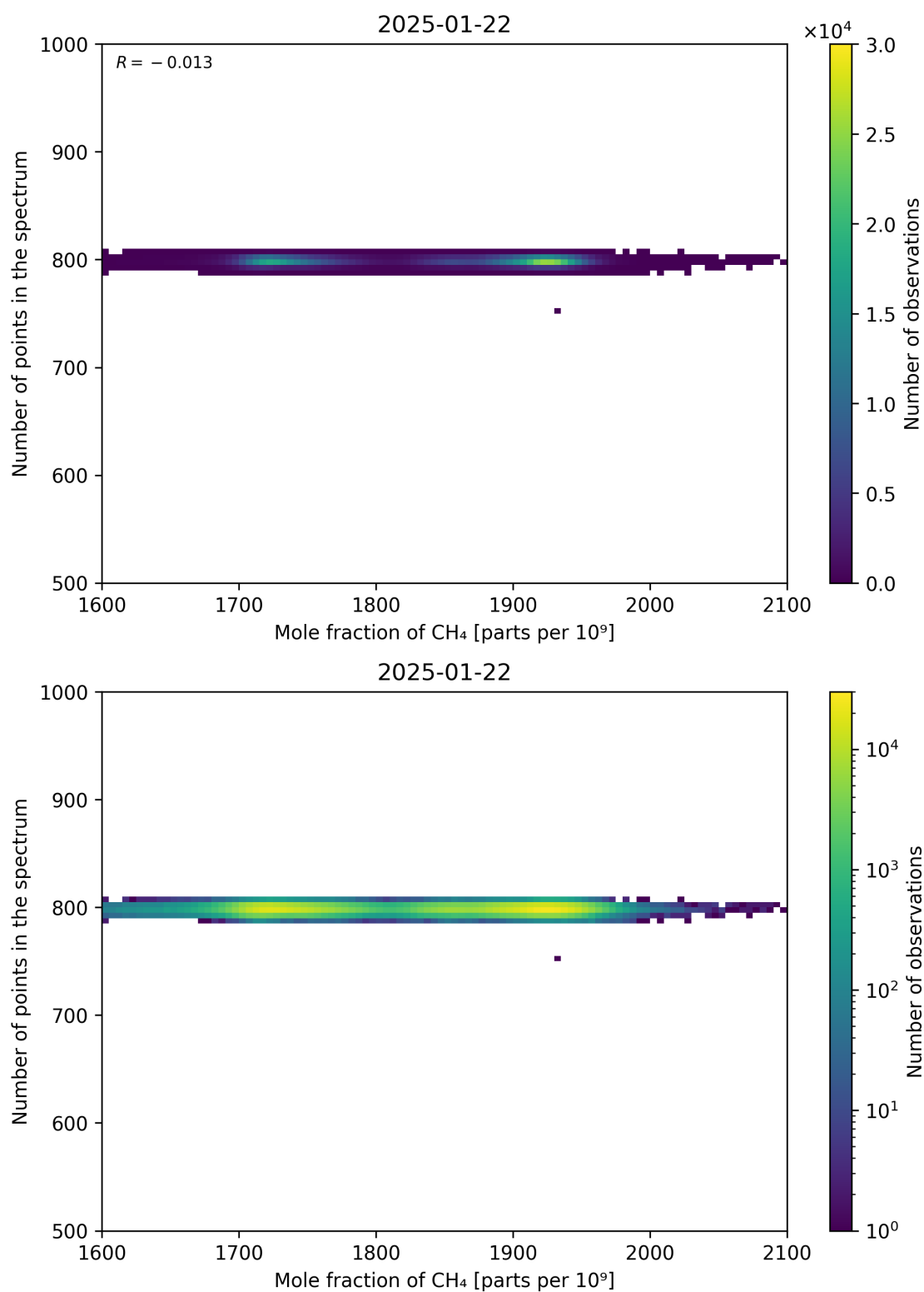
Figure 77: Scatter density plot of “Mole fraction of CH 4 ” against “Number of points in the spectrum” for 2025-01-21 to 2025-01-23.
