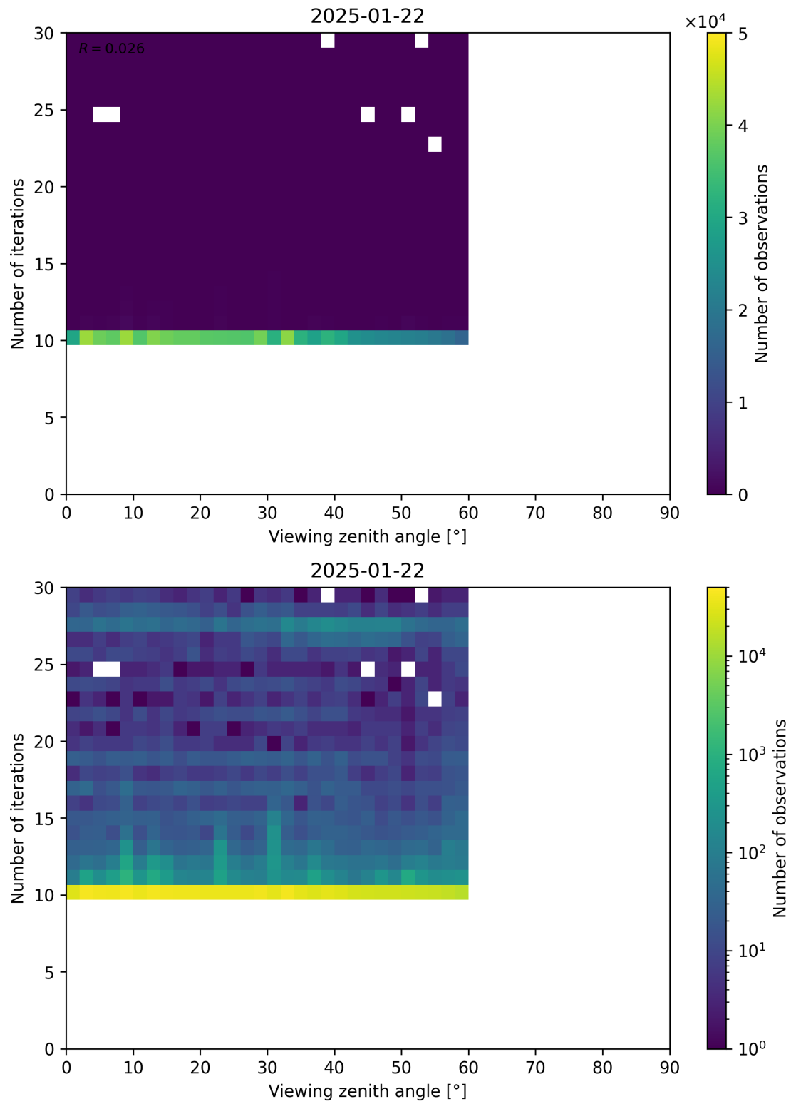
Figure 113: Scatter density plot of “Viewing zenith angle” against “Number of iterations” for 2025-01-21 to 2025-01-23.
