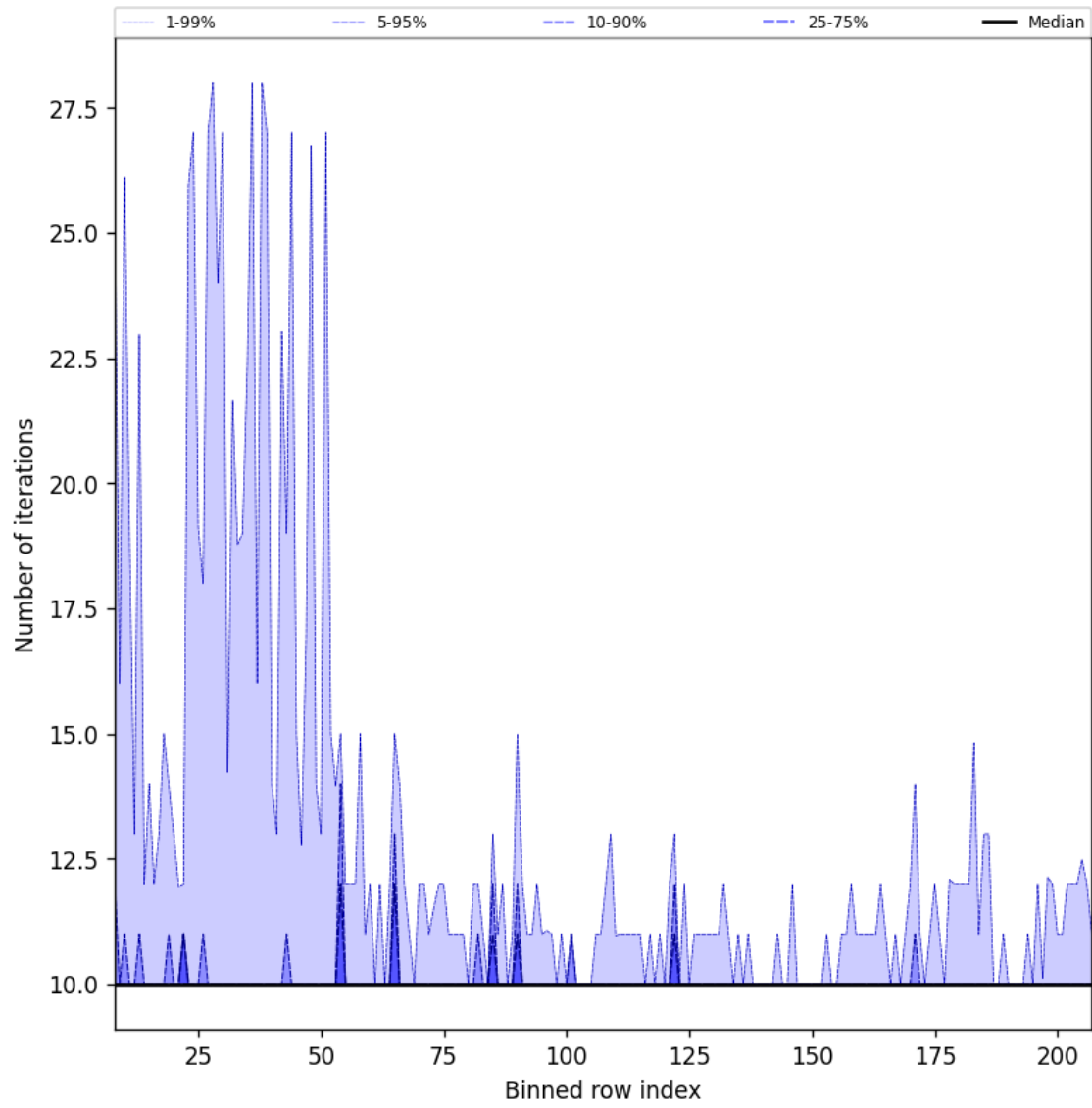
Figure 42: Along track statistics of “Number of iterations” for 2025-01-21 to 2025-01-23
