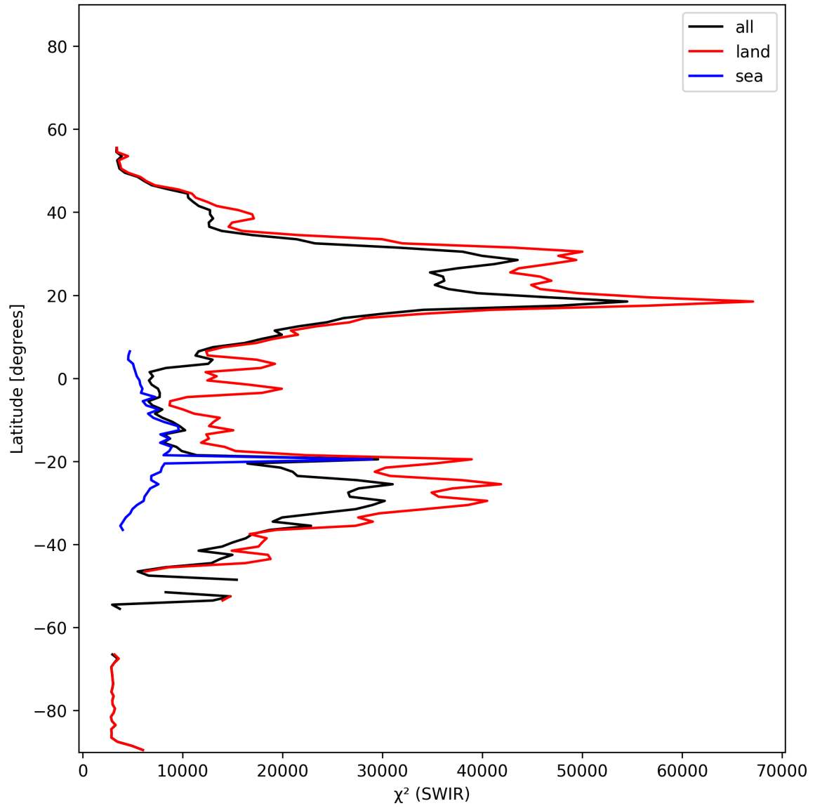
Figure 17: Zonal average of “ \chi^2 (SWIR)” for 2025-01-21 to 2025-01-23.
