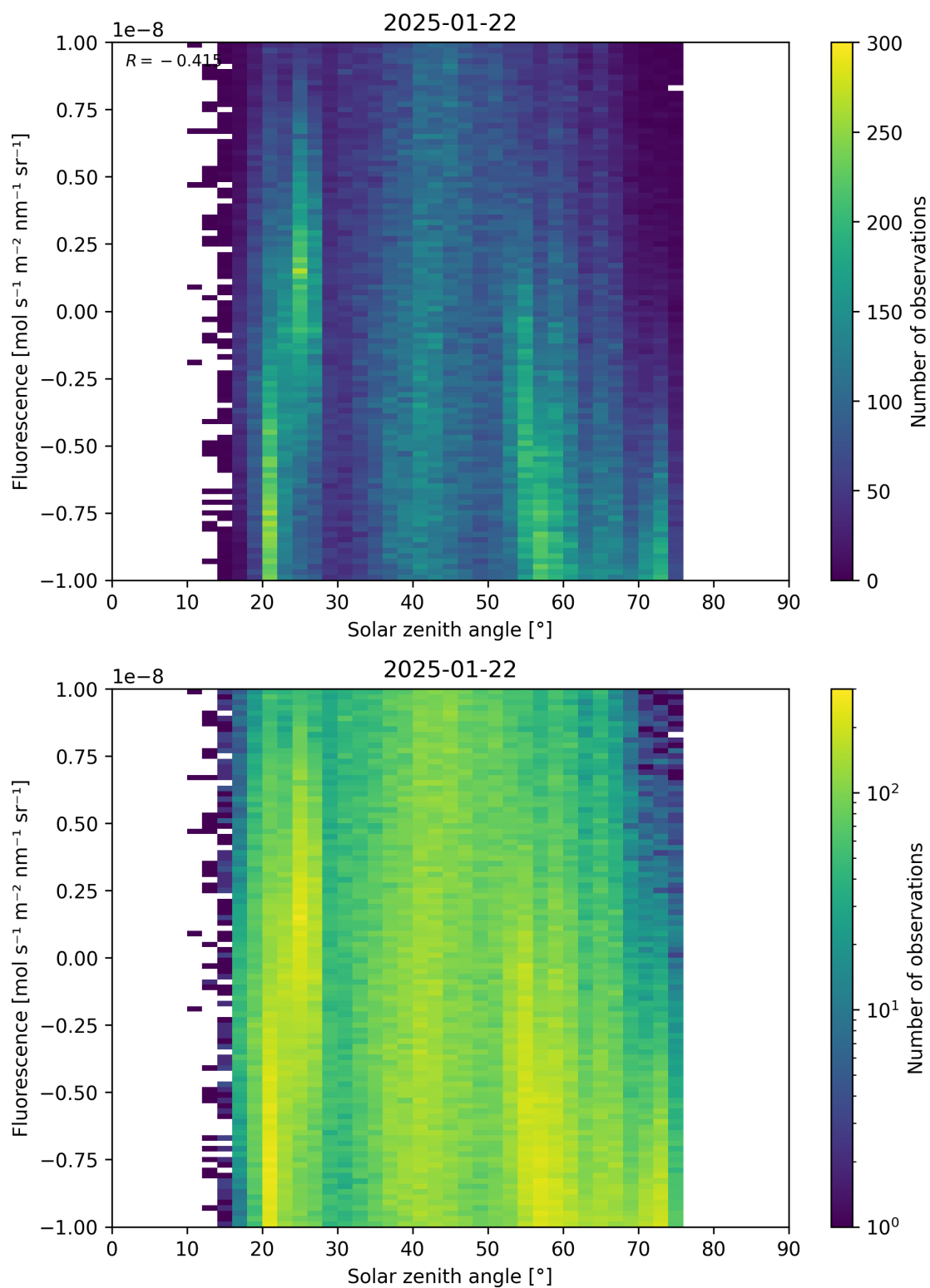
Figure 97: Scatter density plot of “Solar zenith angle” against “Fluorescence” for 2025-01-21 to 2025-01-23.
