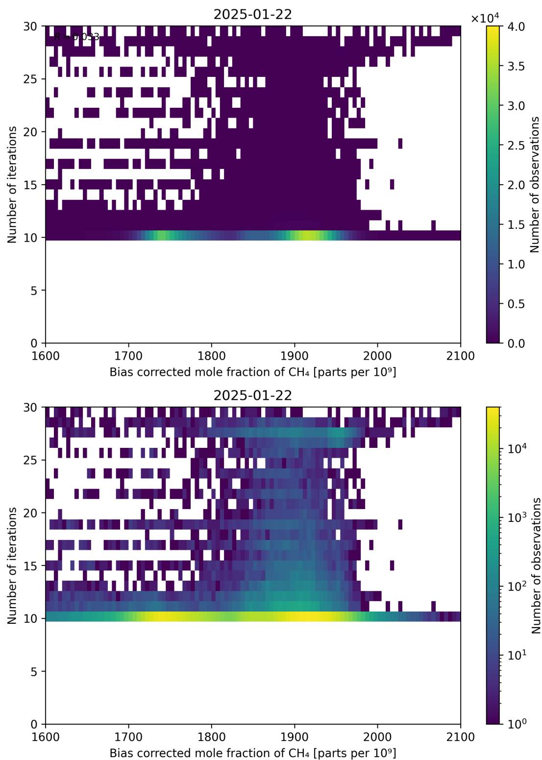
Figure 67: Scatter density plot of “Bias corrected mole fraction of \text{CH}_4 ” against “Number of iterations” for 2025-01-21 to 2025-01-23.
