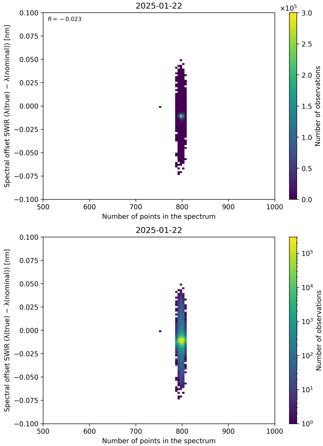
Figure 93: Scatter density plot of “Number of points in the spectrum” against “Spectral offset SWIR ( \lambda_{\text{true}} - \lambda_{\text{nominal}} )” for 2025-01-21 to 2025-01-23.
