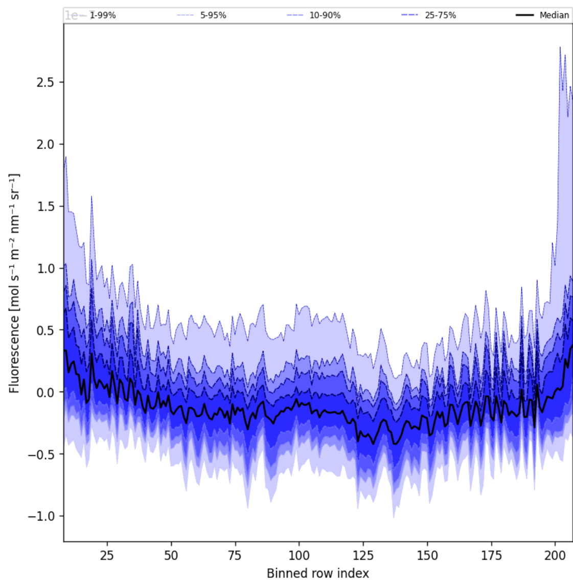
Figure 43: Along track statistics of “Fluorescence” for 2025-01-21 to 2025-01-23
