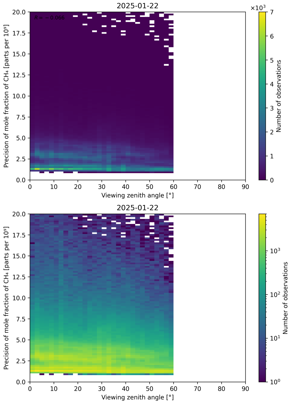
Figure 112: Scatter density plot of “Viewing zenith angle” against “Precision of mole fraction of CH 4 ” for 2025-01-21 to 2025-01-23.
