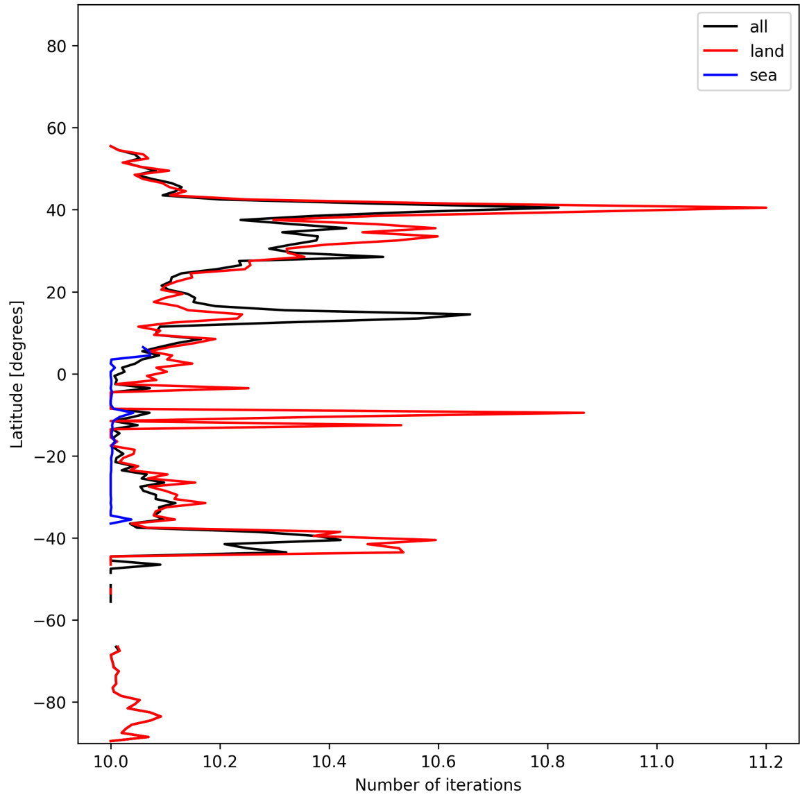
Figure 20: Zonal average of “Number of iterations” for 2025-01-21 to 2025-01-23.
