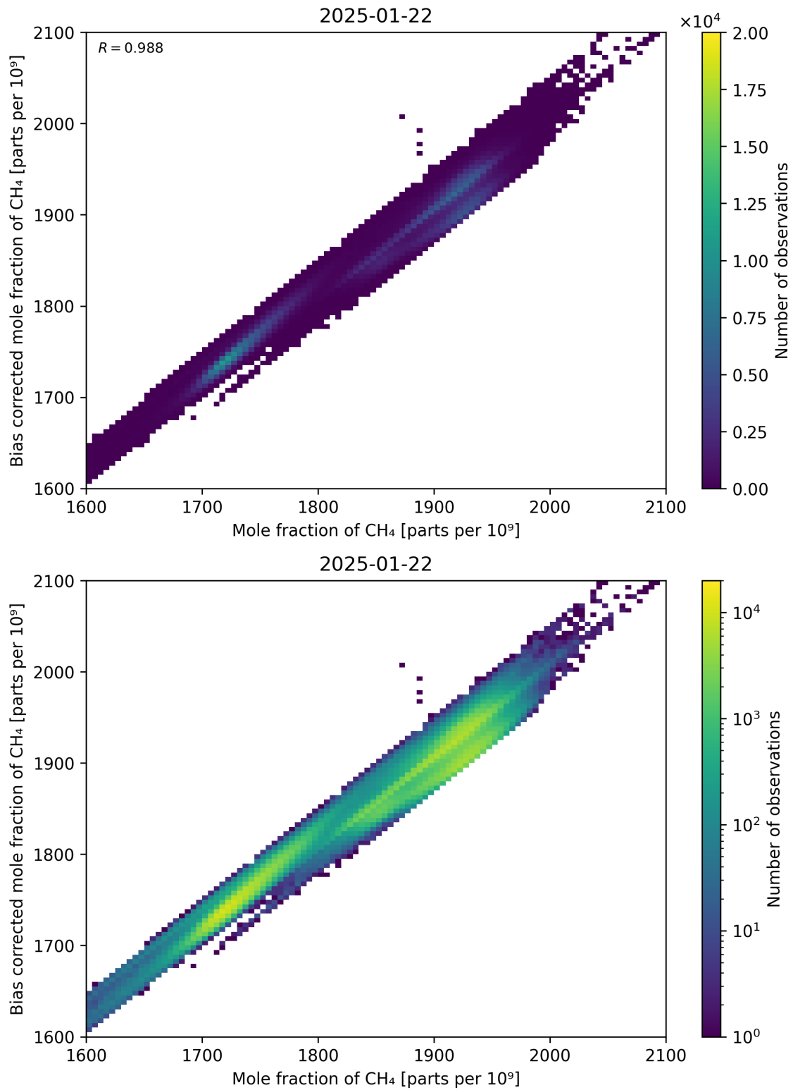
Figure 74: Scatter density plot of “Mole fraction of CH 4 ” against “Bias corrected mole fraction of CH 4 ” for 2025-01-21 to 2025-01-23.
