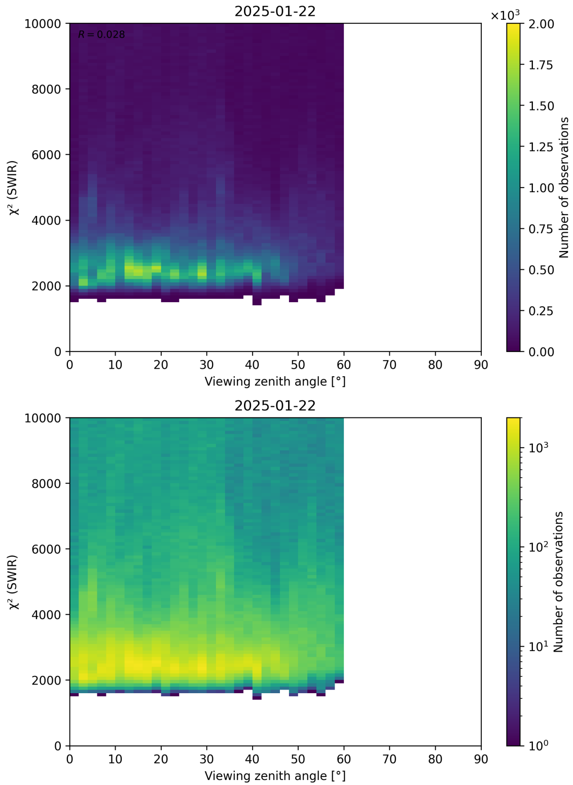
Figure 106: Scatter density plot of “Viewing zenith angle” against “ \chi^2 (SWIR)” for 2025-01-21 to 2025-01-23.
