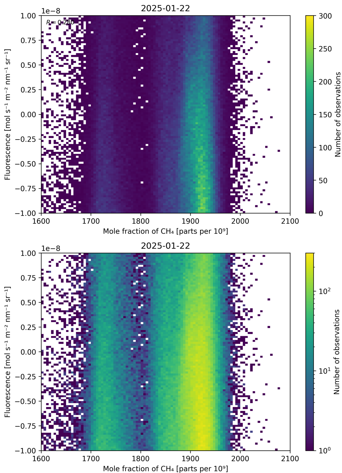
Figure 73: Scatter density plot of “Mole fraction of \text{CH}_4 ” against “Fluorescence” for 2025-01-21 to 2025-01-23.
