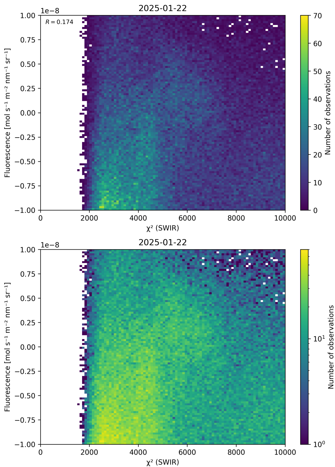
Figure 49: Scatter density plot of “ \chi^2 (SWIR)” against “Fluorescence” for 2025-01-21 to 2025-01-23.
