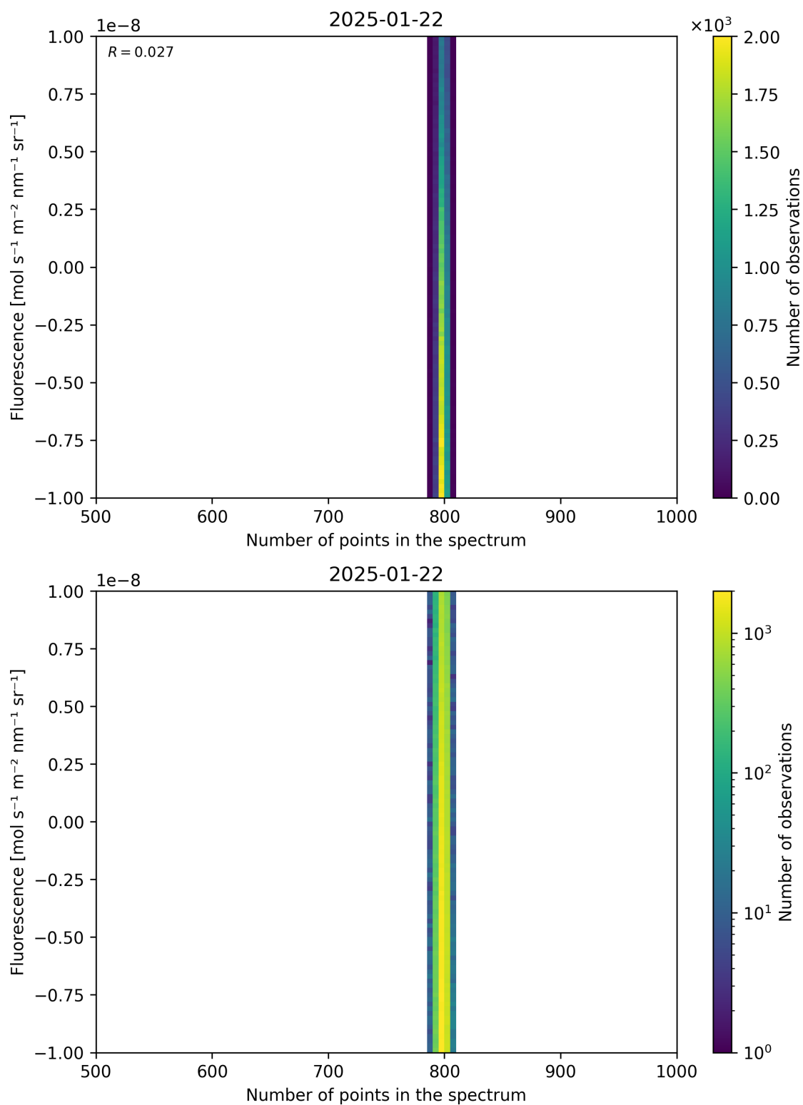
Figure 91: Scatter density plot of “Number of points in the spectrum” against “Fluorescence” for 2025-01-21 to 2025-01-23.
