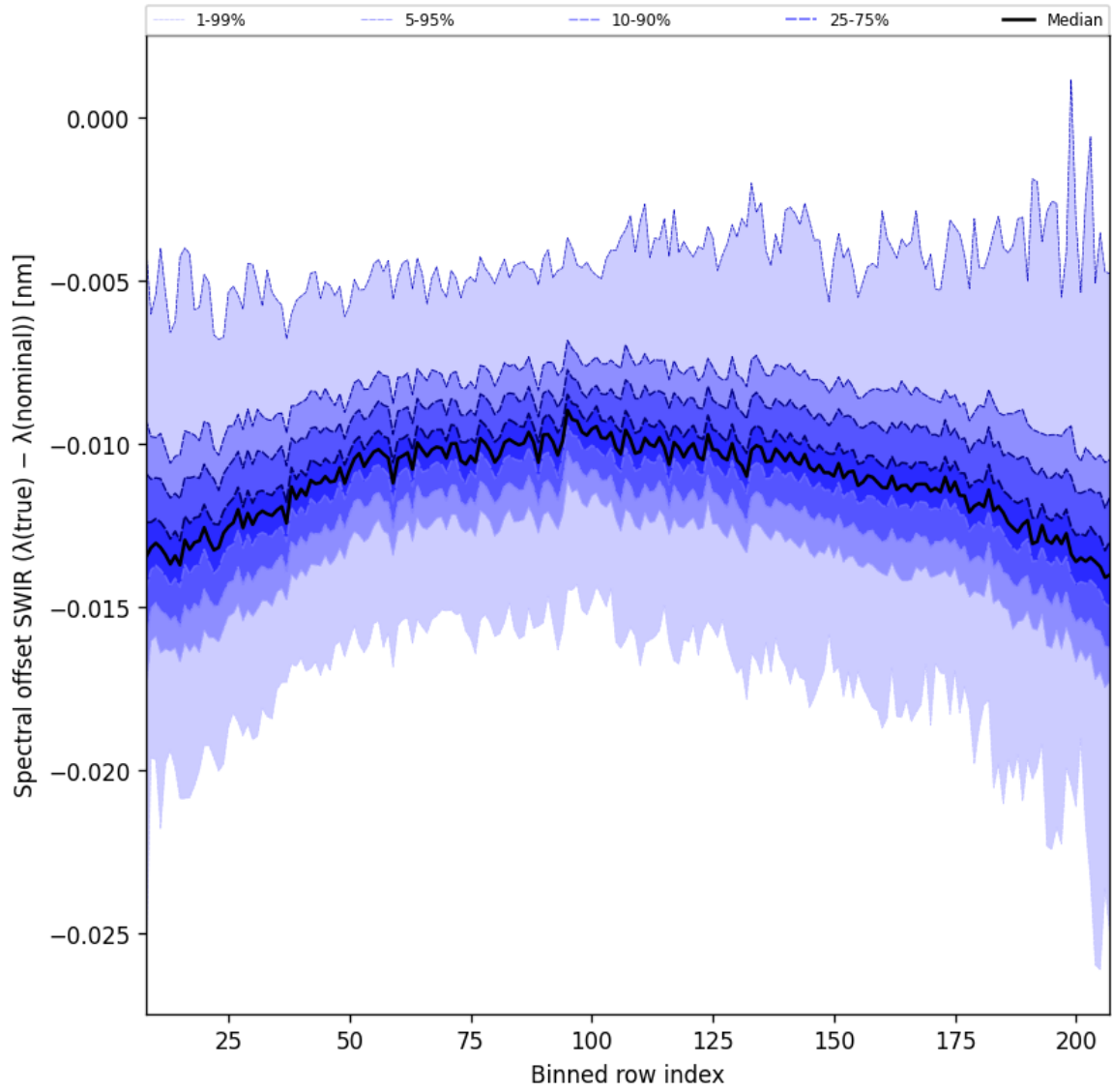
Figure 38: Along track statistics of “Spectral offset SWIR ( \lambda_{\text{true}} - \lambda_{\text{nominal}} )” for 2025-01-21 to 2025-01-23
