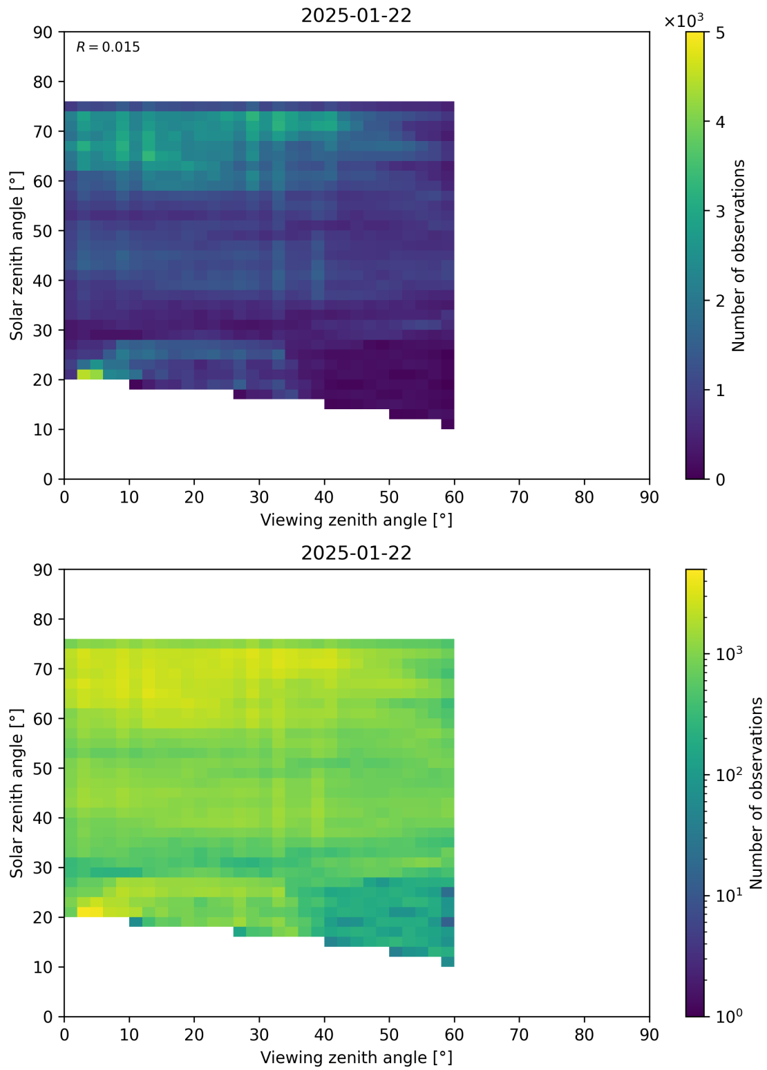
Figure 115: Scatter density plot of “Viewing zenith angle” against “Solar zenith angle” for 2025-01-21 to 2025-01-23.
