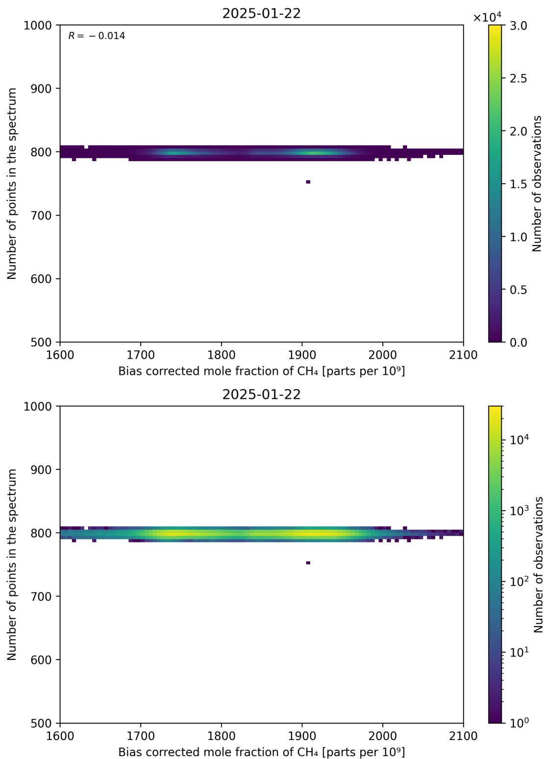
Figure 68: Scatter density plot of “Bias corrected mole fraction of CH 4 ” against “Number of points in the spectrum” for 2025-01-21 to 2025-01-23.
