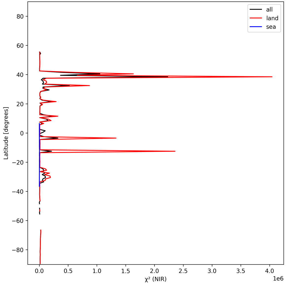
Figure 18: Zonal average of “ \chi^2 (NIR)” for 2025-01-21 to 2025-01-23.
