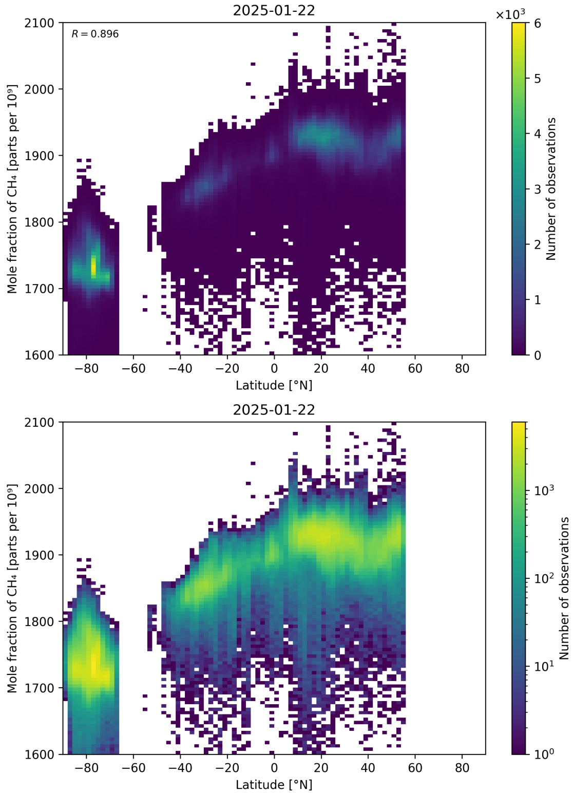
Figure 57: Scatter density plot of “Latitude” against “Mole fraction of CH 4 ” for 2025-01-21 to 2025-01-23.
