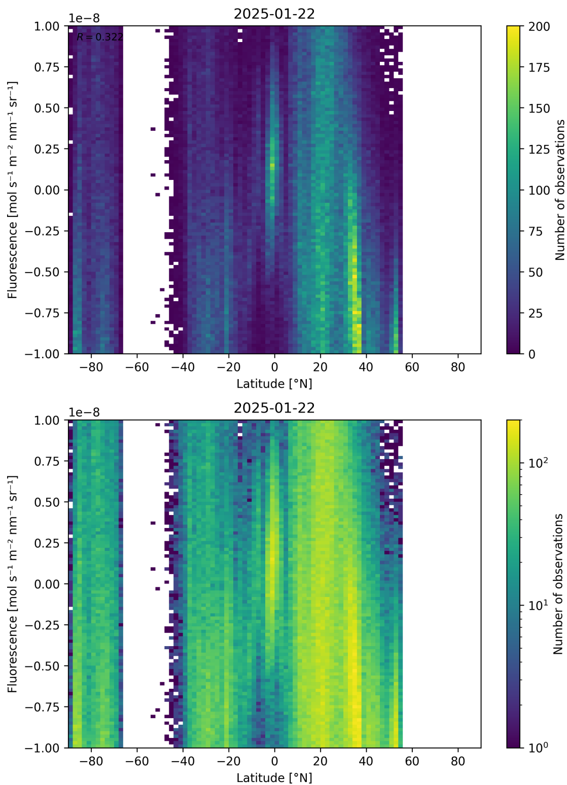
Figure 56: Scatter density plot of “Latitude” against “Fluorescence” for 2025-01-21 to 2025-01-23.
