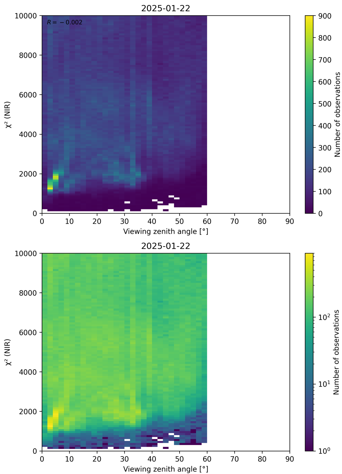
Figure 105: Scatter density plot of “Viewing zenith angle” against “ \chi^2 (NIR)” for 2025-01-21 to 2025-01-23.
