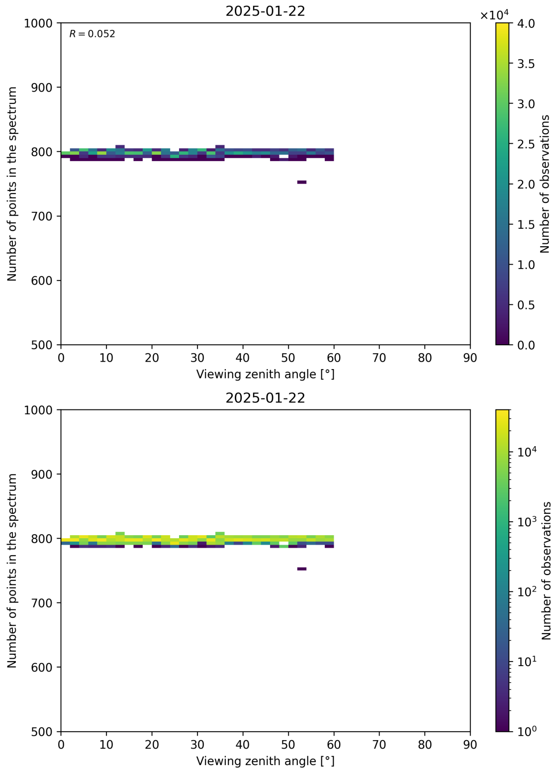
Figure 114: Scatter density plot of “Viewing zenith angle” against “Number of points in the spectrum” for 2025-01-21 to 2025-01-23.
