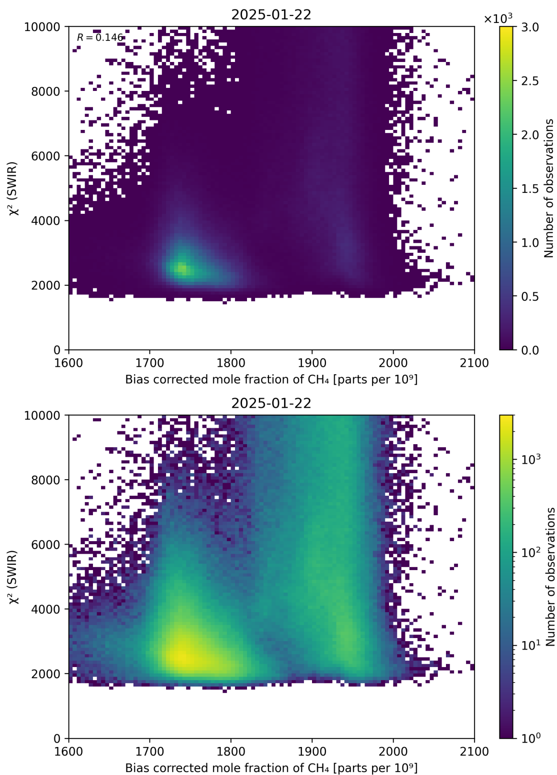
Figure 64: Scatter density plot of “Bias corrected mole fraction of \text{CH}_4 ” against “ \chi^2 (SWIR)” for 2025-01-21 to 2025-01-23.
