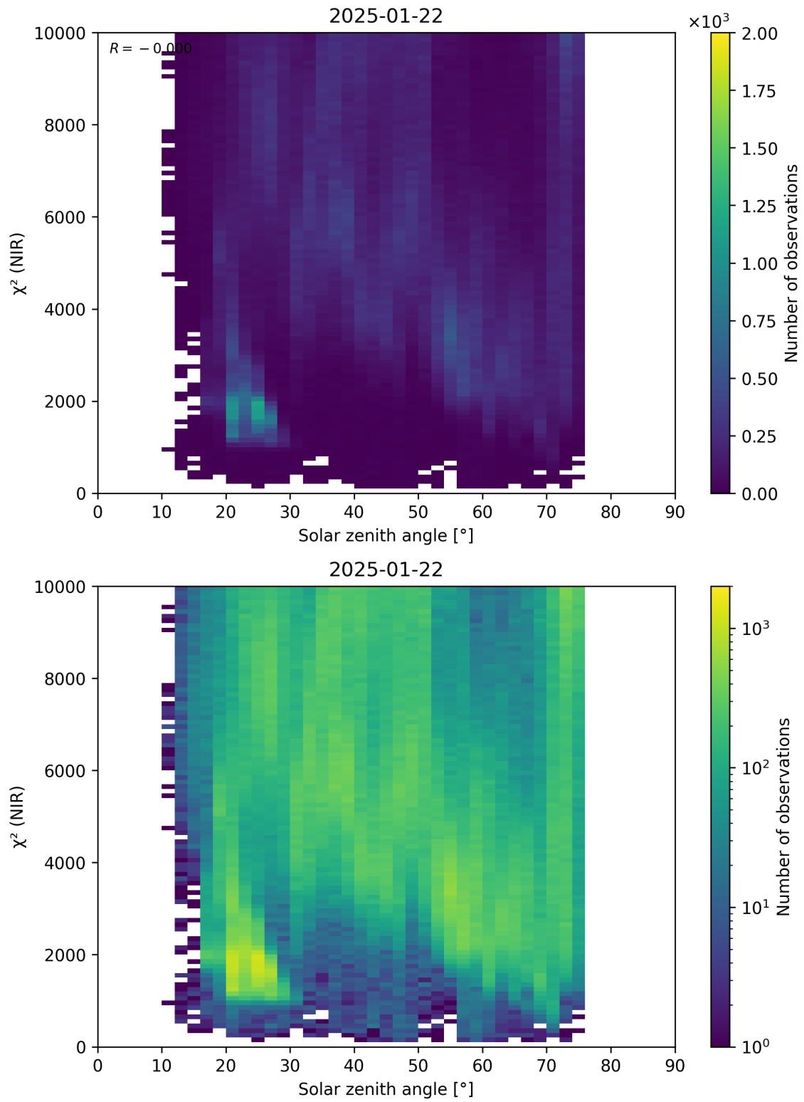
Figure 94: Scatter density plot of “Solar zenith angle” against “ \chi^2 (NIR)” for 2025-01-21 to 2025-01-23.
