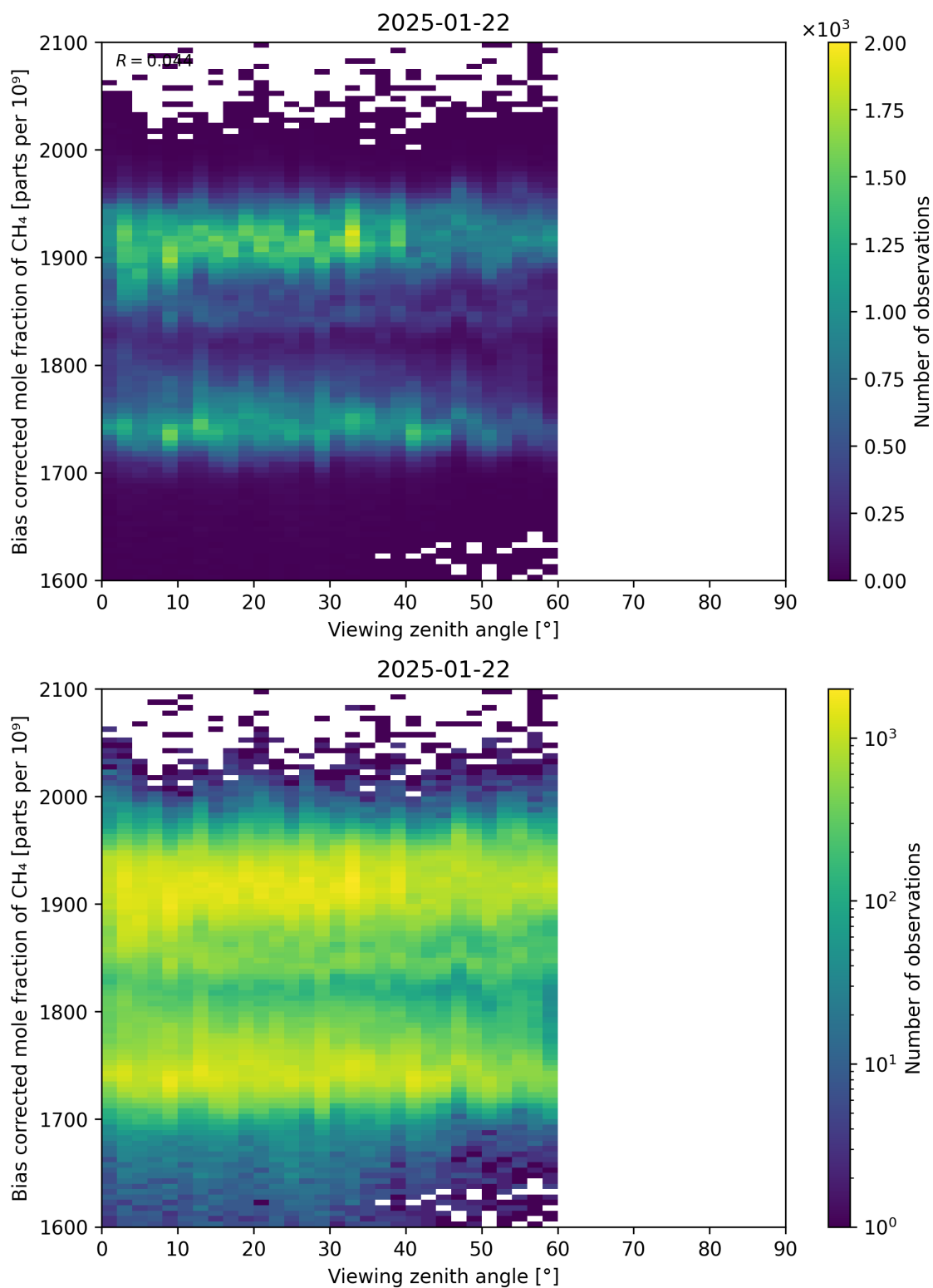
Figure 111: Scatter density plot of “Viewing zenith angle” against “Bias corrected mole fraction of CH 4 ” for 2025-01-21 to 2025-01-23.
