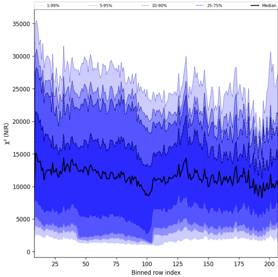
Figure 40: Along track statistics of “ \chi^2 (NIR)” for 2025-01-21 to 2025-01-23
