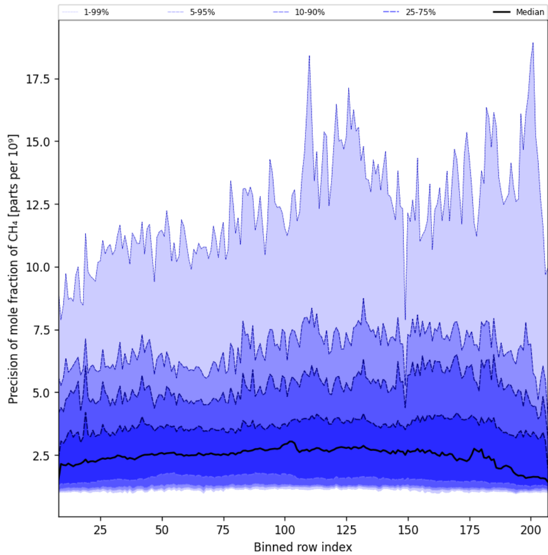
Figure 35: Along track statistics of “Precision of mole fraction of CH 4 ” for 2025-01-21 to 2025-01-23
