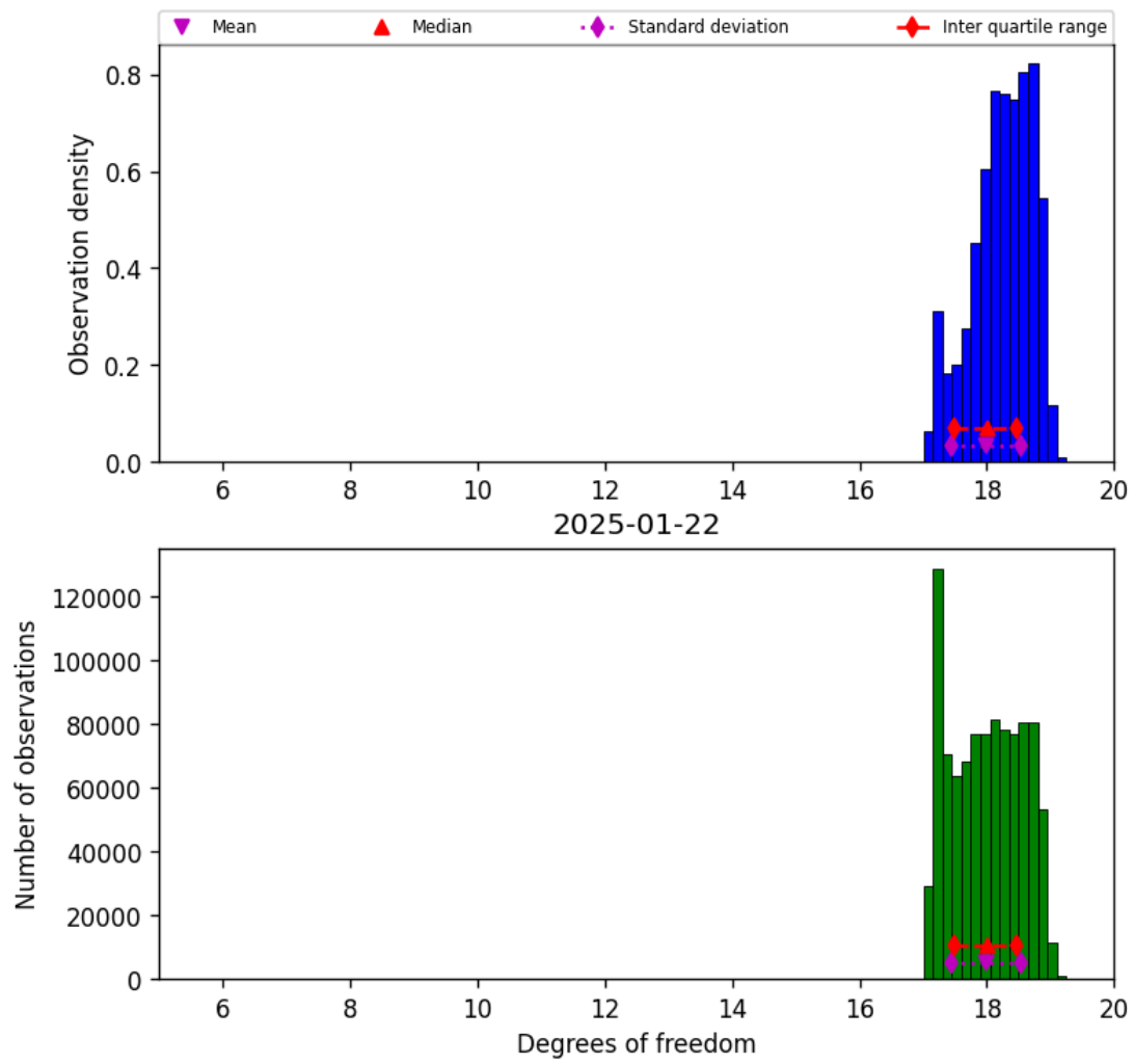
Figure 30: Histogram of “Degrees of freedom” for 2025-01-21 to 2025-01-23
