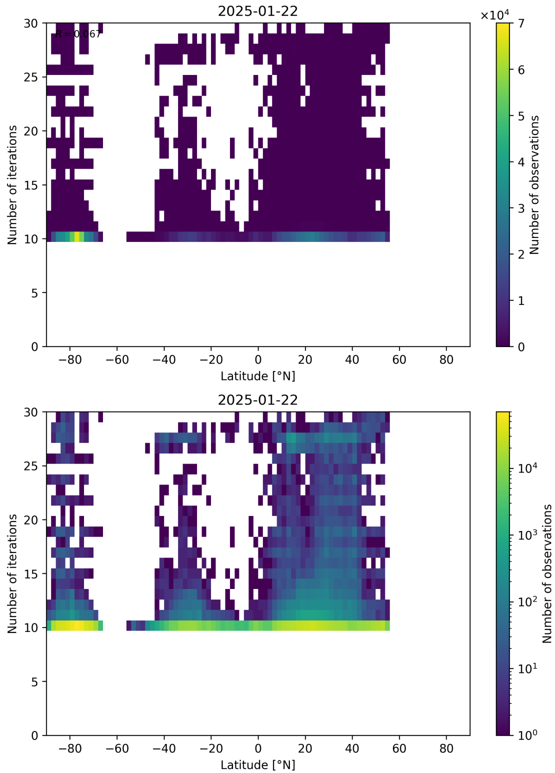
Figure 60: Scatter density plot of “Latitude” against “Number of iterations” for 2025-01-21 to 2025-01-23.
