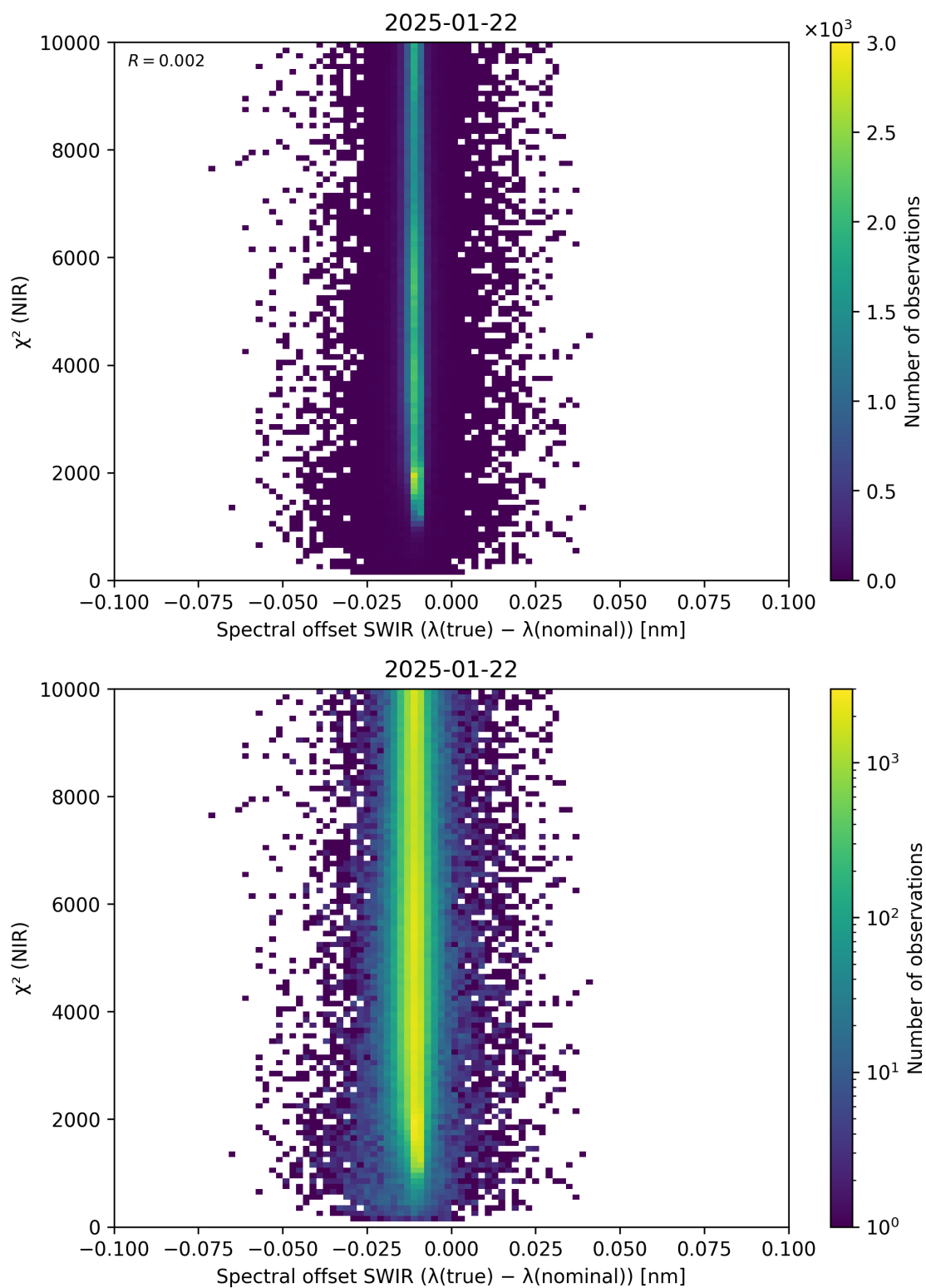
Figure 117: Scatter density plot of “Spectral offset SWIR ( \lambda_{\text{true}} - \lambda_{\text{nominal}} )” against “ \chi^2 (NIR)” for 2025-01-21 to 2025-01-23.
