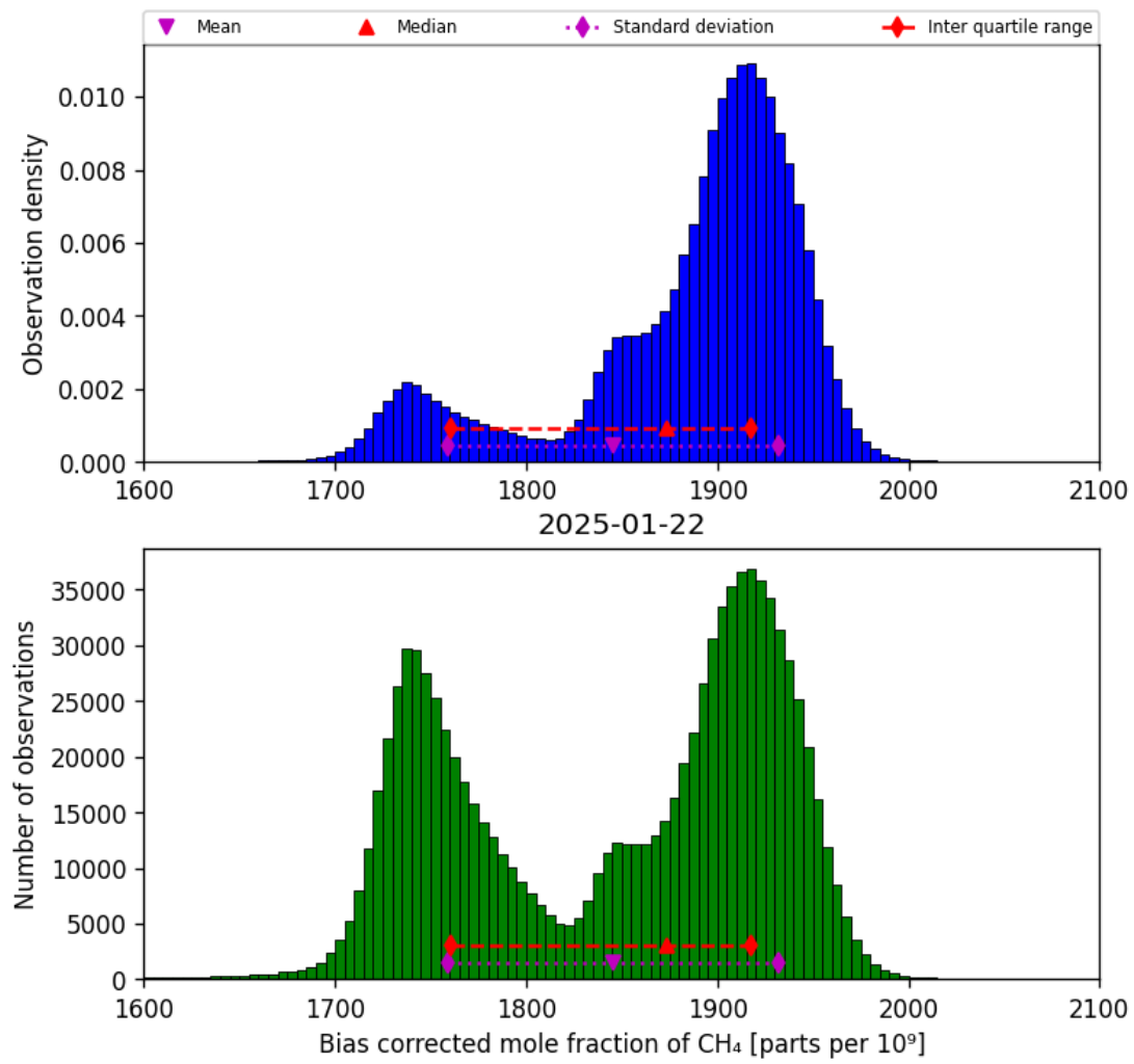
Figure 25: Histogram of “Bias corrected mole fraction of CH 4 ” for 2025-01-21 to 2025-01-23
