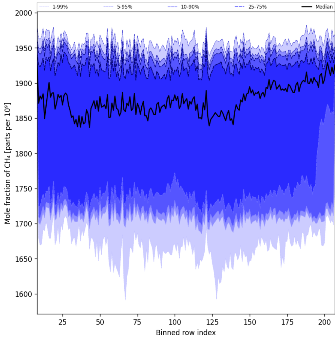
Figure 34: Along track statistics of “Mole fraction of CH 4 ” for 2025-01-21 to 2025-01-23
