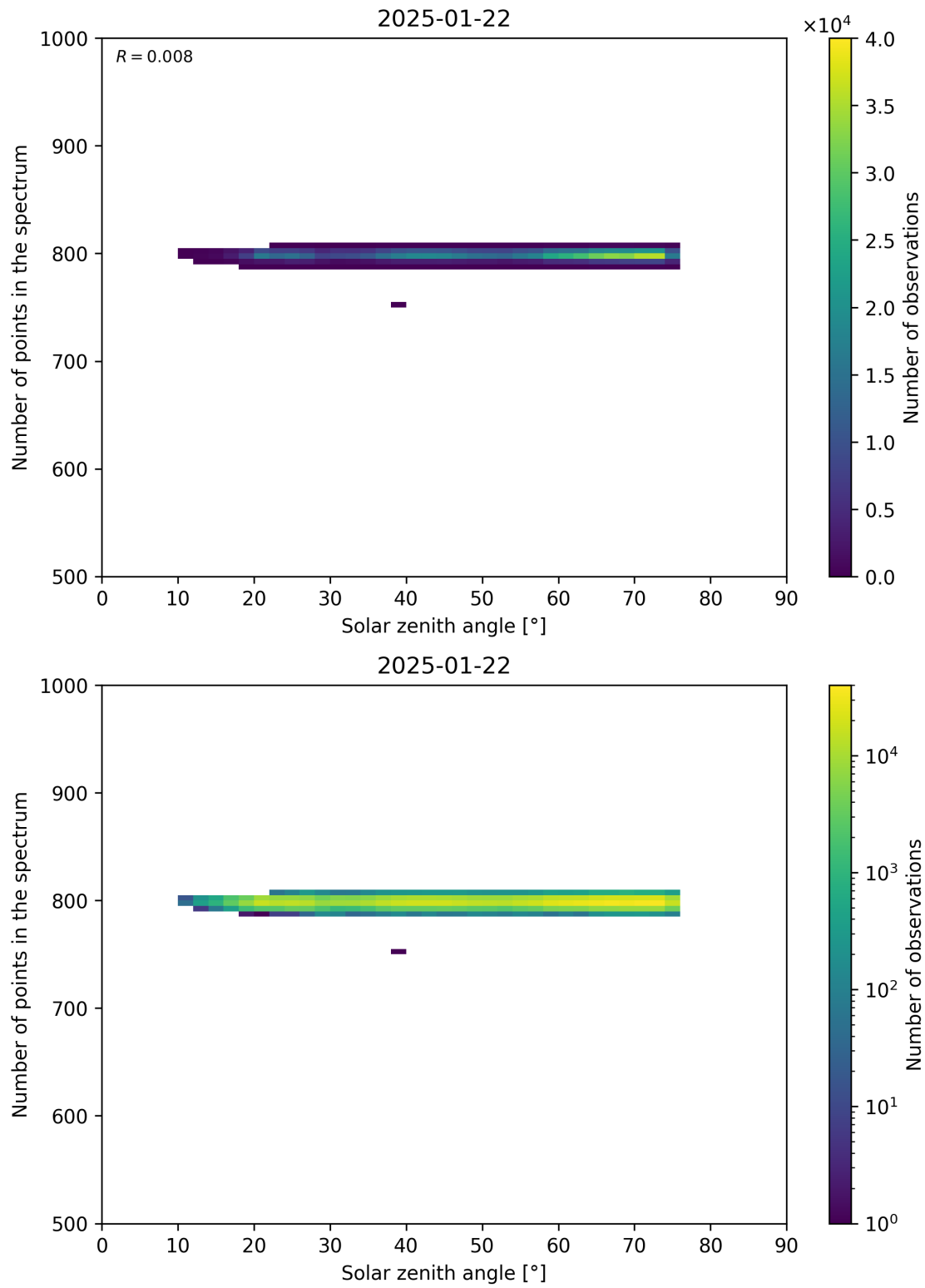
Figure 103: Scatter density plot of “Solar zenith angle” against “Number of points in the spectrum” for 2025-01-21 to 2025-01-23.
