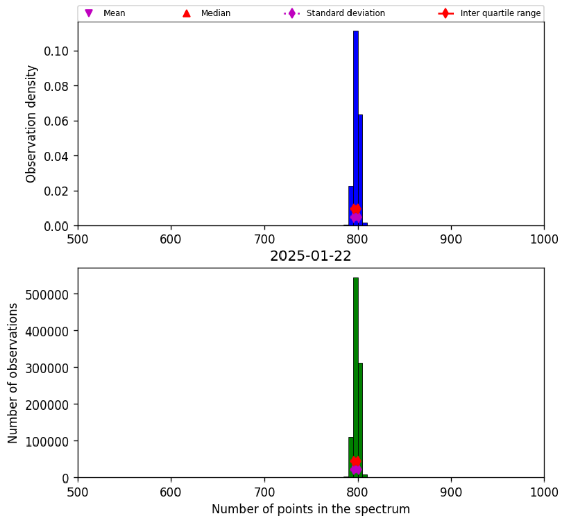
Figure 26: Histogram of “Number of points in the spectrum” for 2025-01-21 to 2025-01-23
