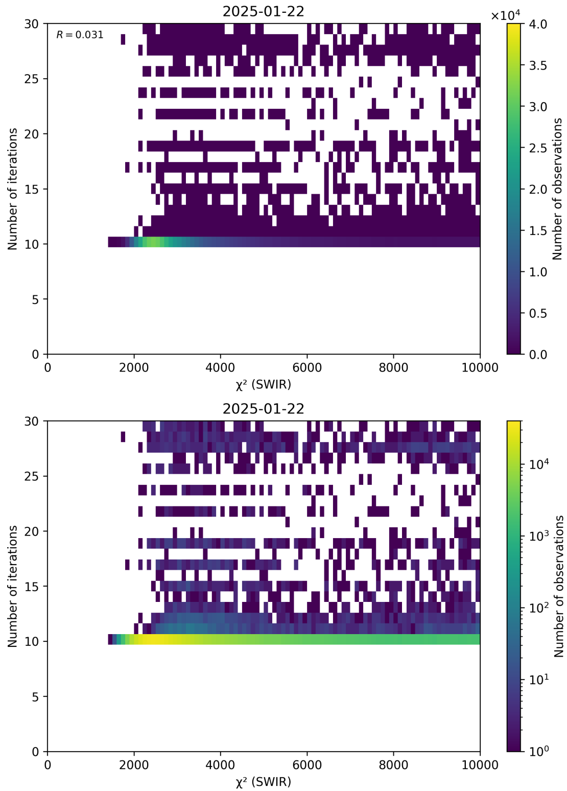
Figure 50: Scatter density plot of “ \chi^2 (SWIR)” against “Number of iterations” for 2025-01-21 to 2025-01-23.
