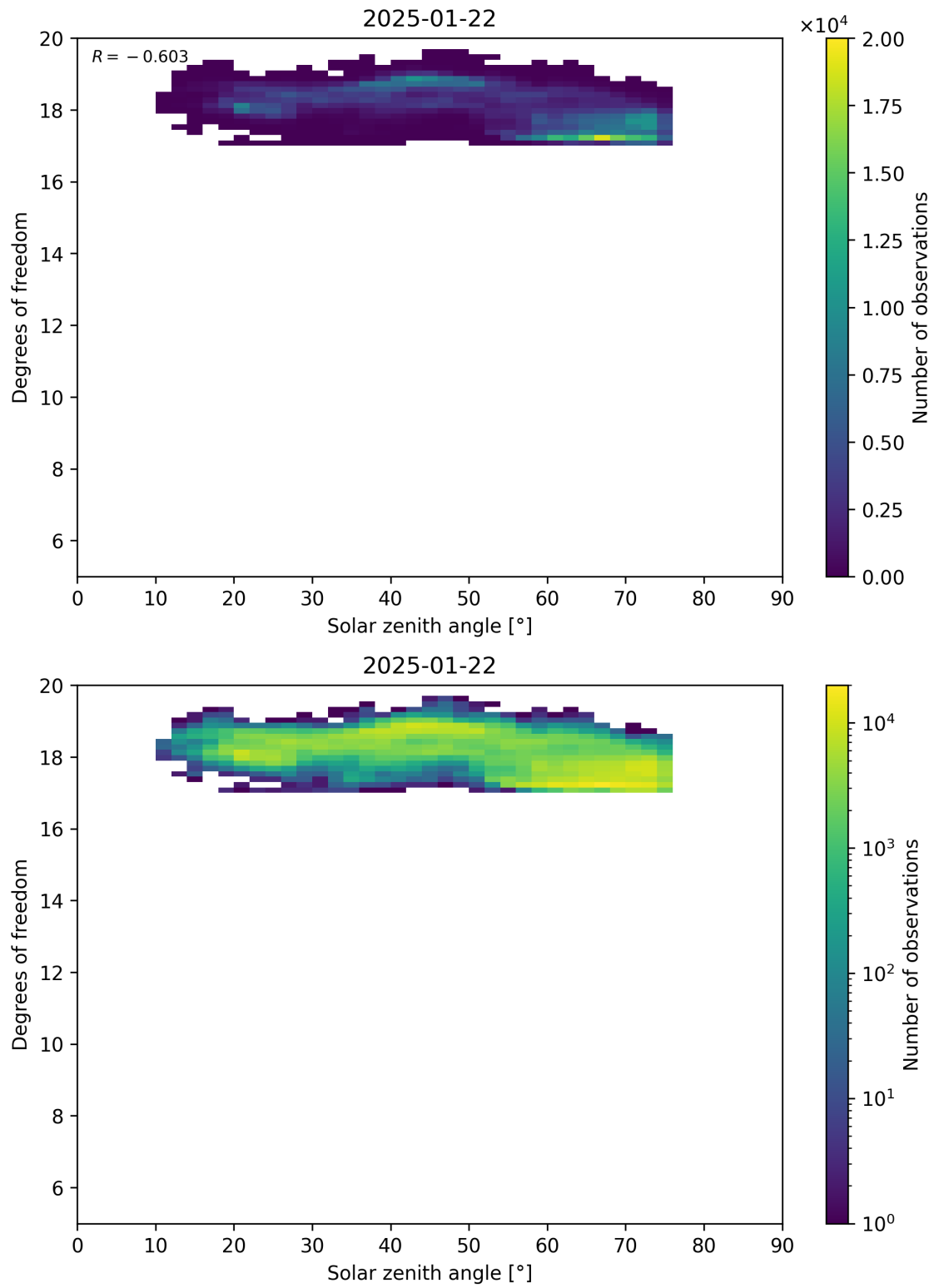
Figure 96: Scatter density plot of “Solar zenith angle” against “Degrees of freedom” for 2025-01-21 to 2025-01-23.
