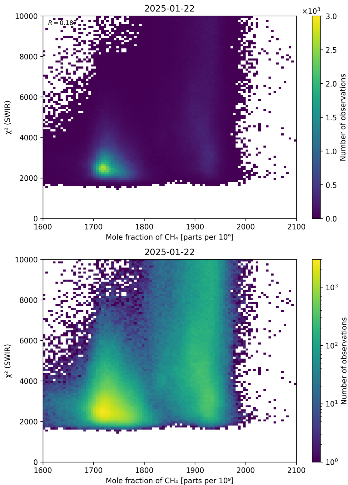
Figure 71: Scatter density plot of “Mole fraction of \text{CH}_4 ” against “ \chi^2 (SWIR)” for 2025-01-21 to 2025-01-23.
