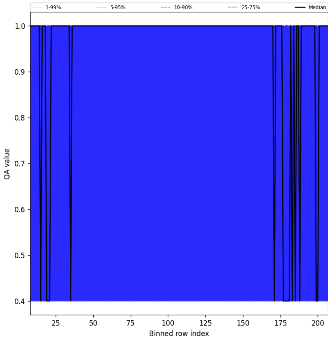
Figure 33: Along track statistics of “QA value” for 2025-01-21 to 2025-01-23
