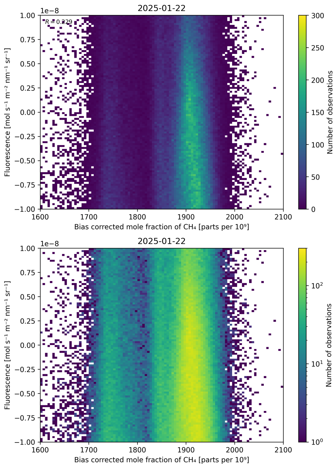
Figure 66: Scatter density plot of “Bias corrected mole fraction of \text{CH}_4 ” against “Fluorescence” for 2025-01-21 to 2025-01-23.
