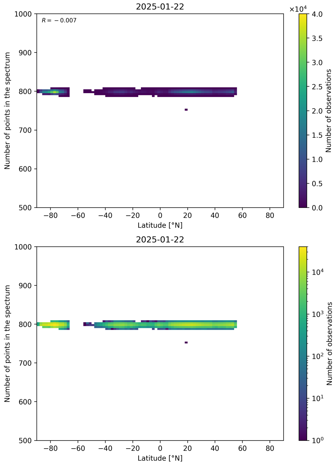
Figure 61: Scatter density plot of “Latitude” against “Number of points in the spectrum” for 2025-01-21 to 2025-01-23.
