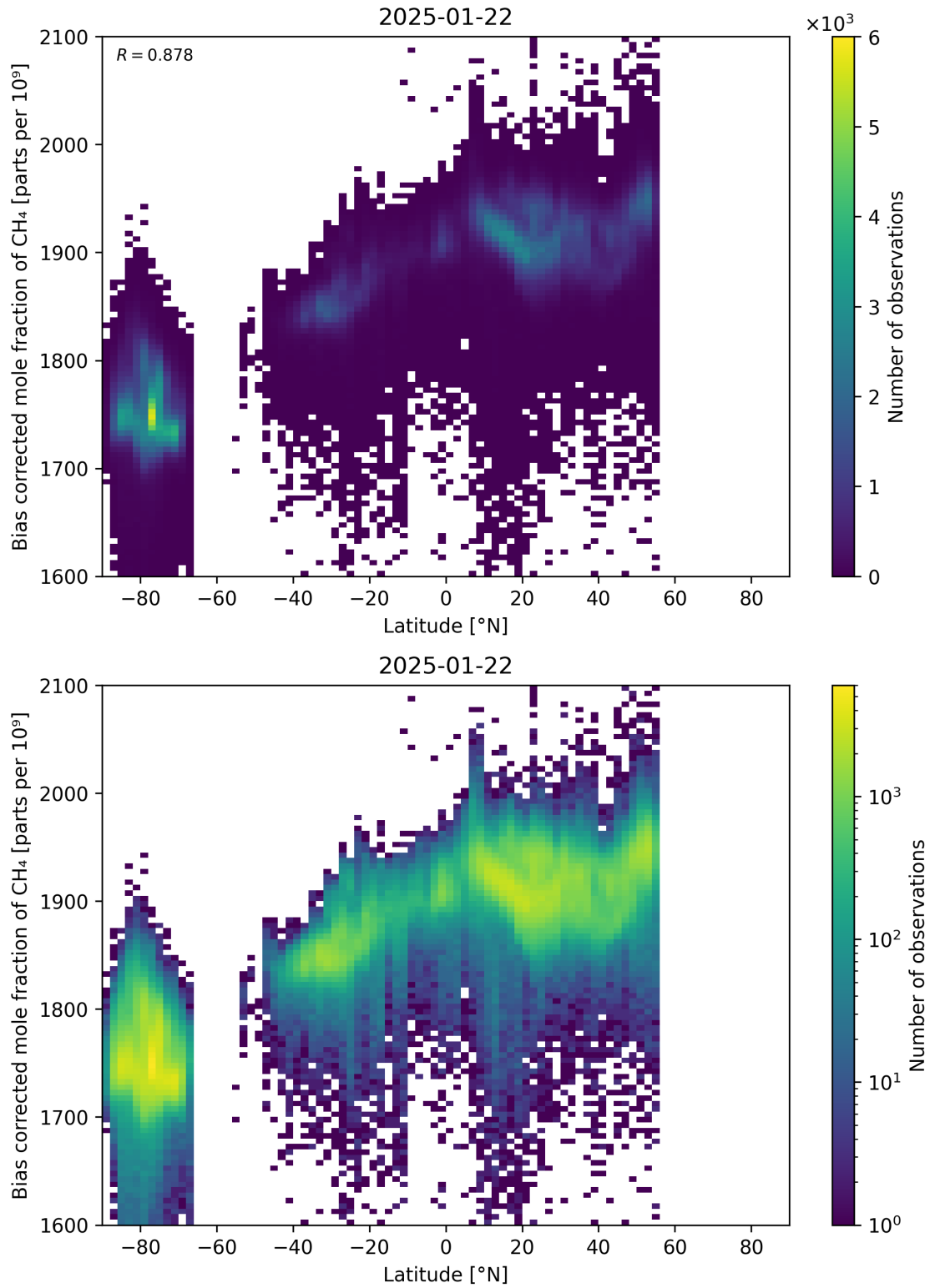
Figure 58: Scatter density plot of “Latitude” against “Bias corrected mole fraction of CH 4 ” for 2025-01-21 to 2025-01-23.
