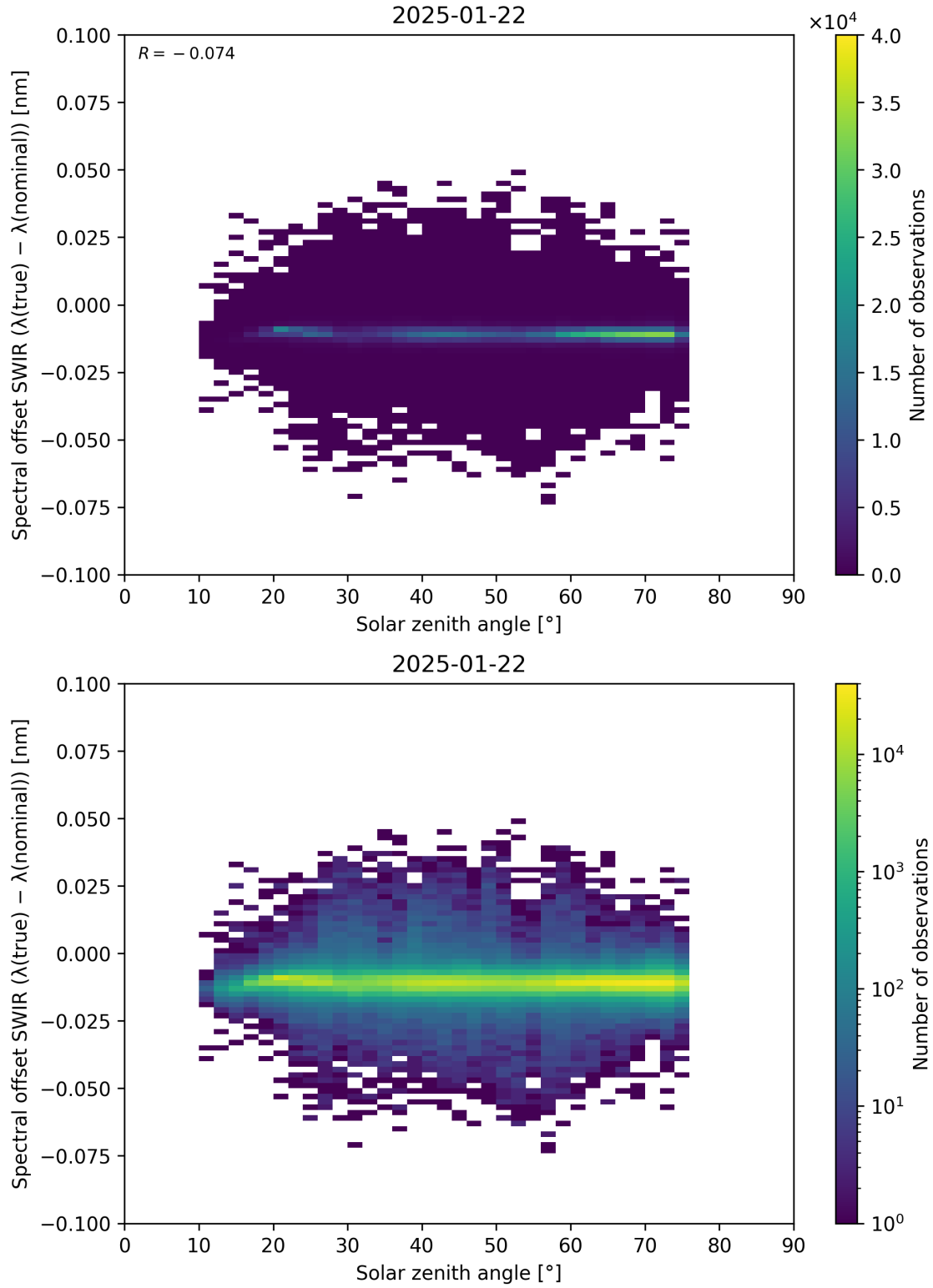
Figure 104: Scatter density plot of “Solar zenith angle” against “Spectral offset SWIR ( \lambda_{\text{true}} - \lambda_{\text{nominal}} )” for 2025-01-21 to 2025-01-23.
