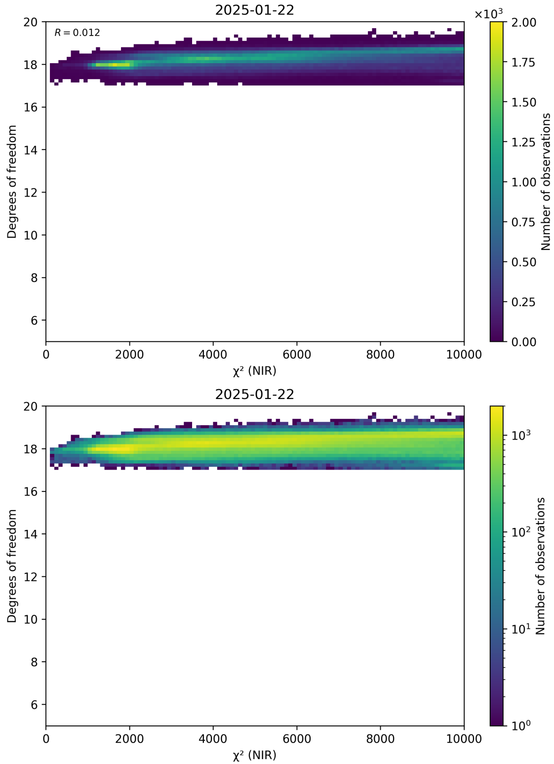
Figure 44: Scatter density plot of “ \chi^2 (NIR)” against “Degrees of freedom” for 2025-01-21 to 2025-01-23.
