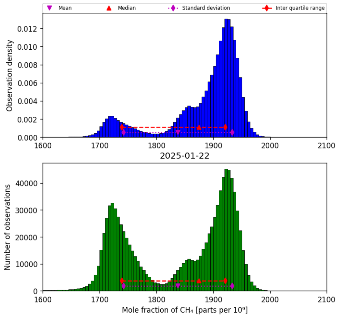
Figure 23: Histogram of “Mole fraction of CH 4 ” for 2025-01-21 to 2025-01-23
