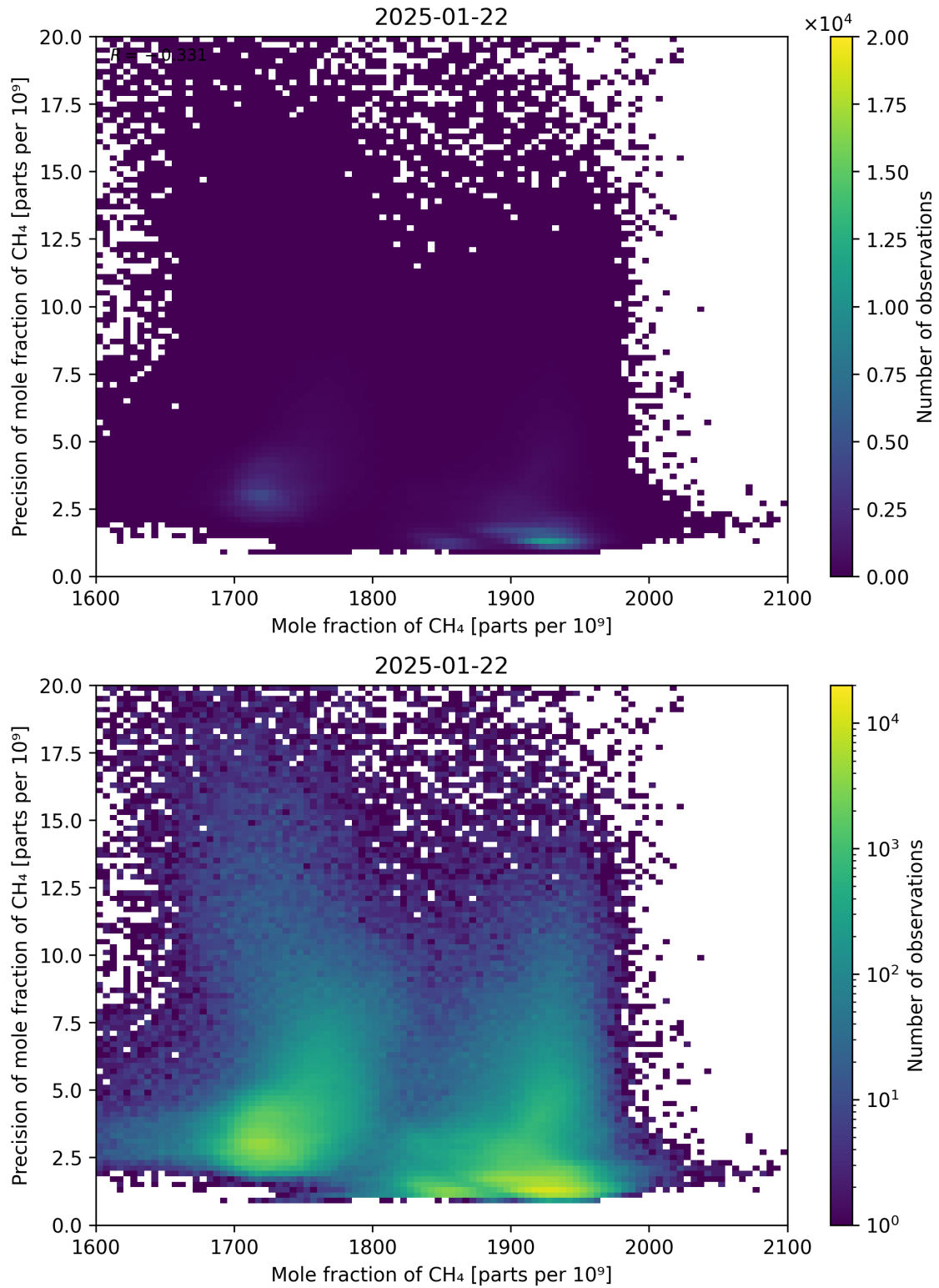
Figure 75: Scatter density plot of “Mole fraction of CH 4 ” against “Precision of mole fraction of CH 4 ” for 2025-01-21 to 2025-01-23.
