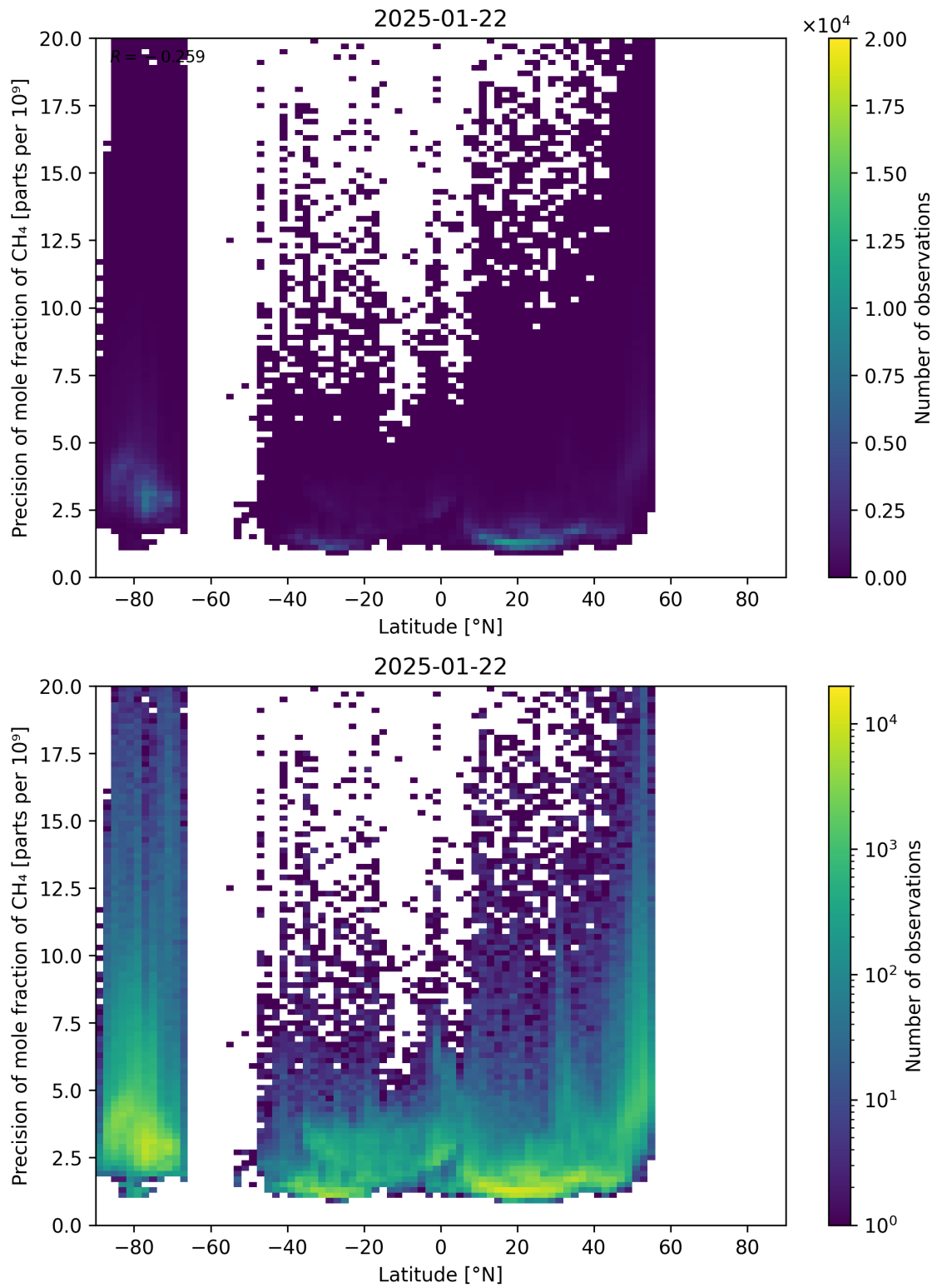
Figure 59: Scatter density plot of “Latitude” against “Precision of mole fraction of \text{CH}_4 ” for 2025-01-21 to 2025-01-23.
