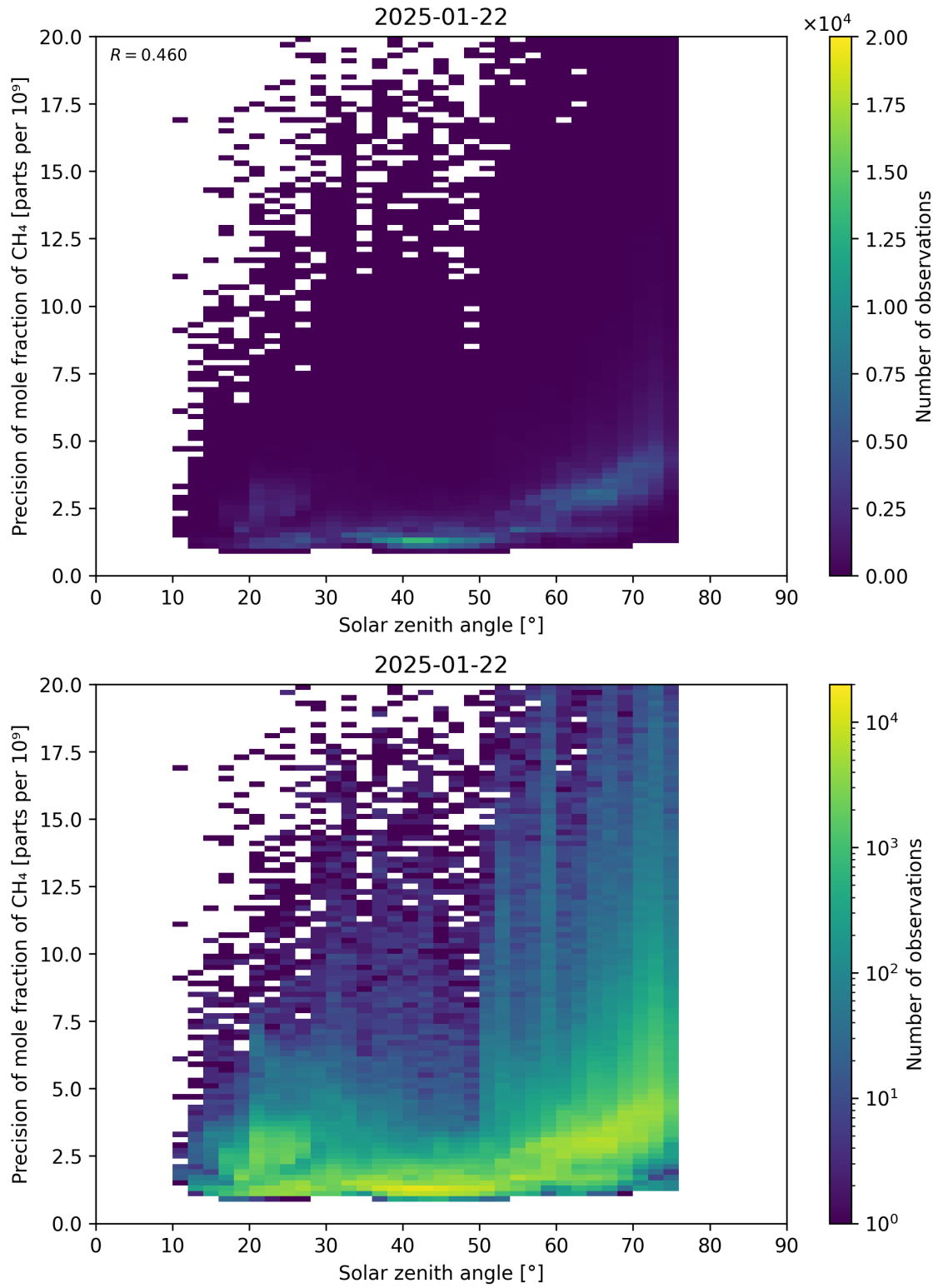
Figure 101: Scatter density plot of “Solar zenith angle” against “Precision of mole fraction of CH 4 ” for 2025-01-21 to 2025-01-23.
