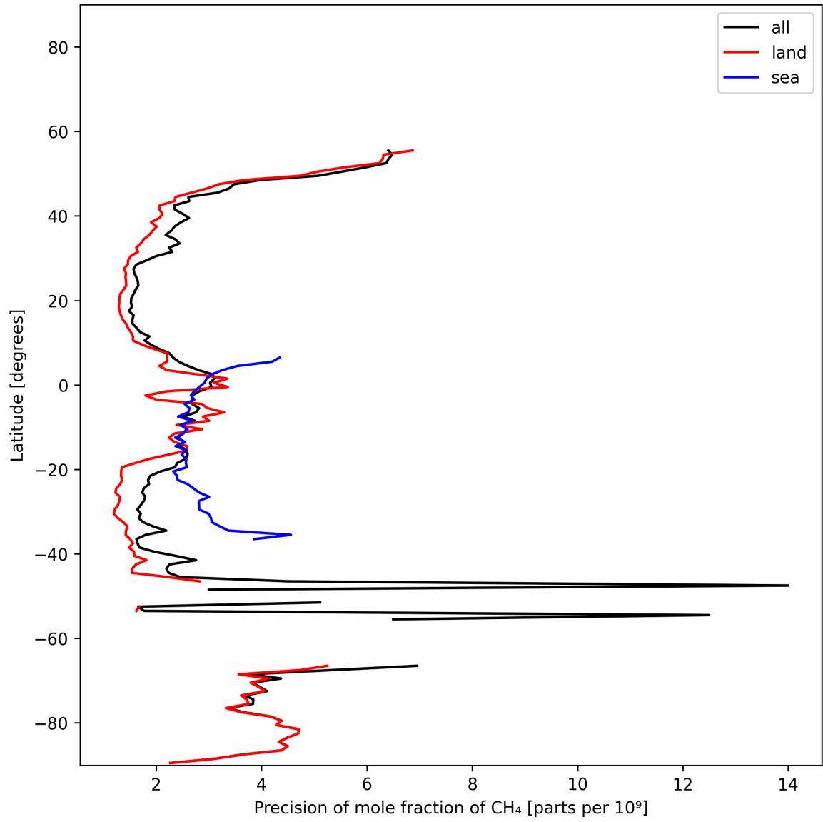
Figure 13: Zonal average of “Precision of mole fraction of CH 4 ” for 2025-01-21 to 2025-01-23.
