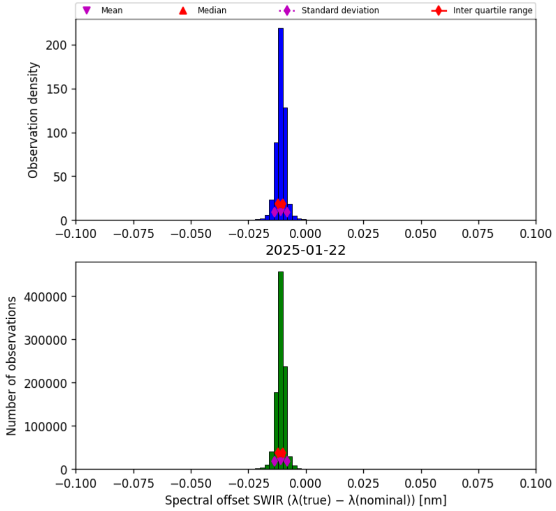
Figure 27: Histogram of “Spectral offset SWIR ( \lambda_{\text{true}} - \lambda_{\text{nominal}} )” for 2025-01-21 to 2025-01-23
