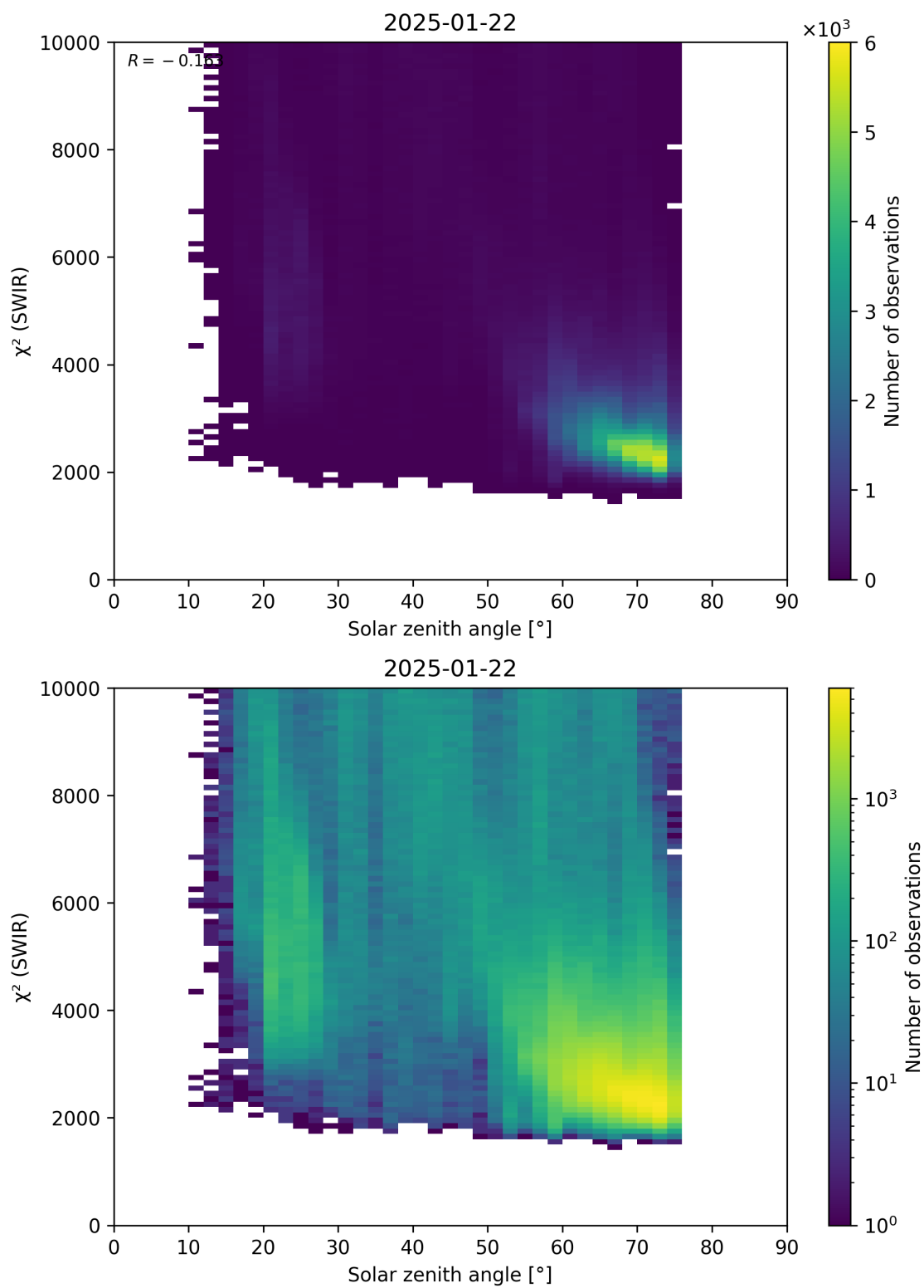
Figure 95: Scatter density plot of “Solar zenith angle” against “ \chi^2 (SWIR)” for 2025-01-21 to 2025-01-23.
