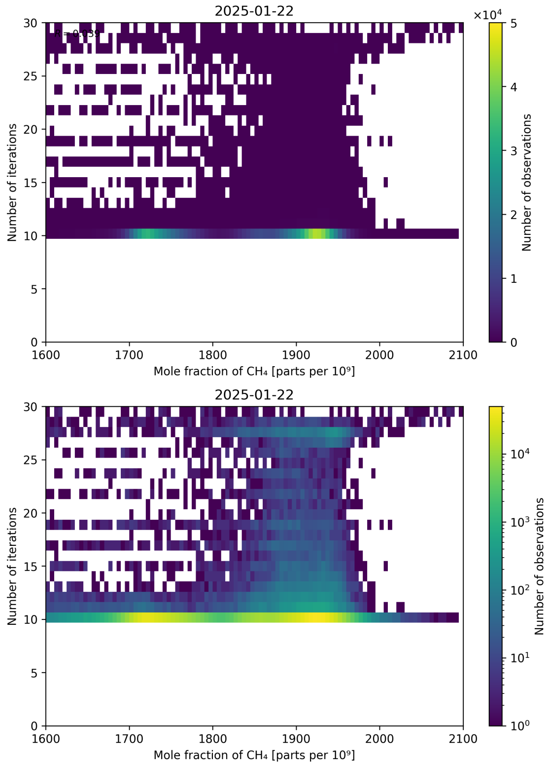
Figure 76: Scatter density plot of “Mole fraction of CH 4 ” against “Number of iterations” for 2025-01-21 to 2025-01-23.
