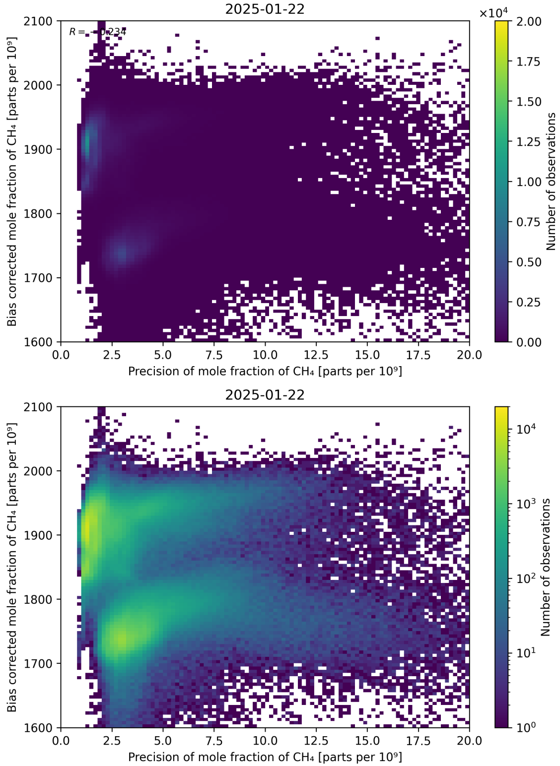
Figure 82: Scatter density plot of “Precision of mole fraction of CH 4 ” against “Bias corrected mole fraction of CH 4 ” for 2025-01-21 to 2025-01-23.
