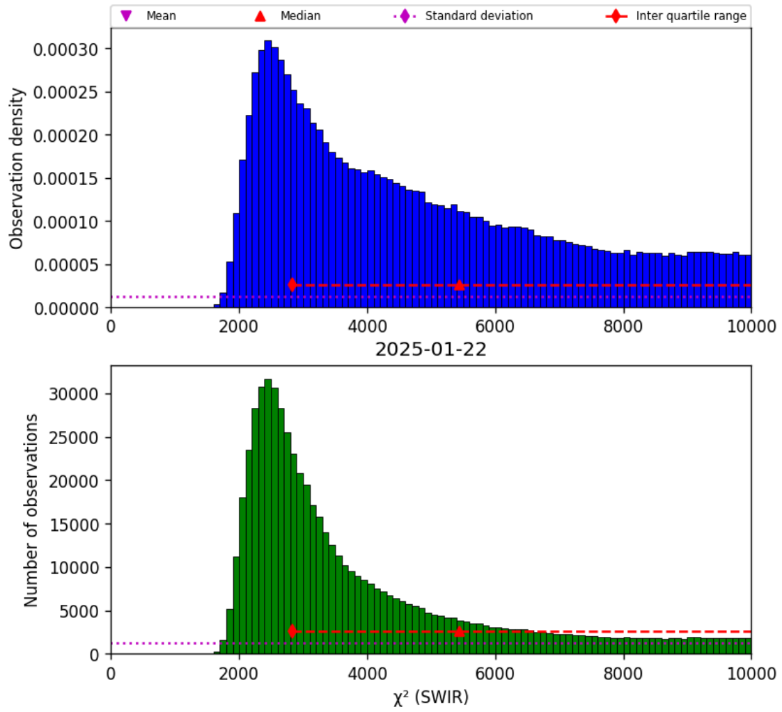
Figure 28: Histogram of “ \chi^2 (SWIR)” for 2025-01-21 to 2025-01-23
