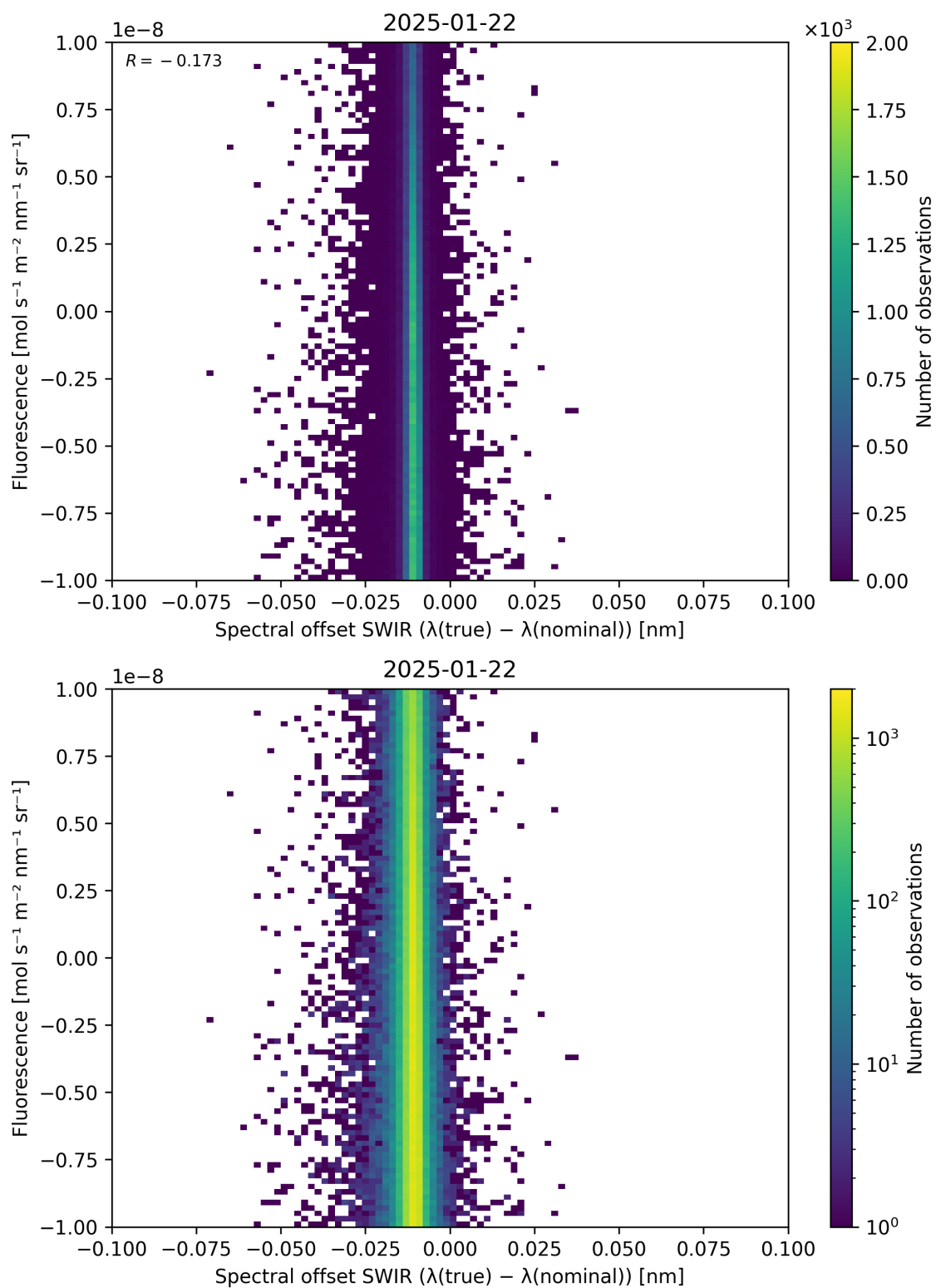
Figure 120: Scatter density plot of “Spectral offset SWIR ( \lambda_{\text{true}} - \lambda_{\text{nominal}} )” against “Fluorescence” for 2025-01-21 to 2025-01-23.
