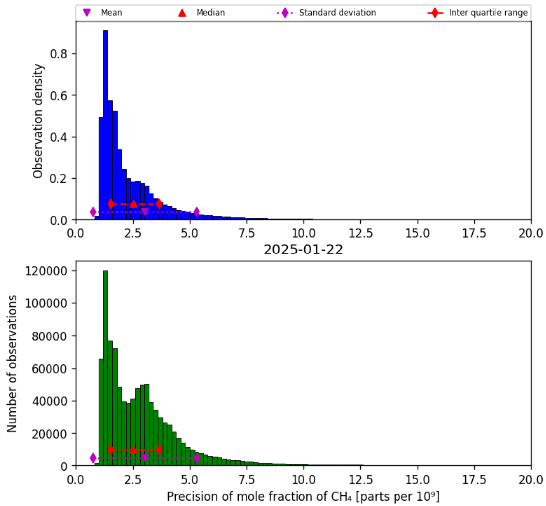
Figure 24: Histogram of “Precision of mole fraction of CH 4 ” for 2025-01-21 to 2025-01-23
