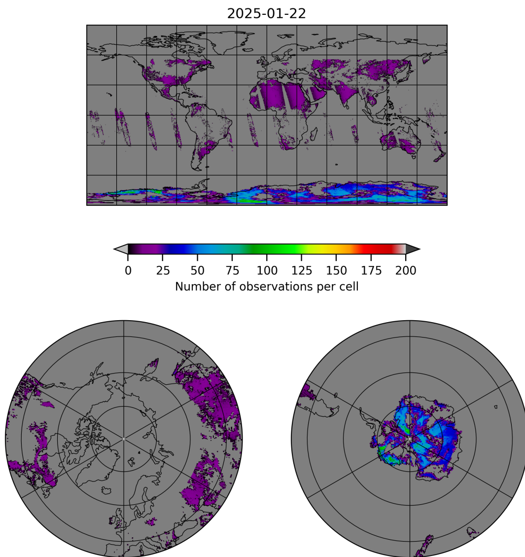
Figure 10: Map of the number of observations for 2025-01-21 to 2025-01-23
